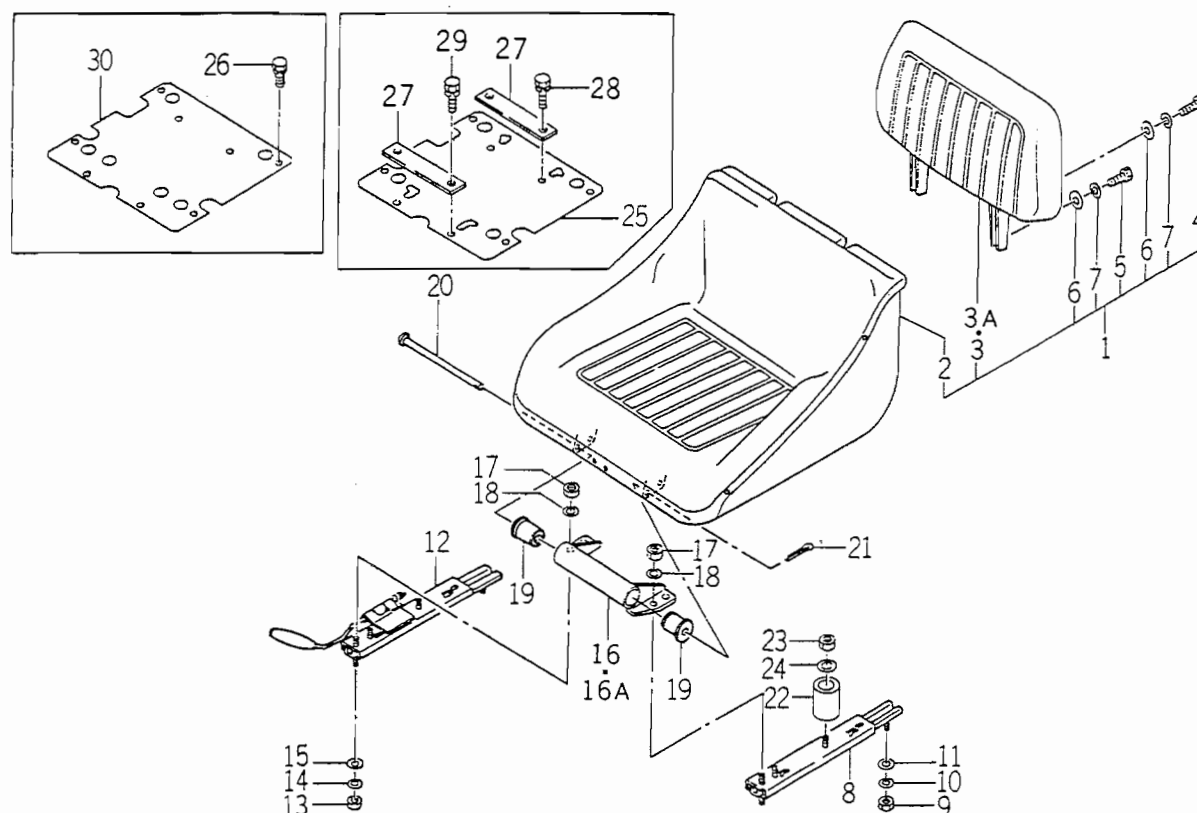
FIG. 83 SEAT SYSTEM
