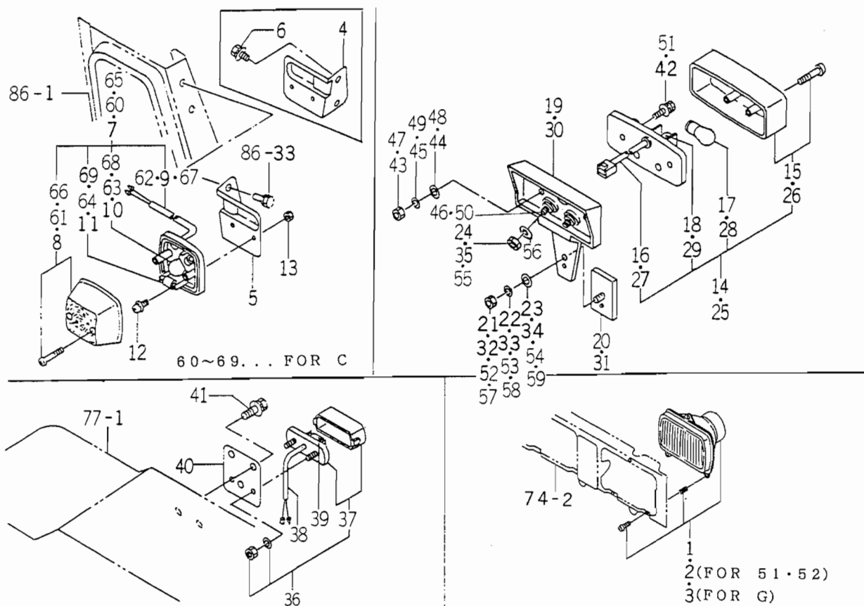
FIG. 90 BULB SYSTEM
