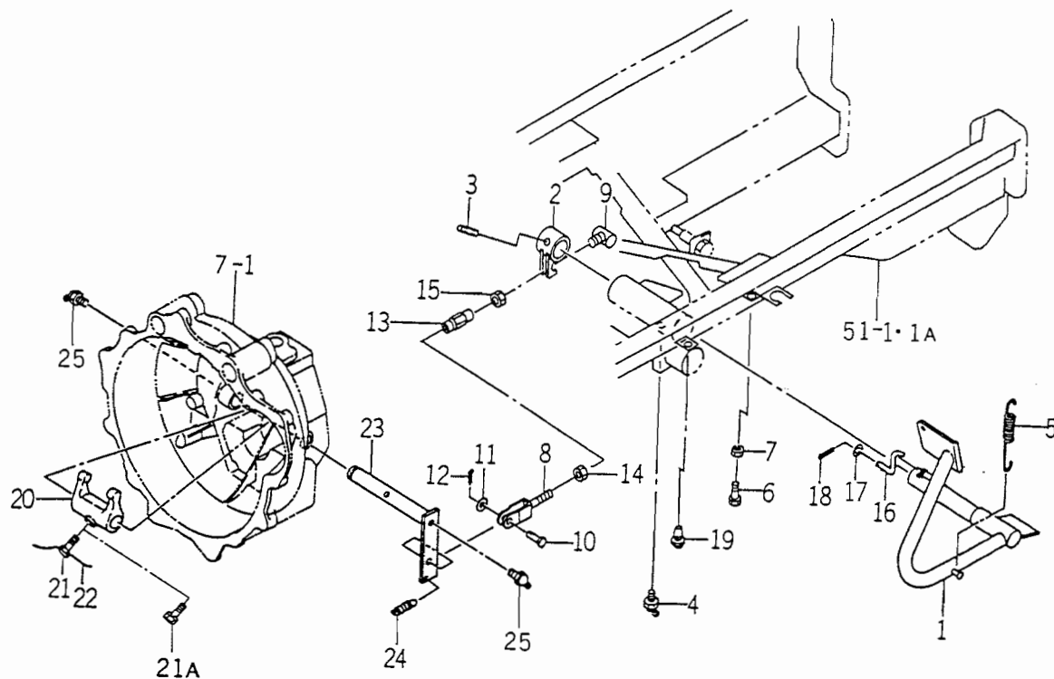
FIG. 9 CLUTCH PEDAL SYSTEM
