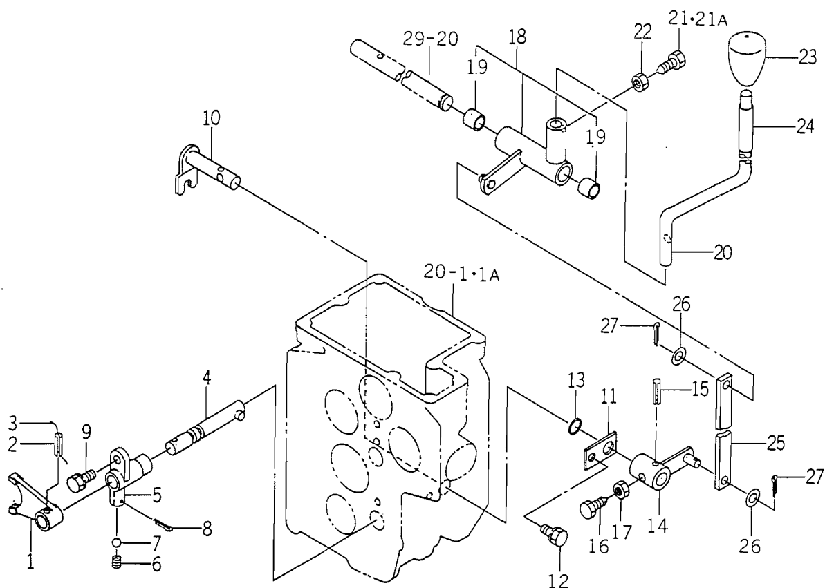
FIG. 32 FRONT SHIFTER SYSTEM (HST)
