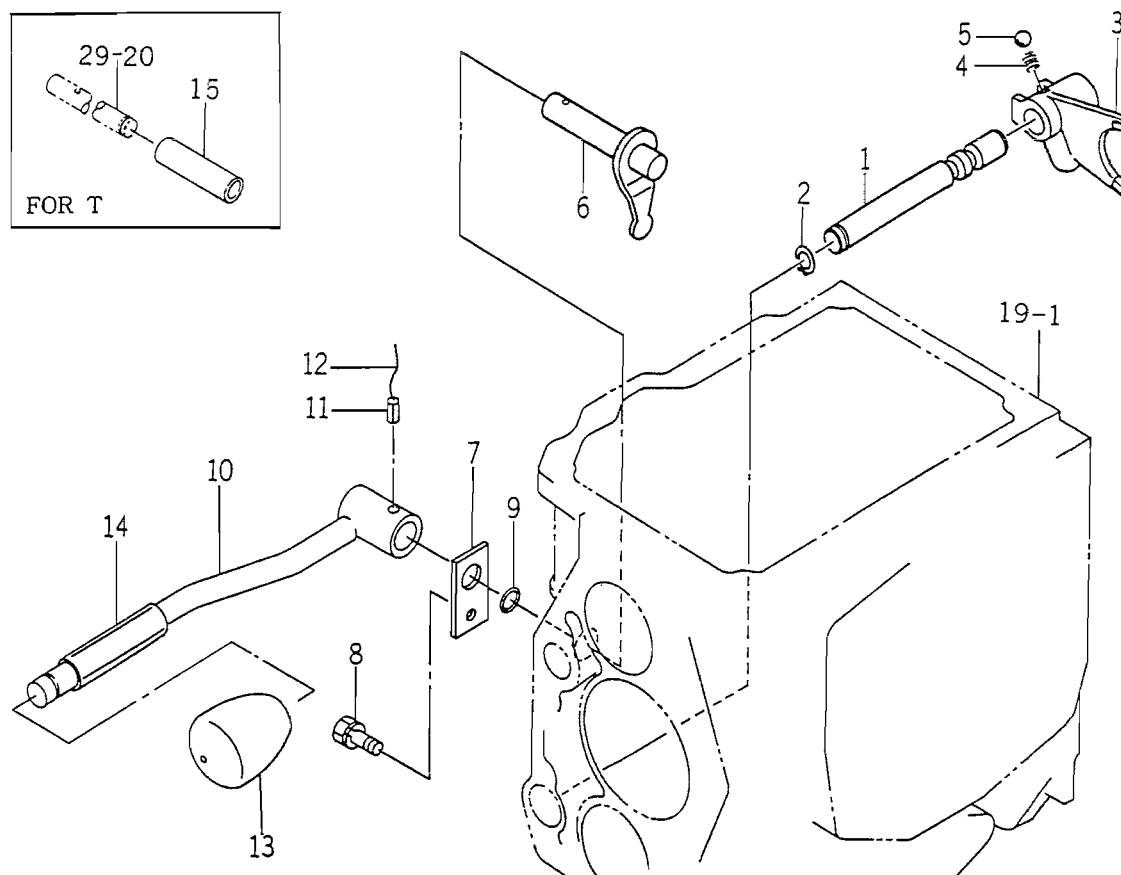
FIG. 31 FRONT SHIFTER SYSTEM
