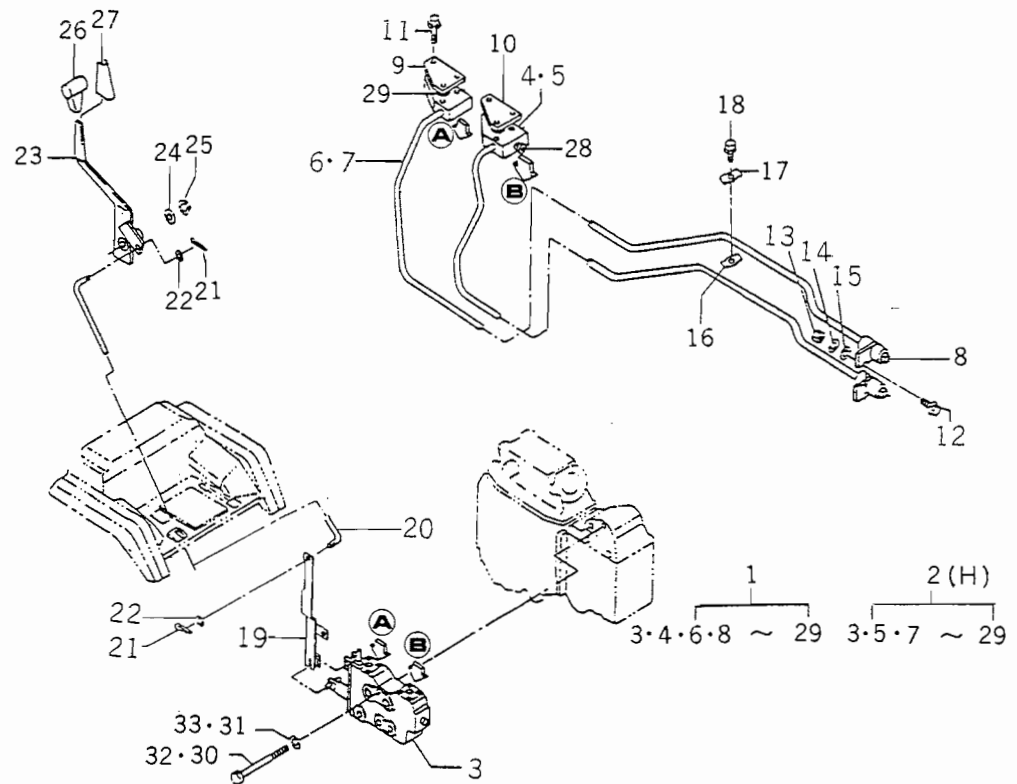
FIG.102 VALVE (SUB/2) SET SYSTEM (OPTION)
