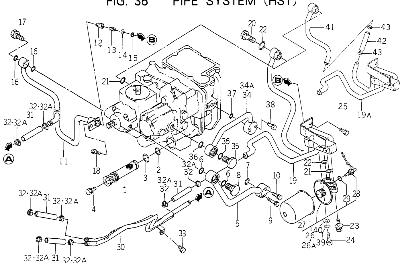
FIG. 36 PIPE SYSTEM (HST)
