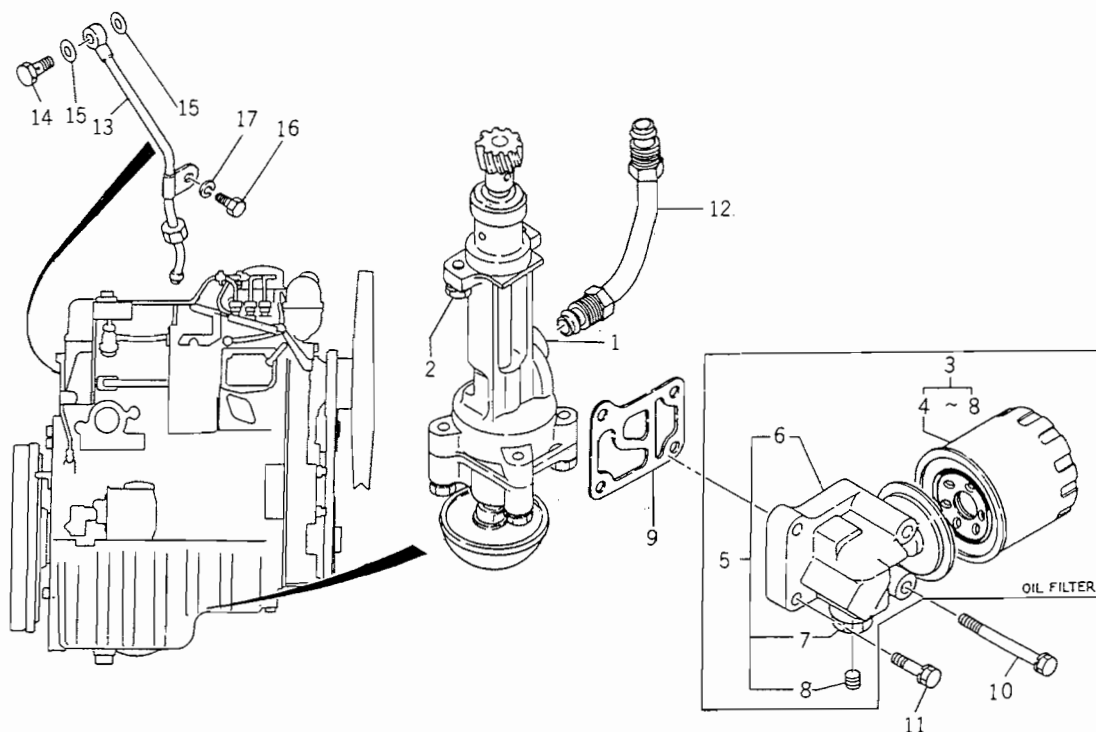
FIG. 16 OIL FILTER AND OIL PUMP
