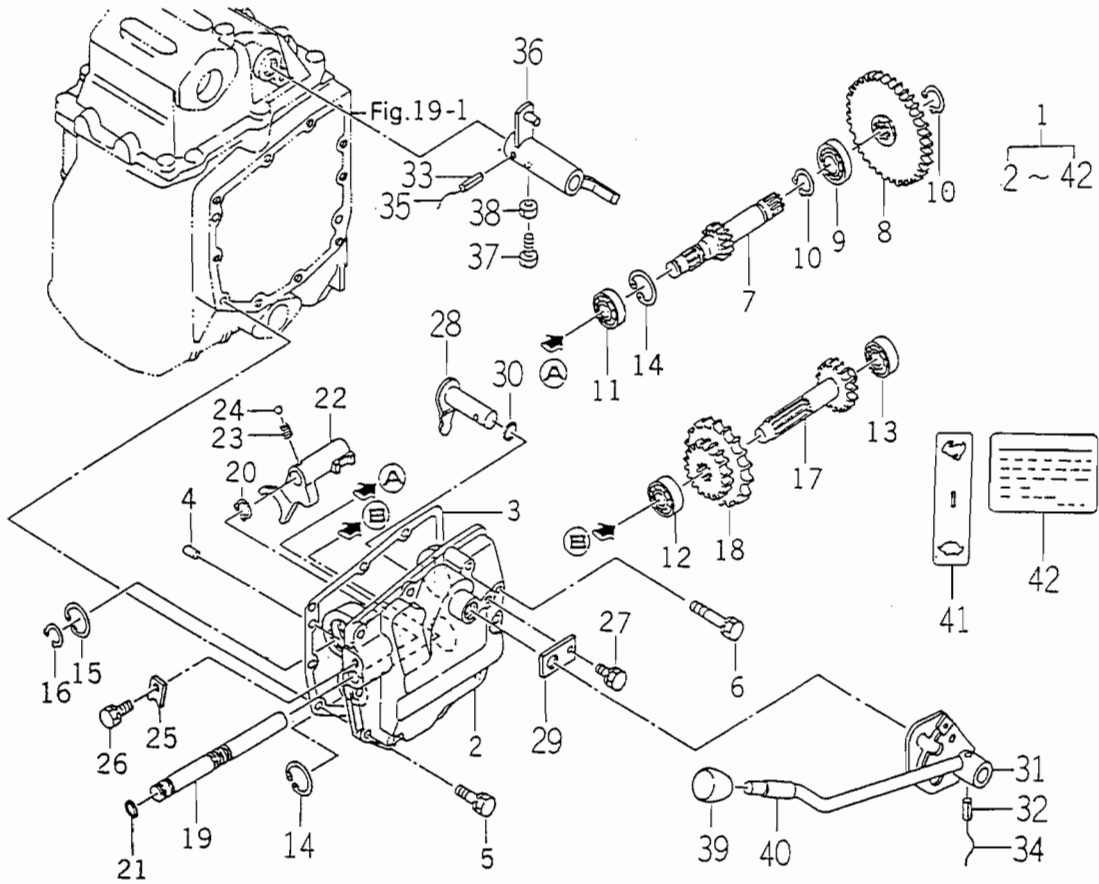
FIG. 97 CREEP MISSION SYSTEM (OPTION) (EXCEPT H • M)
