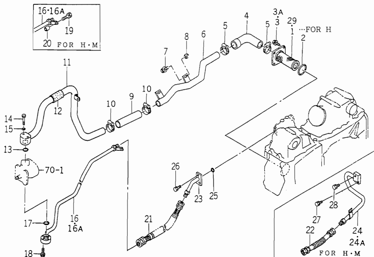
FIG. 69 HYDRAULIC PIPING SYSTEM (1)
