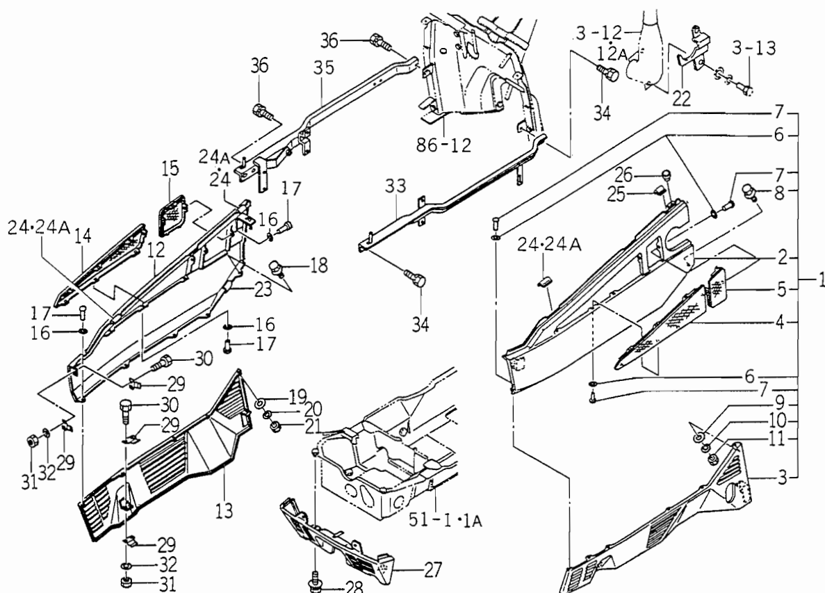
FIG. 76 SIDE COVER SYSTEM (MUFFLER,LENGTH TYPE)
