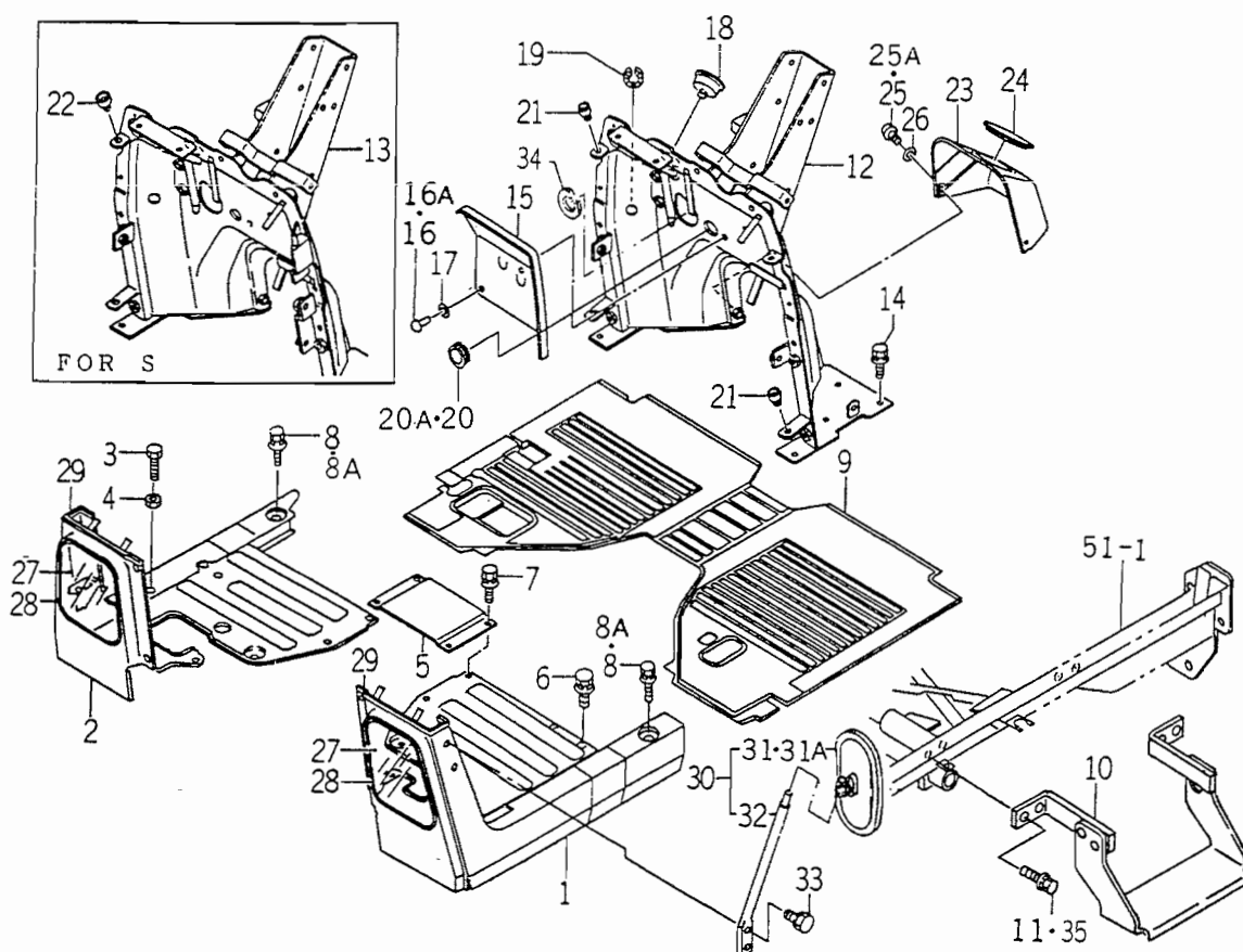
FIG. 86 STEP SYSTEM
