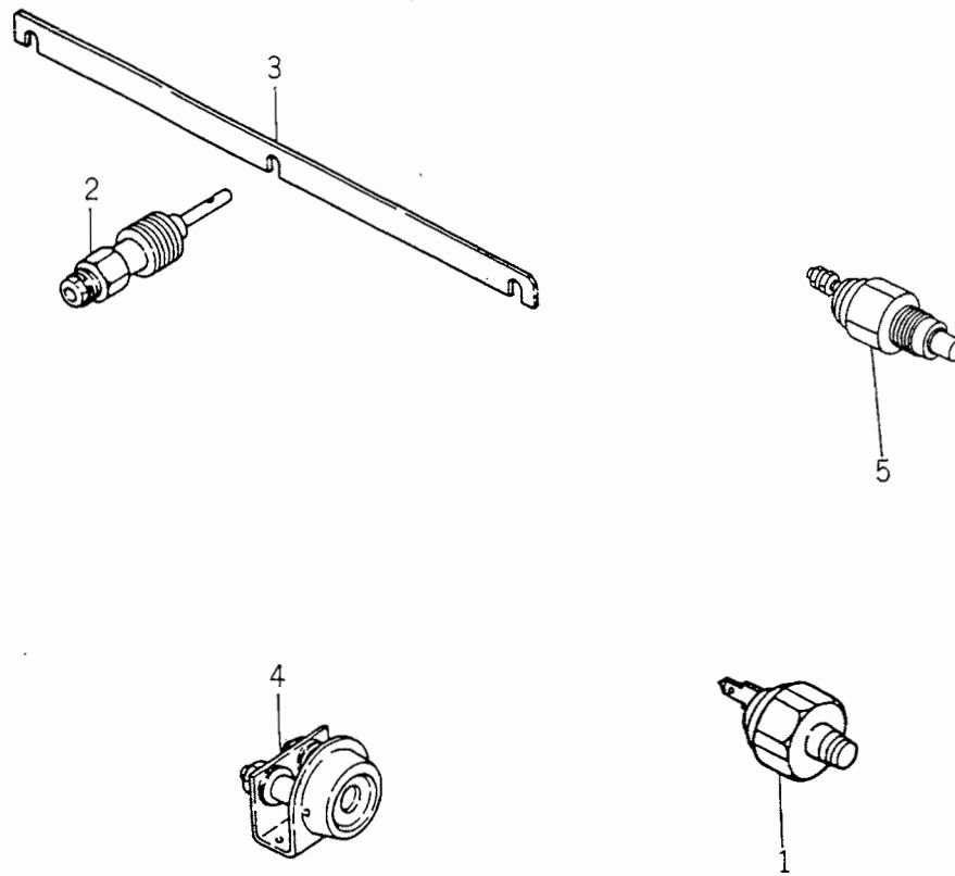
FIG. 24 ELECTRICAL PARTS
