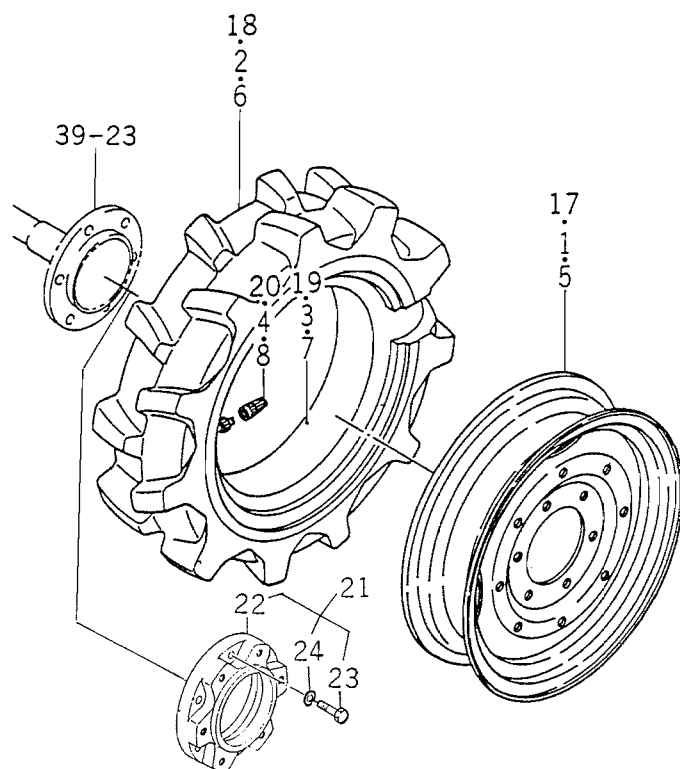
FIG. 46 REAR WHEEL SYSTEM
