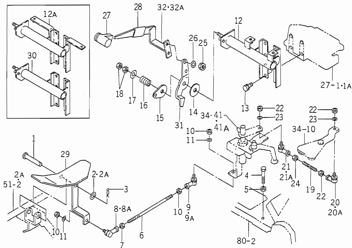
FIG. 35 PEDAL SYSTEM (HST)
