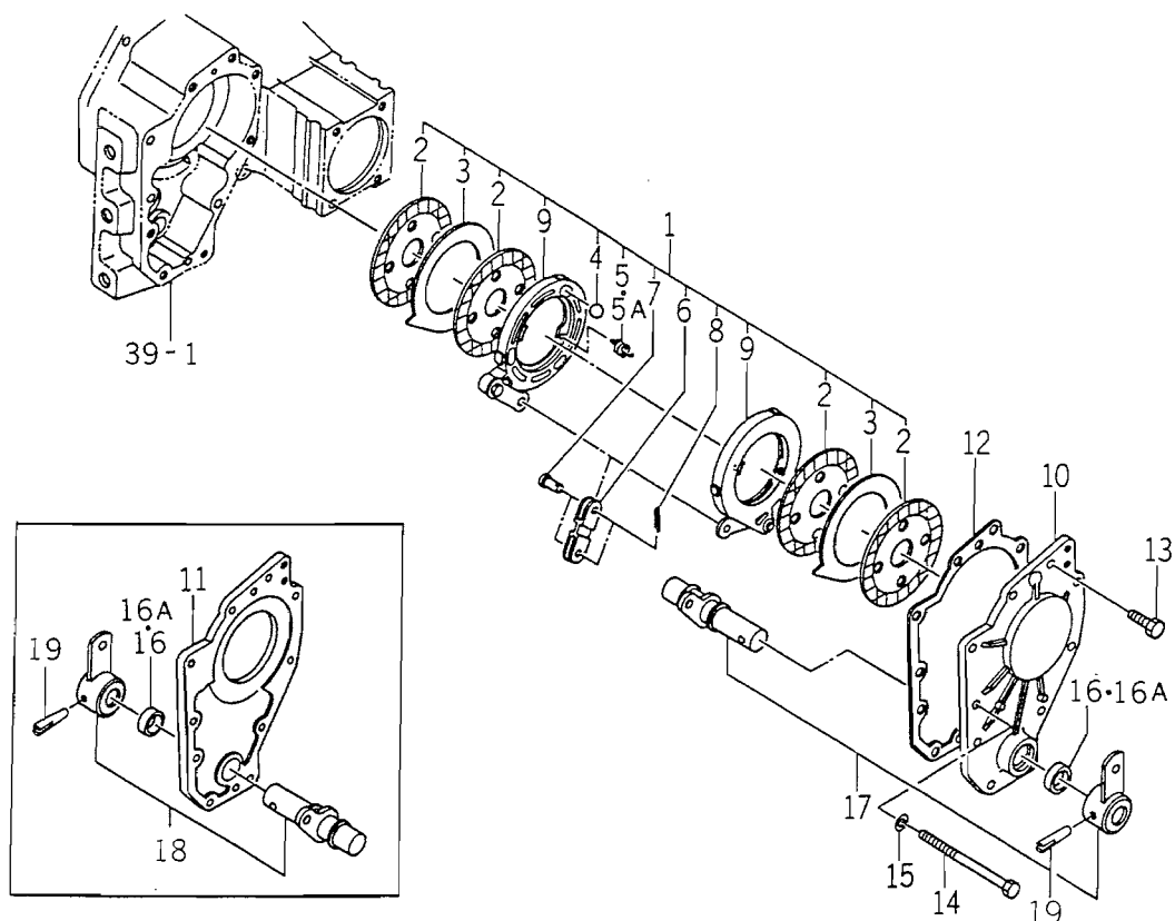
FIG. 42 BRAKE SYSTEM
