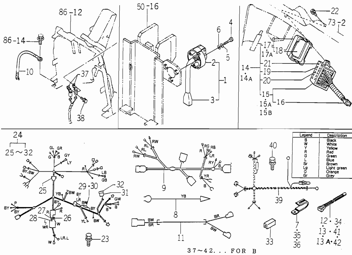
FIG. 93 WIRE HARNESS SYSTEM
