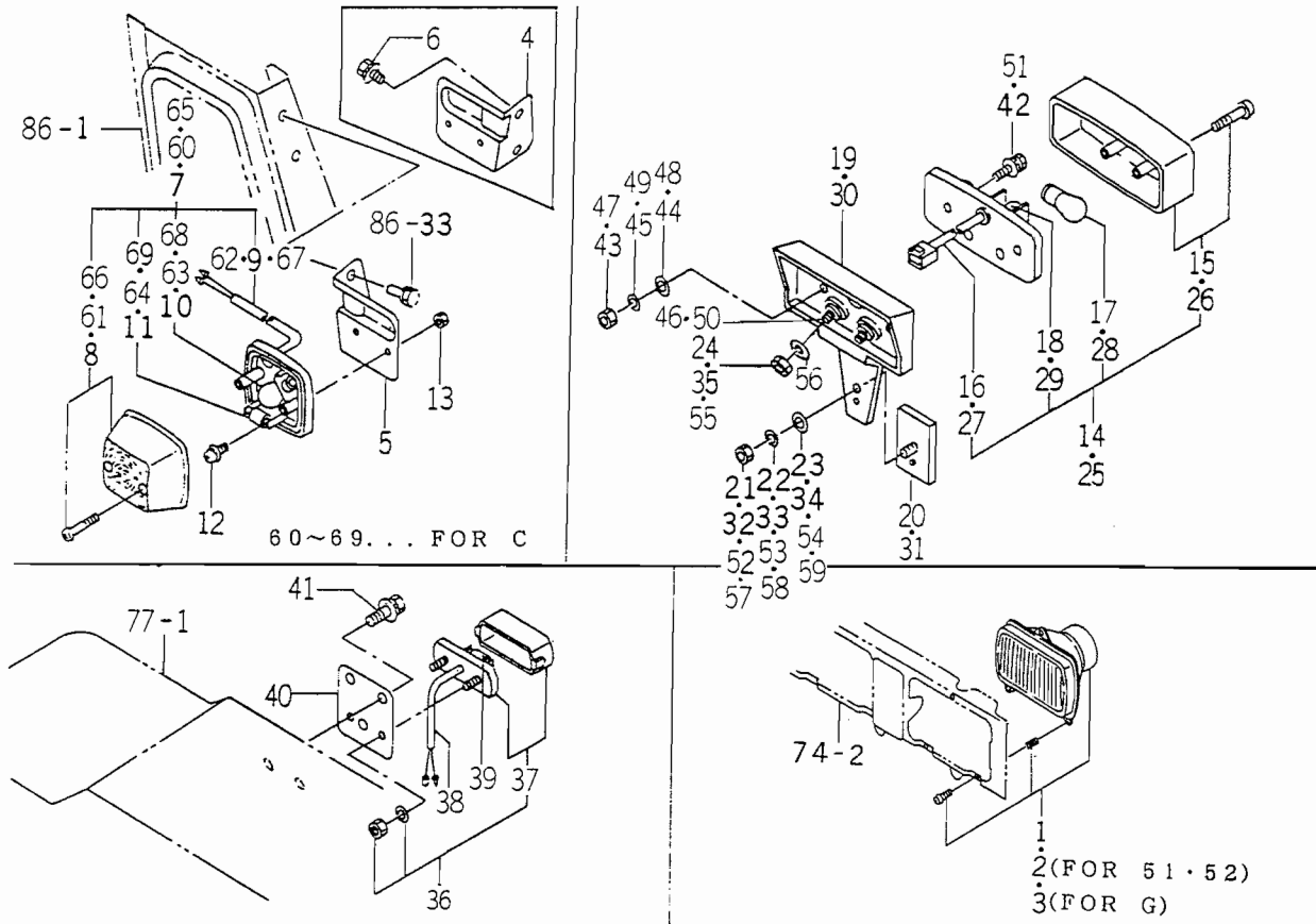
FIG. 90 BULE SYSTEM
