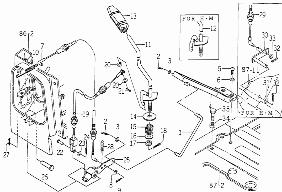
FIG. 6 ACCELE SYSTEM
