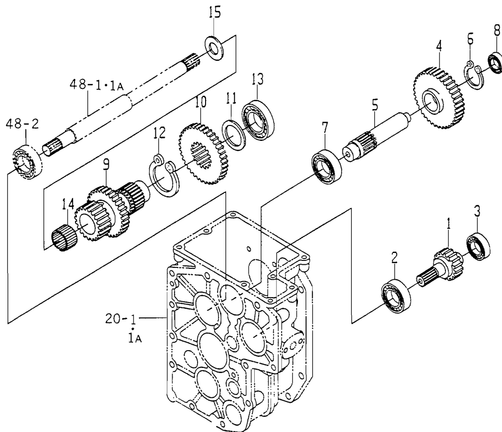
FIG. 22 INPUT GEAR AND CHANGE GEAR SYSTEM (HST)
