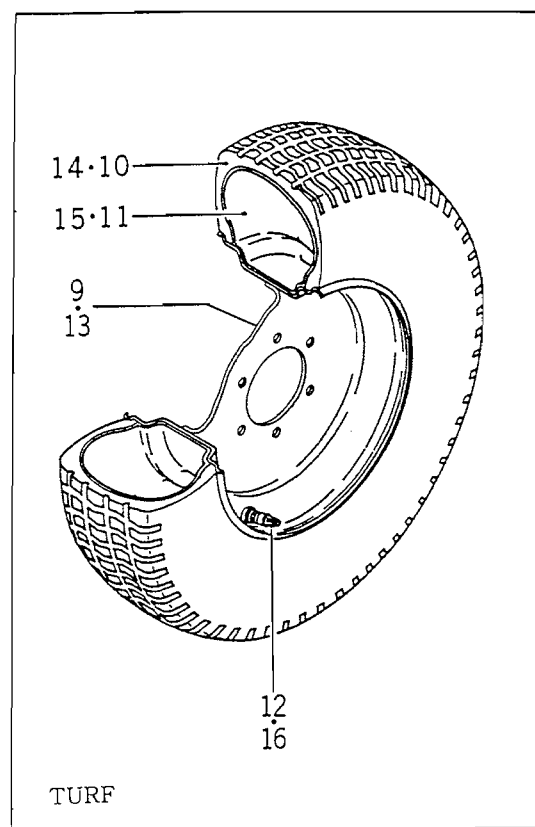
FIG. 46 REAR WHEEL SYSTEM
