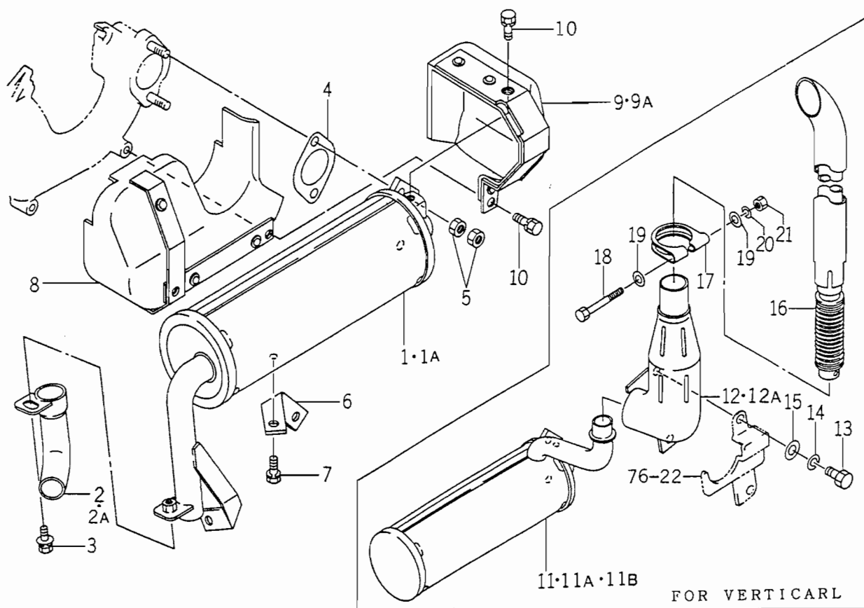
FIG. 3 MUFFLER SYSTEM
