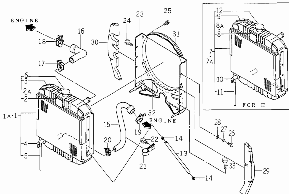
FIG. 2 RADIATOR SYSTEM
