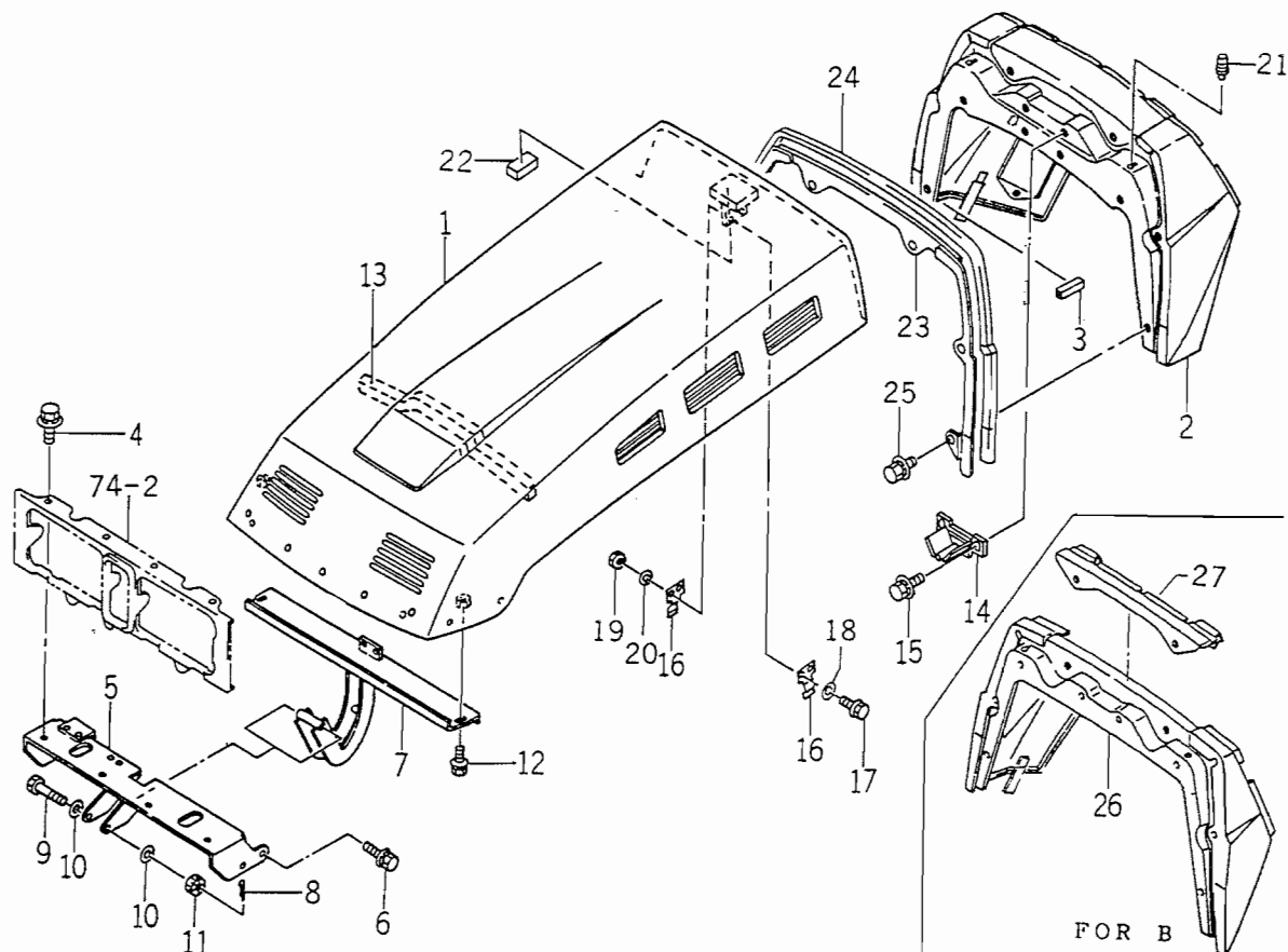
FIG. 73 HOOD SYSTEM
