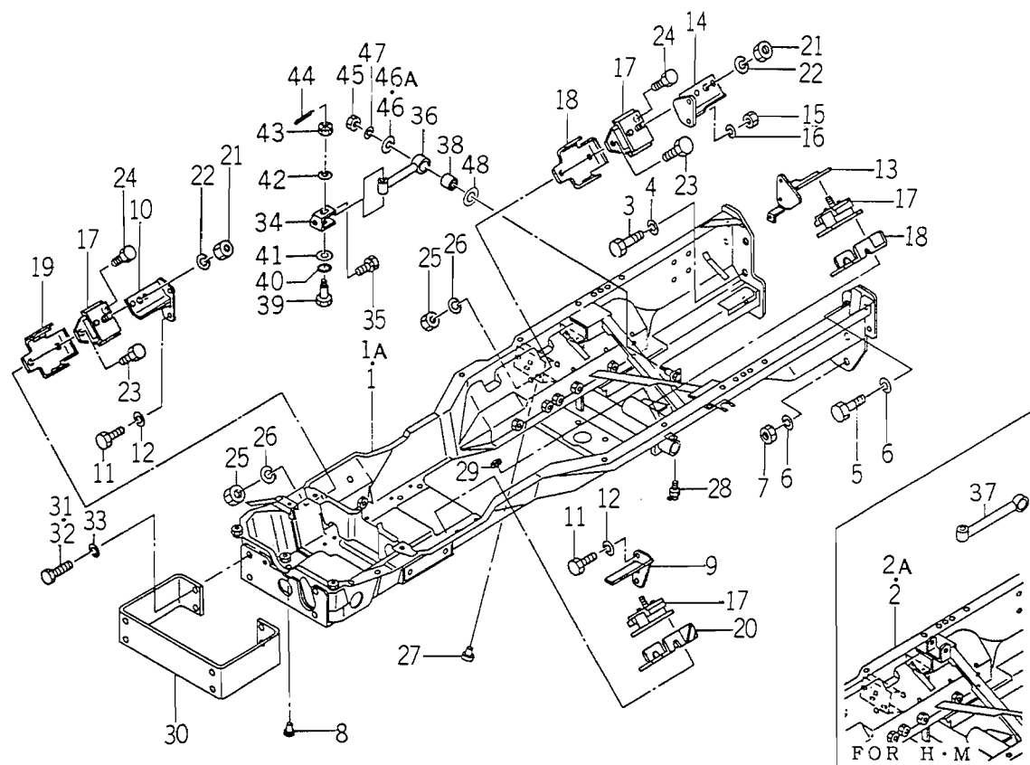
FIG. 51 FRAME SYSTEM
