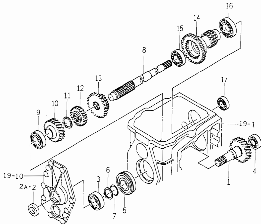
FIG. 21 INPUT GEAR AND CHANGE GEAR SYSTEM
