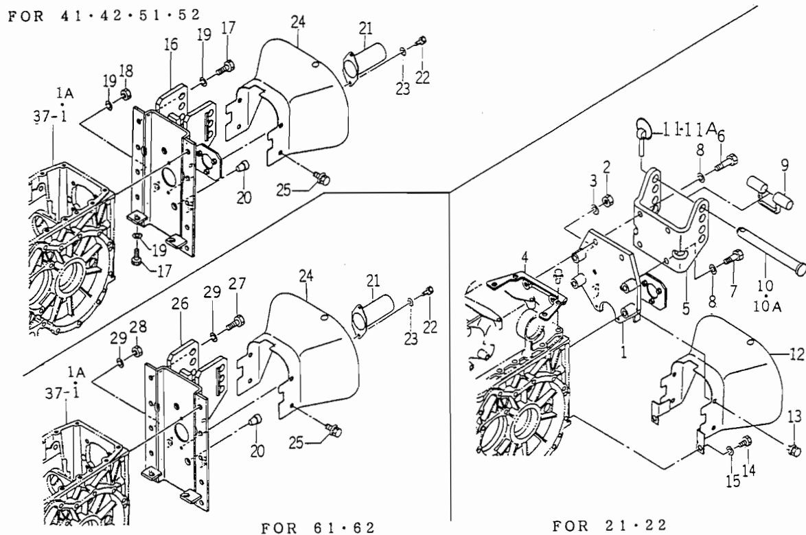
FIG. 50 REAR HITCH SYSTEM
