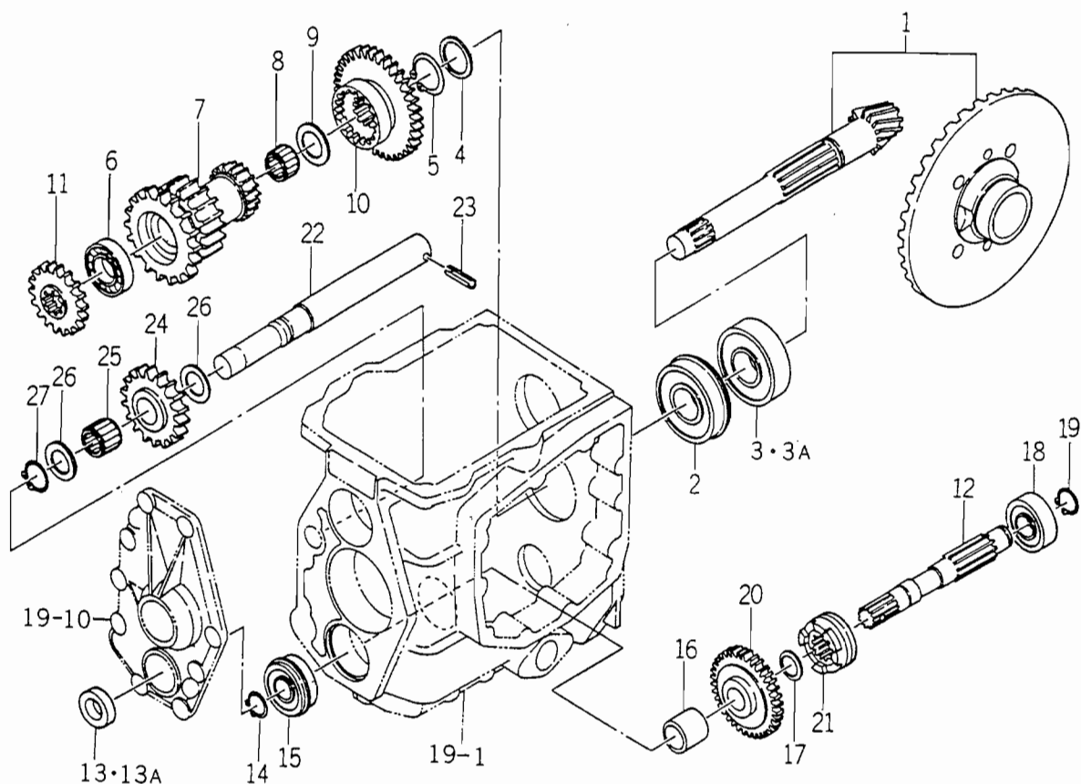
FIG. 23 FRONT TRANSMISSION GEAR SYSTEM
