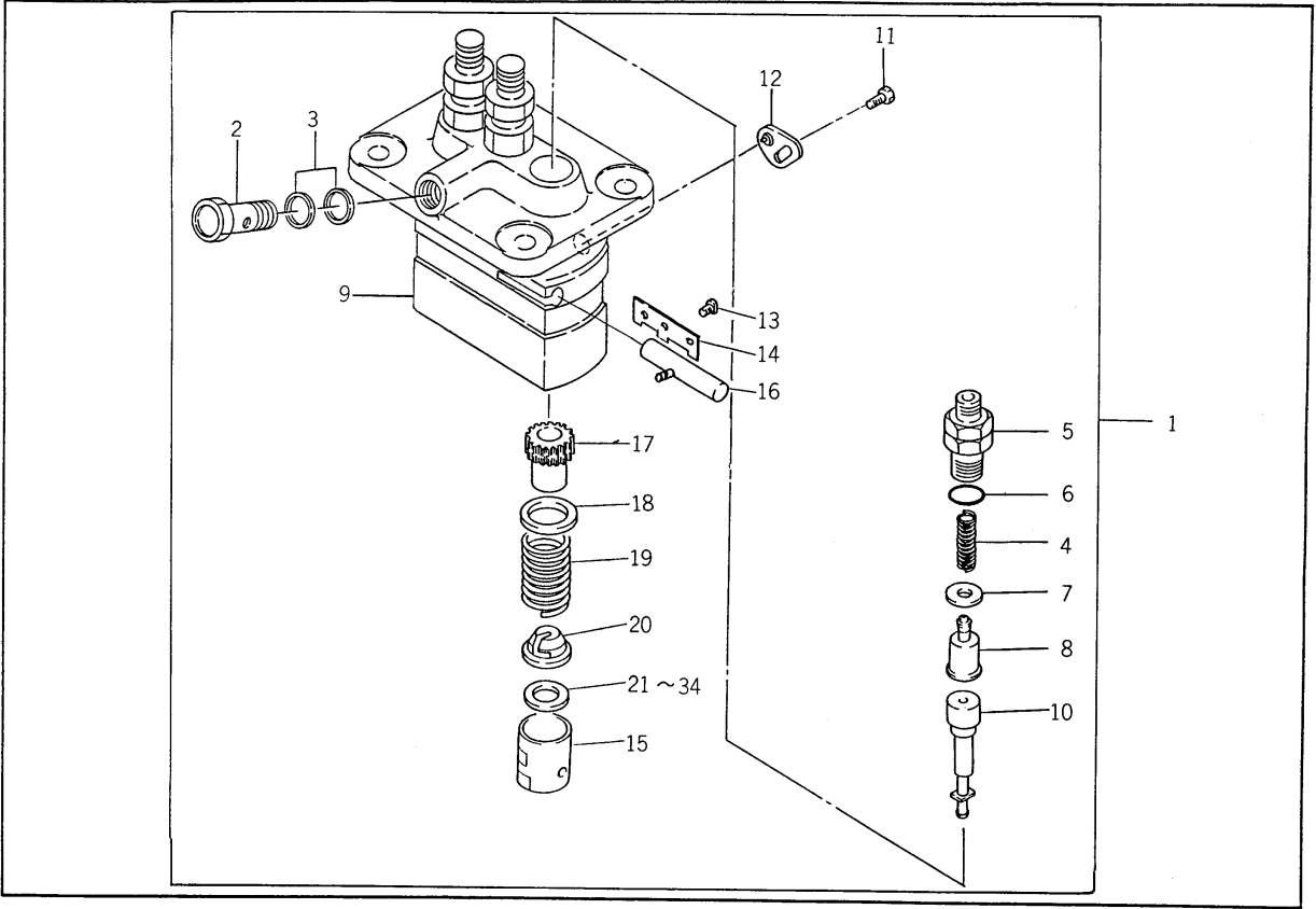
FIG.# 17 INJECTION PUMP AND OTHER PARTS P. 33
