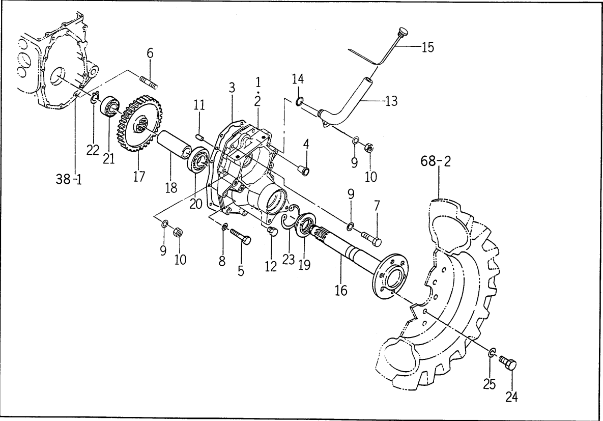
FIG.# 62 REAR AXLE HOUSING SYSTEM P. 133
