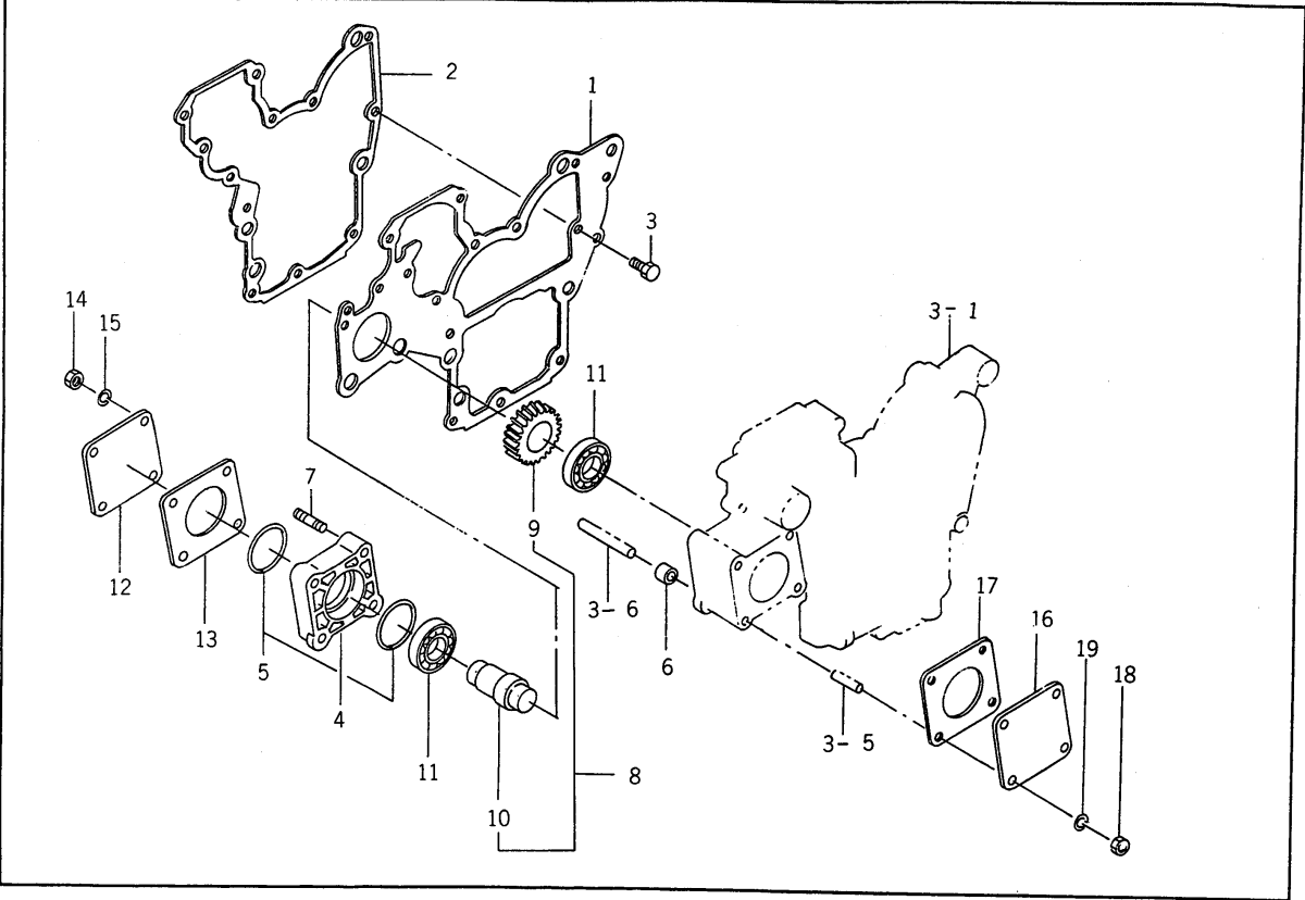
FIG.# 4 TIMING GEAR CASE (2) P. 7
