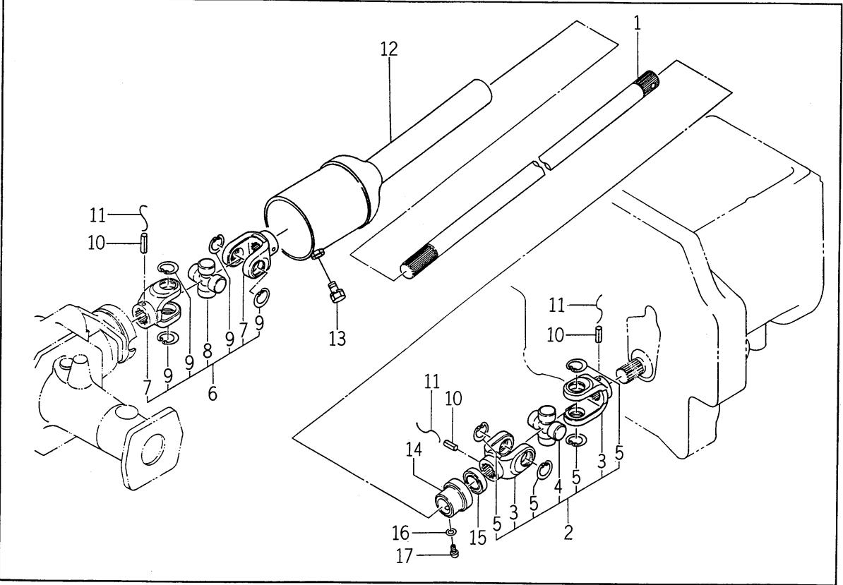
FIG.# 75 DRIVE SHAFT SYSTEM (HST) P. 161 TU315FE
