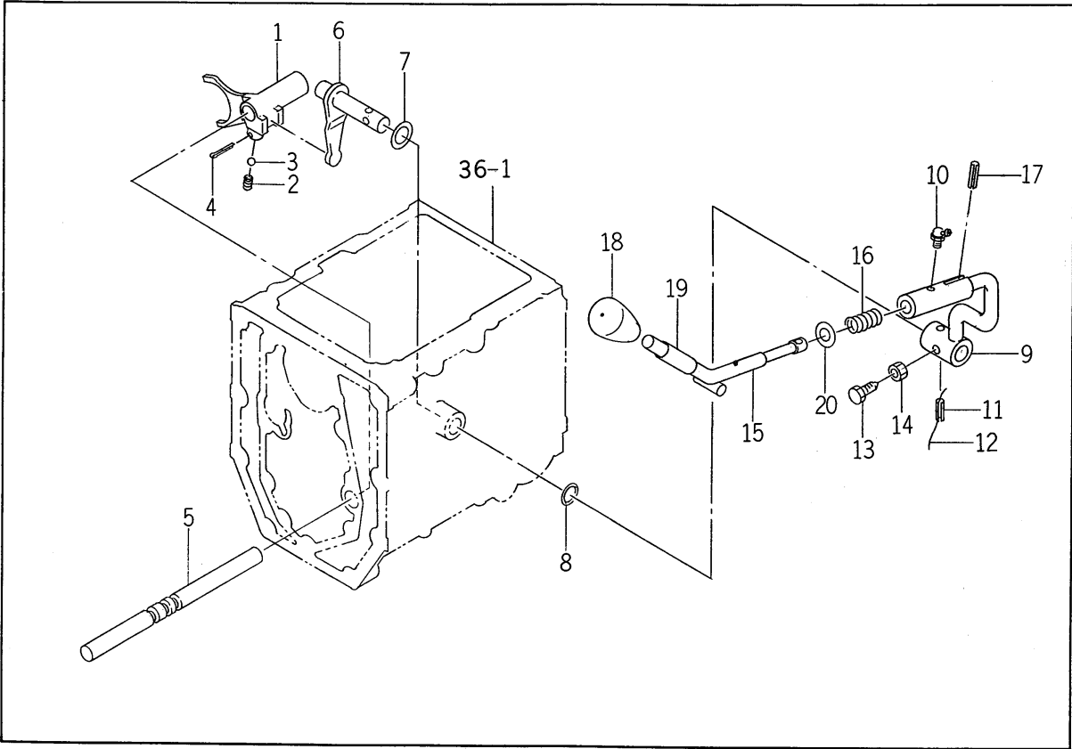
FIG.# 53 P.T.O. CHANGE LEVER SYSTEM P. 115 TU315FE
