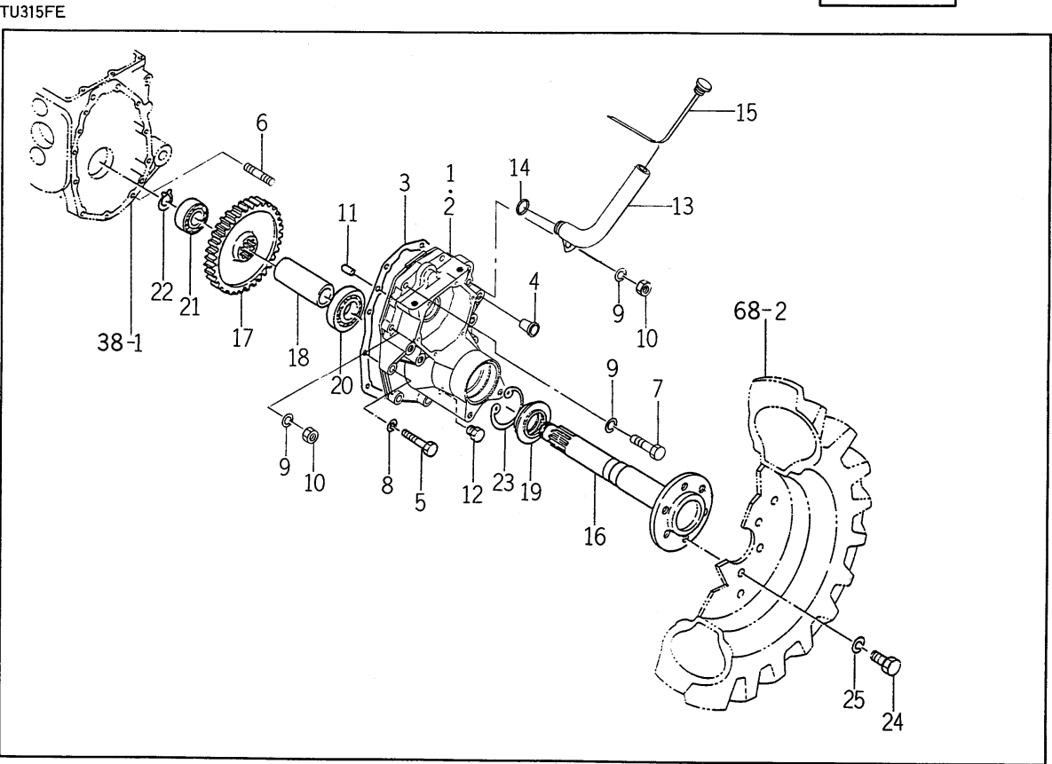
FIG.# 62 REAR AXLE HOUSING SYSTEM P. 133
