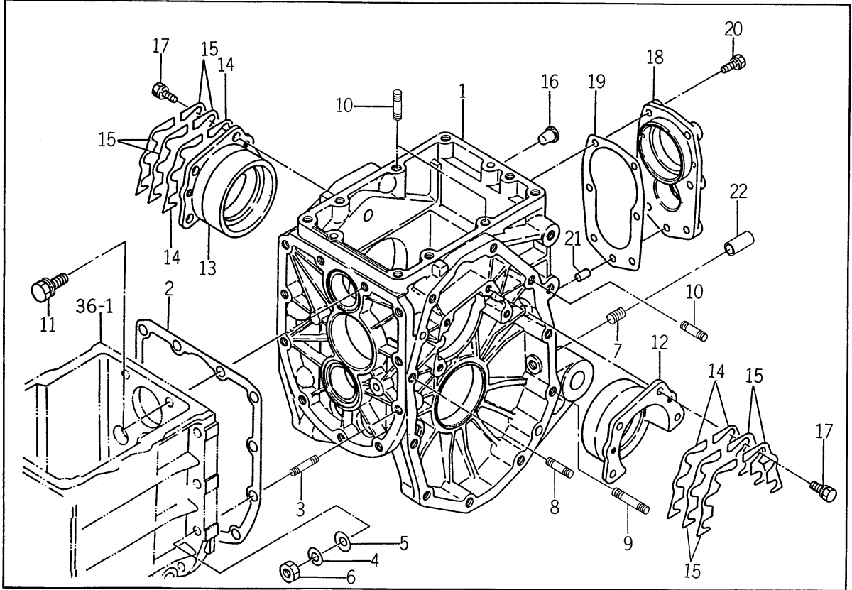
FIG.# 38 REAR TRANSMISSON CASE SYSTEM P. 85 TU315FE
