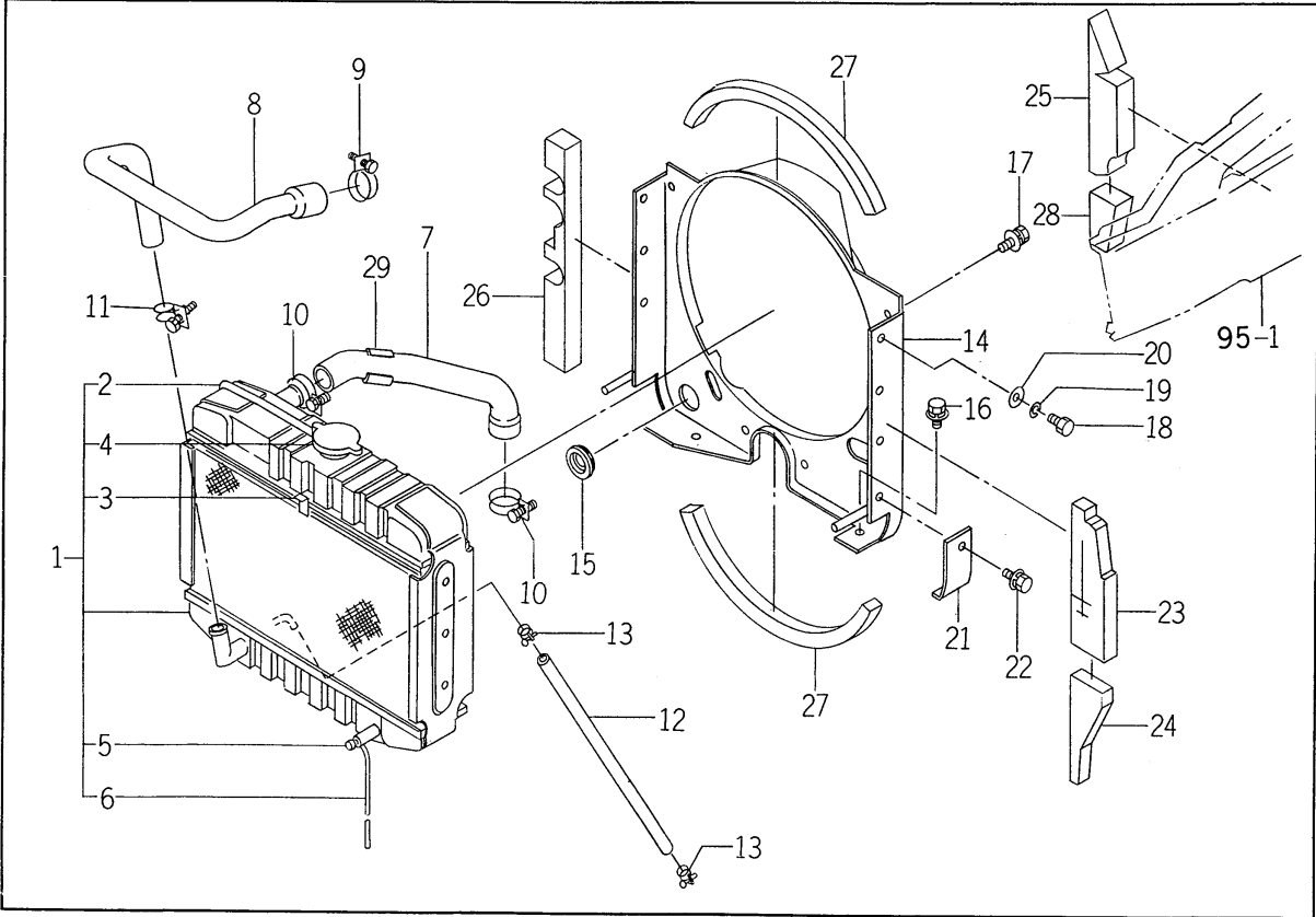
FIG.# 20 RADIATOR SYSTEM P. 39
