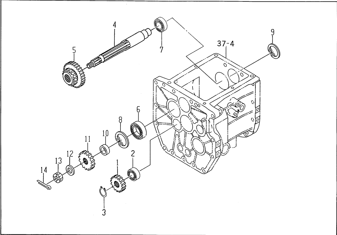
FIG.# 41 INPUT GEAR SYSTEM (HST) P. 91
