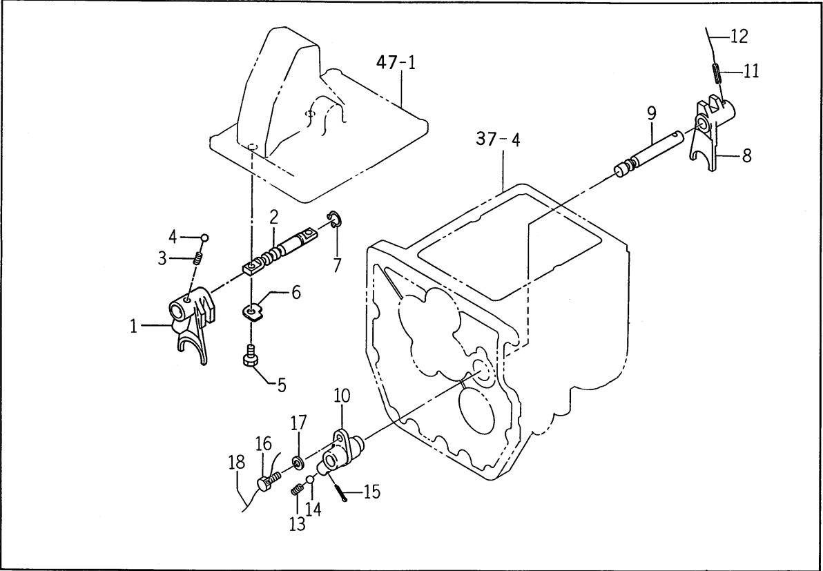
FIG.# 50 CHANGE SHIFT SYSTEM (HST) P. 109 TU315FE
