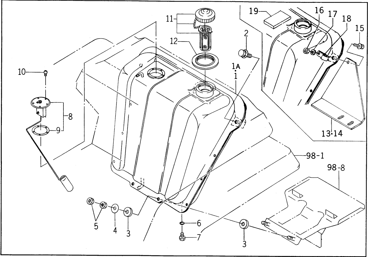
FIG.# 103 UEL TANK SYSTEM P. 217 TU315FE
