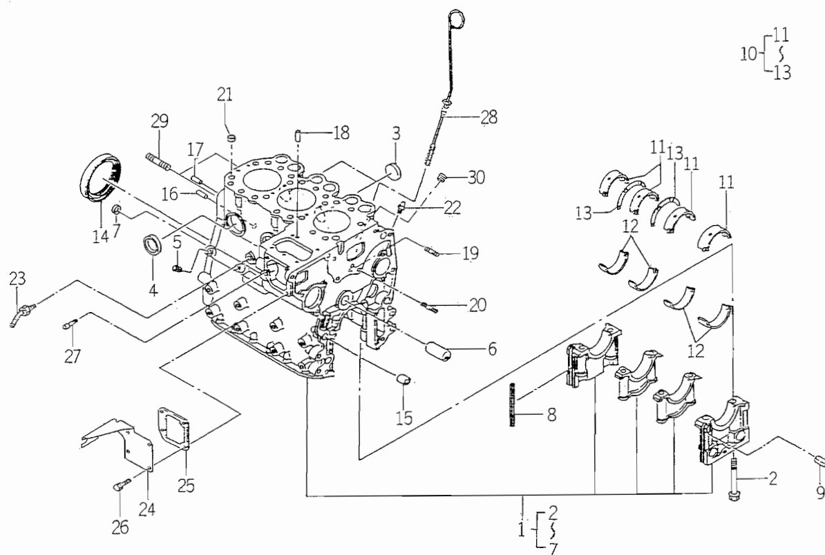
FIG. 5 CYLINDER BLOCK
