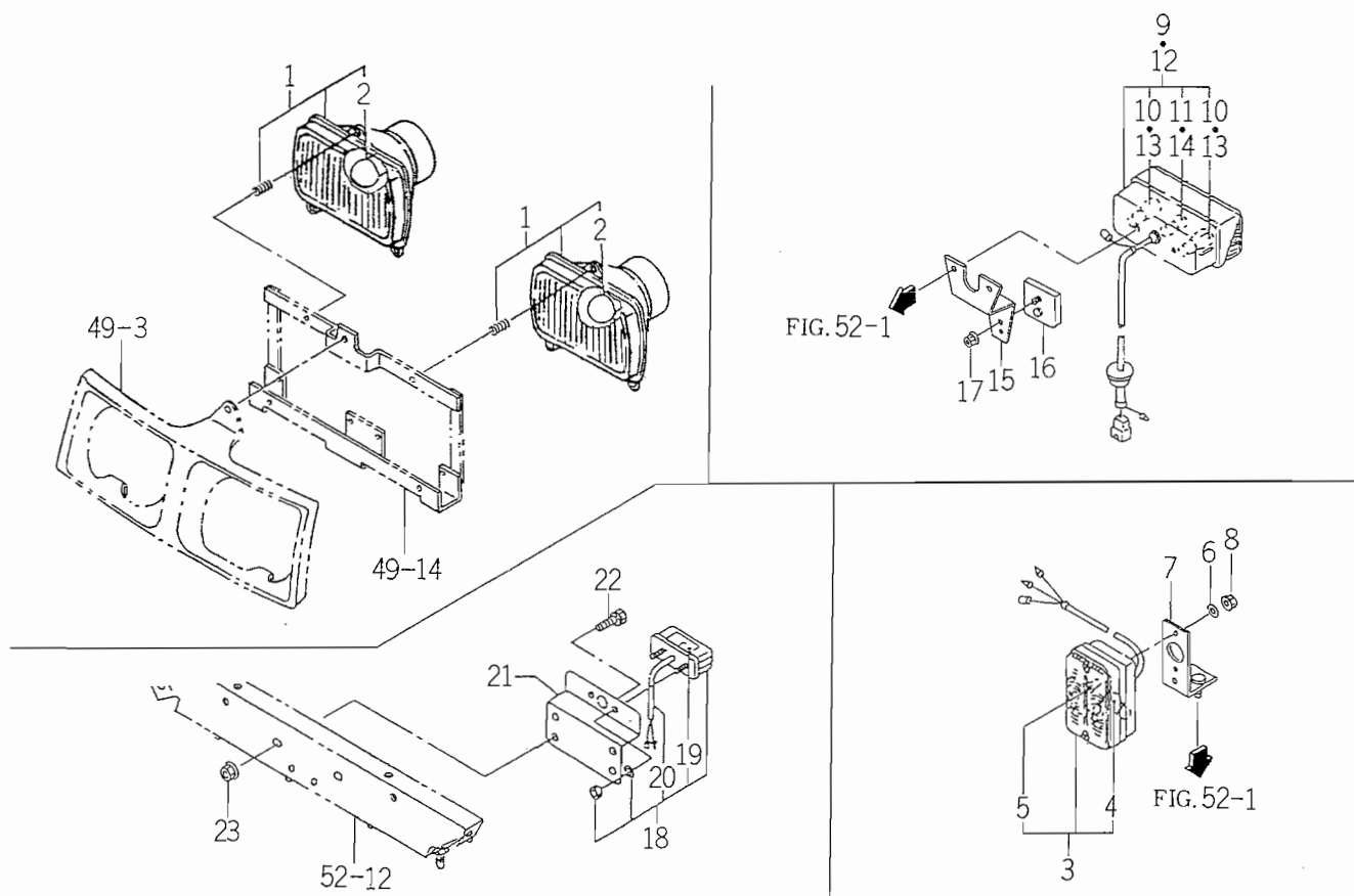
FIG. 55 LAMP SYSTEM
