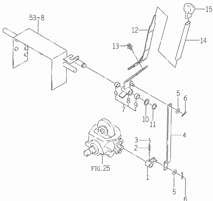
FIG. 26 MID PTO LEVER SYSTEM
