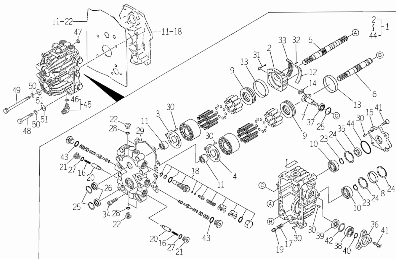
FIG. 13 HST SYSTEM
