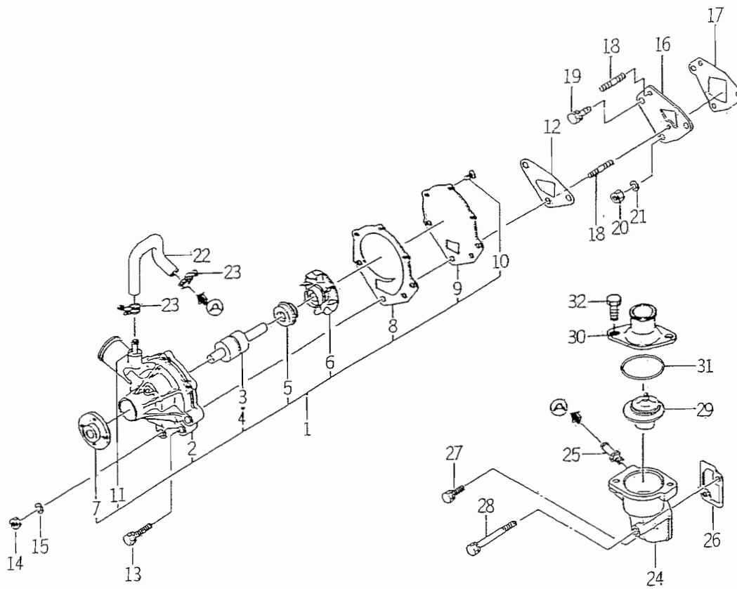
FIG. 17 WATER PUMP
