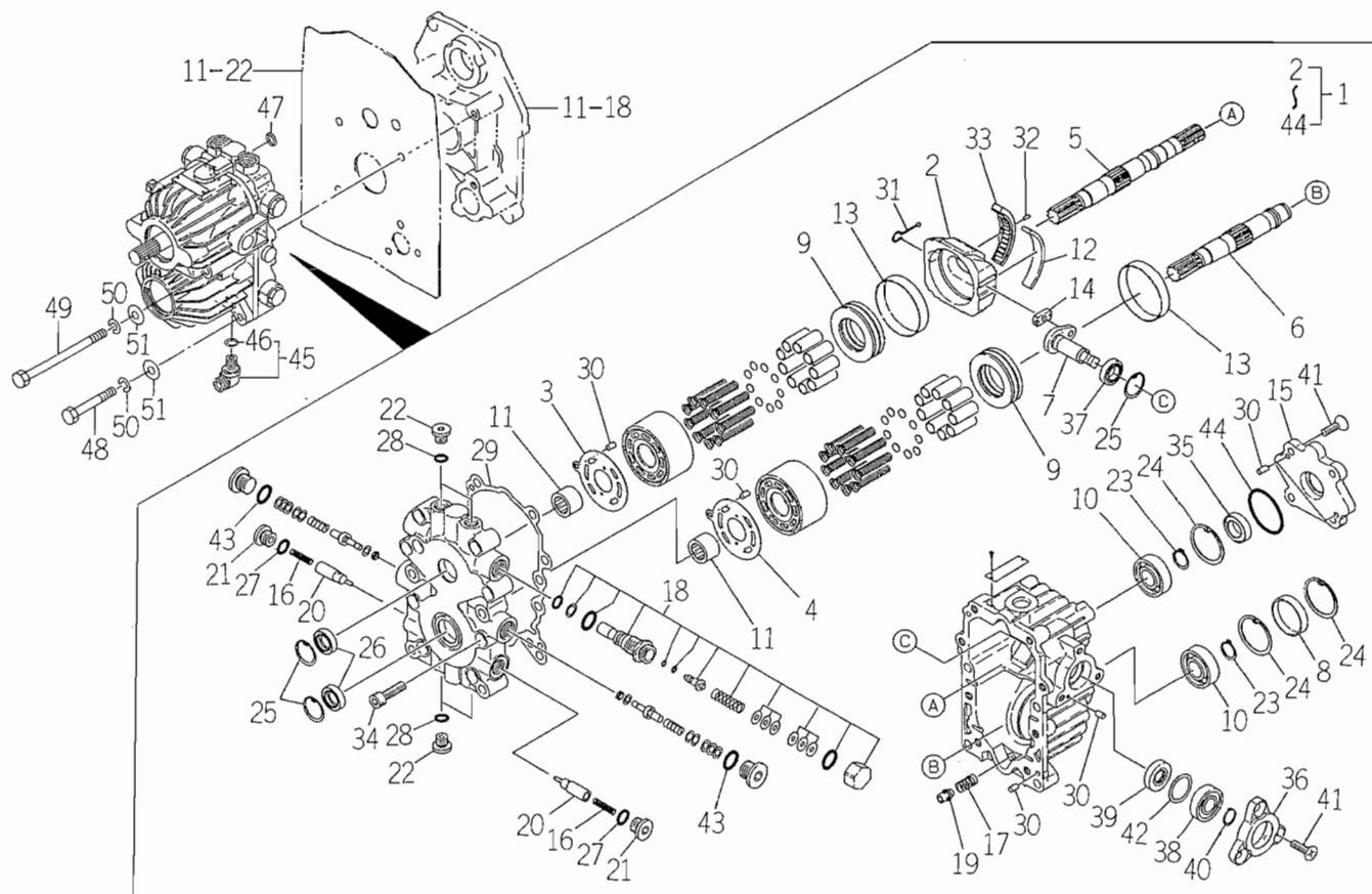
FIG. 13 HST SYSTEM
