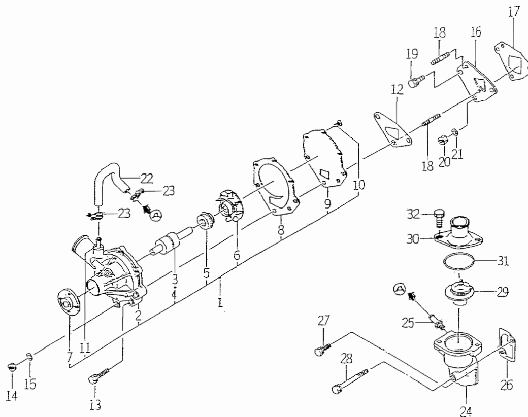
FIG. 17 WATER PUMP
