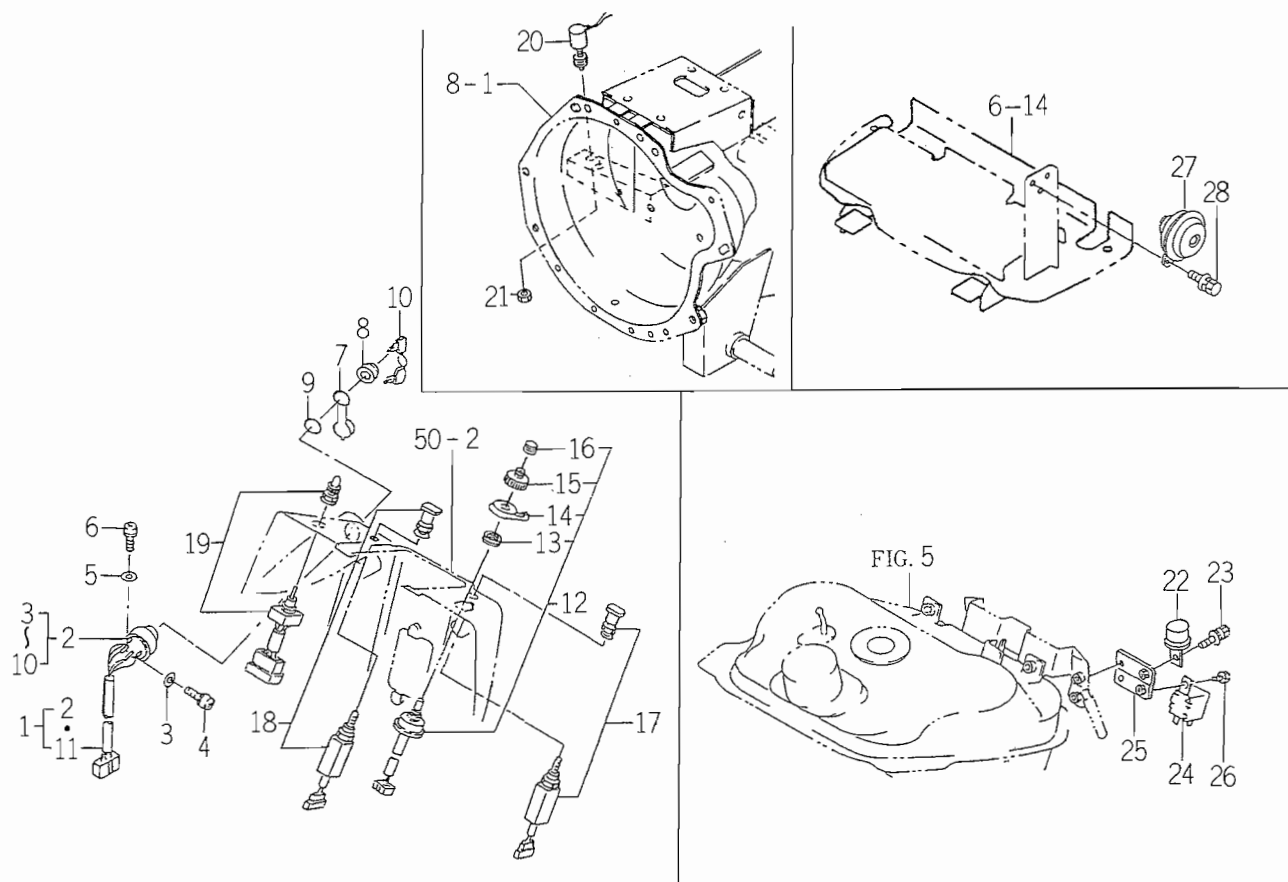
FIG. 57 SWITCH SYSTEM
