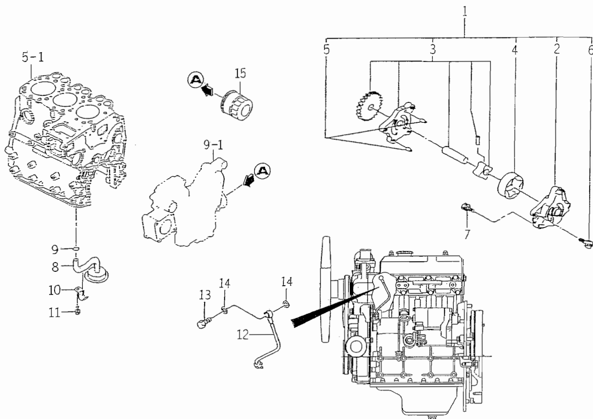
FIG. 16 OIL PUMP
