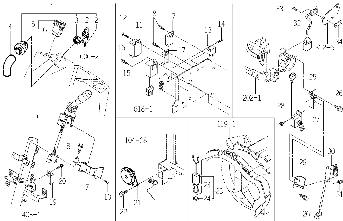
FIG.629 SWITCH SYSTEM (TM3265-H TYPE)
