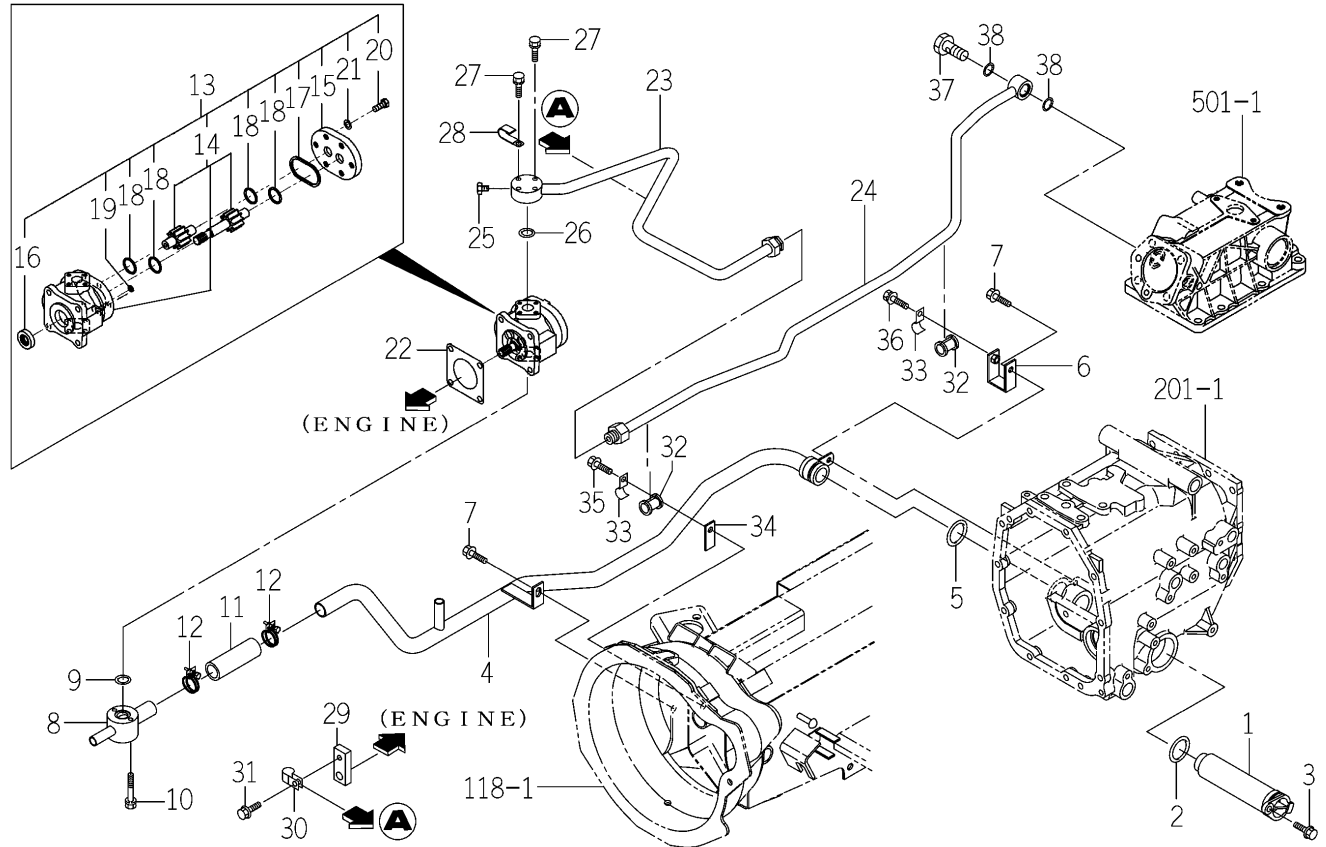
FIG.508 PIPING (MAIN) SYSTEM (TM3265-EXCEPT H TYPE)
