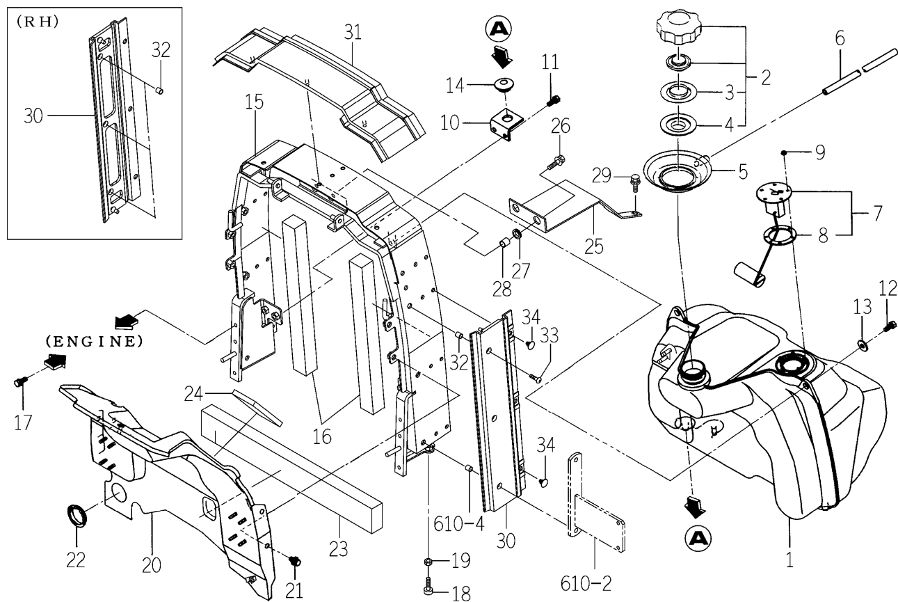
FIG.111 FUEL TANK SYSTEM
