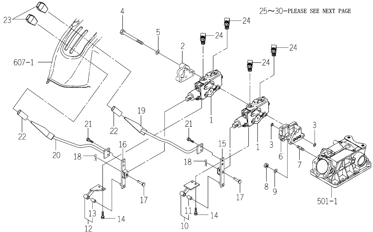
FIG.507 VALVE (REMOTE/2R) SYSTEM(1/2) (WR TYPE)
