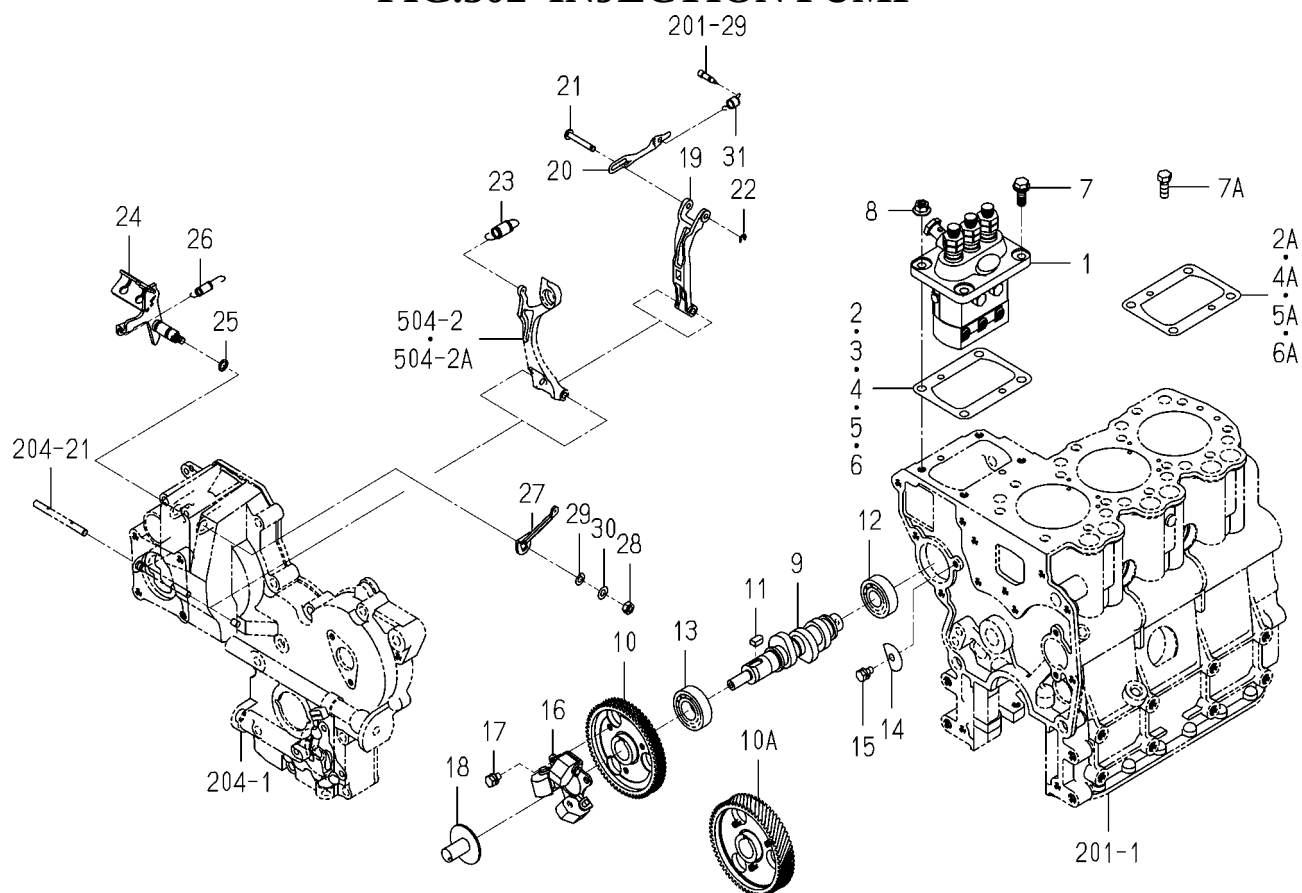
FIG.502 INJECTION PUMP
