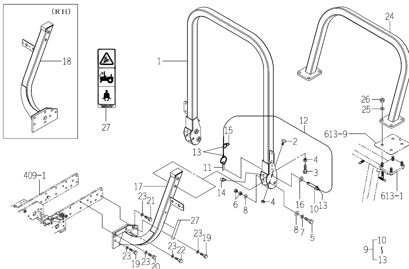
FIG.703 ROPS SYSTEM (TM3265-A TYPE)
