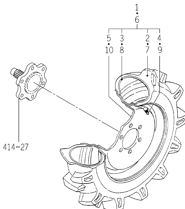
FIG.P08 FRONT WHEEL (4WD) SYSTEM (TM3245,3265-EXCEPT A TYPE) (OPTION)
