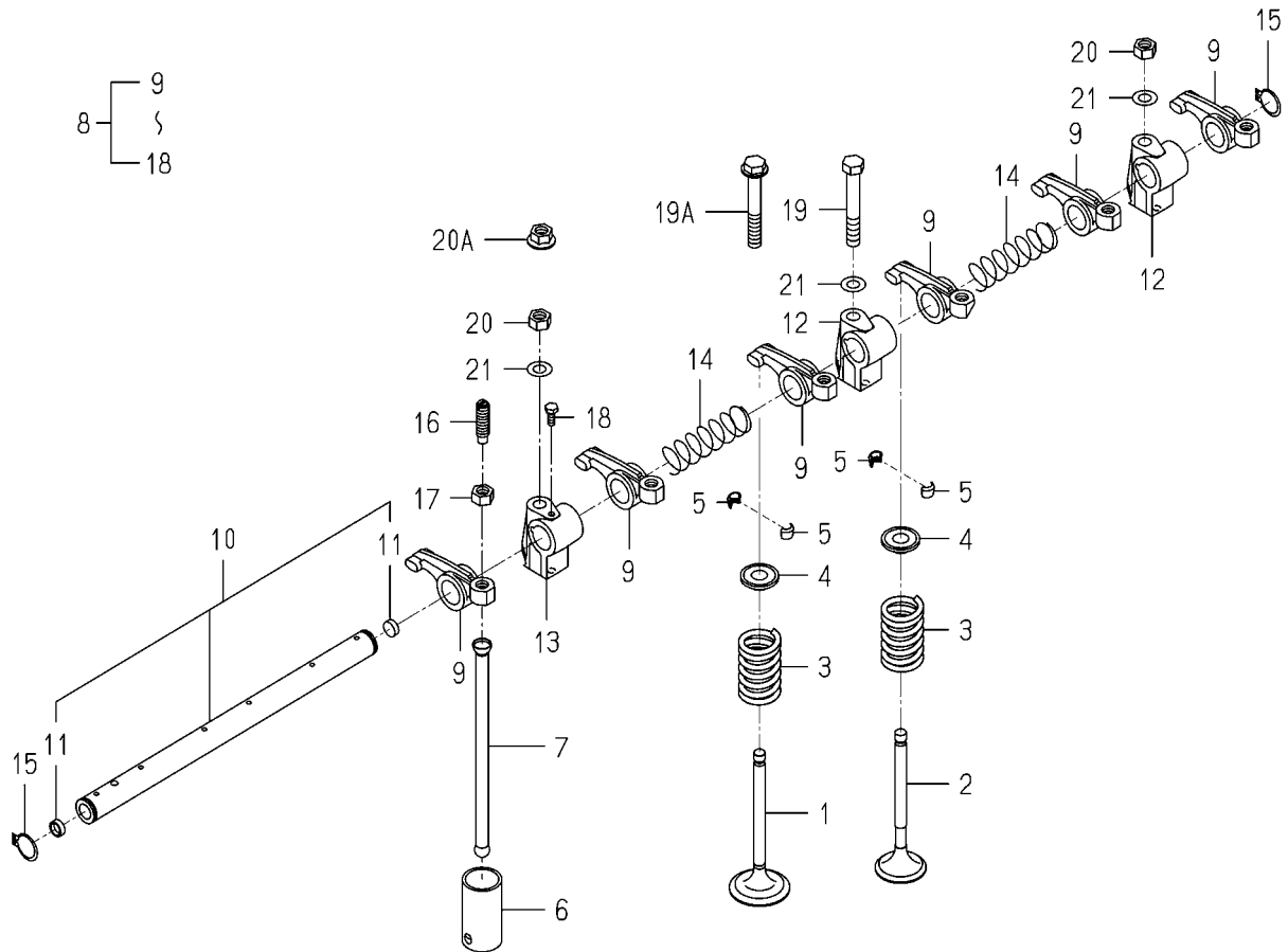
FIG.301 VALVE
