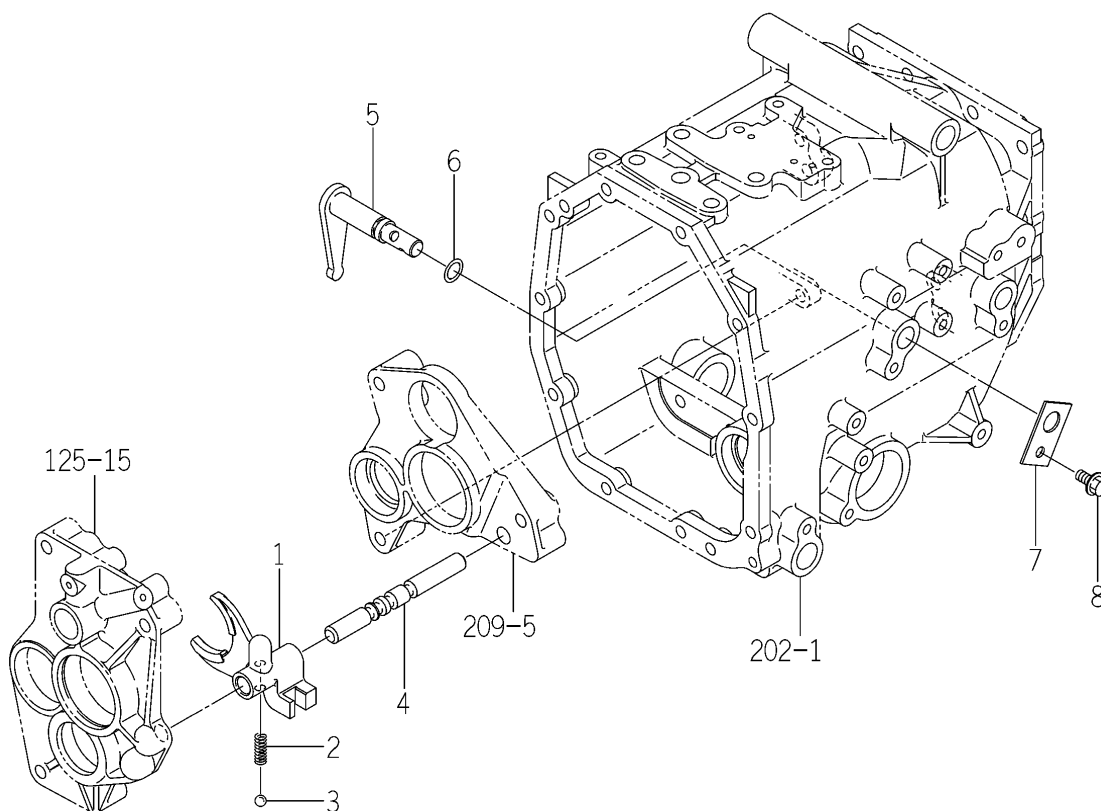
FIG.214 SUB CHANGE SYSTEM (H TYPE)
