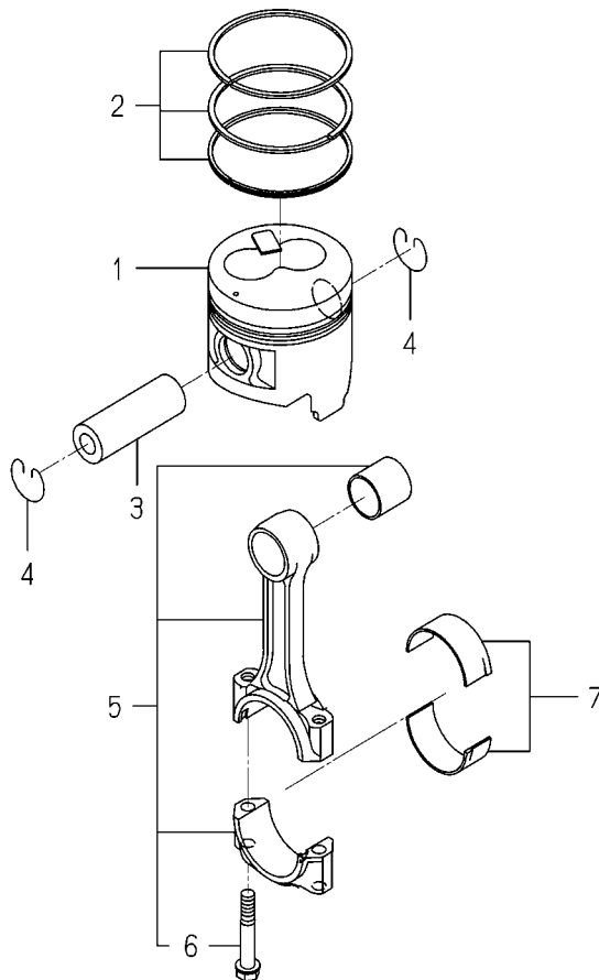
FIG.303 PISTON
