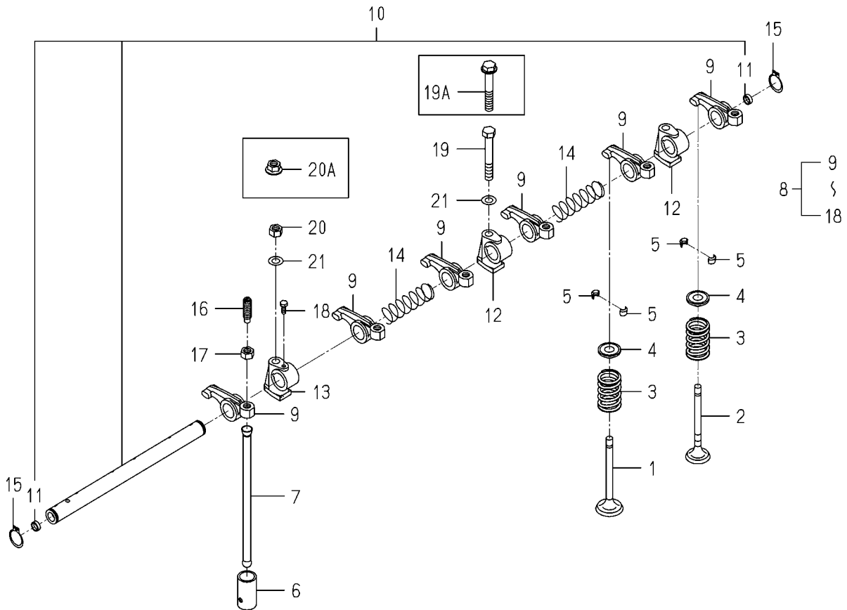
FIG.301 VALVE
