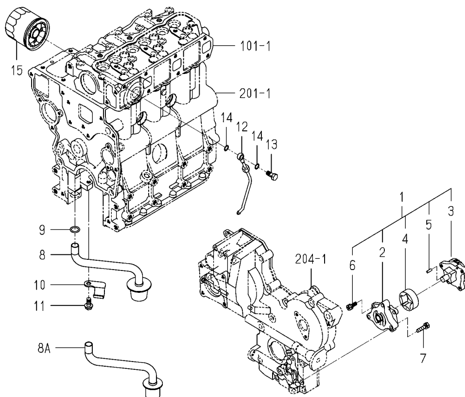
FIG.401 OIL PUMP
