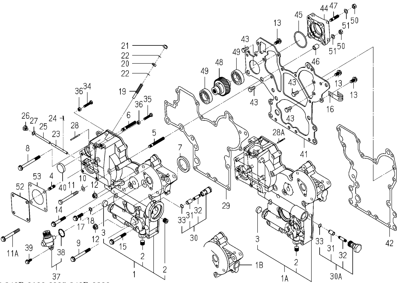
FIG.204 TIMING GEAR CASE
