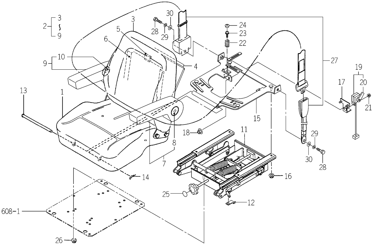
FIG.609 SEAT (NUMBER) SYSTEM (E6 TYPE)
