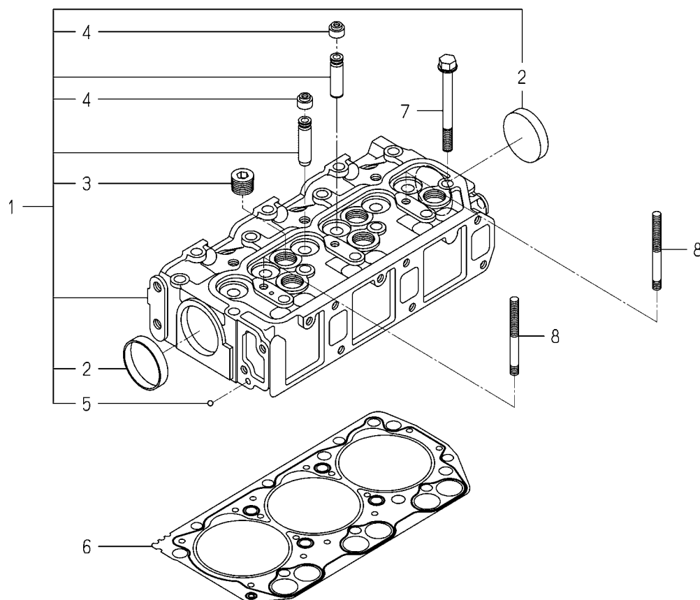
FIG.101 CYLINDER HEAD
