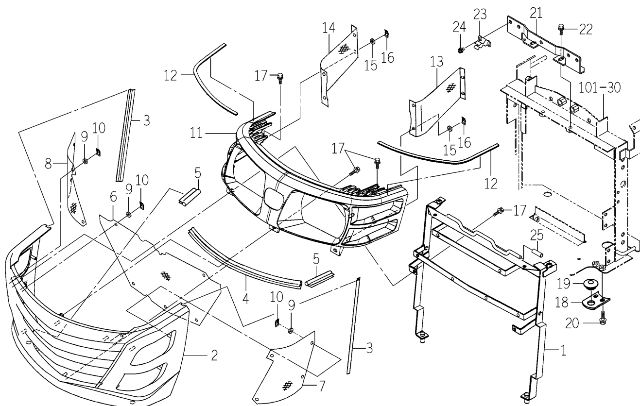
FIG.603 GRILLE SYSTEM (TM3215,3245)
