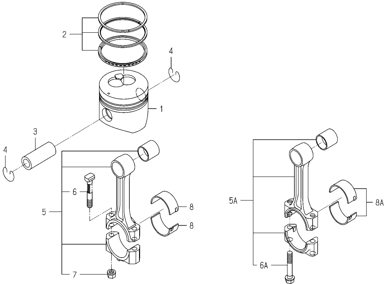
FIG.303 PISTON
