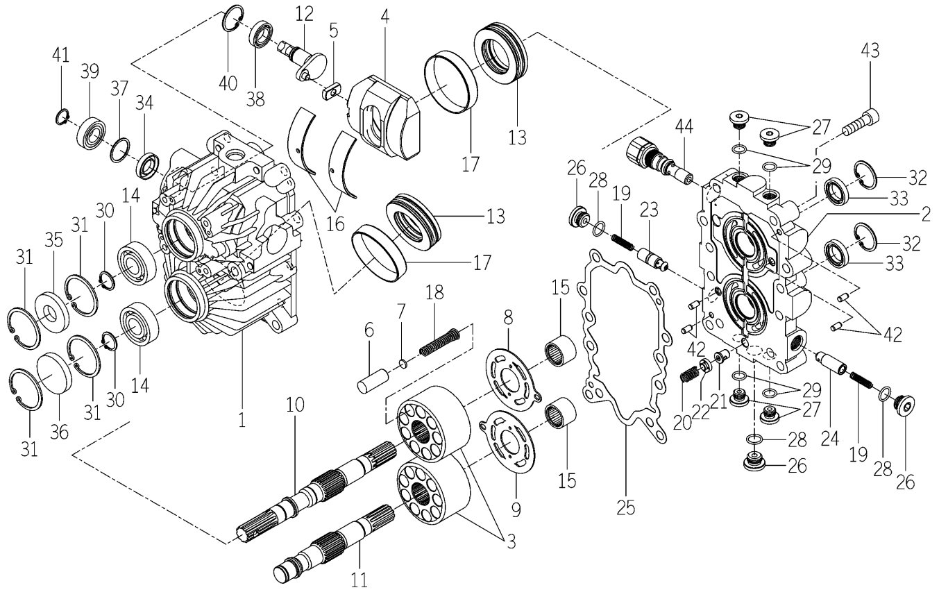
FIG.S03 COMPONENT PARTS FOR K510-014-000-00 ON Fig.203
