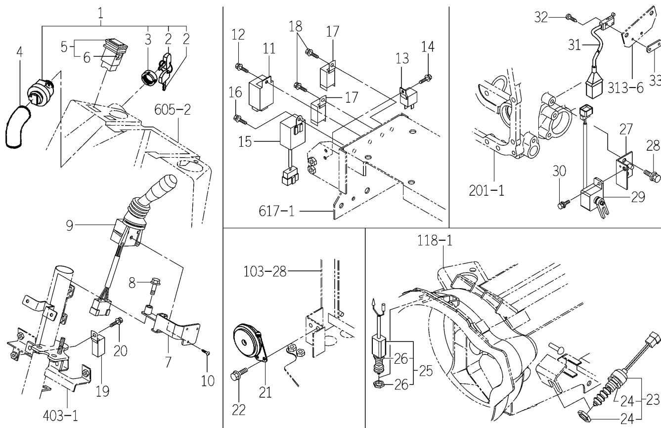
FIG.628 SWITCH SYSTEM (TM3265-EXCEPT H TYPE)
