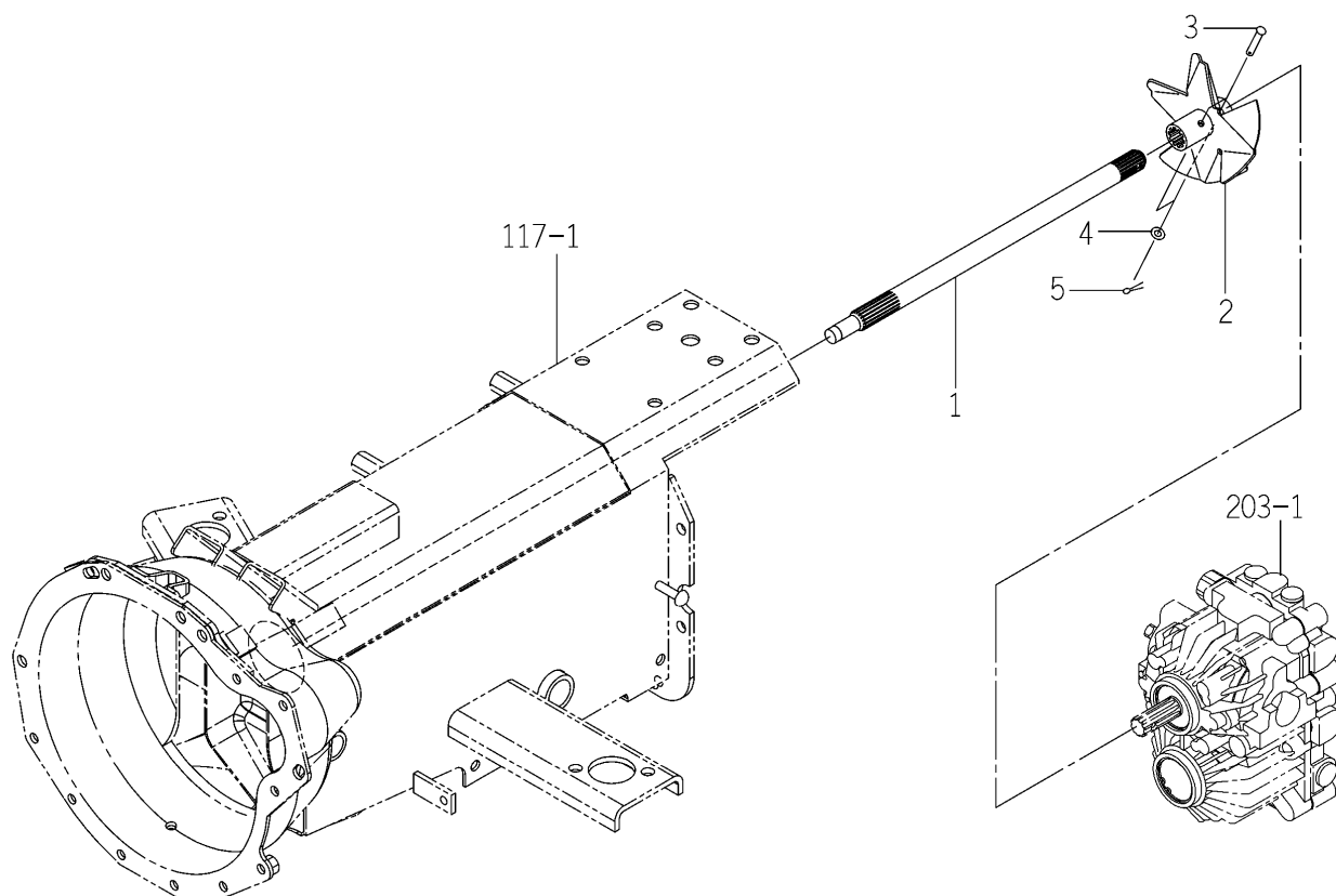
FIG.122 INPUT SHAFT SYSTEM (H TYPE)
