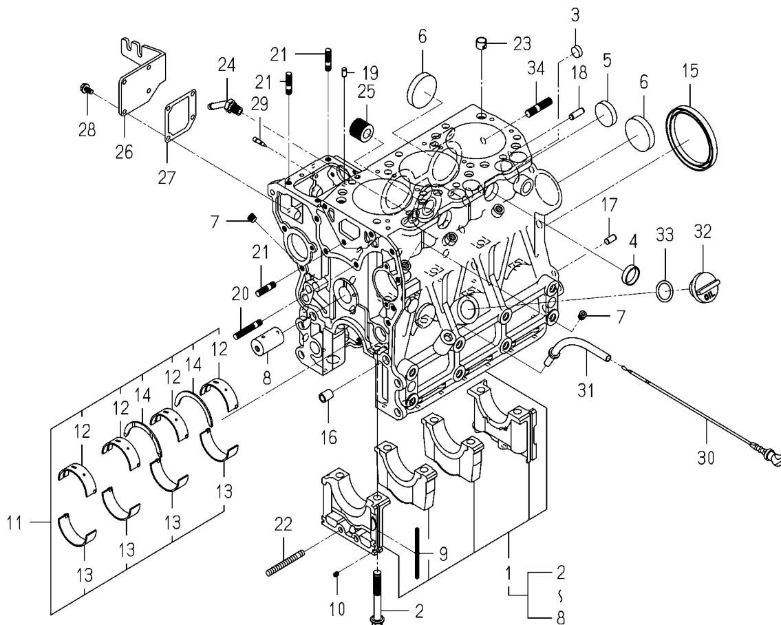
FIG.201 CYLINDER BLOCK
