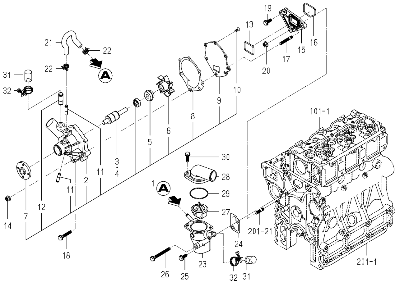
FIG.402 WATER PUMP
