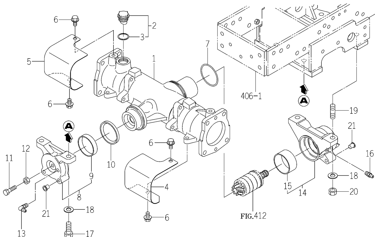
FIG.413 HOUSING (AXLE) SYSTEM
