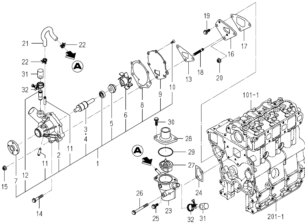
FIG.402 WATER PUMP
