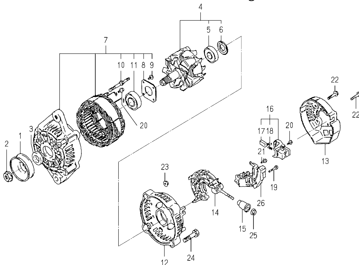
FIG.S04 COMPONENT PARTS FOR 6281-200-005-00 ON Fig.801
