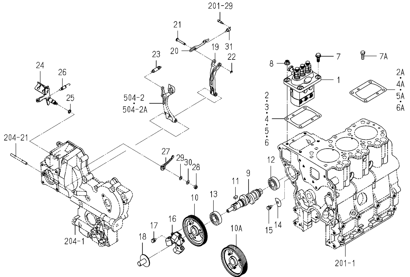
FIG.502 INJECTION PUMP
