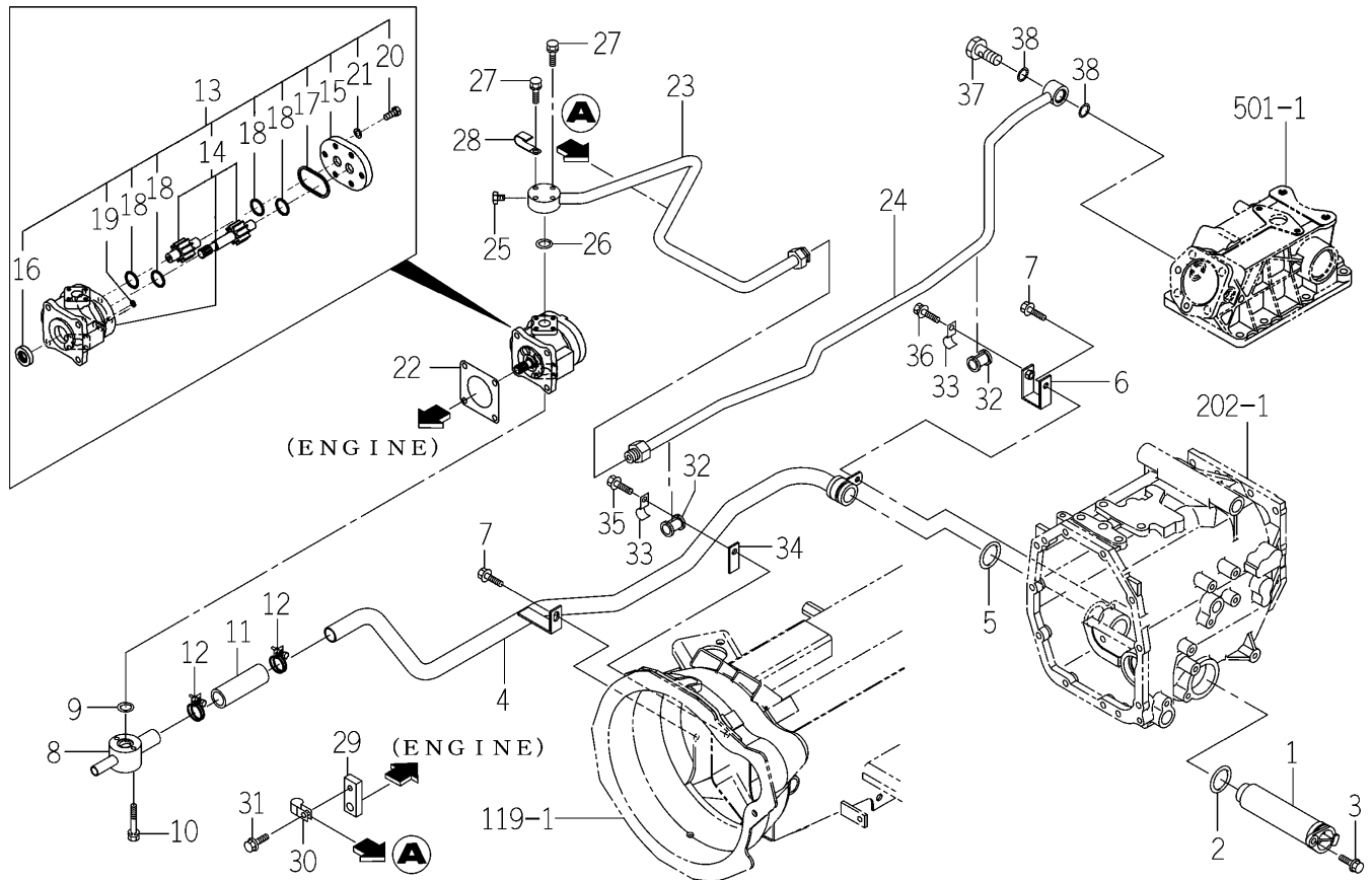
FIG.509 PIPING (MAIN) SYSTEM (TM3265-H TYPE)
