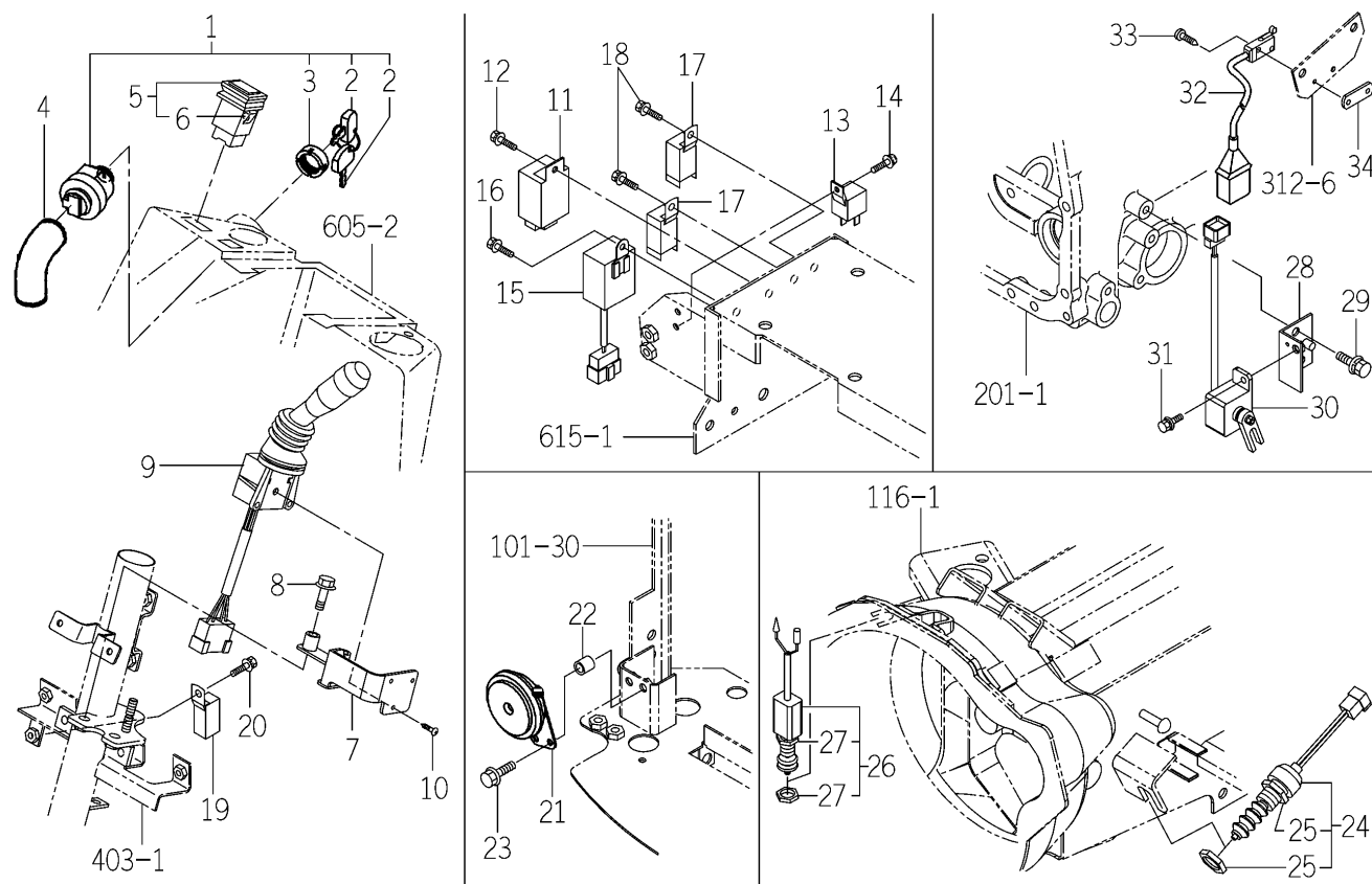
FIG.630 SWITCH SYSTEM (TM3215,3245-EXCEPT H TYPE)
