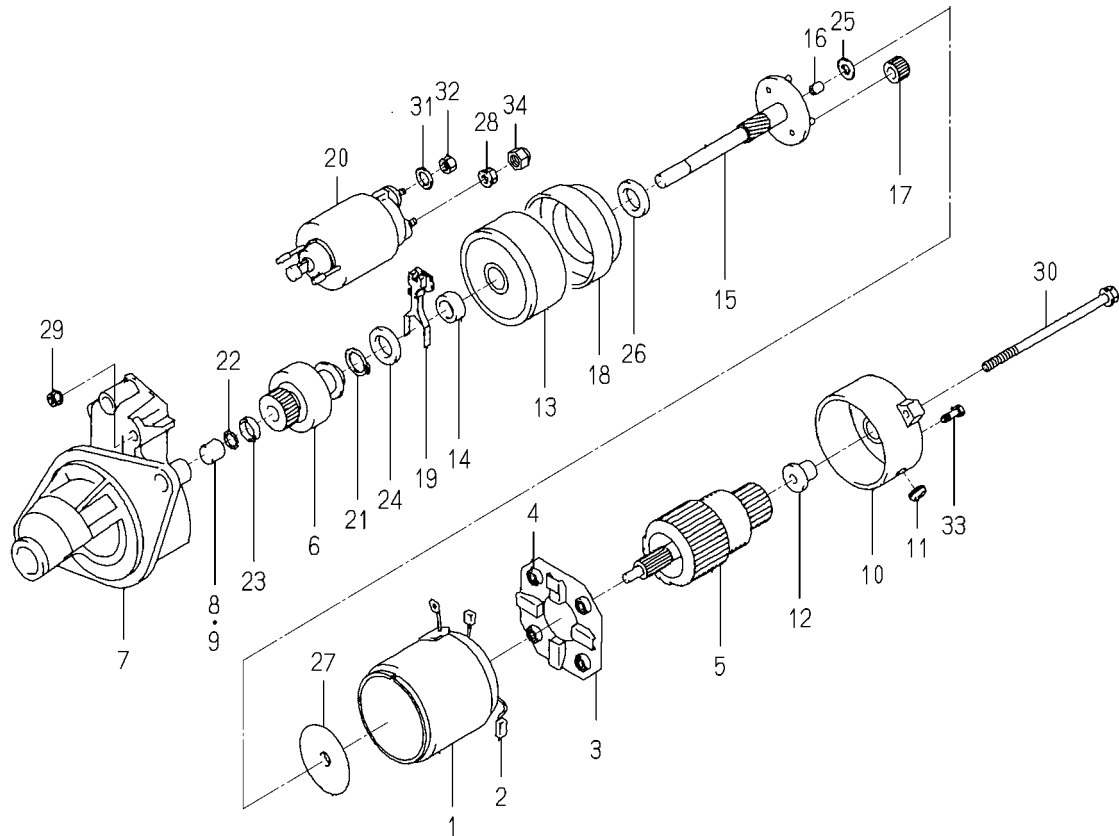
FIG.S03 COMPONENT PARTS FOR 6281-100-014-00 ON Fig.801
