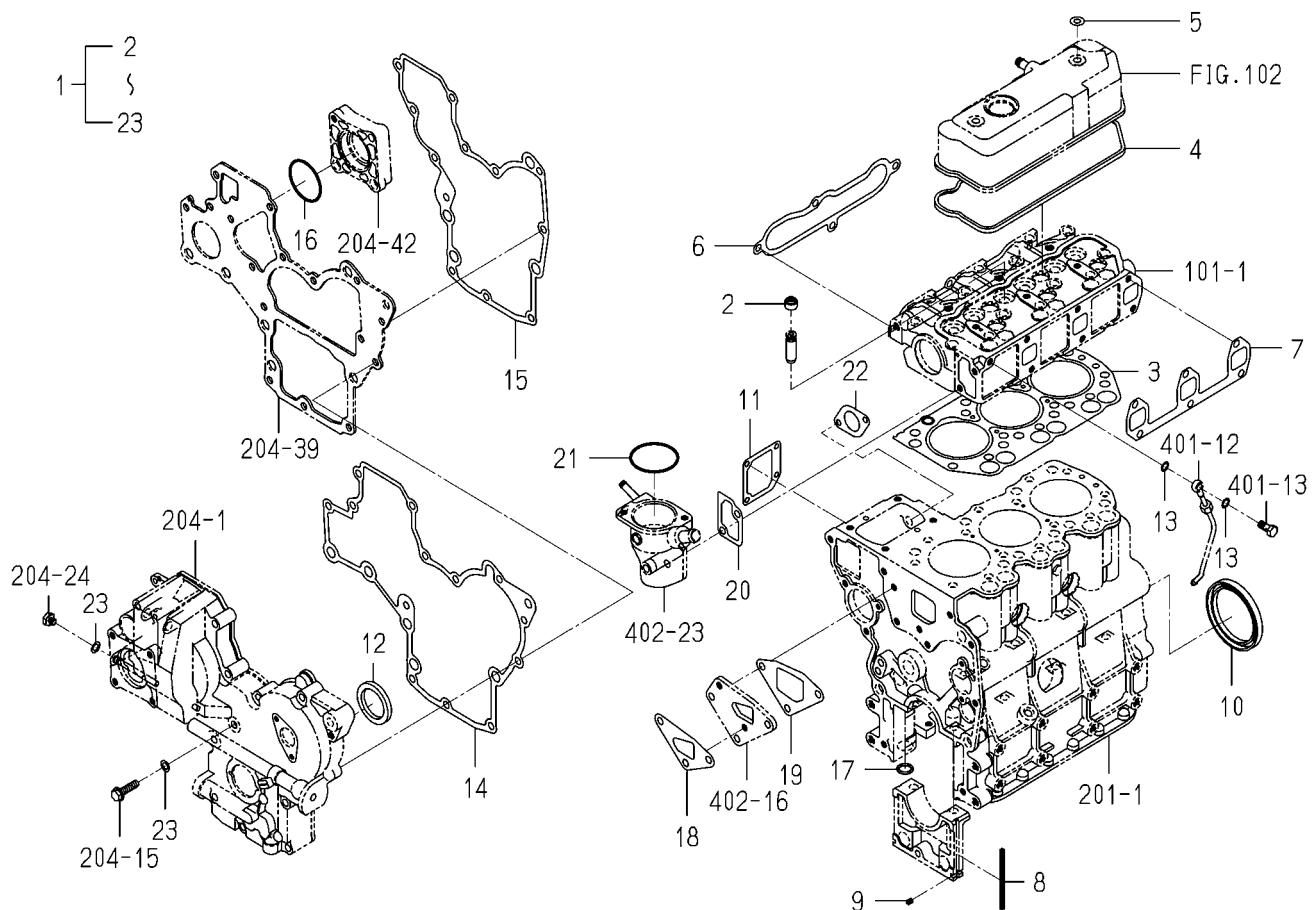
FIG.P04 REPAIR PARTS (OPTION)
