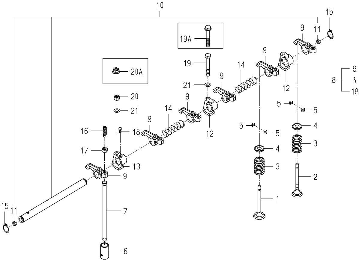
FIG.301 VALVE
