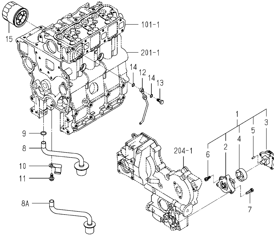
FIG.401 OIL PUMP
