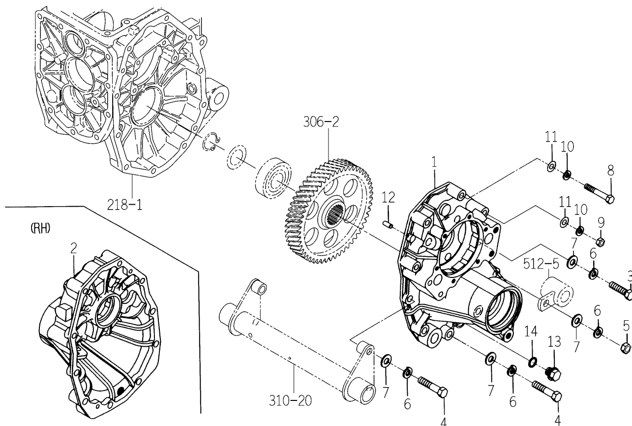
FIG.305 REAR AXLE HOUSING SYSTEM
