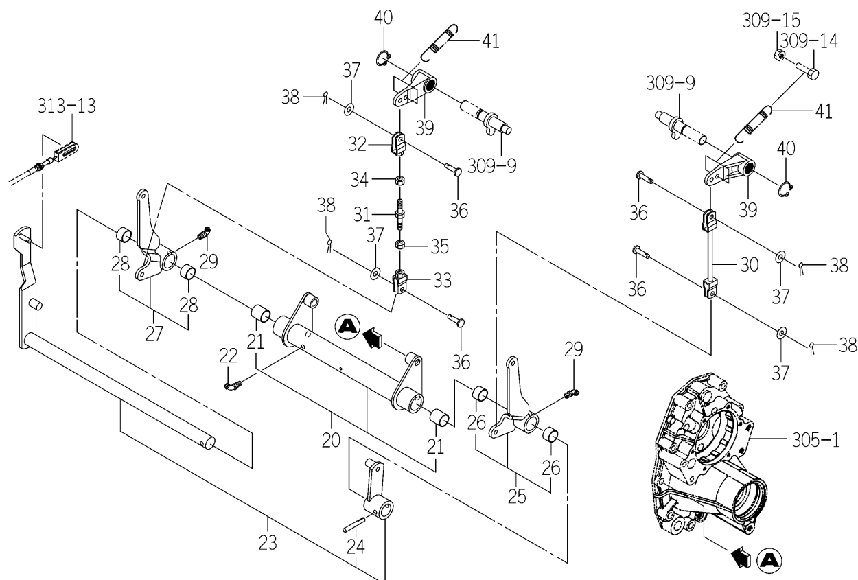
FIG.310 PEDAL (BRAKE) SYSTEM(2/2) (EXCEPT H TYPE)
