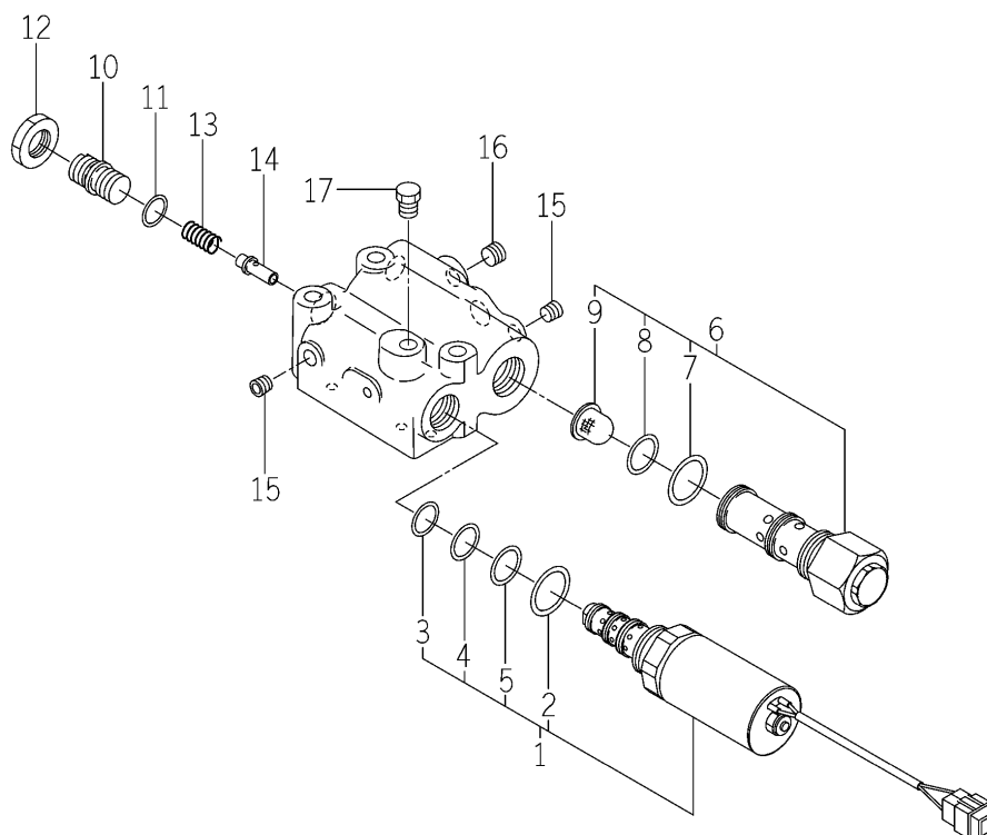
FIG.S01 COMPONENT PARTS FOR K200-208-000-00 ON Fig.405
