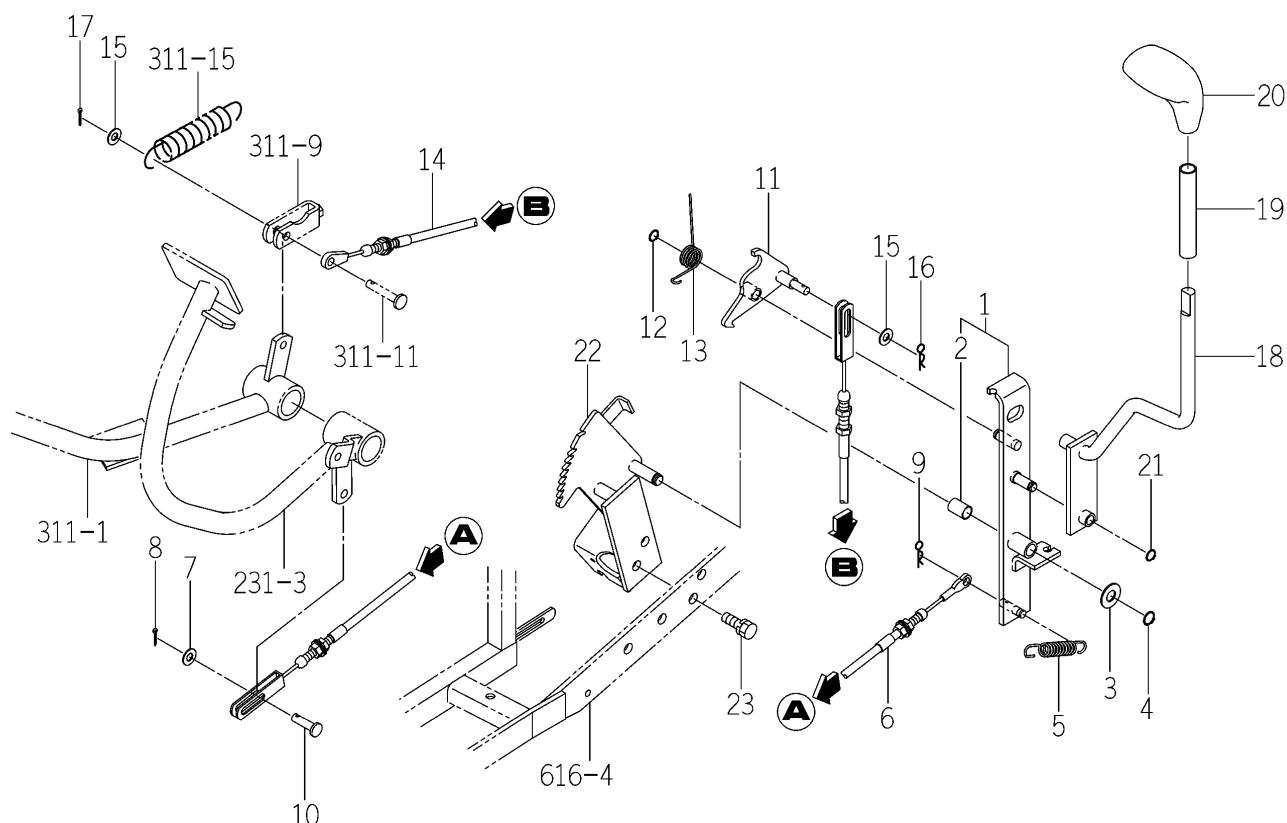
FIG.232 LEVER (HST) SYSTEM (H TYPE)
