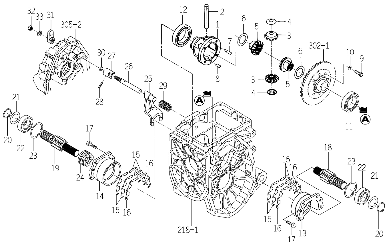
FIG.304 DIFF CASE SYSTEM (H TYPE)
