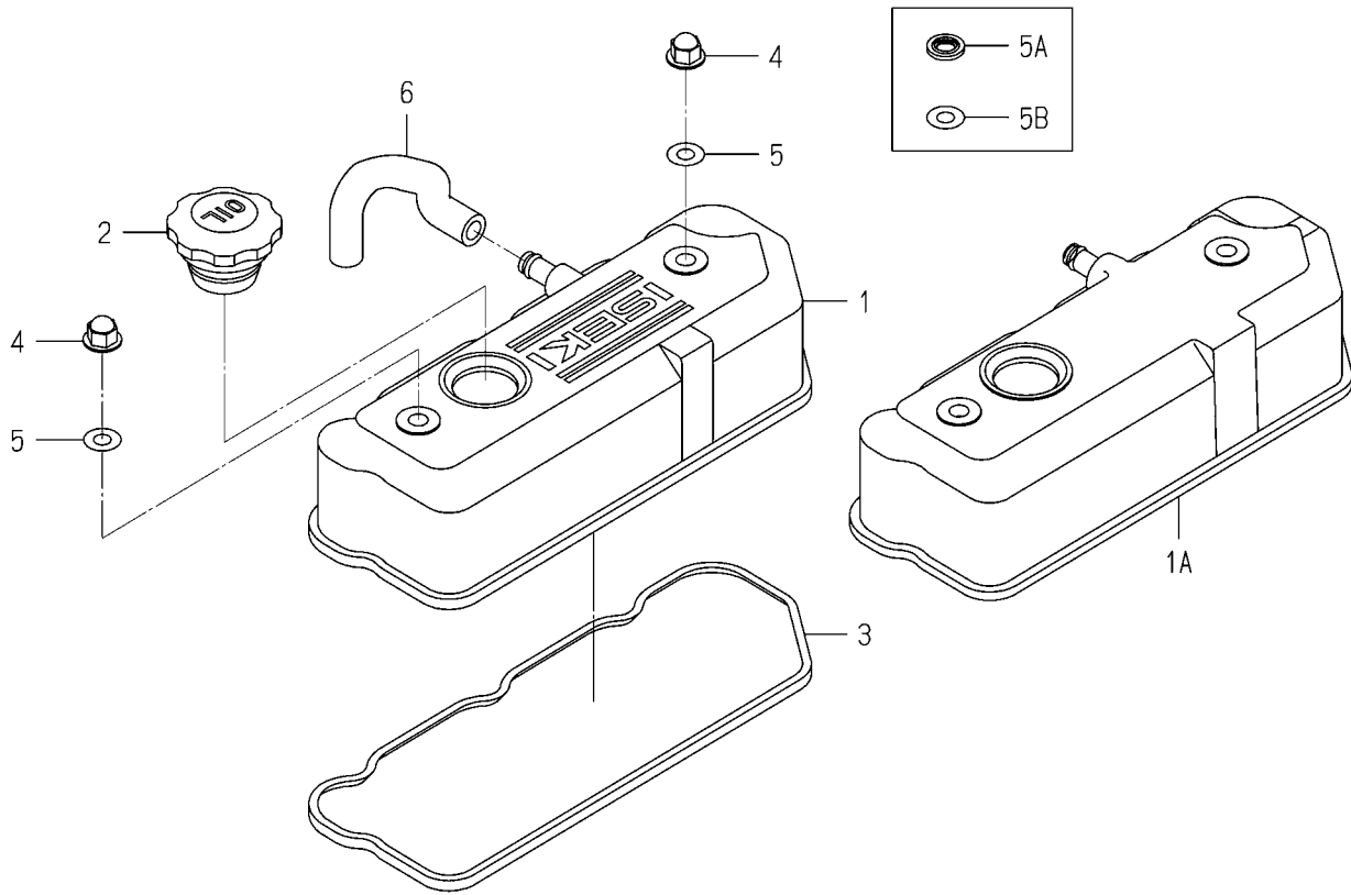
FIG.102 CYLINDER HEAD COVER
