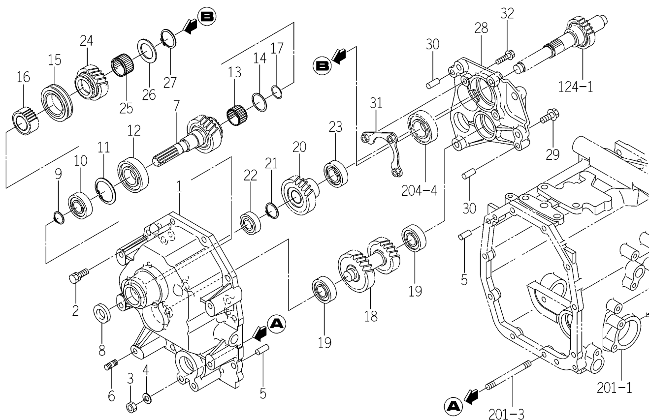
FIG.123 DRIVE GEAR SYSTEM (EXCEPT H TYPE)
