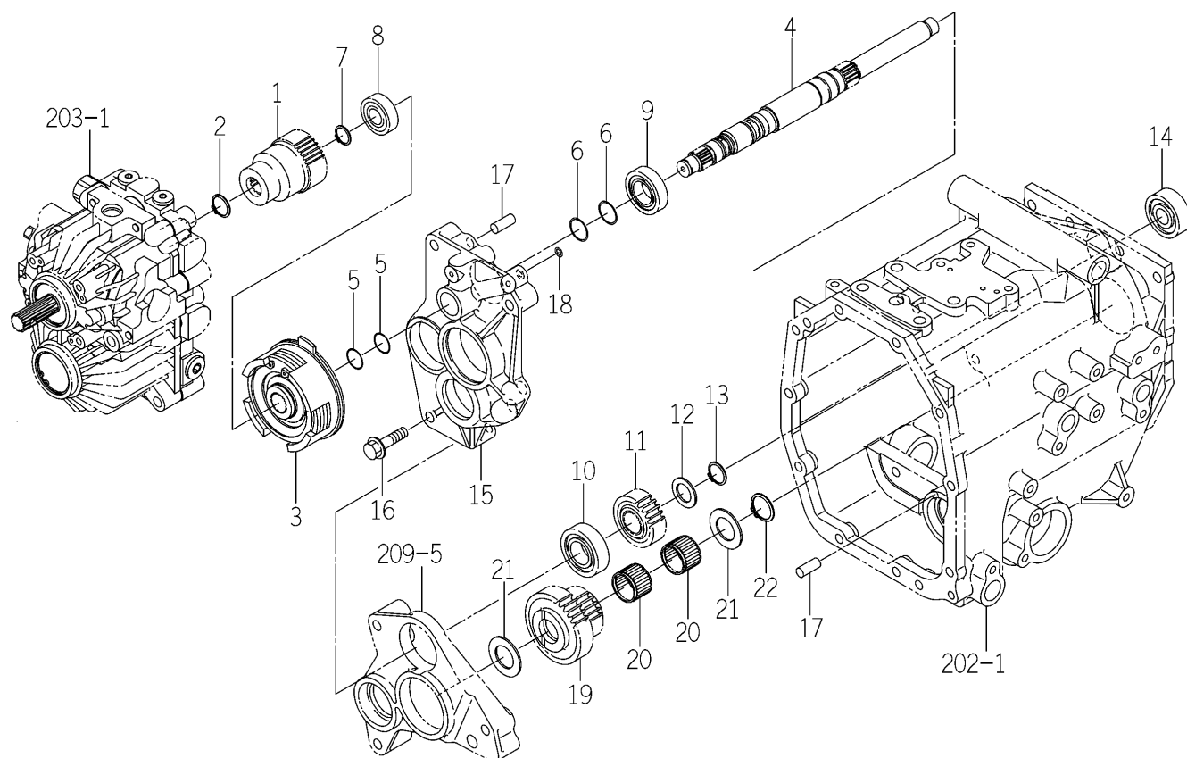
FIG.125 PTO DRIVE GEAR SYSTEM (H TYPE)
