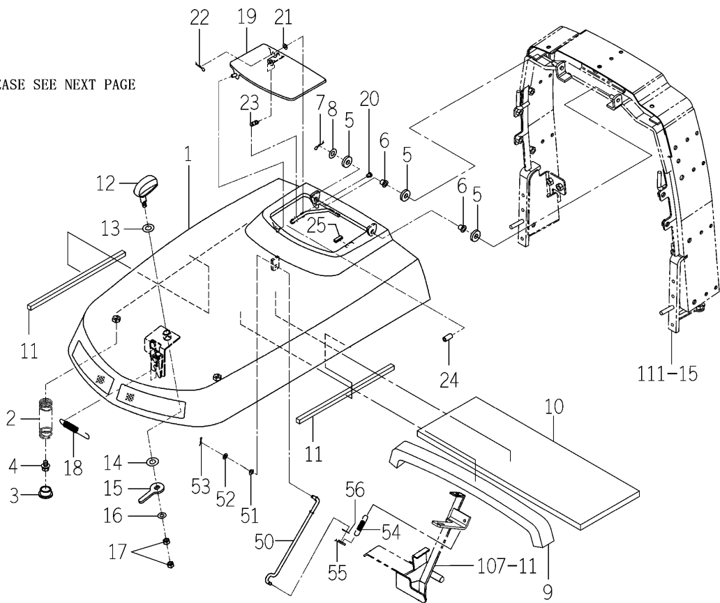
FIG.601 HOOD SYSTEM (TM3215,3245)(1/2)
