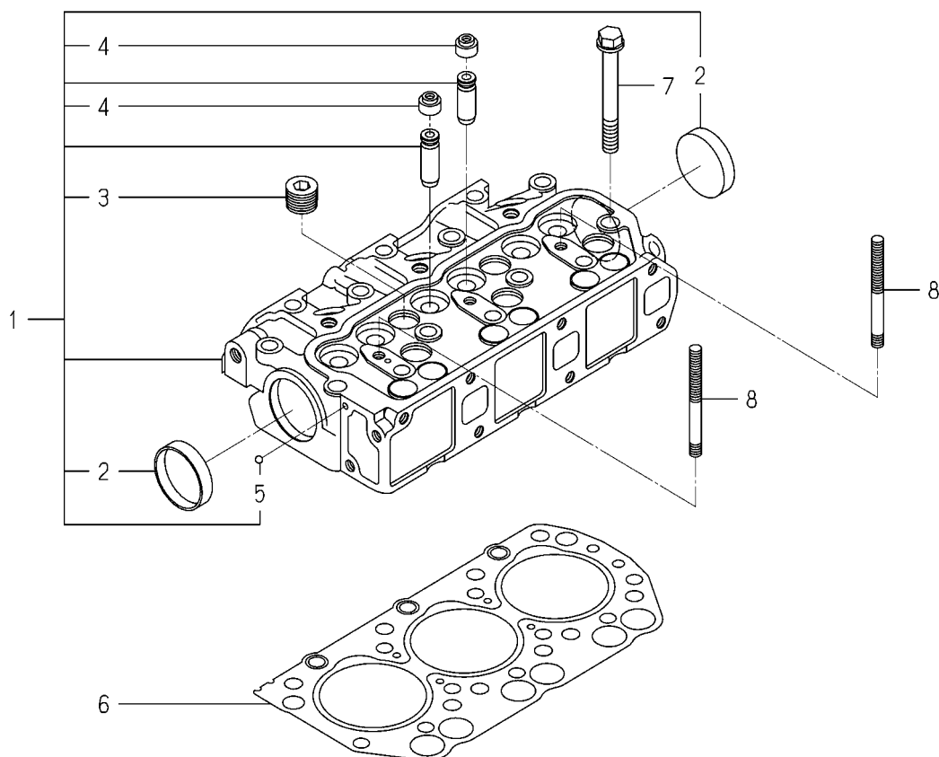
FIG.101 CYLINDER HEAD
