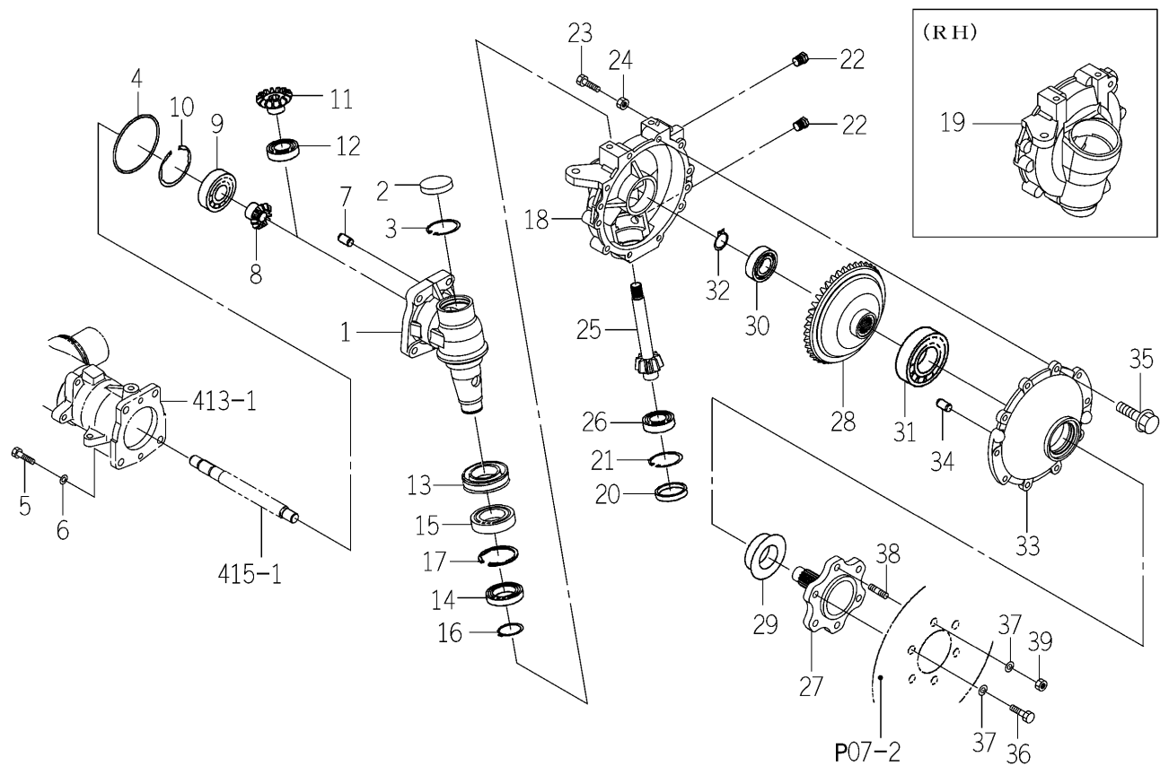
FIG.414 GEAR (FINAL) SYSTEM
