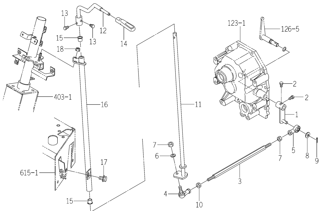
FIG.127 REVERSE LEVER SYSTEM (EXCEPT H TYPE)
