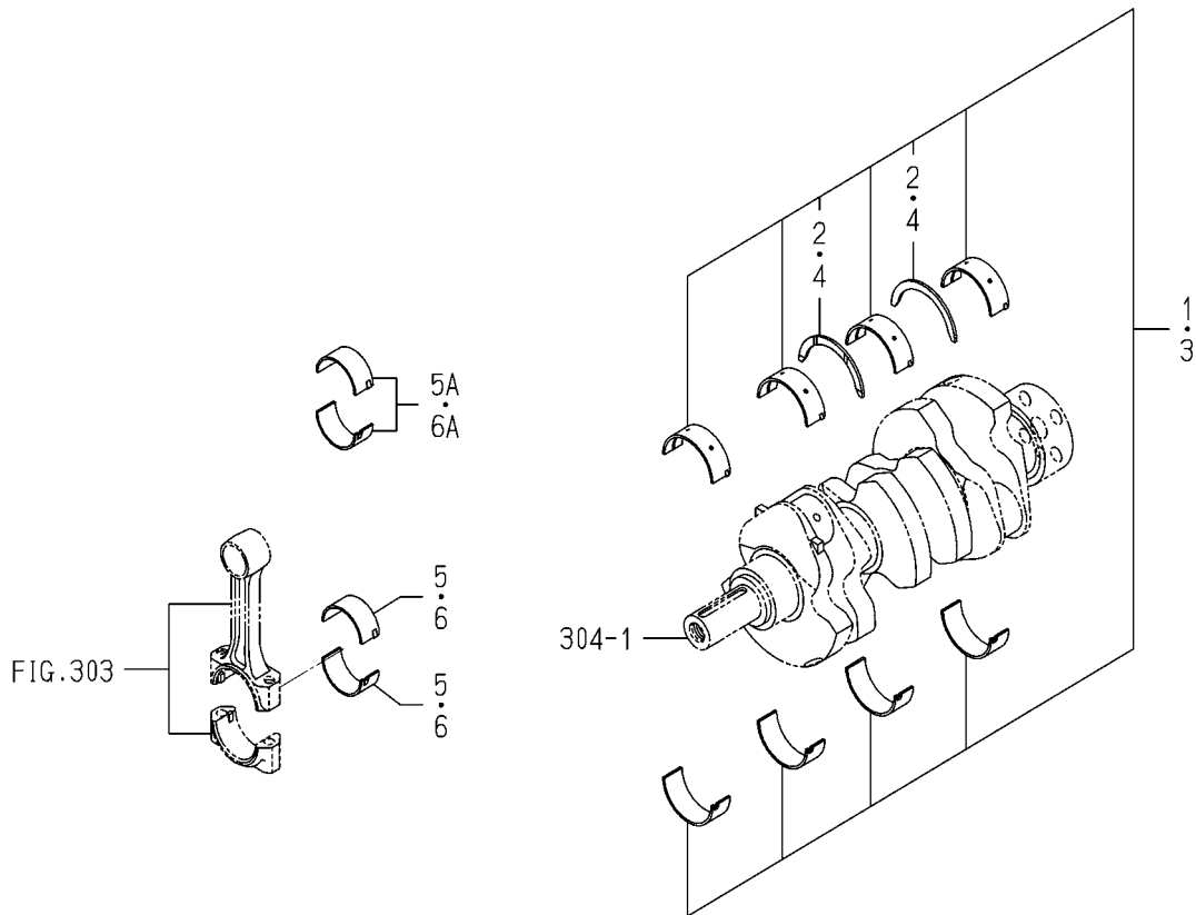
FIG.P02 BEARING/UNDER SIZE (OPTION)
