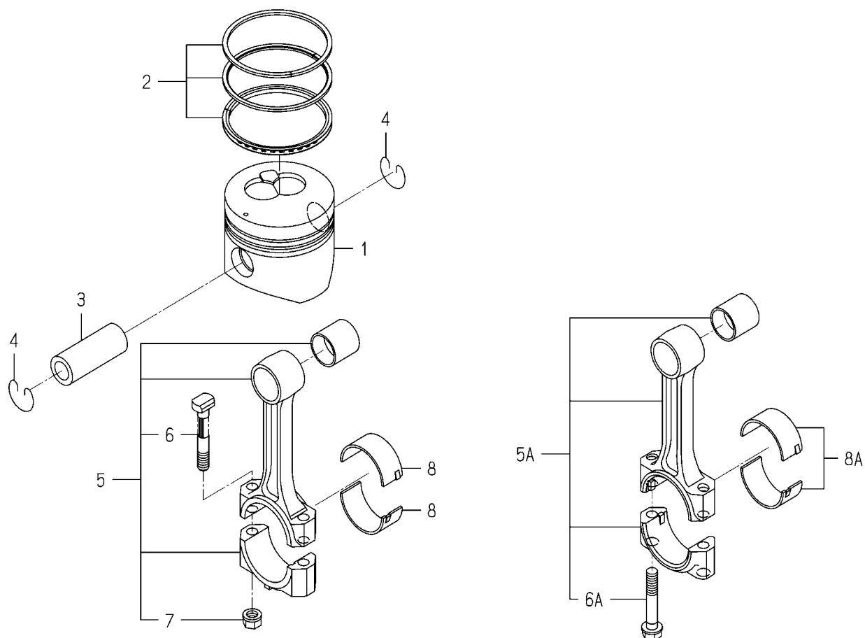
FIG.303 PISTON
