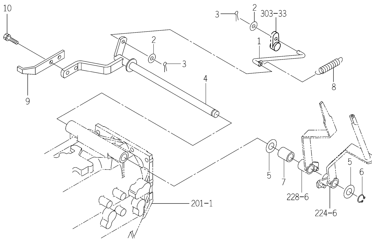
FIG.307 DIFF-LOCK PEDAL SYSTEM (EXCEPT H TYPE)
