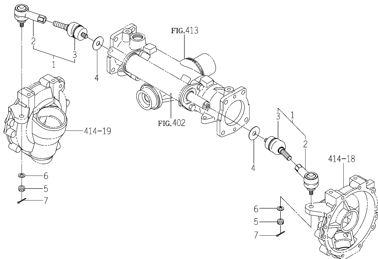
FIG.416 ROD (TIE) SYSTEM
