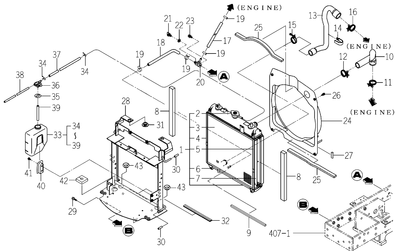
FIG.103 RADIATOR SYSTEM (TM3265-EXCEPT H TYPE)
