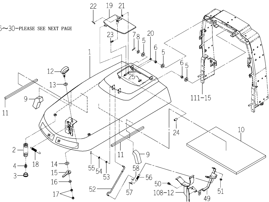
FIG.602 HOOD SYSTEM (TM3265)(1/2)
