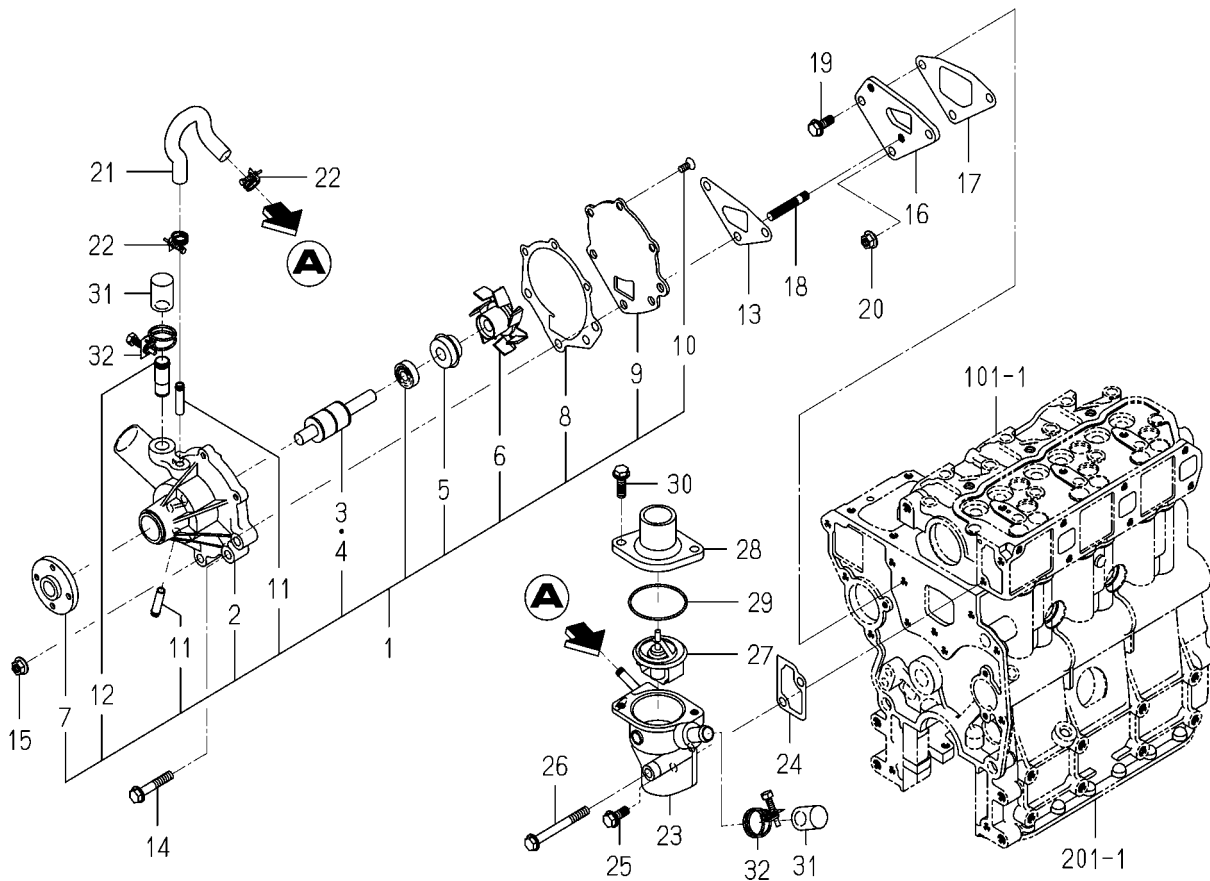
FIG.402 WATER PUMP
