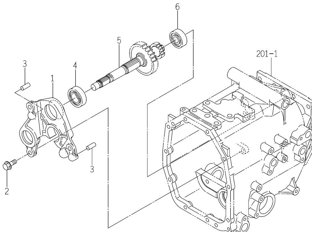
FIG.208 SUB CHANGE GEAR SYSTEM (EXCEPT H TYPE)
