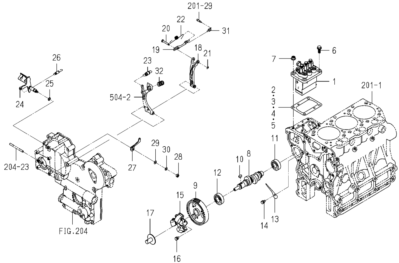
FIG.502 INJECTION PUMP
