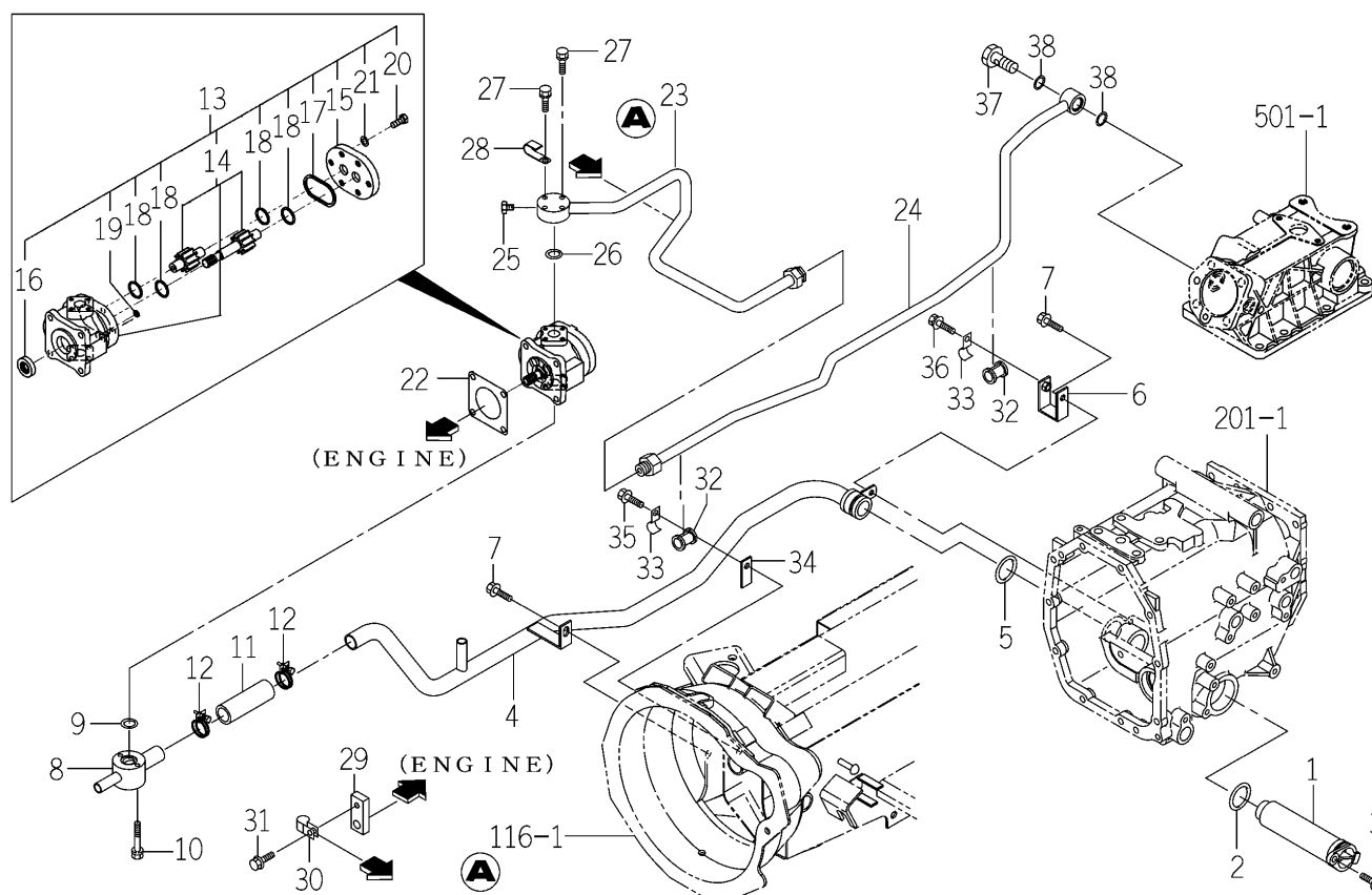
FIG.510 PIPING (MAIN) SYSTEM (TM3215,3245-EXCEPT H TYPE)
