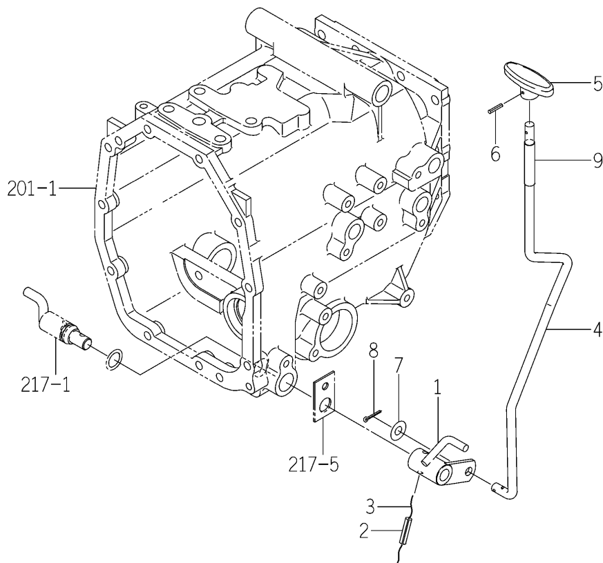
FIG.227 4WD LEVER SYSTEM
