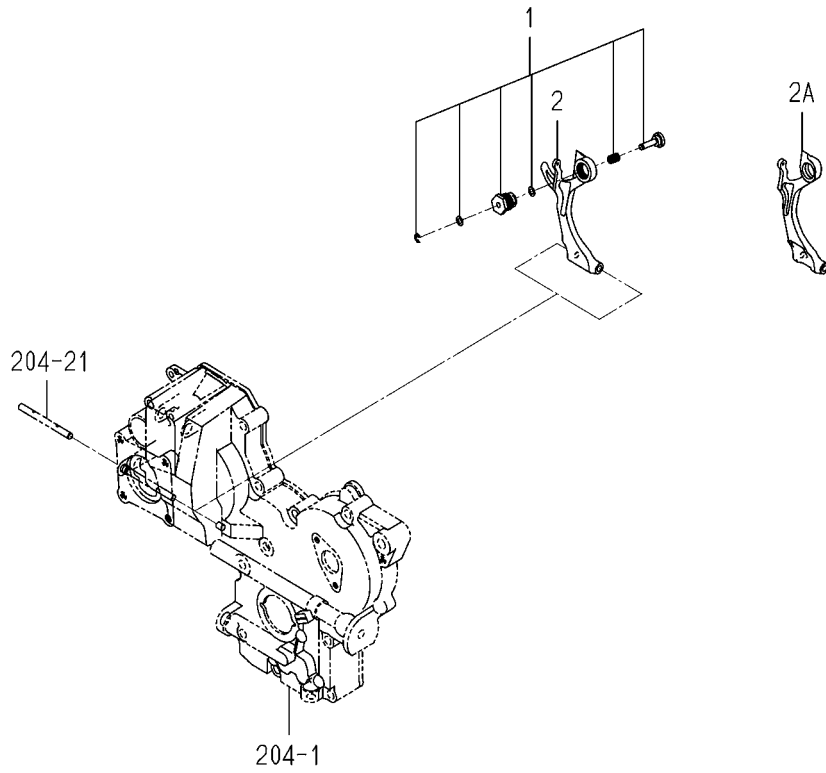
FIG.504 ADAPTER
