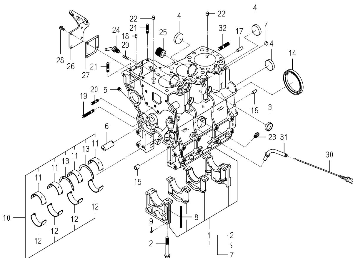
FIG.201 CYLINDER BLOCK
