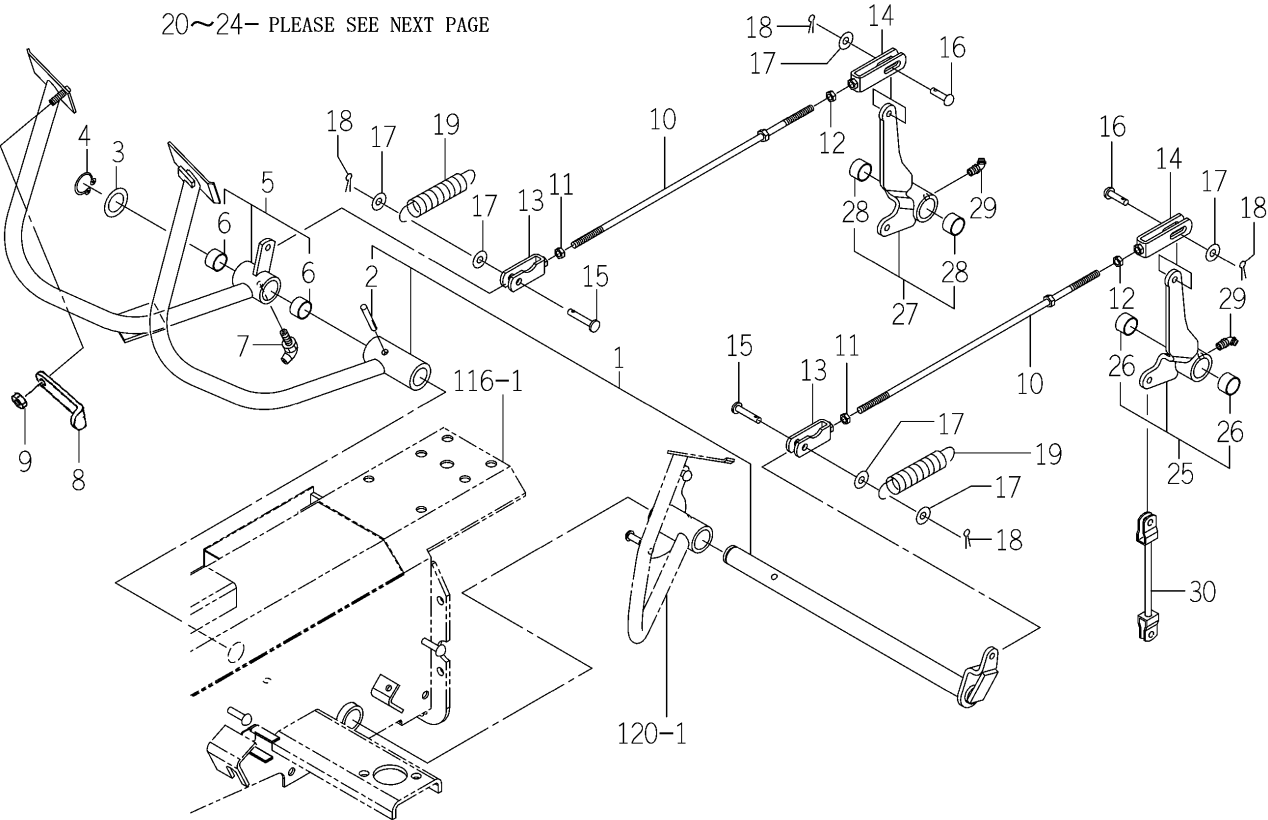
FIG.310 PEDAL (BRAKE) SYSTEM(1/2) (EXCEPT H TYPE)
