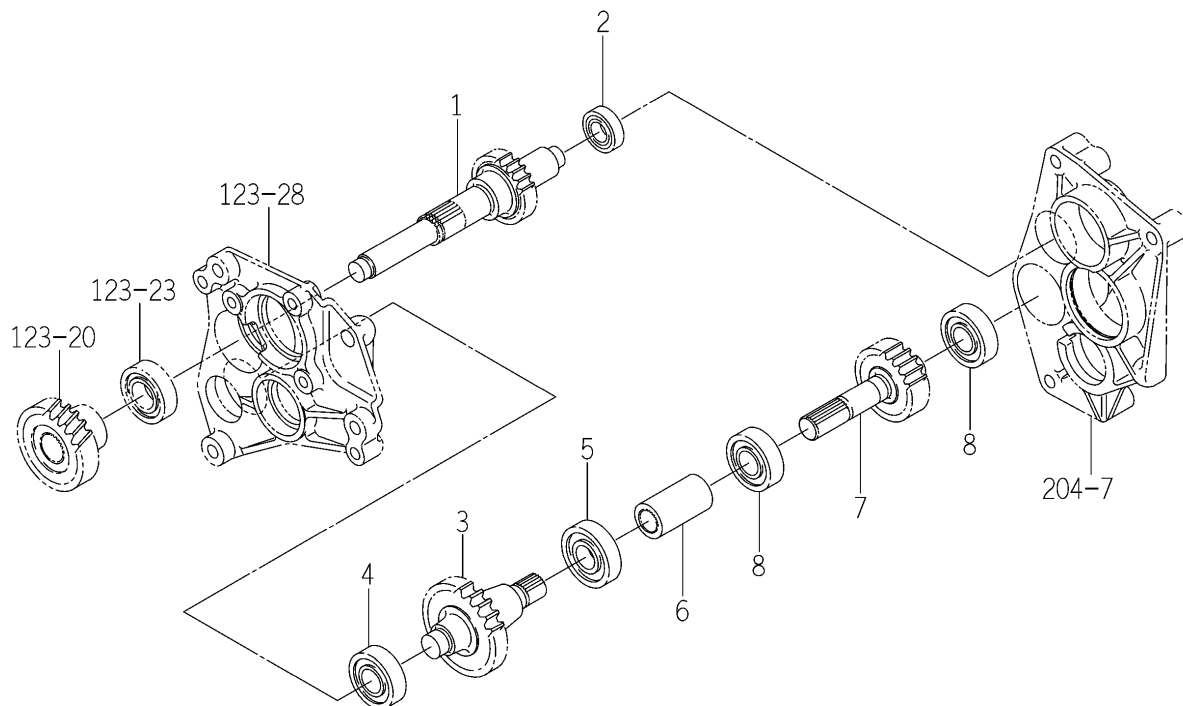
FIG.124 PTO DRIVE GEAR SYSTEM (EXCEPT H TYPE)
