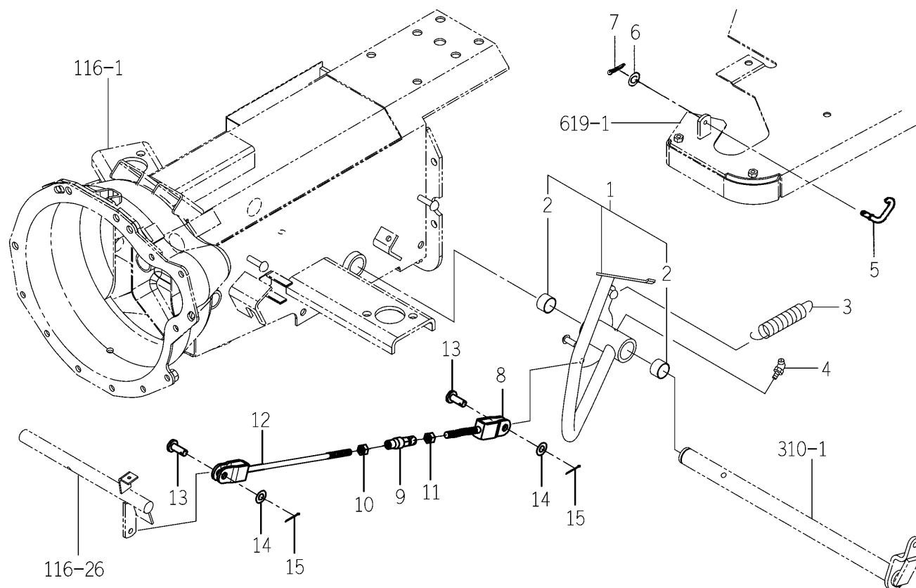
FIG.120 PEDAL (CLUTCH) SYSTEM (EXCEPT H TYPE)
