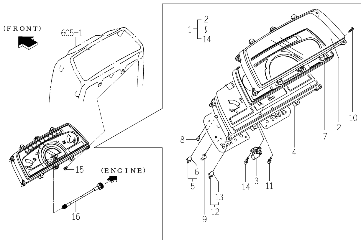
FIG.627 METER PANEL SYSTEM
