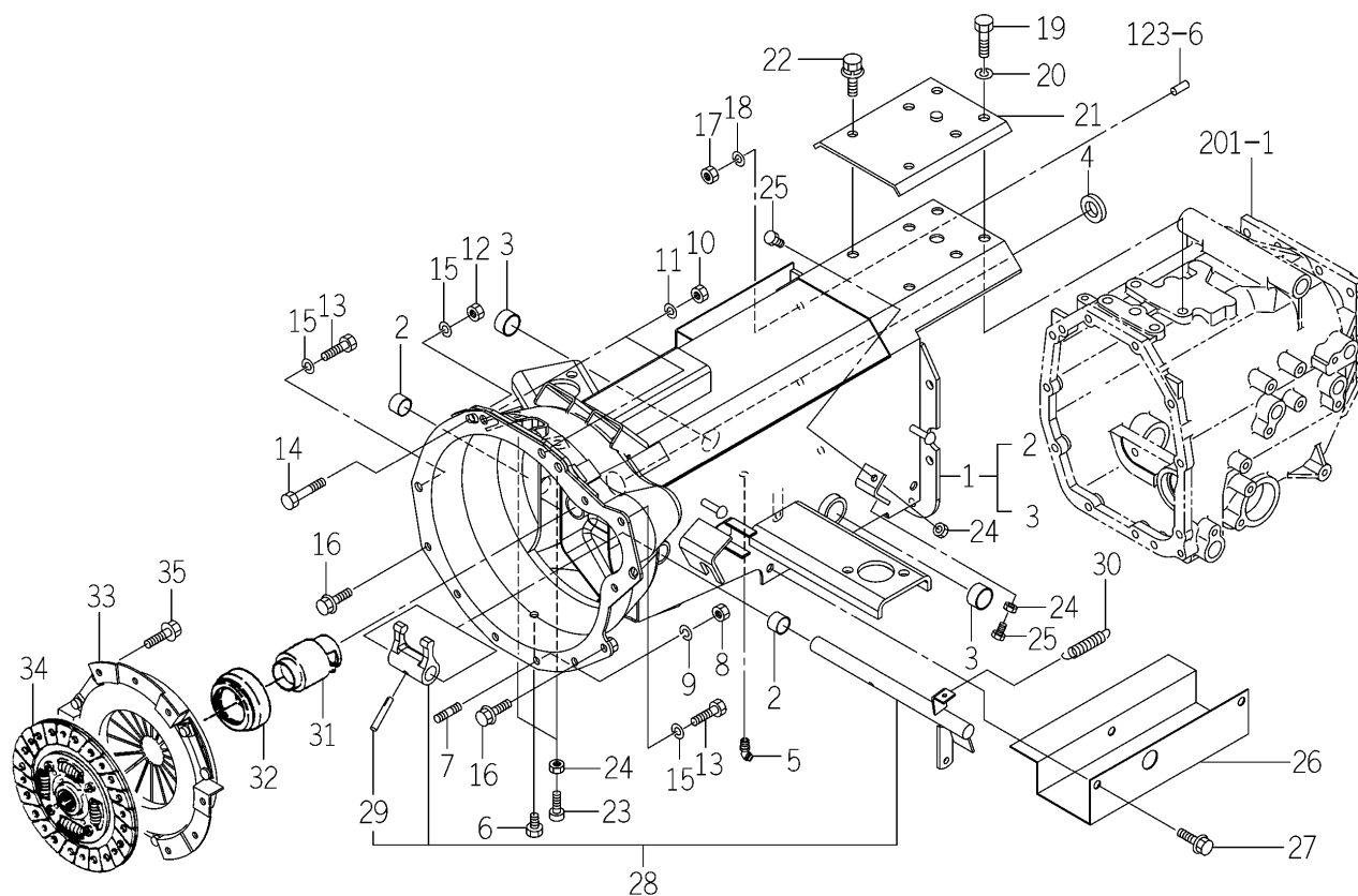
FIG.118 CLUTCH HOUSING SYSTEM (TM3265-EXCEPT H TYPE)
