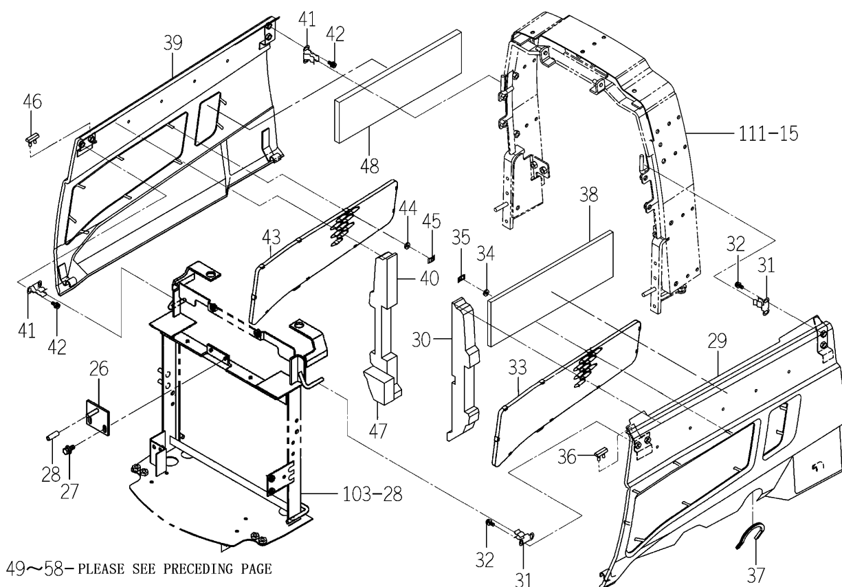
FIG.602 HOOD SYSTEM (TM3265)(2/2)
