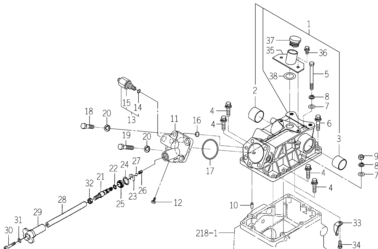
FIG.501 CYLINDER CASE SYSTEM
