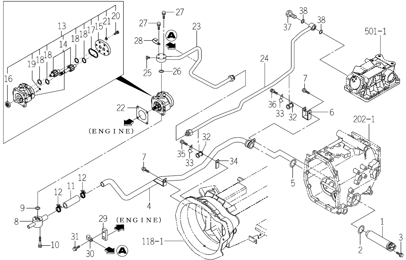
FIG.511 PIPING (MAIN) SYSTEM (TM3215,3245-H TYPE)
