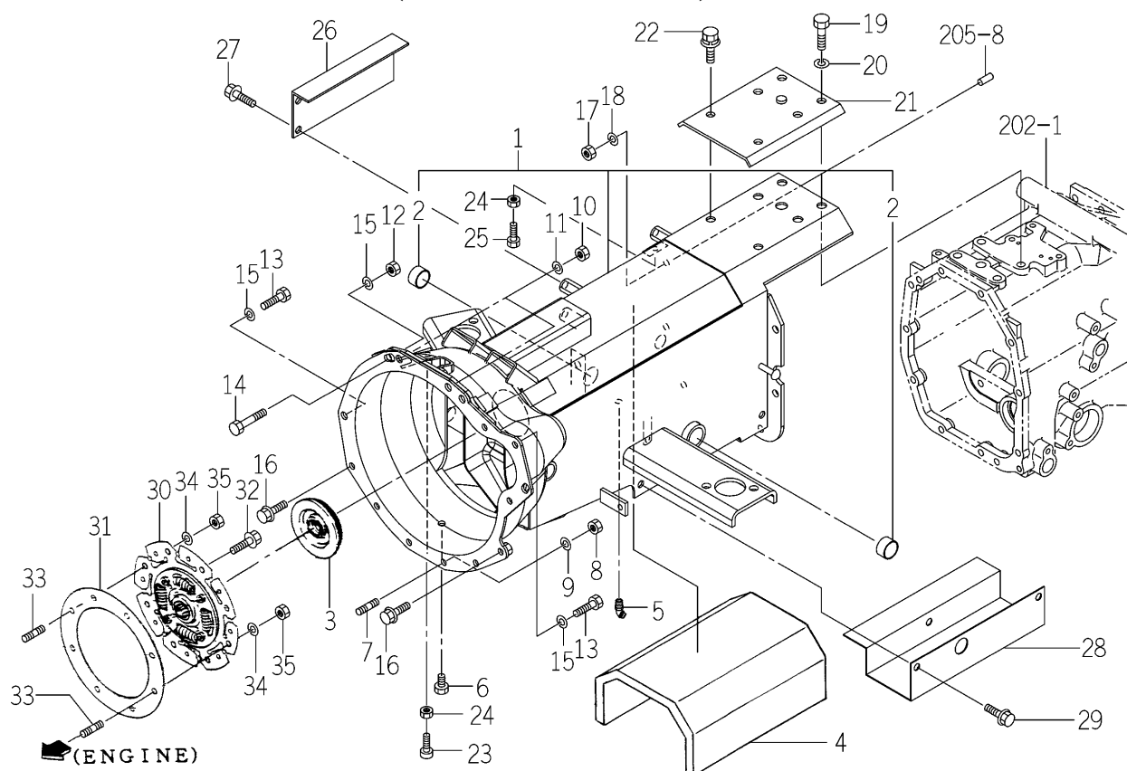
FIG.119 CLUTCH HOUSING SYSTEM (TM3265-H TYPE)
