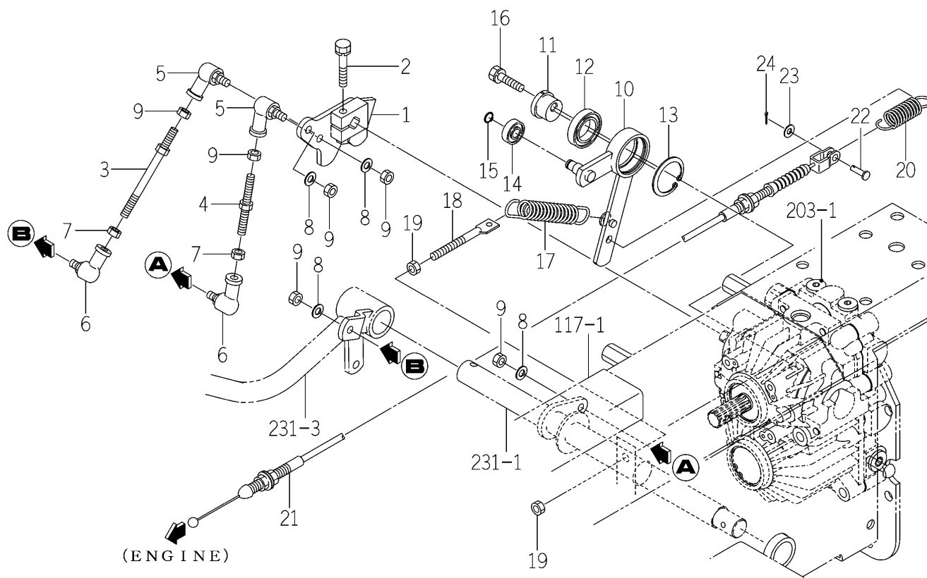
FIG.230 LINK (HST) SYSTEM (H TYPE)
