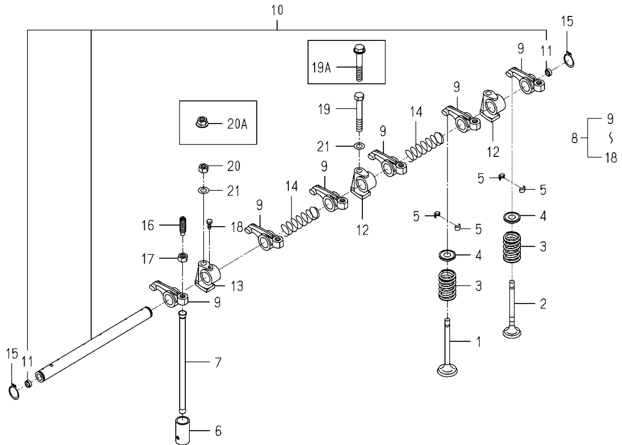
FIG.301 VALVE
