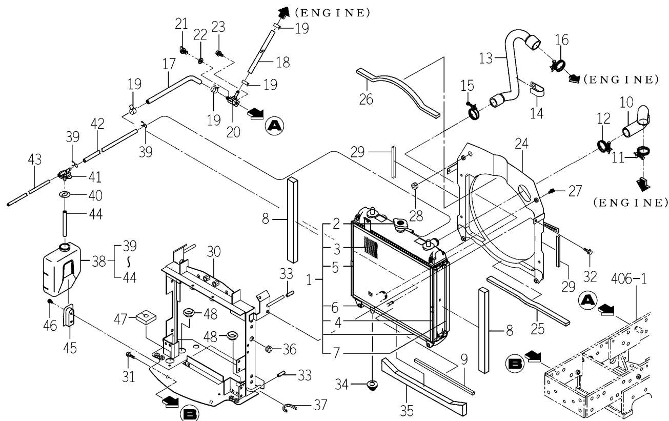
FIG.101 RADIATOR SYSTEM (TM3215,3245-EXCEPT H TYPE)
