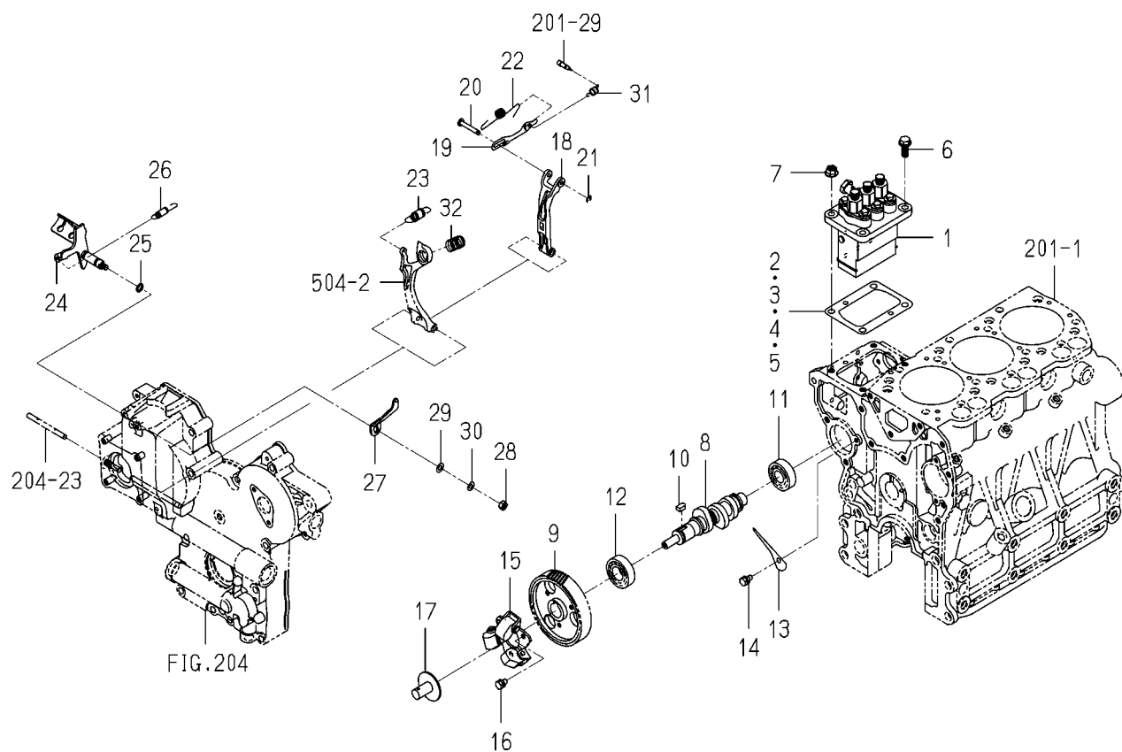
FIG.502 INJECTION PUMP
