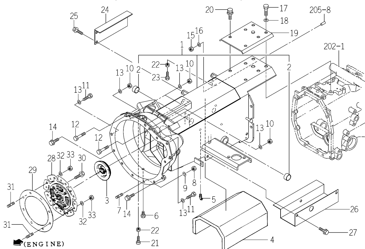
FIG.117 CLUTCH HOUSING SYSTEM (TM3215,3245-H TYPE)
