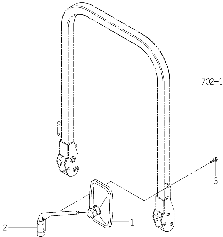
FIG.611 MIRROR SYSTEM (A TYPE)
