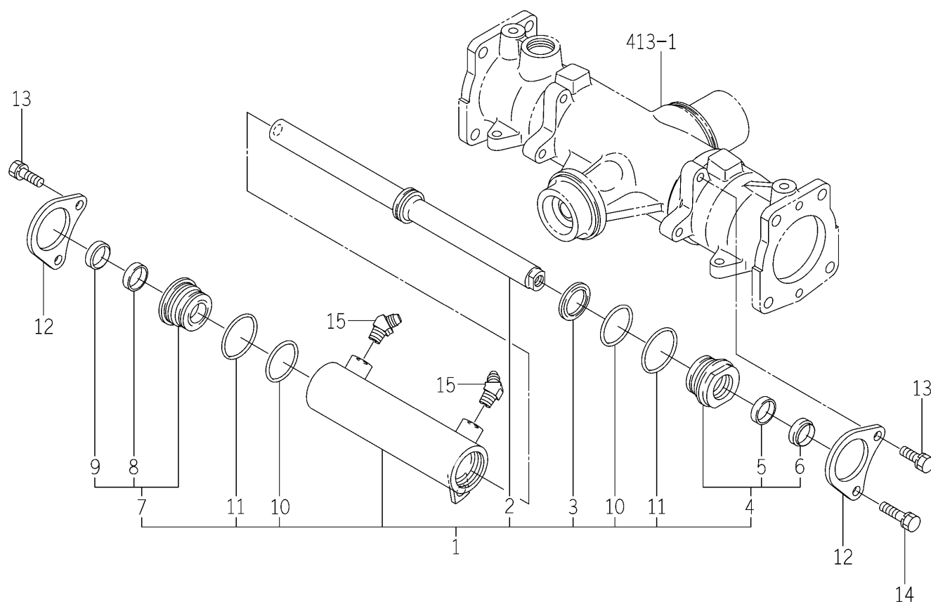
FIG.402 CYLINDER SYSTEM
