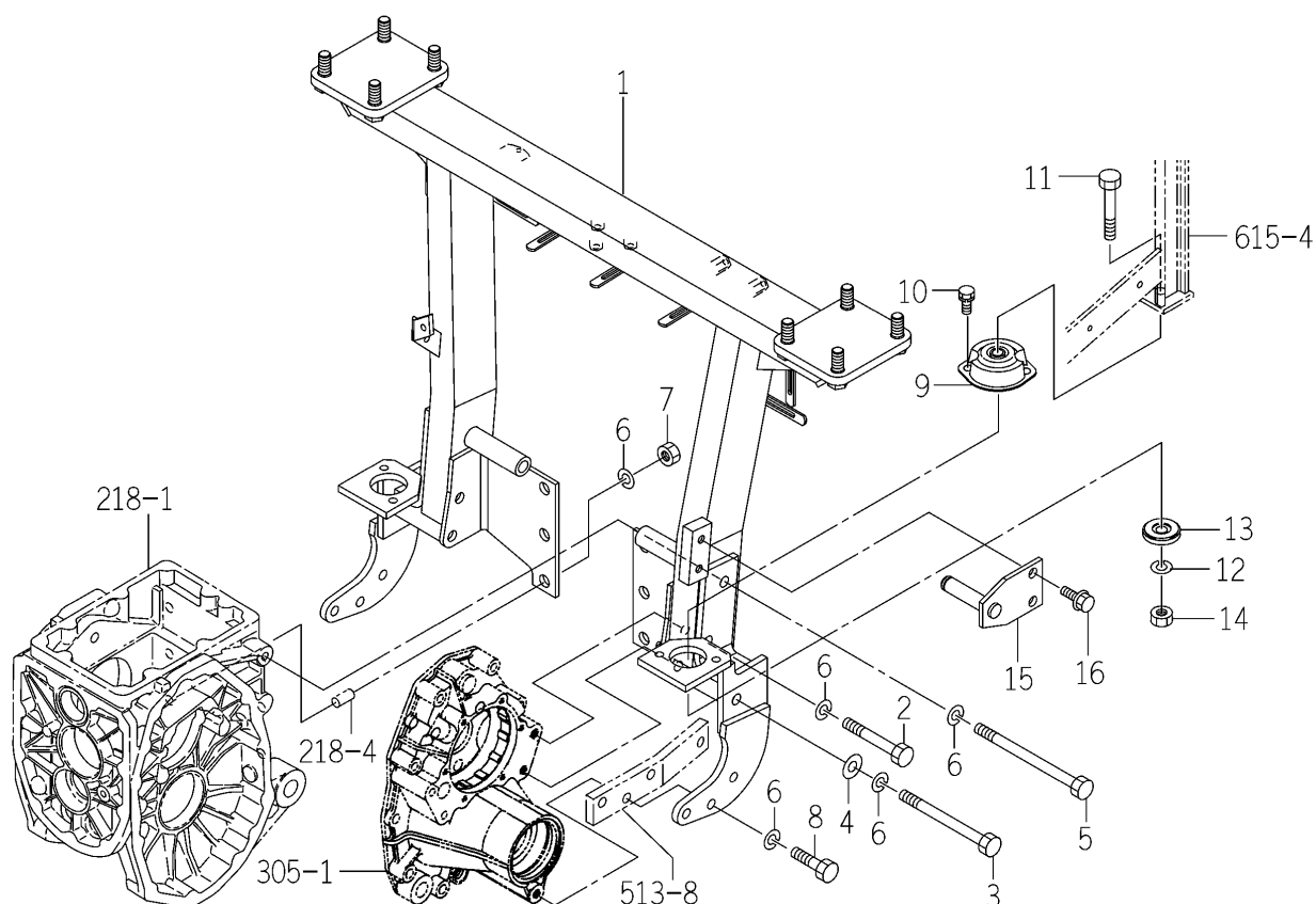
FIG.614 REAR MOUNT SYSTEM (D TYPE)
