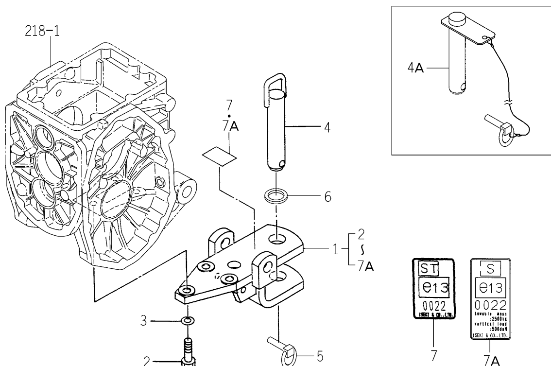
FIG.P11 HITCH (DRAW BAR) SET (OPTION)
