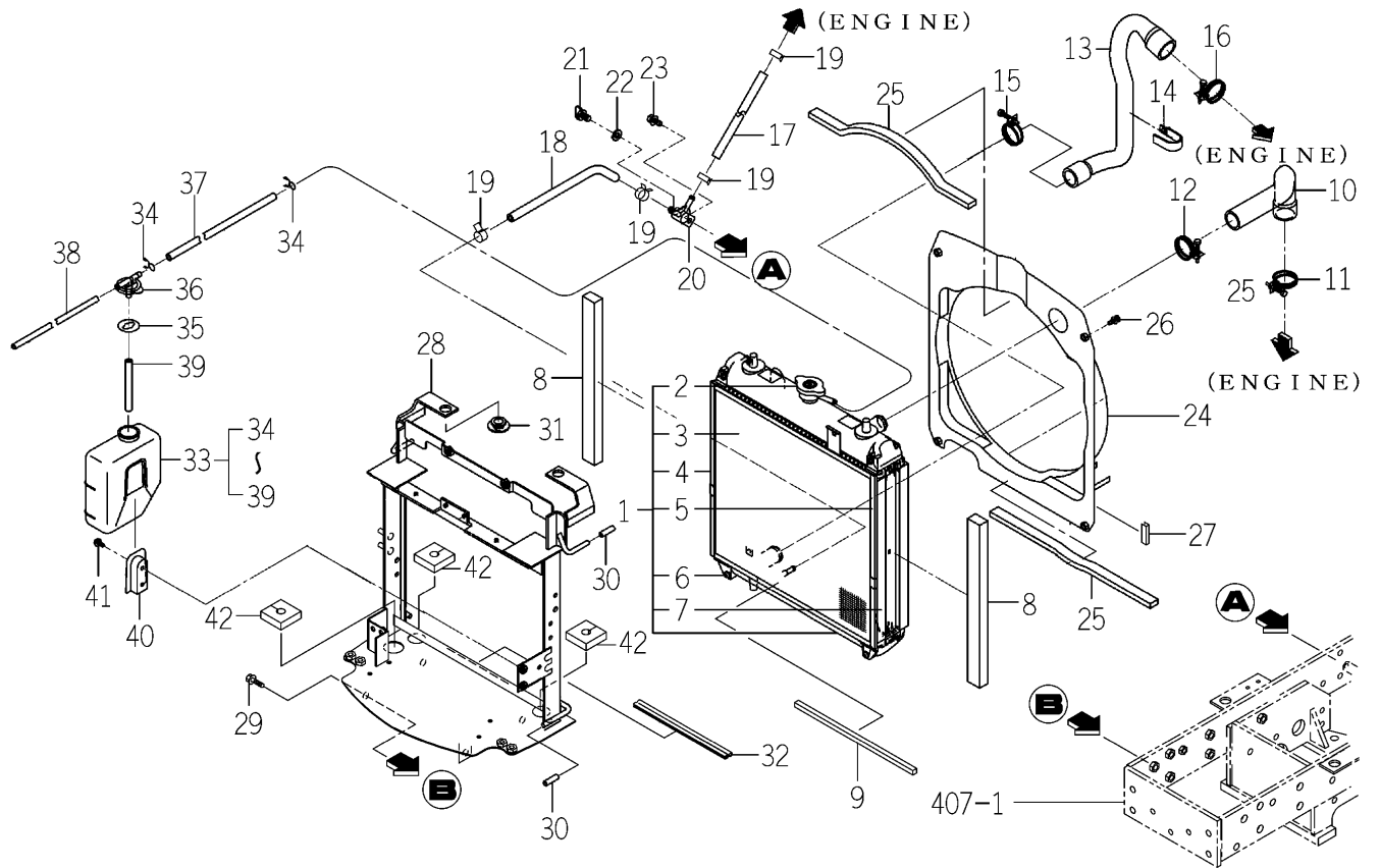
FIG.104 RADIATOR SYSTEM (TM3265-H TYPE)
