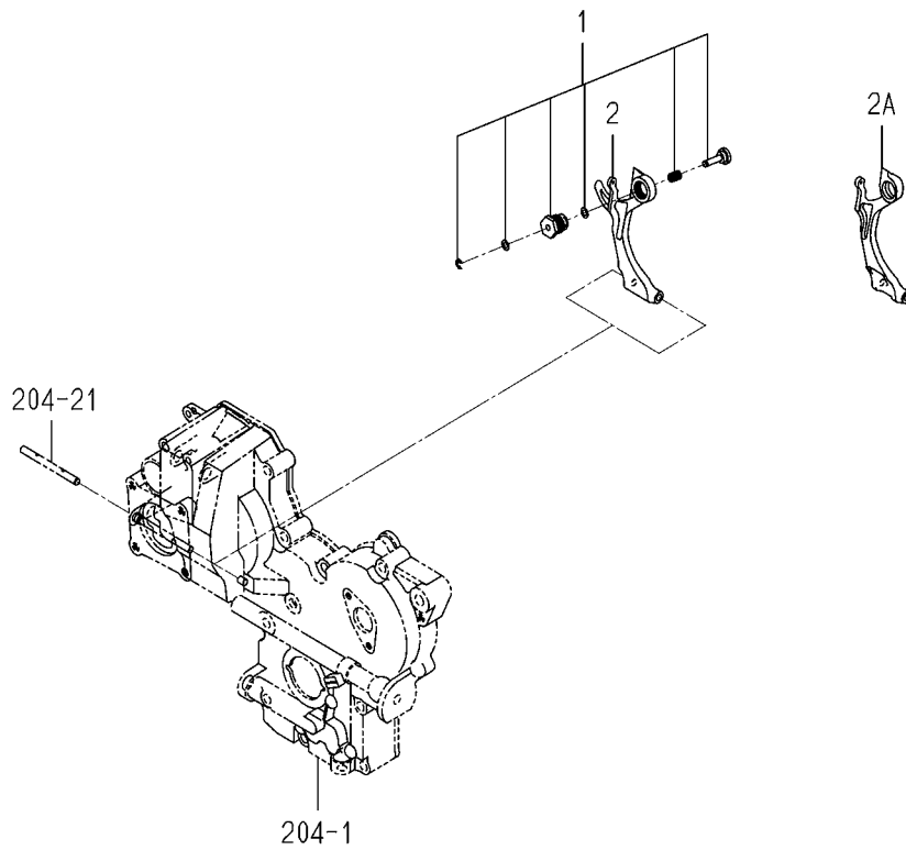
FIG.504 ADAPTER
