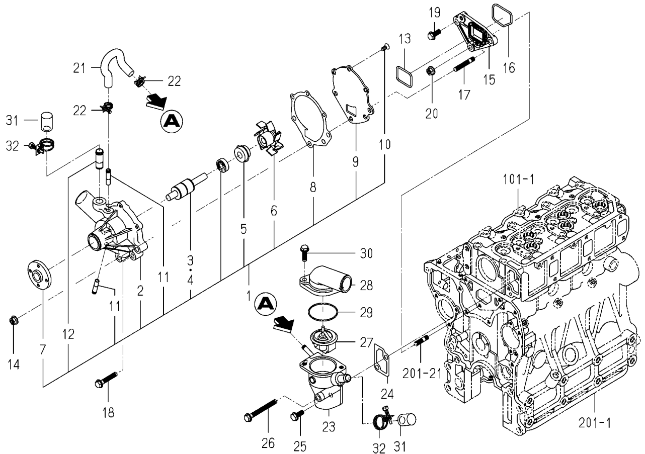
FIG.402 WATER PUMP
