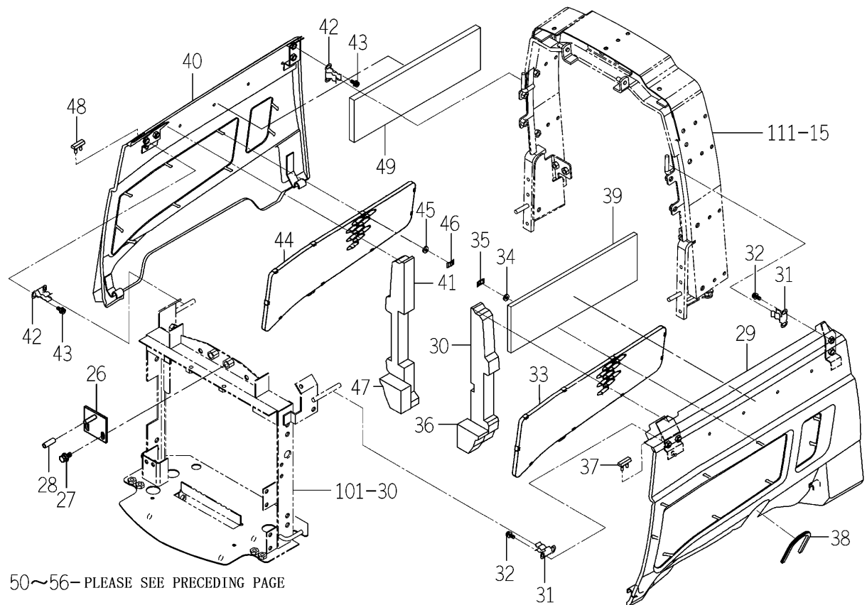
FIG.601 HOOD SYSTEM (TM3215,3245)(2/2)
