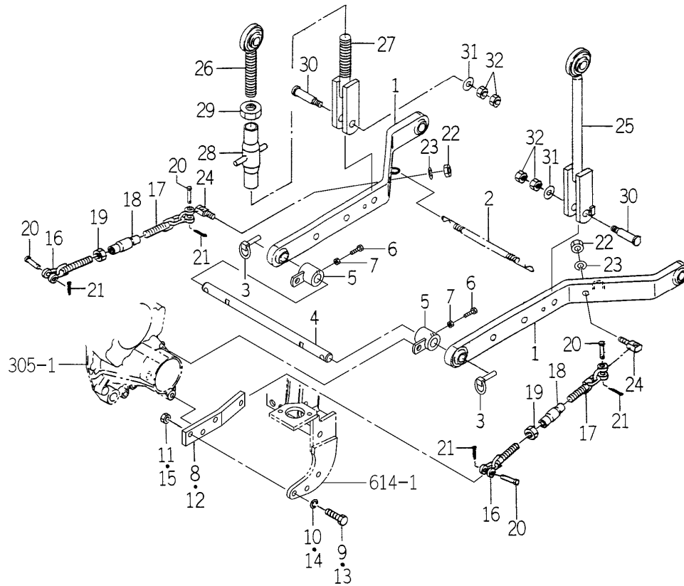
FIG.513 LINK (3P) SYSTEM (D TYPE)
