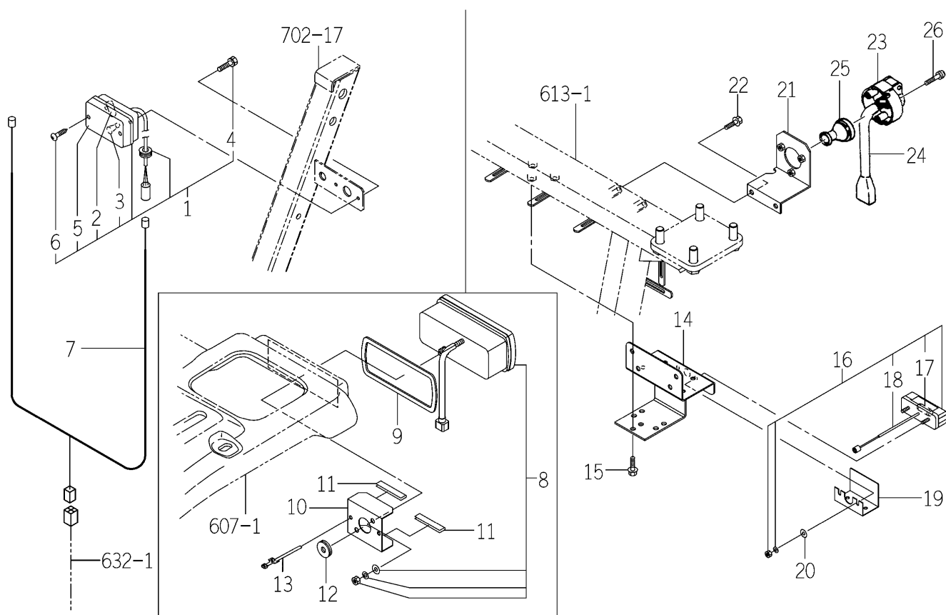
FIG.625 LAMP SYSTEM (A TYPE)
