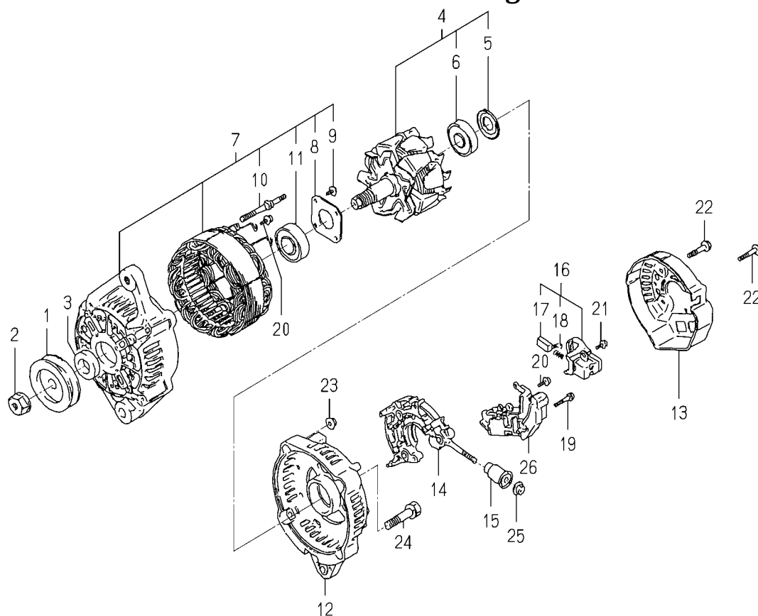
FIG.S04 COMPONENT PARTS FOR 6281-200-021-00 ON Fig.801
