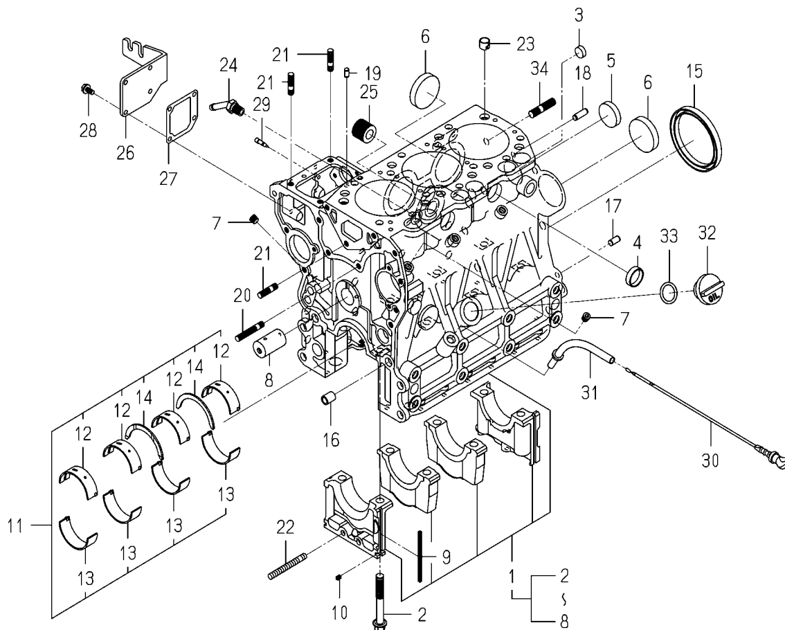
FIG.201 CYLINDER BLOCK
