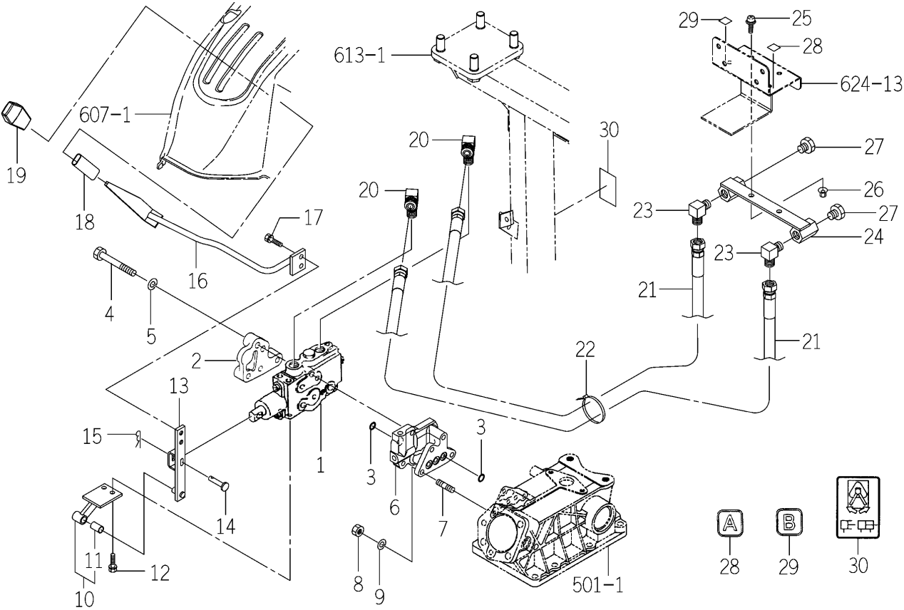
FIG.506 VALVE (REMOTE/1R) SYSTEM (VR TYPE)
