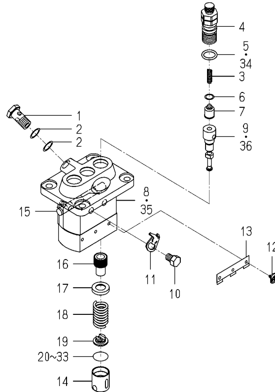
FIG.S02 COMPONENT PARTS FOR 6215-600-103-10 ON Fig.502
