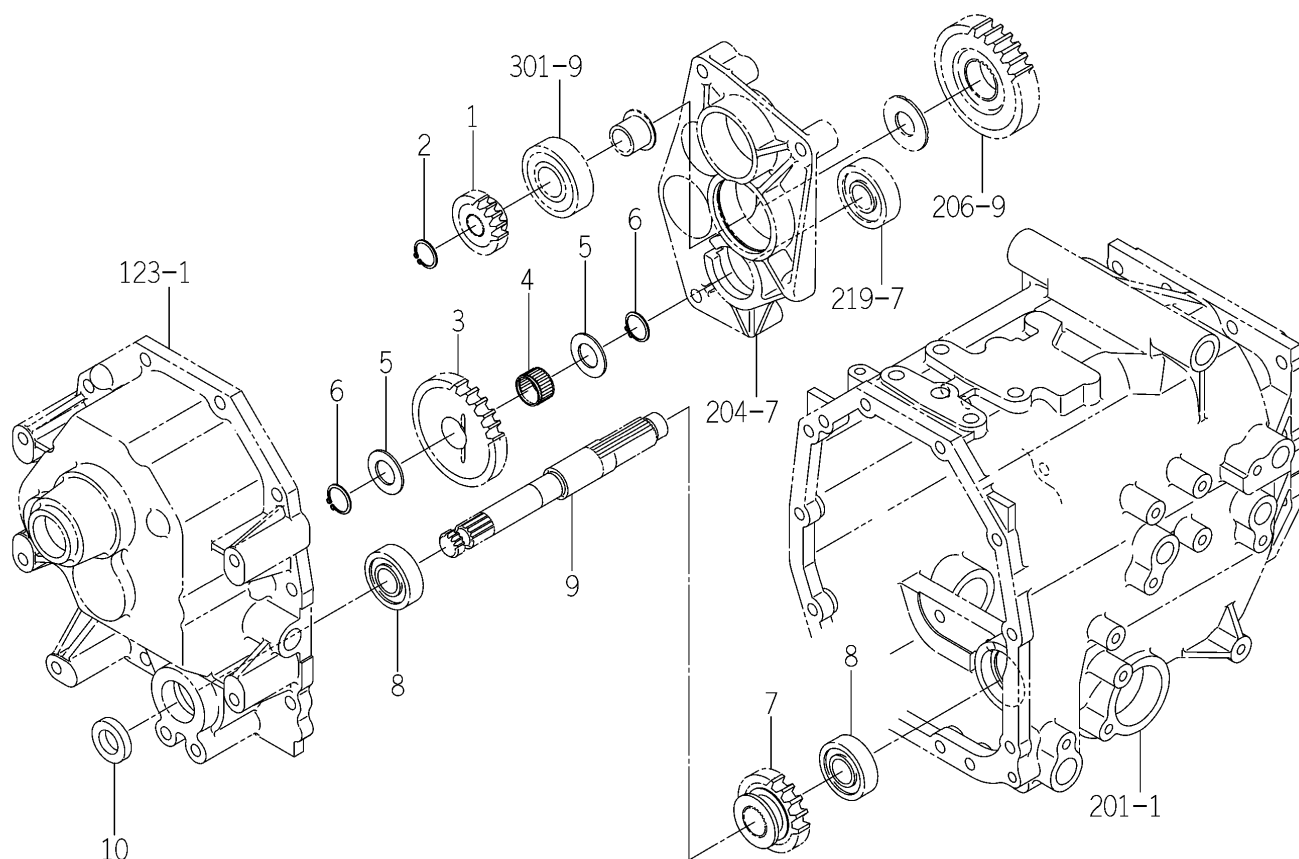
FIG.216 4WD GEAR SYSTEM
