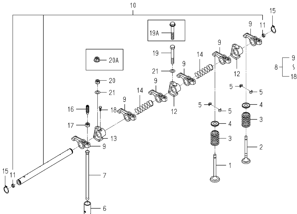
FIG.301 VALVE
