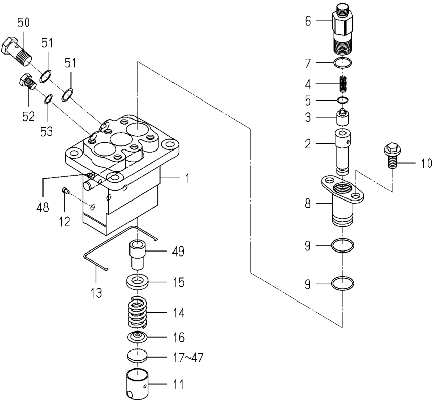
FIG.S02 COMPONENT PARTS FOR 6215-600-155-00 ON Fig.502
