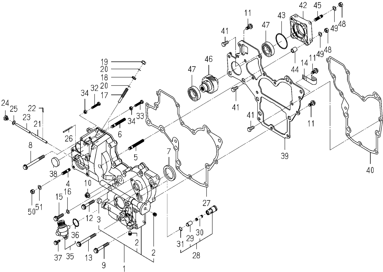
FIG.204 TIMING GEAR CASE
