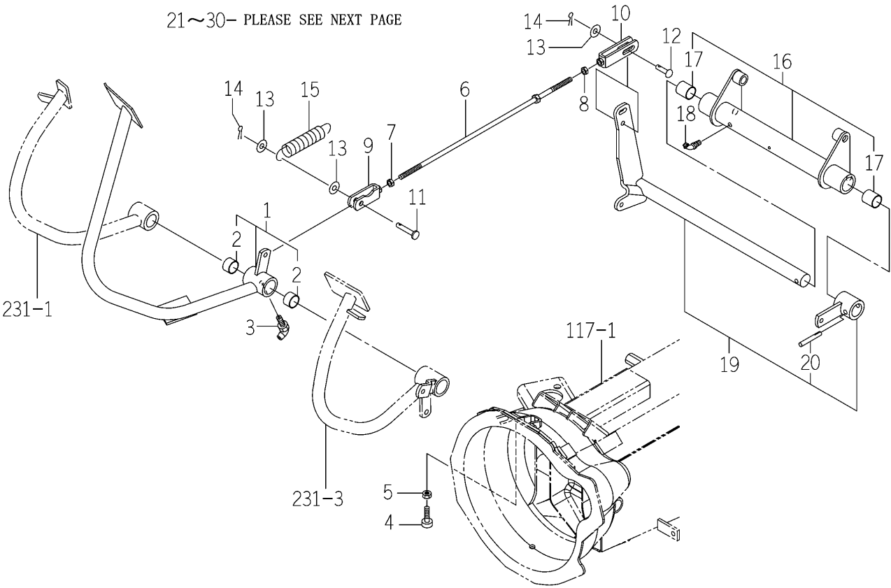
FIG.311 PEDAL (BRAKE) SYSTEM (H TYPE)(1/2)
