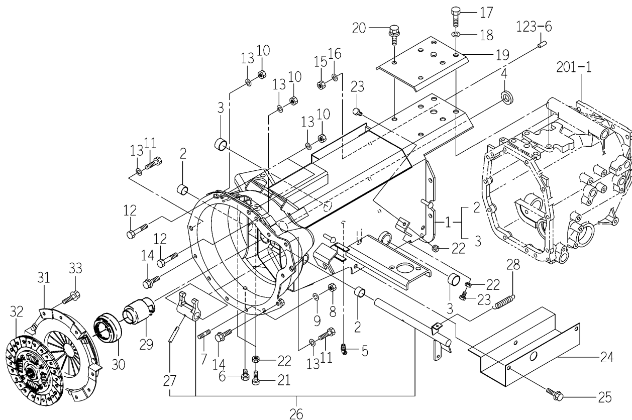
FIG.116 CLUTCH HOUSING SYSTEM (TM3215,3245-EXCEPT H TYPE)
