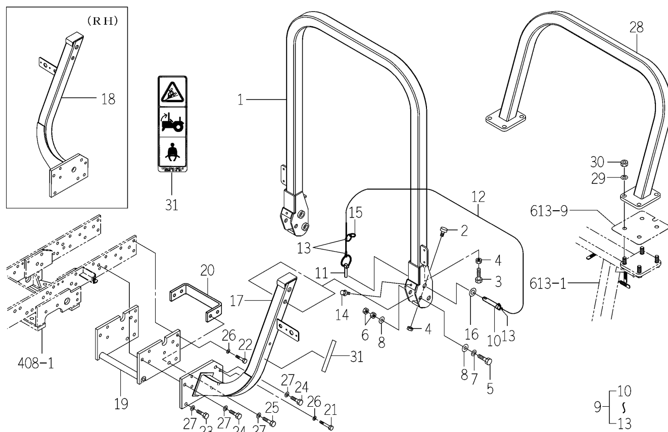
FIG.702 ROPS SYSTEM (TM3215,3245-A TYPE)
