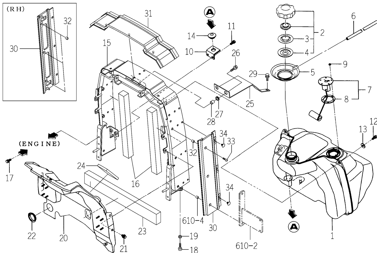
FIG.111 FUEL TANK SYSTEM
