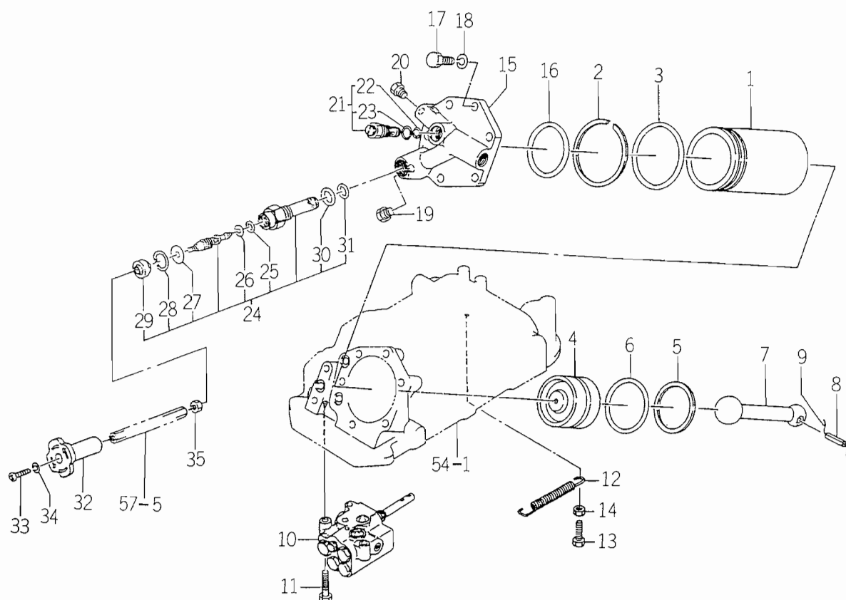
FIG. 56 CYLINDER SYSTEM
