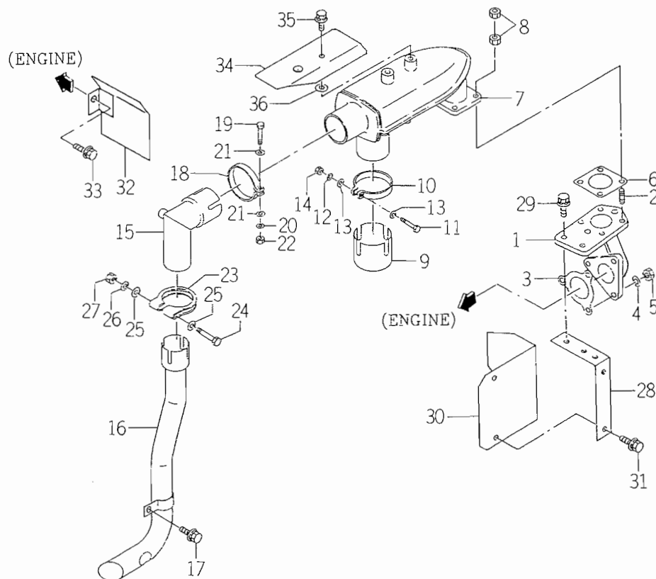
FIG. 4 MUFFLER SYSTEM (EXCEPT C TYPE)
