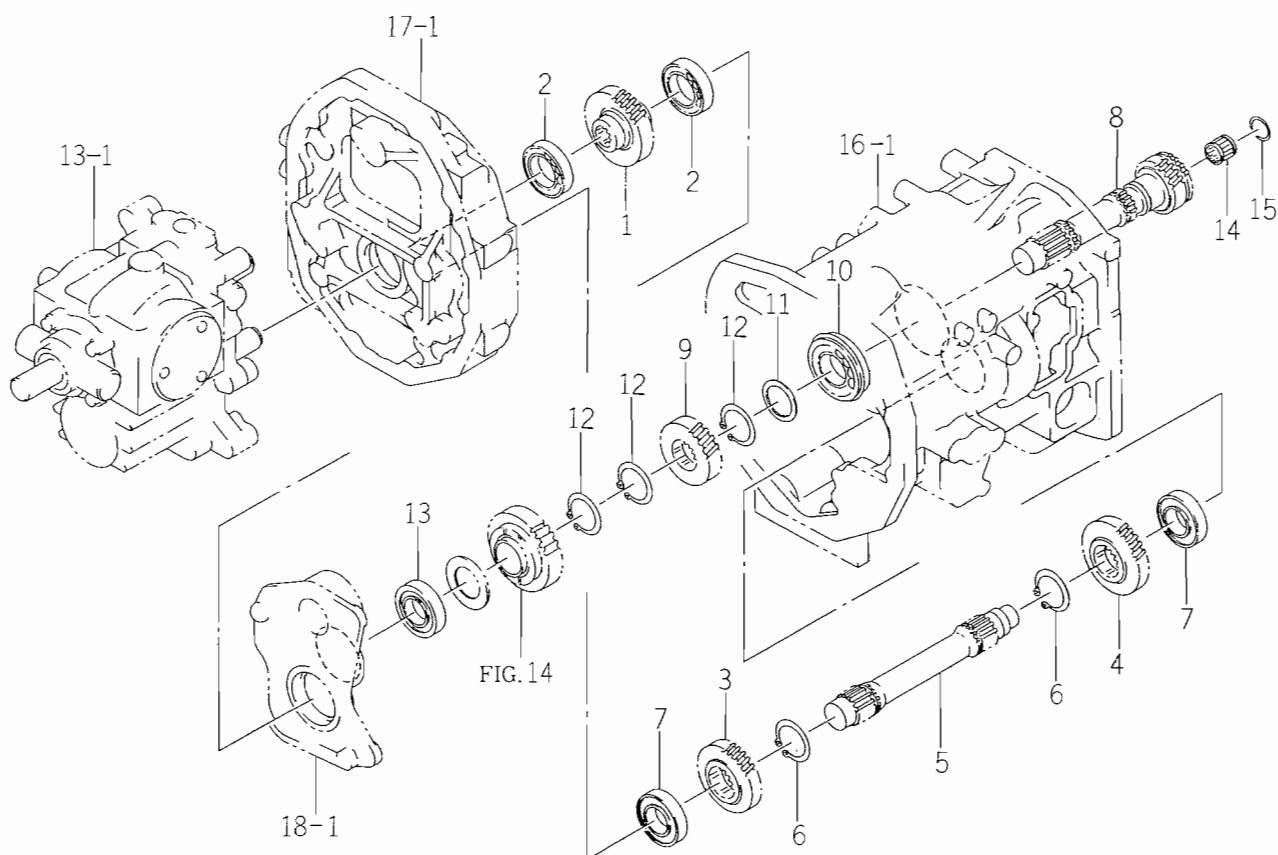
FIG. 12 MAIN GEAR SYSTEM
