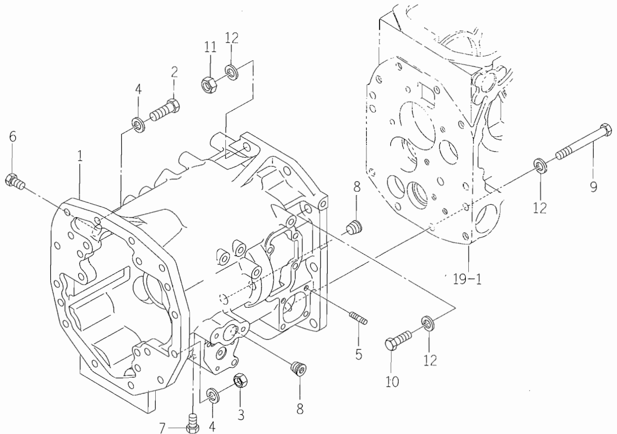
FIG. 16 CASE (MIDDLE) SYSTEM
