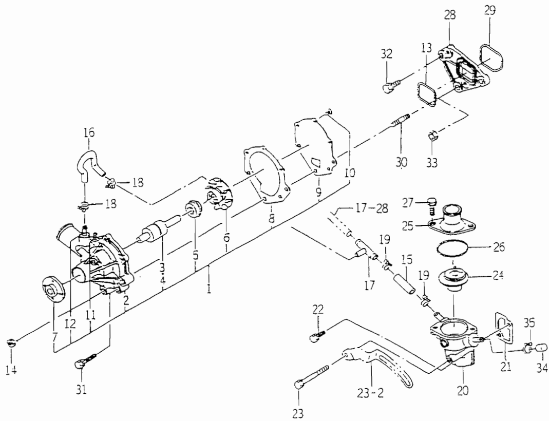
FIG. 18 WATER PUMP
