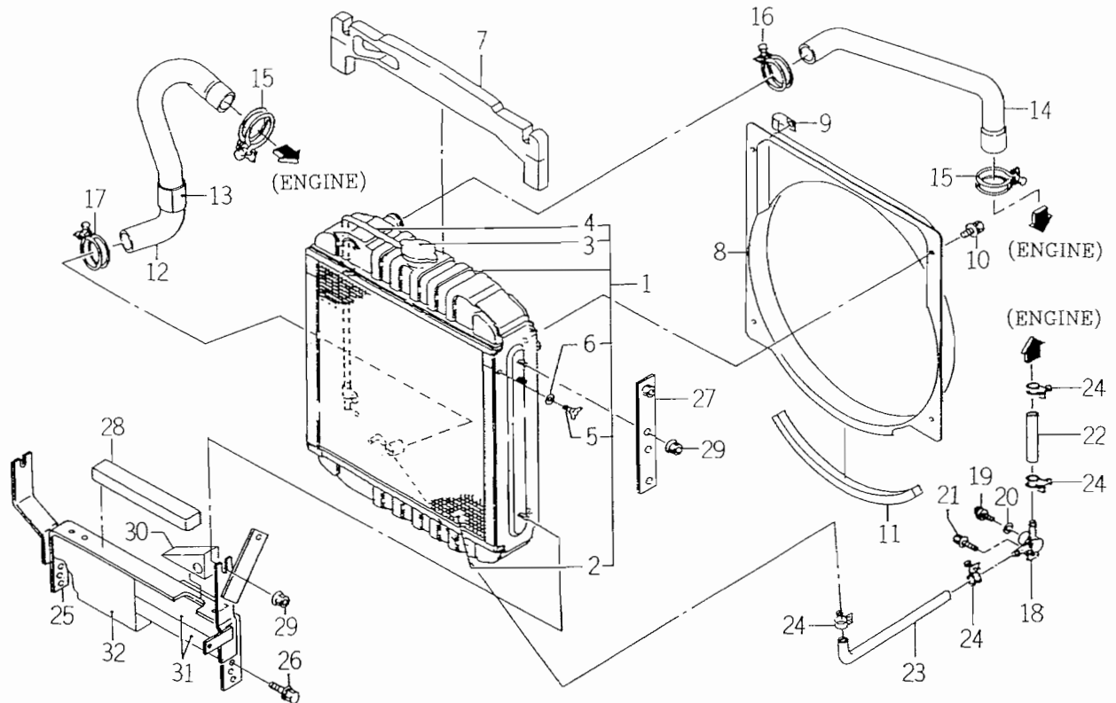
FIG. 3 RADIATOR SYSTEM
