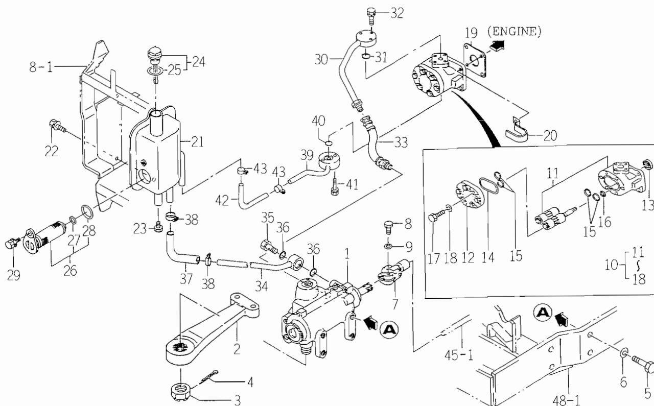
FIG. 47 POWER STEERING SYSTEM
