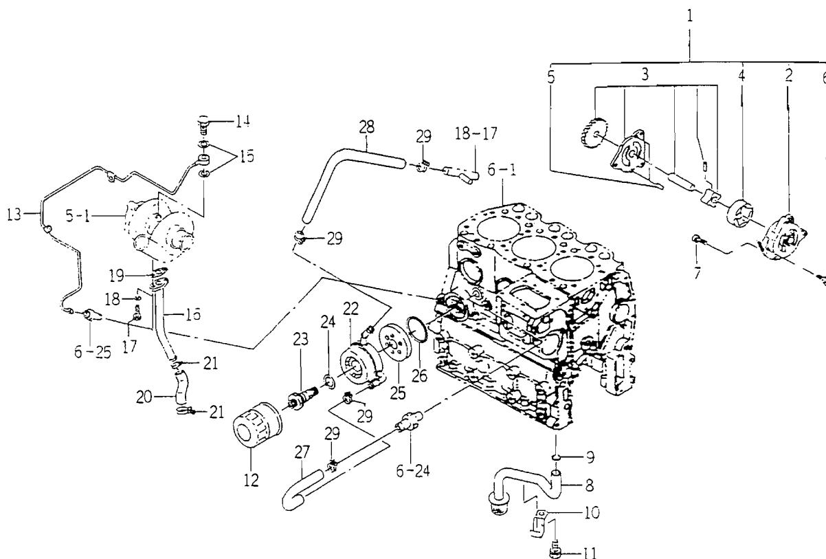
FIG. 17 OIL PUMP
