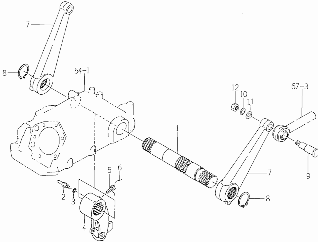
FIG. 55 LIFT ARM SYSTEM
