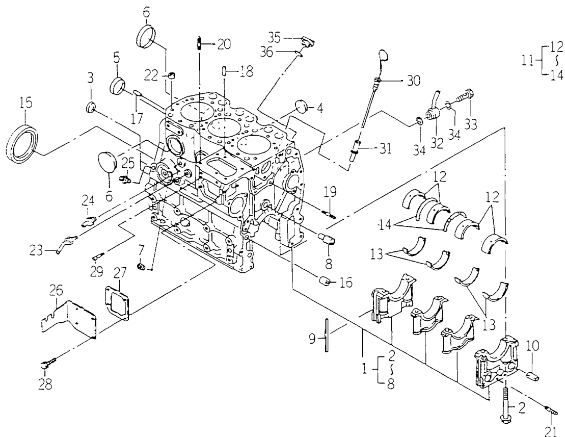
FIG. 6 CYLINDER BLOCK
