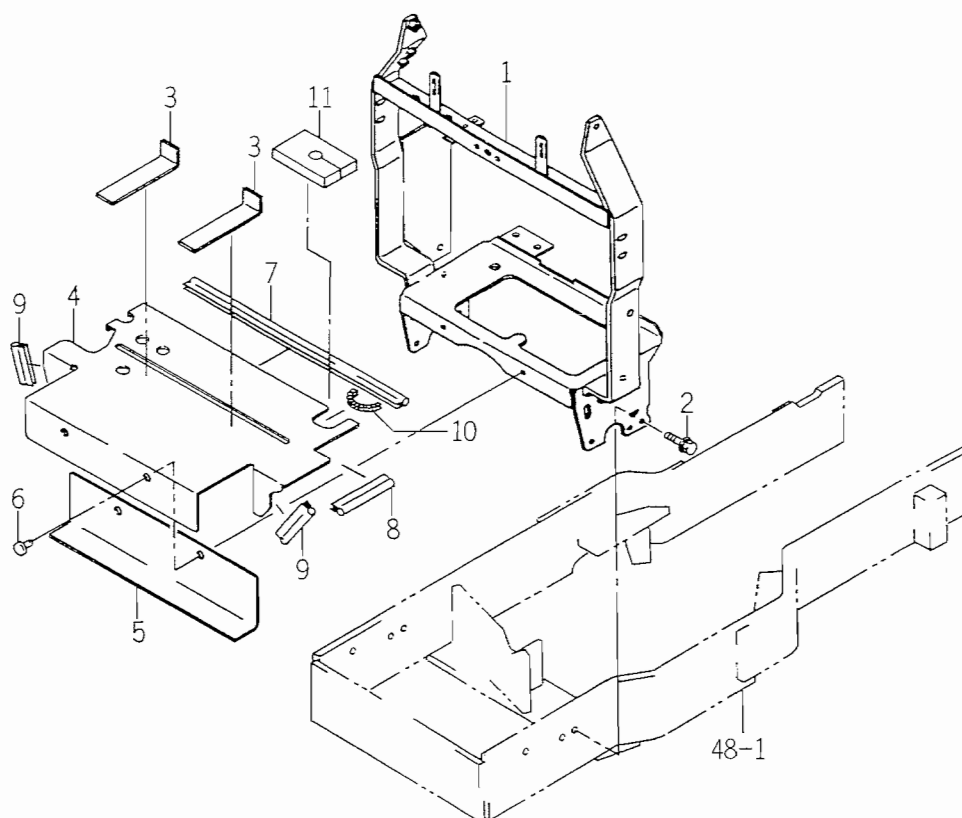
FIG. 8 BATTERY BASE SYSTEM
