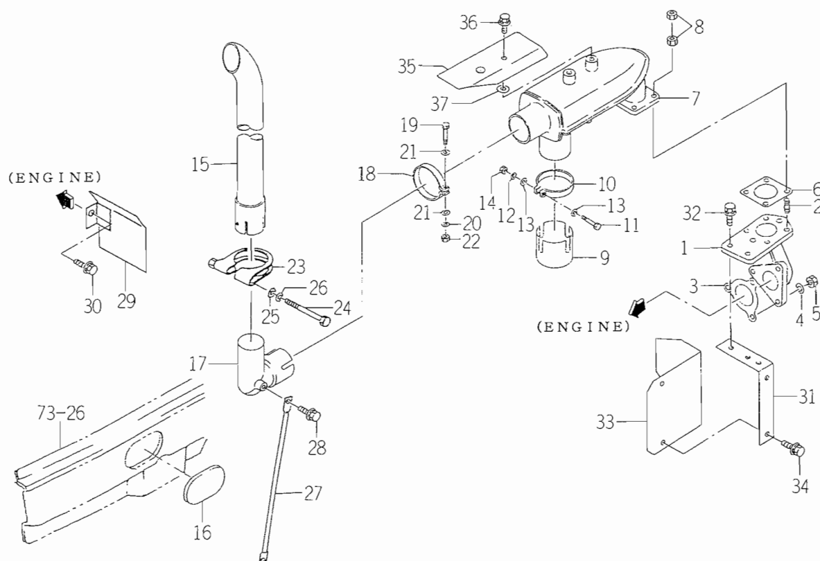
FIG. 5 MUFFLER (UPPER) SYSTEM (C TYPE)
