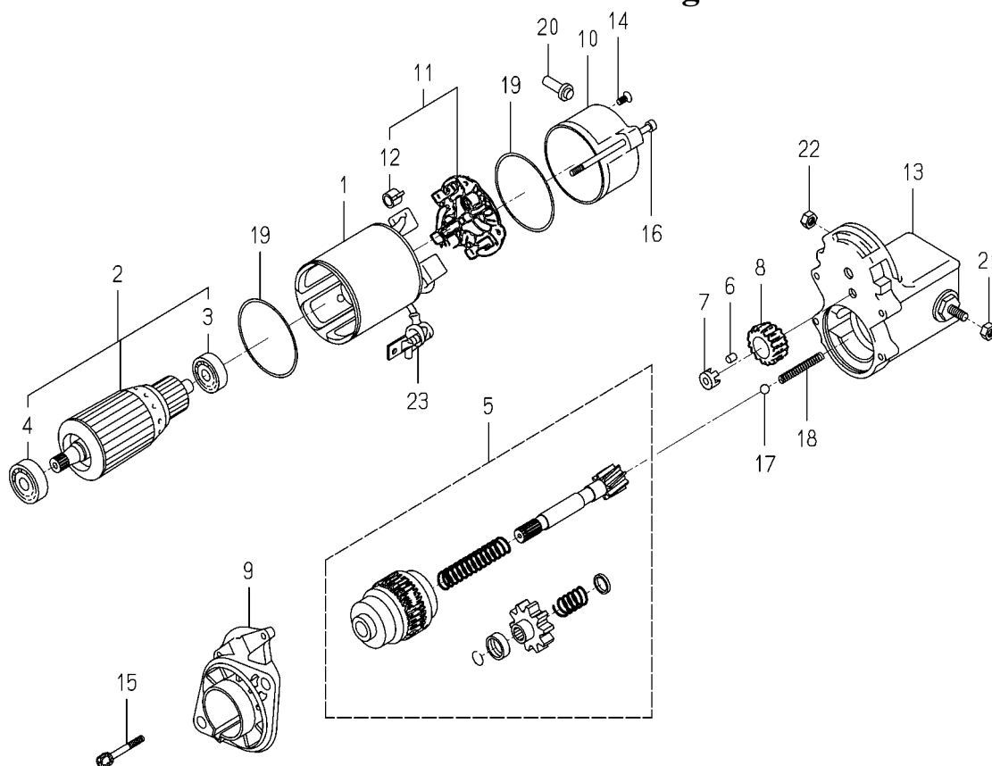
FIG. 29 COMPONENT PARTS FOR 6281-100-007-20 ON Fig.23
