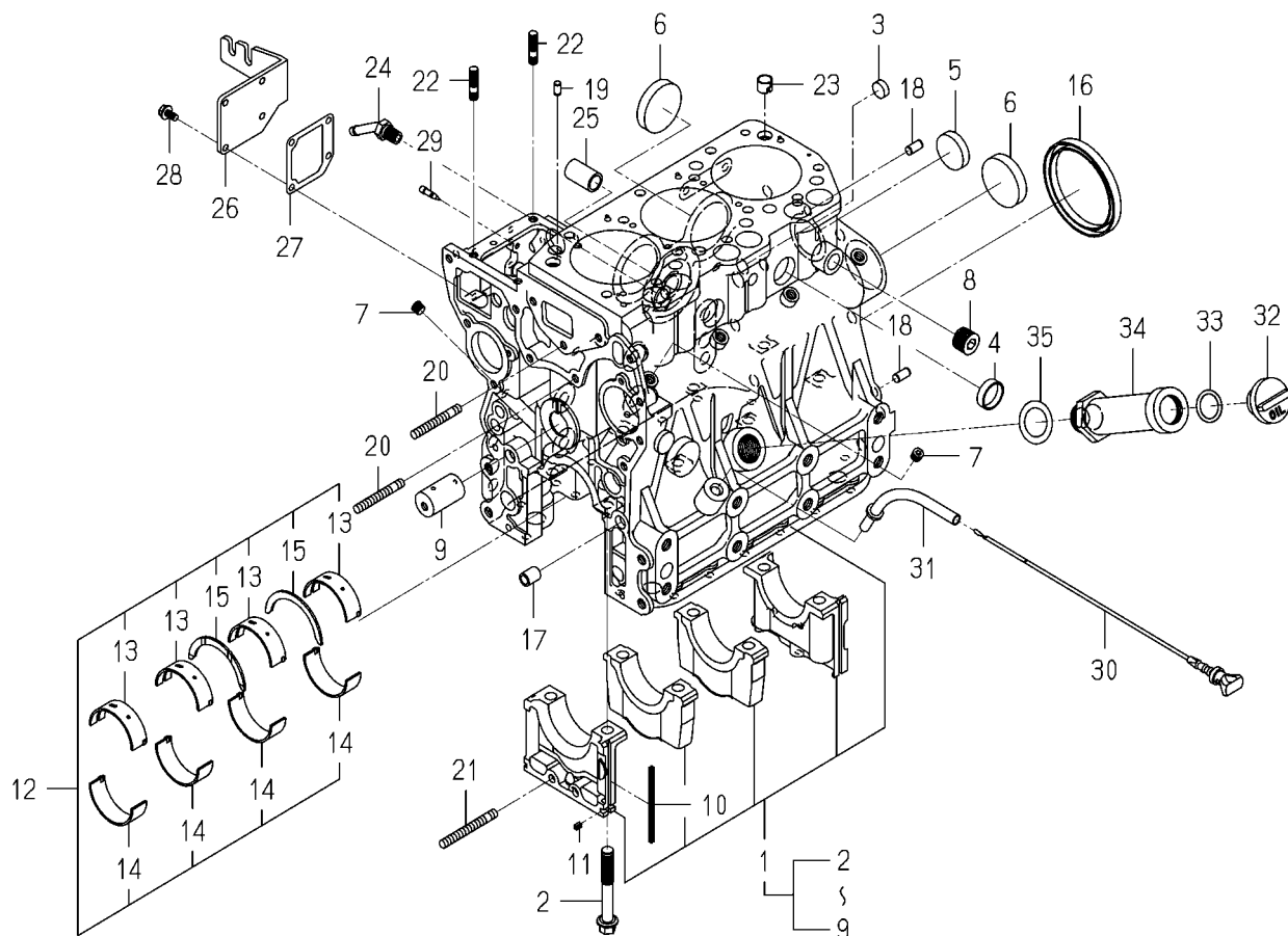
FIG. 6 CYLINDER BLOCK
