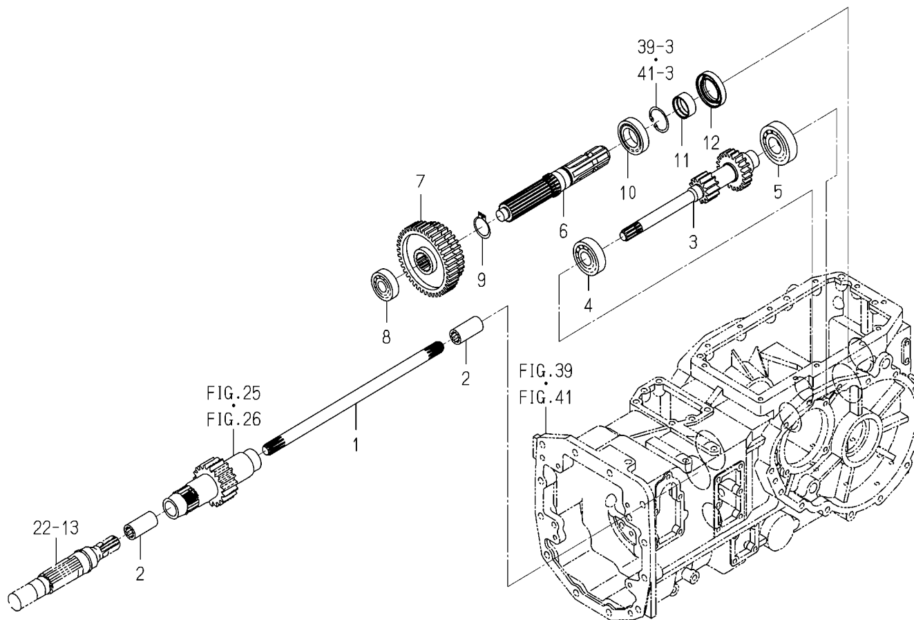
FIG. 34 GEAR(PTO)SYSTEM(EXCEPT H TYPE)
