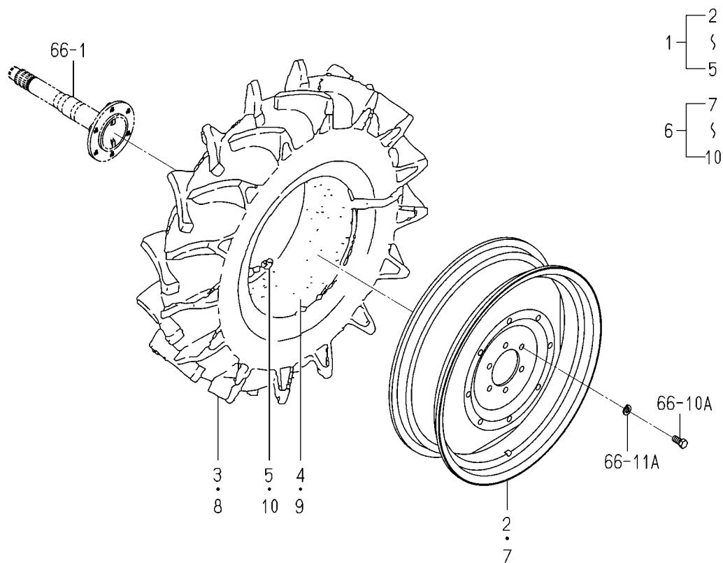
FIG.176 REAR WHEEL(9.5-24)SYSTEM(OPTION)
