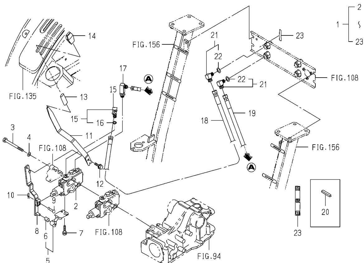
FIG.189 VALVE(REMOTE/PLUS)SET (OPTION)(V TYPE)
