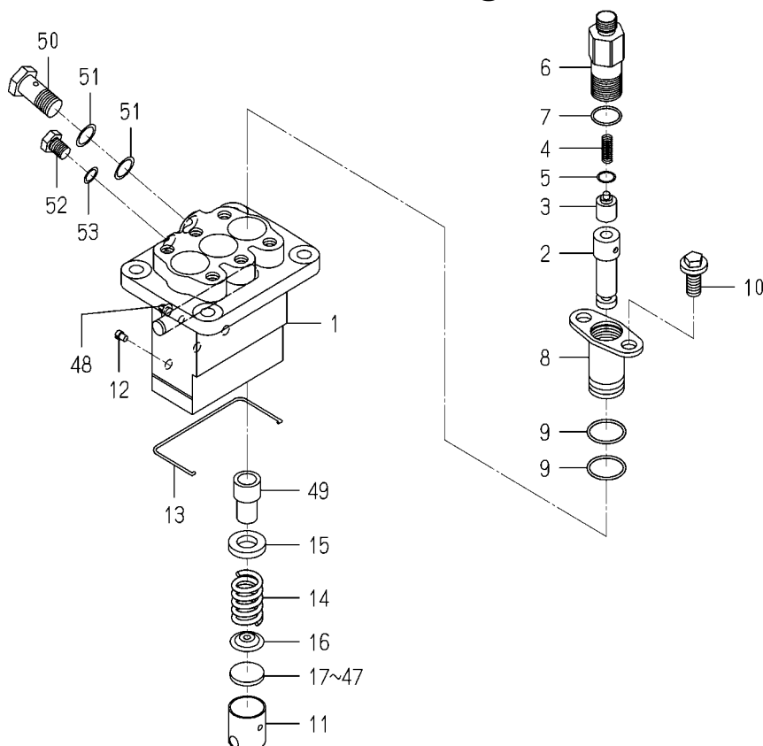
FIG. 29 COMPONENT PARTS FOR 6215-600-104-20 ON Fig.21
