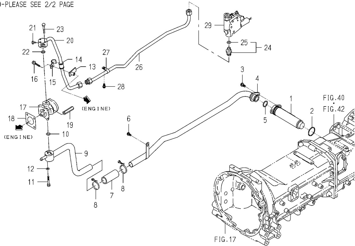
FIG.103 HYD.SYSTEM(MAIN)(1/2) (H TYPE EXCEPT TH4365)
