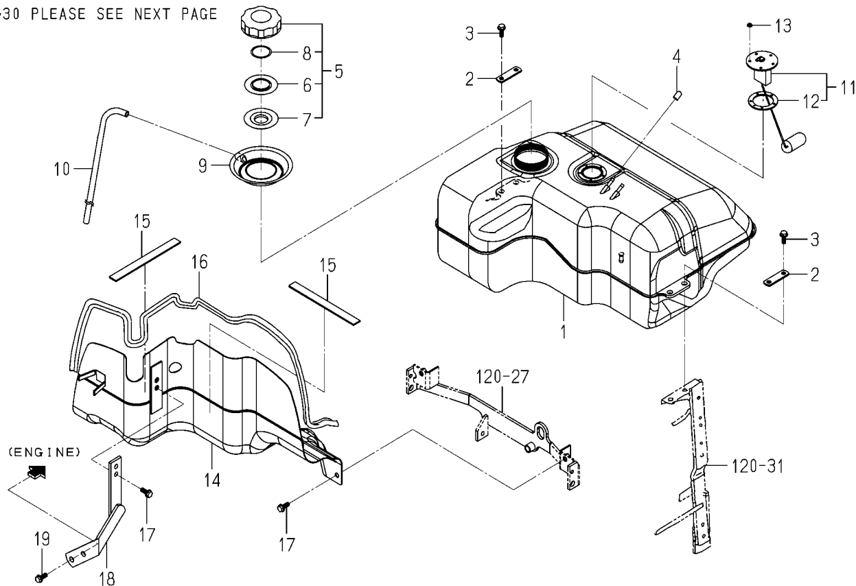
FIG. 7 FUEL SYSTEM(H TYPE ECXCEPT TH4365)(1/2)
