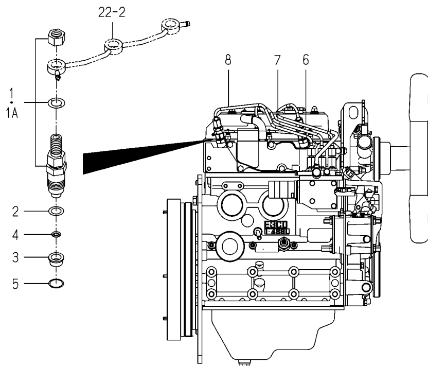
FIG. 20 INJECTION NOZZLE
