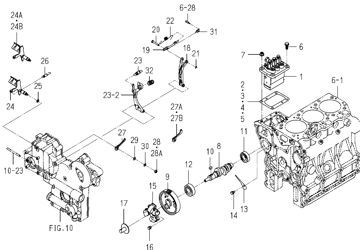
FIG. 21 INJECTION PUMP
