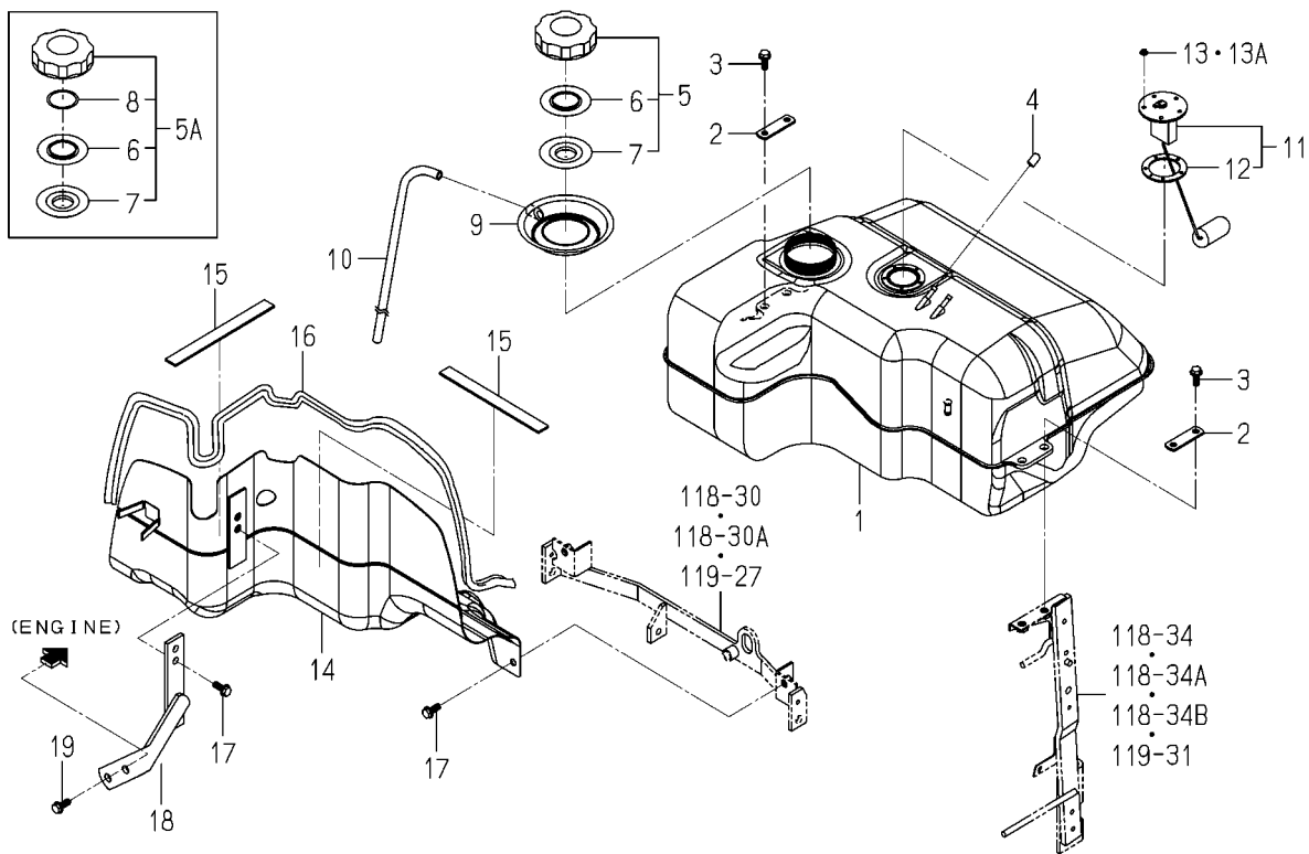
FIG. 8 FUEL SYSTEM(1/2) (TH4295,4335TYPE EXCEPT H)
