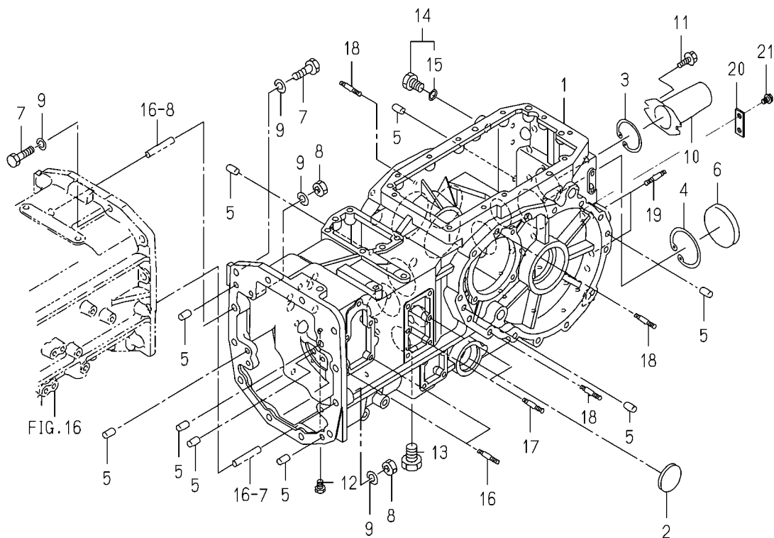
FIG. 41 CASE(TRANSMISSION/REAR)SYSTEM (SK-E4D TYPE)
