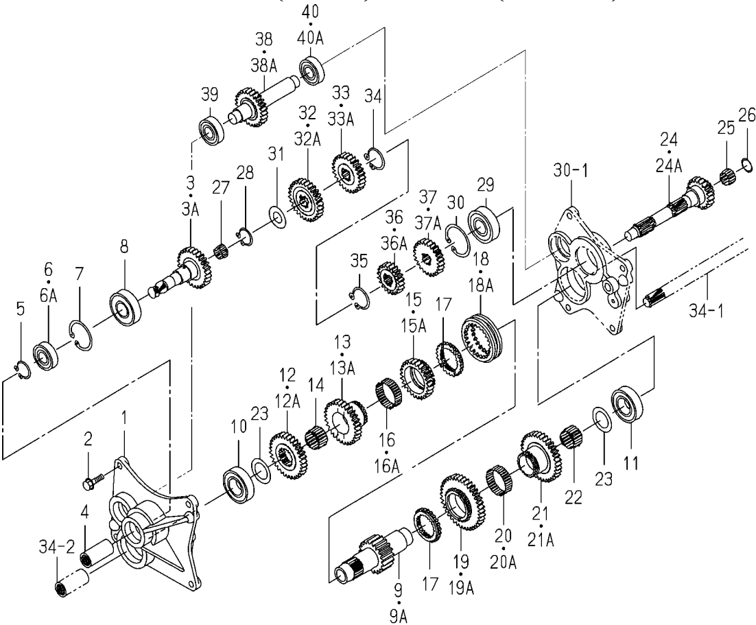
FIG. 25 GEAR(MAIN)SYSTEM(K TYPE)
