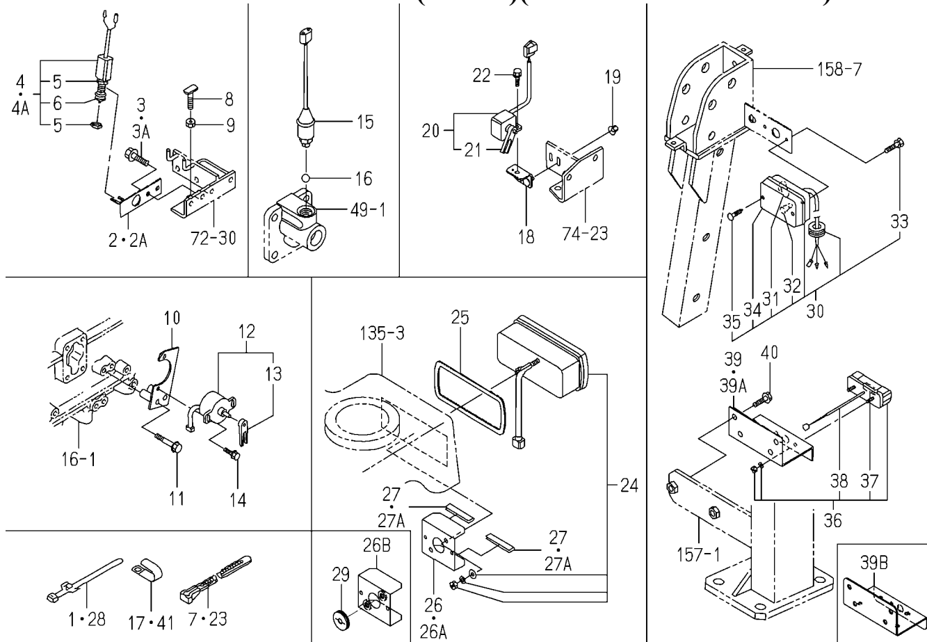
FIG.149 ELC.SYSTEM(REAR)(TH4335-SKE4A TYPE)
