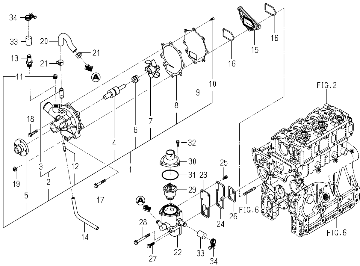
FIG. 18 WATER PUMP
