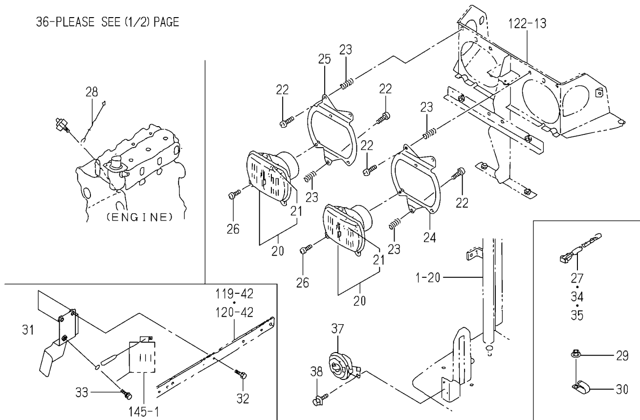
FIG.142 ELC.SYSTEM(FRONT)(E6 TYPE)(2/2)
