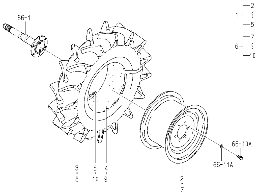
FIG.174 REAR WHEEL(12.4-16)SET(OPTION)
