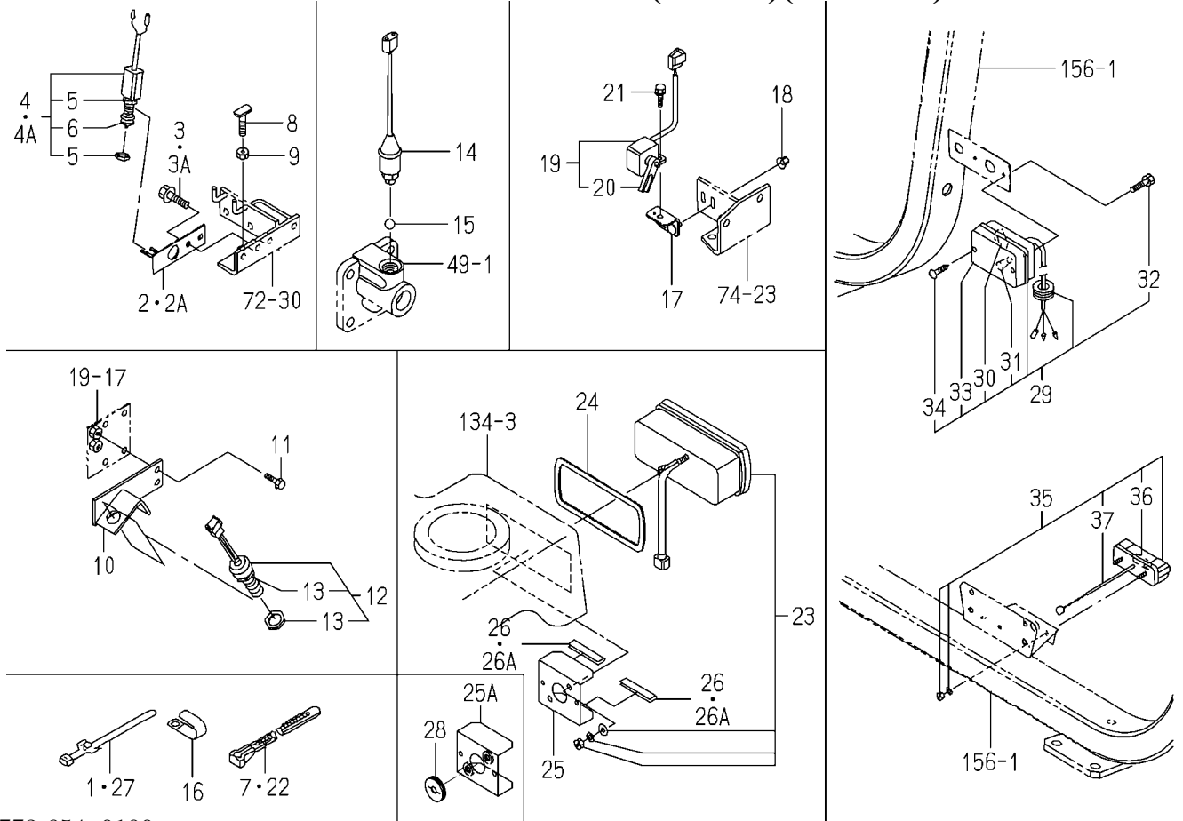
FIG.146 ELC.SYSTEM(REAR)(K TYPE)
