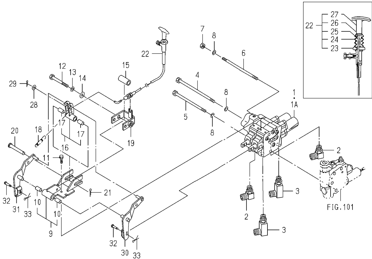
FIG.105 JOY STICK SYSTEM(TH4335-J TYPE)(1/2)
