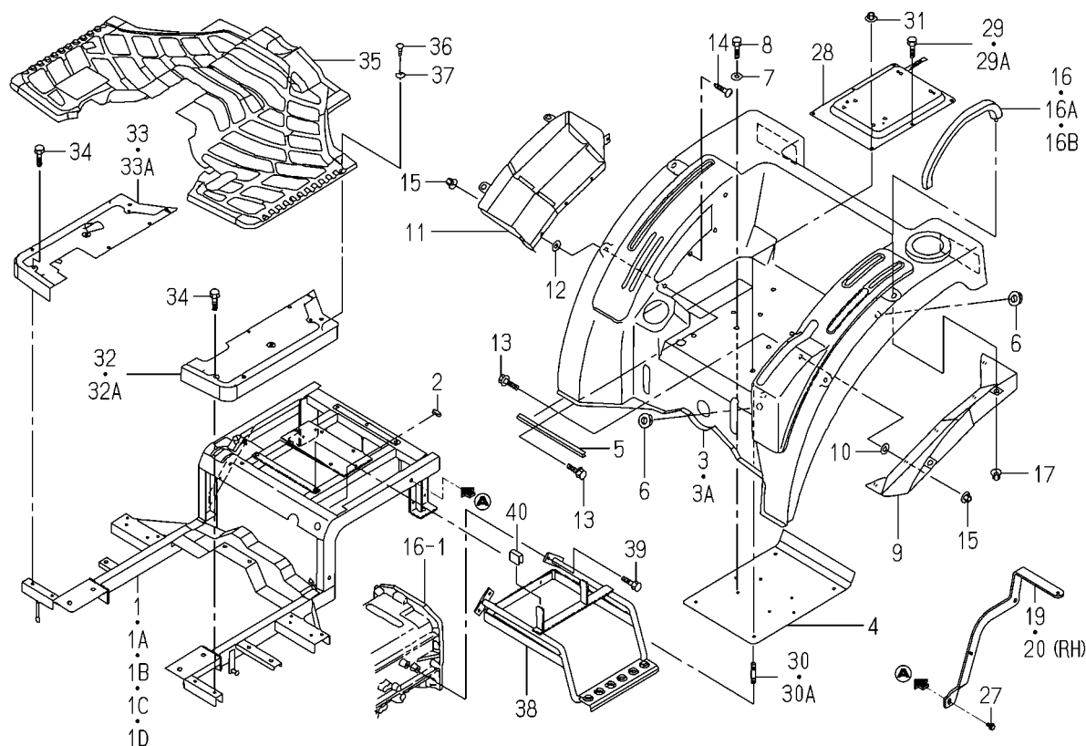
FIG.134 FLOOR(REAR)SYSTEM(1/2) (K,V TYPE EXCEPT SK)
