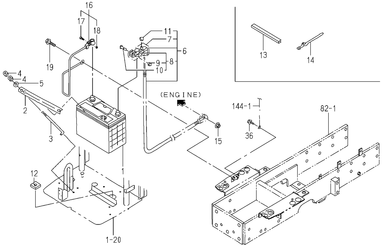
FIG.140 ELC.SYSTEM(FRONT)(1/2) (V TYPE EXCEPT SK)
