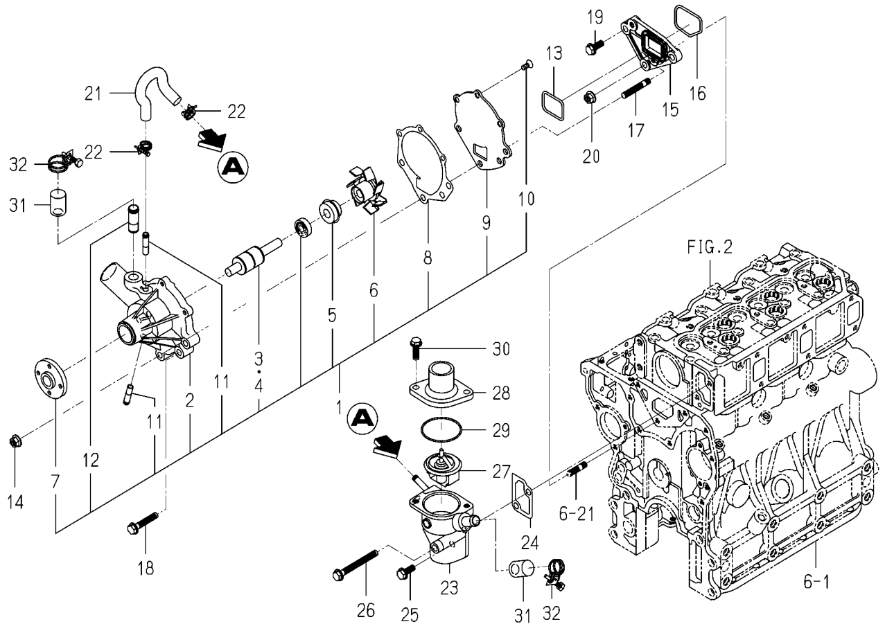
FIG. 18 WATER PUMP
