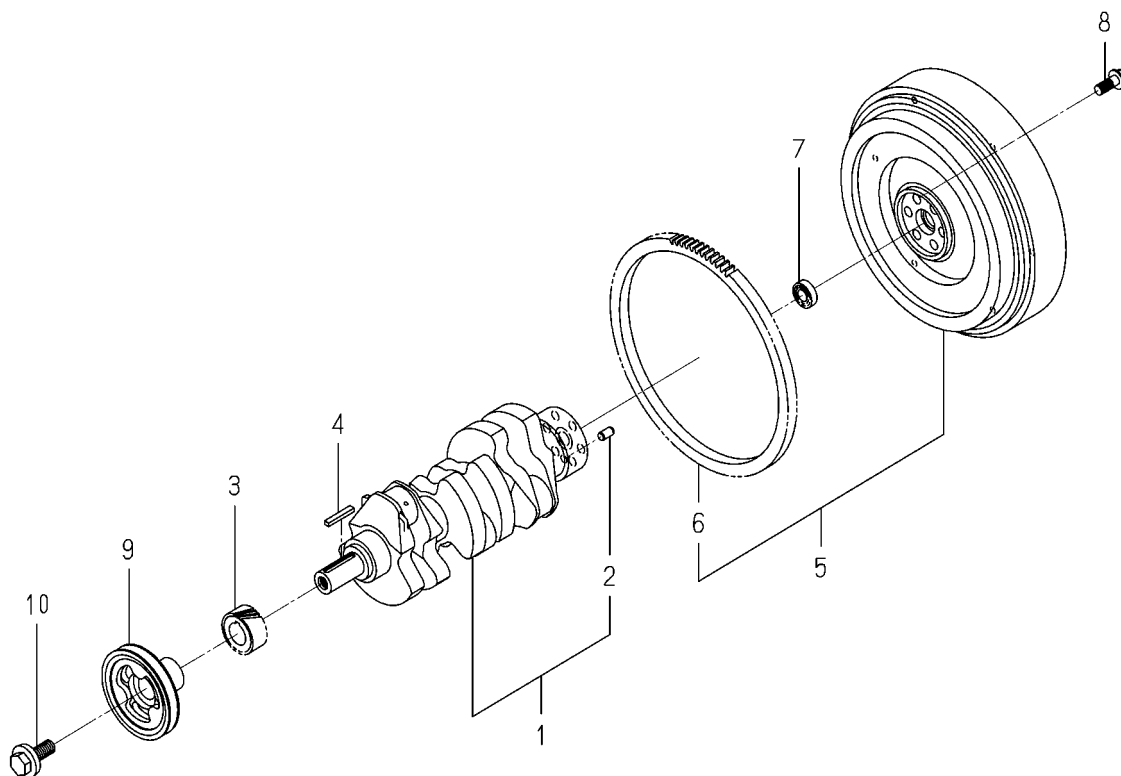
FIG. 16 CRANK SHAFT
