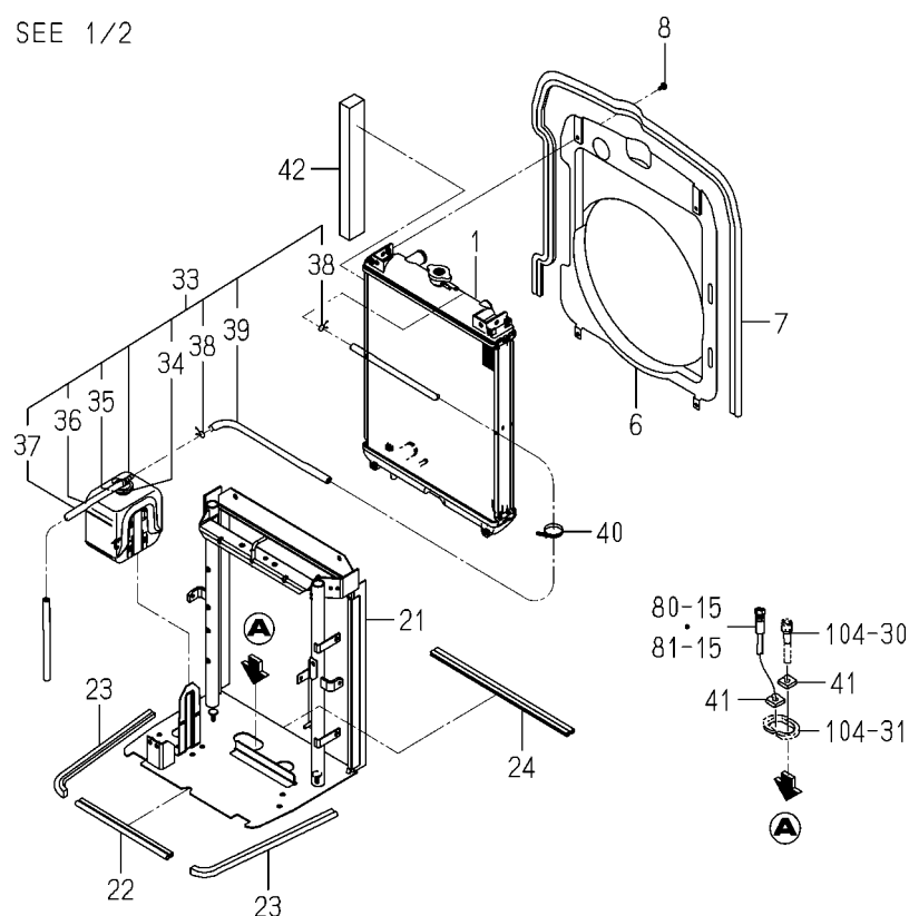
FIG. 3 RADIATOR SYSTEM(2/2) (H TYPE EXCEPT TH4365)
