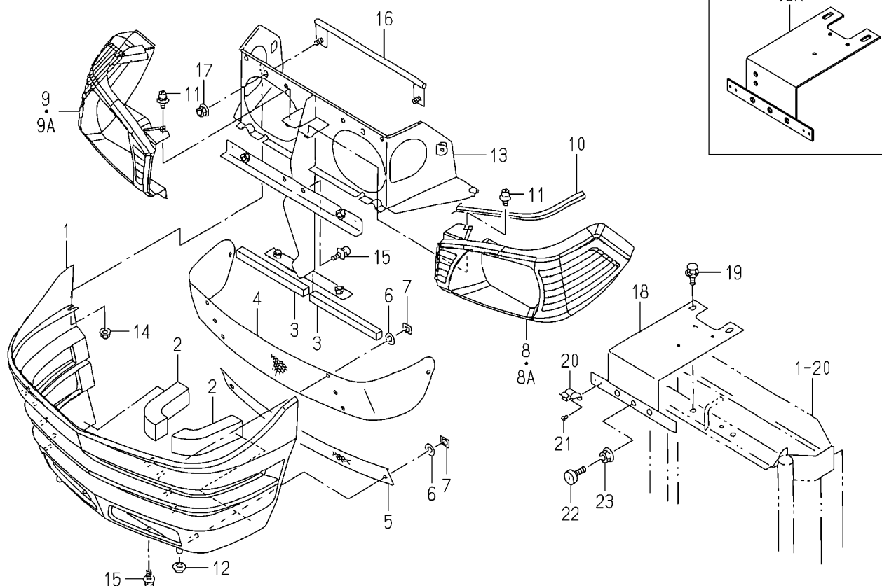
FIG.121 GRILLE SYSTEM(EXCEPT H TYPE)
