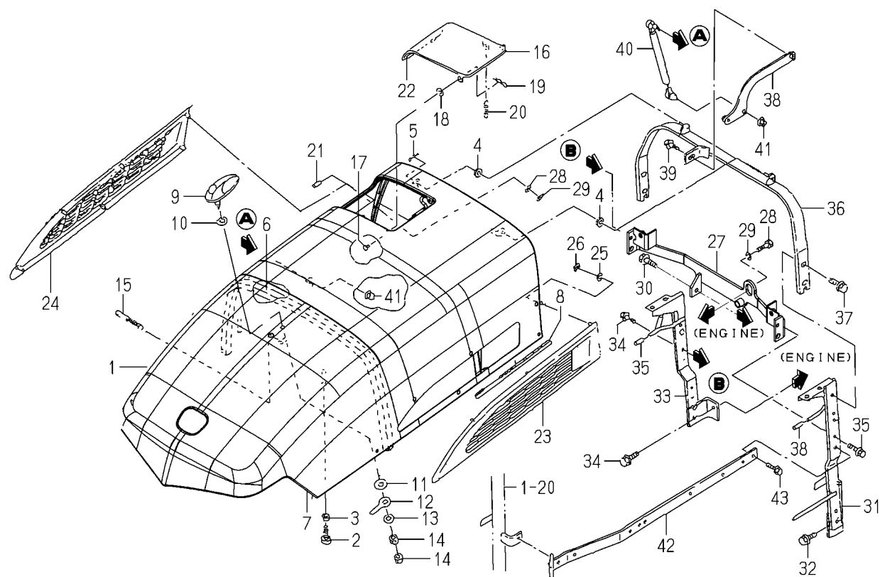
FIG.120 HOOD(SLANT) SYSTEM (H TYPE EXCEPT TH4365)
