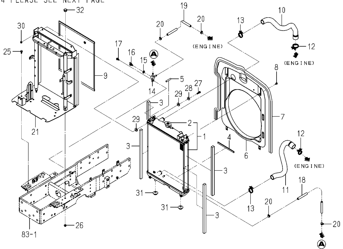
FIG. 2 RADIATOR SYSTEM(TH4365)(1/2)
