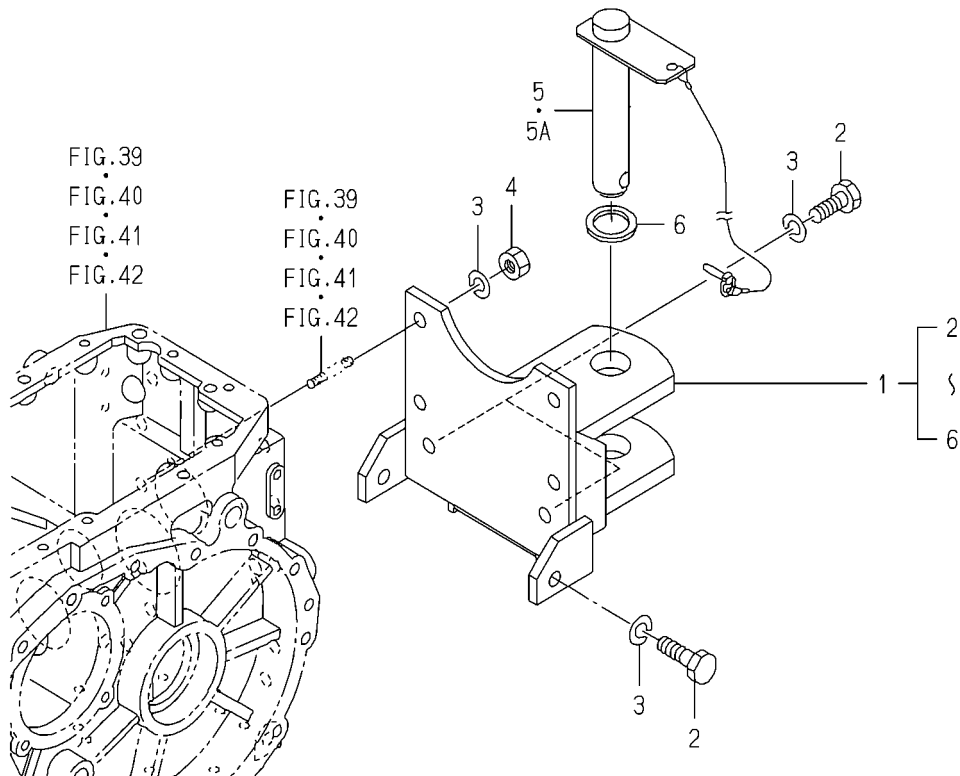
FIG.191 HITCH(TRAILER)SET (OPTION)(EXCEPT J TYPE)
