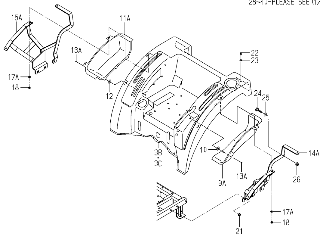
FIG.134 FLOOR(REAR)SYSTEM(2/2) (K,V TYPE EXCEPT SK)
