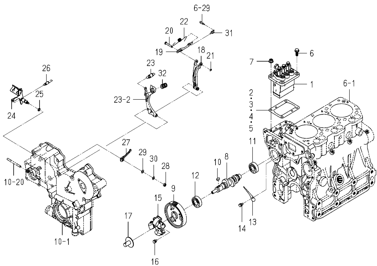
FIG. 21 INJECTION PUMP
