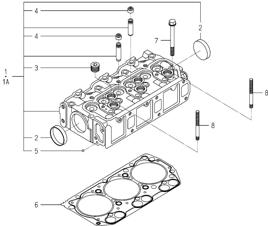
FIG. 2 CYLINDER HEAD
