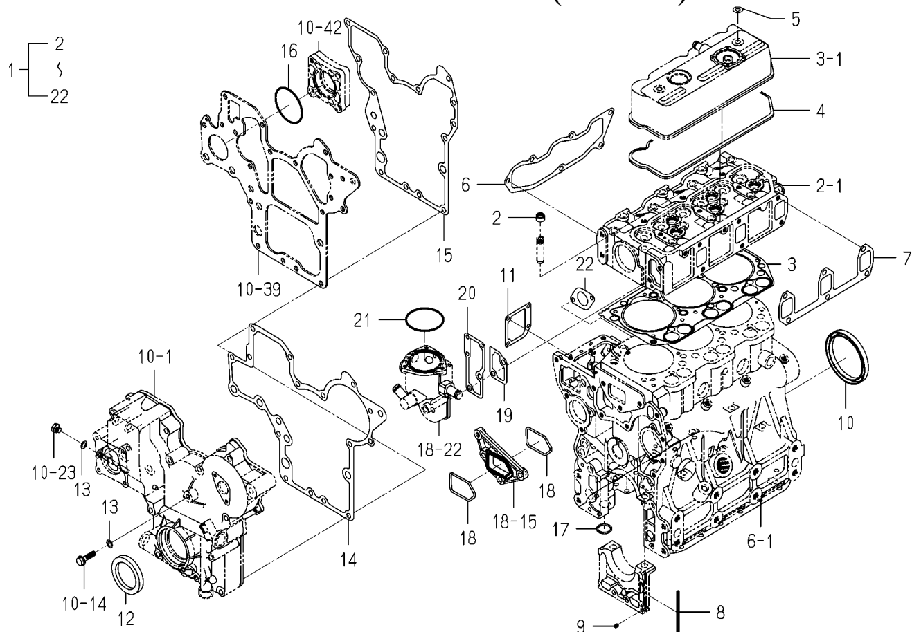
FIG. 26 REPAIR PARTS(OPTION)
