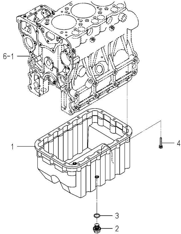
FIG. 10 OIL PAN
