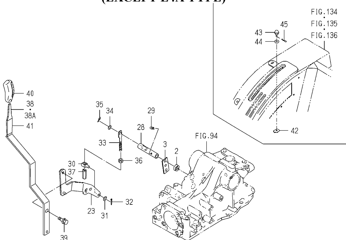
FIG. 96 MECHANICAL LINK(POSITION)SYSTEM(2/2) (EXCEPT E4A TYPE)
