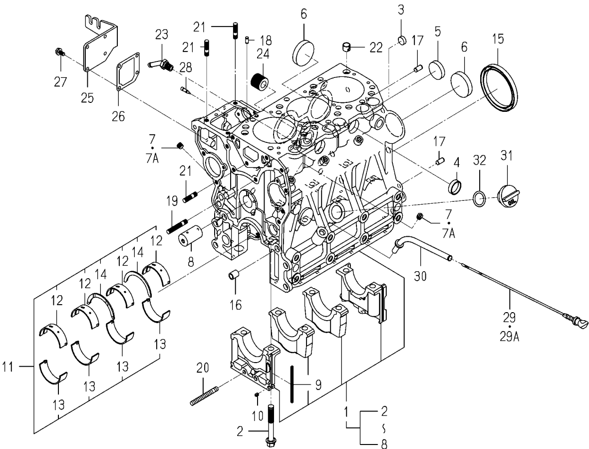
FIG. 6 CYLINDER BLOCK
