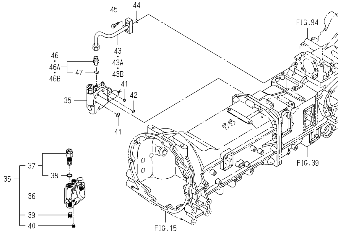
FIG. 99 HYD.SYSTEM(MAIN)(2/2) (V TYPE EXCEPT SK)
