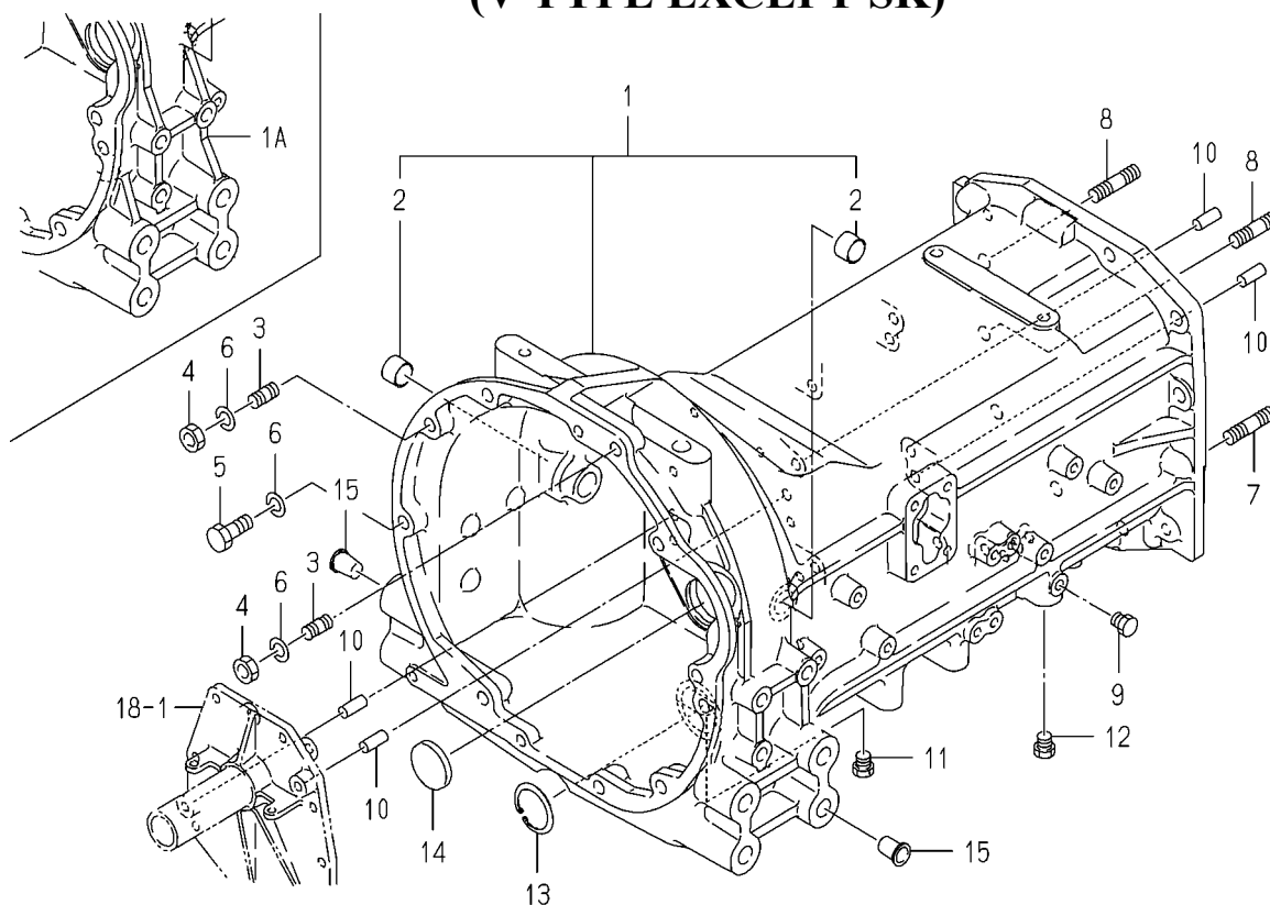
FIG. 15 CASE(TRANSMISSION/FRONT)SYSTEM (V TYPE EXCEPT SK)
