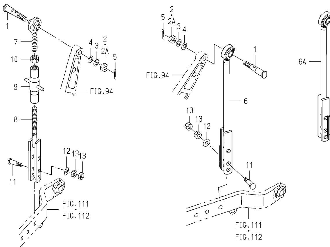
FIG.113 LIFT ROD SYSTEM
