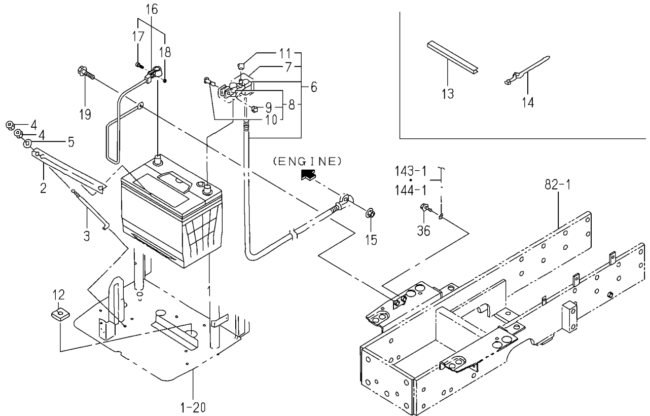
FIG.139 ELC.SYSTEM(FRONT)(K,SK TYPE)(1/2)
