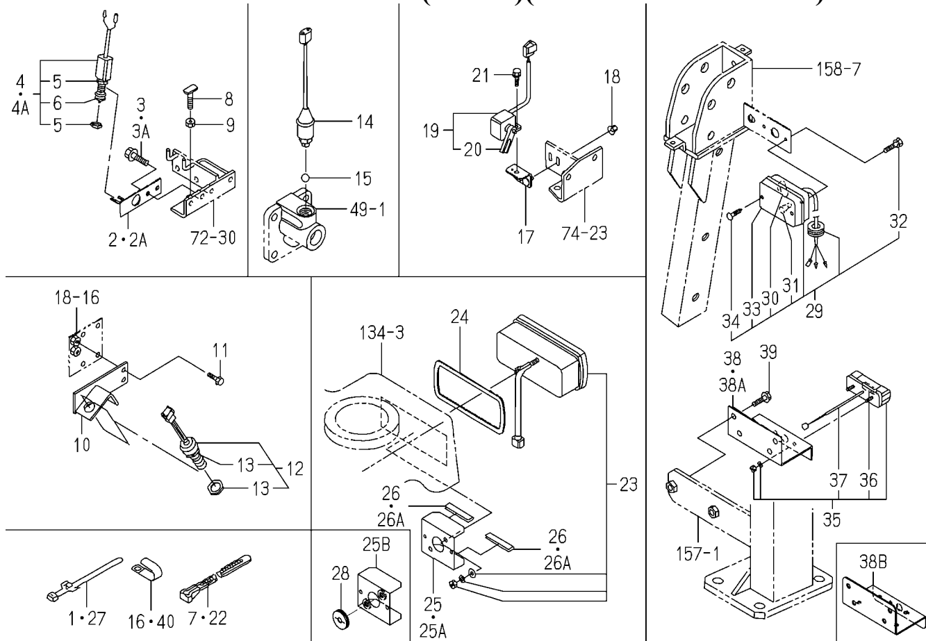
FIG.148 ELC.SYSTEM(REAR)(V TYPE EXCEPT SK)
