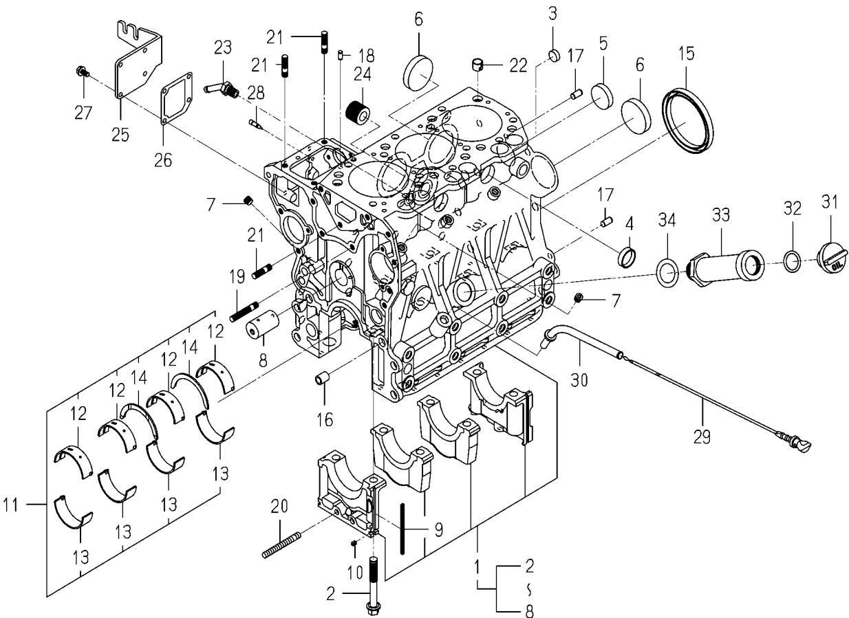
FIG. 6 CYLINDER BLOCK
