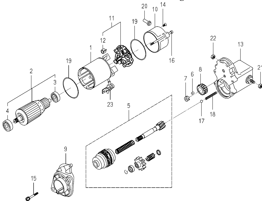
FIG. 30 COMPONENT PARTS FOR 6281-100-007-20 ON Fig.25
