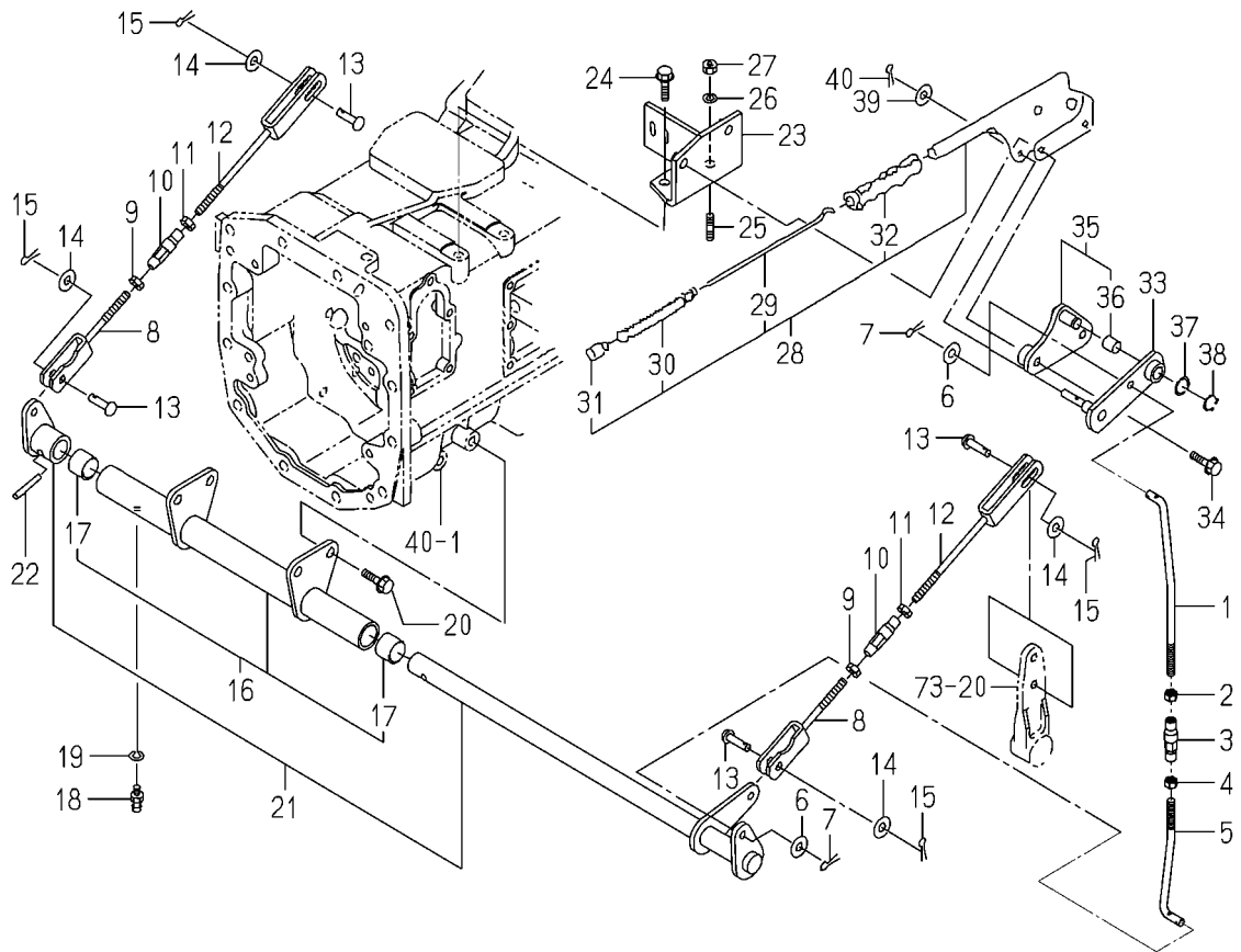
FIG. 75 BRAKE(PARKING)SYSTEM(H TYPE)
