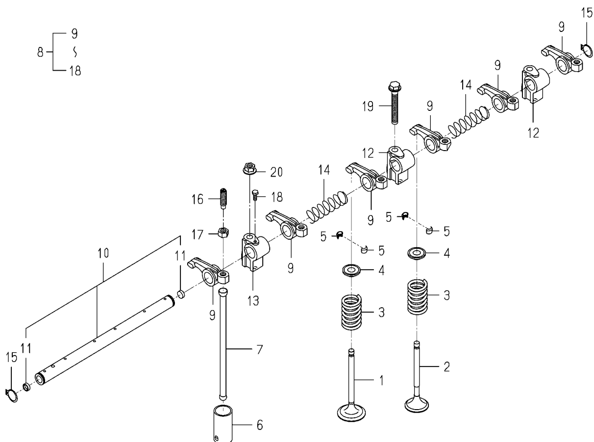
FIG. 12 VALVE
