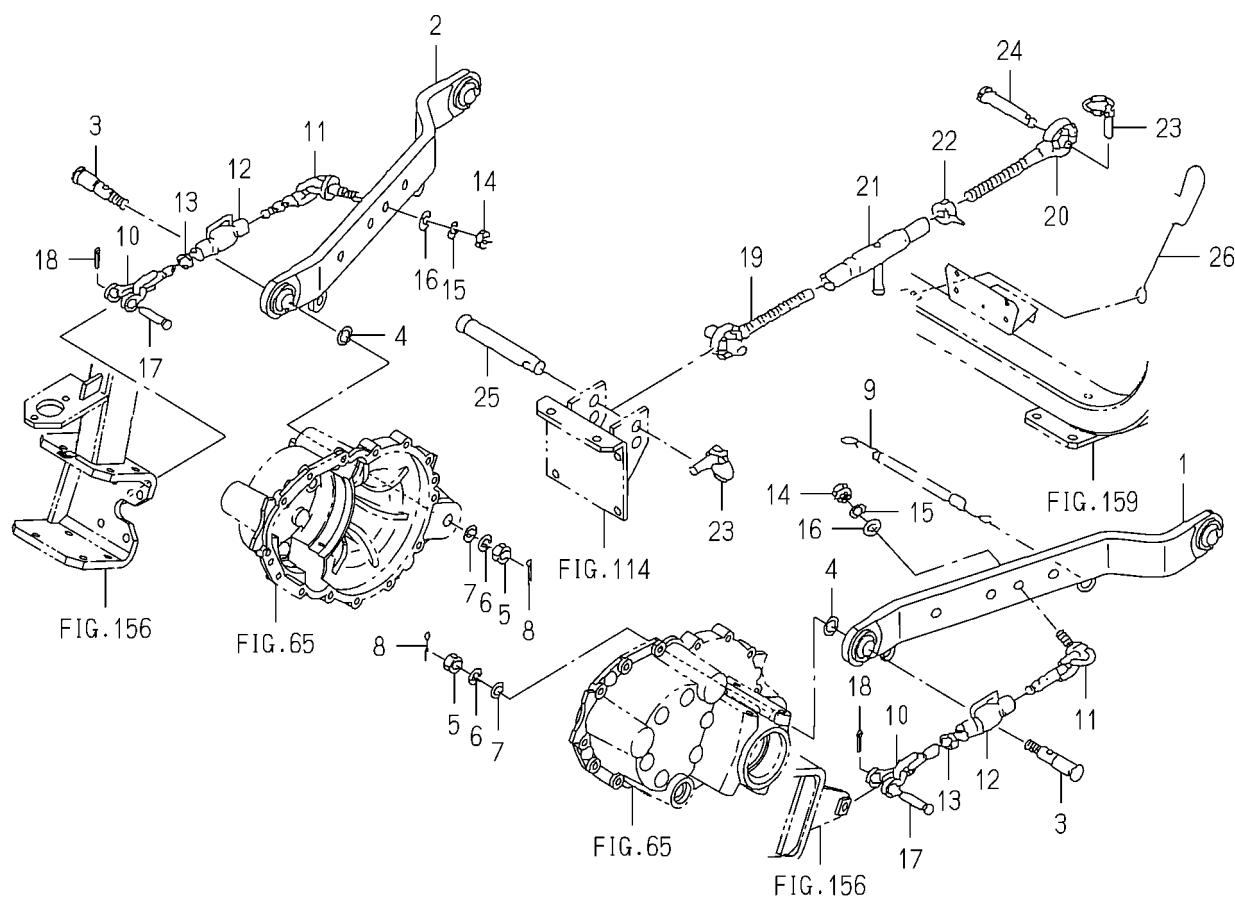
FIG.112 3P LINK SYSTEM(E4 TYPE)
