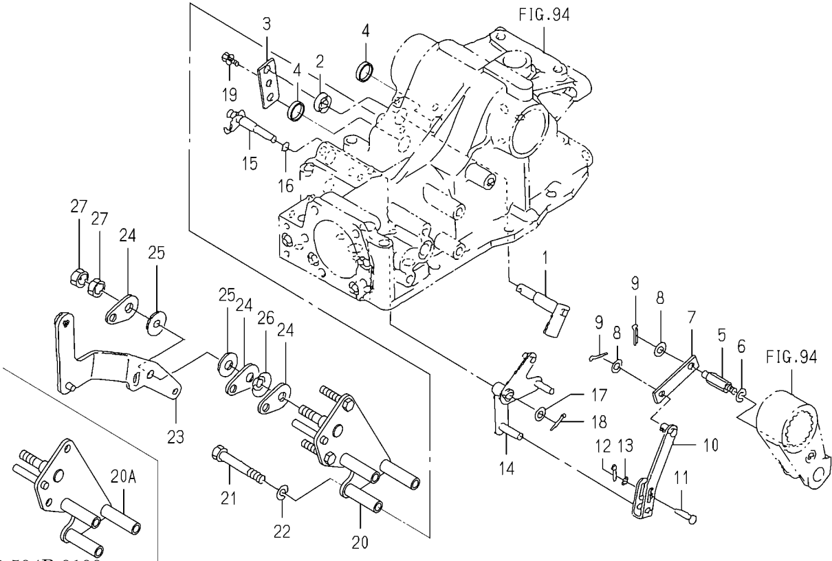
FIG. 96 MECHANICAL LINK(POSITION)SYSTEM(1/2) (EXCEPT E4A TYPE)
