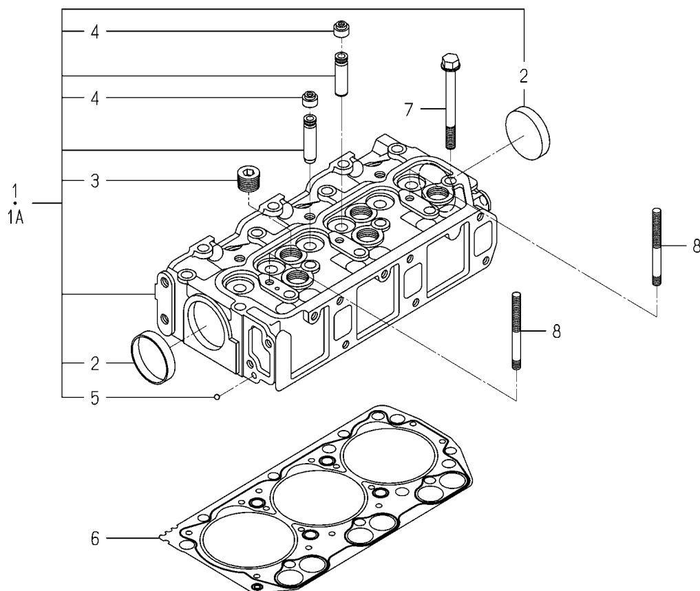
FIG. 2 CYLINDER HEAD
