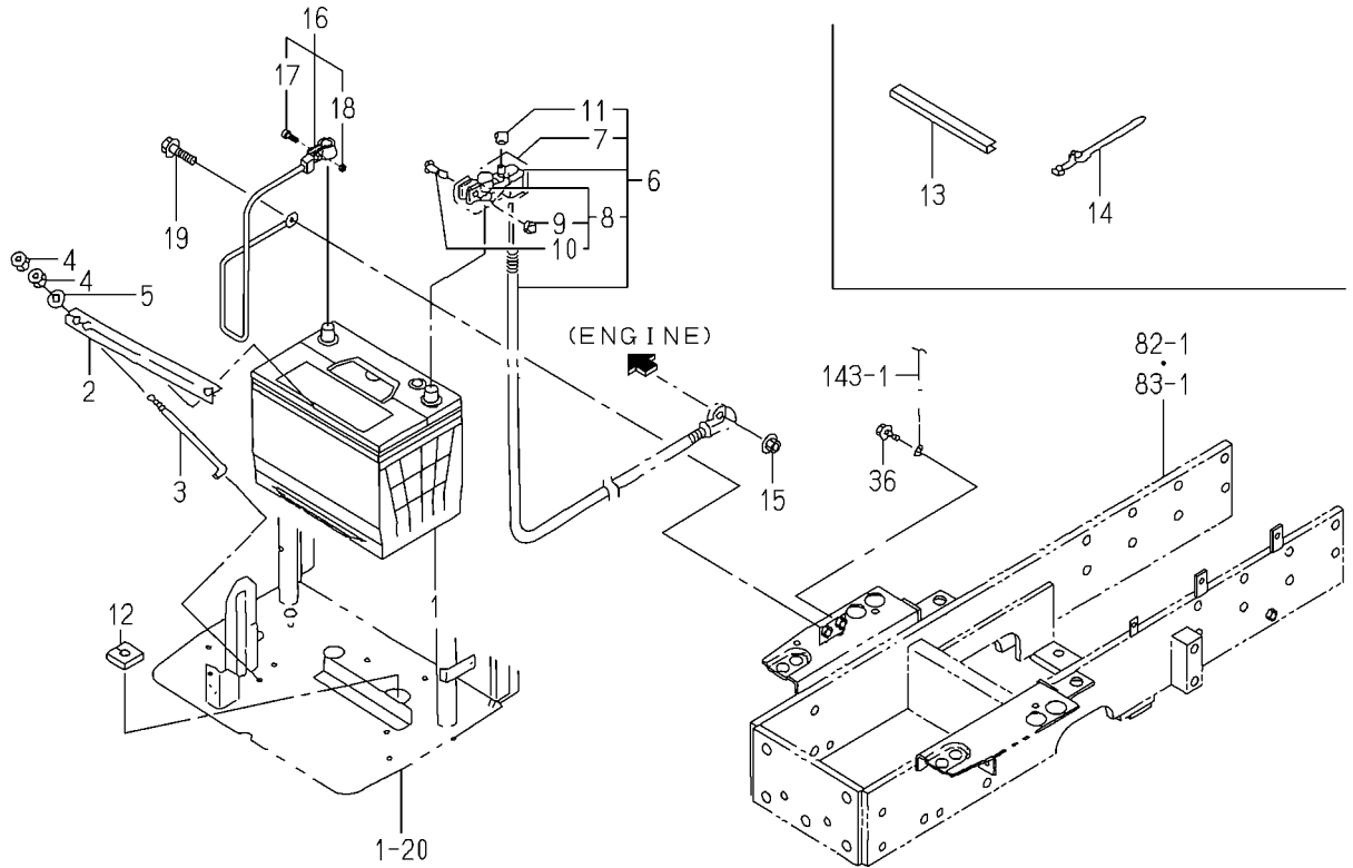
FIG.141 ELC.SYSTEM(FRONT)(1/2) (J TYPE EXCEPT H)
