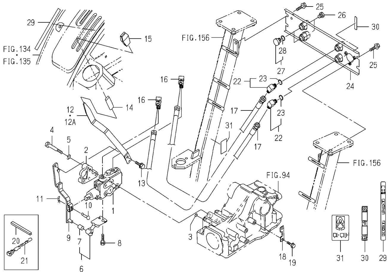
FIG.108 VALVE(REMOTE/1R)SYSTEM(V TYPE)
