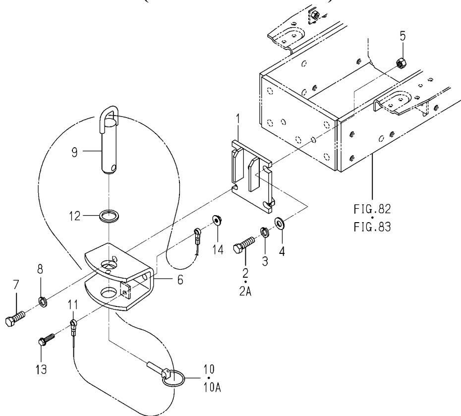
FIG. 85 FRONT HITCH(BUMPER)SYSTEM (EXCEPT HJ TYPE)
