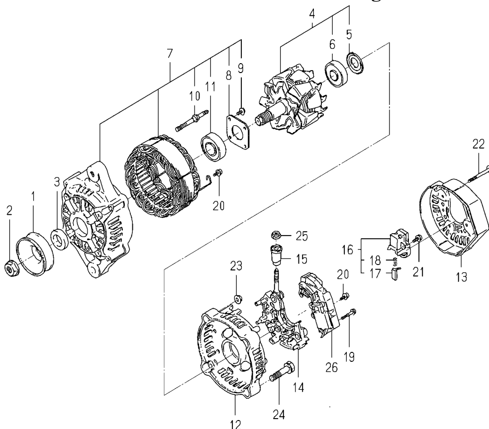
FIG. 31 COMPONENT PARTS FOR 6281-200-020-00 ON Fig.25
