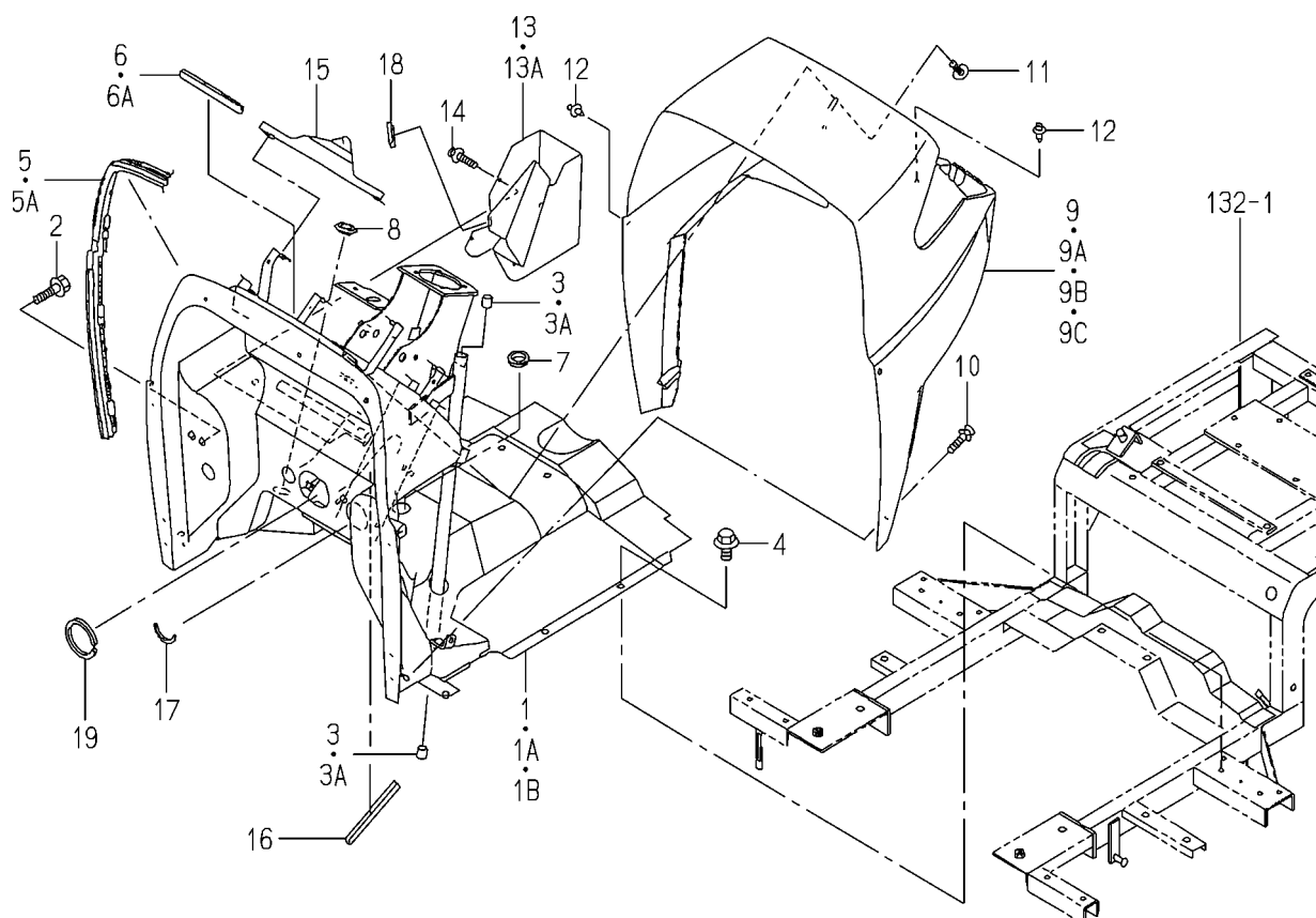
FIG.132 DASHBOARD SYSTEM(SK TYPE)
