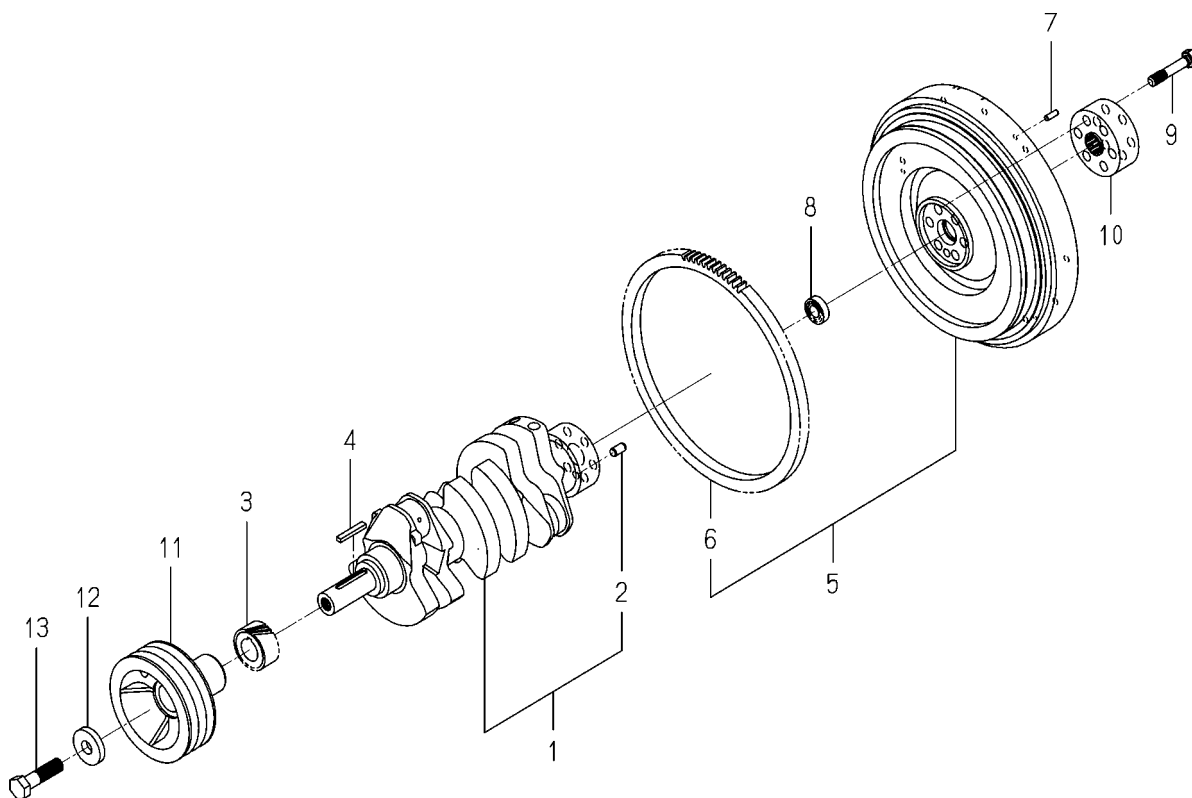
FIG. 16 CRANK SHAFT
