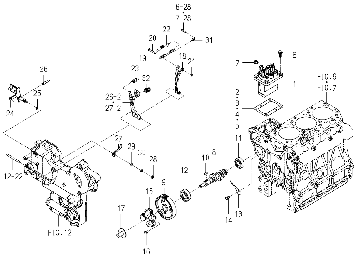
FIG. 24 INJECTION PUMP
