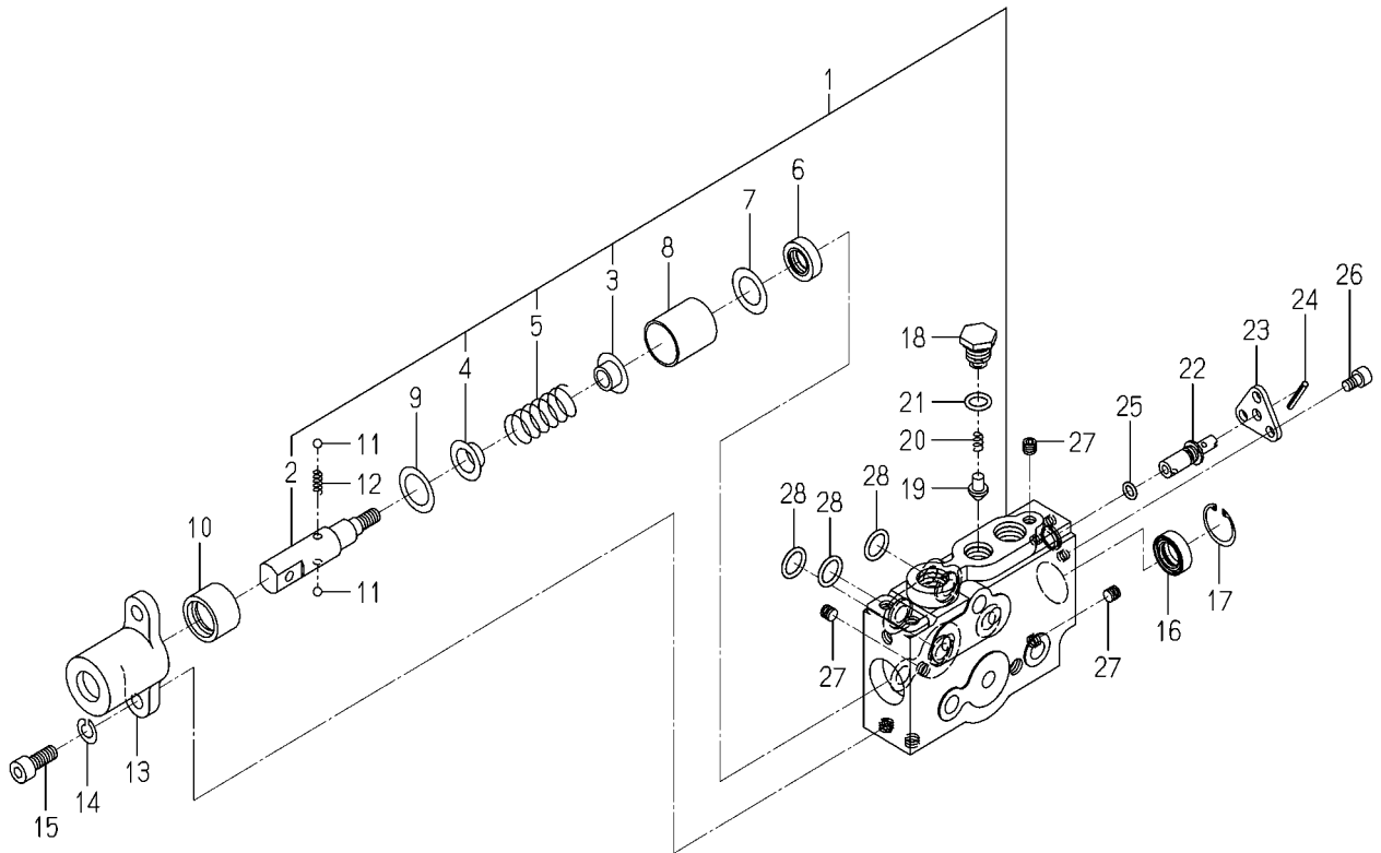
FIG.200 COMPONENT PARTS FOR 1640-530-600-10 ON Fig.188,189,190
