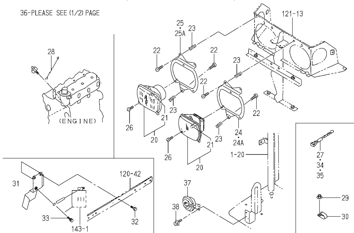
FIG.141 ELC.SYSTEM(FRONT)(2/2) (J TYPE EXCEPT H)
