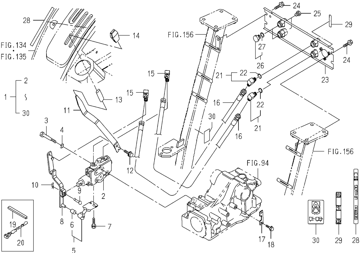
FIG.188 VALVE(REMOTE/1R)SET (OPTION)(TH4335-J TYPE)
