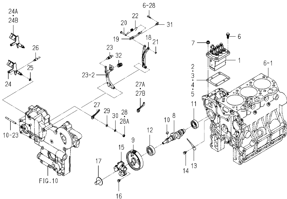
FIG. 21 INJECTION PUMP
