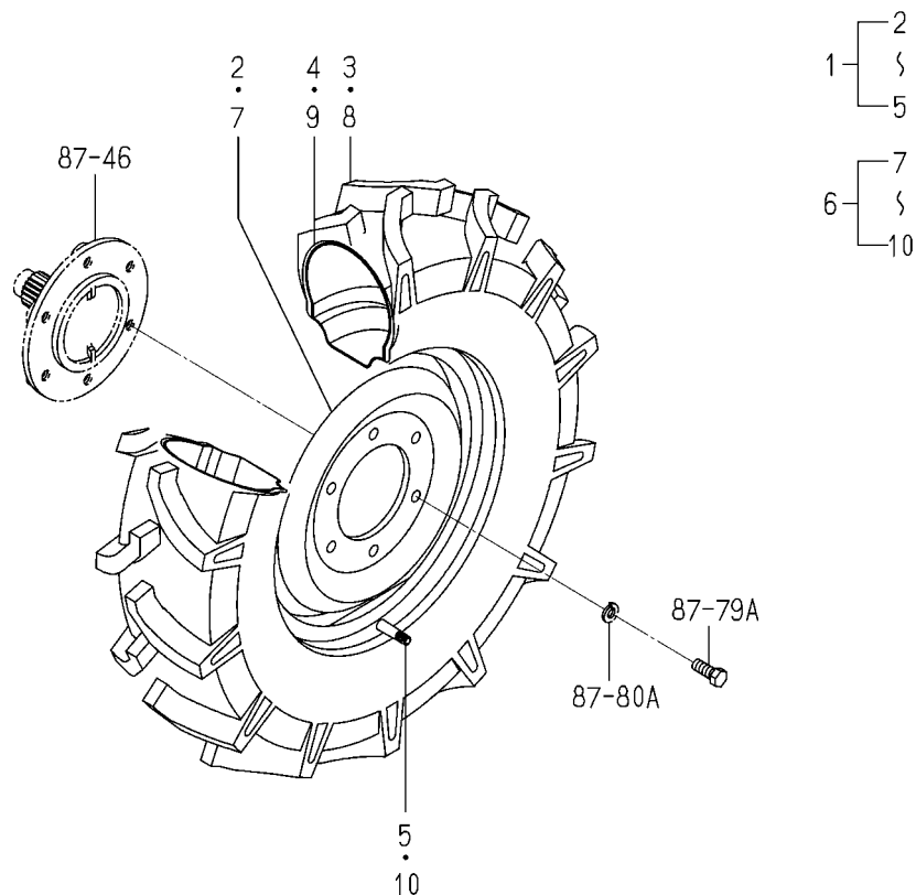
FIG.180 FRONT WHEEL(4WD)SET(OPTION)
