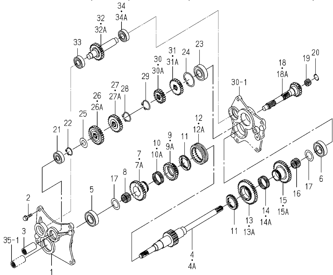
FIG. 27 GEAR(MAIN)SYSTEM(V TYPE EXCEPT SK)
