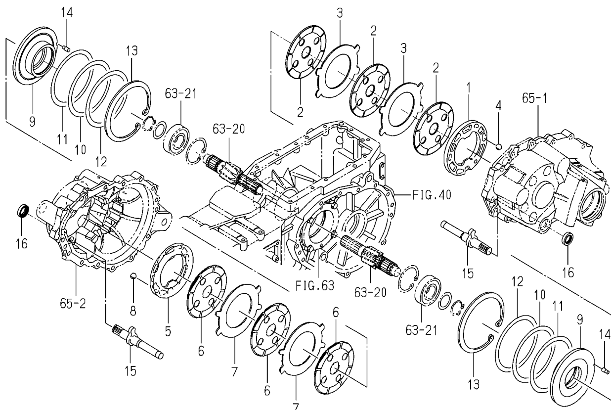
FIG. 71 BRAKE SYSTEM(H TYPE)
