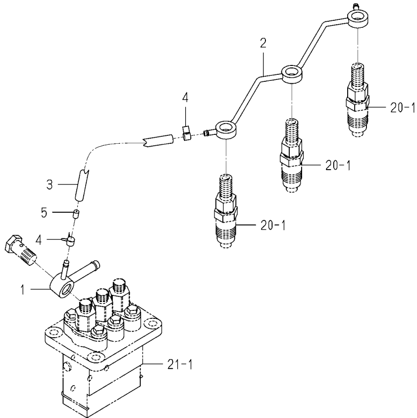
FIG. 22 FUEL PIPE
