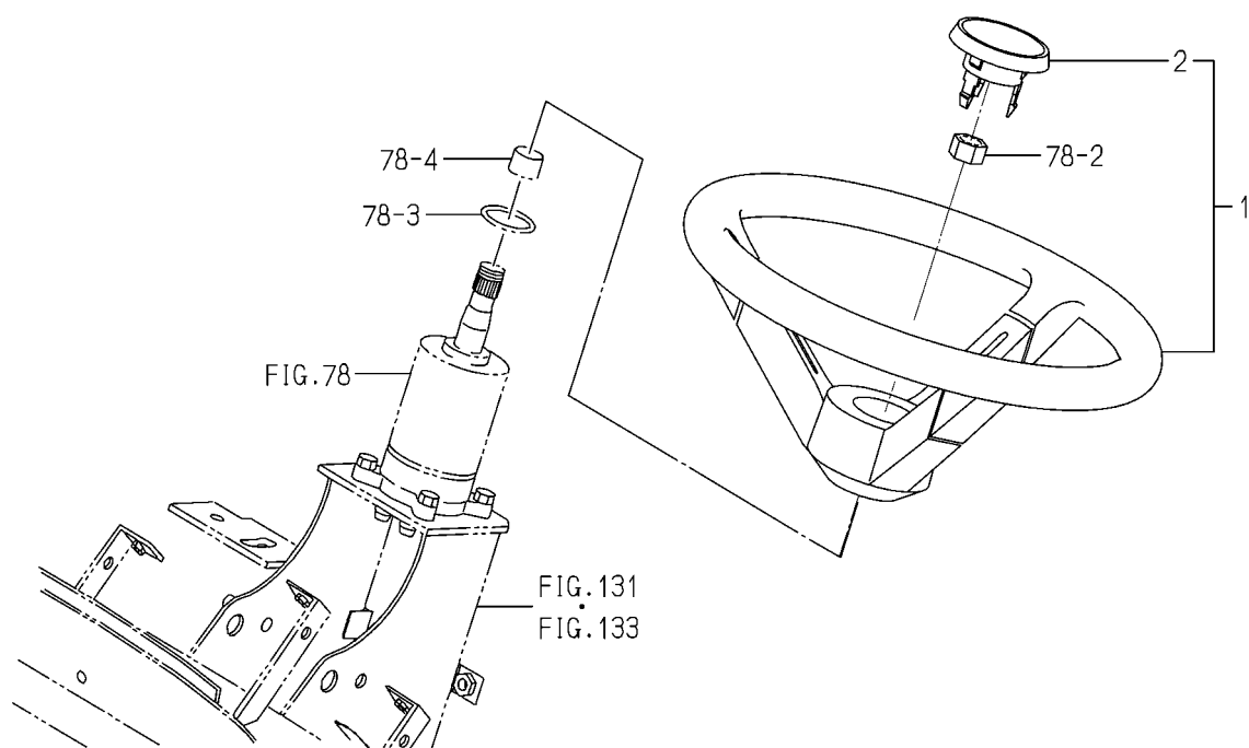
FIG. 76 WHEEL(STEERING)SYSTEM
