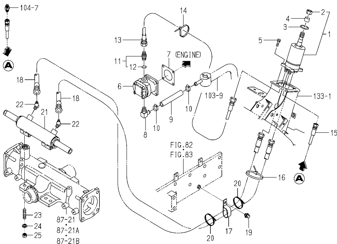
FIG. 80 STEERING(POWER)SYSTEM (H TYPE EXCEPT J)
