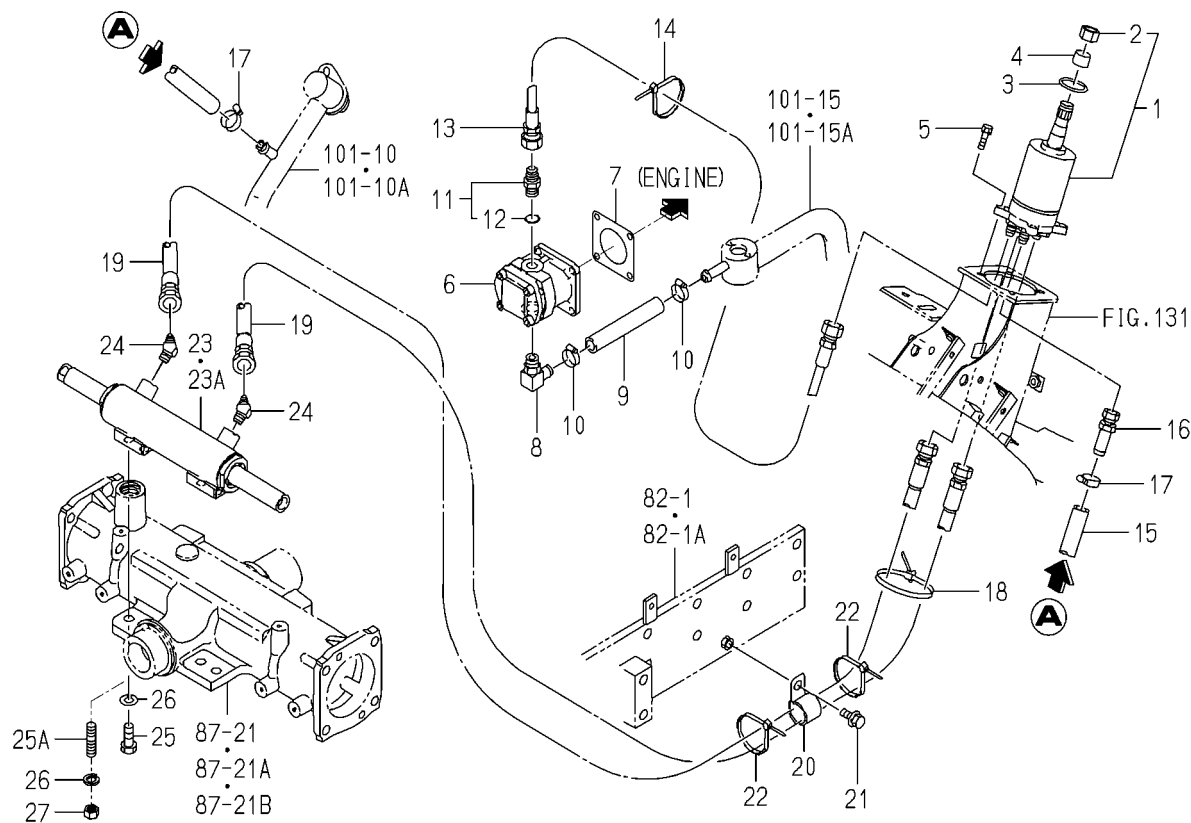
FIG. 79 STEERING(POWER)SYSTEM (K,SK TYPE EXCEPT J,V)
