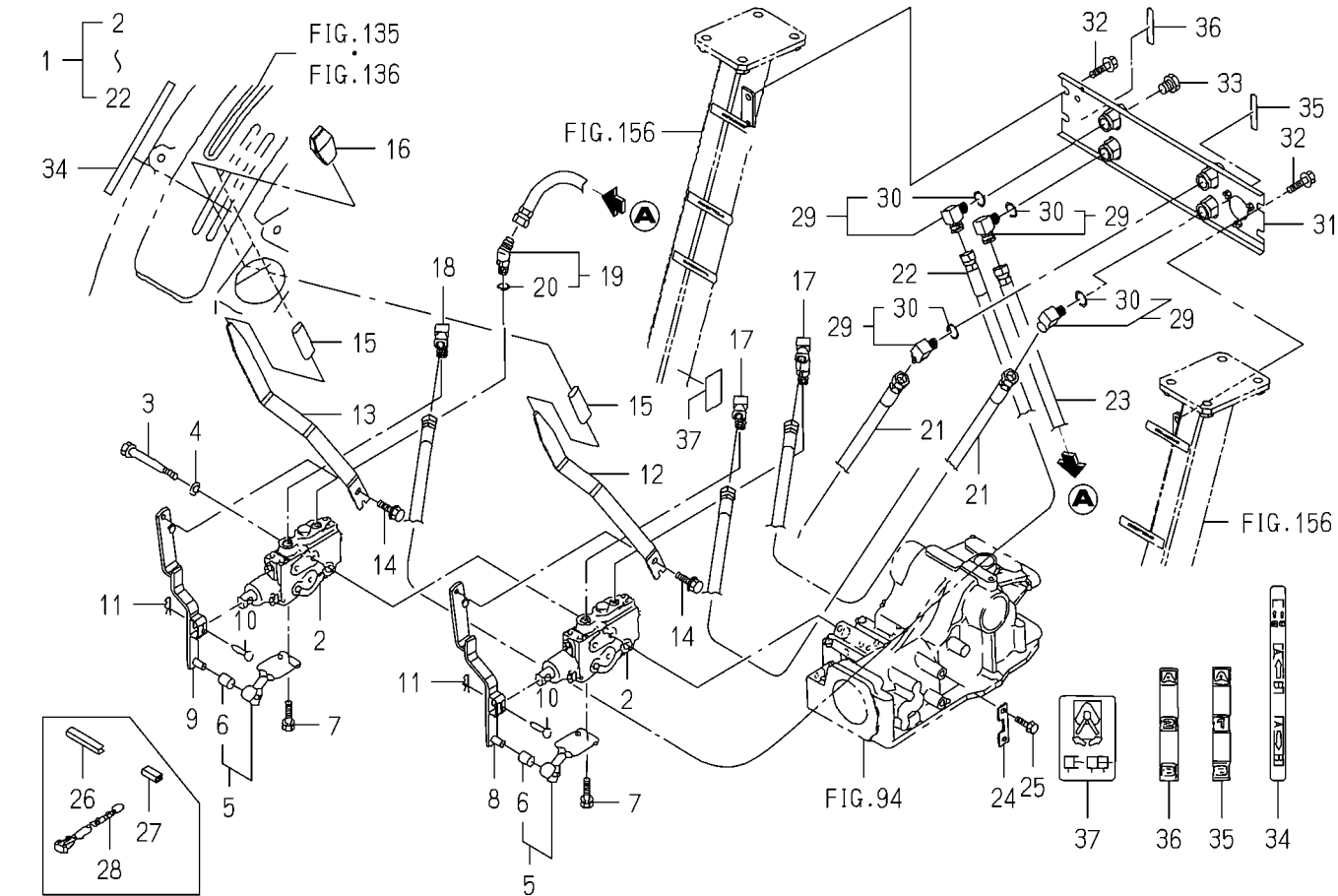
FIG.190 VALVE(REMOTE/2R)SET(OPTION)(J TYPE)
