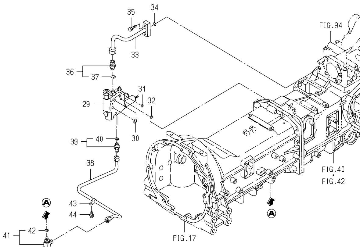
FIG.103 HYD.SYSTEM(MAIN)(2/2) (H TYPE EXCEPT TH4365)
