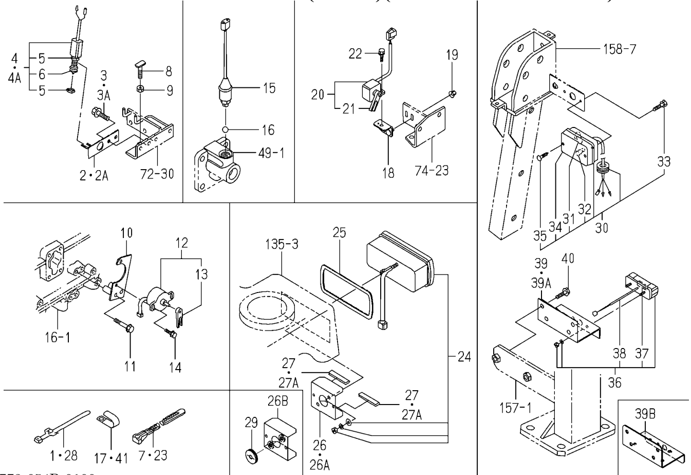
FIG.149 ELC.SYSTEM(REAR)(TH4335-SKE4A TYPE)
