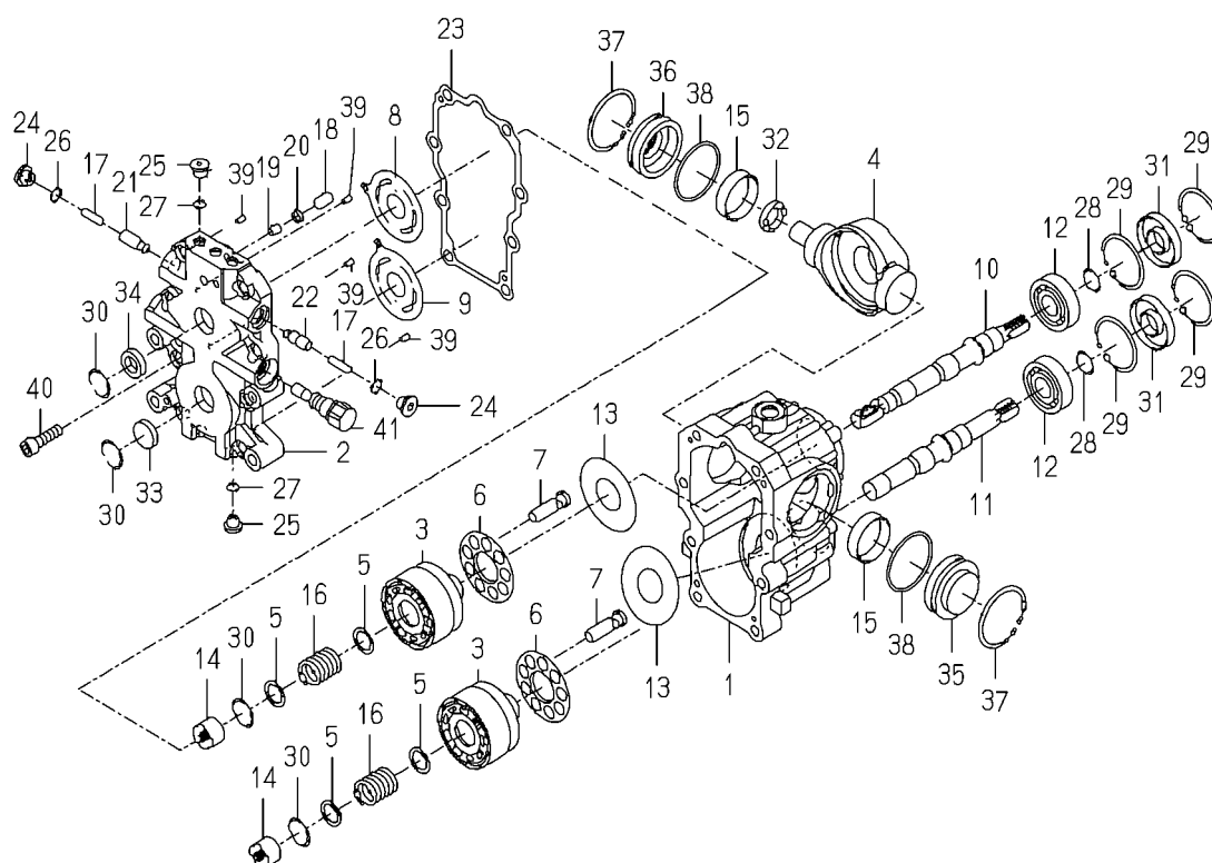
FIG.199 COMPONENT PARTS FOR K500-001-000-10 ON Fig.21
