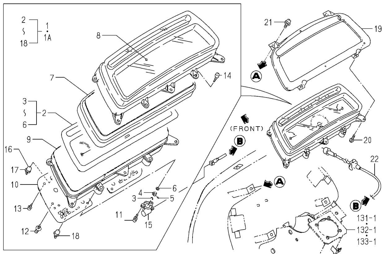
FIG.151 METER PANEL SYSTEM
