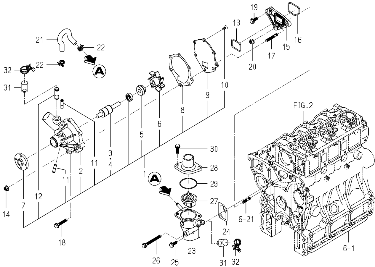
FIG. 18 WATER PUMP
