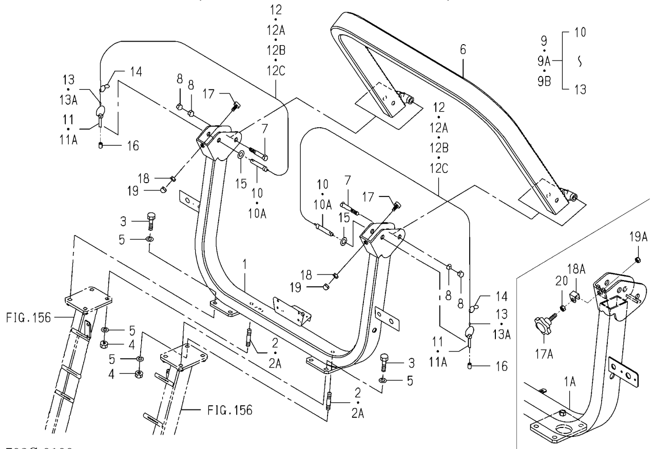
FIG.159 FRAME(REAR)SYSTEM (EXCEPT E4D,E4A TYPE)
