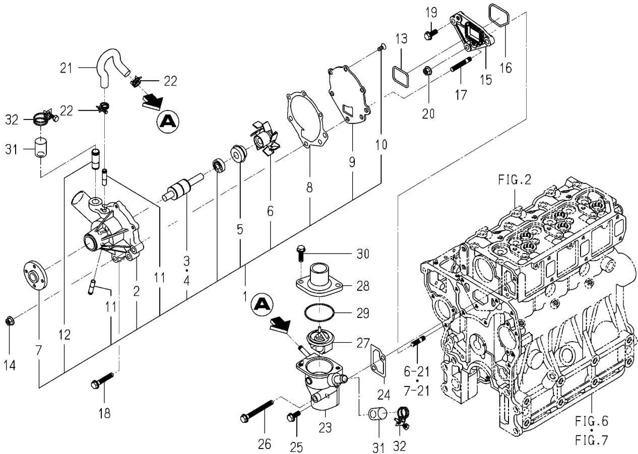
FIG. 21 WATER PUMP
