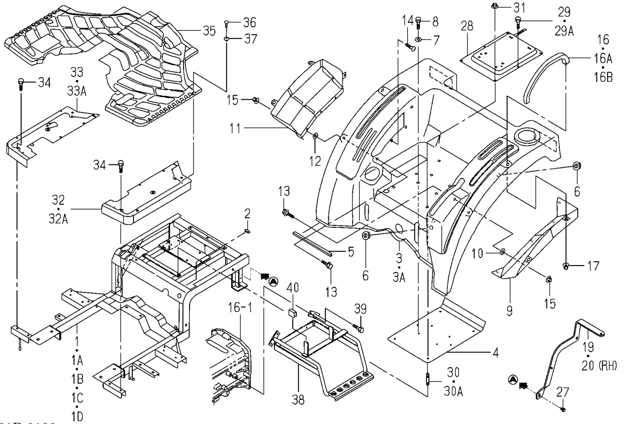
FIG.135 FLOOR(REAR)SYSTEM(SK TYPE)(1/2)
