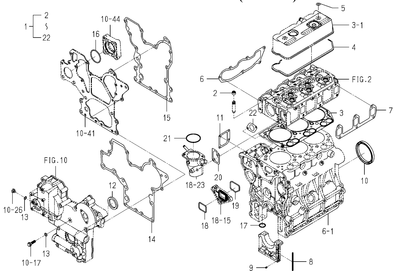
FIG. 27 REPAIR PARTS(OPTION)
