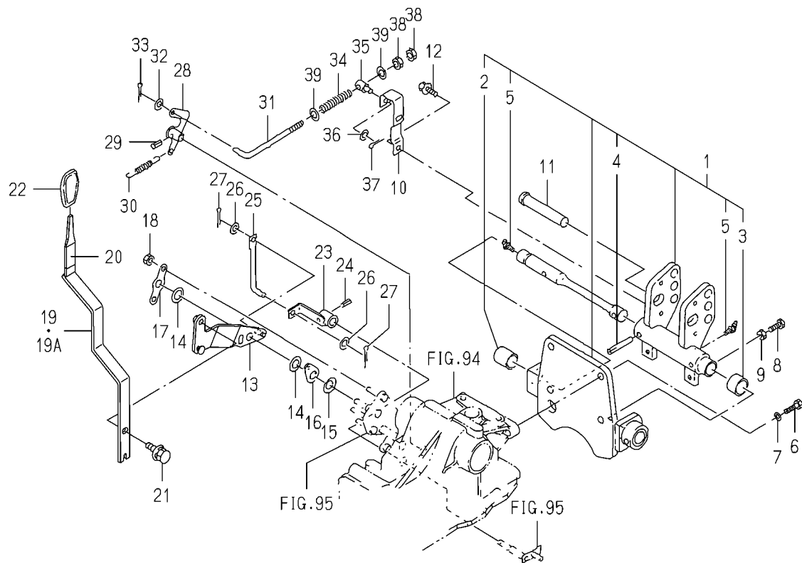
FIG. 97 MECHANICAL LINK(DRAFT)SYSTEM (E4A TYPE)
