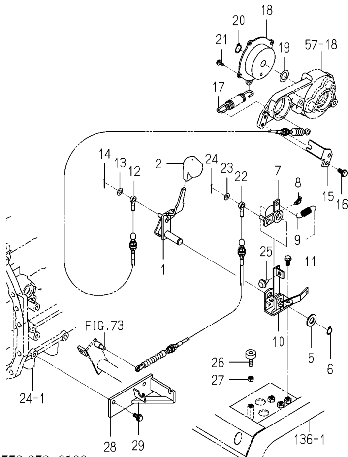
FIG. 58 AUTO CRUISE SYSTEM(H TYPE)
