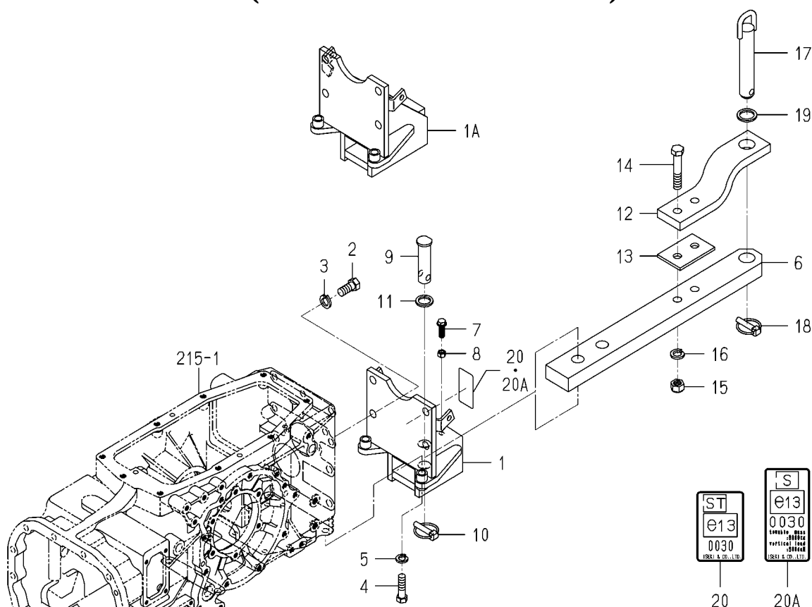
FIG.519 DRAW BAR(FIX)SYSTEM (TG5475 TYPE EXCEPT D)
