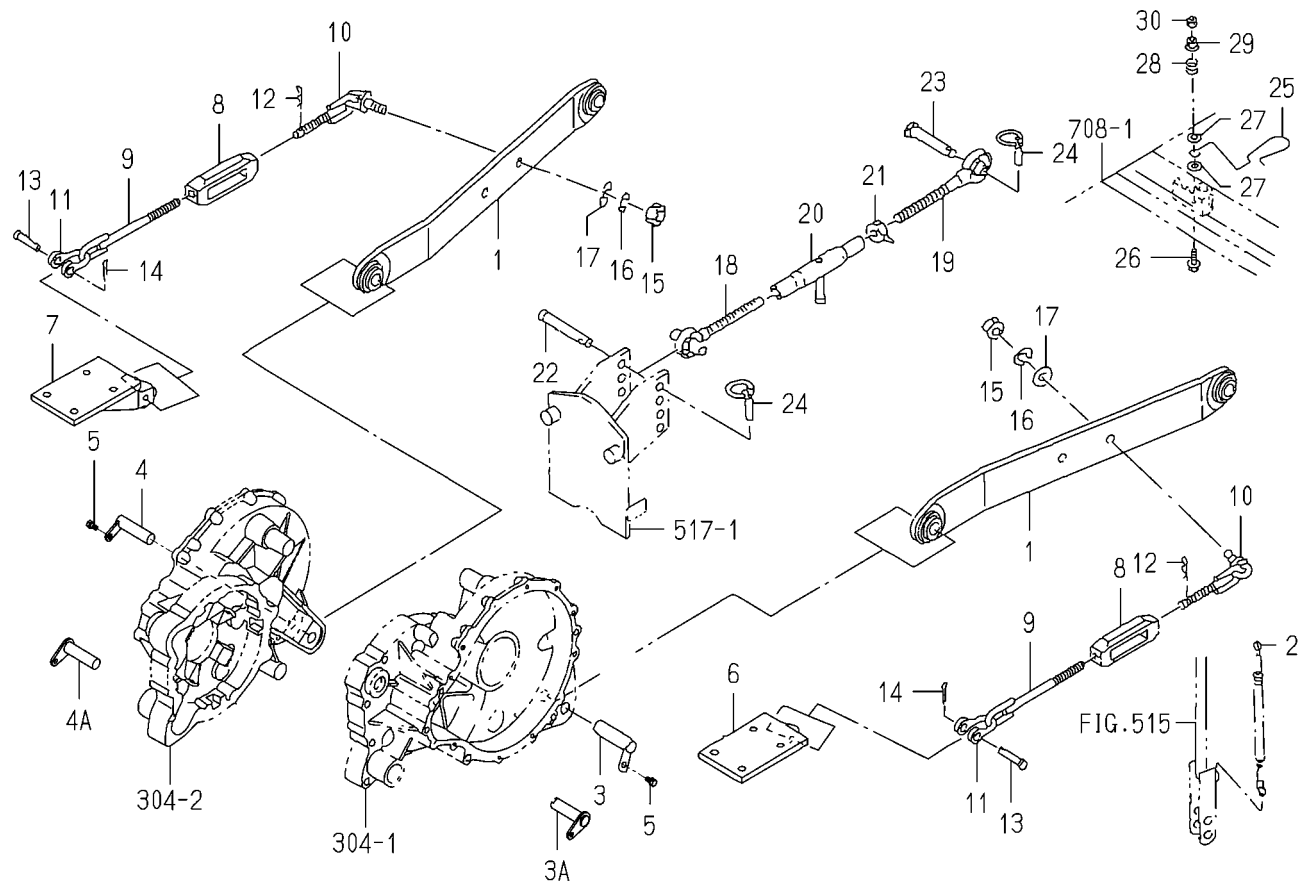
FIG.513 3P LINK SYSTEM(TG5475-C TYPE)
