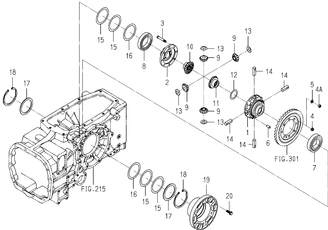
FIG.303 DIFF SYSTEM
