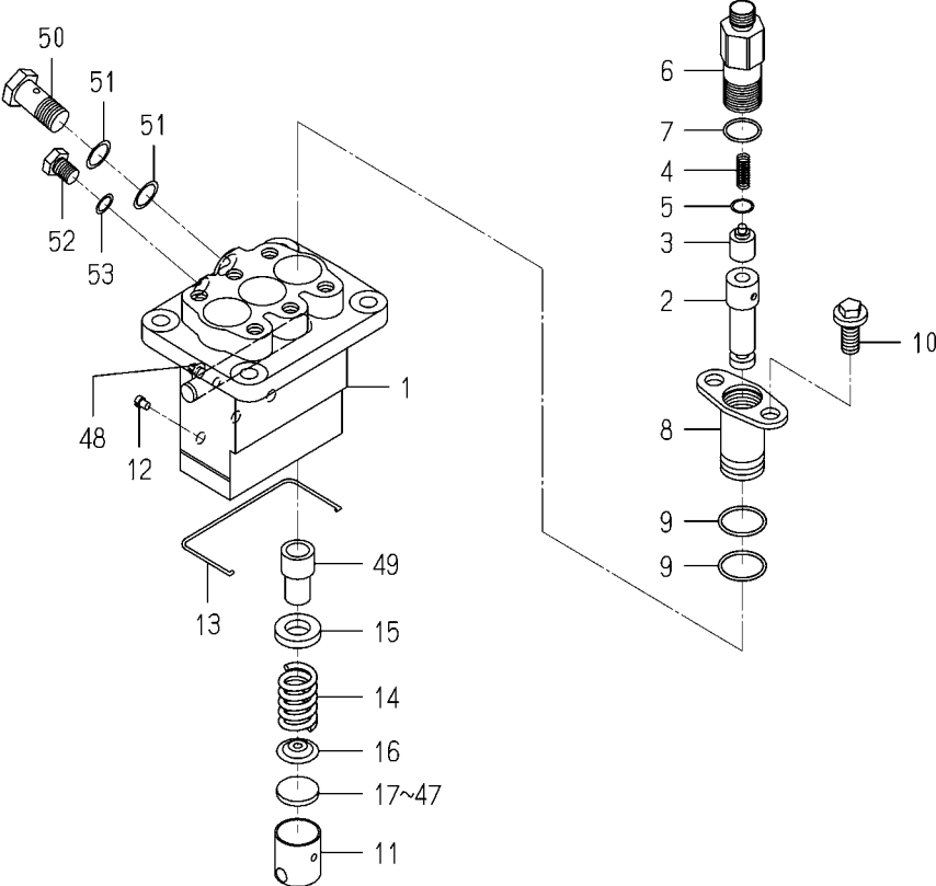
FIG.S02 COMPONENT PARTS FOR 6215-600-078-10 ON Fig.502
