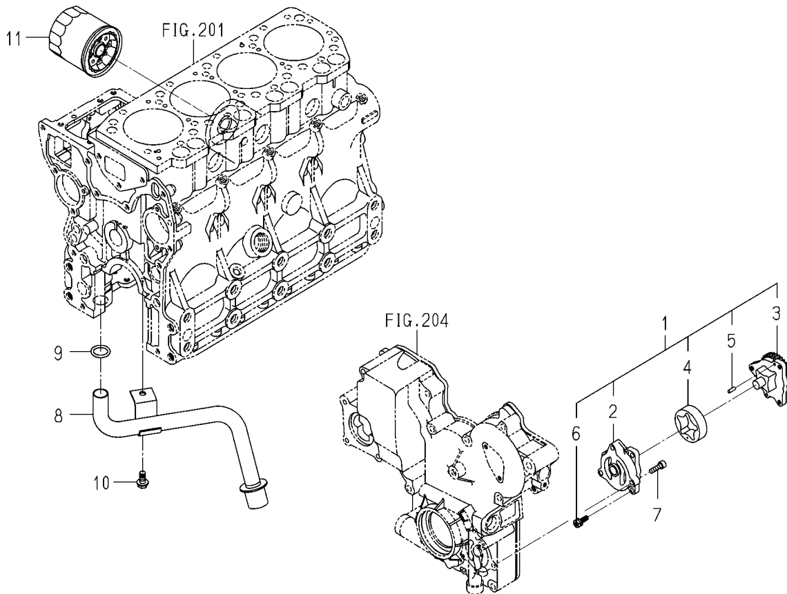
FIG.401 OIL PUMP
