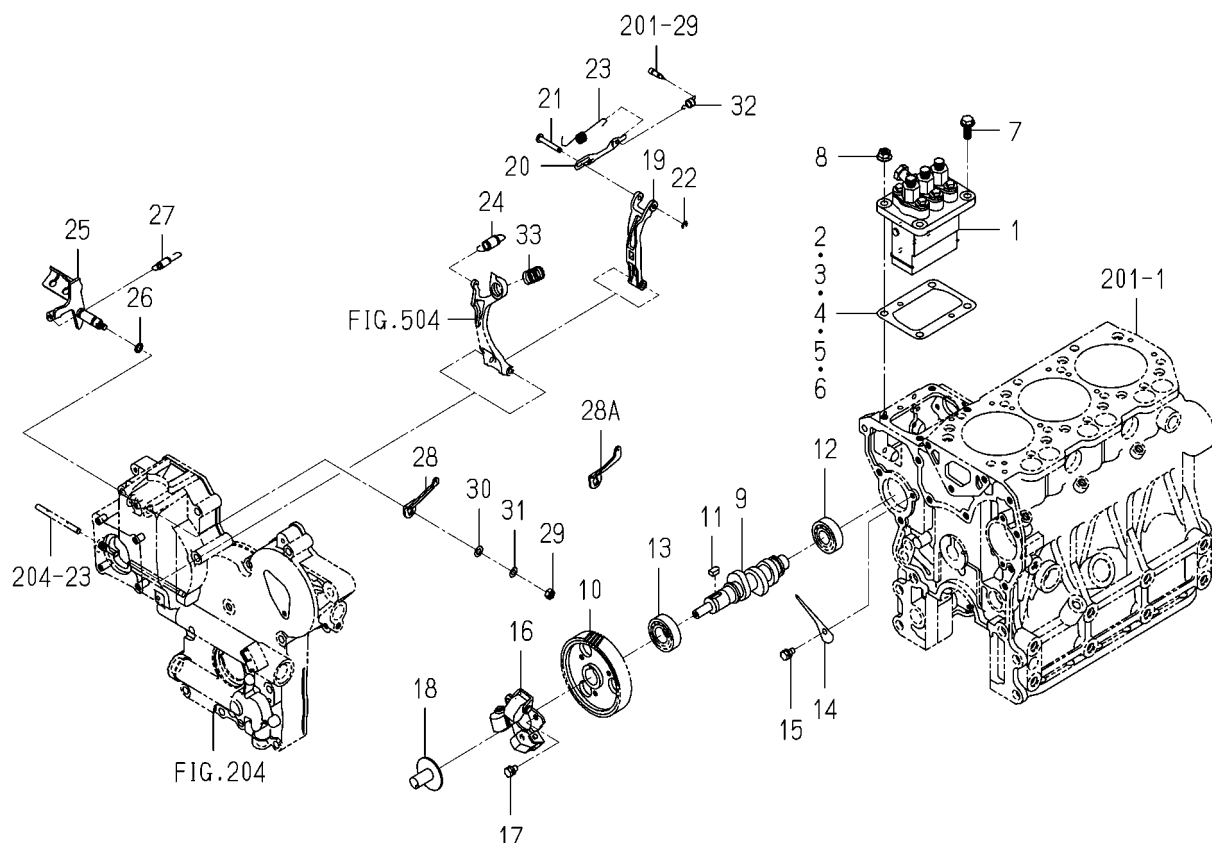
FIG.502 INJECTION PUMP
