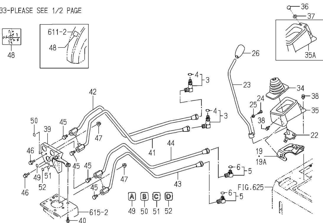
FIG.P17 JOY STICK VALVE SET(2/2) (OPTION)(TG5475)
