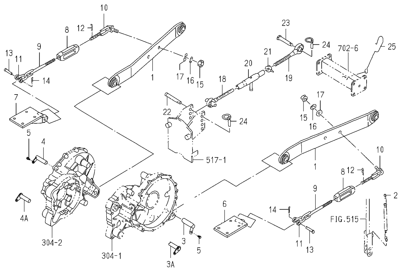
FIG.512 3P LINK SYSTEM(TG5475-R TYPE)
