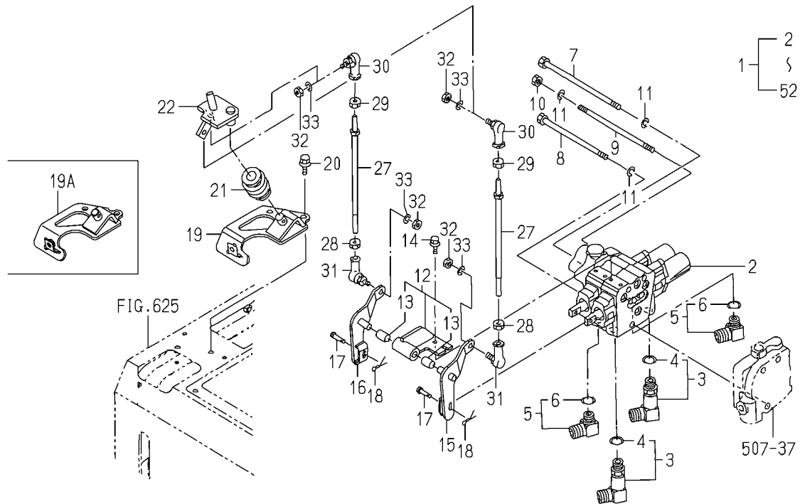
FIG.P17 JOY STICK VALVE SET(1/2) (OPTION)(TG5475)
