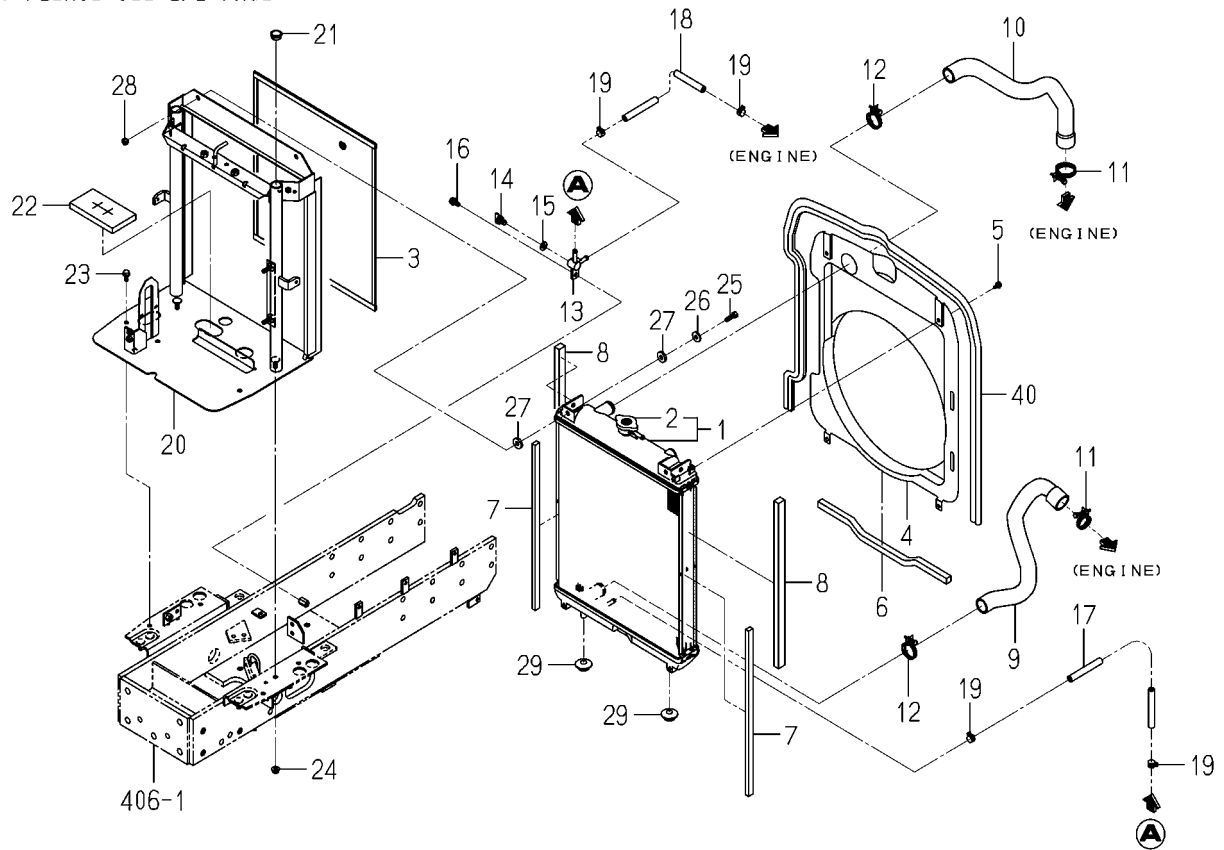
FIG.101 RADIATOR SYSTEM(TG5395)(1/2)
