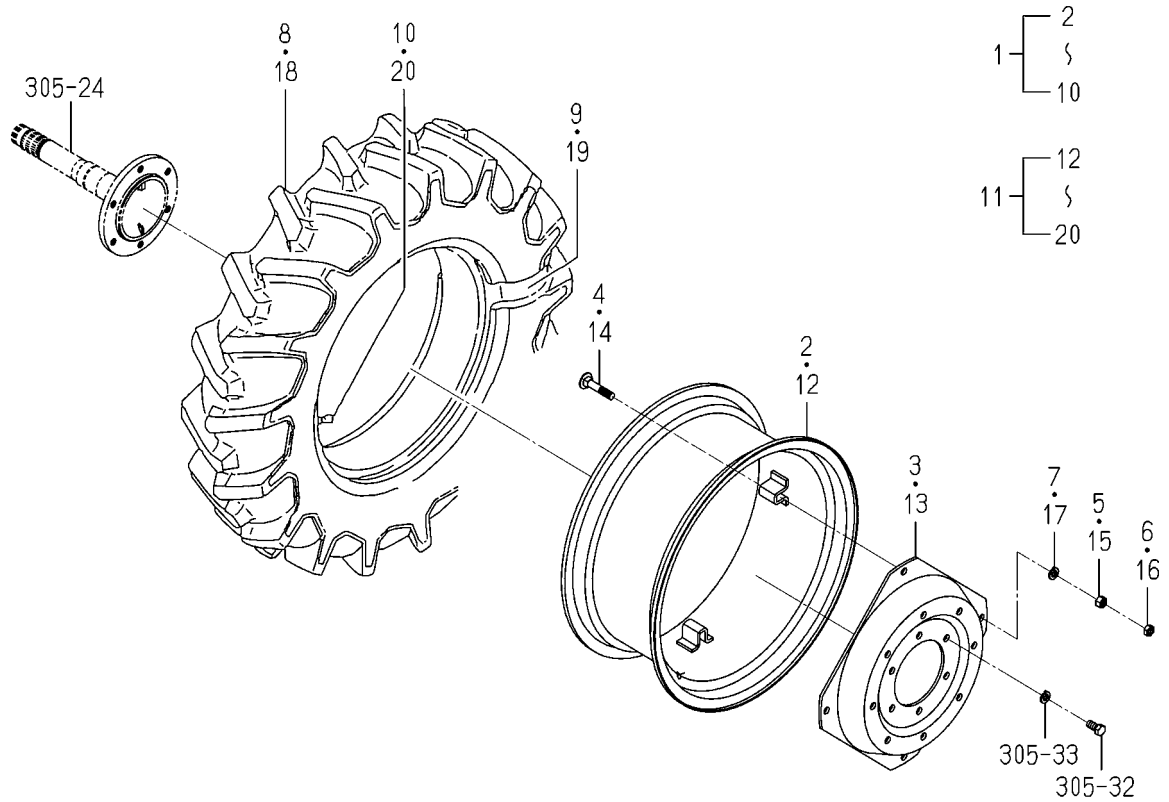
FIG.P03 REAR WHEEL(OPTION)SYSTEM
