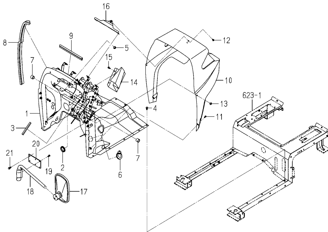
FIG.620 FLOOR(FRONT)SYSTEM(TG5395-R TYPE)
