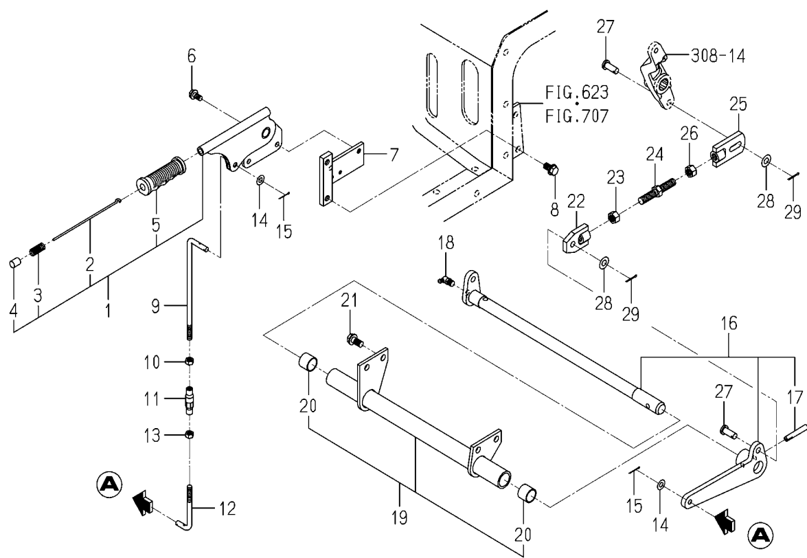
FIG.312 BRAKE(PARKING)SYSTEM(TG5395)
