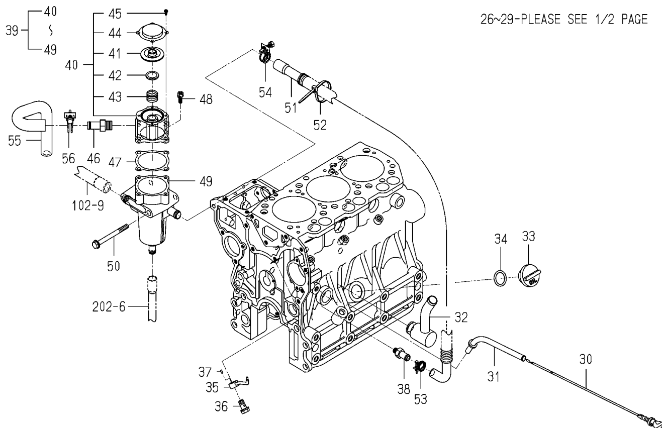
FIG.201 CYLINDER BLOCK(2/2)
