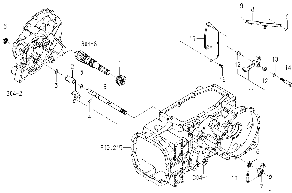
FIG.307 DIFF-LOCK(HST) SYSTEM(TG5475)
