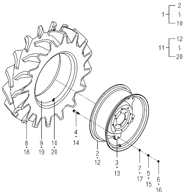
FIG.P01 REAR WHEEL SYSTEM(OPTION)(TG5475)
