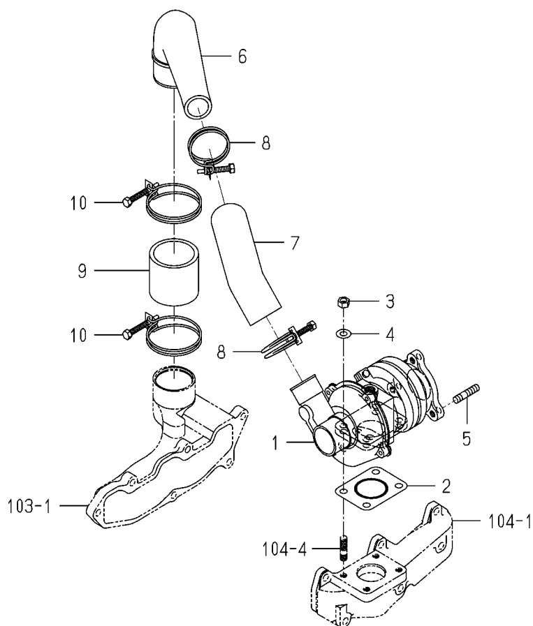
FIG.105 TURBO CHARGER
