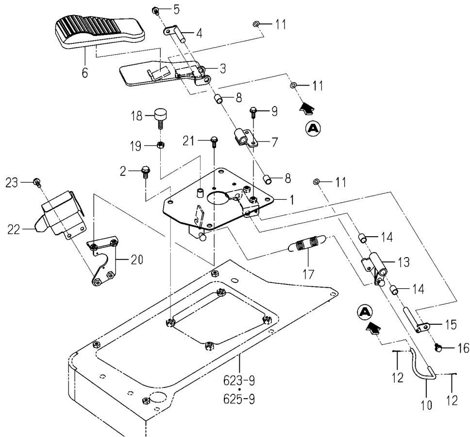
FIG.111 PEDAL(HST)SYSTEM
