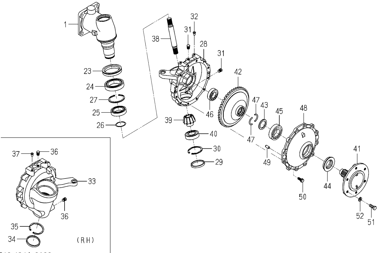
FIG.415 CASE(GEAR/FRONT)SYSTEM(TG5395)(2/2)
