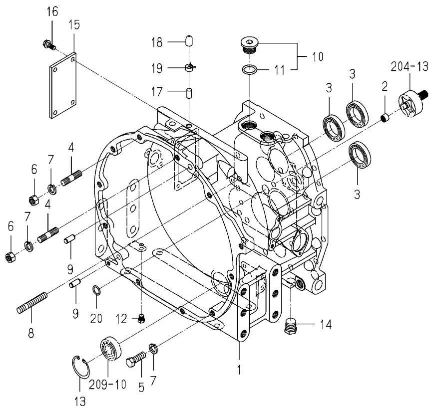
FIG.201 CASE(TRANSMISSION/FRONT)SYSTEM (TG5395)
