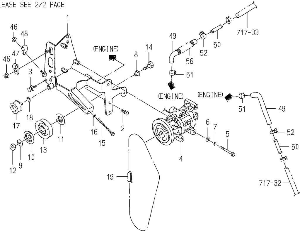
FIG.715 AIR CODITIONER(ENGINE)SYSTEM(1/2) (TG5475-C TYPE)
