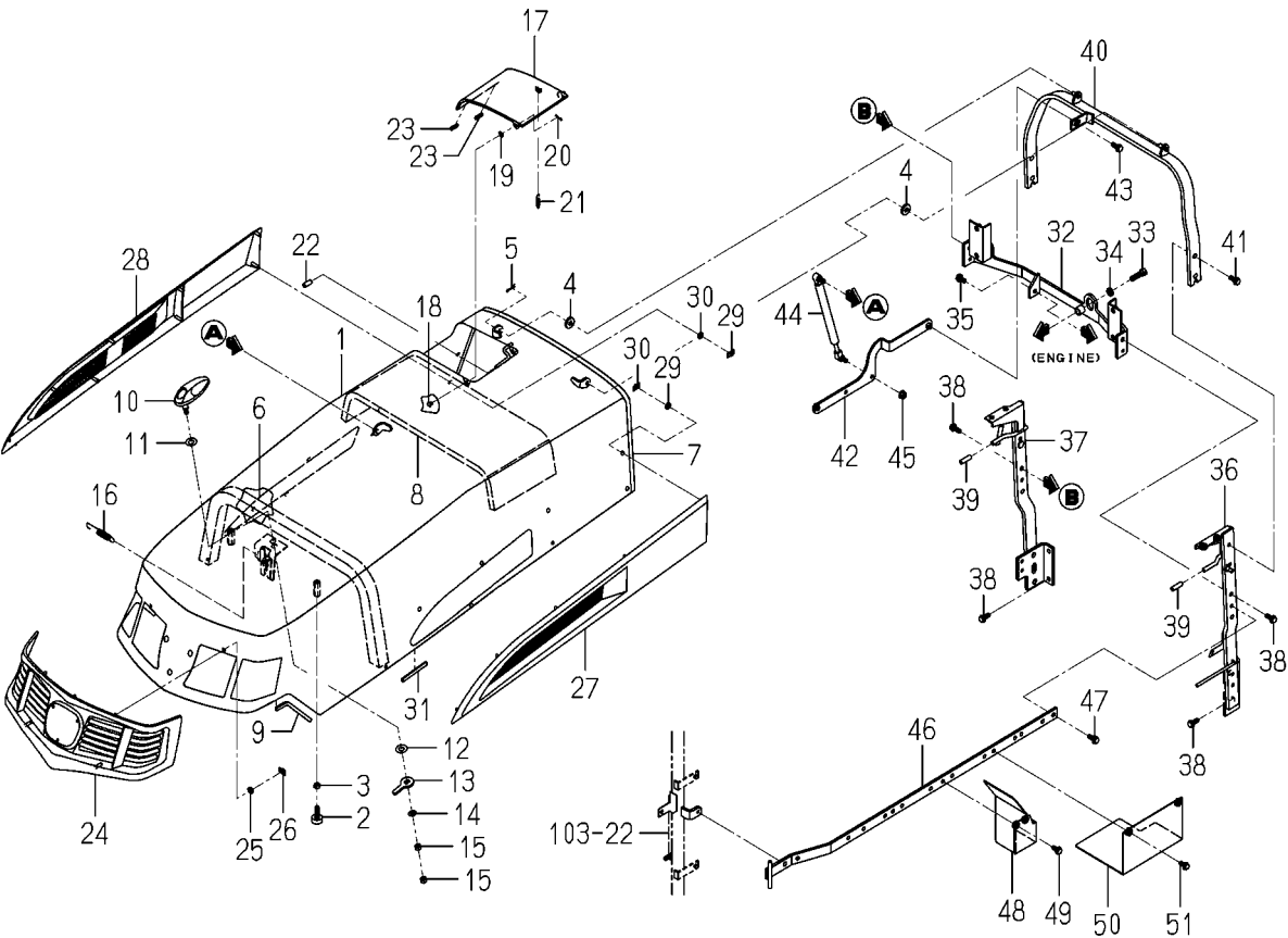
FIG.603 HOOD SYSTEM(TG5475-C TYPE)
