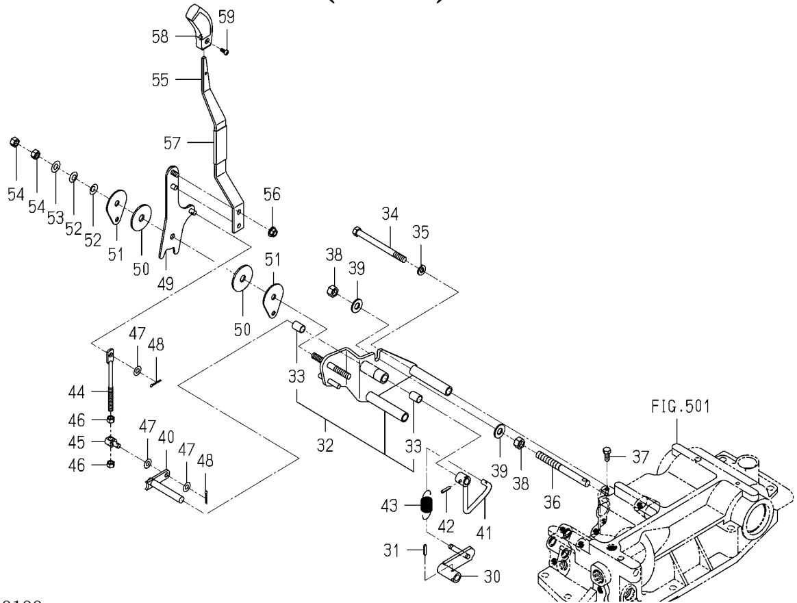
FIG.503 MECHANICAL LINK(POSITION)SYSTEM(2/2) (TG5395)
