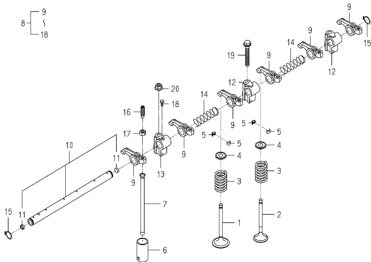
FIG.301 VALVE
