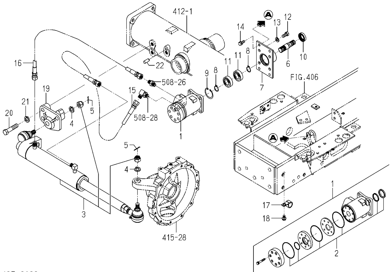
FIG.404 STEERING(POWER)SYSTEM(TG5395)
