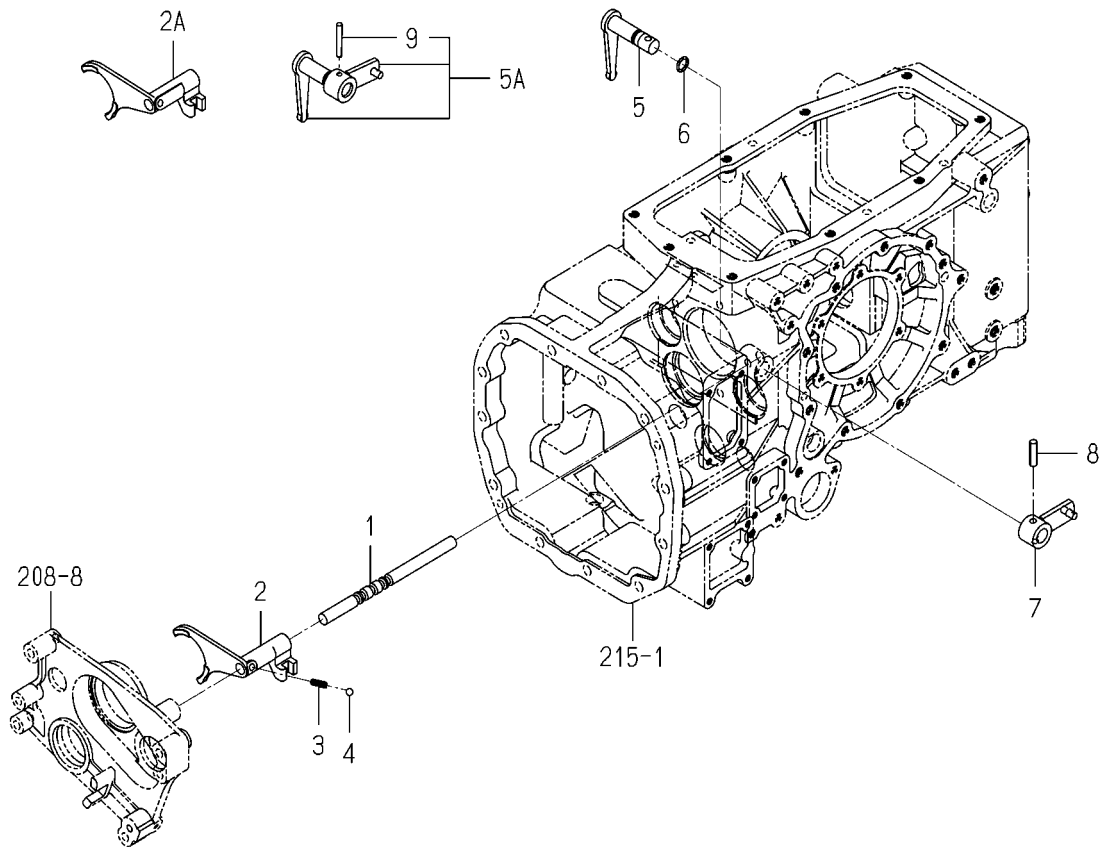
FIG.216 FORK(SHIFT/SUB)SYSTEM
