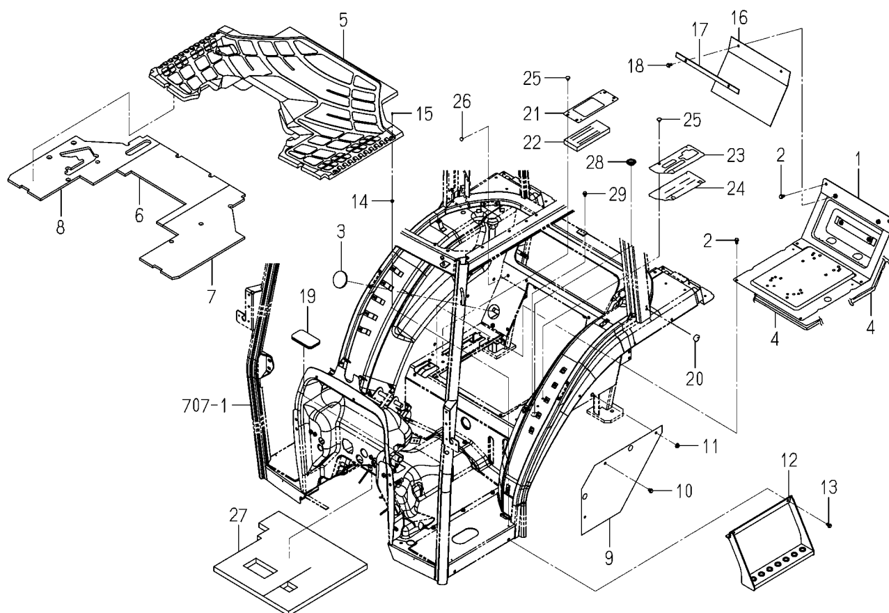
FIG.626 FLOOR(REAR)SYSTEM(TG5475-C TYPE)
