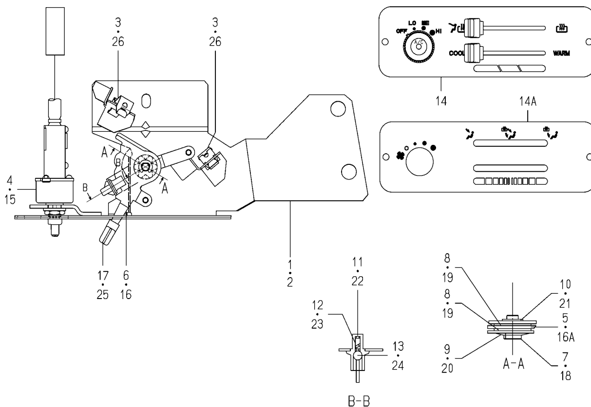
FIG.S15 COMPONENT PARTS FOR 1746-781-220-10 ON Fig.716
