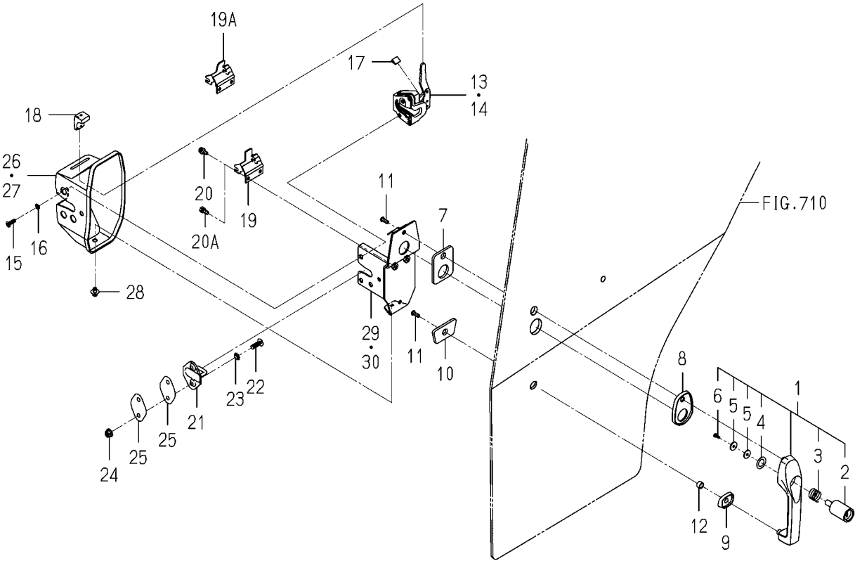
FIG.711 LOCK(DOOR)SYSTEM(C TYPE)
