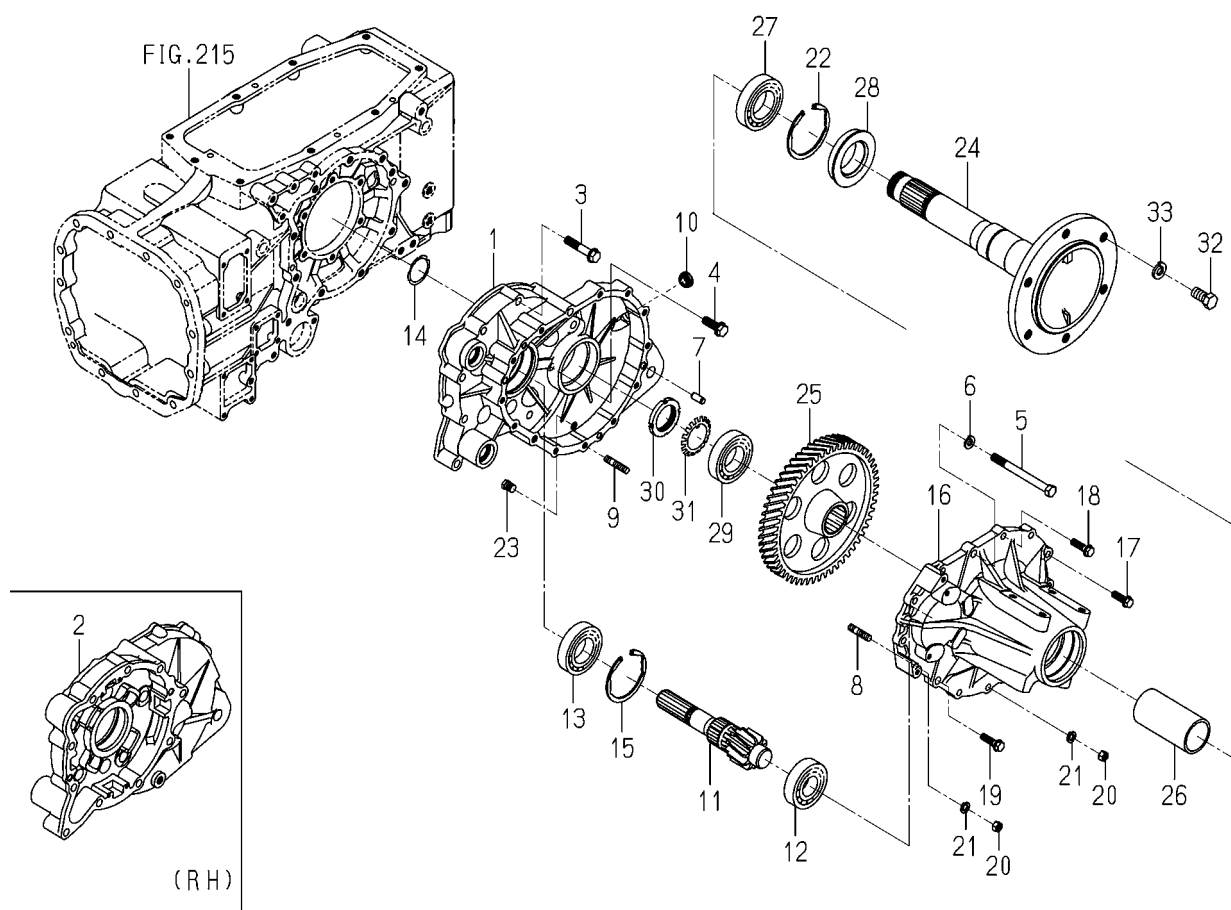
FIG.305 HOUSING(AXLE)SYSTEM(TG5395)
