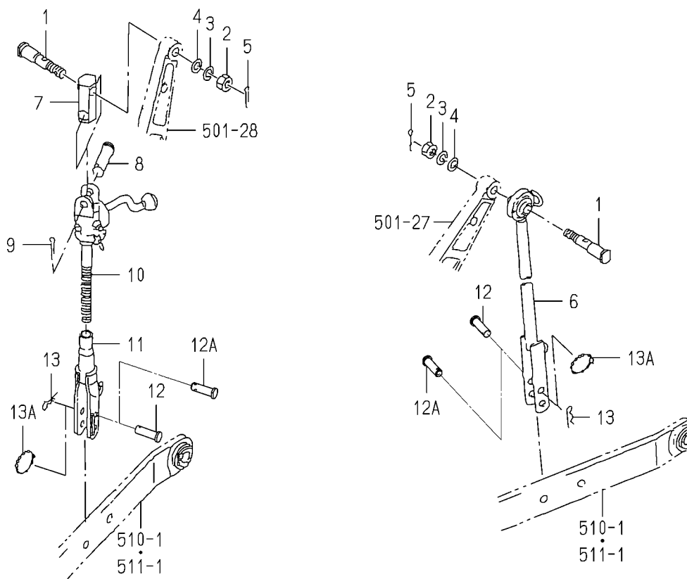
FIG.514 LIFT ROD(BEVEL)SYSTEM(TG5395)
