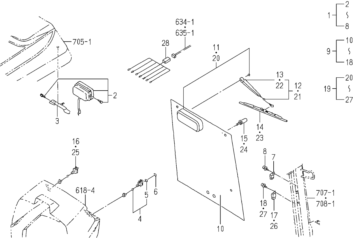
FIG.P22 ELC.SYSTEM(CABIN)SET(OPTION)(C TYPE)
