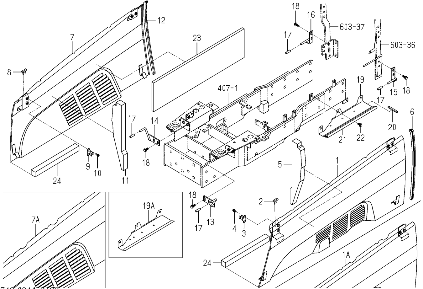
FIG.608 COVER(SIDE)SYSTEM(TG5475-C TYPE)
