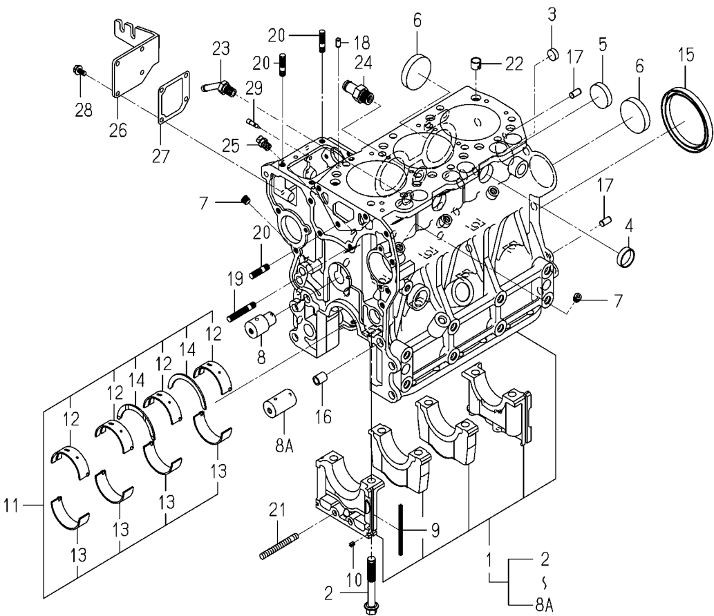
FIG.201 CYLINDER BLOCK(1/2)
