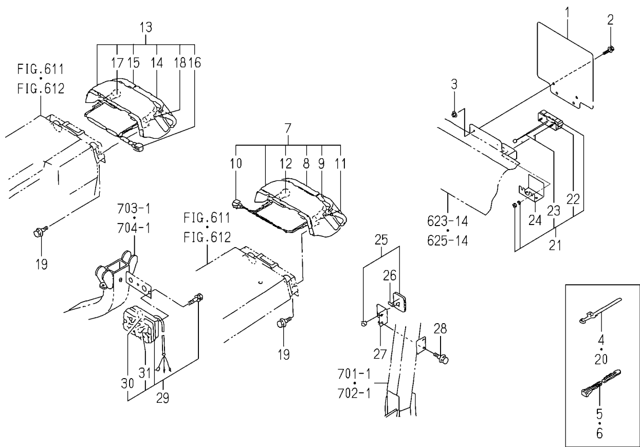
FIG.631 ELC.SYSTEM(REAR)(R TYPE)
