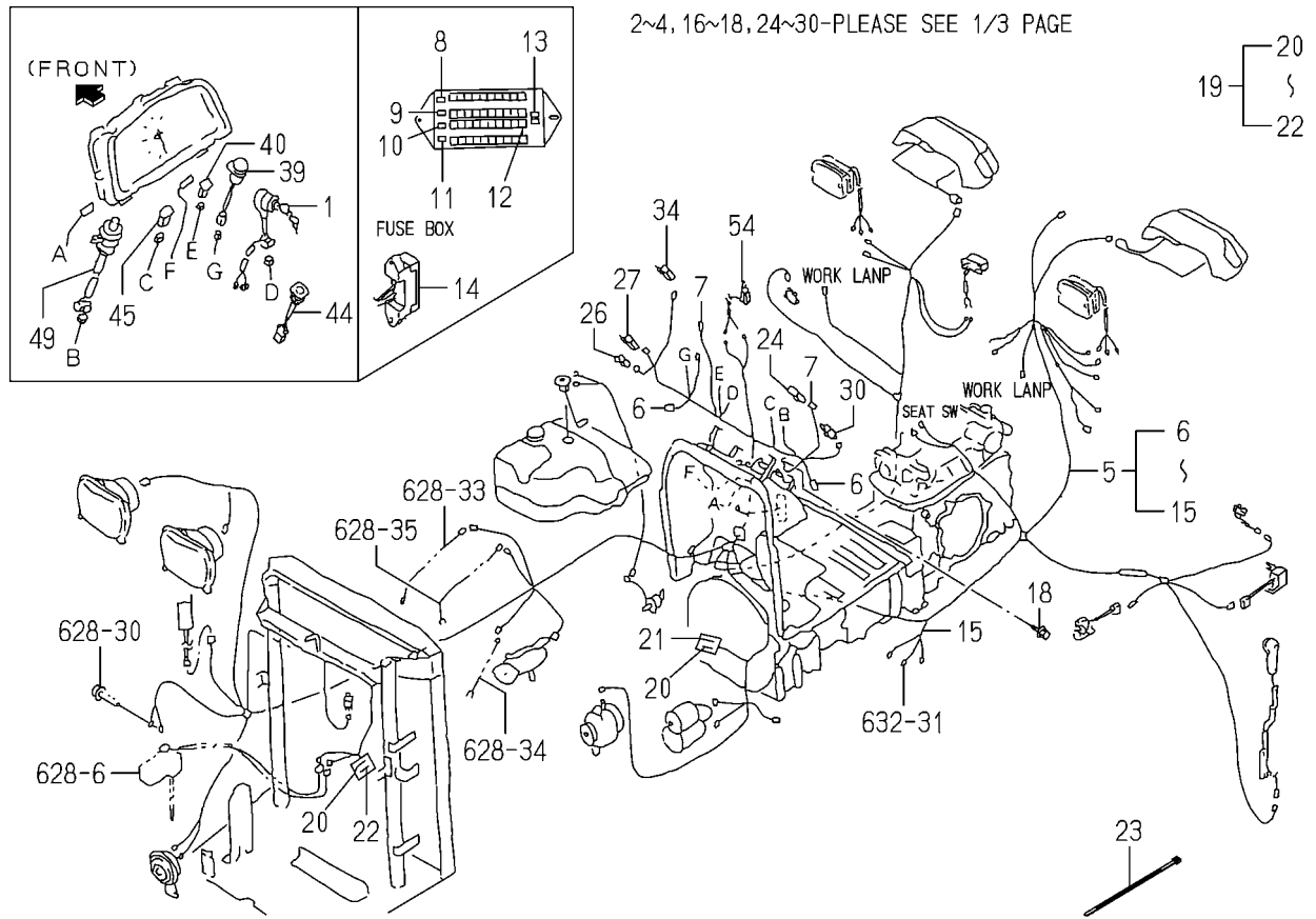
FIG.630 ELC.SYSTEM(MAIN)(TG5475)(1/3)
