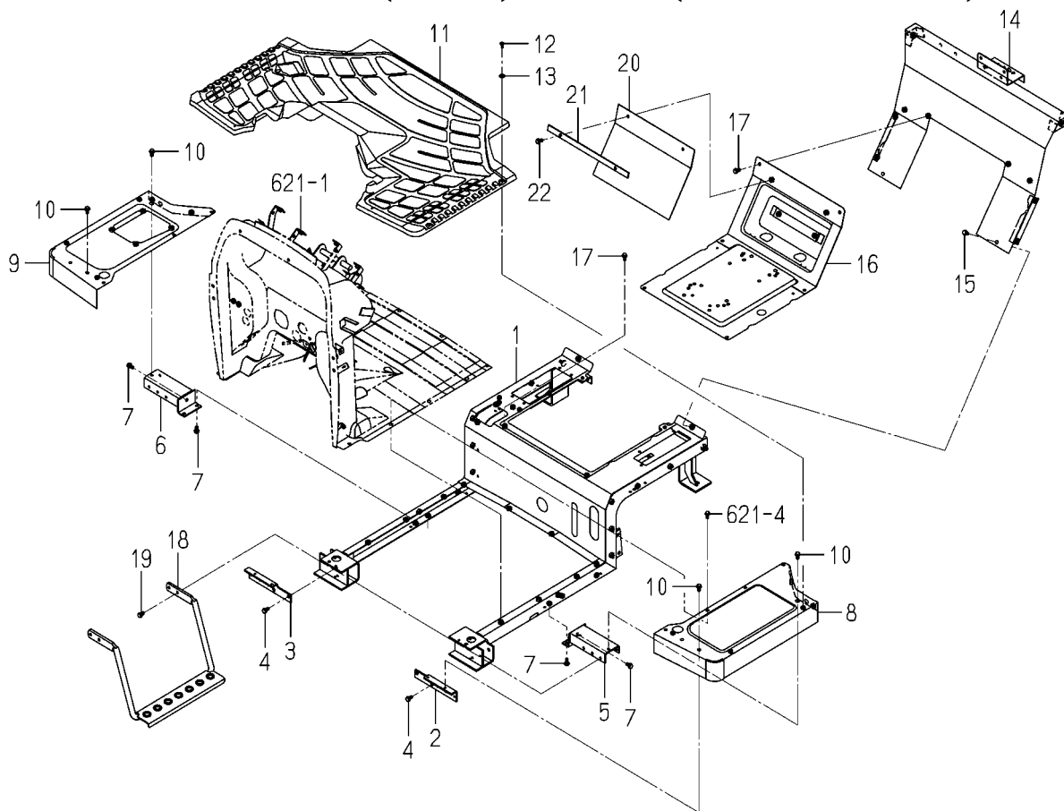
FIG.625 FLOOR(REAR)SYSTEM(TG5475-R TYPE)
