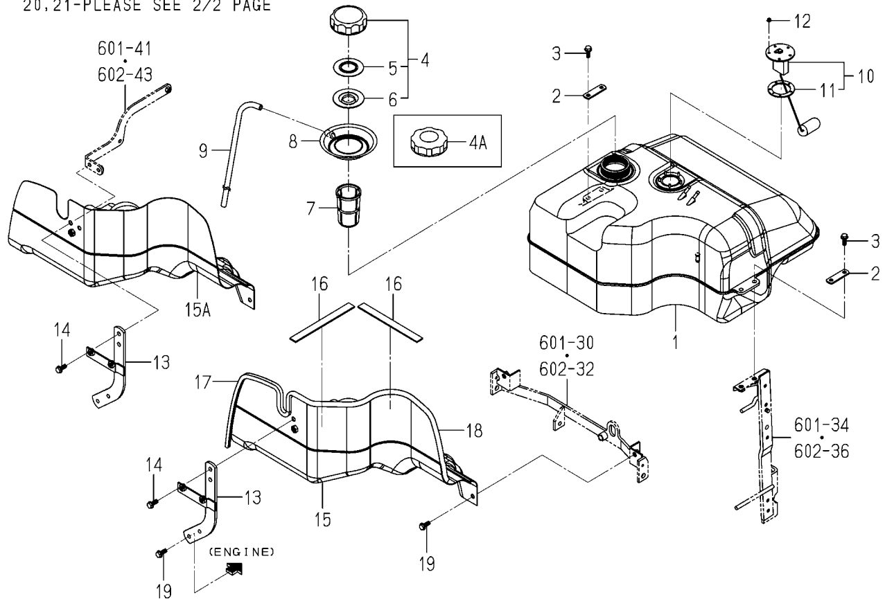
FIG.108 TANK SYSTEM(TG5395 TYPE)(1/2)
