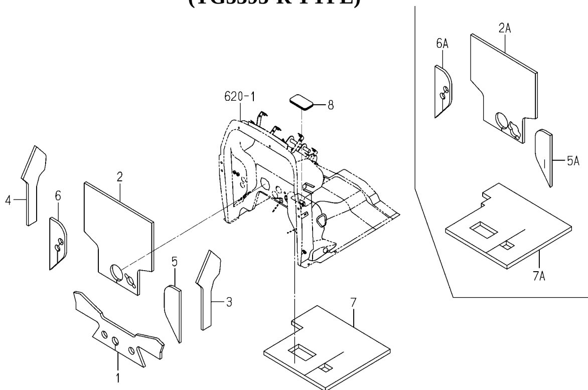
FIG.619 INSULATOR(FLOOR)SYSTEM (TG5395-R TYPE)
