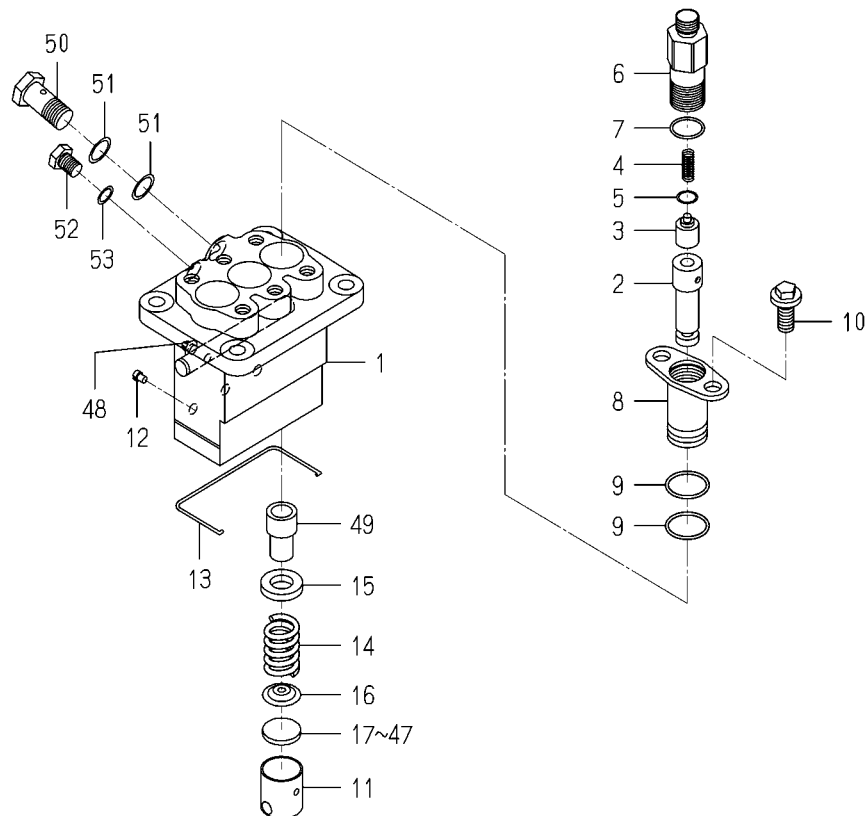
FIG.S02 COMPONENT PARTS FOR 6215-600-078-10 ON Fig.502
