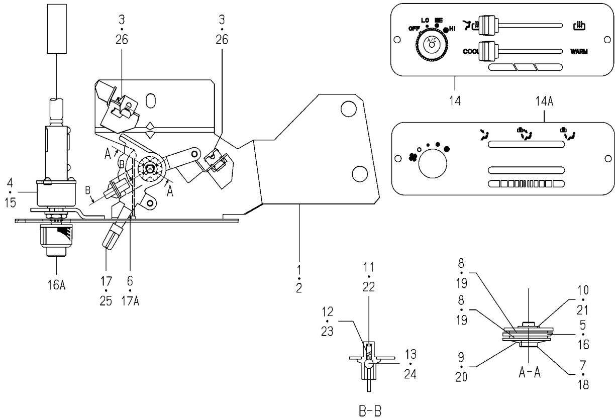
FIG.S11 COMPONENT PARTS FOR 1729-782-610-20 ON Fig.717
