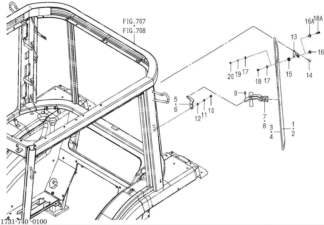
FIG.712 GLASS(SIDE)SYSTEM(C TYPE)
