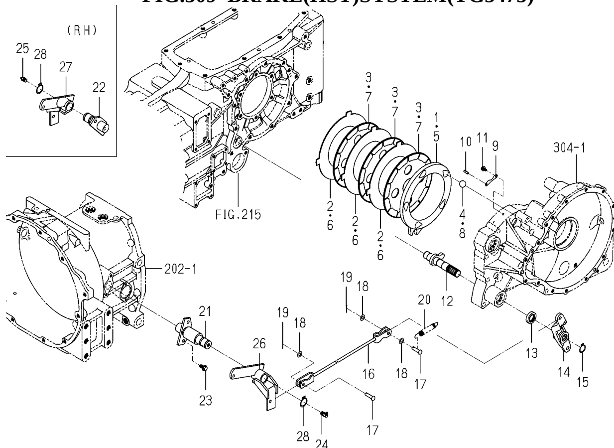
FIG.309 BRAKE(HST)SYSTEM(TG5475)
