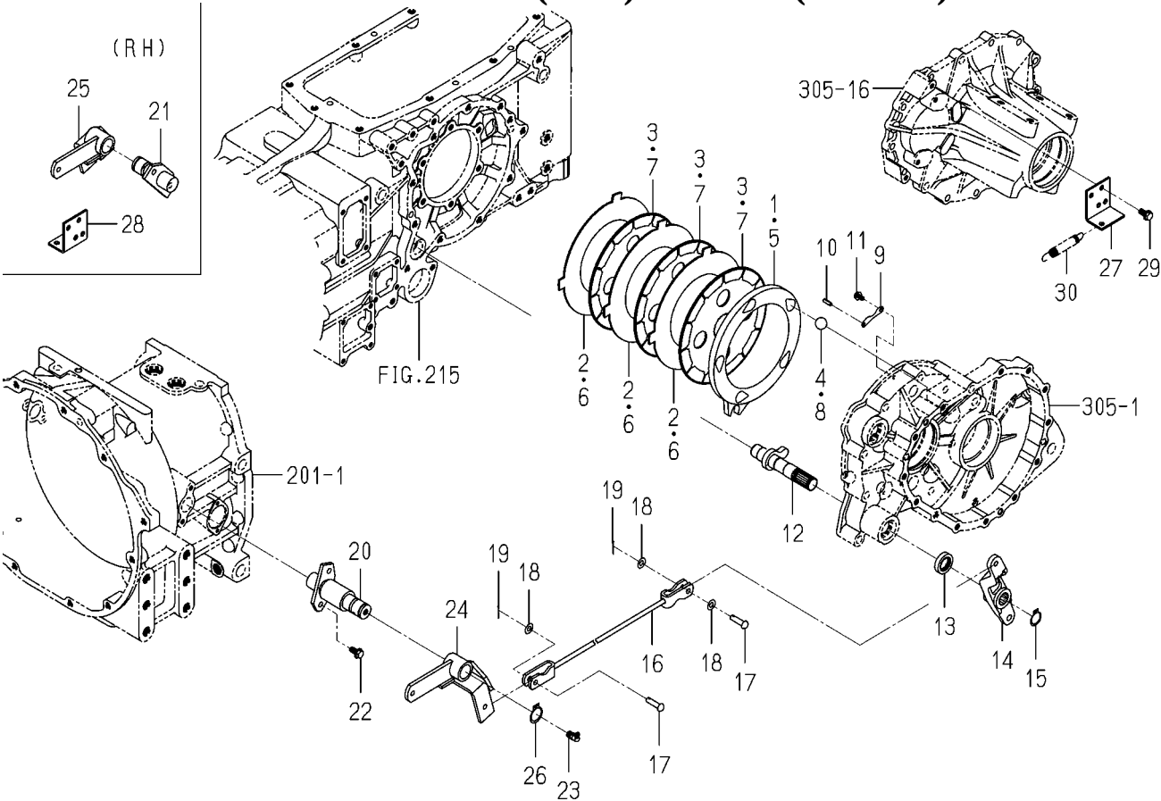
FIG.308 BRAKE(HST)SYSTEM(TG5395)
