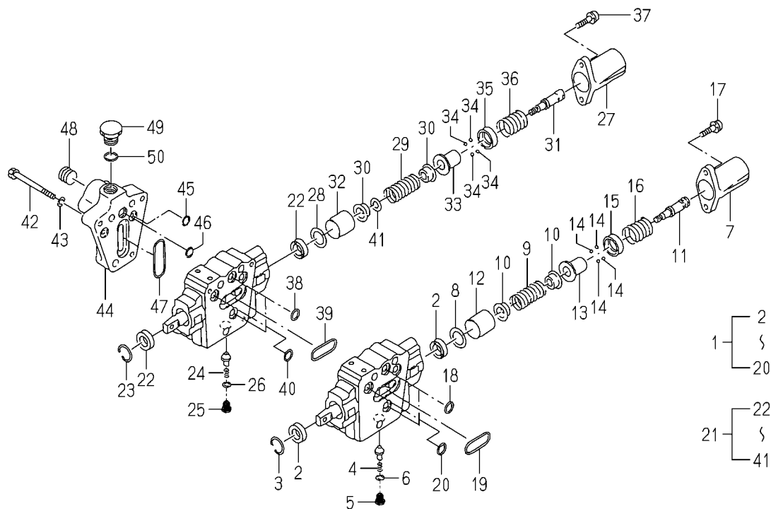
FIG.S04 COMPONENT PARTS FOR K211-074-000-20 ON Fig.P16,17
