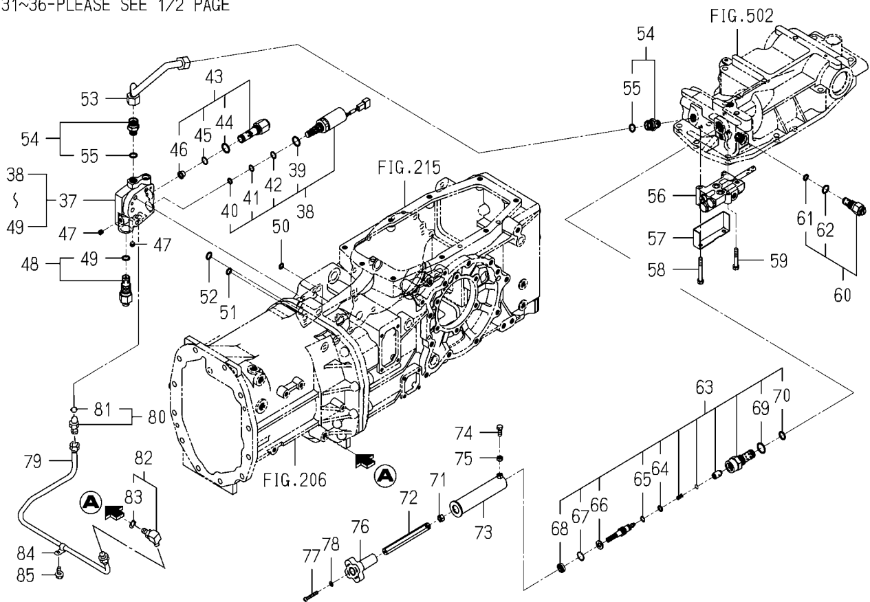
FIG.507 HYD.SYSTEM(MAIN)(TG5475)(2/2)
