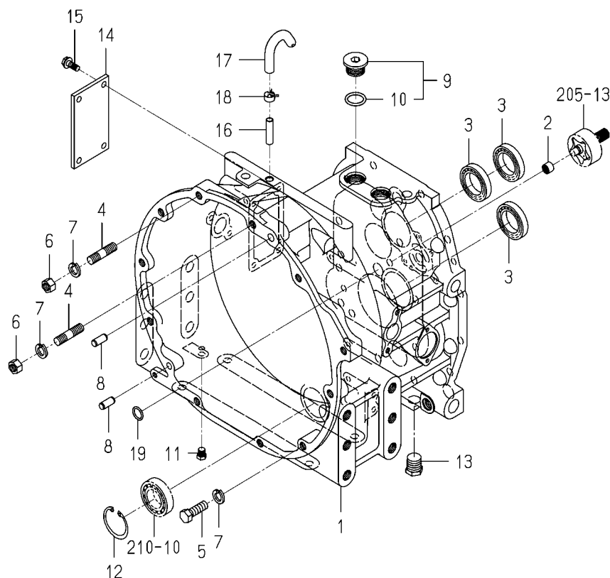
FIG.202 CASE(TRANSMISSION/FRONT)SYSTEM (TG5475)
