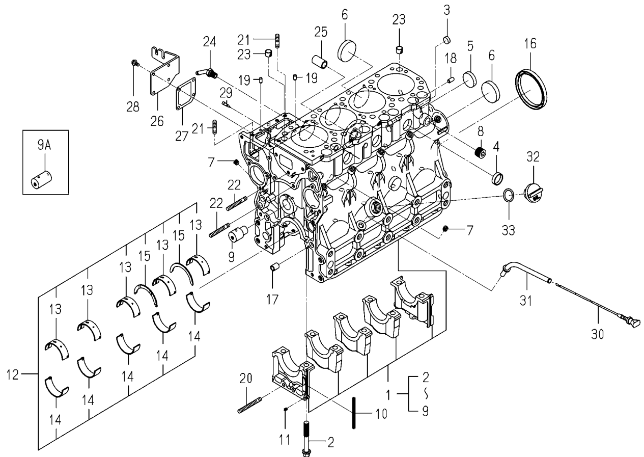
FIG.201 CYLINDER BLOCK
