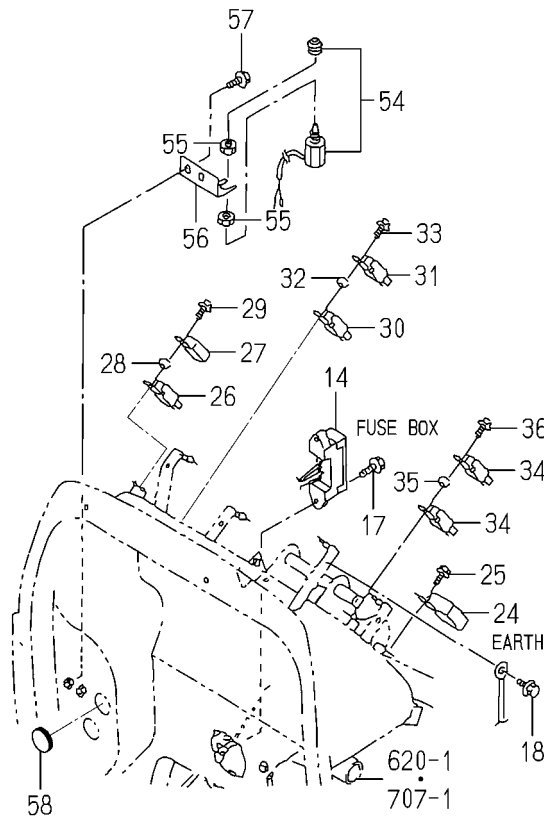
FIG.629 ELC.SYSTEM(MAIN)(TG5395)(2/3)
