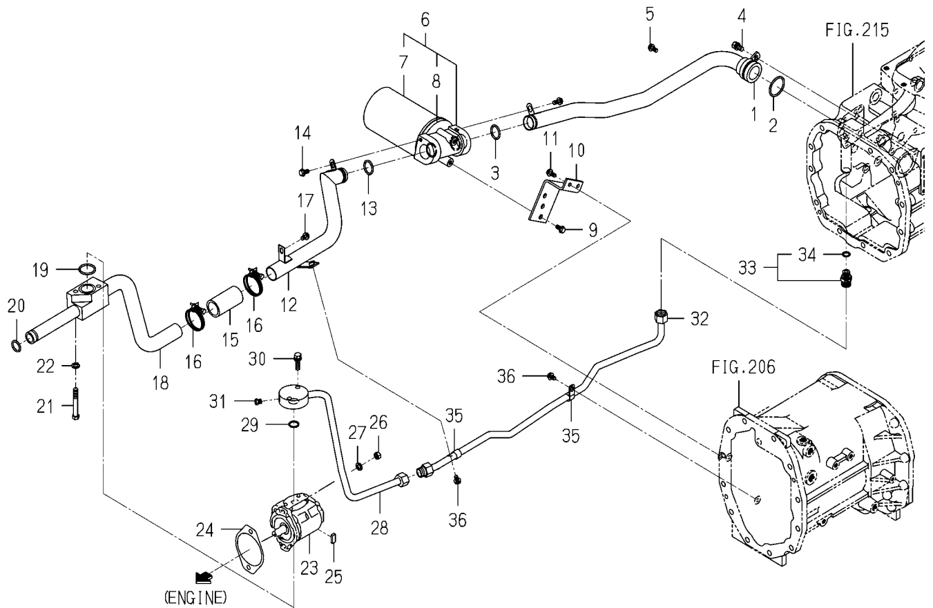
FIG.507 HYD.SYSTEM(MAIN)(TG5475)(1/2)
