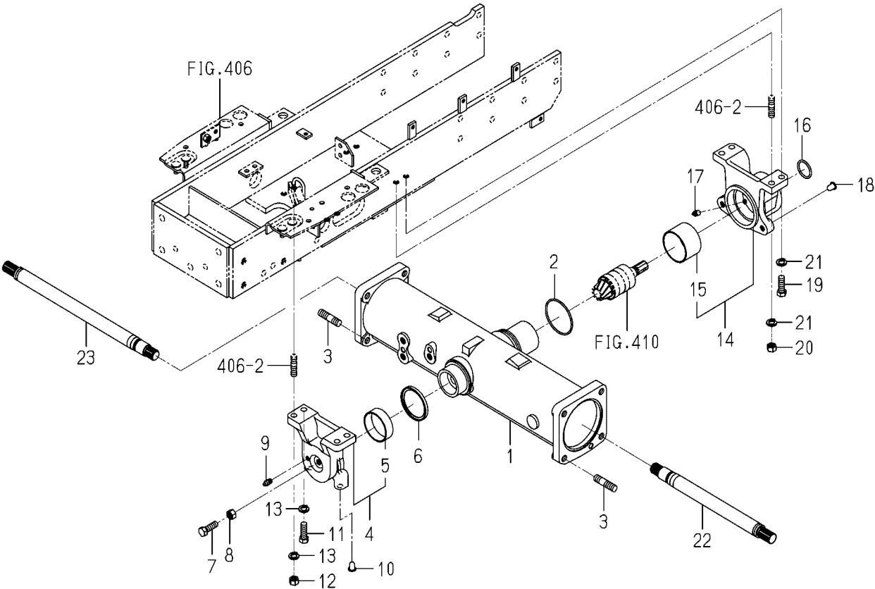
FIG.412 HOUSING(AXLE)SYSTEM(TG5395)
