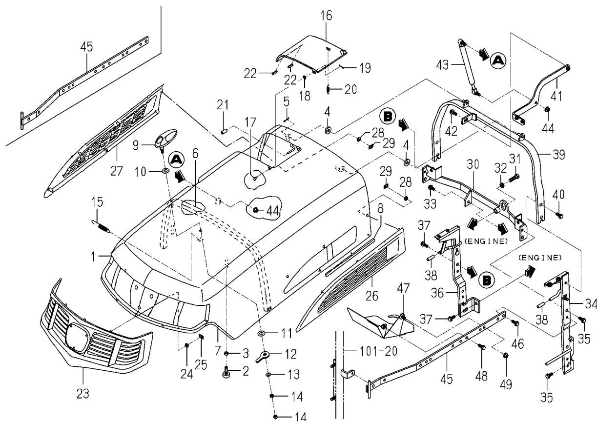
FIG.601 HOOD SYSTEM(TG5395-R TYPE)
