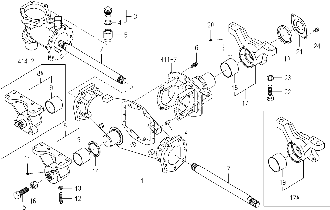
FIG.413 HOUSING(AXLE)SYSTEM(TG5475)
