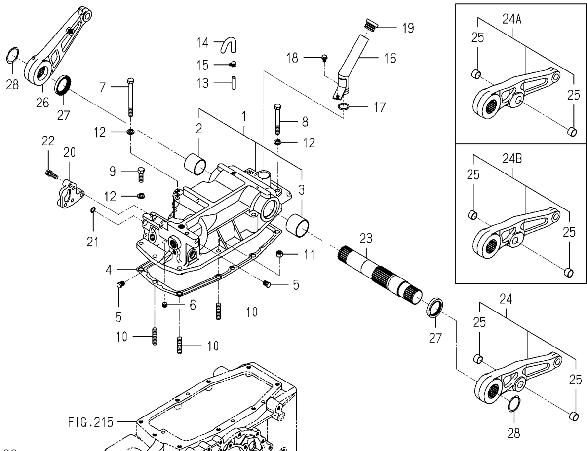
FIG.502 CYLINDER CASE SYSTEM(TG5475)(1/2)
