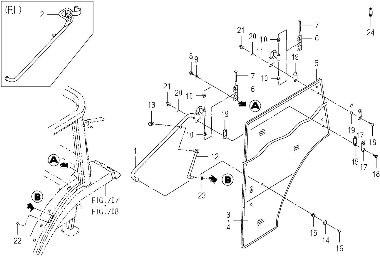
FIG.710 DOOR SYSTEM(C TYPE)
