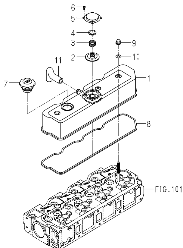
FIG.102 CYLINDER HEAD COVER
