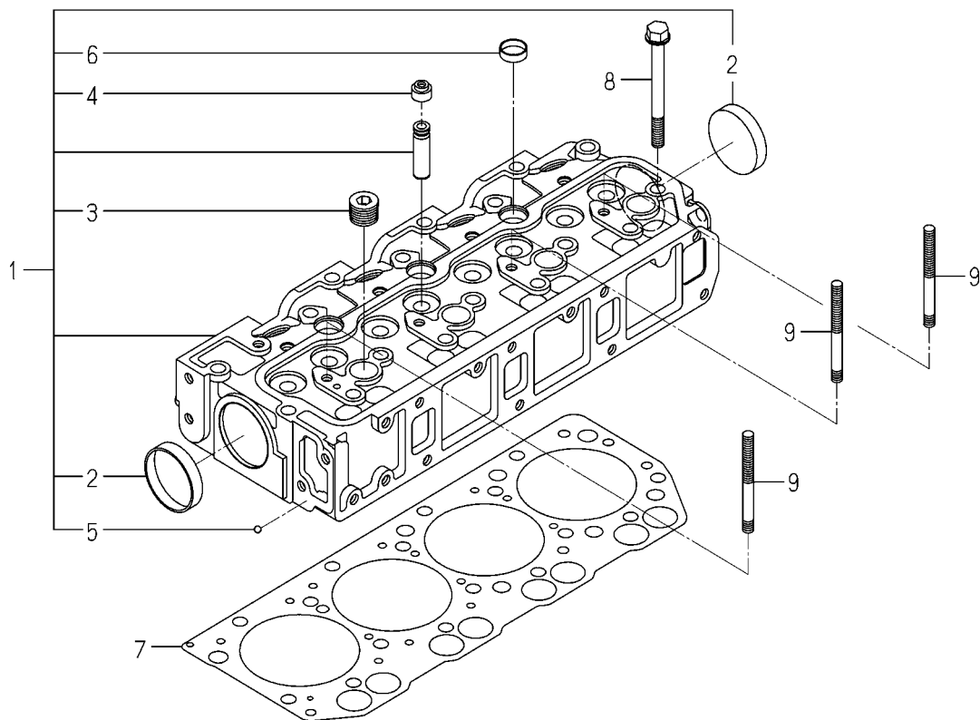
FIG.101 CYLINDER HEAD
