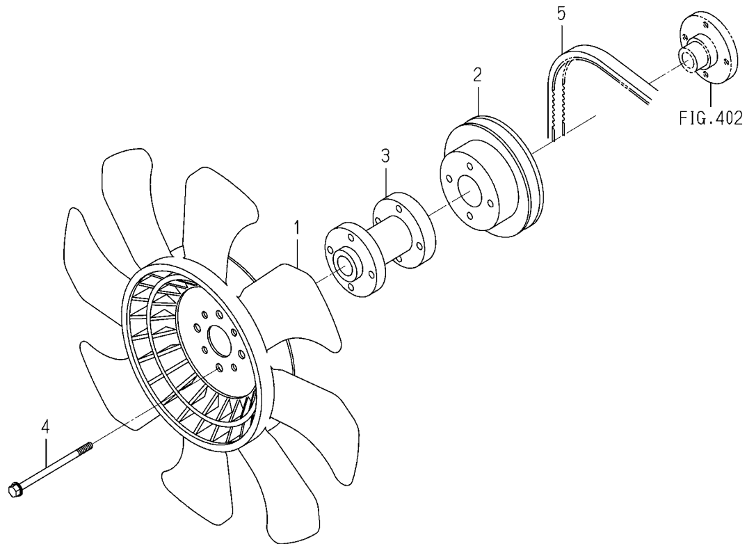
FIG.403 COOLING FAN
