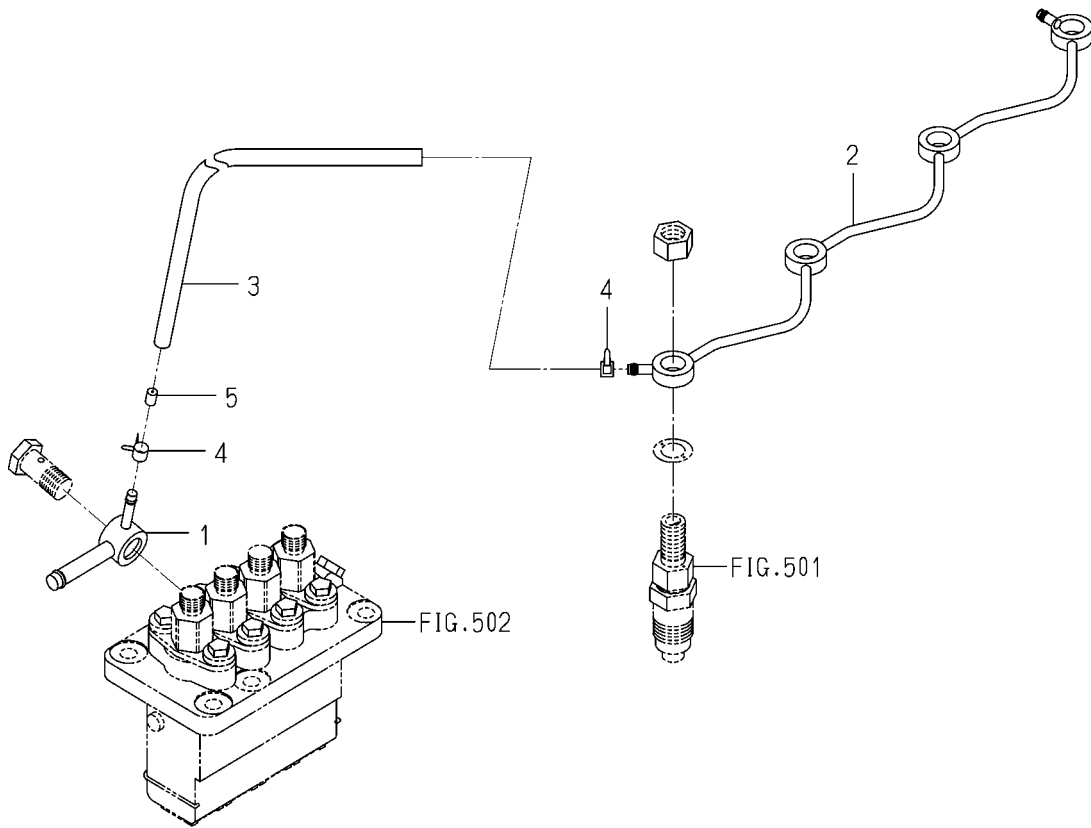
FIG.503 FUEL PIPE
