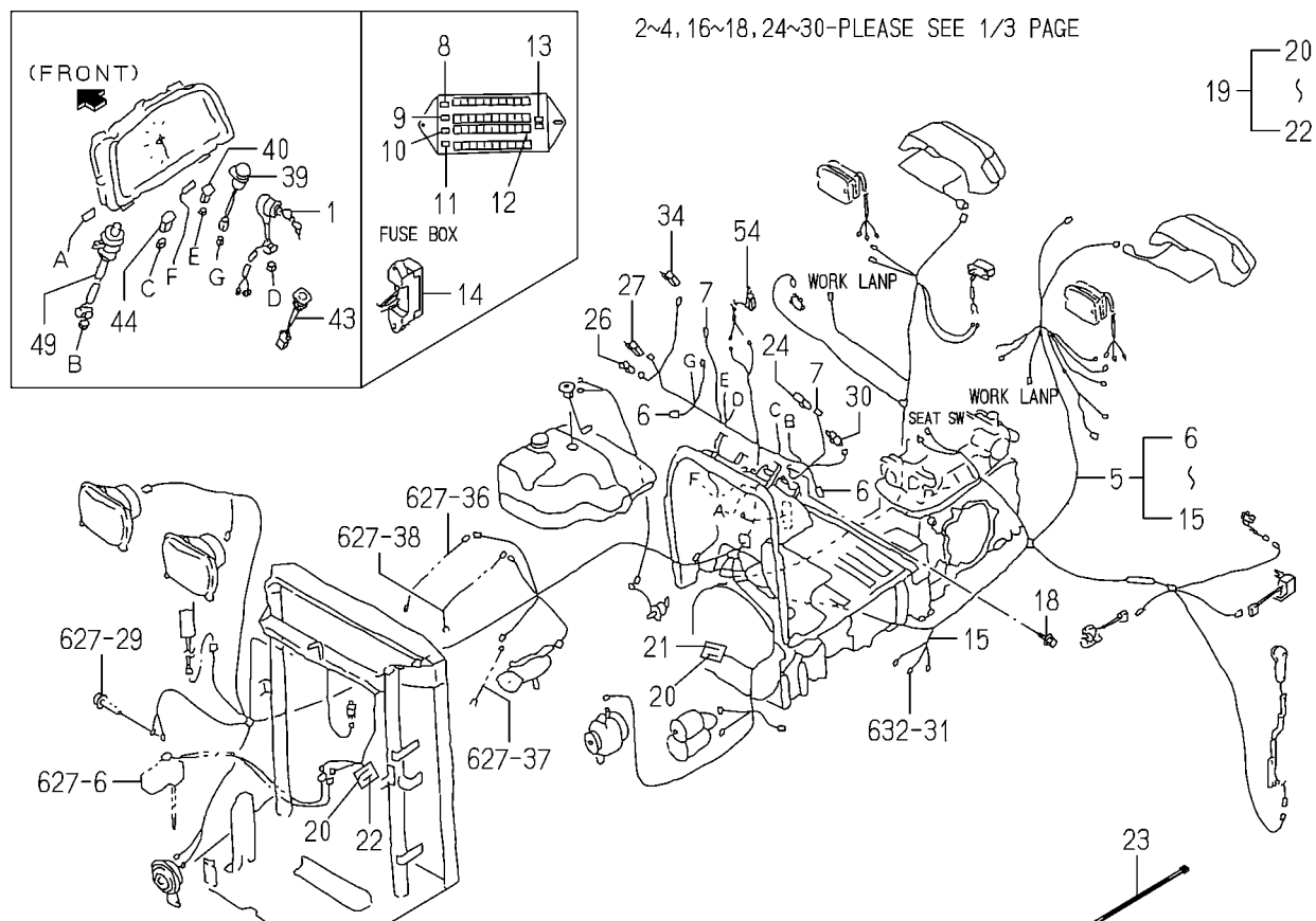
FIG.629 ELC.SYSTEM(MAIN)(TG5395)(1/3)
