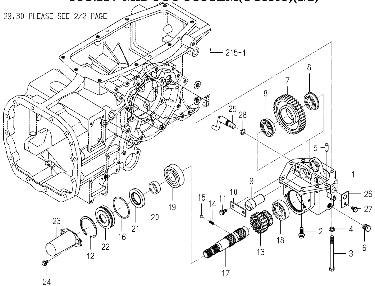
FIG.214 MID PTO SYSTEM(TG5395)(1/2)
