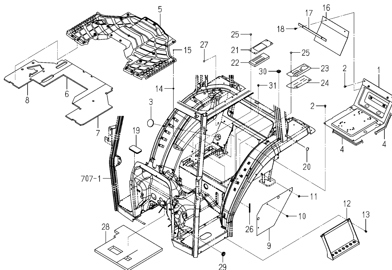
FIG.624 FLOOR(REAR)SYSTEM(TG5395-C TYPE)
