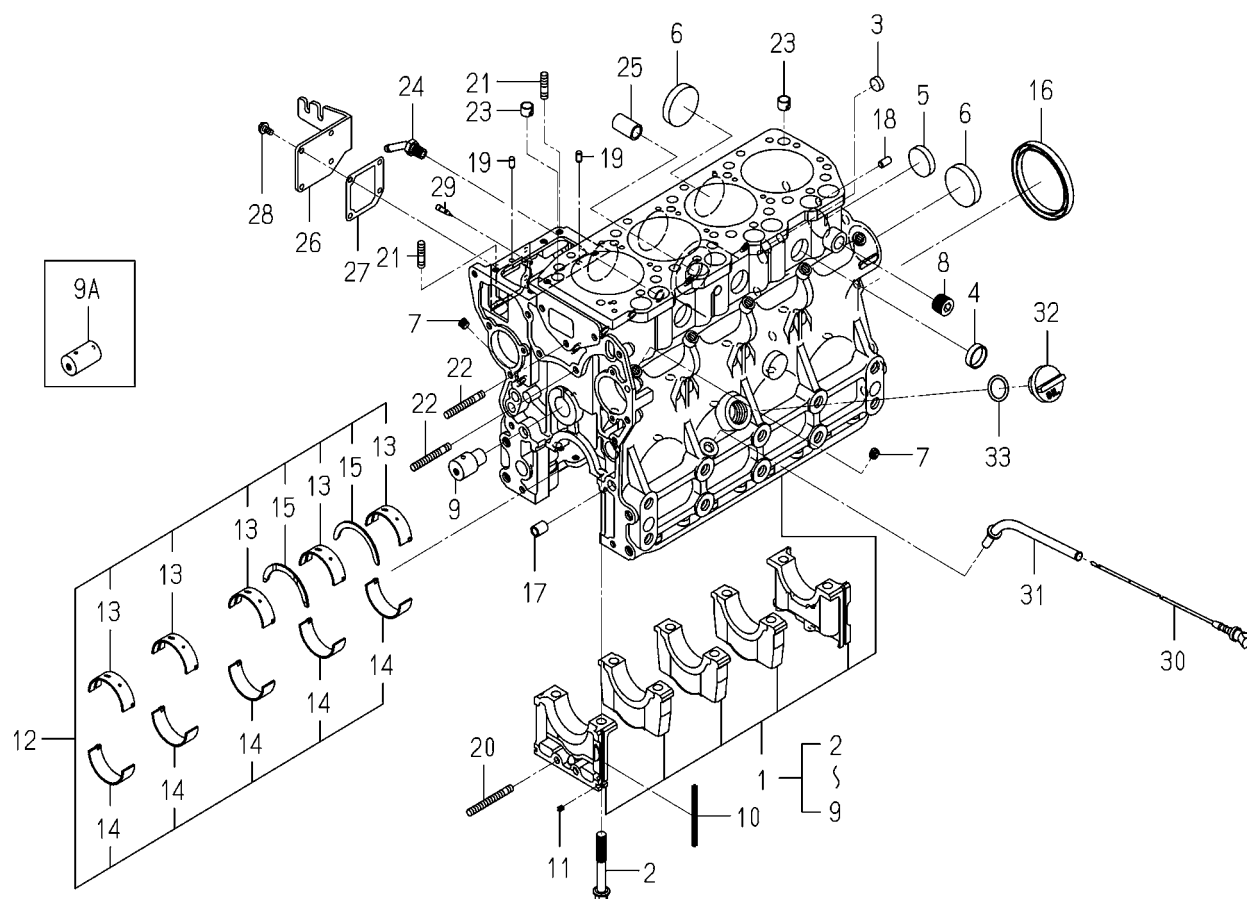
FIG.201 CYLINDER BLOCK
