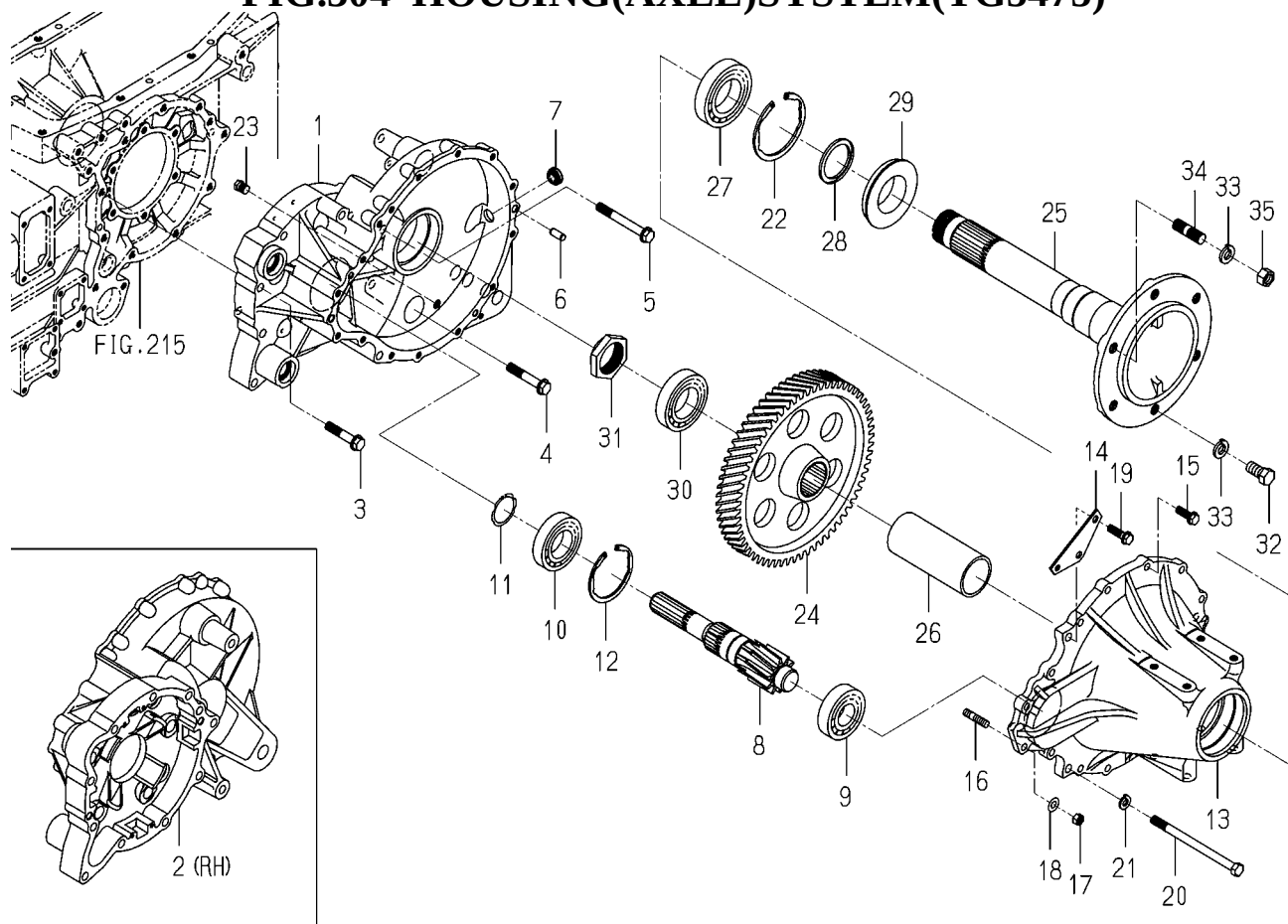
FIG.304 HOUSING(AXLE)SYSTEM(TG5475)
