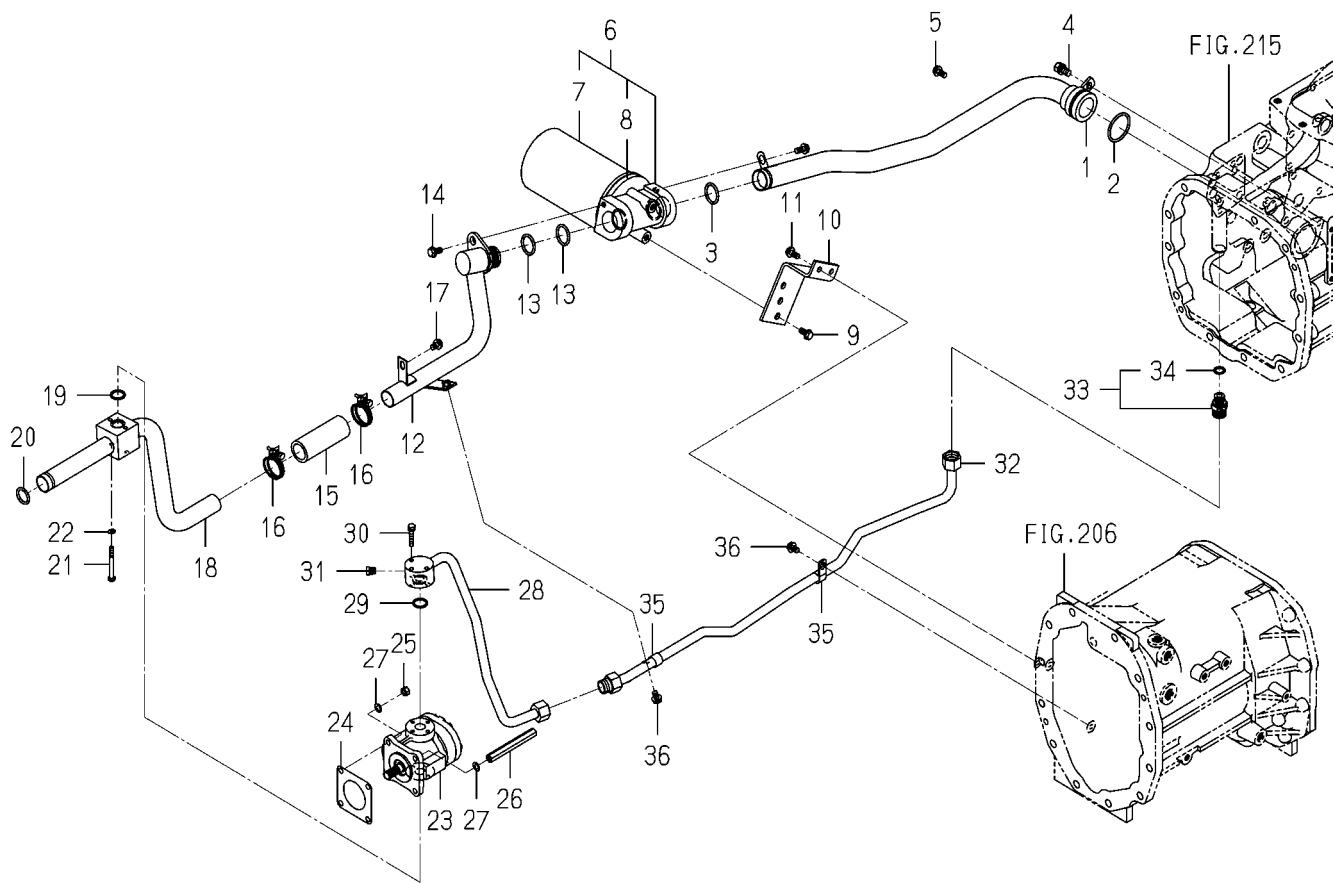
FIG.506 HYD.SYSTEM(MAIN)(TG5395)(1/2)
