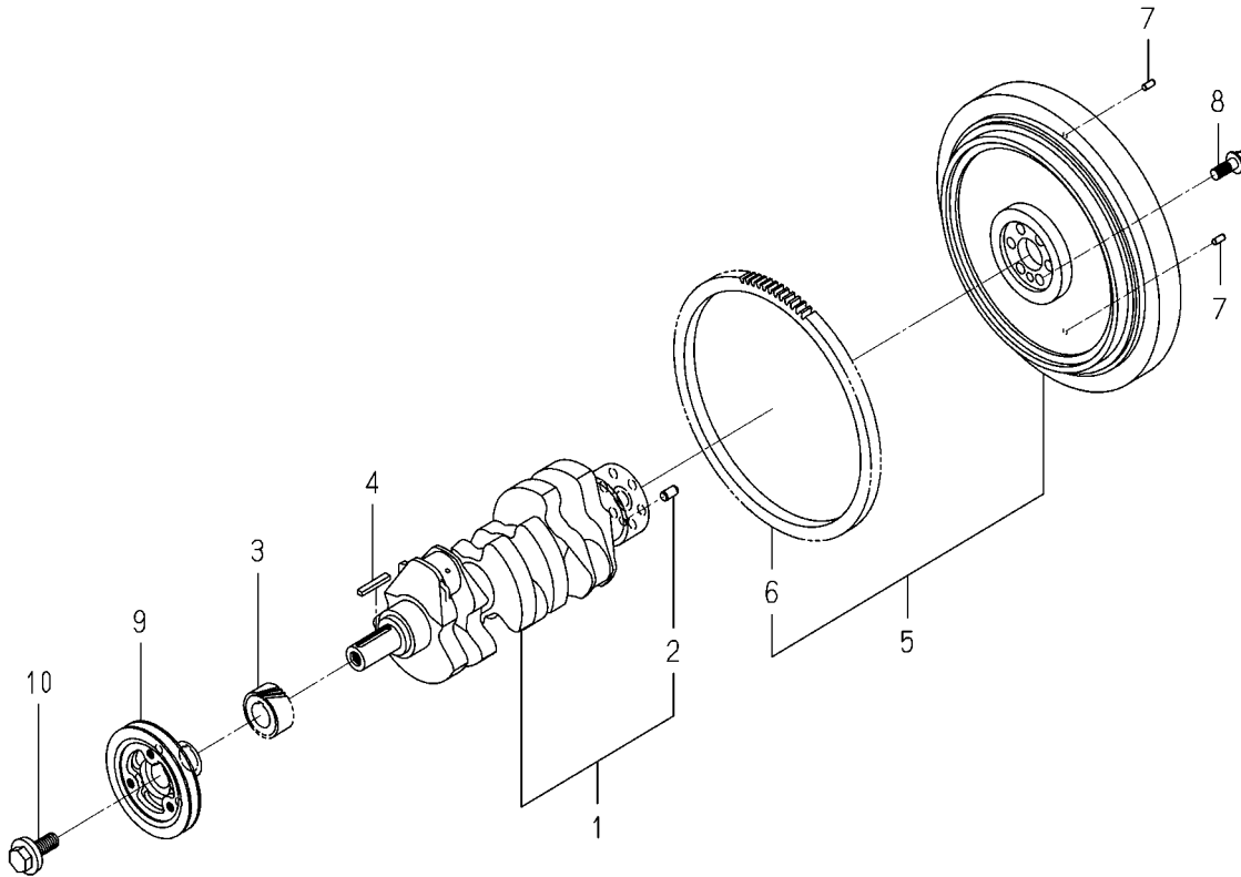
FIG.304 CRANK SHAFT
