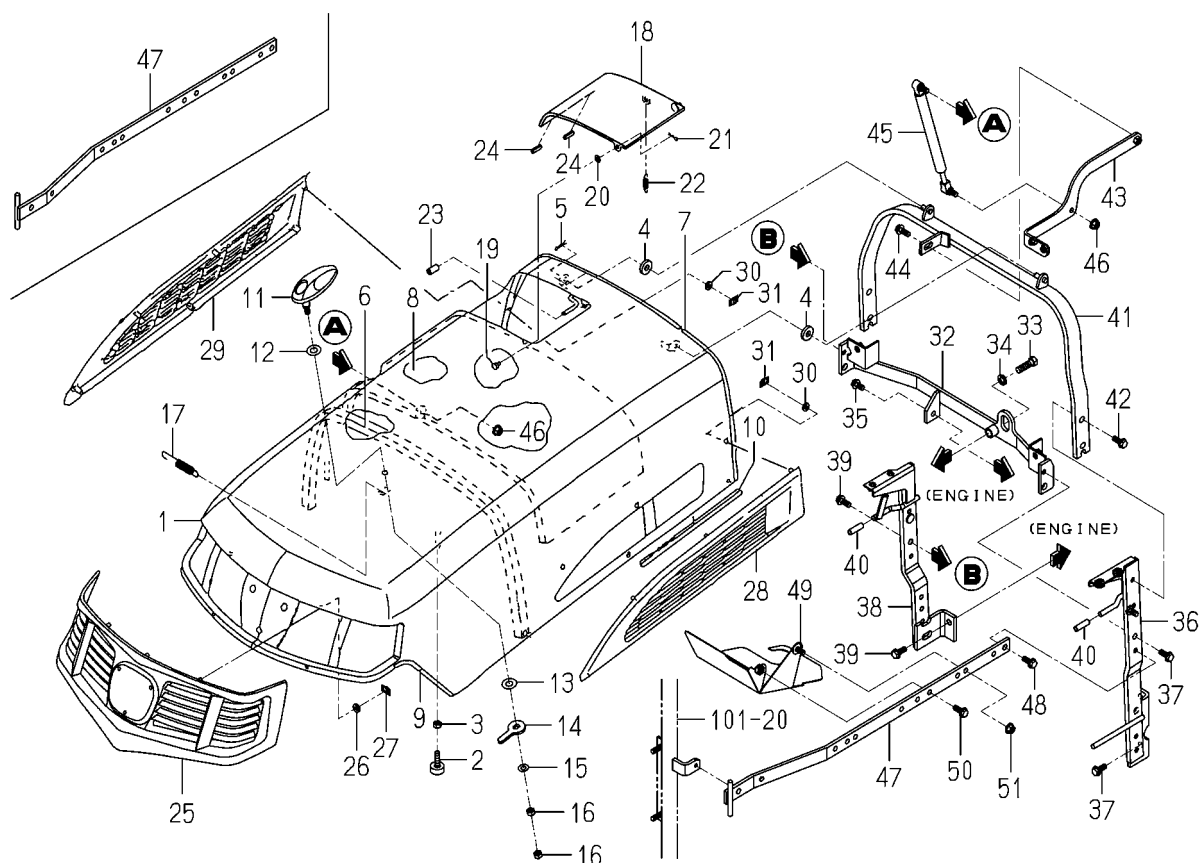
FIG.602 HOOD SYSTEM(TG5395-C TYPE)
