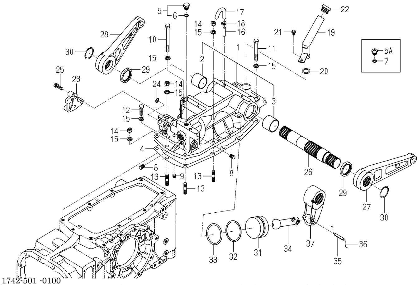
FIG.501 CYLINDER CASE SYSTEM(TG5395)
