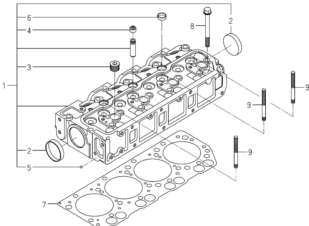
FIG.101 CYLINDER HEAD
