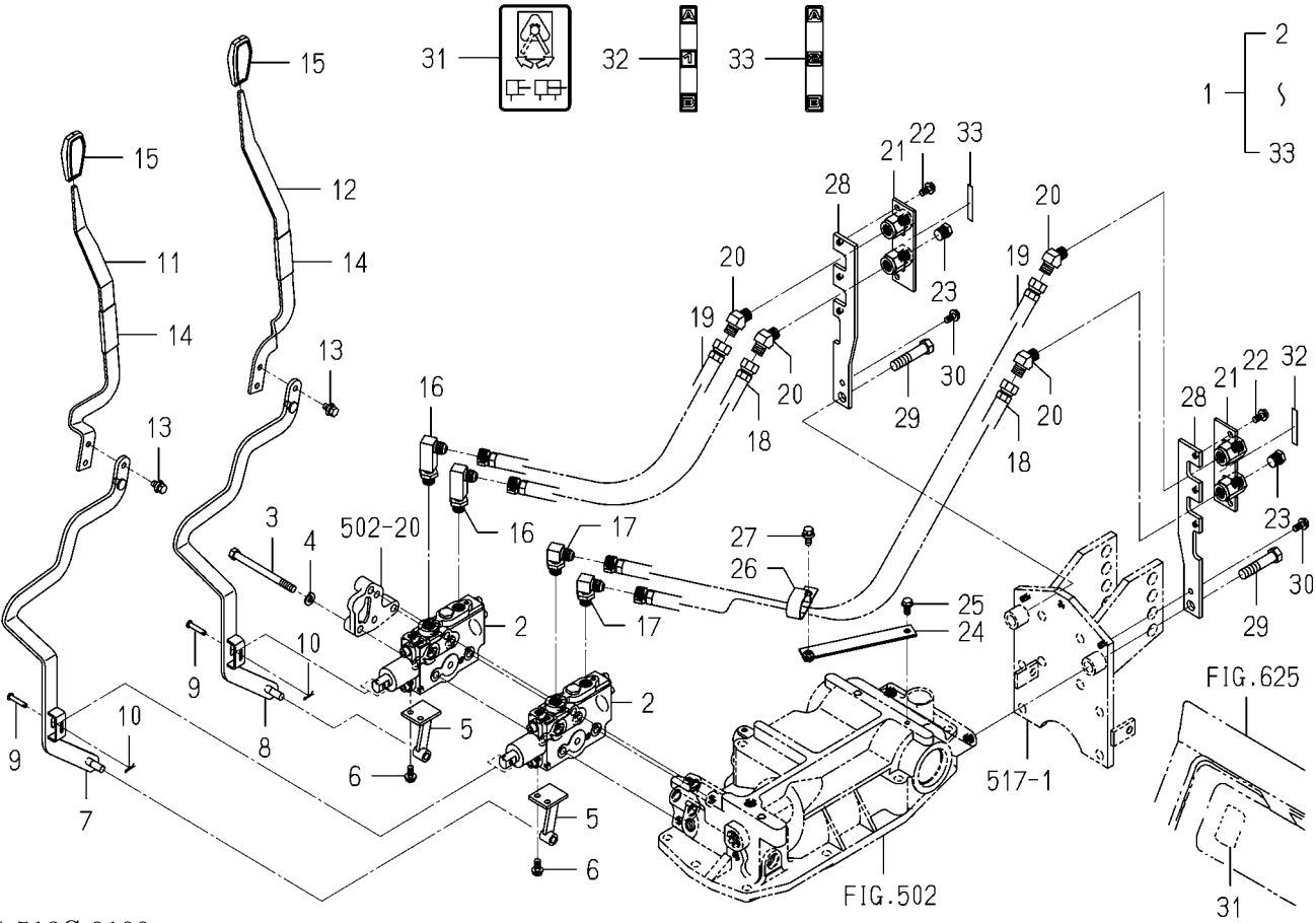
FIG.P21 VALVE(REMOTE/2R)SET(OPTION)(TG5475)
