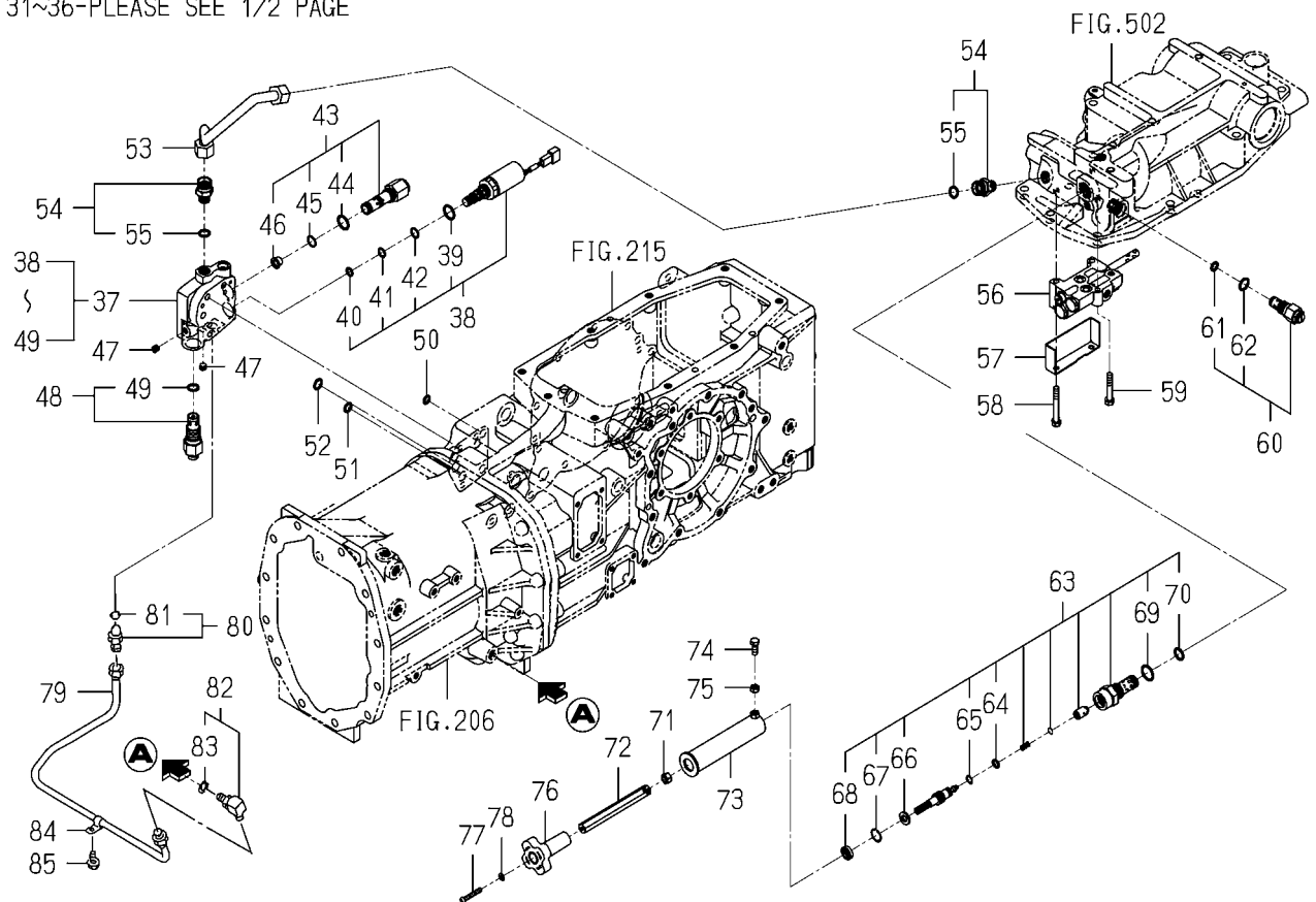
FIG.507 HYD.SYSTEM(MAIN)(TG5475)(2/2)
