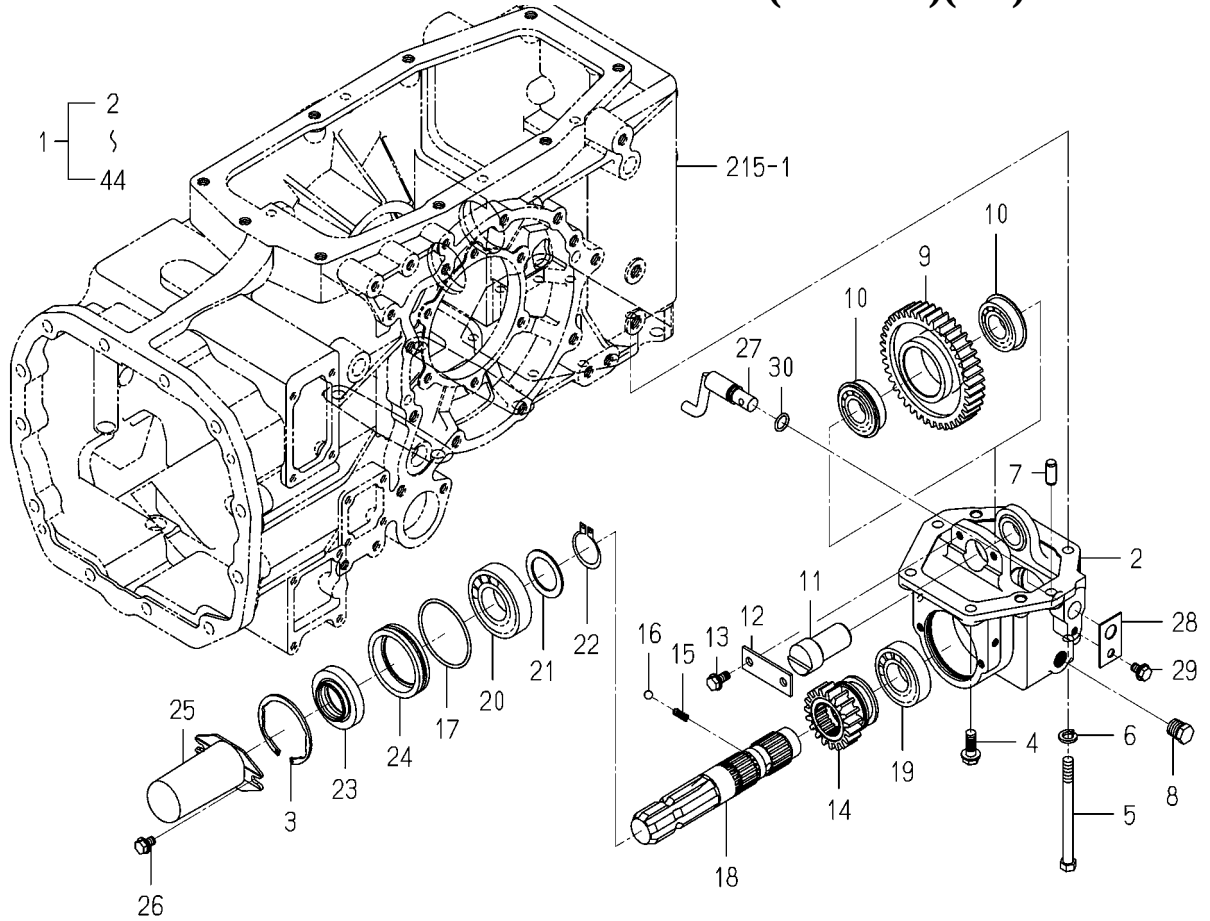
FIG.213 MID PTO SYSTEM(TG5475)(1/2)
