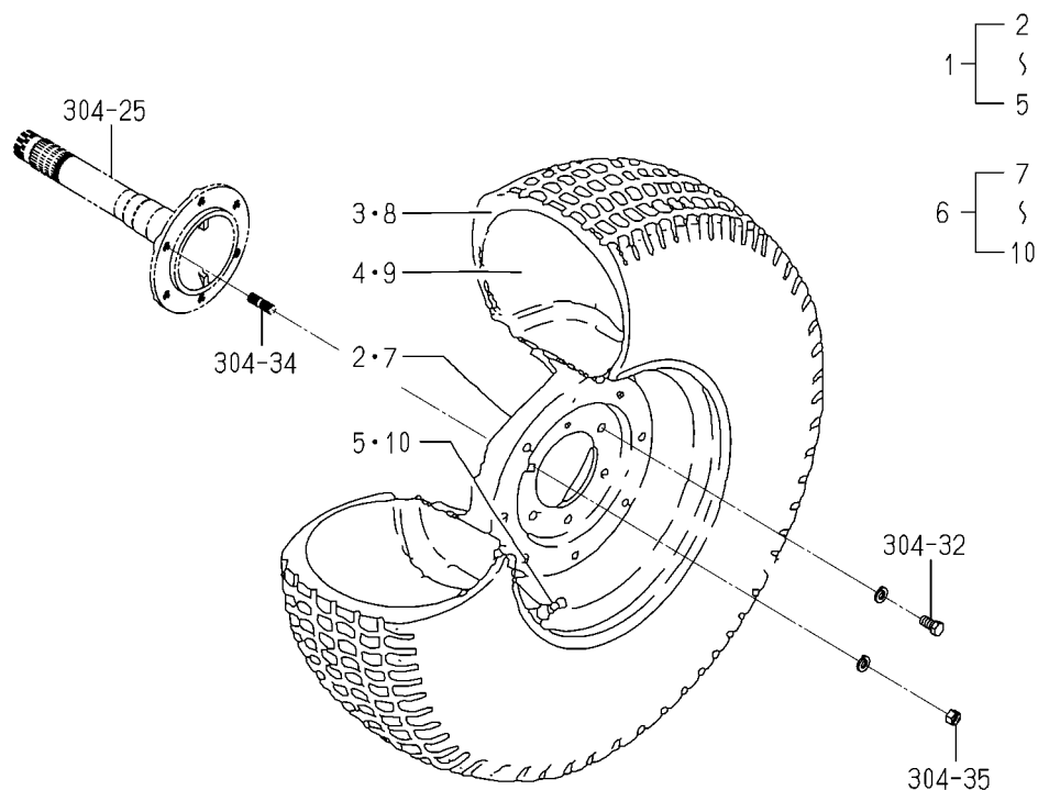
FIG.P05 REAR WHEEL(TURF)SYSTEM (OPTION)(TG5475)
