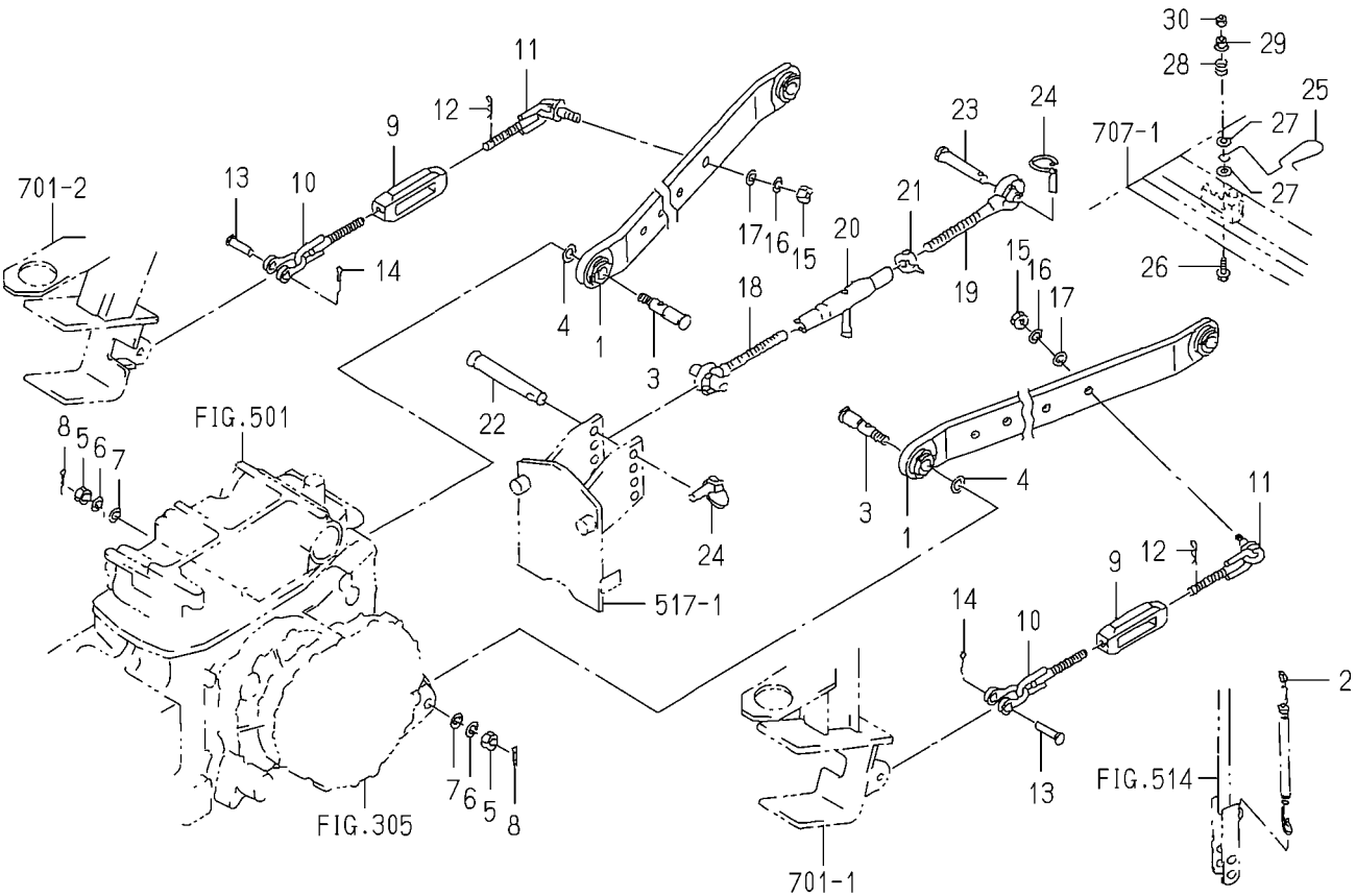
FIG.511 3P LINK SYSTEM(TG5395-C TYPE)
