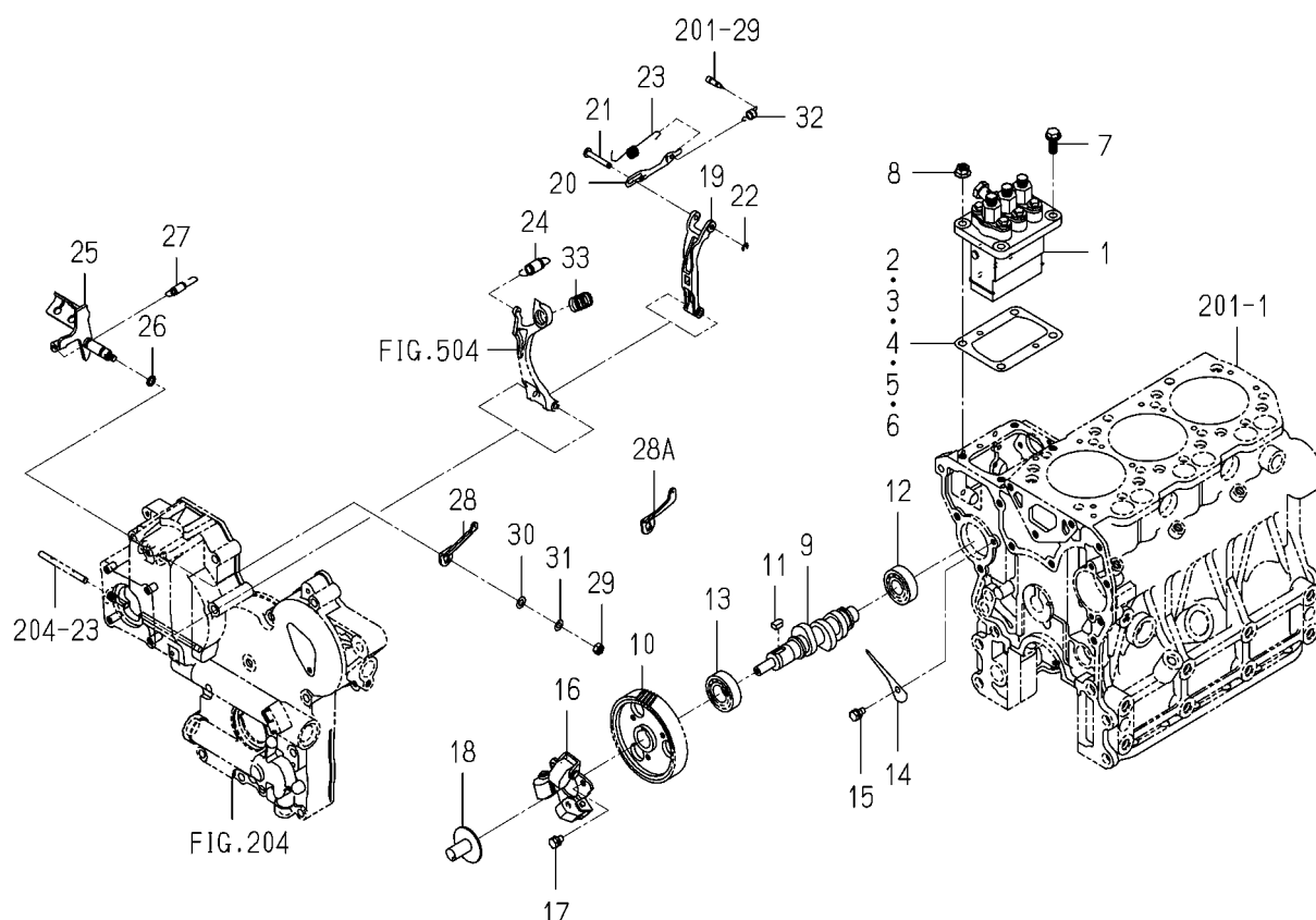
FIG.502 INJECTION PUMP
