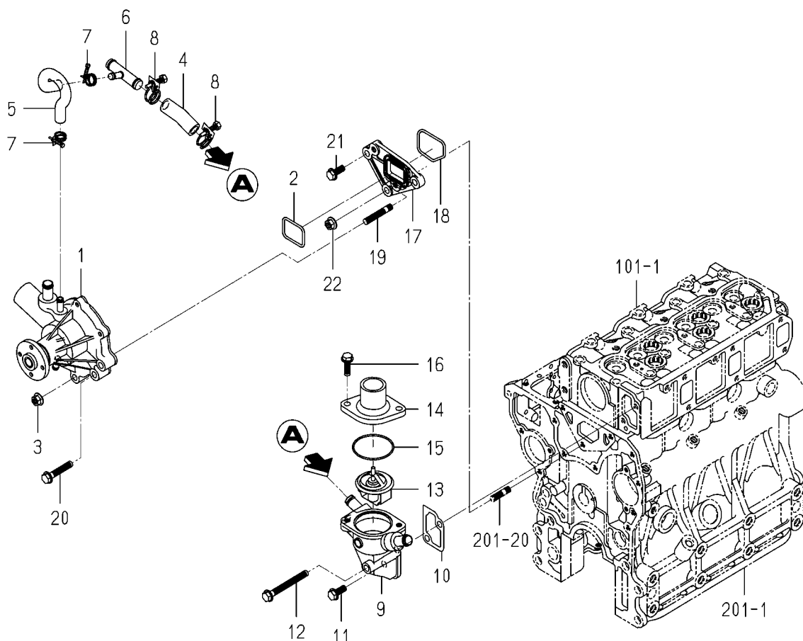
FIG.402 WATER PUMP
