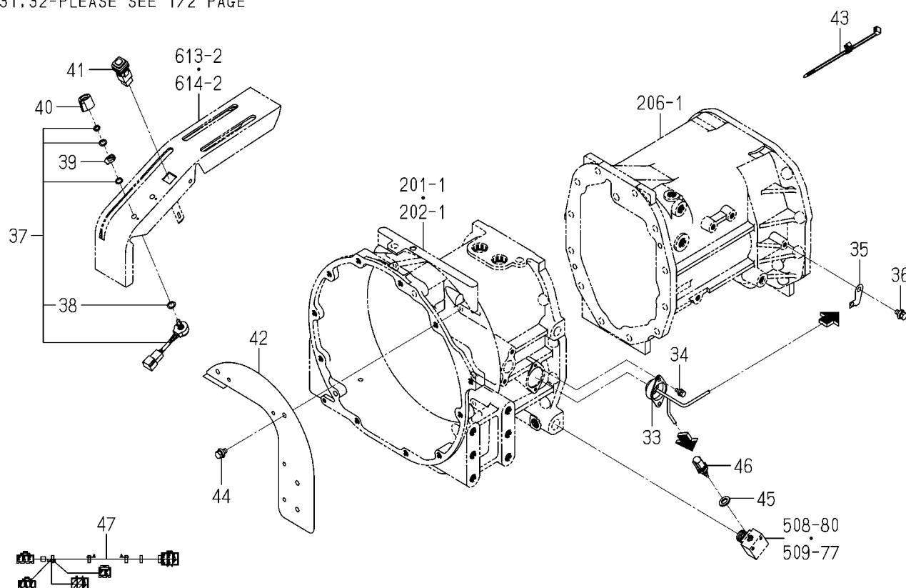
FIG.636 CONTROLLER SYSTEM(2/2)
