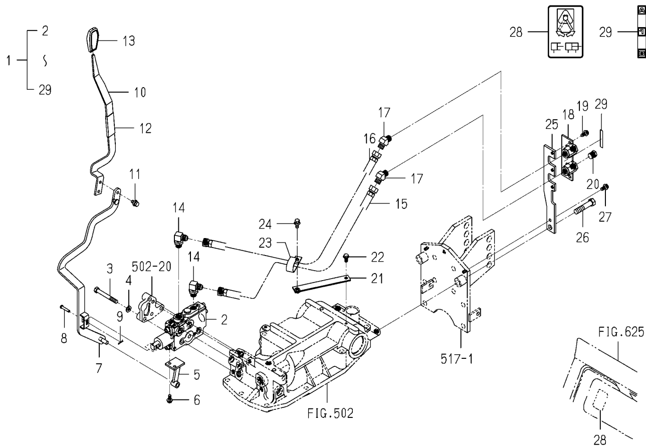
FIG.P19 VALVE(REMOTE/1R)SET(OPTION)(TG5475)
