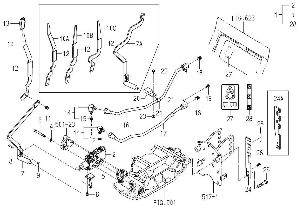
FIG.P18 VALVE(REMOTE/1R)SET (OPTION)(TG5395-R TYPE)
