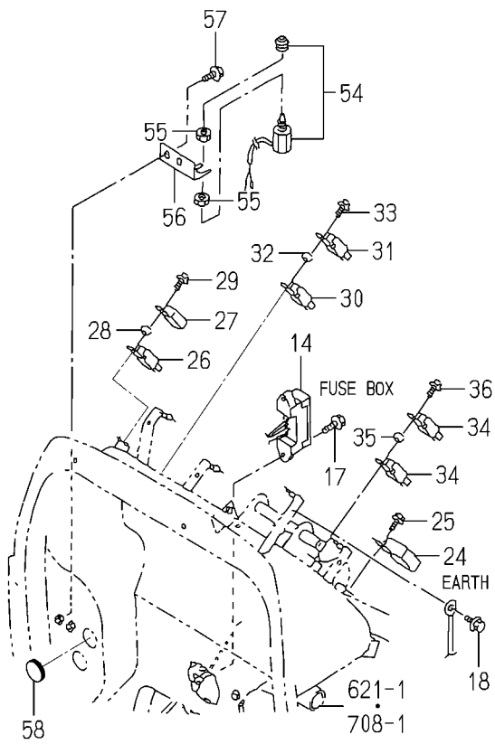
FIG.630 ELC.SYSTEM(MAIN)(TG5475)(2/3)
