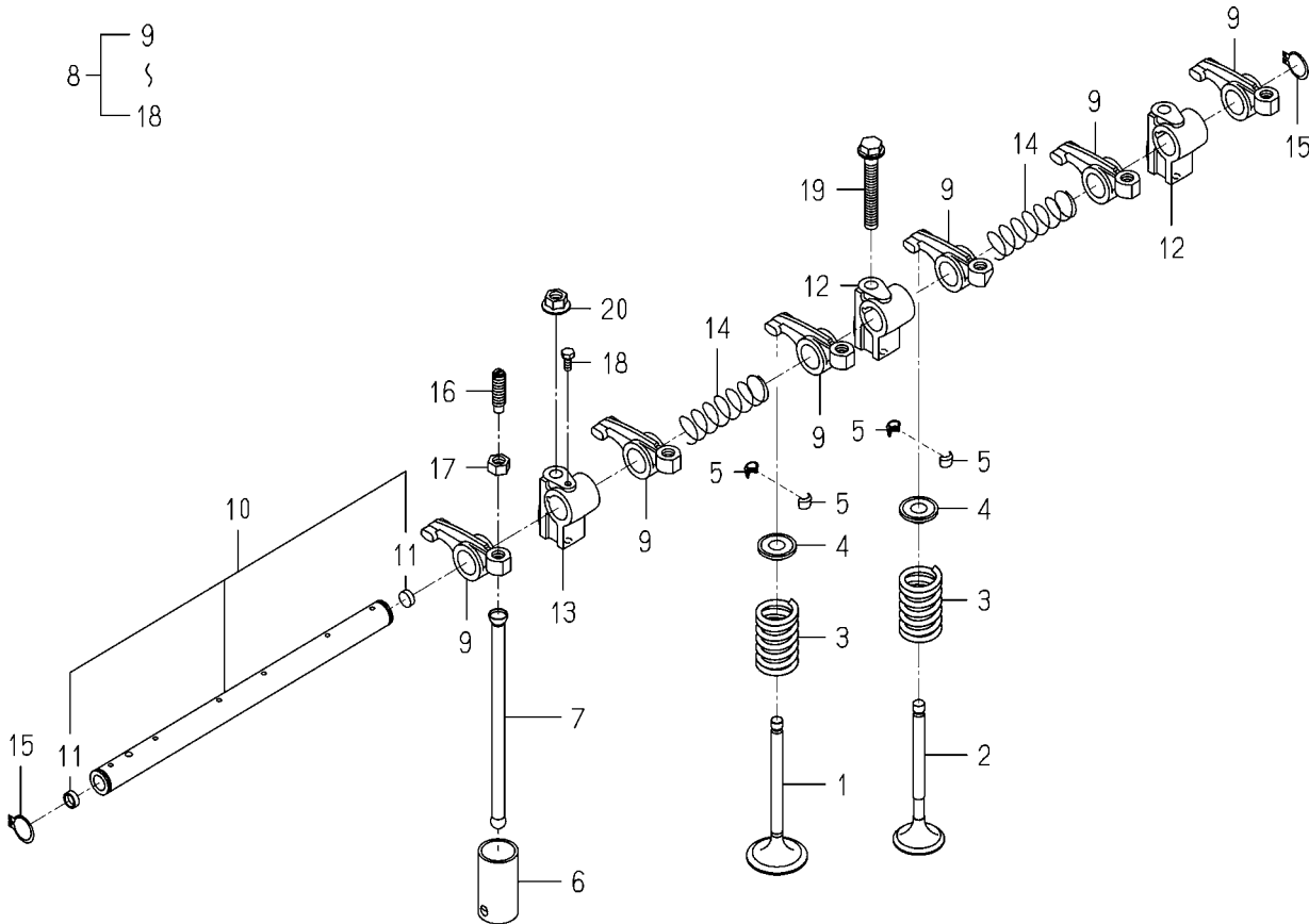
FIG.301 VALVE
