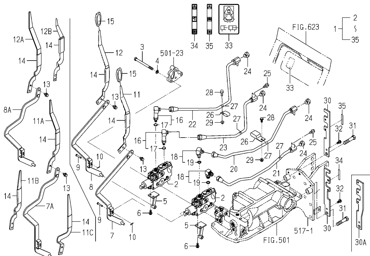
FIG.P20 VALVE(REMOTE/2R)SET (OPTION)(TG5395-R TYPE)
