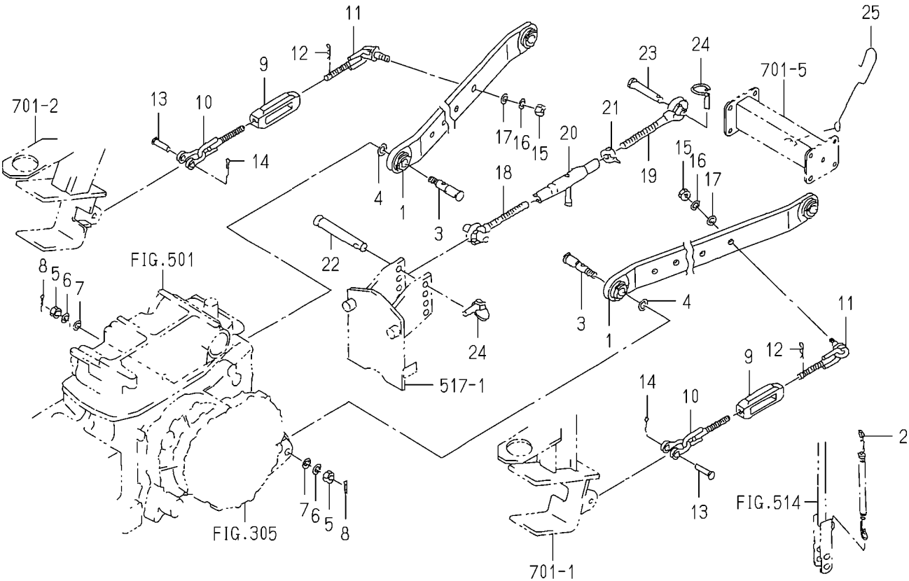
FIG.510 3P LINK SYSTEM(TG5395-R TYPE)
