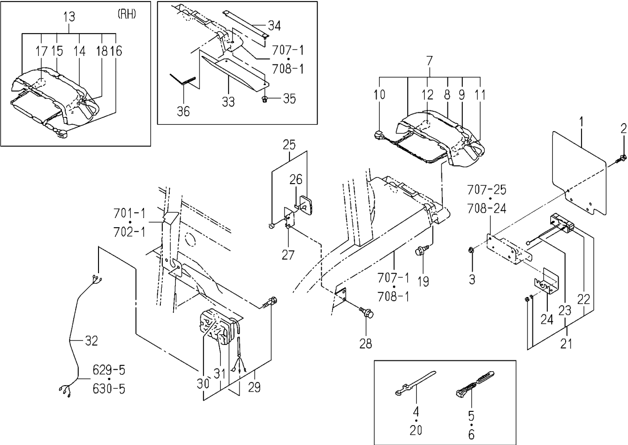
FIG.632 ELC.SYSTEM(REAR)(C TYPE)
