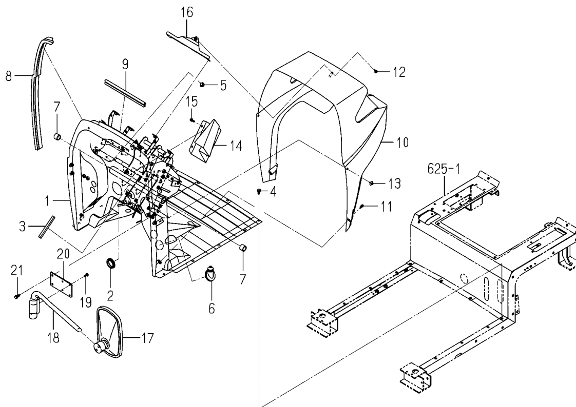
FIG.621 FLOOR(FRONT)SYSTEM(TG5475-R TYPE)
