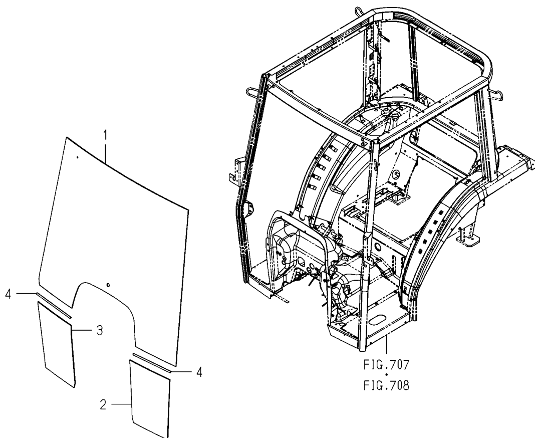
FIG.709 GLASS(FRONT)SYSTEM(C TYPE)
