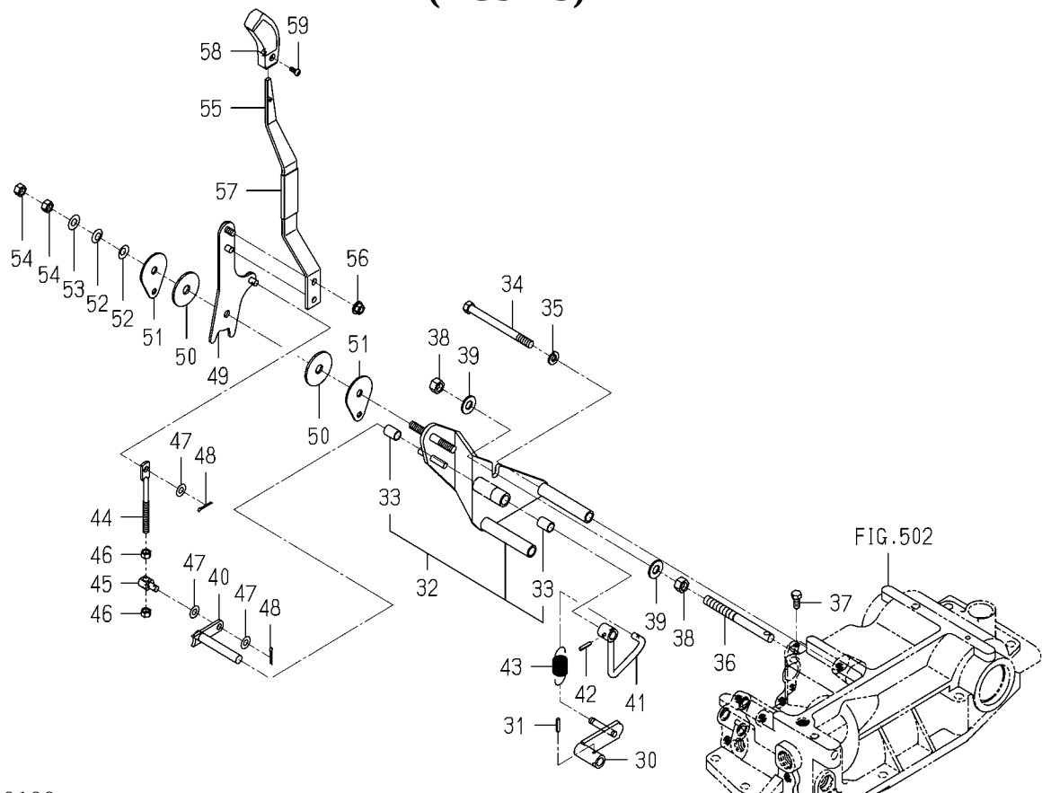
FIG.504 MECHANICAL LINK(POSITION)SYSTEM(2/2) (TG5475)
