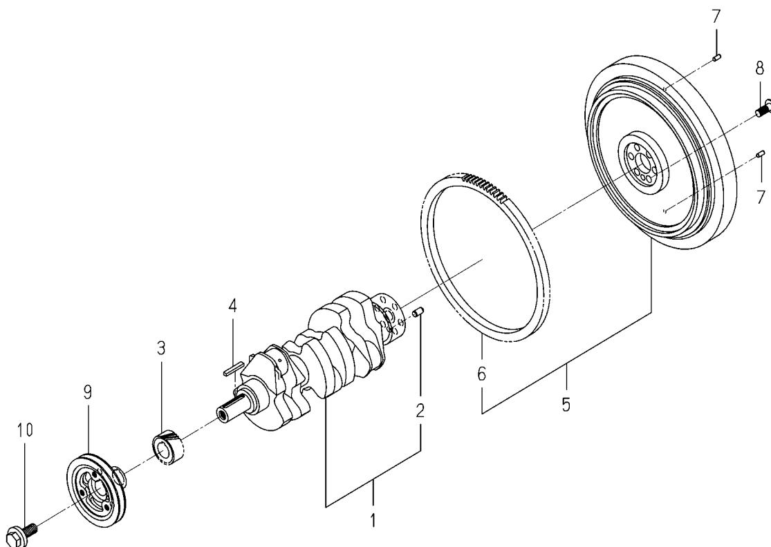
FIG.304 CRANK SHAFT
