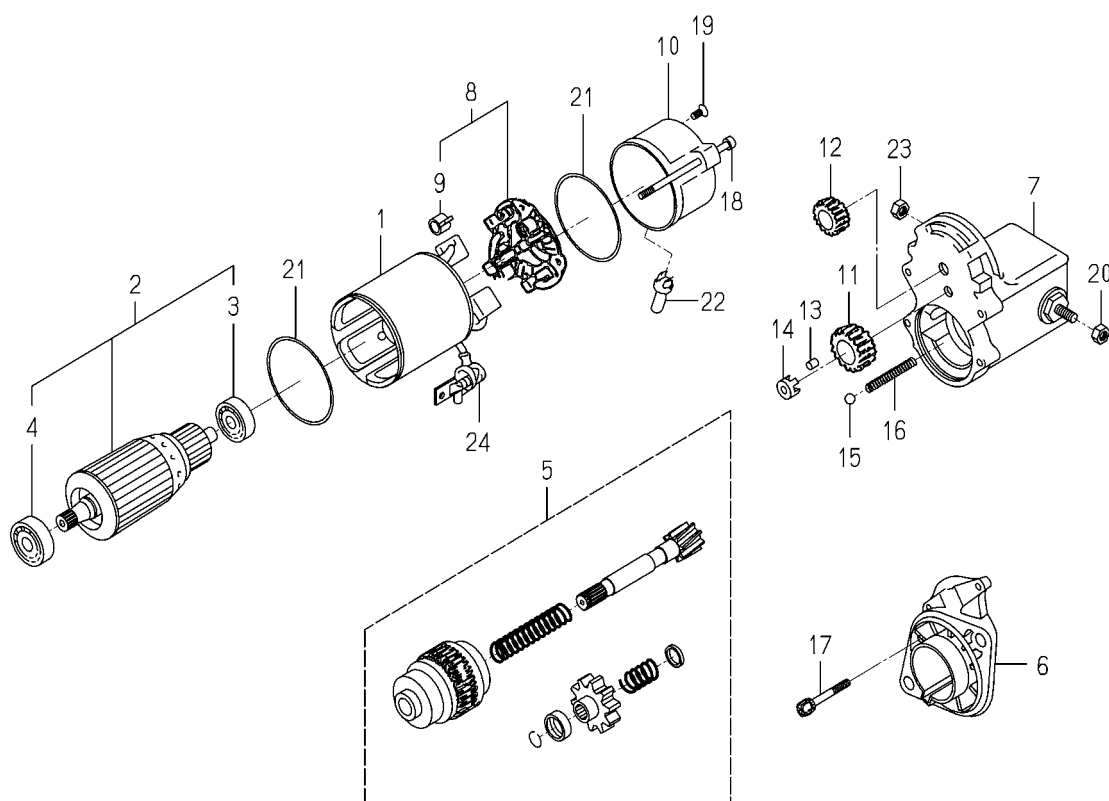
FIG.S03 COMPONENT PARTS FOR 6281-100-010-30 ON Fig.801
