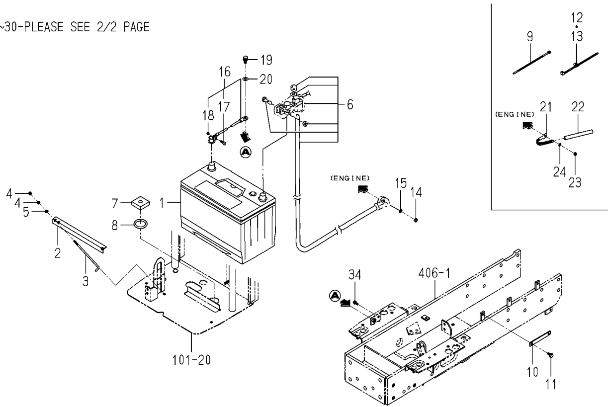
FIG.627 ELC.SYSTEM(FRONT)(TG5395)(1/2)
