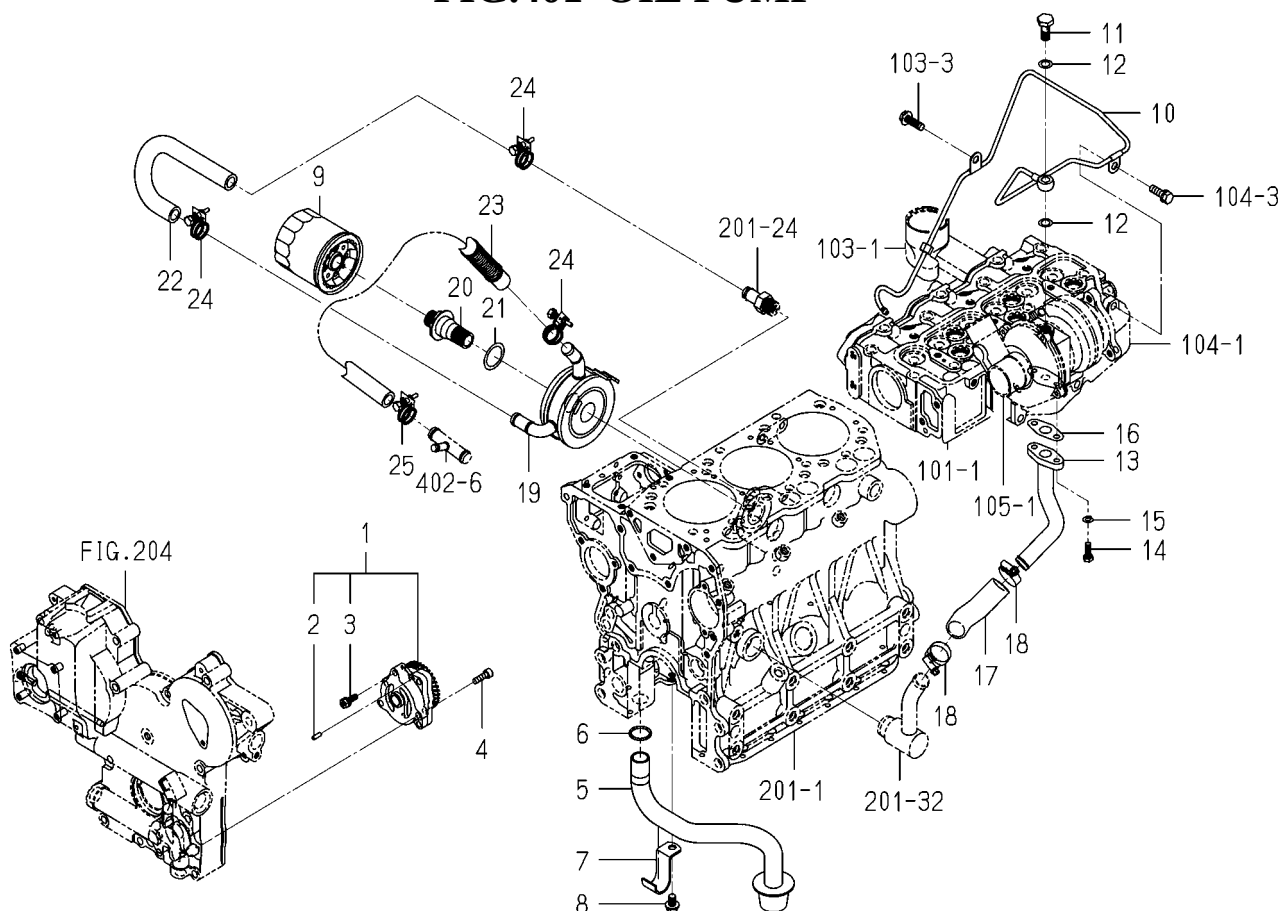
FIG.401 OIL PUMP
