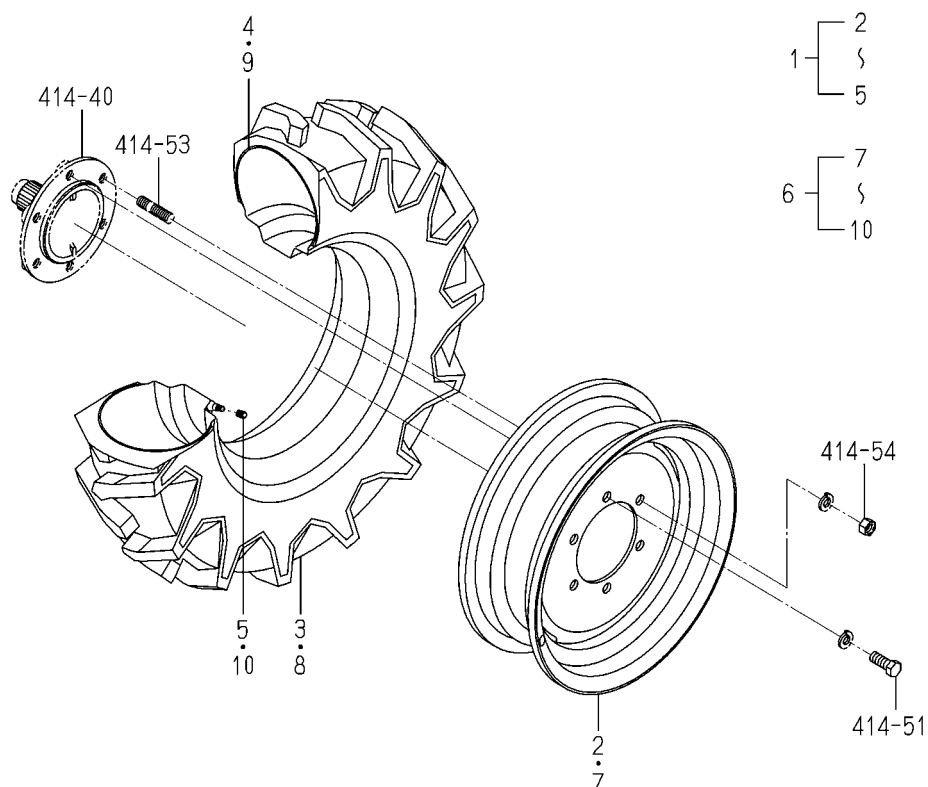
FIG.P11 FRONT WHEEL(8-16)SYSTEM (OPTION)(TG5475)
