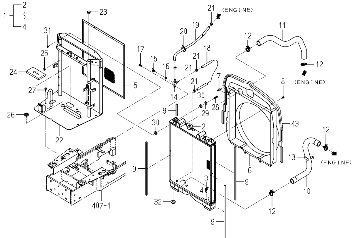
FIG.103 RADIATOR SYSTEM(TG5475-C TYPE)(1/2)
