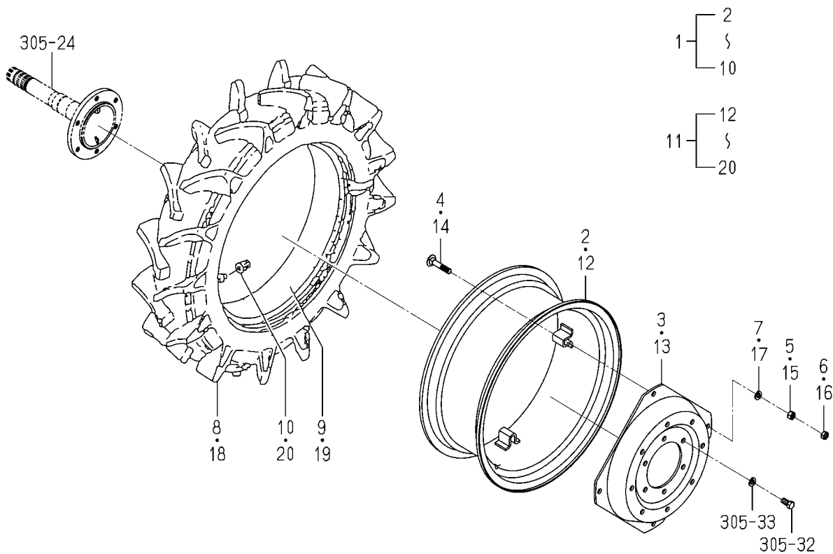
FIG.P02 REAR WHEEL SYSTEM(OPTION)(TG5395)
