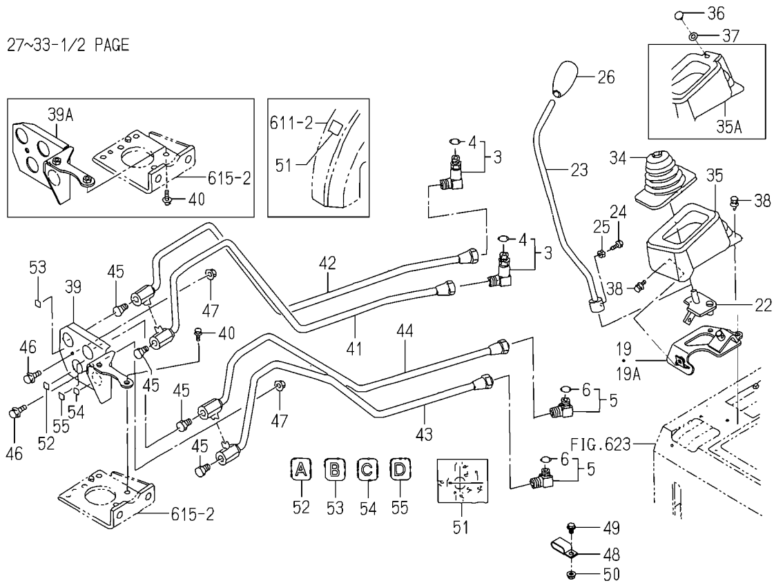
FIG.P16 JOY STICK VALVE SET(2/2) (OPTION)(TG5395)
