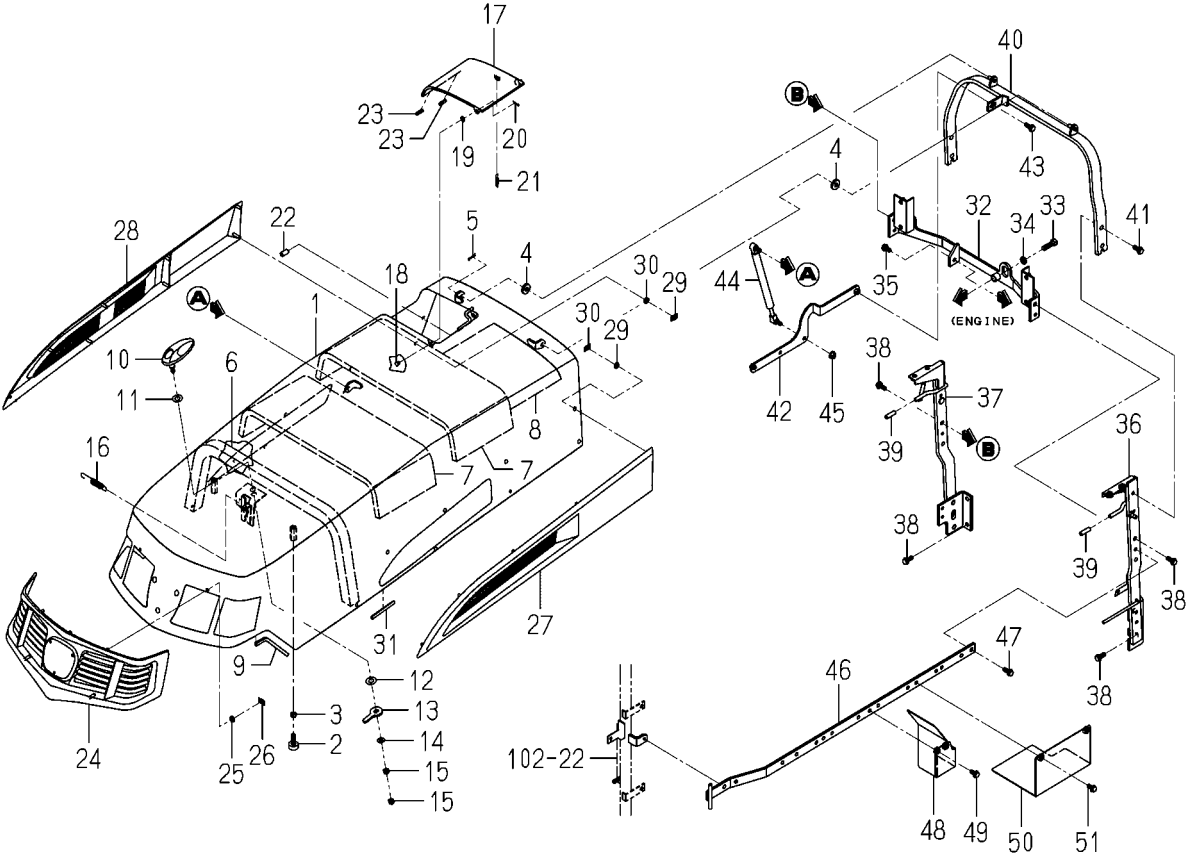
FIG.604 HOOD SYSTEM(TG5475-R TYPE)
