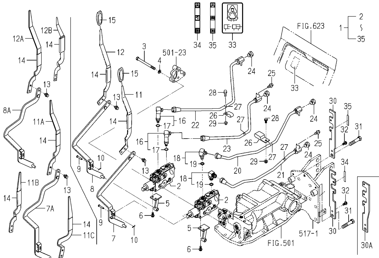
FIG.P20 VALVE(REMOTE/2R)SET (OPTION)(TG5395-R TYPE)
