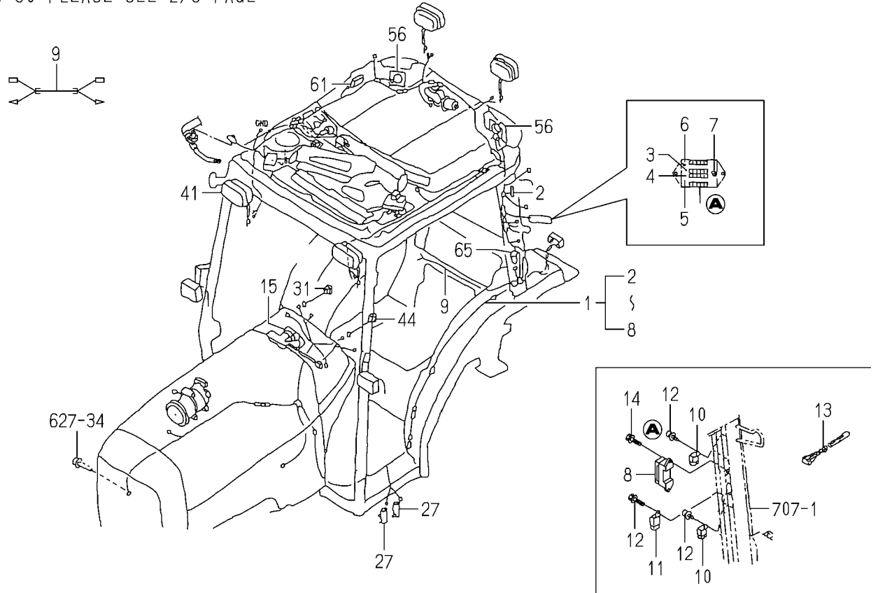
FIG.634 ELC.SYSTEM(TG5395-C TYPE)(1/3)
