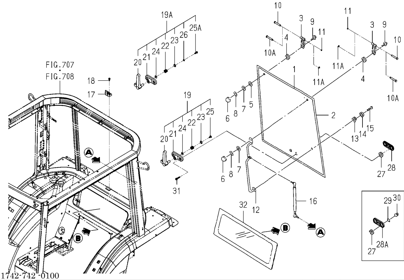
FIG.713 GLASS(REAR)SYSTEM(C TYPE)
