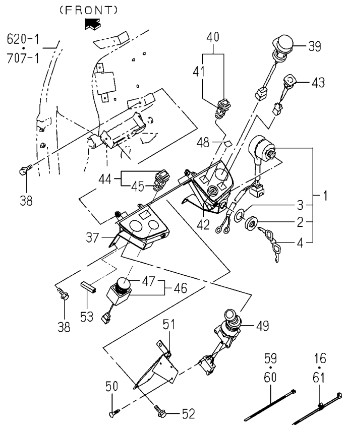
FIG.629 ELC.SYSTEM(MAIN)(TG5395)(2/3)
