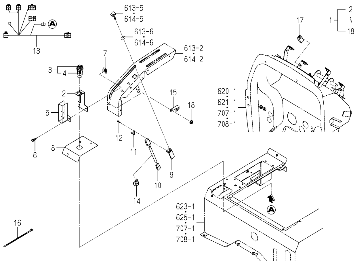
FIG.P24 PTO UP-STOP SET(OPTION)
