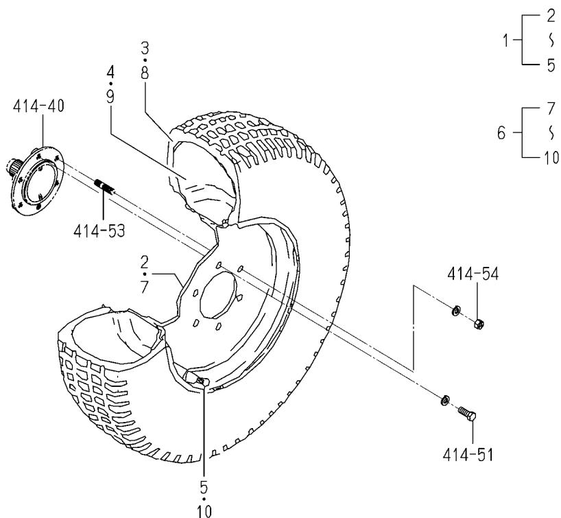
FIG.P13 FRONT WHEEL(TURF)SYSTEM (OPTION)(TG5475)
