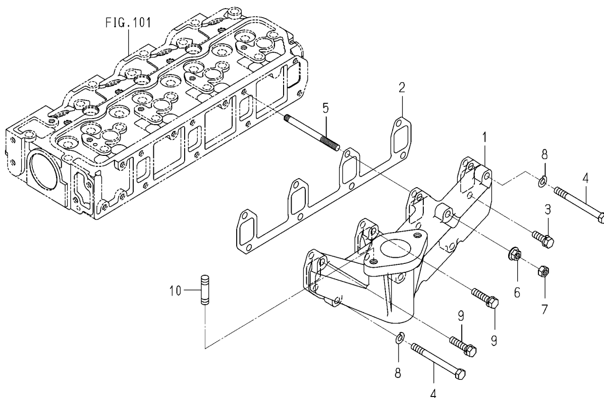
FIG.104 EXHAUST MANIFOLD
