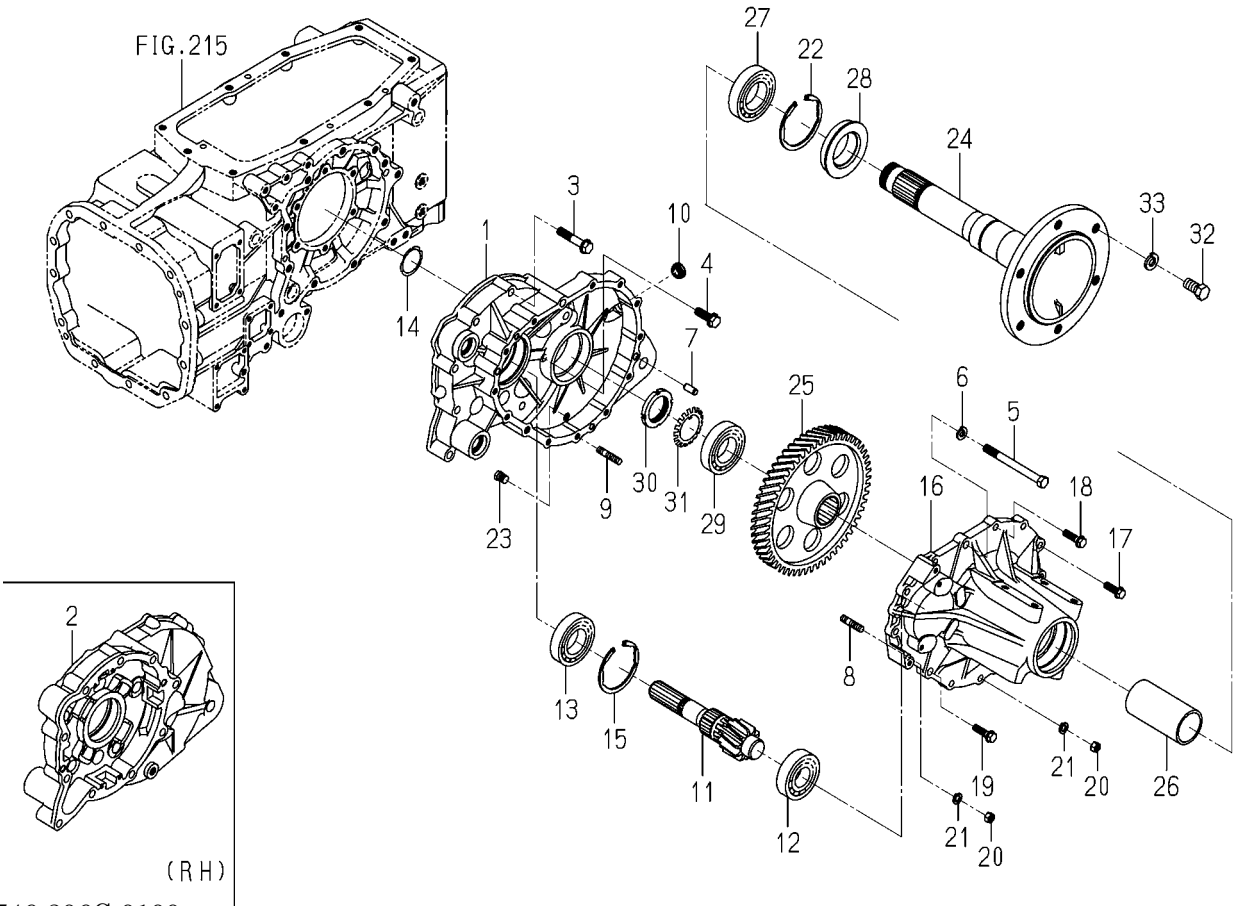
FIG.305 HOUSING(AXLE)SYSTEM(TG5395)
