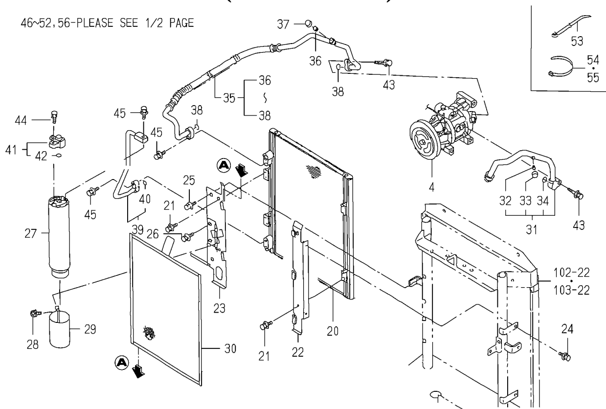
FIG.715 AIR CODITIONER(ENGINE)SYSTEM(2/2) (TG5475-C TYPE)
