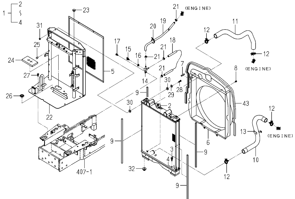
FIG.102 RADIATOR SYSTEM(TG5475-R TYPE)(1/2)
