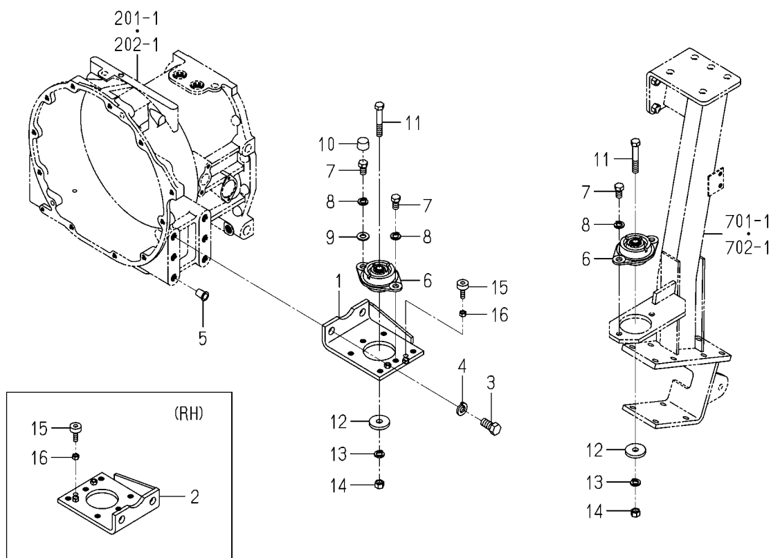
FIG.615 MOUNT SYSTEM(R TYPE)
