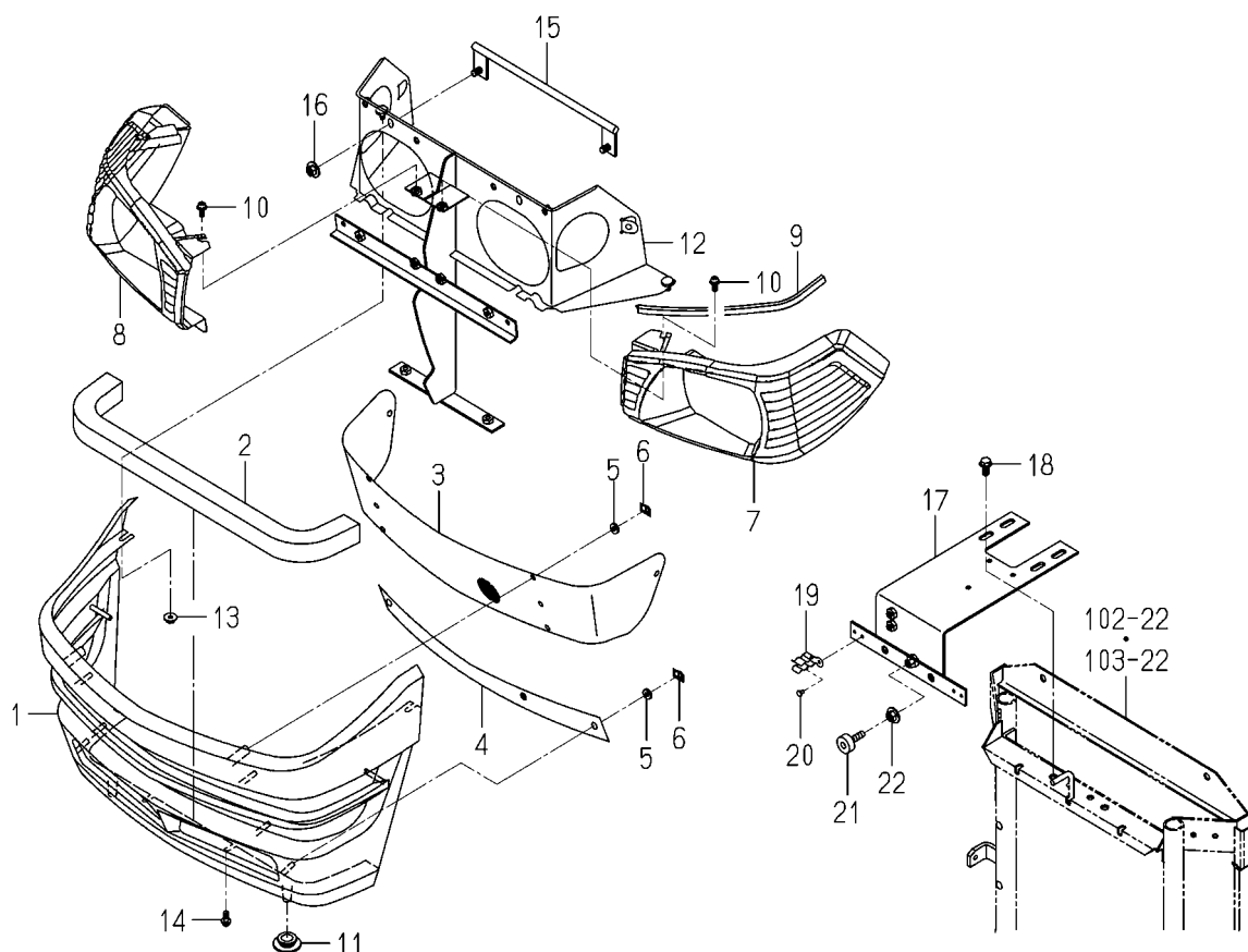
FIG.606 GRILLE SYSTEM(TG5475 TYPE)
