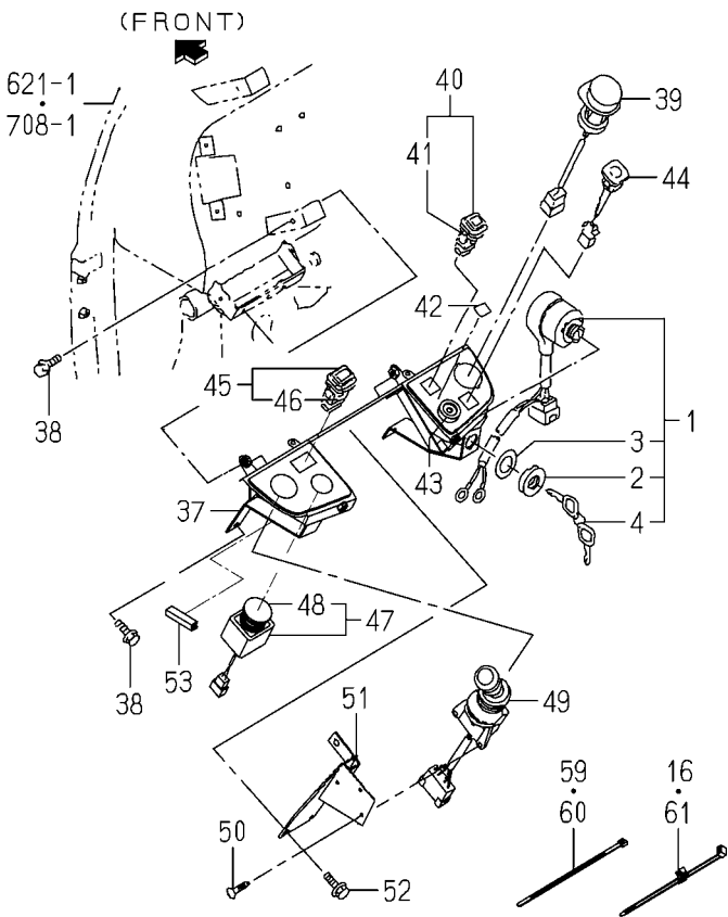
FIG.630 ELC.SYSTEM(MAIN)(TG5475)(2/3)
