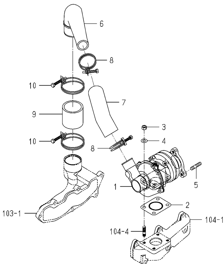
FIG.105 TURBO CHARGER
