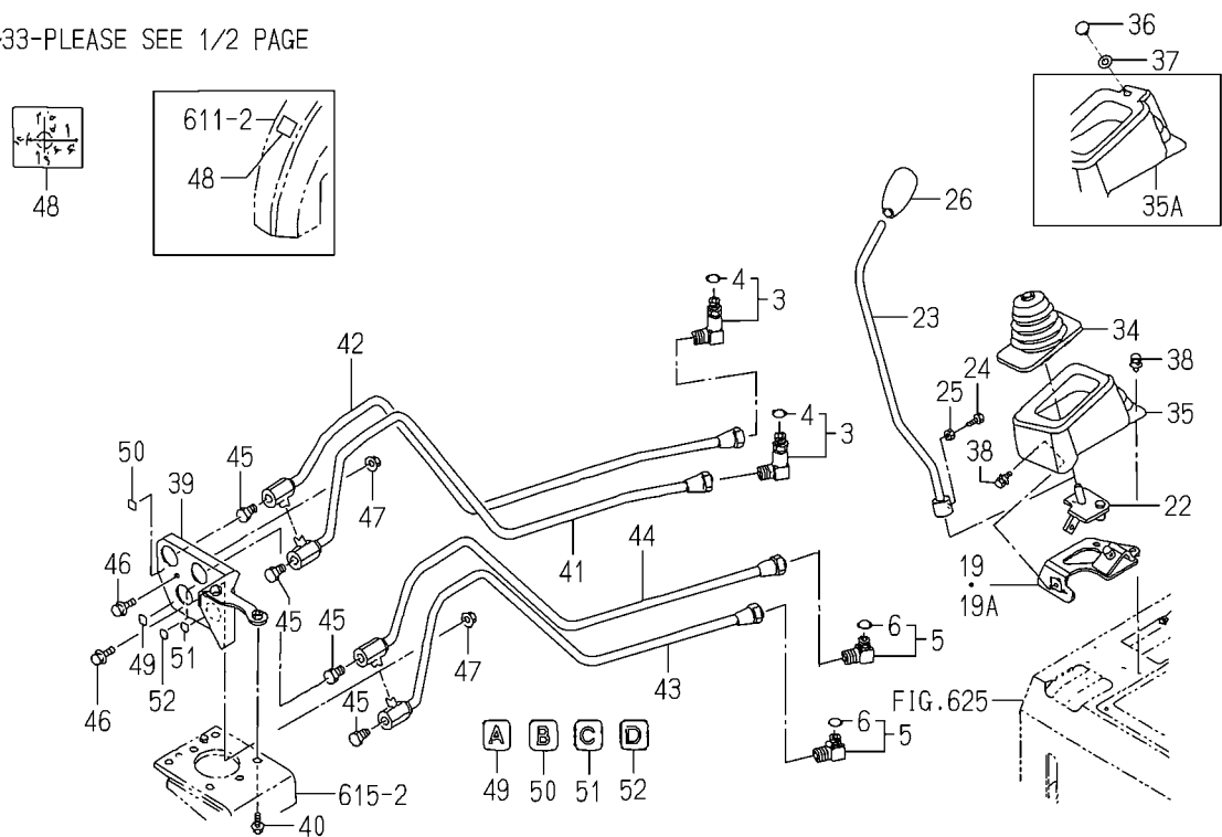
FIG.P17 JOY STICK VALVE SET(2/2) (OPTION)(TG5475)
