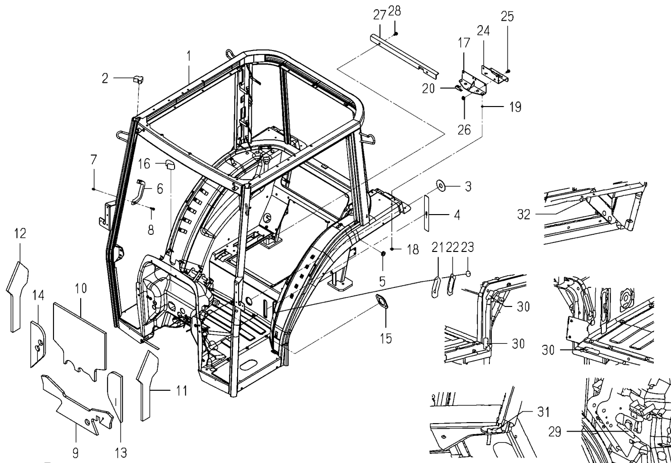
FIG.708 FRAME SYSTEM(TG5475-C TYPE)
