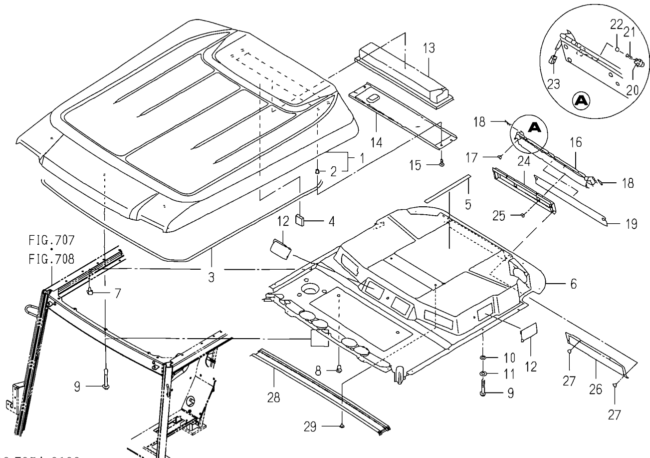
FIG.705 ROOF SYSTEM(C TYPE)
