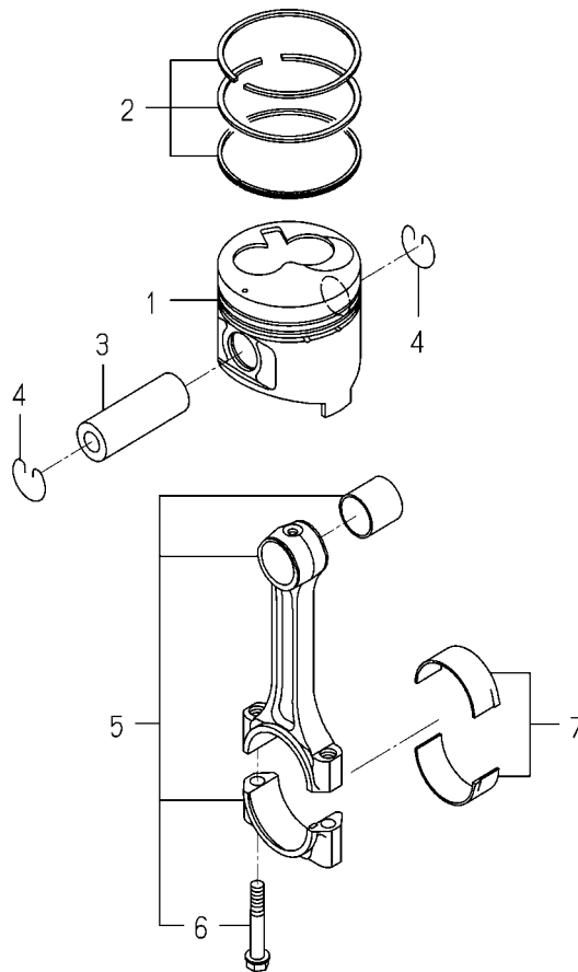
FIG.303 PISTON
