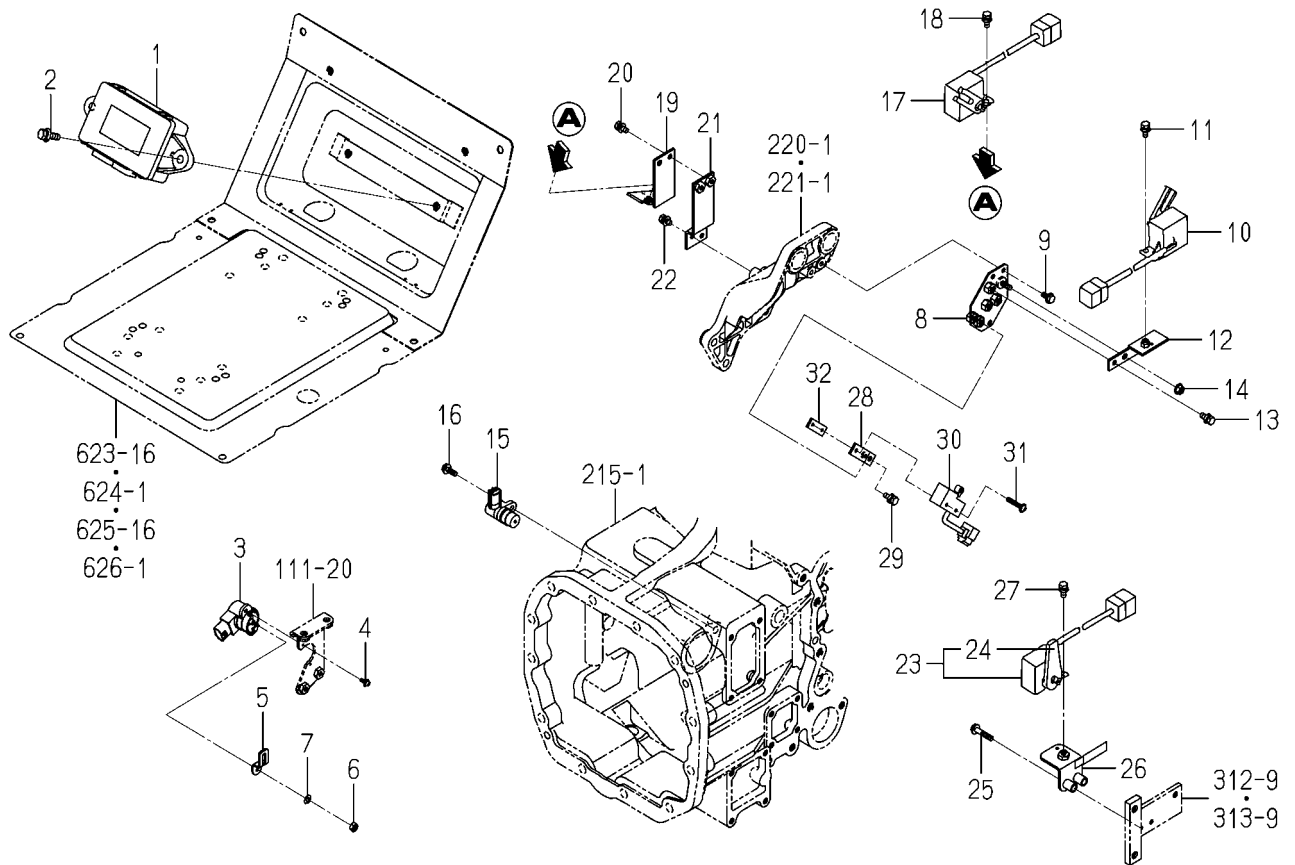
FIG.636 CONTROLLER SYSTEM(1/2)
