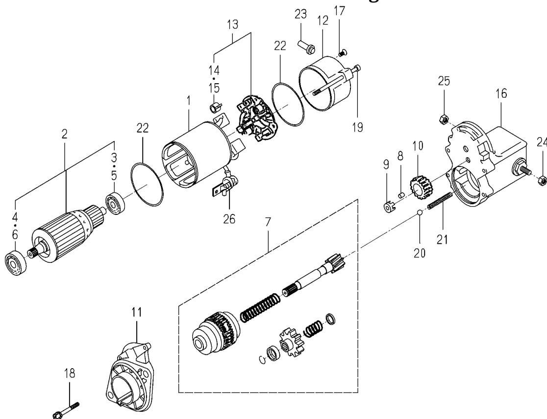
FIG.S03 COMPONENT PARTS FOR 6281-100-007-20 ON Fig.801
