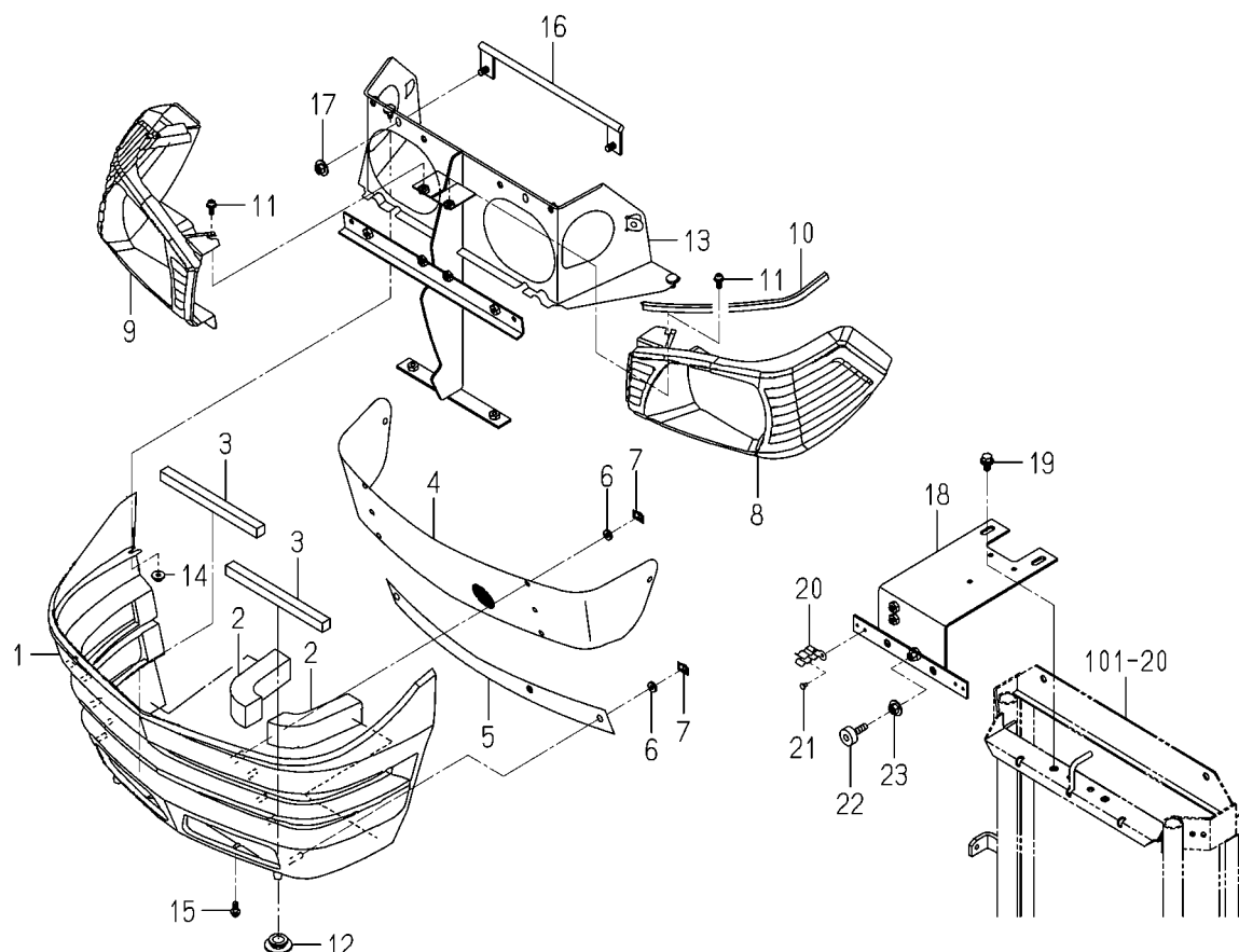
FIG.605 GRILLE SYSTEM(TG5395 TYPE)
