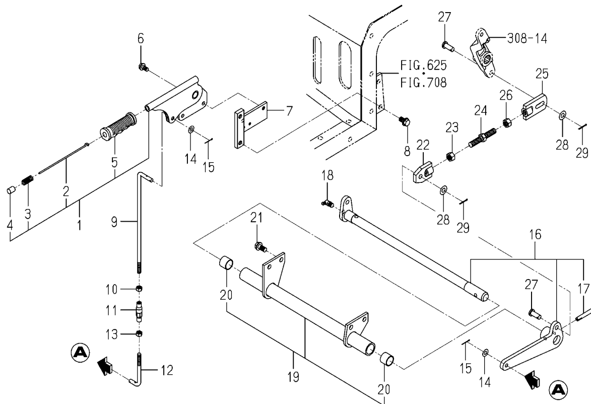
FIG.313 BRAKE(PARKING)SYSTEM(TG5475)
