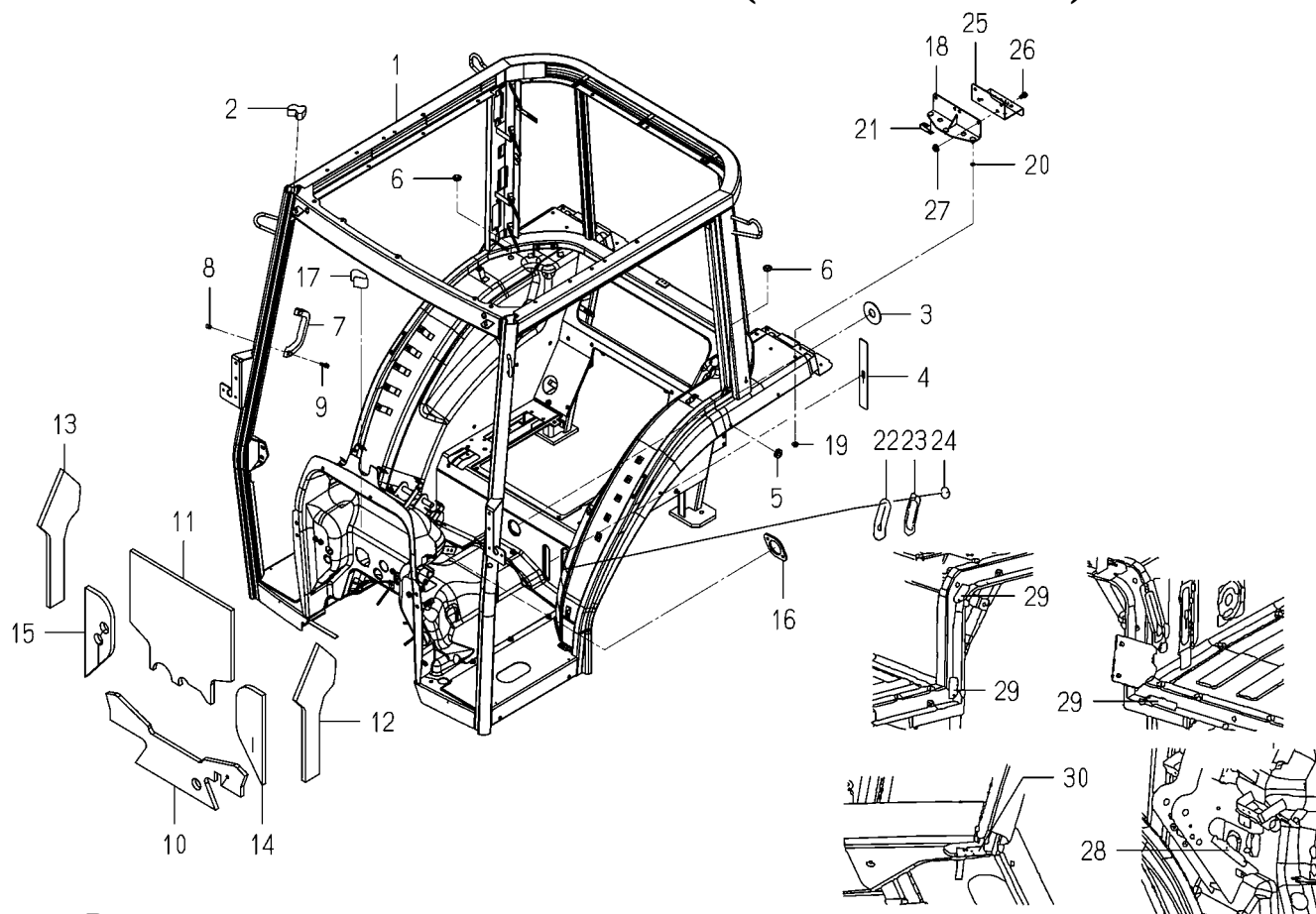
FIG.707 FRAME SYSTEM(TG5395-C TYPE)
