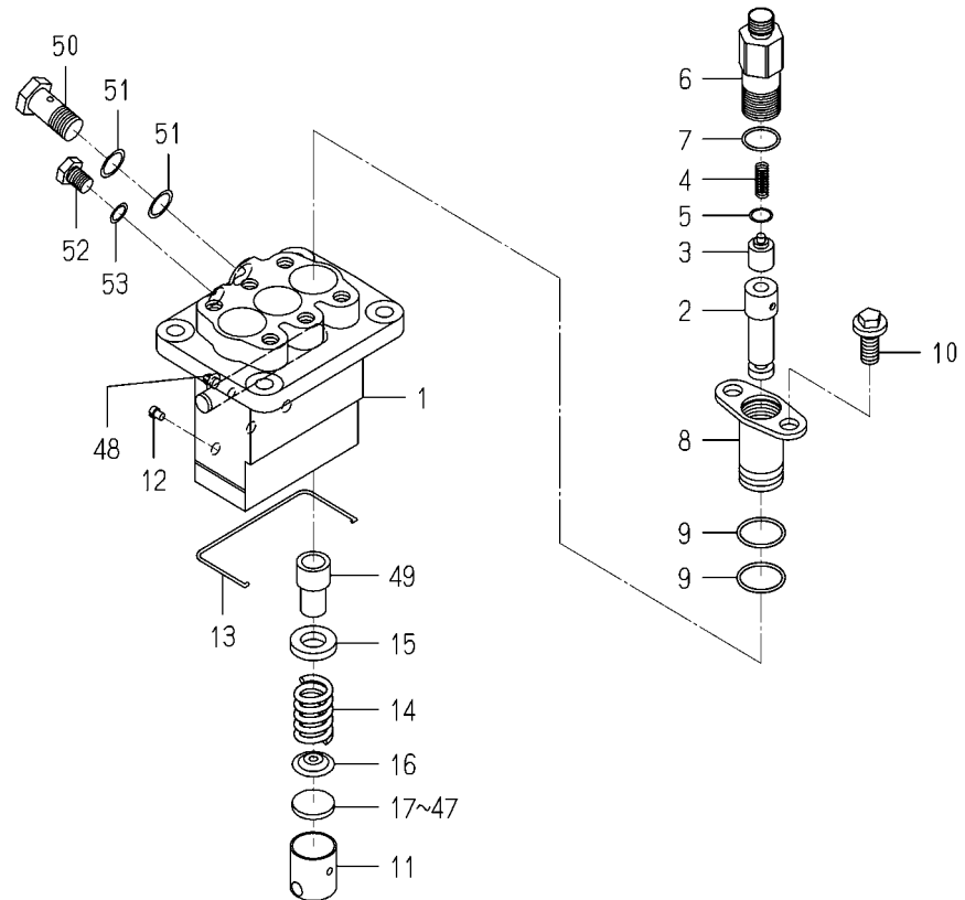
FIG.S02 COMPONENT PARTS FOR 6215-600-078-10 ON Fig.502
