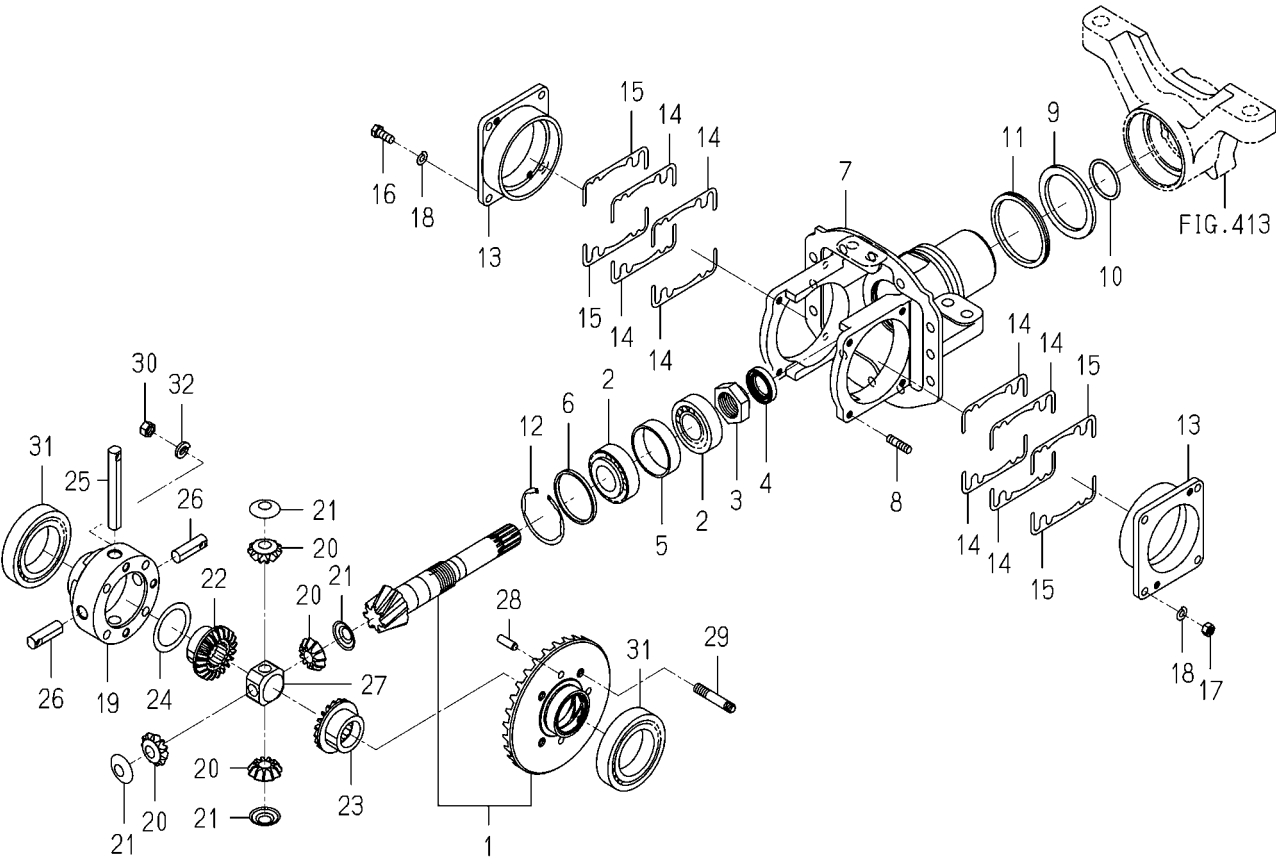
FIG.411 CASE(BEVEL)SYSTEM(TG5475)
