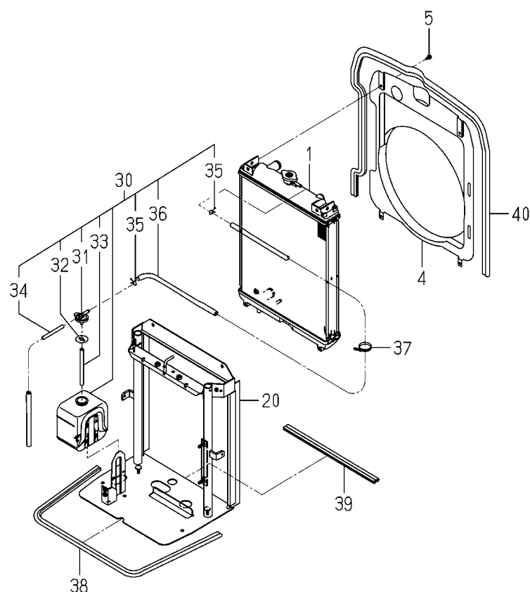
FIG.101 RADIATOR SYSTEM(TG5395)(2/2)
