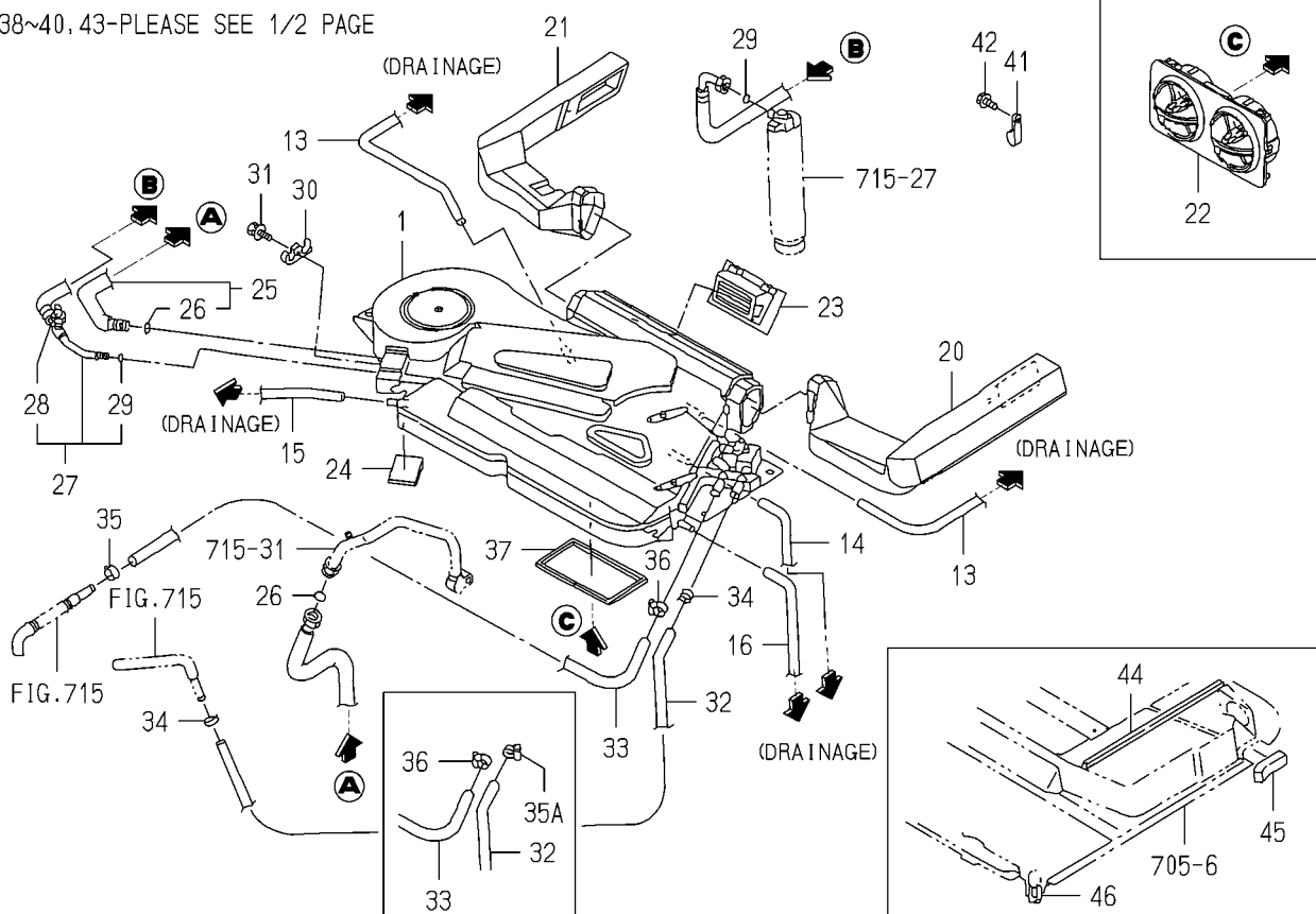
FIG.717 AIR CODITIONER(CABIN)SYSTEM(2/2) (TG5475-C TYPE)
