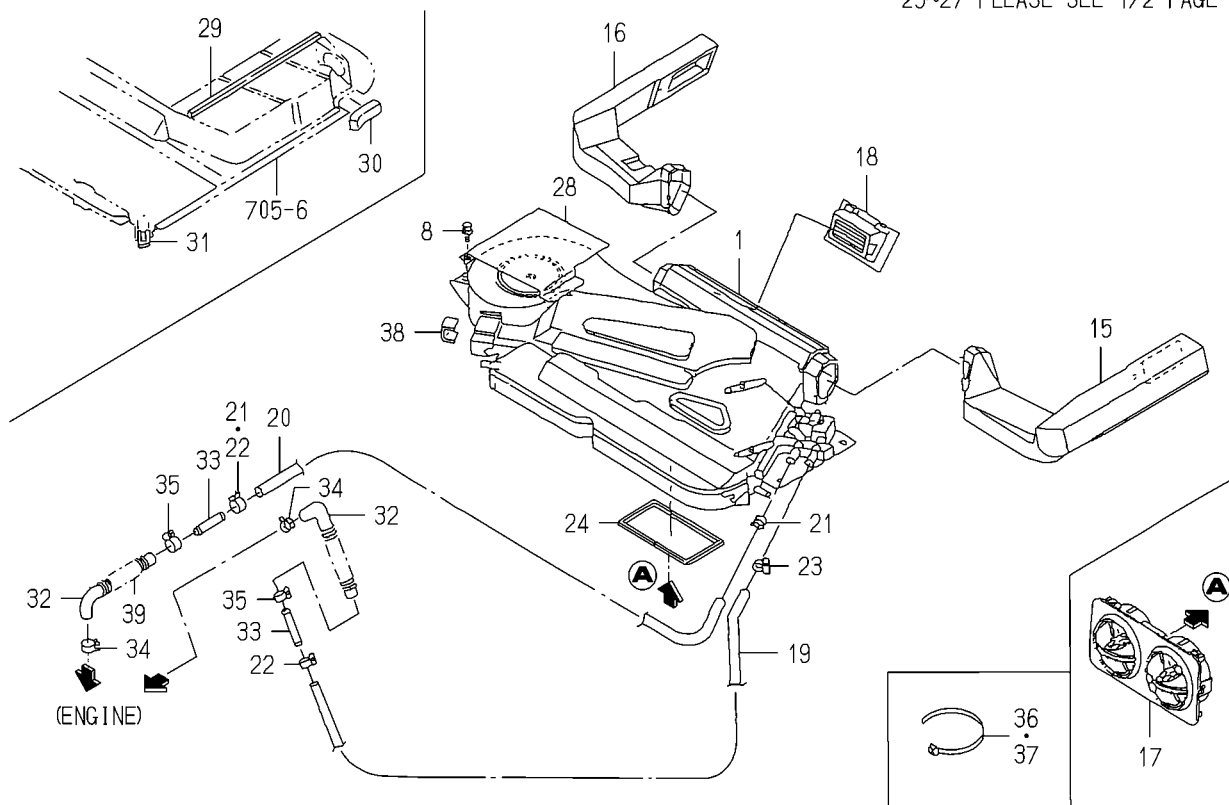
FIG.716 HEATER(CABIN)SYSTEM(2/2) (TG5395-C TYPE)
