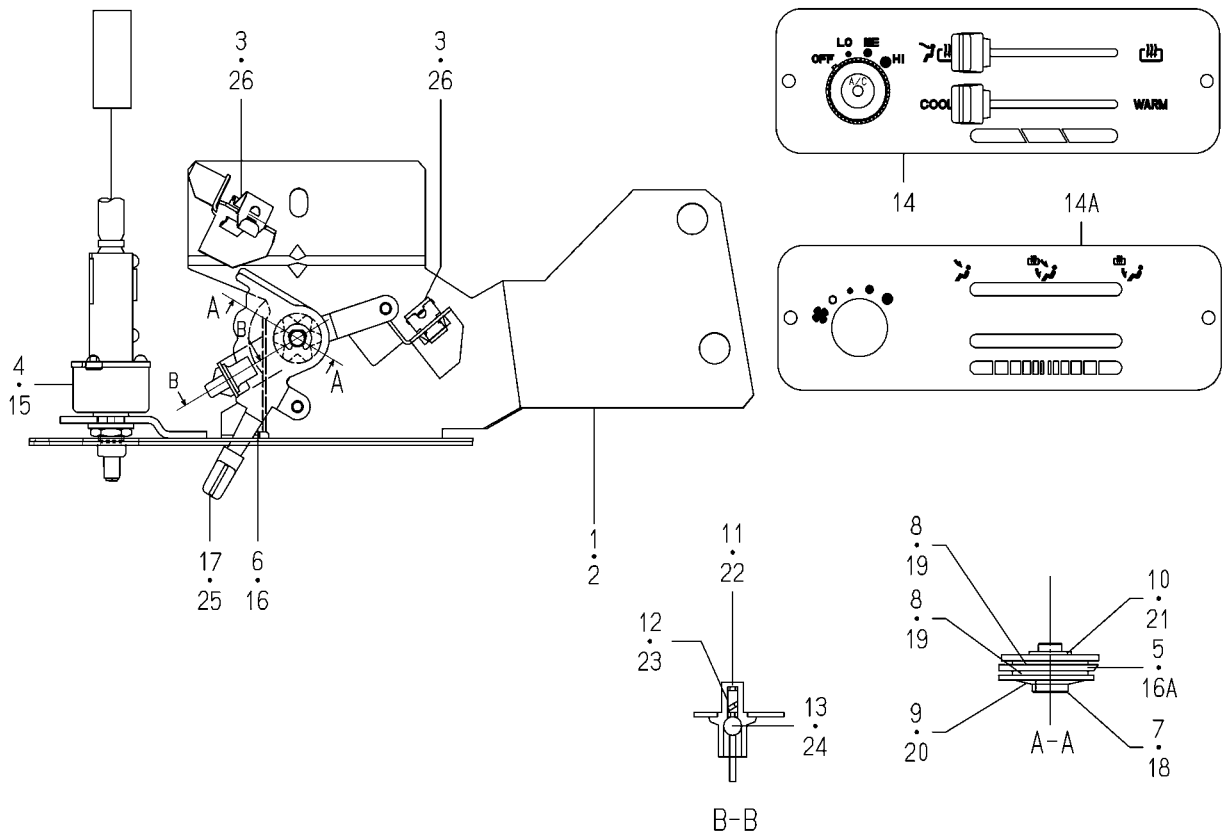
FIG.S15 COMPONENT PARTS FOR 1746-781-220-10 ON Fig.716
