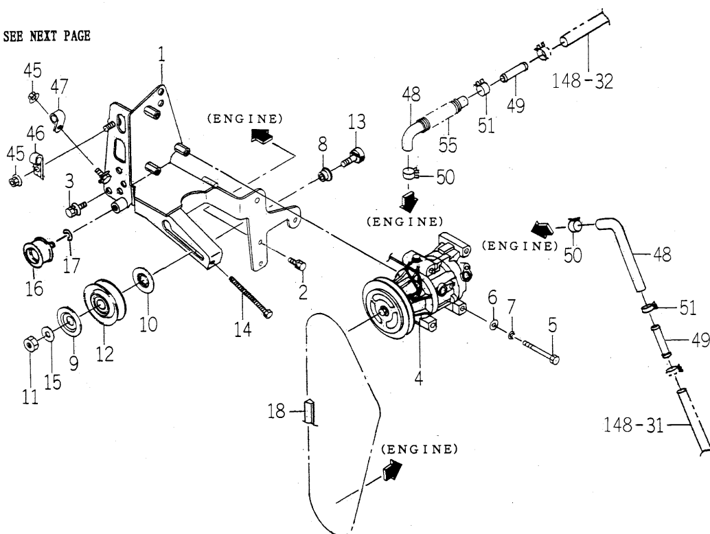
FIG.147 AIR CONDITIONER (ENGINE) SYSTEM(1/2) (CY TYPE)
