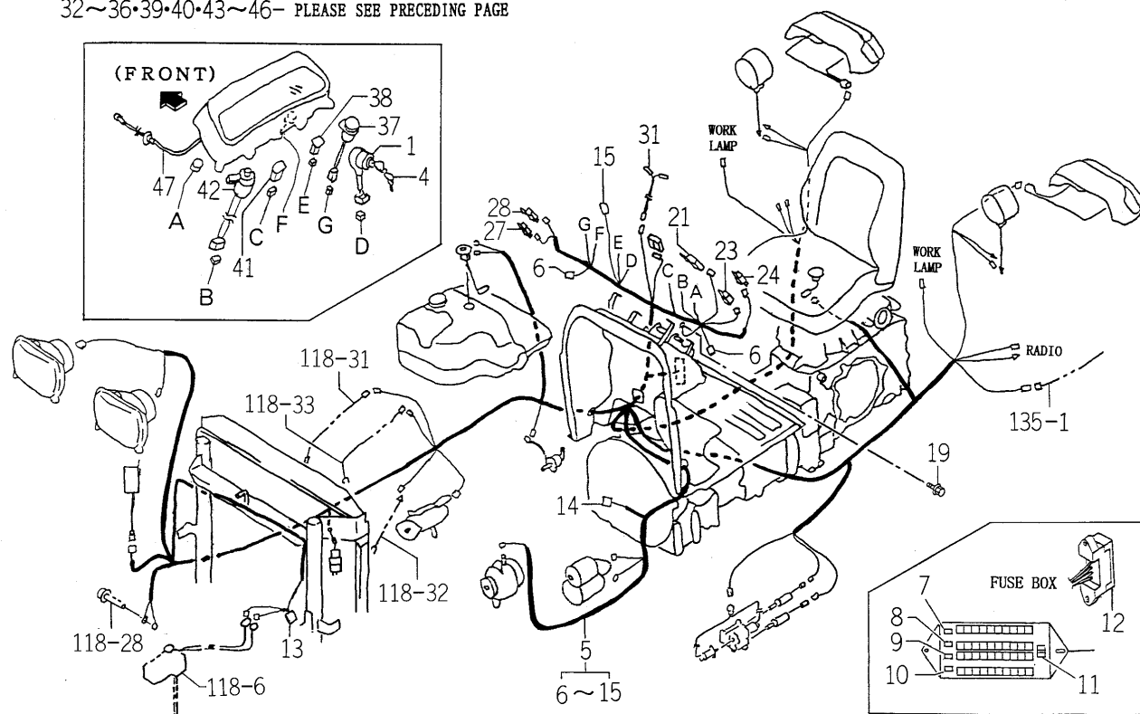
FIG.123 ELC. SYSTEM (MAIN) (PE6 TYPE)(2/2)
