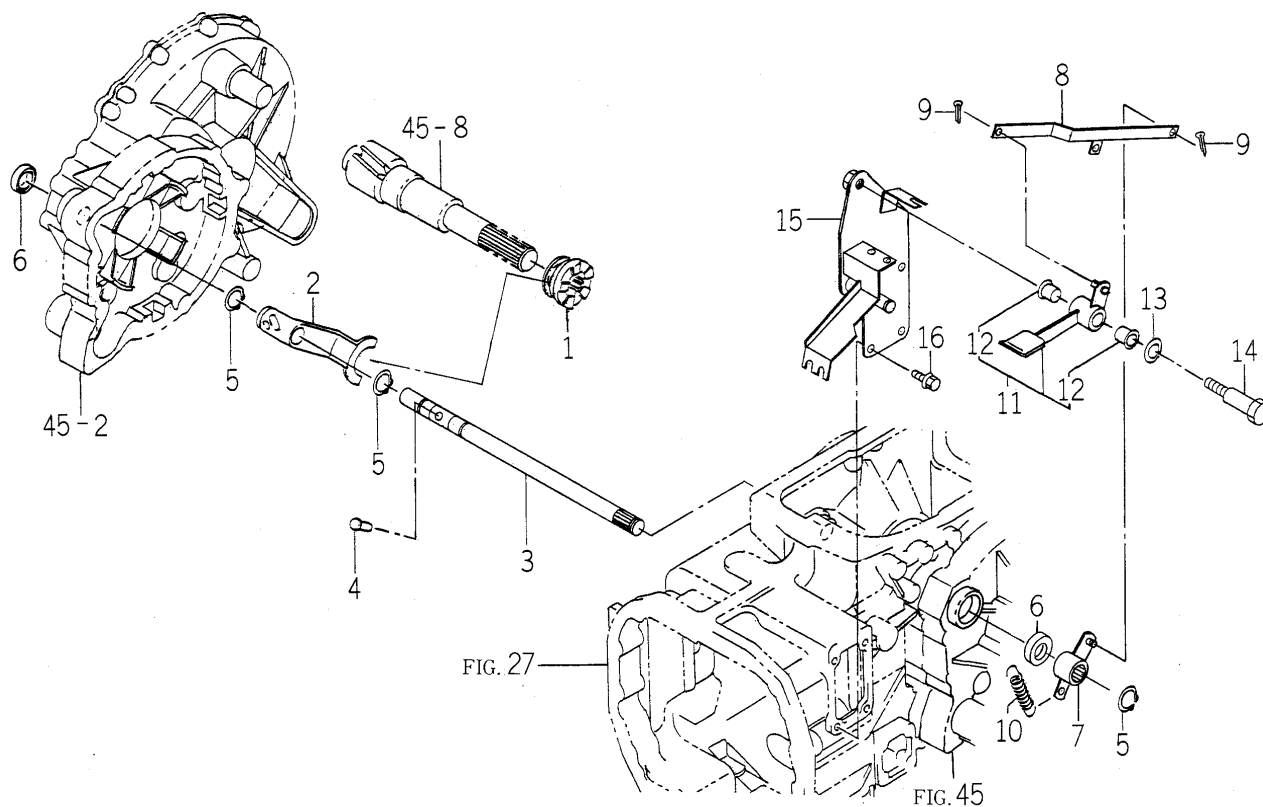
FIG. 47 DIFF-LOCK SYSTEM (H TYPE)
