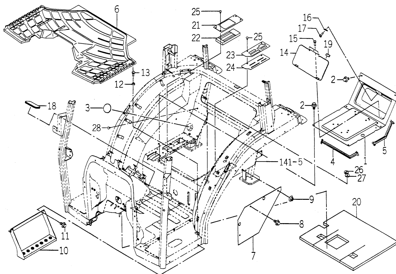
FIG.111 FLOOR (REAR) SYSTEM (HCY TYPE)
