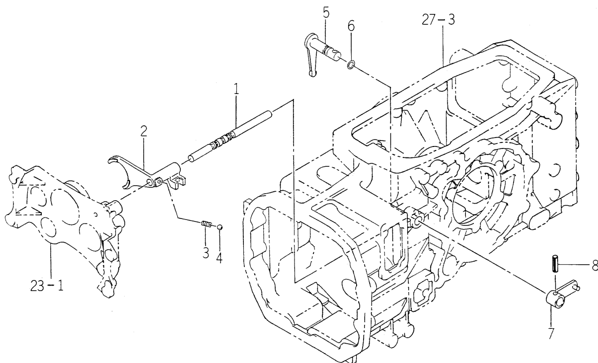
FIG. 33 FORK (SHIFT/SUB) SYSTEM
