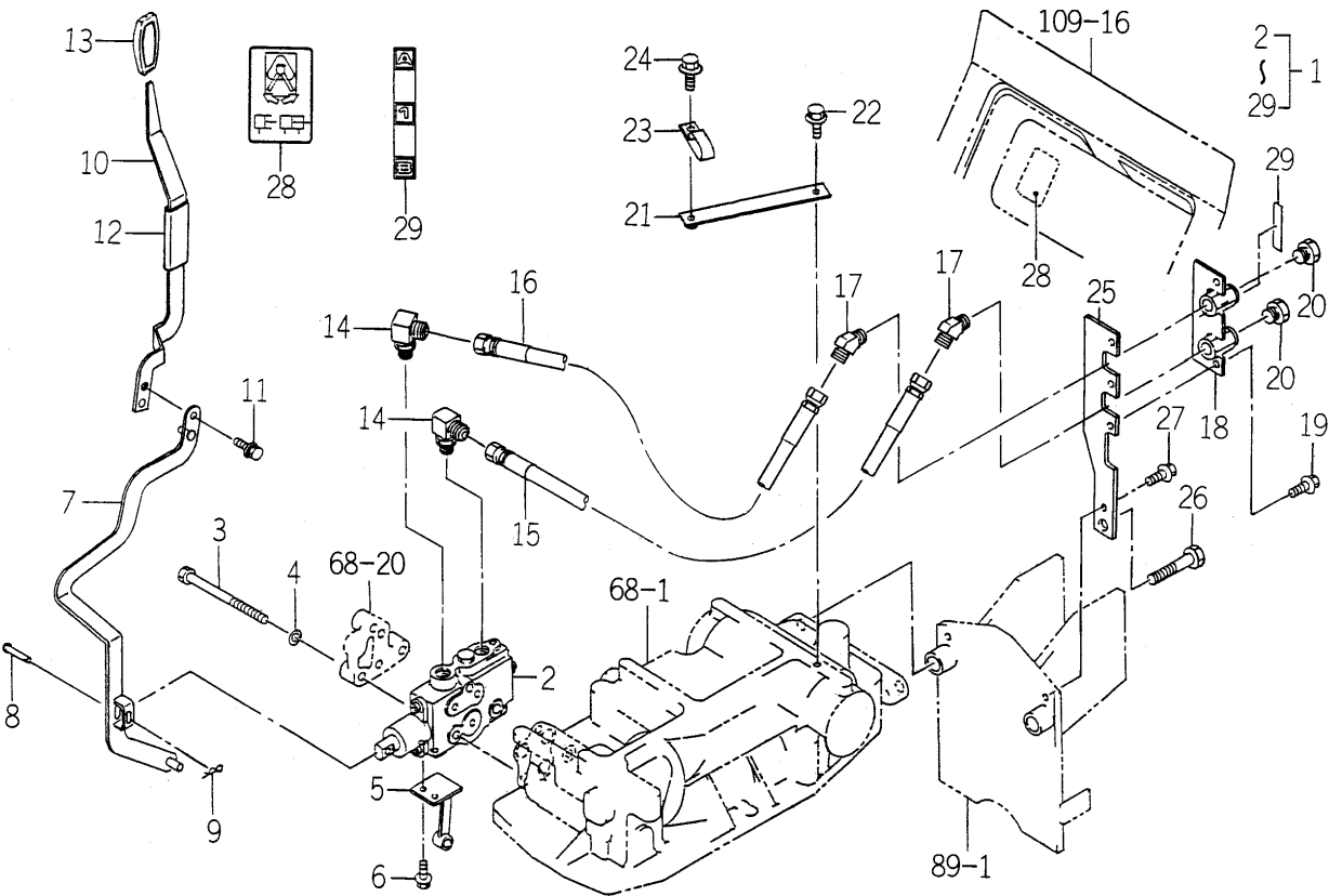
FIG.165 VALVE (REMOTE/1R) SET (E4 TYPE-OPTION)
