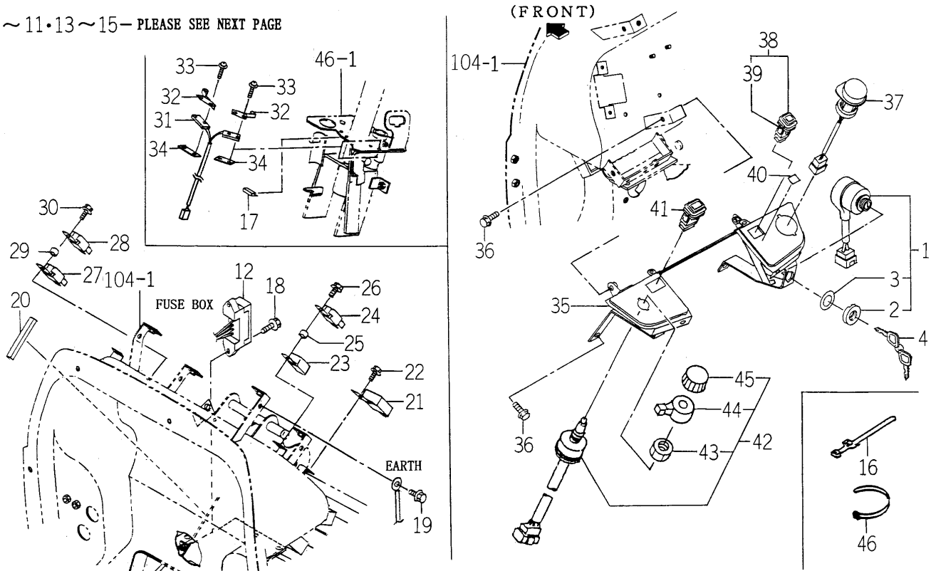
FIG.123 ELC. SYSTEM (MAIN) (PE6 TYPE)(1/2)
