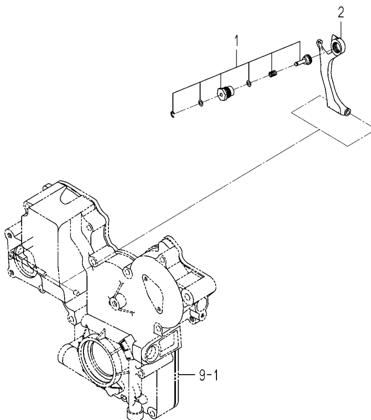
FIG. 22 ADAPTER
