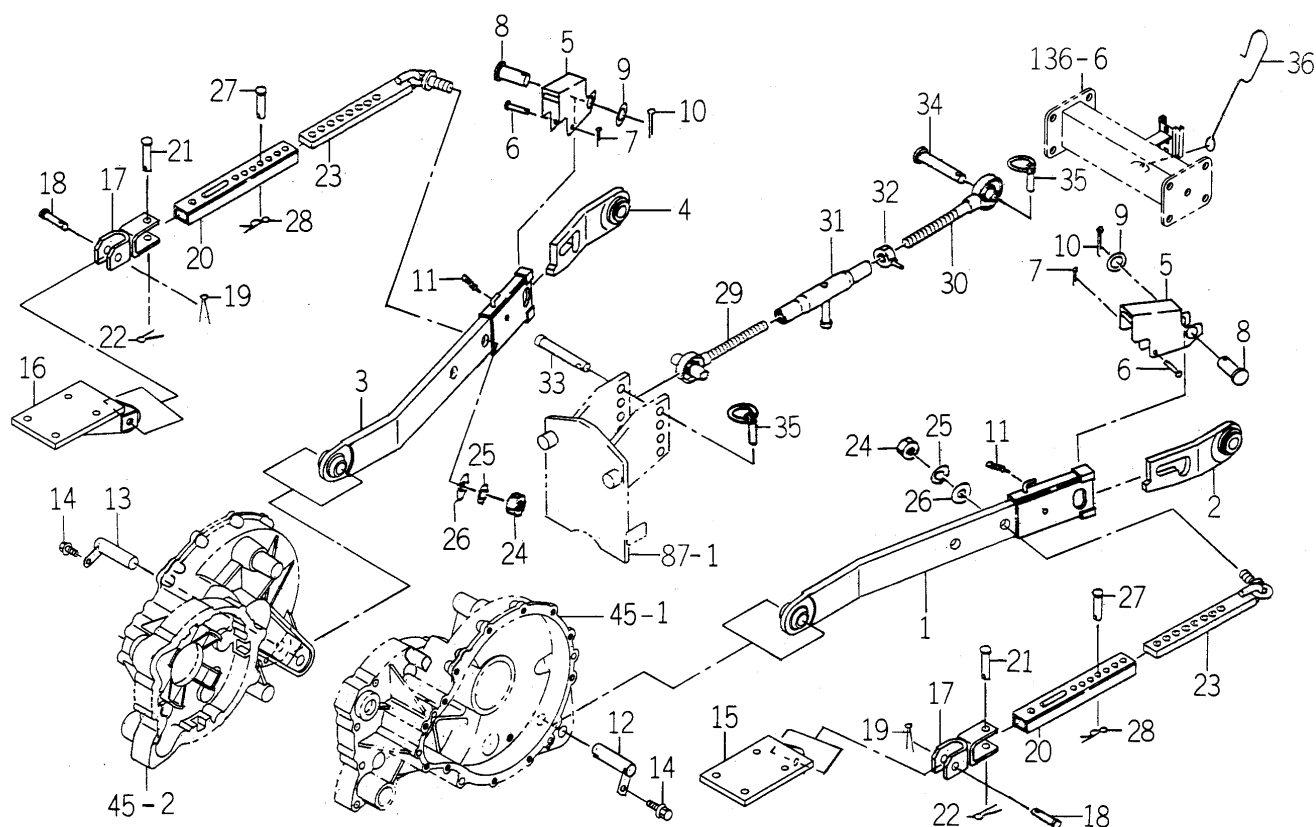
FIG. 81 3P LINK SYSTEM (E6 TYPE EXCEPT CY)
