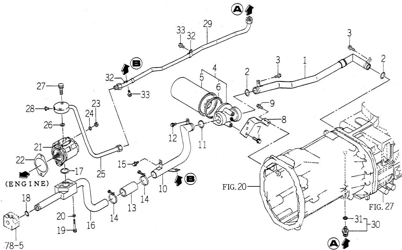
FIG. 73 HYD. SYSTEM (MAIN) (H TYPE)(1/2)
