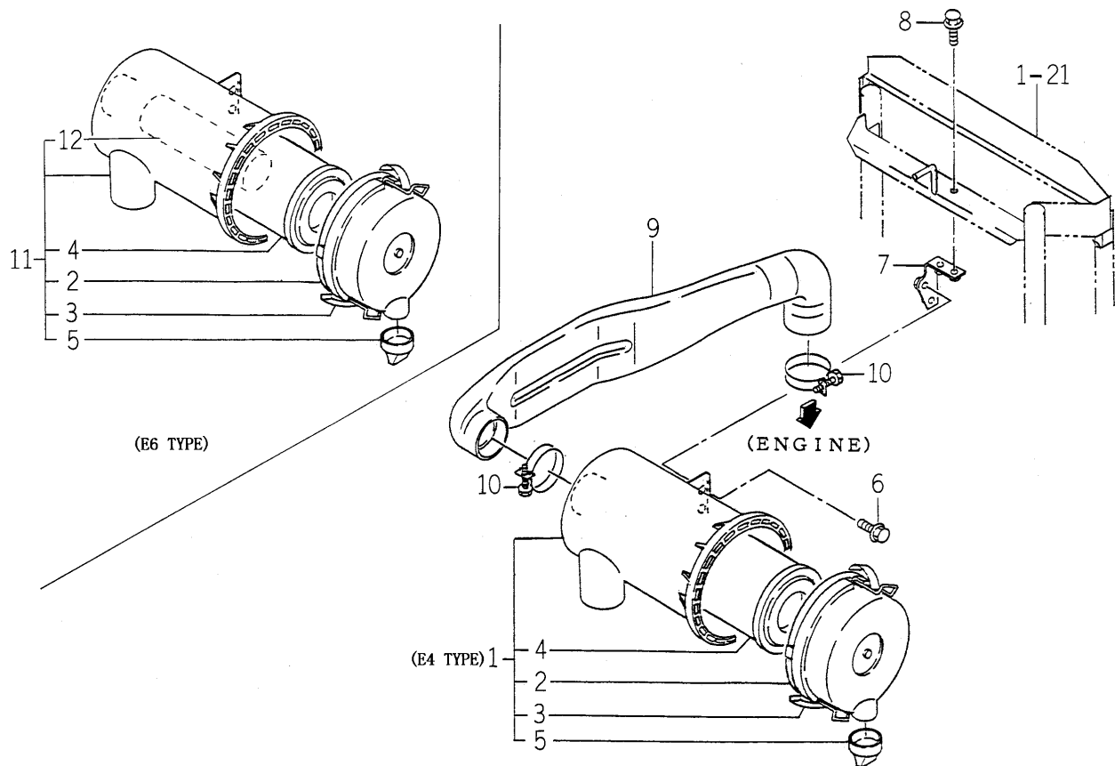
FIG. 4 CLEANER (AIR) SYSTEM
