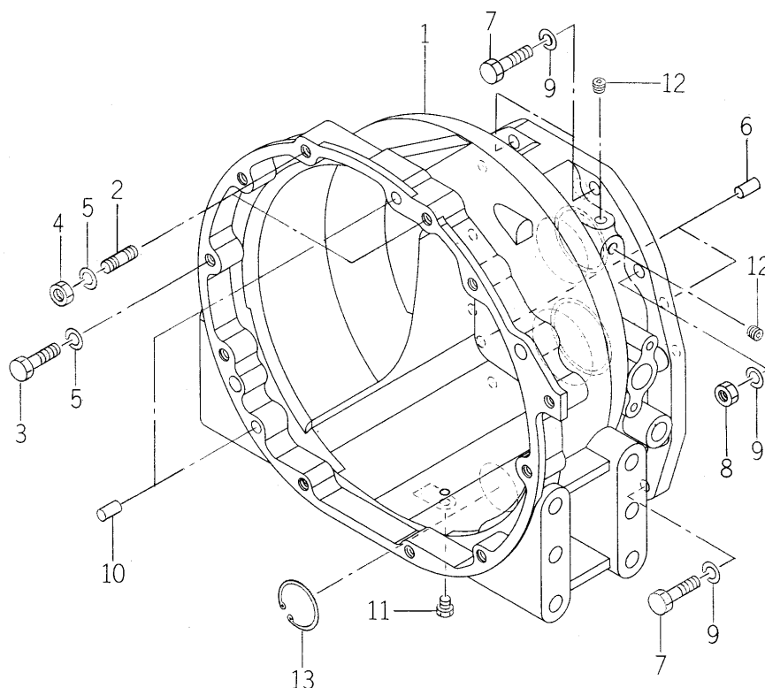
FIG. 14 CASE (TRANSMISSION/FRONT) SYSTEM (H TYPE)
