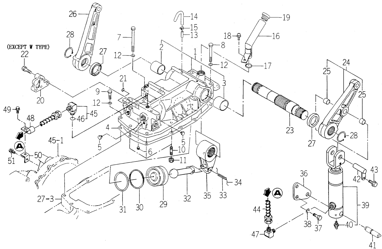
FIG. 68 CYLINDER CASE SYSTEM
