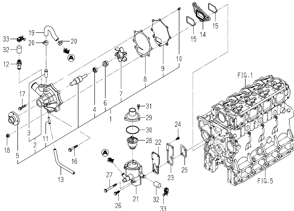
FIG. 17 WATER PUMP
