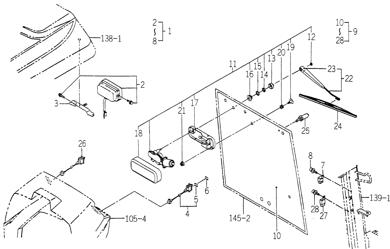
FIG.168 ELC. SYSTEM (CY TYPE-OPTION)
