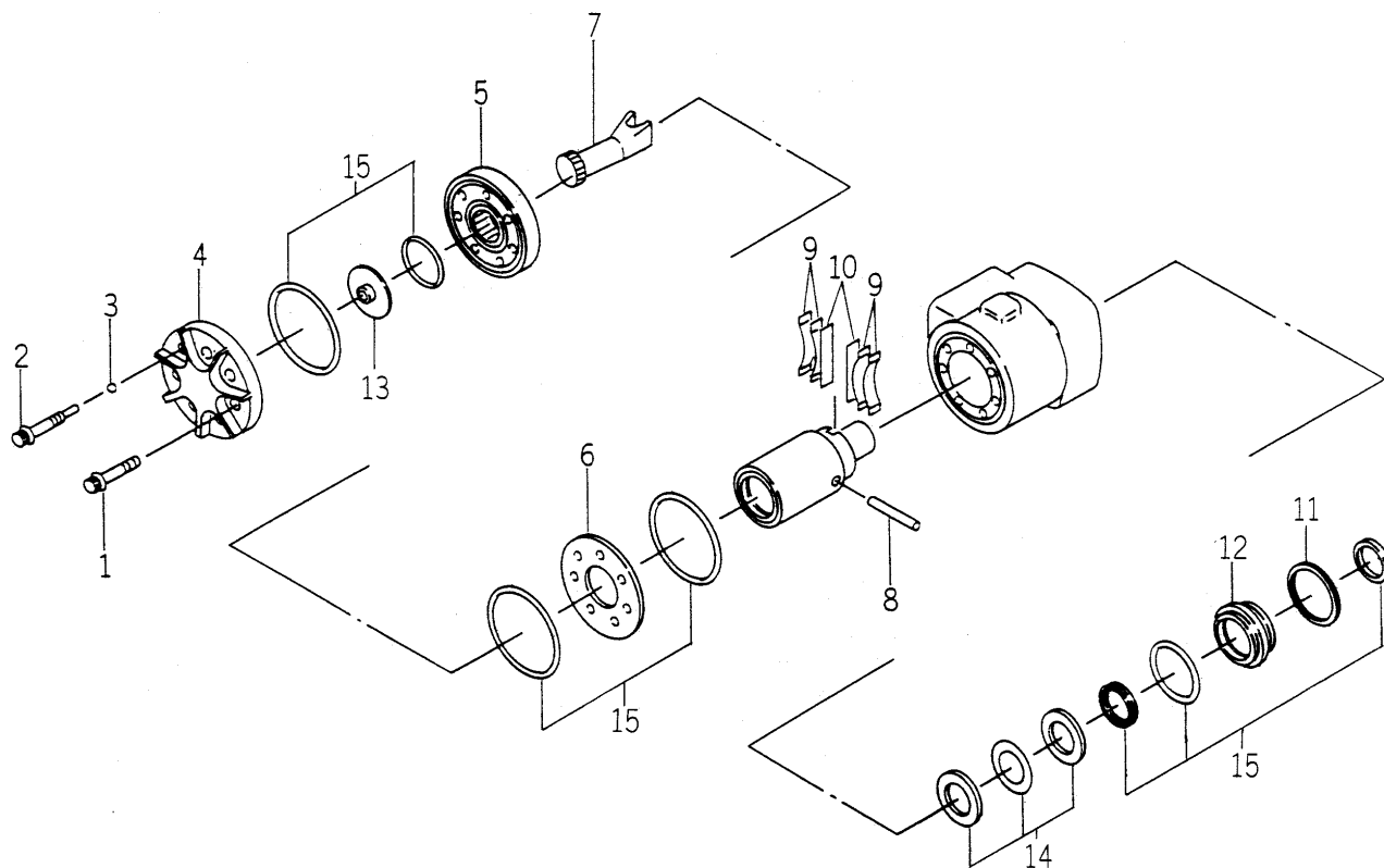
FIG.179 COMPONENT PARTS FOR 1646-407-670-00 ON Fig.57,58
