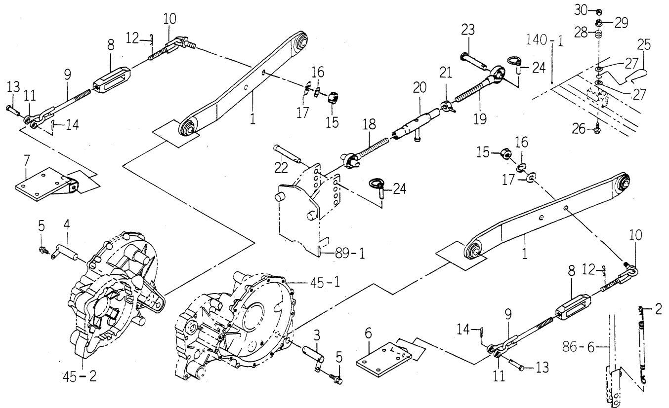
FIG. 84 3P LINK SYSTEM (CYE4 TYPE)
