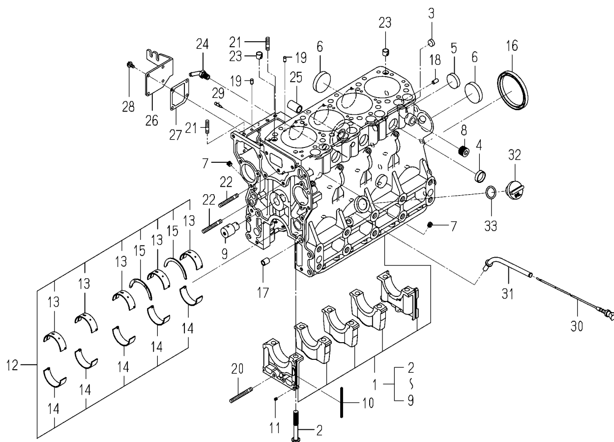
FIG. 5 CYLINDER BLOCK
