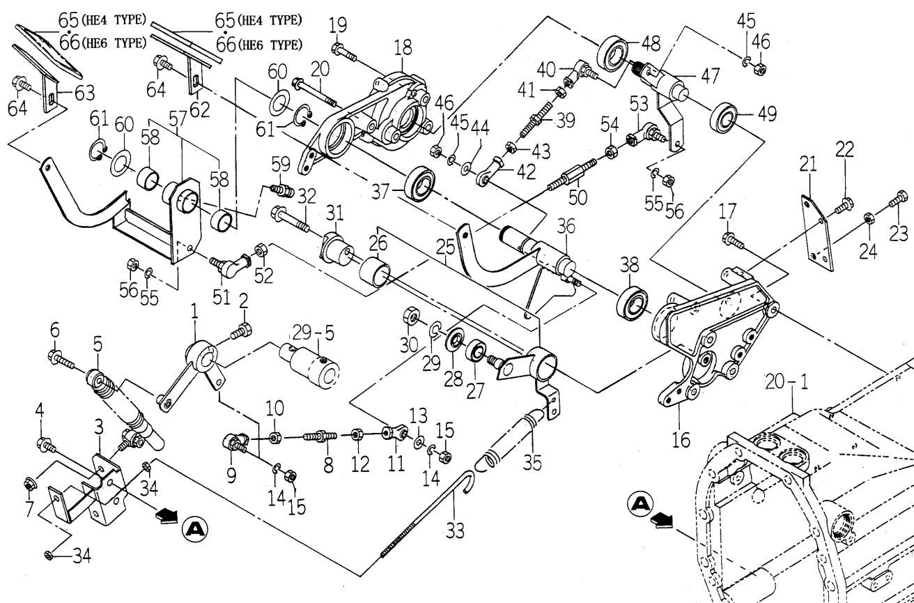
FIG.115 PEDAL (HST) SYSTEM (H TYPE)
