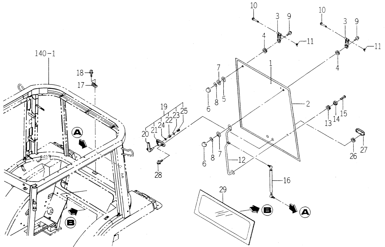
FIG.145 GLASS (REAR) SYSTEM (CY TYPE)
