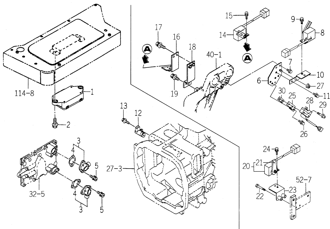
FIG.133 CONTROL SYSTEM (QE4 TYPE)
