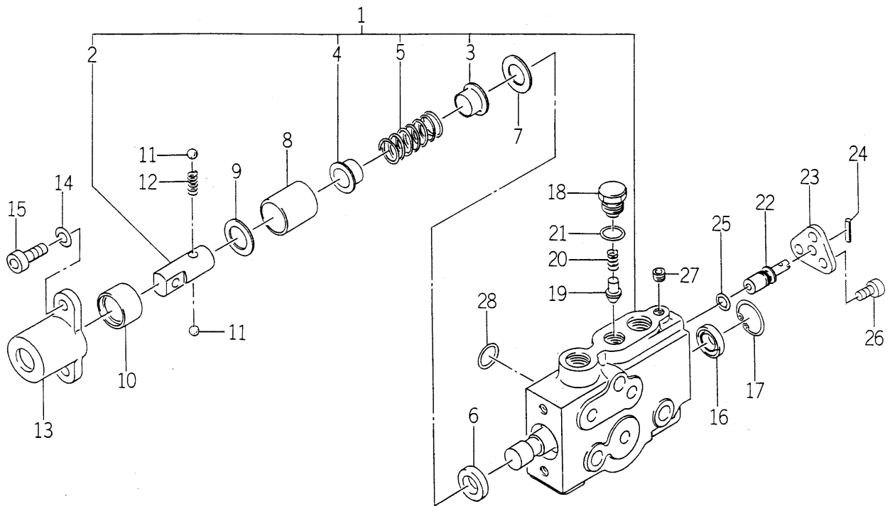
FIG.178 COMPONENT PARTS FOR 1640-530-600-10 ON Fig.80,165,166
