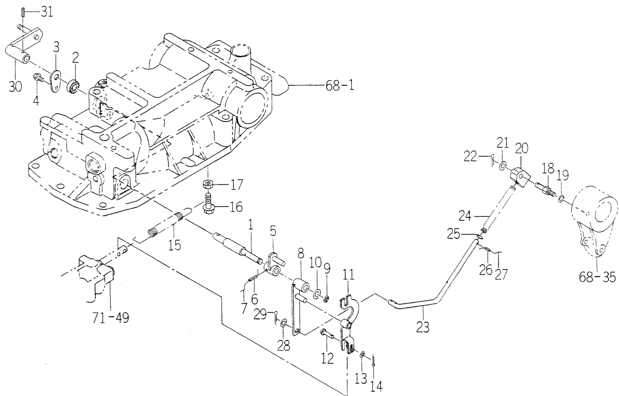
FIG. 69 MECHANICAL LINK(1/2) (POSITION) SYSTEM
