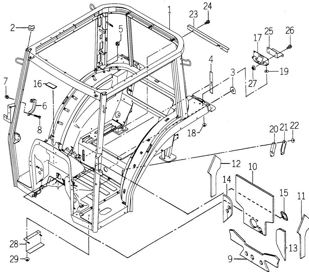
FIG.140 FRAME SYSTEM (CYE4 TYPE EXCEPT H)
