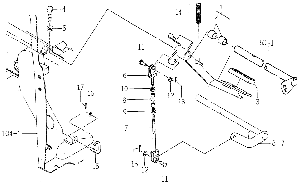
FIG. 9 PEDAL (CLUTCH) SYSTEM (Q,S TYPE)
