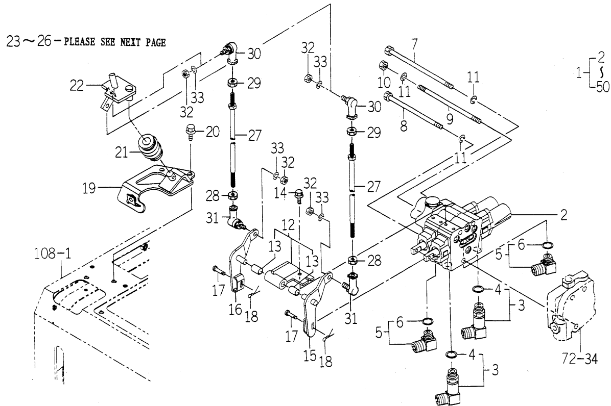
FIG. 79 JOY STICK VALVE SYSTEM (J TYPE-STANDARD/EXCEPT J TYPE-OPTION)(1/2)
