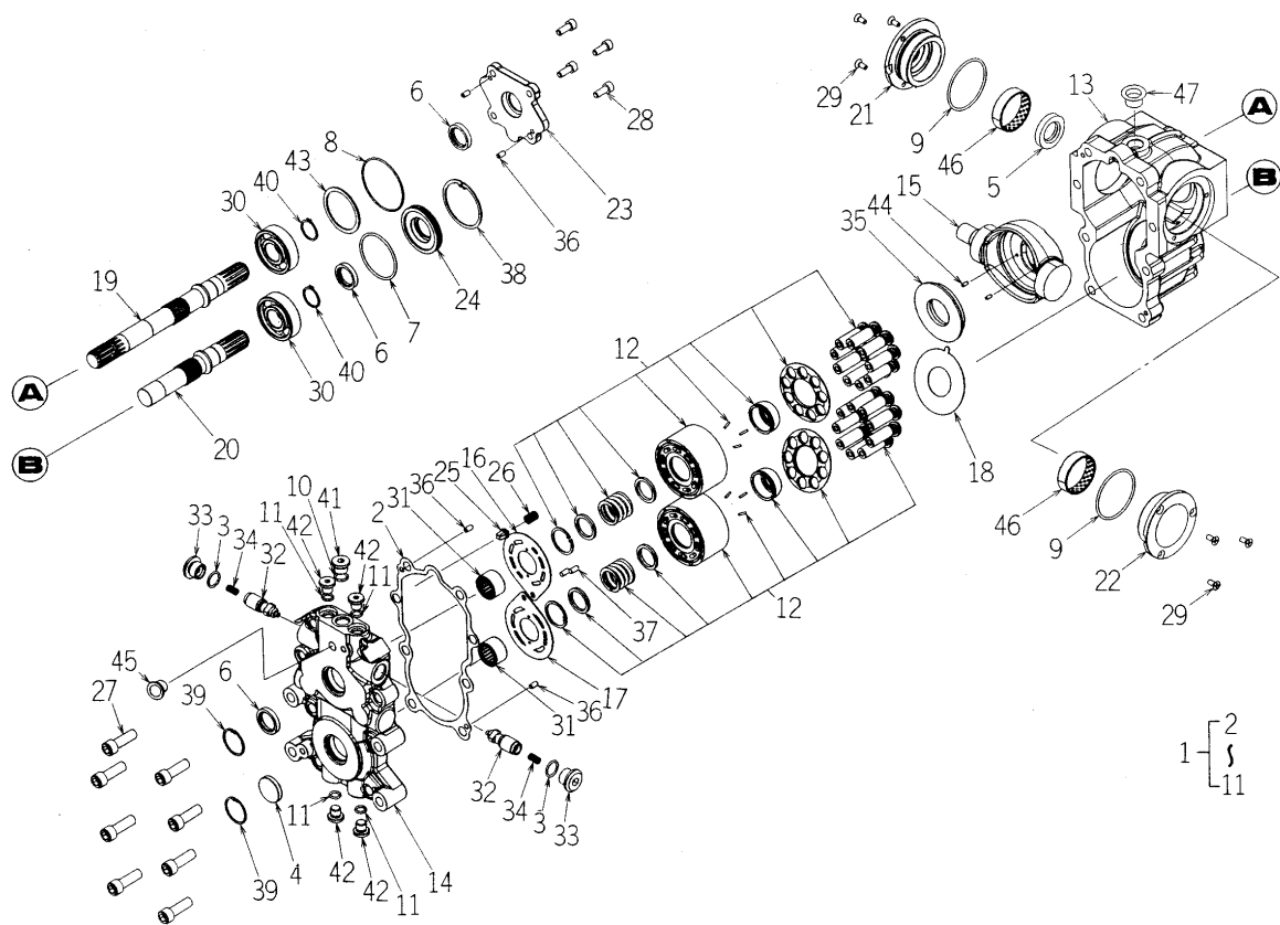
FIG.184 COMPONENT PARTS FOR 1743-203-510-10 ON Fig.17
