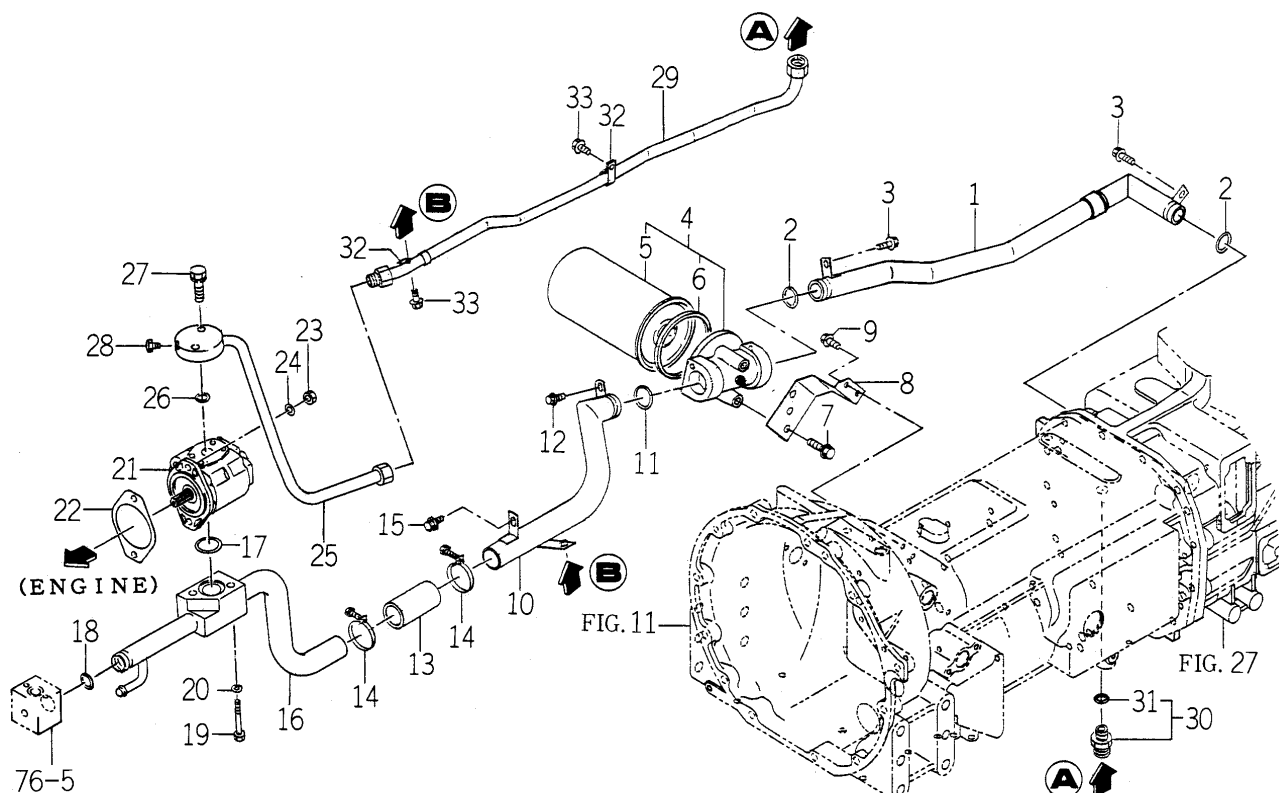
FIG. 72 HYD. SYSTEM (MAIN) (P,Q TYPE)(1/2)
