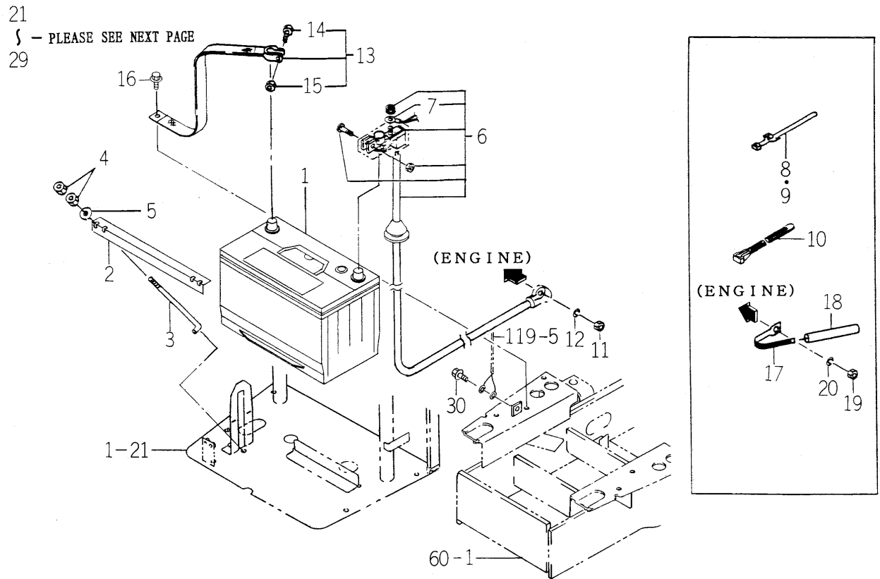
FIG.117 ELC. SYSTEM (FRONT) (E4 TYPE)(1/2)
