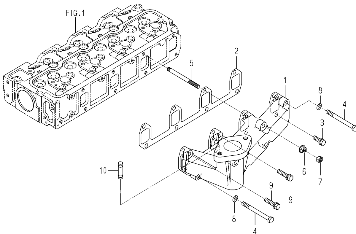
FIG. 4 EXHAUST MANIFOLD
