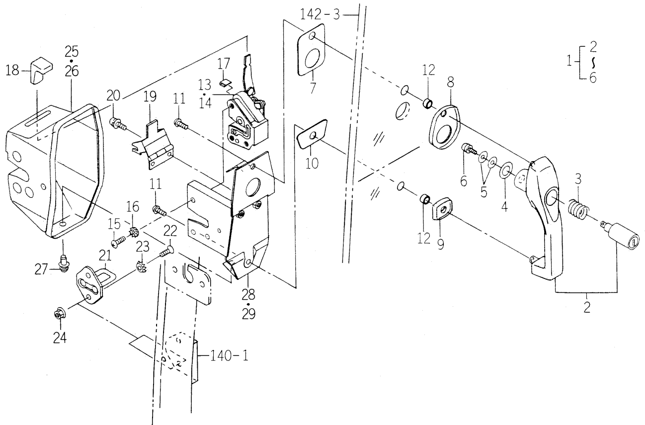
FIG.143 LOCK (DOOR) SYSTEM (CY TYPE)
