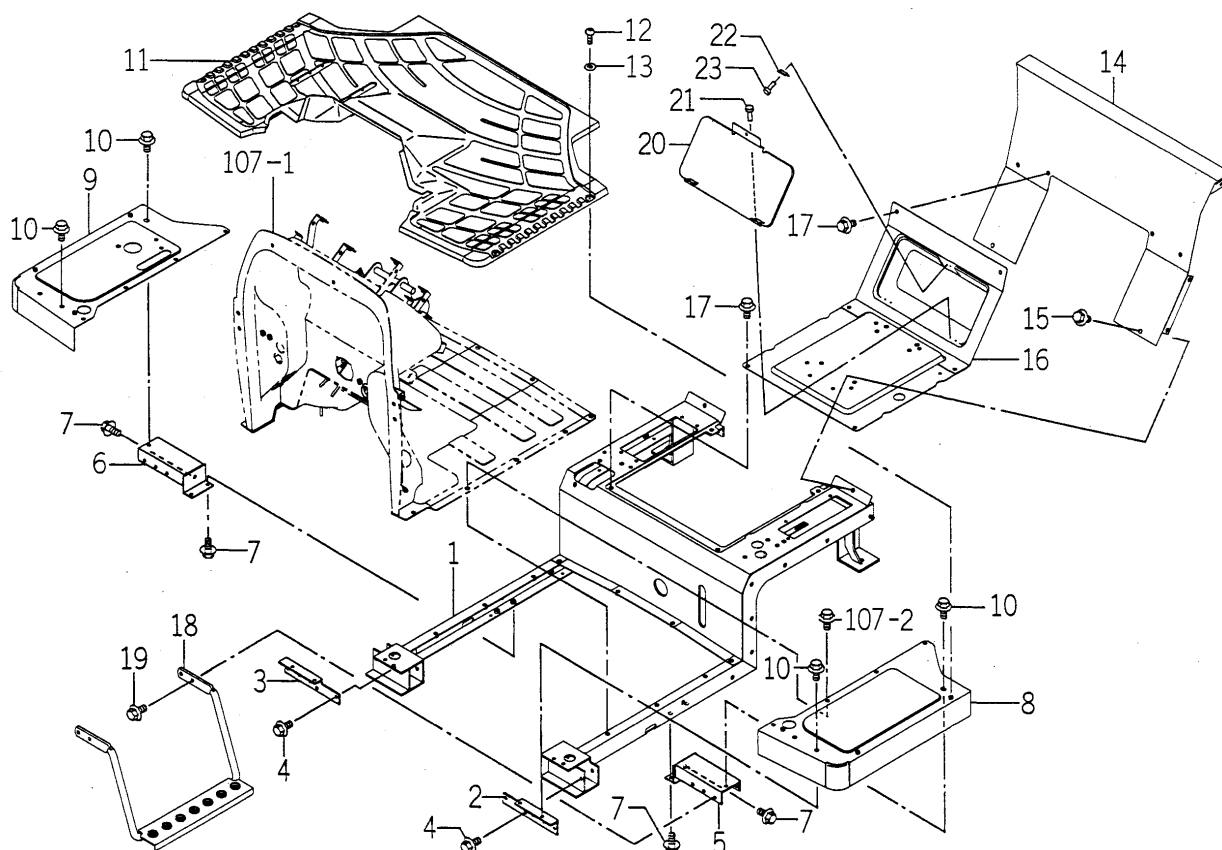
FIG.113 FLOOR (REAR) SYSTEM (HE6 TYPE EXCEPT CY)
