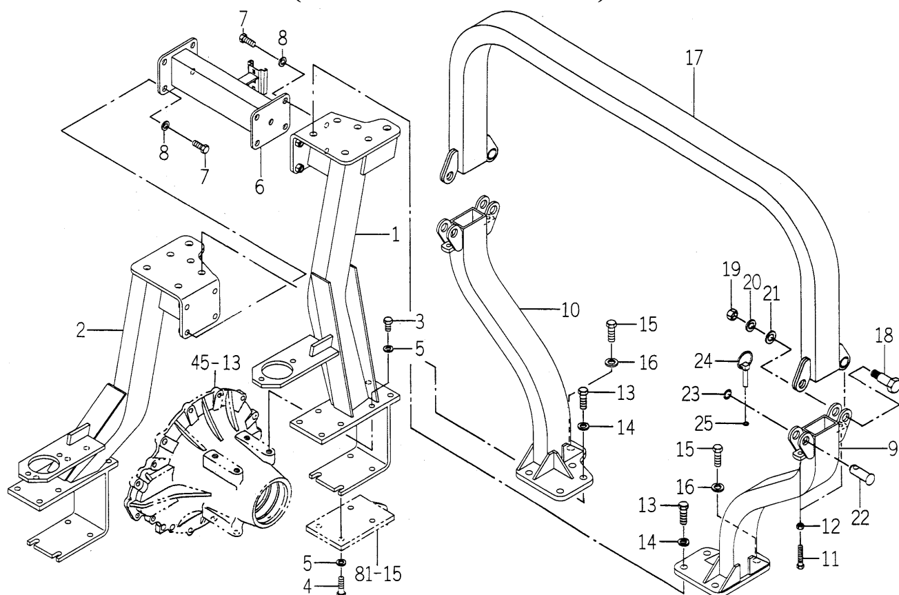
FIG.136 FRAME (REAR) SYSTEM (E6 TYPE EXCEPT CY)
