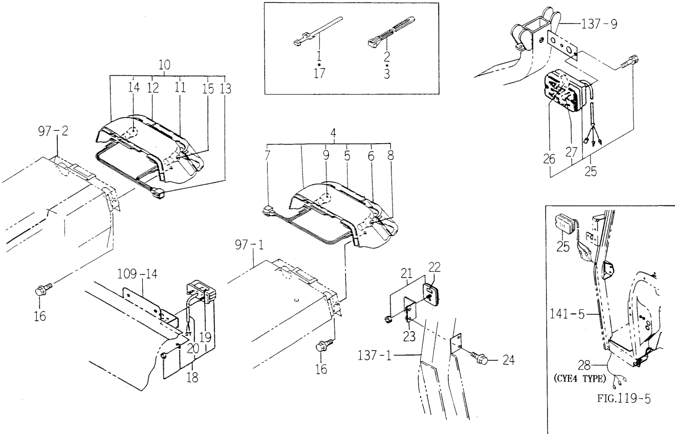
FIG.126 ELC. SYSTEM (REAR) (E4 TYPE)
