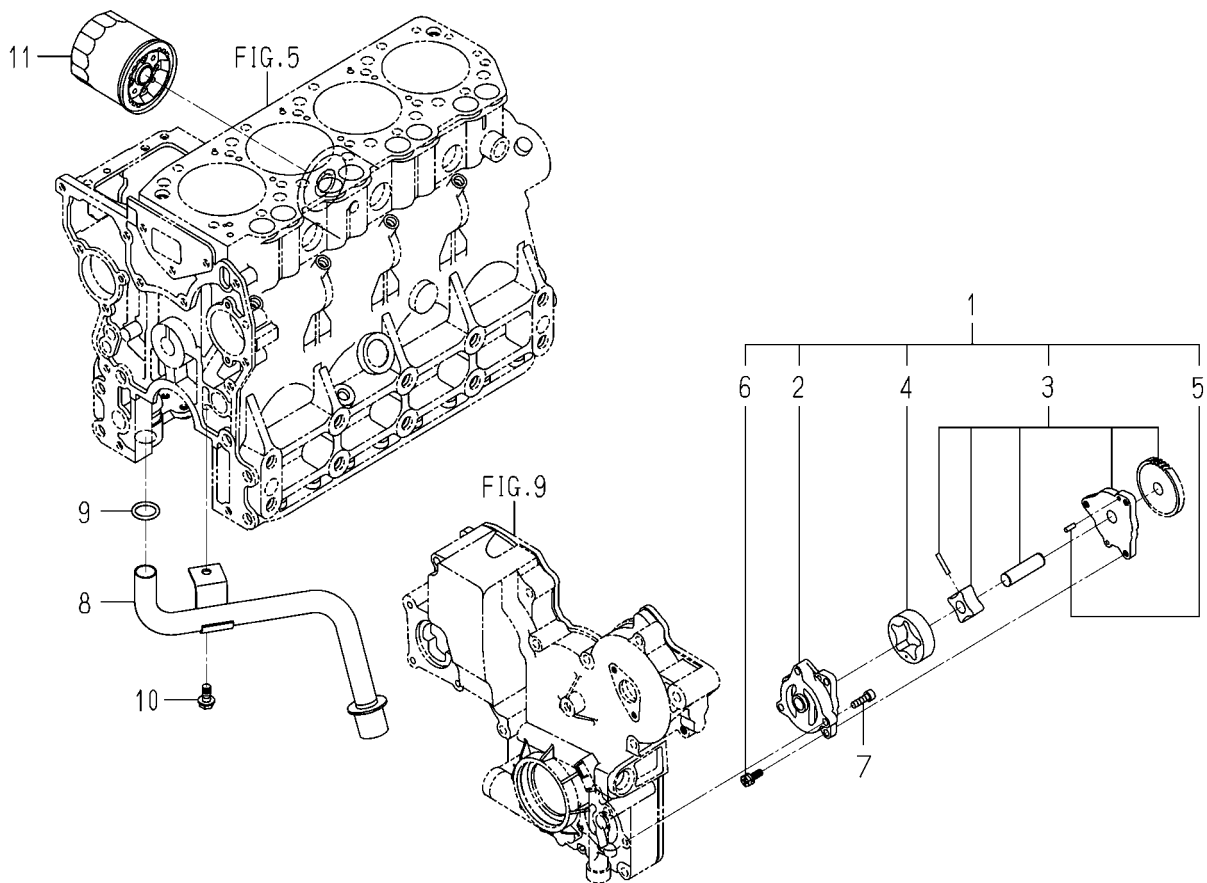
FIG. 16 OIL PUMP
