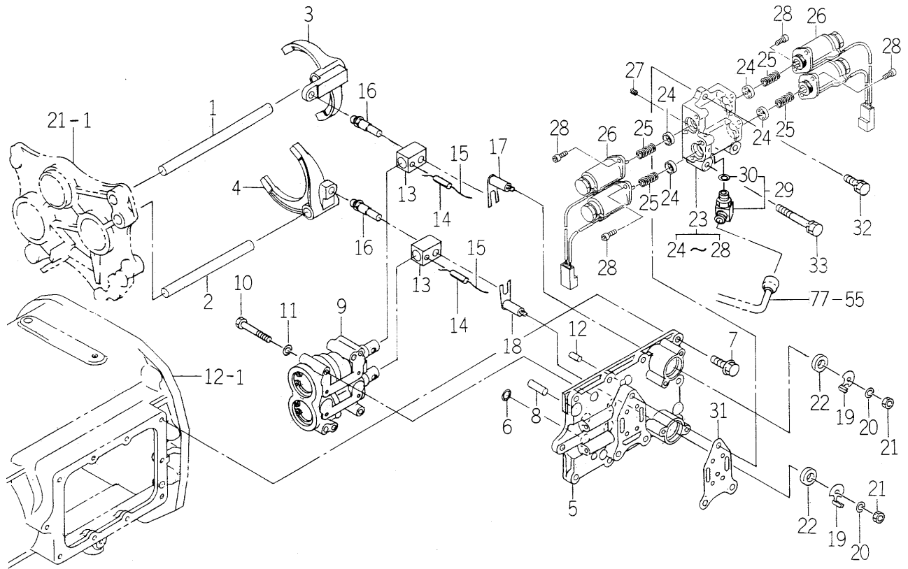
FIG. 32 FORK (SHIFT/MAIN) SYSTEM (Q TYPE)
