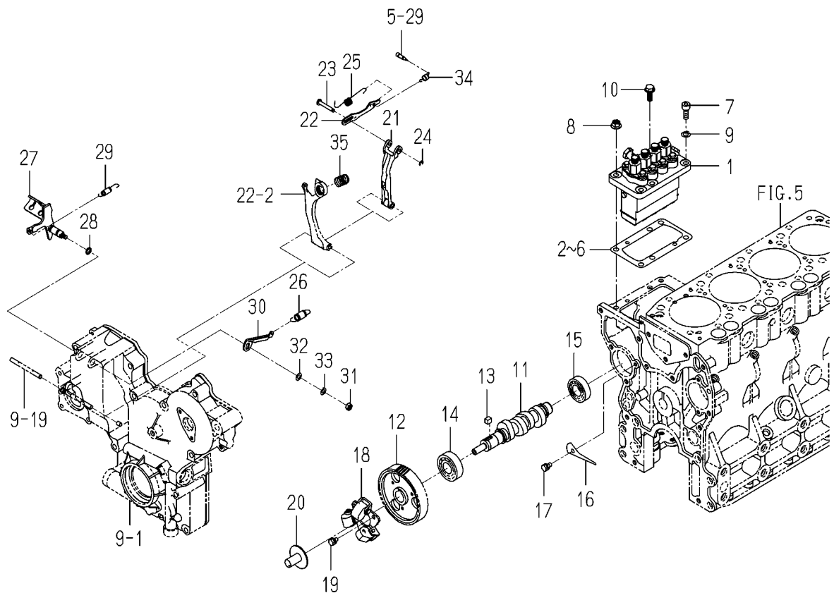
FIG. 20 INJECTION PUMP
