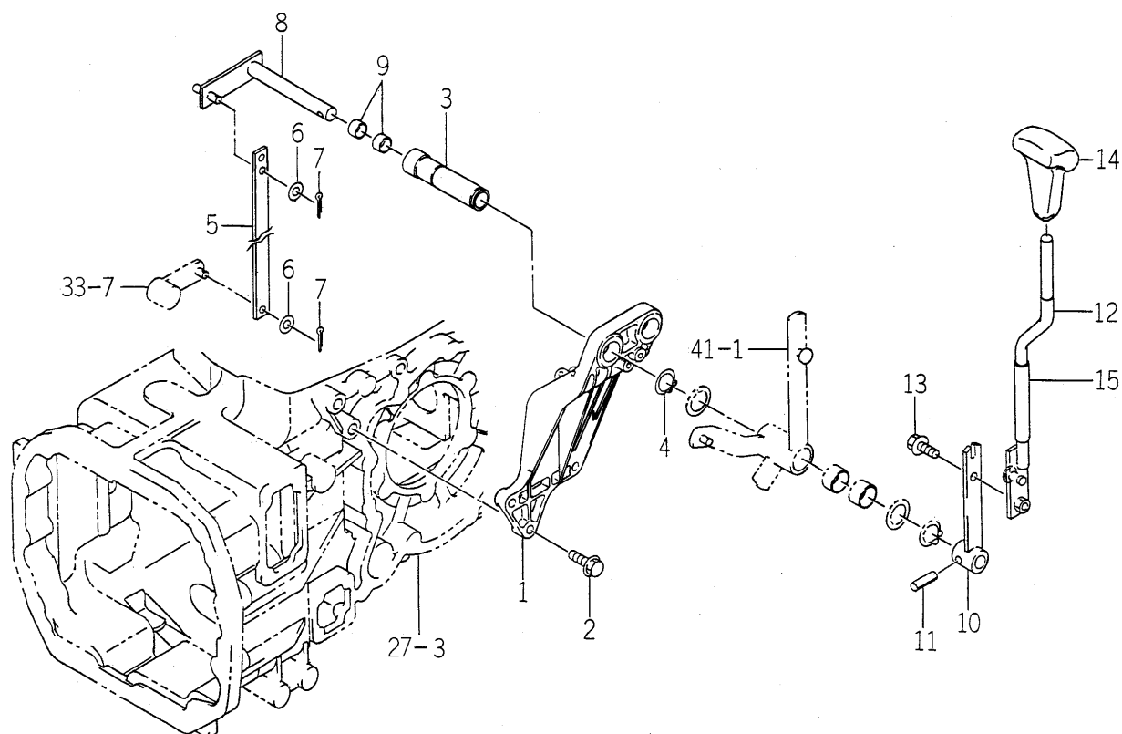
FIG. 39 LEVER (SHIFT/SUB) SYSTEM (EXCEPT Q TYPE)
