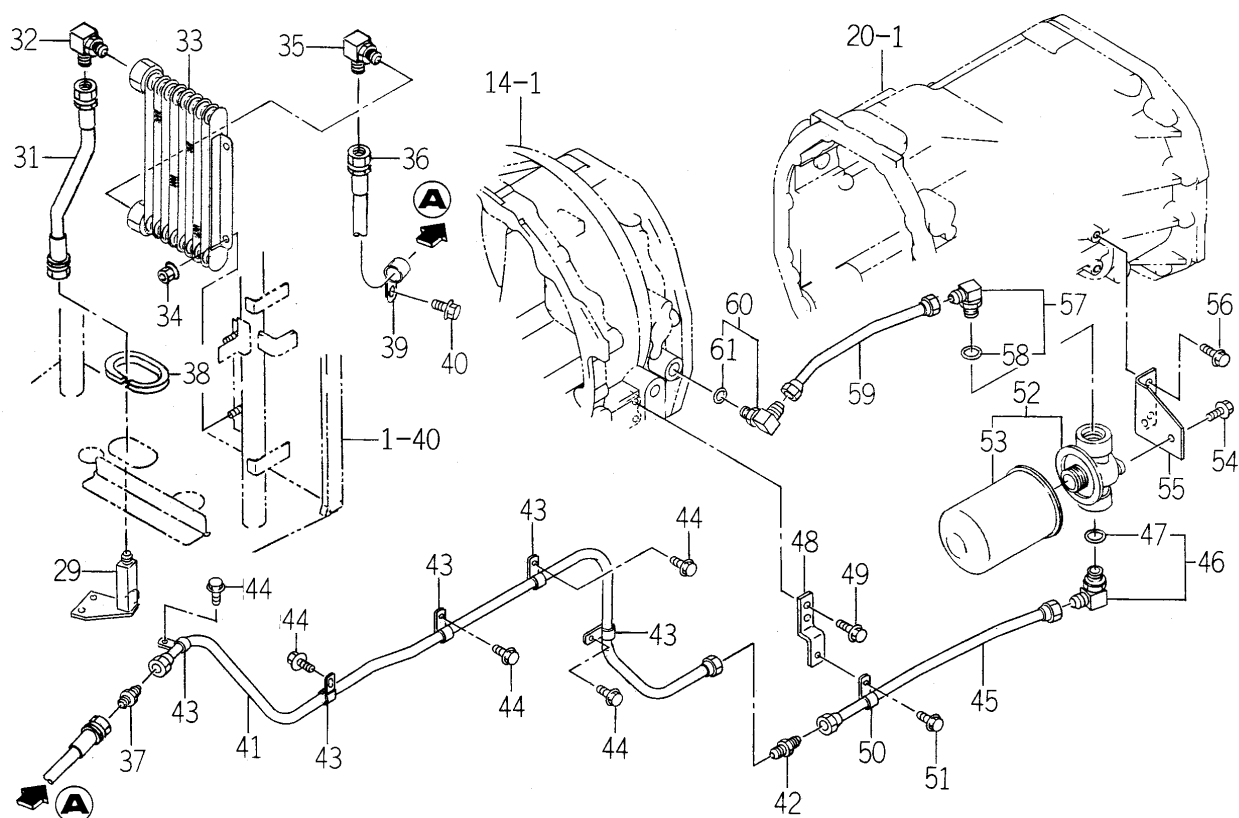
FIG. 78 HYD. SYSTEM (SUB) (H TYPE)(2/2)
