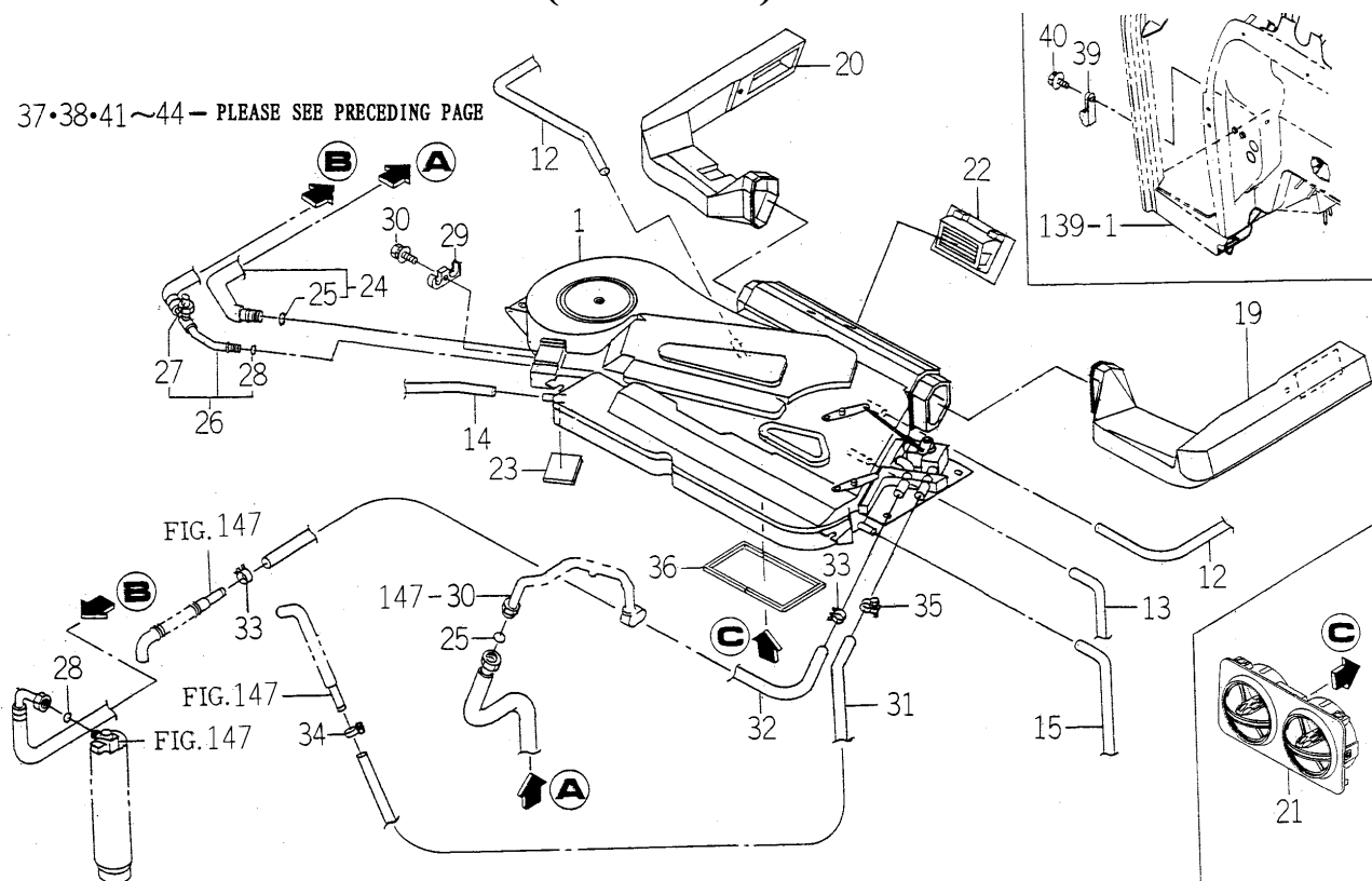
FIG.148 AIR CONDITIONER (CABIN) SYSTEM(2/2) (CY TYPE)
