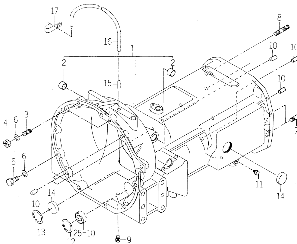
FIG. 13 CASE (TRANSMISSION/FRONT) SYSTEM (S TYPE)
