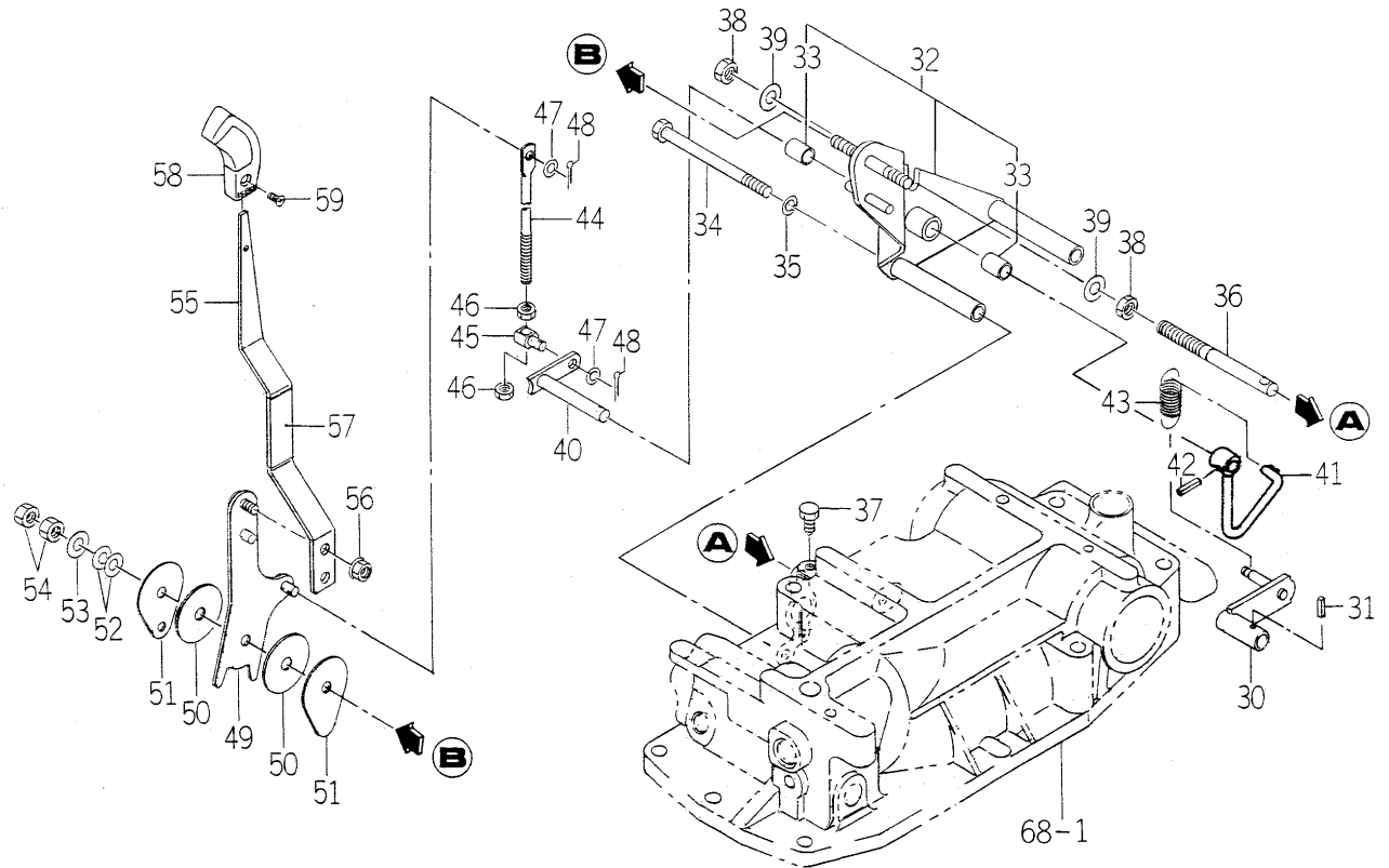
FIG. 69 MECHANICAL LINK(2/2) (POSITION) SYSTEM
