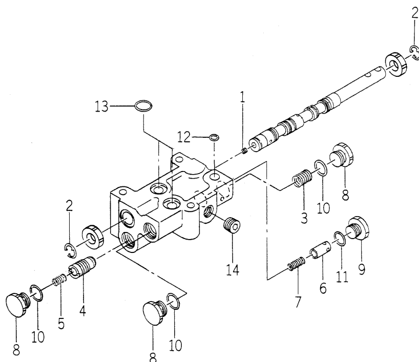
FIG.174 COMPONENT PARTS FOR K211-073-000-00 ON Fig.71-73
