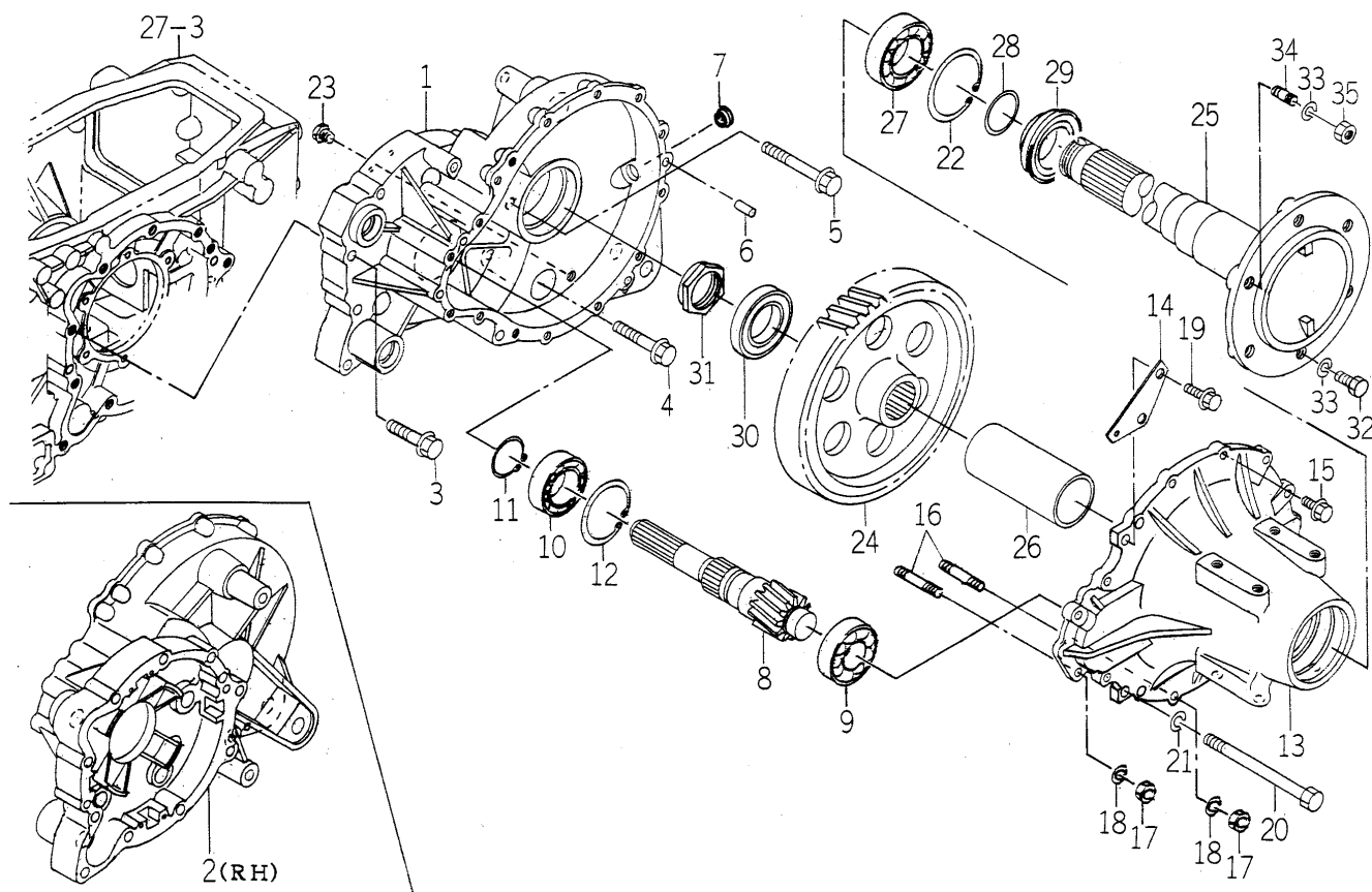
FIG. 45 HOUSING (AXLE) SYSTEM
