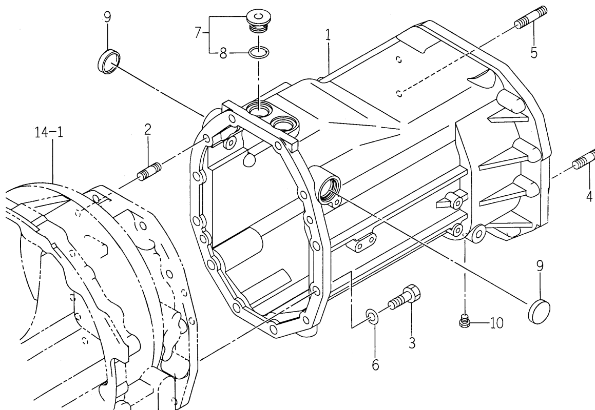
FIG. 20 CASE (TRANSMISSION/MID) SYSTEM (H TYPE)
