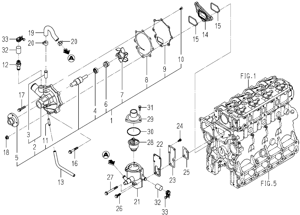
FIG. 17 WATER PUMP
