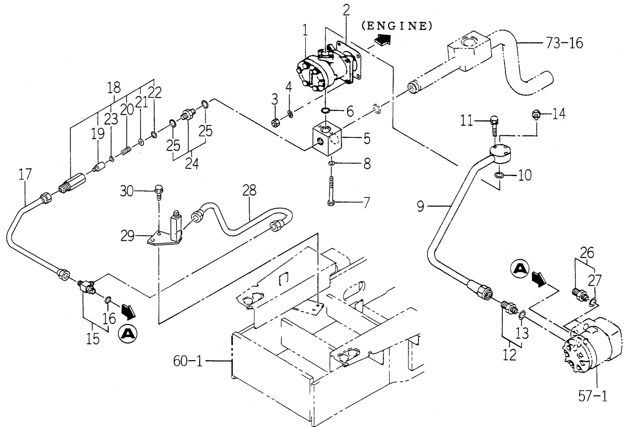
FIG. 78 HYD. SYSTEM (SUB) (H TYPE)(1/2)
