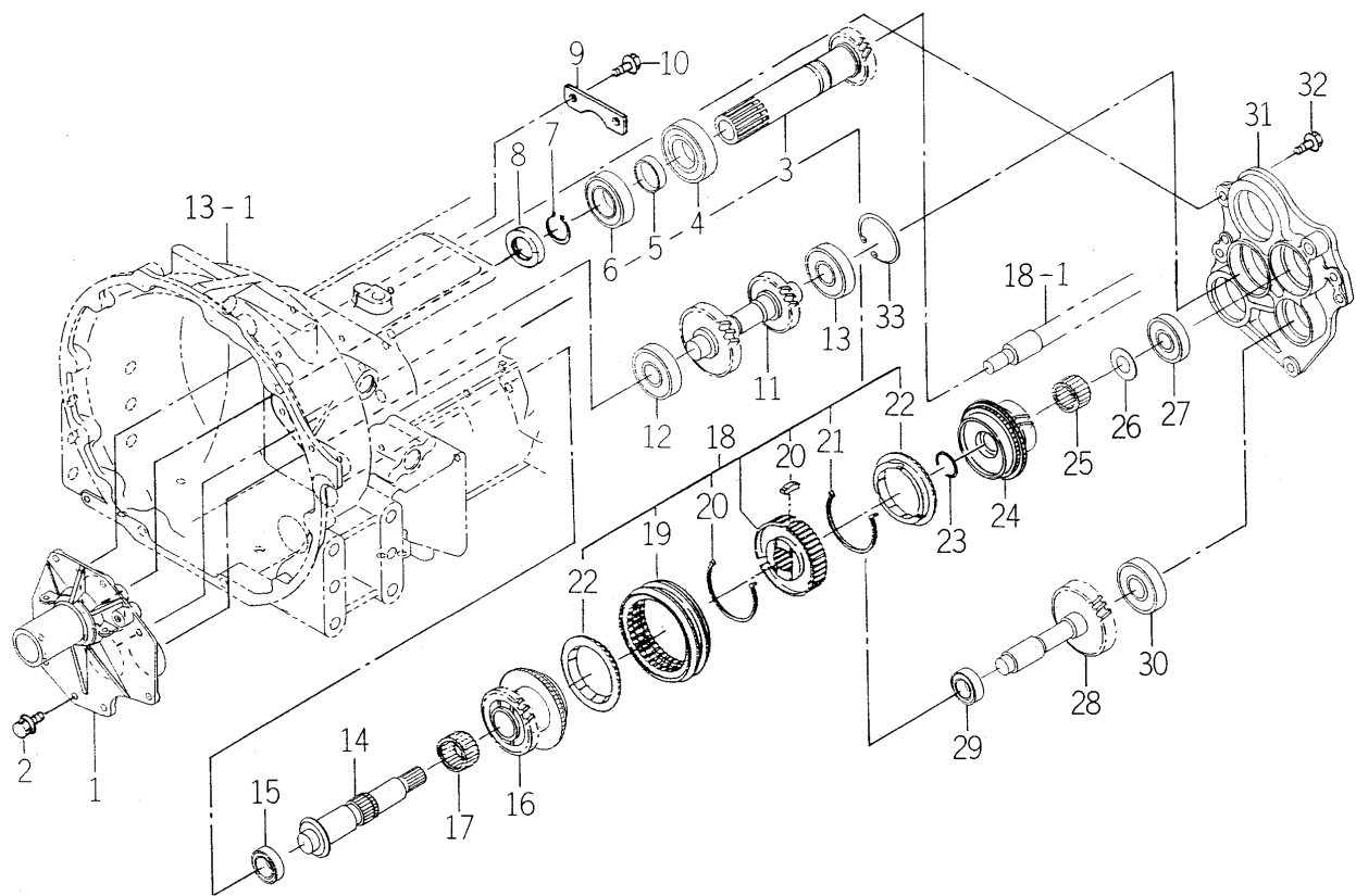
FIG. 16 GEAR (REVERSE) SYSTEM (S TYPE)
