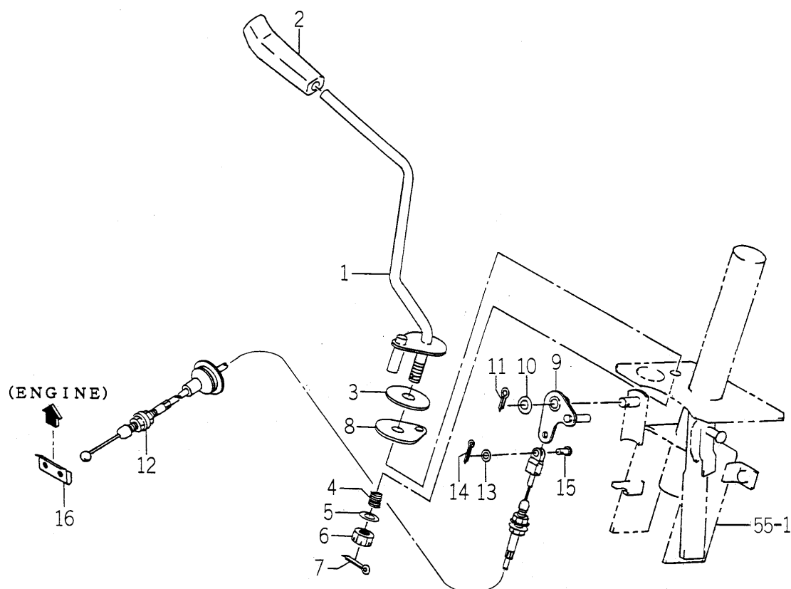
FIG. 7 ACCELERATOR SYSTEM (H TYPE)
