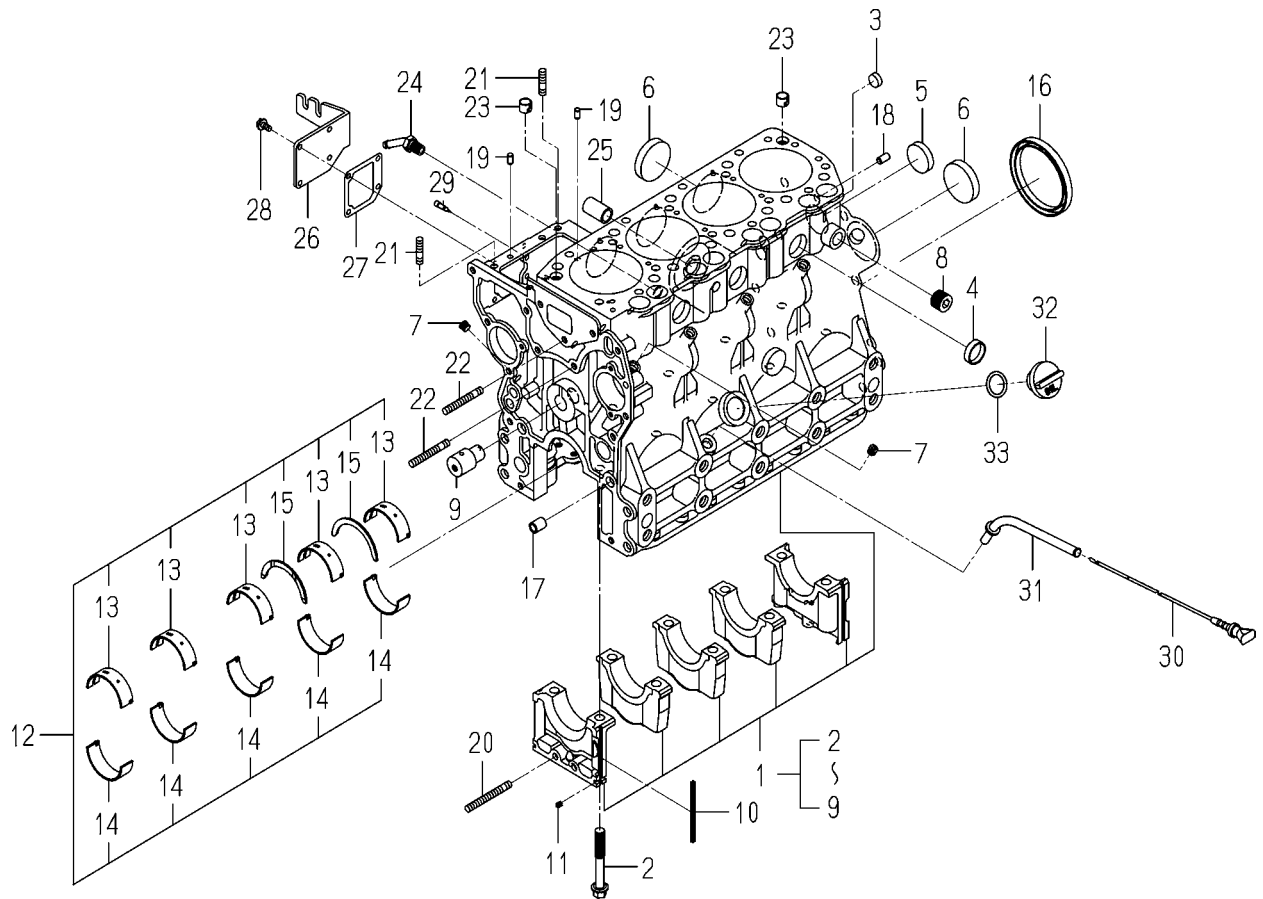
FIG. 5 CYLINDER BLOCK
