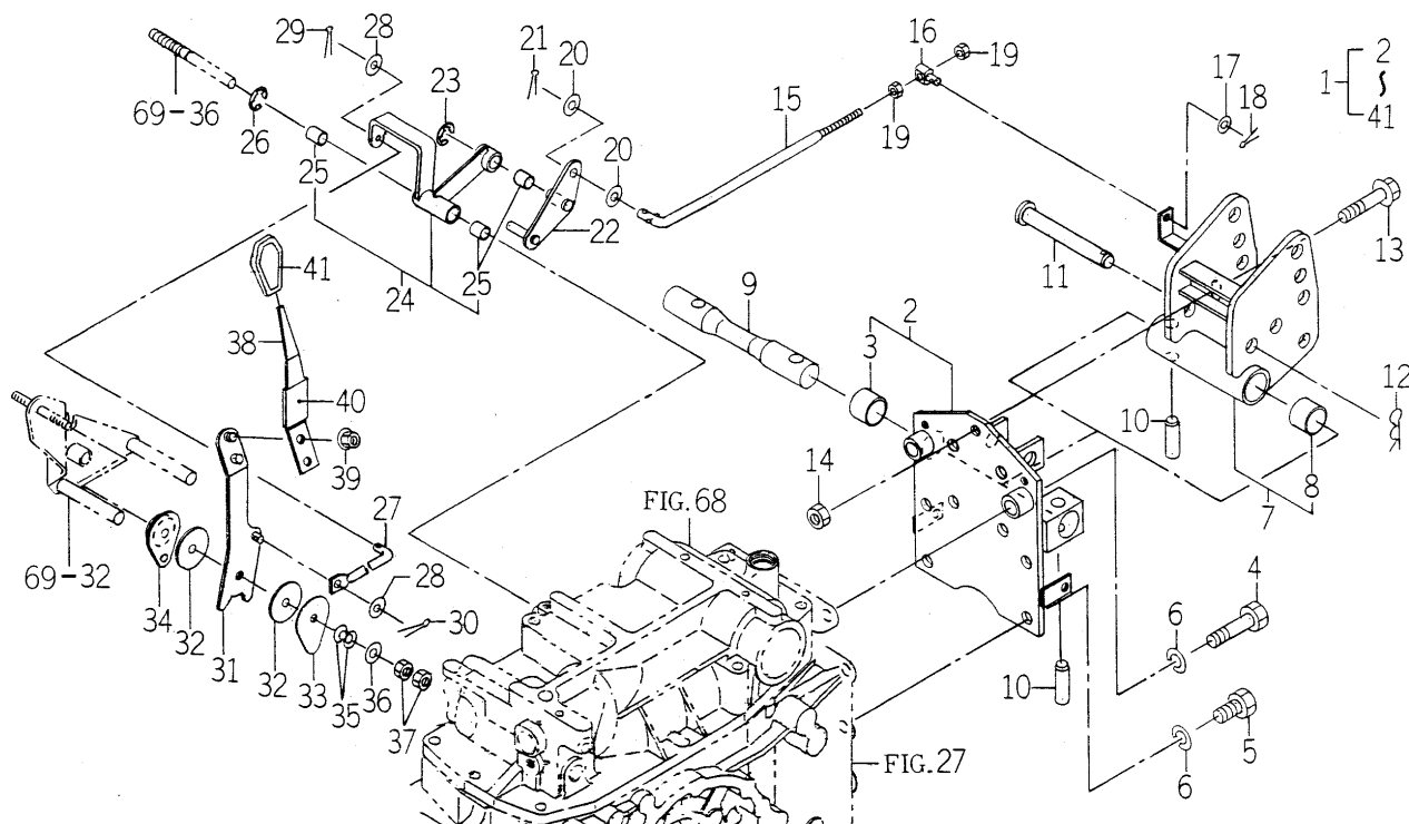
FIG. 70 MECHANICAL LINK (DRAFT) SET (S TYPE-STANDARD/EXCEPT S TYPE-OPTION)
