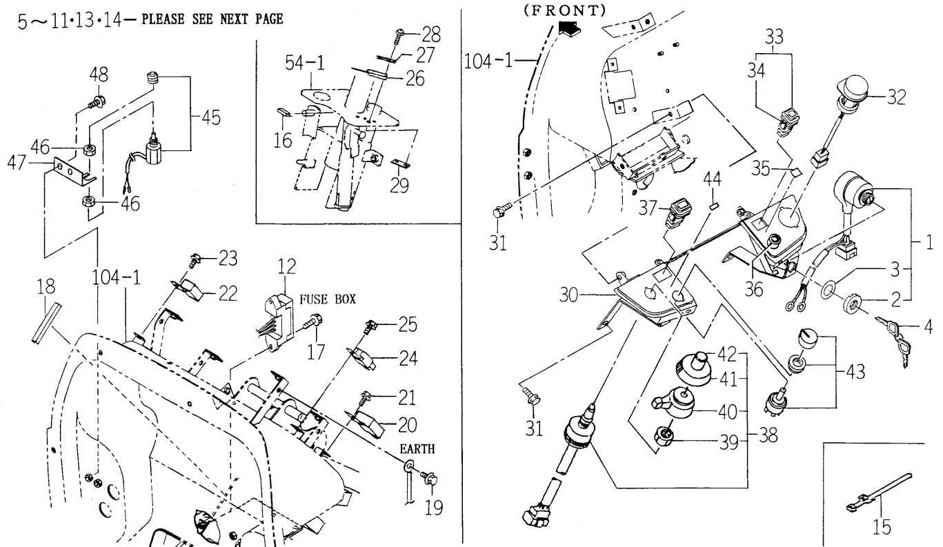
FIG.120 ELC. SYSTEM (MAIN) (SE4 TYPE)(1/2)
