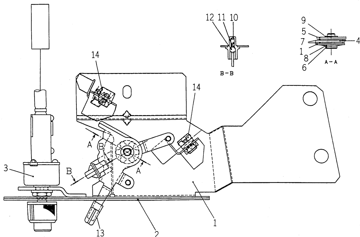
FIG.182 COMPONENT PARTS FOR 1729-782-610-10 ON Fig.148
