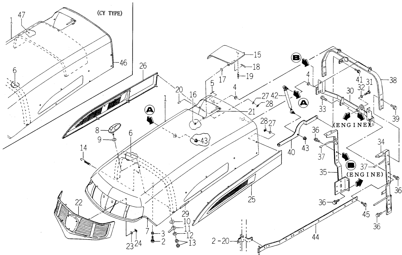
FIG. 93 HOOD SYSTEM
