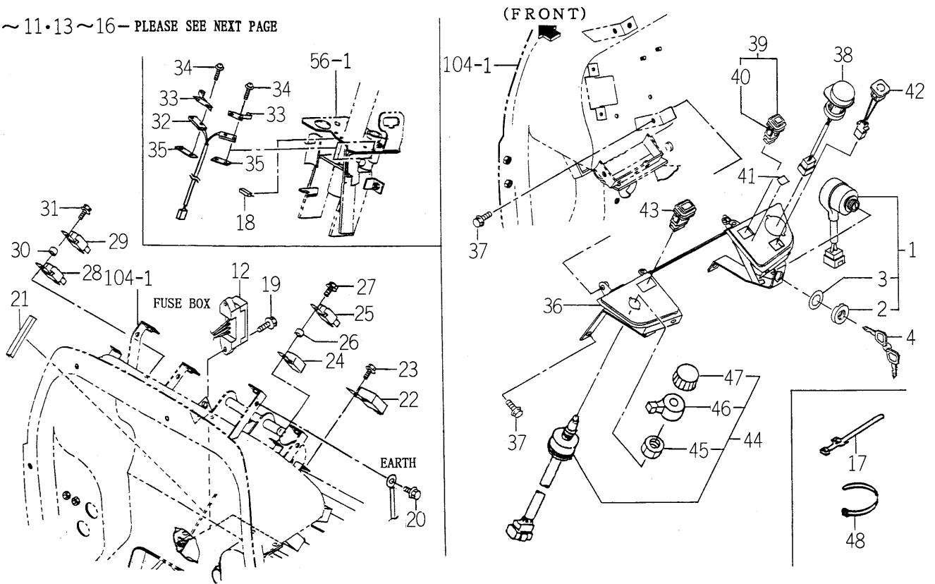
FIG.122 ELC. SYSTEM (MAIN) (QE6 TYPE)(1/2)
