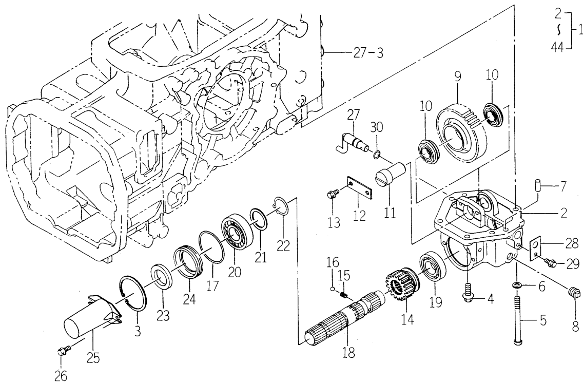
FIG. 28 MID PTO SET (M TYPE-STANDARD/(1/2) EXCEPT Q,M TYPE-OPTION)
