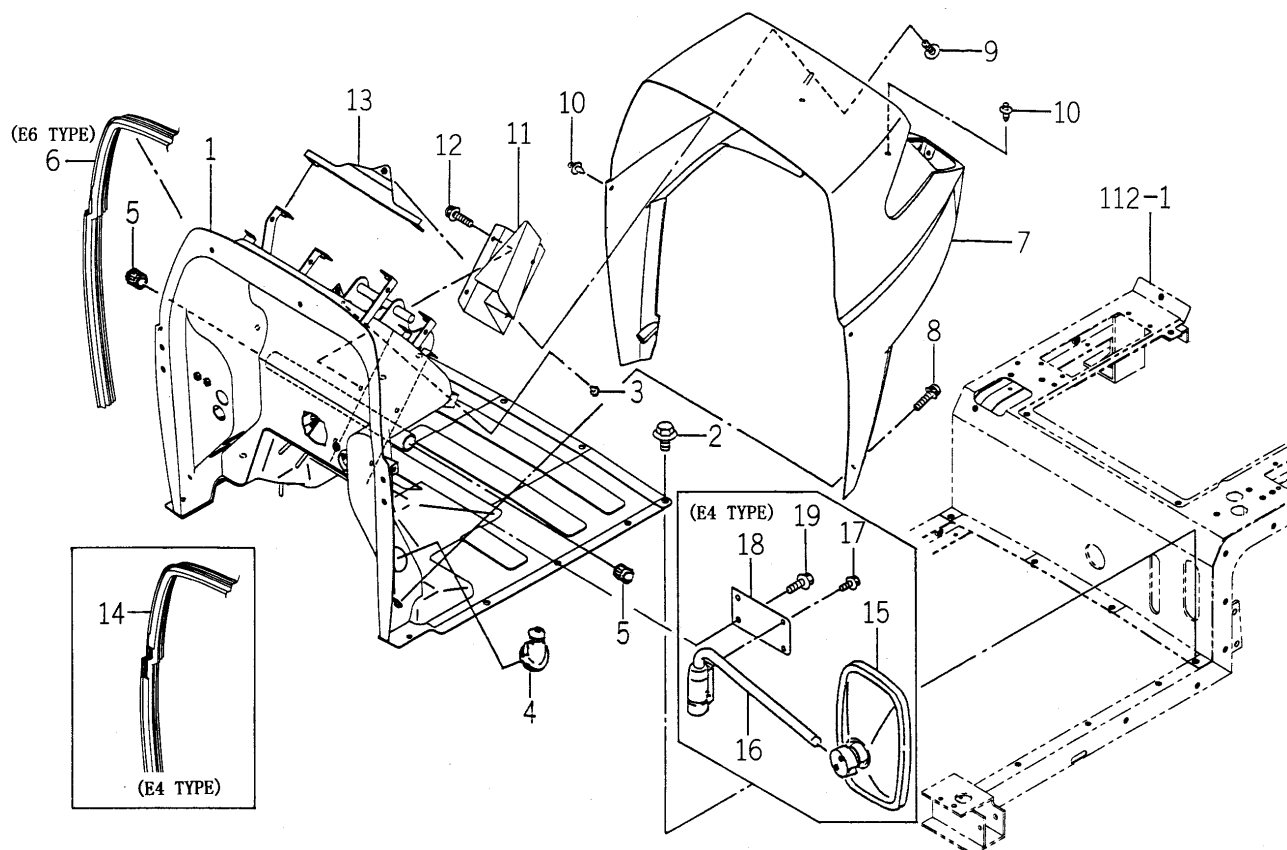
FIG.107 FLOOR (FRONT) SYSTEM (H TYPE EXCEPT CY)
