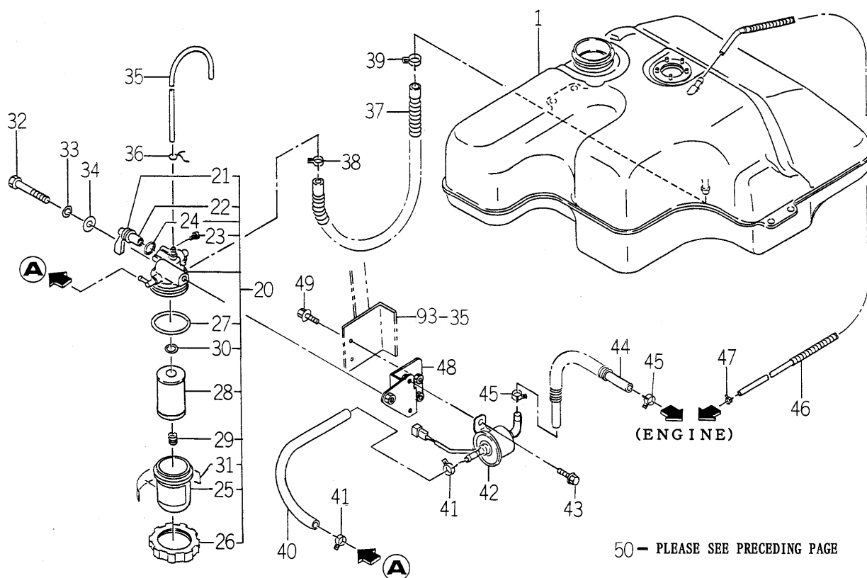
FIG. 5 TANK (FUEL) SYSTEM(2/2)
