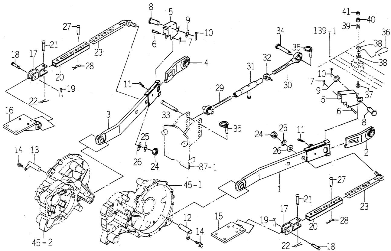
FIG. 82 3P LINK SYSTEM (CYE6 TYPE)
