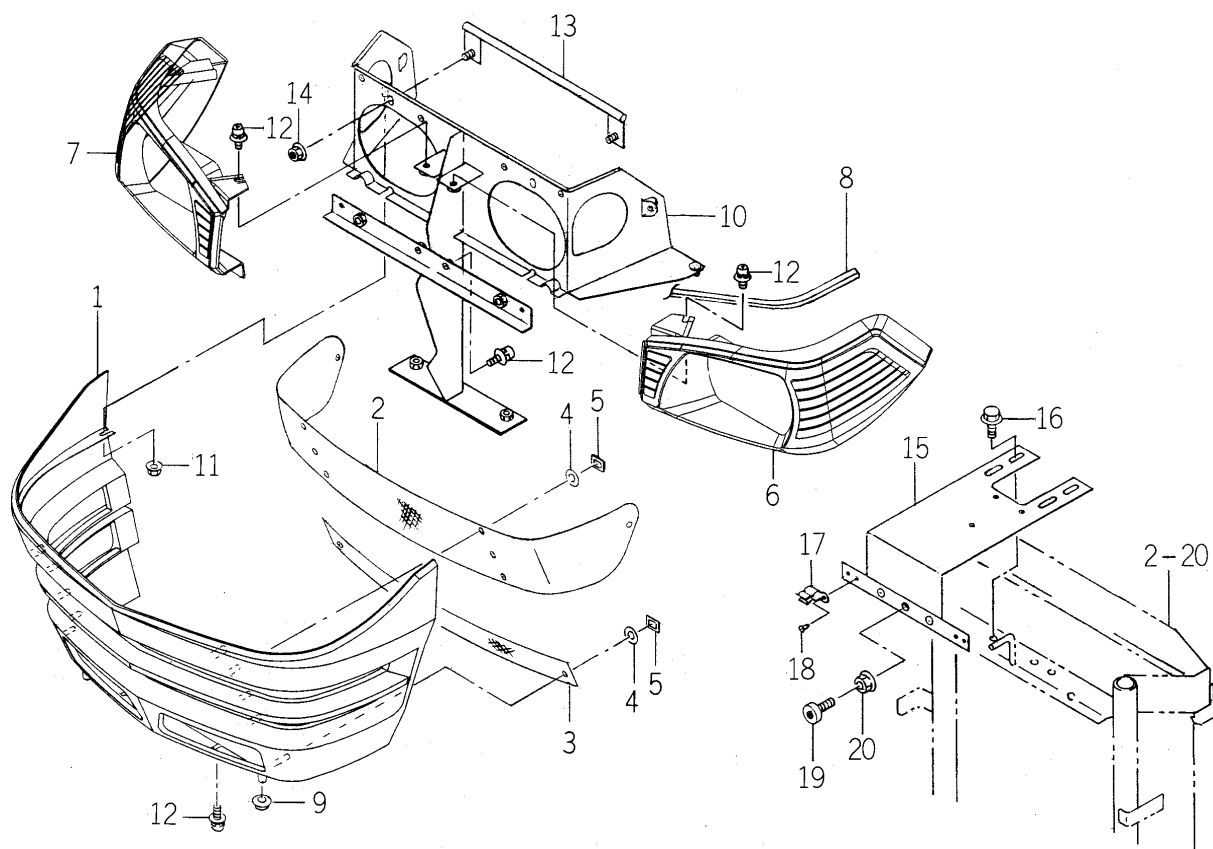
FIG. 94 GRILLE SYSTEM
