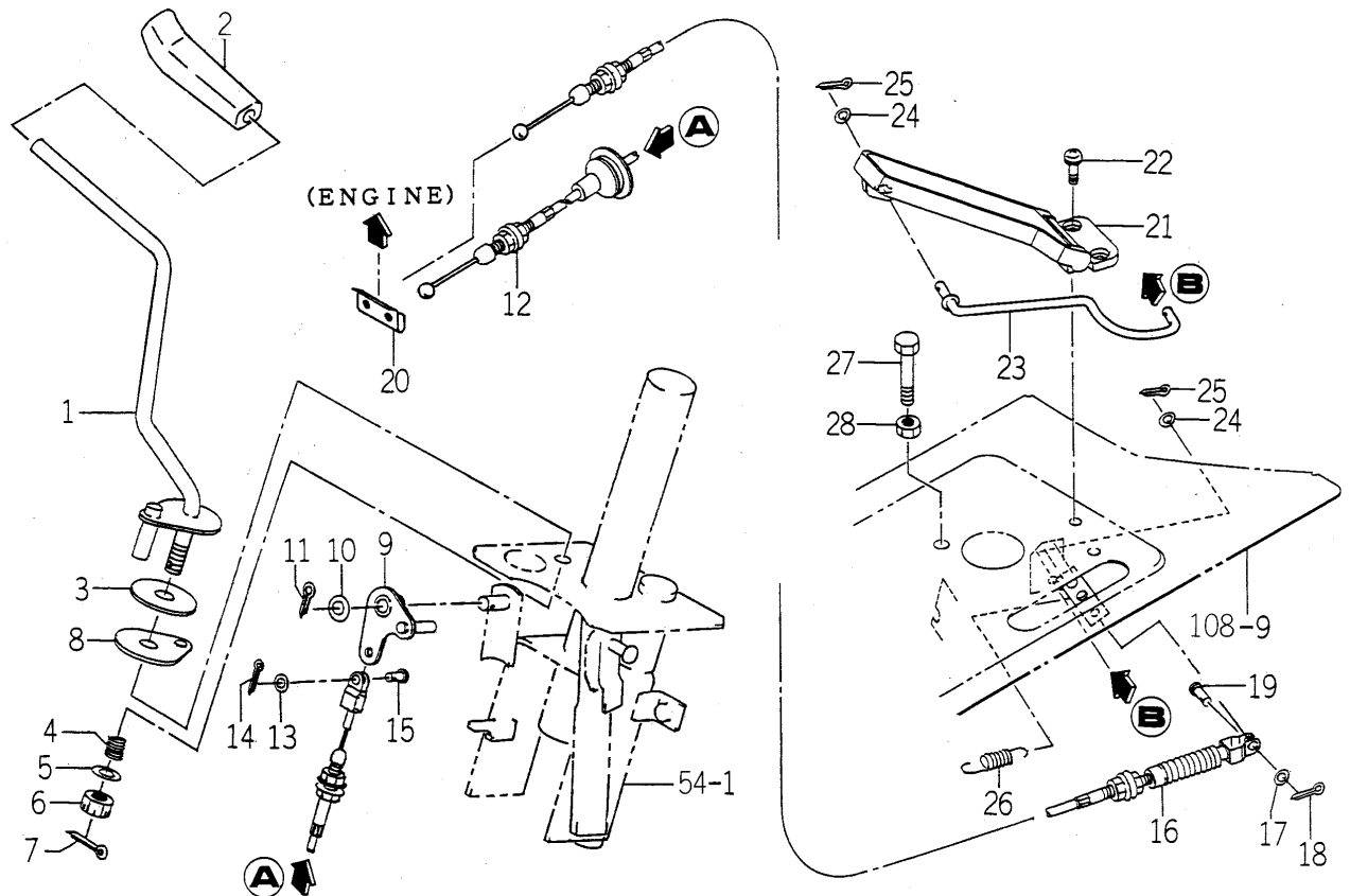
FIG. 6 ACCELERATOR SYSTEM (EXCEPT H TYPE)
