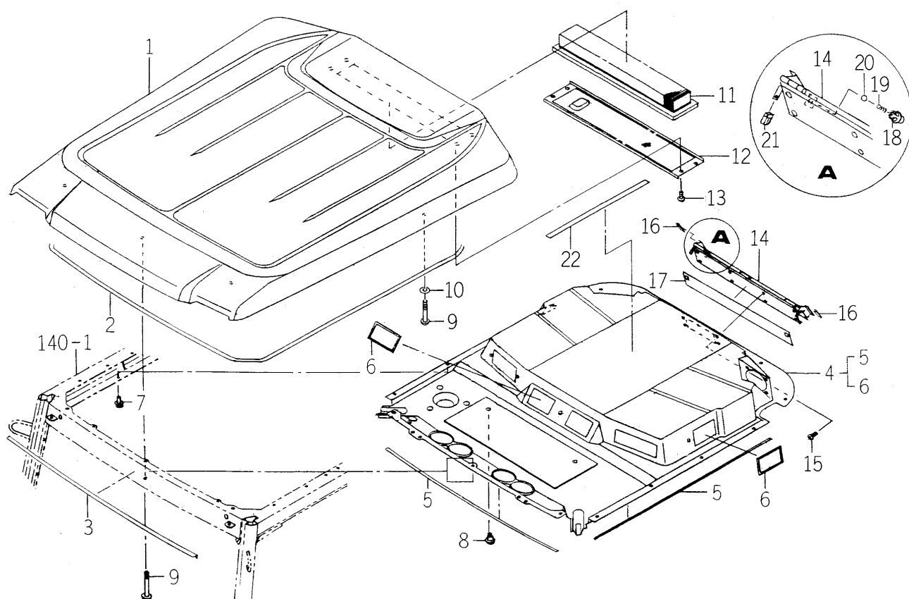
FIG.138 ROOF SYSTEM (CY TYPE)
