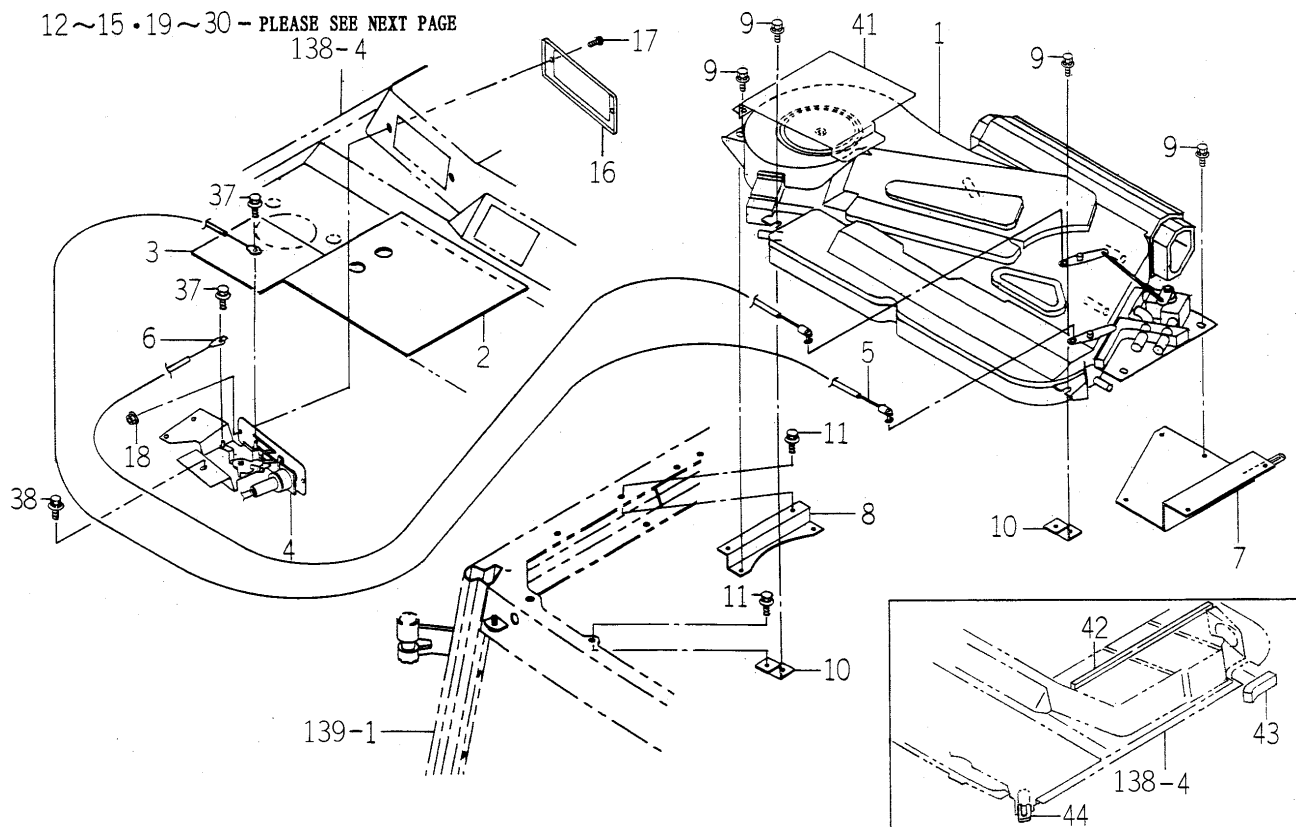
FIG.148 AIR CONDITIONER (CABIN) SYSTEM(1/2) (CY TYPE)
