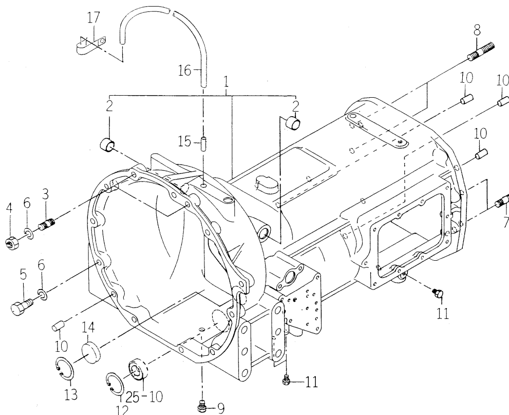
FIG. 12 CASE (TRANSMISSION/FRONT) SYSTEM (Q TYPE)
