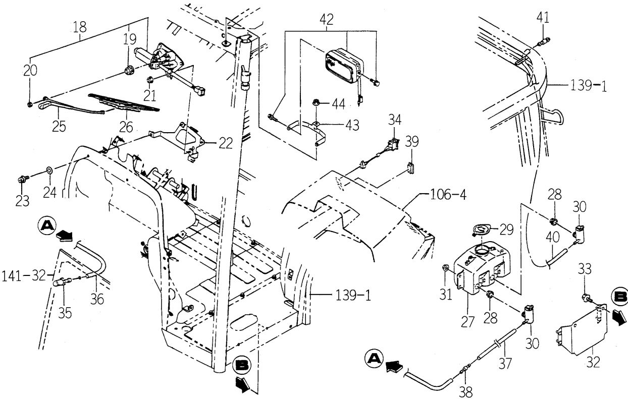
FIG.129 ELC. SYSTEM (CY TYPE)(2/3)
