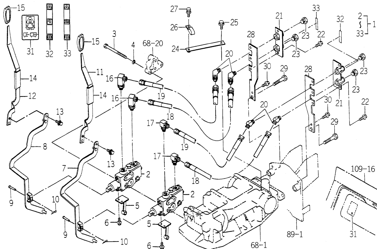
FIG.166 VALVE (REMOTE/2R) SET (E4 TYPE-OPTION)
