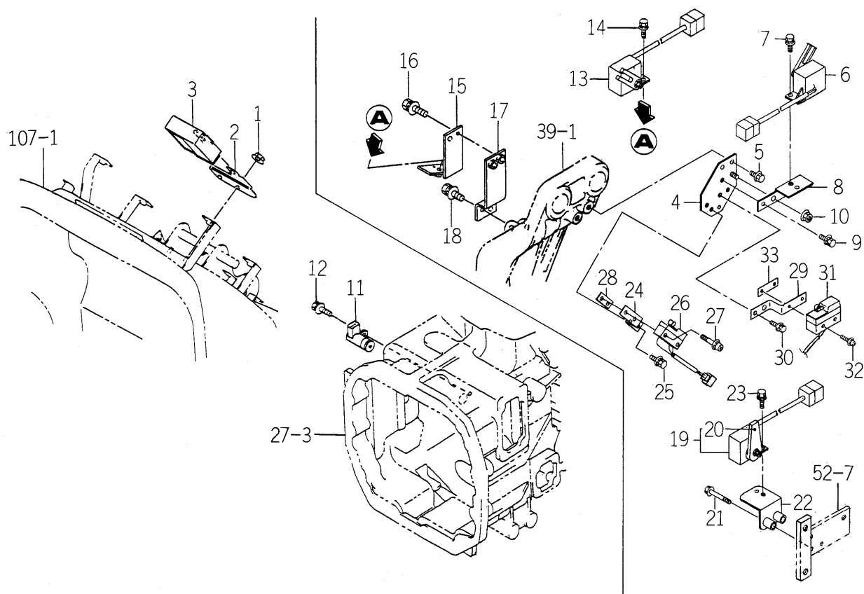
FIG.134 CONTROL SYSTEM (HM TYPE)
