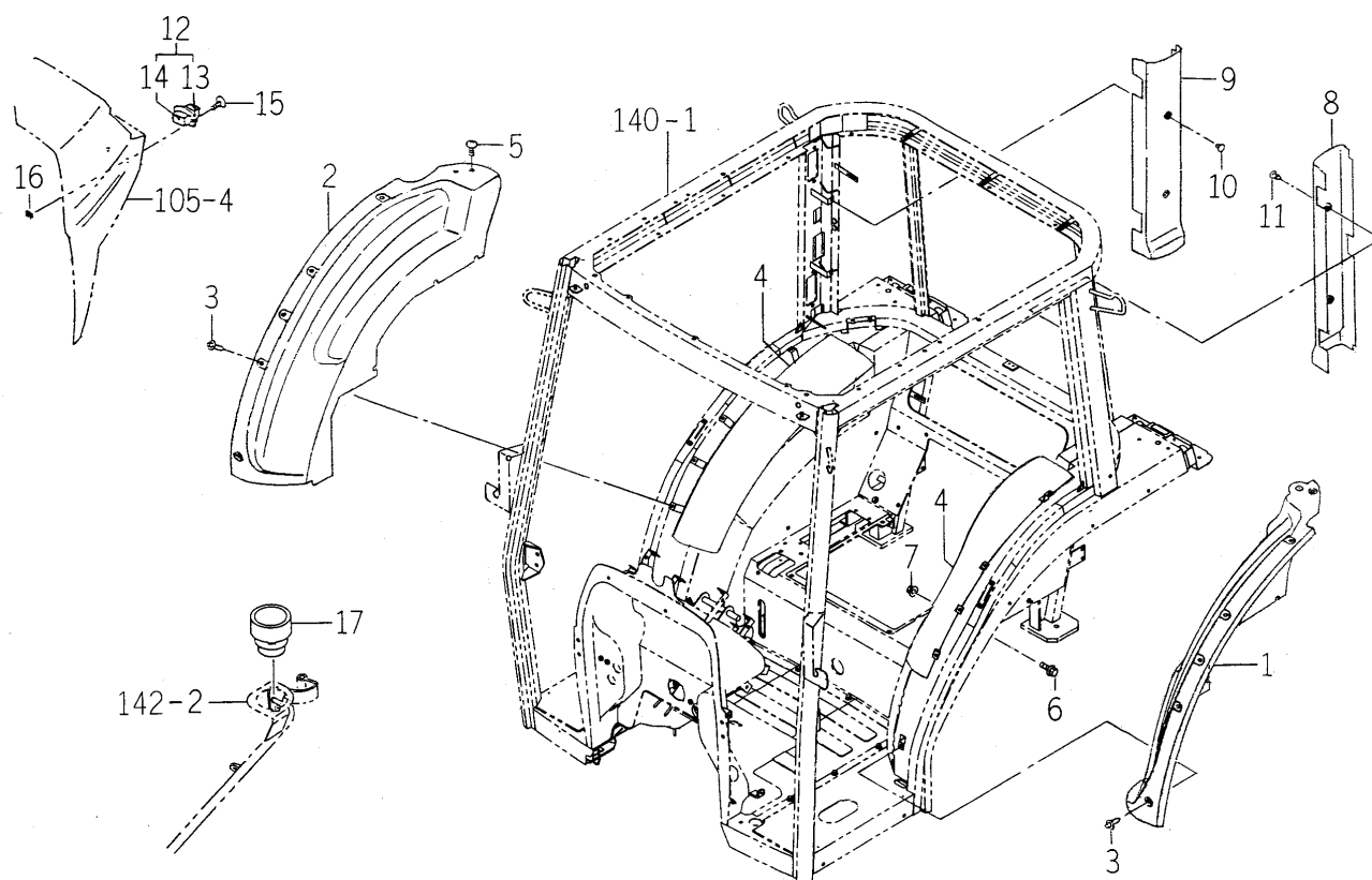
FIG.146 INTERIOR SYSTEM (CY TYPE)
