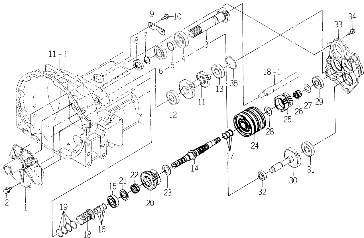
FIG. 15 GEAR (REVERSE) SYSTEM (P,Q TYPE)
