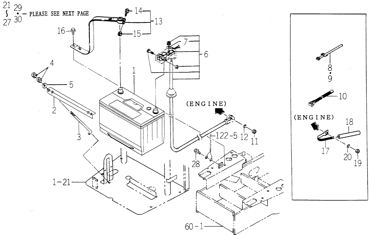
FIG.118 ELC. SYSTEM (FRONT) (E6 TYPE)(1/2)
