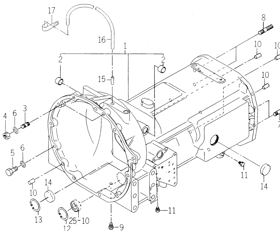
FIG. 11 CASE (TRANSMISSION/FRONT) SYSTEM (P TYPE)
