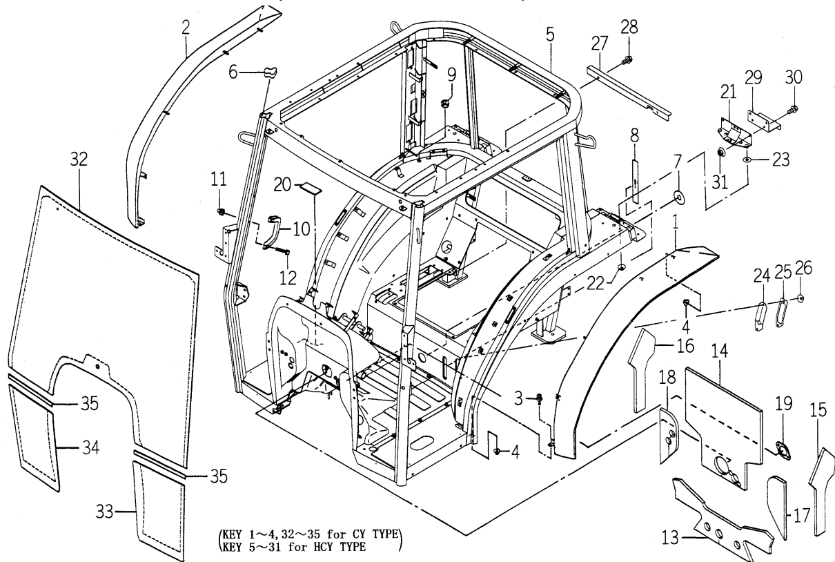
FIG.141 FRAME (HCY TYPE), FENDER (OVER/CY TYPE), GLASS (FRONT/CY TYPE) SYSTEM
