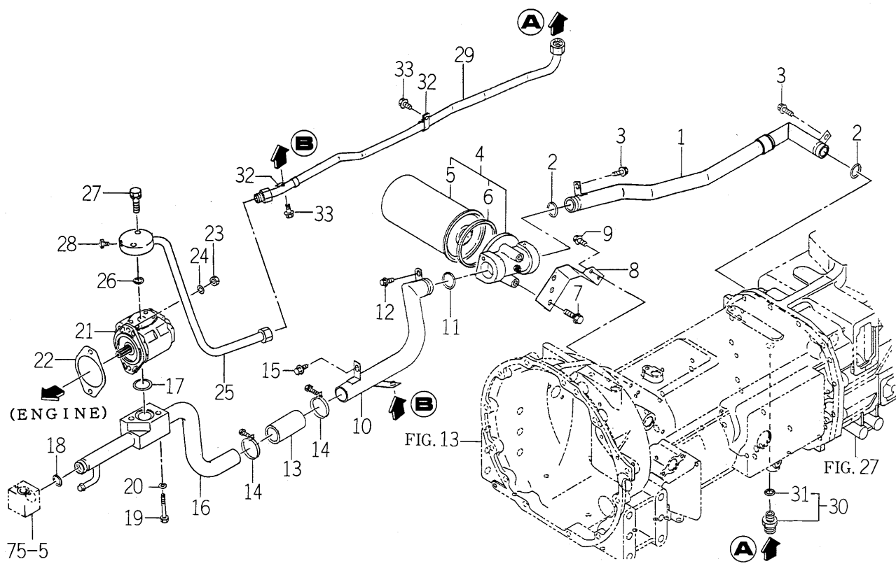
FIG. 71 HYD. SYSTEM (MAIN) (S TYPE)(1/2)
