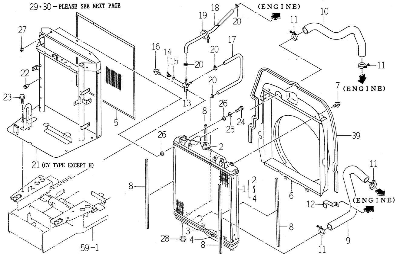
FIG. 1 RADIATOR SYSTEM (H,CY TYPE)(1/2)
