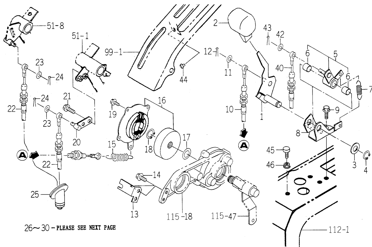
FIG.116 CRUISE CONTROL SYSTEM (H TYPE)(1/2)
