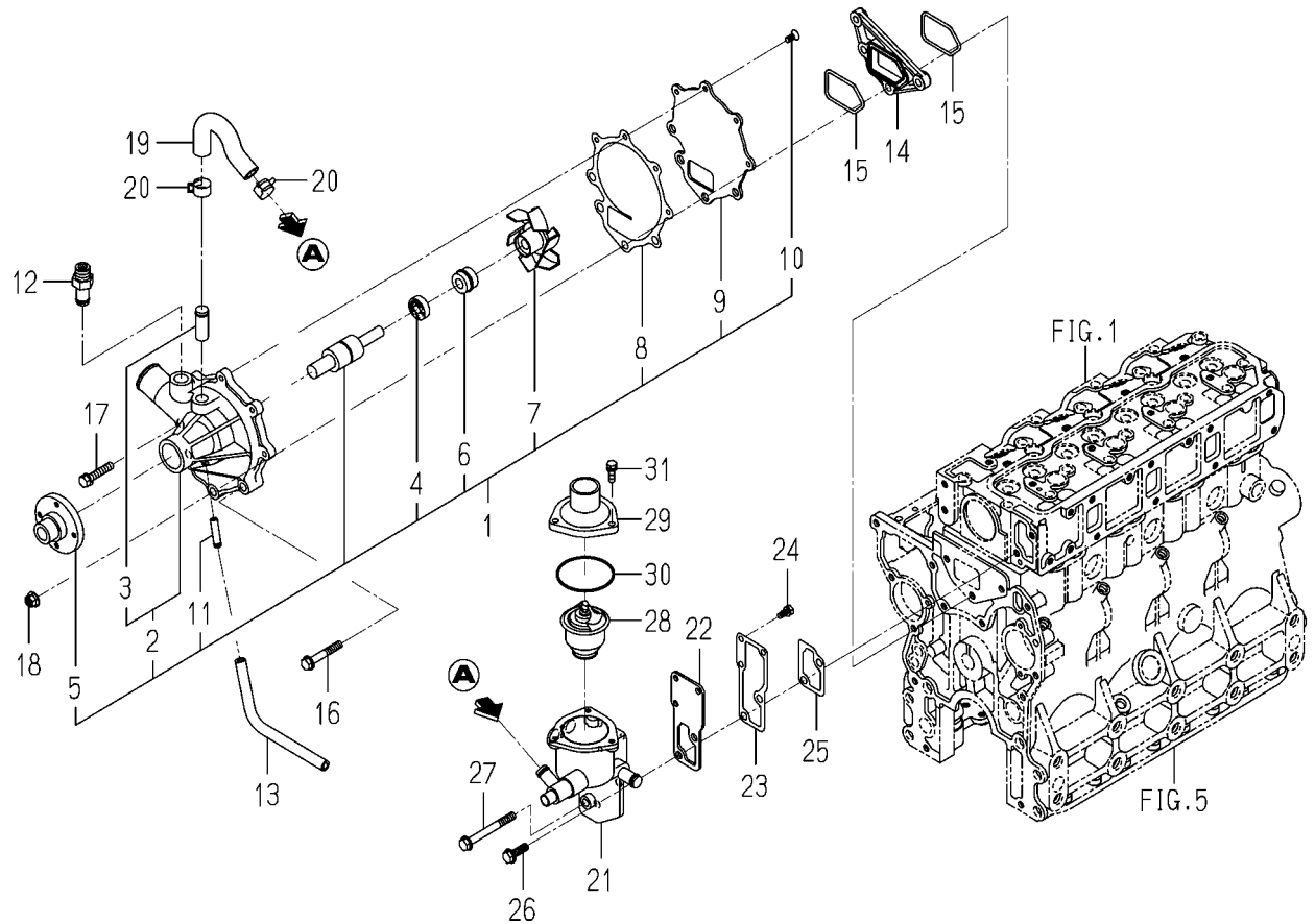
FIG. 17 WATER PUMP
