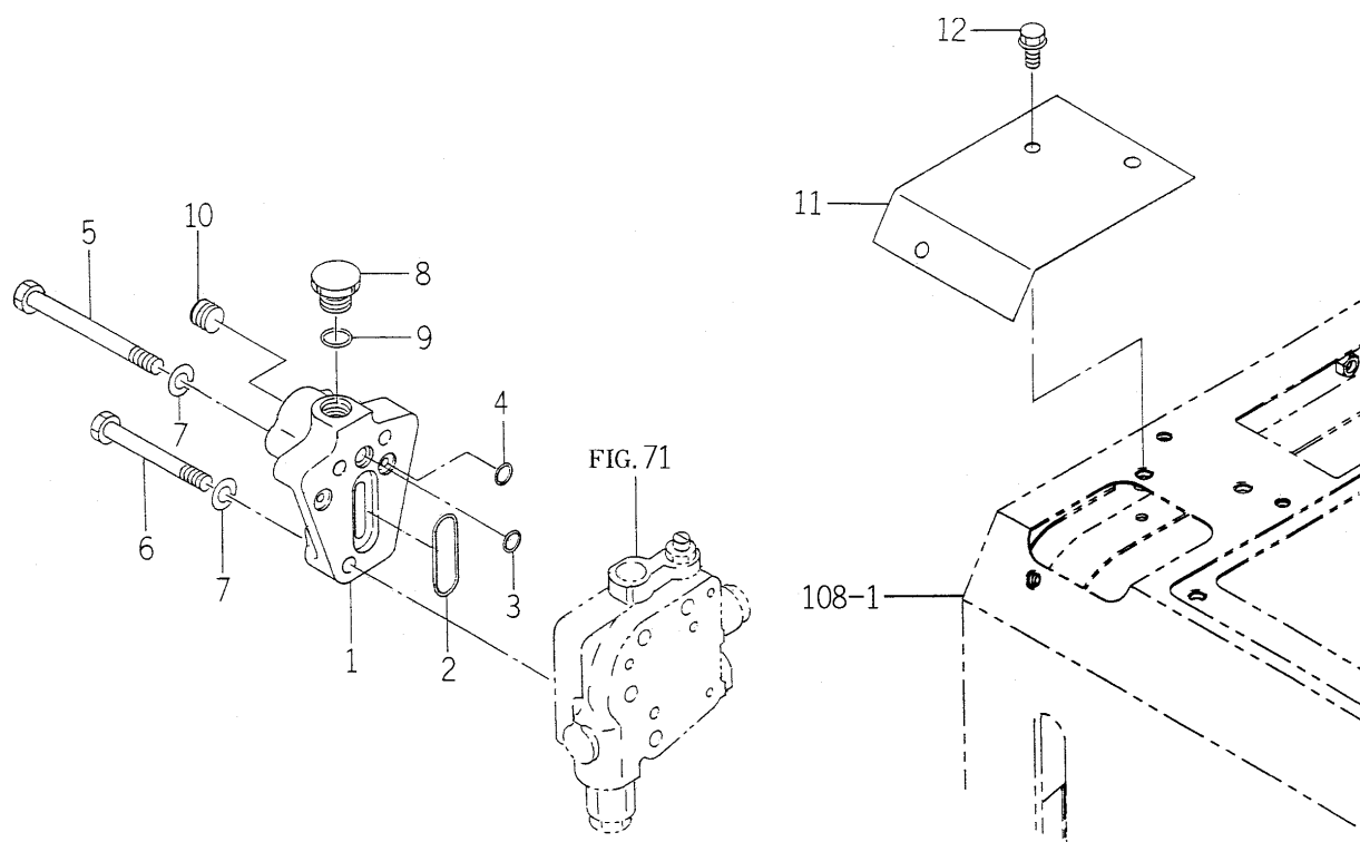
FIG. 74 COVER (RELIEF METAL) SYSTEM (EXCEPT J TYPE)
