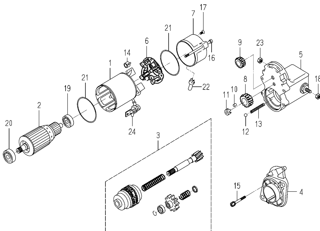
FIG. 28 COMPONENT PARTS FOR 6281-100-010-30 ON Fig.23
