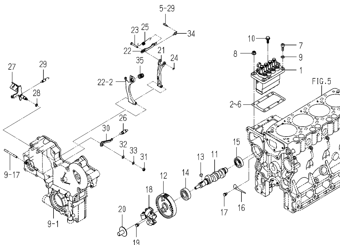
FIG. 20 INJECTION PUMP
