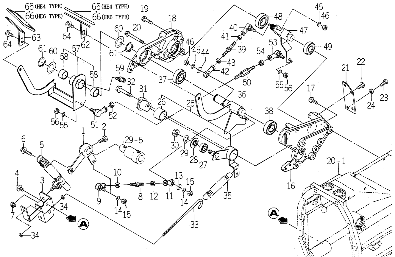
FIG.115 PEDAL (HST) SYSTEM (H TYPE)
