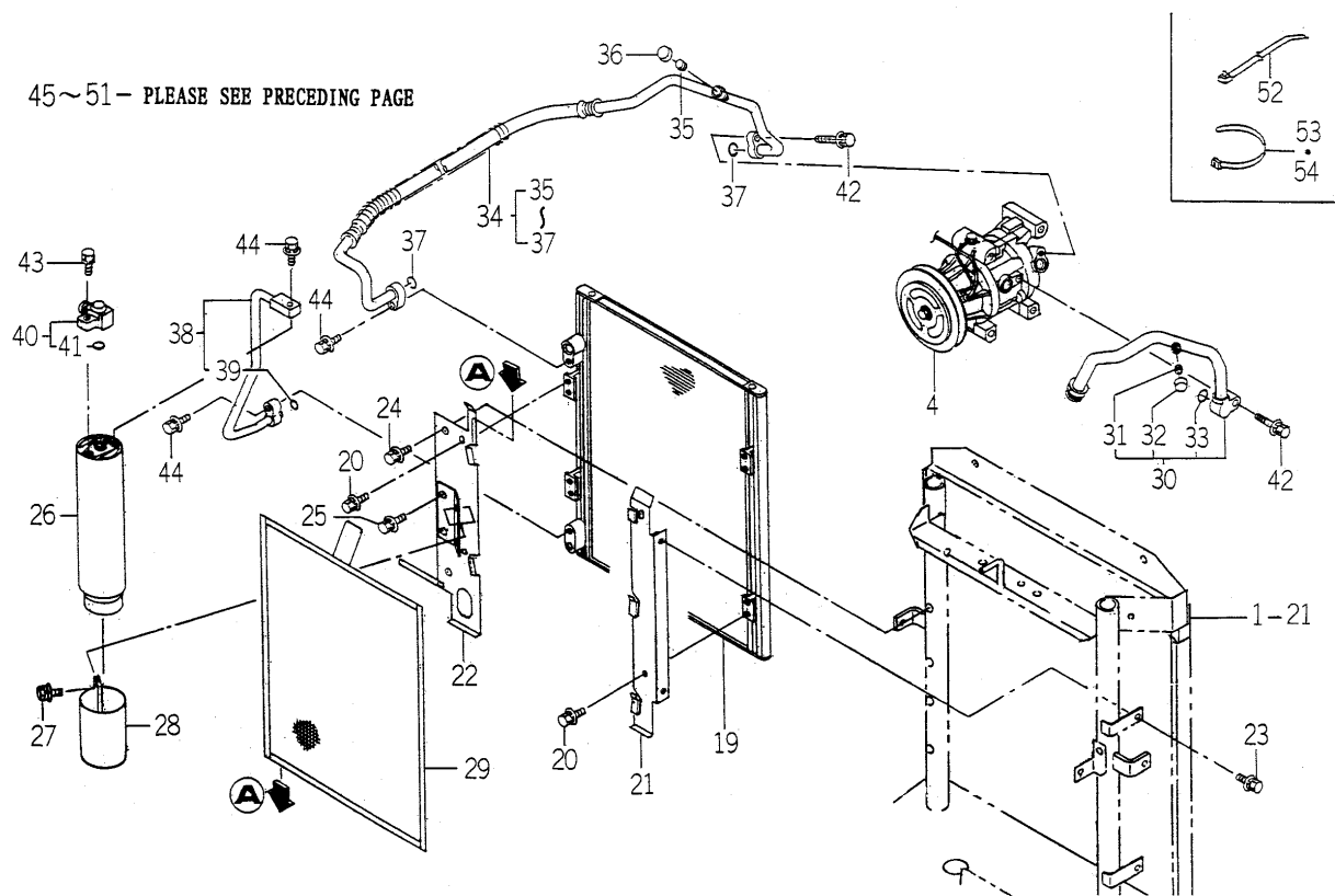
FIG.147 AIR CONDITIONER (ENGINE) SYSTEM(2/2) (CY TYPE)
