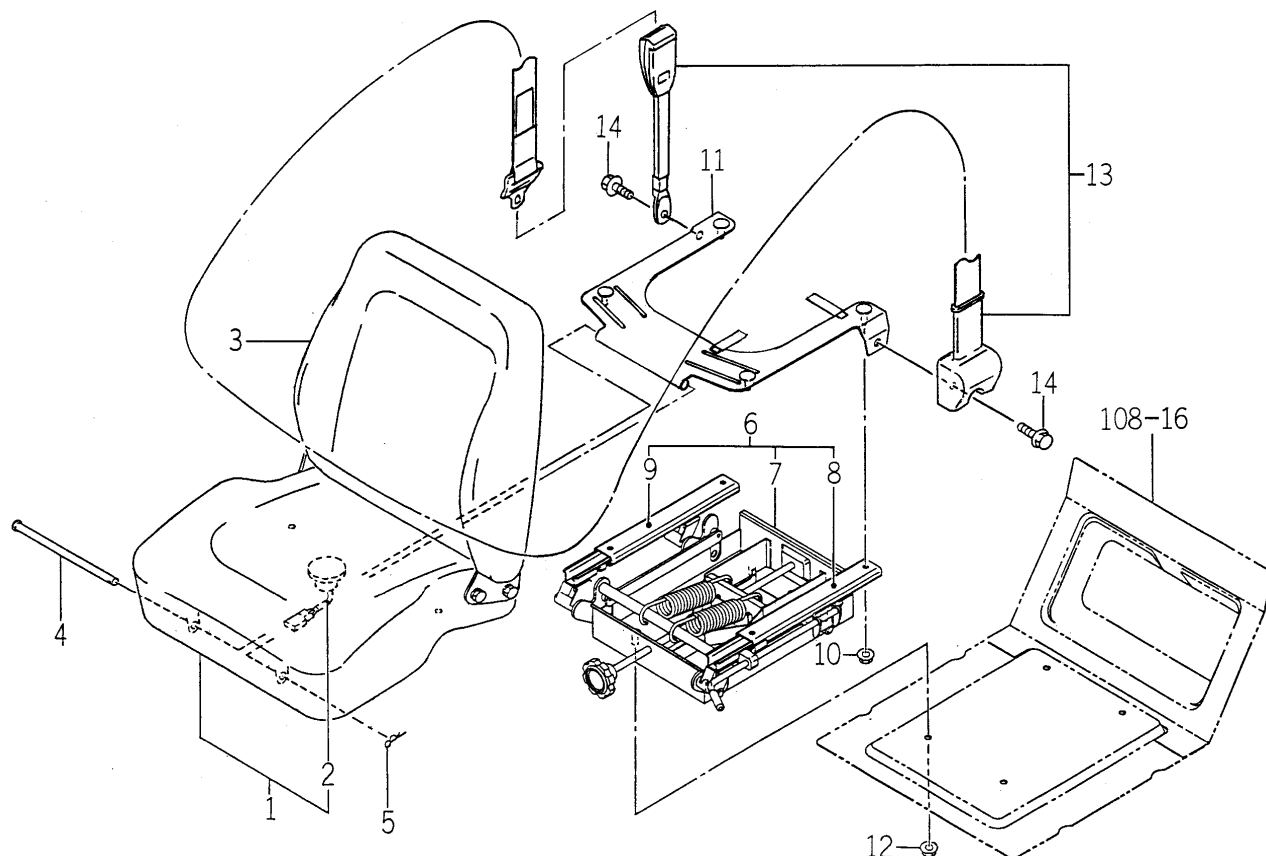
FIG.101 SEAT SYSTEM (E6 TYPE)
