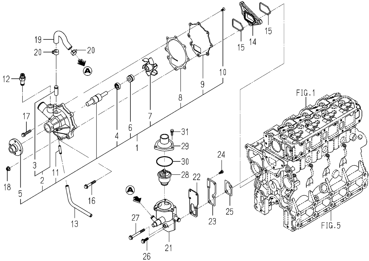
FIG. 17 WATER PUMP
