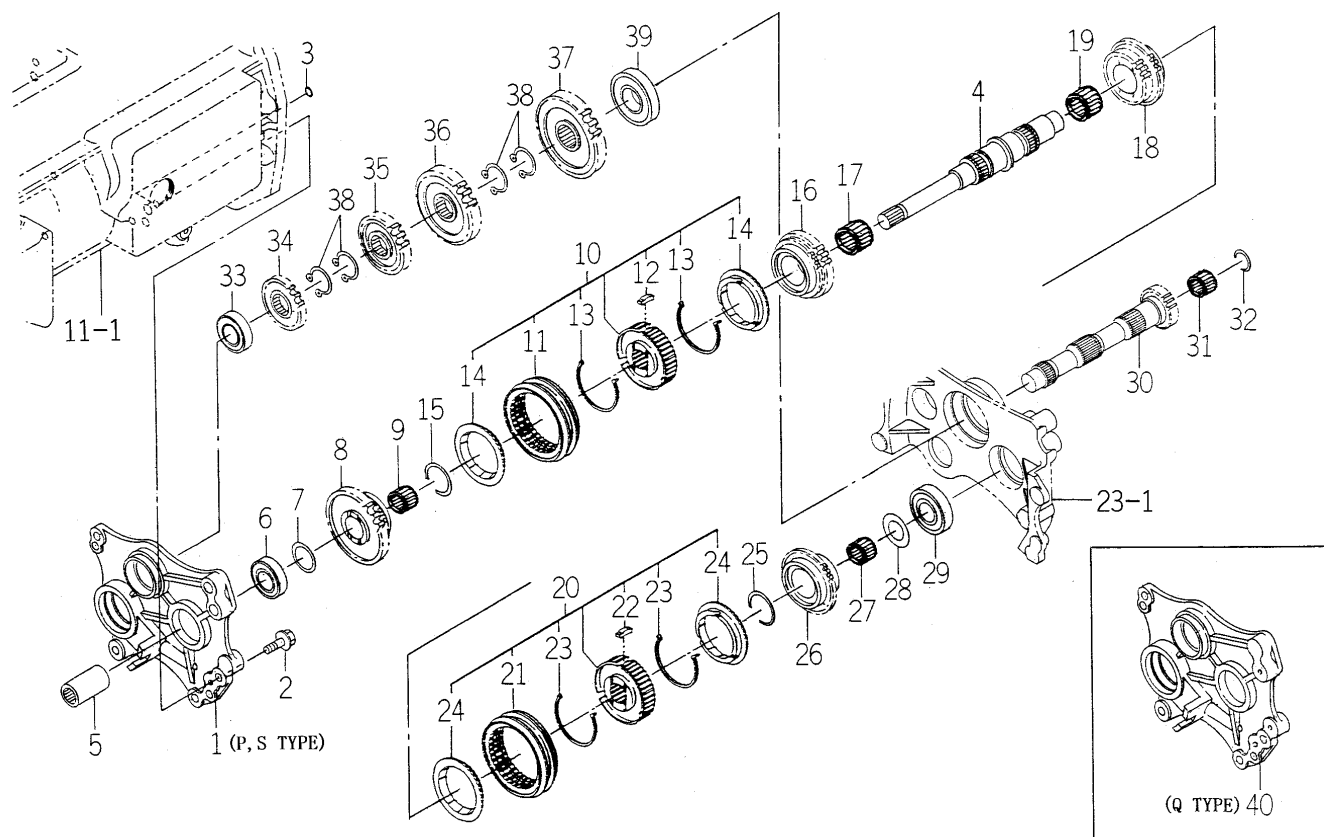
FIG. 21 GEAR (MAIN) SYSTEM (EXCEPT H TYPE)
