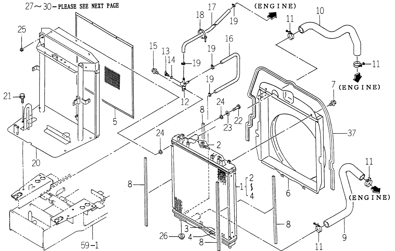
FIG. 2 RADIATOR SYSTEM(1/2) (EXCEPT H,CY TYPE)
