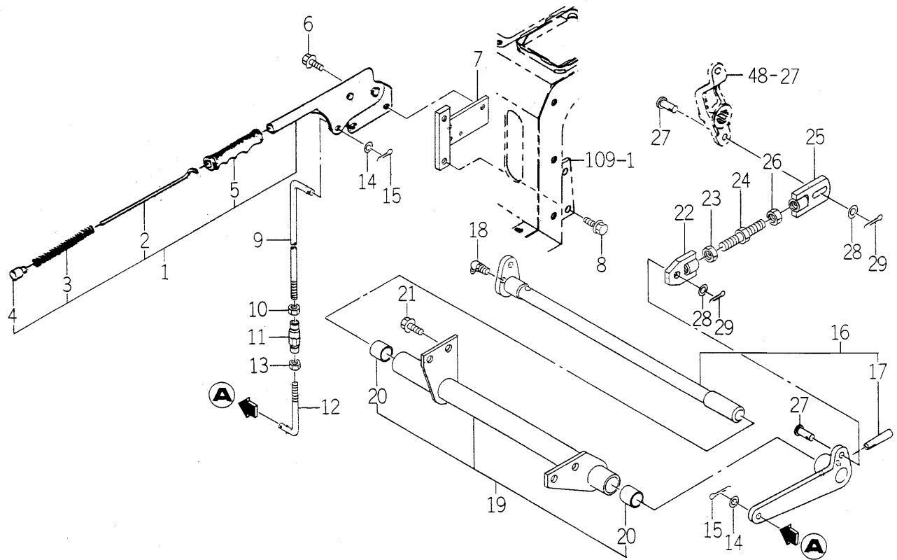
FIG. 52 BRAKE (PARKING) SYSTEM (E4 TYPE)
