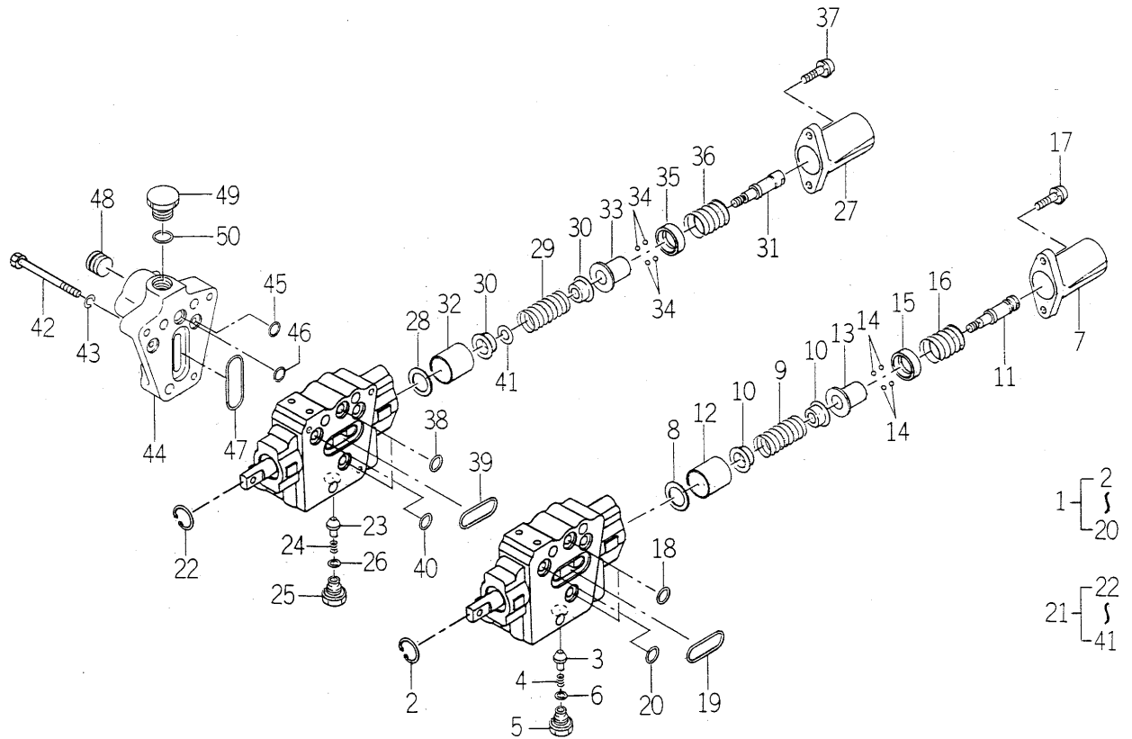
FIG.175 COMPONENT PARTS FOR K211-074-000-00 ON Fig.79
