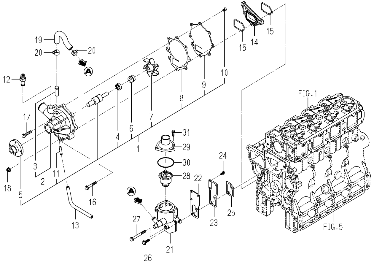
FIG. 17 WATER PUMP
