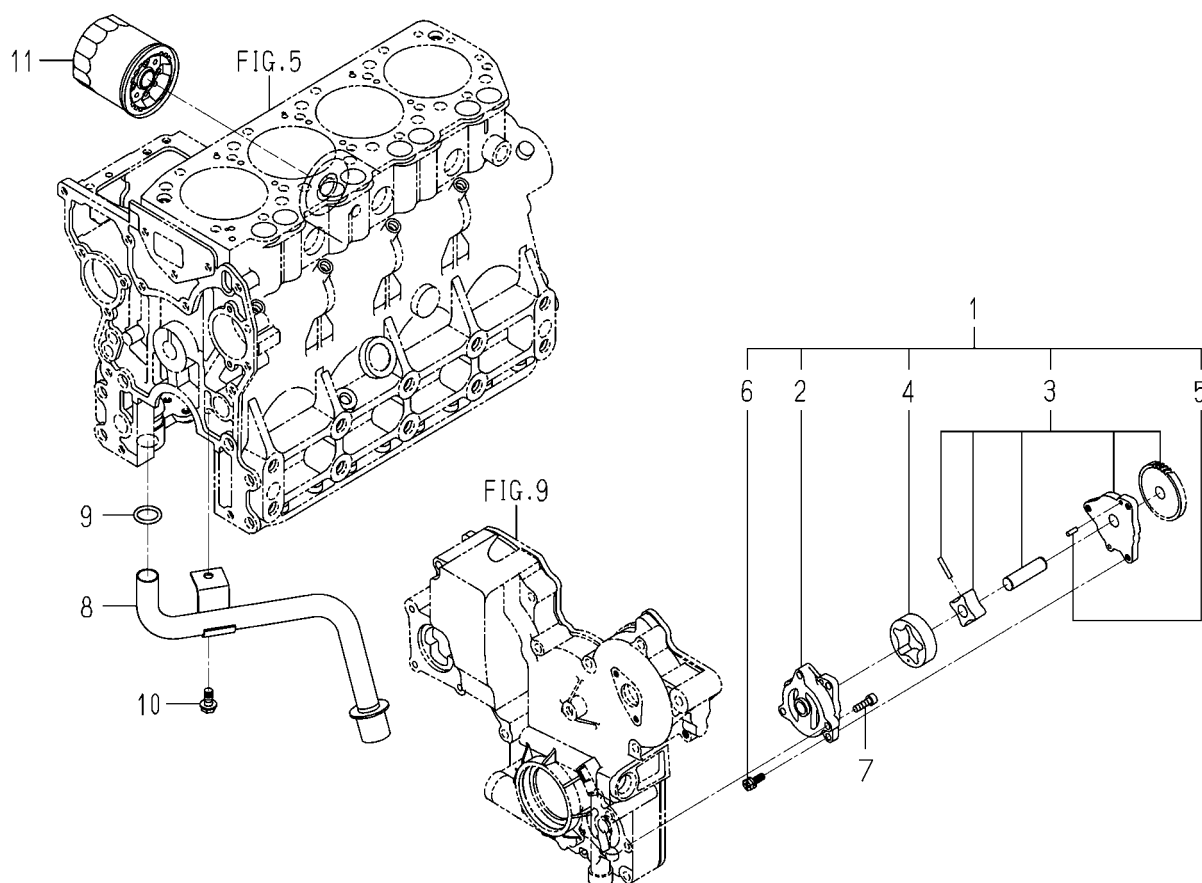
FIG. 16 OIL PUMP
