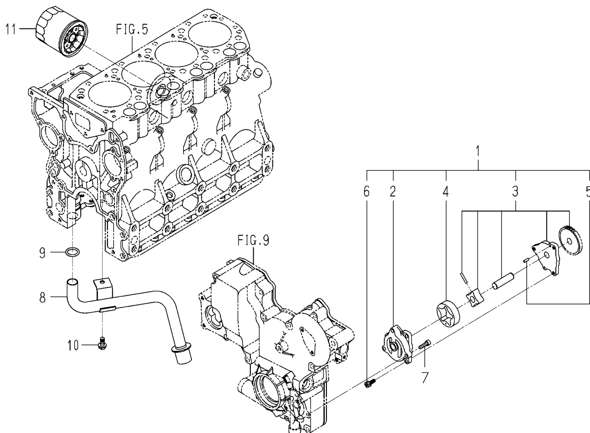
FIG. 16 OIL PUMP
