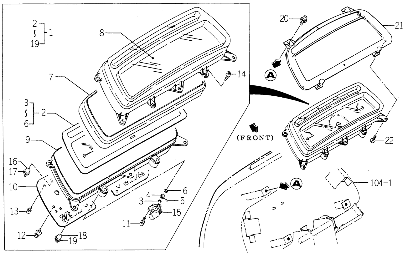
FIG.127 METER PANEL SYSTEM (EXCEPT Q,M TYPE)
