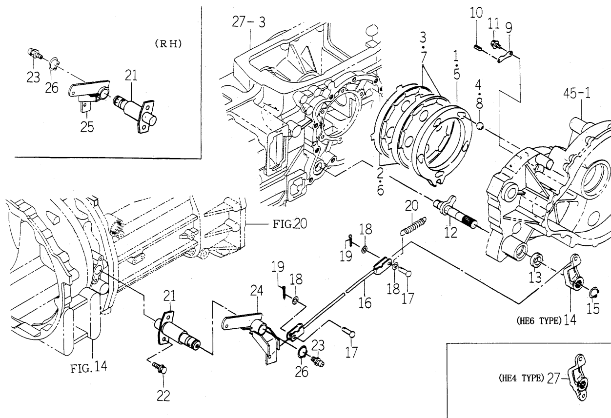
FIG. 49 BRAKE SYSTEM (H TYPE)
