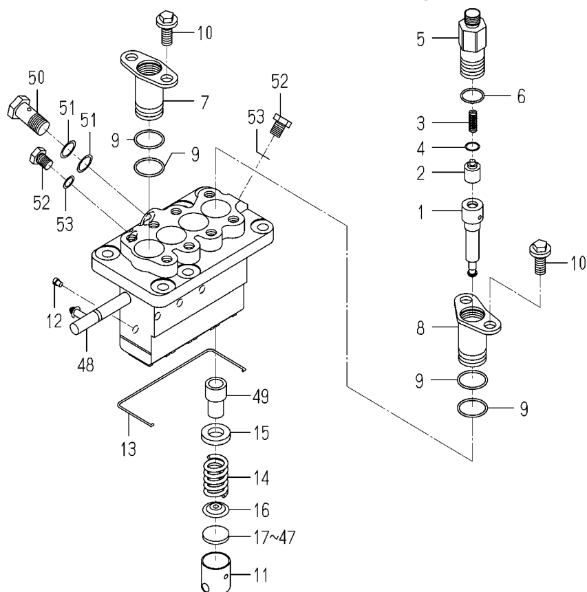
FIG. 27 COMPONENT PARTS FOR 6215-600-119-20 ON Fig.20
