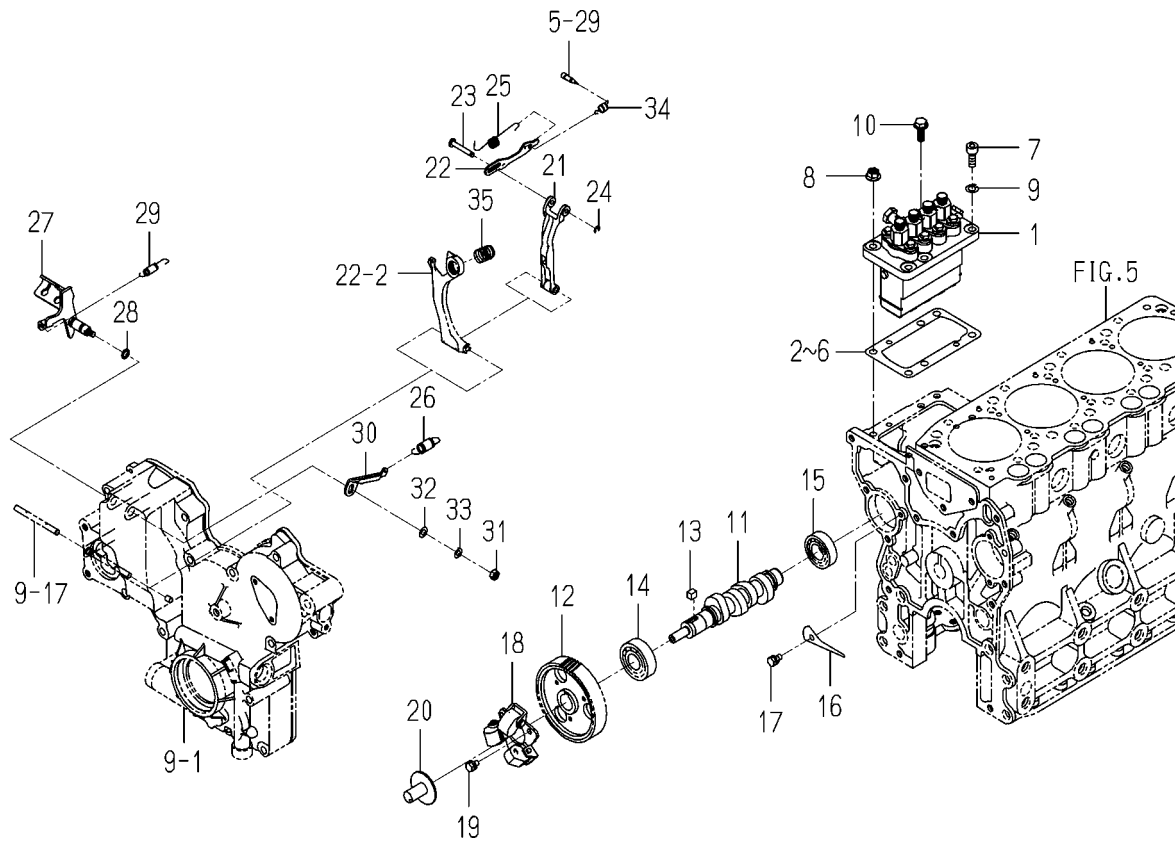
FIG. 20 INJECTION PUMP
