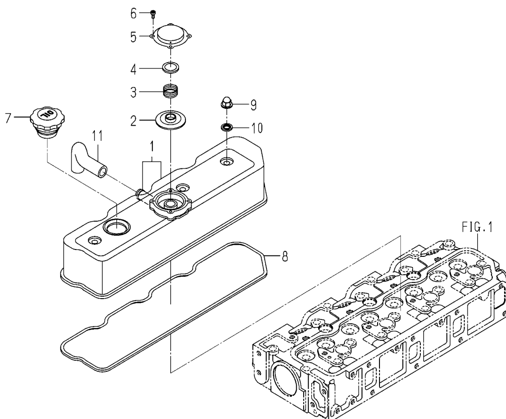
FIG. 2 CYLINDER HEAD COVER
