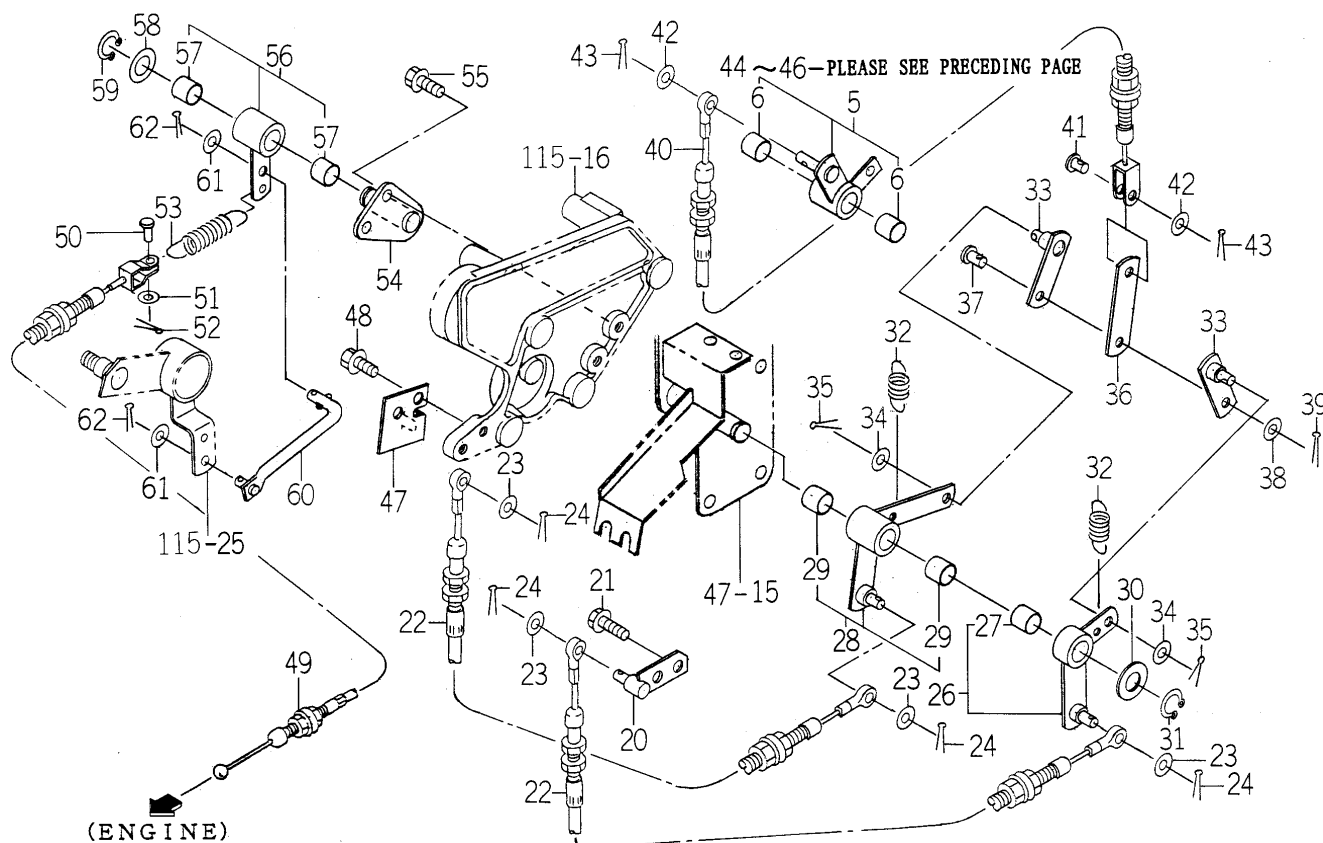
FIG.116 CRUISE CONTROL SYSTEM (H TYPE)(2/2)
