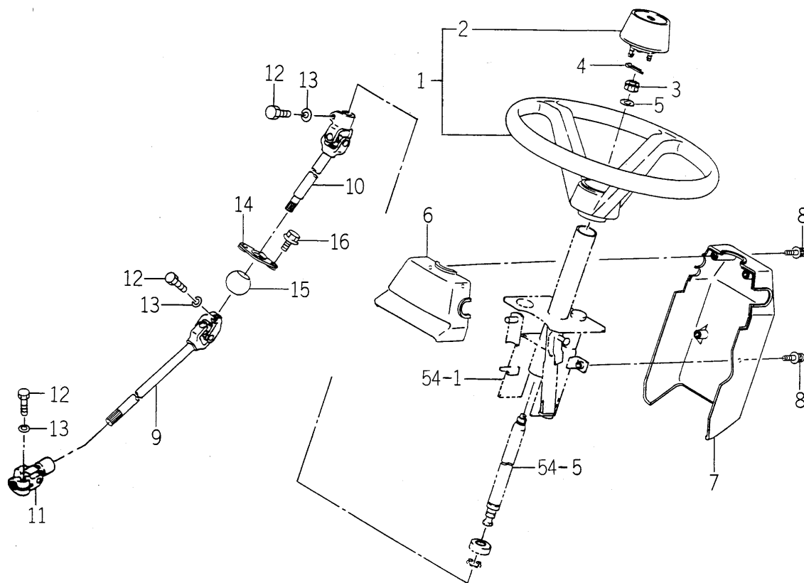
FIG. 53 WHEEL (STEERING) SYSTEM
