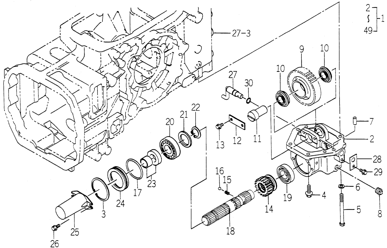
FIG.153 MID PTO SET (Q TYPE-OPTION)(1/2)
