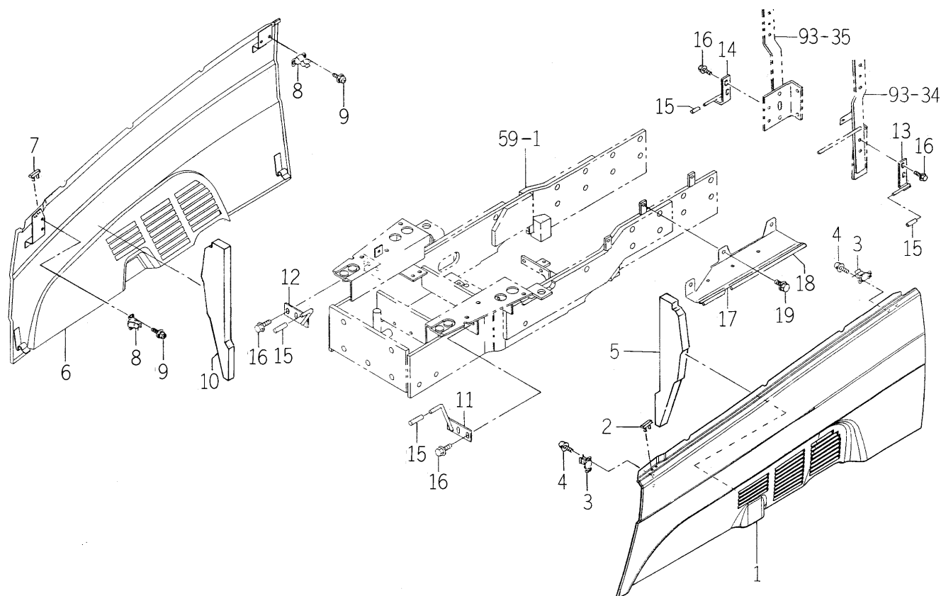
FIG. 96 COVER (SIDE) SYSTEM (EXCEPT CY TYPE)
