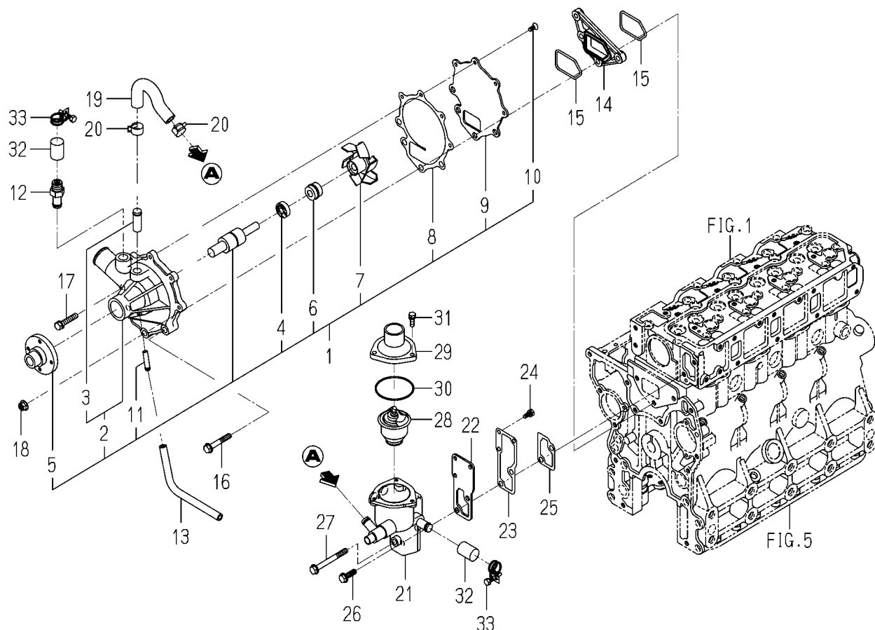
FIG. 17 WATER PUMP
