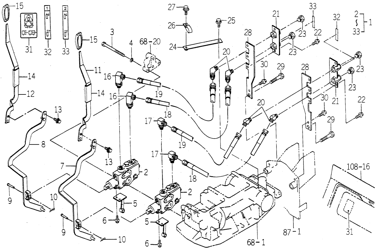
FIG. 80 VALVE (REMOTE/2R) SET (W TYPE)
