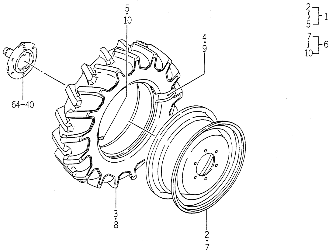
FIG.150 FRONT WHEEL SYSTEM (OPTION)
