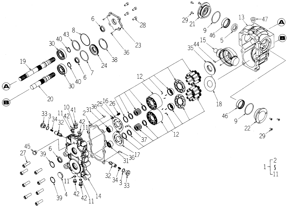
FIG.171 COMPONENT PARTS FOR 1743-203-510-10 ON Fig.16
