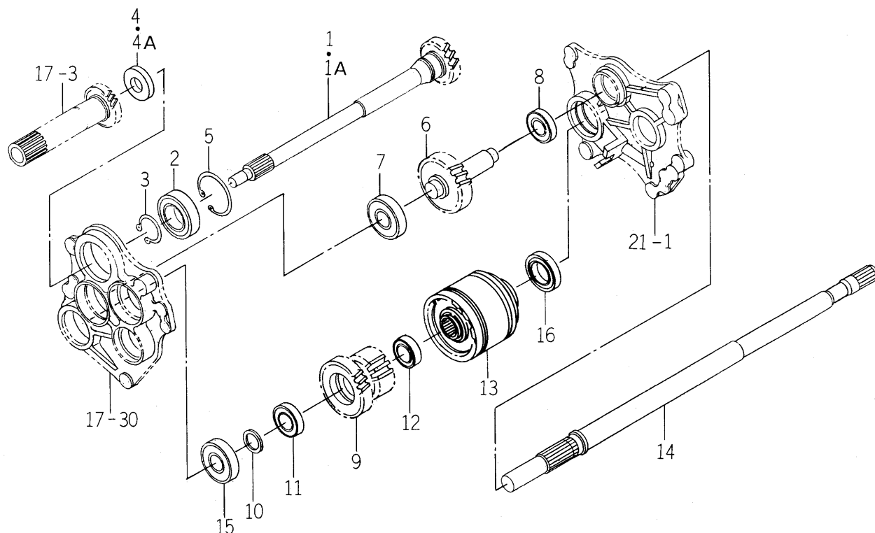
FIG. 18 GEAR (PTO/FRONT) SYSTEM (EXCEPT H TYPE)
