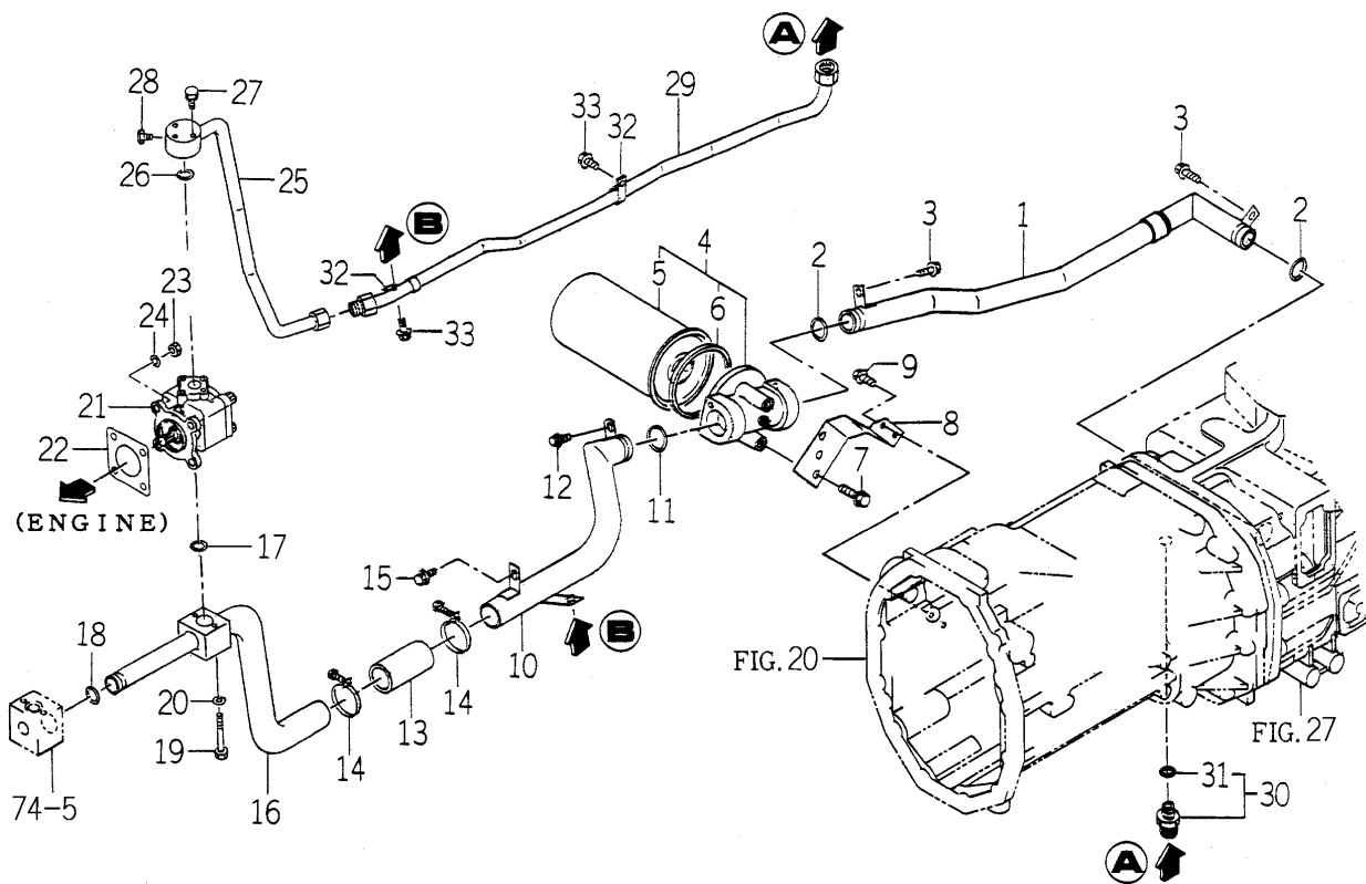
FIG. 70 HYD. SYSTEM (MAIN) (H TYPE)(1/2)
