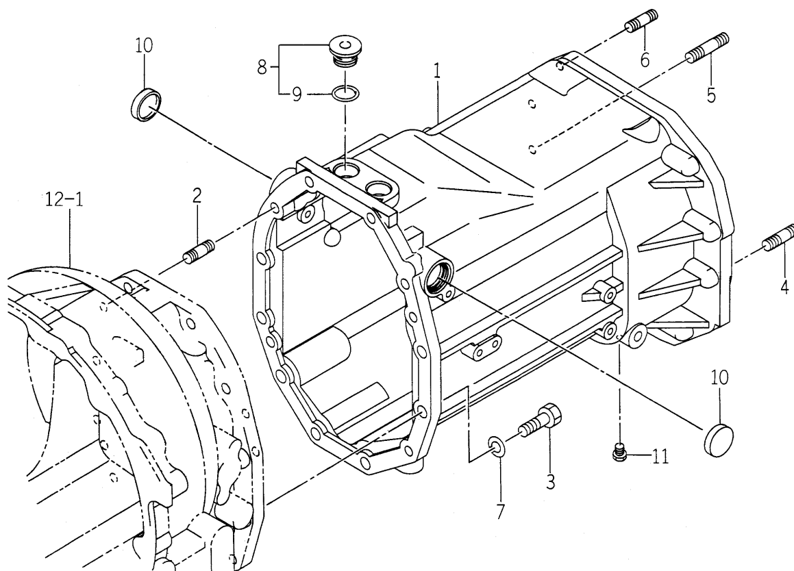
FIG. 20 CASE (TRANSMISSION/MID) SYSTEM (H TYPE)
