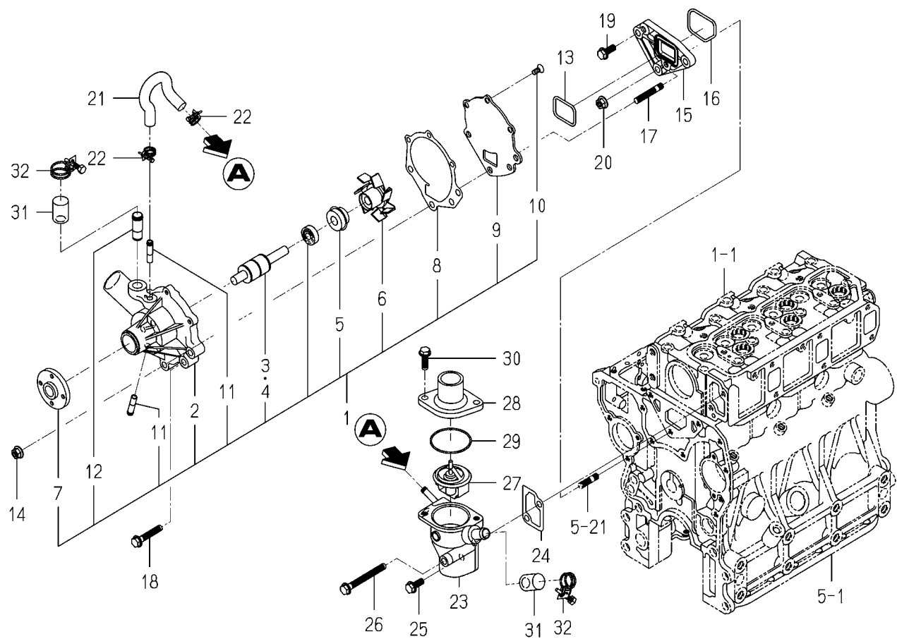
FIG. 18 WATER PUMP
