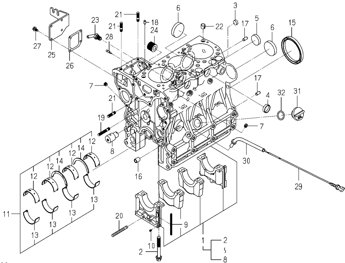
FIG. 5 CYLINDER BLOCK
