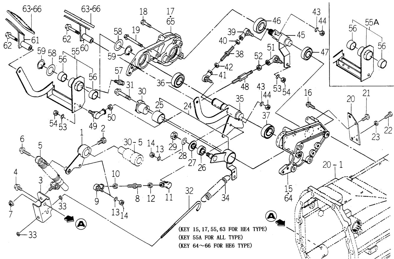
FIG.108 PEDAL (HST) SYSTEM (H TYPE)
