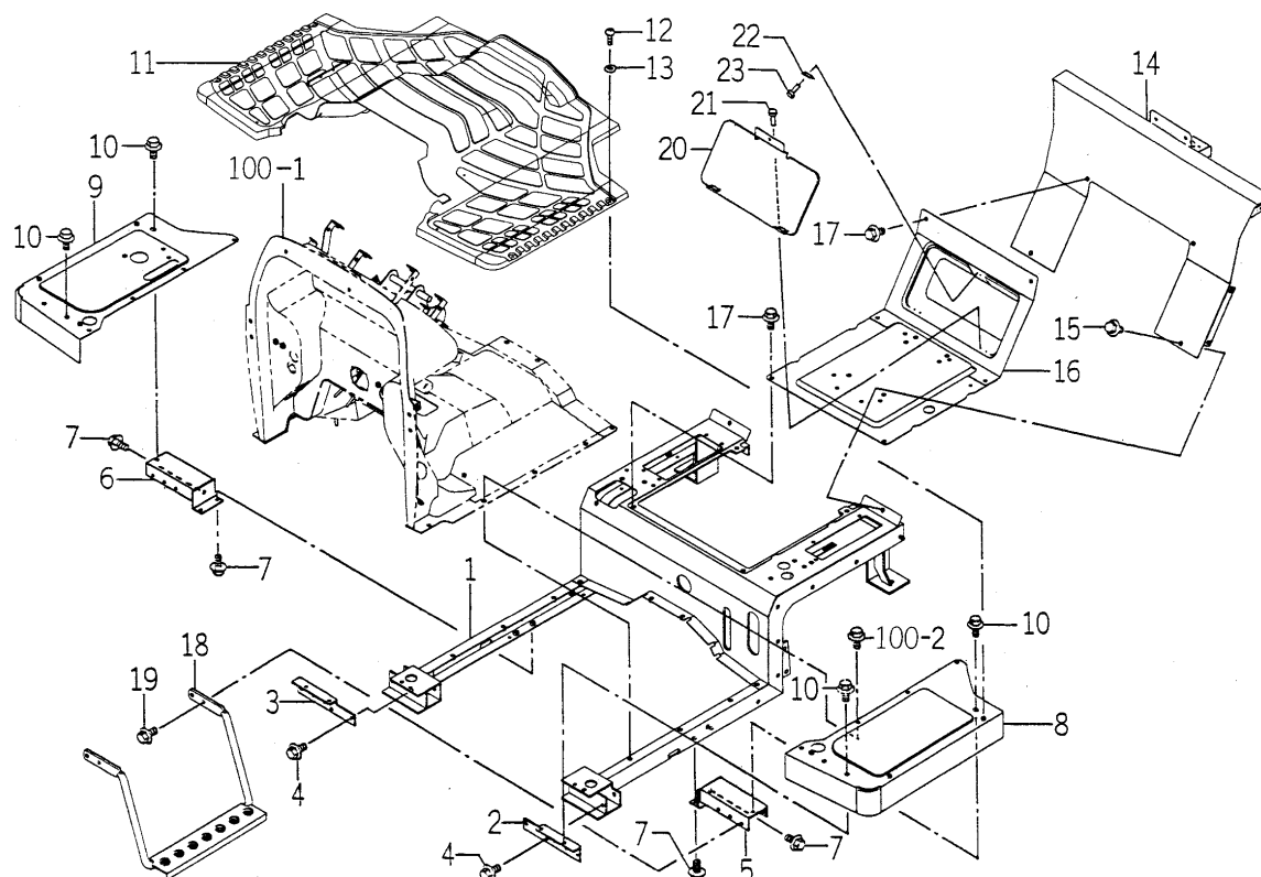
FIG.104 FLOOR (REAR) SYSTEM (HE4 TYPE EXCEPT C)
