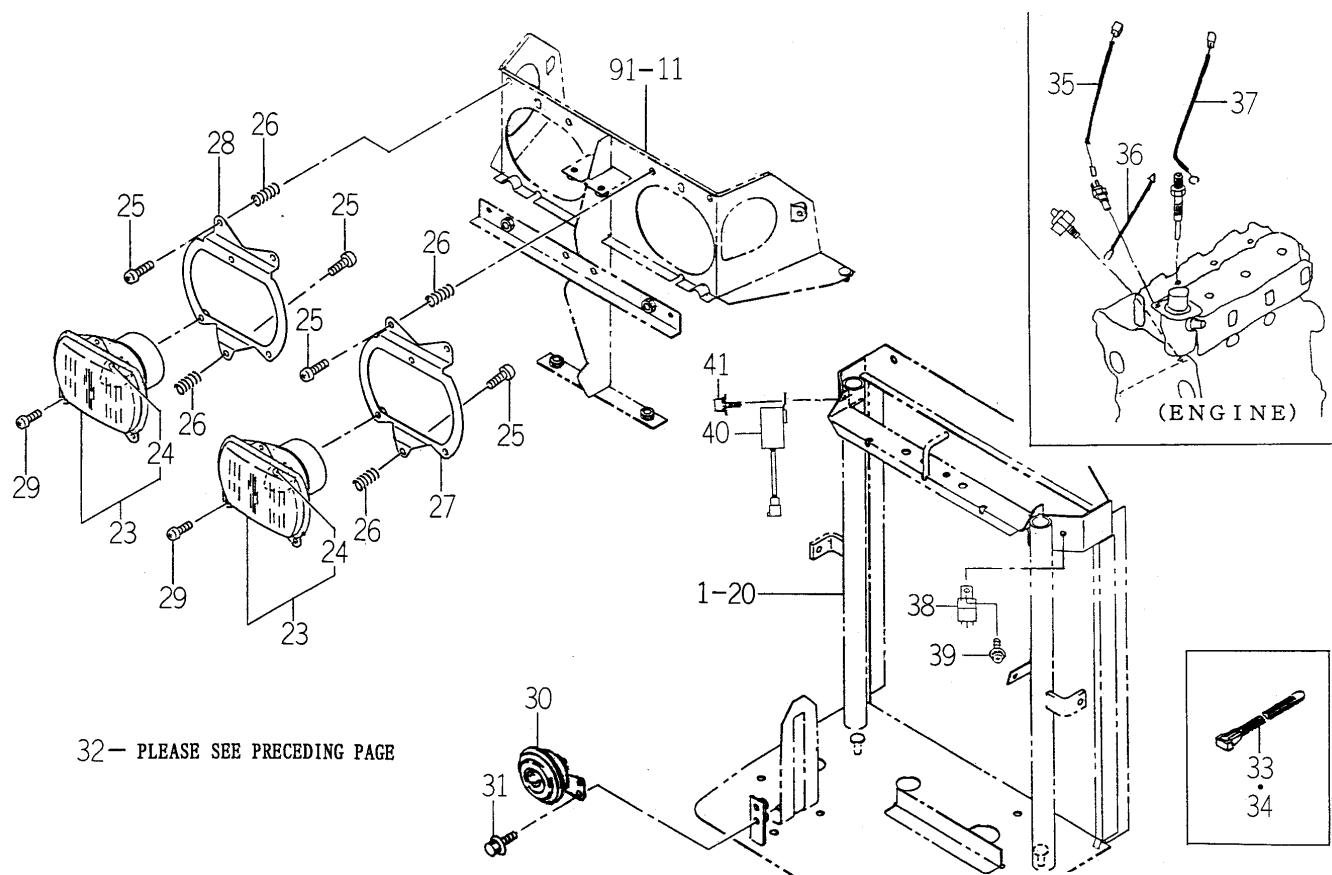
FIG.110 ELC. SYSTEM (FRONT) (SE4 TYPE)(2/2)
