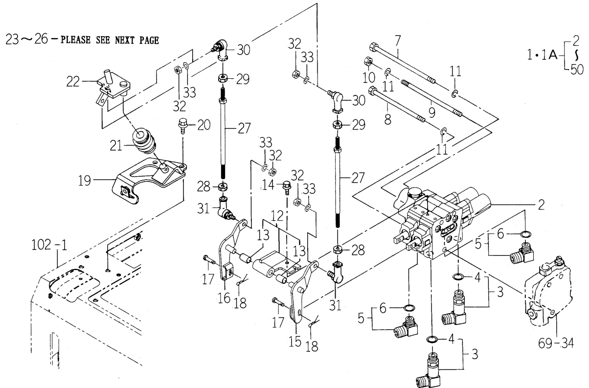
FIG. 77 JOY STICK VALVE SET (E6 TYPE-STANDARD/E4 TYPE-OPTION)(1/2)
