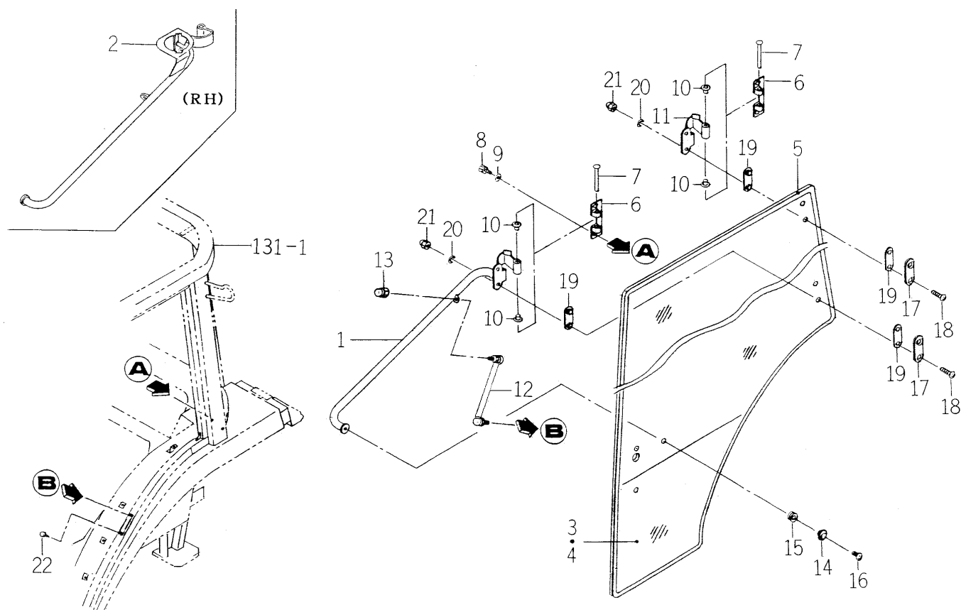
FIG.133 DOOR SYSTEM (C TYPE)
