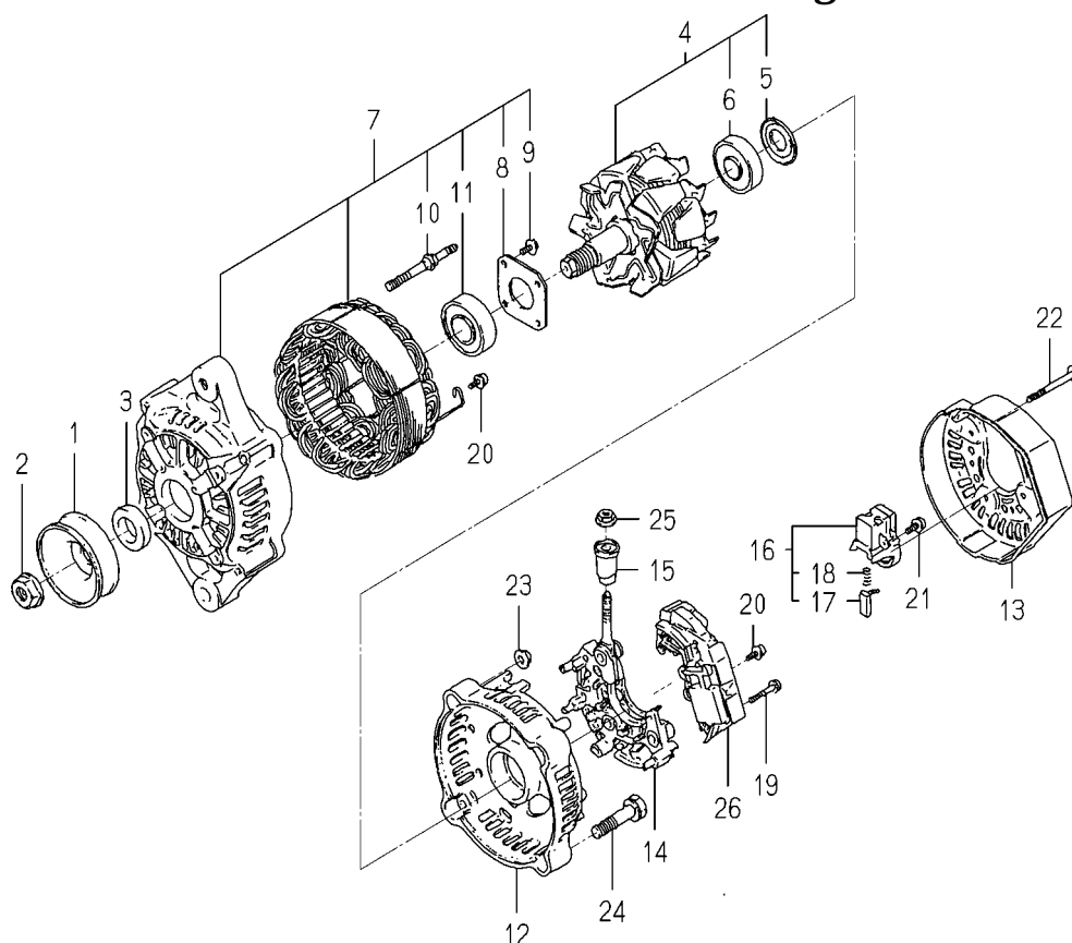
FIG. 30 COMPONENT PARTS FOR 6281-200-020-00 ON Fig.24
