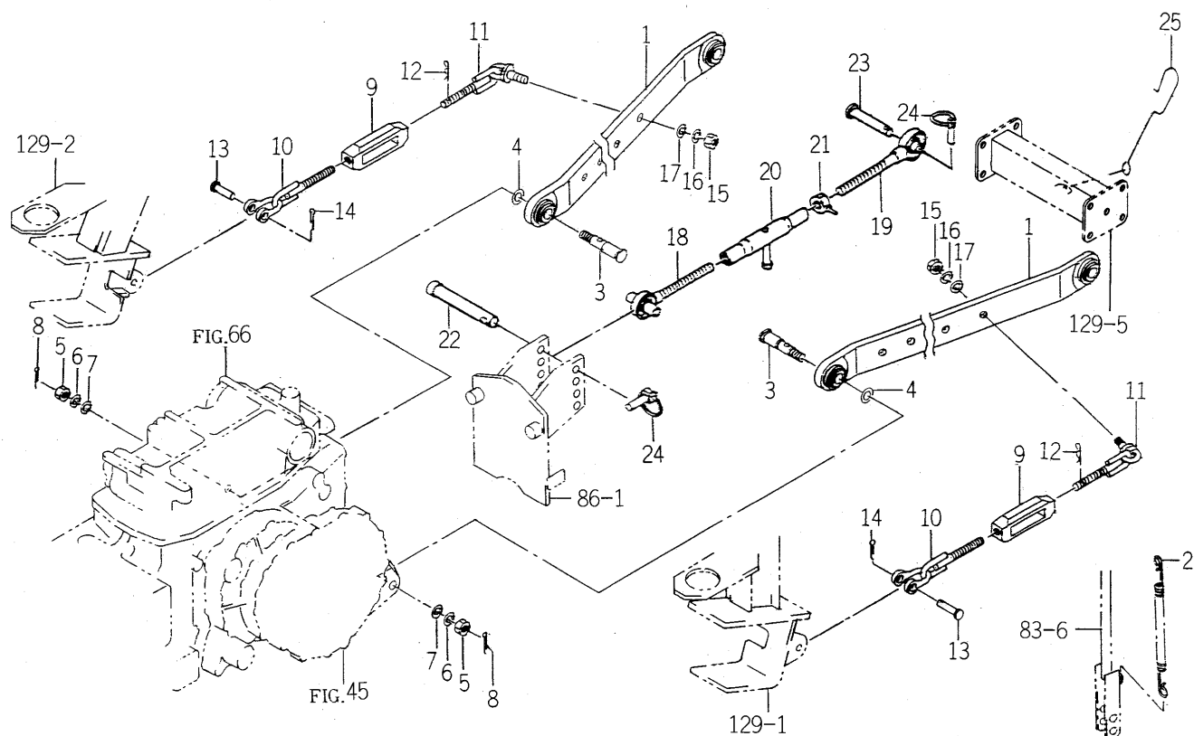
FIG. 80 3P LINK SYSTEM (E4 TYPE EXCEPT C)
