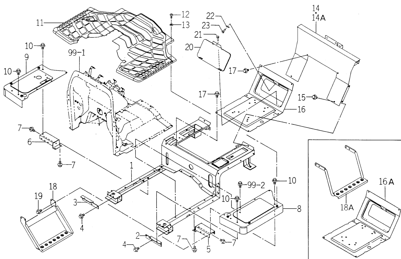
FIG.103 FLOOR (REAR) SYSTEM (S TYPE)
