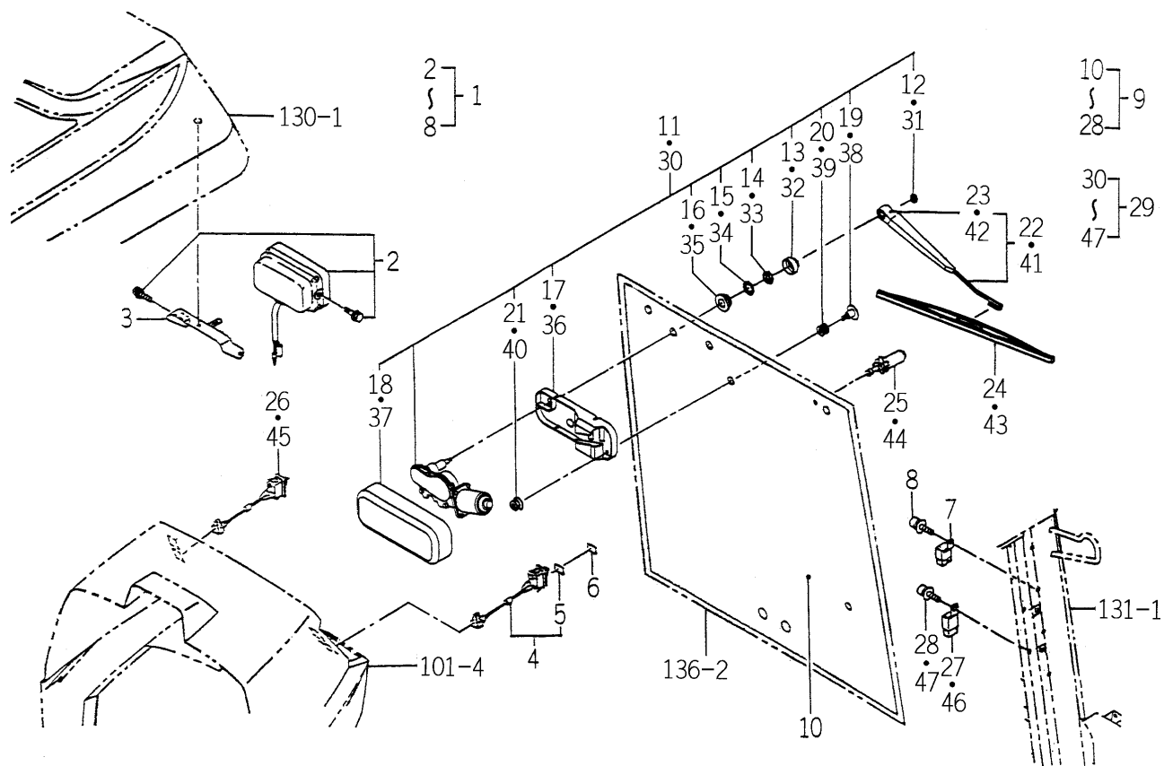
FIG.156 ELC. SYSTEM (C TYPE) (OPTION)
