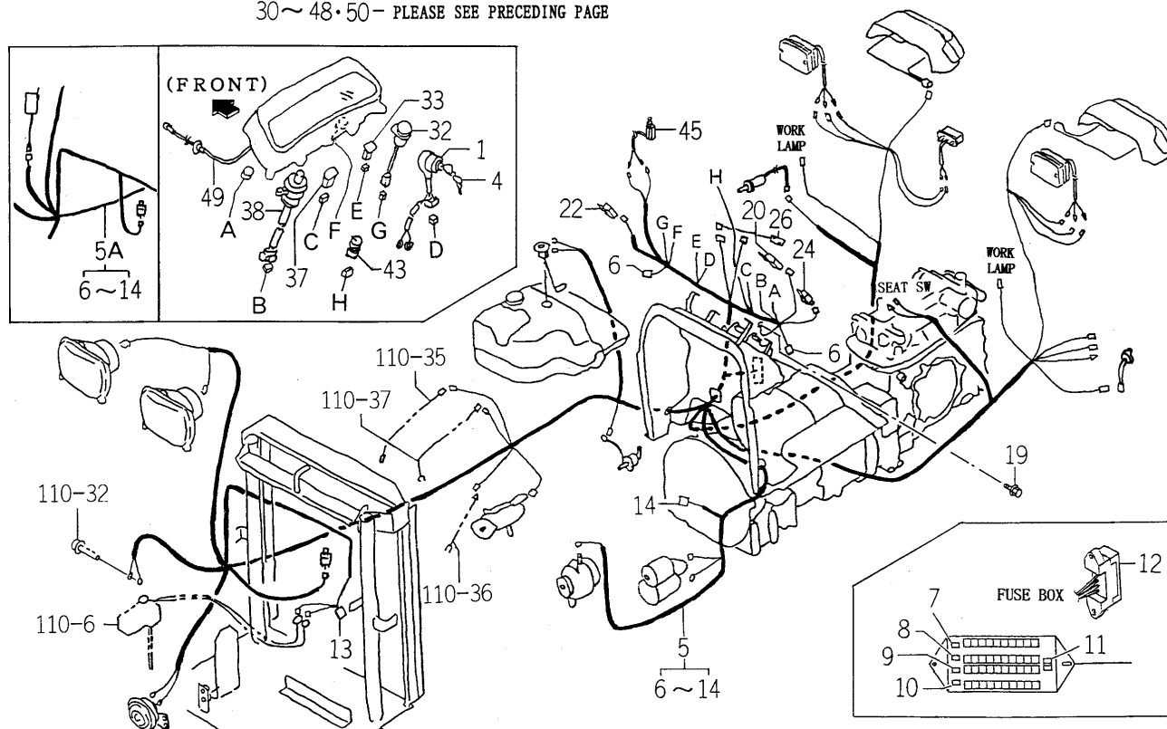
FIG.113 ELC. SYSTEM (MAIN) (S TYPE)(2/2)
