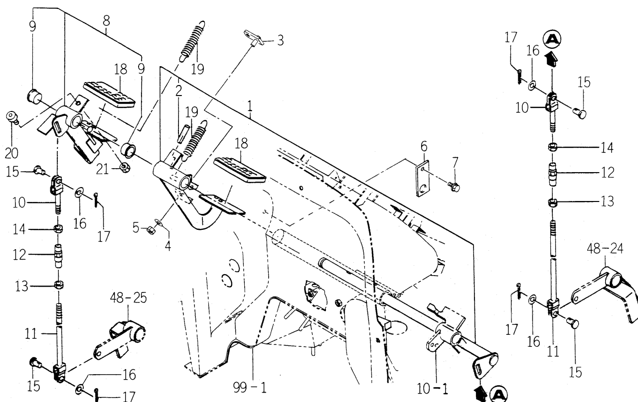
FIG. 51 PEDAL (BRAKE) SYSTEM (E4 TYPE EXCEPT H)
