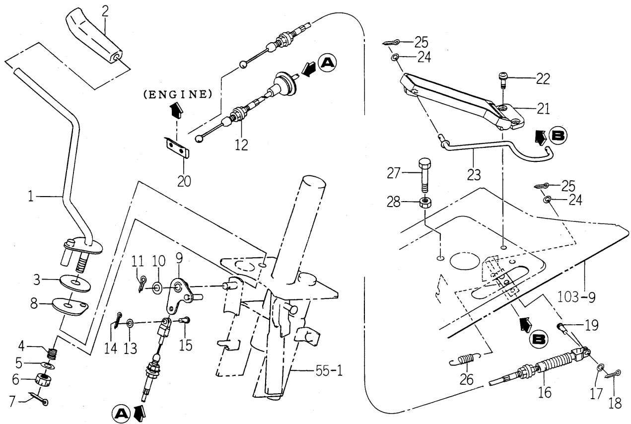
FIG. 7 ACCELERATOR SYSTEM (EXCEPT H TYPE)
