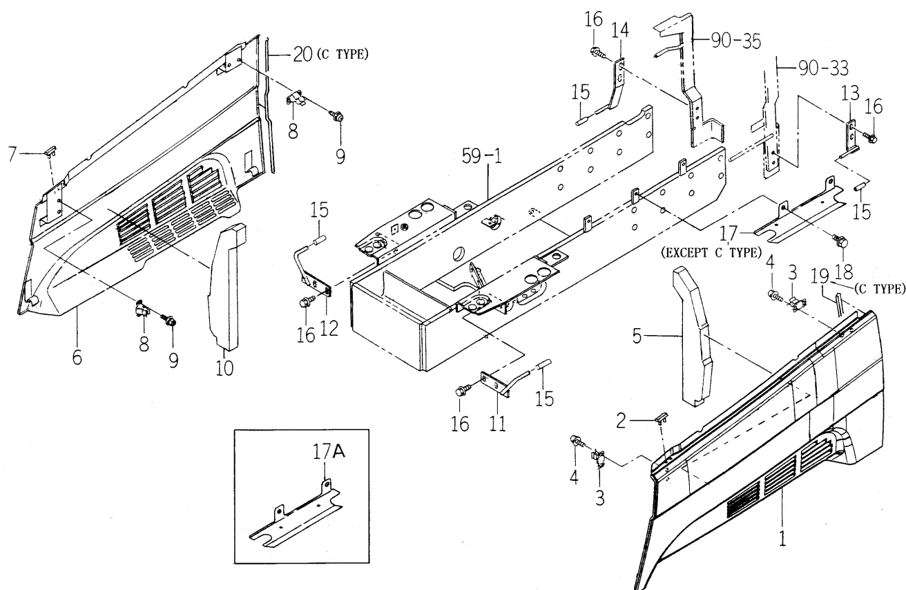
FIG. 92 COVER (SIDE) SYSTEM
