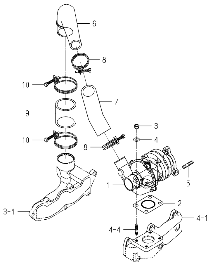
FIG. 5 TURBO CHARGER
