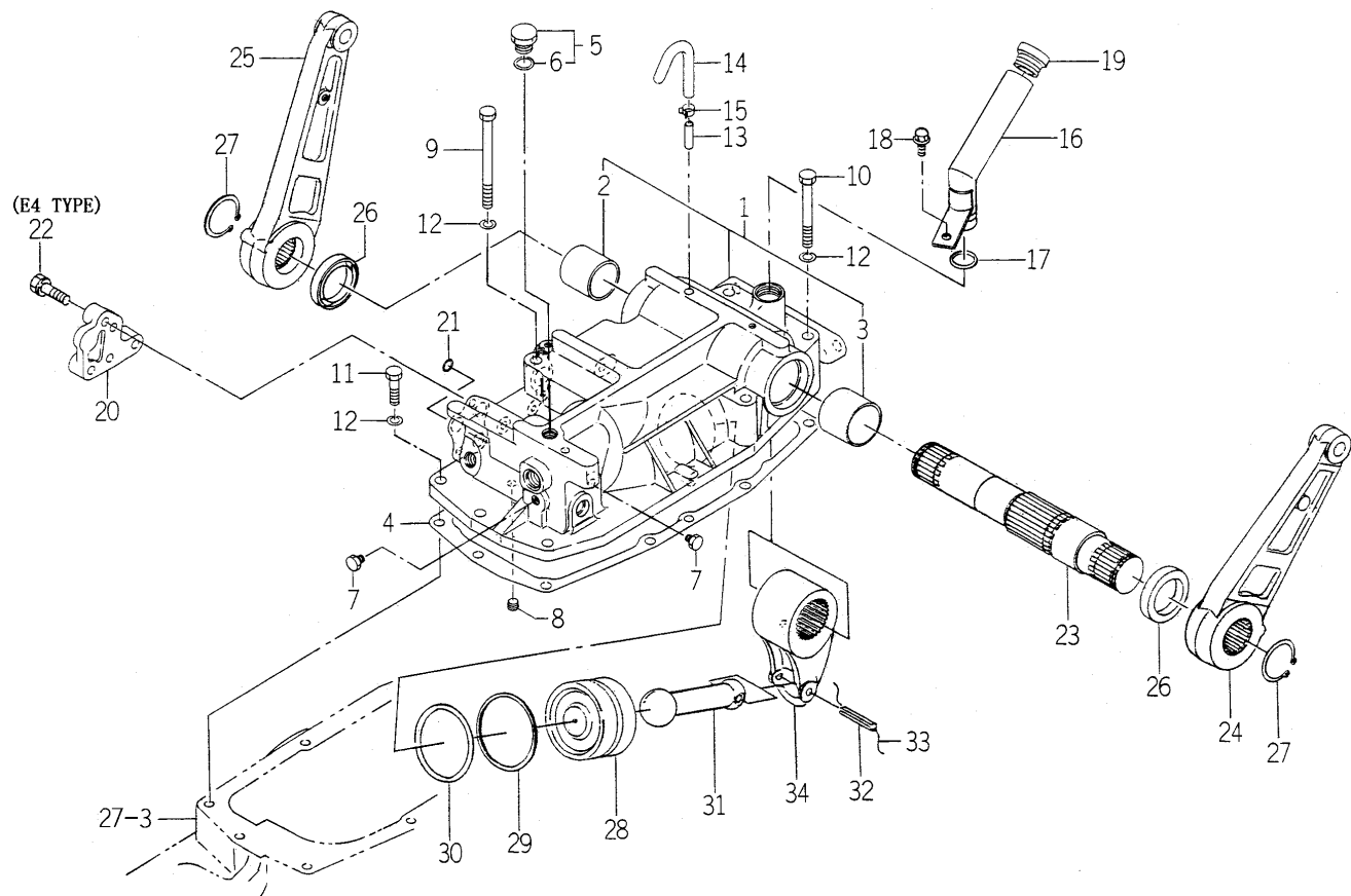
FIG. 66 CYLINDER CASE SYSTEM
