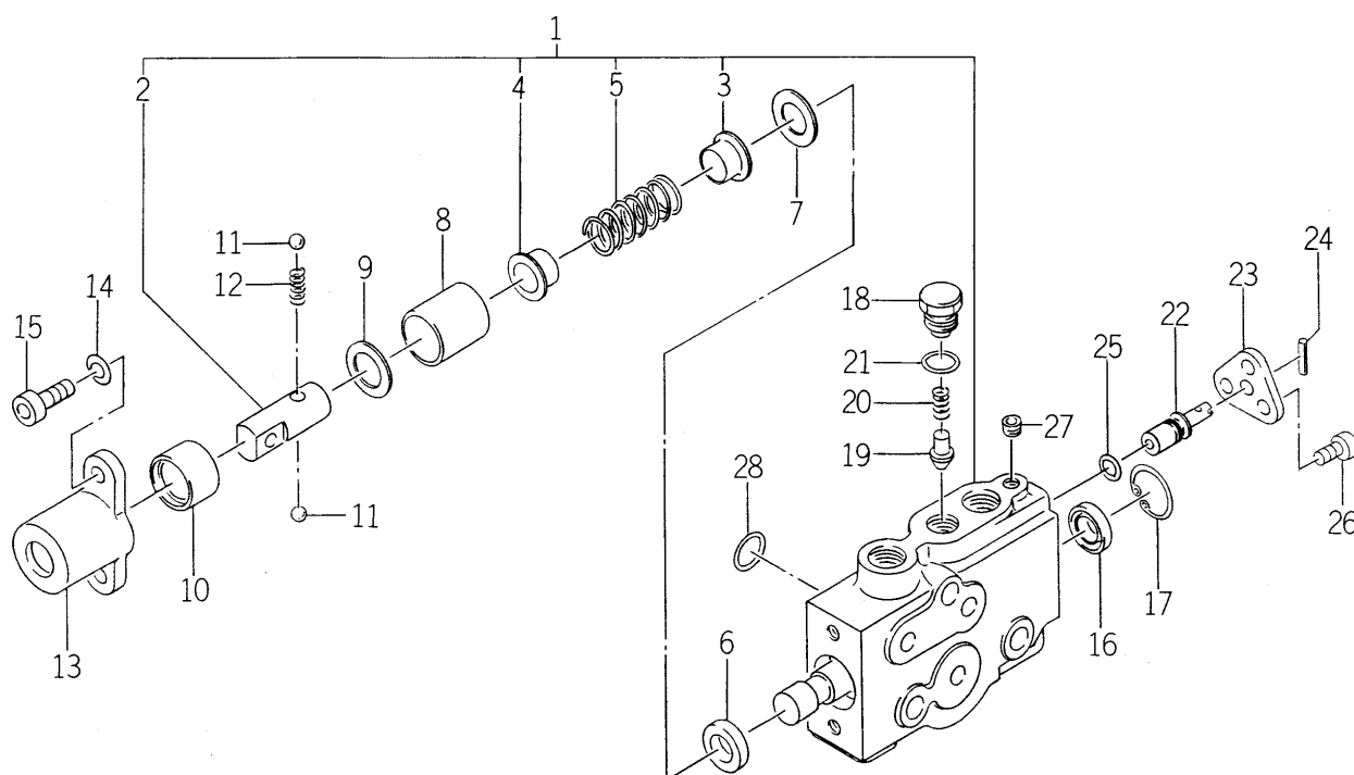
FIG.165 COMPONENT PARTS FOR 1640-530-600-10 ON Fig.78,152-155
