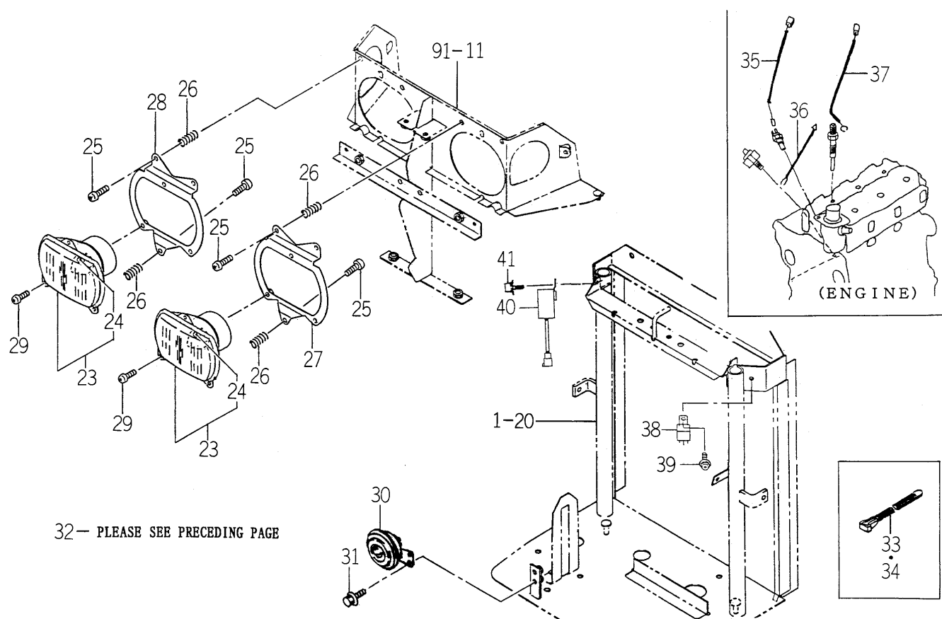
FIG.112 ELC. SYSTEM (FRONT) (HE4,QE4 TYPE)(2/2)
