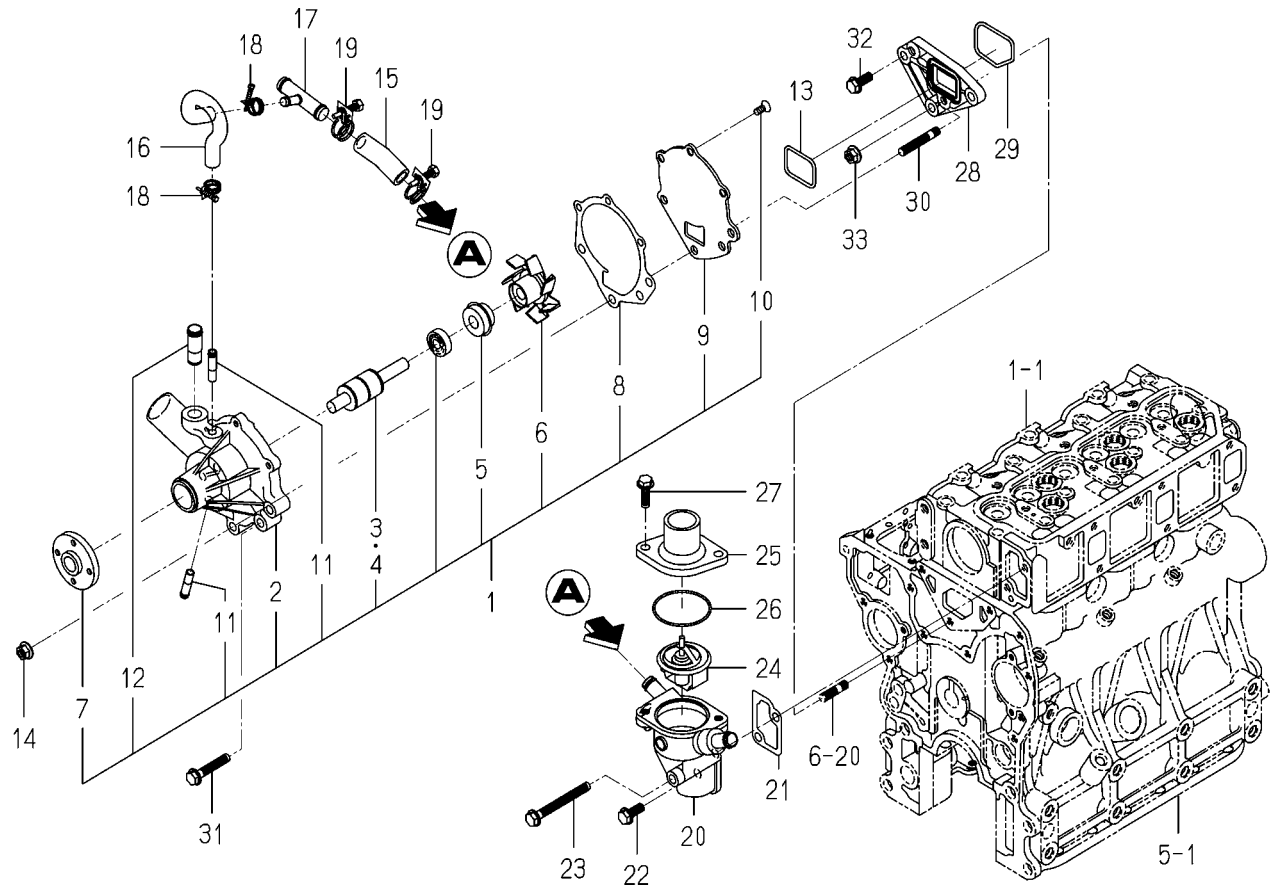
FIG. 18 WATER PUMP
