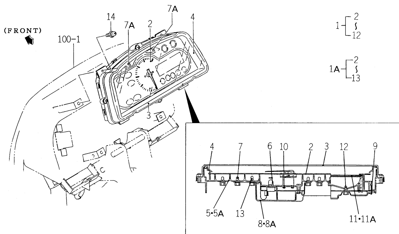
FIG.121 METER PANEL SYSTEM (HE4,QE4 TYPE)
