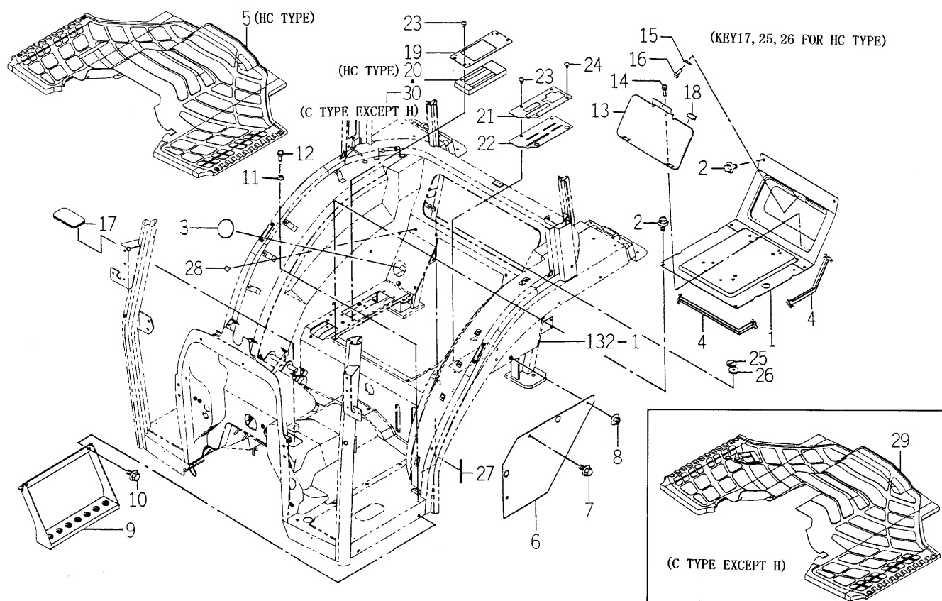
FIG.105 FLOOR (REAR) SYSTEM (C TYPE)
