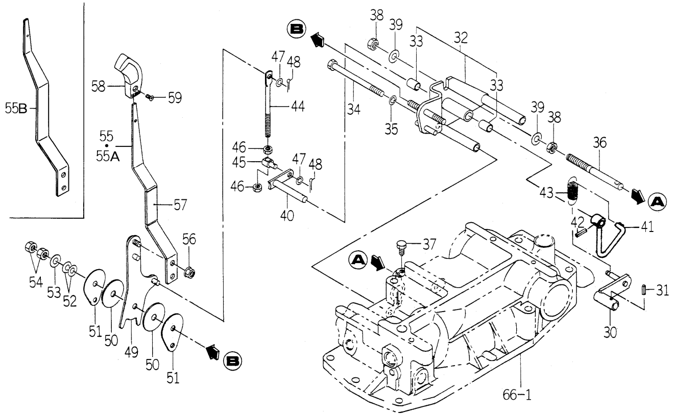
FIG. 67 MECHANICAL LINK(2/2) (POSITION) SYSTEM
