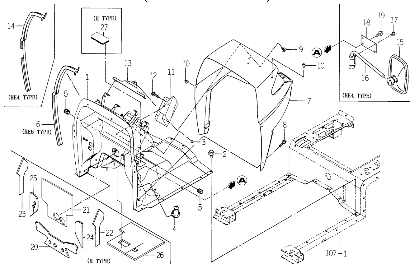
FIG.100 FLOOR (FRONT) SYSTEM (H TYPE EXCEPT C)
