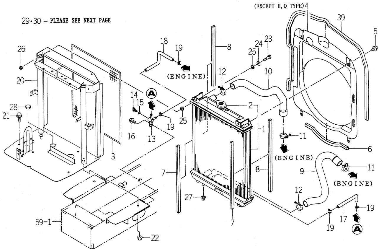
FIG. 1 RADIATOR SYSTEM (EXCEPT H TYPE)(1/2)
