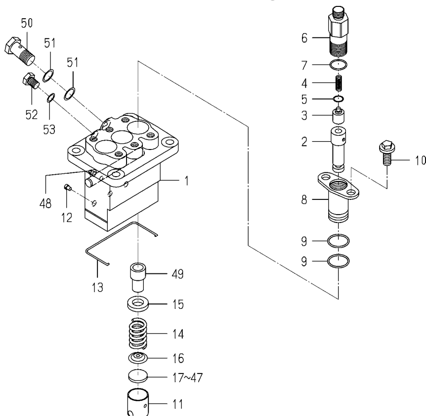
FIG. 27 COMPONENT PARTS FOR 6215-600-104-20 ON Fig.20
