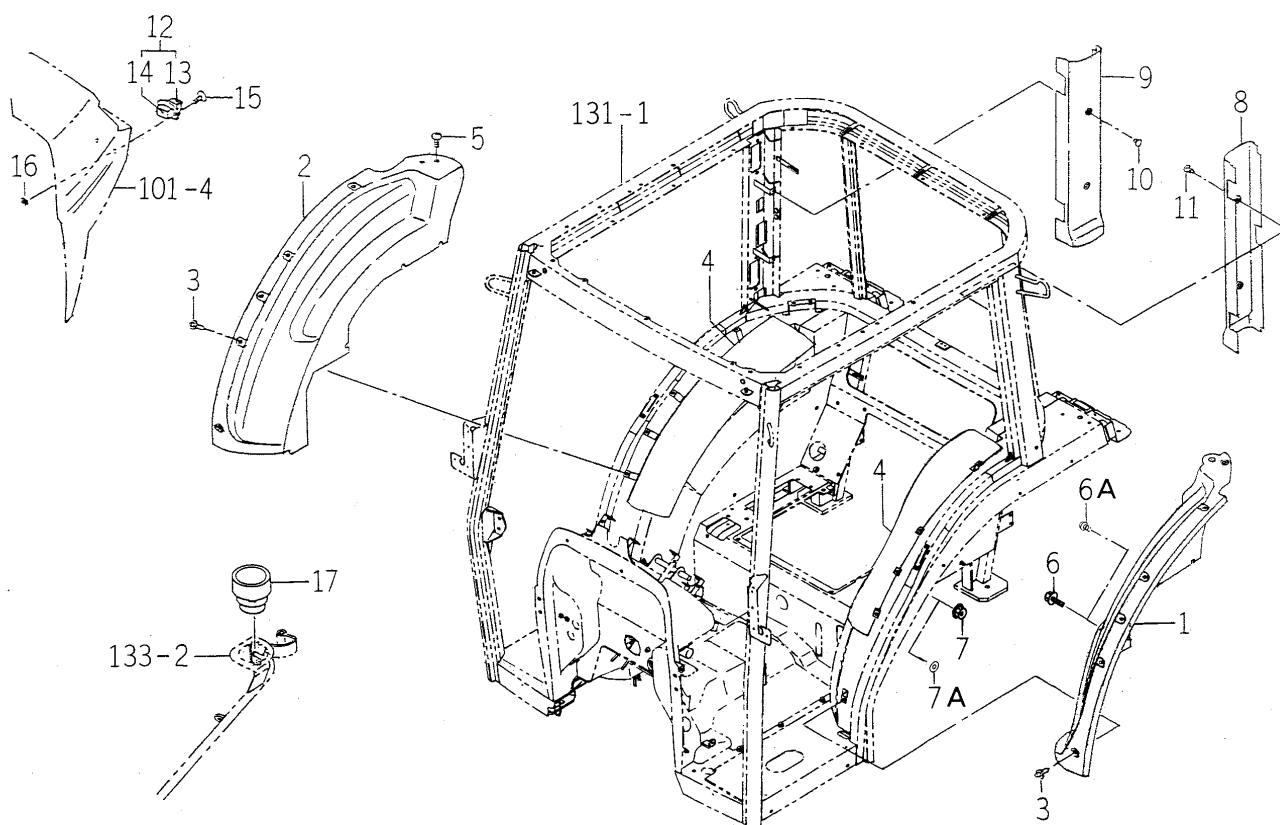
FIG.137 INTERIOR SYSTEM (C TYPE)
