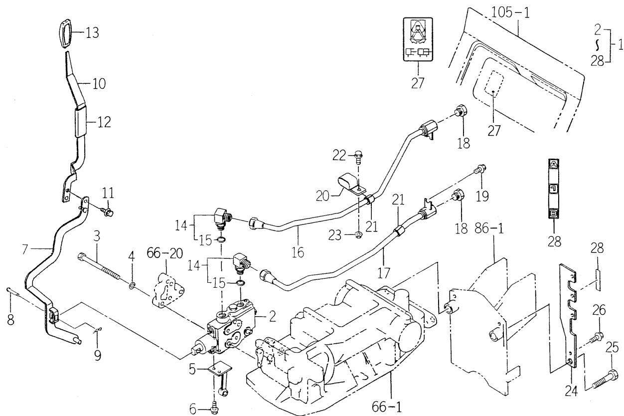
FIG.154 VALVE (REMOTE/1R) SET (C TYPE) (OPTION)
