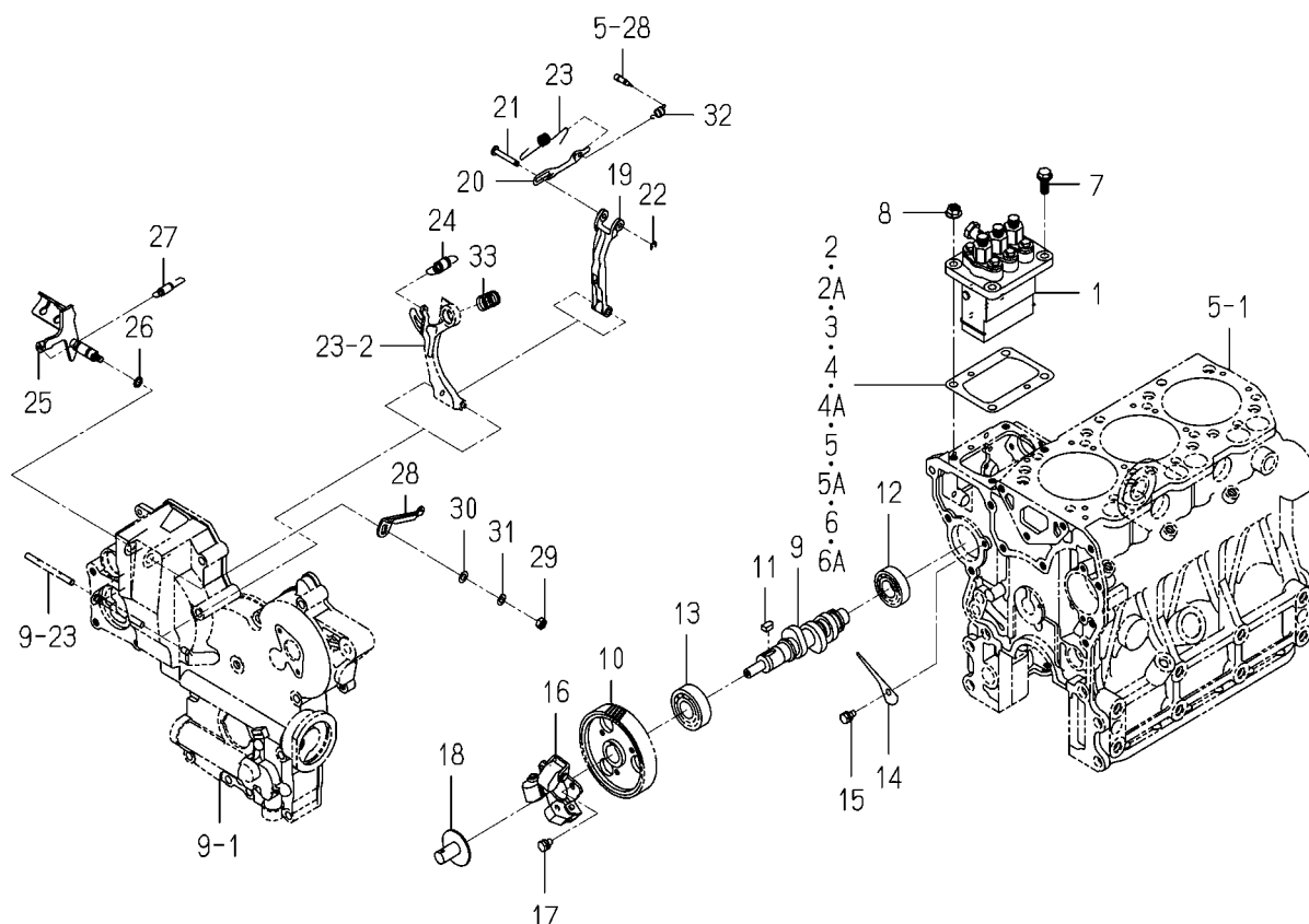
FIG. 21 INJECTION PUMP
