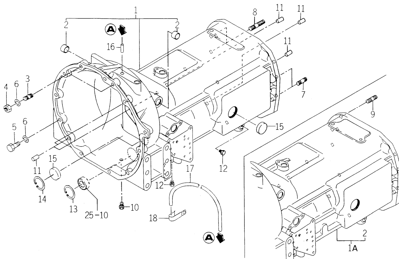
FIG. 11 CASE (TRANSMISSION/FRONT) SYSTEM (P TYPE)
