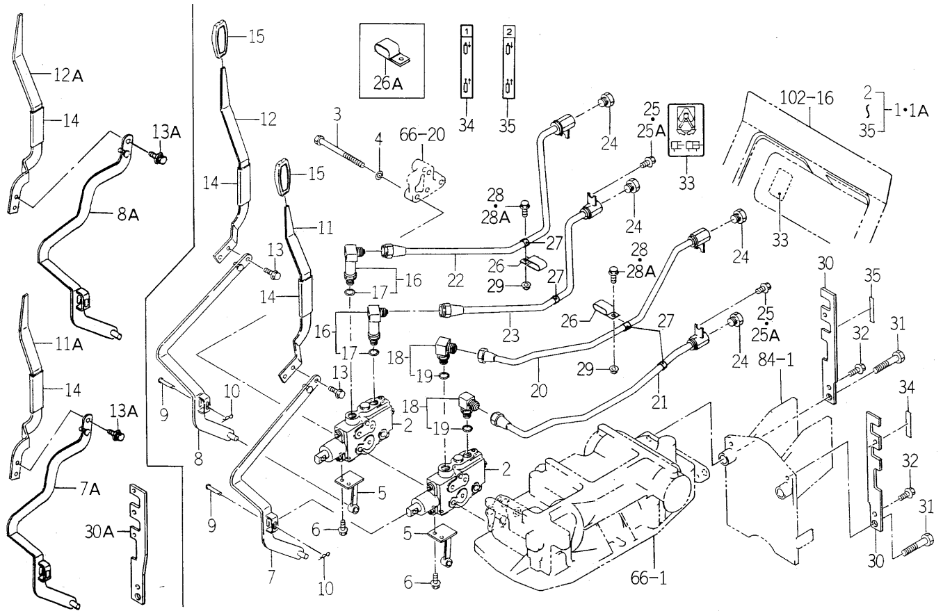
FIG. 78 VALVE (REMOTE/2R) SET (E6 TYPE)
