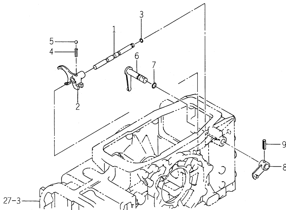
FIG. 35 FORK (SHIFT/PTO) SYSTEM
