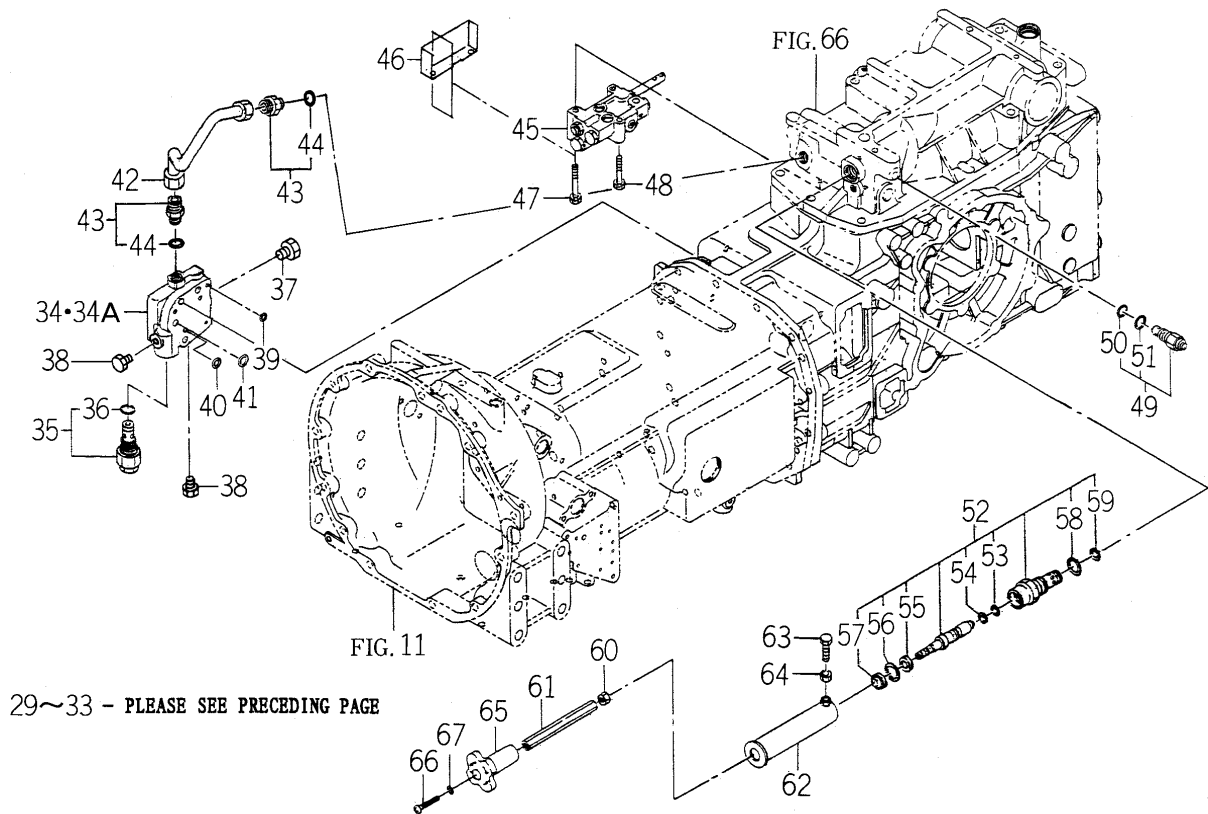
FIG. 71 HYD. SYSTEM (MAIN) (P,Q TYPE)(2/2)
