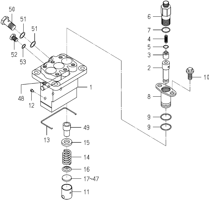
FIG. 28 COMPONENT PARTS FOR 6215-600-078-10 ON Fig.21
