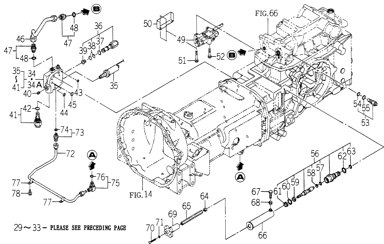
FIG. 69 HYD. SYSTEM (MAIN) (S TYPE)(2/2)
