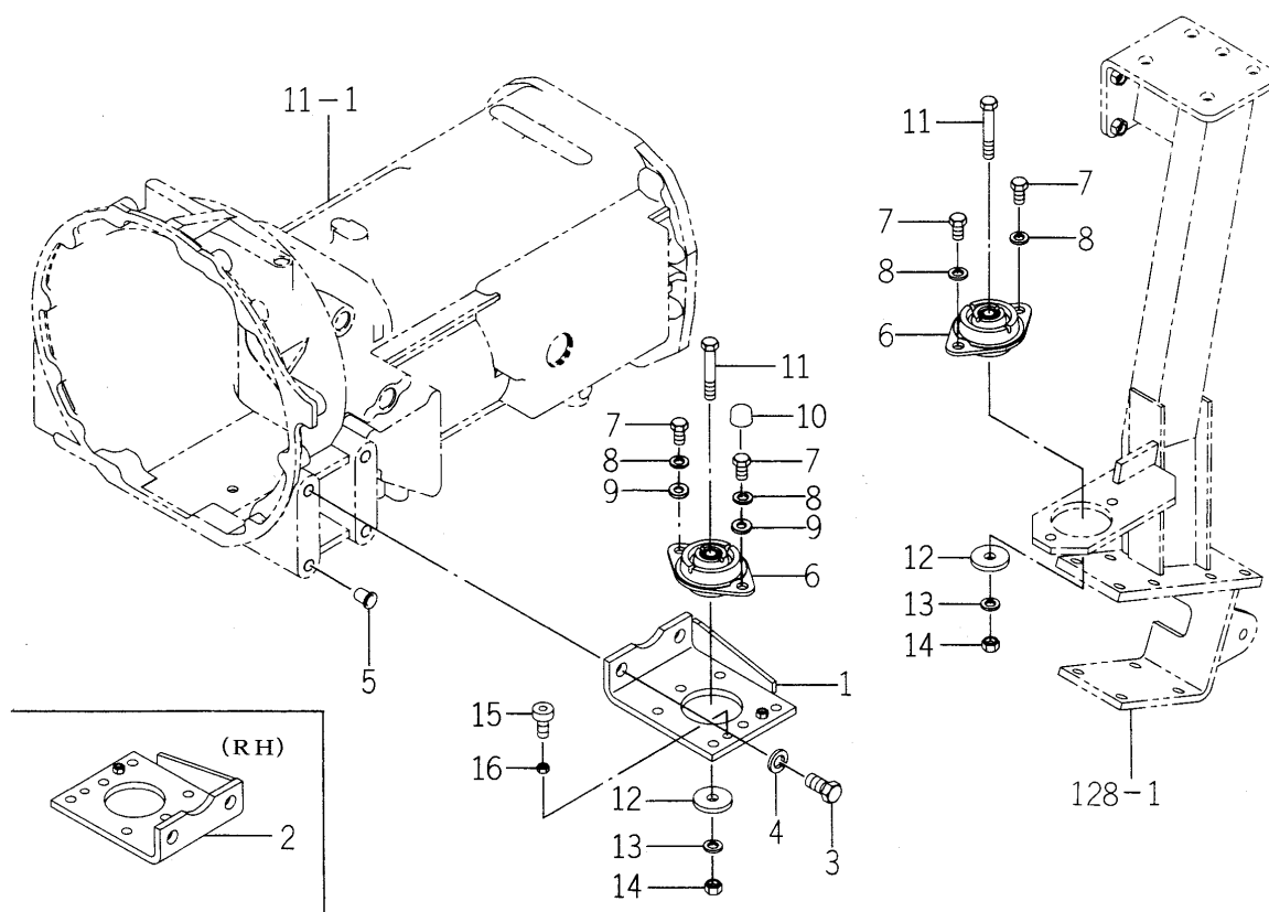
FIG. 97 MOUNT SYSTEM (EXCEPT C TYPE)
