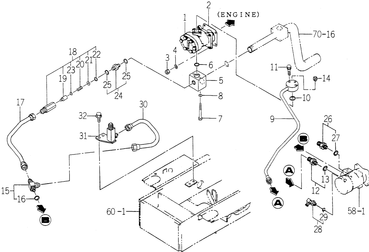
FIG. 74 HYD. SYSTEM (SUB) (H TYPE)(1/2)
