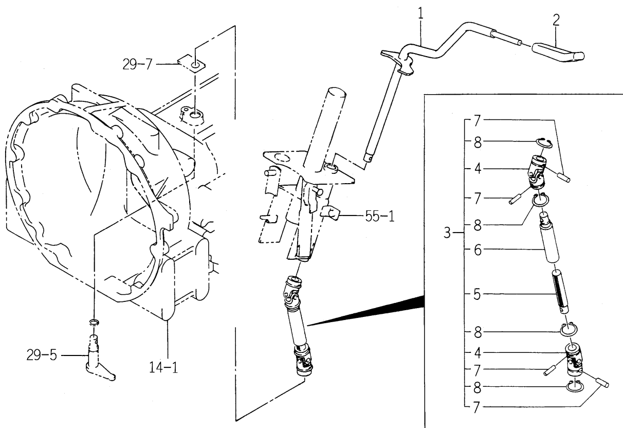
FIG. 36 LEVER (REVERSE) SYSTEM (S TYPE)
