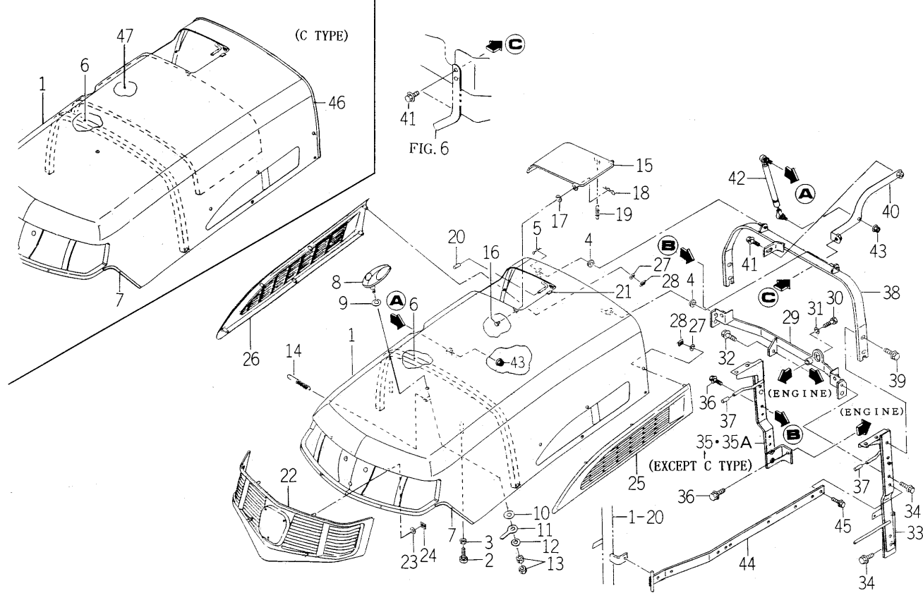
FIG. 90 HOOD SYSTEM
