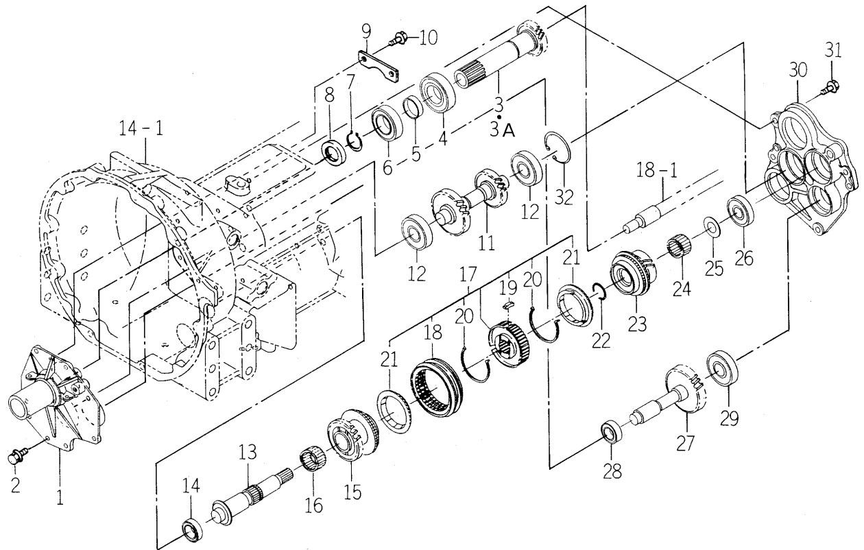
FIG. 17 GEAR (REVERSE) SYSTEM (S TYPE)
