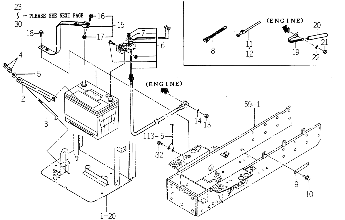
FIG.110 ELC. SYSTEM (FRONT) (SE4 TYPE)(1/2)
