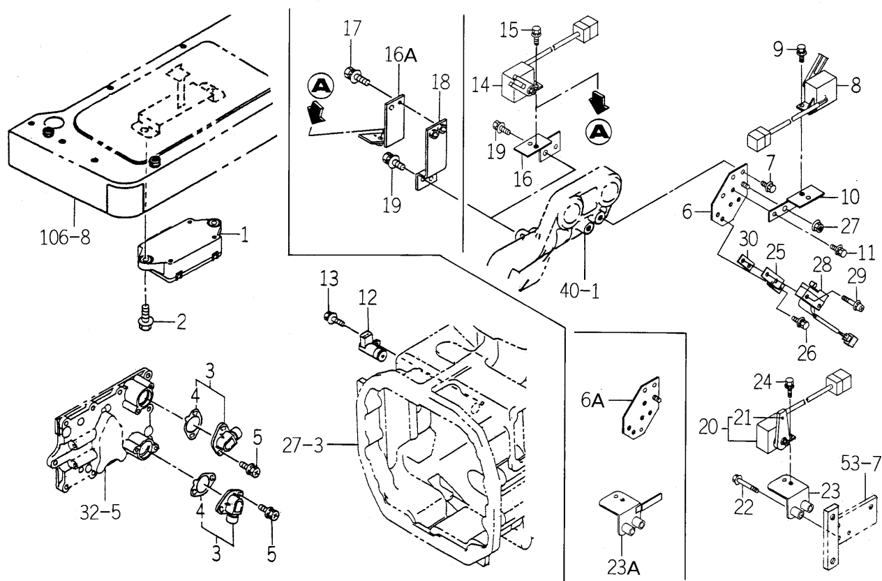
FIG.125 CONTROL SYSTEM (Q TYPE)
