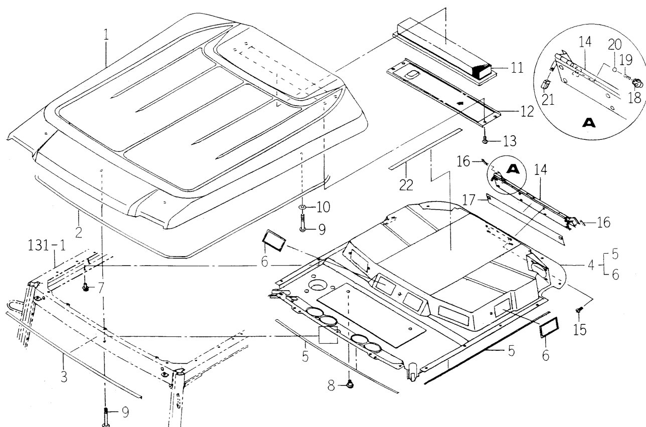
FIG.130 ROOF SYSTEM (C TYPE)
