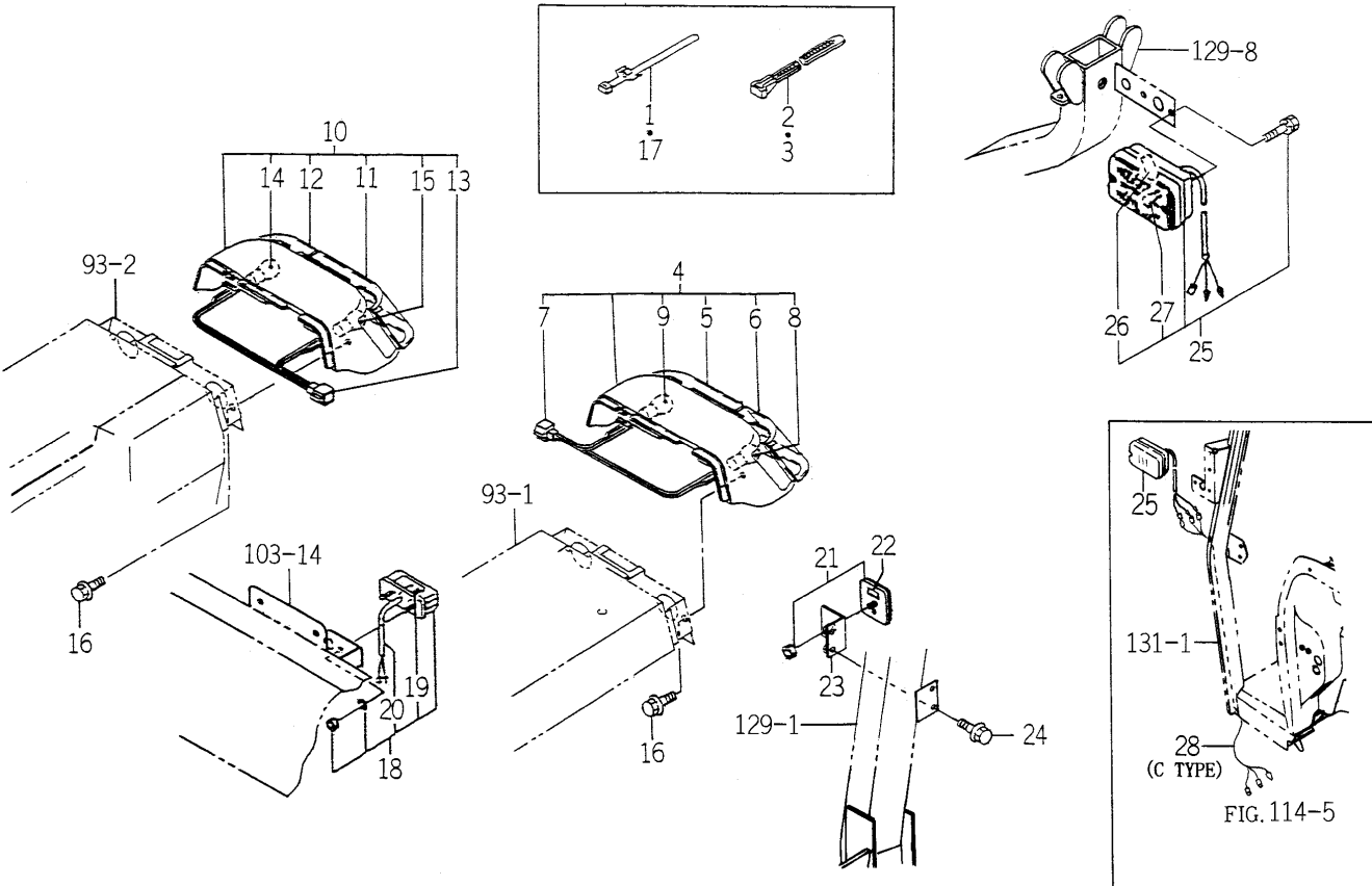
FIG.119 ELC. SYSTEM (REAR) (E4 TYPE)
