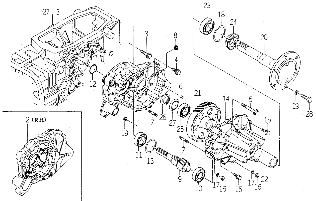
FIG. 45 HOUSING (AXLE/REAR) SYSTEM
