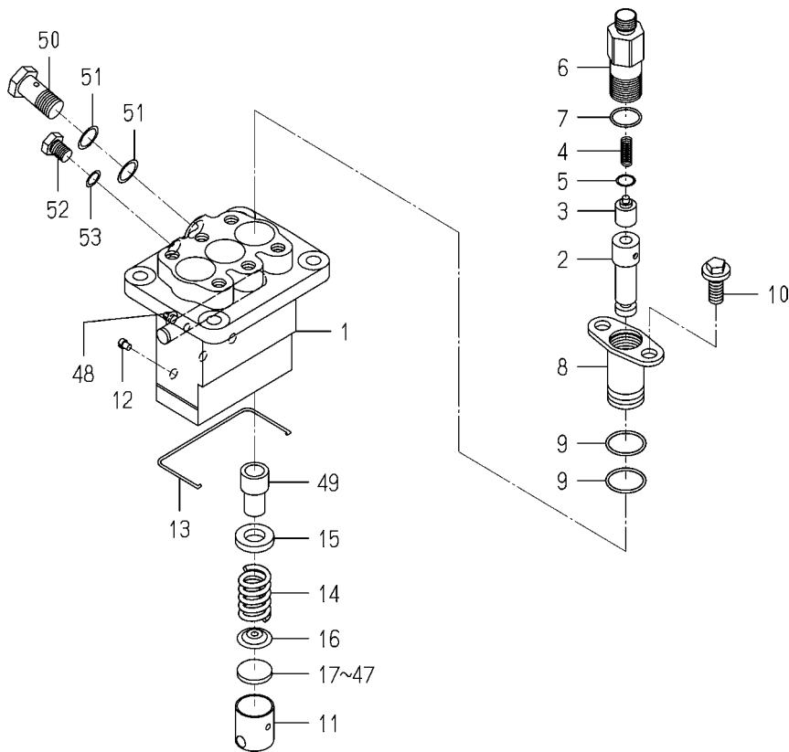
FIG. 28 COMPONENT PARTS FOR 6215-600-078-10 ON Fig.21
