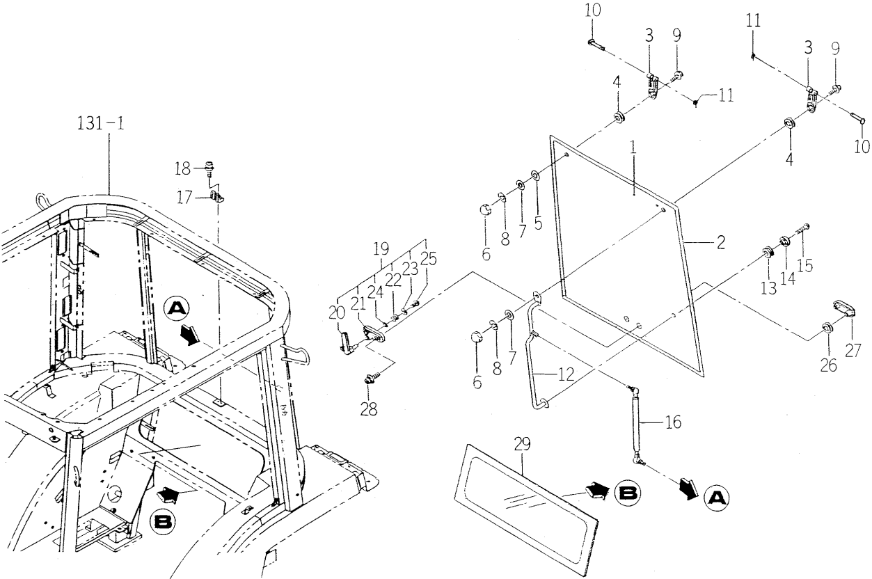
FIG.136 GLASS (REAR) SYSTEM (C TYPE)
