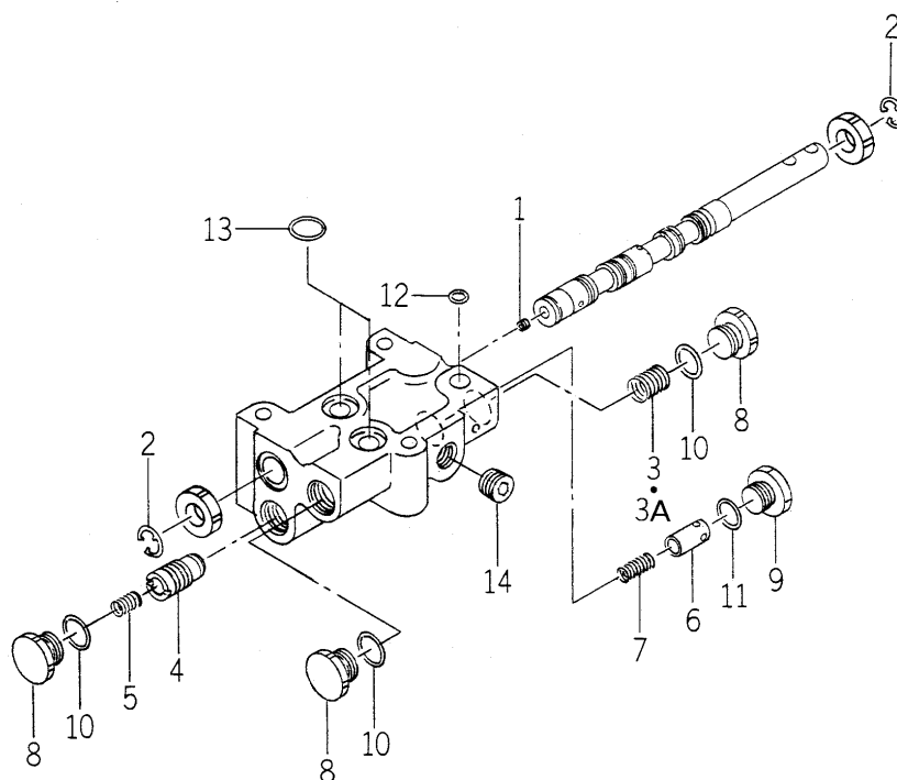
FIG.161 COMPONENT PARTS FOR K211-073-000-00 ON Fig.69-71
