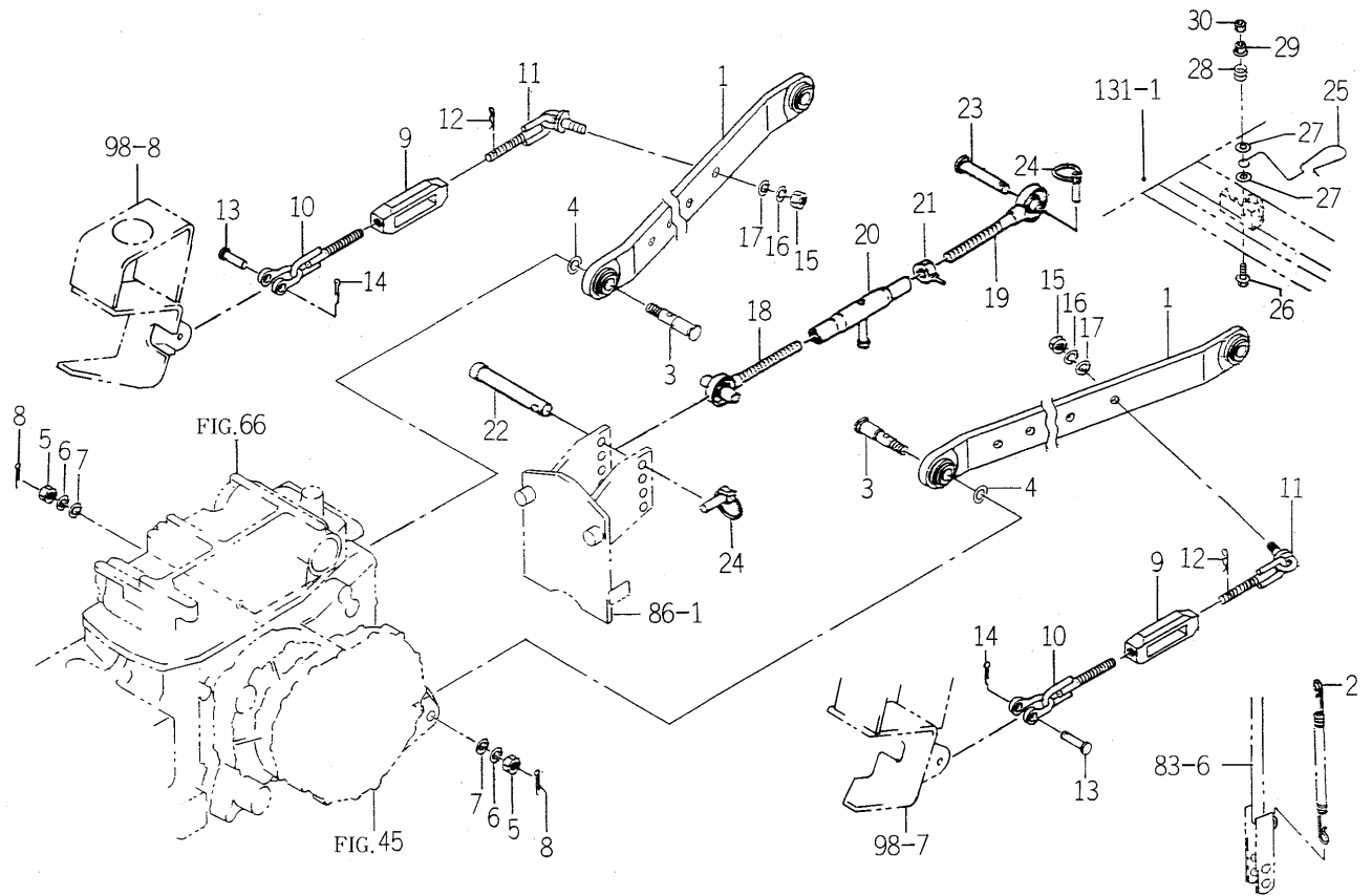
FIG. 81 3P LINK SYSTEM (C TYPE)
