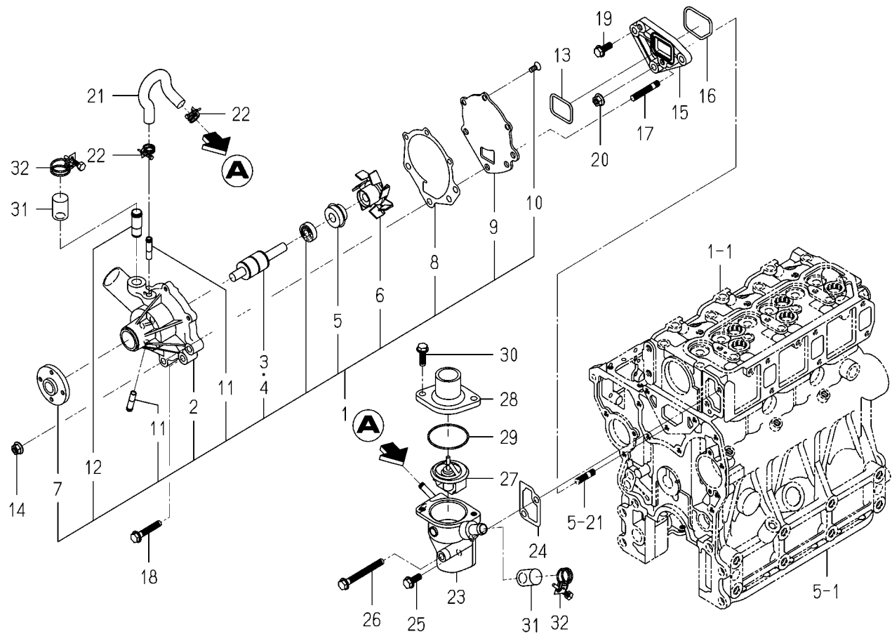
FIG. 18 WATER PUMP
