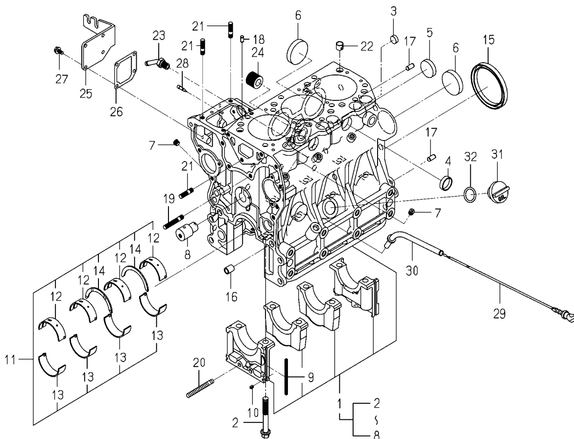
FIG. 5 CYLINDER BLOCK
