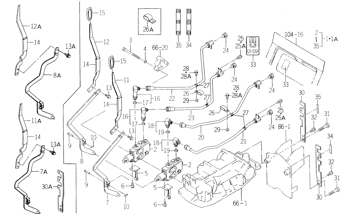
FIG.153 VALVE (REMOTE/2R) SET (E4 TYPE EXCEPT C) (OPTION)
