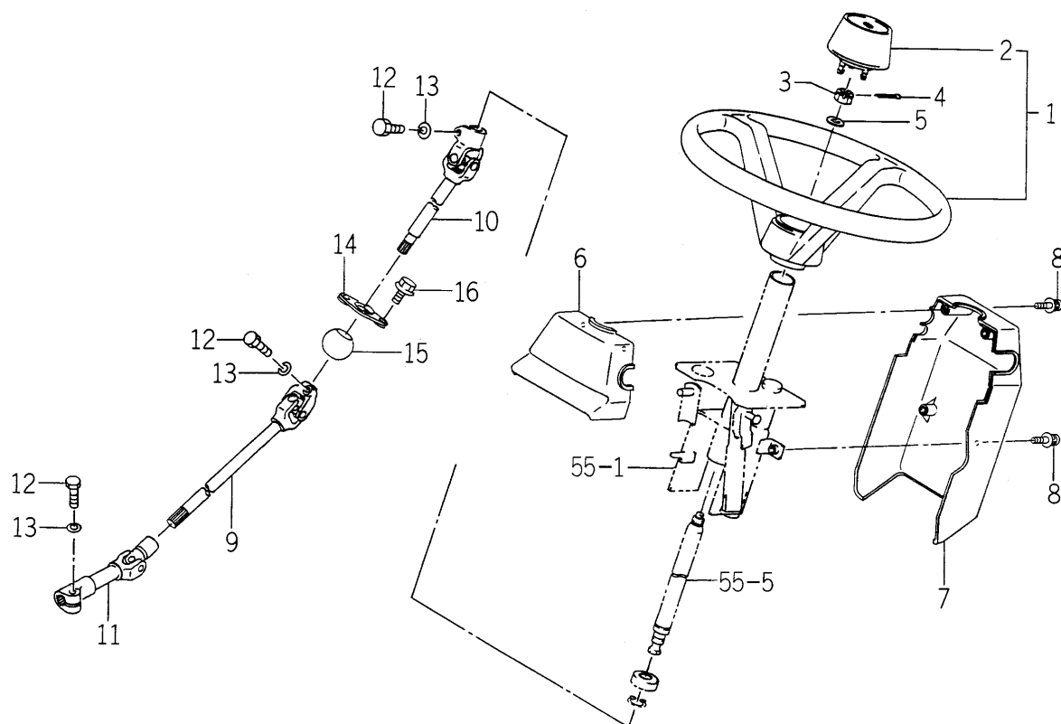
FIG. 54 WHEEL (STEERING) SYSTEM
