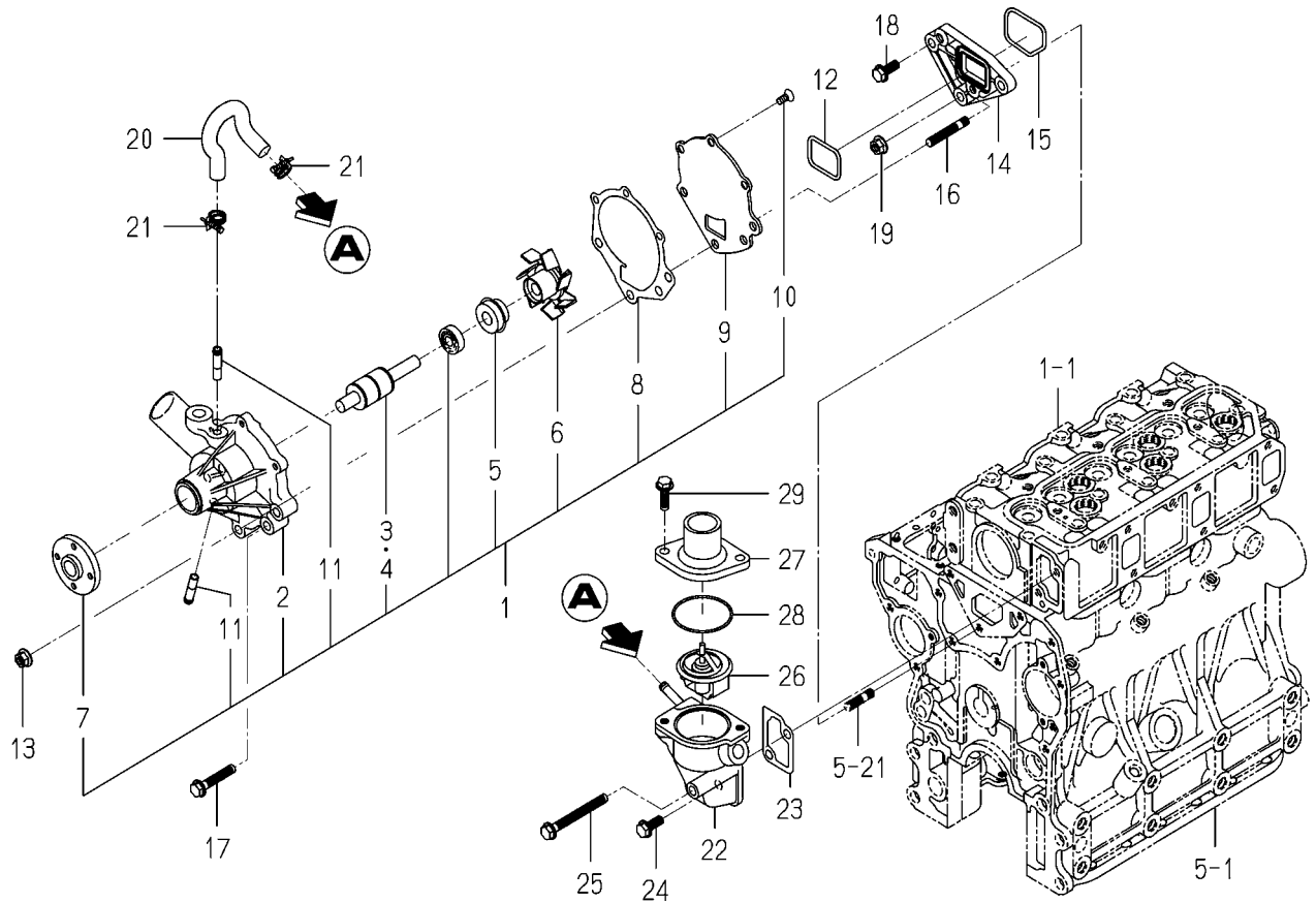
FIG. 17 WATER PUMP
