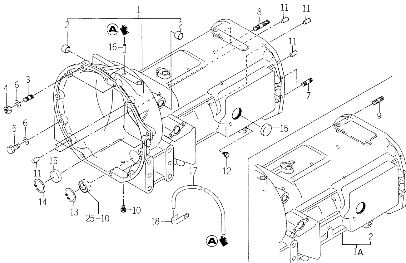
FIG. 14 CASE (TRANSMISSION/FRONT) SYSTEM (S TYPE)
