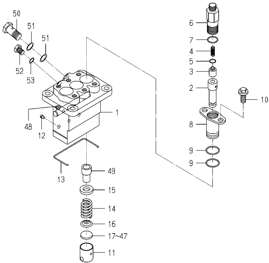
FIG. 28 COMPONENT PARTS FOR 6215-600-104-20 ON Fig.21
