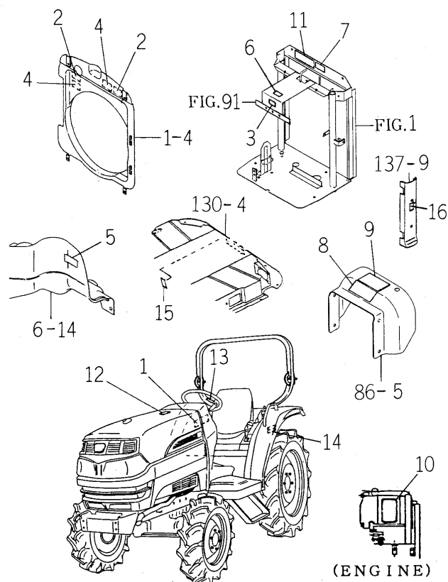
FIG.141 LABEL (CAUTION)
