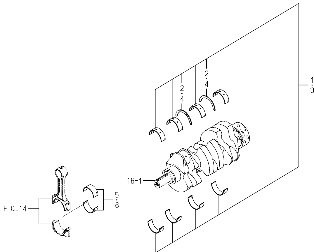
FIG. 7 BEARING/UNDER SIZE
