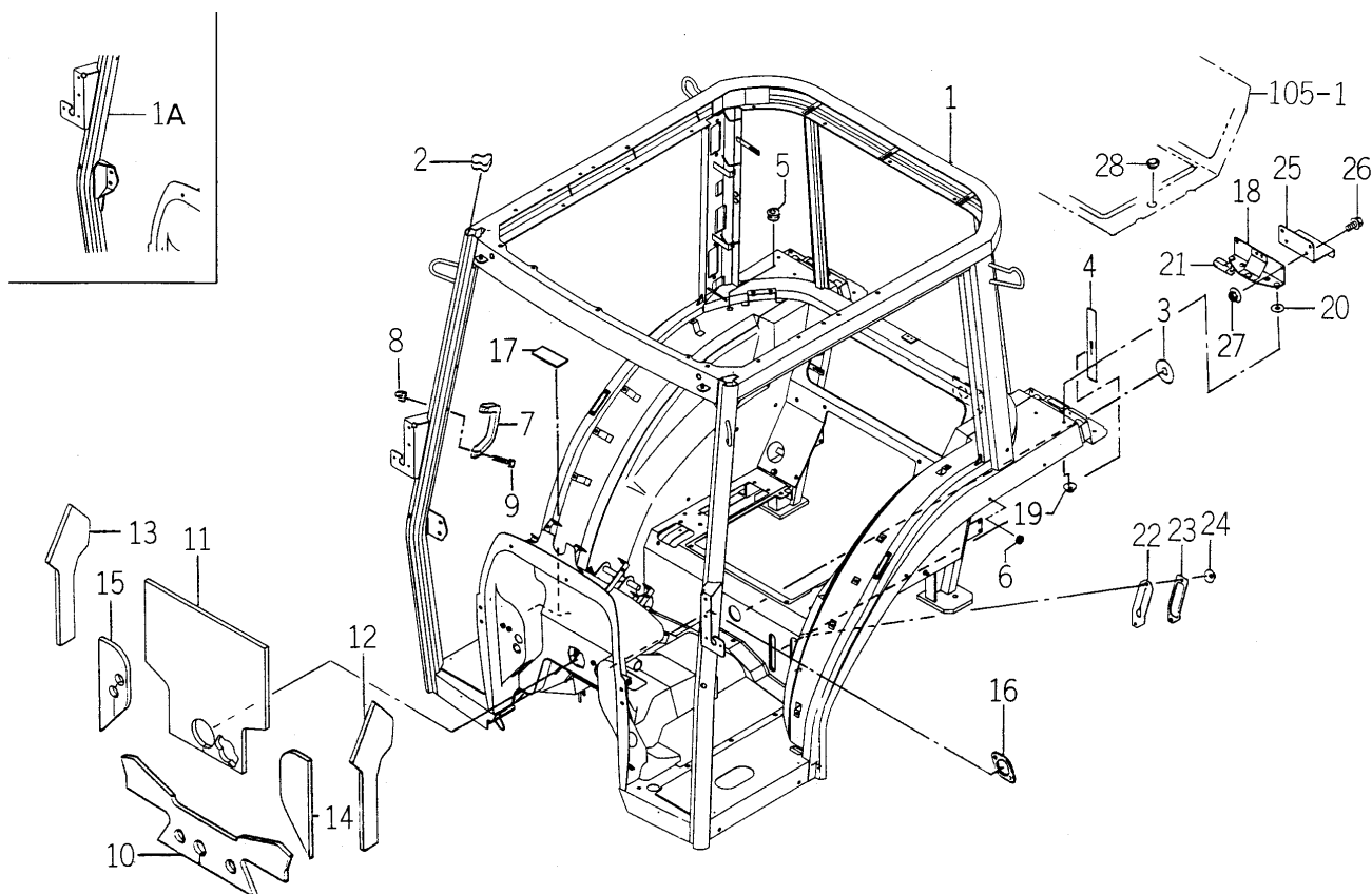
FIG.132 FRAME SYSTEM (HC TYPE)
