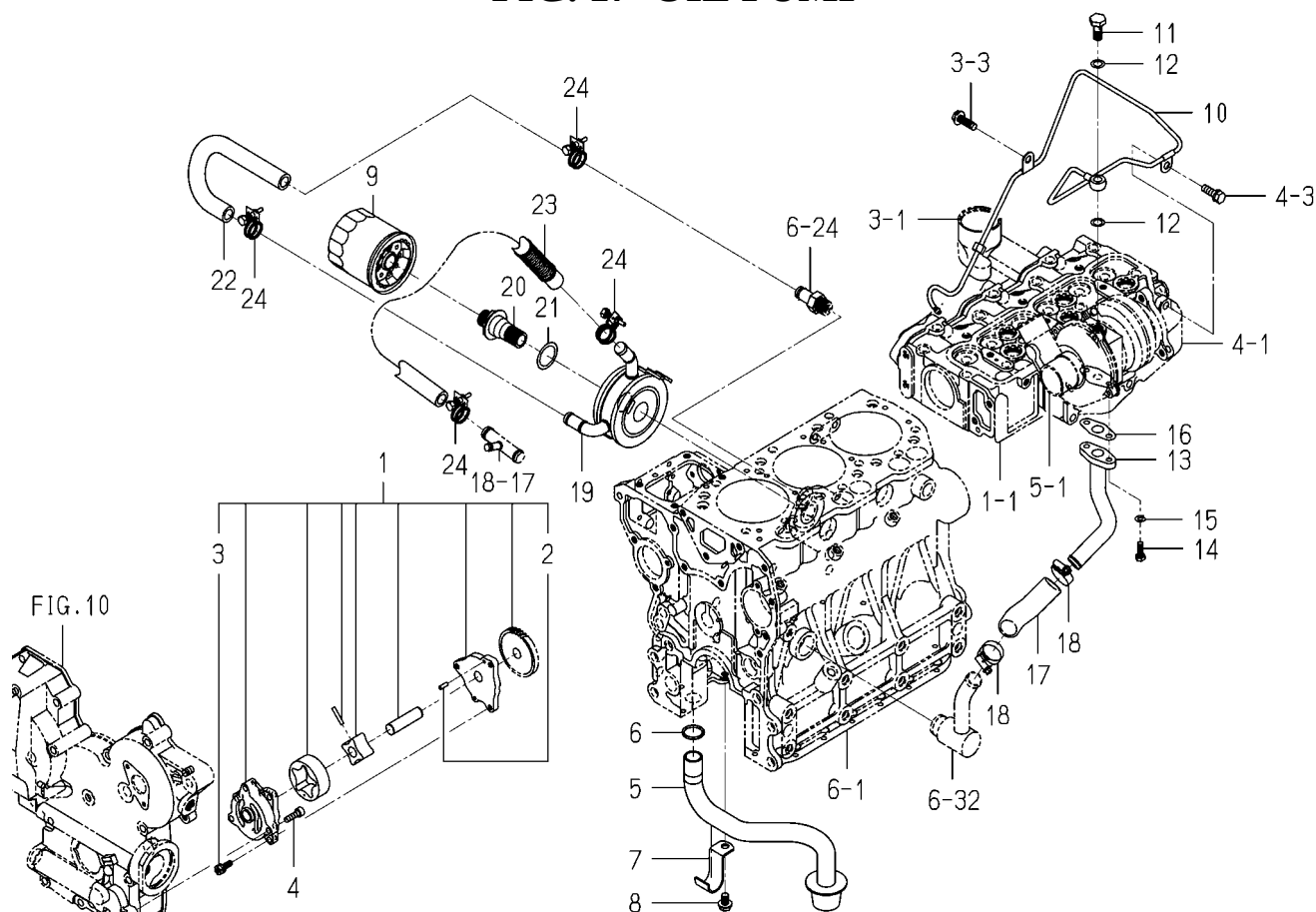
FIG. 17 OIL PUMP
