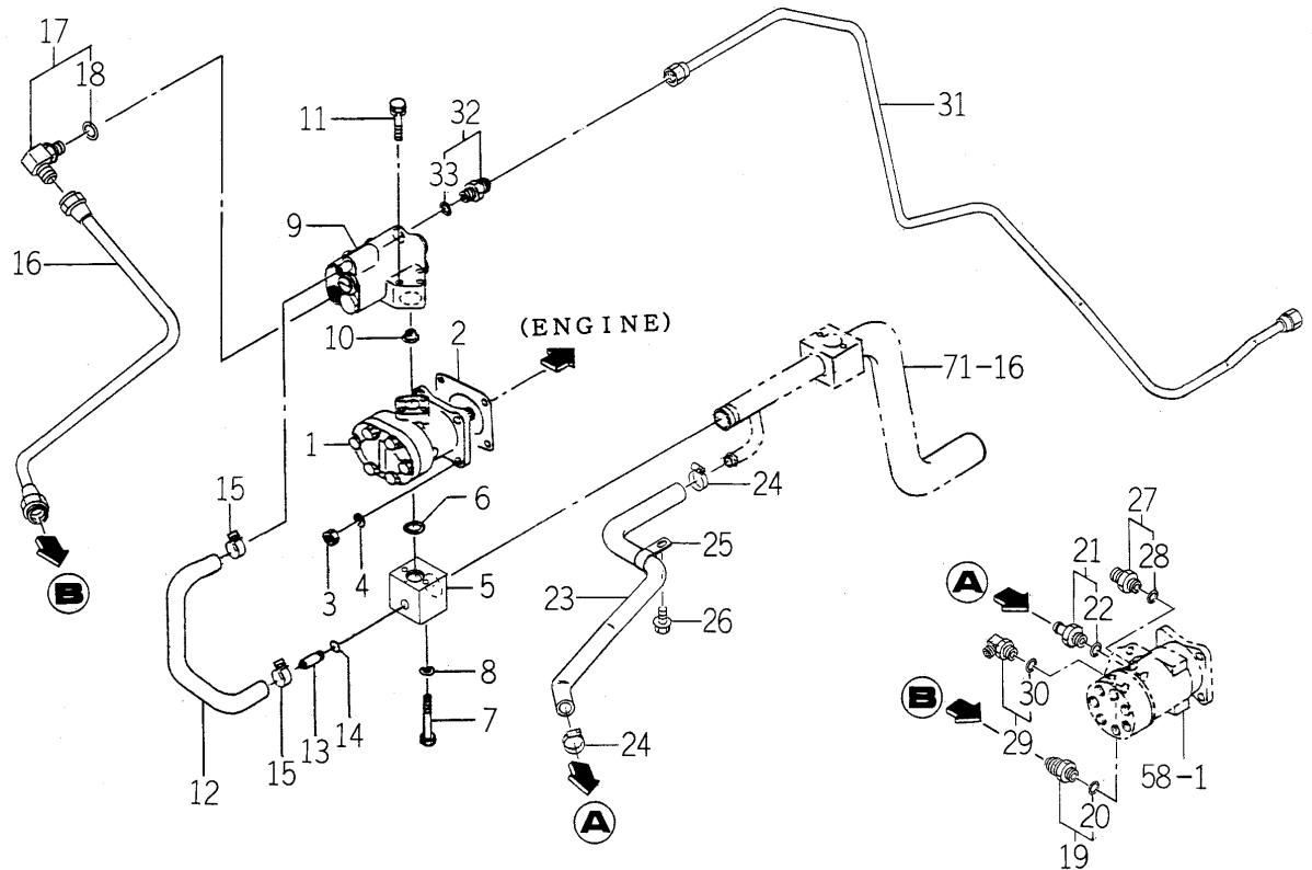
FIG. 75 HYD. SYSTEM (SUB) (P TYPE)(1/2)
