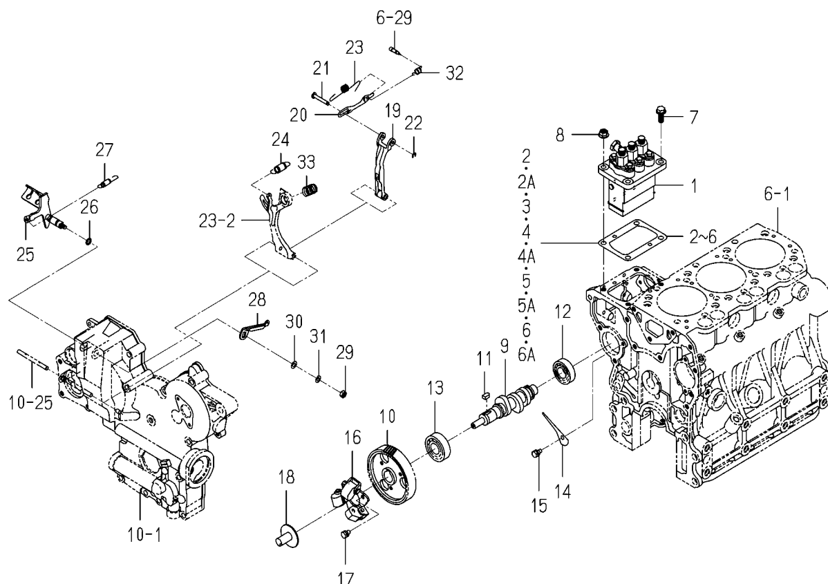
FIG. 21 INJECTION PUMP
