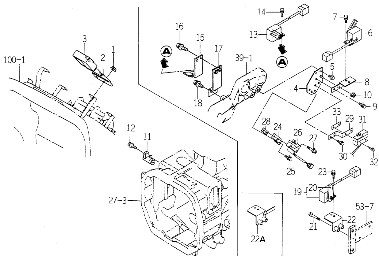
FIG.126 CONTROL SYSTEM (HE4 TYPE)
