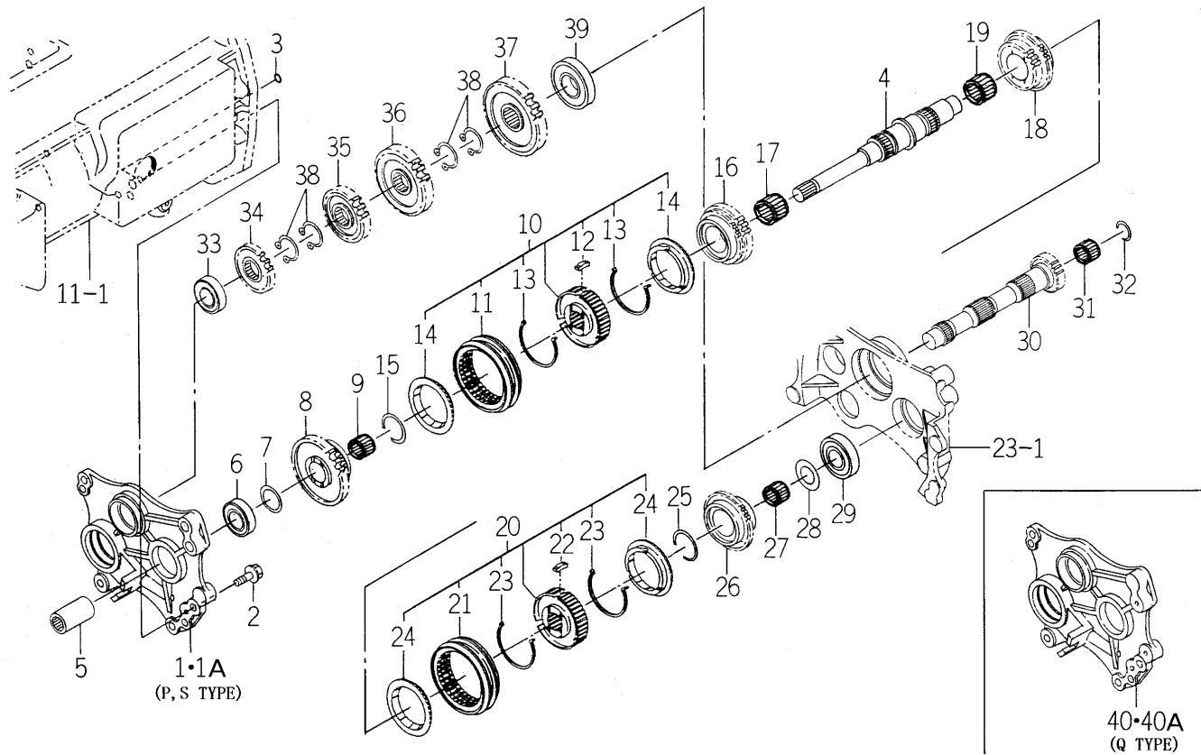
FIG. 21 GEAR (MAIN) SYSTEM (EXCEPT H TYPE)
