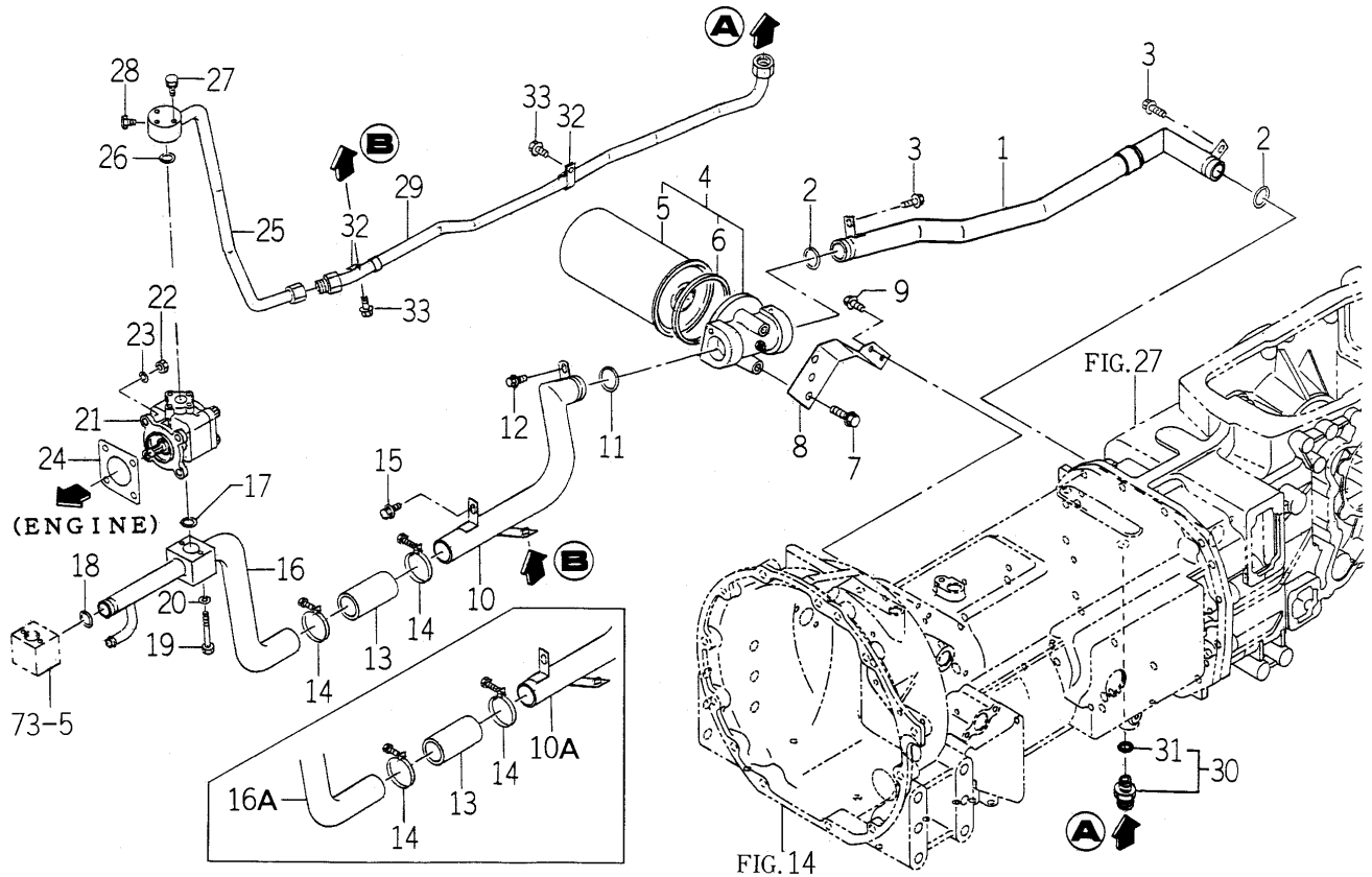
FIG. 69 HYD. SYSTEM (MAIN) (S TYPE)(1/2)
