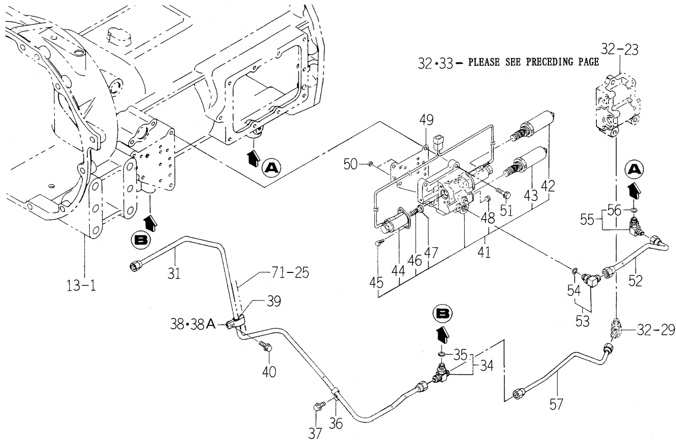
FIG. 76 HYD. SYSTEM (SUB) (Q TYPE)(2/2)
