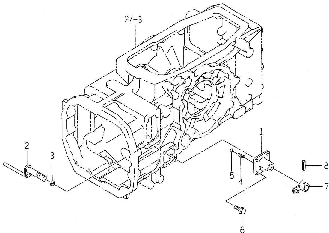
FIG. 34 ARM (SHIFT/4WD) SYSTEM
