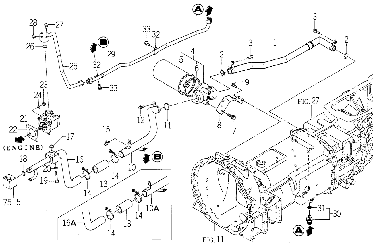
FIG. 71 HYD. SYSTEM (MAIN) (P,Q TYPE)(1/2)
