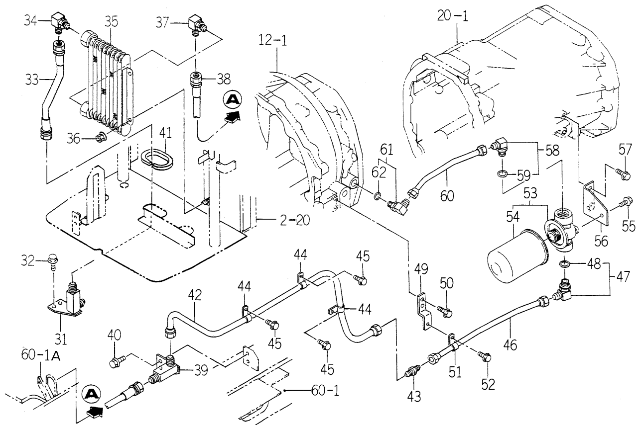
FIG. 74 HYD. SYSTEM (SUB) (H TYPE)(2/2)
