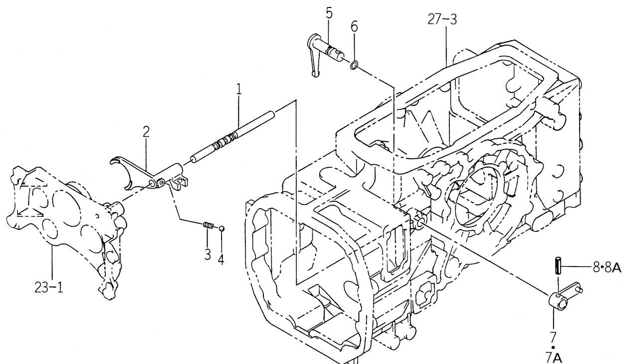
FIG. 33 FORK (SHIFT/SUB) SYSTEM
