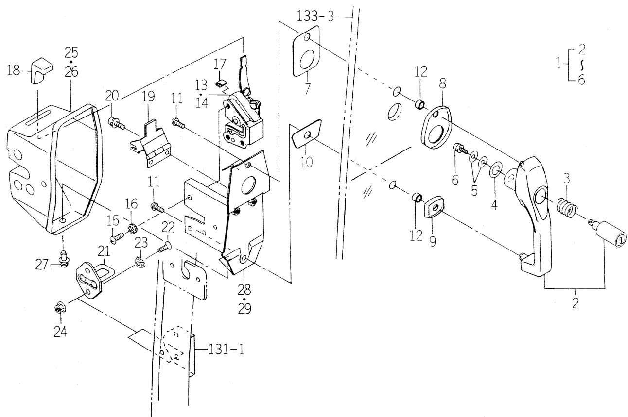
FIG.134 LOCK (DOOR) SYSTEM (C TYPE)
