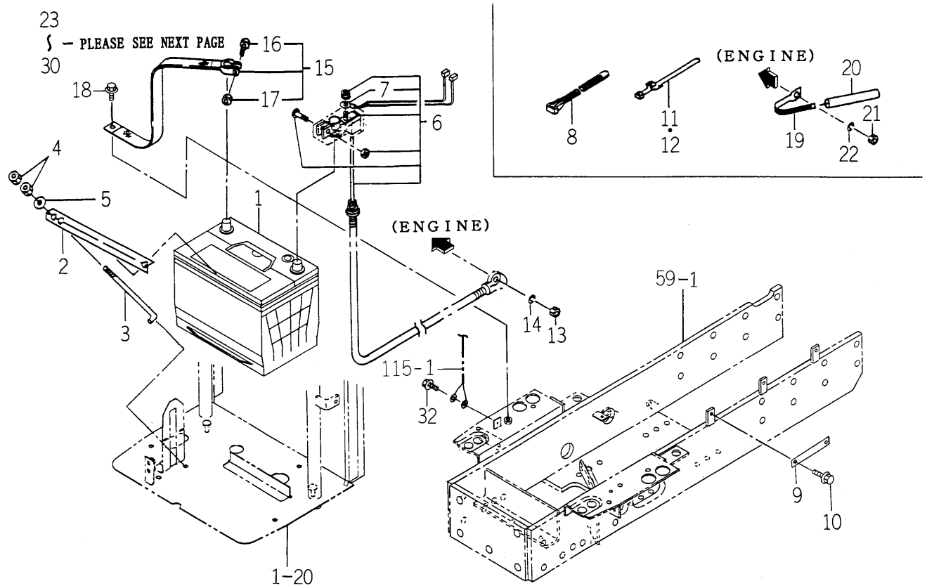
FIG.112 ELC. SYSTEM (FRONT) (HE4, QE4 TYPE)(1/2)
