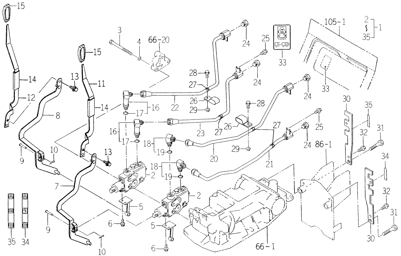
FIG.155 VALVE (REMOTE/2R) SET (C TYPE) (OPTION)
