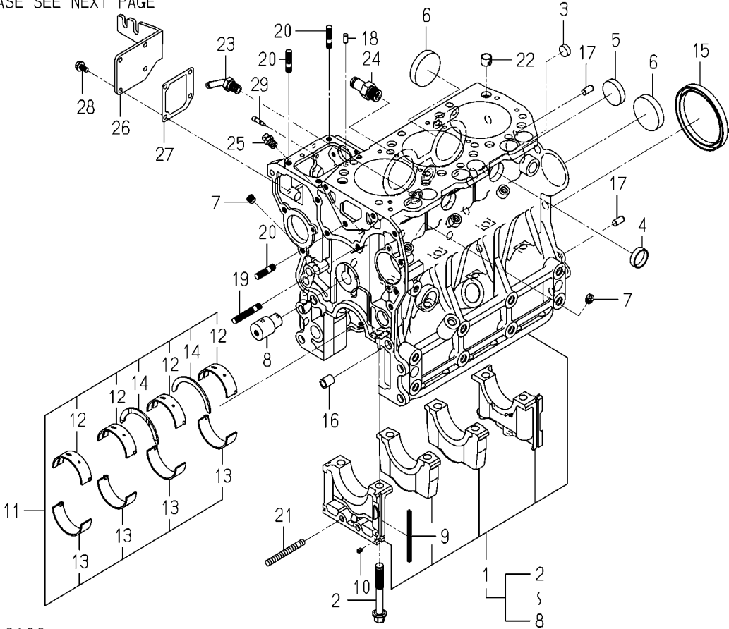
FIG. 6 CYLINDER BLOCK(1/2)
