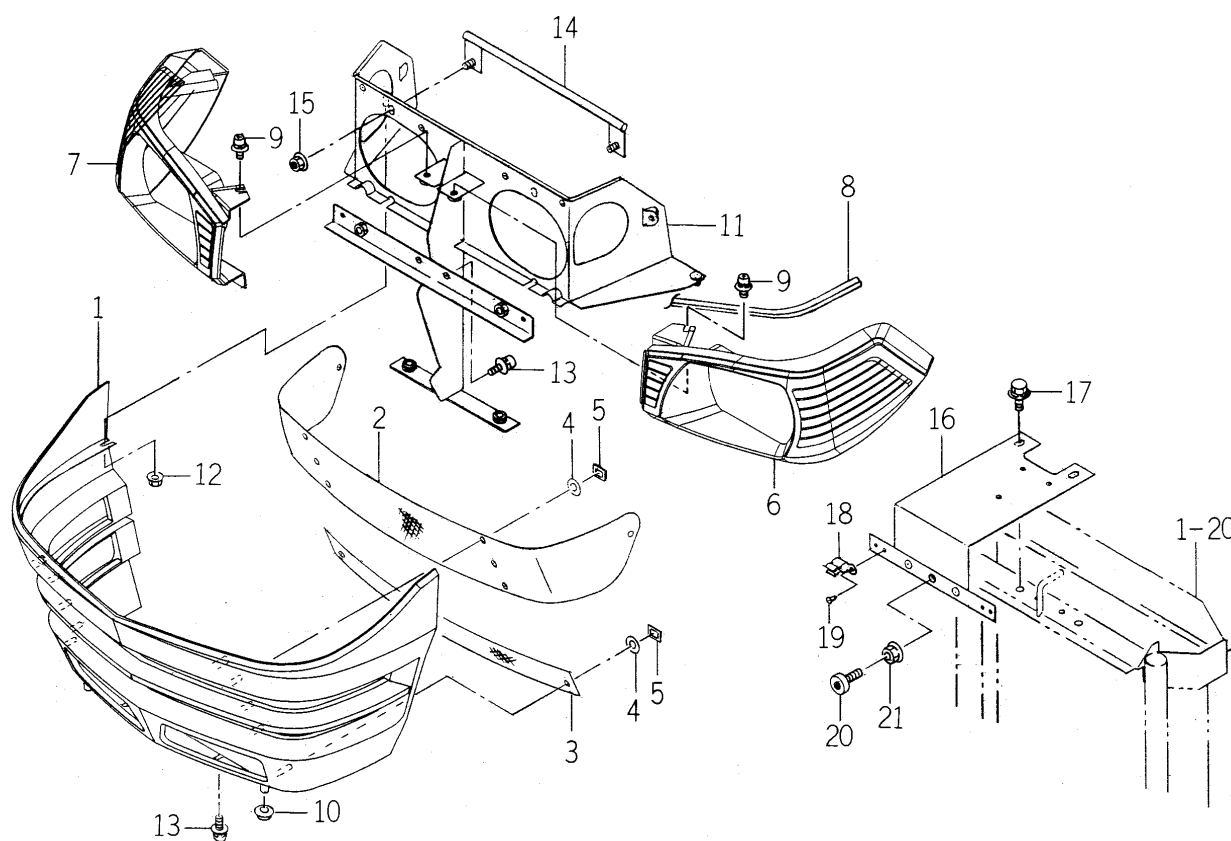
FIG. 91 GRILLE SYSTEM
