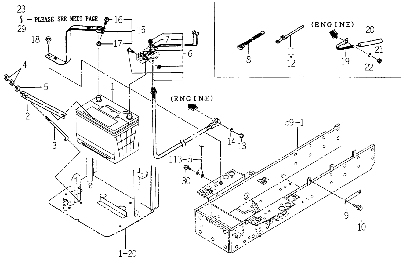
FIG.111 ELC. SYSTEM (FRONT) (E6 TYPE)(1/2)
