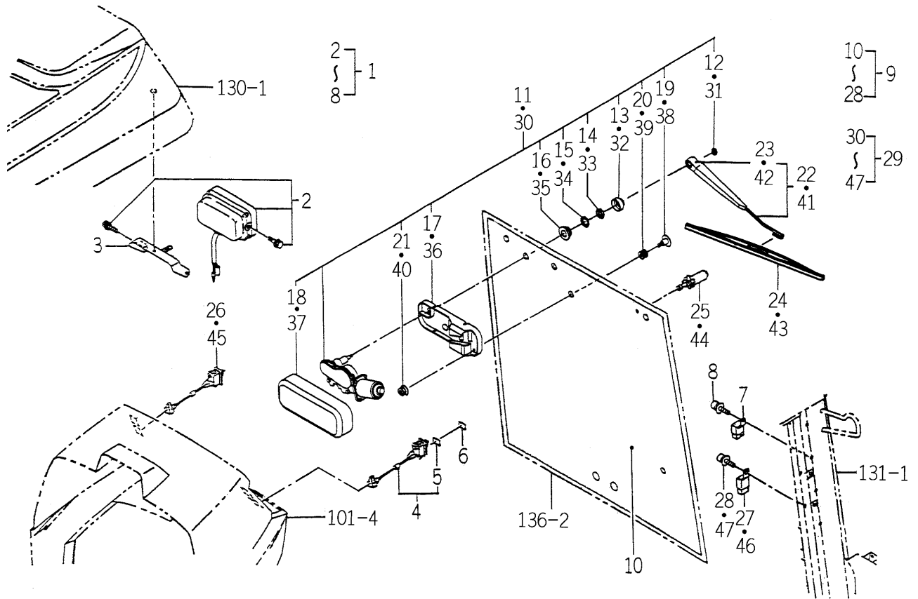
FIG.156 ELC. SYSTEM (C TYPE) (OPTION)
