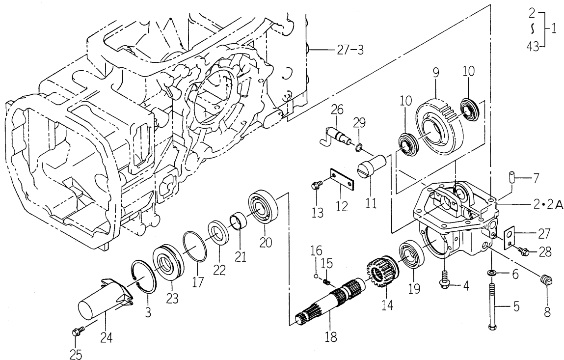
FIG. 28 MID PTO SET (M TYPE-STANDARD/(1/2) EXCEPT Q,M TYPE-OPTION)
