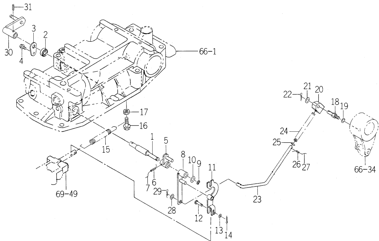
FIG. 67 MECHANICAL LINK(1/2) (POSITION) SYSTEM
