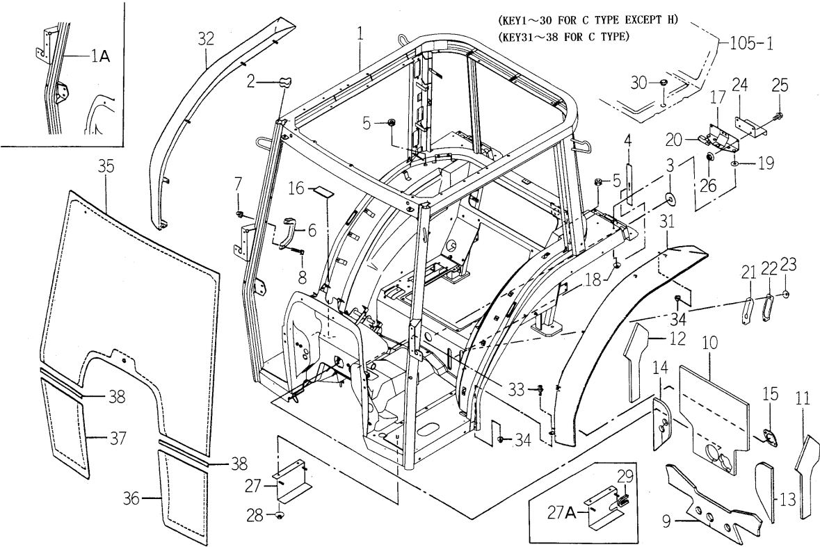
FIG.131 FRAME (C TYPE EXCEPT H), FENDER (OVER/C TYPE), GLASS (FRONT/C TYPE) SYSTEM
