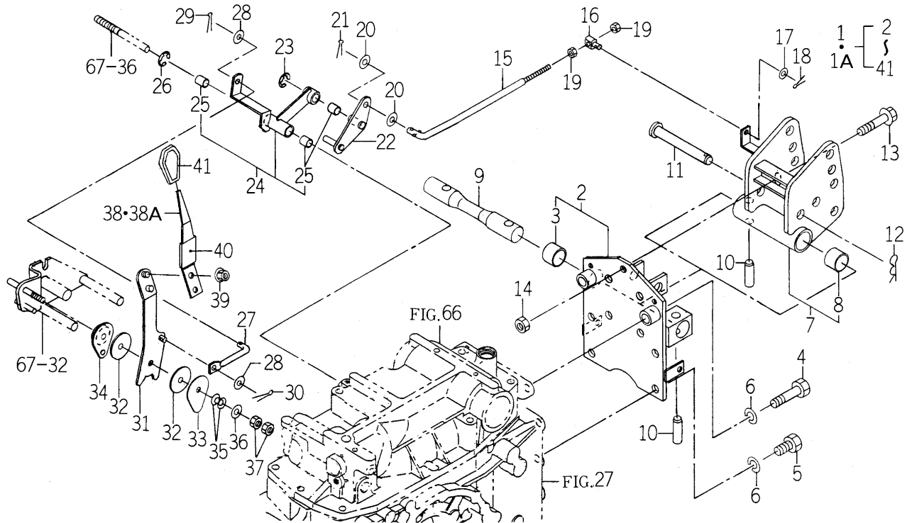
FIG. 68 MECHANICAL LINK (DRAFT) SYSTEM (S TYPE-STANDARD/EXCEPT S TYPE-OPTION)
