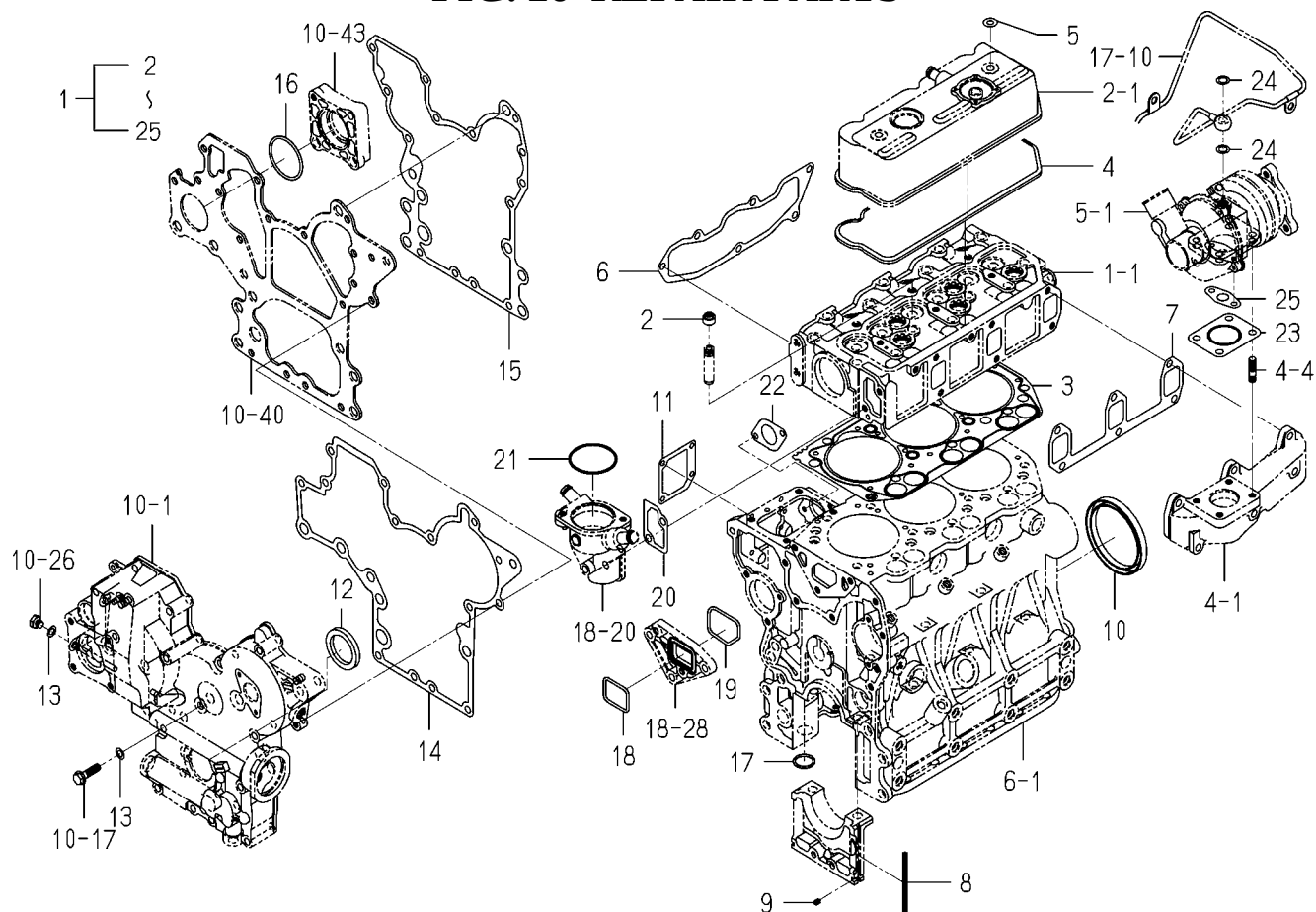
FIG. 26 REPAIR PARTS
