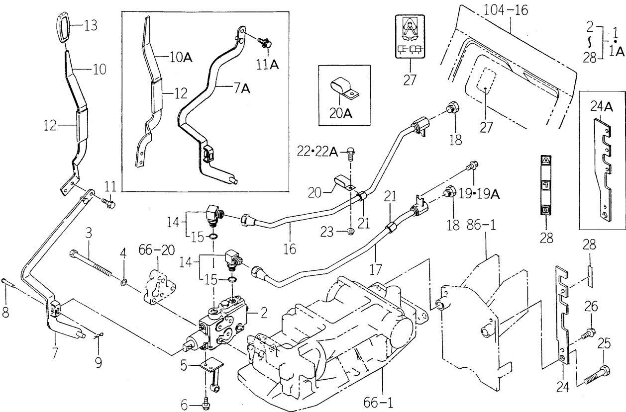
FIG.152 VALVE (REMOTE/1R) SET (E4 TYPE EXCEPT C) (OPTION)
