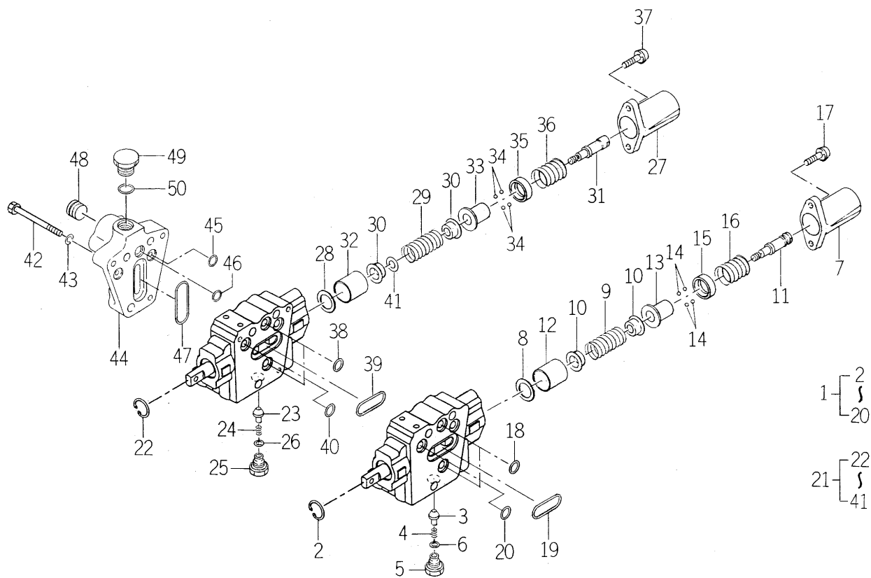
FIG.162 COMPONENT PARTS FOR K211-074-000-00 ON Fig.77
