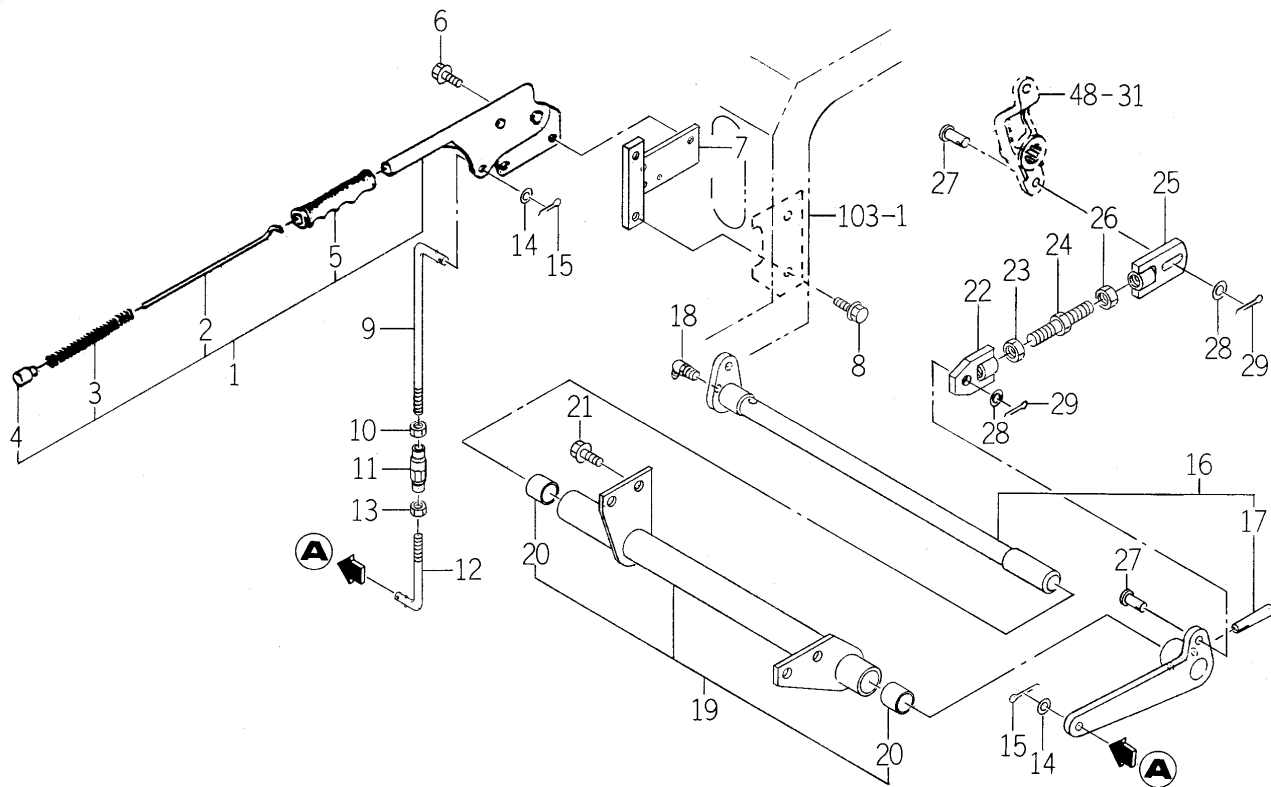
FIG. 53 BRAKE (PARKING) SYSTEM (E4 TYPE)
