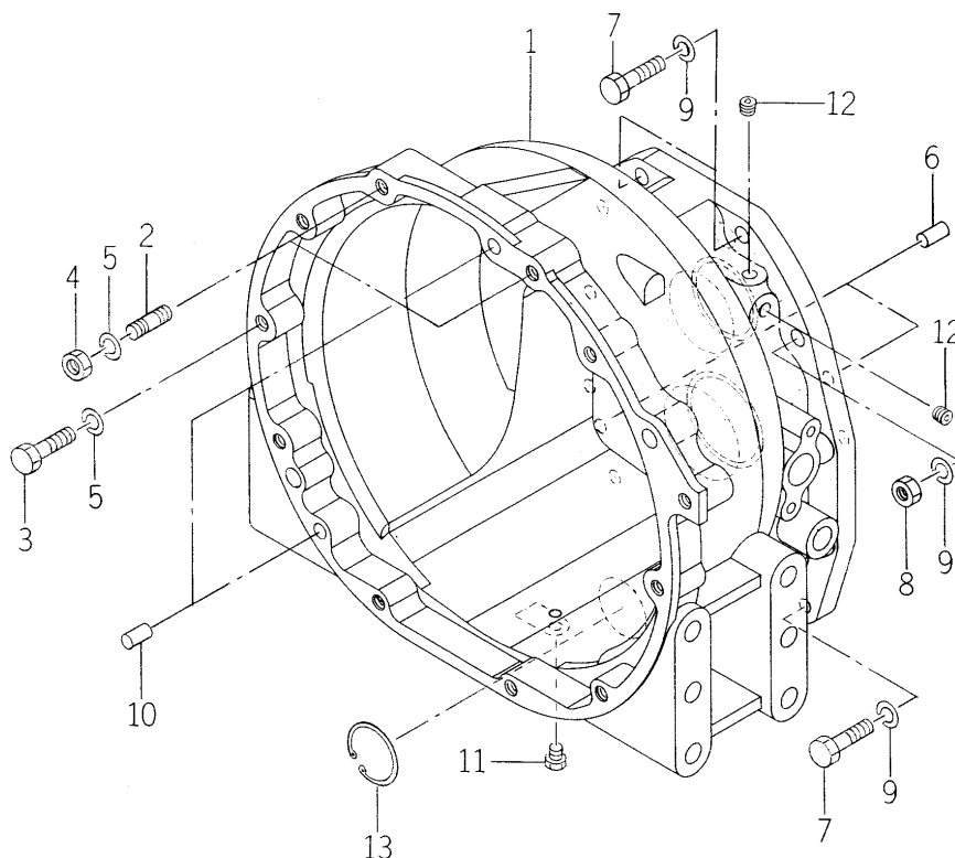
FIG. 12 CASE (TRANSMISSION/FRONT) SYSTEM (H TYPE)
