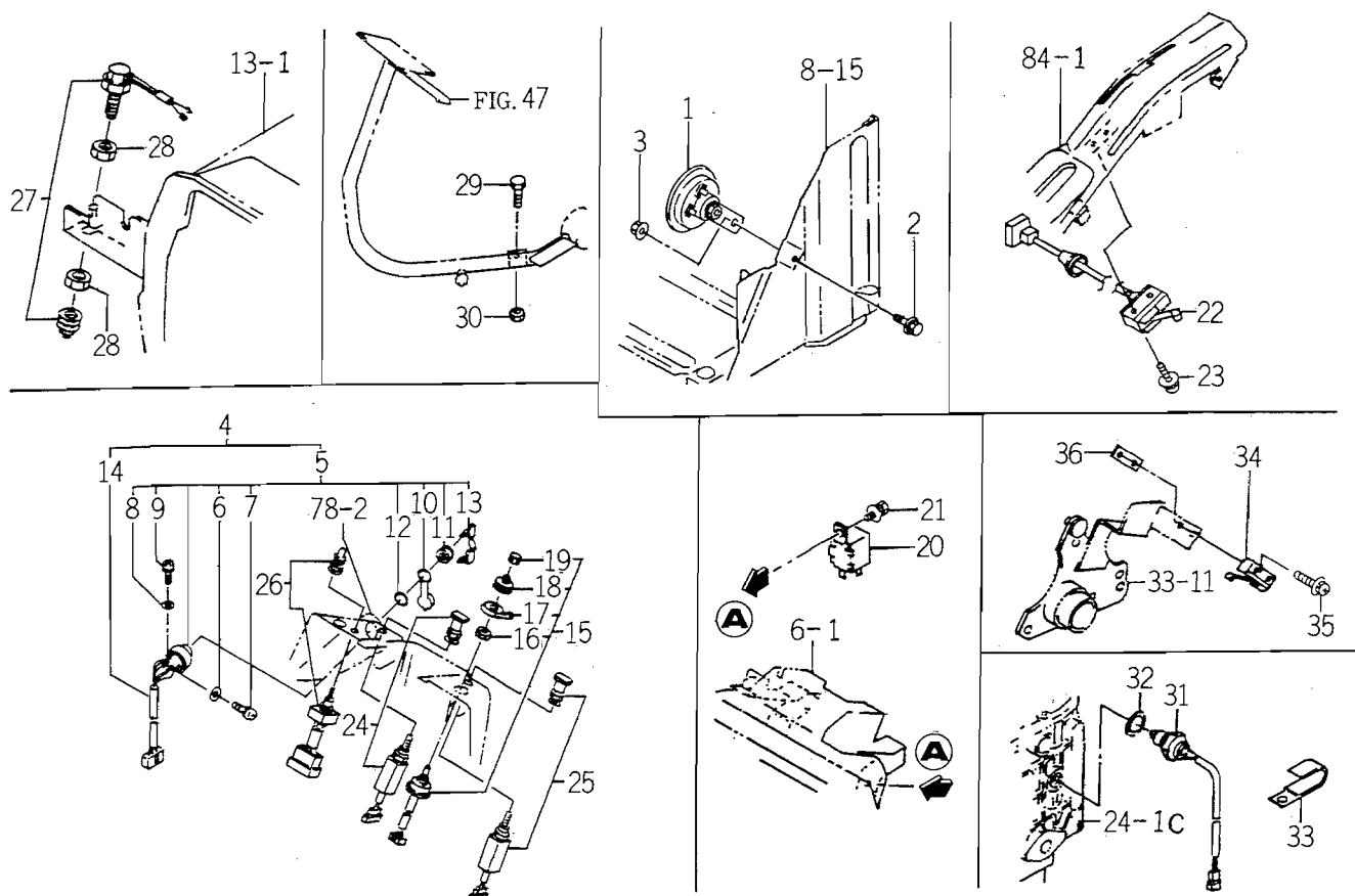
FIG. 97 SWITCH SYSTEM (TF330 – E4)
