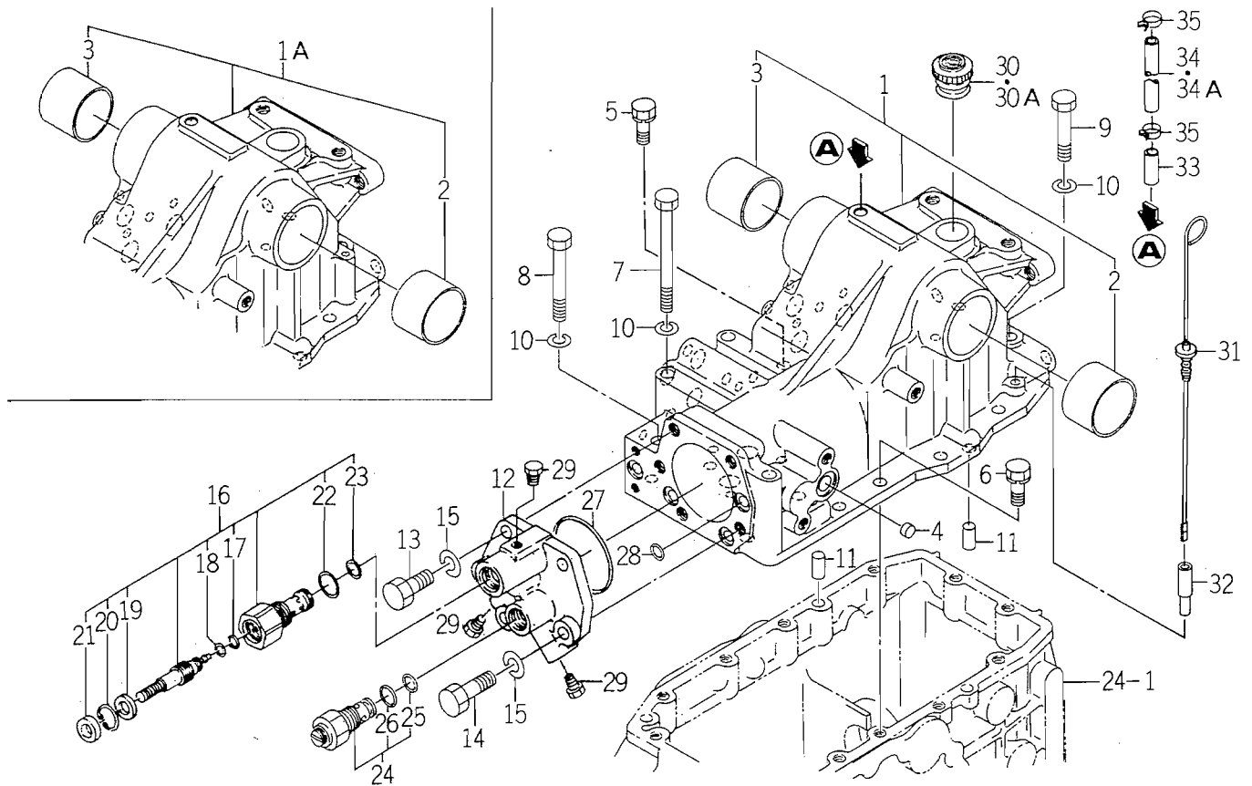
FIG. 64 CYLINDER CASE SYSTEM
