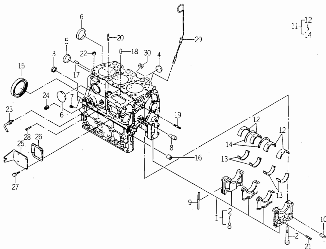
FIG. 5 CYLINDER BLOCK
