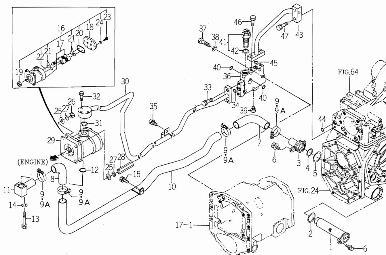
FIG. 72 PIPING SYSTEM
