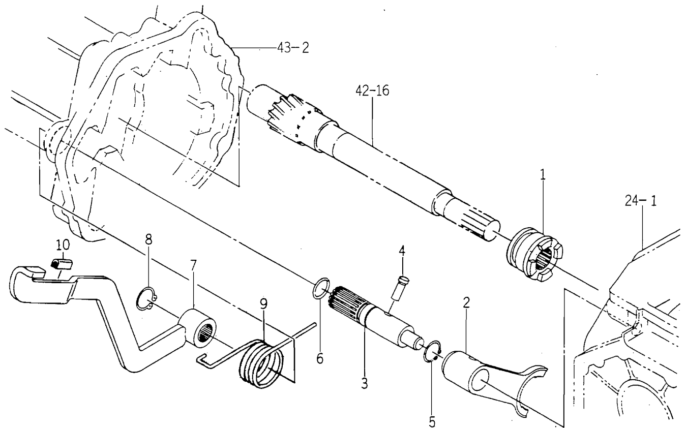
FIG. 45 DIFF LOCK SYSTEM
