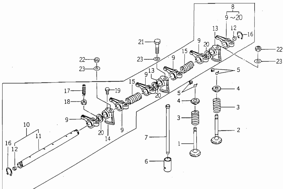
FIG. 11 VALVE
