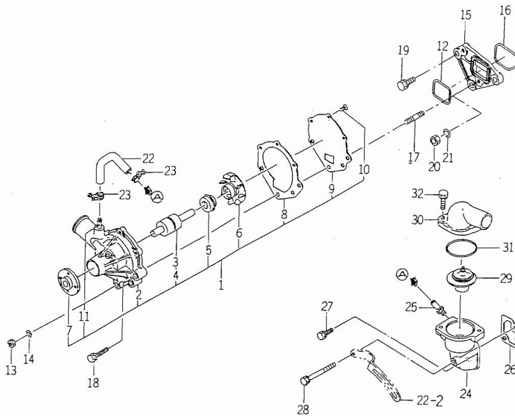
FIG. 17 WATER PUMP
