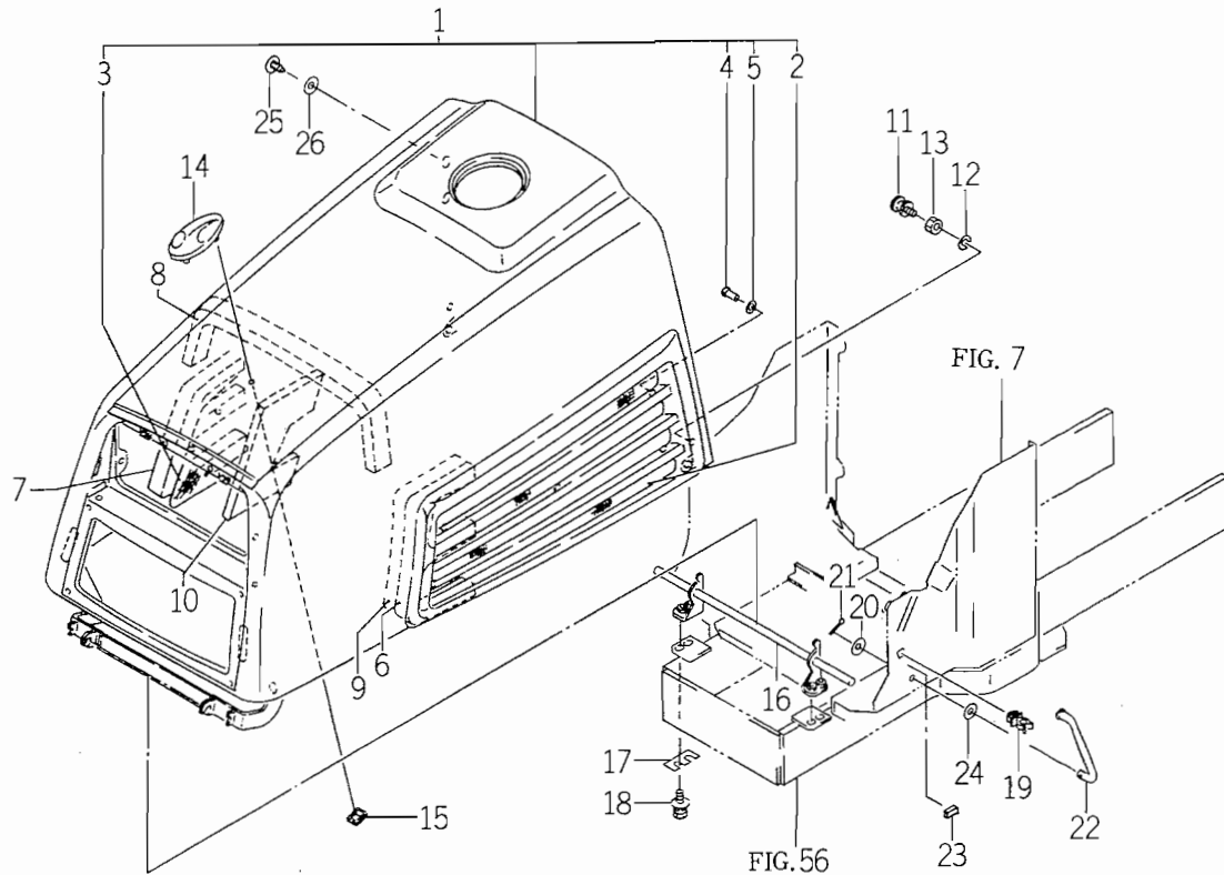
FIG. 76 HOOD SYSTEM
