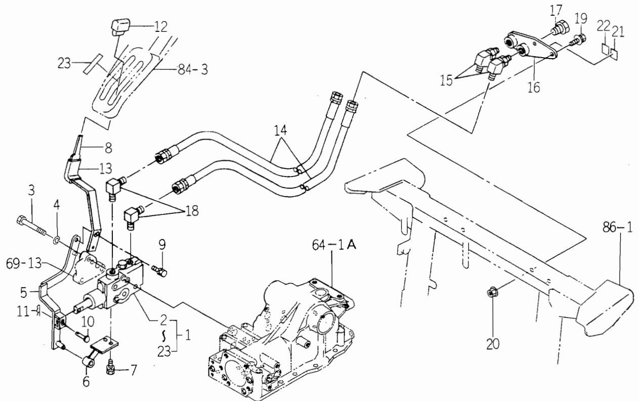
FIG. 70 VALVE (STACK/R1) SET (OPTION)
