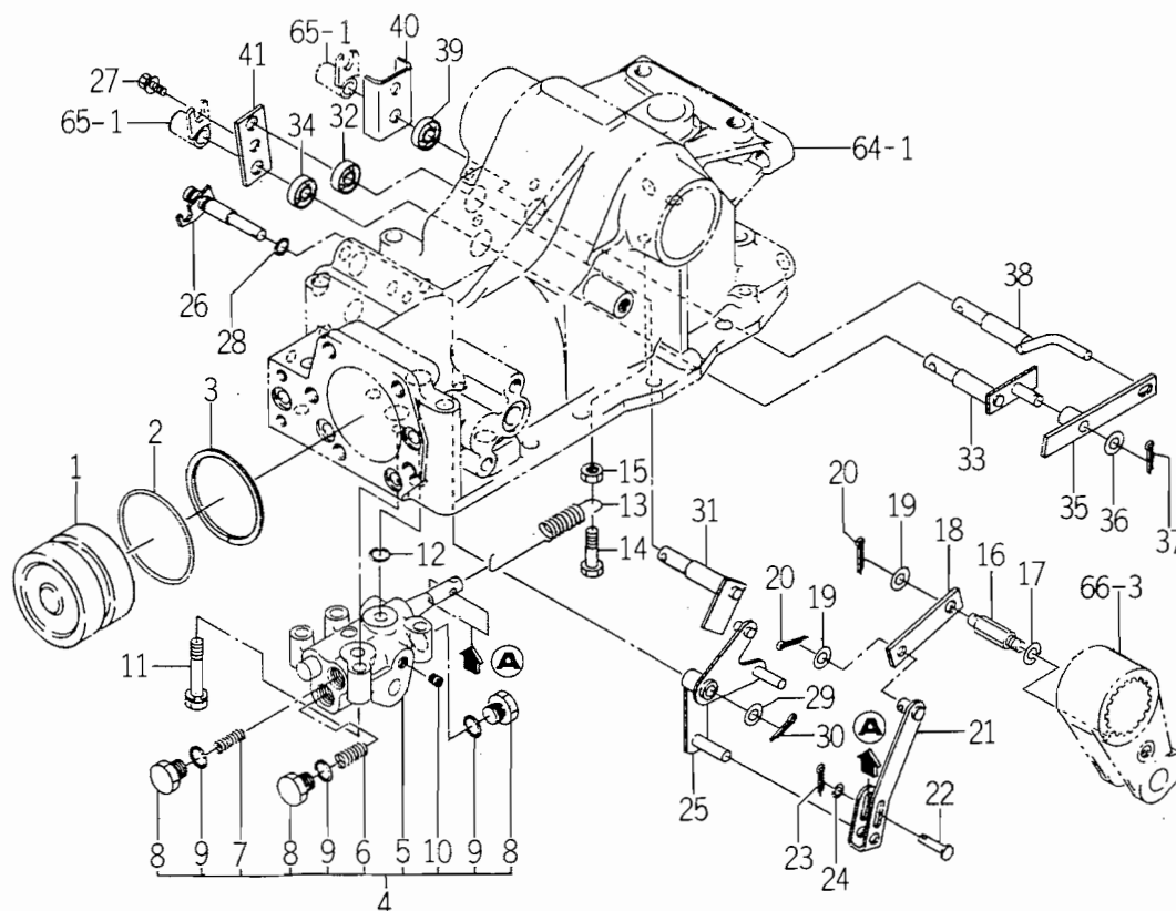
FIG. 67 CYLINDER SYSTEM
