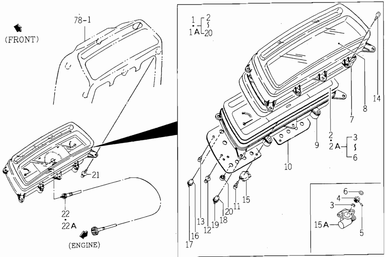
FIG. 95 PANEL SYSTEM
