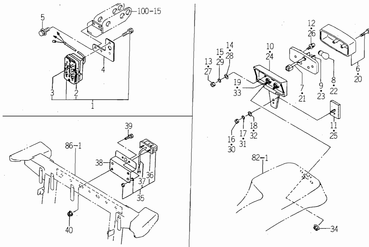
FIG. 94 LAMP SYSTEM (TF330 – E4)
