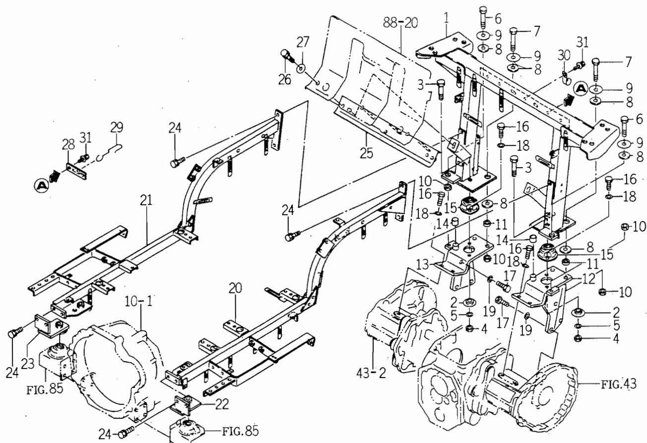
FIG. 86 MOUNT (REAR/H.S.T.) SYSTEM (TF330 - E4)
