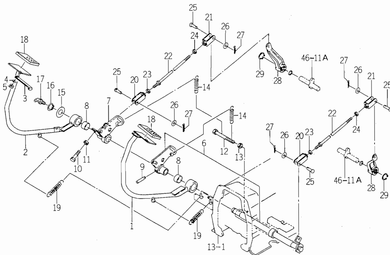
FIG. 47 PEDAL (BRAKE) SYSTEM (TF330 – E4)
