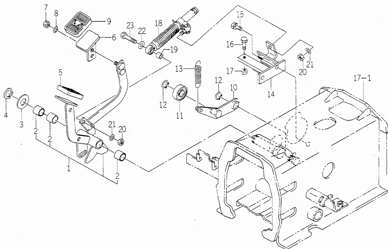
FIG. 48 PEDAL (HST) SYSTEM (MU TYPE)
