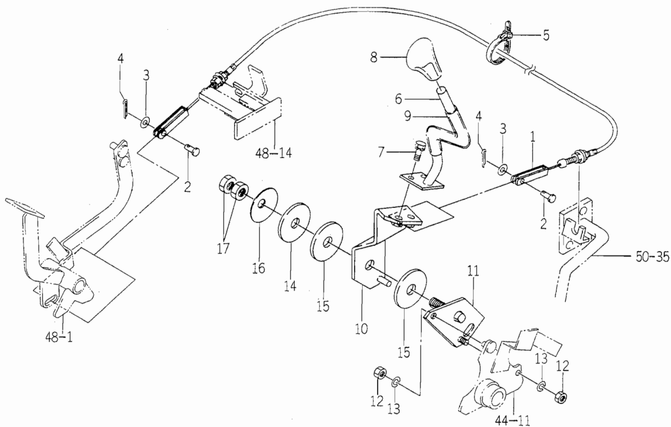
FIG. 49 LEVER (HST) SYSTEM (MU TYPE)
