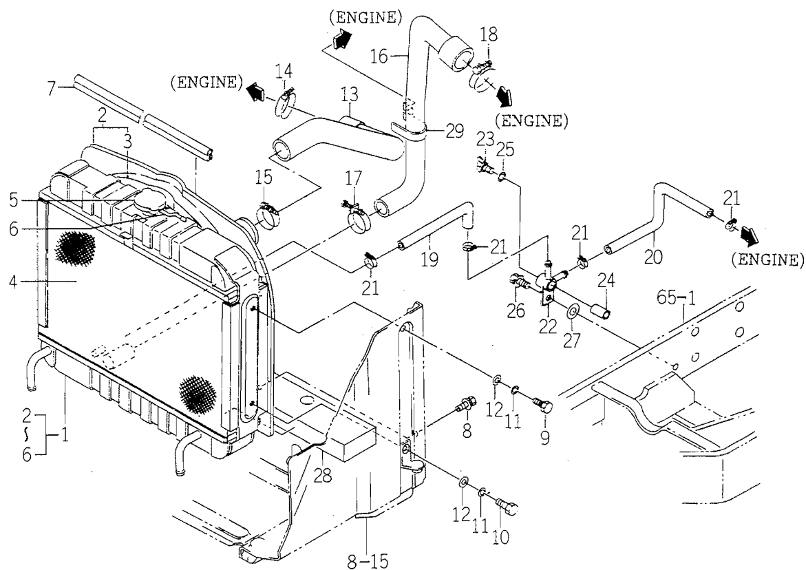
FIG. 2 RADIATOR (HST) SYSTEM (MU TYPE)
