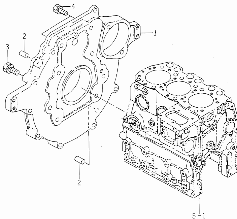
FIG. 8 REAR PLATE
