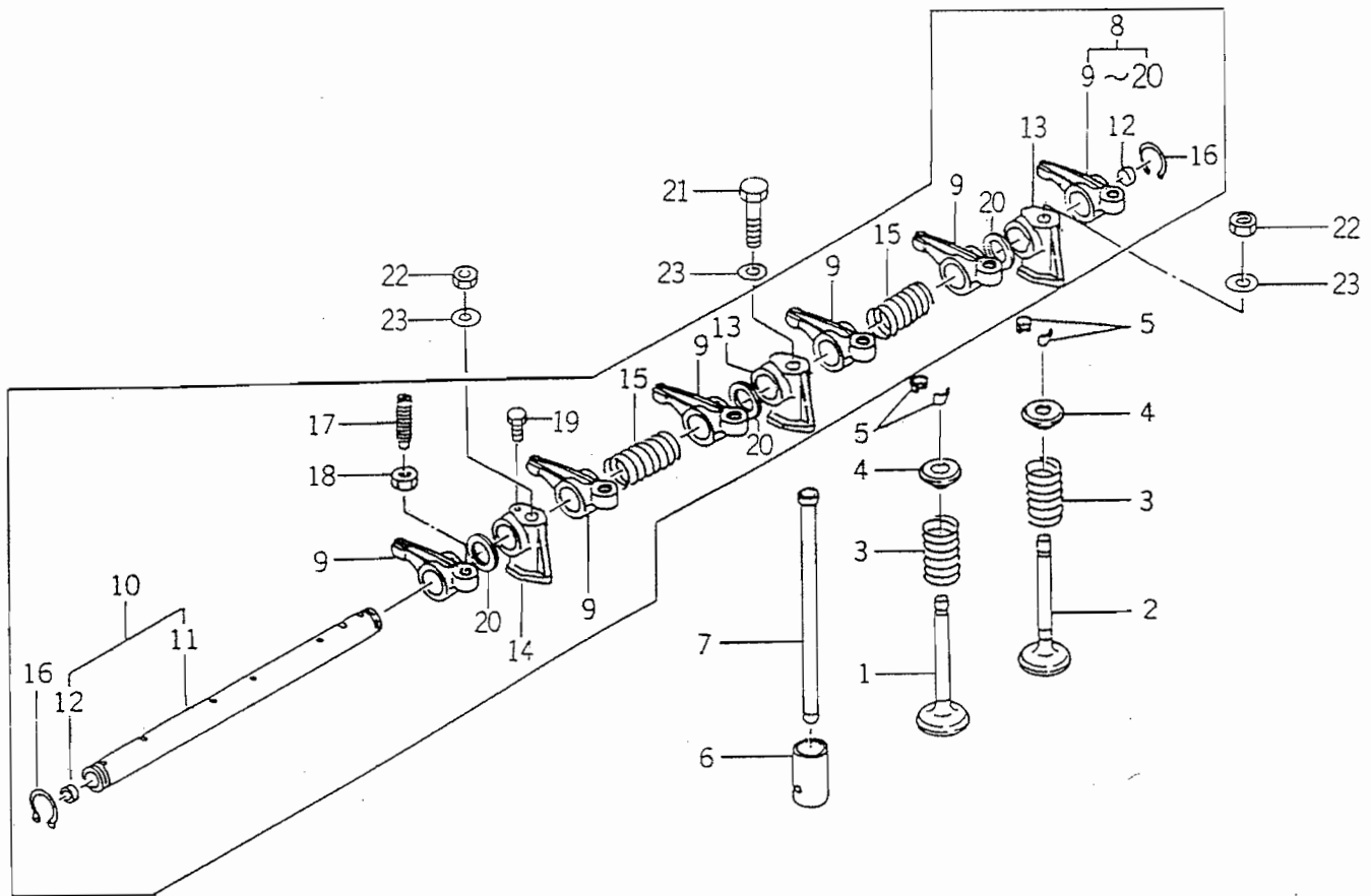
FIG. 11 VALVE
