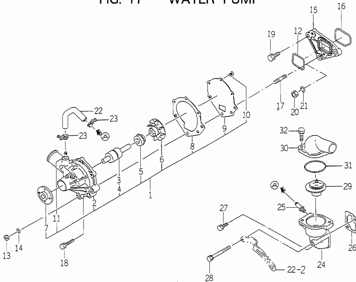
FIG. 17 WATER PUMP
