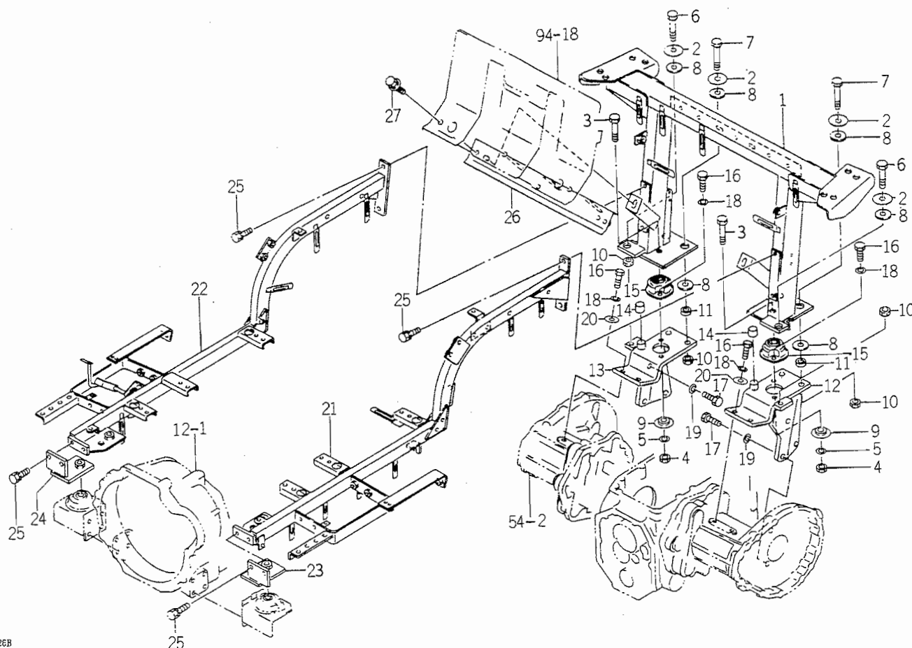
FIG. 92 MOUNT (REAR/E40) SYSTEM (MDU TYPE)
