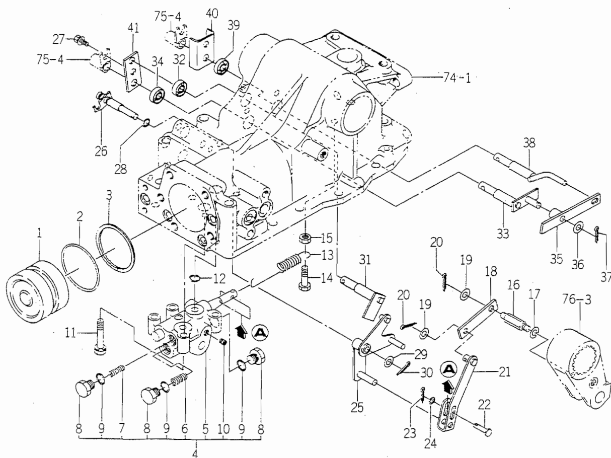
FIG. 77 CYLINDER SYSTEM
