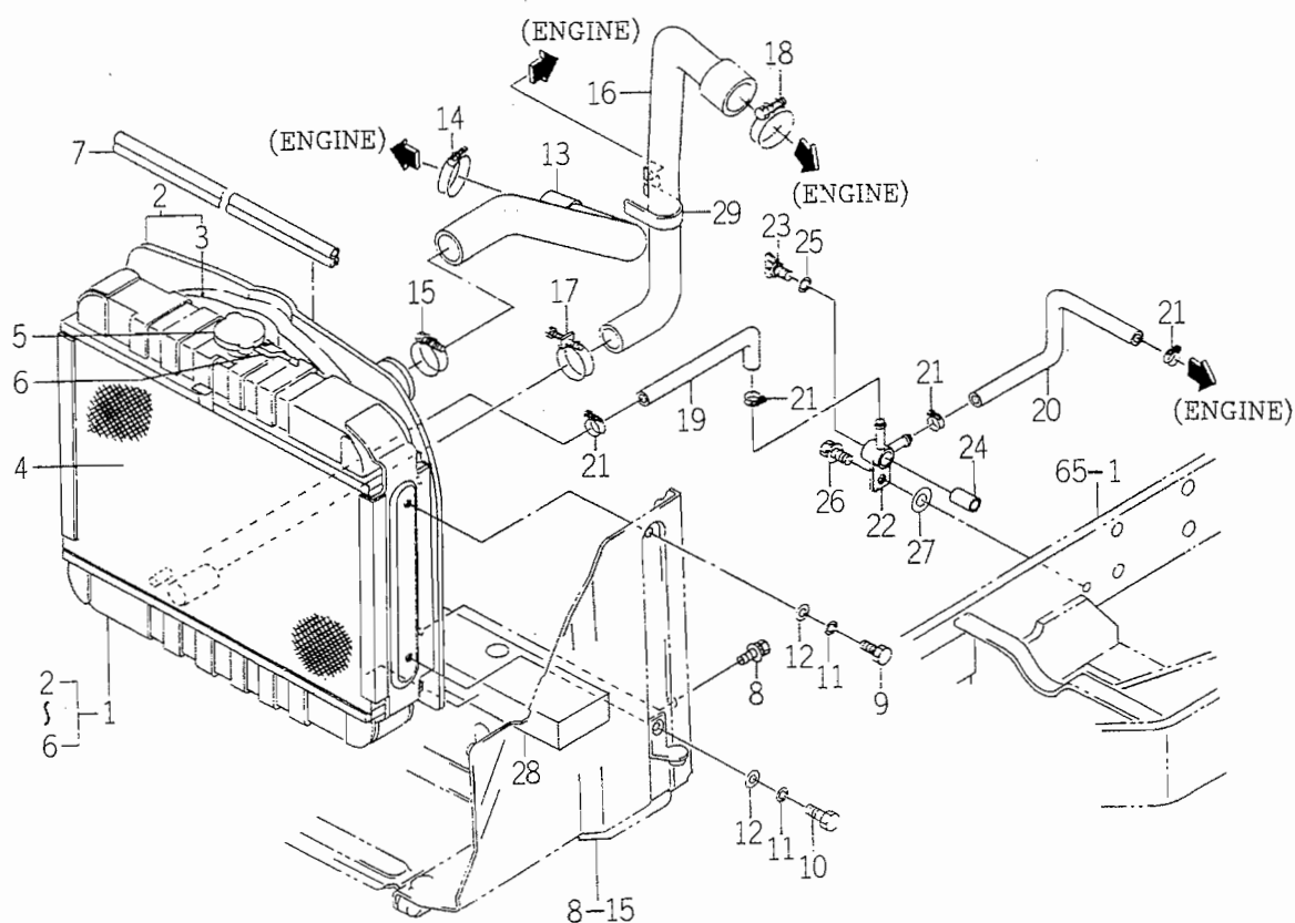
FIG. 1 RADIATOR SYSTEM (MDU TYPE)
