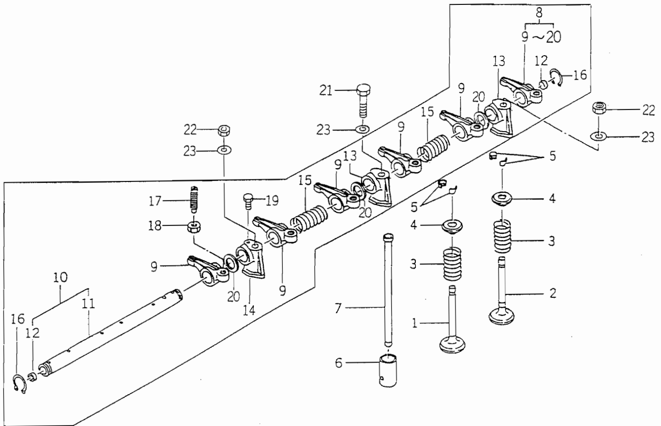
FIG. 11 VALVE
