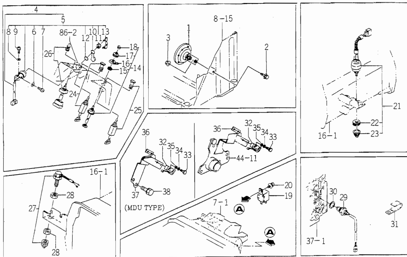
FIG.100 SWITCH SYSTEM
