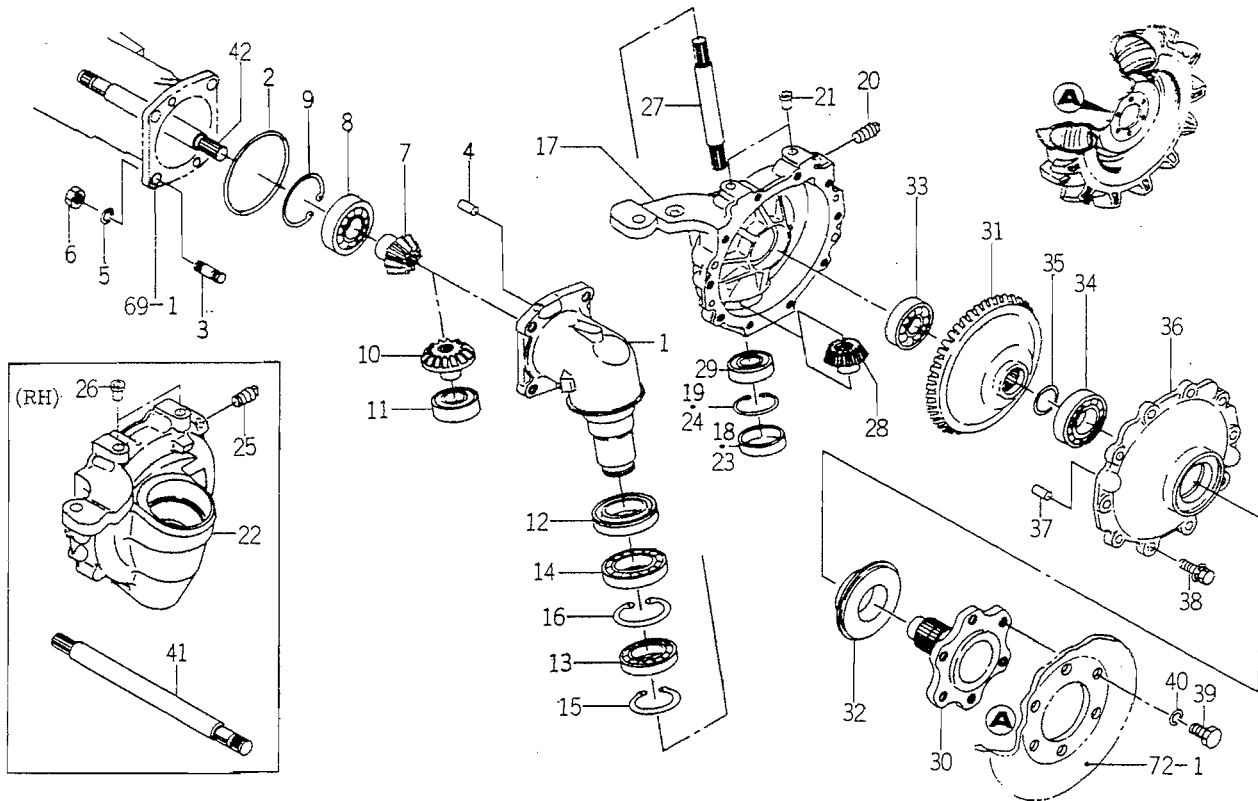
FIG. 70 FAINAL GEAR CASE SYSTEM
