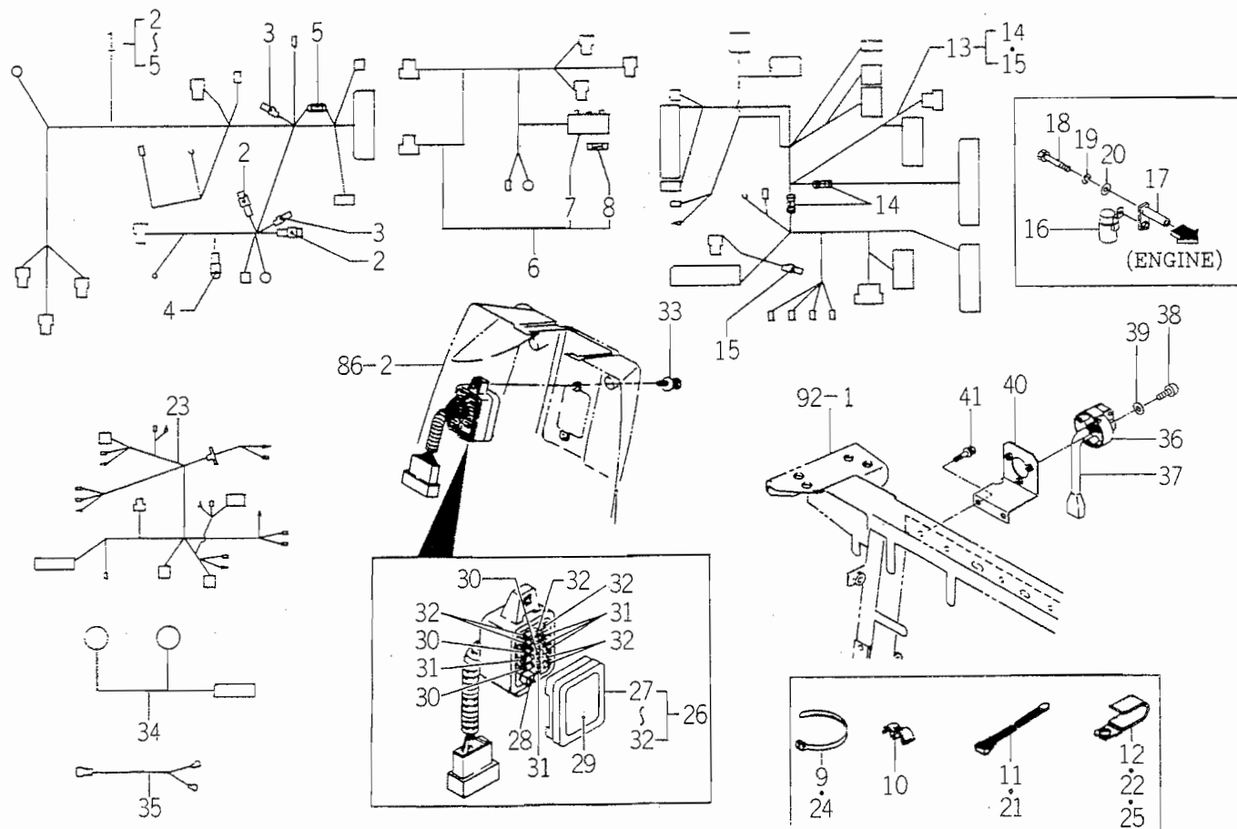
FIG.101 HARNESS SYSTEM
