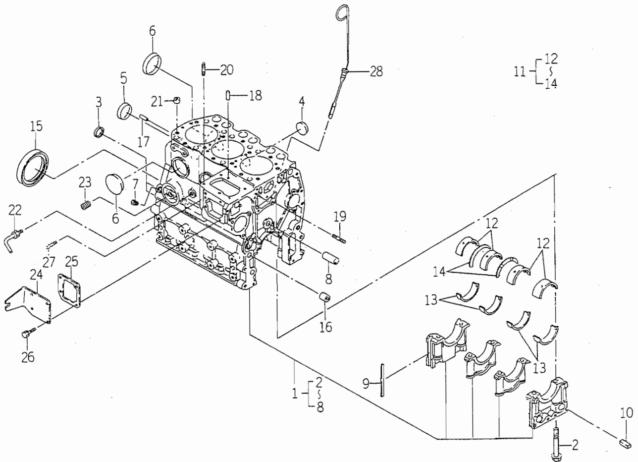
FIG. 5 CYLINDER BLOCK
