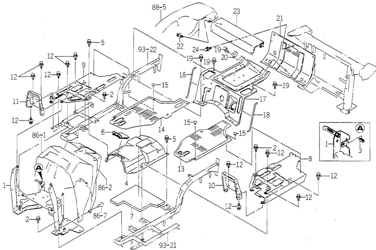
FIG. 95 FLOOR (HST) SYSTEM (MU TYPE)
