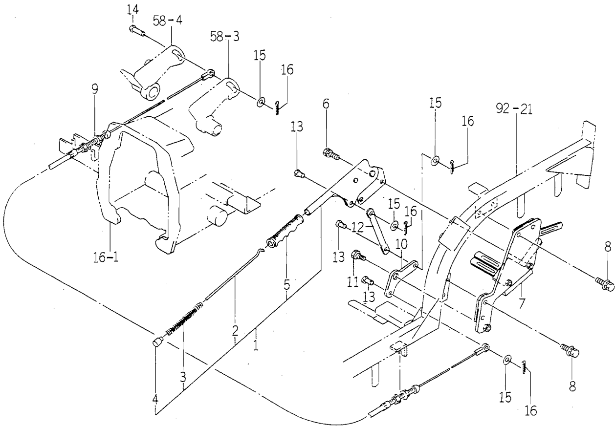
FIG. 59 BRAKE (PARKING) SYSTEM
