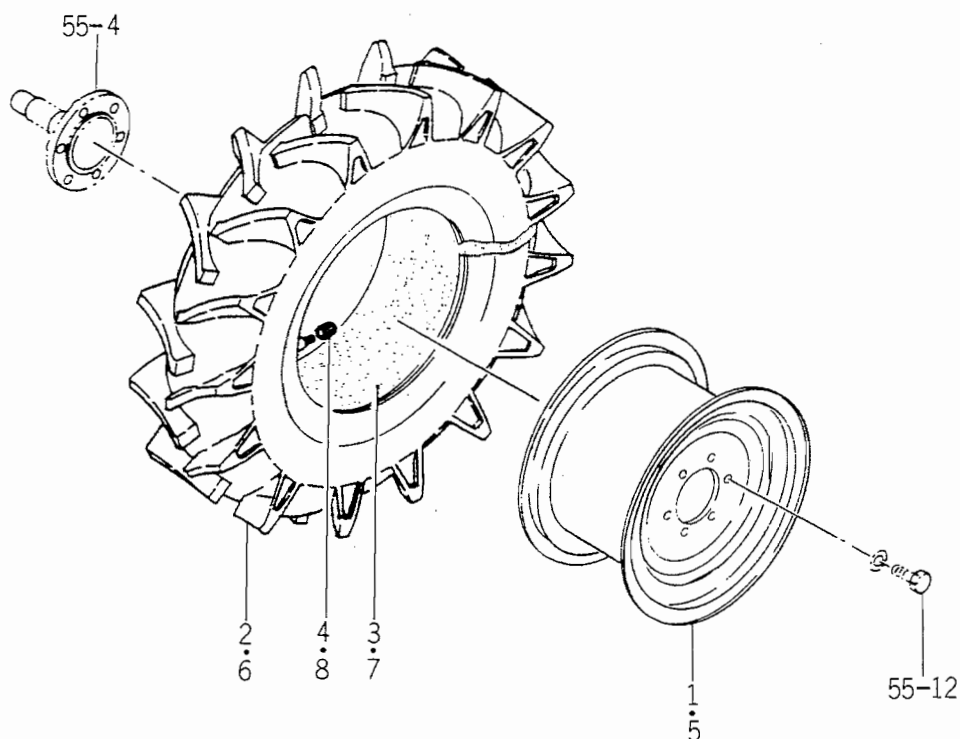
FIG. 60 REAR WHEEL SYSTEM (TF325/41 TYPE OPTION•42 TYPE STANDARD)
