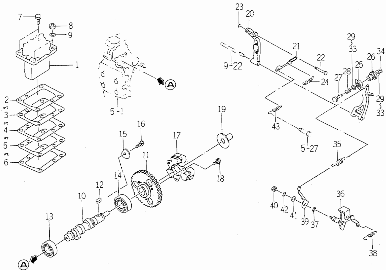
FIG. 20 INJECTION PUMP
