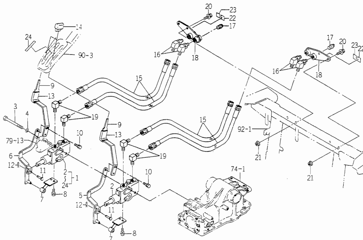
FIG. 81 VALVE (STACK/R2) SET (OPTION)
