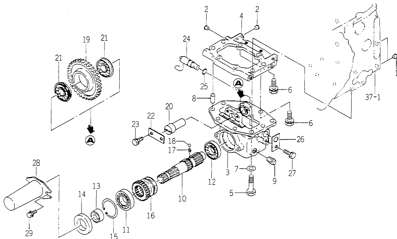
FIG. 41 PTO (MID) SYSTEM
