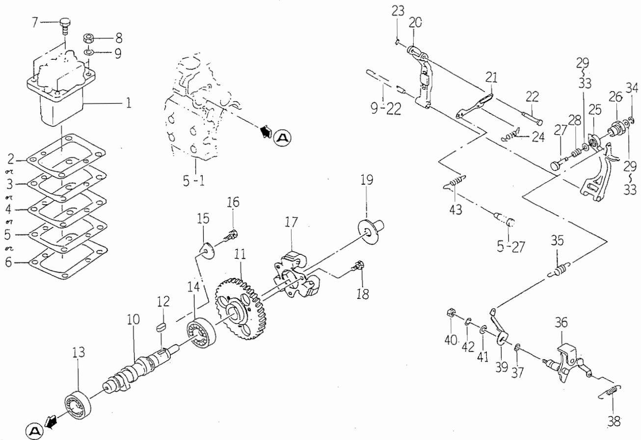
FIG. 20 INJECTION PUMP
