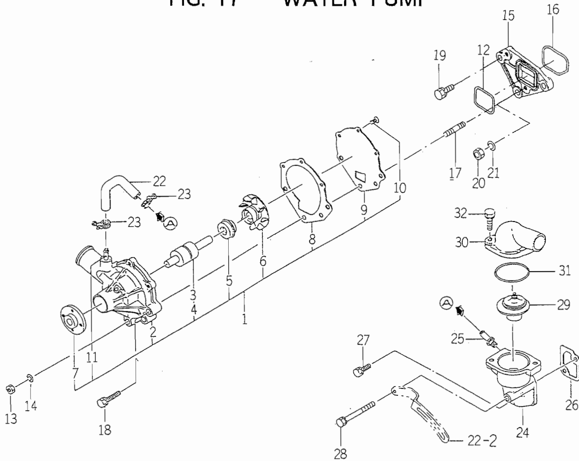
FIG. 17 WATER PUMP
