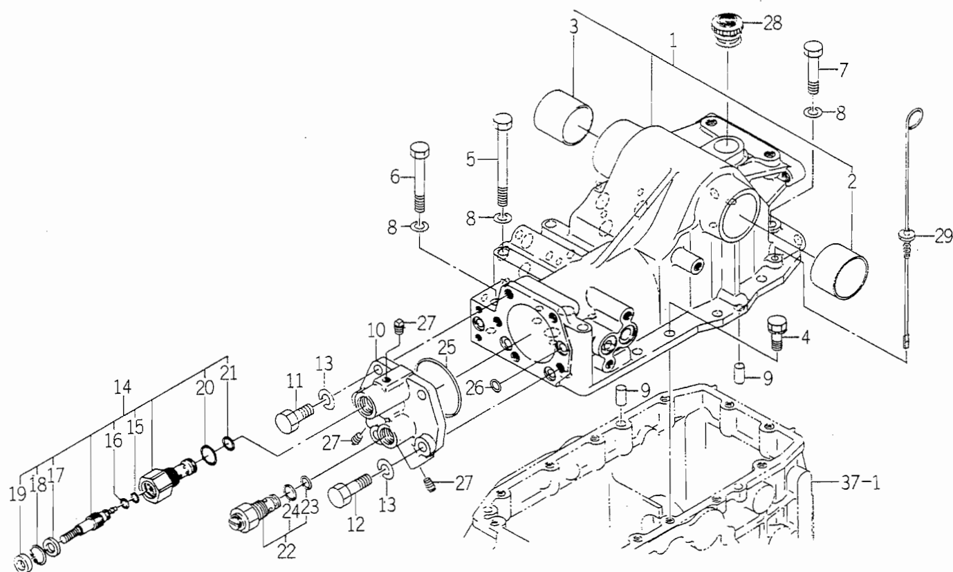
FIG. 74 CYLINDER CASE SYSTEM
