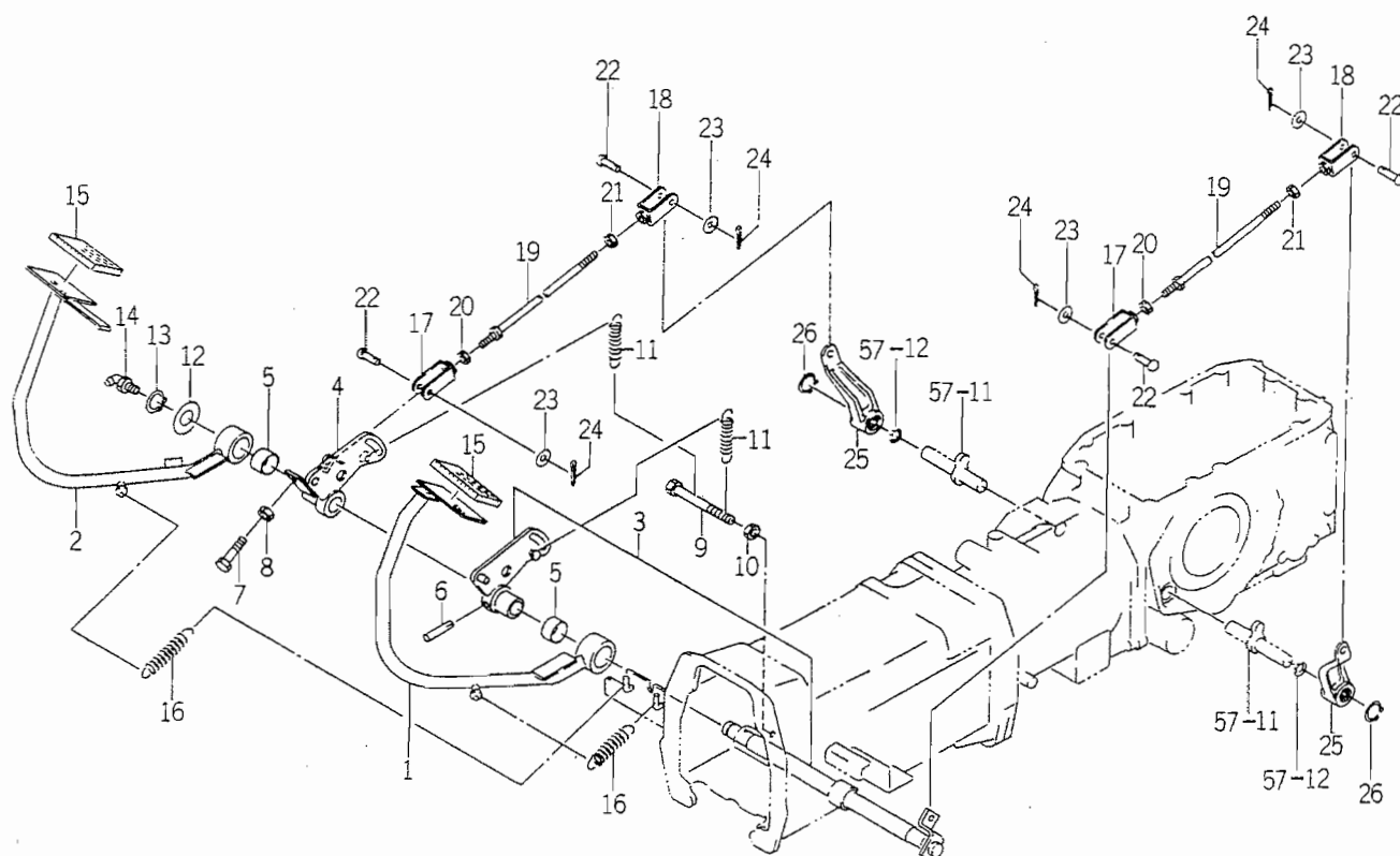
FIG. 58 PEDAL (BRAKE) SYSTEM
