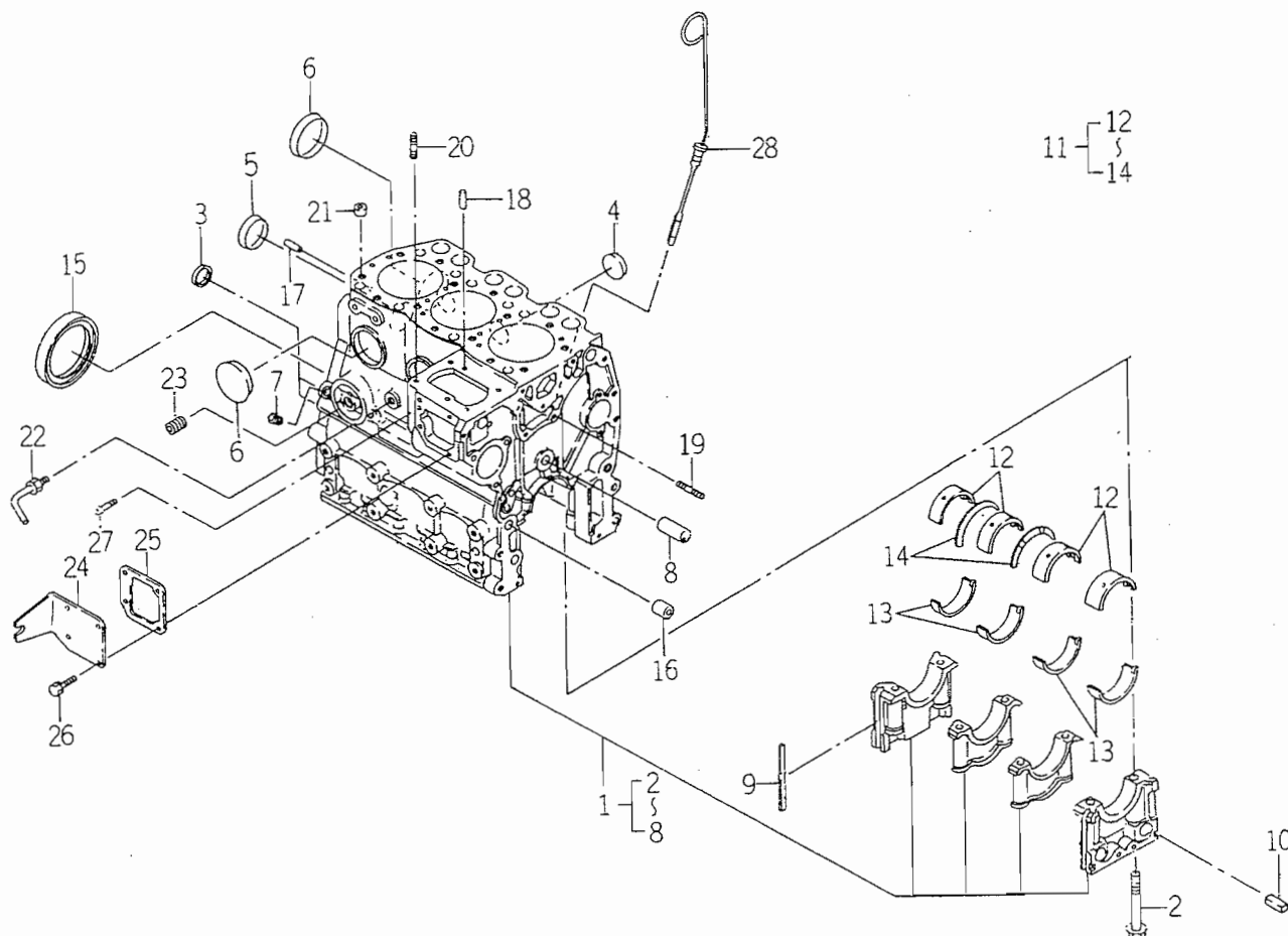
FIG. 5 CYLINDER BLOCK
