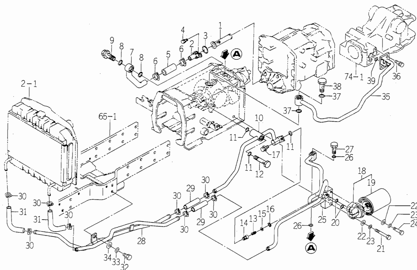
FIG. 50 PIPING (HST) SYSTEM (MU TYPE)
