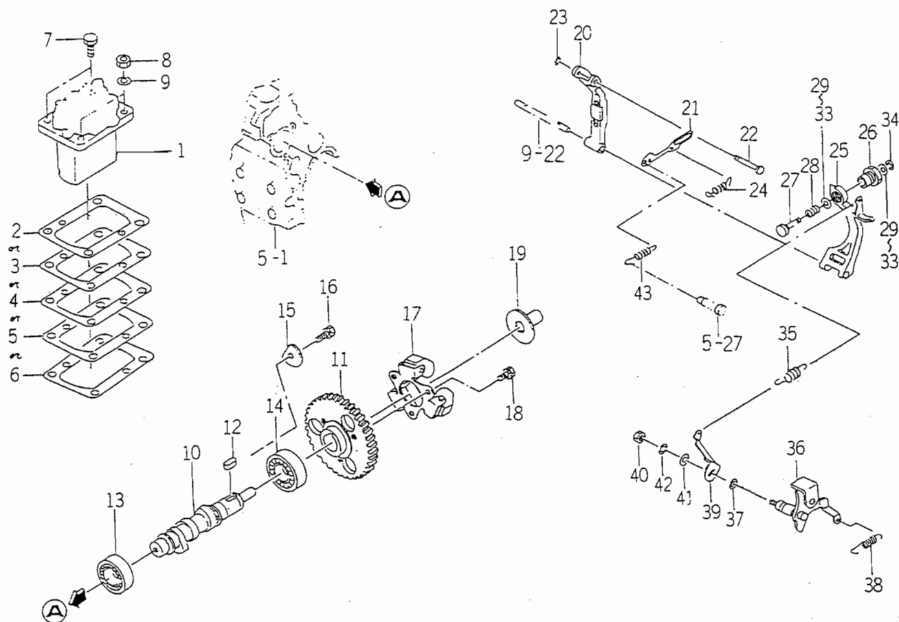
FIG. 20 INJECTION PUMP
