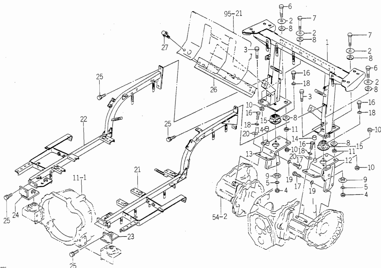
FIG. 93 MOUNT (REAR/HST/E40) SYSTEM (MU TYPE)
