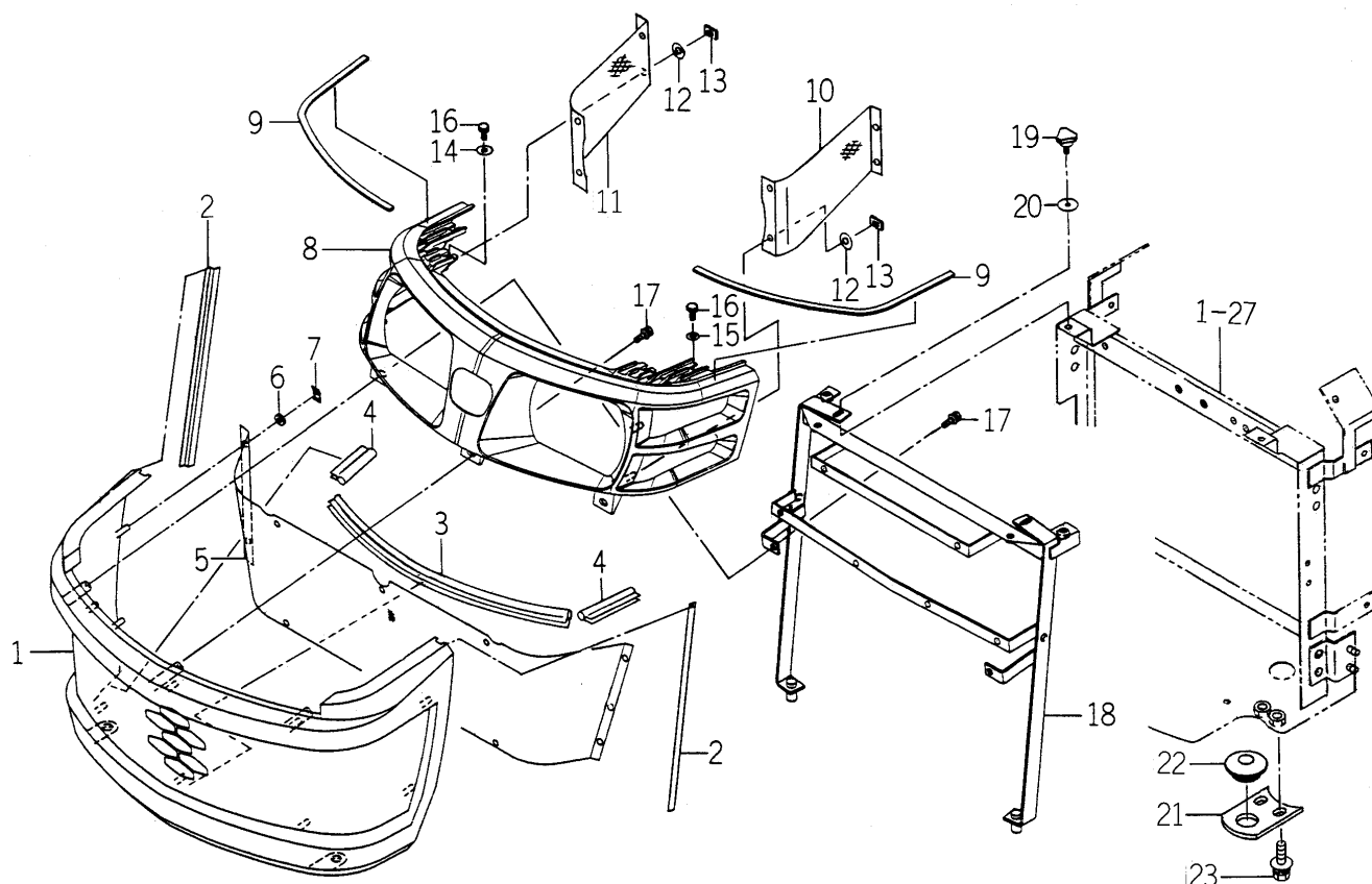
FIG. 73 GRILLE SYSTEM
