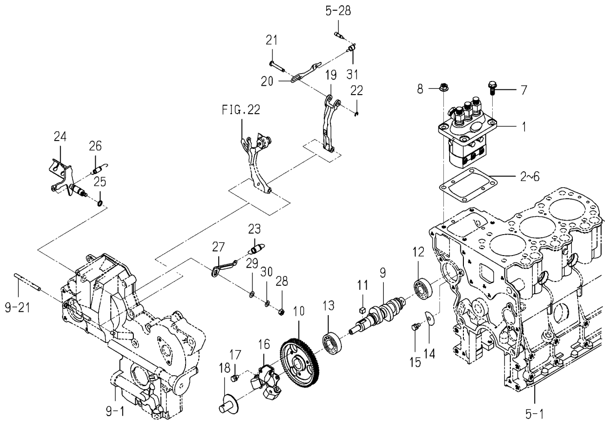
FIG. 20 INJECTION PUMP
