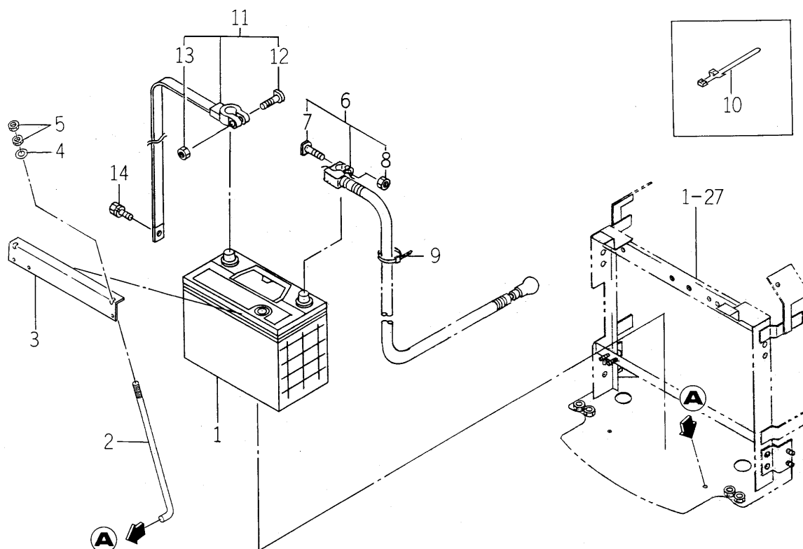
FIG. 7 BATTERY SYSTEM
