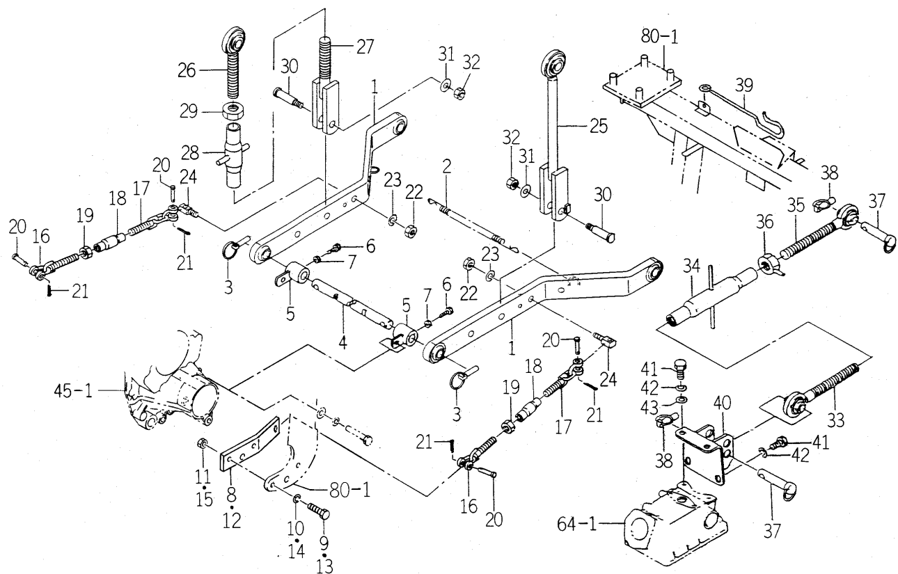
FIG. 70 LINK (3P) SYSTEM
