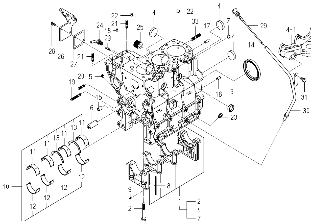
FIG. 5 CYLINDER BLOCK
