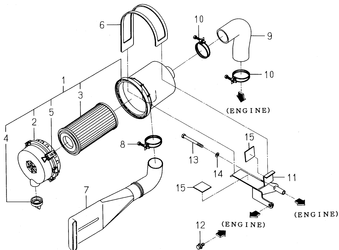
FIG. 4 AIR CLEANER SYSTEM
