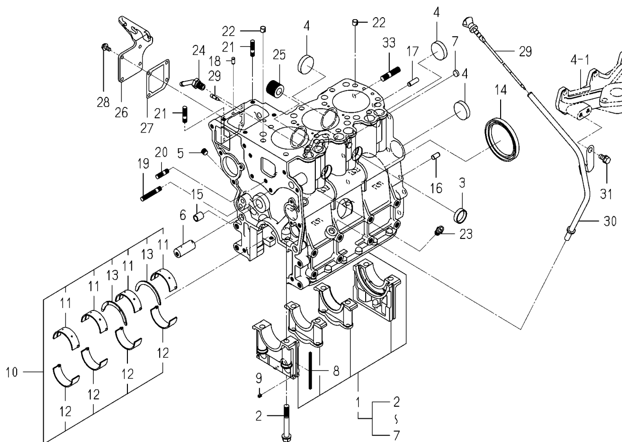
FIG. 5 CYLINDER BLOCK
