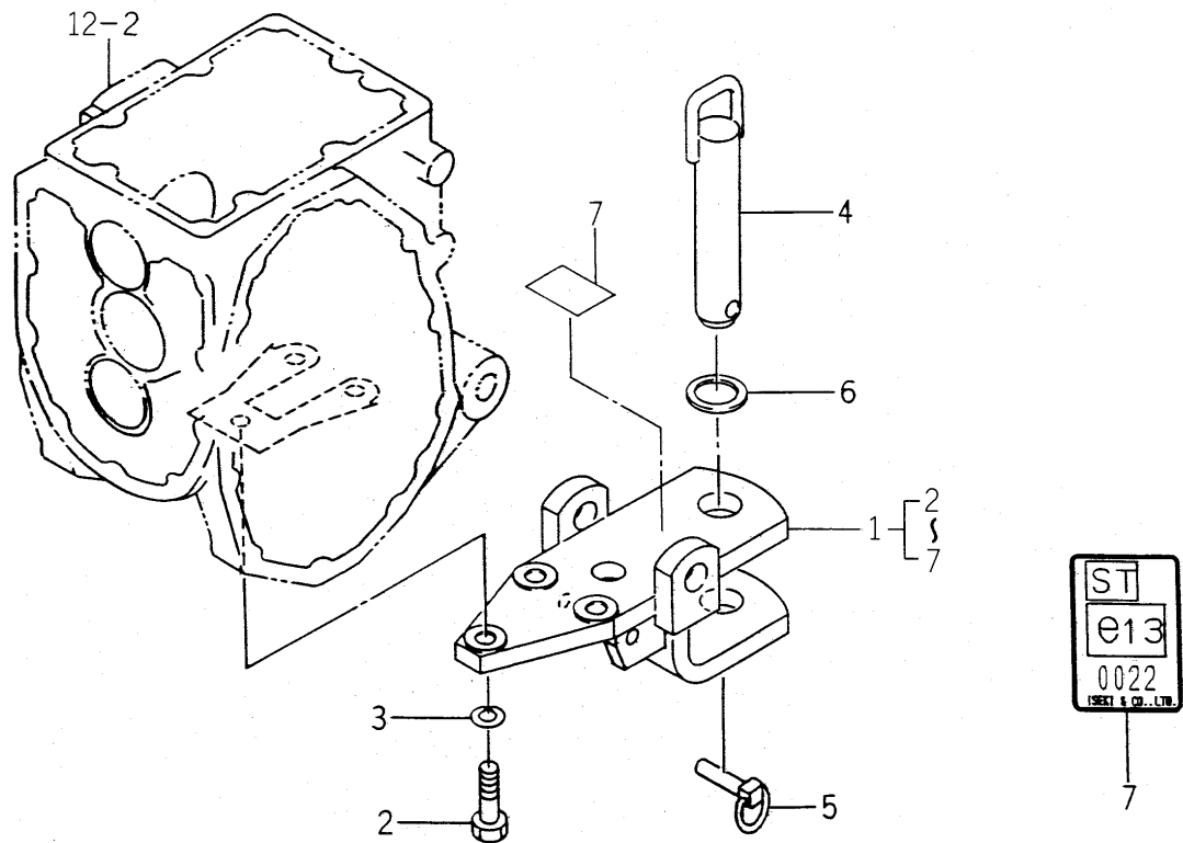
FIG.105 HITCH (DRAW BAR) SET (EXCEPT R TYPE) (OPTION)
