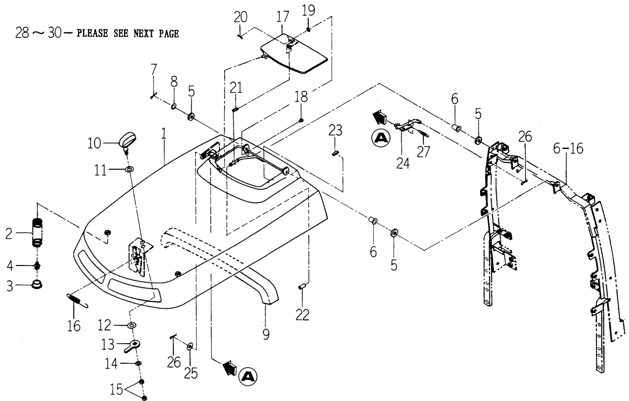
FIG. 72 HOOD SYSTEM(1/2)
