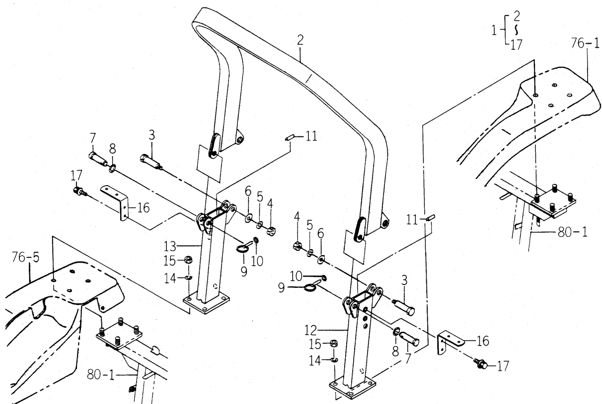
FIG.106 ROPS SET (EXCEPT R TYPE) (OPTION)
