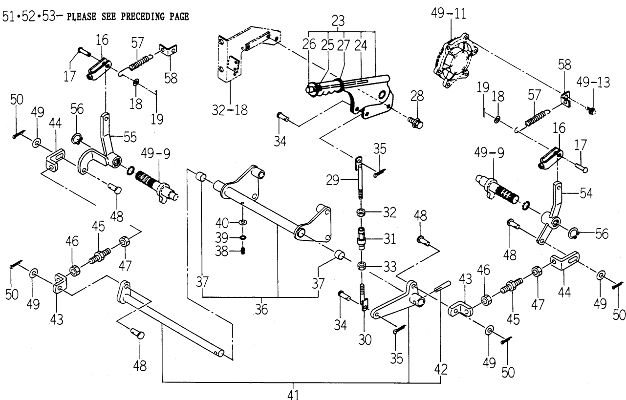
FIG. 50 PEDAL (BRAKE) SYSTEM(2/2) (EXCEPT H TYPE)
