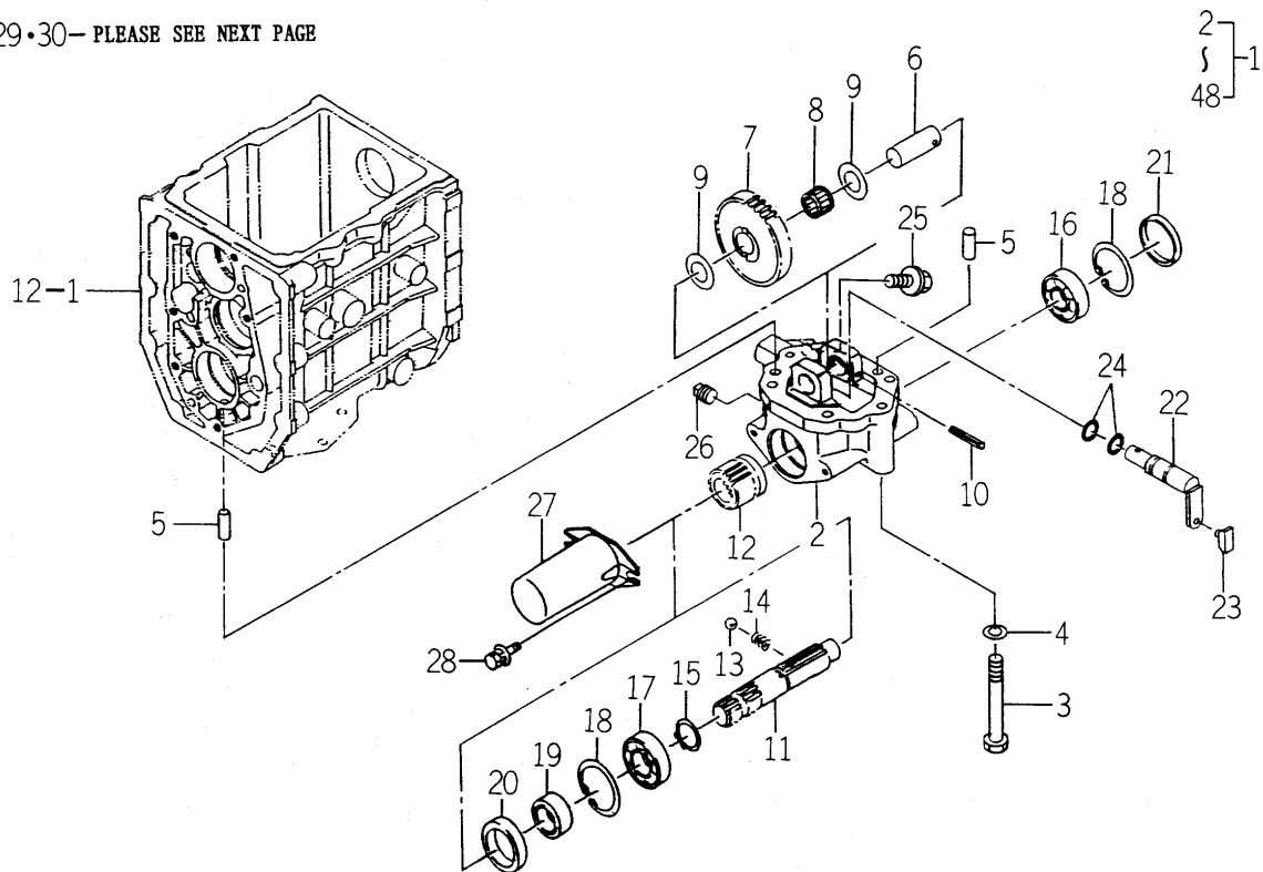
FIG. 95 MID PTO SET (EXCEPT M TYPE)(1/2) (OPTION)
