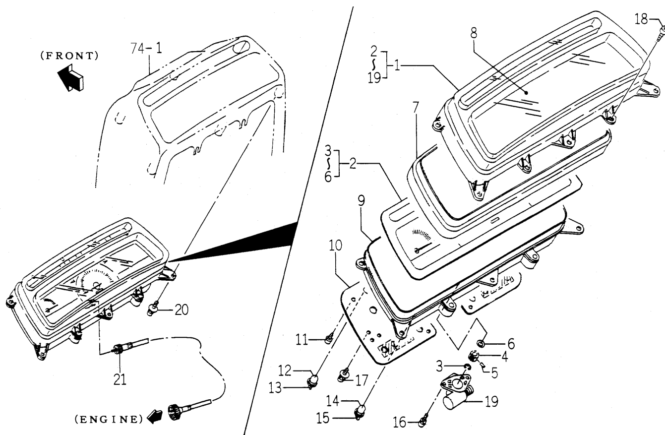
FIG. 84 PANEL SYSTEM
