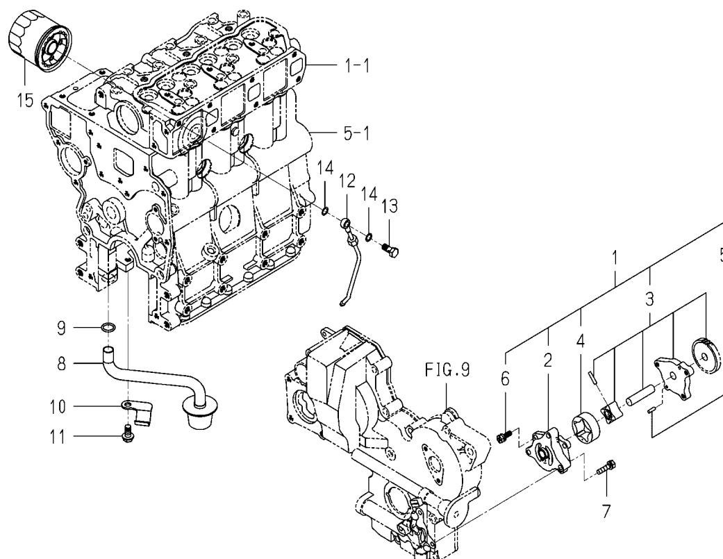
FIG. 16 OIL PUMP
