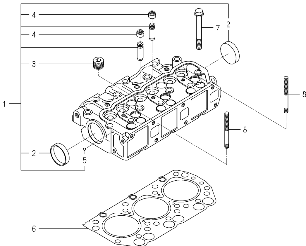
FIG. 1 CYLINDER HEAD
