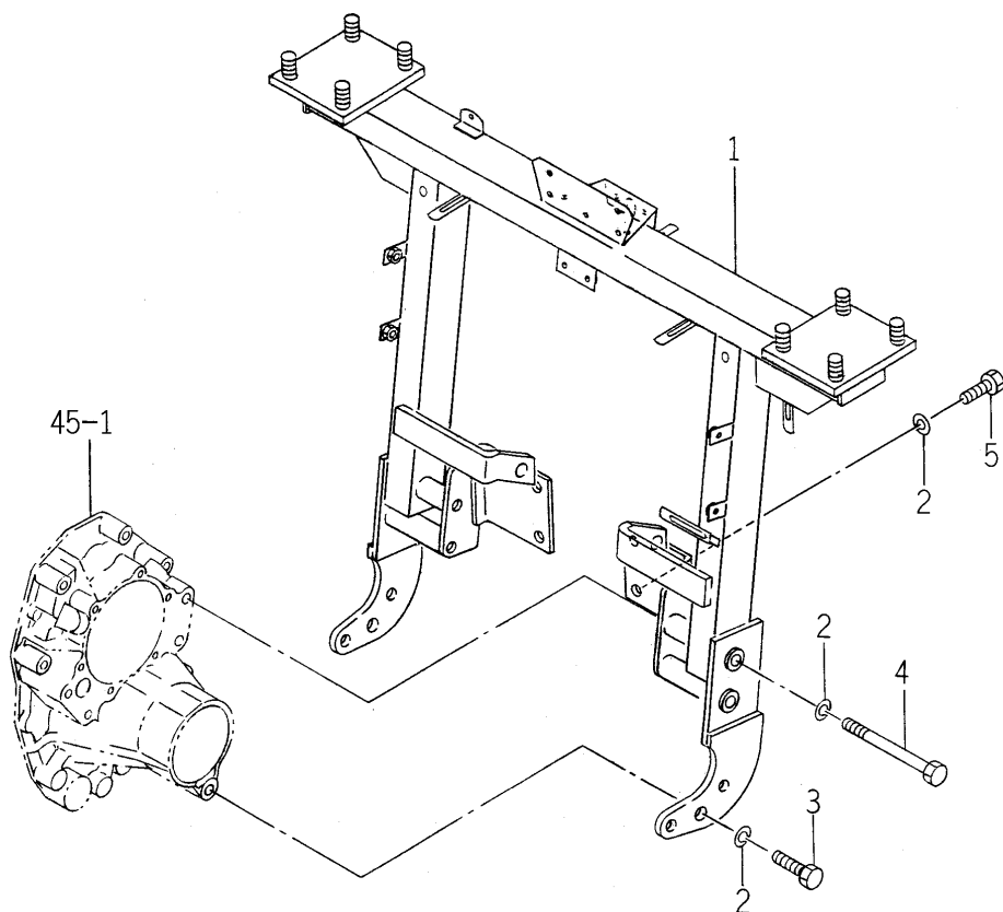
FIG. 80 FRAME SYSTEM
