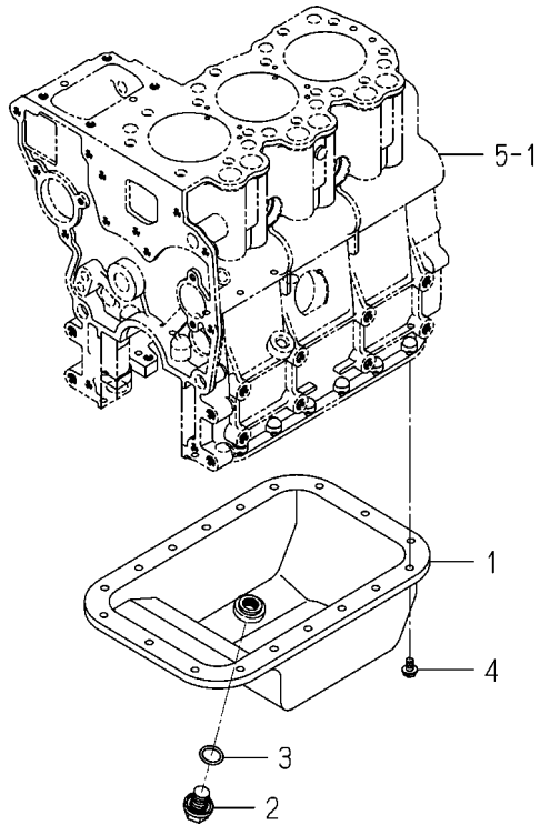
FIG. 7 OIL PAN
