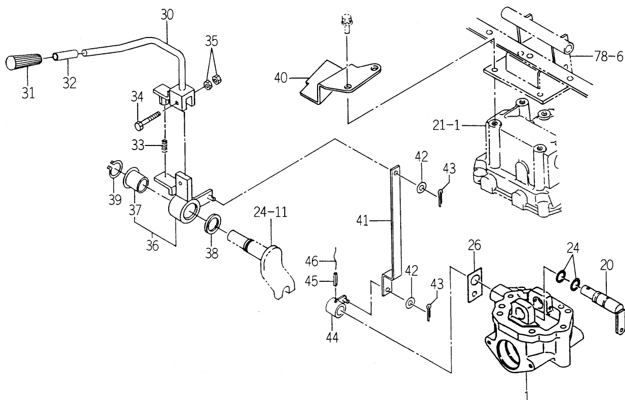
FIG. 36 MID PTO SYSTEM (M TYPE EXCEPT H)(2/2)
