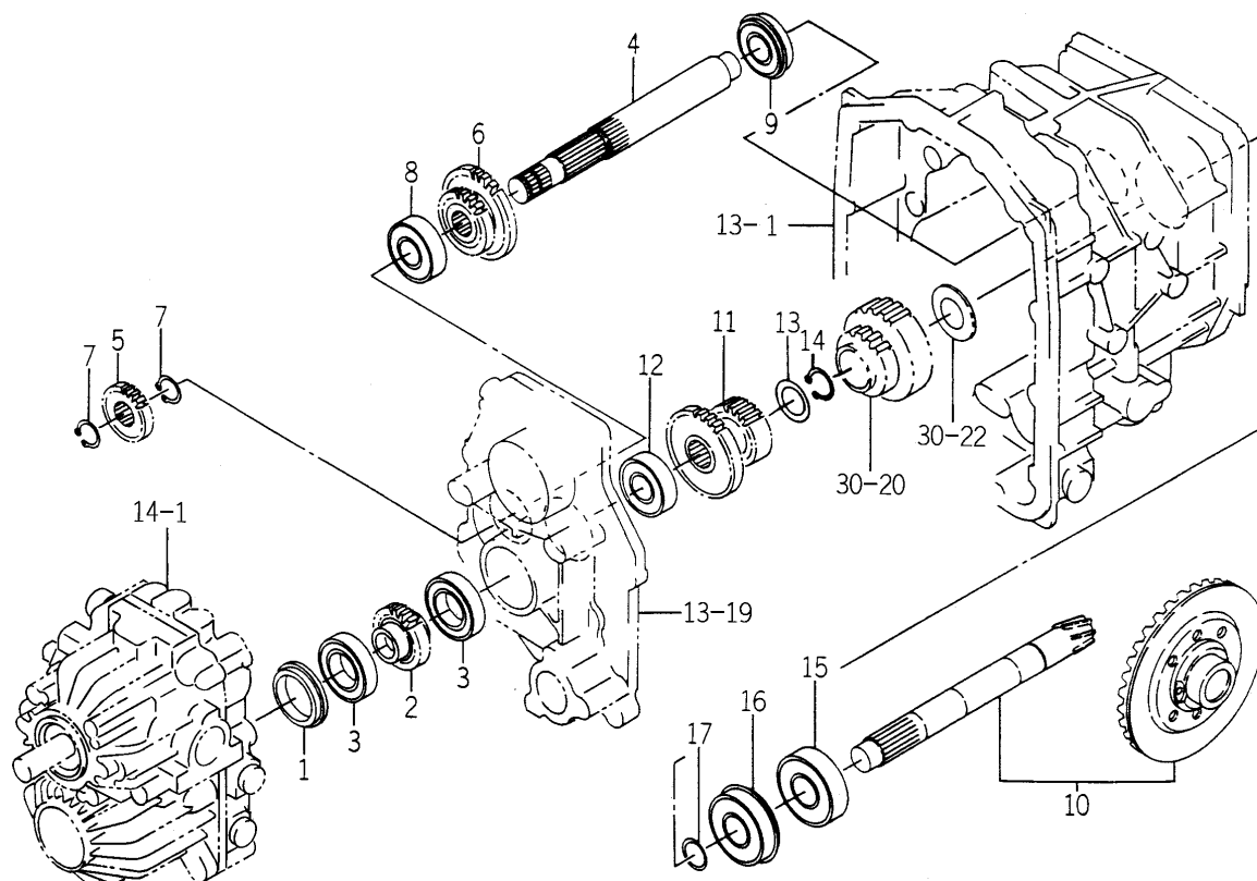
FIG. 16 GEAR (DRIVE) SYSTEM (H TYPE)
