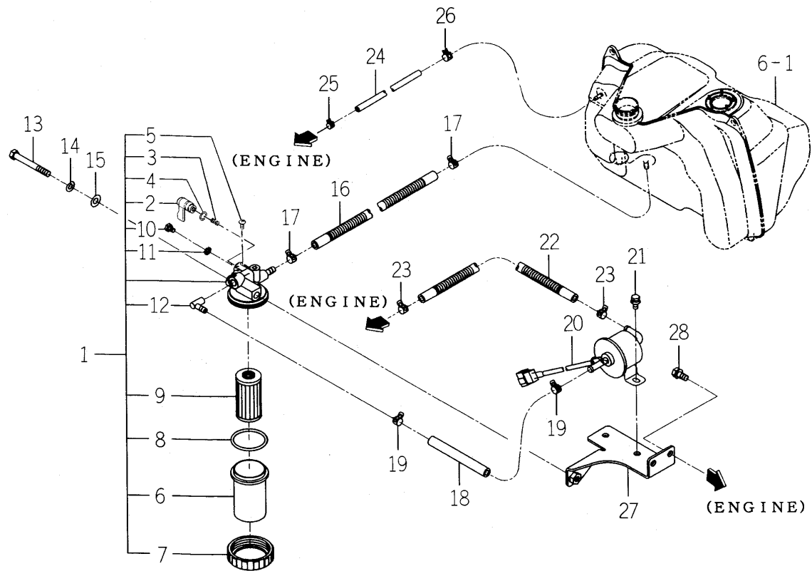
FIG. 5 FILTER SYSTEM
