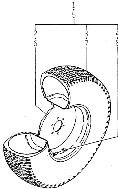
FIG. 99 REAR WHEEL (TURF) SYSTEM (TM3200) (OPTION)
