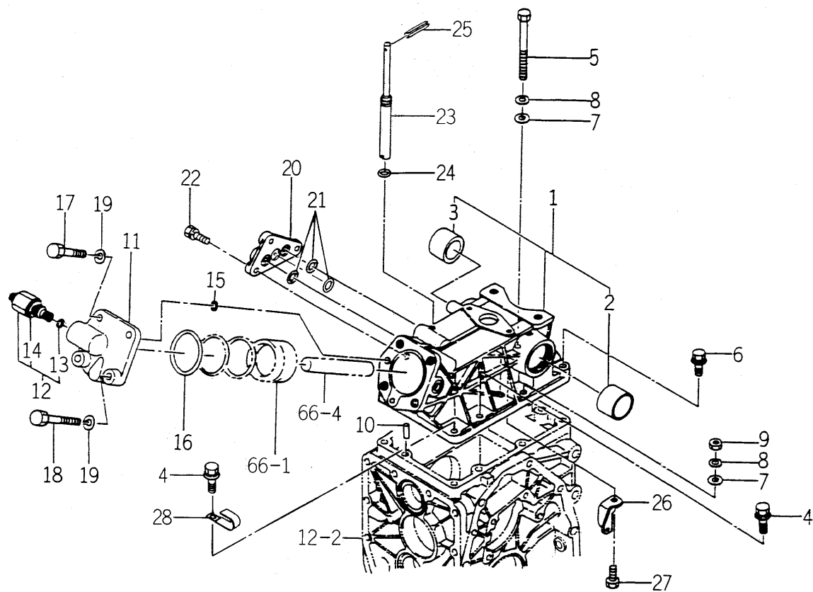
FIG. 64 CYLINDER CASE SYSTEM
