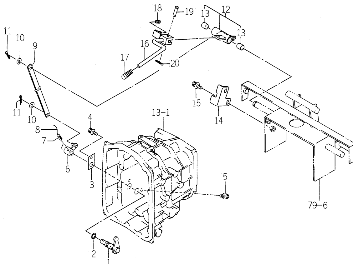
FIG. 33 LEVER (PTO) SYSTEM (H TYPE)
