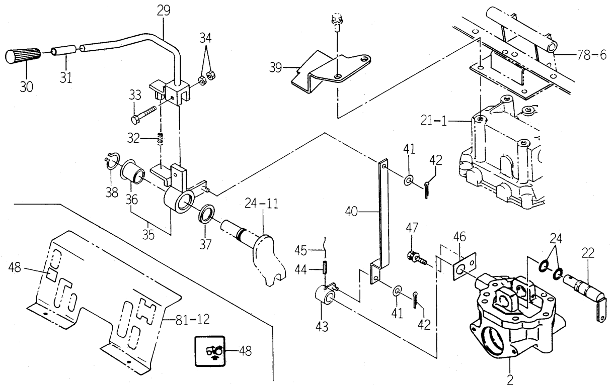
FIG. 95 MID PTO SET (EXCEPT M TYPE)(2/2) (OPTION)
