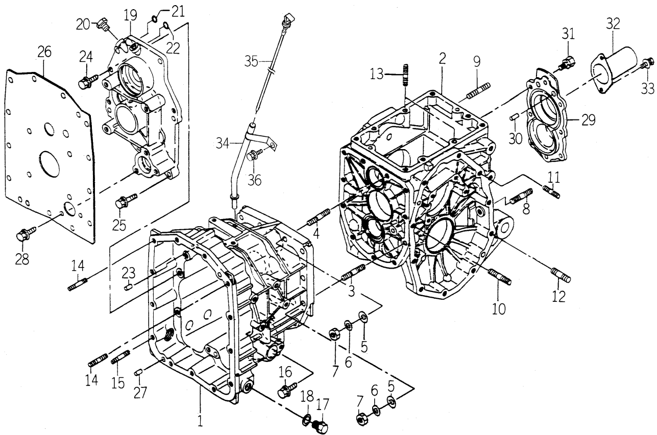
FIG. 13 CASE (TRANSMISSION) SYSTEM (H TYPE)
