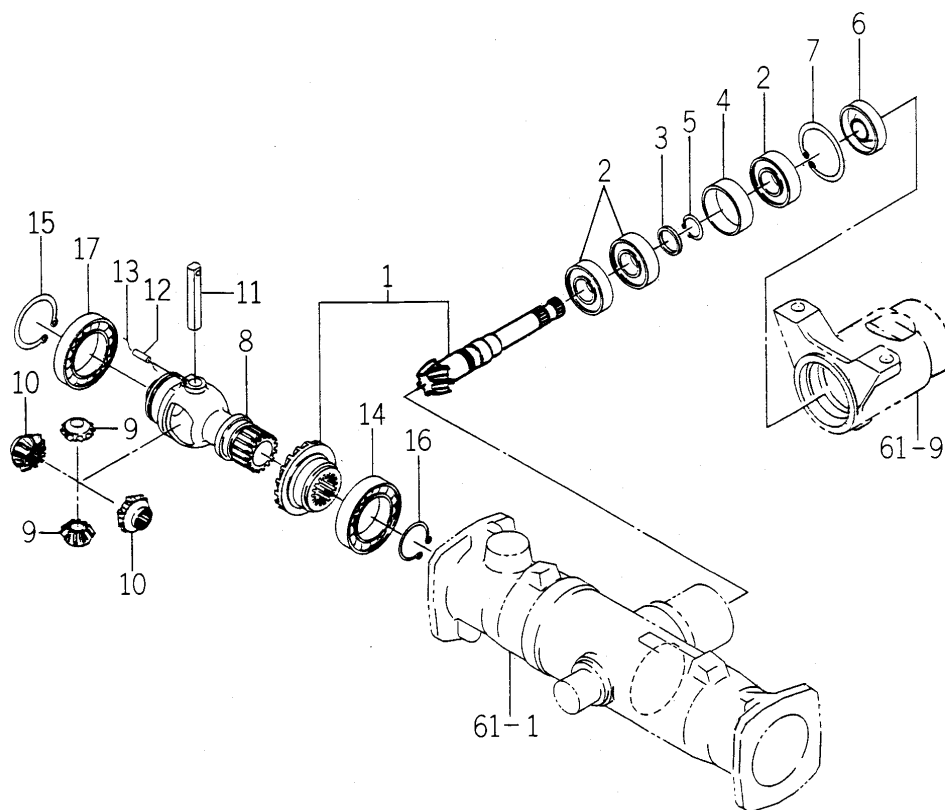
FIG. 60 PINION (DRIVE) SYSTEM
