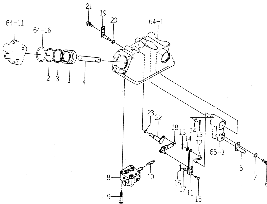
FIG. 66 CYLINDER SYSTEM
