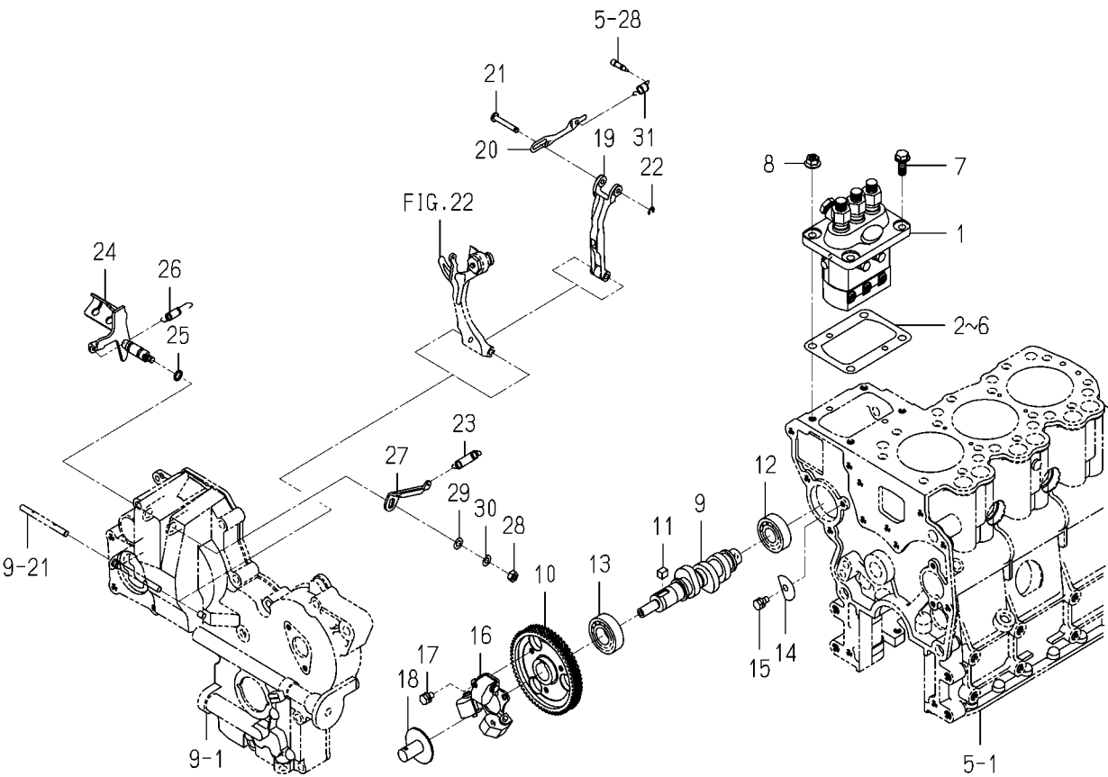
FIG. 20 INJECTION PUMP
