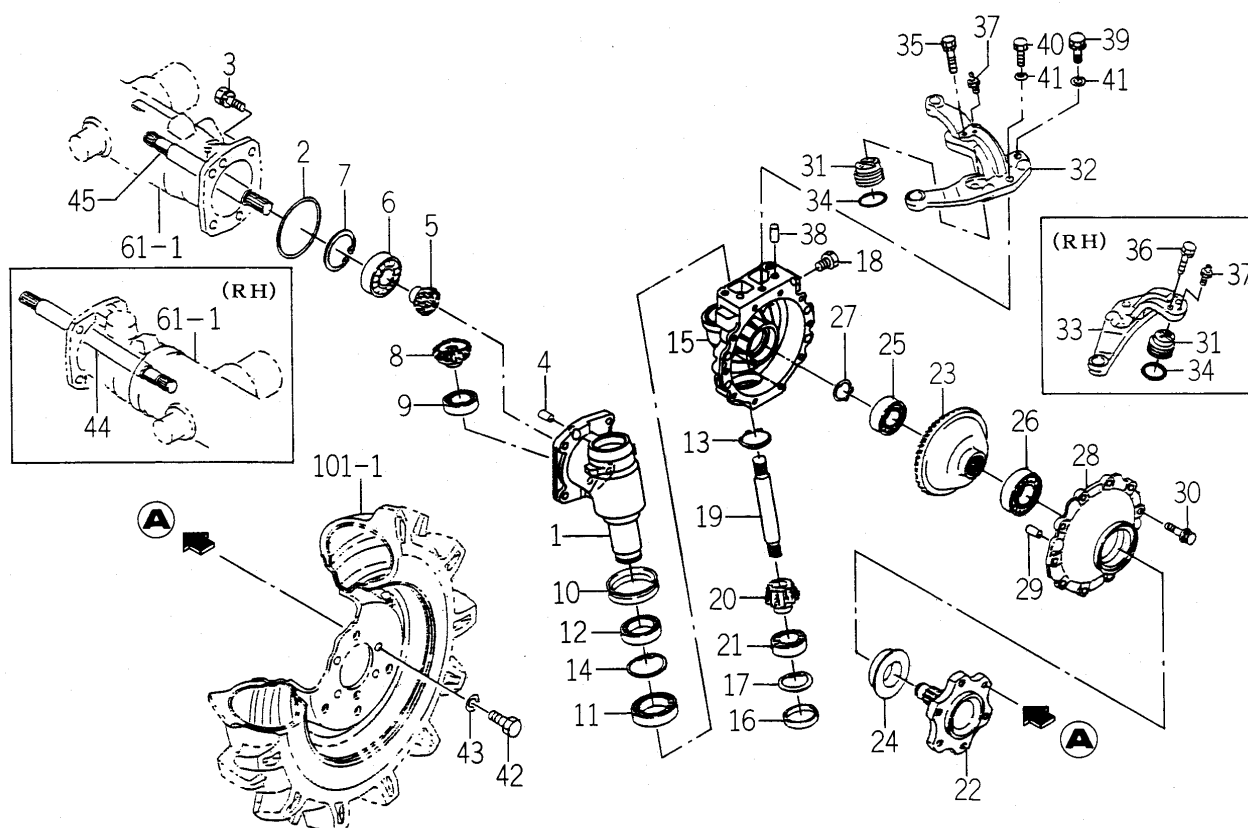
FIG. 62 GEAR (FINAL) SYSTEM
