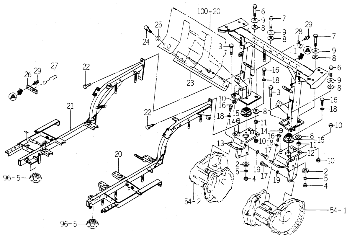
FIG. 98 MOUNT (REAR) SYSTEM (EXCEPT H TYPE)
