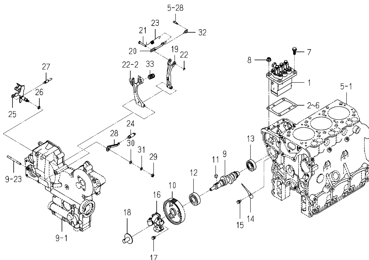
FIG. 20 INJECTION PUMP
