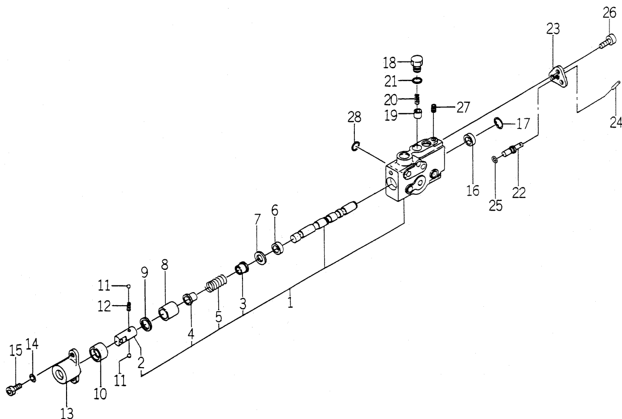
FIG.138 COMPONENT PARTS FOR 1640-530-600-10 ON Fig.128,129
