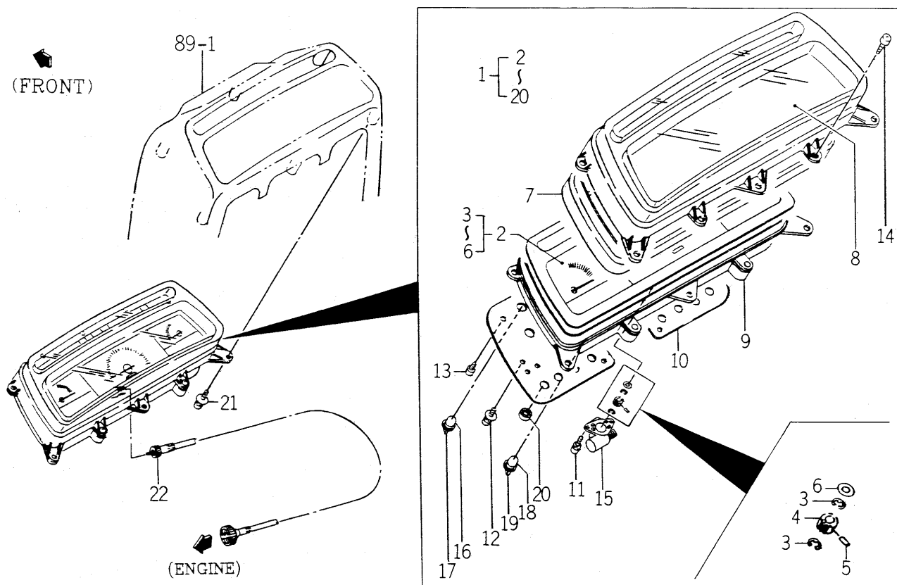
FIG.104 PANEL SYSTEM
