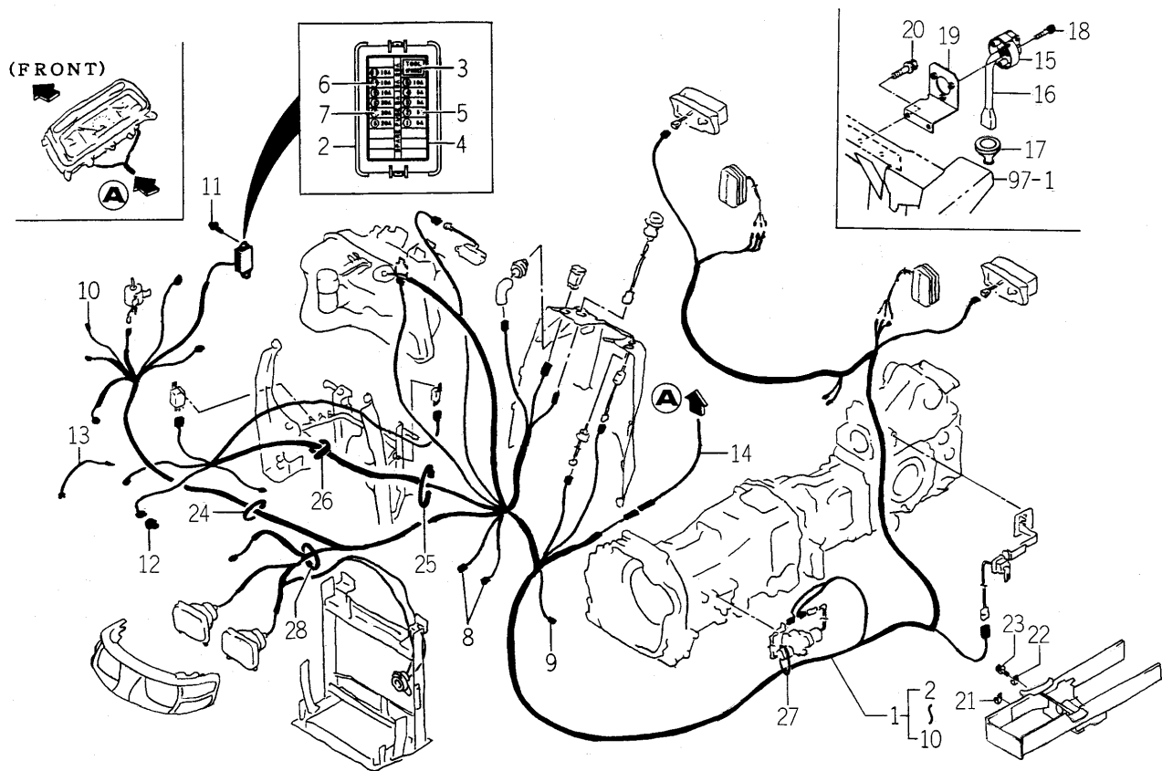
FIG.107 HARNESS SYSTEM (TH4260-H TYPE)
