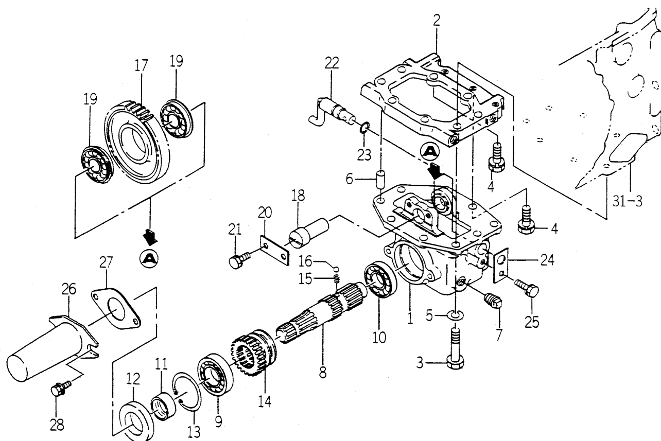
FIG. 36 MID PTO SYSTEM (H TYPE)
