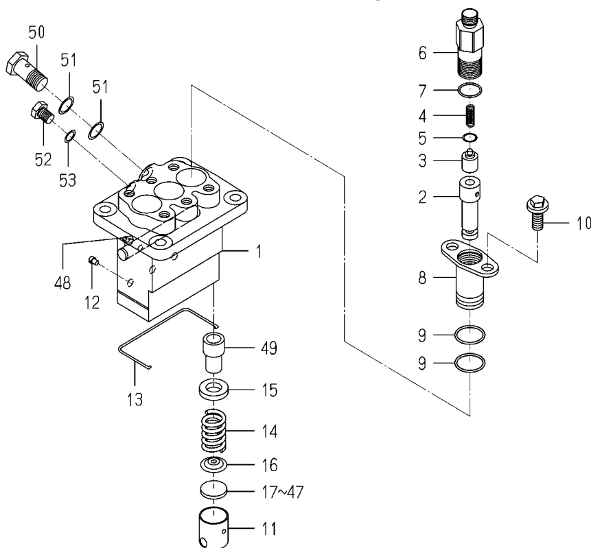
FIG. 29 COMPONENT PARTS FOR 6215-600-104-20 ON Fig.20
