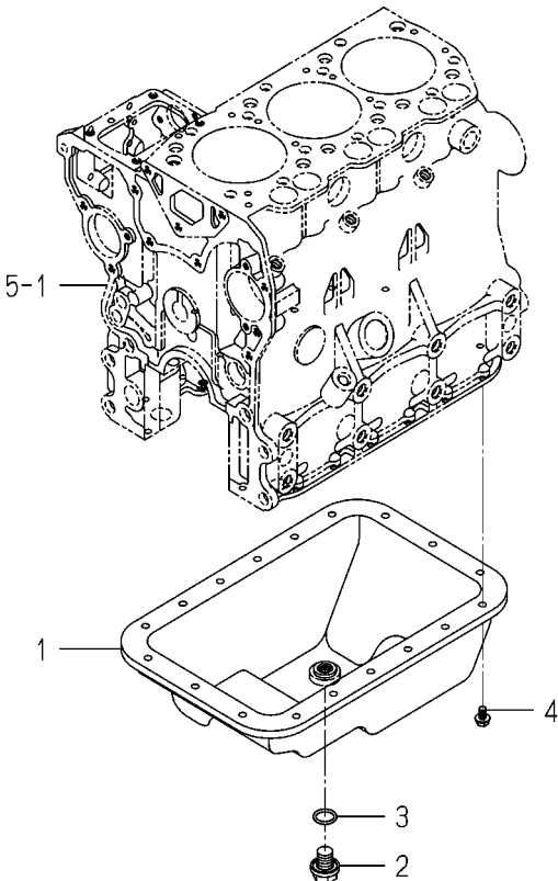
FIG. 7 OIL PAN
