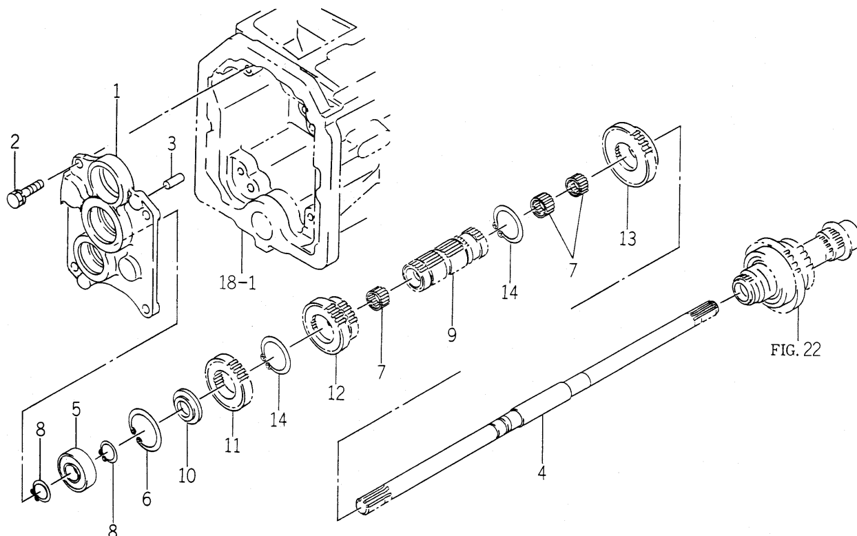
FIG. 20 INPUT METAL, MAIN CHANGE GEAR SYSTEM (EXCEPT H TYPE)
