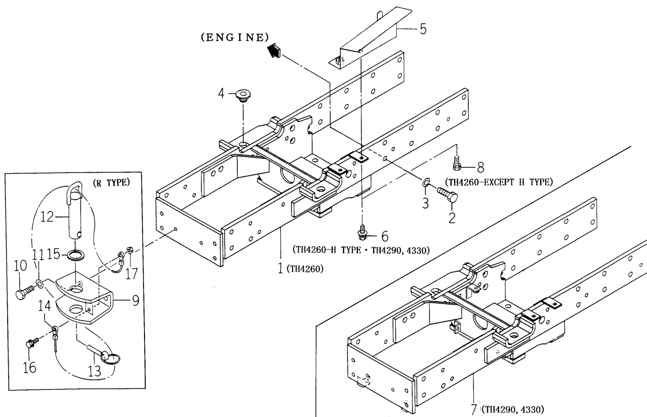
FIG. 64 BRACKET (AXLE), HITCH (FRONT/R TYPE) SYSTEM
