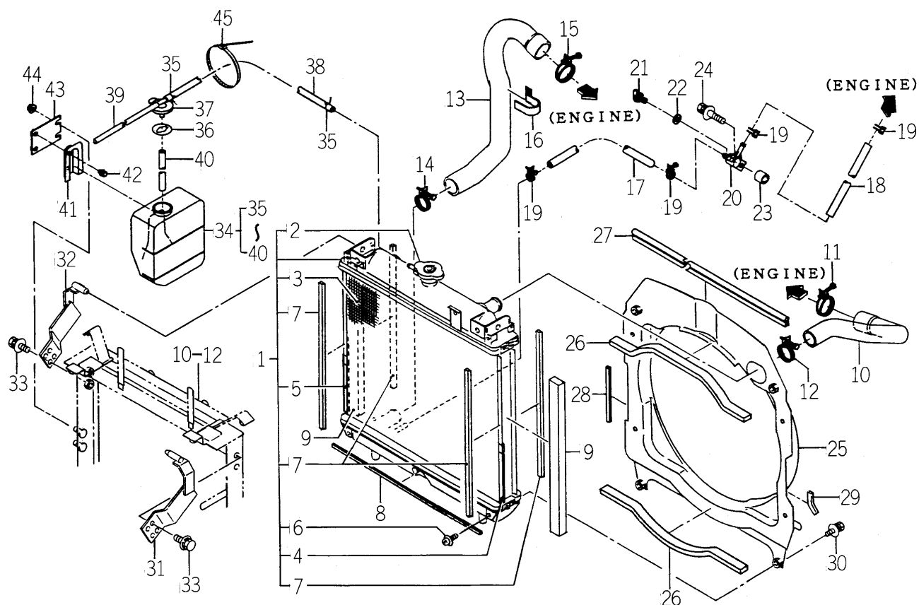
FIG. 1 RADIATOR SYSTEM
