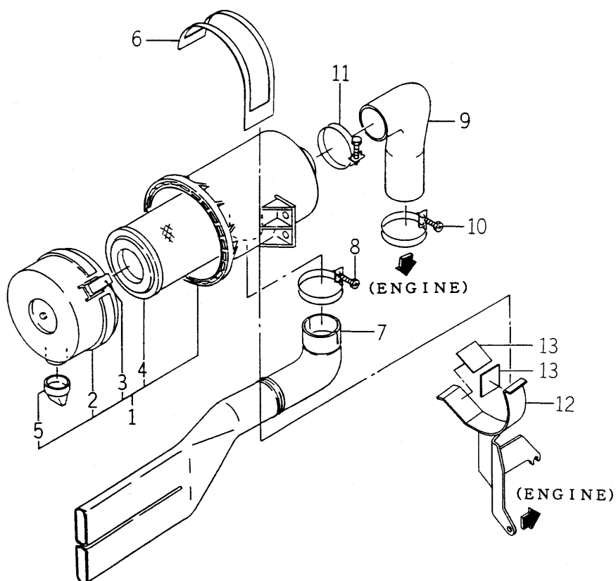
FIG. 3 AIR CLEANER SYSTEM
