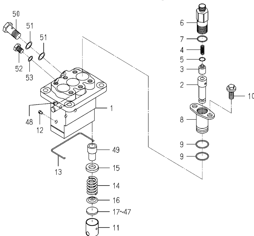
FIG. 28 COMPONENT PARTS FOR 6215-600-078-10 ON Fig.20
