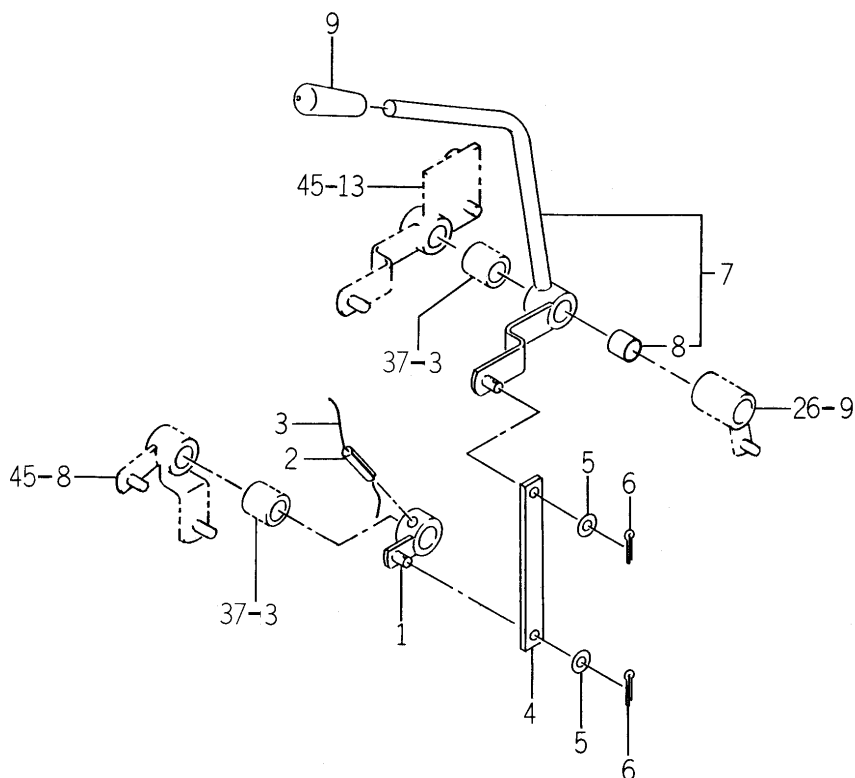
FIG. 42 CHANGE LEVER (4WD) SYSTEM (EXCEPT H TYPE)
