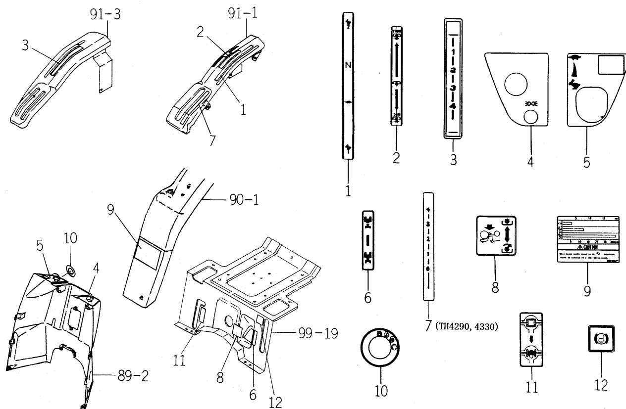
FIG.113 LABEL (H TYPE)
