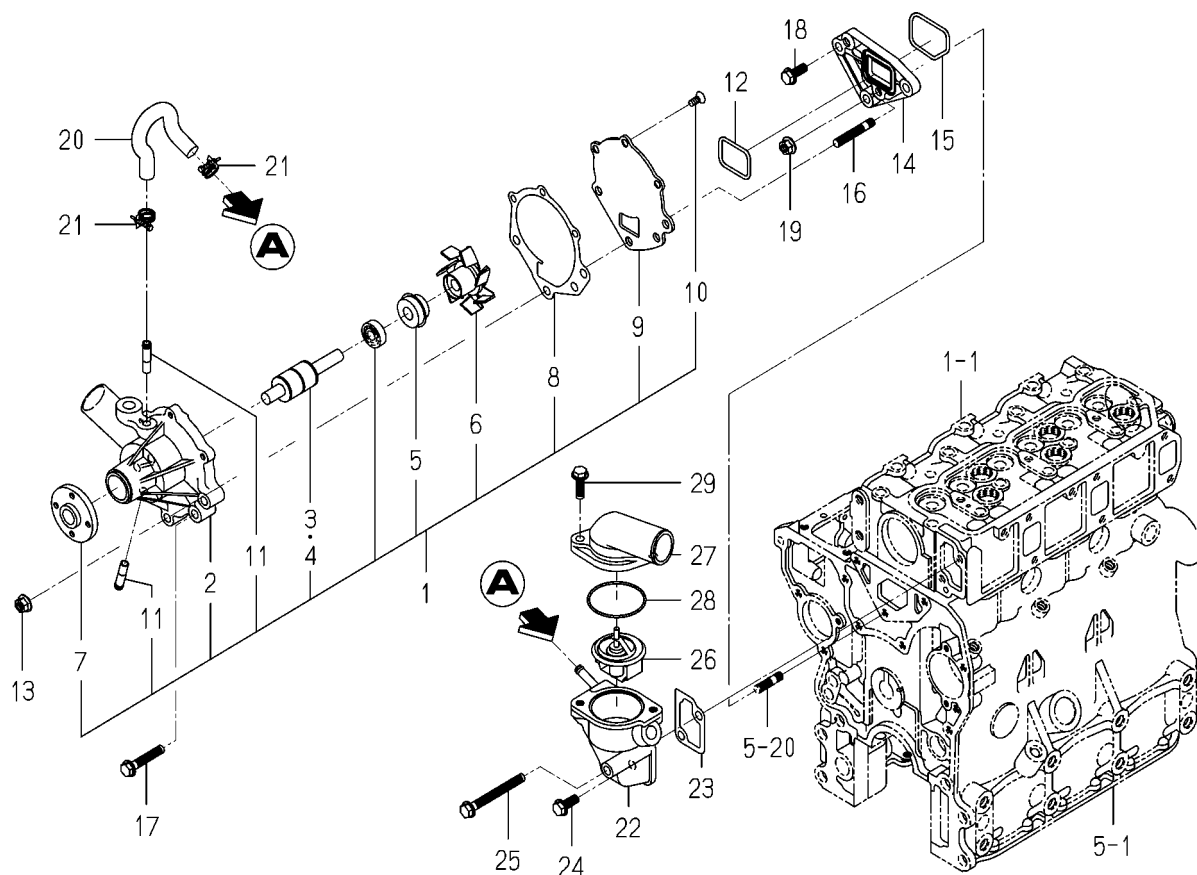
FIG. 17 WATER PUMP
