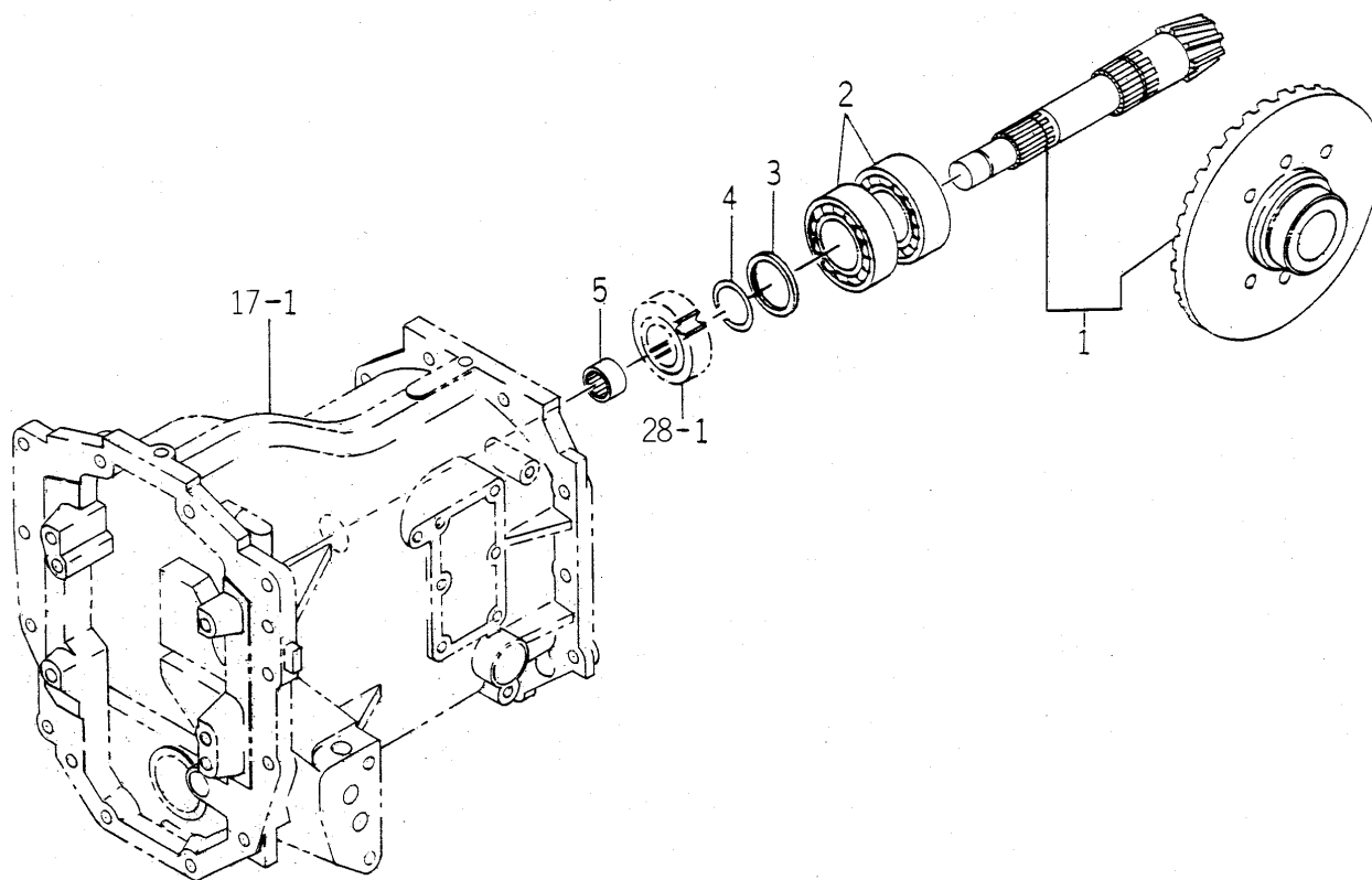
FIG. 50 DRIVE PINION SYSTEM (H TYPE)
