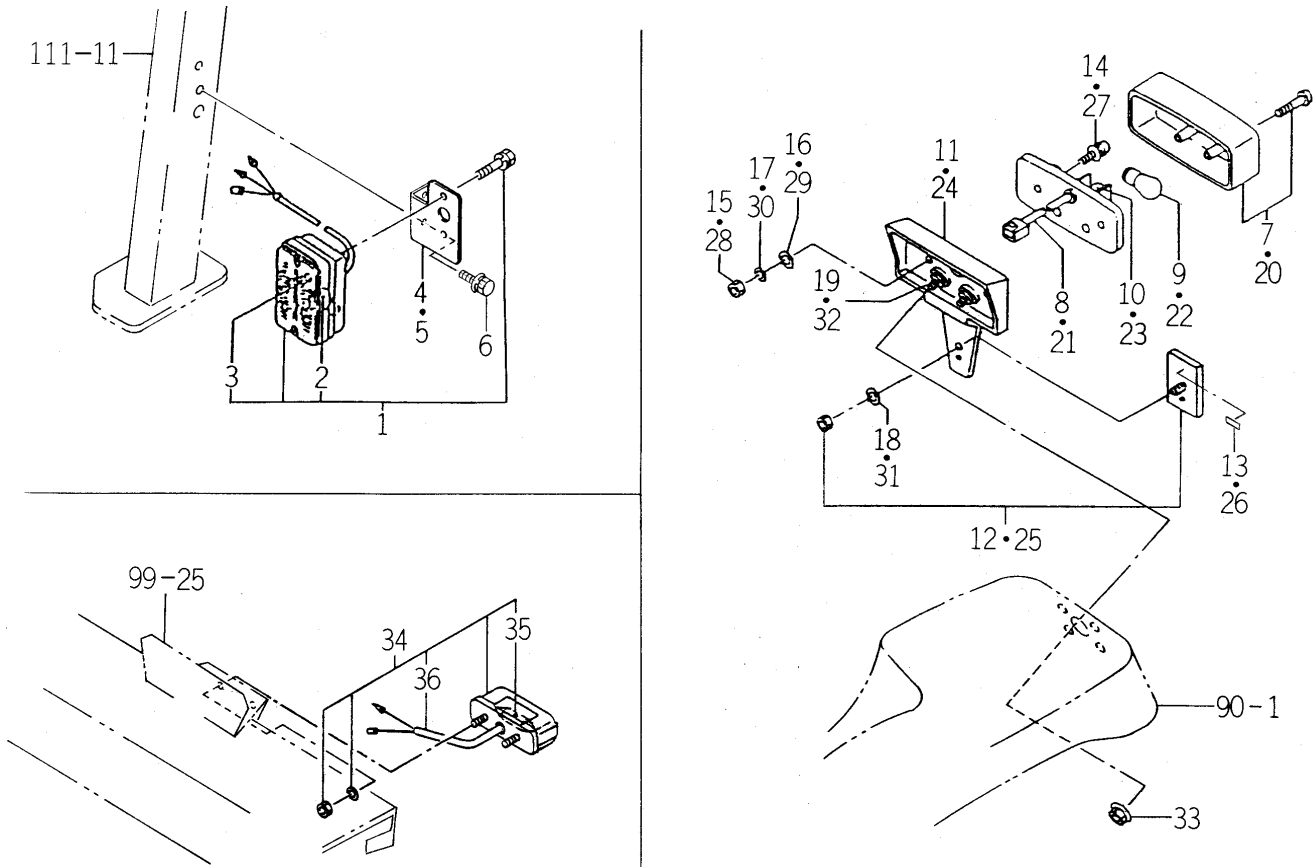
FIG.102 LAMP SYSTEM (H TYPE)
