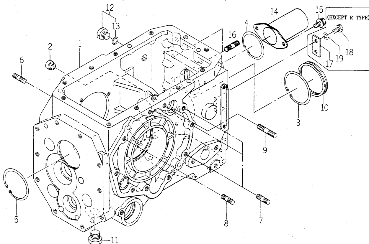
FIG. 32 REAR MISSION CASE SYSTEM (EXCEPT H TYPE)
