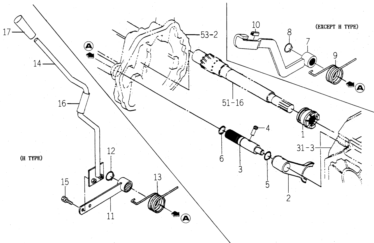
FIG. 56 DIFF-LOCK SYSTEM
