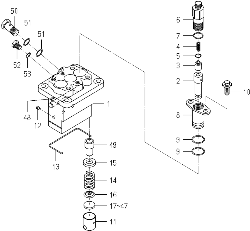
FIG. 29 COMPONENT PARTS FOR 6215-600-078-10 ON Fig.20
