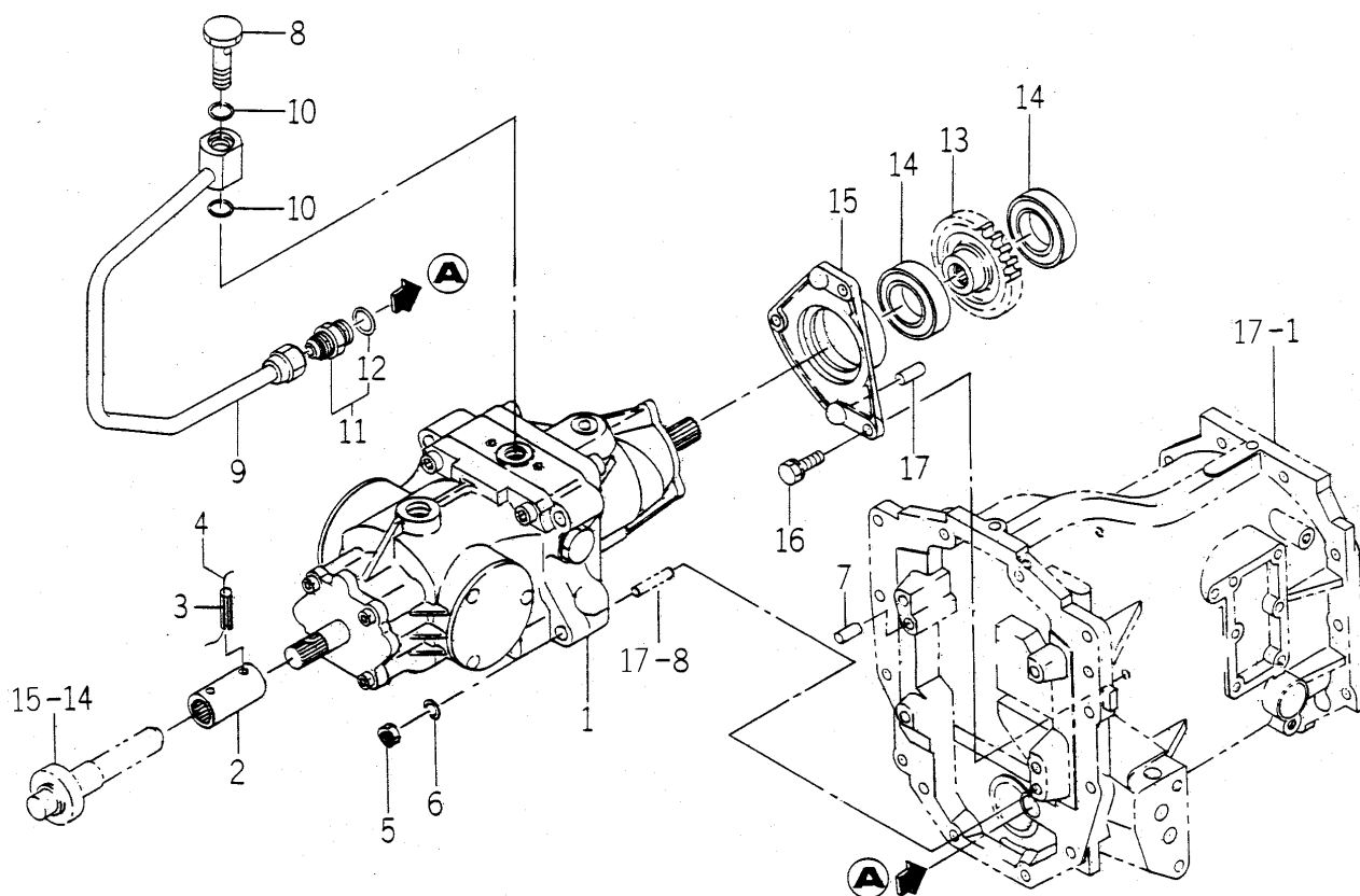
FIG. 19 HST UNIT,INPUT GEAR SYSTEM (H TYPE)
