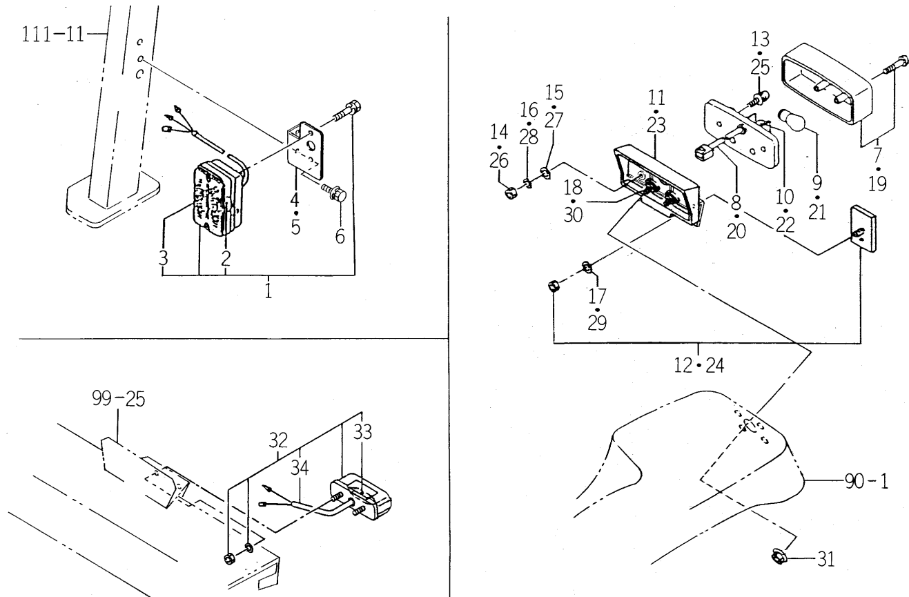
FIG.103 LAMP SYSTEM (EXCEPT H TYPE)
