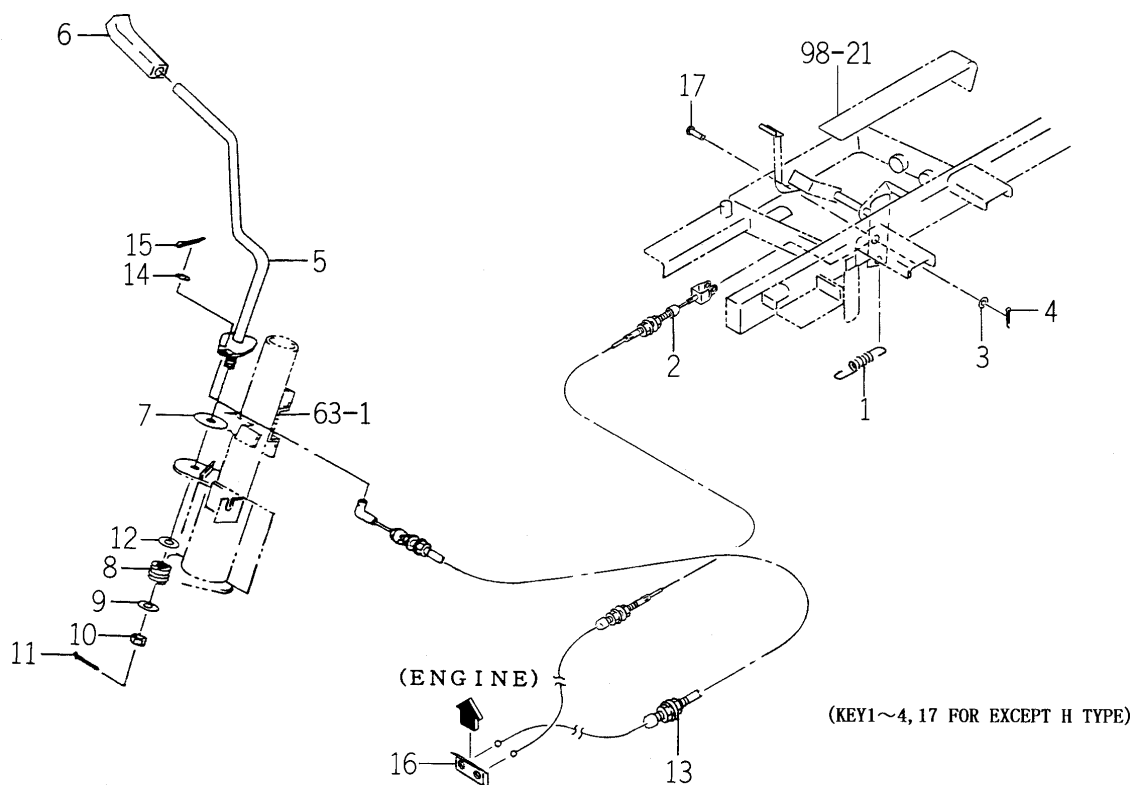
FIG. 11 ACCELERATOR SYSTEM
