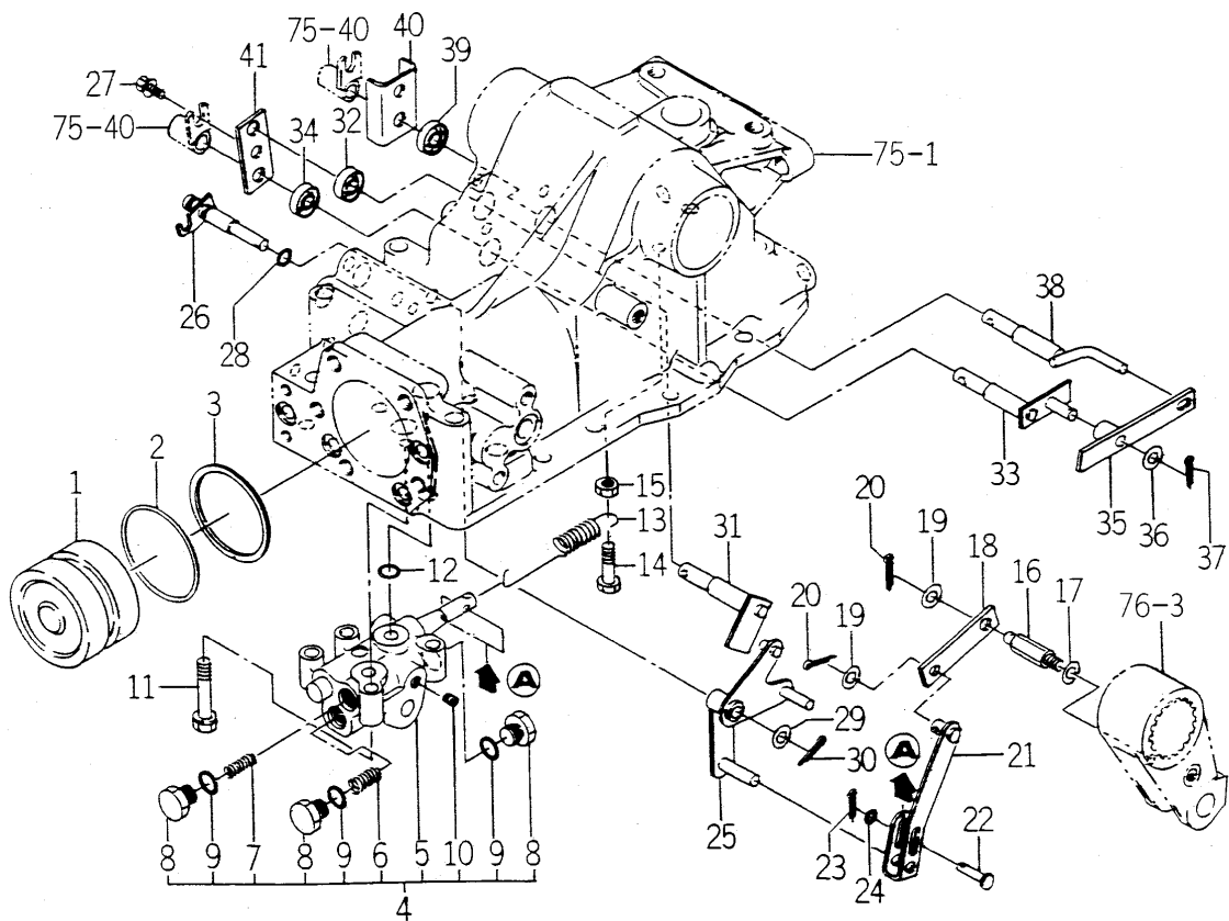
FIG. 77 CYLINDER SYSTEM
