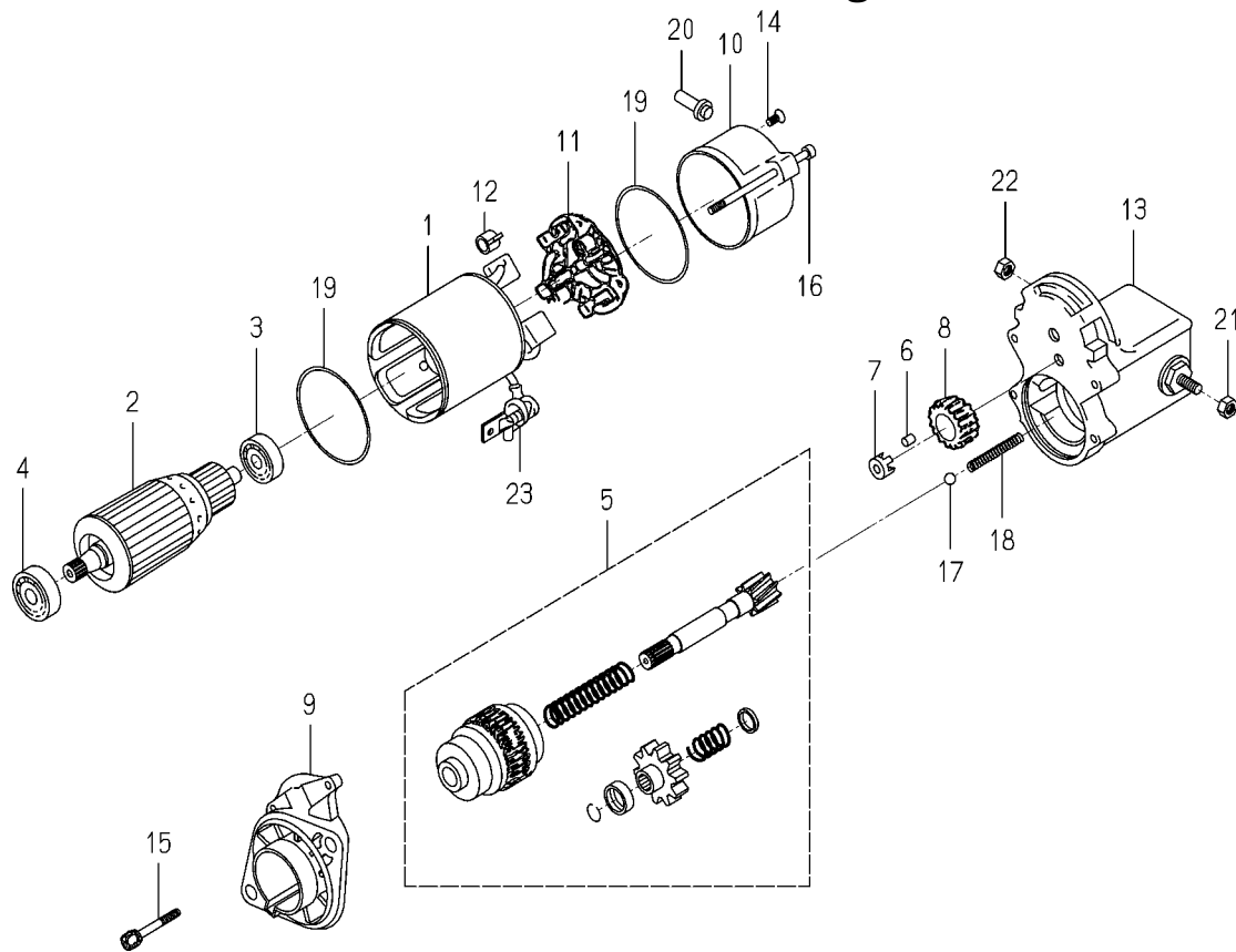
FIG. 30 COMPONENT PARTS FOR 6281-100-002-30 ON Fig.23
