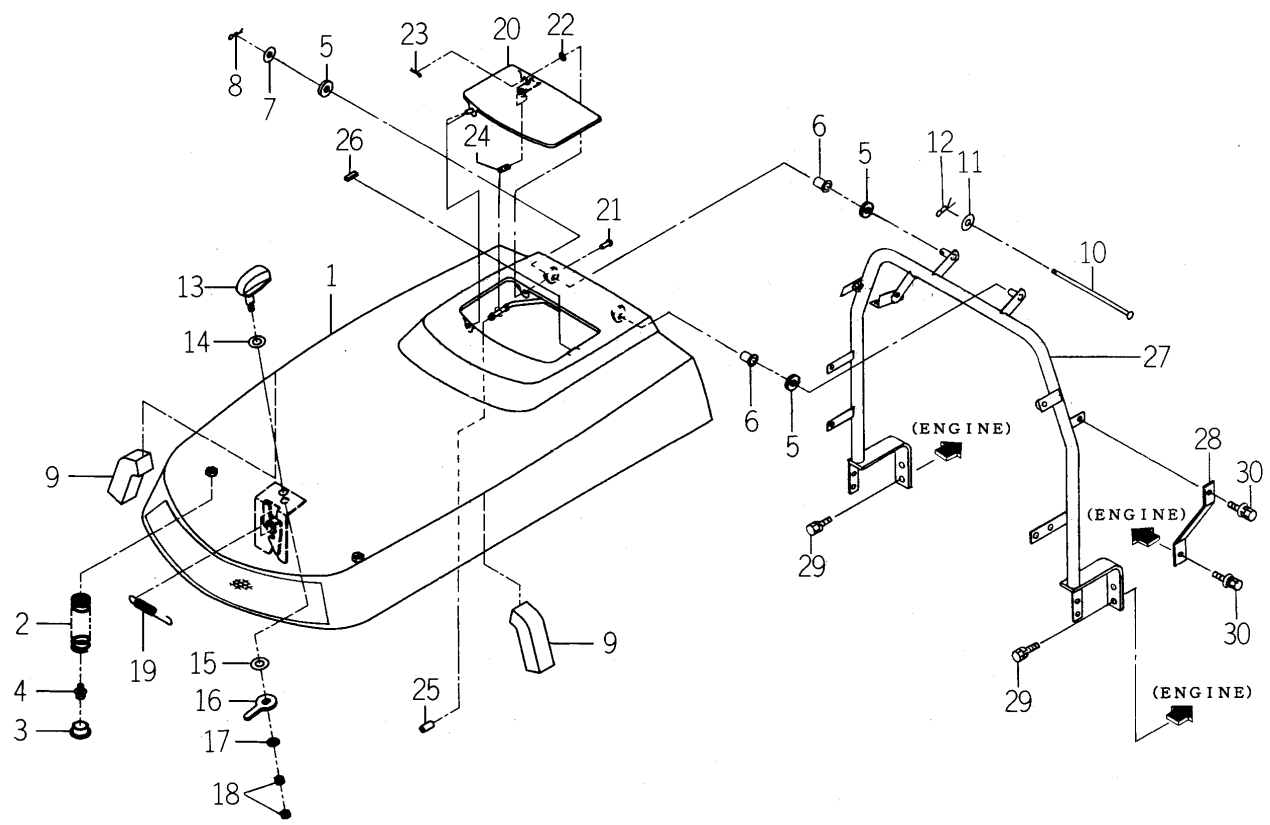
FIG. 87 HOOD SYSTEM(1/2)
