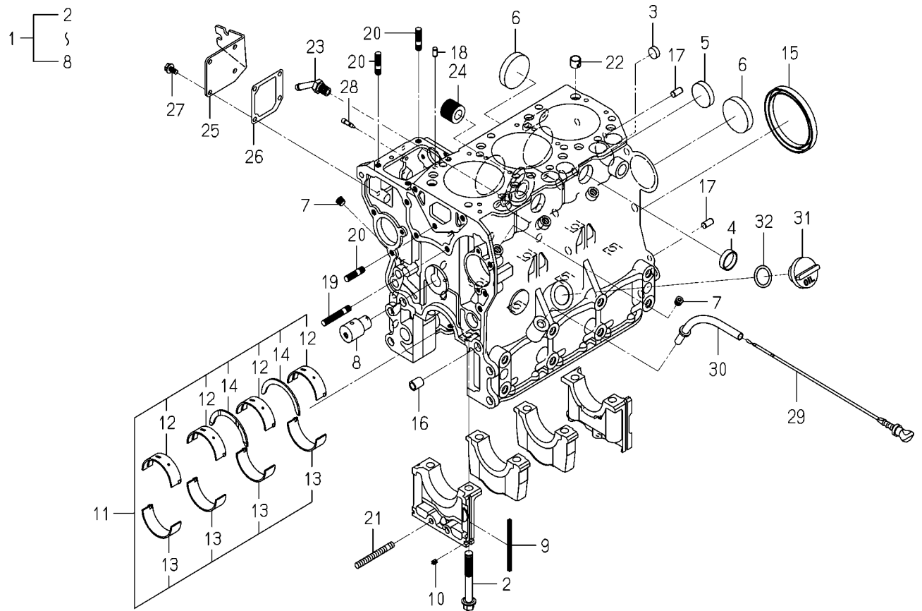
FIG. 5 CYLINDER BLOCK
