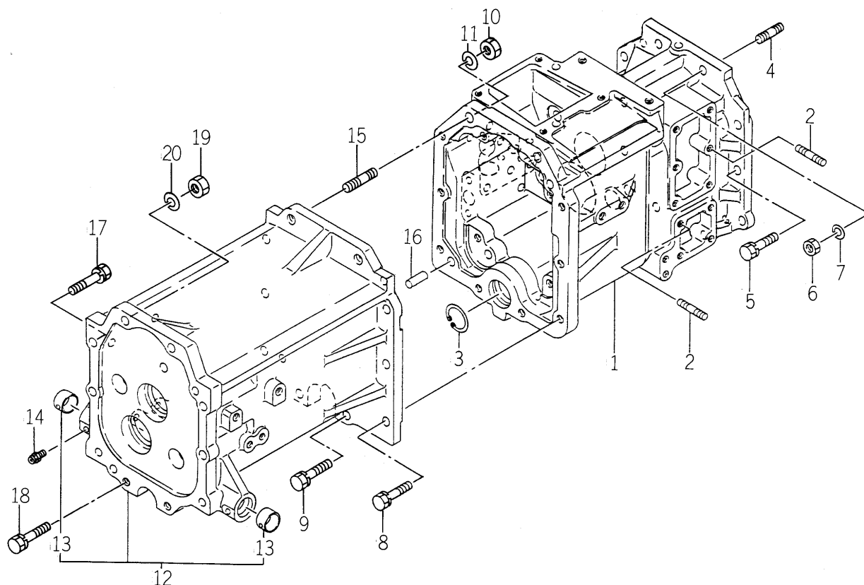
FIG. 18 FRONT MISSION CASE SYSTEM (EXCEPT H TYPE)
