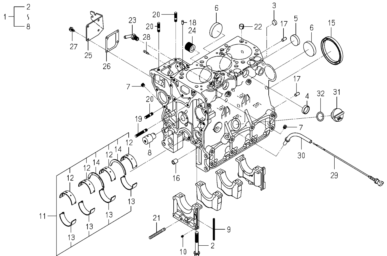
FIG. 5 CYLINDER BLOCK
