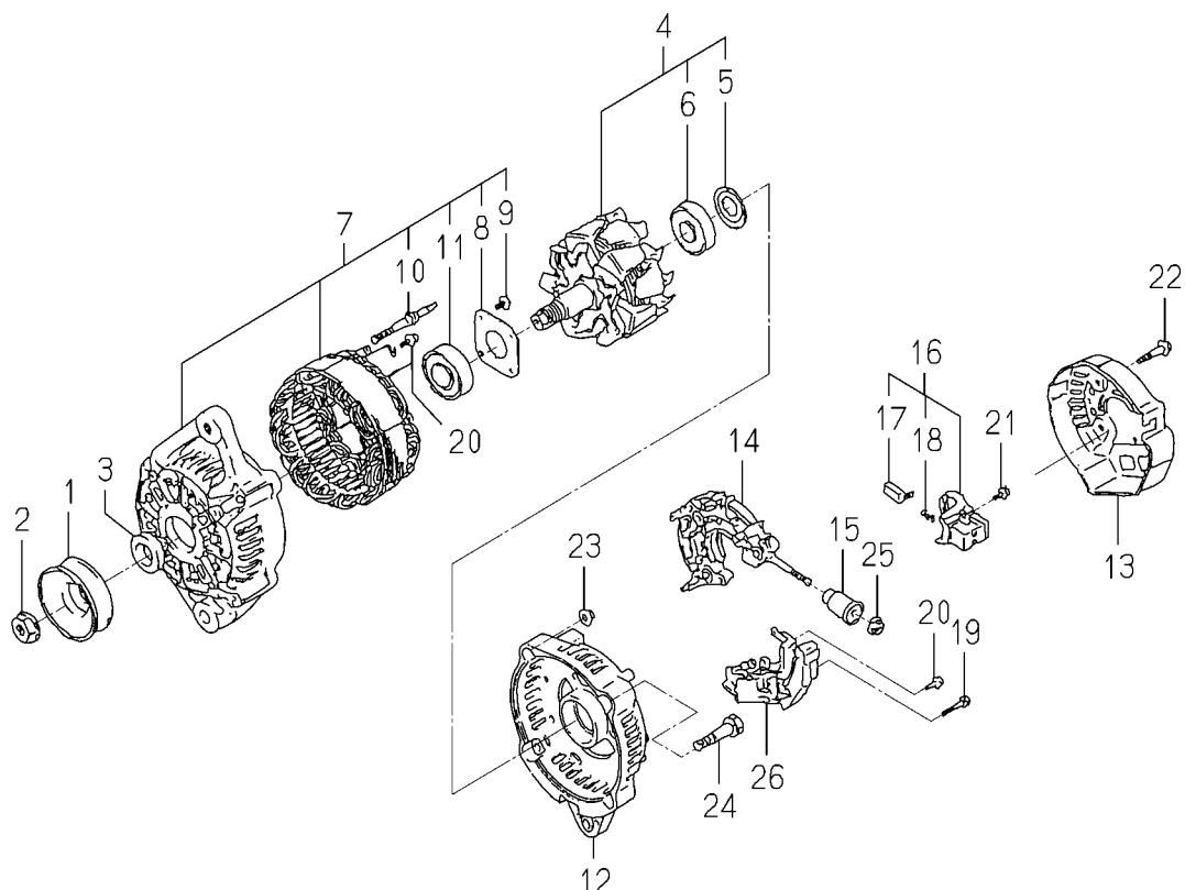
FIG. 31 COMPONENT PARTS FOR 6281-200-021-00 ON Fig.23
