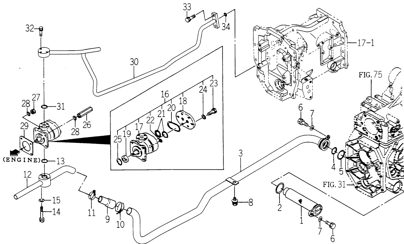
FIG. 80 PIPING SYSTEM (H TYPE)(1/2)
