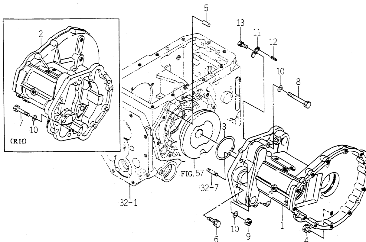
FIG. 54 REAR AXLE HOUSING SYSTEM (EXCEPT H TYPE)
