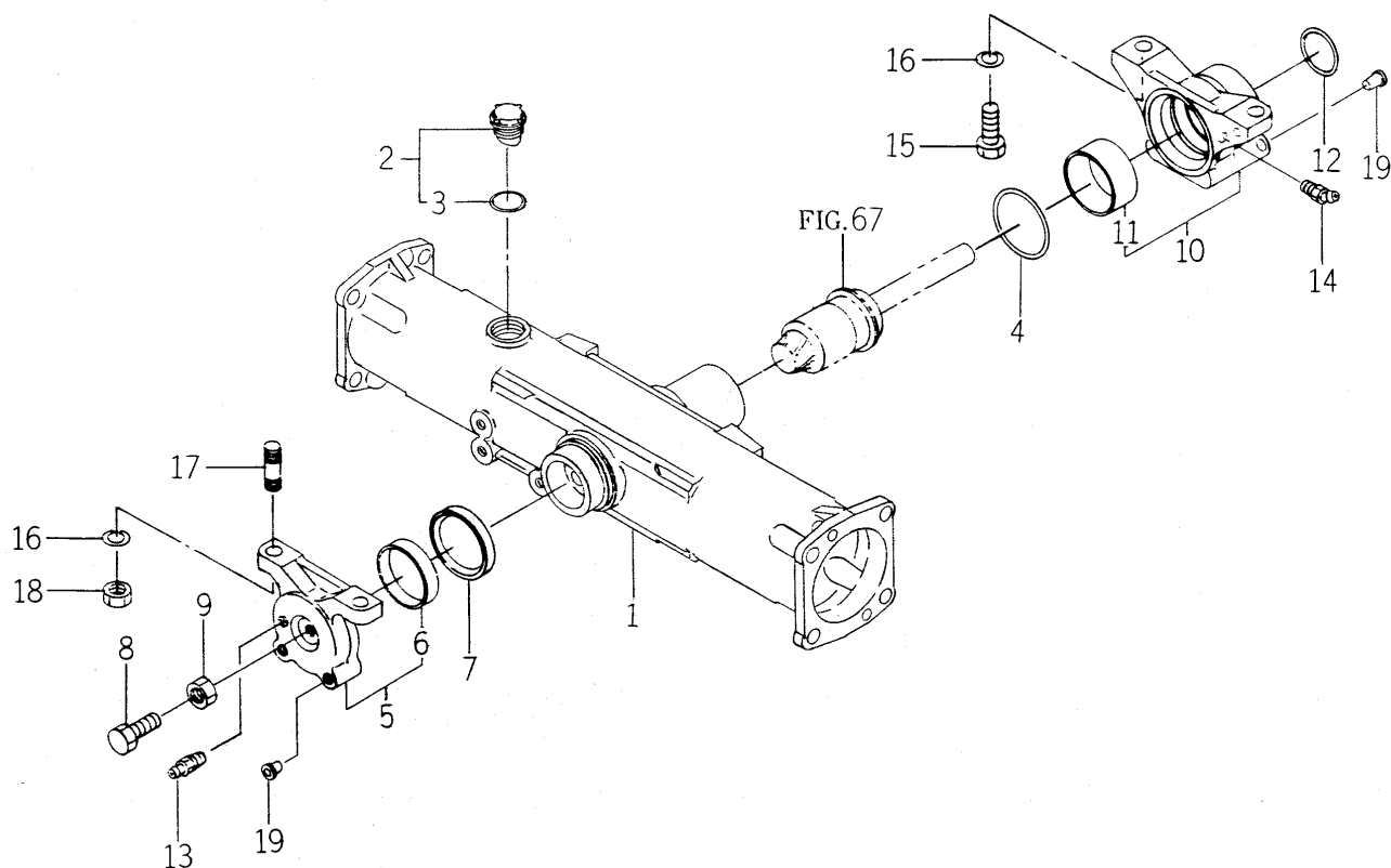
FIG. 69 HOUSING (AXLE) SYSTEM (EXCEPT H TYPE)
