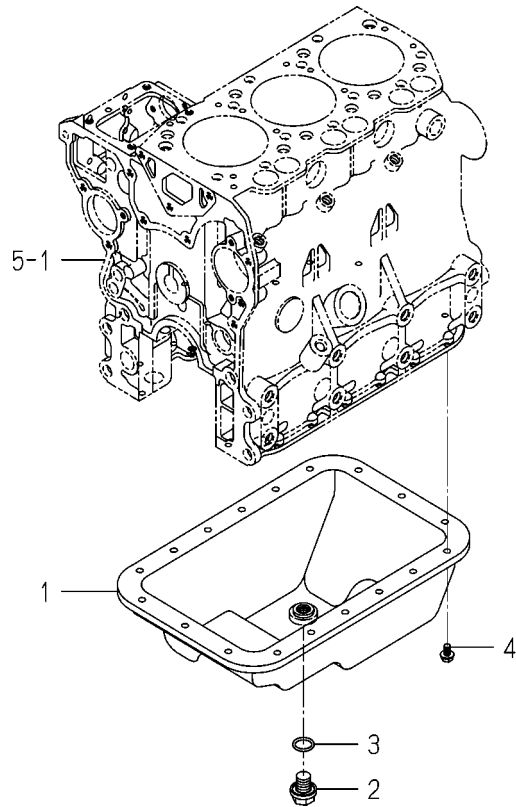
FIG. 7 OIL PAN
