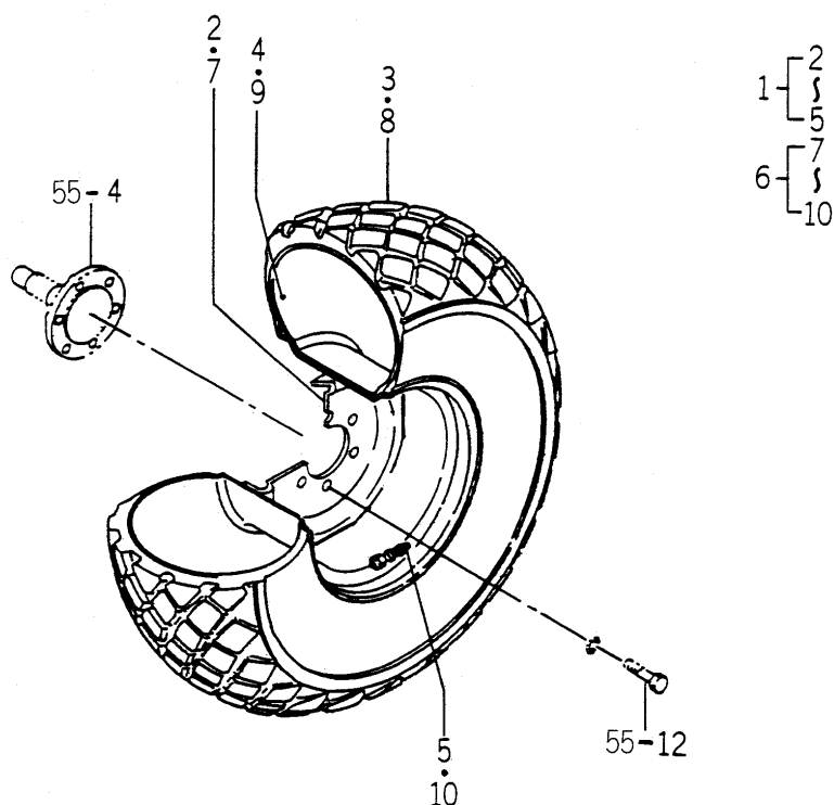
FIG.118 REAR WHEEL (TURF/OVER SIZE) SYSTEM (EXCEPT H TYPE) (OPTION)
