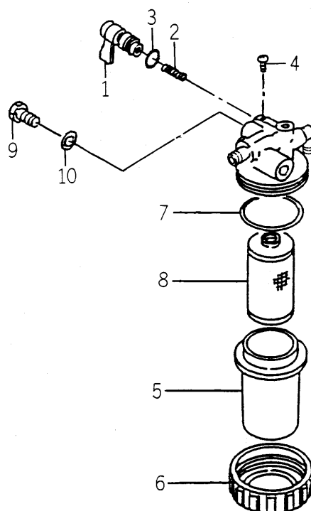
FIG.137 COMPONENT PARTS FOR 1588-105-220-00 ON Fig.4,5
