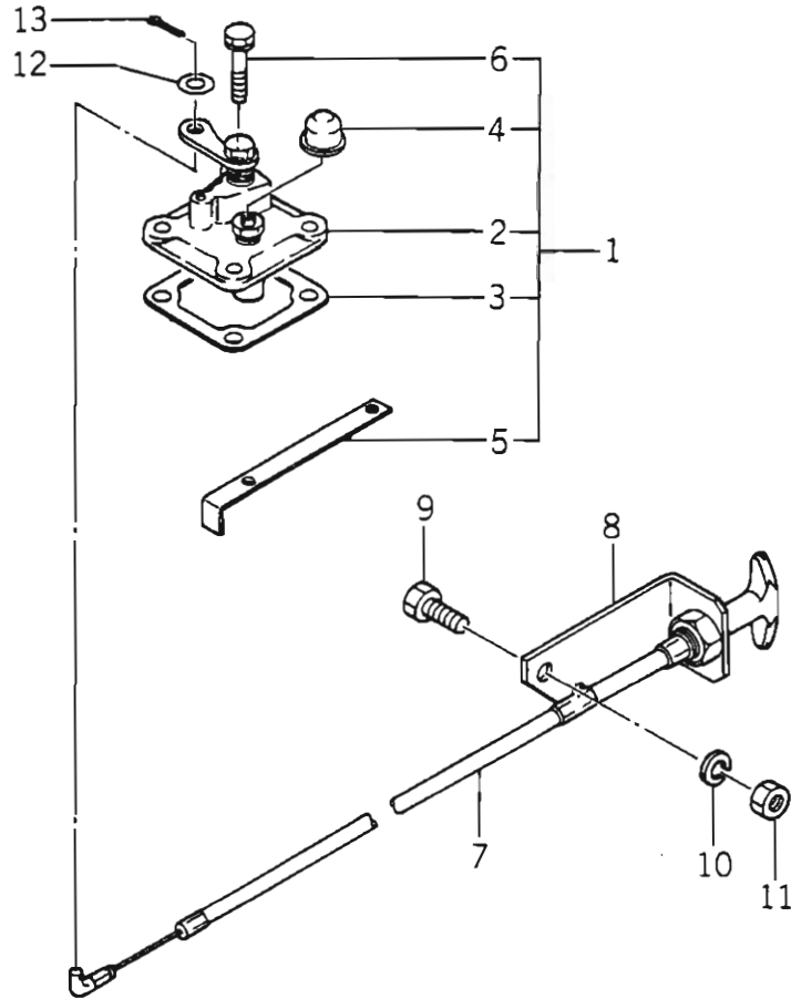
Fig. 61 EMERGENCY STOP LEVER SET (OPTION FOR E20,21,22 40,41.42.43.50,51 52)
