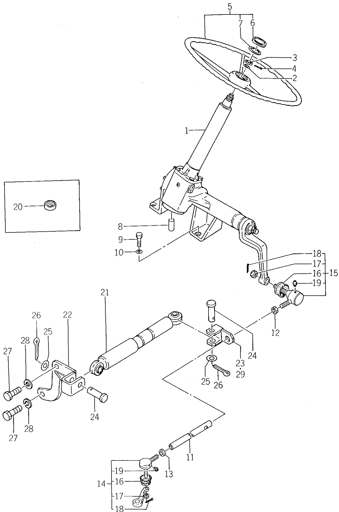
Fig. 35 STEERING WHEEL (MECHANICAL TYPE) (FOR S,D,SG,DG TYPE)
