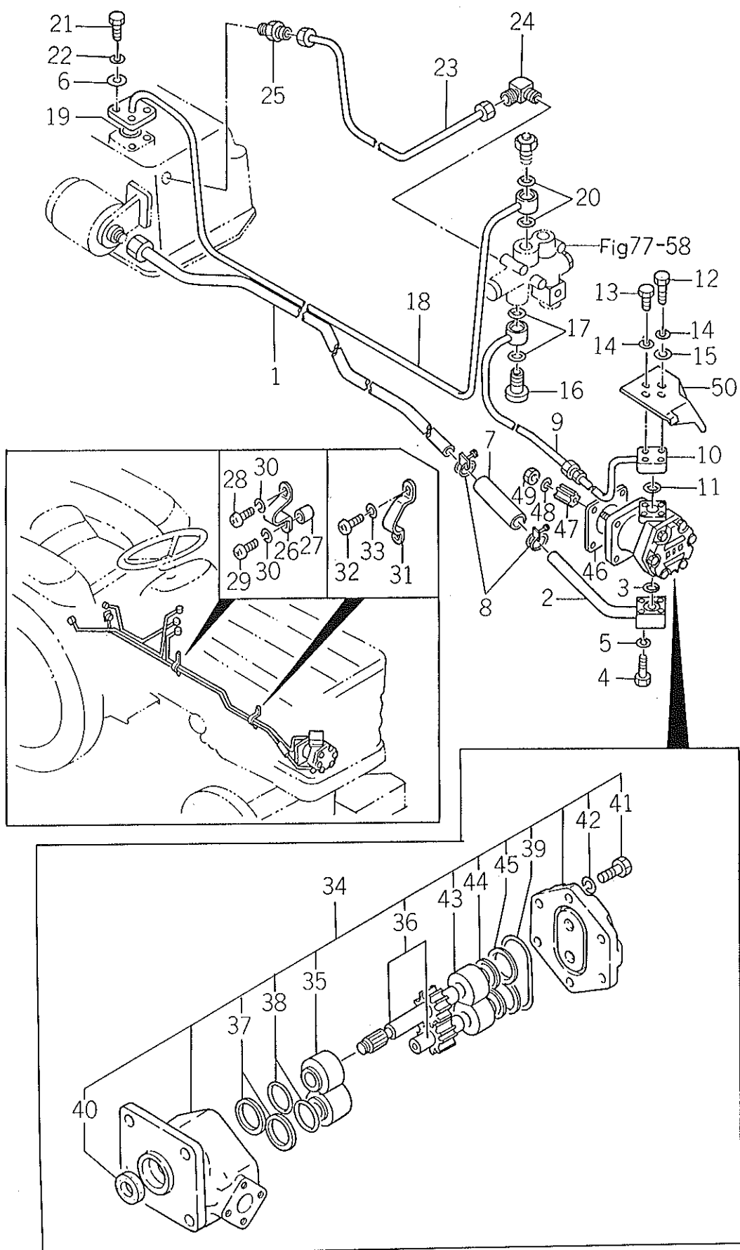
Fig. 65 HYDRAULIC PIPING (FOR DUG, F-UG, F-DUG, LF-DUG TYPE)
