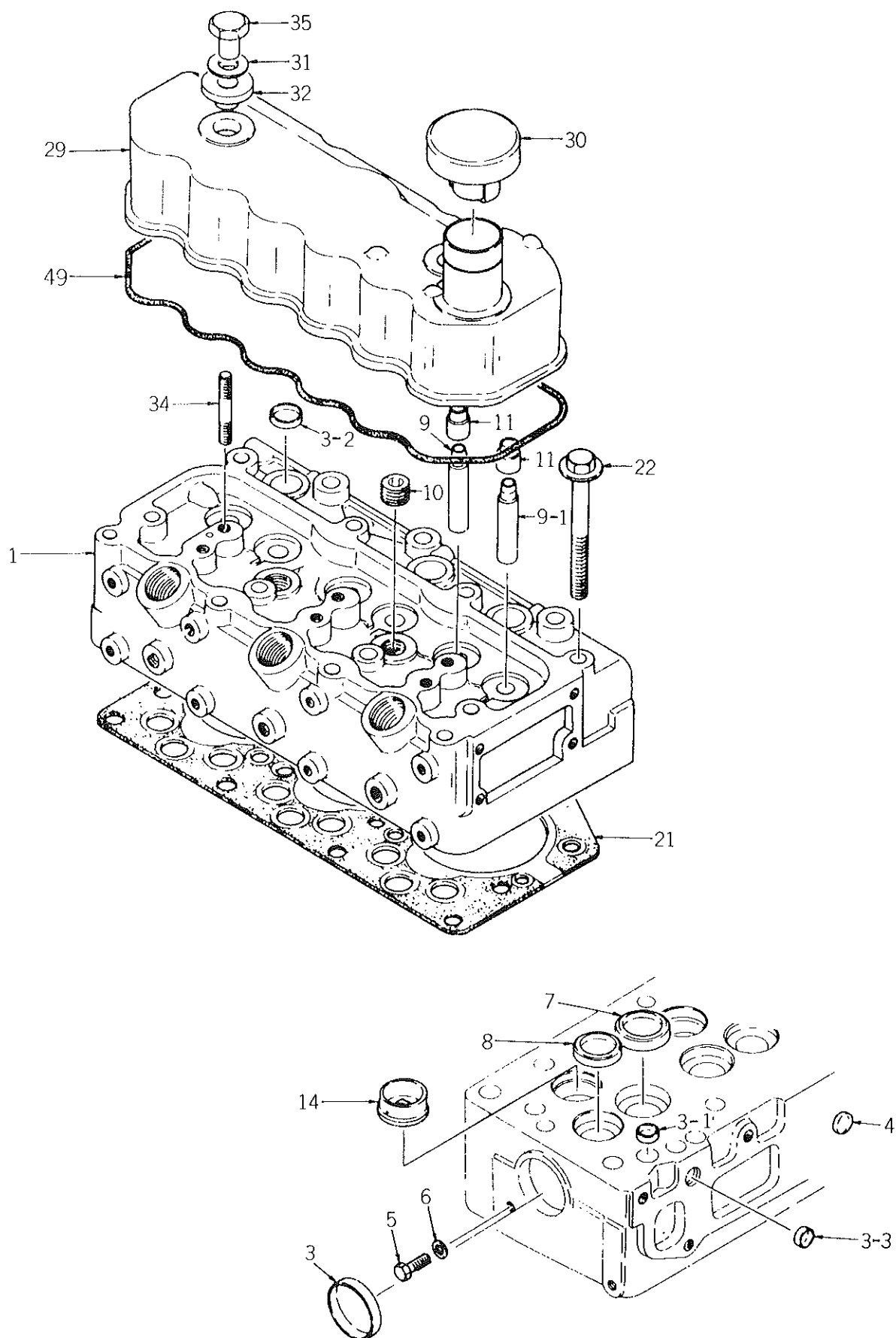
Fig. 1 CYLINDER HEAD AND OTHER PARTS
