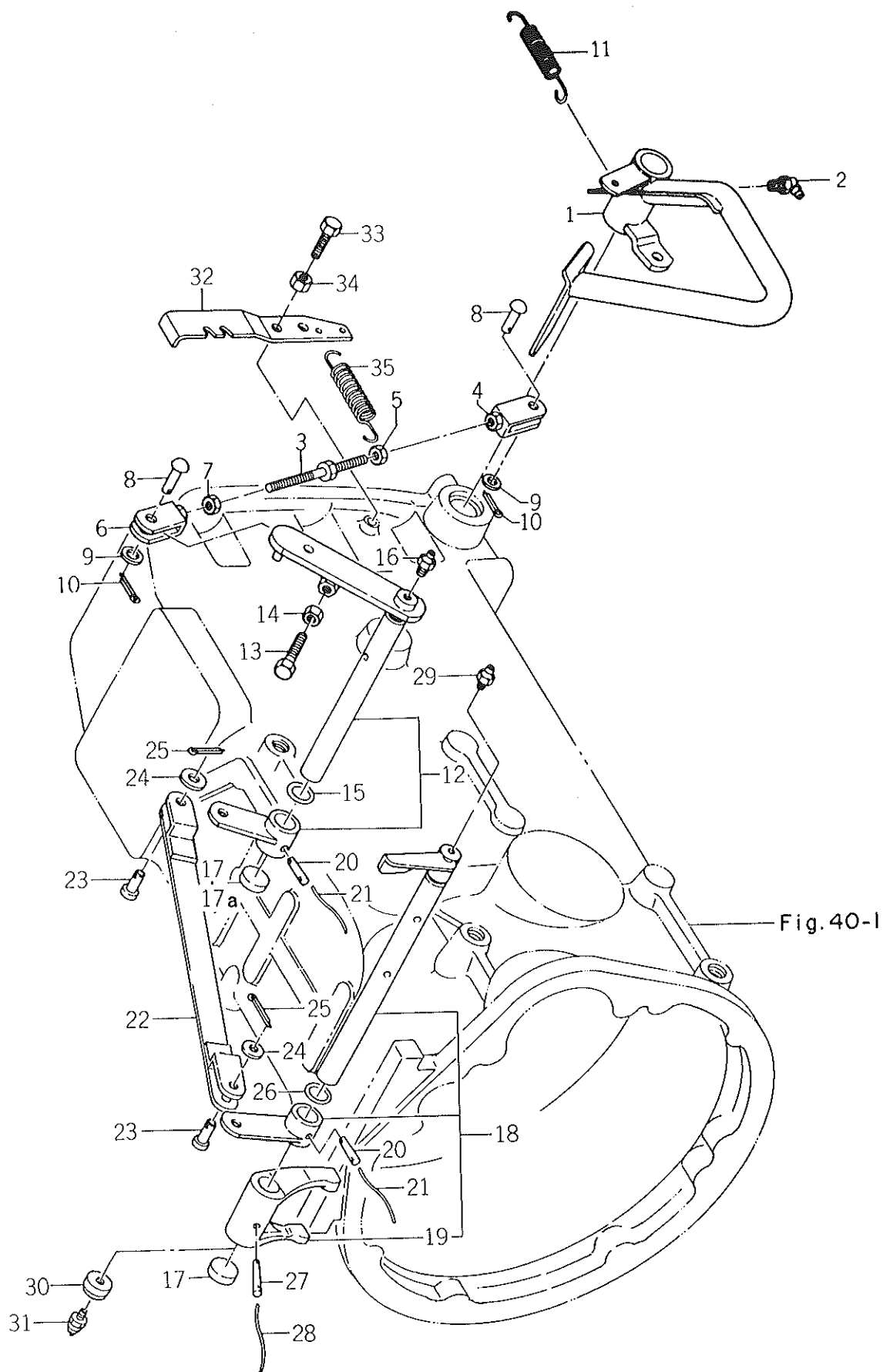
Fig. 45 CLUTCH PEDAL (4WD, CREEP TYPE) (FOR LF-DU, LF-DUG TYPE)
