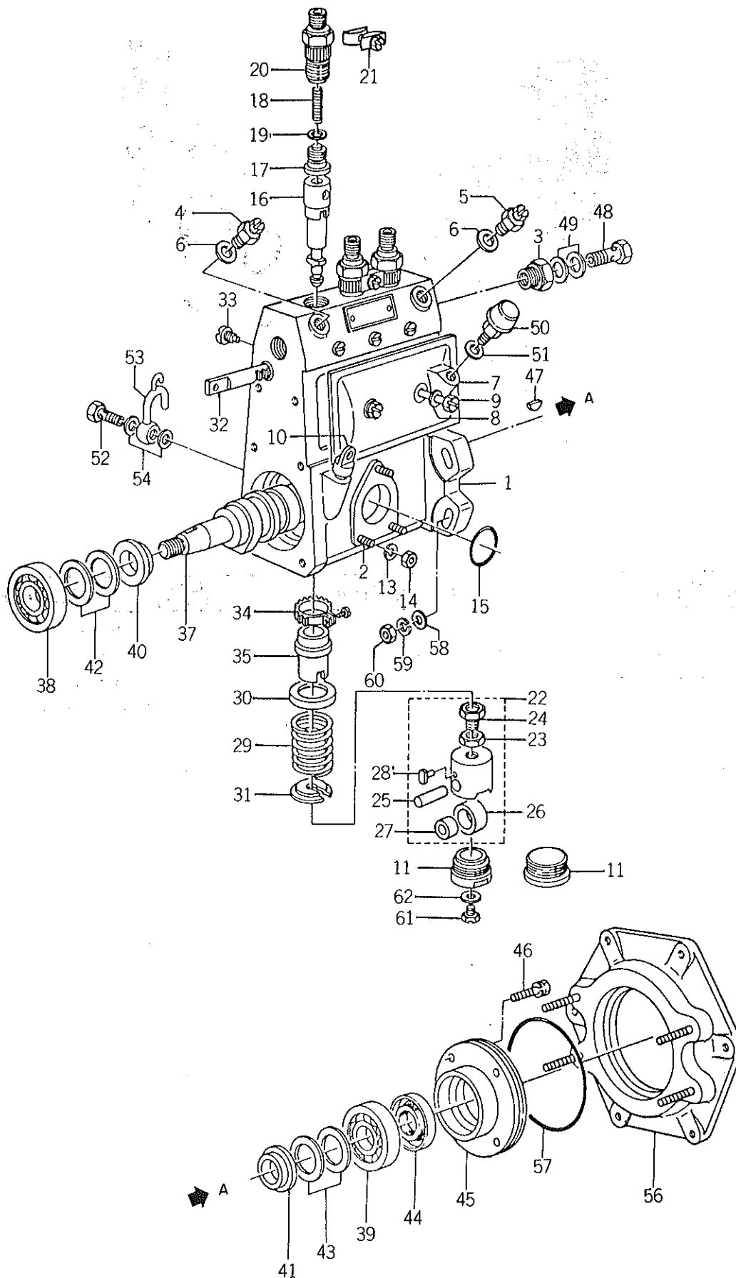
Fig. 17 INJECTION PUMP; PROPER
