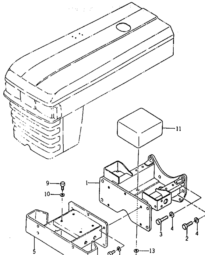
Fig. 27 AXLE BRACKET AND BALANCE WEIGHT (2WD TYPE)
