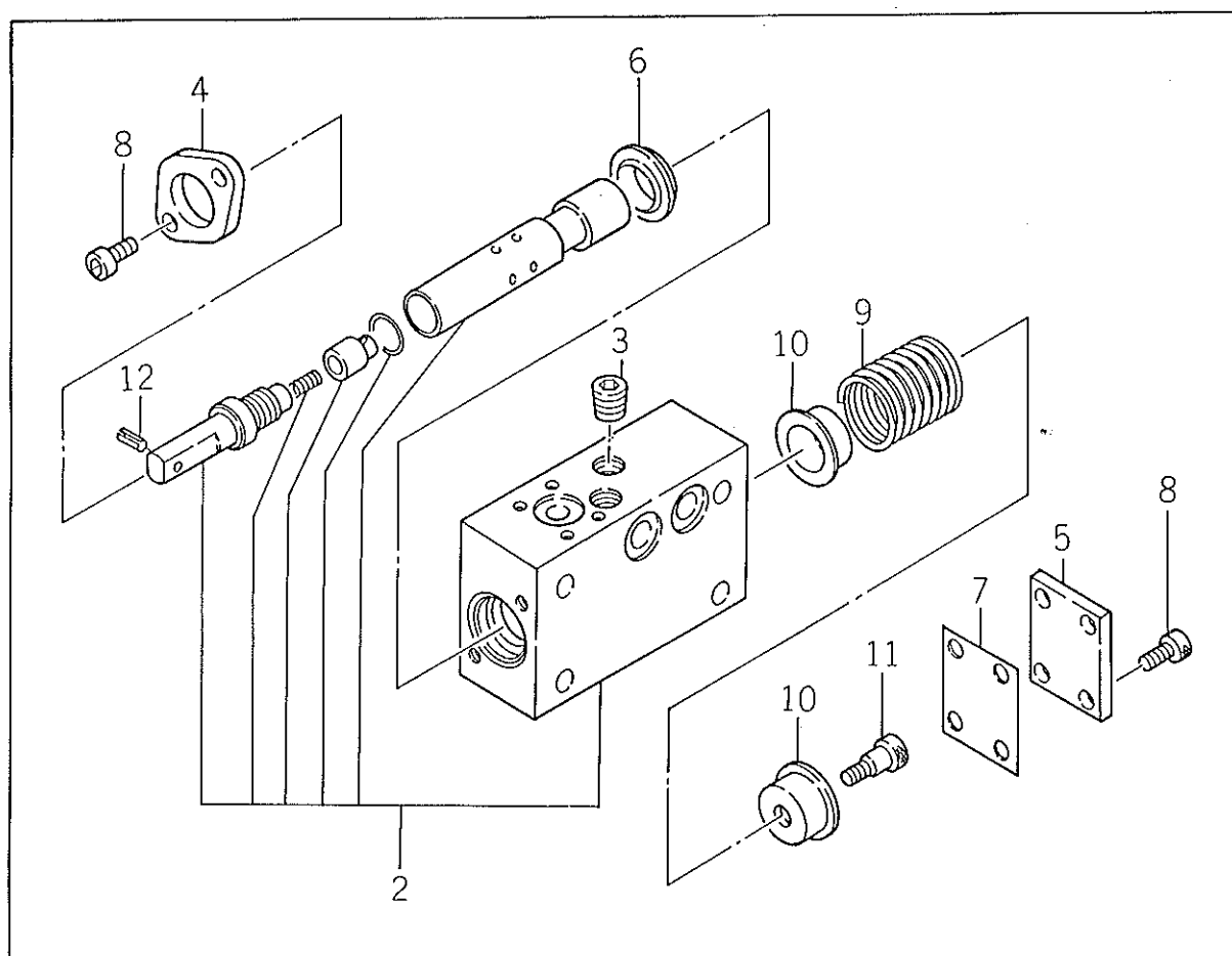
Fig. 81 SUB CONTROL VALVE (OPTION) (FOR SG, DG, DUG, F-UG, F-DUG, LF-DUG TYPE)
