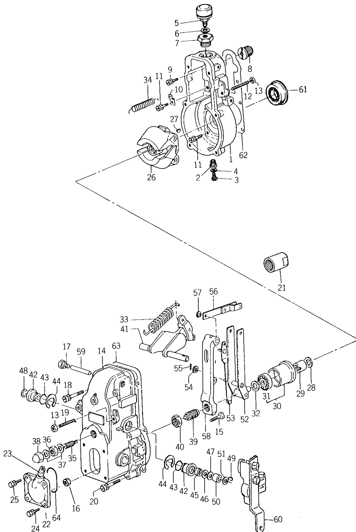
Fig. 18 GOVERNOR (MECHANICAL); INJECTION PUMP
