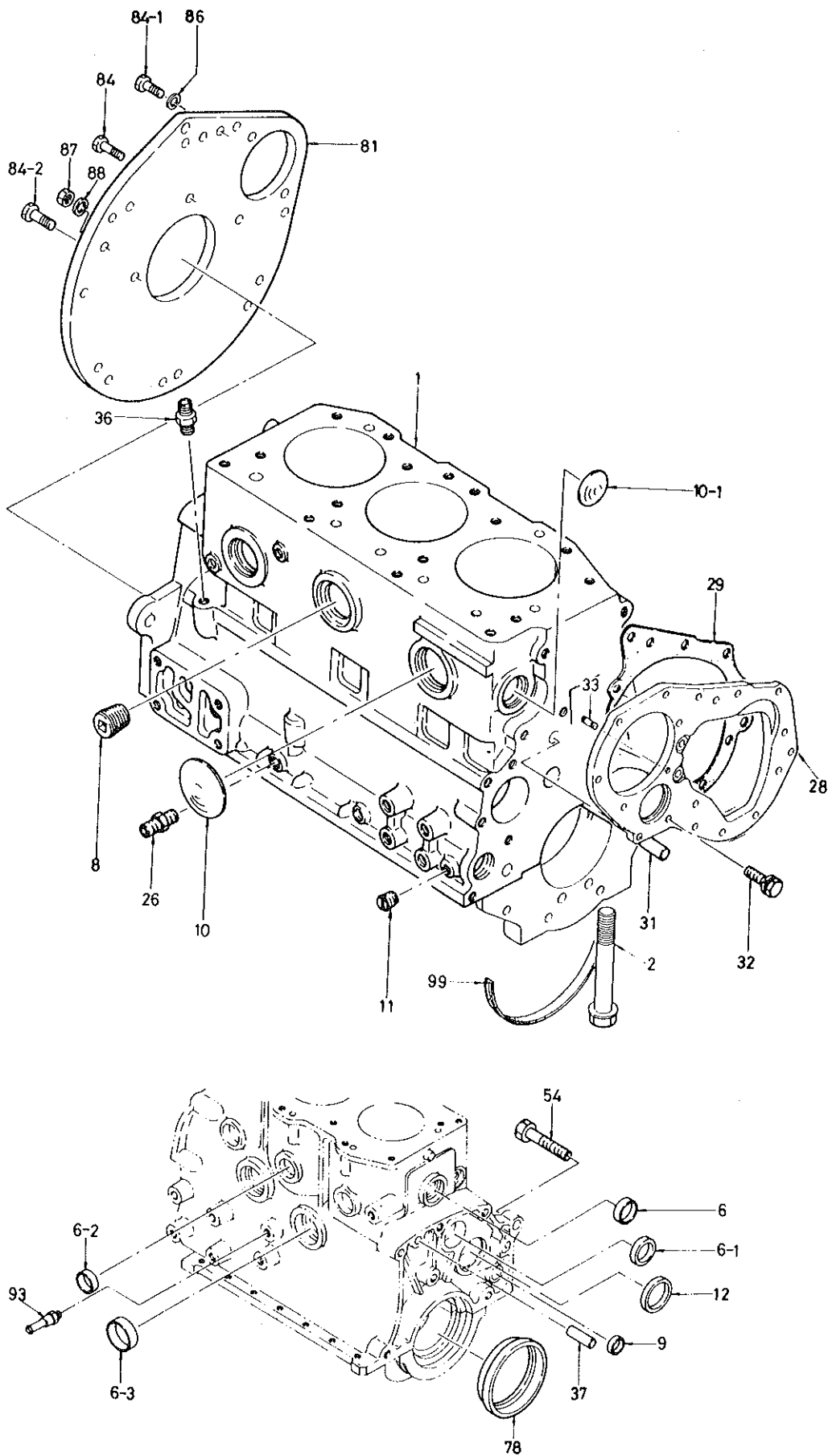
Fig. 2 CYLINDER BLOCK AND OTHER PARTS
