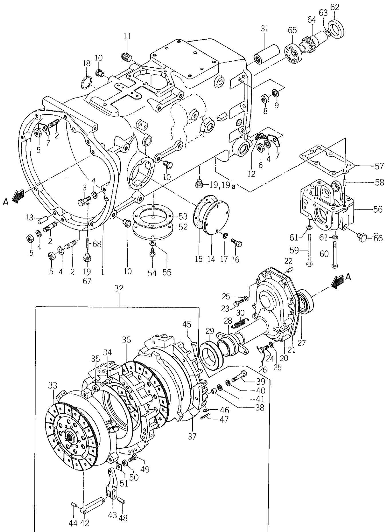
Fig. 40 CLUTCH HOUSING (4WD, CREEP TYPE) (FOR LF-DU, LF-DUG TYPE)
