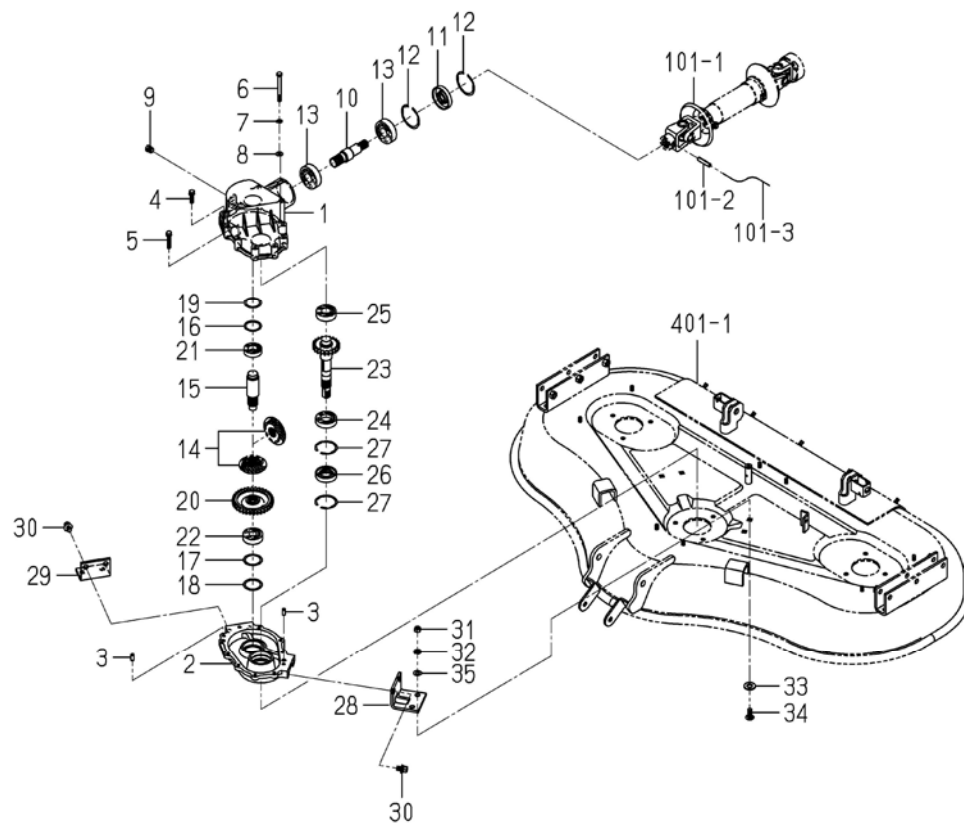
FIG.201 CASE(BEVEL) SYSTEM
