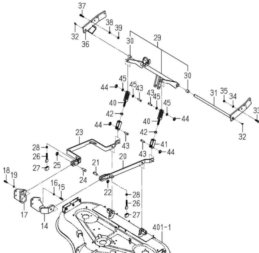
FIG.601 LINK SYSTEM(TM3265)(2/2)
