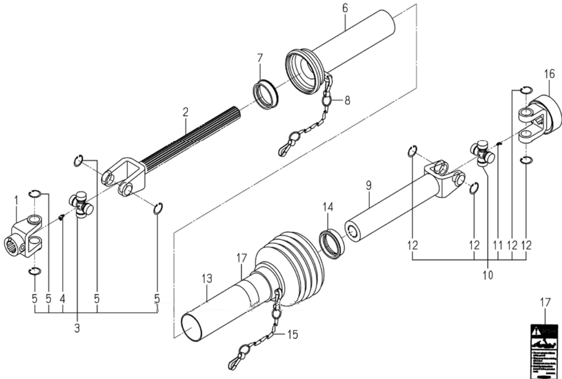
FIG.S01 COMPONENT PARTS FOR 8658-101-820-00 ON Fig.101
