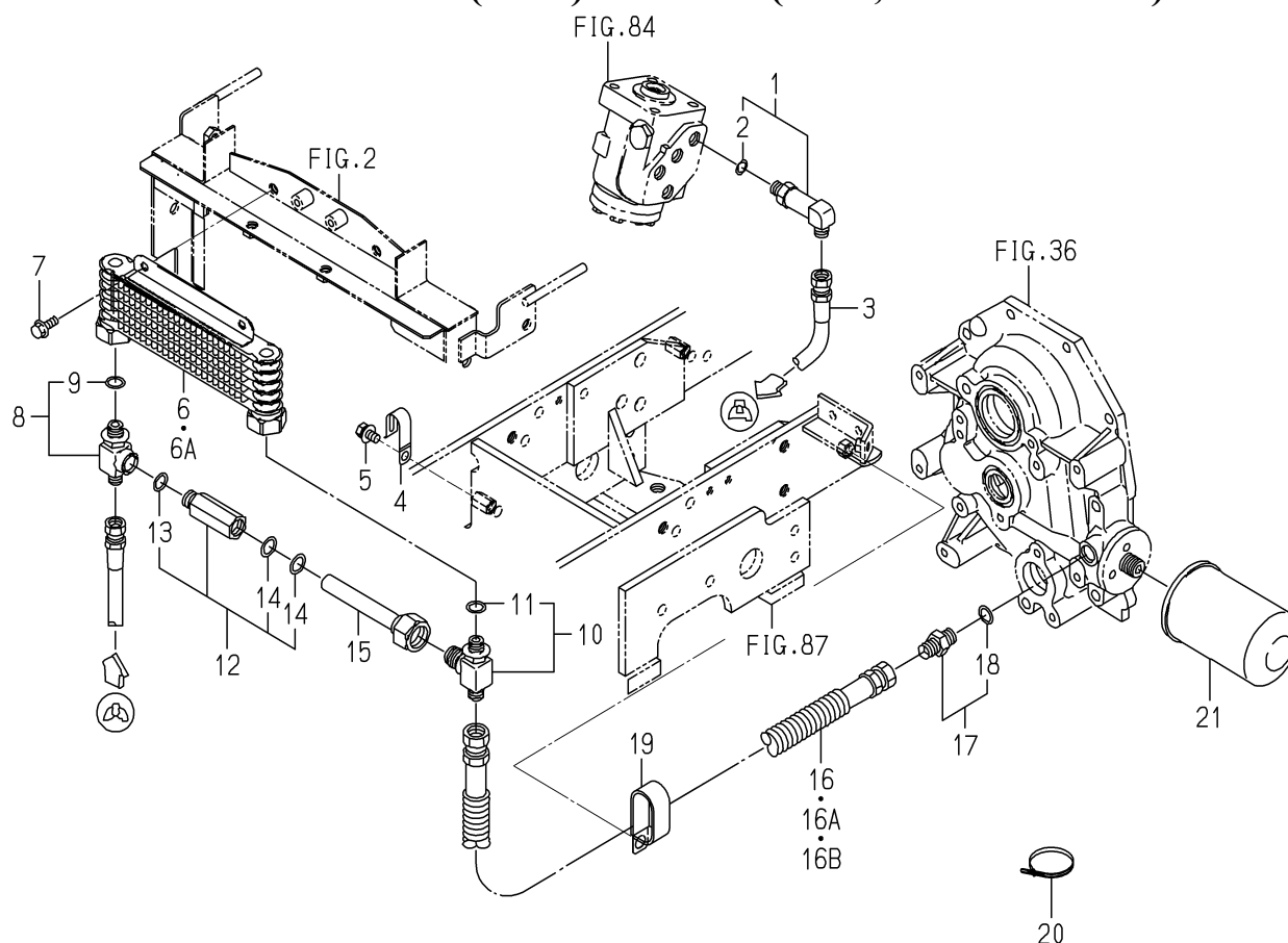
FIG. 65 PIPING(HST)SYSTEM(3215,3245-H TYPE)
