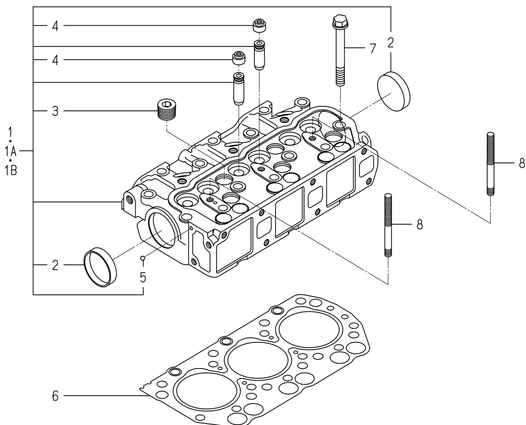
FIG. 2 CYLINDER HEAD
