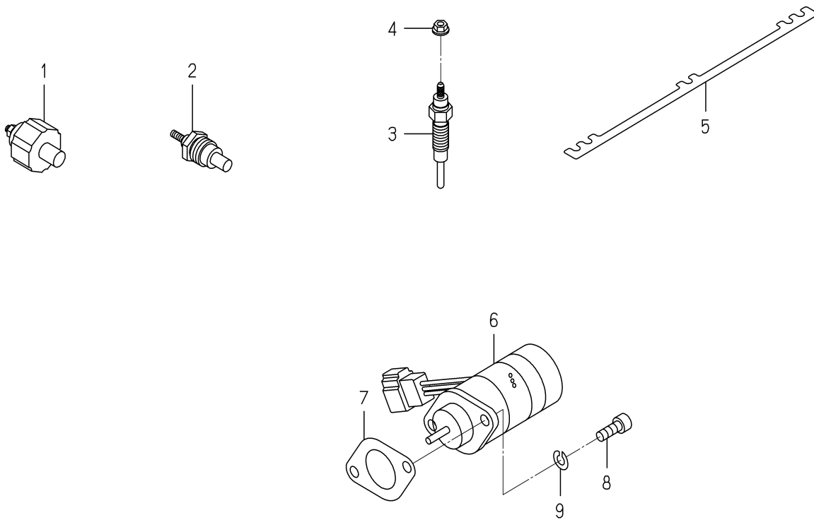
FIG. 27 ELECTRIC (2)
