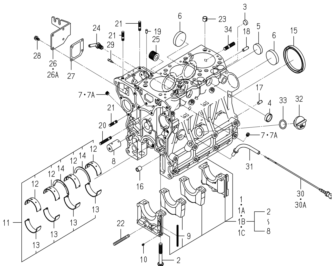
FIG. 7 CYLINDER BLOCK
