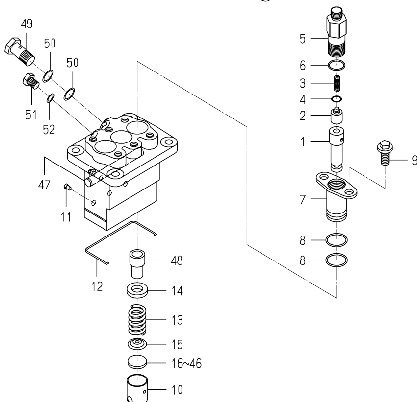
FIG. 31 COMPONENT PARTS FOR 6215-600-155-00 ON Fig.023
