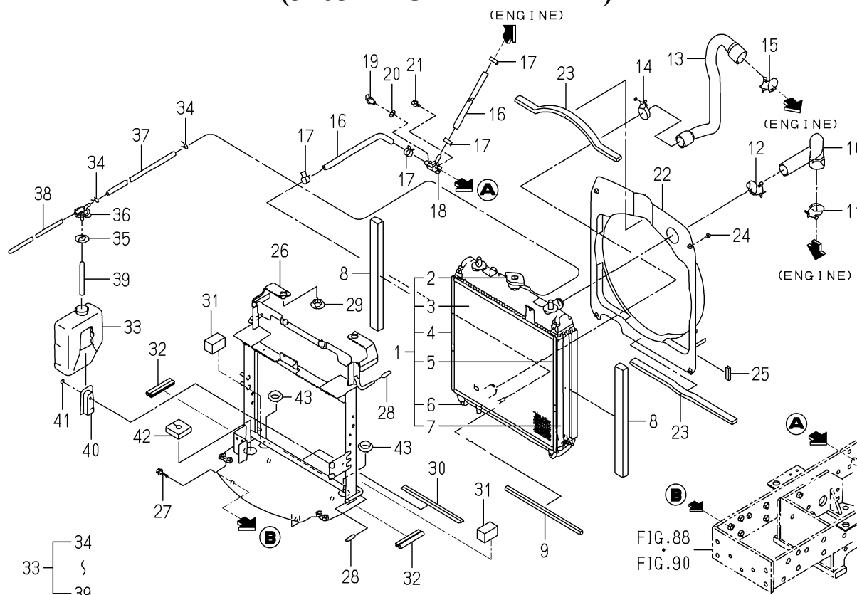
FIG. 3 RADIATOR SYSTEM (3265-EXCEPT H TYPE)
