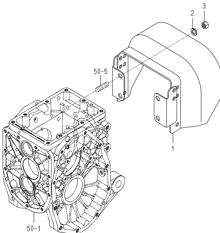
FIG. 46 COVER(SHIELD)SYSTEM(R TYPE) (3215-NO.1-1538/3245-NO.1-351/ 3265-NO.1-887)
