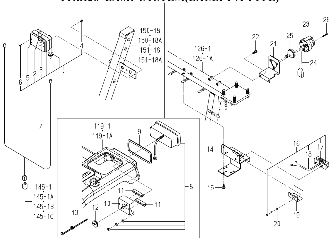
FIG.138 LAMP SYSTEM(EXCEPT A TYPE)
