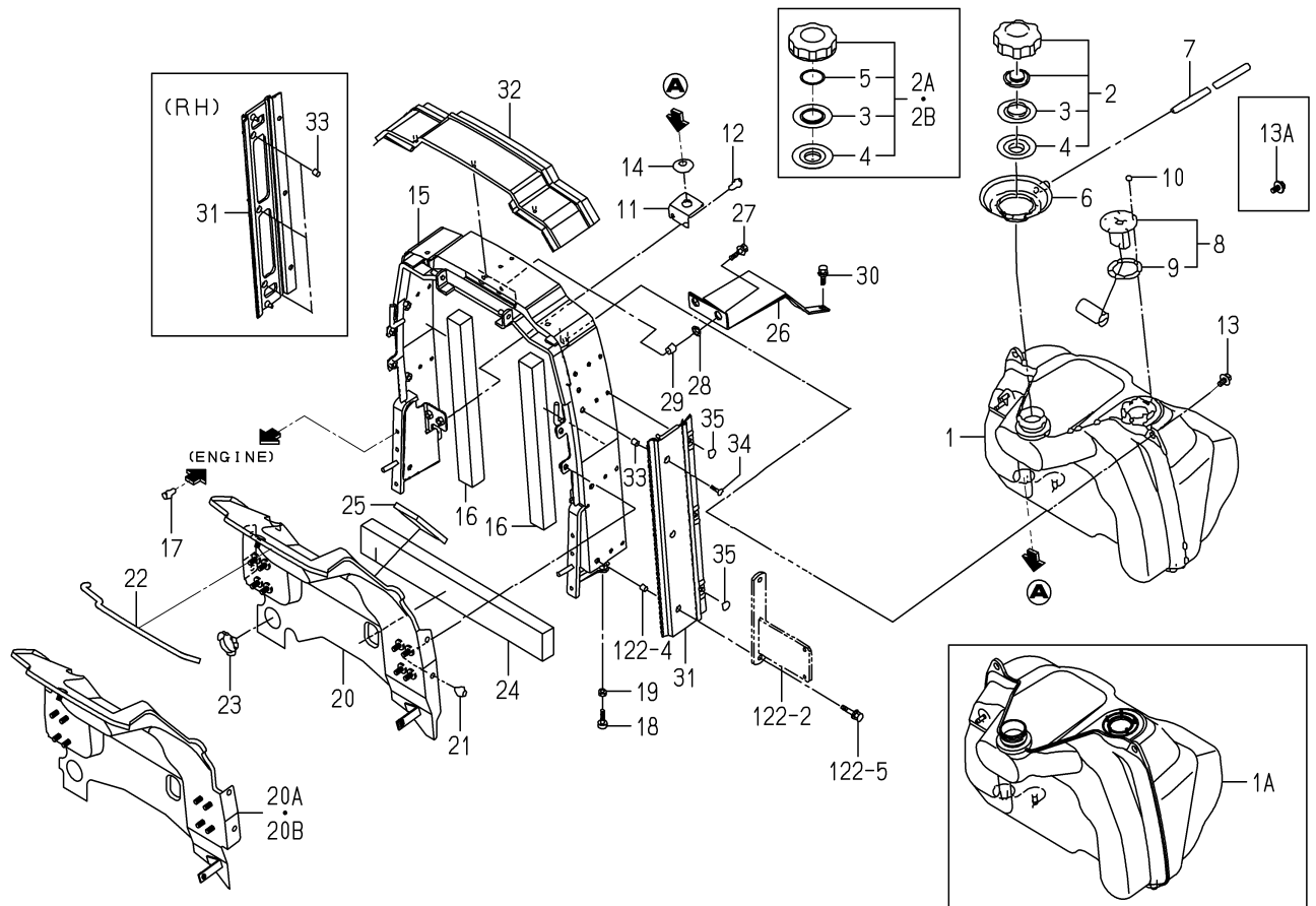
FIG. 11 TANK(FUEL)SYSTEM(3265-NO.1-62)
