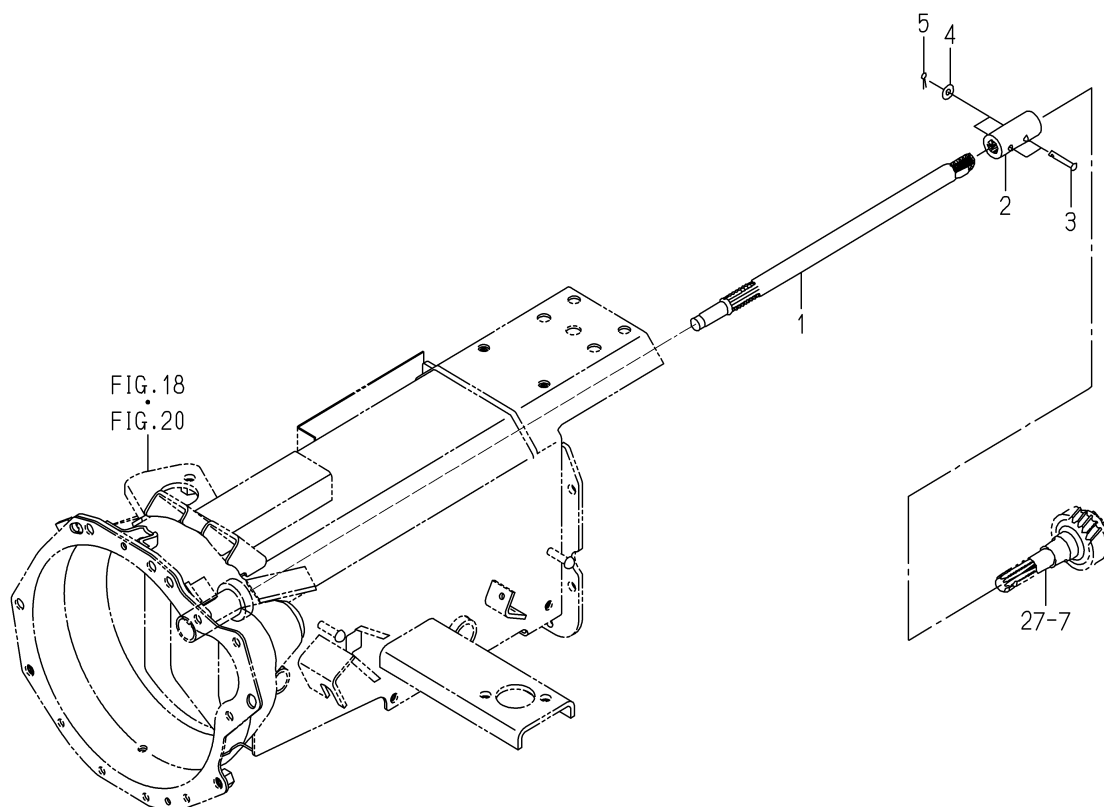
FIG. 25 SHAFT(INPUT)SYSTEM (EXCEPT H TYPE)
