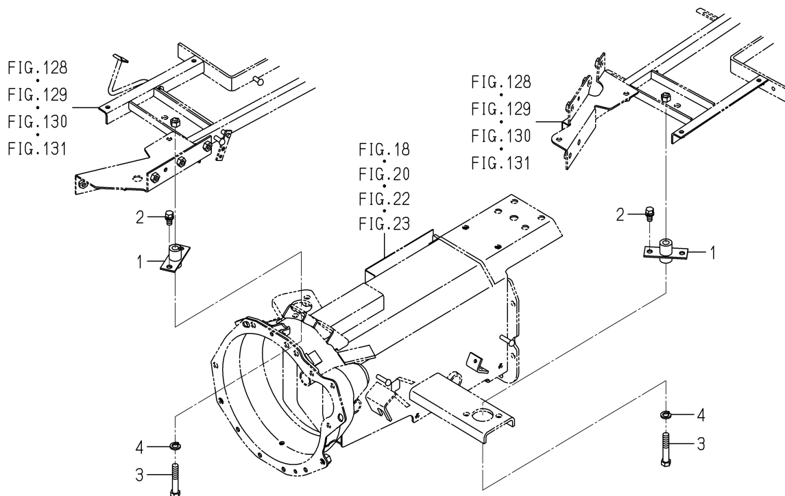
FIG.125 MOUNT(FRONT)SYSTEM(D TYPE) (3215-NO.1907-/3245-NO.390-/3265-NO.1090-)
