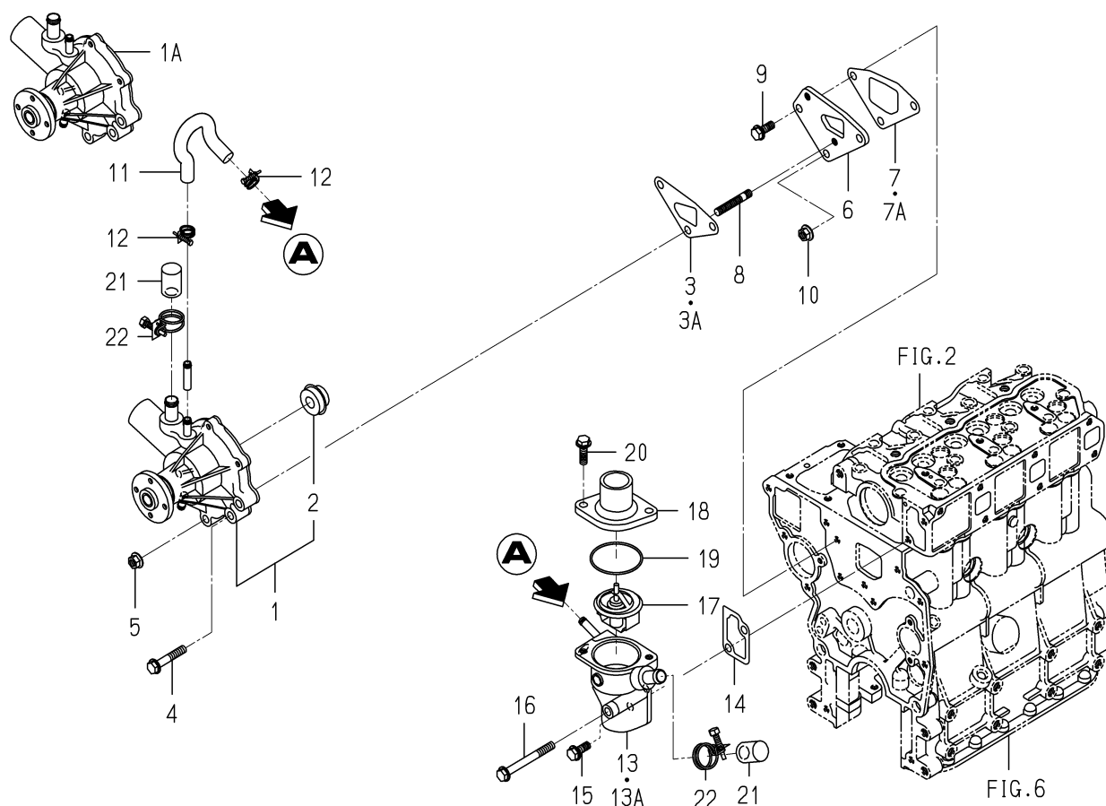
FIG. 18 WATER PUMP
