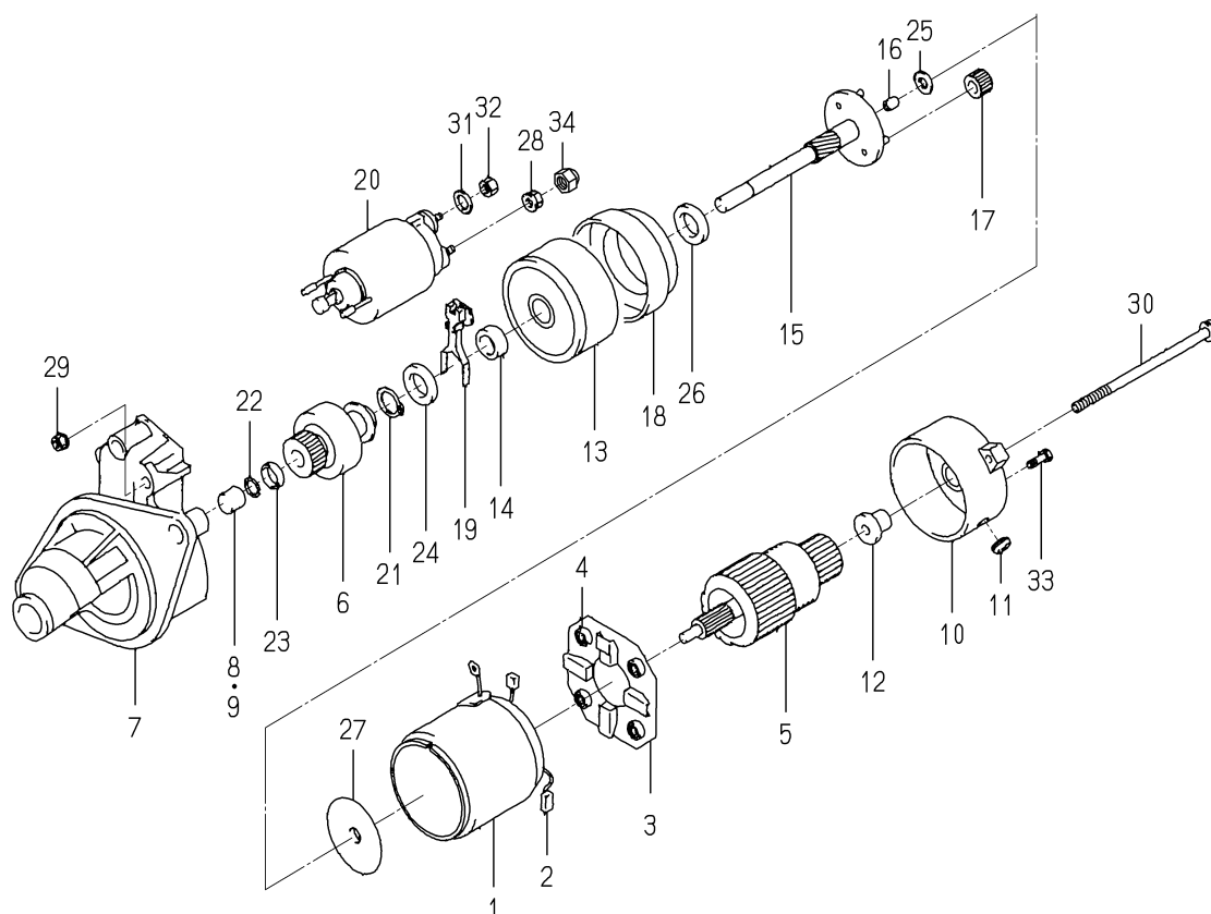
FIG. 30 COMPONENT PARTS FOR 6281-100-014-00 ON Fig.024
