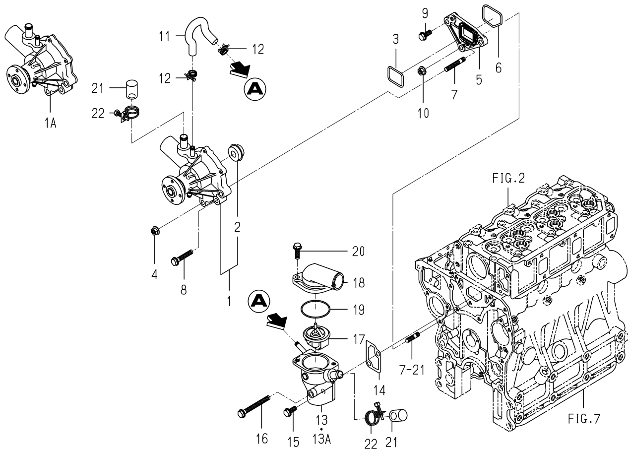
FIG. 20 WATER PUMP
