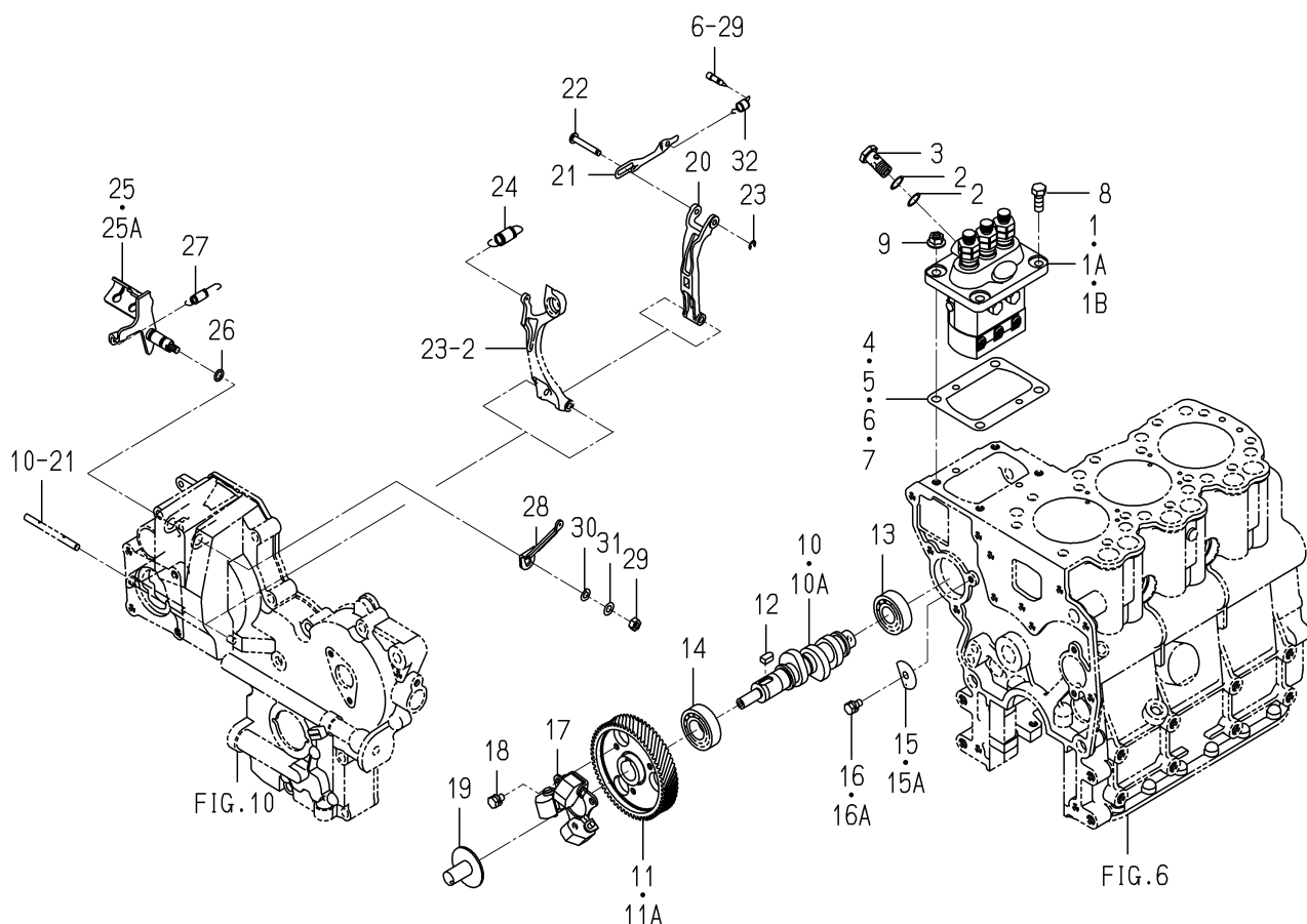
FIG. 21 INJECTION PUMP
