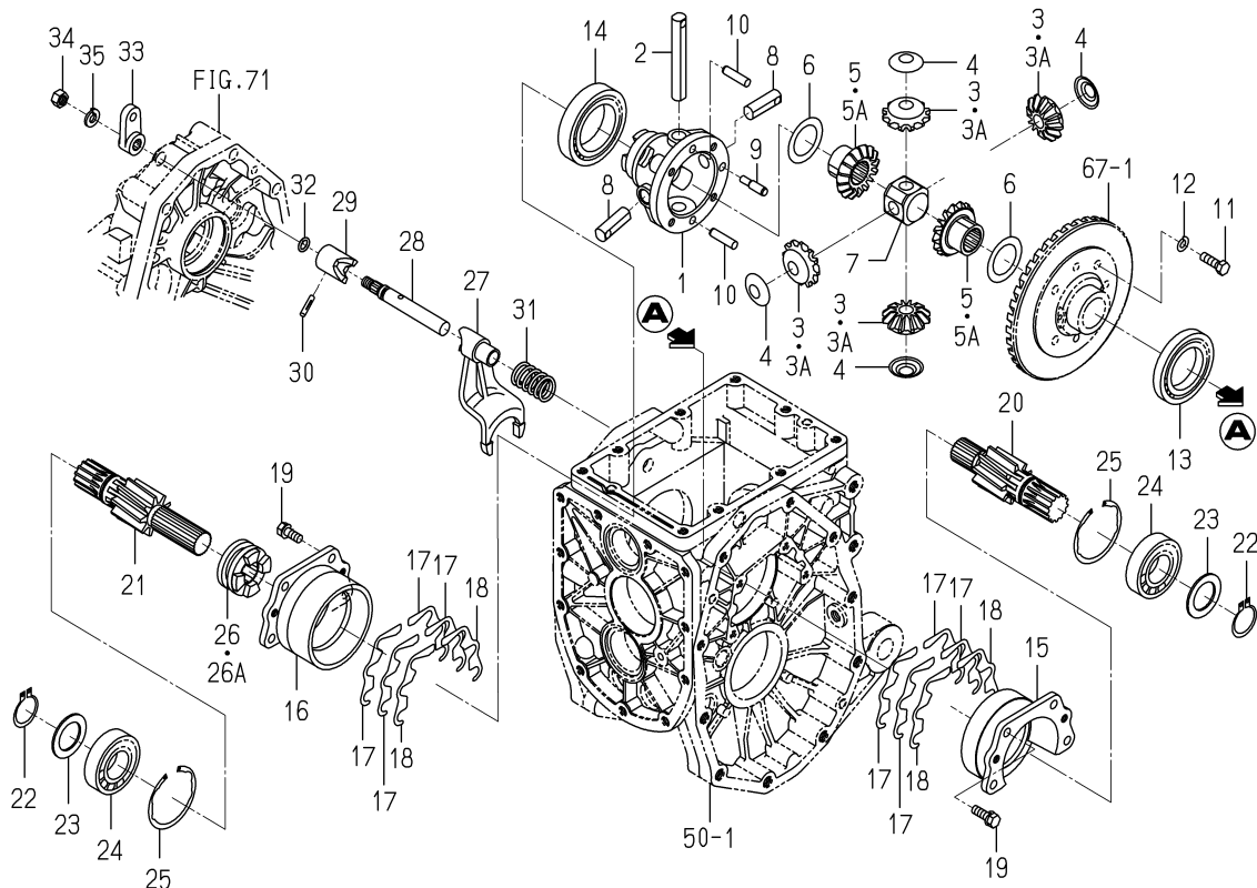
FIG. 69 CASE (DIFFERENTIAL GEAR/REAR)SYSTEM (EXCEPT H TYPE)
