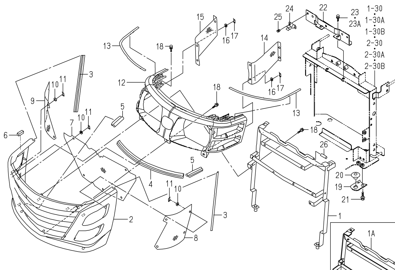
FIG.115 GRILLE SYSTEM(3215,3245)
