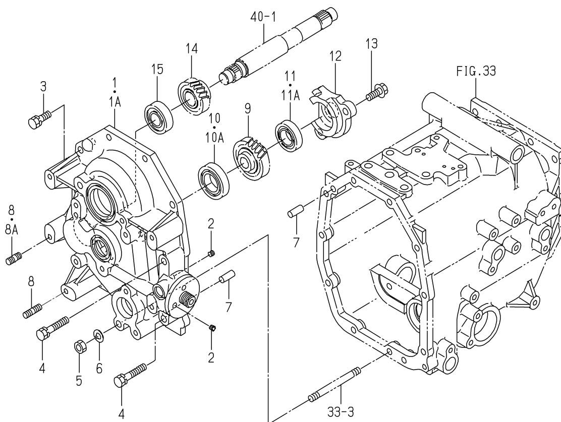
FIG. 36 GEAR(INPUT/HST)SYSTEM(H TYPE)
