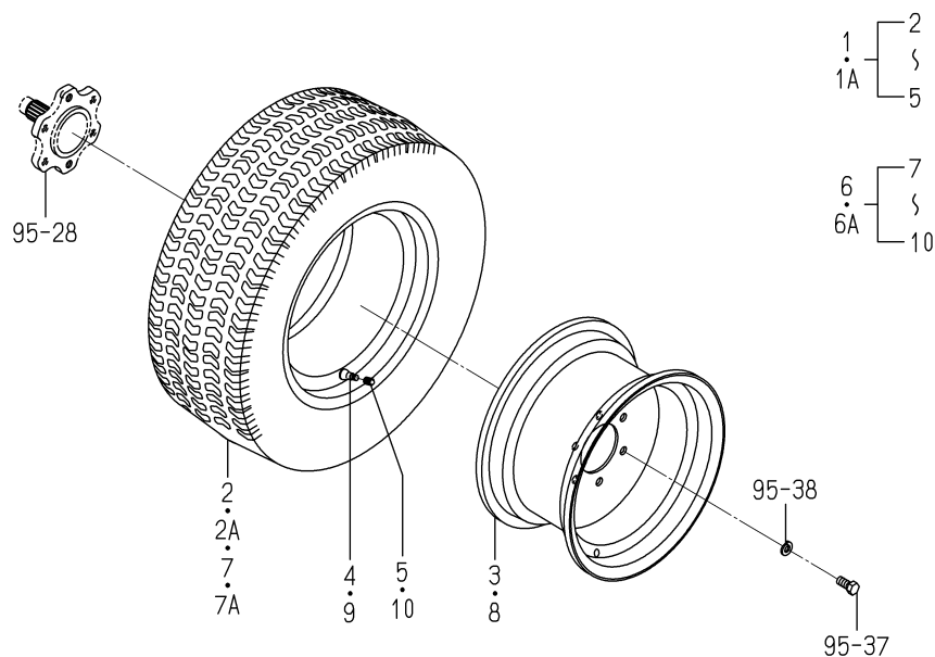
FIG.172 WHEEL (FRONT/22X8.50-12-4)SYSTEM (3215/3245,3265-A TYPE)(OPTION)
