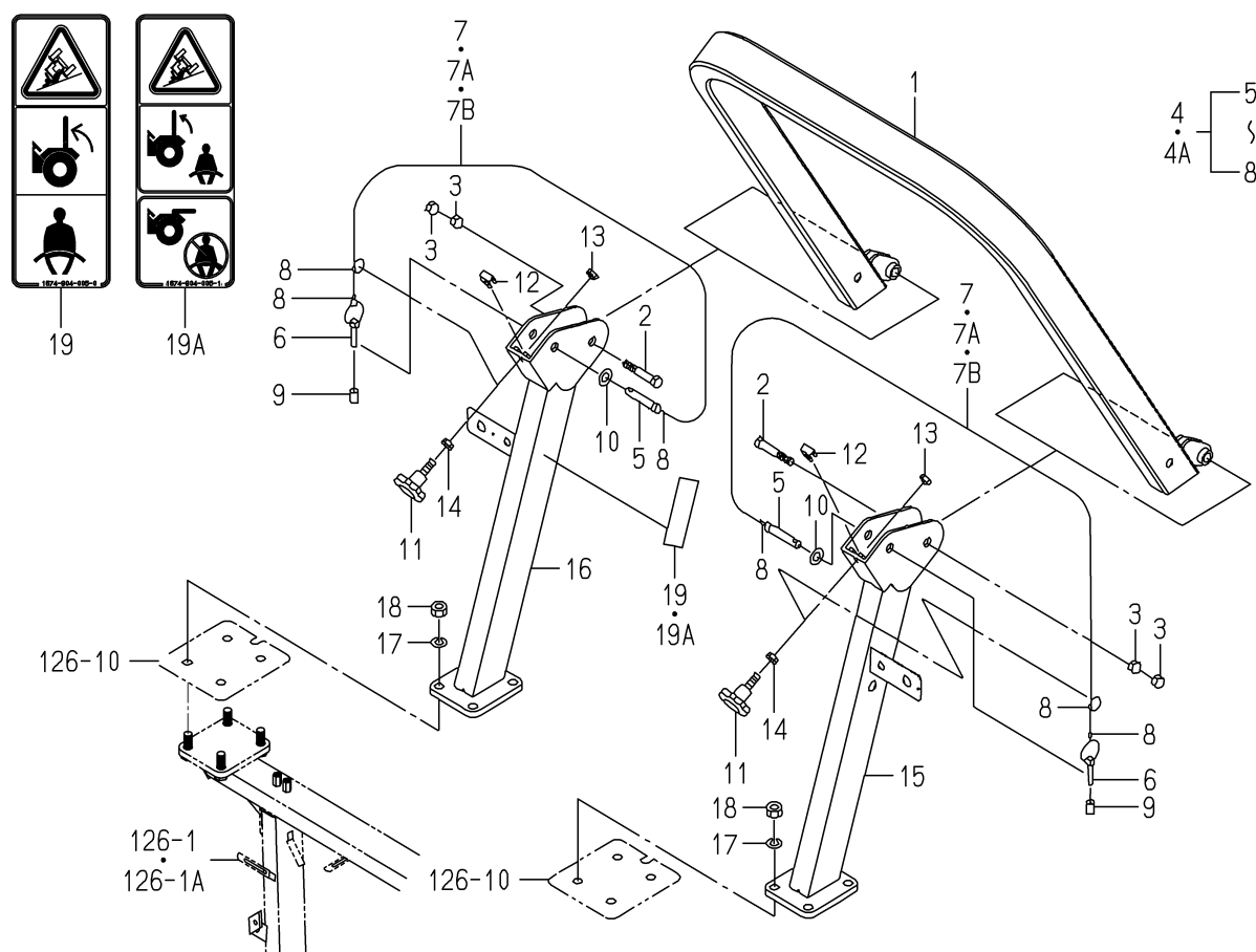
FIG.149 ROPS SYSTEM(R TYPE EXCEPT A)
