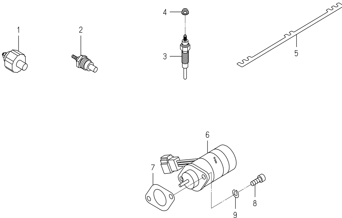
FIG. 27 ELECTRIC (2)
