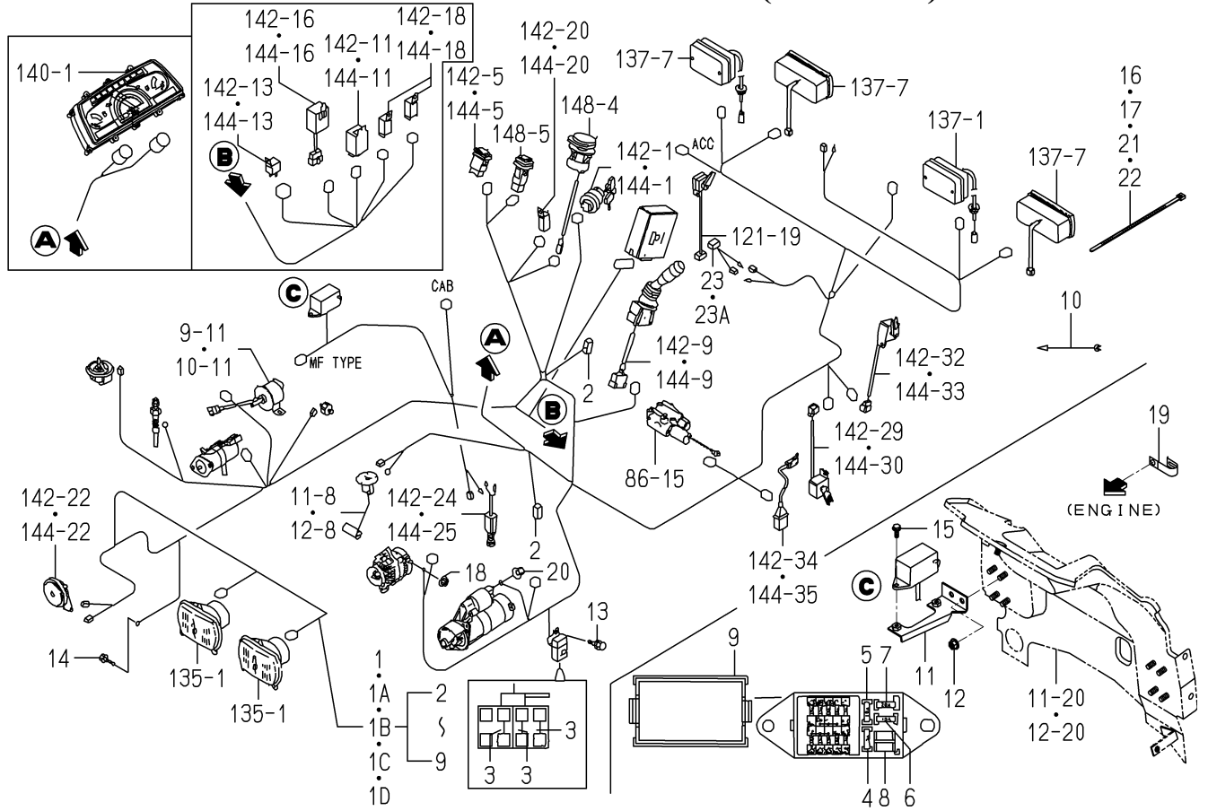
FIG.147 HARNESS SYSTEM(E6 TYPE)
