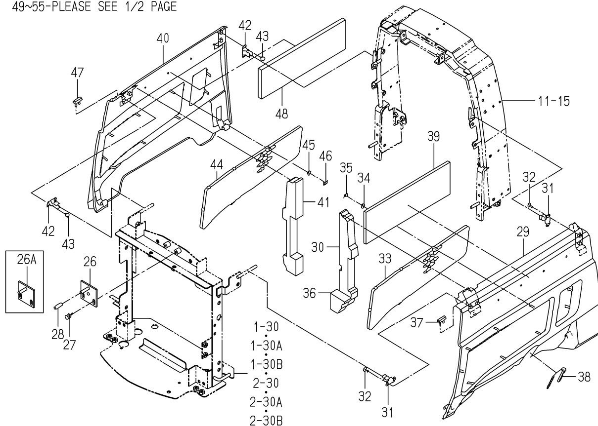
FIG.113 HOOD SYSTEM(3215,3245)(2/2)
