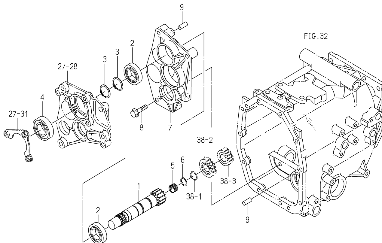
FIG. 35 GEAR(INPUT)SYSTEM(EXCEPT H TYPE)
