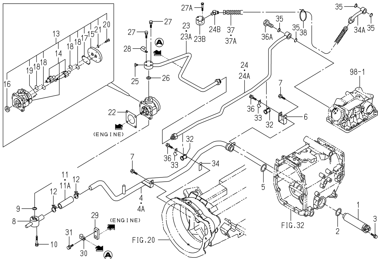
FIG.106 PIPING(MAIN)SYSTEM (3265-EXCEPT H TYPE)
