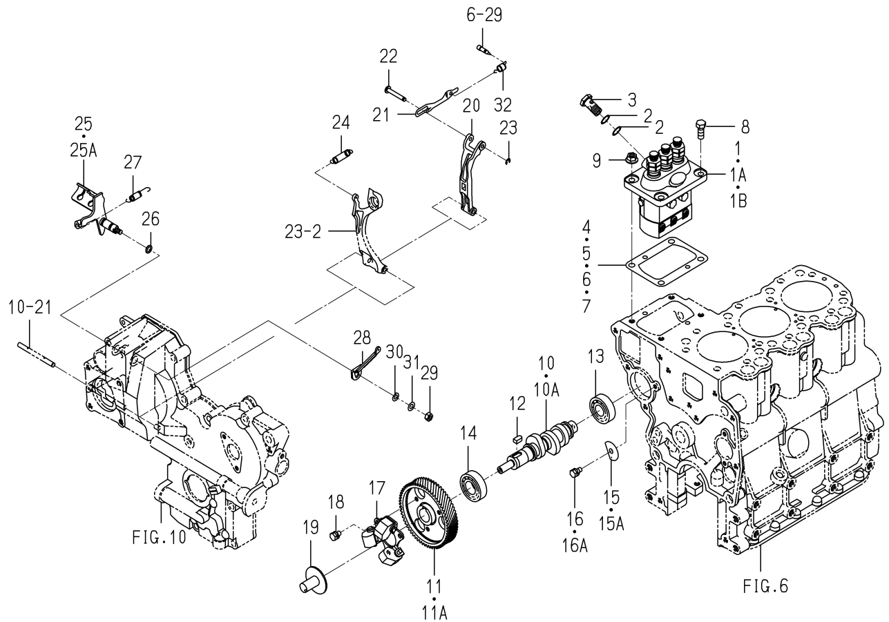
FIG. 21 INJECTION PUMP
