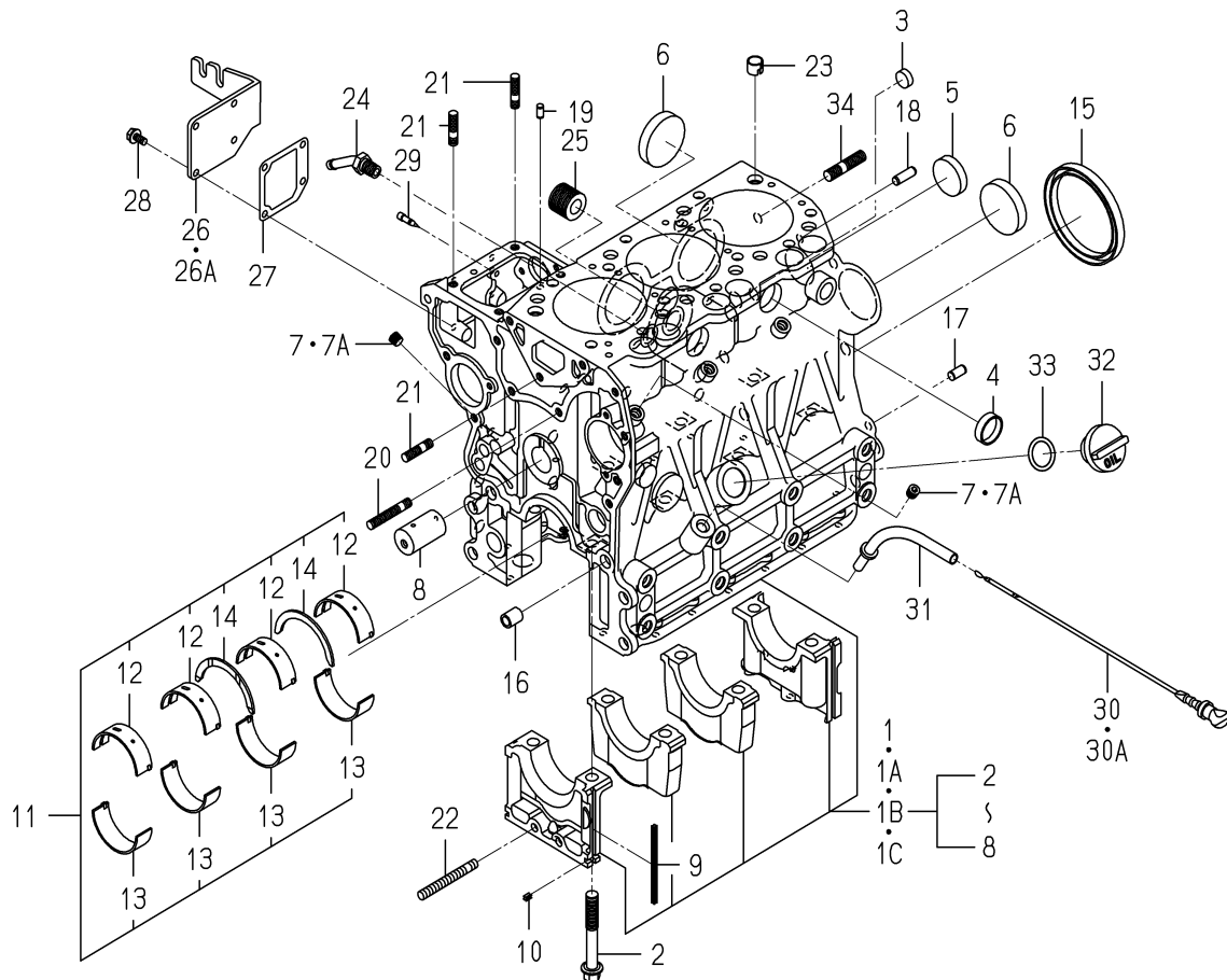
FIG. 7 CYLINDER BLOCK
