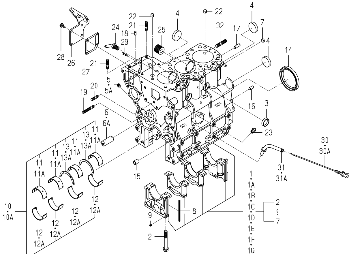
FIG. 6 CYLINDER BLOCK
