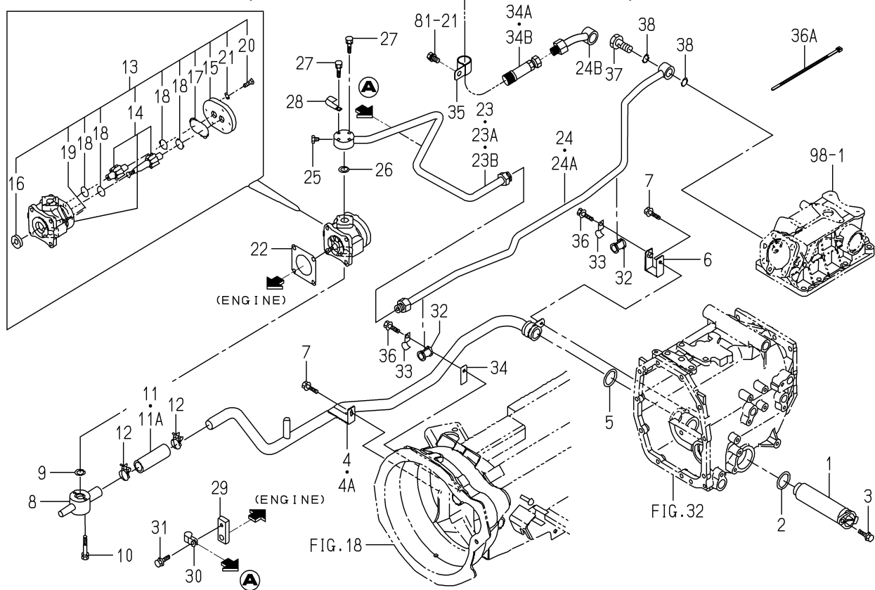
FIG.108 PIPING(MAIN)SYSTEM (3215,3245-EXCEPT H TYPE)
