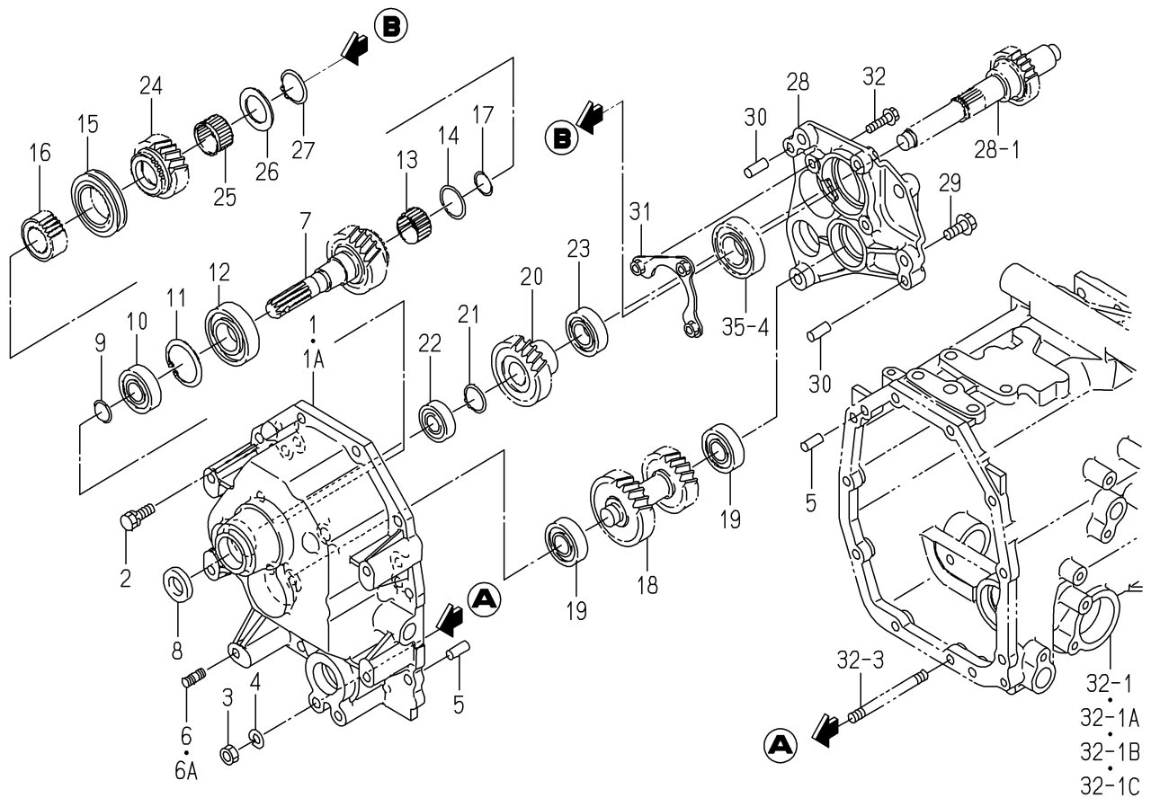
FIG. 27 GEAR(DRIVE)SYSTEM(EXCEPT H TYPE)
