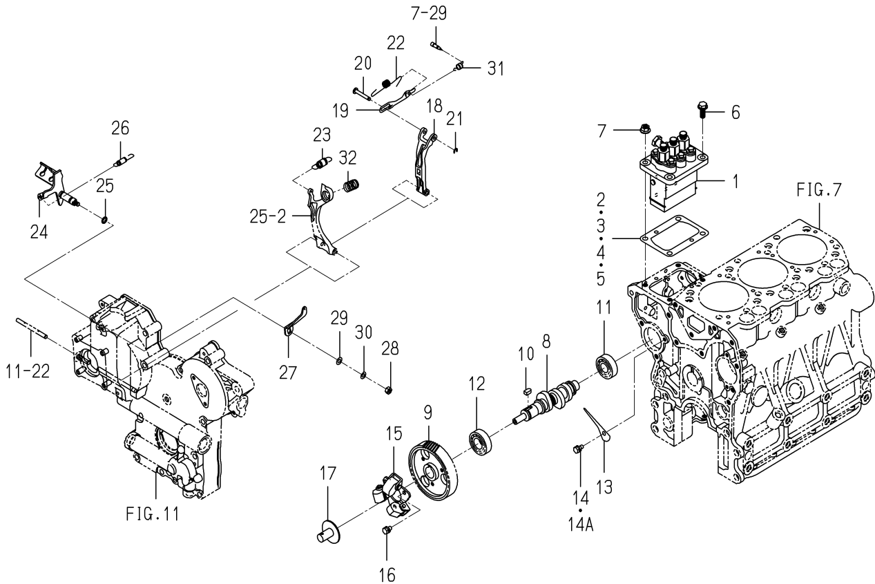
FIG. 23 INJECTION PUMP
