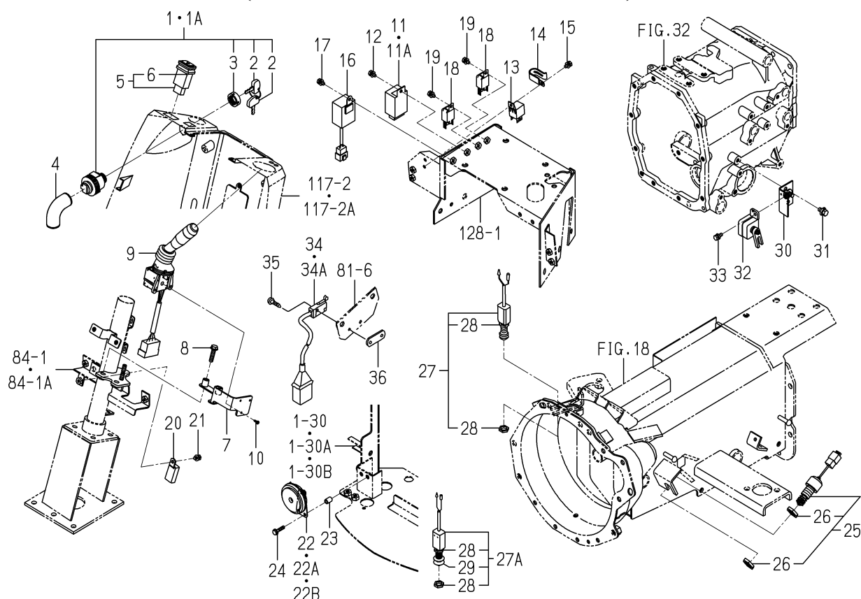
FIG.143 SWITCH SYSTEM (3215,3245-EXCEPT H TYPE)
