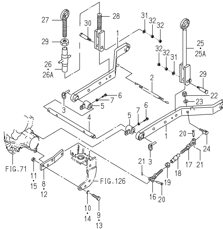
FIG.111 LINK(3P)SYSTEM(EXCEPT R TYPE) (3215-NO.1-1906/3245-NO.1-389/ 3265-NO.1-1089)
