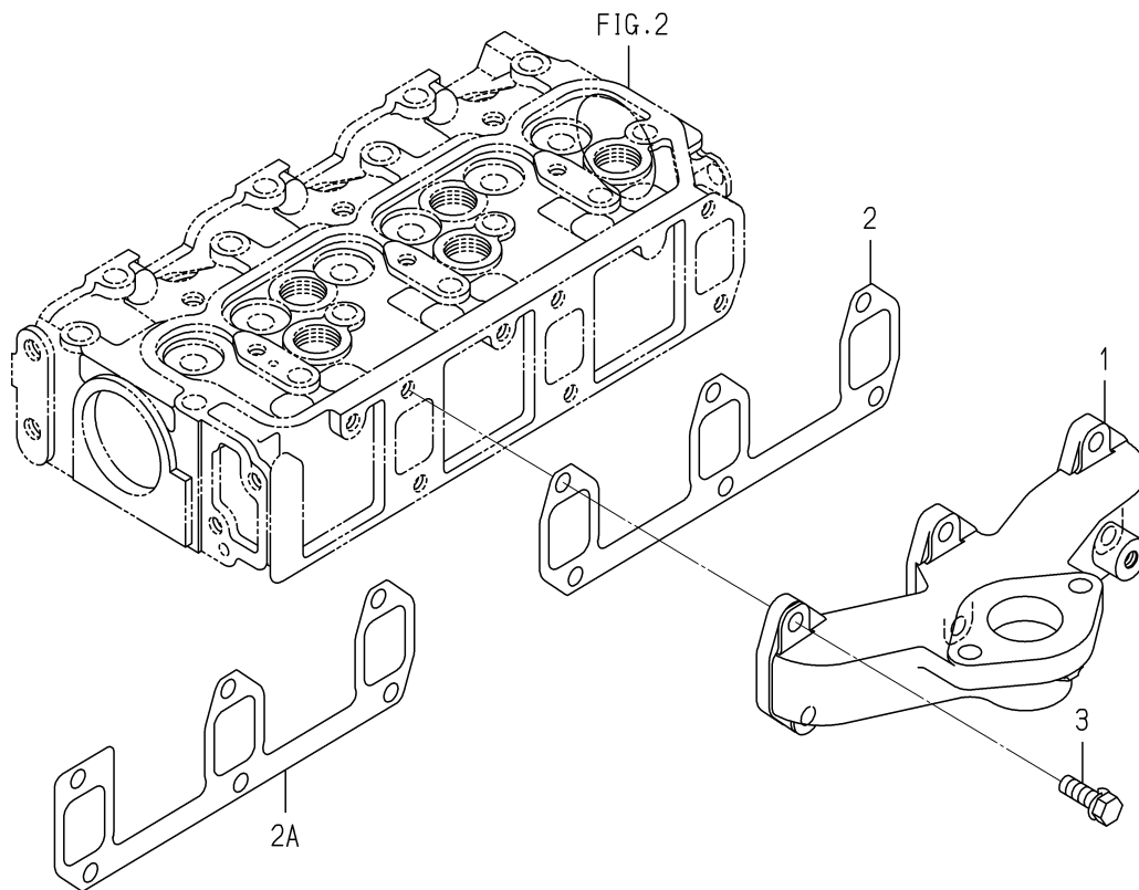
FIG. 6 EXHAUST MANIFOLD
