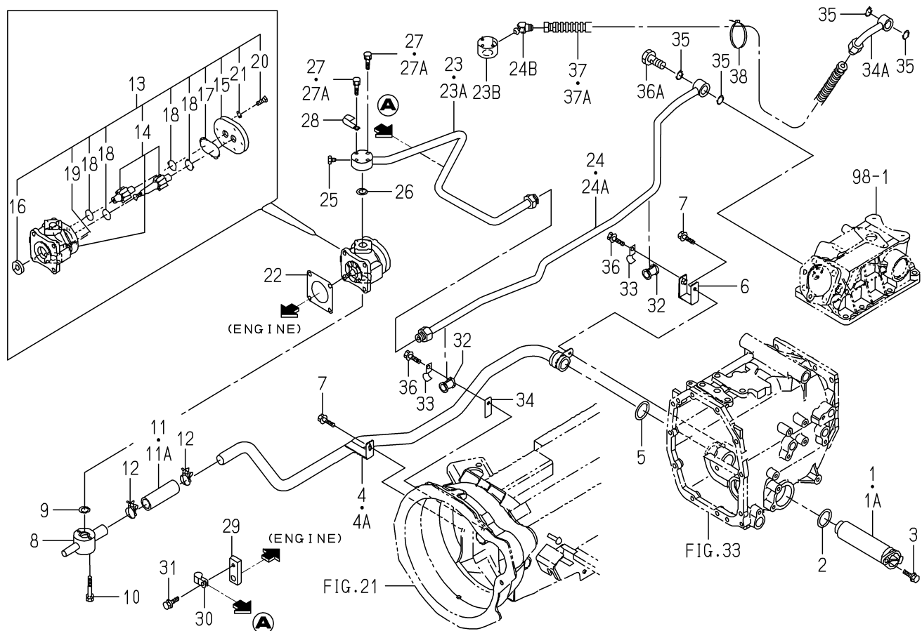
FIG.107 PIPING(MAIN)SYSTEM(3265-H TYPE)
