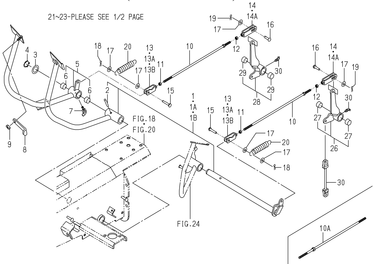
FIG. 78 PEDAL(BRAKE)SYSTEM(1/2) (EXCEPT H TYPE)
