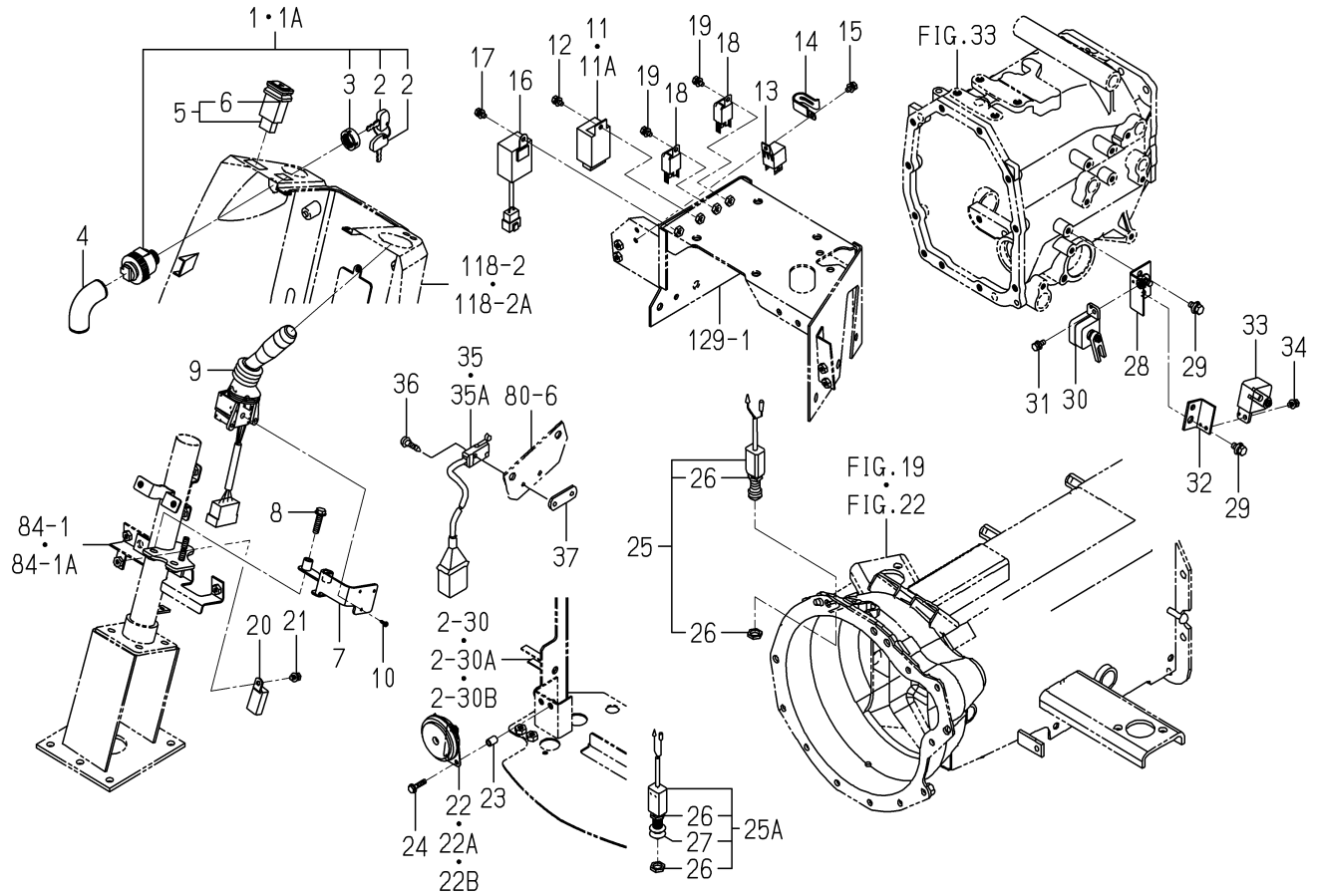
FIG.144 SWITCH SYSTEM(3215,3245-H TYPE)
