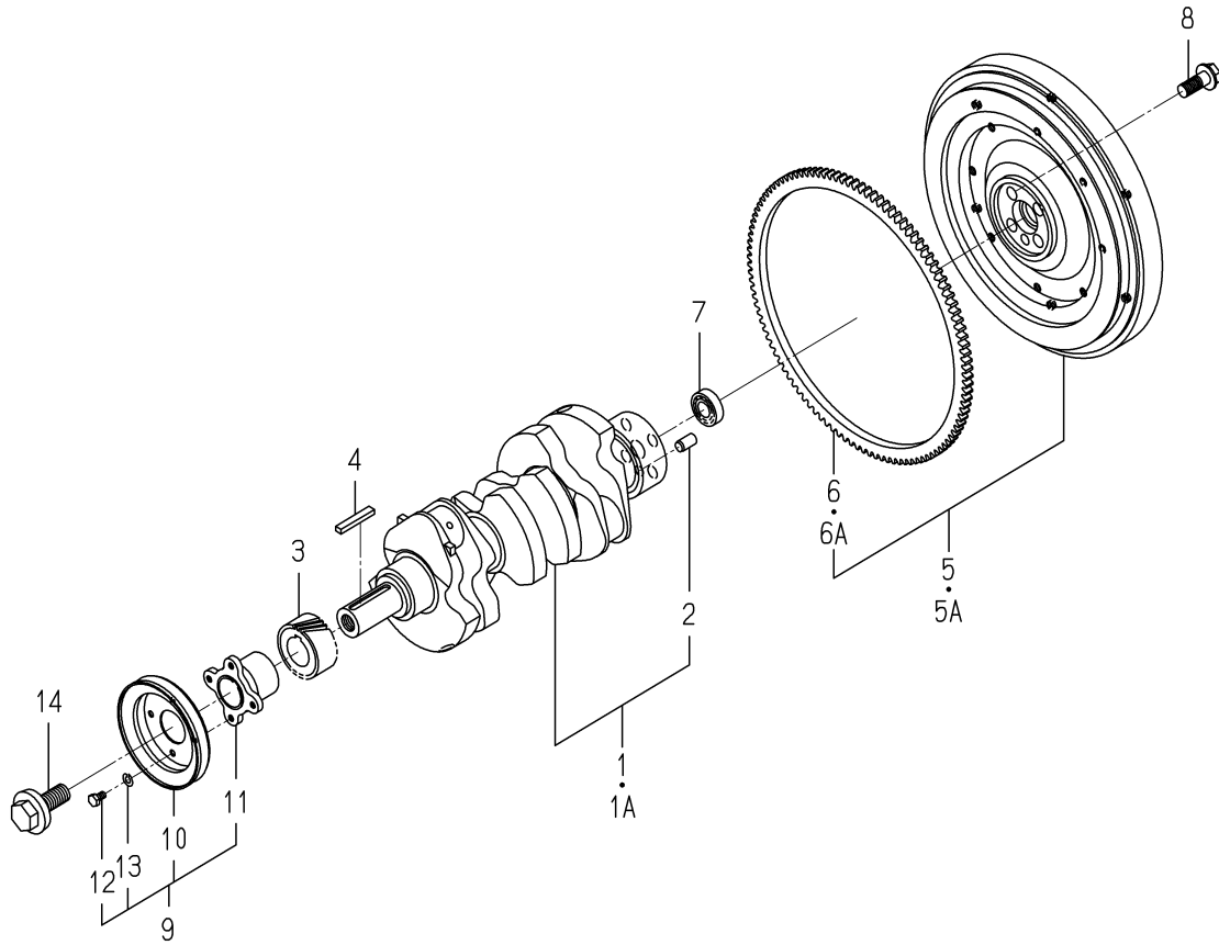
FIG. 16 CRANK SHAFT
