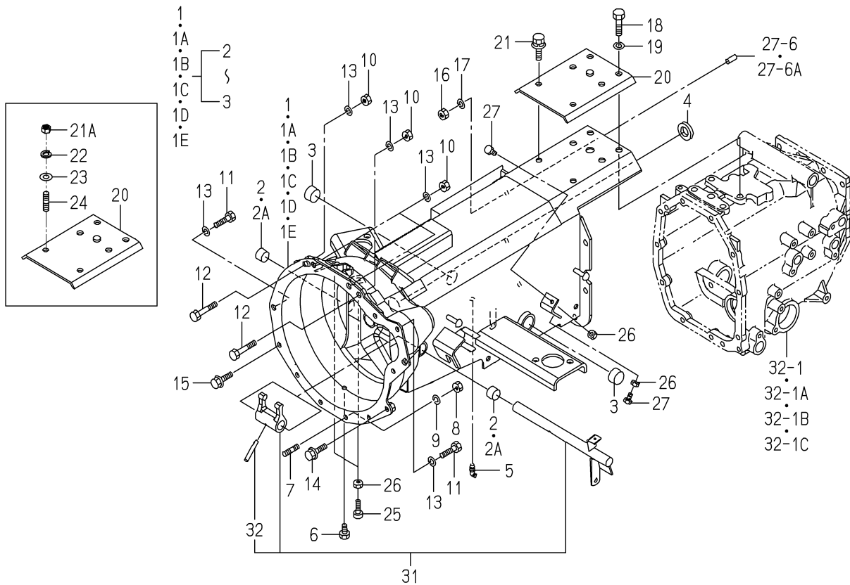
FIG. 18 HOUSING(CLUTCH)SYSTEM(1/2) (3215,3245-EXCEPT H TYPE)
