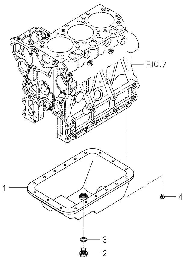
FIG. 9 OIL PAN
