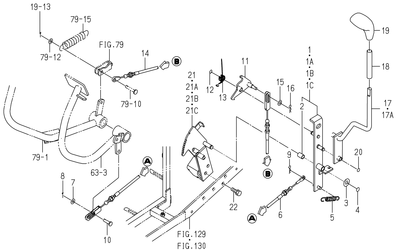
FIG. 64 LEVER(HST)SYSTEM(H TYPE)
