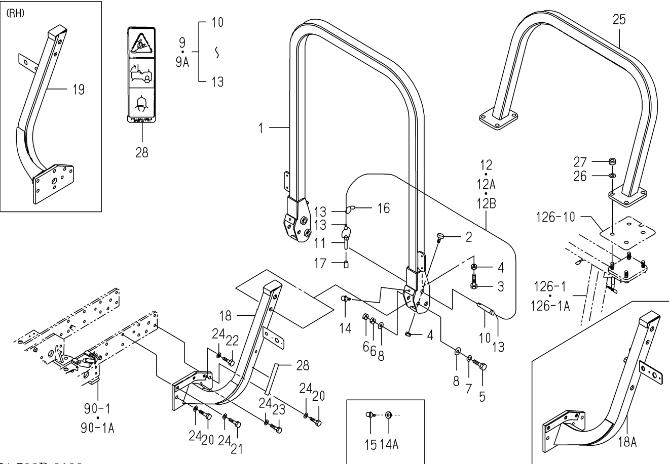
FIG.151 ROPS SYSTEM(3265-A TYPE)
