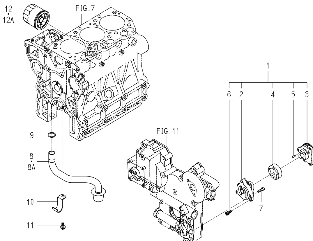
FIG. 19 OIL PUMP
