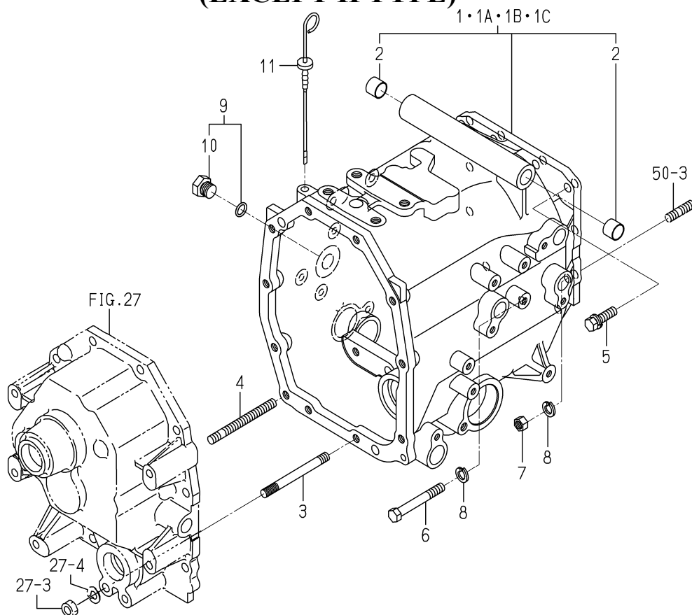
FIG. 32 CASE(TRANSMISSION/FRONT)SYSTEM (EXCEPT H TYPE)
