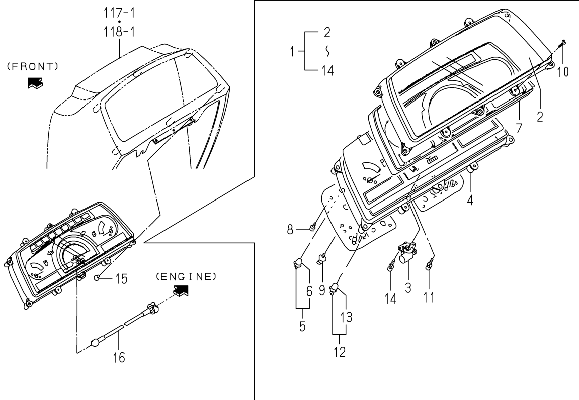
FIG.140 PANEL(METER)SYSTEM
