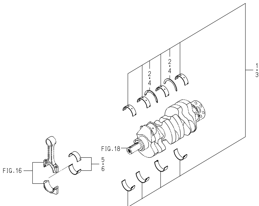
FIG. 8 BEARING/UNDER SIZE (OPTION)
