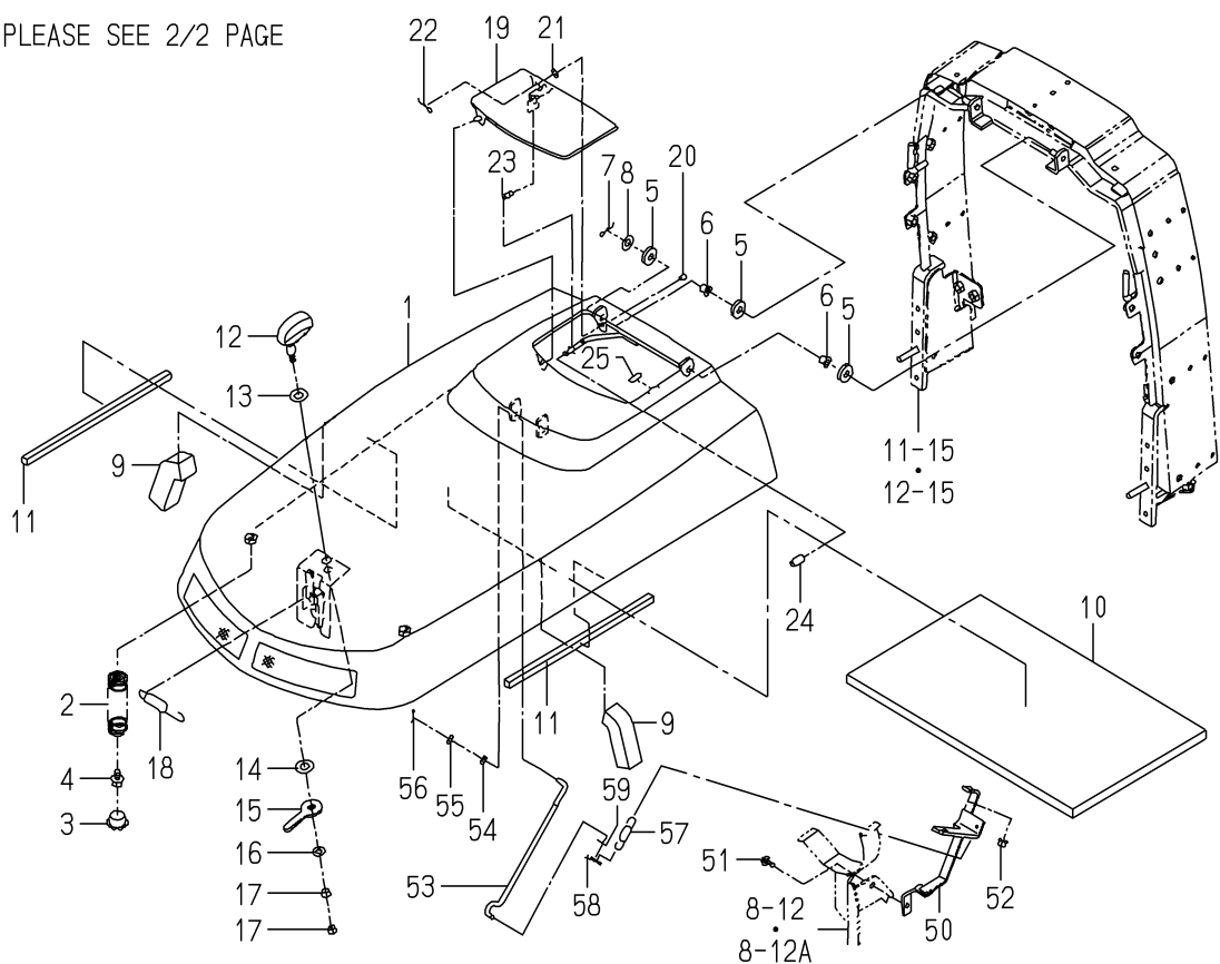
FIG.114 HOOD SYSTEM(3265)(1/2)
