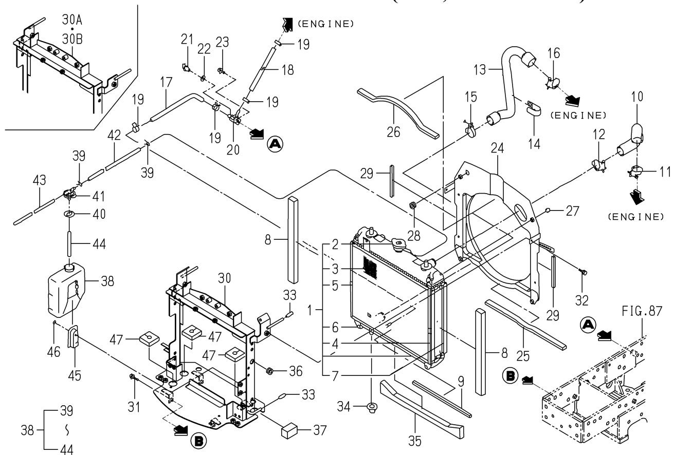
FIG. 2 RADIATOR SYSTEM(3215,3245-H TYPE)
