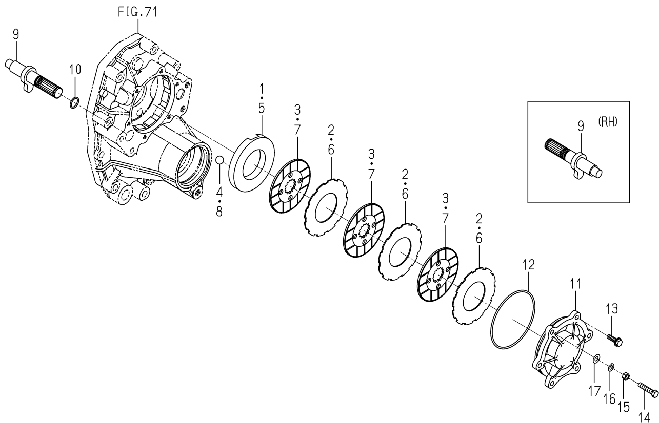
FIG. 77 BRAKE SYSTEM
