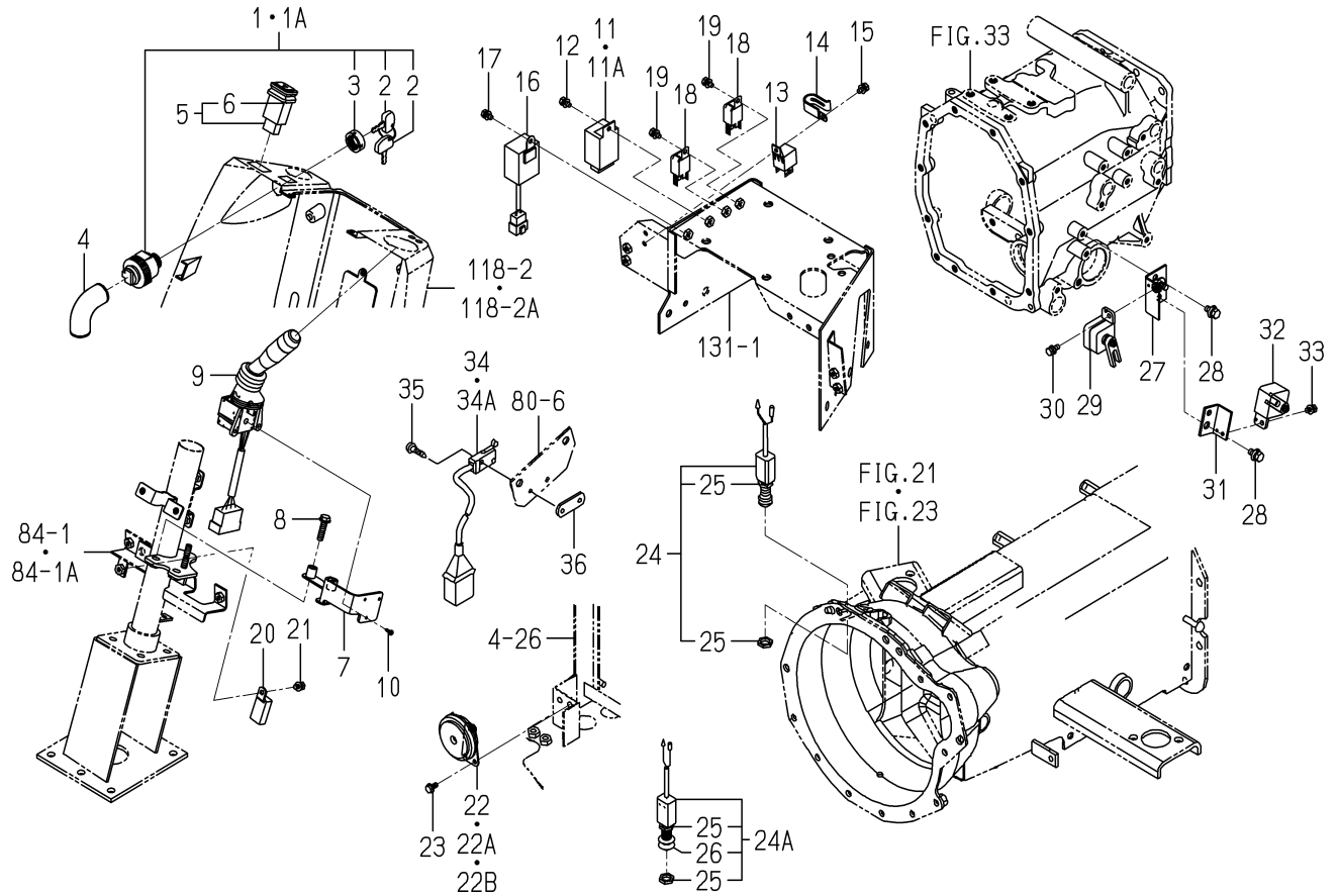
FIG.142 SWITCH SYSTEM(3265-H TYPE)
