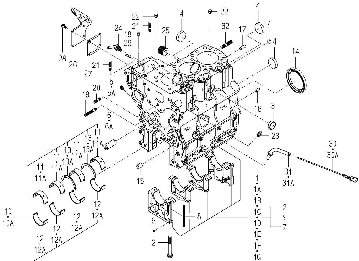
FIG. 6 CYLINDER BLOCK
