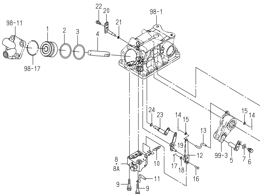
FIG.100 CYLINDER SYSTEM
