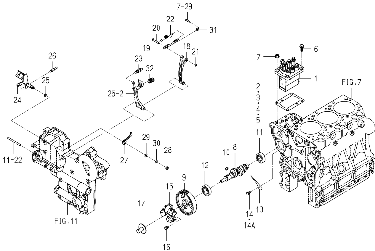
FIG. 23 INJECTION PUMP
