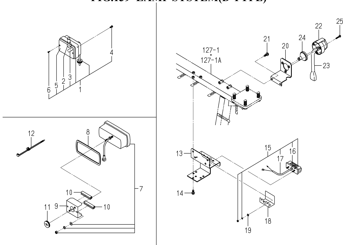
FIG.139 LAMP SYSTEM(D TYPE)
