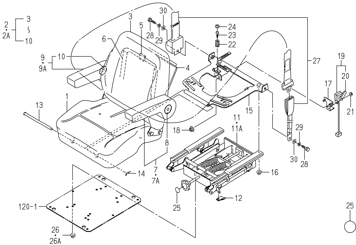
FIG.121 SEAT(NUMBER)SYSTEM(E6 TYPE)
