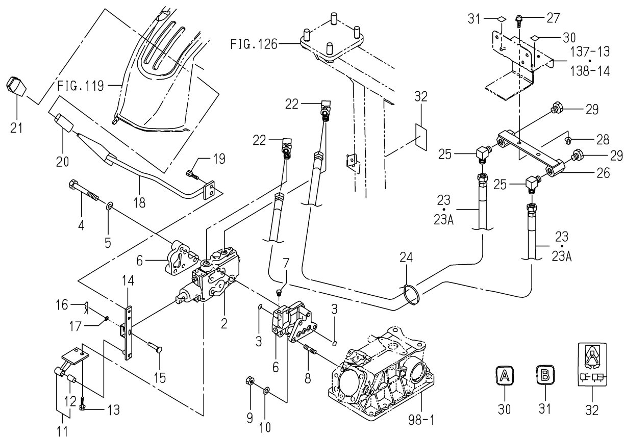
FIG.104 VALVE(REMOTE)SYSTEM(V TYPE)
