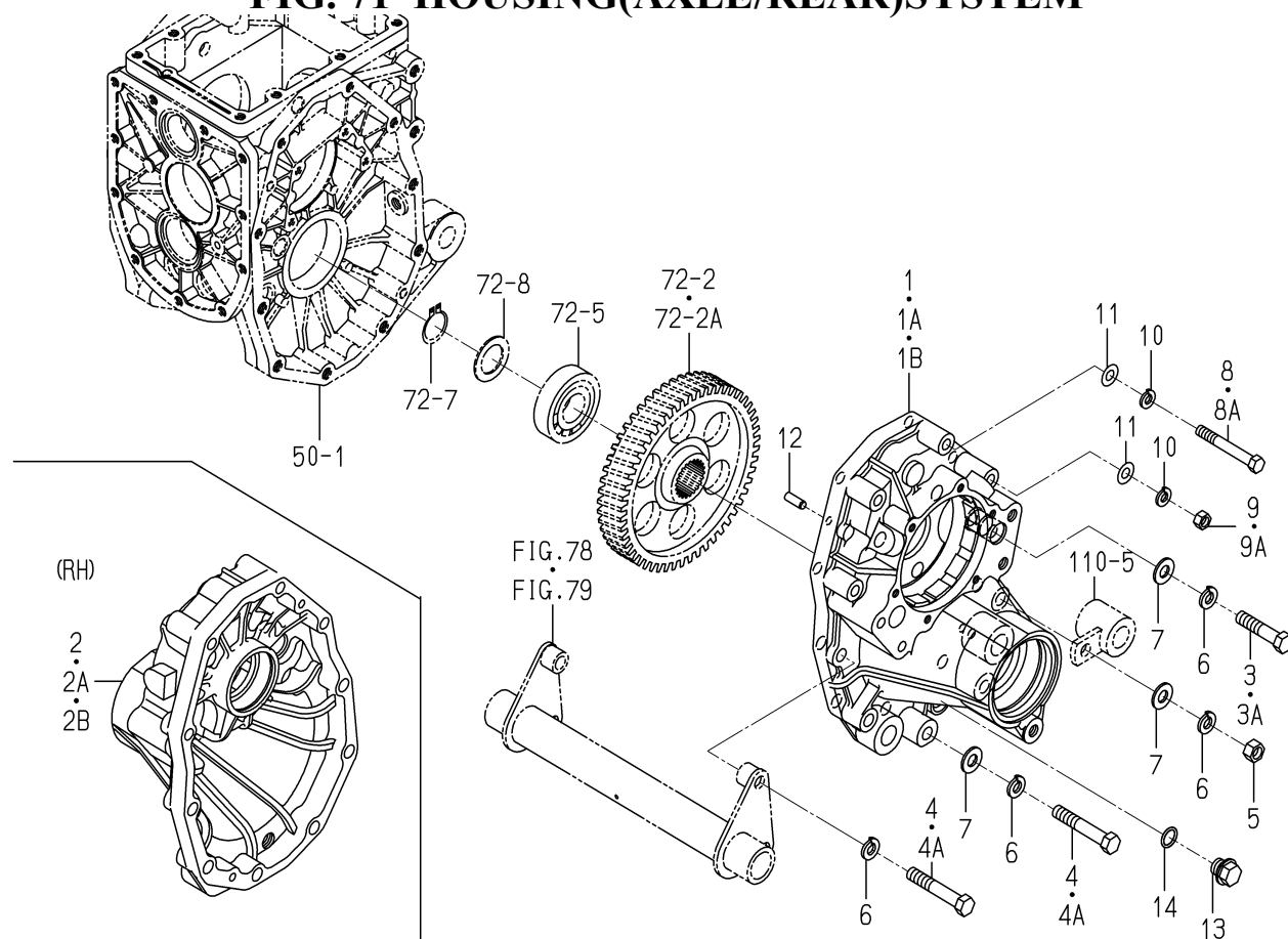
FIG. 71 HOUSING(AXLE/REAR)SYSTEM
