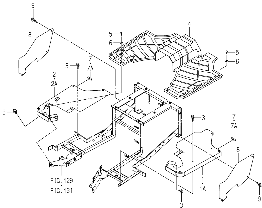
FIG.133 STEP SYSTEM(FHW TYPE)
