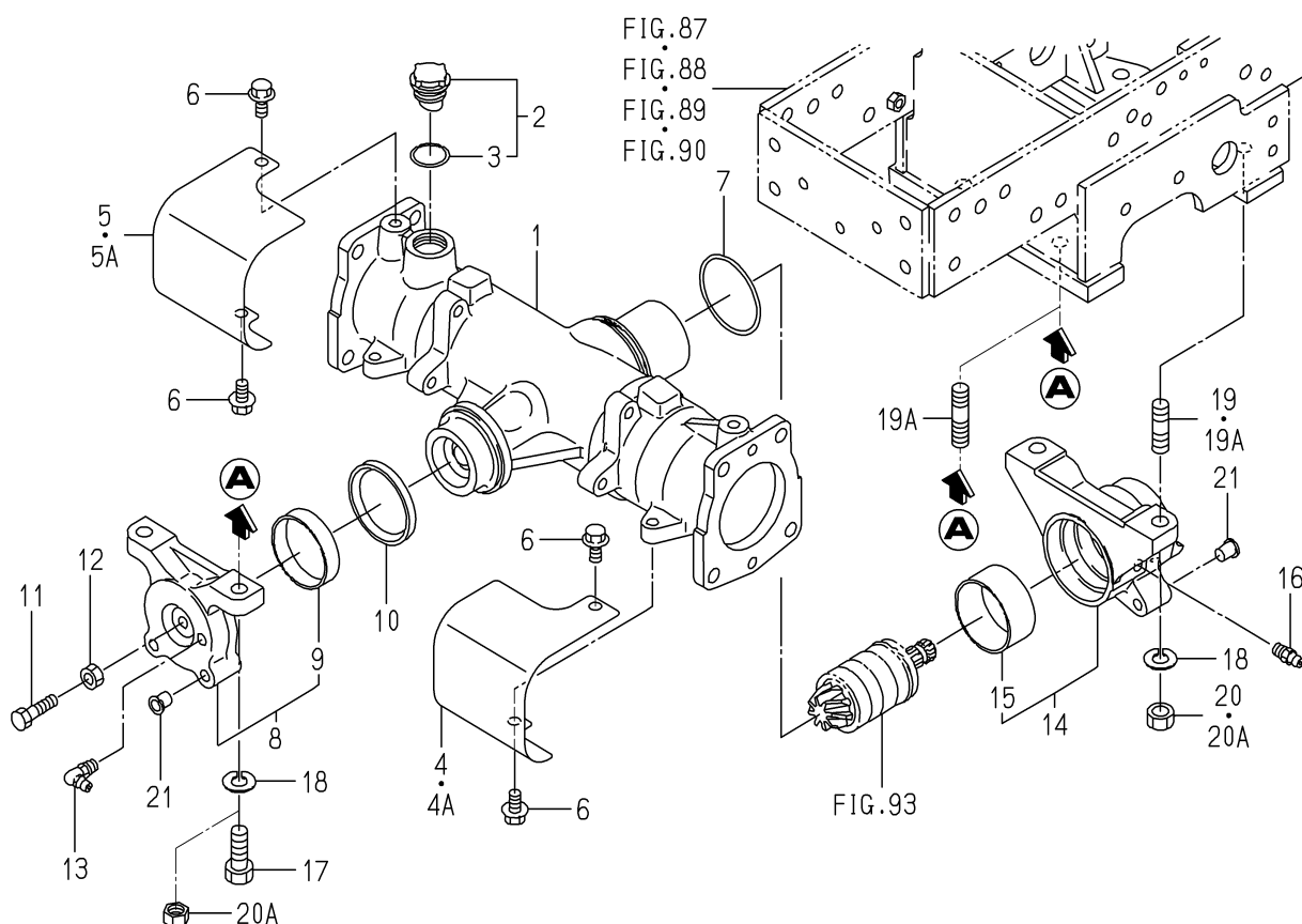
FIG. 94 HOUSING(AXLE)SYSTEM
