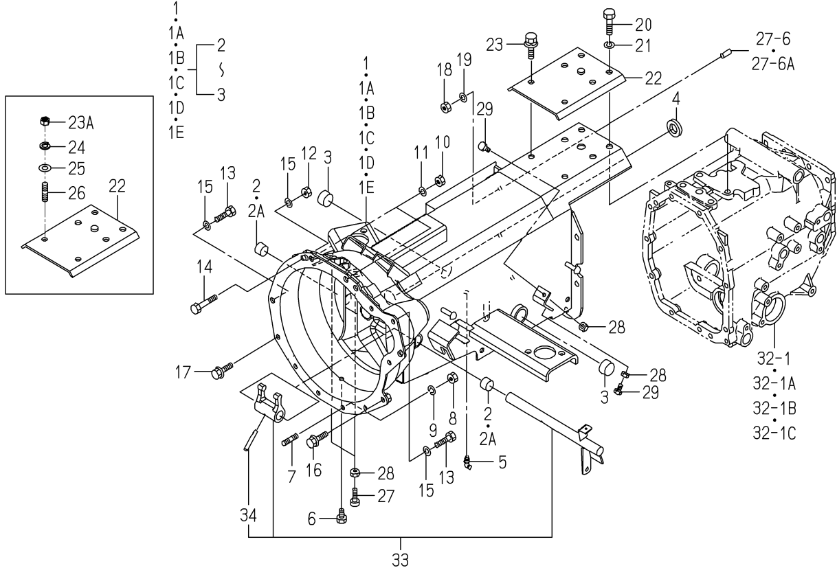
FIG. 20 HOUSING(CLUTCH)SYSTEM(1/2) (3265-EXCEPT H TYPE)
