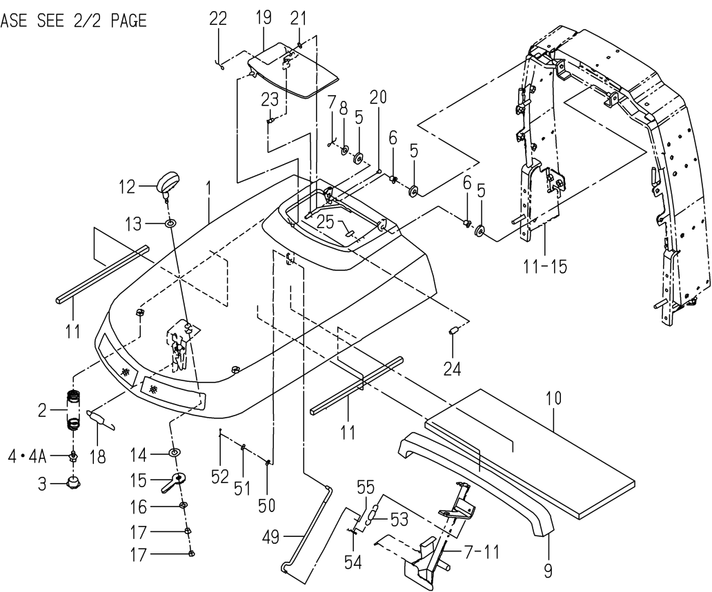
FIG.113 HOOD SYSTEM(3215,3245)(1/2)
