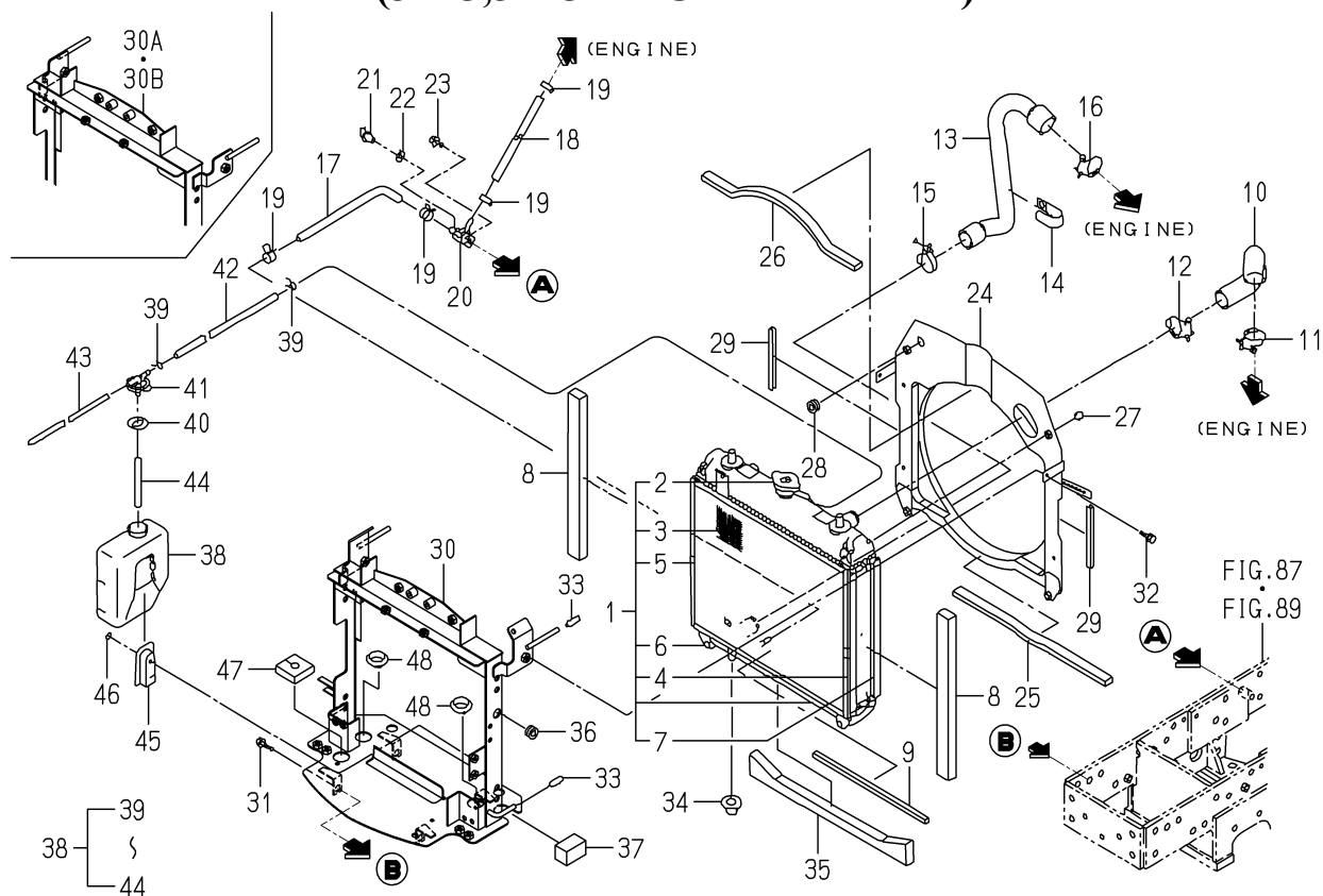
FIG. 1 RADIATOR SYSTEM (3215,3245-EXCEPT H TYPE)
