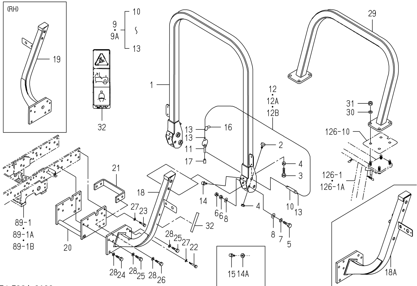
FIG.150 ROPS SYSTEM(3215,3245-A TYPE)
