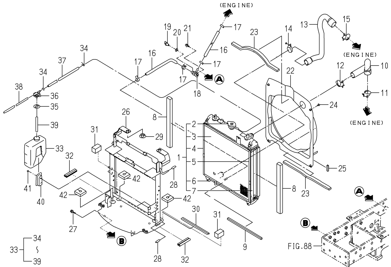
FIG. 4 RADIATOR SYSTEM(3265-H TYPE)
