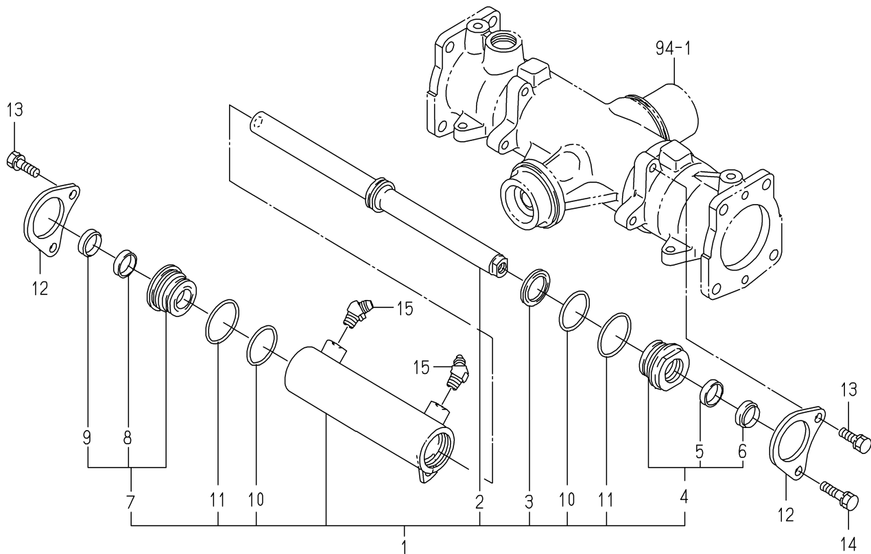
FIG. 83 CYLINDER SYSTEM
