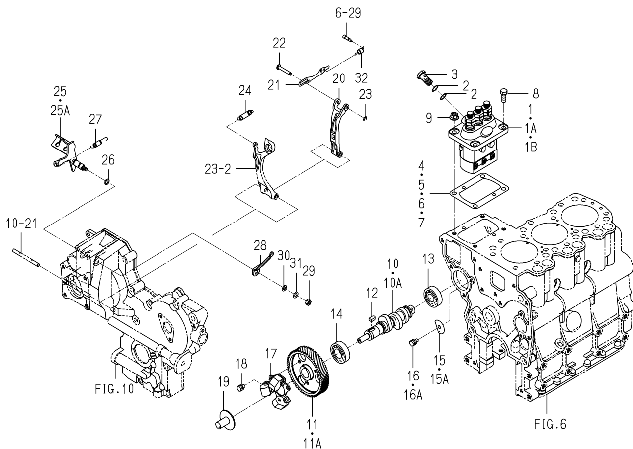
FIG. 21 INJECTION PUMP
