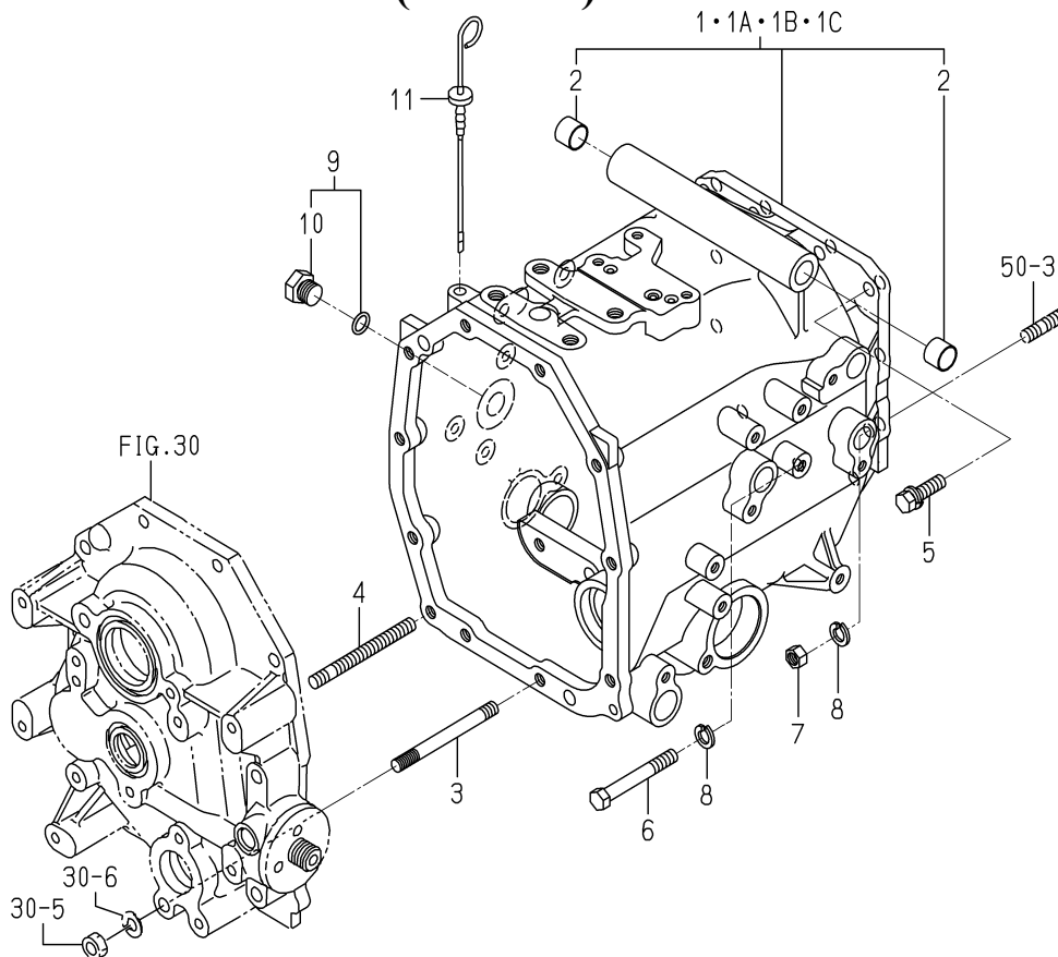
FIG. 33 CASE(TRANSMISSION/FRONT)SYSTEM (H TYPE)
