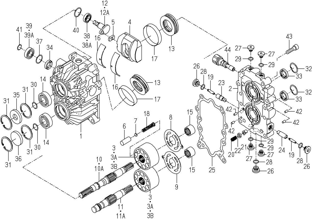
FIG.183 COMPONENT PARTS FOR K510-014-000-40 ON Fig.34
