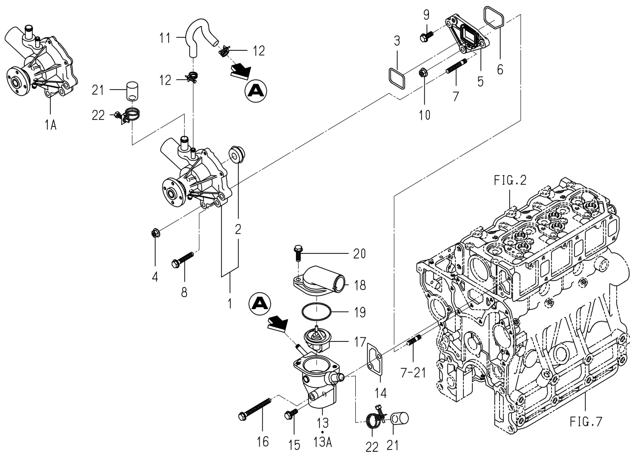
FIG. 20 WATER PUMP
