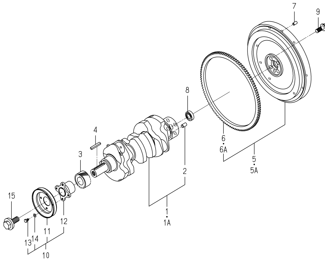
FIG. 16 CRANK SHAFT
