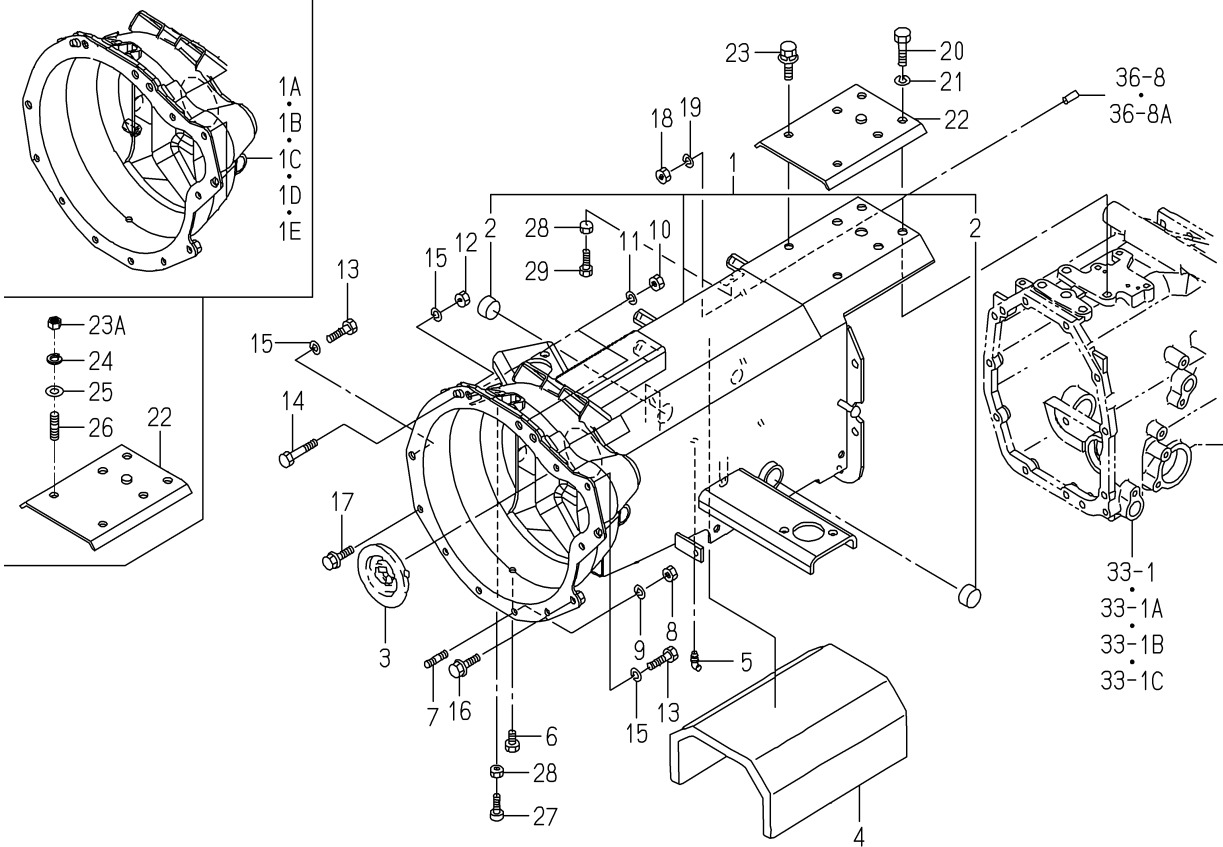
FIG. 21 HOUSING(CLUTCH)SYSTEM(1/2) (3265-H TYPE)(D TYPE-NO.1-1089)
