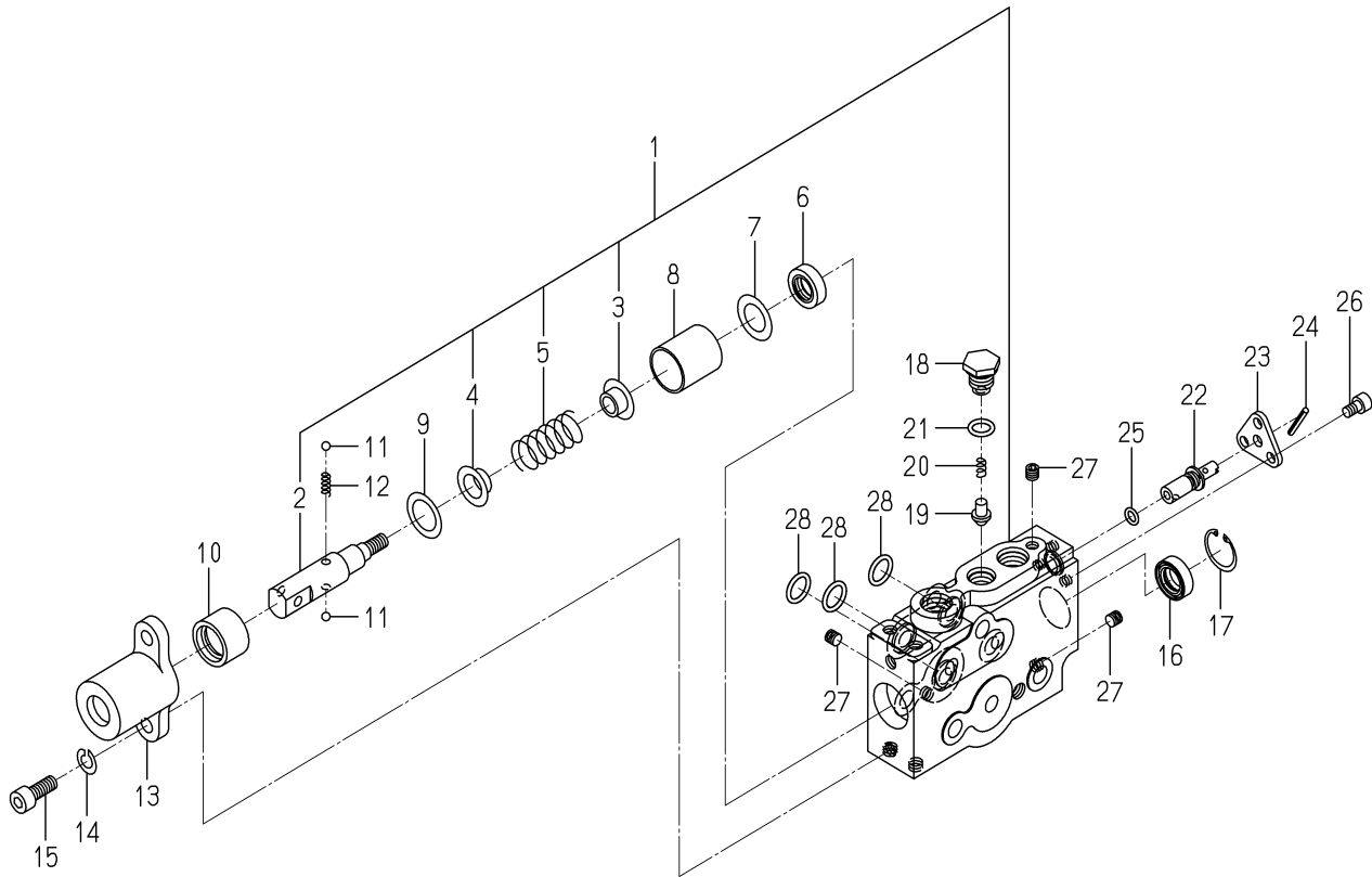
FIG.184 COMPONENT PARTS FOR 1719-511-350-00 ON Fig.104,105,176
