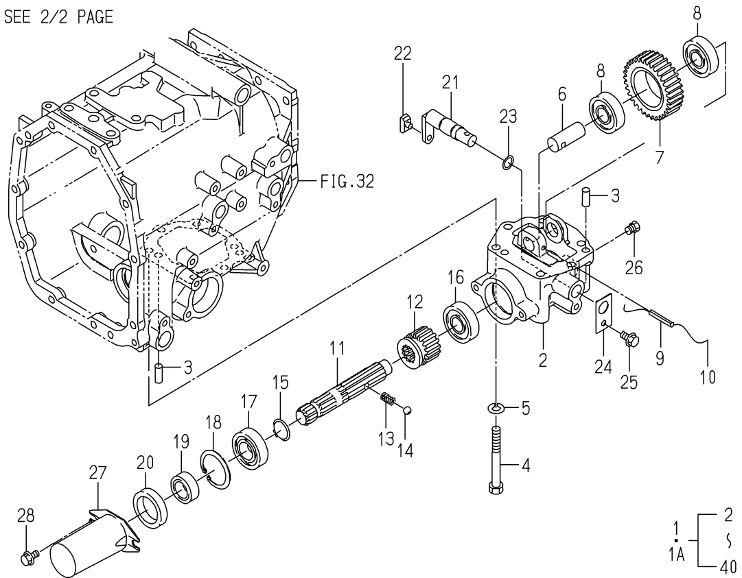
FIG.167 PTO(MID)SET(A TYPE)(OPTION)(1/2)
