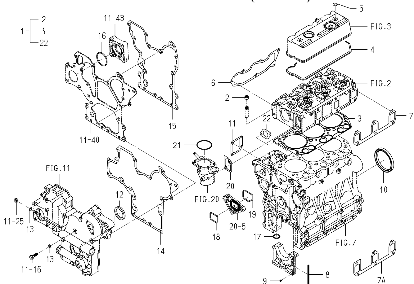
FIG. 29 REPAIR PARTS(OPTION)
