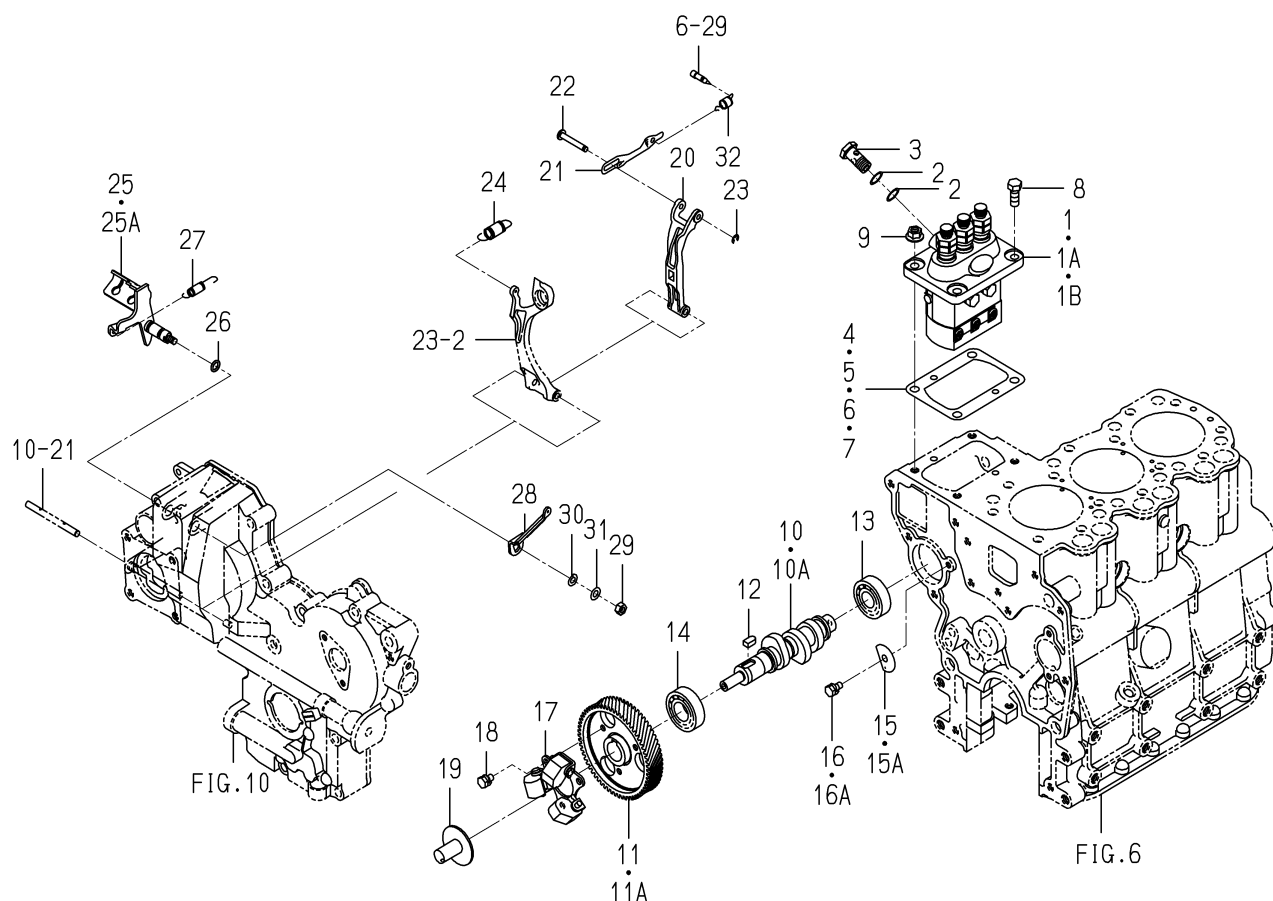
FIG. 21 INJECTION PUMP
