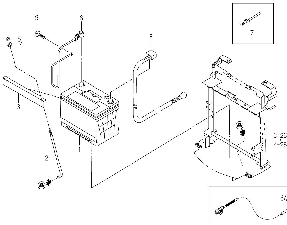
FIG. 15 BATTERY SYSTEM(3265)
