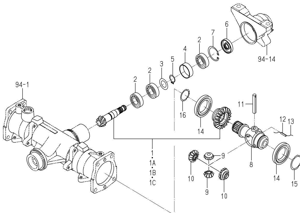
FIG. 93 PINION(DRIVE)SYSTEM
