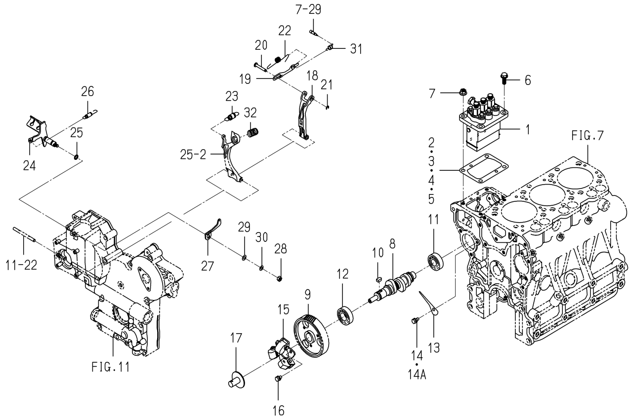
FIG. 23 INJECTION PUMP
