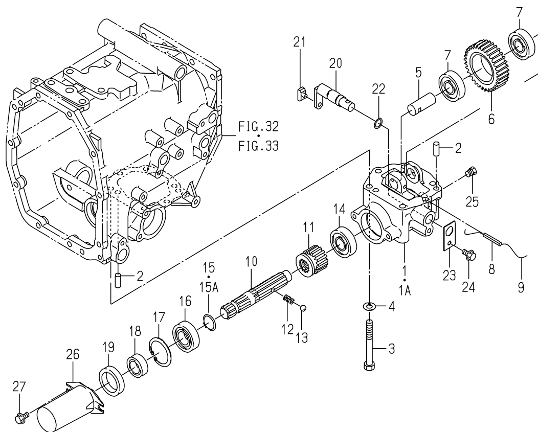
FIG. 54 PTO(MID)SYSTEM(H,M TYPE)
