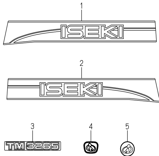
FIG.152 ORNAMENT(3265-R TYPE)
