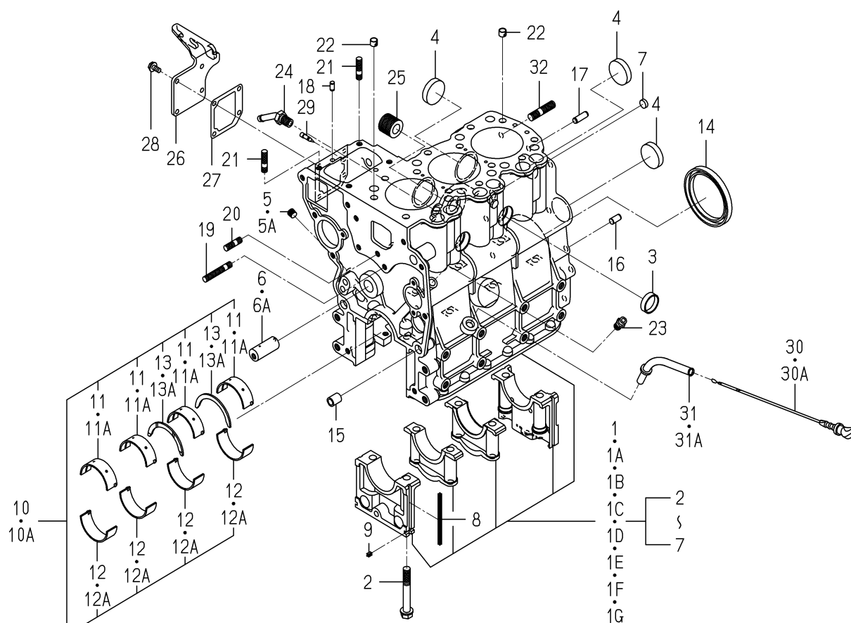
FIG. 6 CYLINDER BLOCK
