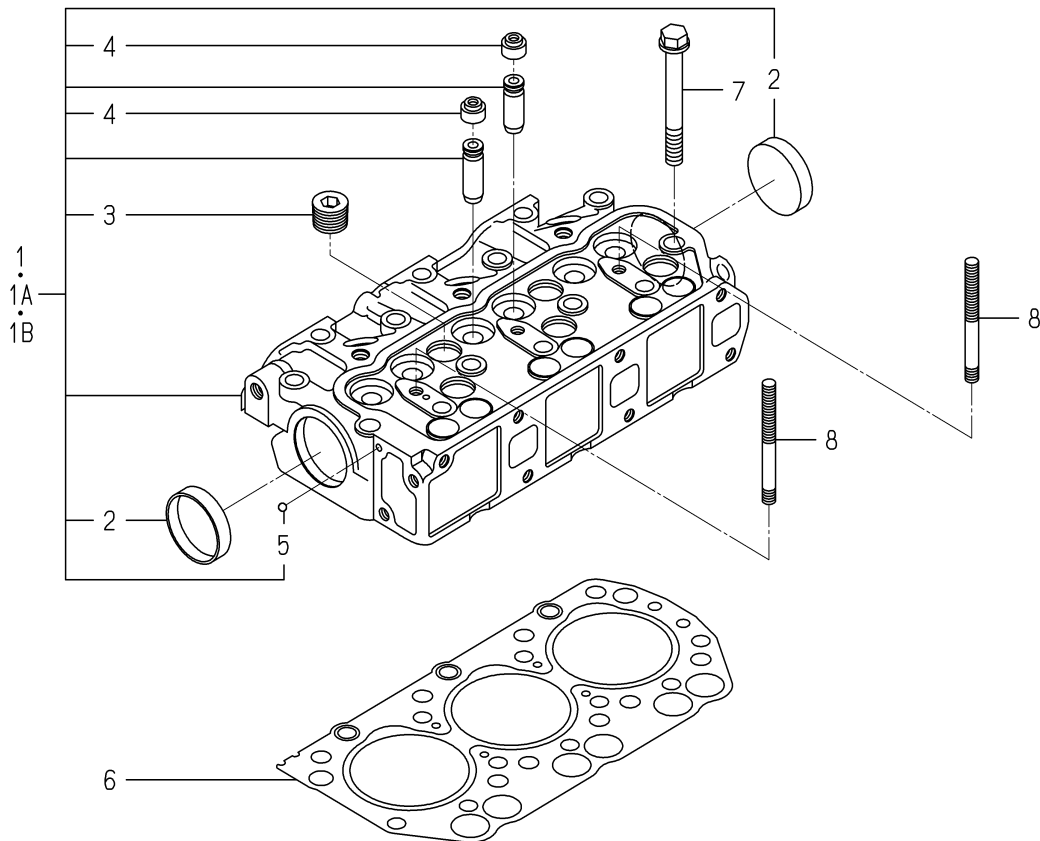
FIG. 2 CYLINDER HEAD
