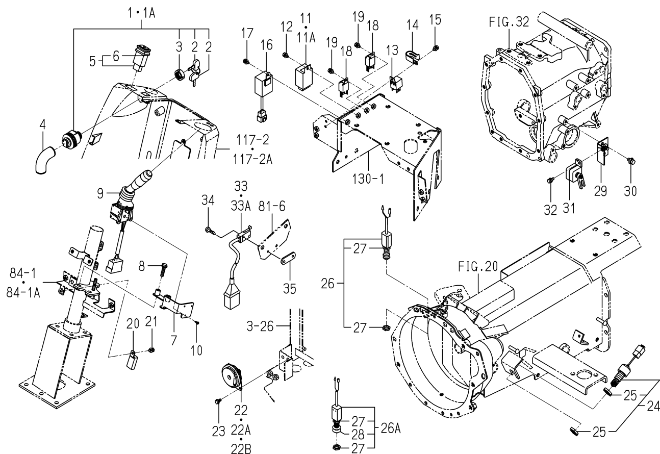
FIG.141 SWITCH SYSTEM(3265-EXCEPT H TYPE)
