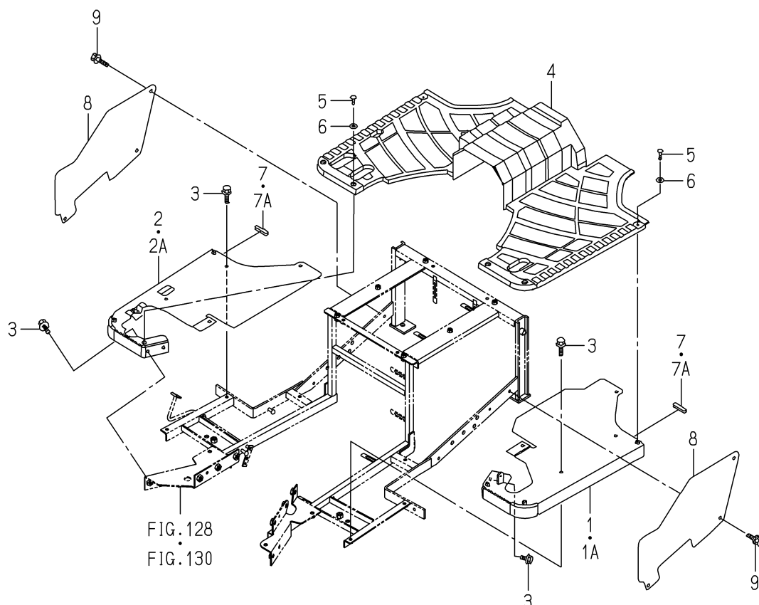
FIG.132 STEP SYSTEM(EXCEPT S,D TYPE)
