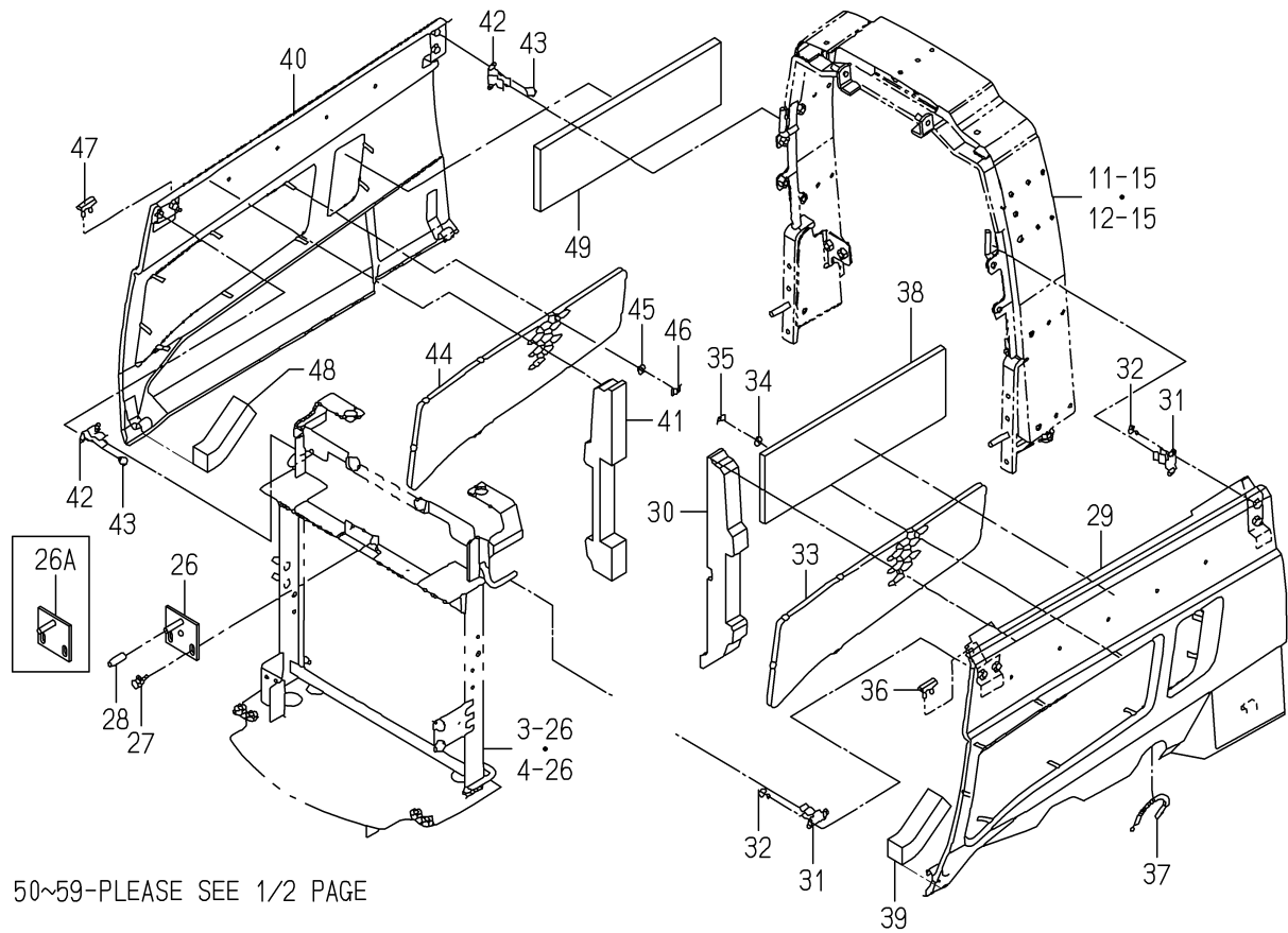
FIG.114 HOOD SYSTEM(3265)(2/2)
