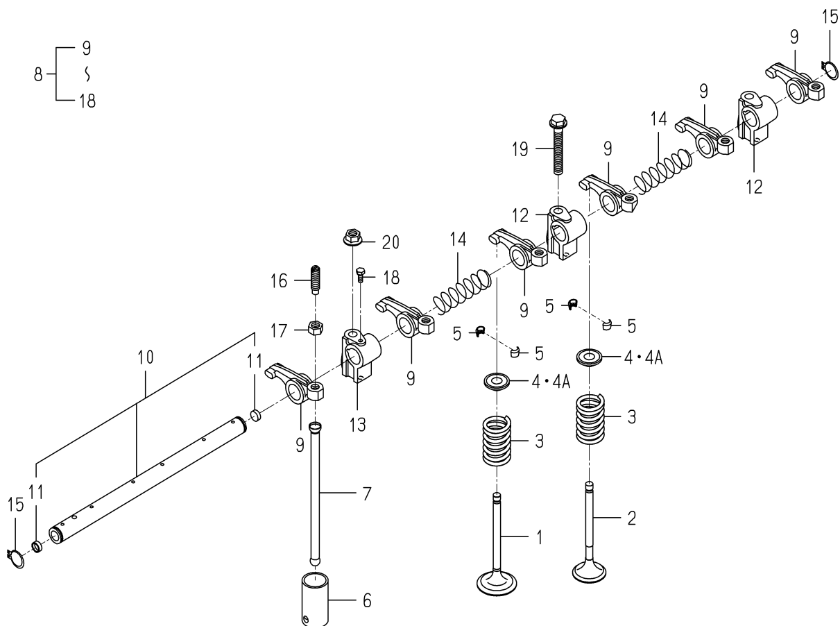
FIG. 14 VALVE
