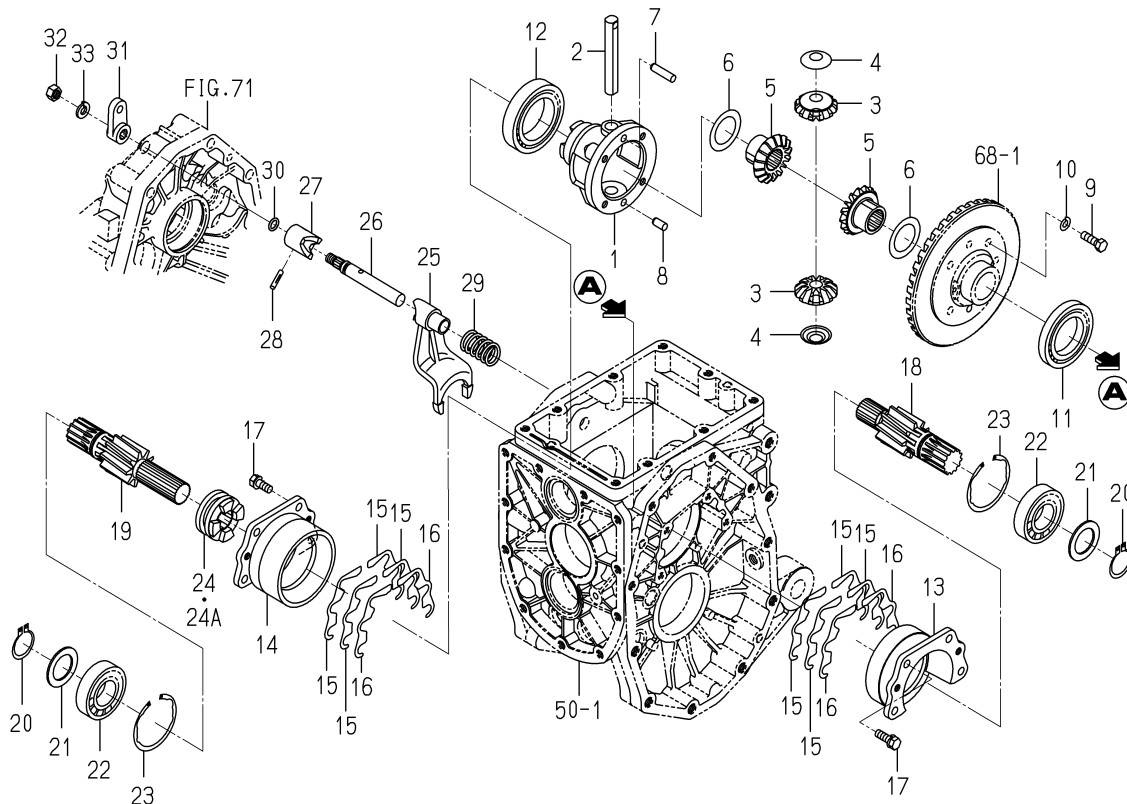
FIG. 70 CASE (DIFFERENTIAL GEAR/REAR)SYSTEM (H TYPE)
