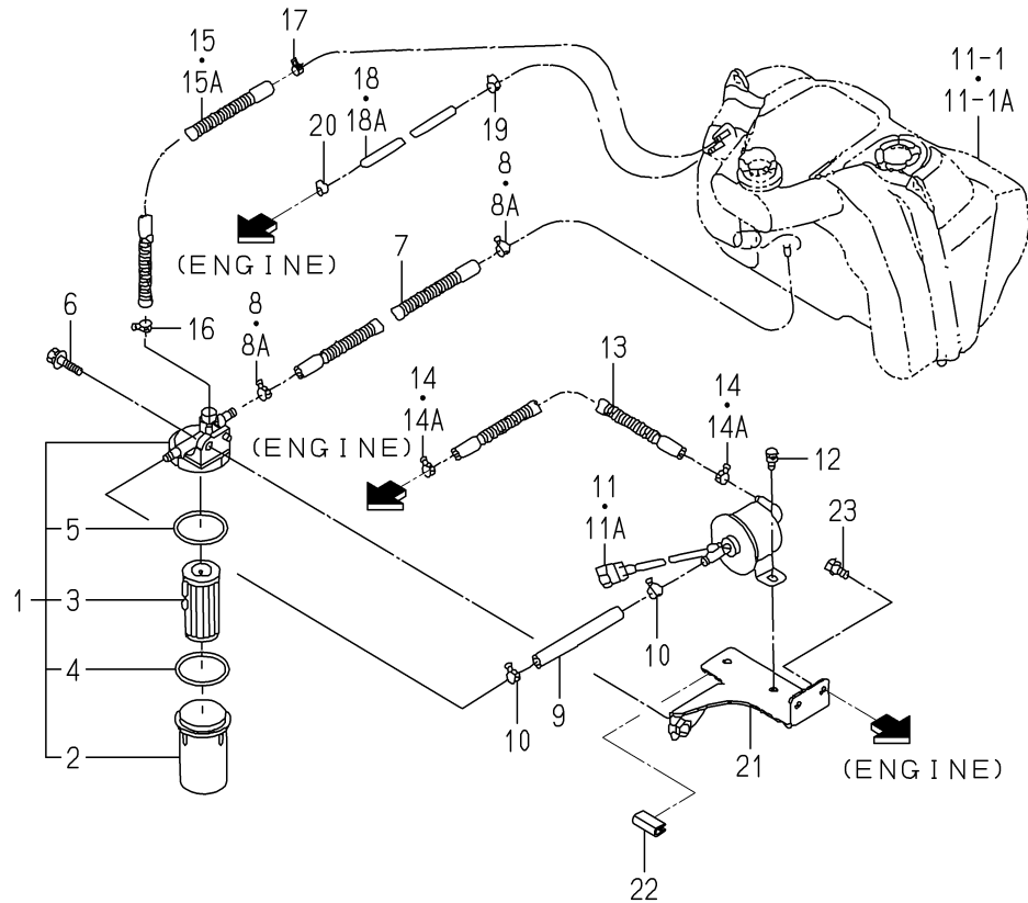
FIG. 9 FILTER SYSTEM(3215,3245)
