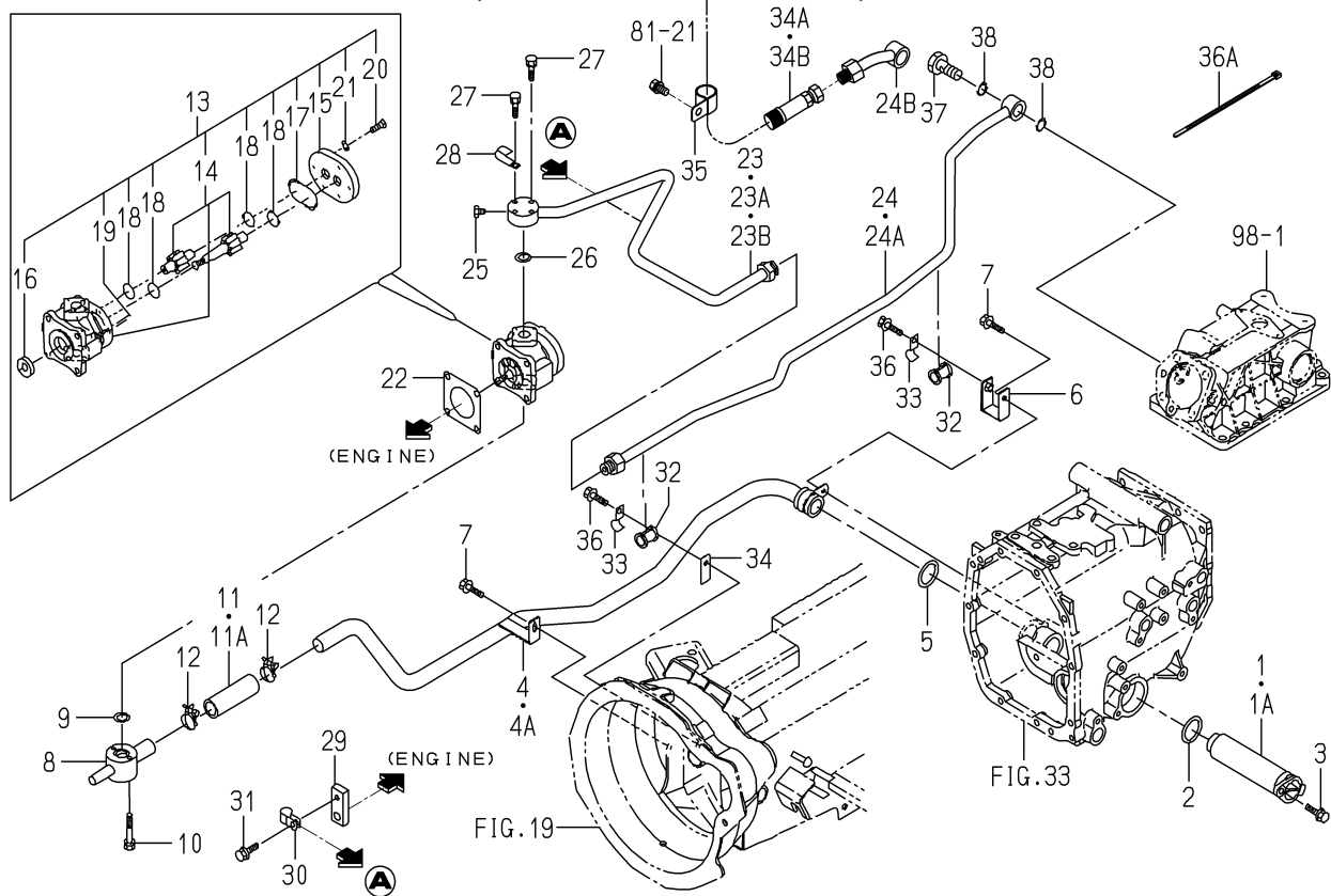
FIG.109 PIPING(MAIN)SYSTEM (3215,3245-H TYPE)
