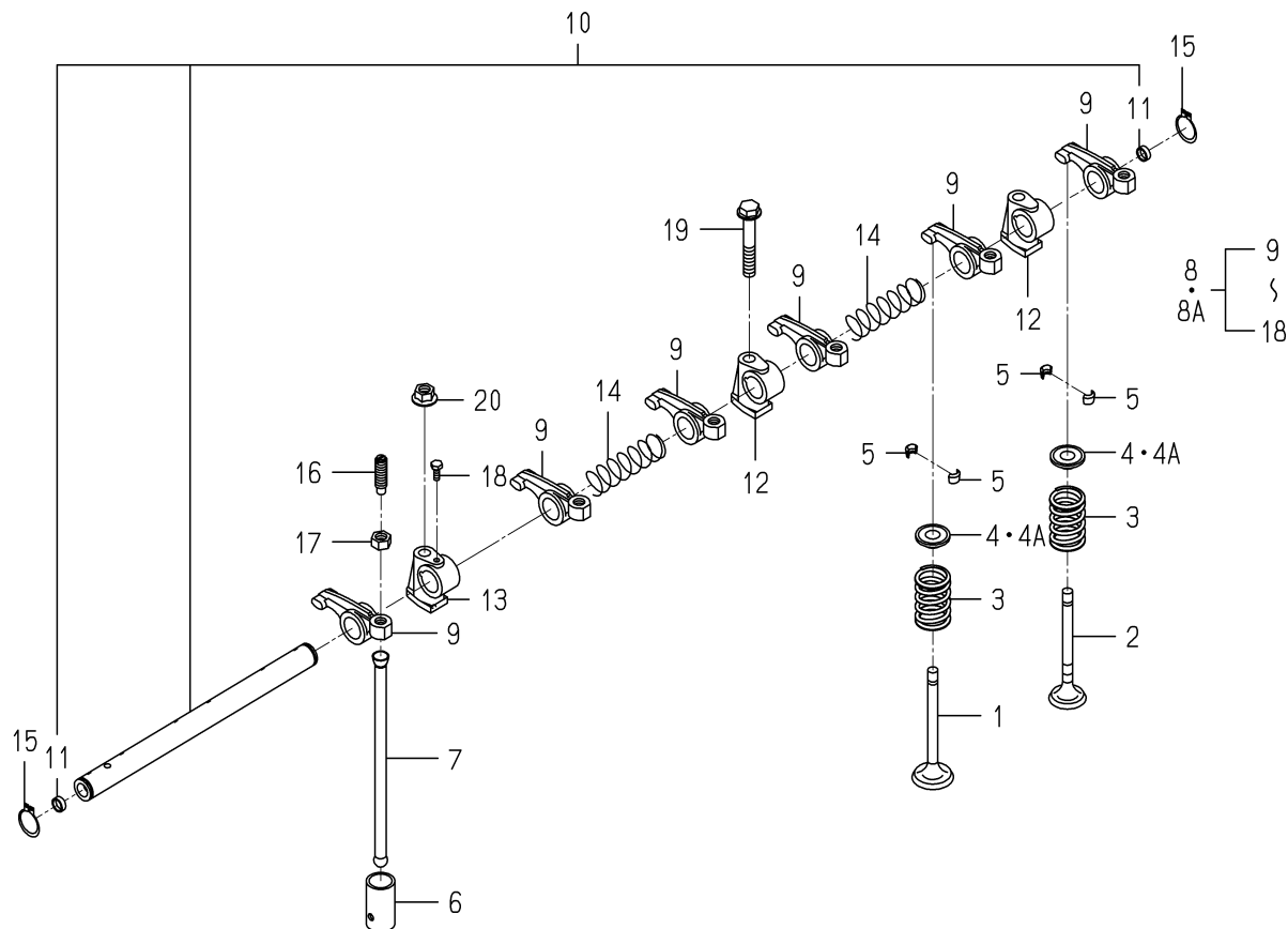
FIG. 12 VALVE
