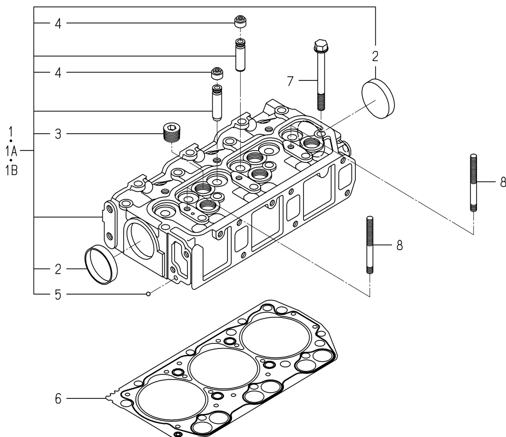
FIG. 2 CYLINDER HEAD
