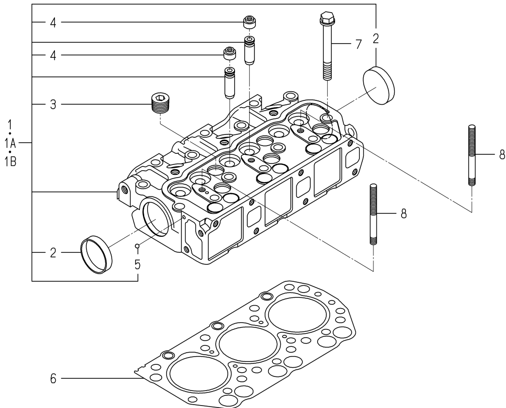
FIG. 2 CYLINDER HEAD
