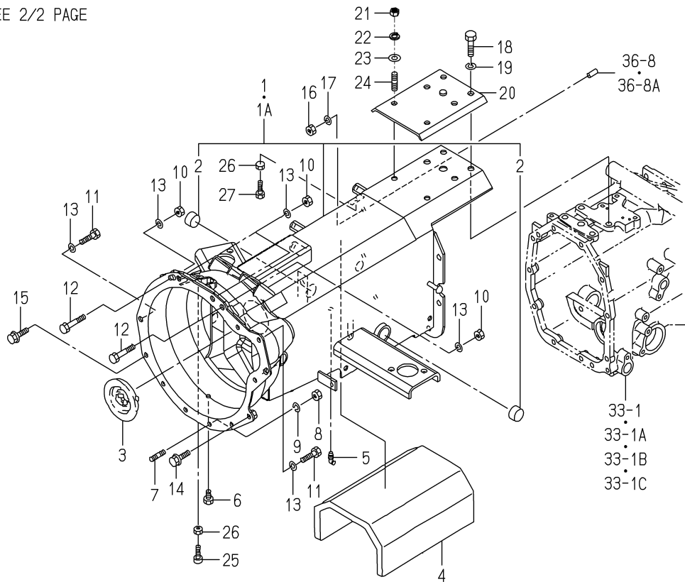
FIG. 22 HOUSING(CLUTCH)SYSTEM(1/2) (3215,3245-D TYPE) (3215-NO.1907-/3245-NO.390-)
