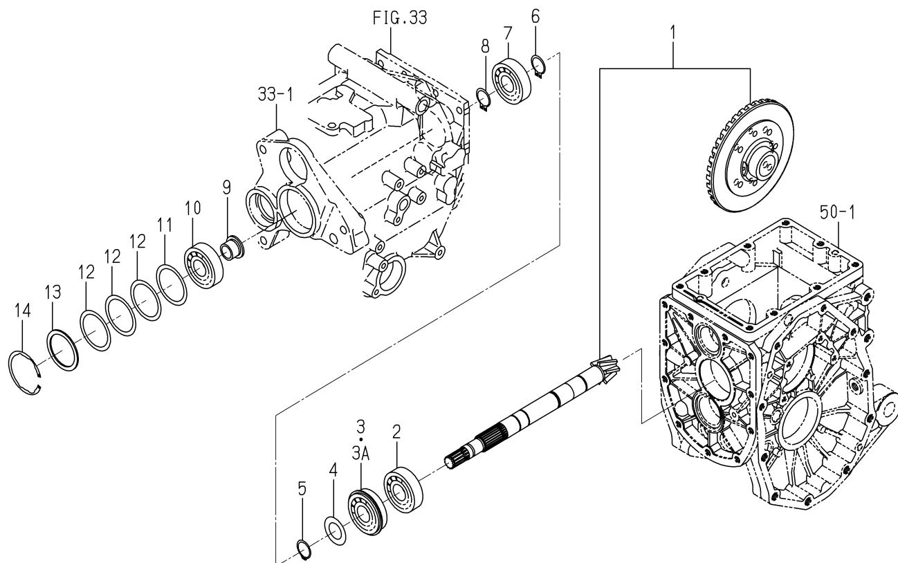
FIG. 68 PINION(DRIVE)SYSTEM(H TYPE)
