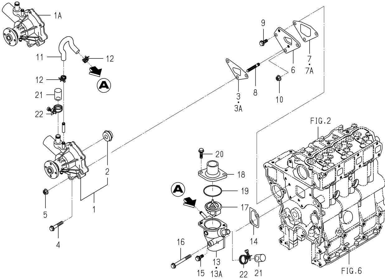
FIG. 18 WATER PUMP
