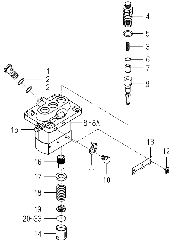
FIG. 29 COMPONENT PARTS FOR 6215-600-103-30 ON Fig.021
