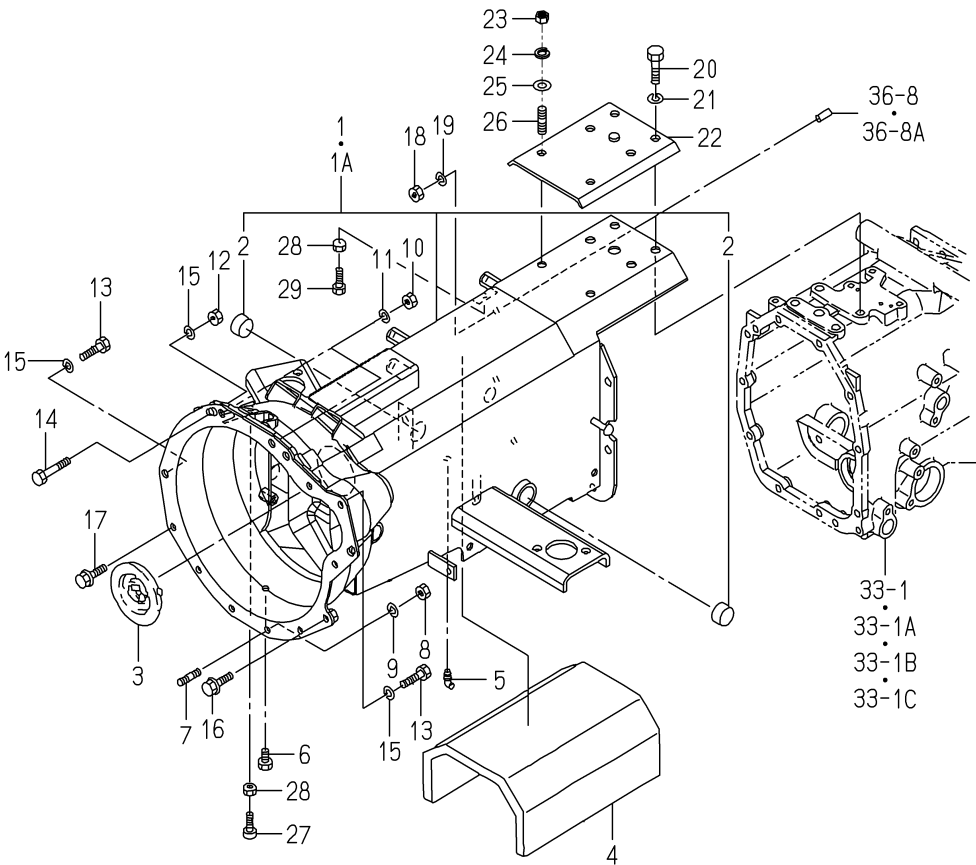
FIG. 23 HOUSING(CLUTCH)SYSTEM(1/2) (3265-D TYPE)(NO.1090-)
