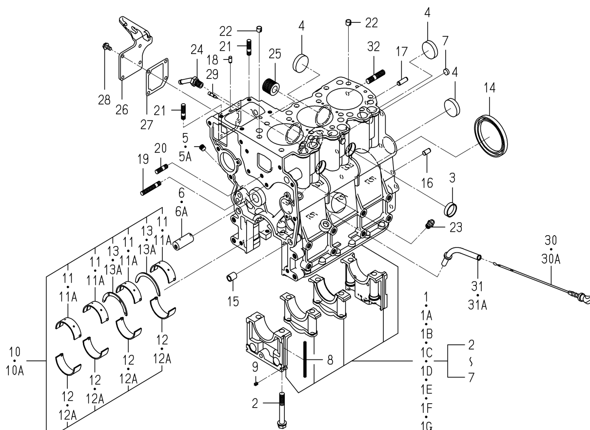
FIG. 6 CYLINDER BLOCK
