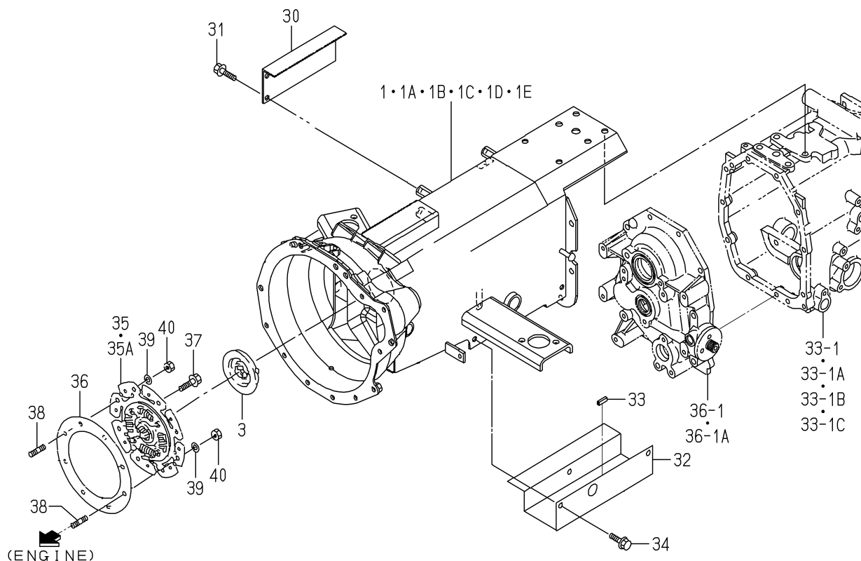
FIG. 21 HOUSING(CLUTCH)SYSTEM(2/2) (3265-H TYPE)(D TYPE-NO.1-1089)
