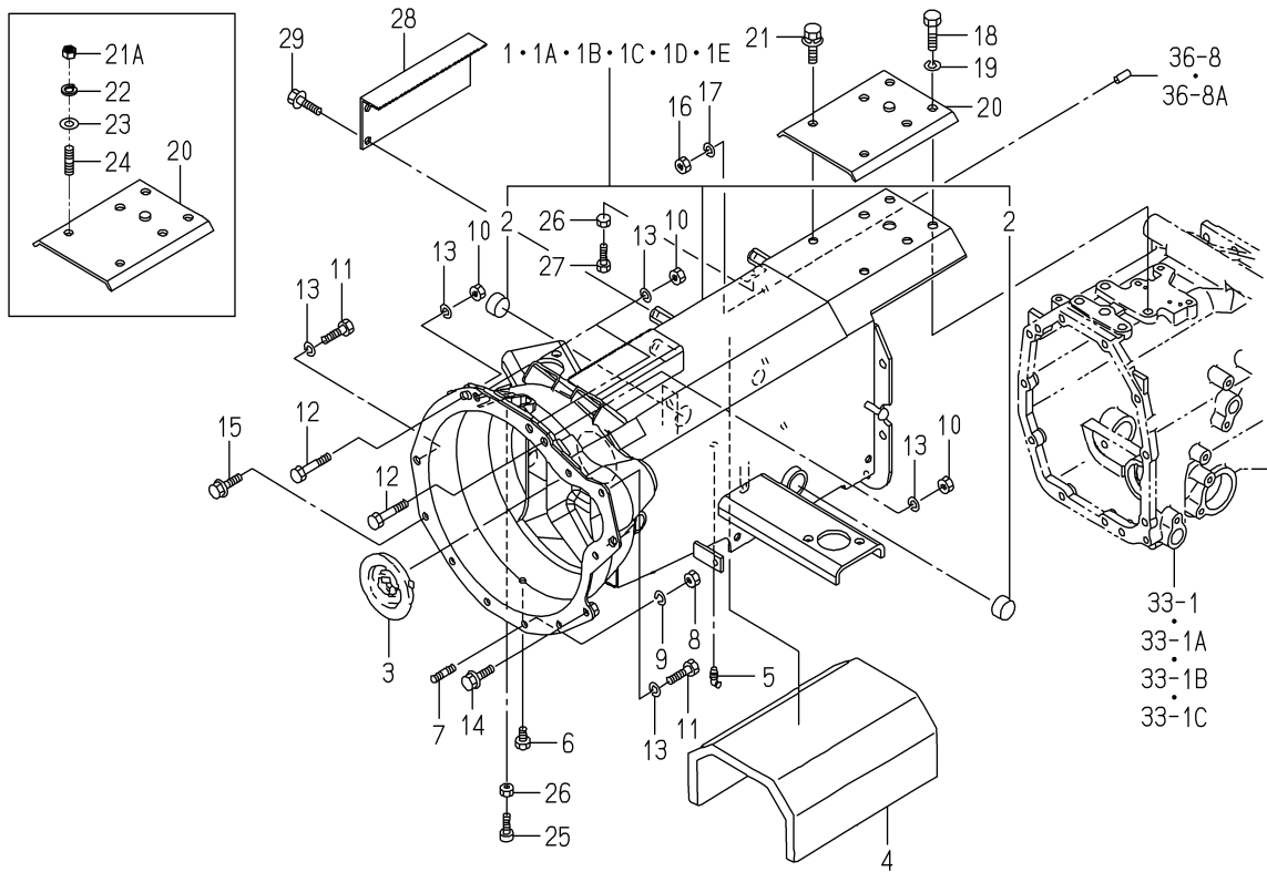
FIG. 19 HOUSING(CLUTCH)SYSTEM(1/2) (3215,3245-H TYPE) (D TYPE-3215-NO.1-1906,3245-NO.1-389)
