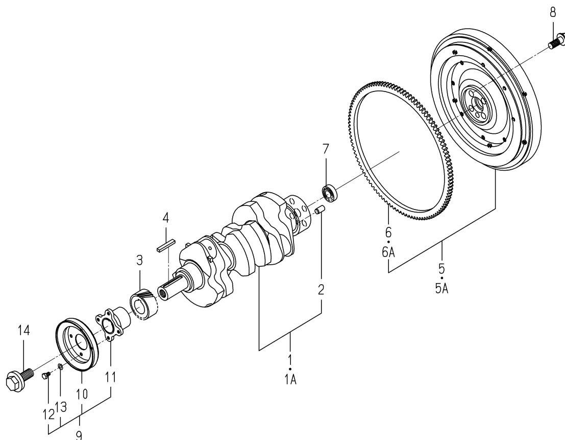
FIG. 16 CRANK SHAFT
