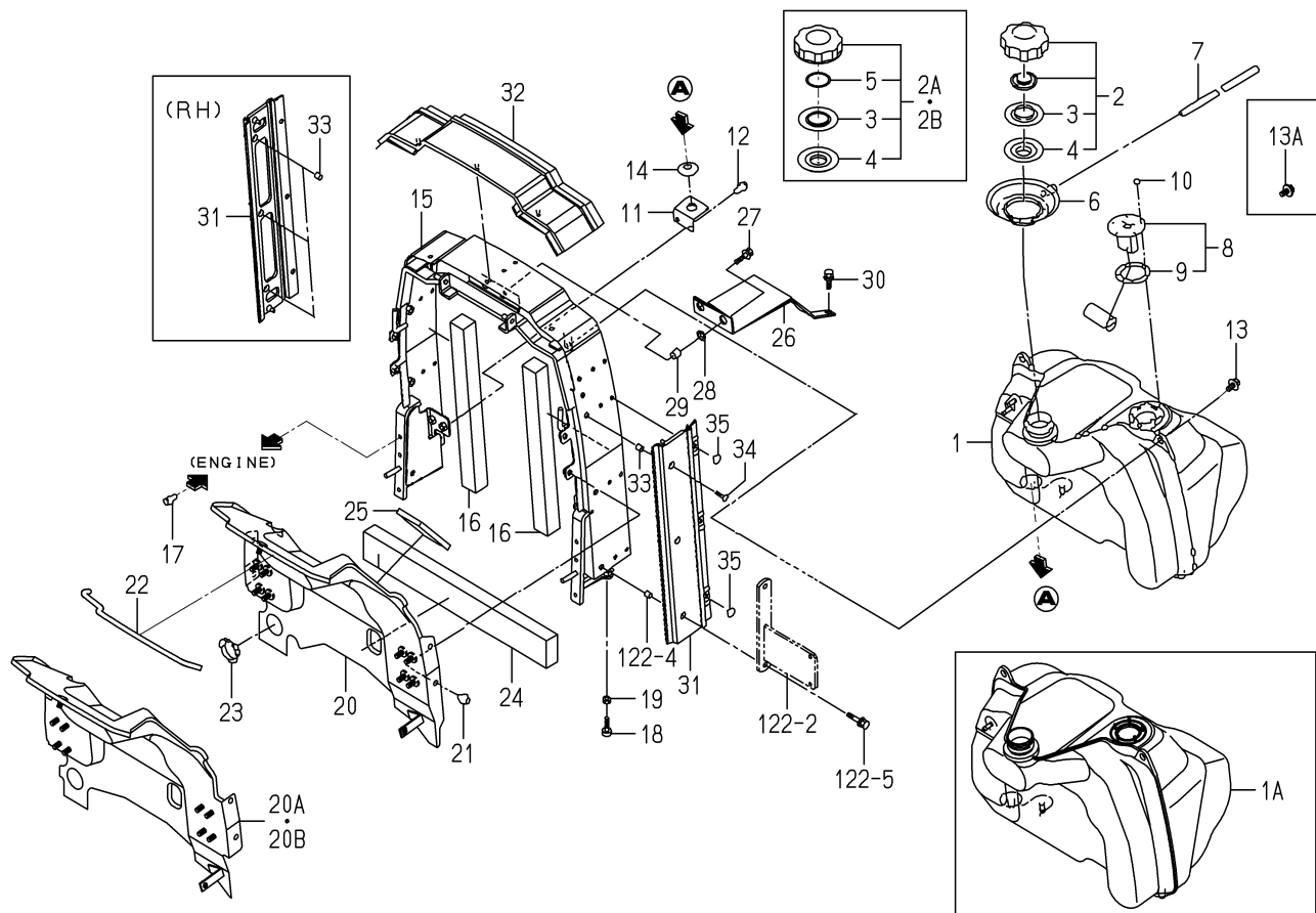
FIG. 11 TANK(FUEL)SYSTEM(3265-NO.1-62)
