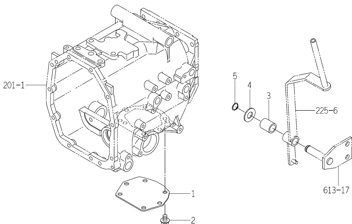
FIG.223 COVER (PTO/MID) SYSTEM (EXCEPT M TYPE)
