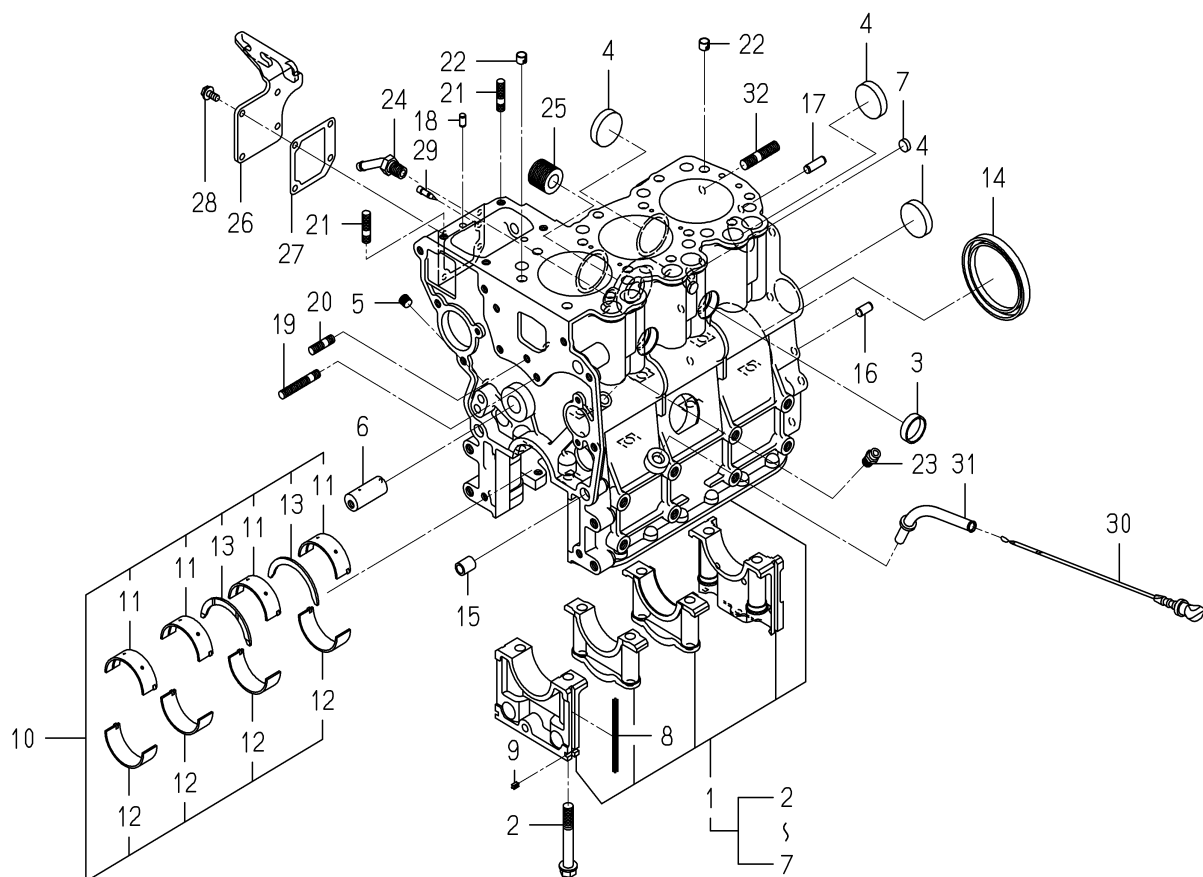
FIG.201 CYLINDER BLOCK
