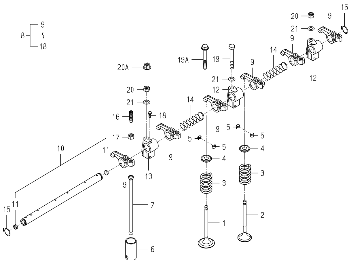
FIG.301 VALVE
