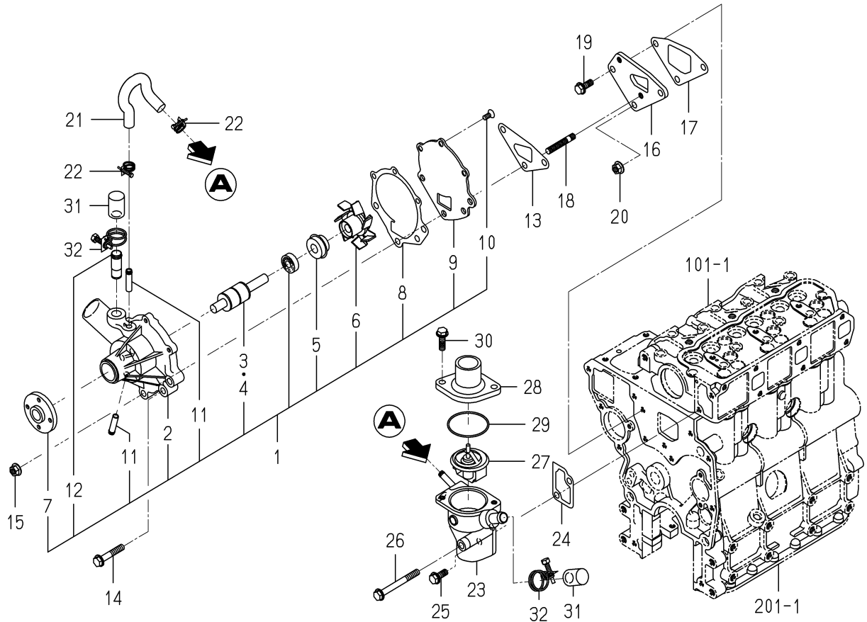
FIG.402 WATER PUMP
