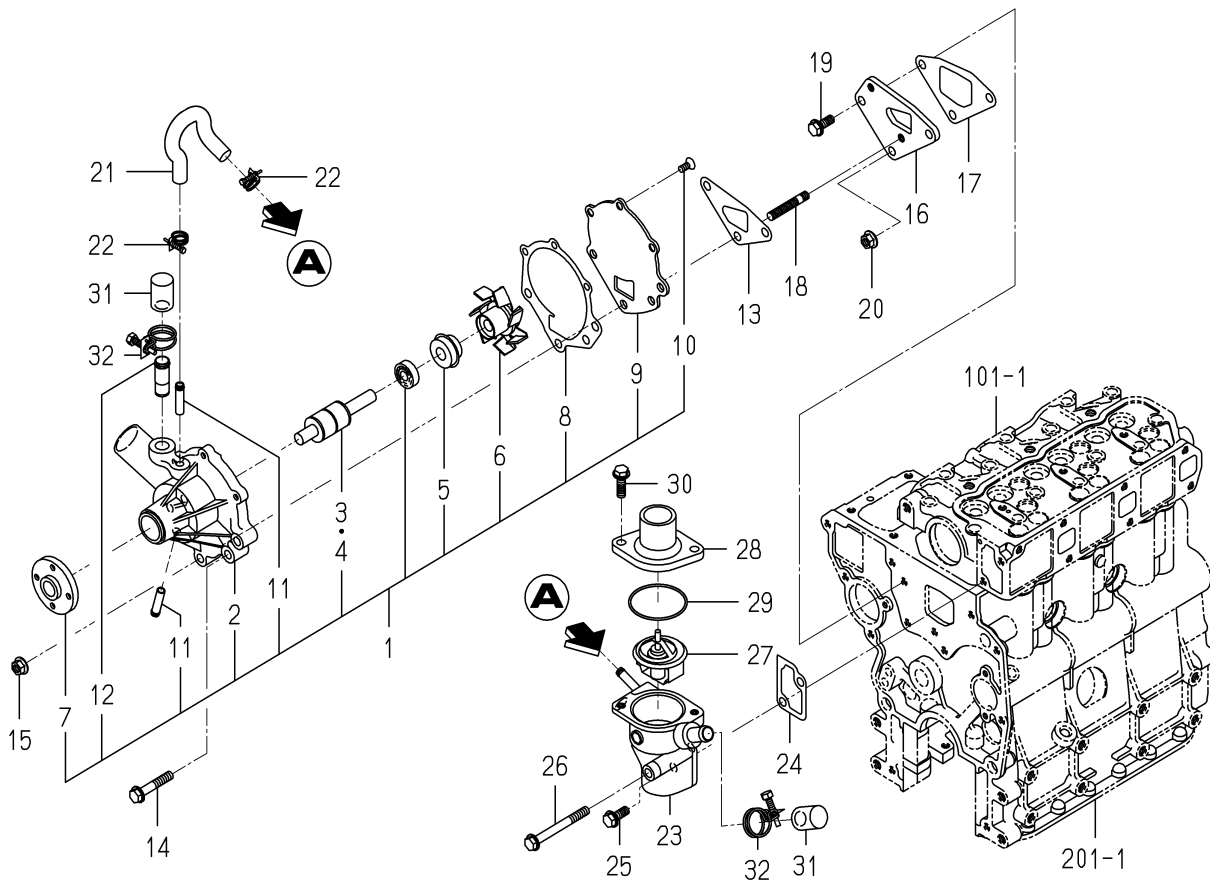
FIG.402 WATER PUMP
