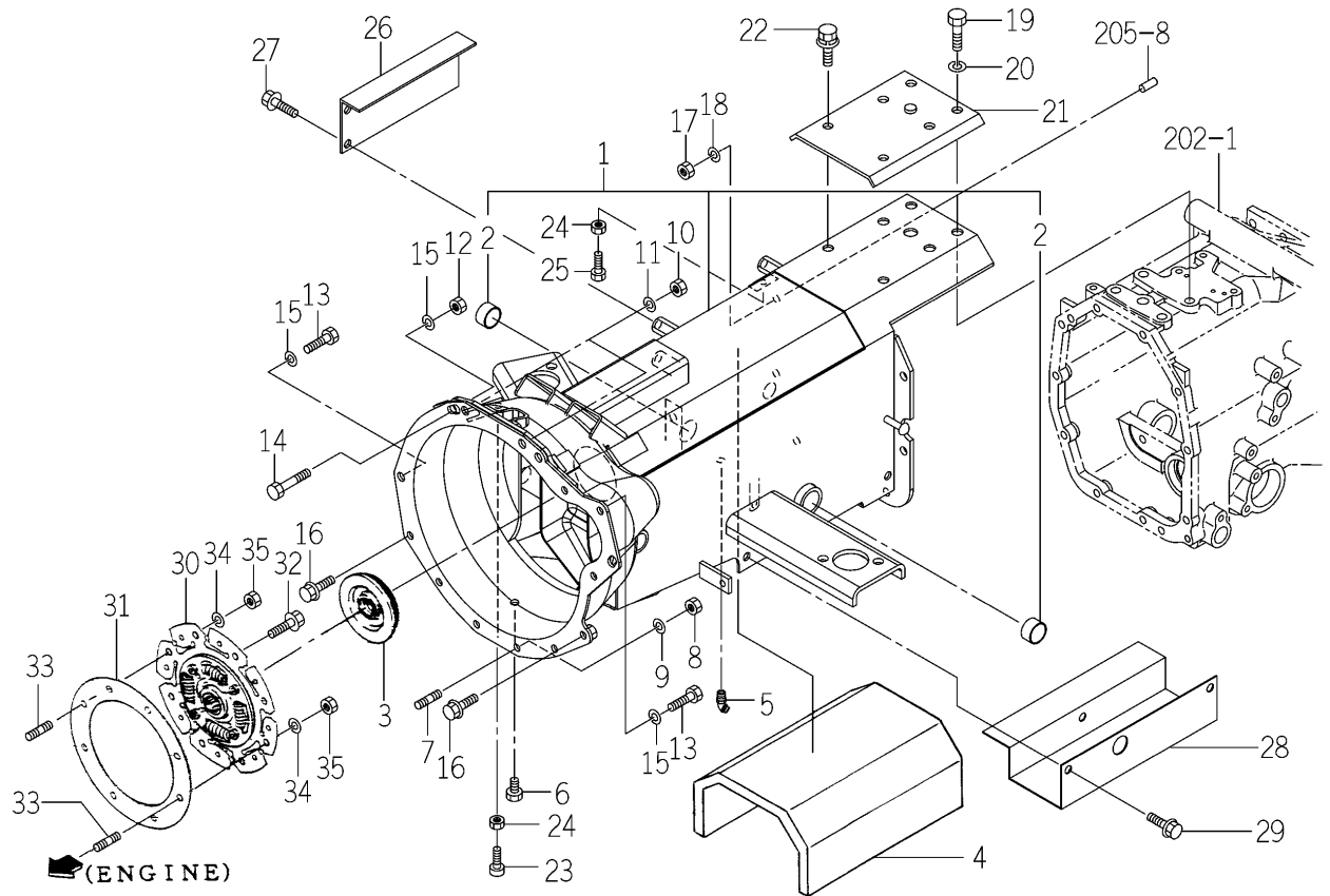
FIG.119 CLUTCH HOUSING SYSTEM (TM3265-H TYPE)
