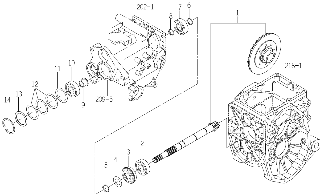
FIG.302 DRIVE PINION SYSYTEM (H TYPE)
