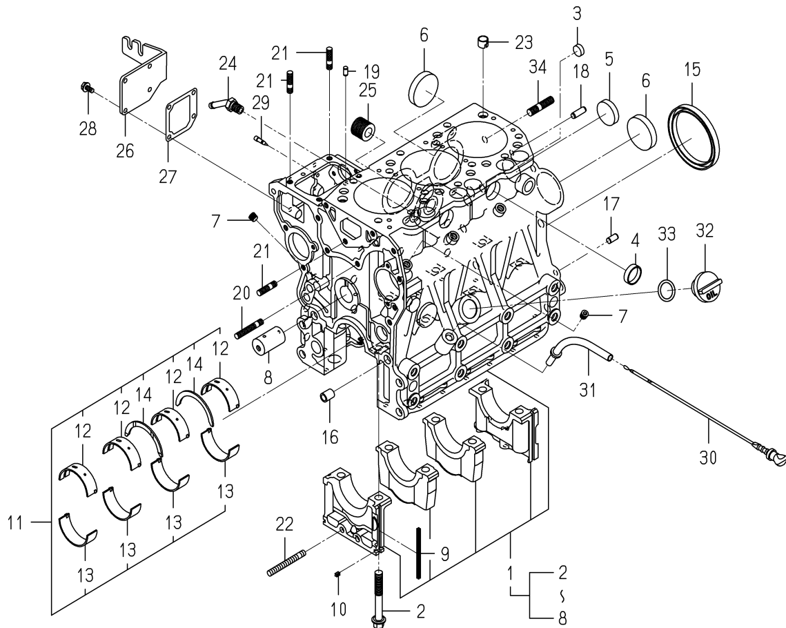
FIG.201 CYLINDER BLOCK
