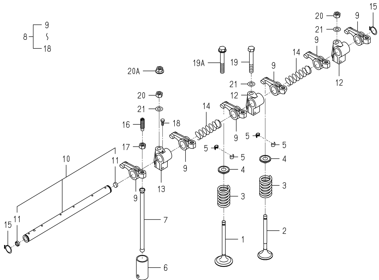
FIG.301 VALVE
