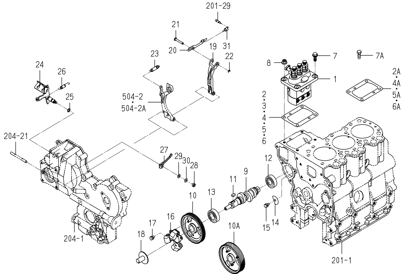
FIG.502 INJECTION PUMP
