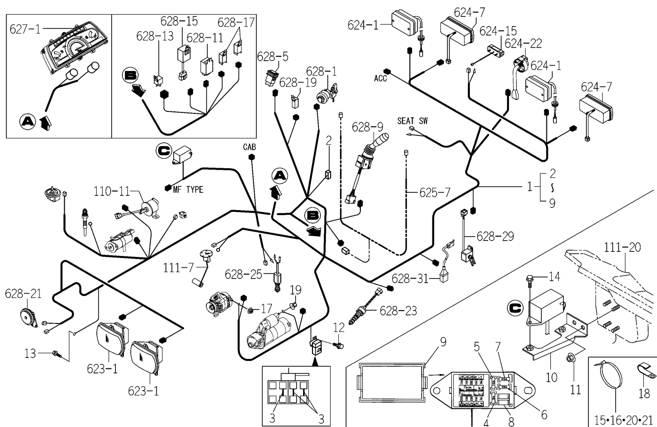
FIG.632 HARNESS SYSTEM (EXCEPT H TYPE)
