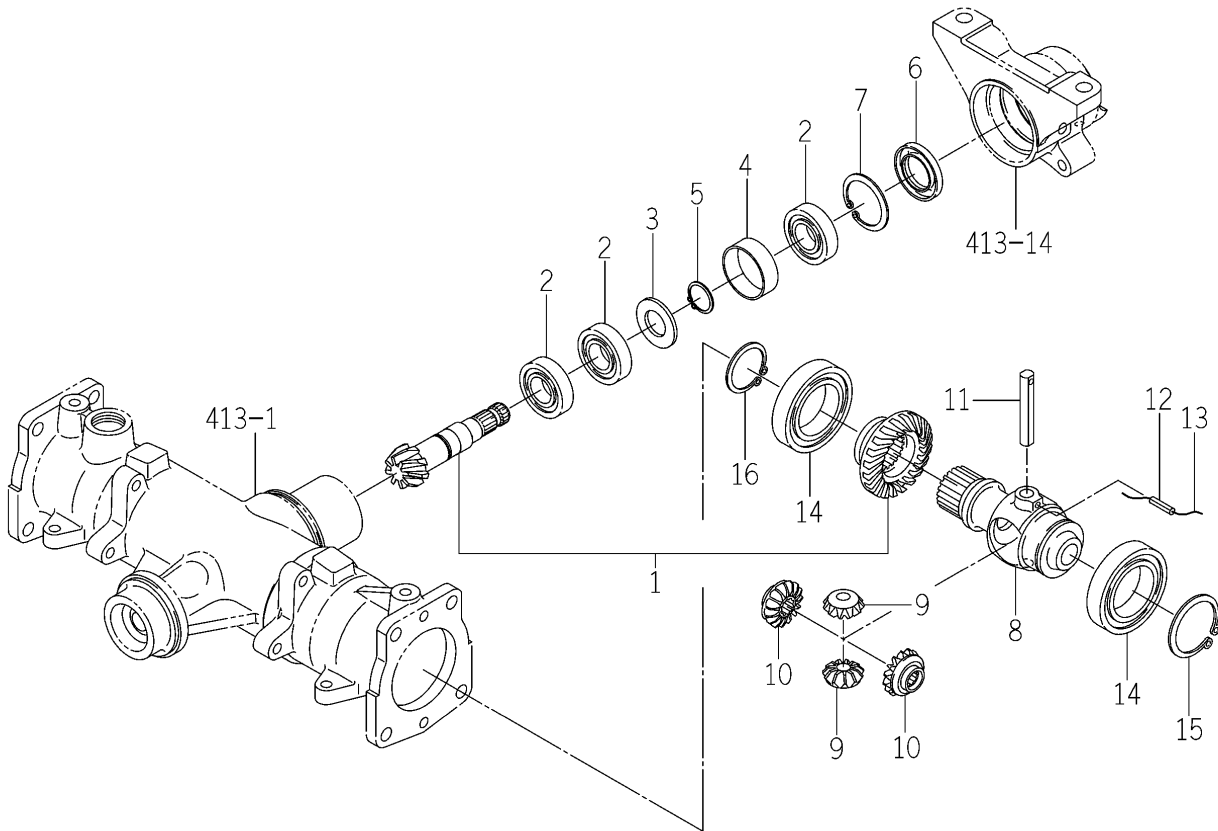
FIG.412 PINION (DRIVE) SYSYTEM
