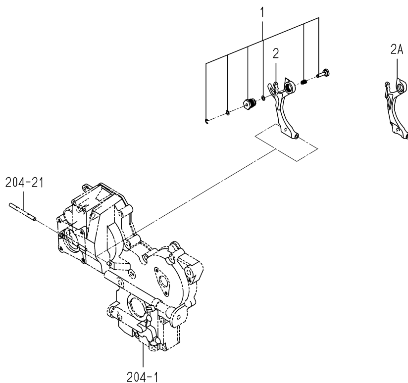
FIG.504 ADAPTER
