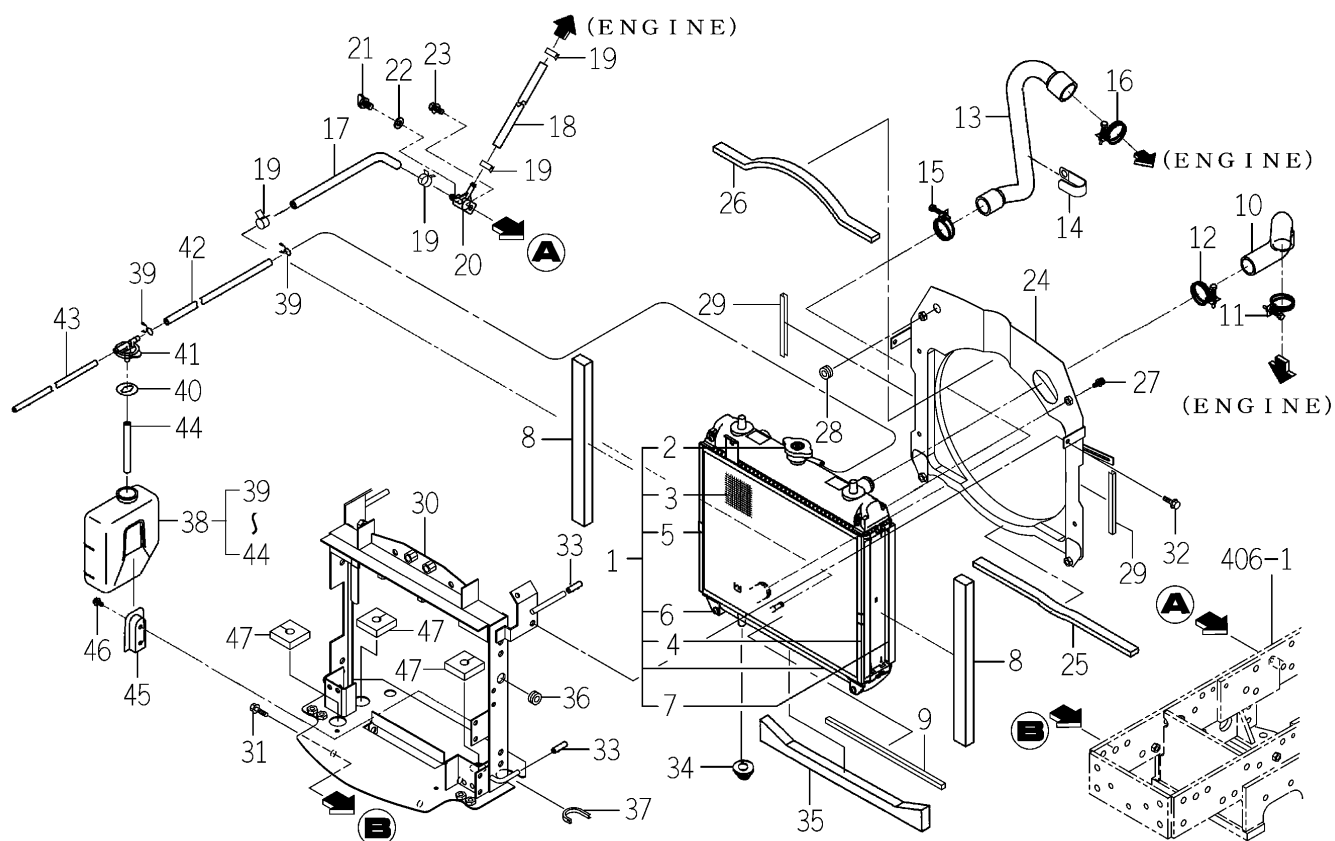
FIG.102 RADIATOR SYSTEM (TM3215,3245-H TYPE)
