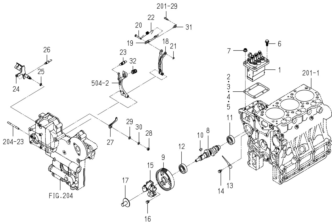
FIG.502 INJECTION PUMP
