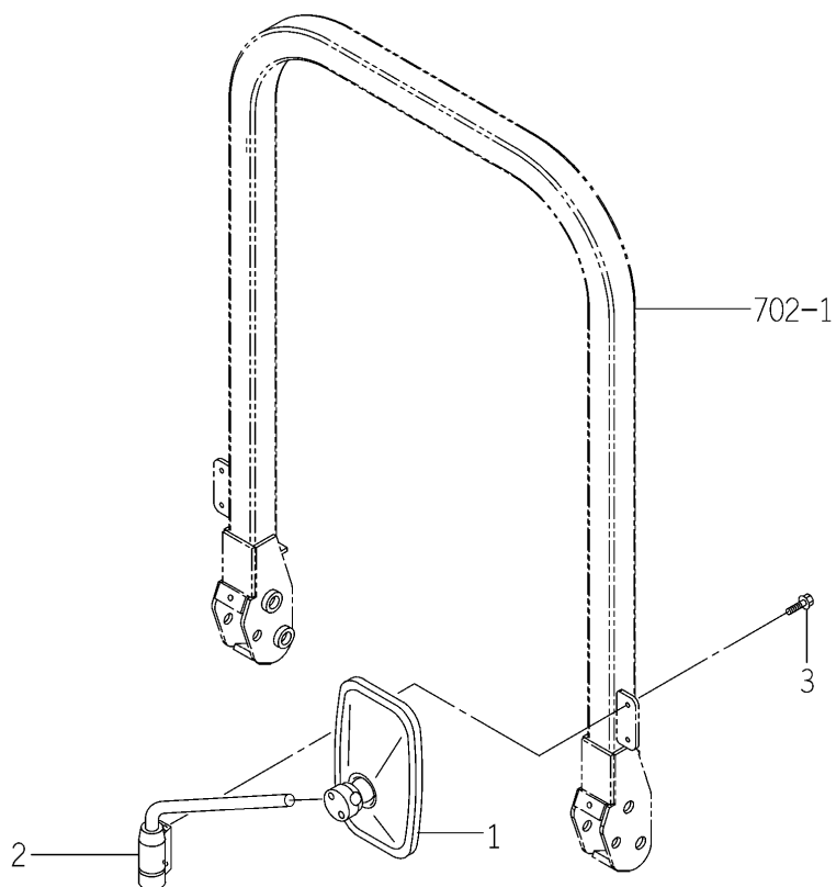
FIG.611 MIRROR SYSTEM (A TYPE)
