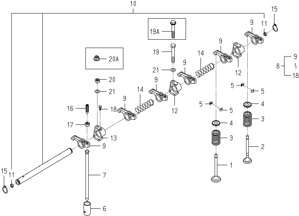
FIG.301 VALVE
