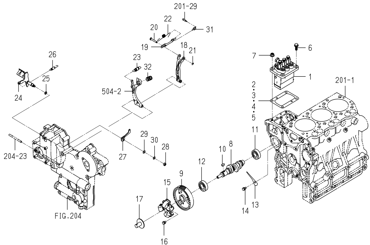
FIG.502 INJECTION PUMP
