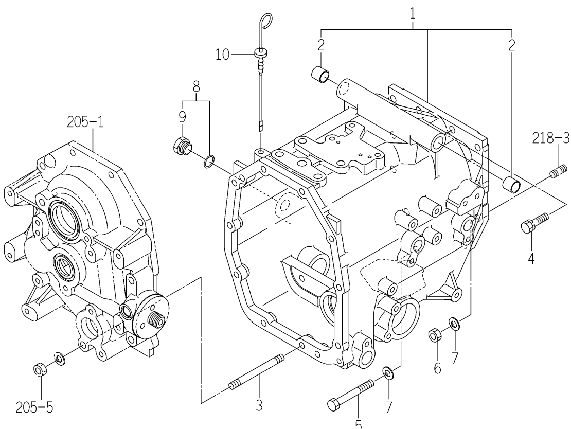
FIG.202 FRONT MISSION CASE SYSTEM (H TYPE)
