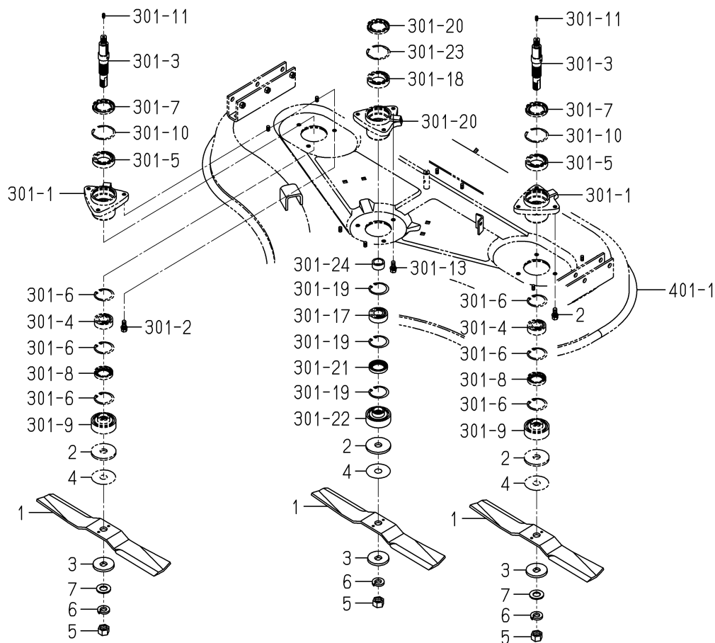
FIG.302 BLADE SYSTEM
