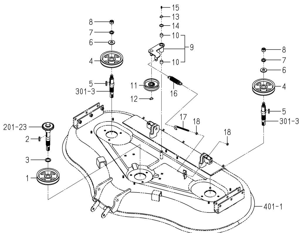
FIG.202 PULLEY SYSTEM
