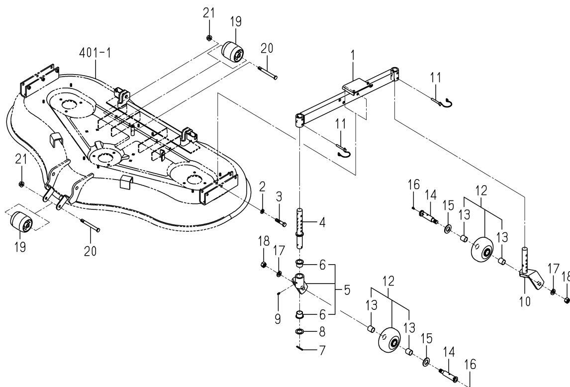
FIG.501 WHEEL(GAUGE) SYSTEM
