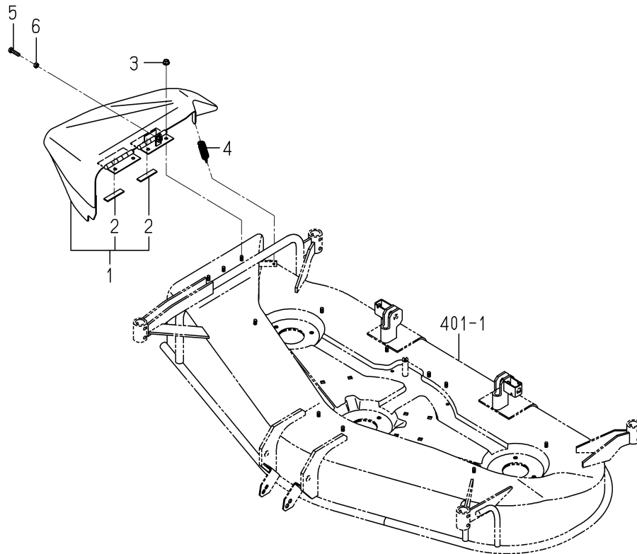
FIG.402 COVER(DISCHARGE)(54) SYSTEM
