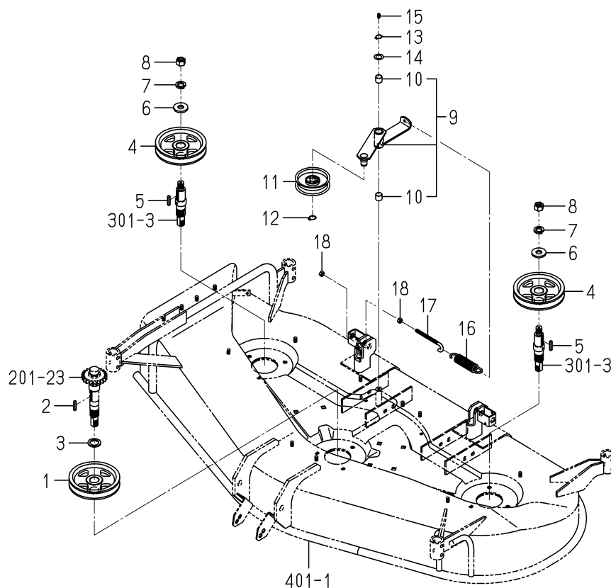
FIG.202 PULLEY SYSTEM
