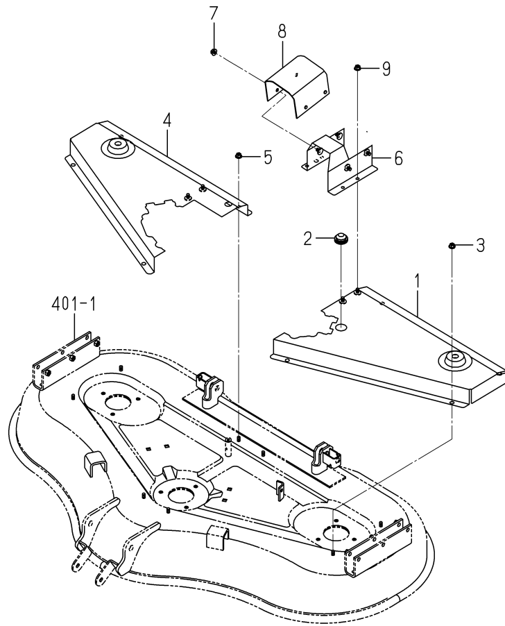
FIG.402 COVER(BELT) SYSTEM
