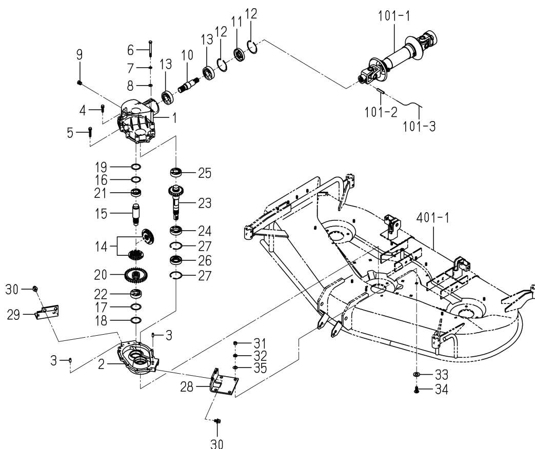
FIG.201 CASE(BEVEL) SYSTEM
