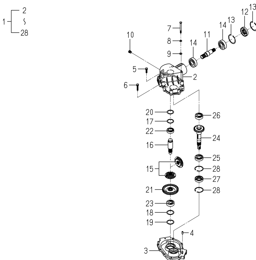
FIG.P01 CASE(BEVEL)ASSY(REPAIR)
