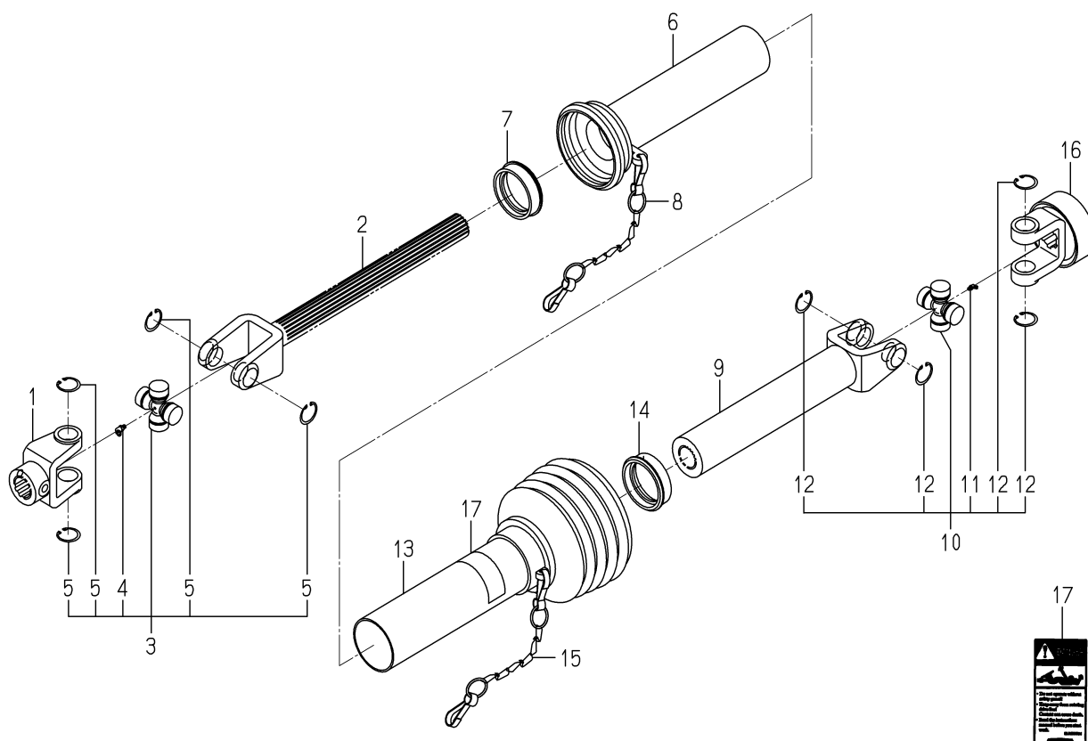
FIG.S01 COMPONENT PARTS FOR 8658-101-820-00 ON Fig.101
