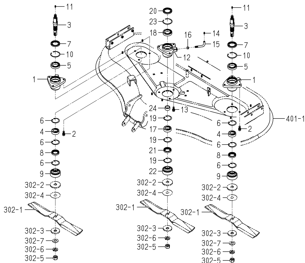
FIG.301 METAL SYSTEM
