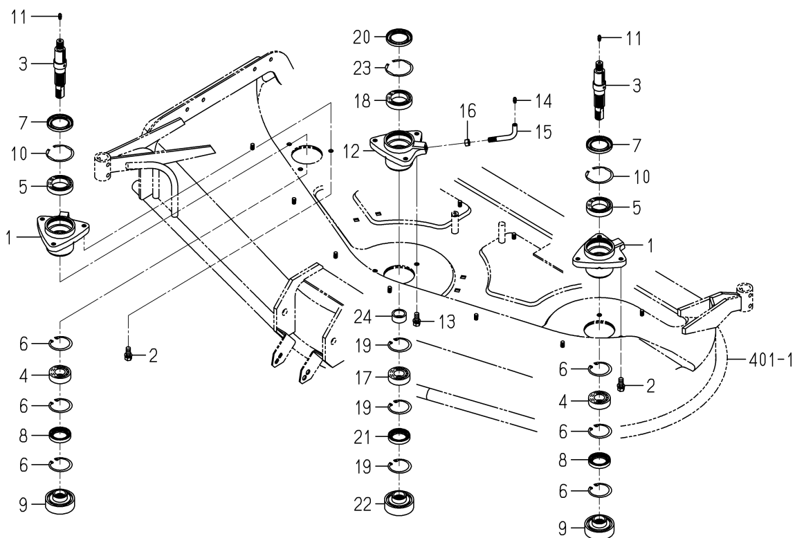
FIG.301 METAL SYSTEM
