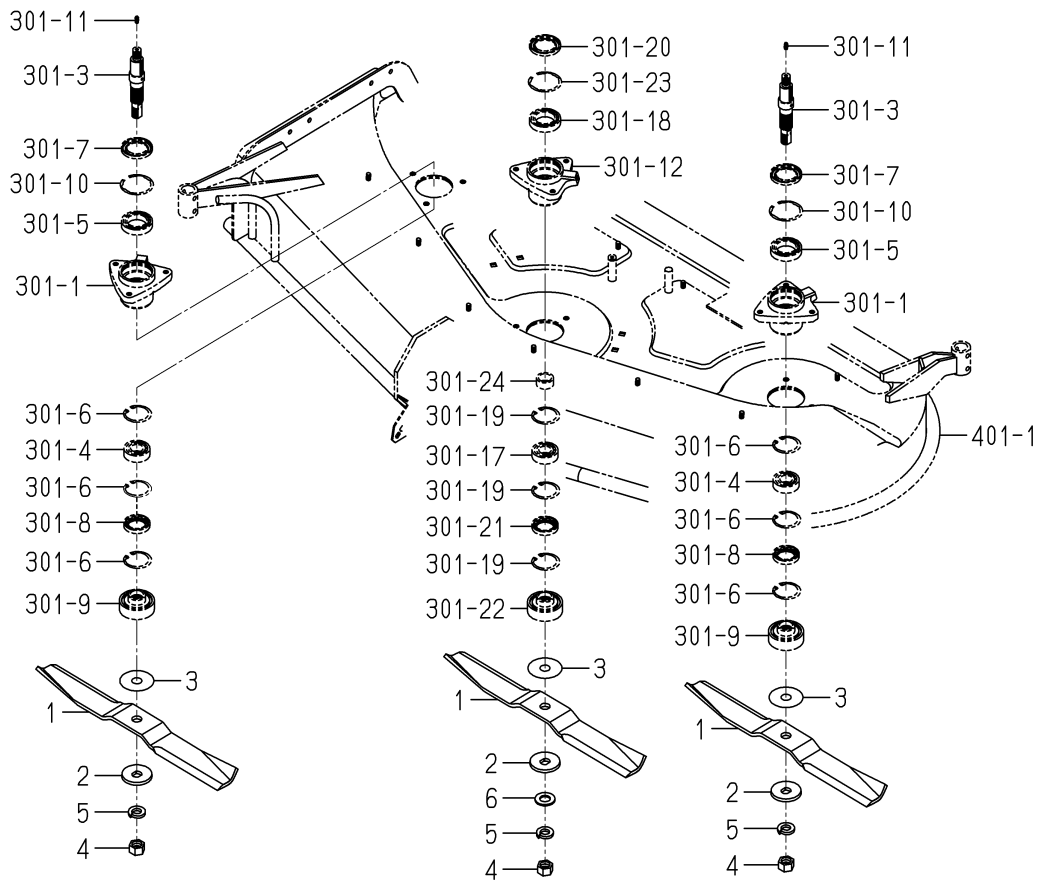
FIG.302 BLADE SYSTEM
