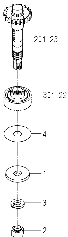
FIG.302 BLADE SYSTEM
