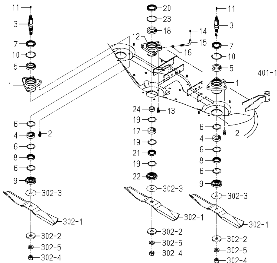
FIG.301 METAL SYSTEM
