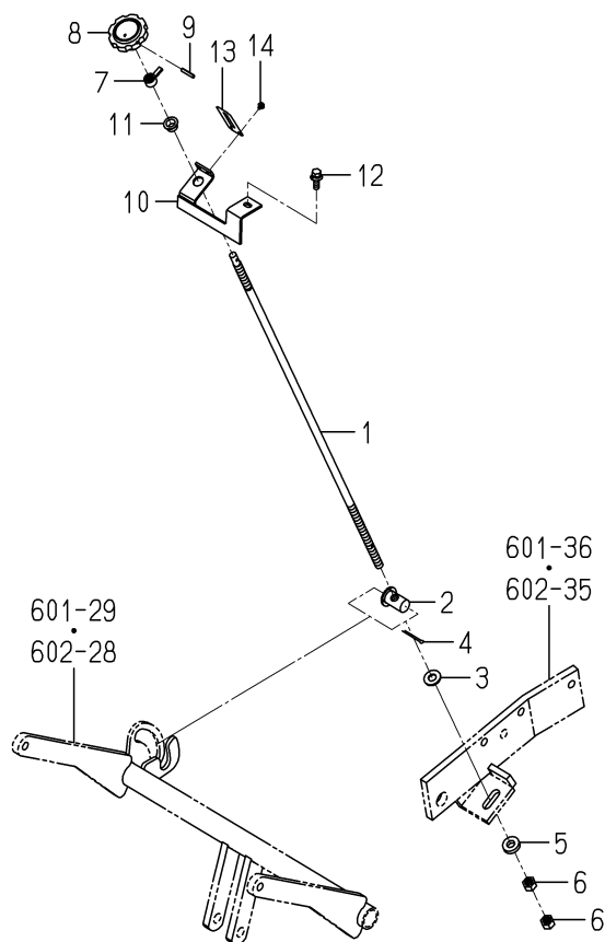
FIG.604 ADJUST(HEIGHT) SYSTEM
