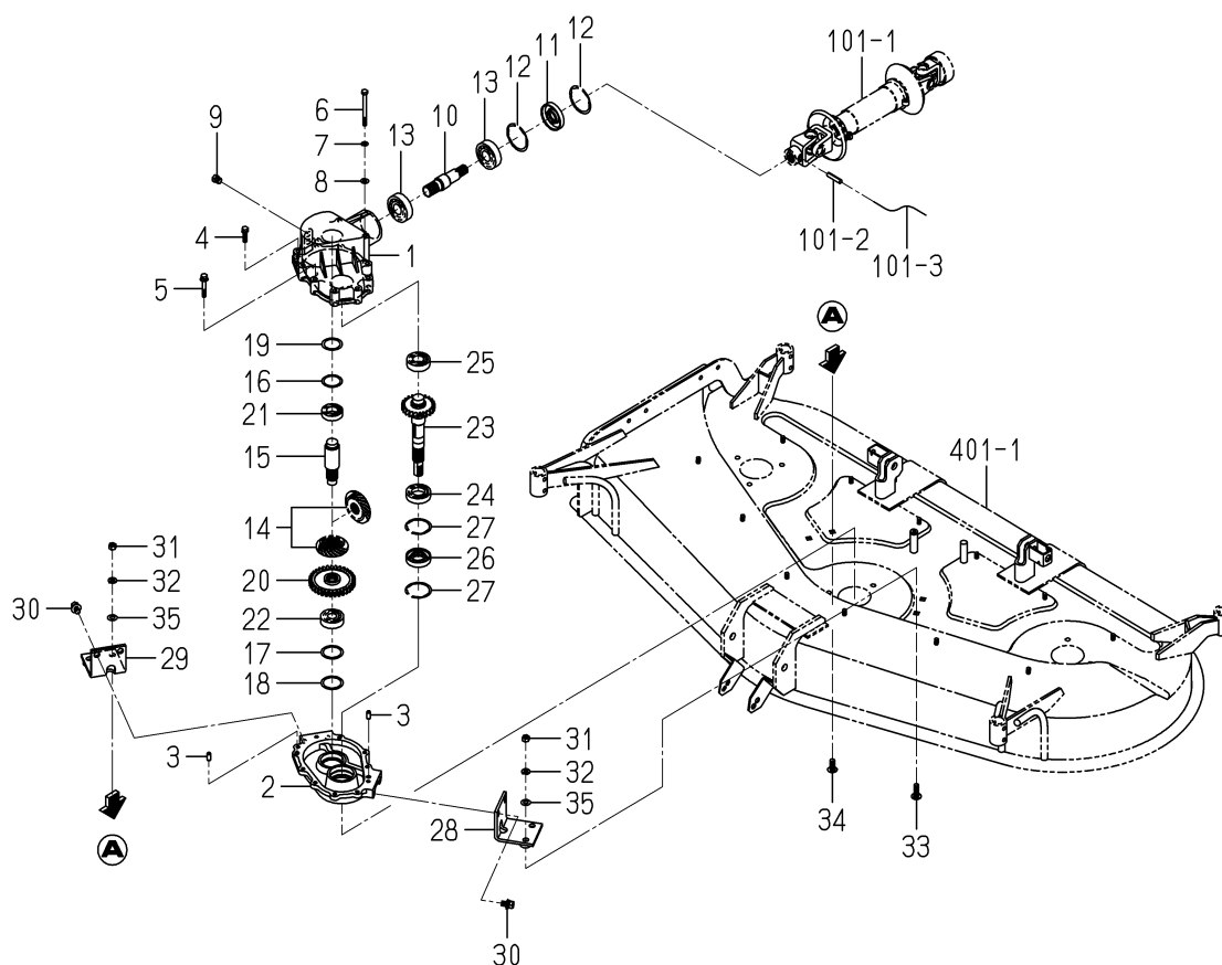
FIG.201 CASE(BEVEL) SYSTEM
