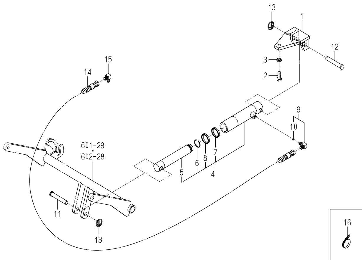
FIG.603 CYLINDER SYSTEM
