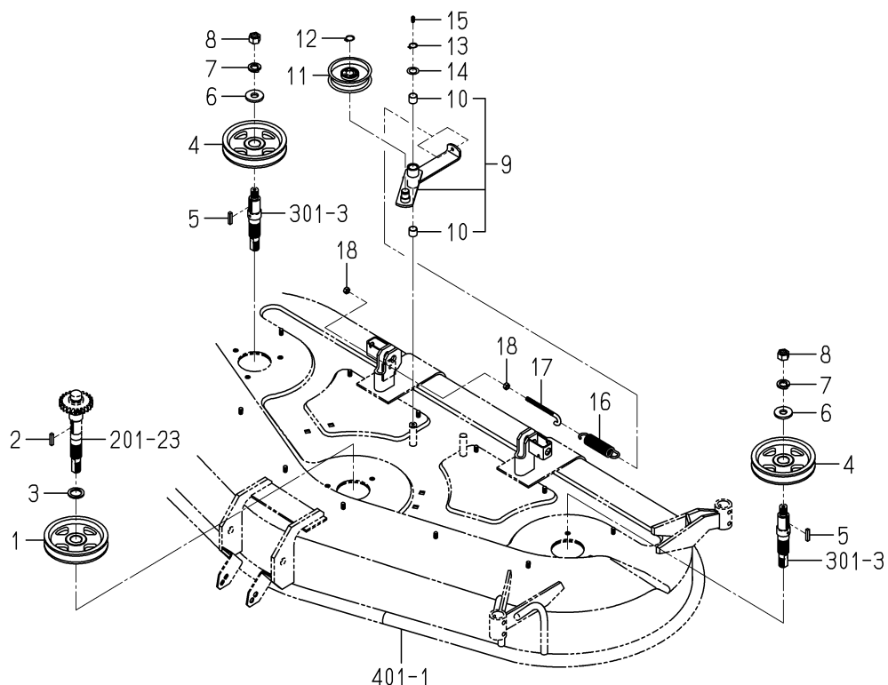
FIG.202 PULLEY SYSTEM
