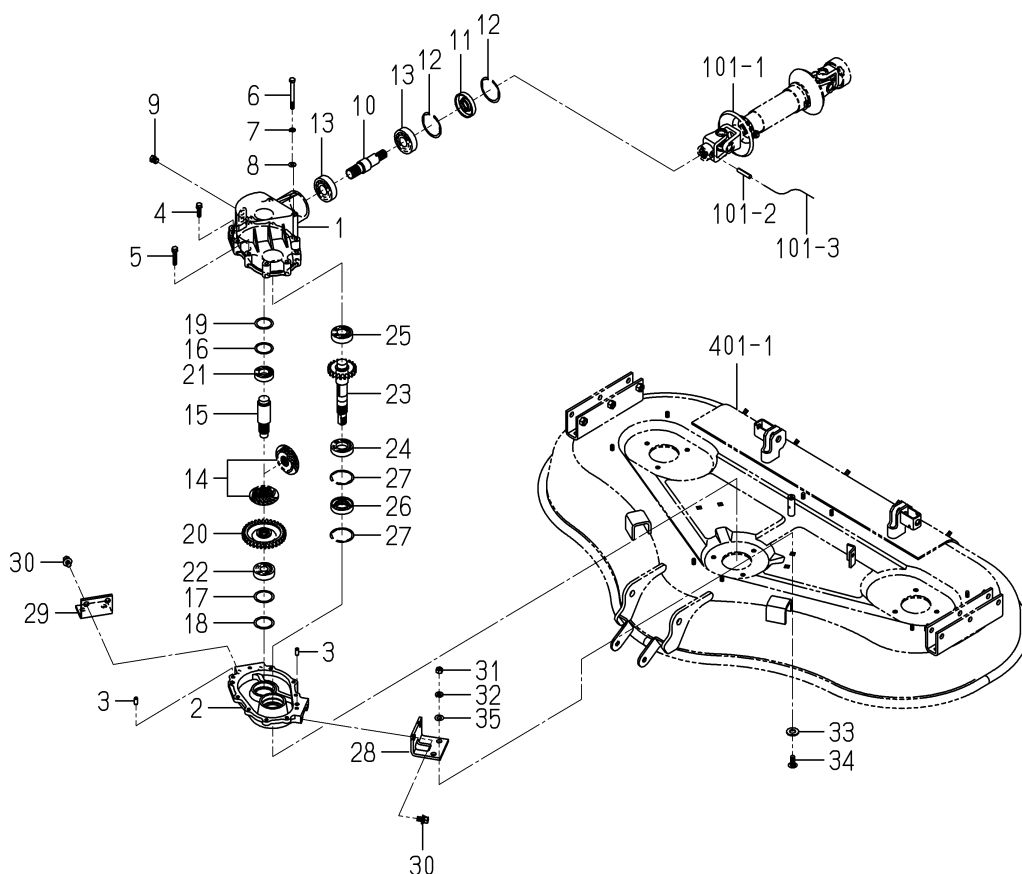
FIG.201 CASE(BEVEL) SYSTEM
