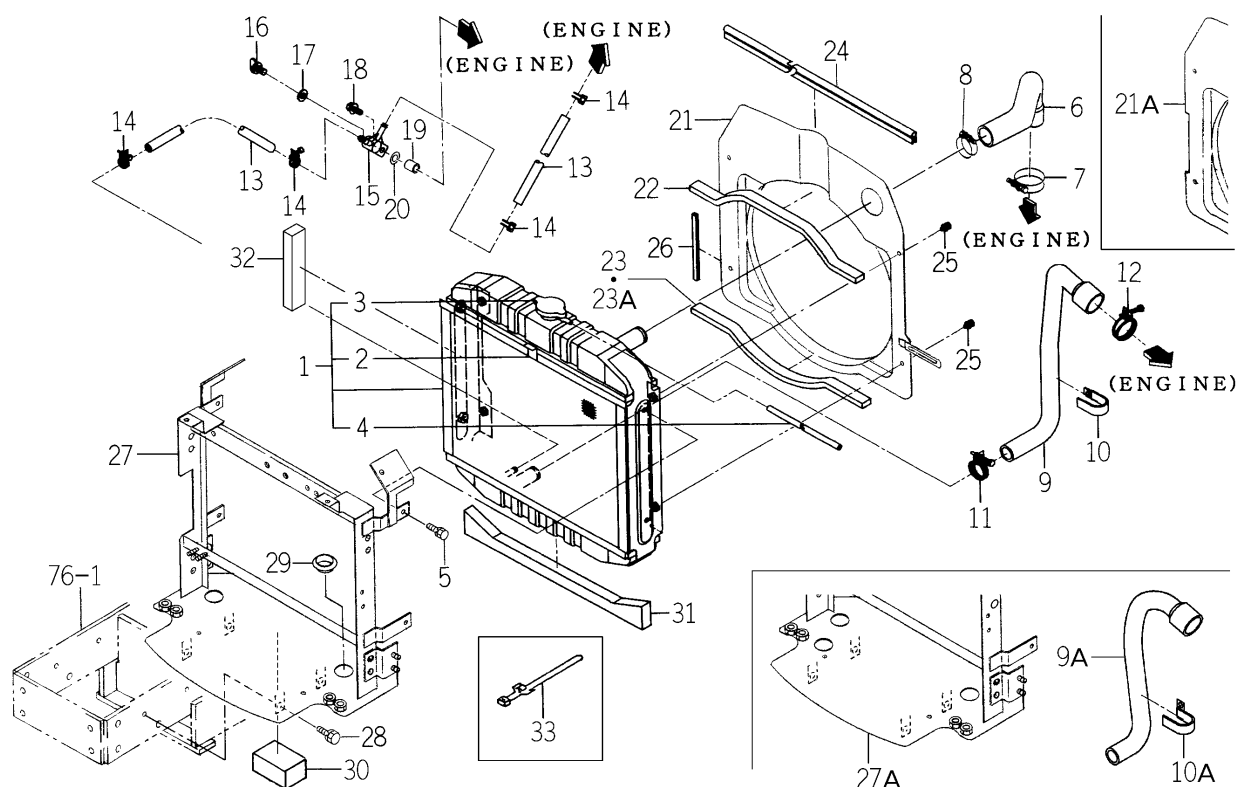
FIG. 1 RADIATOR SYSTEM (EXCEPT H TYPE-TM3200-No.1-1307/ TM3240-No.1-932)
