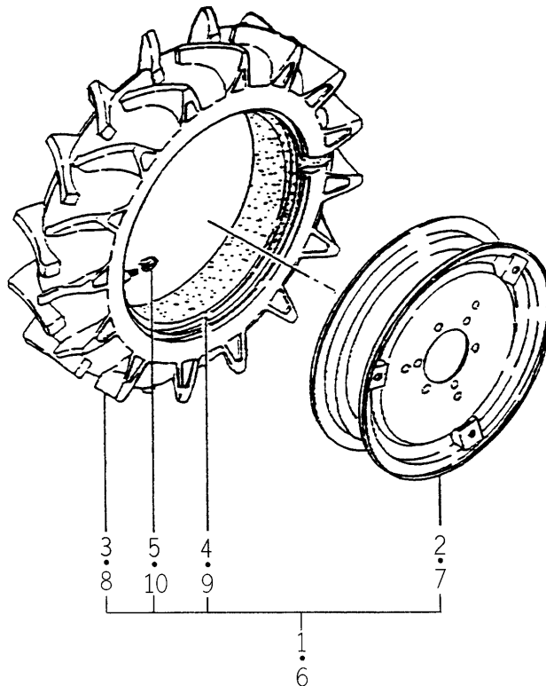
FIG.140 REAR WHEEL (LOW LUG) SYSTEM (TM3200-OPTION)
