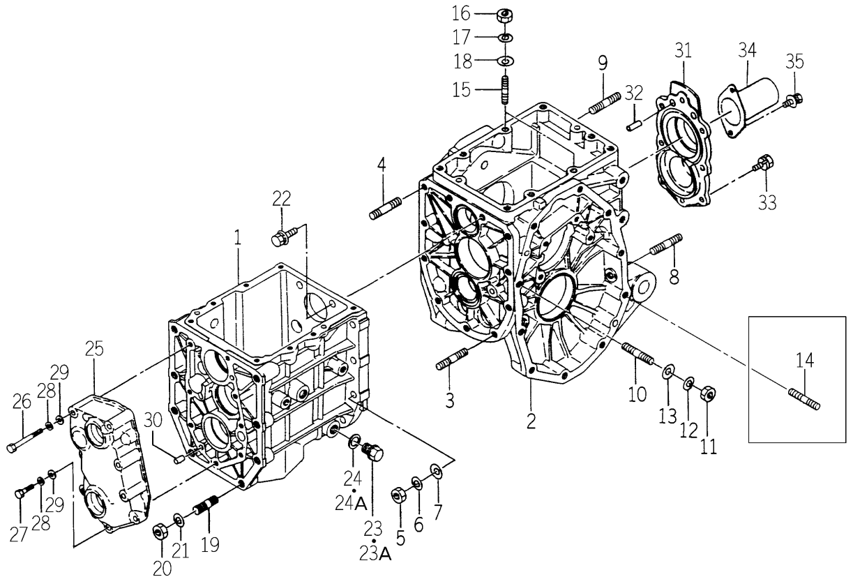
FIG. 19 CASE (TRANSMISSION) SYSTEM (EXCEPT H TYPE)
