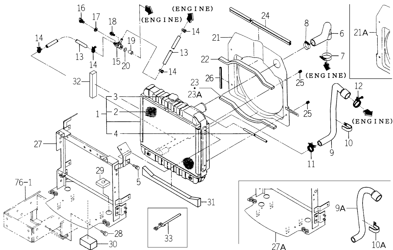
FIG. 2 RADIATOR SYSTEM (H TYPE-TM3200H-No.1-1307/TM3240H-No.1-932)
