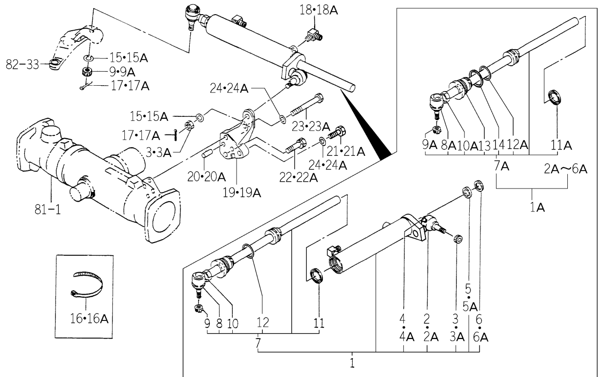
FIG. 69 STEERING SYSTEM (1) (TM3200,3200H-1-270/TM3240,3240H-1-236) (TM3200,3200H-1703-/TM3240,3240H-1214-)
