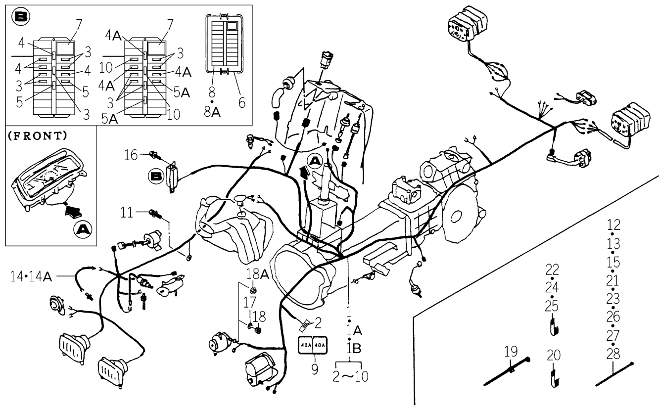
FIG.122 HARNESS SYSTEM (EXCEPT H TYPE)
