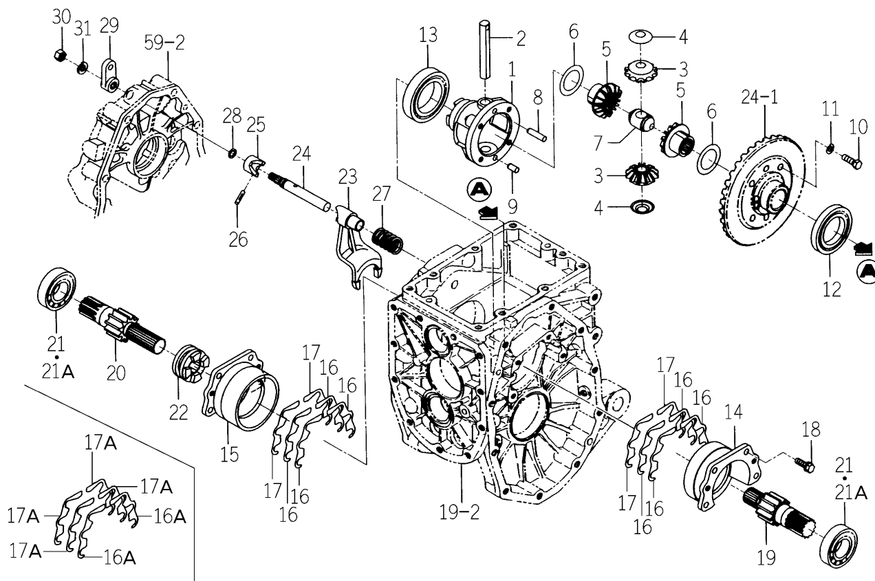
FIG. 58 DIFF CASE SYSTEM
