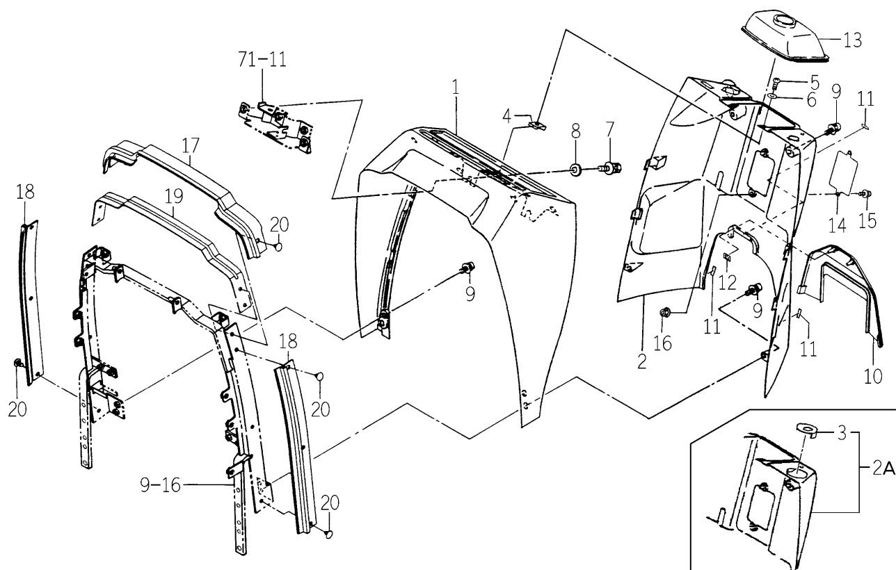
FIG.100 STEERING COVER SYSTEM (EXCEPT H TYPE)
