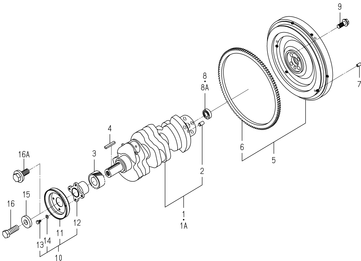
FIG. 17 CRANK SHAFT
