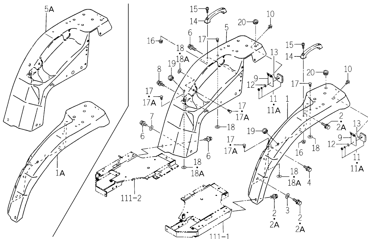
FIG.104 FENDER SYSTEM (TM3200/TM3240-EXCEPT H TYPE)
