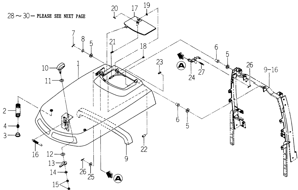
FIG. 97 HOOD SYSTEM(1/2) (TM3200-No.1-1307/TM3200H-No.1-1307/ TM3240-No.1-932/TM3240H-No.1-932)
