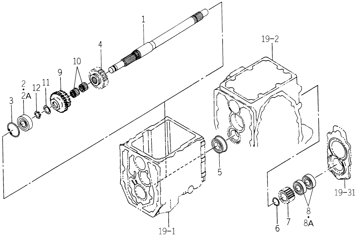
FIG. 38 GEAR (PTO) SYSTEM (TM3200-EXCEPT H TYPE)
