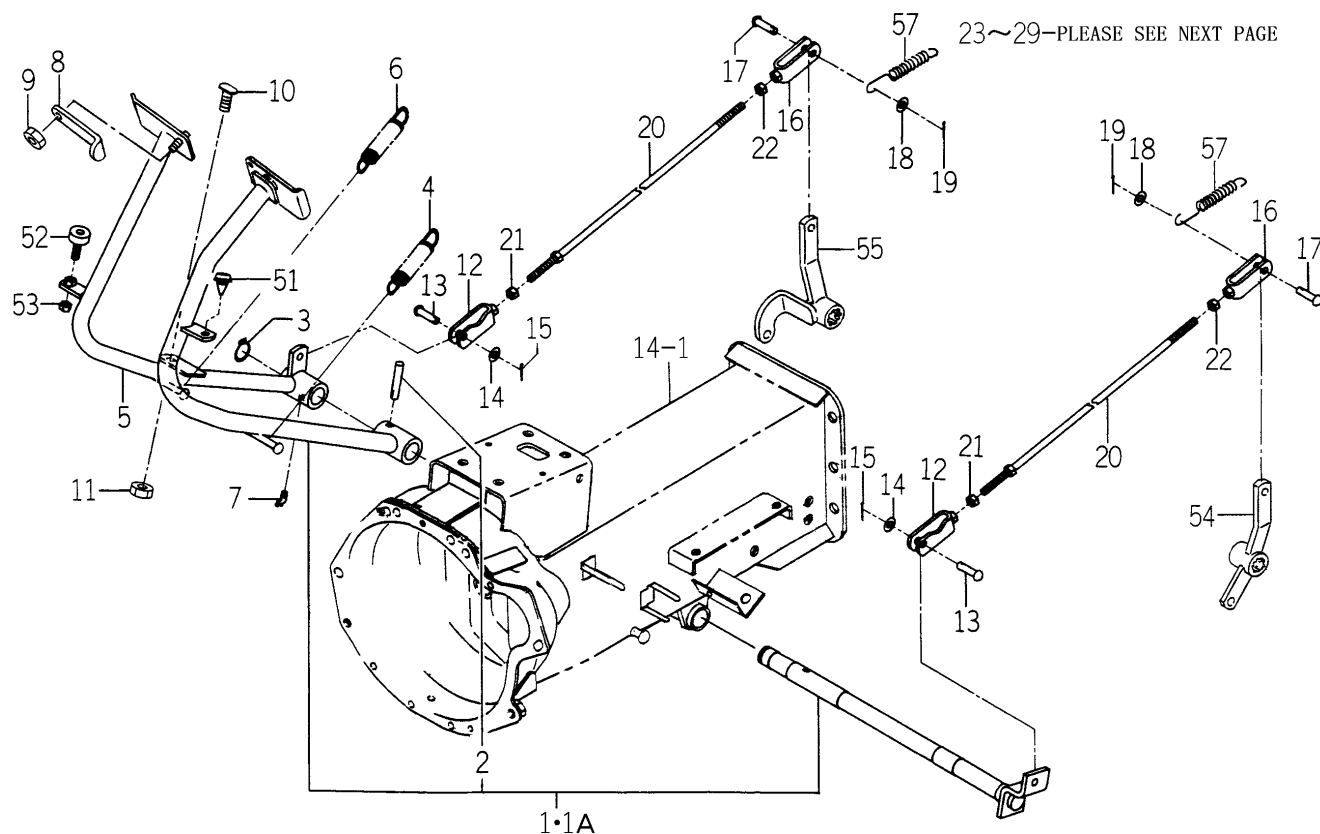
FIG. 65 PEDAL (BRAKE) SYSTEM(1/2) (EXCEPT H TYPE)
