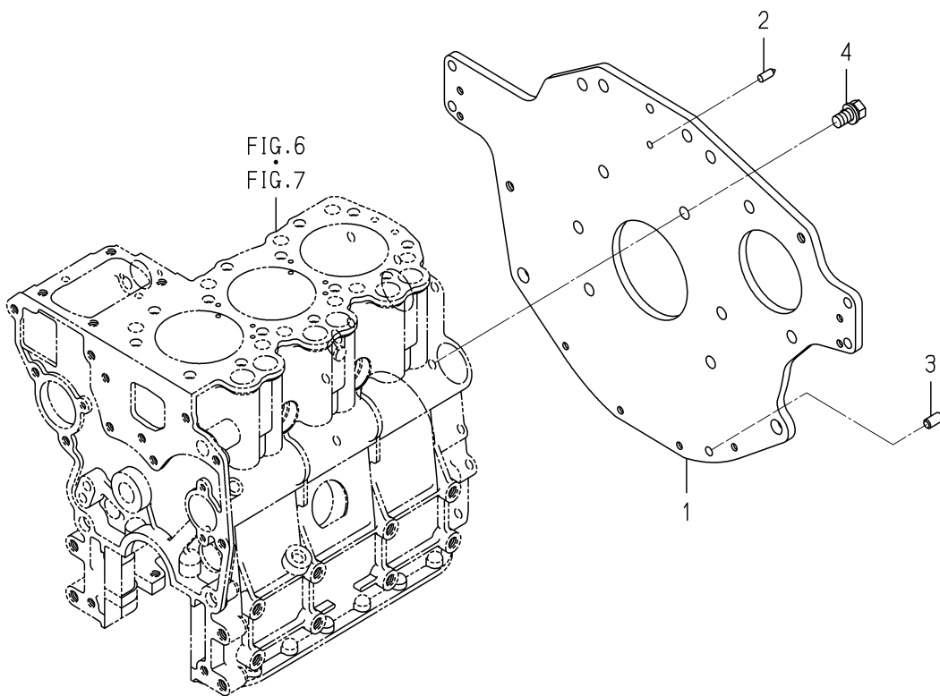
FIG. 10 REAR PLATE
