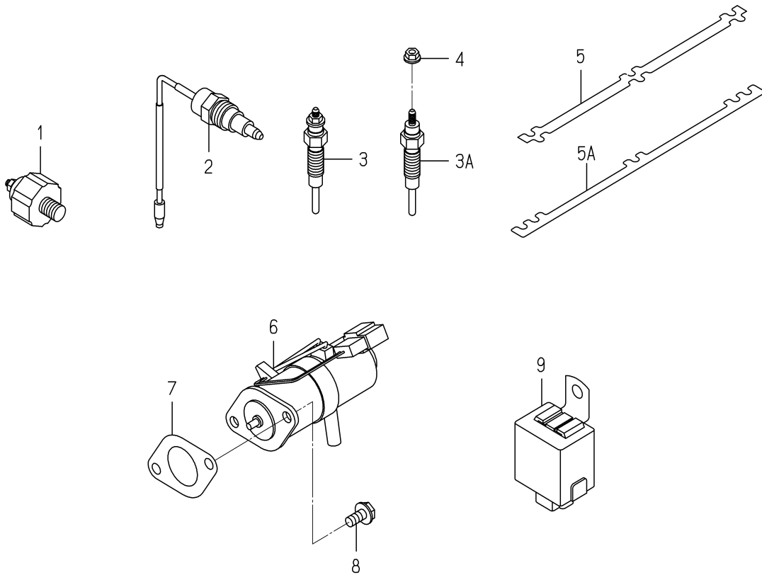
FIG. 28 ELECTRIC (2)
