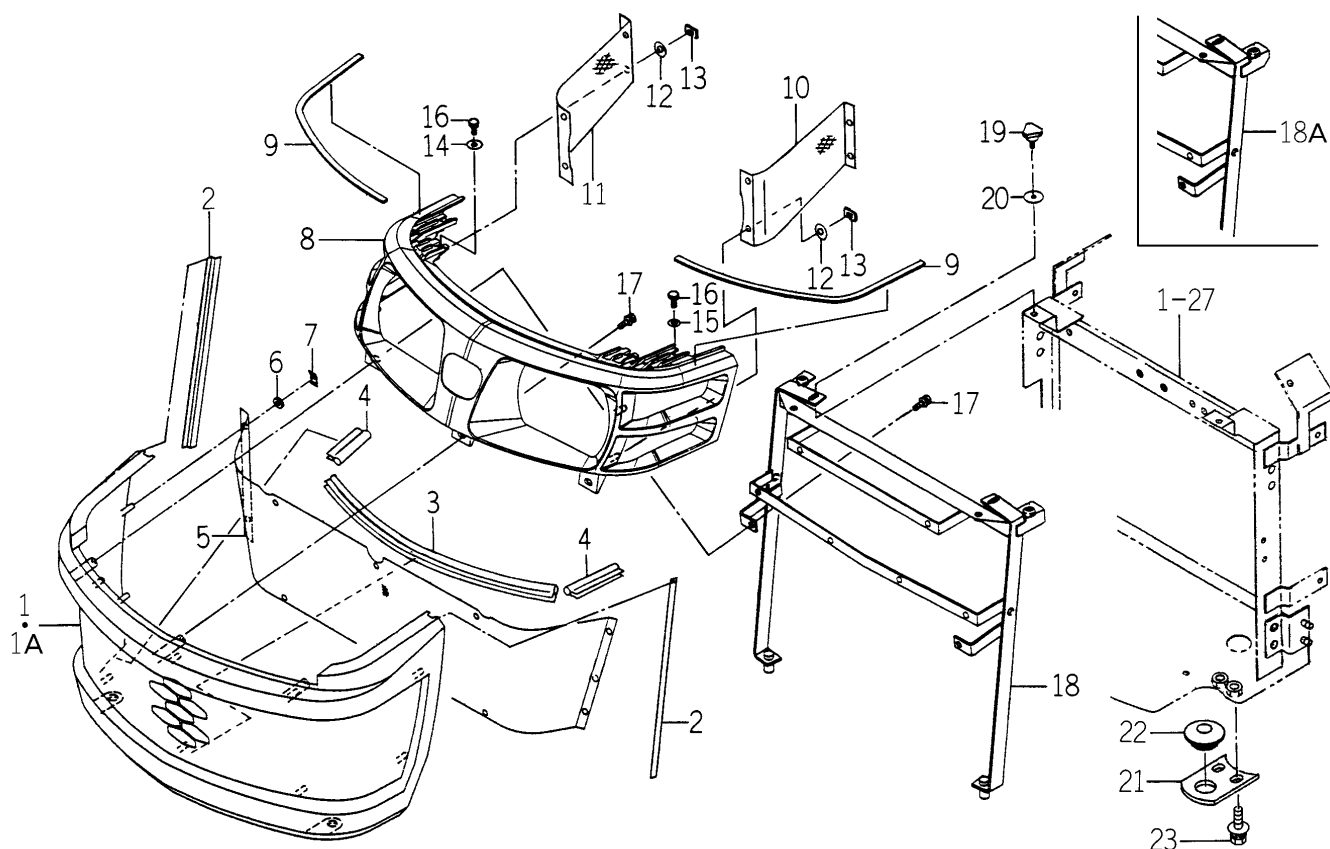
FIG. 99 GRILLE SYSTEM
