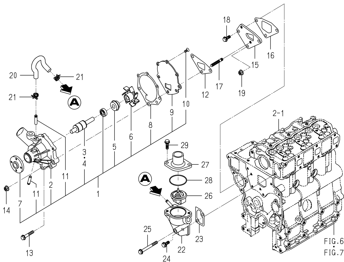
FIG. 19 WATER PUMP
