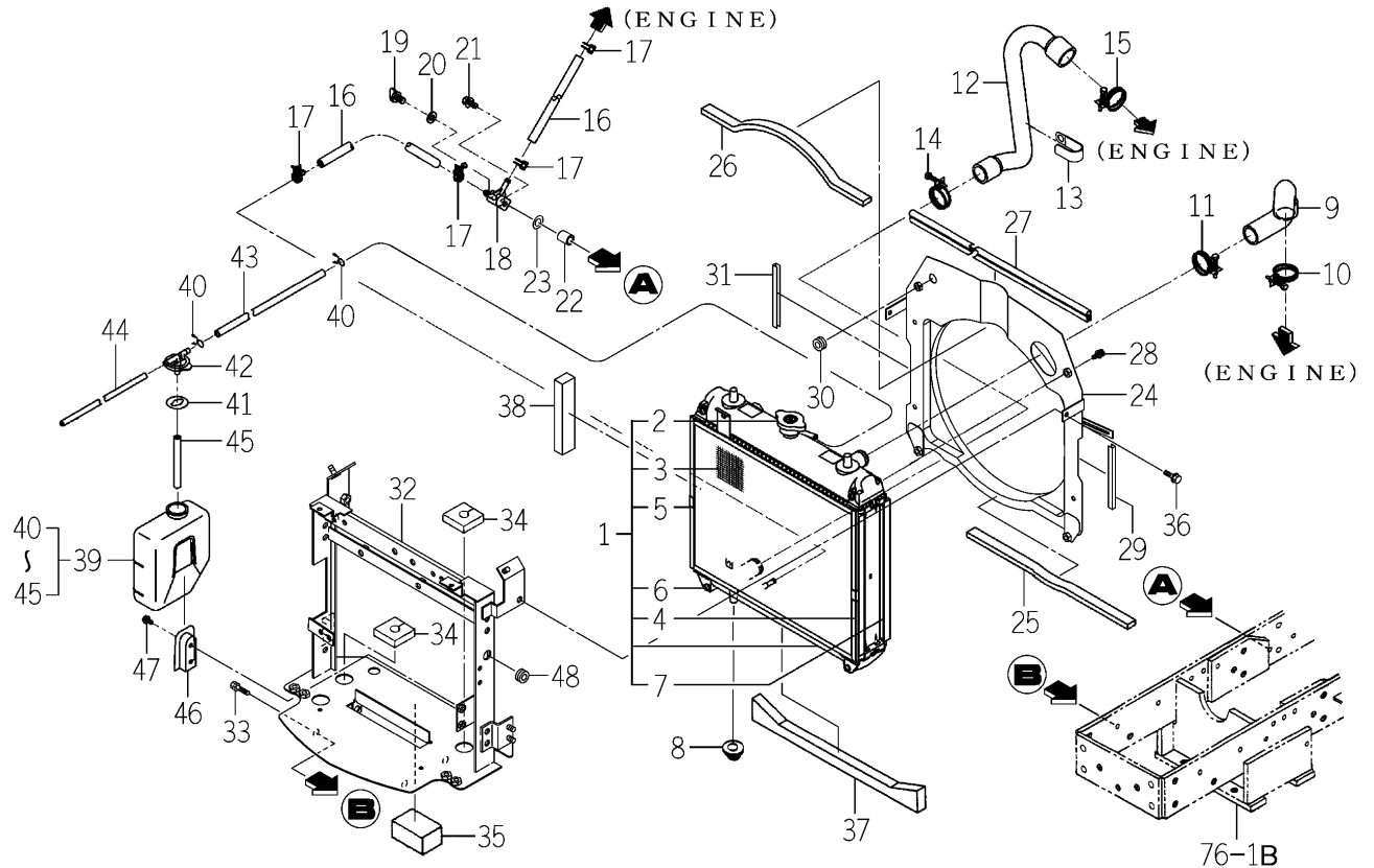
FIG. 4 RADIATOR SYSTEM (H TYPE-TM3200H-No.1308-/TM3240H-No.933-)
