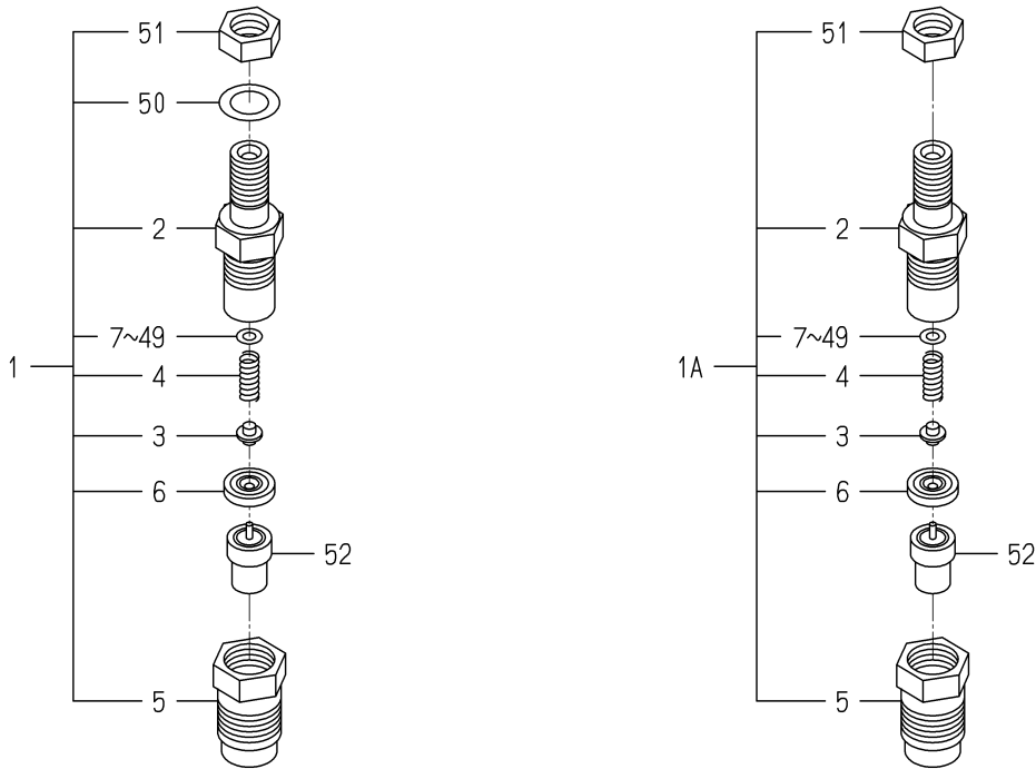
FIG. 30 COMPONENT PARTS FOR 6215-300-036-10 ON Fig.21
