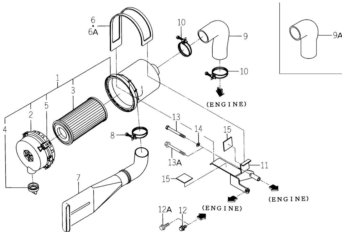
FIG. 6 AIR CLEANER SYSTEM
