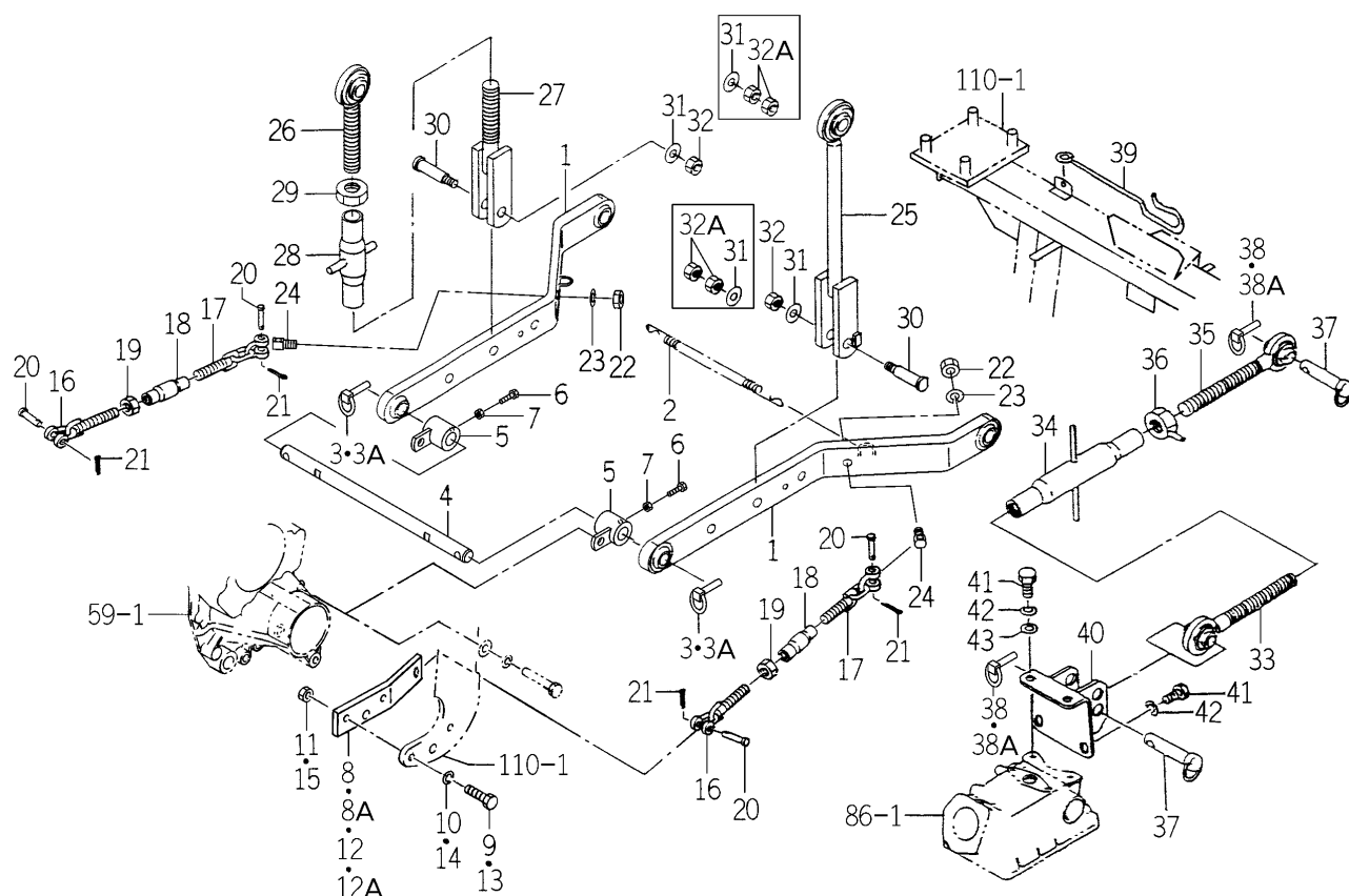
FIG. 95 LINK (3P) SYSTEM
