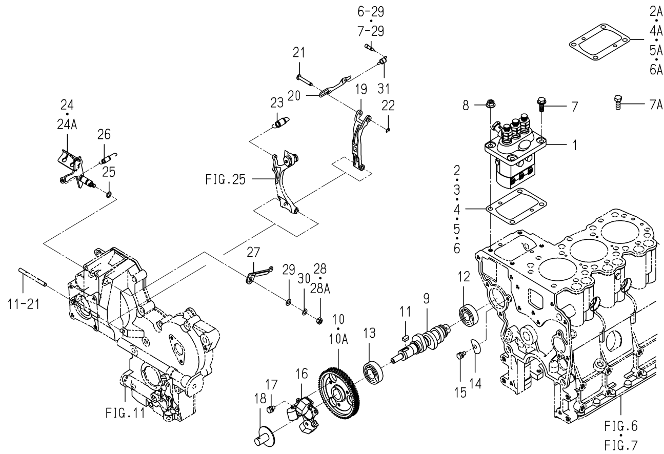
FIG. 23 INJECTION PUMP
