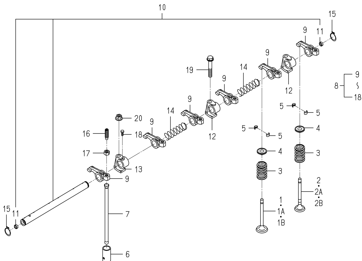
FIG. 13 VALVE
