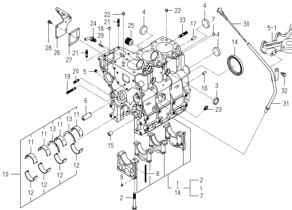
FIG. 6 CYLINDER BLOCK
