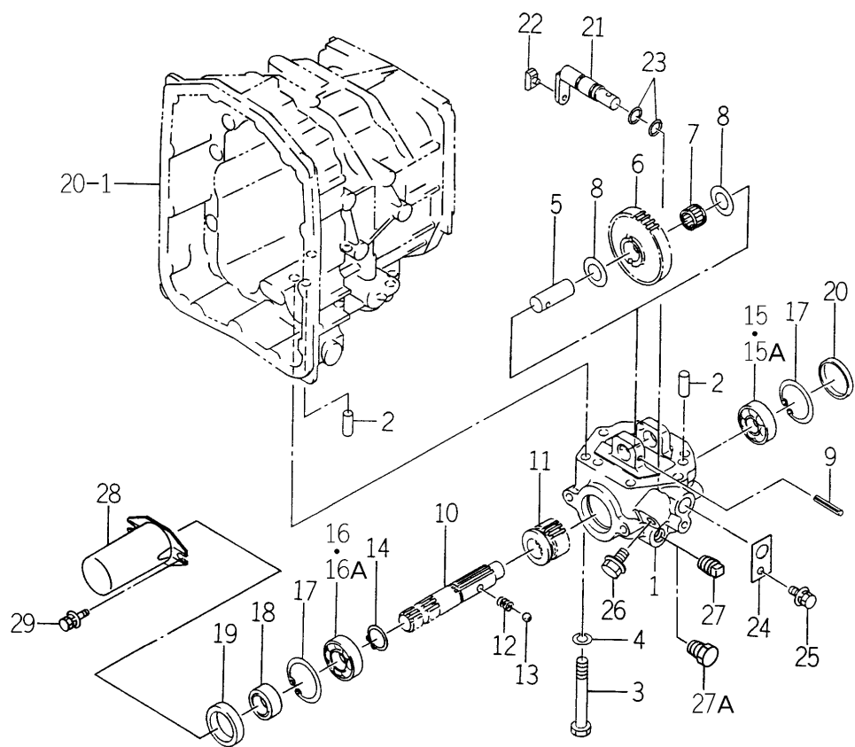
FIG. 45 MID PTO SYSTEM (H TYPE)
