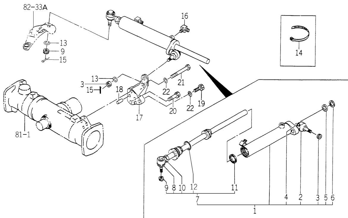
FIG. 70 CYLINDER SYSTEM (TM3200-No.271-1702/TM3200H-No.271-1702/ TM3240-No.237-1213/TM3240H-No.237-1213)
