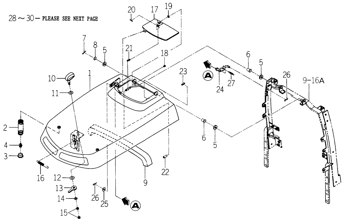
FIG. 98 HOOD SYSTEM(1/2) (TM3200-No.1308-/TM3200H-No.1308-/ TM3240-No.933-/TM3240H-No.933-)
