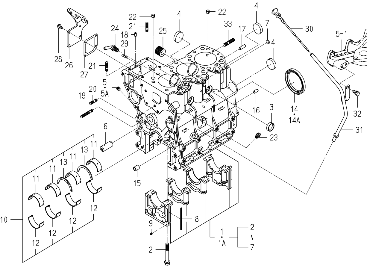
FIG. 7 CYLINDER BLOCK
