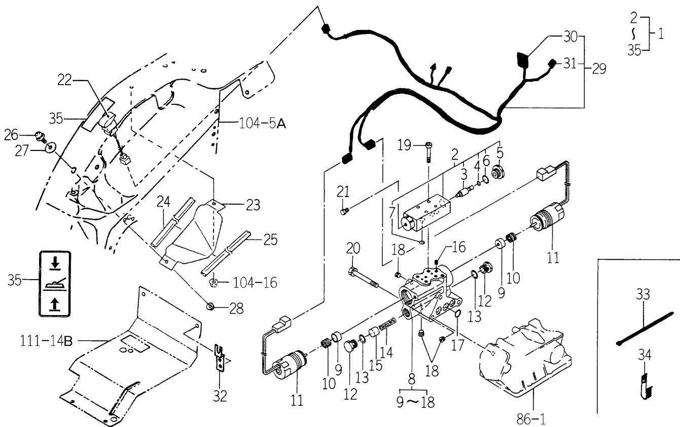
FIG.147 VALVE (AUX/SOL) SET (OPTION)
