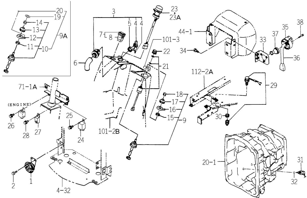
FIG.121 SWITCH SYSTEM (H TYPE-TM3200H-No.1308-/TM3240H-No.933-)
