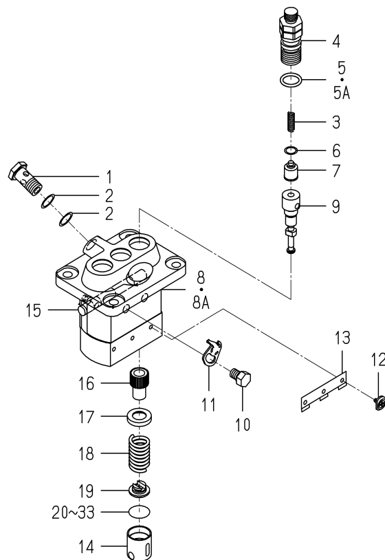
FIG. 31 COMPONENT PARTS FOR 6215-600-103-10 ON Fig.22
