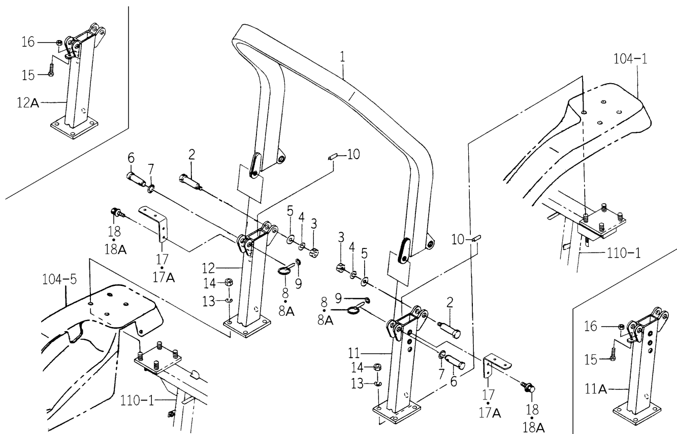
FIG.124 ROPS SYSTEM (R TYPE)
