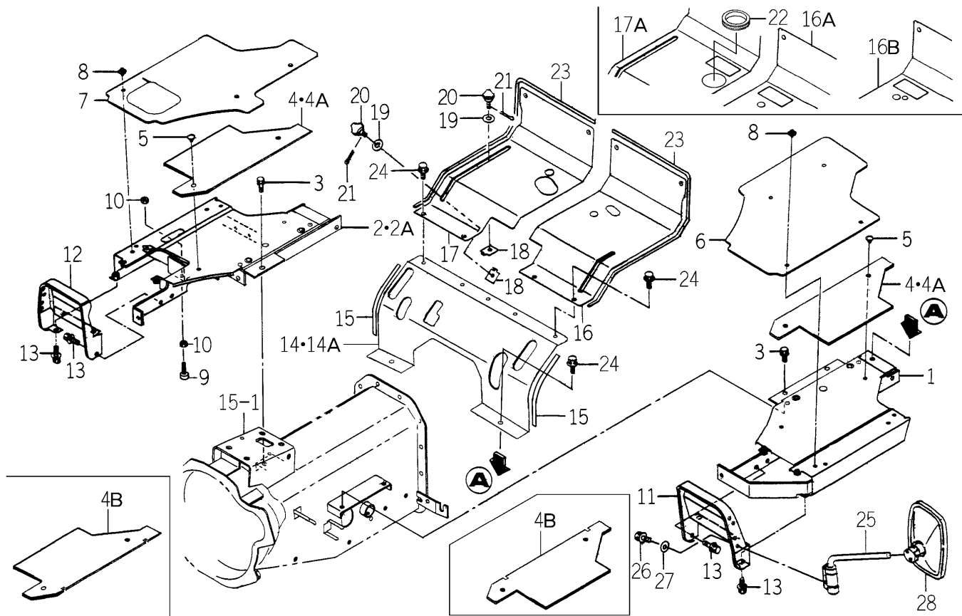
FIG.112 STEP SYSTEM (H TYPE)
