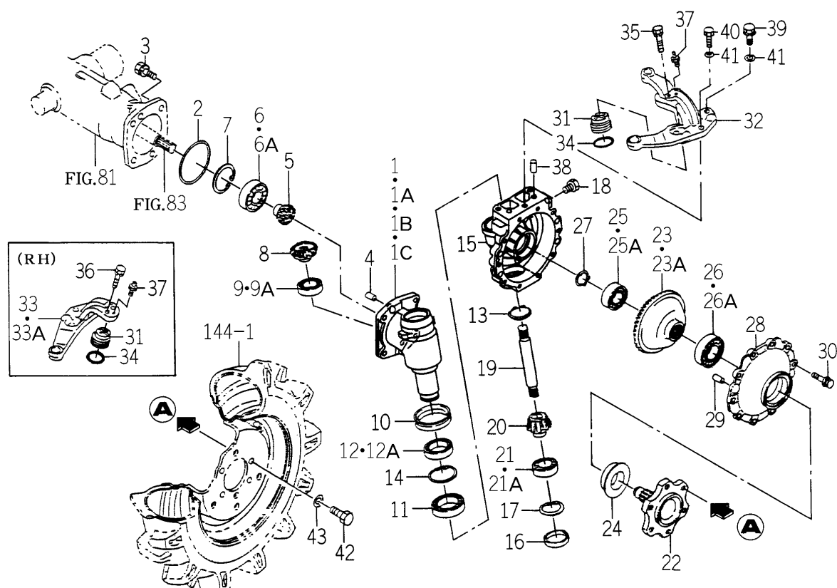
FIG. 82 GEAR (FINAL) SYSTEM
