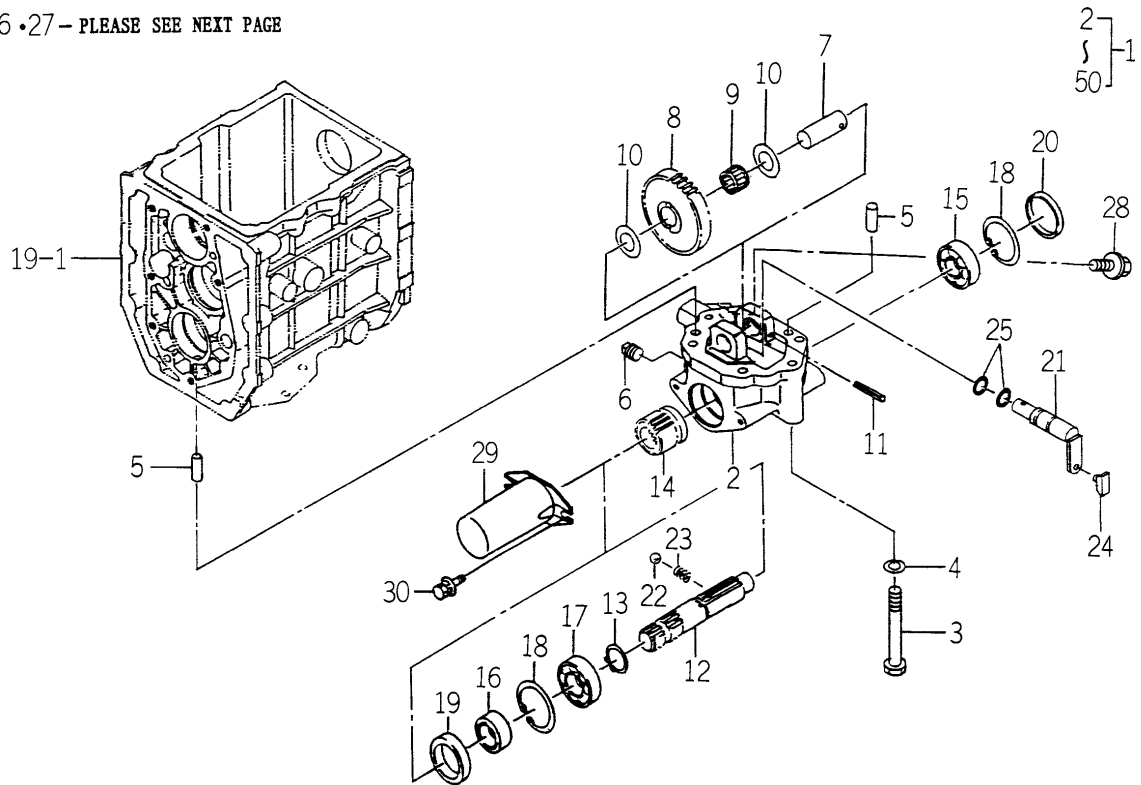
FIG.138 MID PTO SET (2)(1/2) (EXCEPT M TYPE-OPTION)
