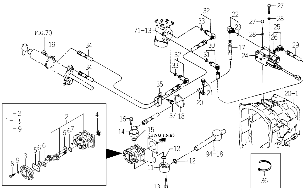
FIG. 75 PIPING SYSTEM (H TYPE-TM3200H-No.1308-/TM3240H-No.933-)
