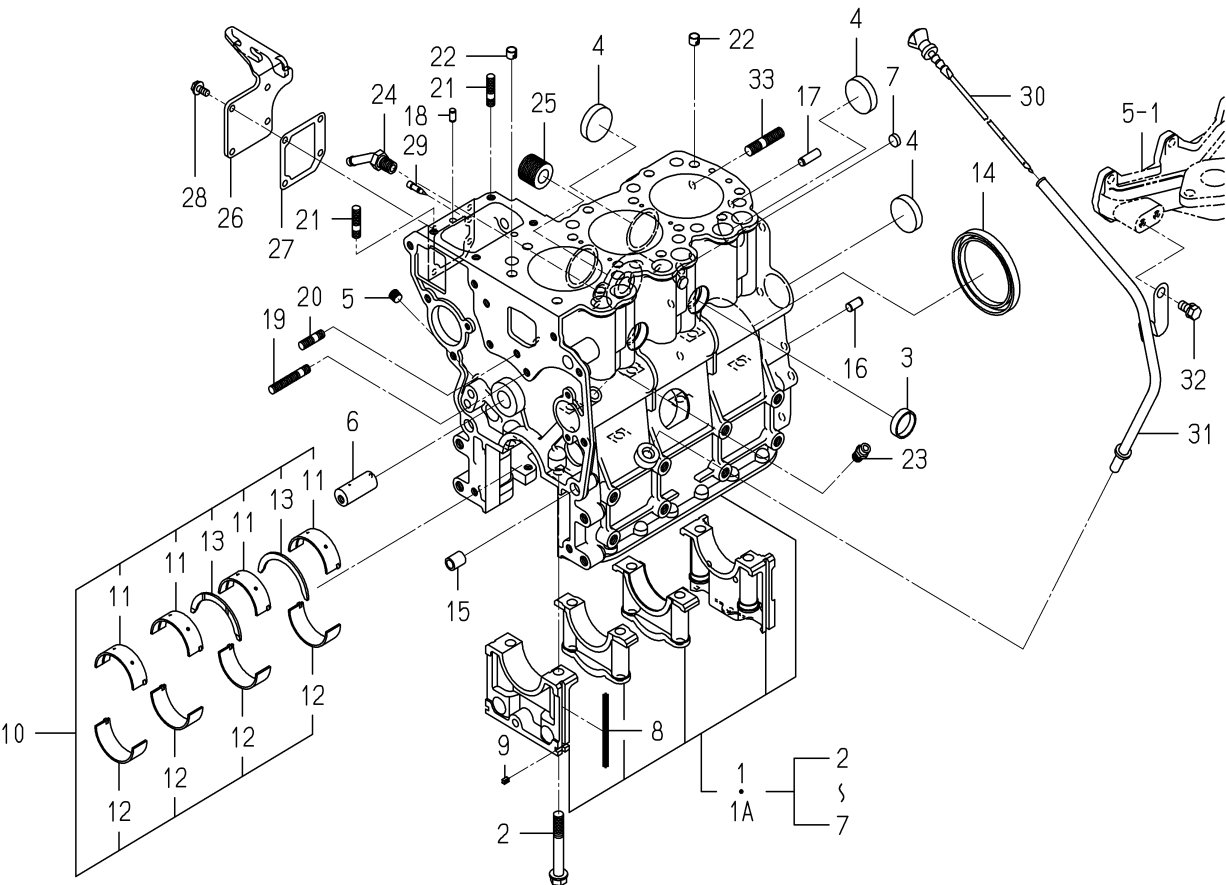
FIG. 6 CYLINDER BLOCK
