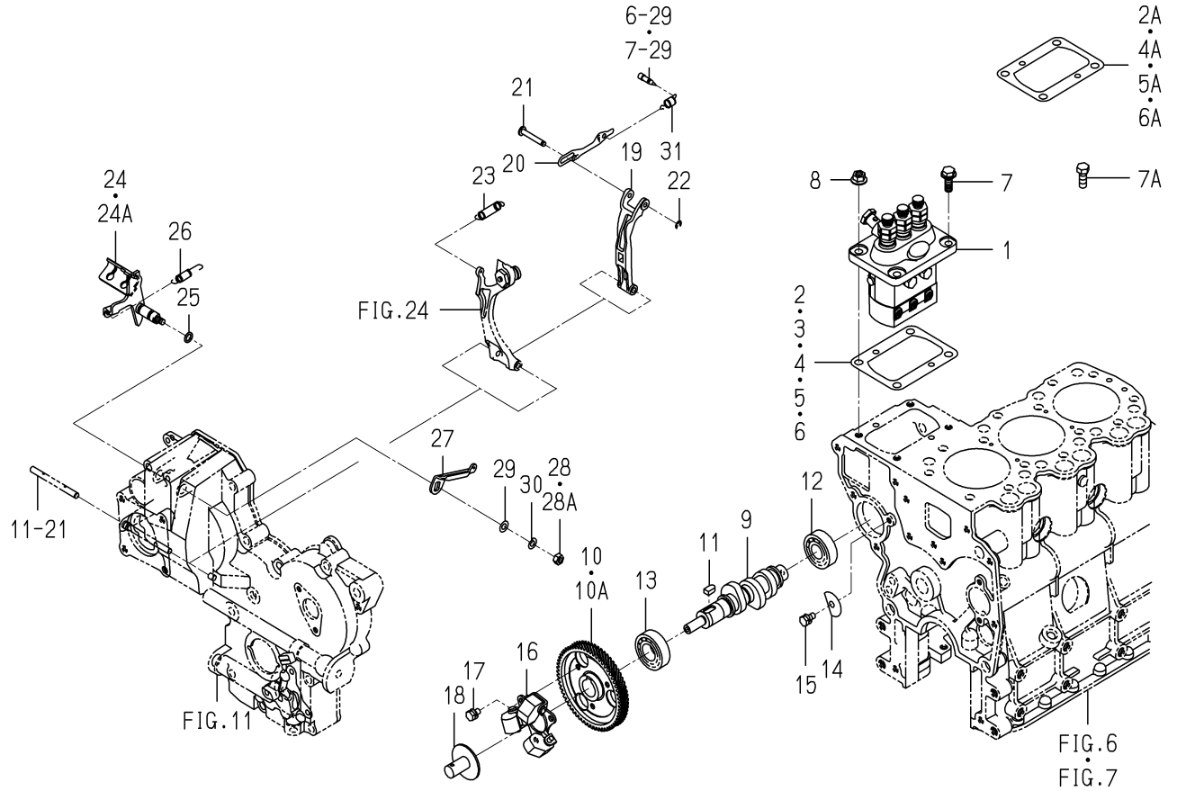
FIG. 22 INJECTION PUMP
