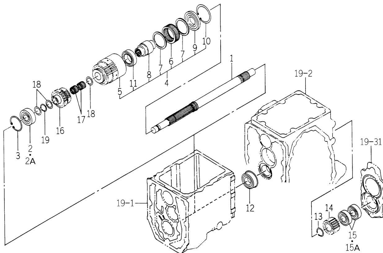
FIG. 37 GEAR (PTO) SYSTEM (TM3240-EXCEPT H TYPE)
