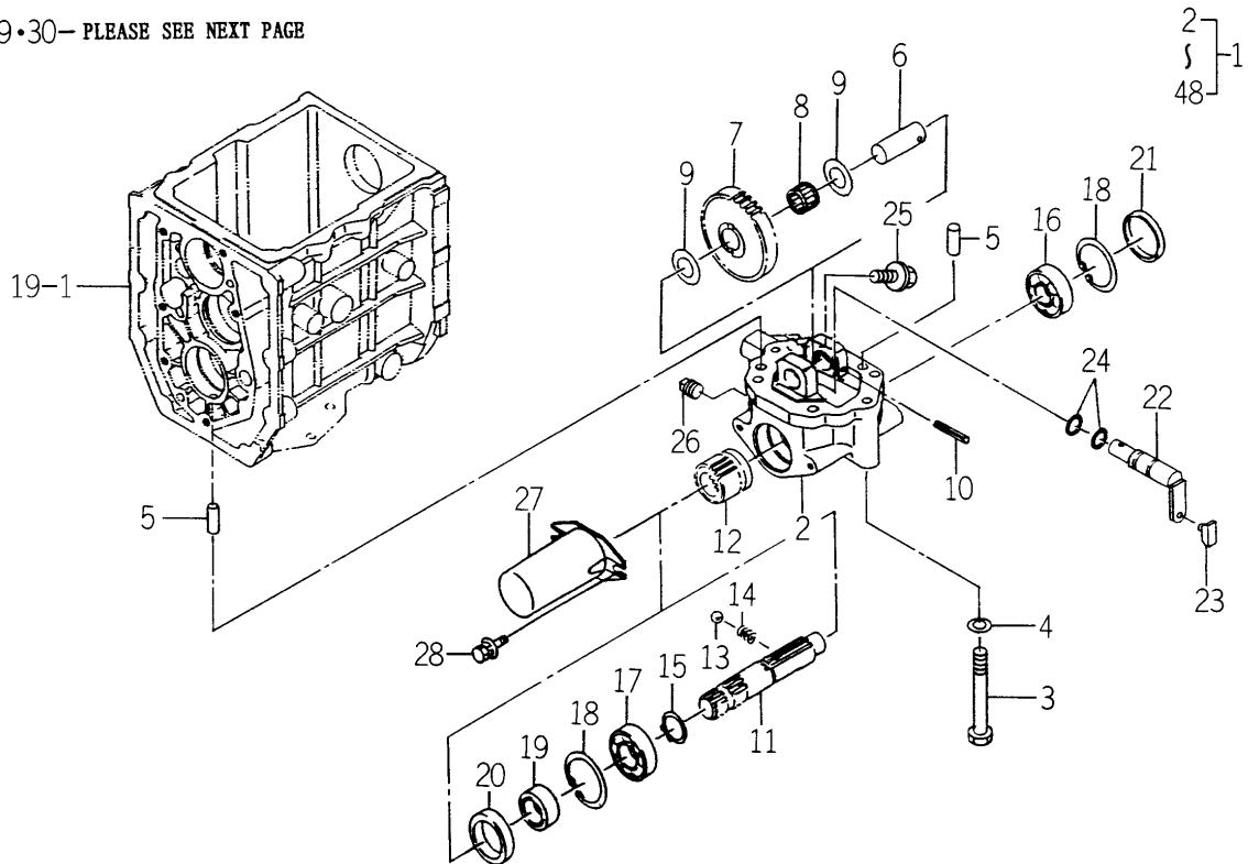
FIG.137 MID PTO SET (1)(1/2) (EXCEPT M TYPE-OPTION)
