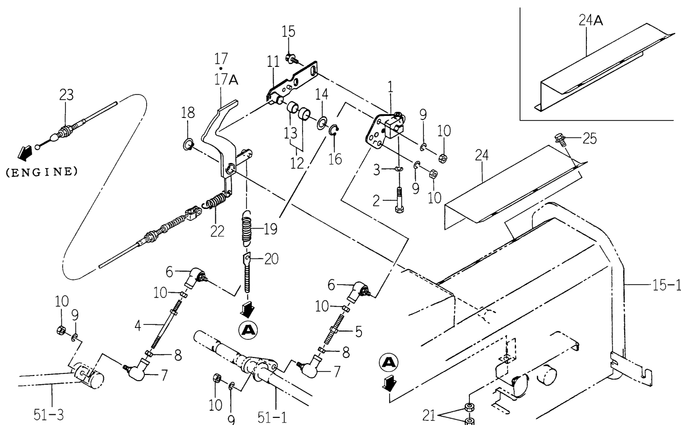
FIG. 50 LINK (HST) SYSTEM (H TYPE)
