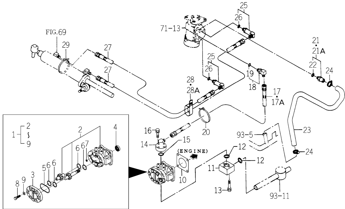
FIG. 72 PIPING SYSTEM (EXCEPT H TYPE-TM3200-No.1-1307/ TM3240-No.1-932)
