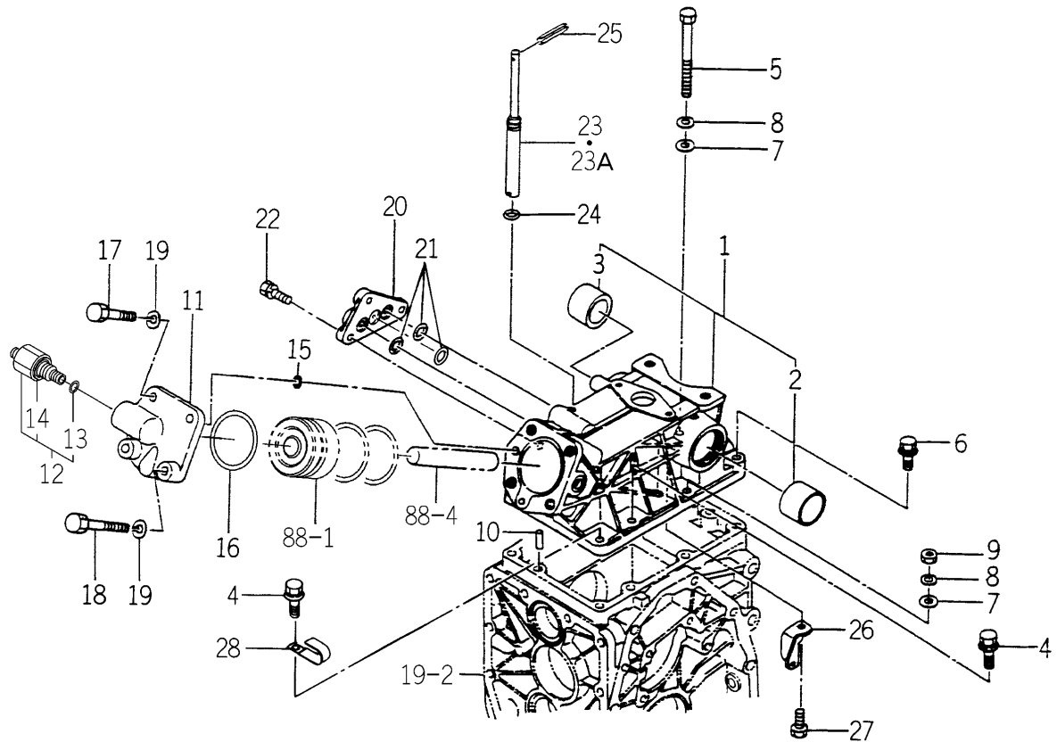
FIG. 86 CYLINDER CASE SYSTEM
