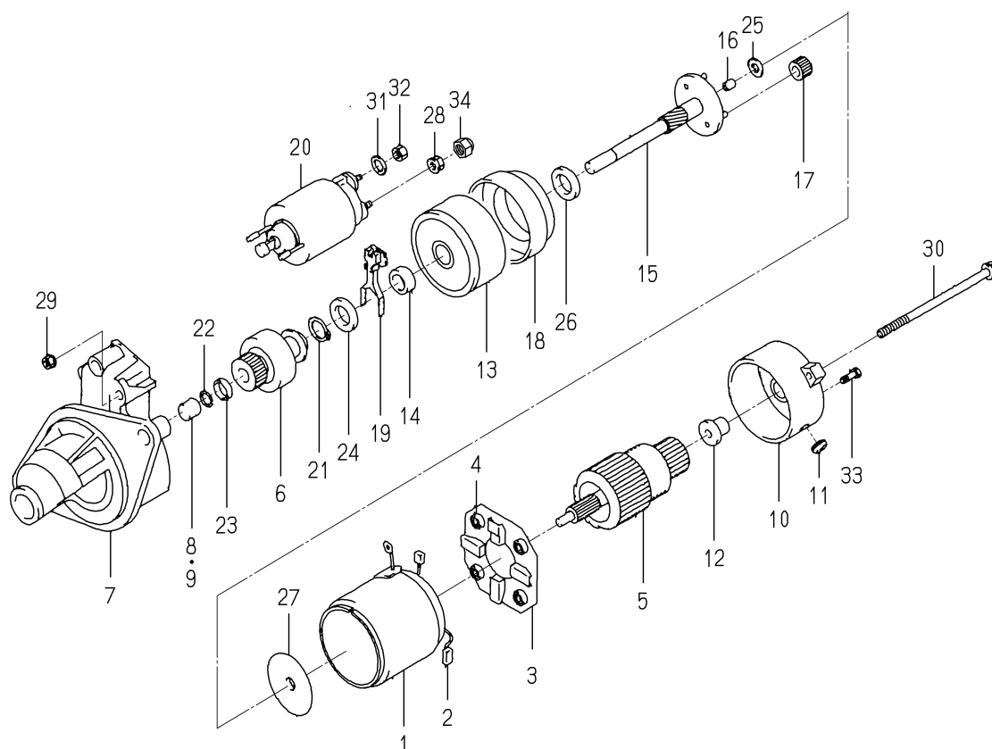
FIG. 32 COMPONENT PARTS FOR 6281-100-014-00 ON Fig.25
