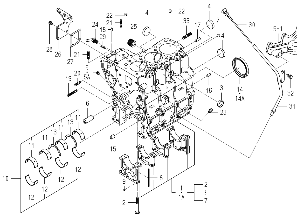
FIG. 7 CYLINDER BLOCK
