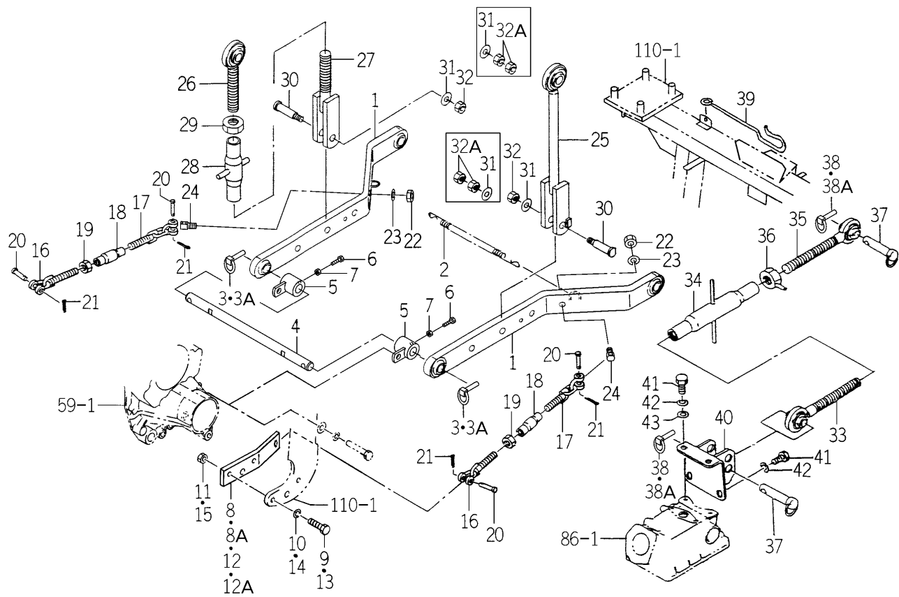
FIG. 95 LINK (3P) SYSTEM
