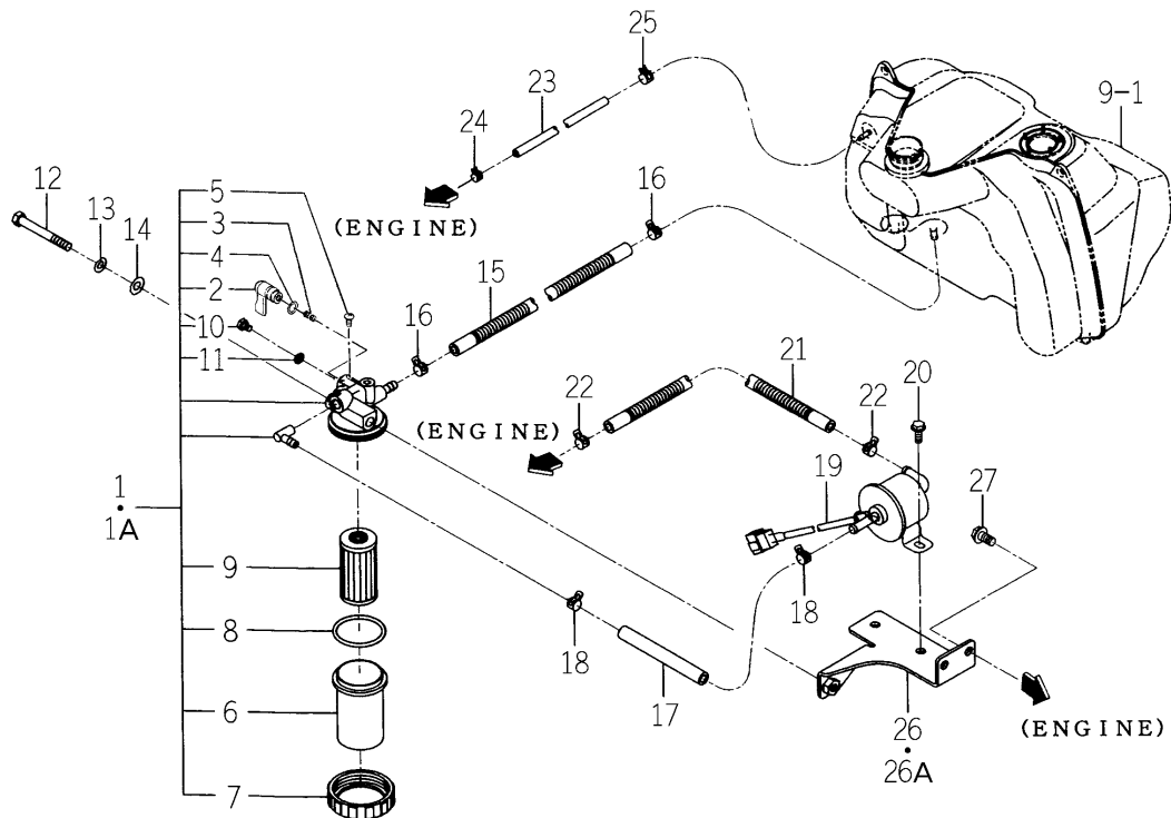
FIG. 8 FILTER SYSTEM (TM3200-No.742-/TM3200H-No.742-/ TM3240-No.582-/TM3240H-No.582-)
