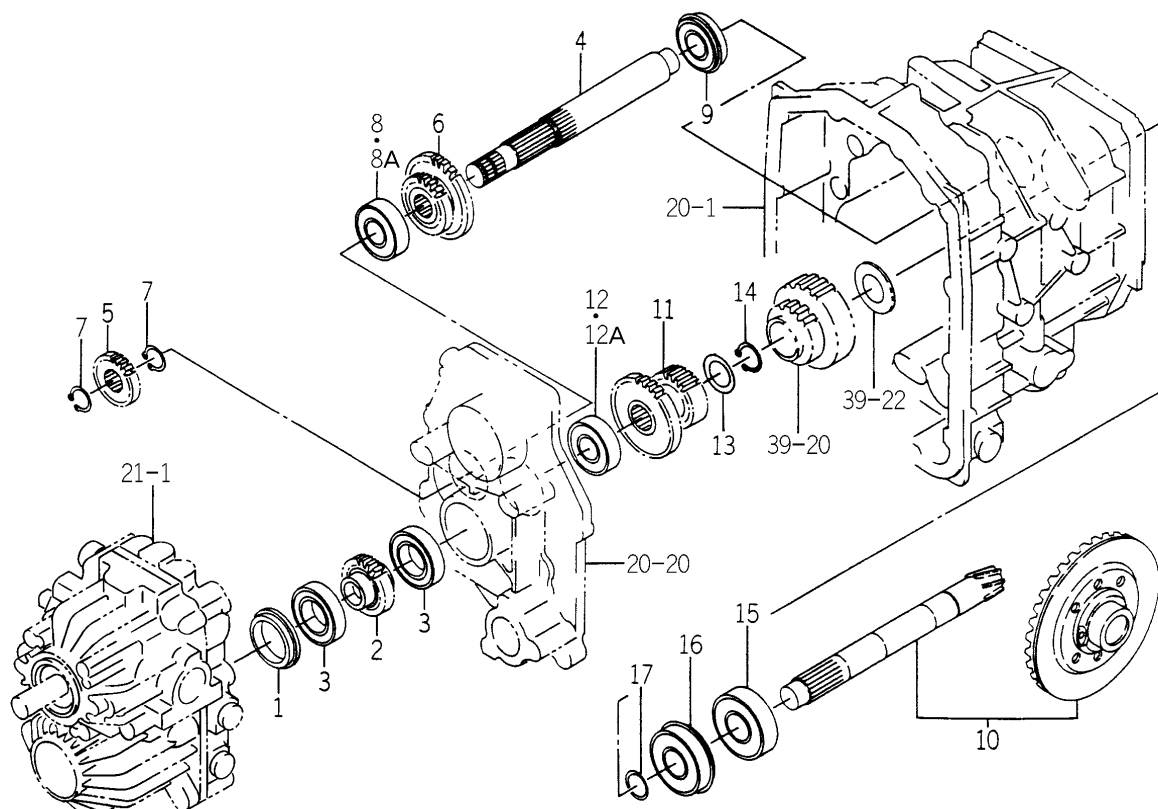
FIG. 23 GEAR (DRIVE) SYSTEM (H TYPE)
