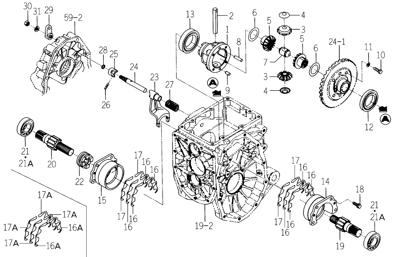
FIG. 58 DIFF CASE SYSTEM
