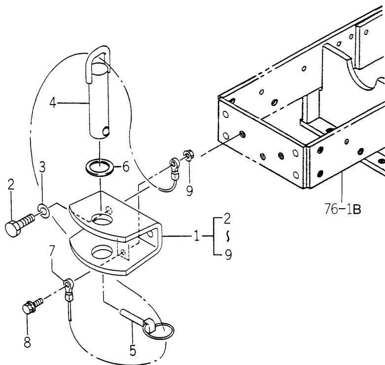
FIG.143 HITCH (FRONT) SET (M TYPE EXCEPT R-OPTION)
