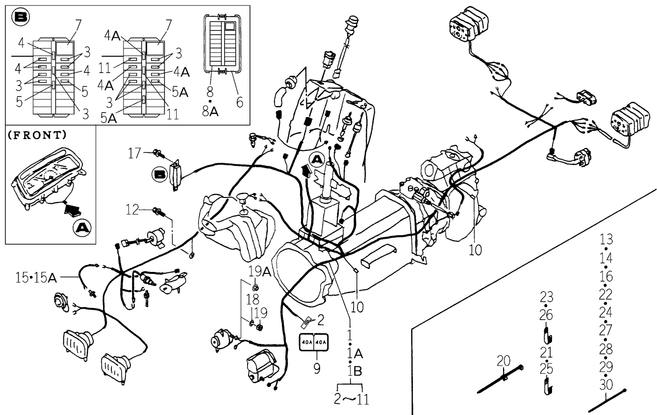
FIG.123 HARNESS SYSTEM (H TYPE)
