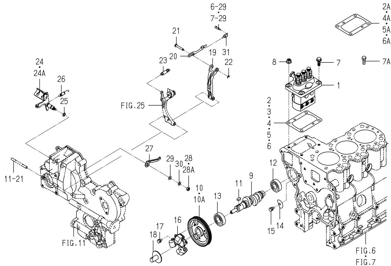
FIG. 23 INJECTION PUMP
