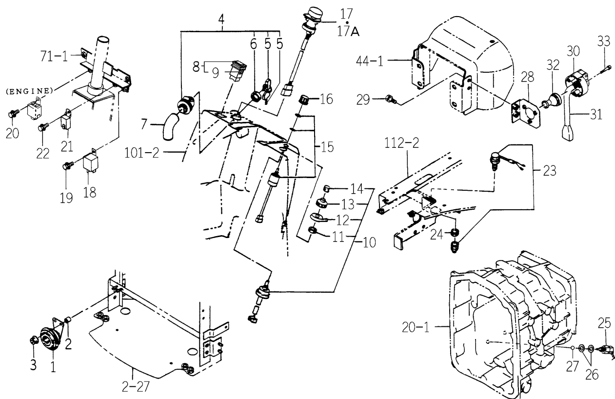
FIG.119 SWITCH SYSTEM (H TYPE-TM3200H-No.1-1307/TM3240H-No.1-932)
