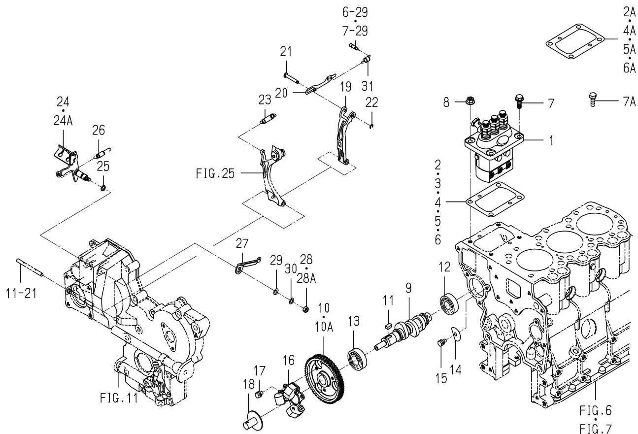
FIG. 23 INJECTION PUMP
