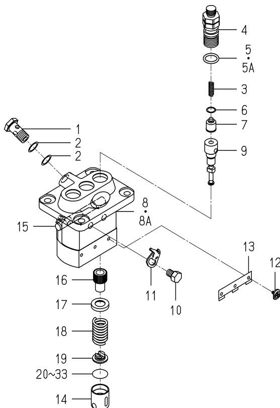
FIG. 32 COMPONENT PARTS FOR 6215-600-103-10 ON Fig.23
