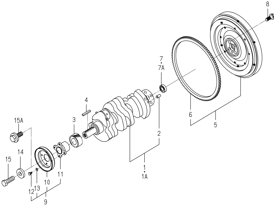
FIG. 17 CRANK SHAFT
