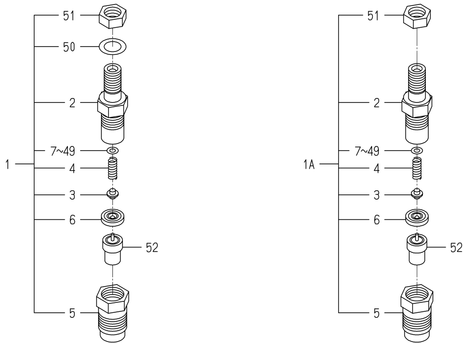
FIG. 31 COMPONENT PARTS FOR 6215-300-036-10 ON Fig.22
