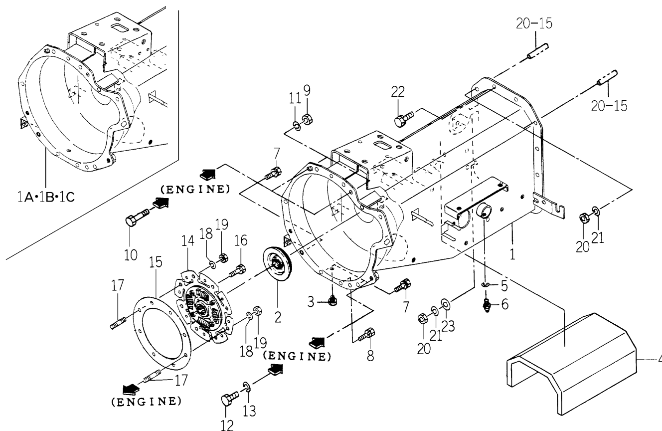
FIG. 15 CLUTCH HOUSING SYSTEM (H TYPE)
