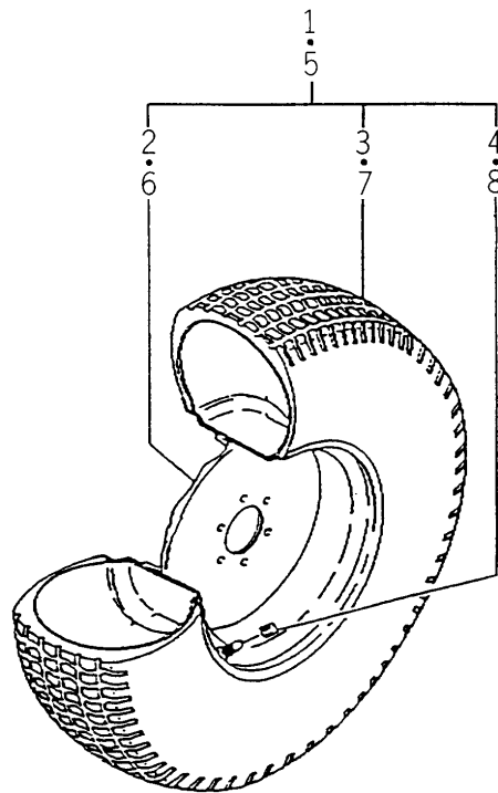
FIG.142 REAR WHEEL (TURF/PD) SYSTEM (TM3200-OPTION)
