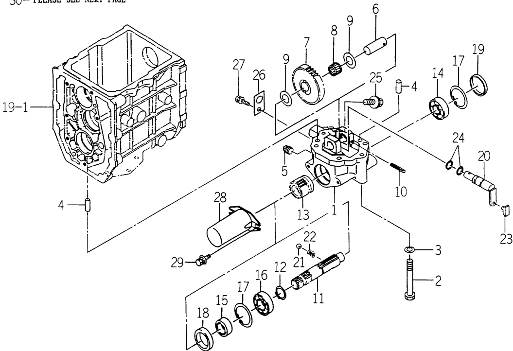
FIG. 46 MID PTO SYSTEM(1/2) (M TYPE EXCEPT H-TM3200-No.1-481/ TM3240-No.1-379)
