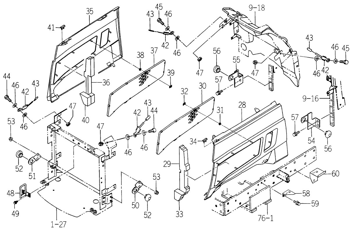
FIG. 97 HOOD SYSTEM(2/2) (TM3200-No.1-1307/TM3200H-No.1-1307/ TM3240-No.1-932/TM3240H-No.1-932)
