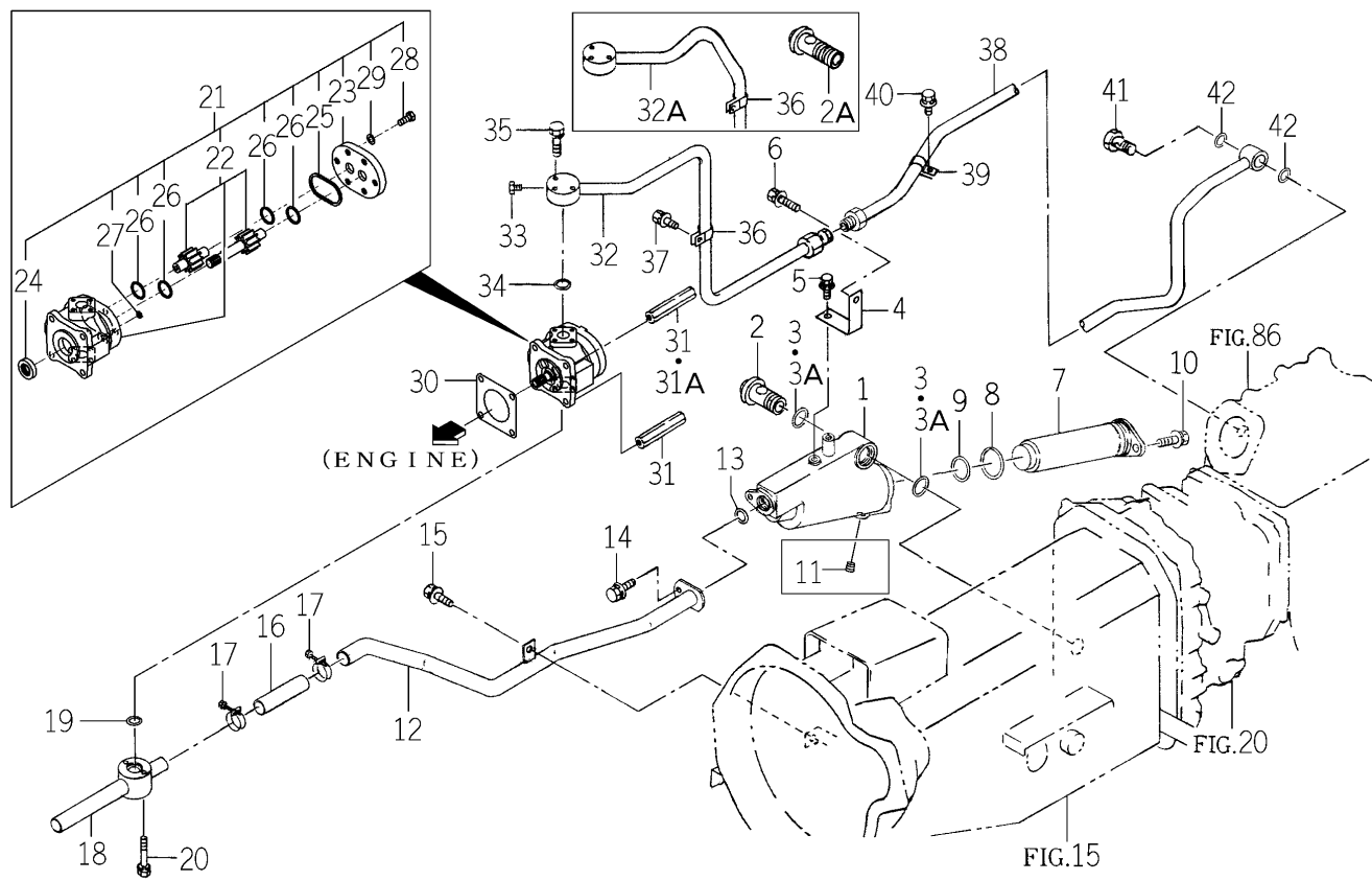
FIG. 94 PIPING SYSTEM (H TYPE)
