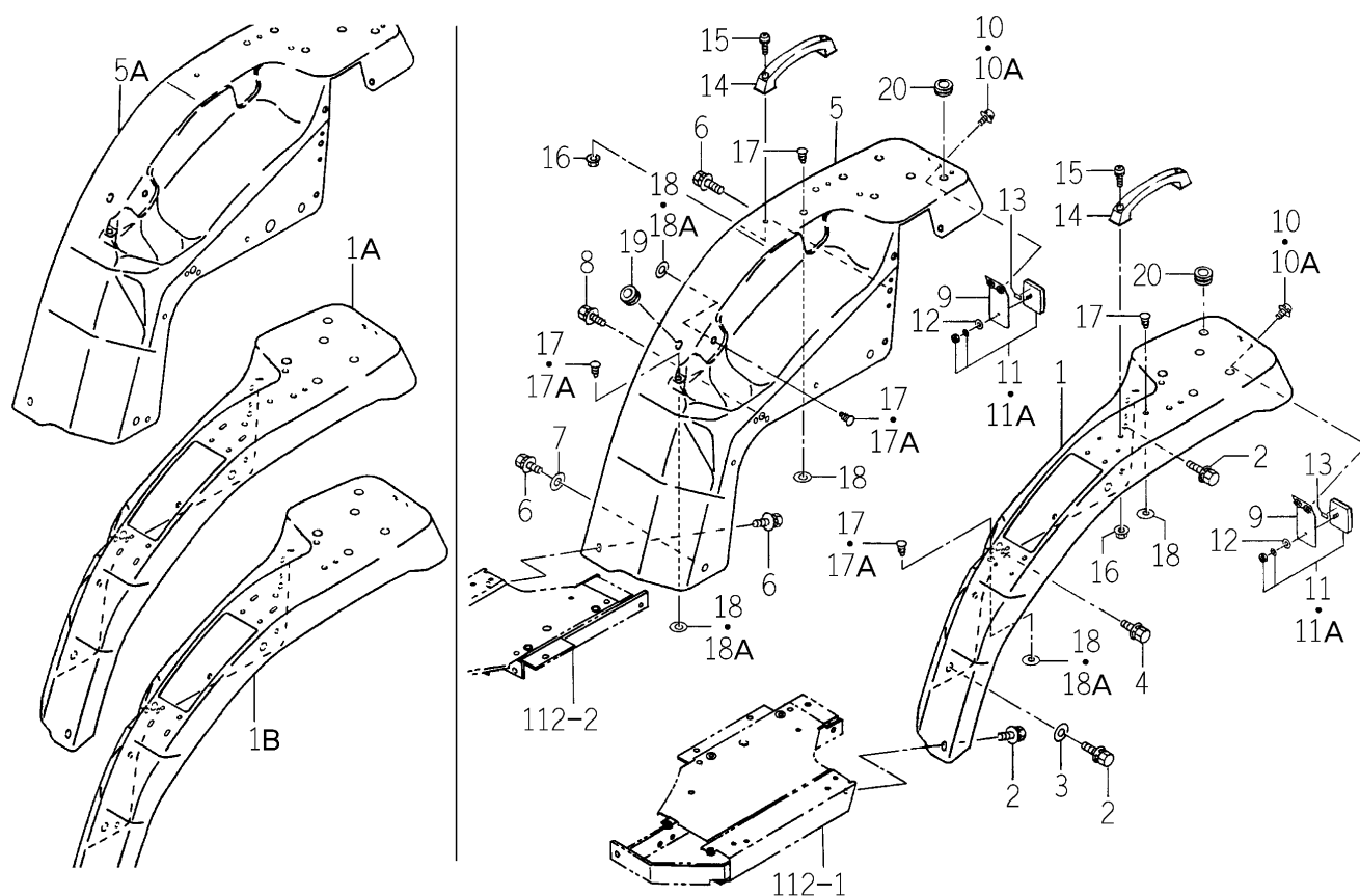
FIG.105 FENDER SYSTEM (TM3240-H TYPE)
