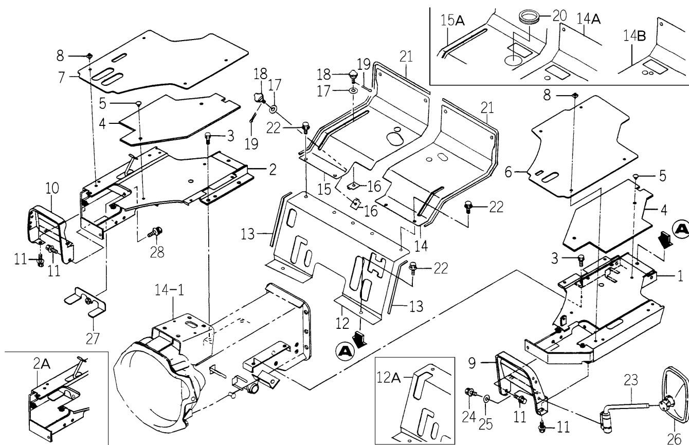
FIG.111 STEP SYSTEM (EXCEPT H TYPE)
