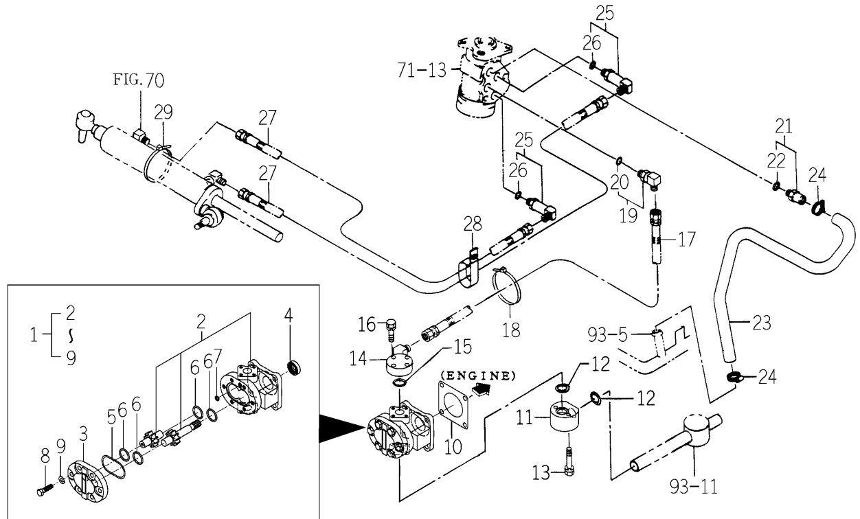
FIG. 74 PIPING SYSTEM (EXCEPT H TYPE-TM3200-No.1308-/TM3240-No.933-)
