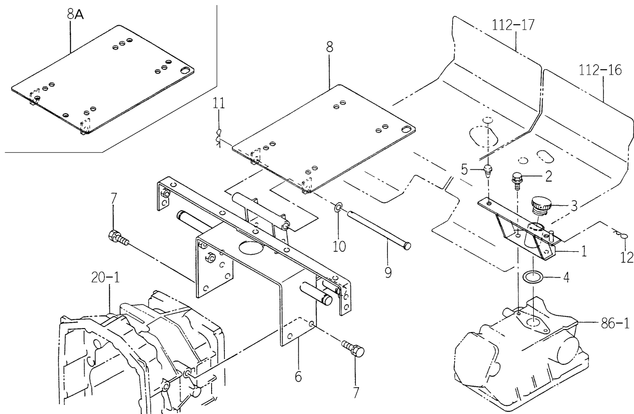
FIG.107 SEAT BASE SYSTEM
