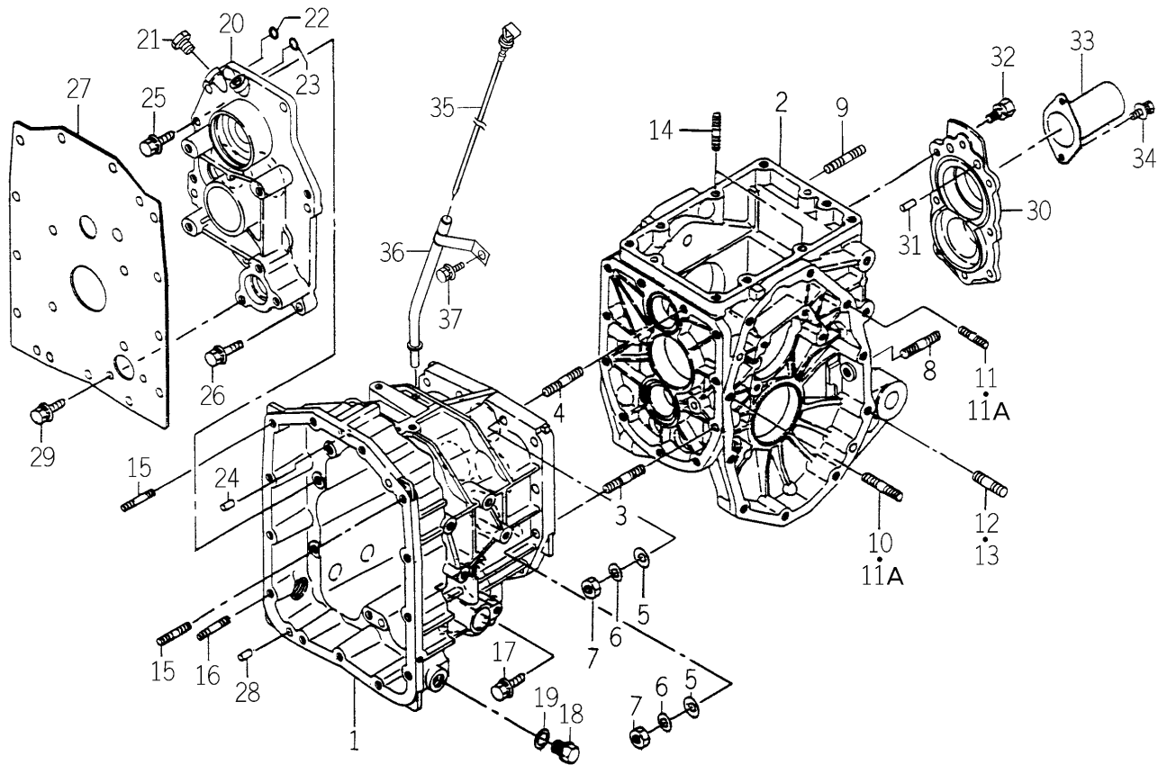
FIG. 20 CASE (TRANSMISSION) SYSTEM (H TYPE)
