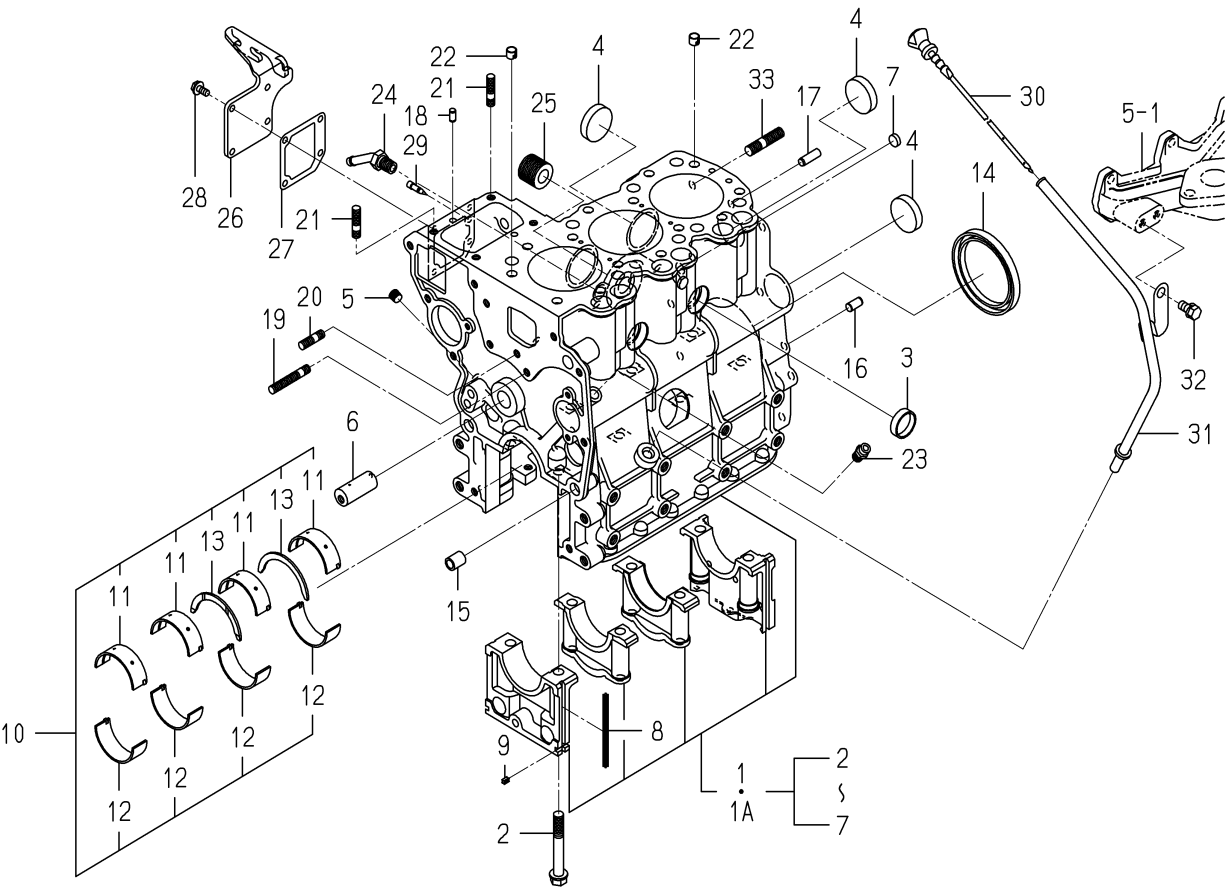
FIG. 6 CYLINDER BLOCK
