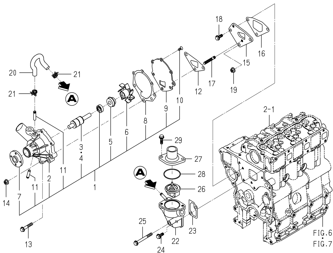
FIG. 19 WATER PUMP
