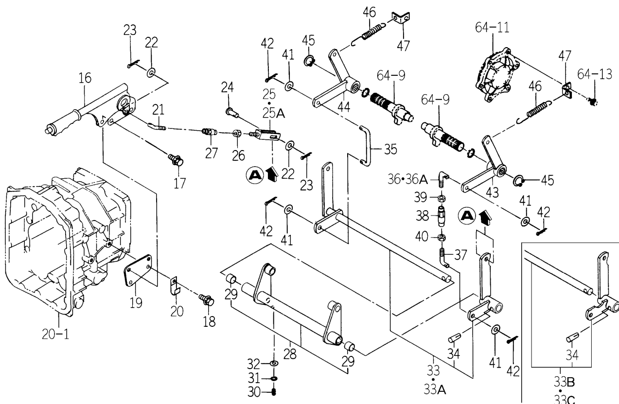
FIG. 66 PEDAL (BRAKE) SYSTEM(2/2) (TM3240-H TYPE)
