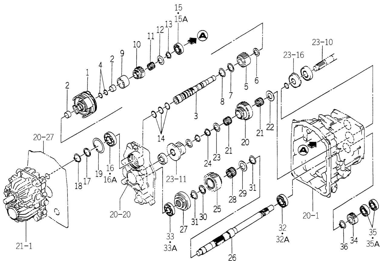
FIG. 39 GEAR (PTO) SYSTEM (H TYPE)
