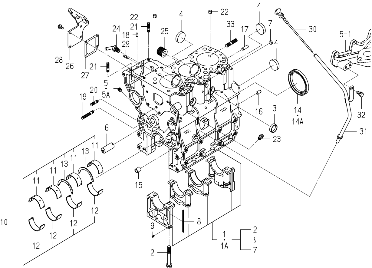
FIG. 7 CYLINDER BLOCK
