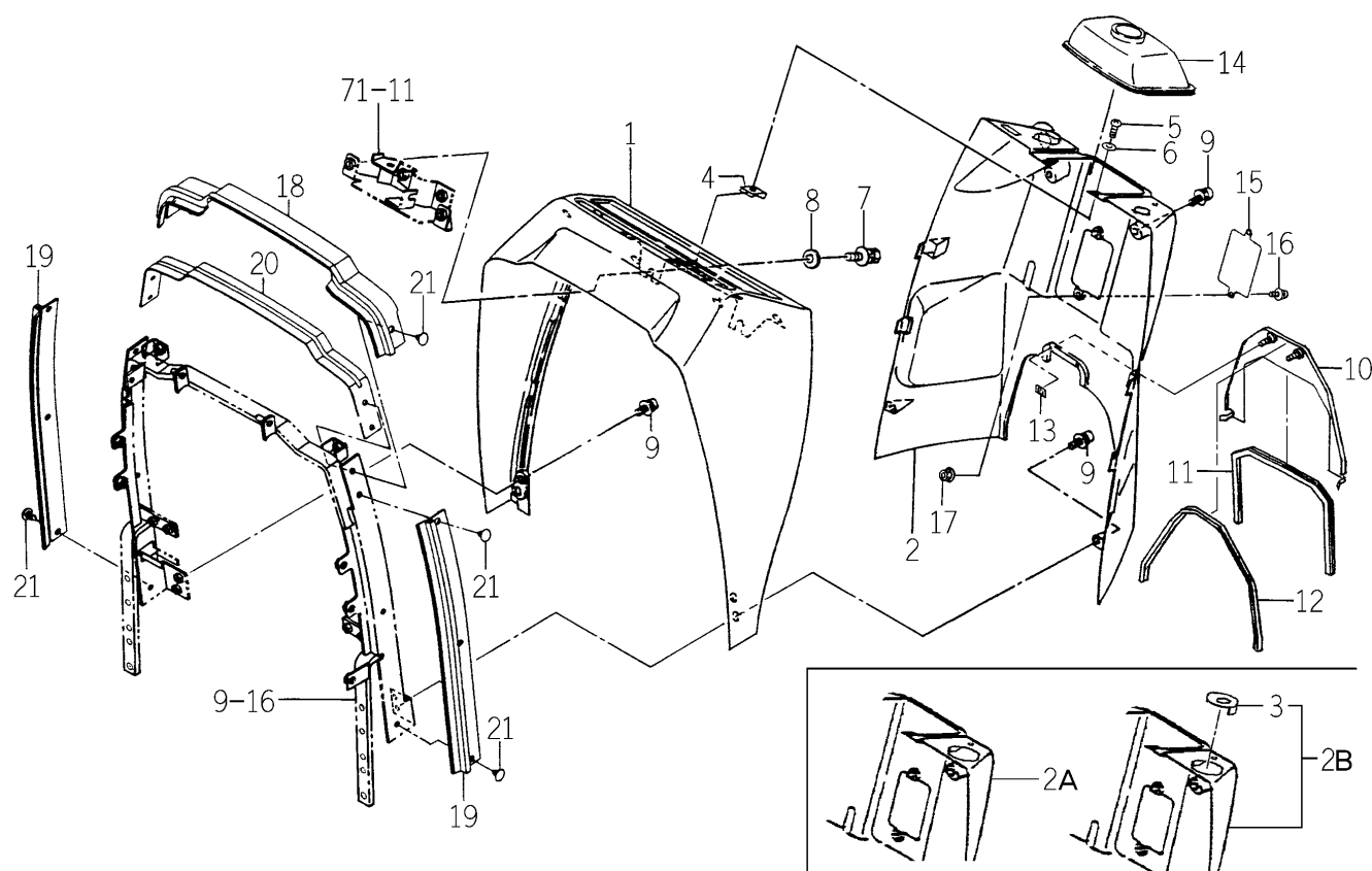
FIG.101 STEERING COVER SYSTEM (H TYPE)
