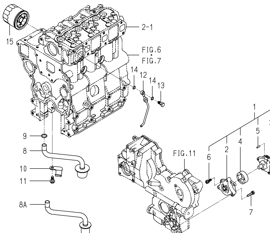
FIG. 18 OIL PUMP
