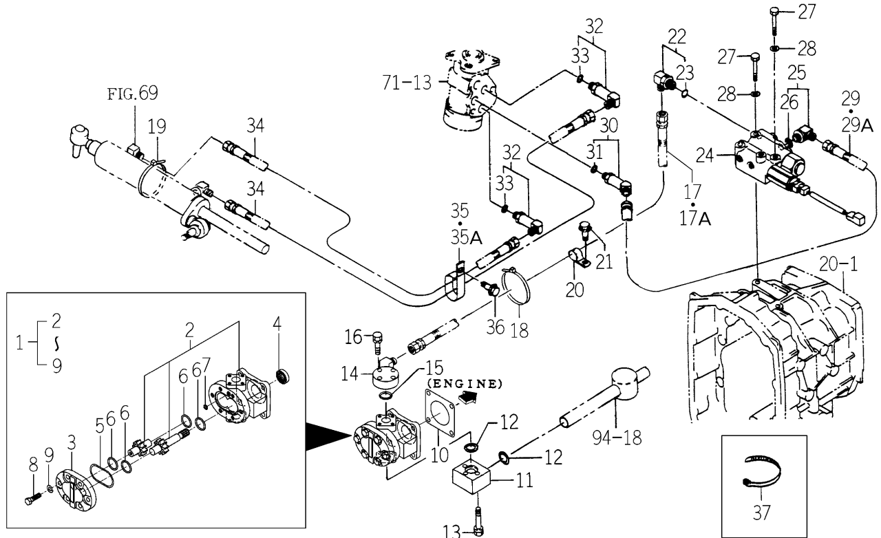
FIG. 73 PIPING SYSTEM (H TYPE-TM3200H-No.1-1307/TM3240H-No.1-932)
