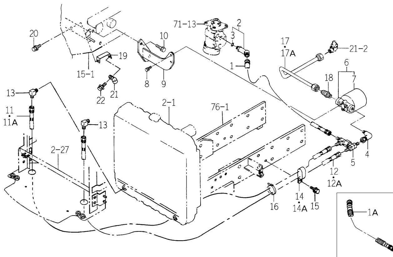
FIG. 54 PIPING SYSTEM (TM3200-H TYPE-TM3200H-No.1-1307)
