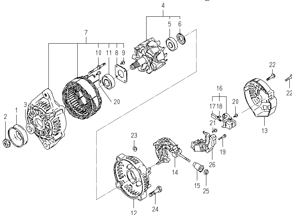
FIG. 34 COMPONENT PARTS FOR 6281-200-005-00 ON Fig.26
