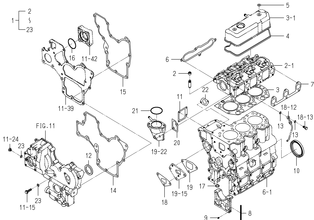
FIG. 30 REPAIR PARTS(OPTION)
