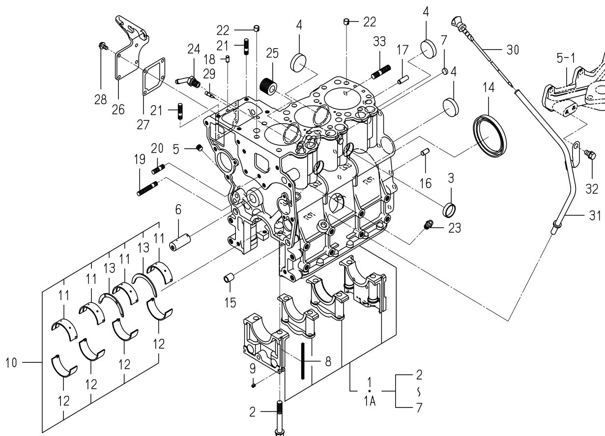
FIG. 6 CYLINDER BLOCK
