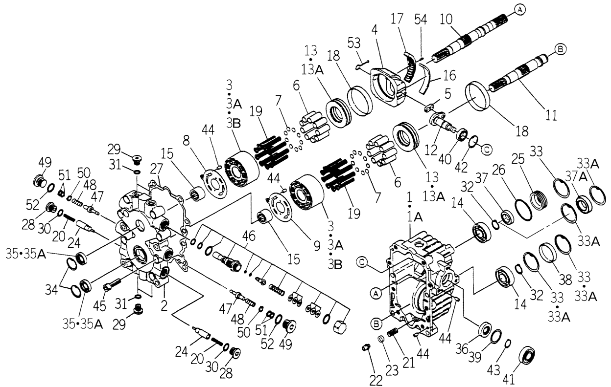
FIG.154 COMPONENT PARTS FOR K510-008-000-00,10 ON Fig.21
