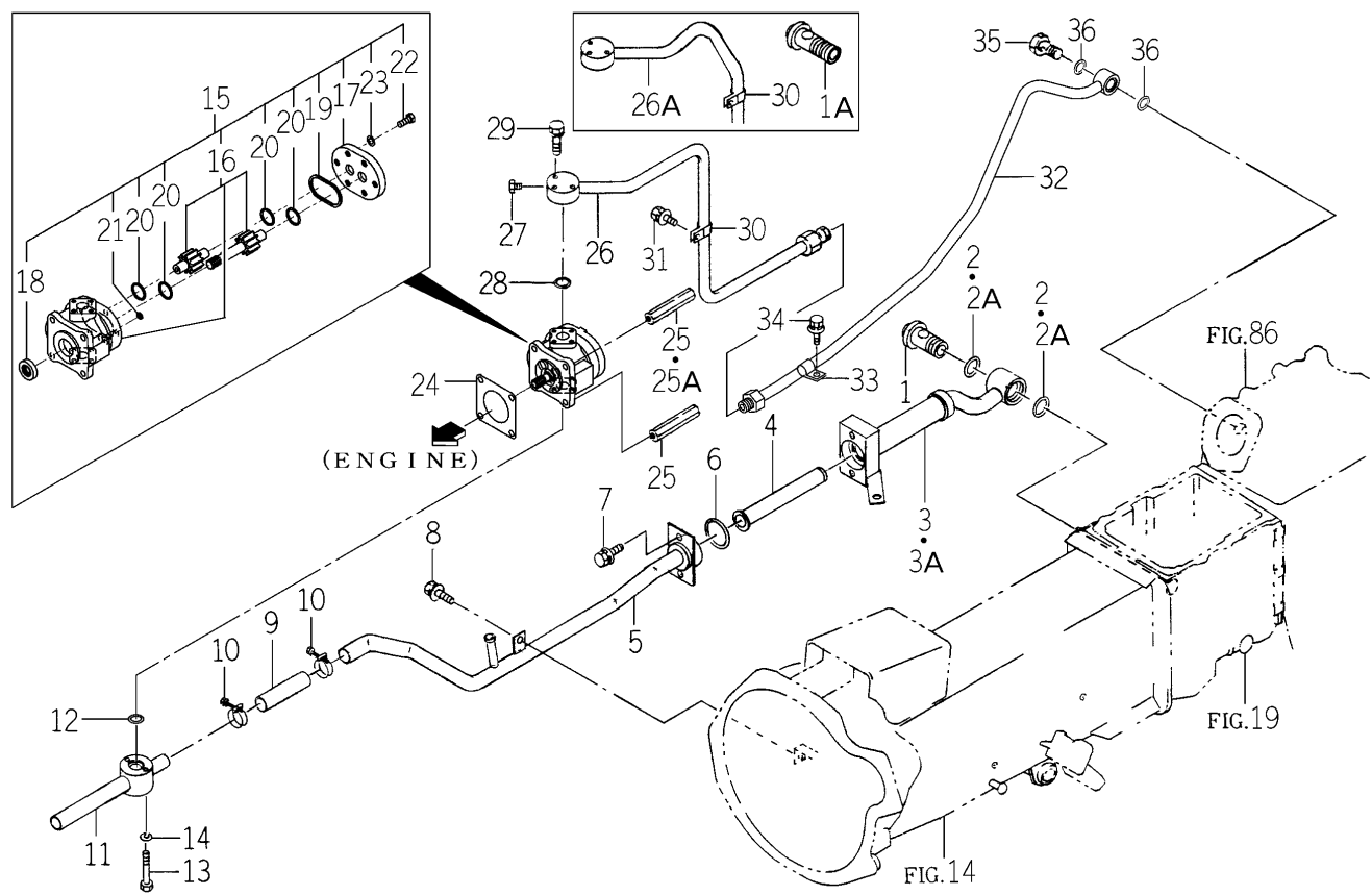
FIG. 93 PIPING (MAIN) SYSTEM (EXCEPT H TYPE)
