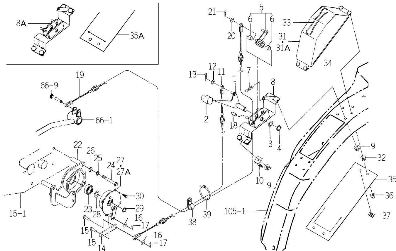
FIG. 52 CRUISE SYSTEM (TM3240-H TYPE)
