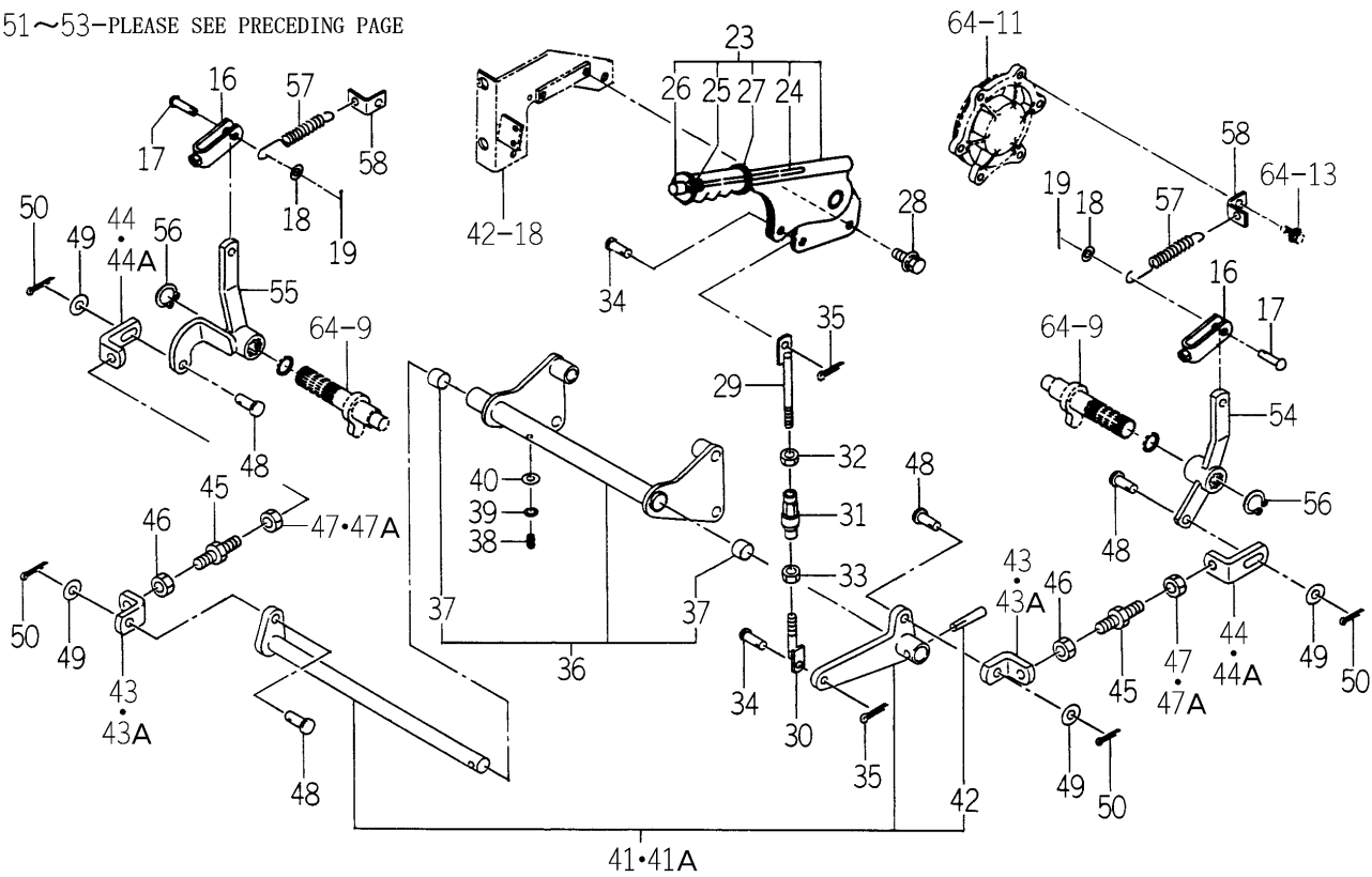
FIG. 65 PEDAL (BRAKE) SYSTEM(2/2) (EXCEPT H TYPE)
