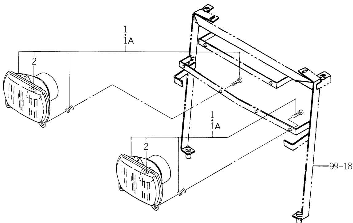
FIG.114 HEAD LAMP SYSTEM
