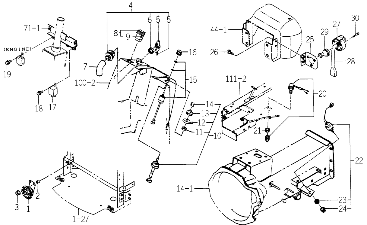
FIG.118 SWITCH SYSTEM (EXCEPT H TYPE-TM3200-No.1-1307/ TM3240-No.1-932)
