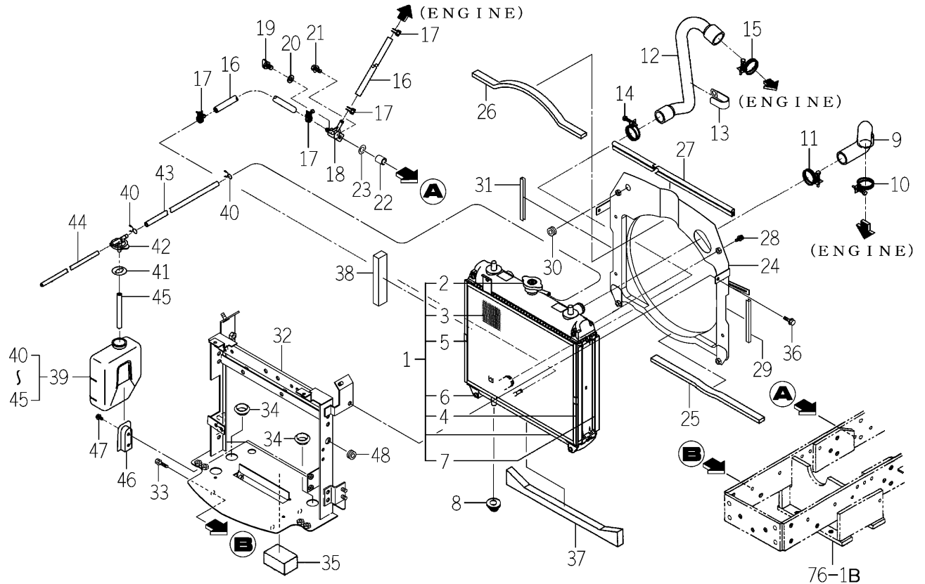
FIG. 3 RADIATOR SYSTEM (EXCEPT H TYPE-TM3200-No.1308-/TM3240-No.933-)
