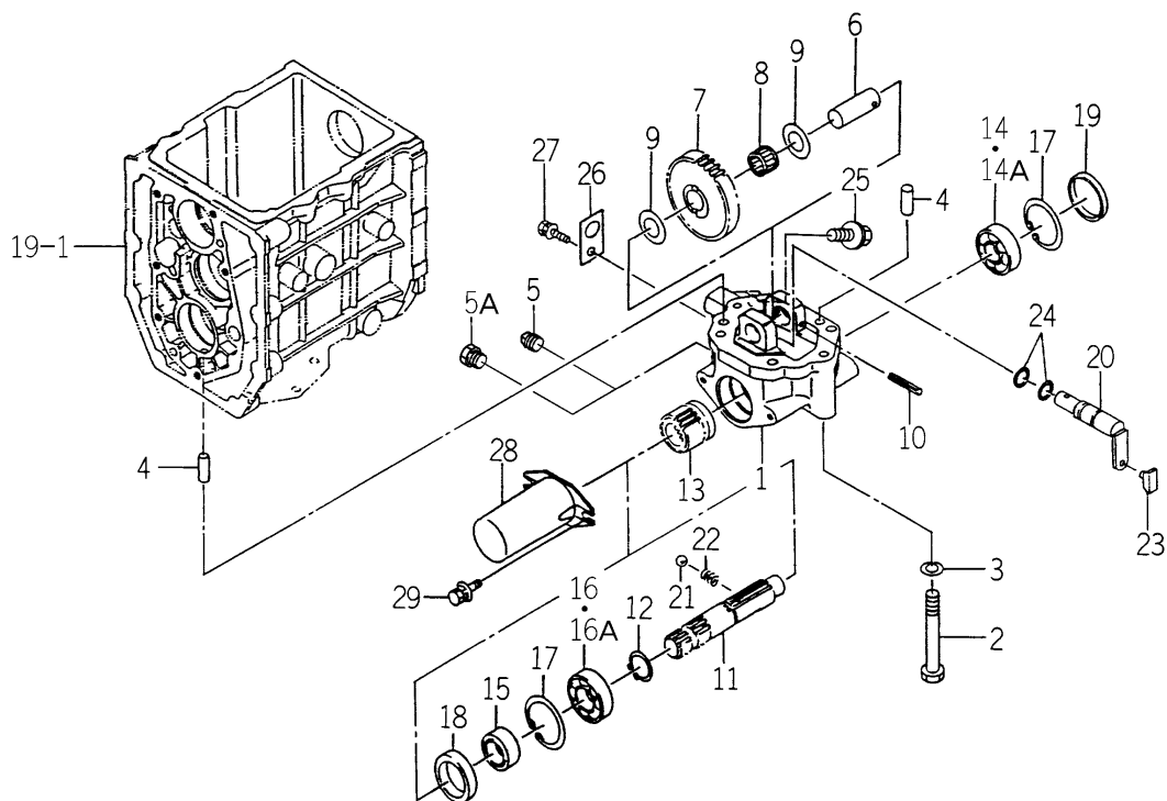
FIG. 48 MID PTO SYSTEM(1/2) (M TYPE EXCEPT H-TM3200-No.482-/ TM3240-No.380-)
