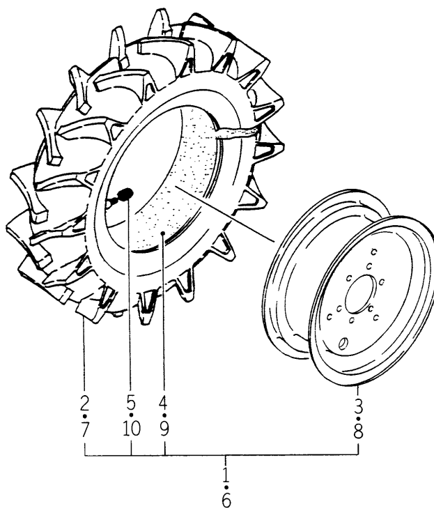
FIG.139 REAR WHEEL (FL/9.5-16) SYSTEM (TM3240-OPTION)
