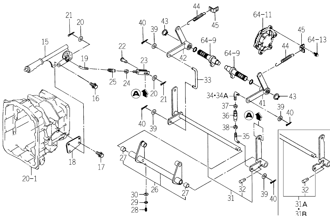
FIG. 67 PEDAL (BRAKE) SYSTEM(2/2) (TM3200-H TYPE)
