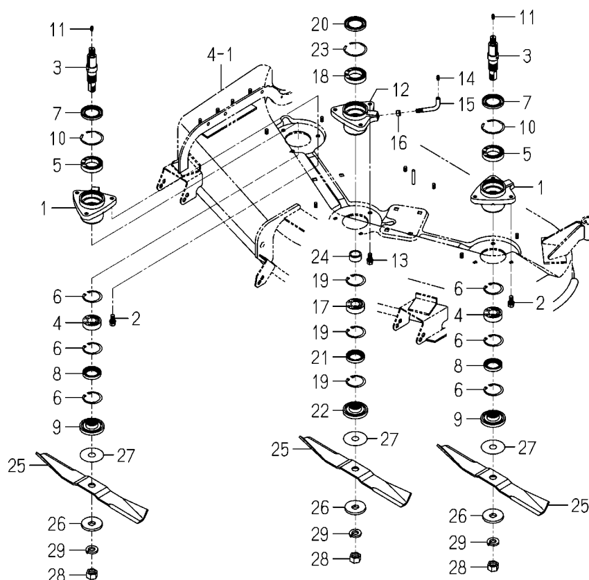
FIG. 3 METAL, BLADE SYSTEM
