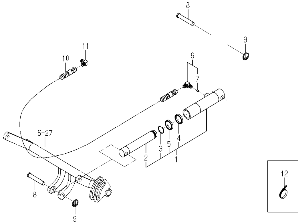
FIG. 7 CYLINDER SYSTEM
