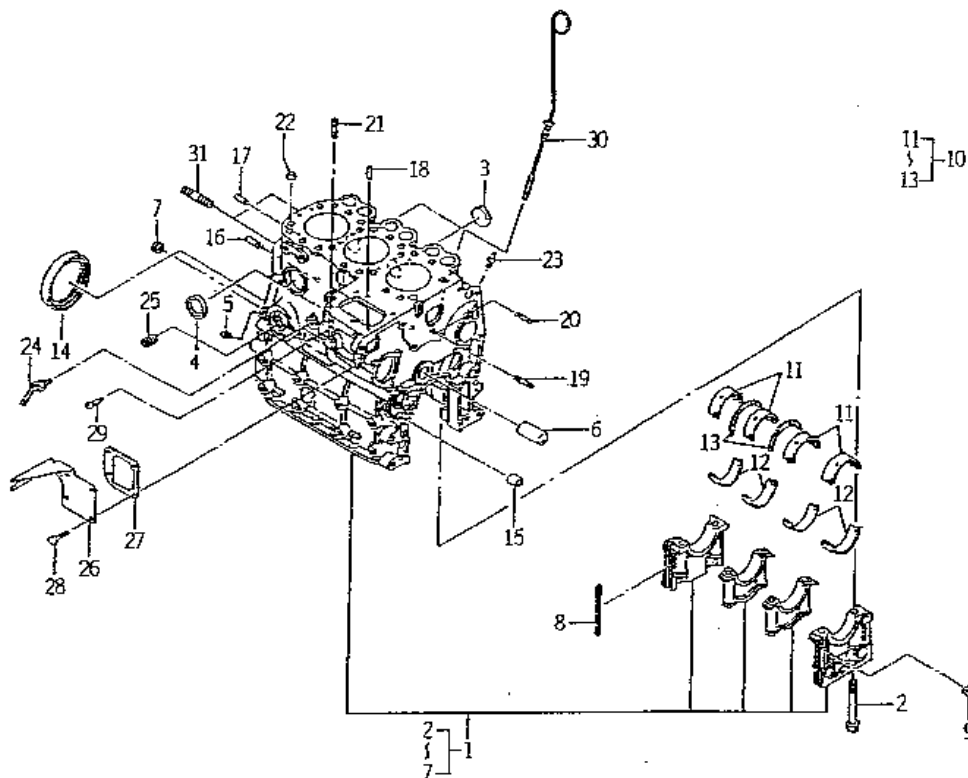
FIG. 5 CYLINDER BLOCK
