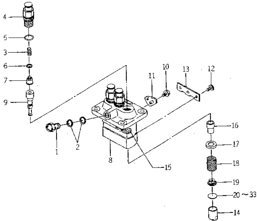
FIG. 25 COMPONENT PARTS FOR 6215 – 600 – 103 – 10 ON Fig.20
