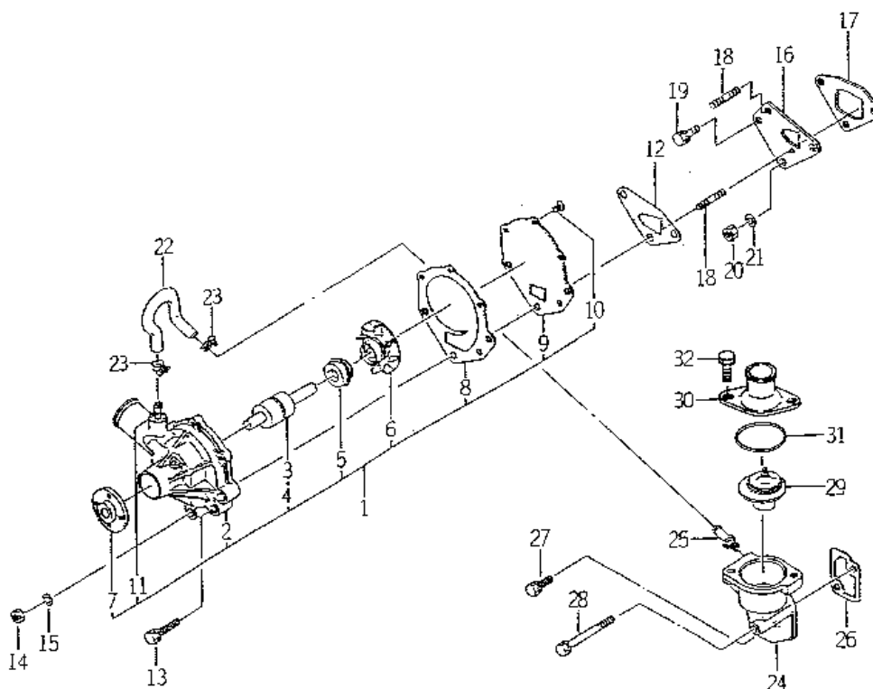
FIG. 17 WATER PUMP
