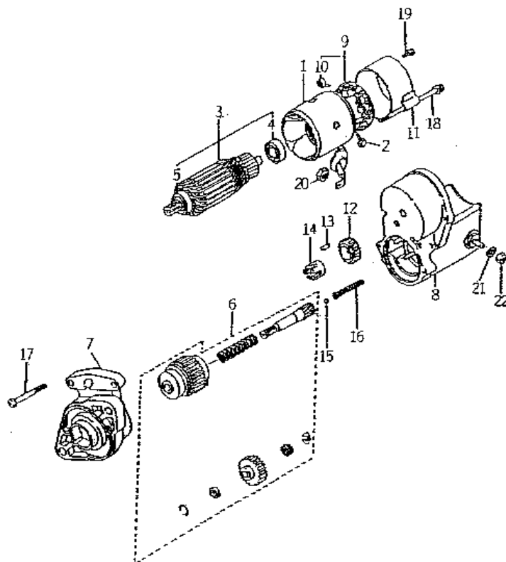
FIG. 26 COMPONENT PARTS FOR 6281 – 100 – 005 – 10 ON Fig.22
