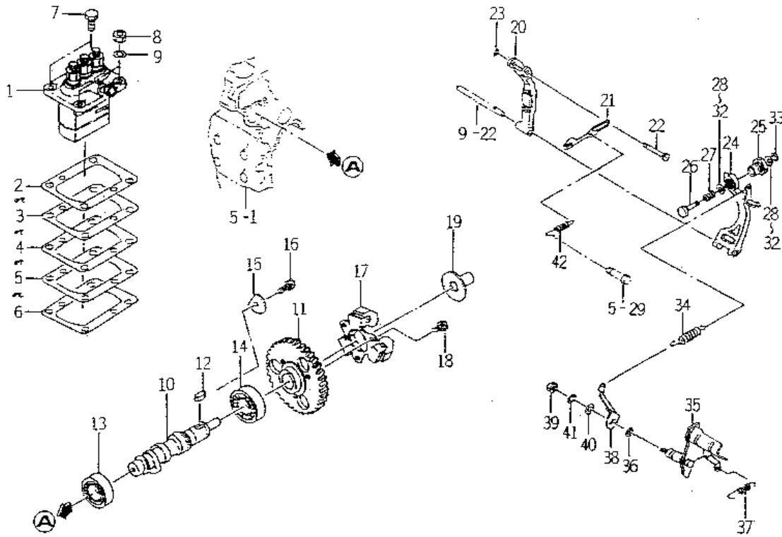
FIG. 20 INJECTION PUMP
