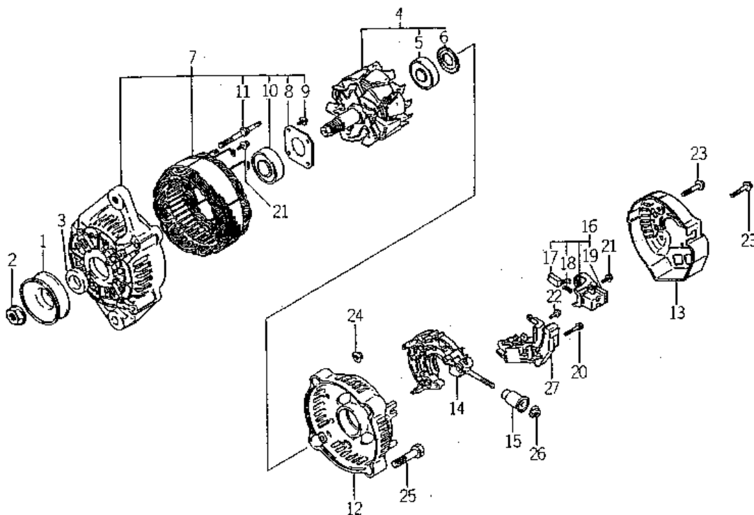
FIG. 27 COMPONENT PARTS FOR 6281 - 200 - 005 - 00 ON Fig.22
