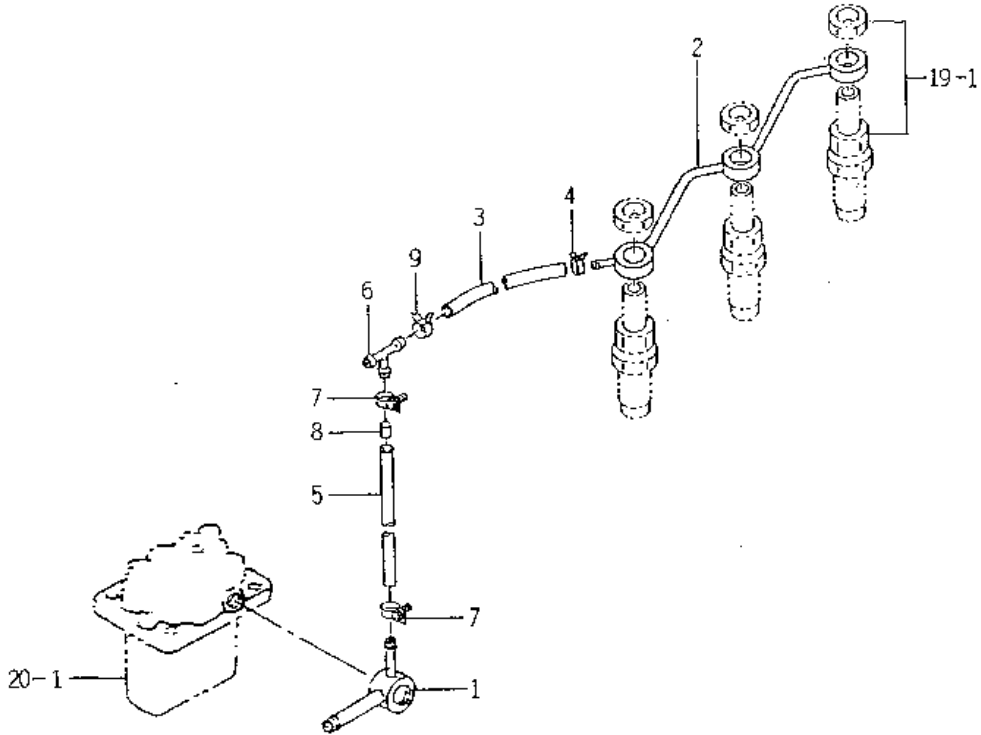
FIG. 21 FUEL PIPE
