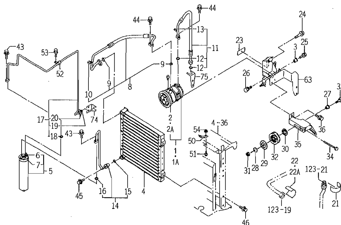
FIG.122 AIR CONDITIONER (ENGINE) SYSTEM(1/3) (CY TYPE)
