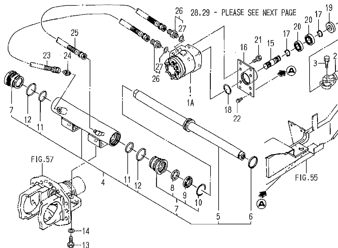
FIG. 54 STEERING (POWER) SYSTEM (P TYPE)(1/2)
