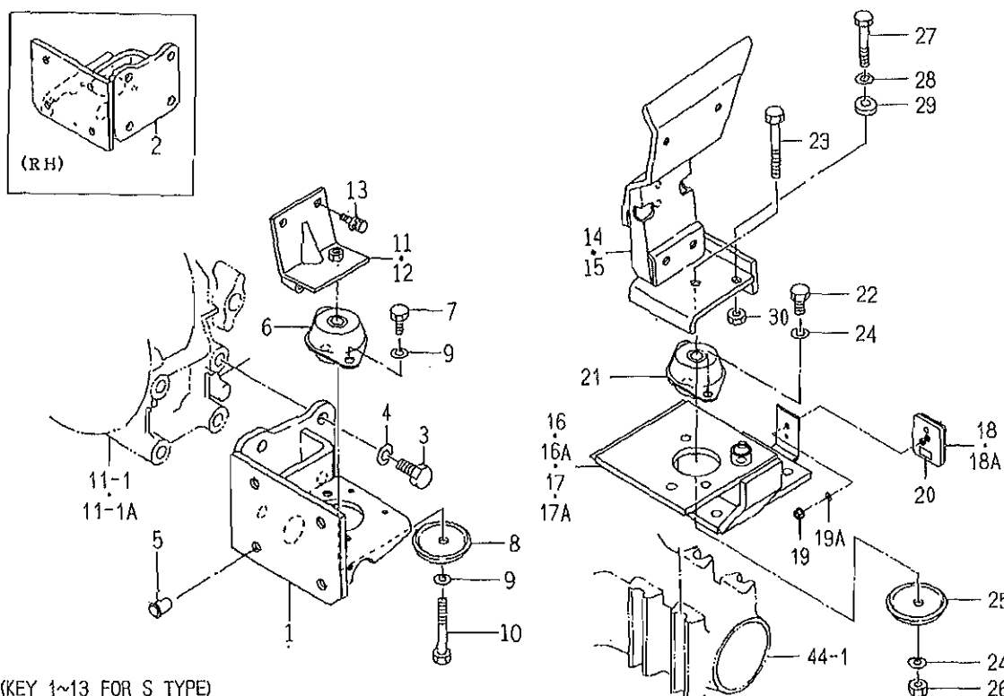
FIG. 90 FRONT MOUNT (S TYPE EXCEPT CY), REAR MOUNT (P TYPE EXCEPT CY) SYSTEM
