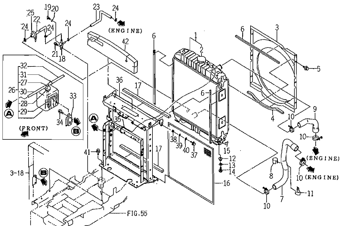
FIG. 4 RADIATOR SYSTEM
