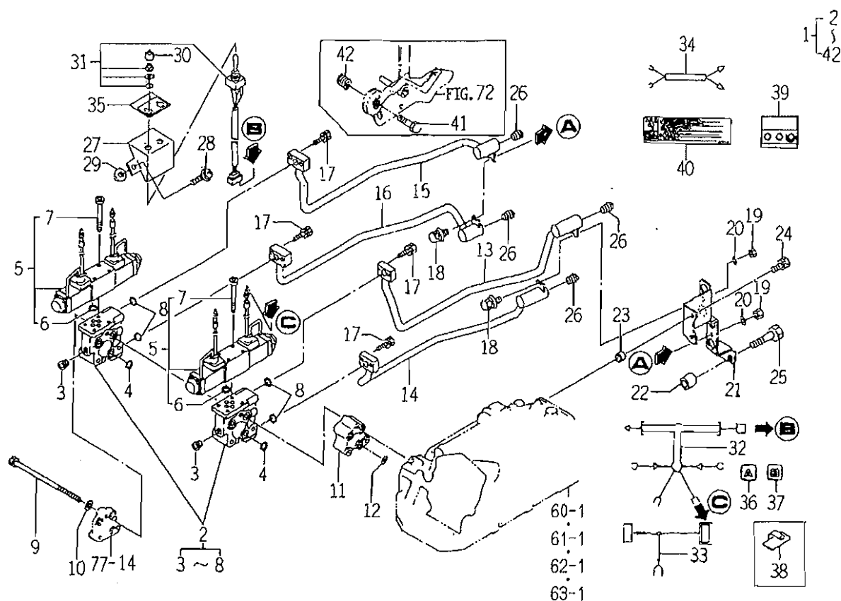
FIG.145 VALVE (REMOTE/DD) SET (OPTION)
