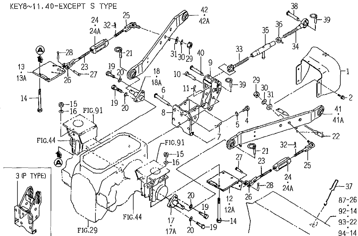
FIG. 78 COVER (SHIELD),REAR HITCH, 3P LINK,LOWER LINK SYSTEM
