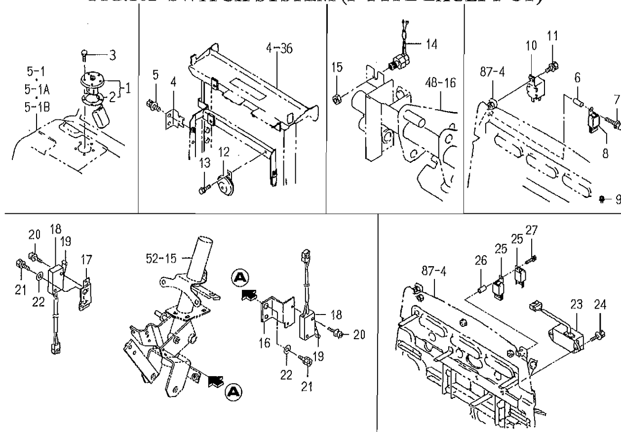
FIG.102 SWITCH SYSTEM (P TYPE EXCEPT CY)
