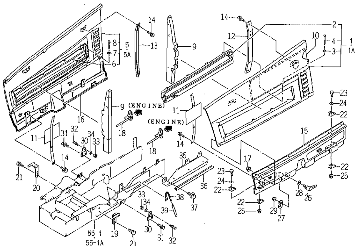
FIG. 84 FAN COVER SYSTEM
