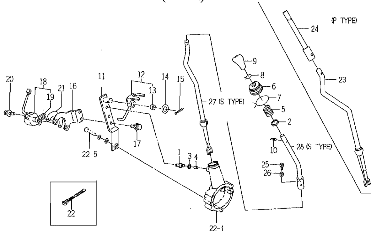
FIG. 41 MAIN CHANGE (SAFETY), LEVER (MAIN) SYSTEM
