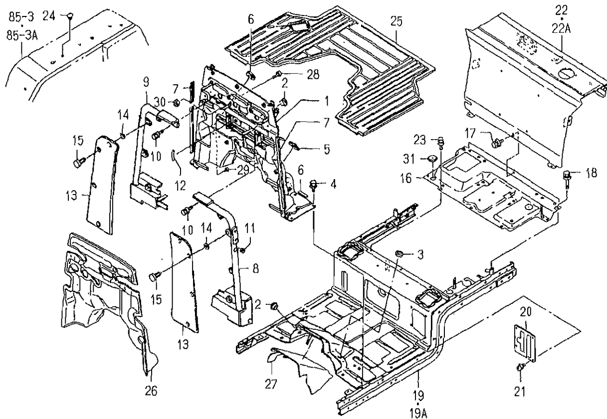
FIG. 93 FLOOR SYSTEM (P TYPE EXCEPT CY)
