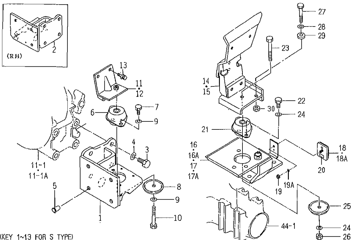
FIG. 90 FRONT MOUNT (S TYPE EXCEPT CY), REAR MOUNT (P TYPE EXCEPT CY) SYSTEM
