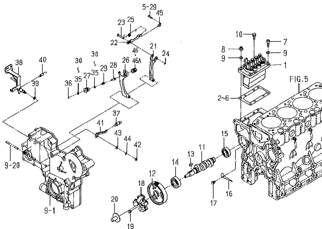
FIG. 21 INJECTION PUMP (No.1-3834)
