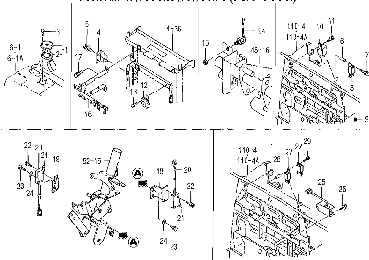
FIG.103 SWITCH SYSTEM (PCY TYPE)
