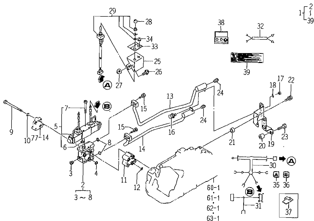
FIG.144 VALVE (REMOTE/D) SET (OPTION)
