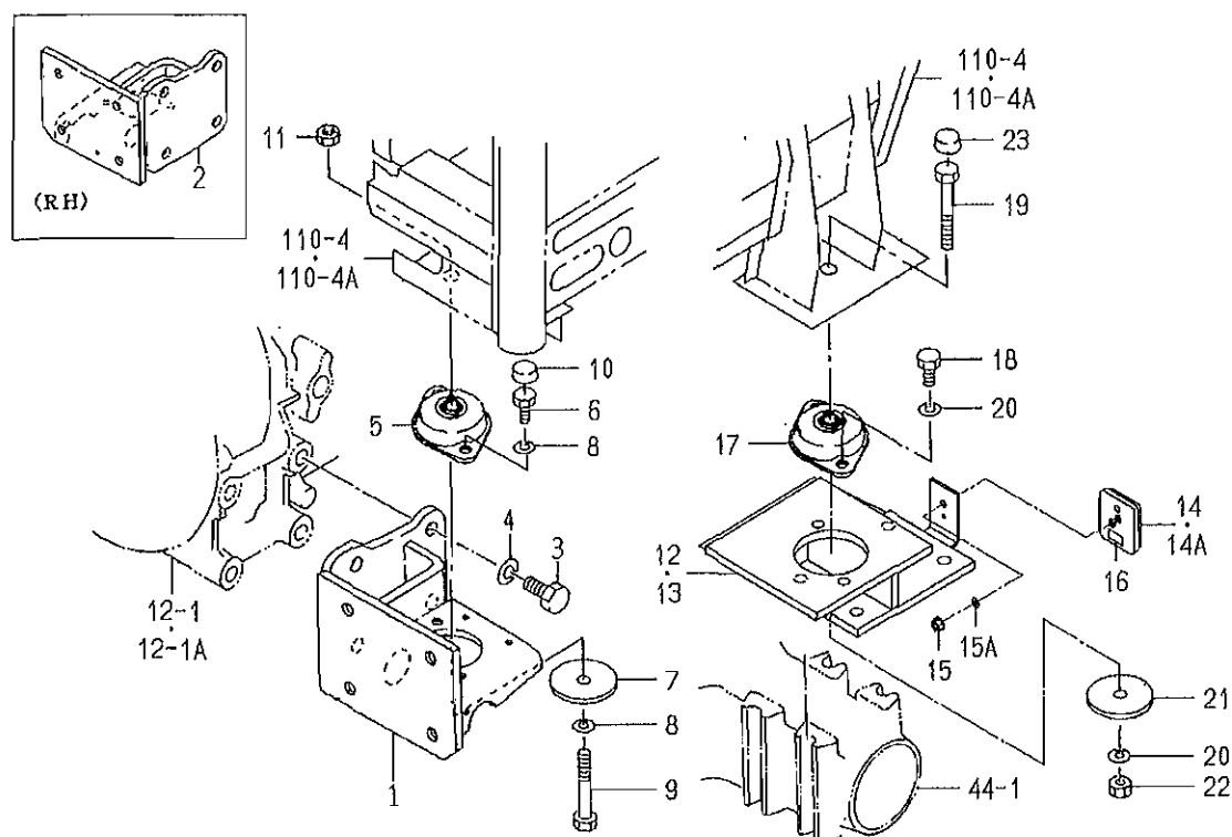
FIG. 89 FRONT MOUNT, REAR MOUNT SYSTEM (PCY TYPE)
