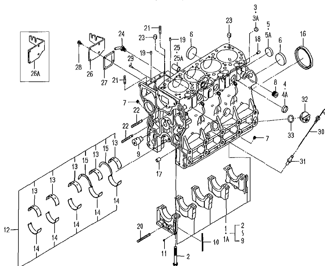
FIG. 5 CYLINDER BLOCK
