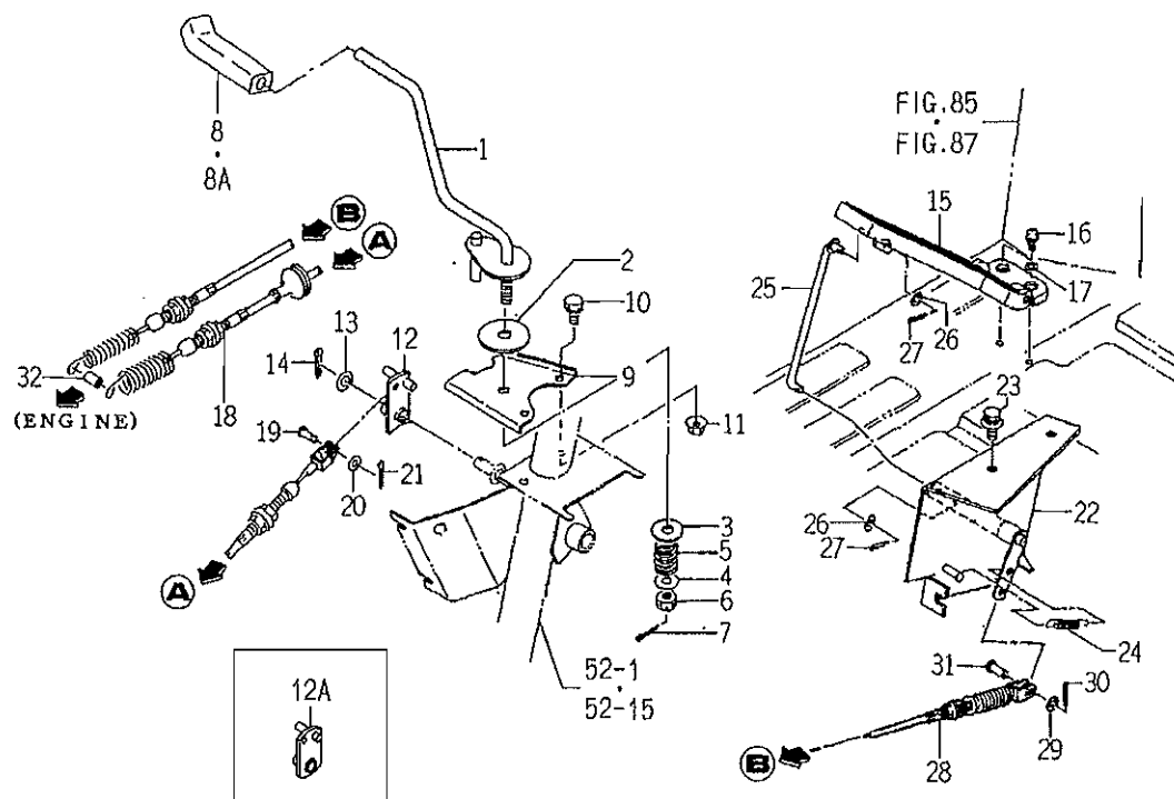
FIG. 8 ACCELERATOR SYSTEM
