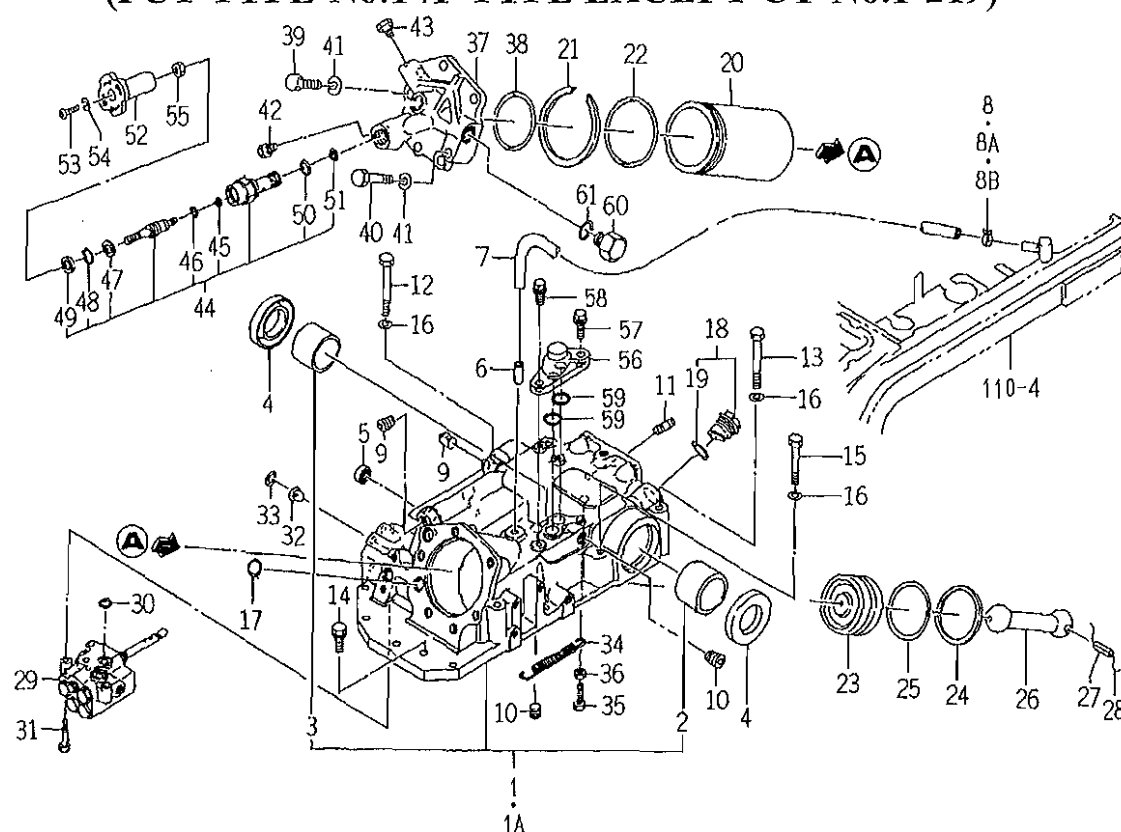
FIG. 61 CYLINDER CASE SYSTEM (PCY TYPE-No.1-/P TYPE EXCEPT CY-No.1-219)
