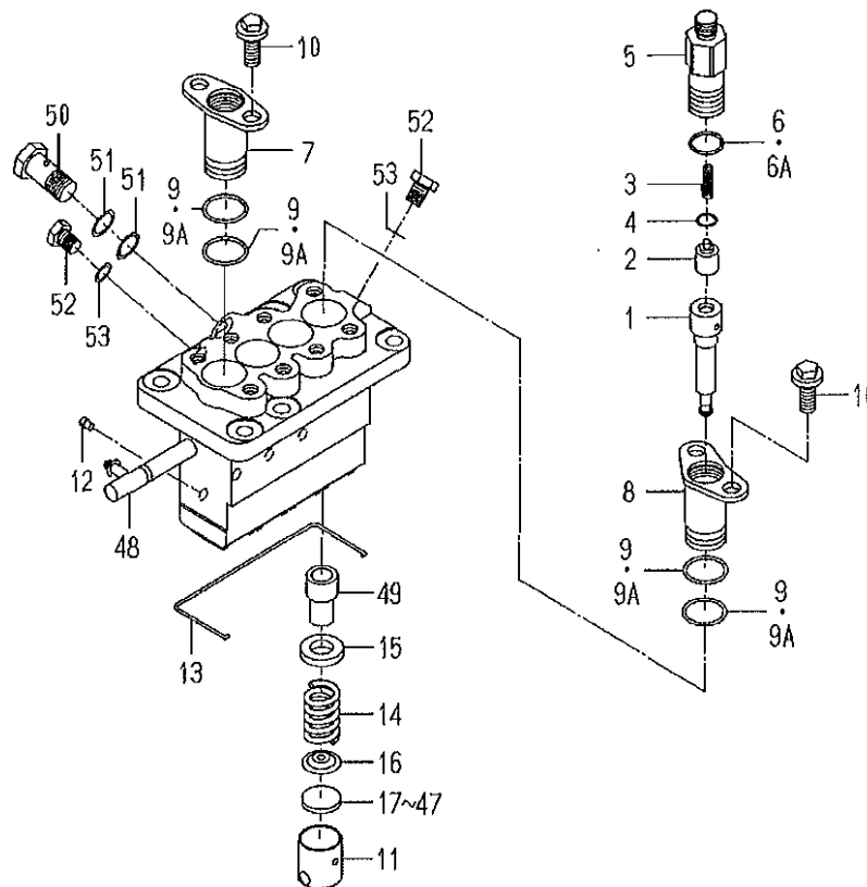
FIG. 30 COMPONENT PARTS FOR 6215-600-119-10,20 ON Fig.20,21
