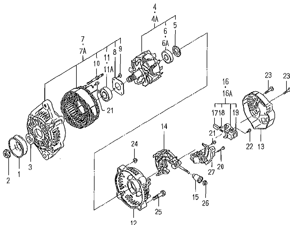
FIG. 32 COMPONENT PARTS FOR 6281-200-015-00 ON Fig.24
