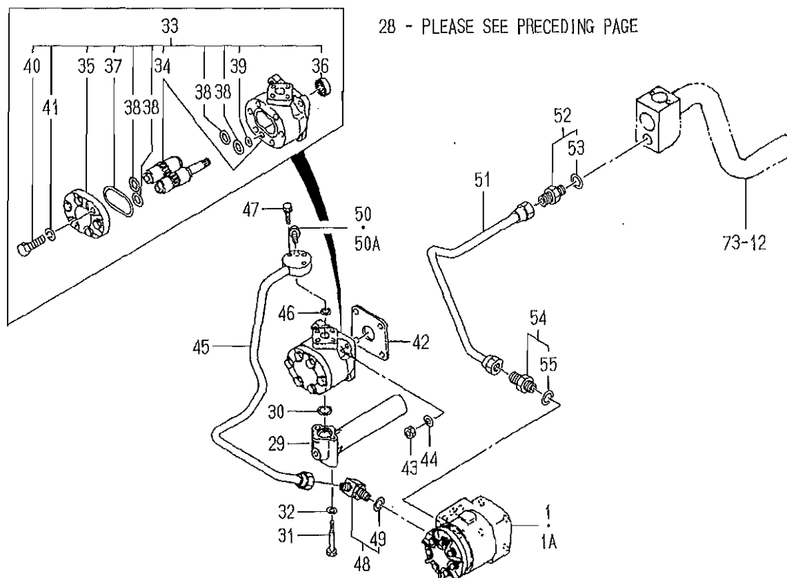
FIG. 53 STEERING (POWER) SYSTEM (S TYPE)(2/2)
