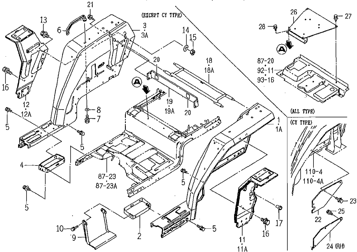
FIG. 85 FENDER,BRACKET (SEAT) SYSTEM
