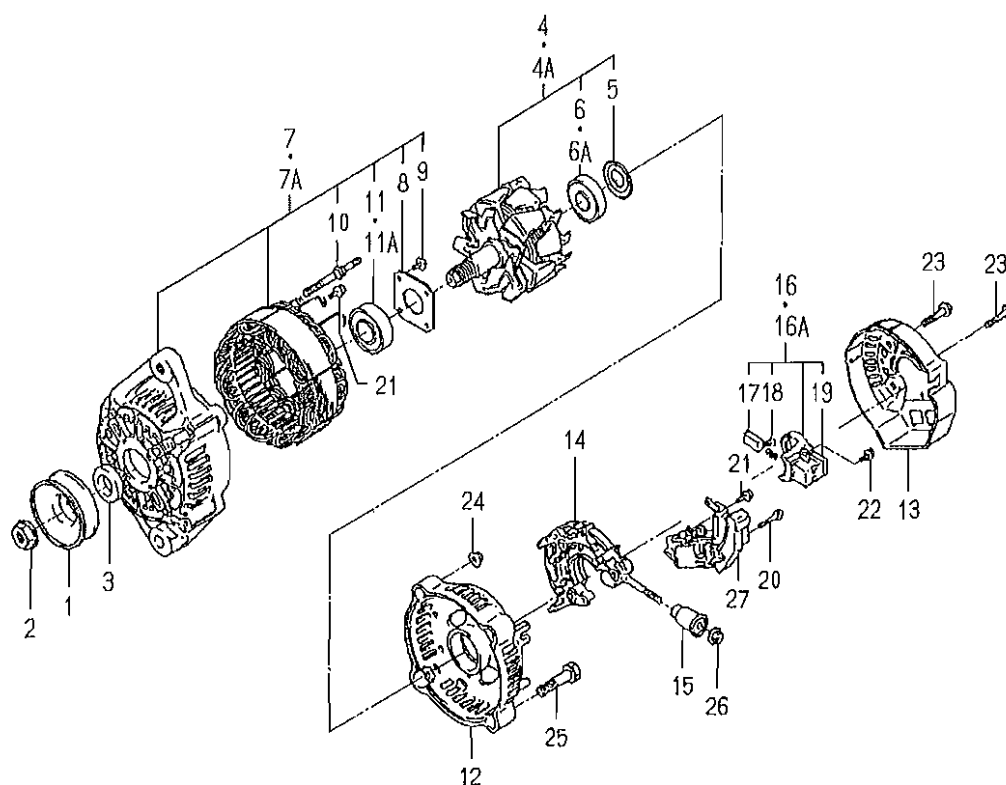
FIG. 33 COMPONENT PARTS FOR 6281-200-015-00 ON Fig.24,25
