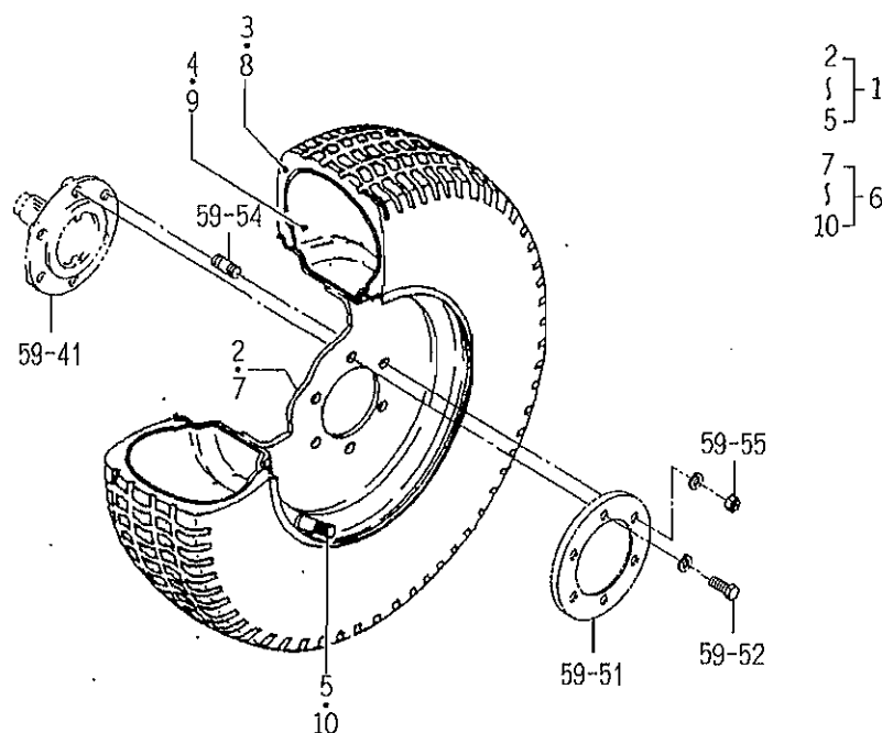
FIG.138 FRONT WHEEL (TURF) SYSTEM (2) (OPTION)
