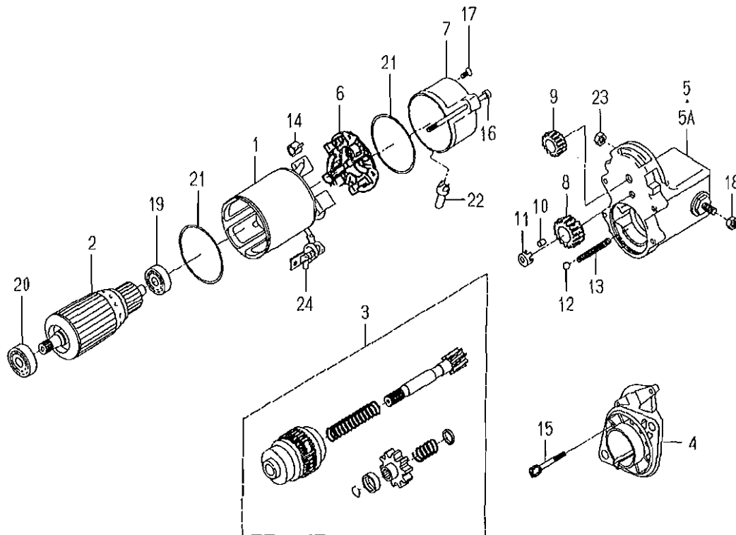
FIG. 32 COMPONENT PARTS FOR 6281-100-010-20,30 ON Fig.24,25
