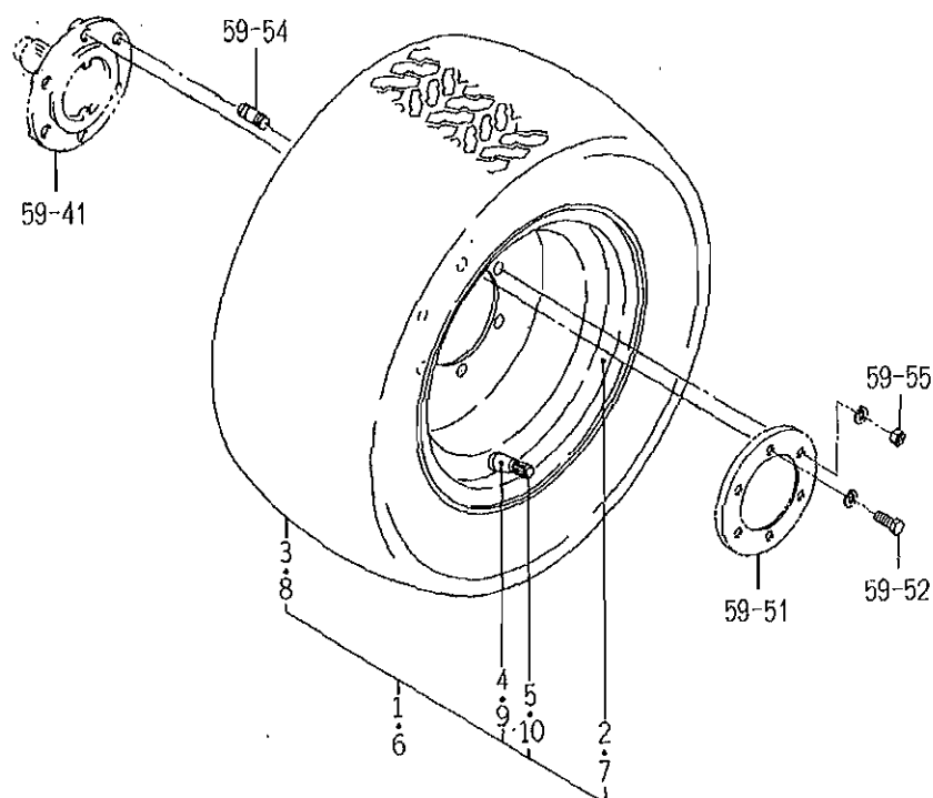
FIG.137 FRONT WHEEL (TURF) SYSTEM (1) (OPTION)
