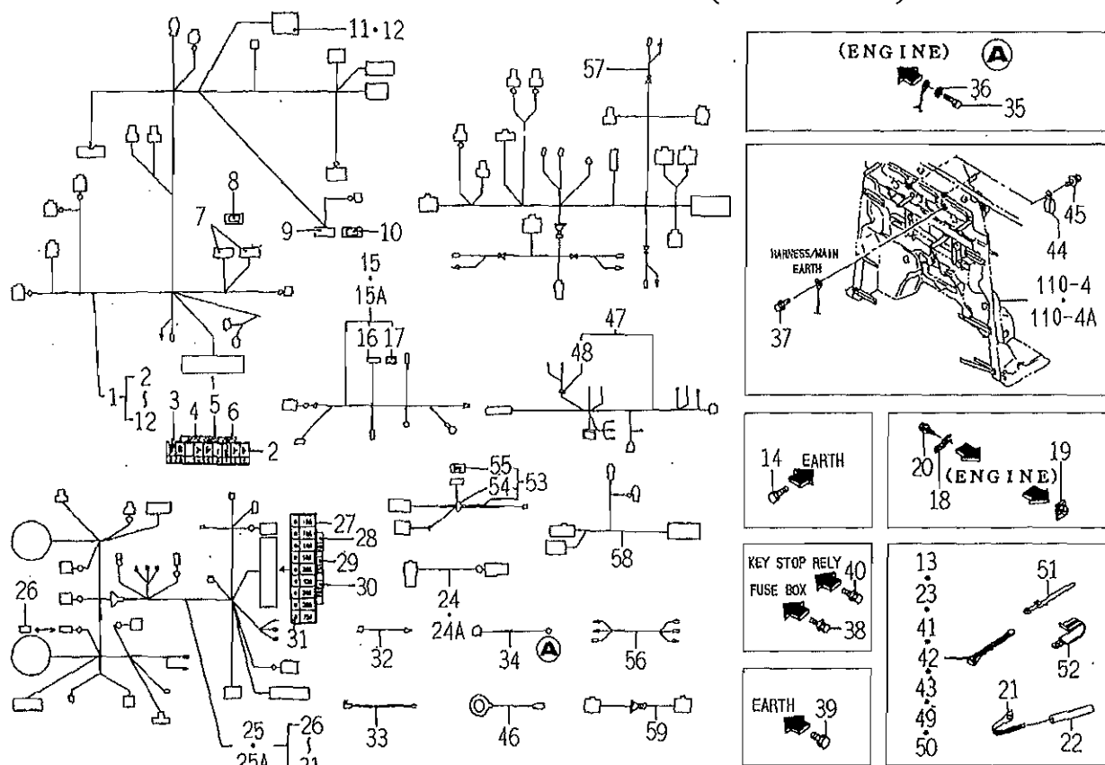
FIG.105 HARNESS SYSTEM (SCY TYPE)
