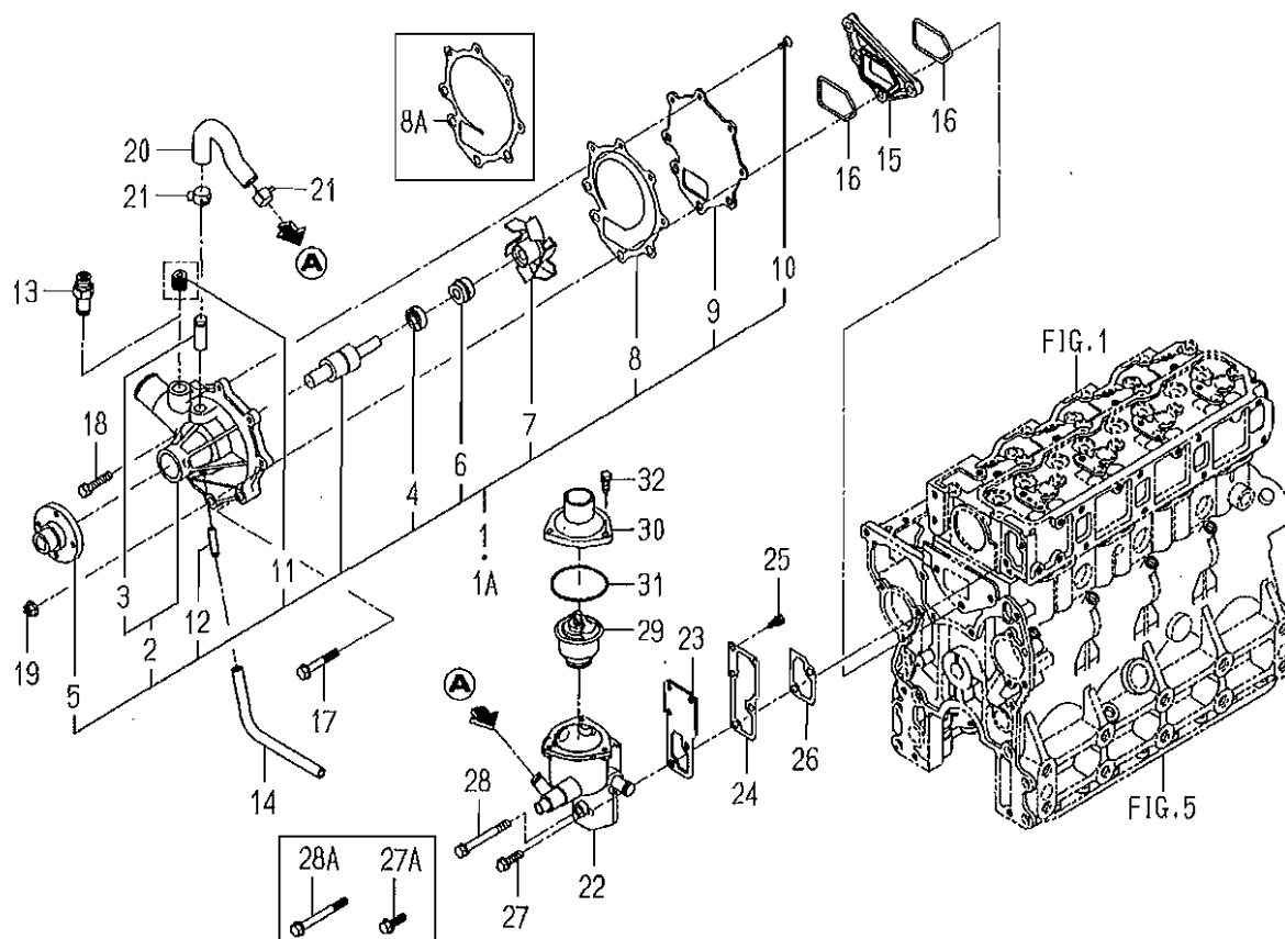
FIG. 17 WATER PUMP
