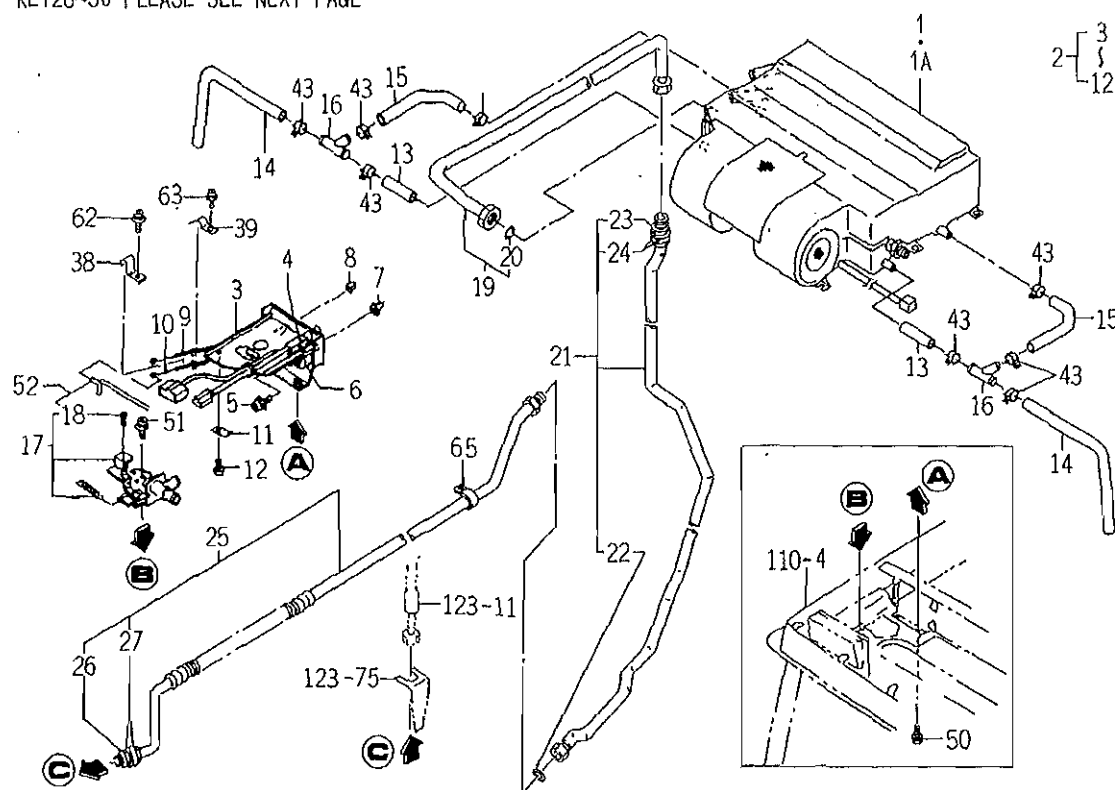
FIG.123 AIR CONDITIONER (CABIN) SYSTEM(1/3) (CY TYPE)
