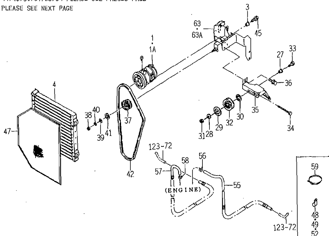
FIG.122 AIR CONDITIONER (ENGINE) SYSTEM(2/3) (CY TYPE)
