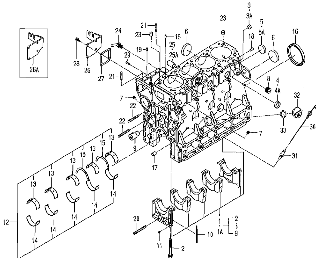
FIG. 5 CYLINDER BLOCK
