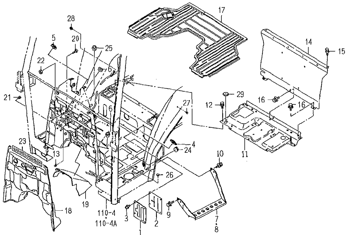
FIG. 94 FLOOR SYSTEM (PCY TYPE)
