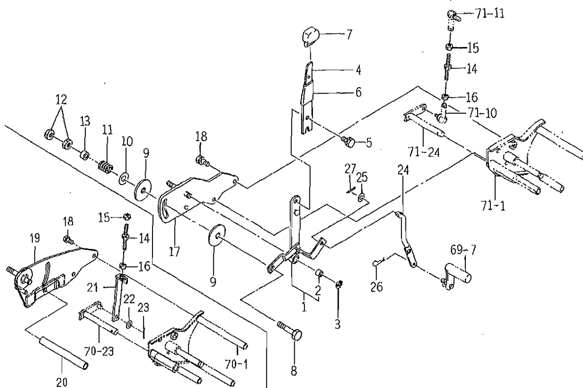
FIG. 72 LEVER (DEPTH/S TYPE), ROD (POSITION), ROD (DRAFT/S TYPE) SYSTEM
