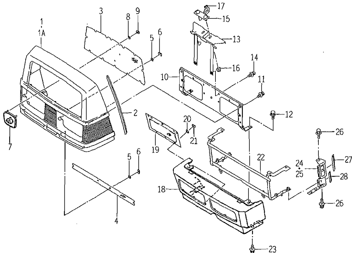
FIG. 81 GRILLE SYSTEM
