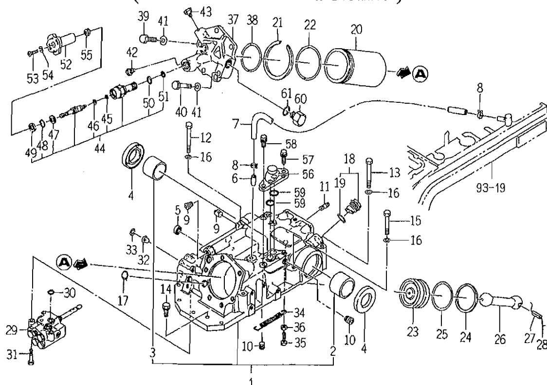
FIG. 63 CYLINDER CASE SYSTEM (P TYPE EXCEPT CY-No.220-)
