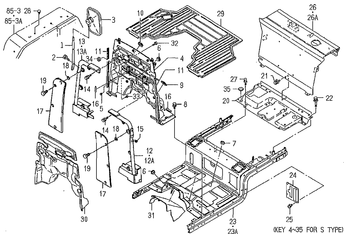
FIG. 87 BACK MIRROR (EXCEPT CY TYPE), FLOOR (S TYPE EXCEPT CY) SYSTEM
