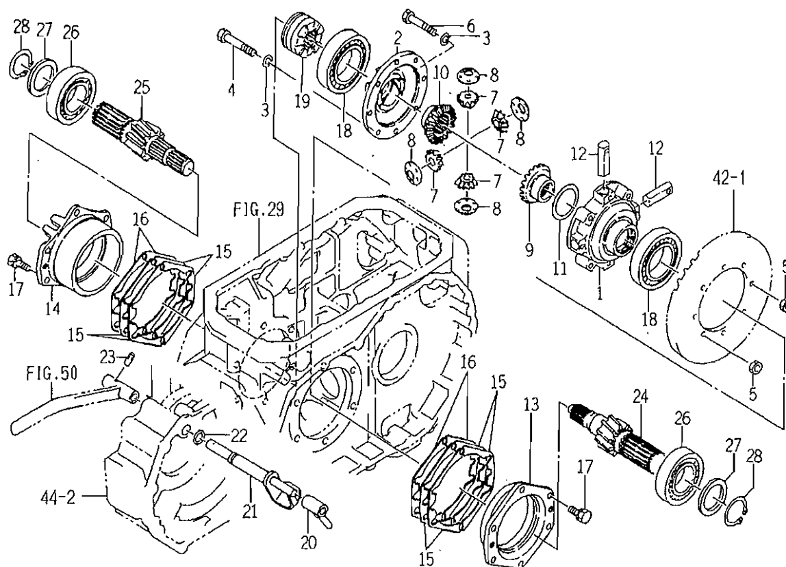
FIG. 43 DIFF, WHEEL PINION SYSTEM
