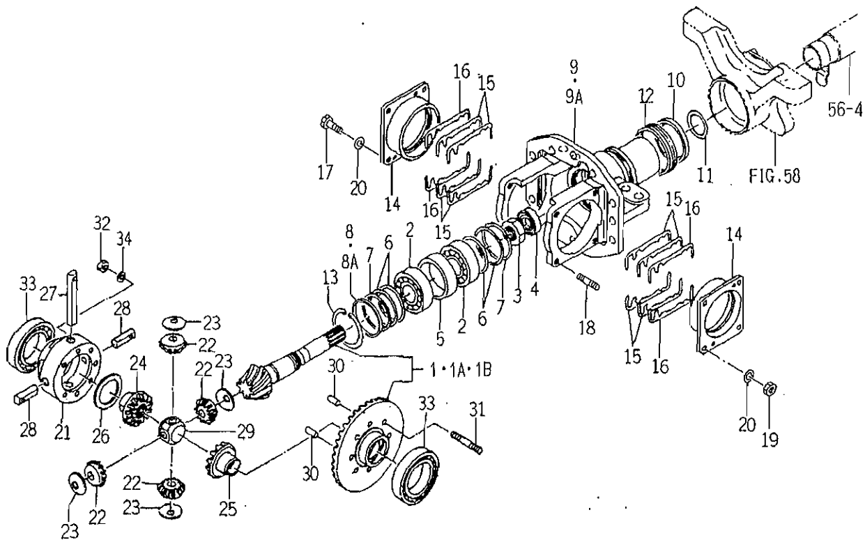
FIG. 57 CASE (BEVEL) SYSTEM
