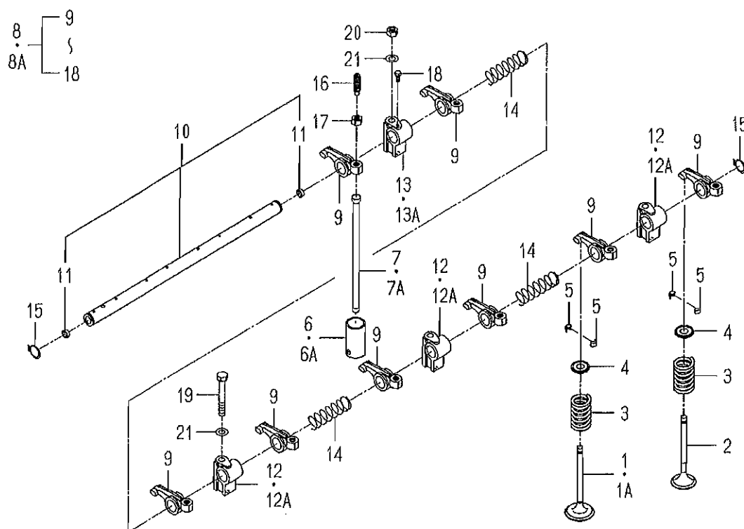
FIG. 11 VALVE
