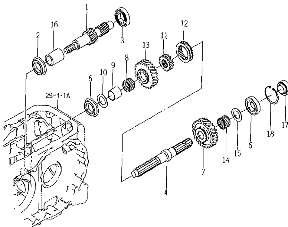
FIG. 34 PTO COUNTER GEAR, PTO CHANGE GEAR SYSTEM
