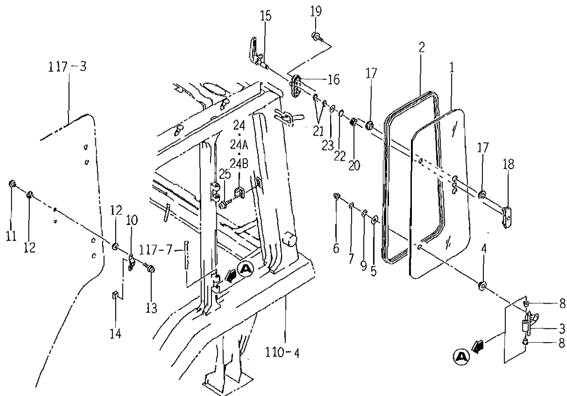
FIG.119 GLASS (SIDE) SYSTEM (CY TYPE)
