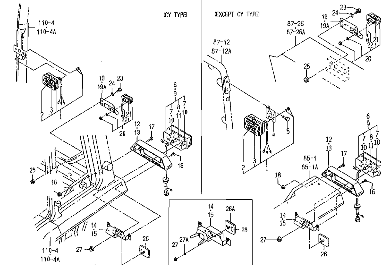
FIG. 97 LAMP SYSTEM
