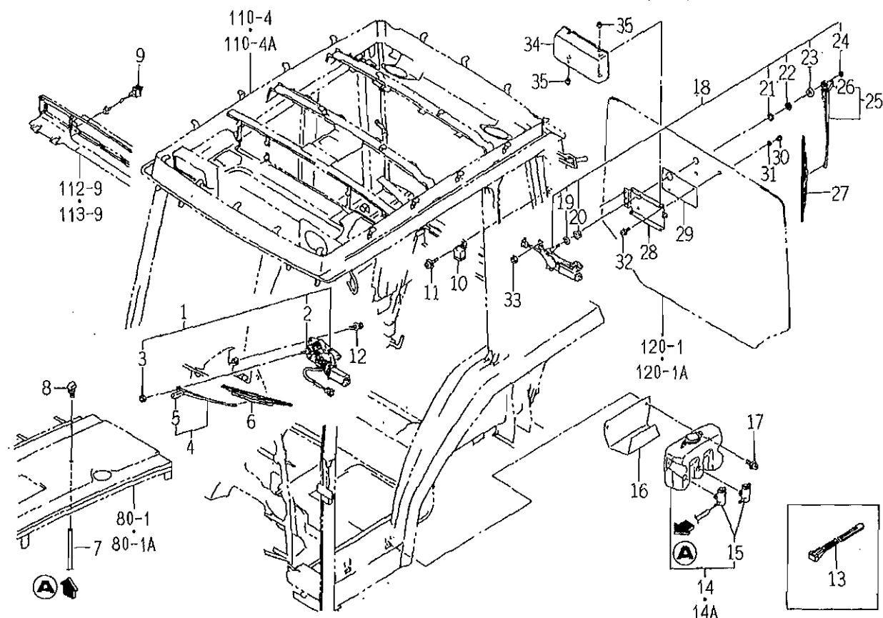
FIG.106 ELC.SYSTEM (CY TYPE)(1/3)
