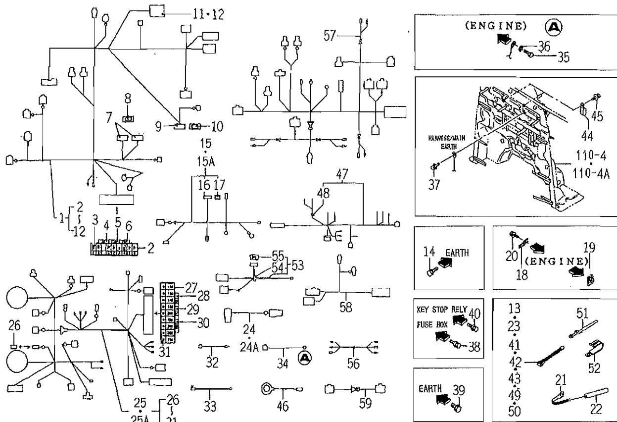
FIG.105 HARNESS SYSTEM (SCY TYPE)
