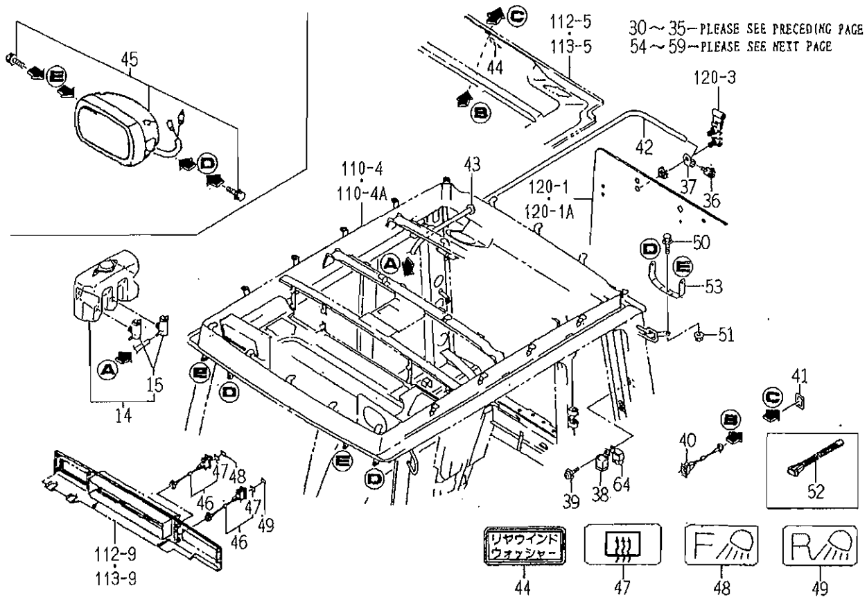
FIG.106 ELC.SYSTEM (CY TYPE)(2/3)
