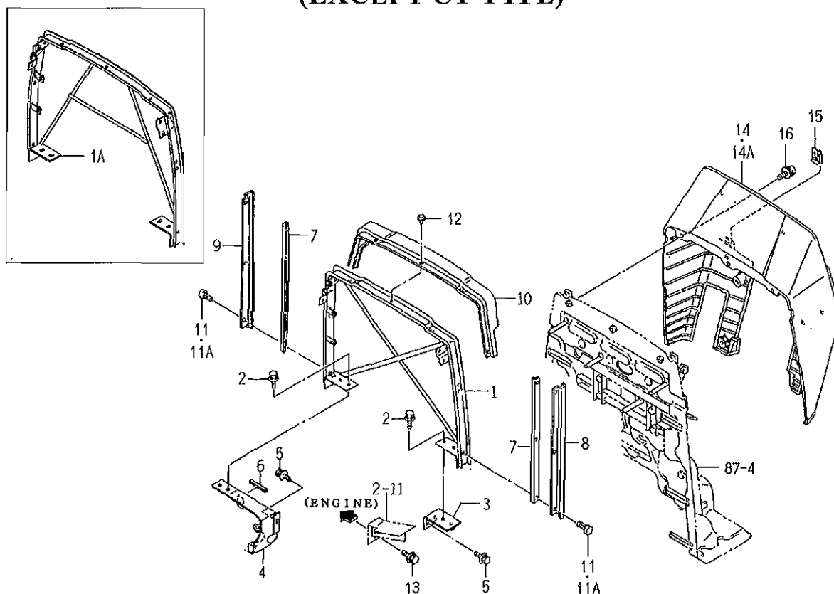
FIG. 82 FRAME,DASH BOARD SYSTEM (EXCEPT CY TYPE)
