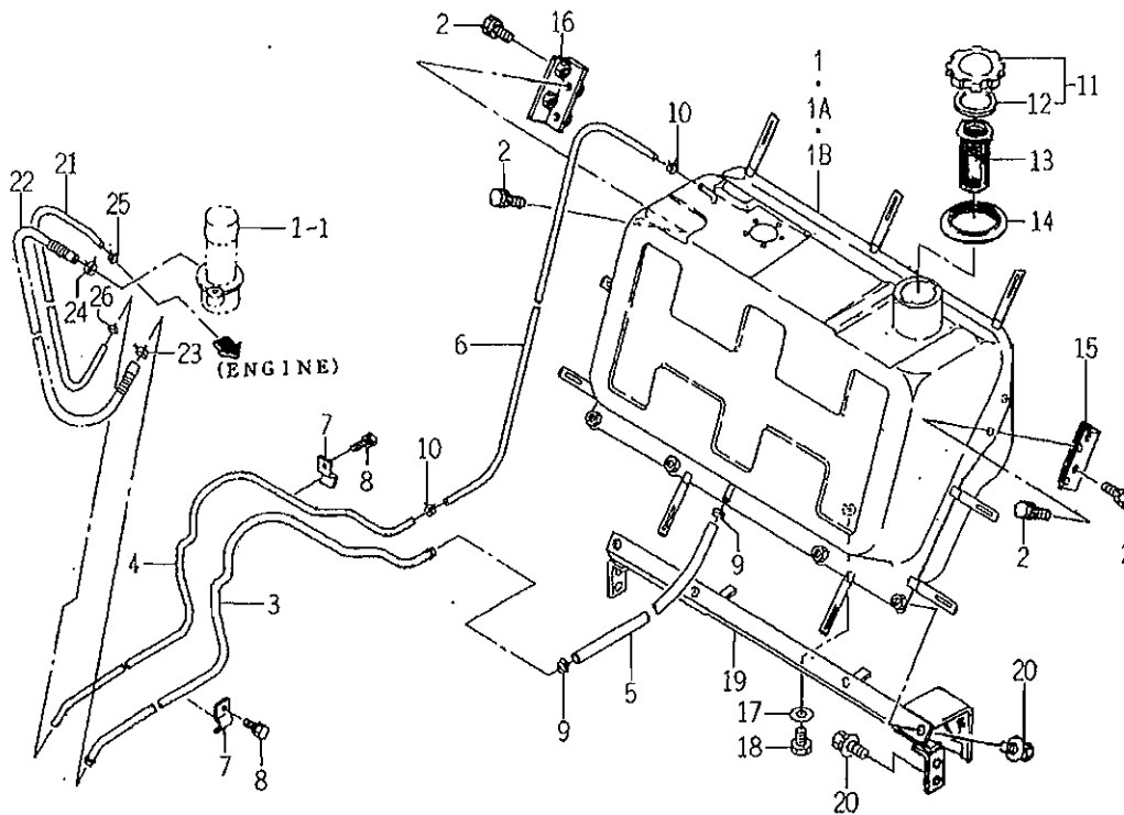
FIG. 5 FUEL TANK SYSTEM (EXCEPT CY TYPE)
