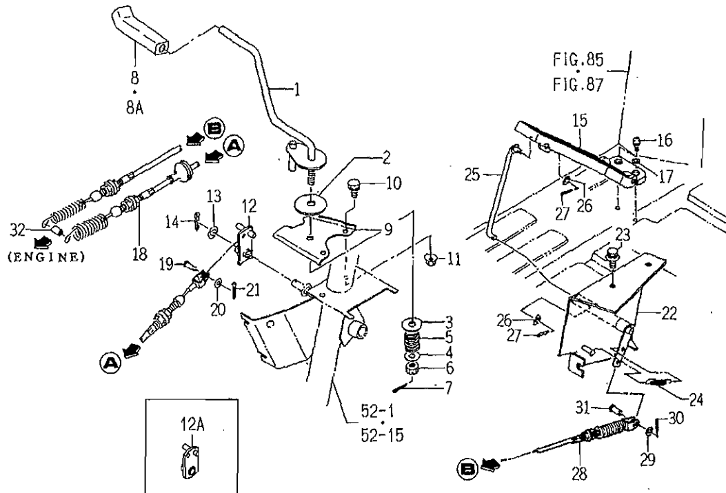
FIG. 8 ACCELERATOR SYSTEM
