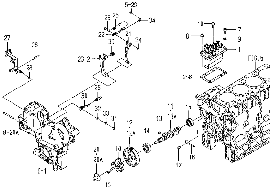
FIG. 20 INJECTION PUMP (No.3763-)
