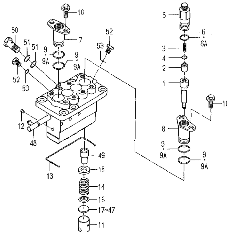
FIG. 31 COMPONENT PARTS FOR 6215-600-119-10,20 ON Fig.20,21
