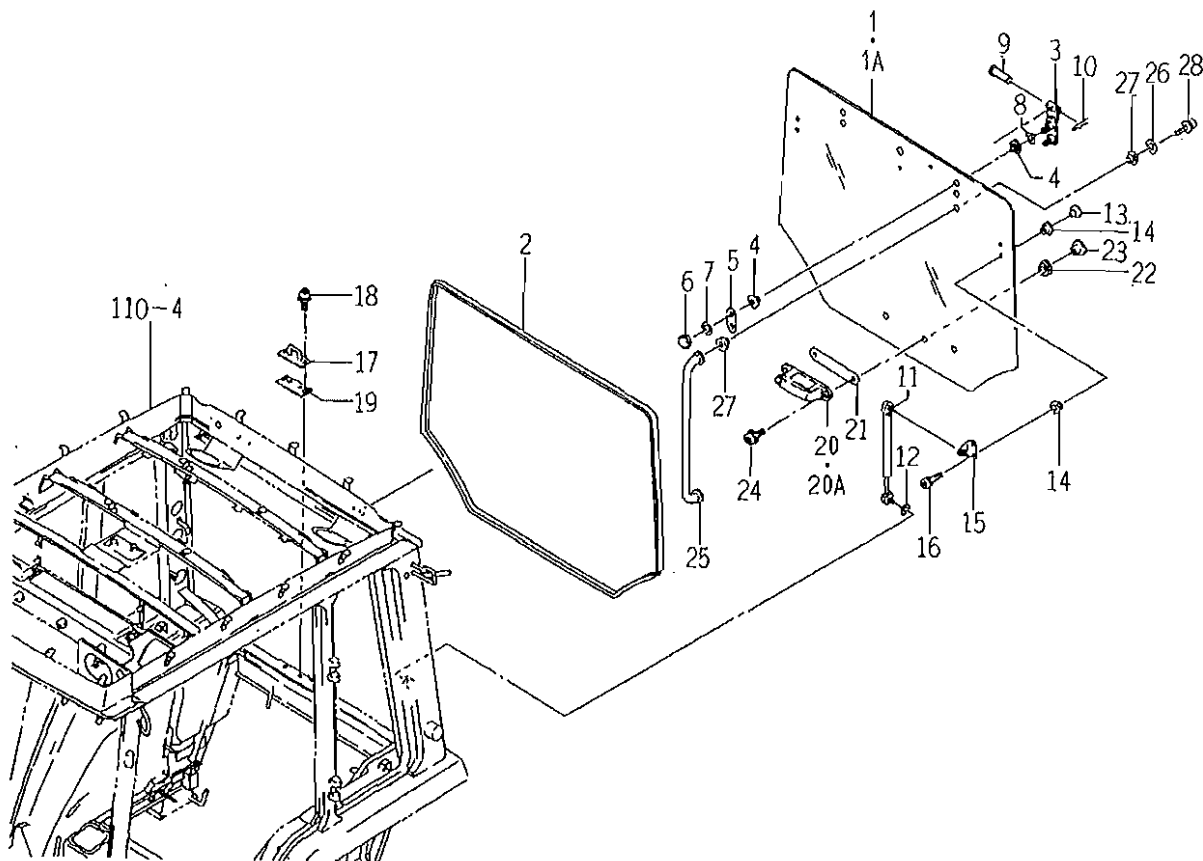
FIG.120 GLASS (REAR) SYSTEM (CY TYPE)
