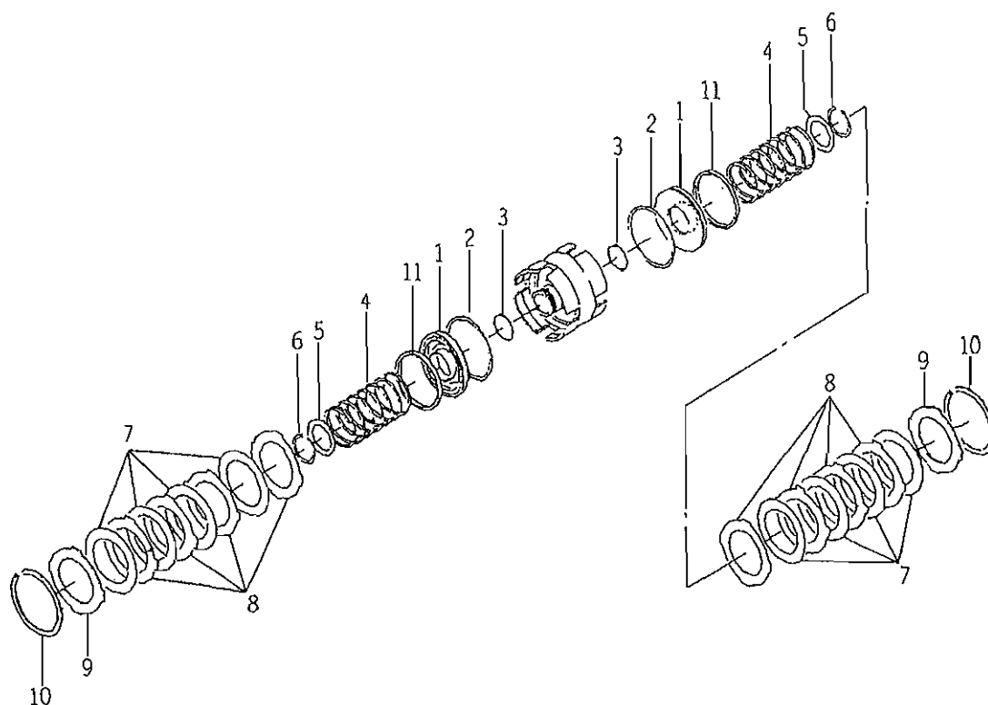
FIG.154 COMPONENT PARTS FOR 1646-217-310-00 ON Fig.18
