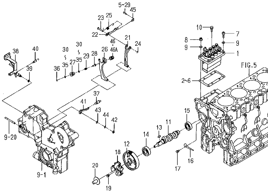
FIG. 21 INJECTION PUMP (No.1-3762)
