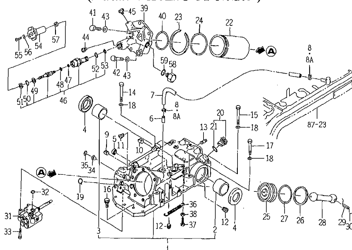
FIG. 62 CYLINDER CASE SYSTEM (S TYPE EXCEPT CY-No.205-)
