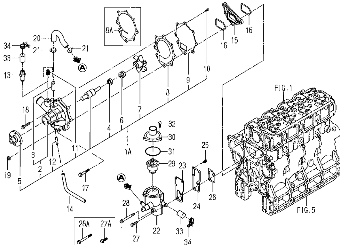
FIG. 17 WATER PUMP
