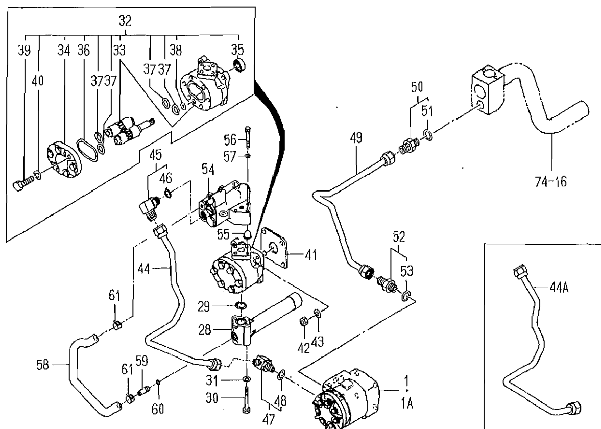
FIG. 54 STEERING (POWER) SYSTEM (P TYPE)(2/2)
