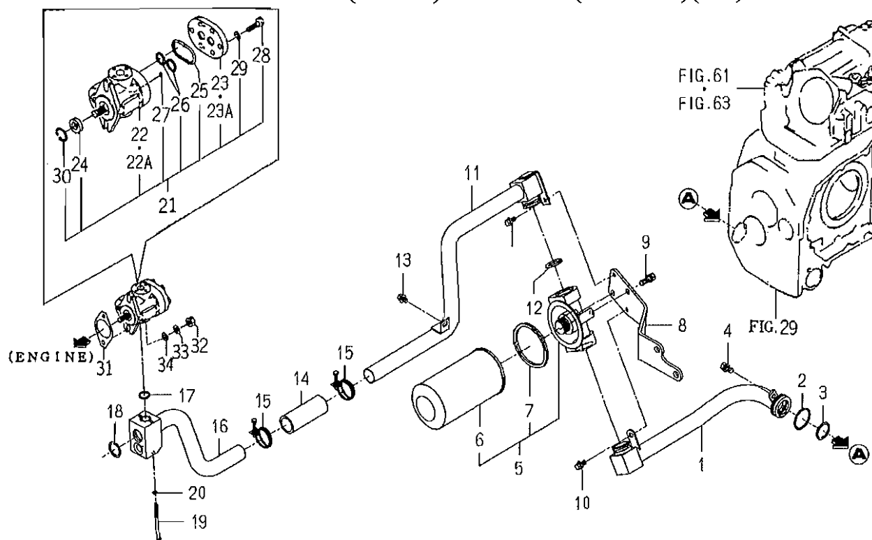
FIG. 74 PIPING (MAIN) SYSTEM (P TYPE)(1/2)
