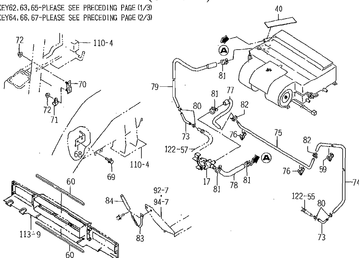
FIG.123 AIR CONDITIONER (CABIN) SYSTEM(3/3) (CY TYPE)
