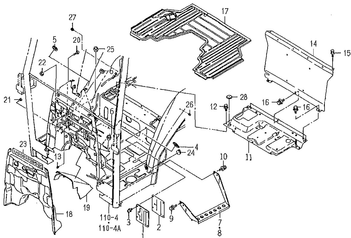
FIG. 92 FLOOR SYSTEM (SCY TYPE)
