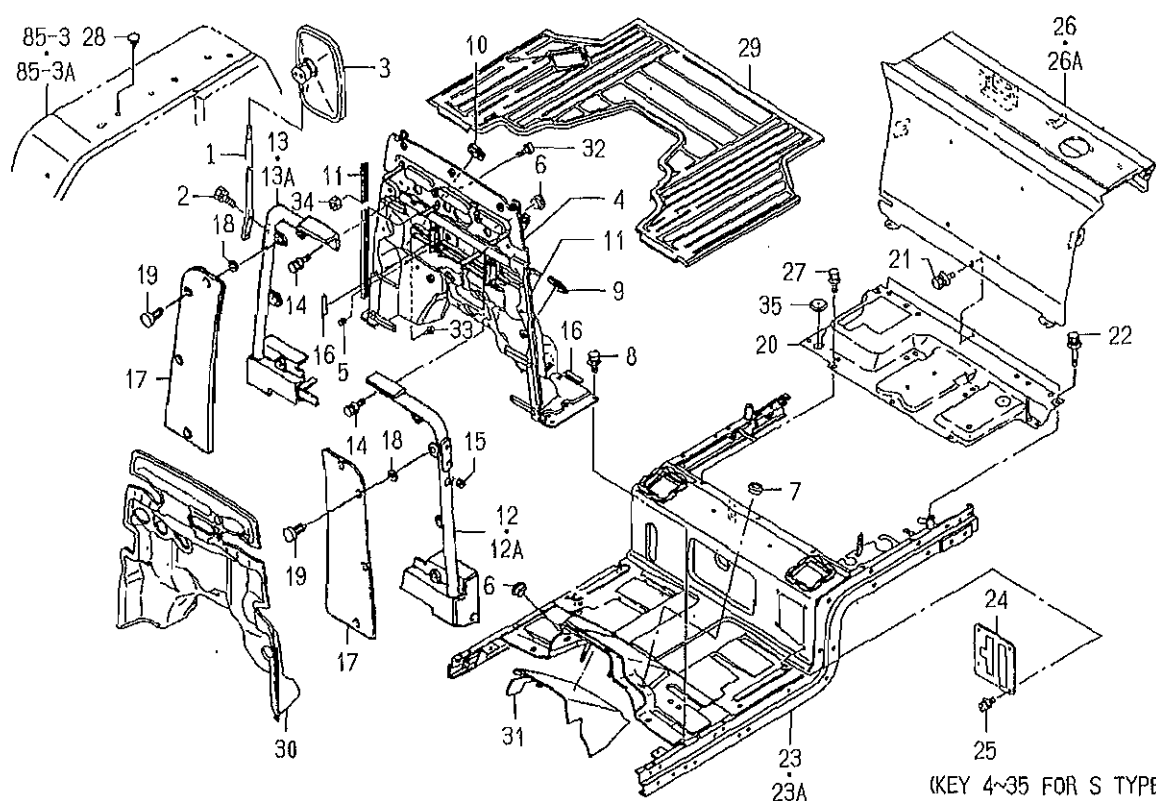
FIG. 87 BACK MIRROR (EXCEPT CY TYPE), FLOOR (S TYPE EXCEPT CY) SYSTEM
