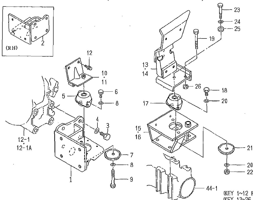
FIG. 91 FRONT MOUNT (P TYPE EXCEPT CY), REAR MOUNT (S TYPE EXCEPT CY) SYSTEM
