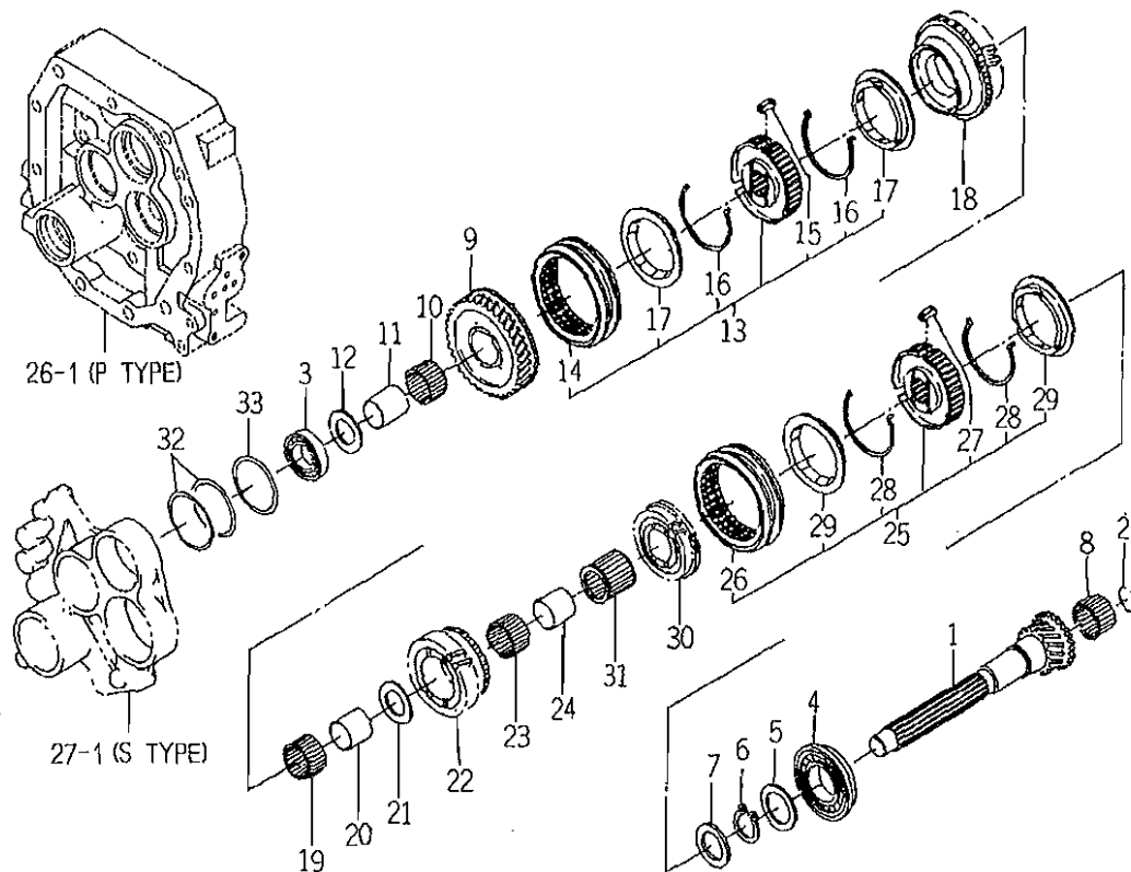
FIG. 15 CHANGE GEAR SYSTEM
