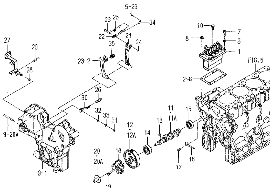
FIG. 20 INJECTION PUMP (No.3835-)
