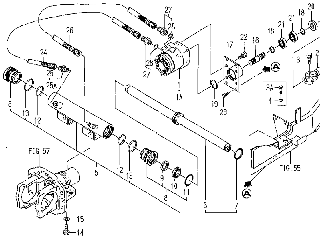
FIG. 53 STEERING (POWER) SYSTEM (S TYPE)(1/2)
