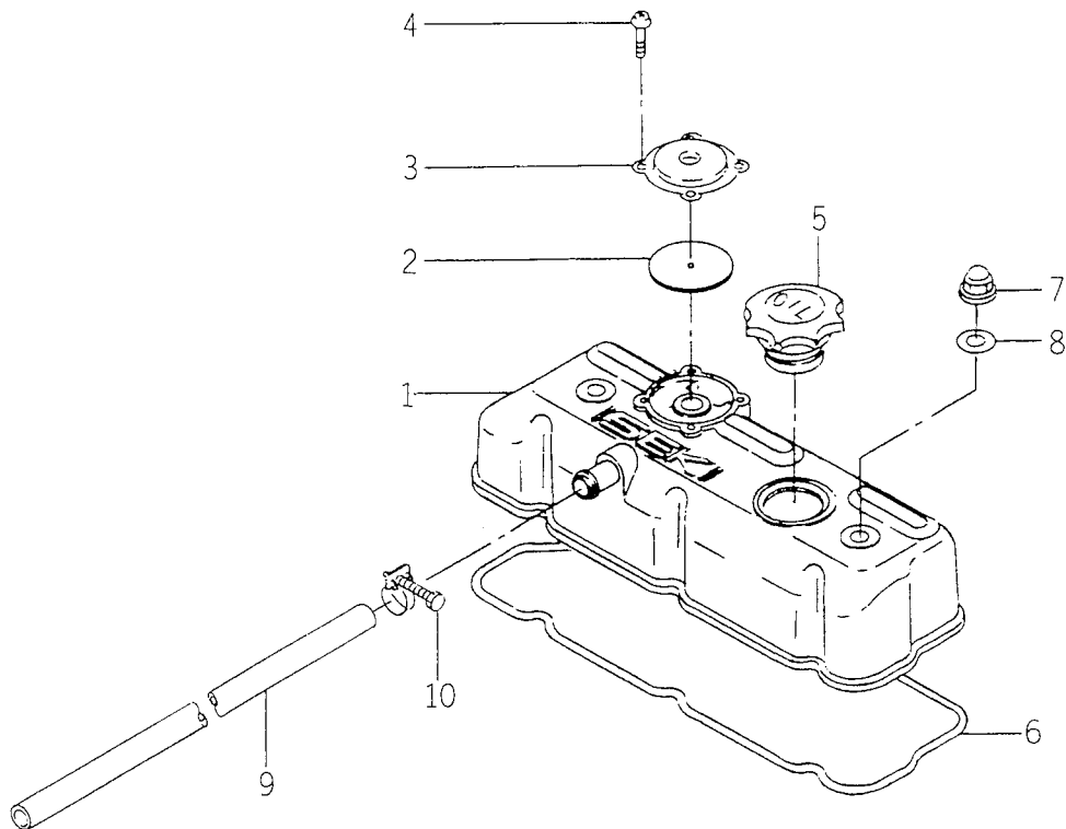
FIG. 2 CYLINDER HEAD COVER
