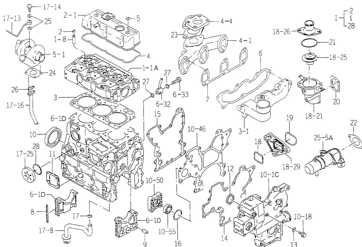
FIG. 25 REPAIR PARTS (OPTION)
