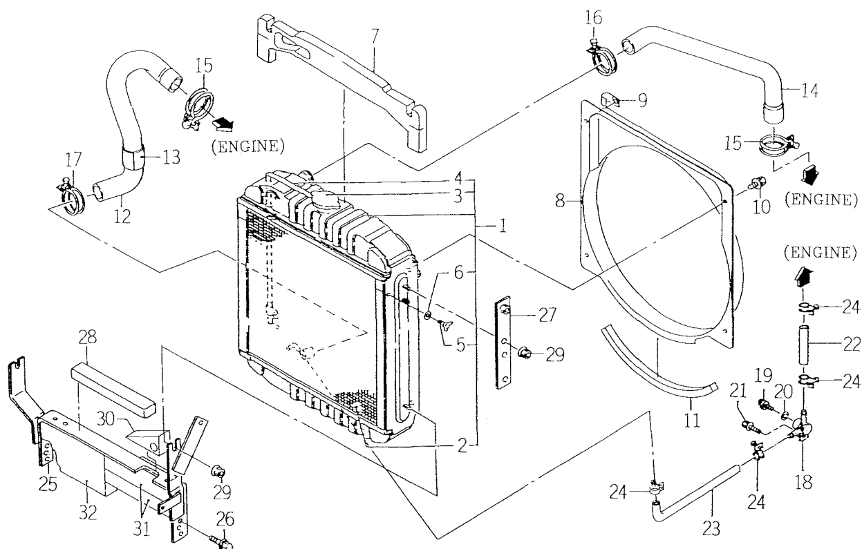
FIG. 3 RADIATOR SYSTEM
