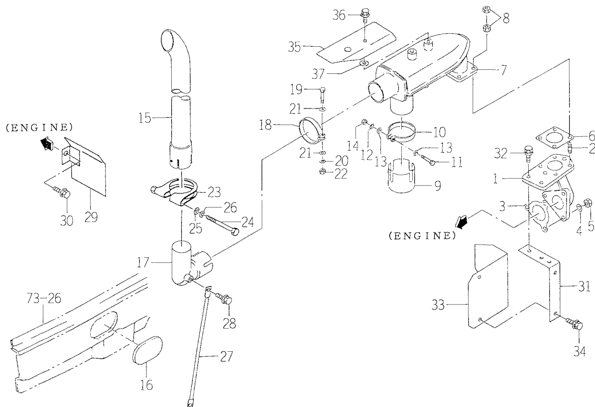
FIG. 5 MUFFLER (UPPER) SYSTEM (C TYPE)
