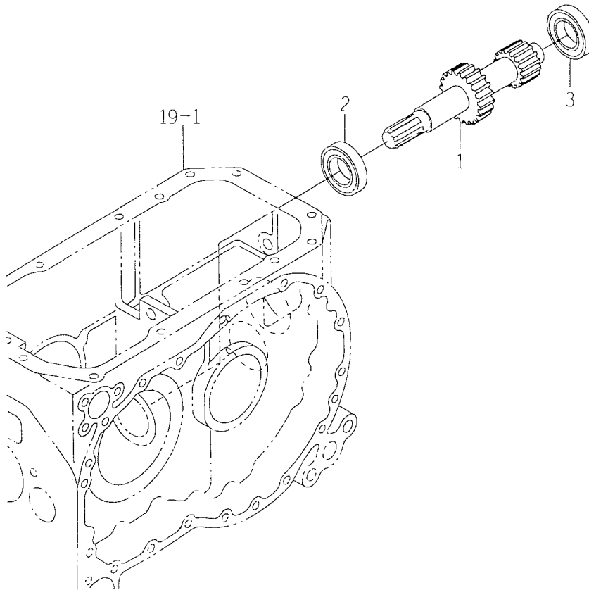
FIG. 25 PTO COUNTER SYSTEM
