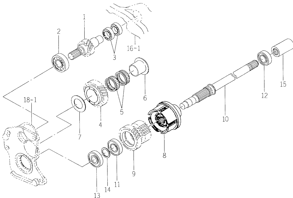
FIG. 14 GEAR (PTO) SYSTEM
