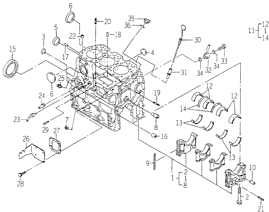
FIG. 6 CYLINDER BLOCK
