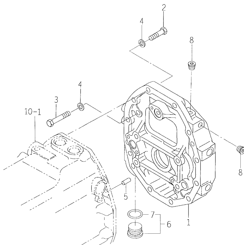
FIG. 17 CASE (SPACER) SYSTEM
