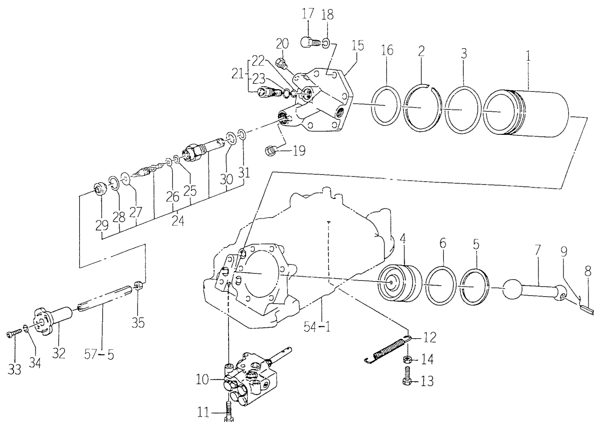
FIG. 56 CYLINDER SYSTEM
