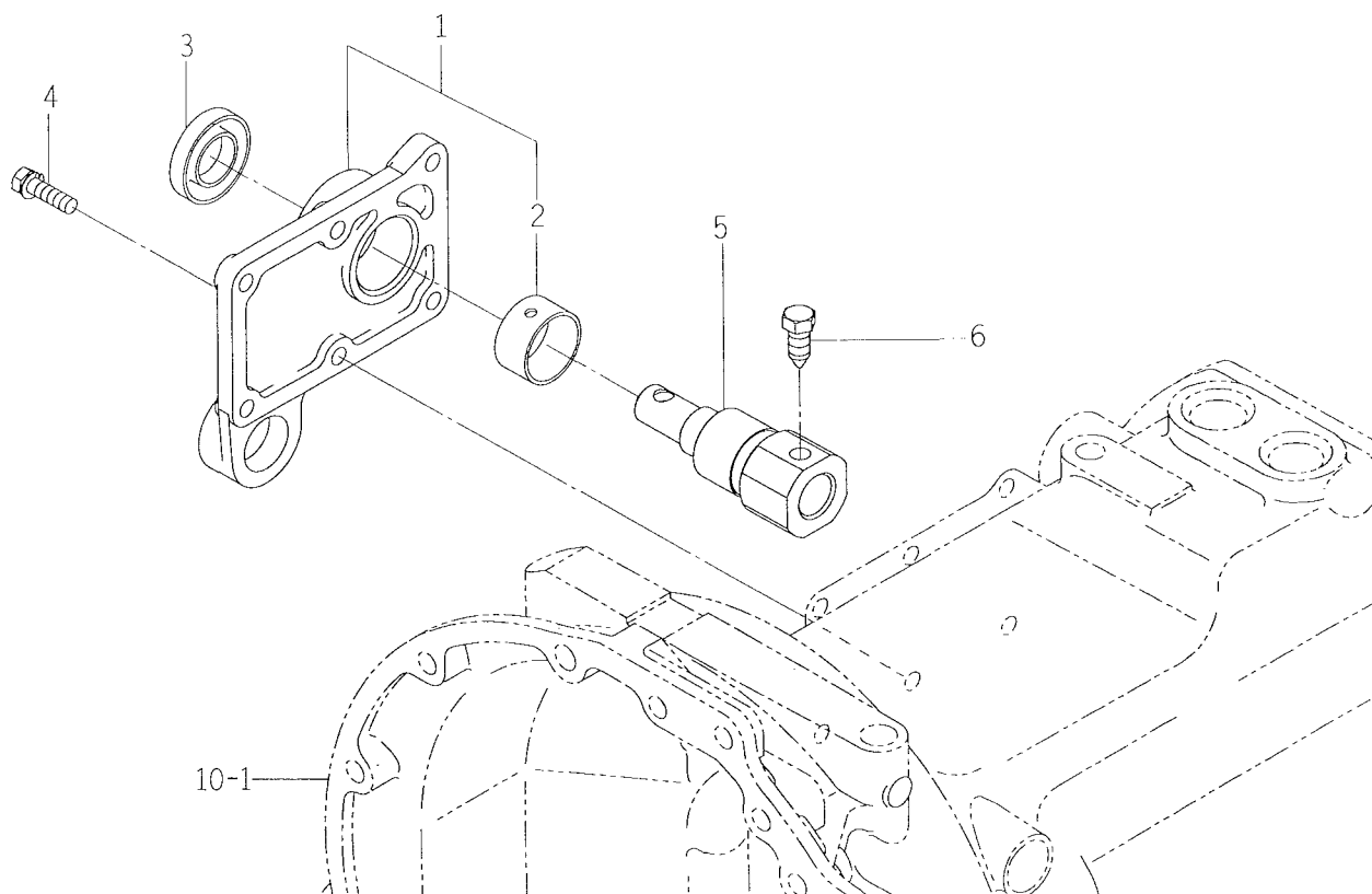
FIG. 15 METAL (TRUNNION) SYSTEM
