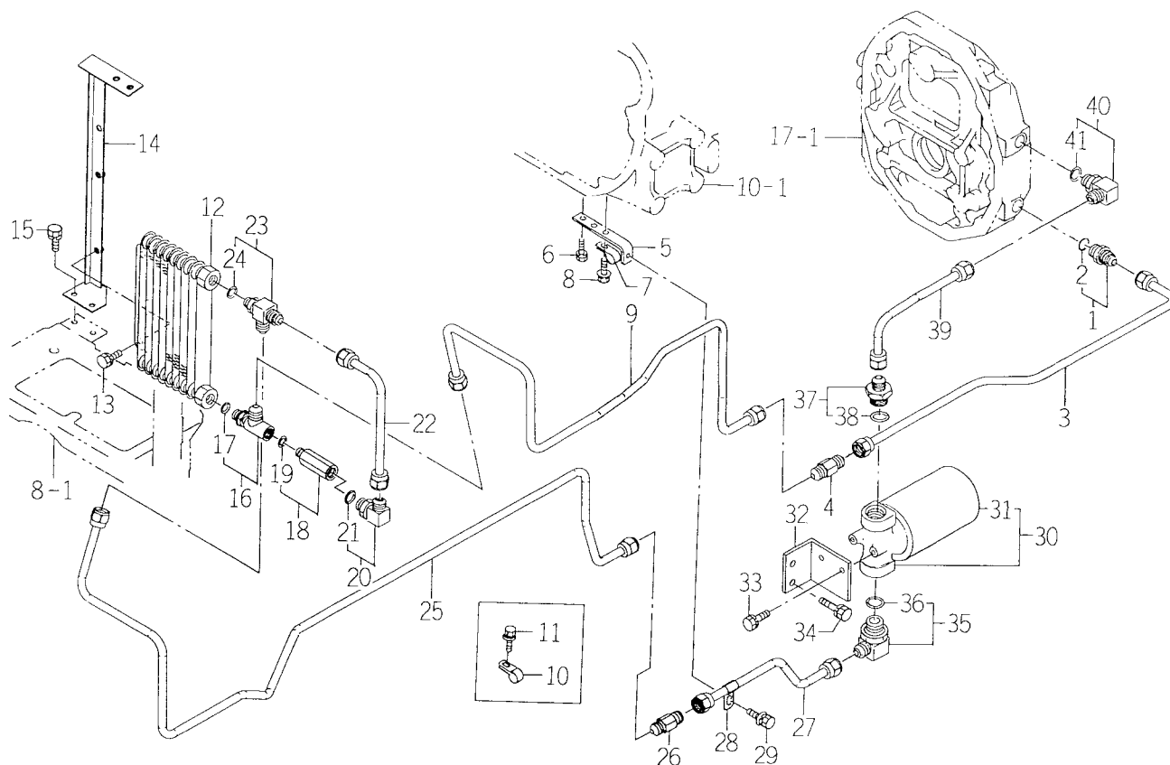
FIG. 64 PIPING (COOLER) SYSTEM
