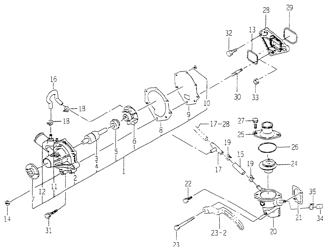
FIG. 18 WATER PUMP
