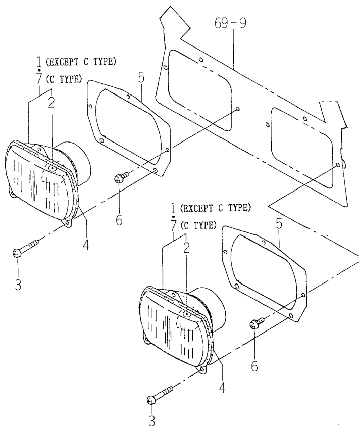
FIG. 90 HEAD LAMP SYSTEM
