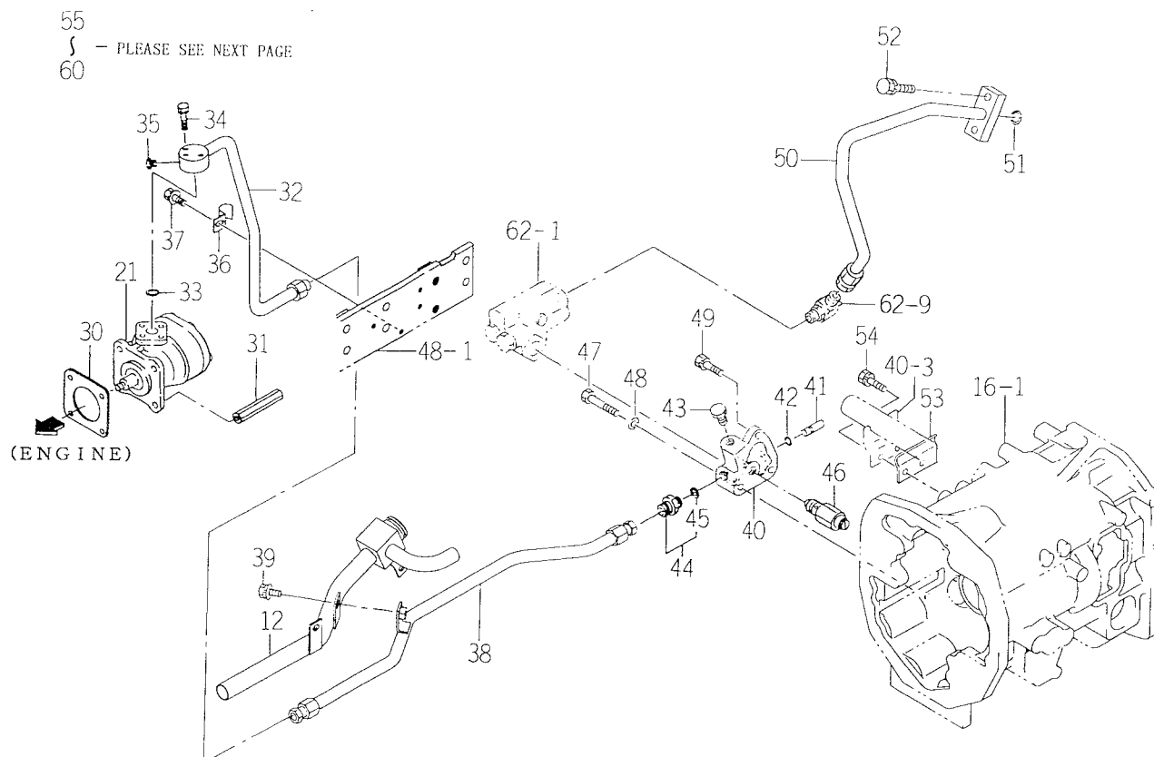
FIG. 61 PIPING (MAIN) SYSTEM (2/3)
