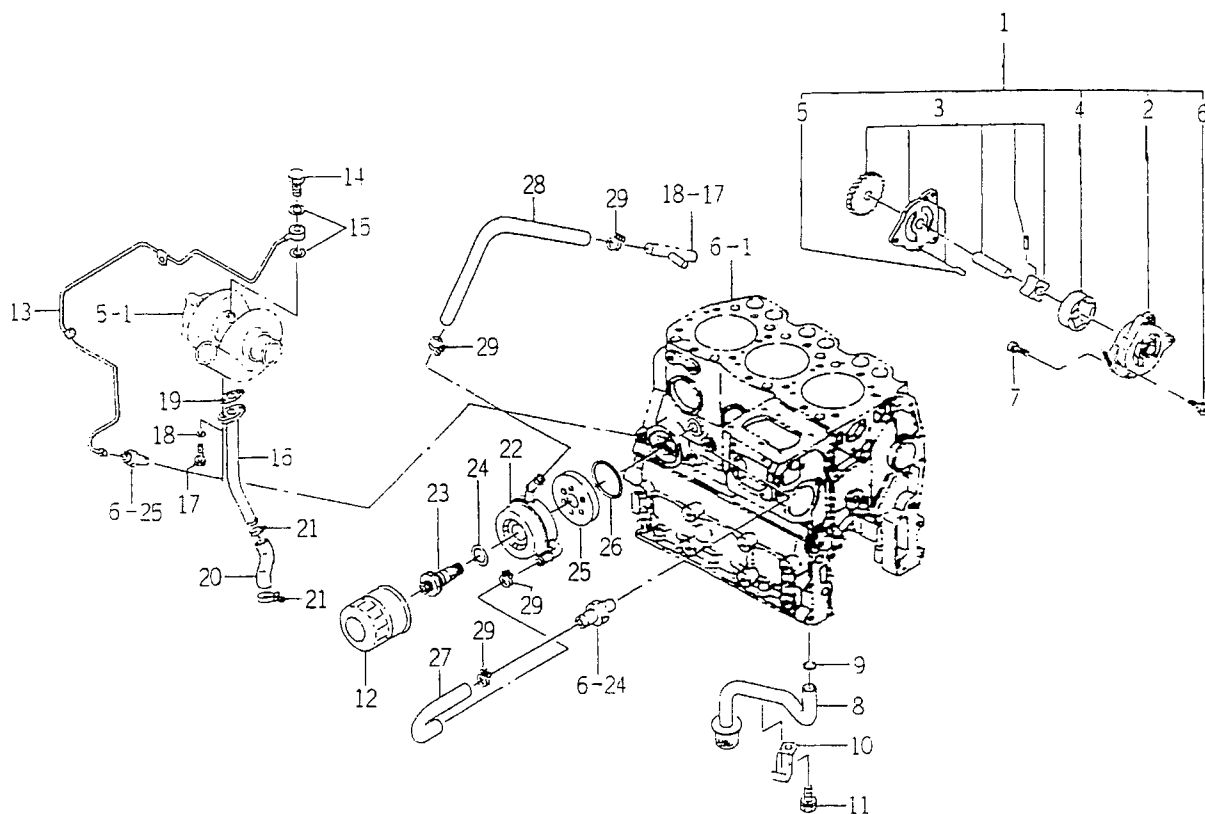
FIG. 17 OIL PUMP
