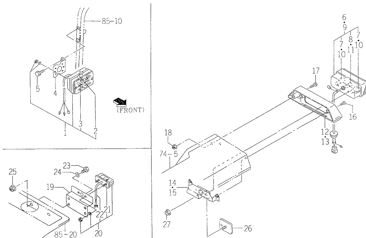
FIG. 91 LAMP SYSTEM (EXCEPT C TYPE)
