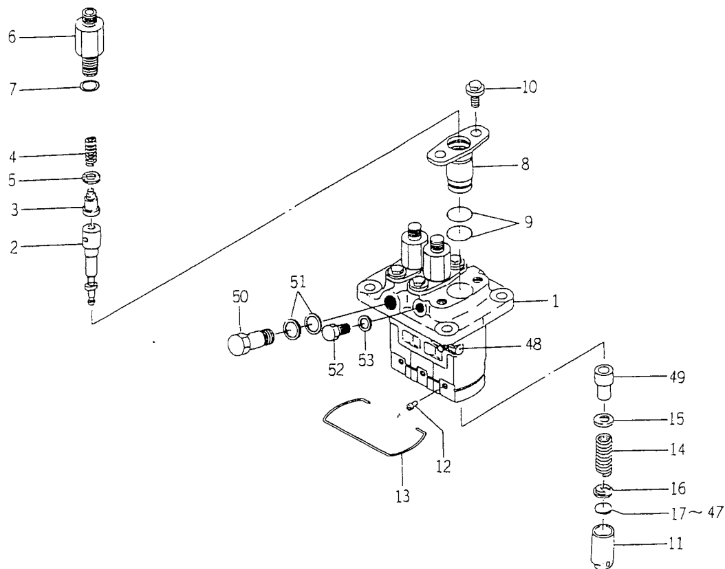
FIG. 27 COMPONENT PARTS FOR 6215-600-078-00 ON Fig.21
