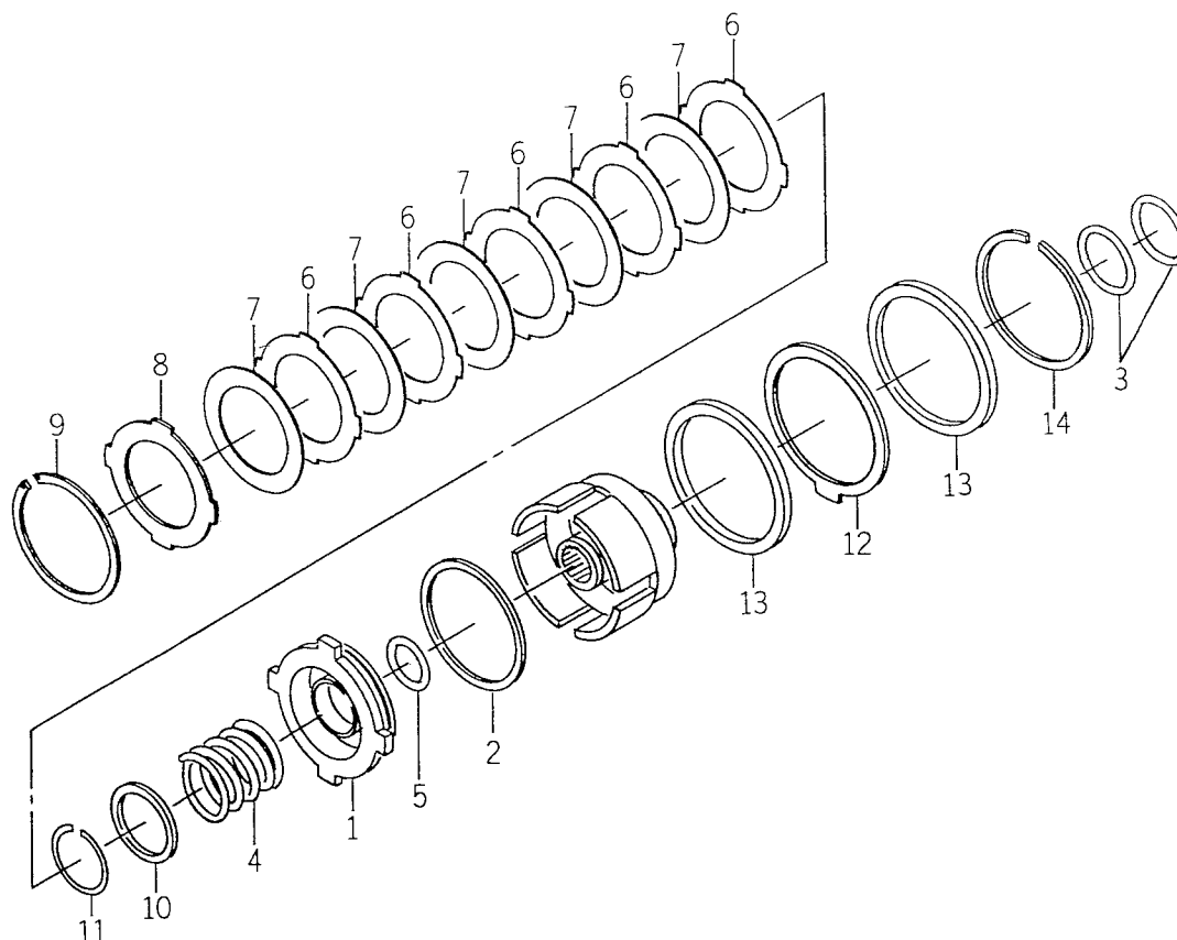
FIG.146 COMPONENT PARTS FOR 1561 - 221 - 500 - 10 ON Fig.14
