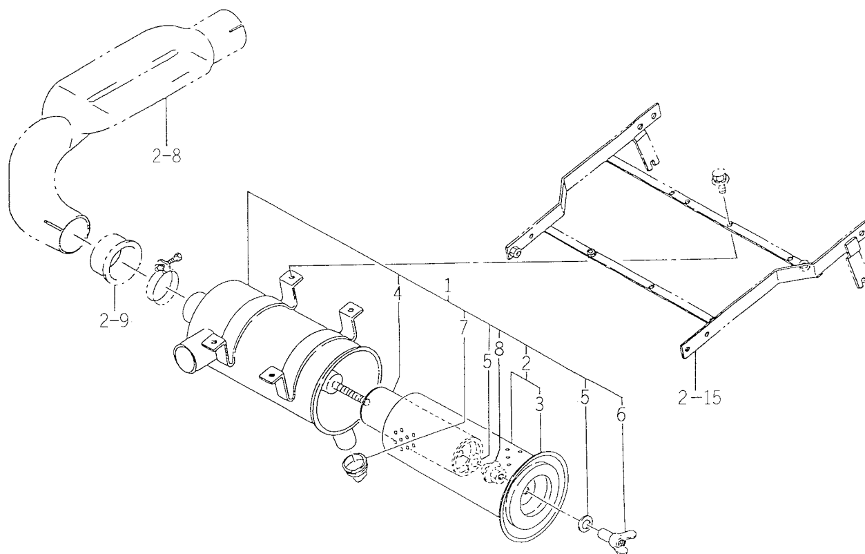
FIG.116 AIR CLEANER ASSY (OPTION)
