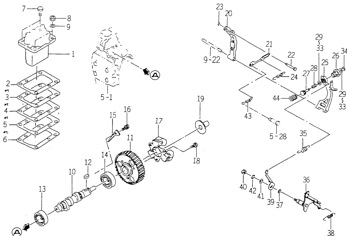
FIG. 20 INJECTION PUMP
