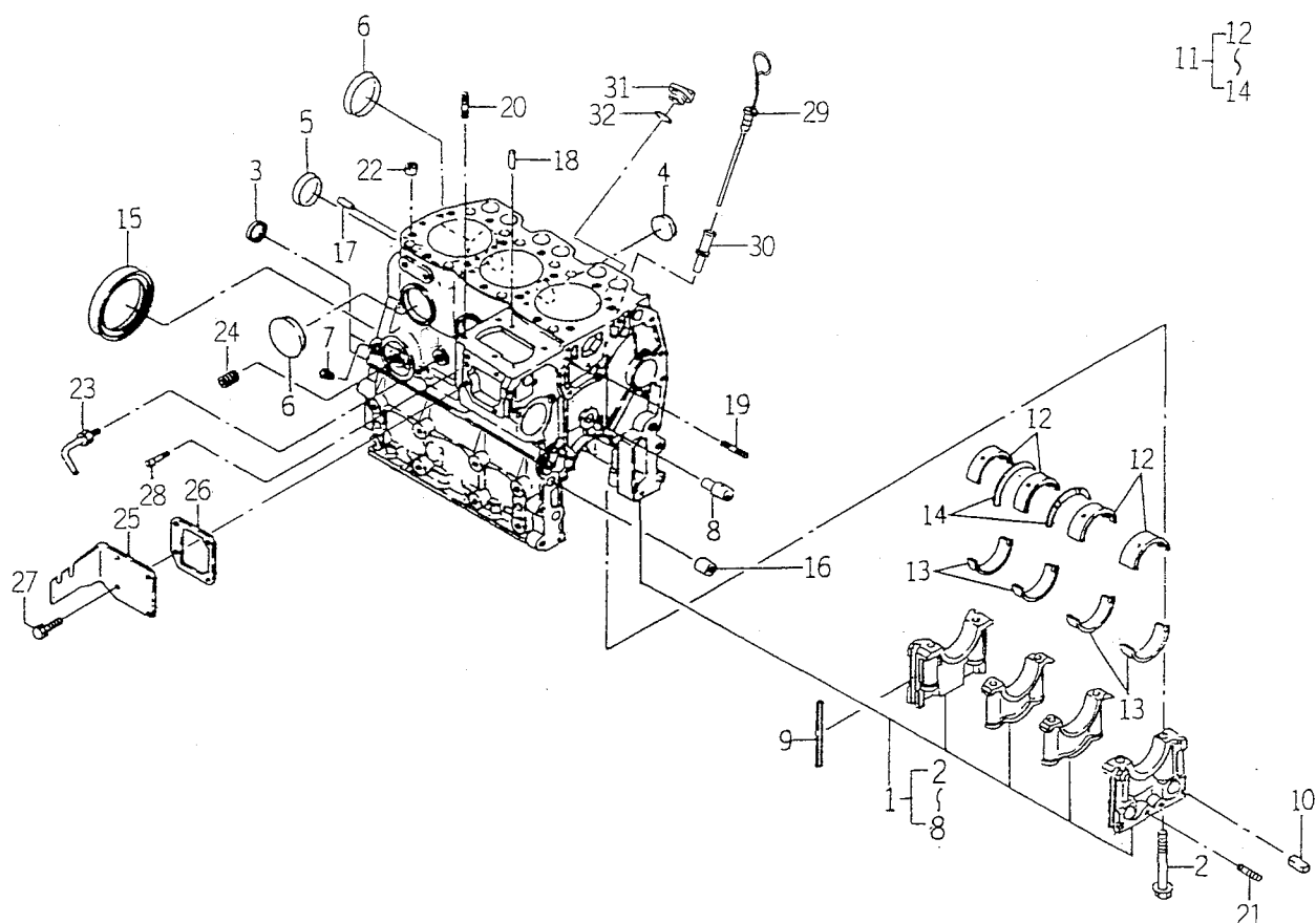
FIG. 5 CYLINDER BLOCK
