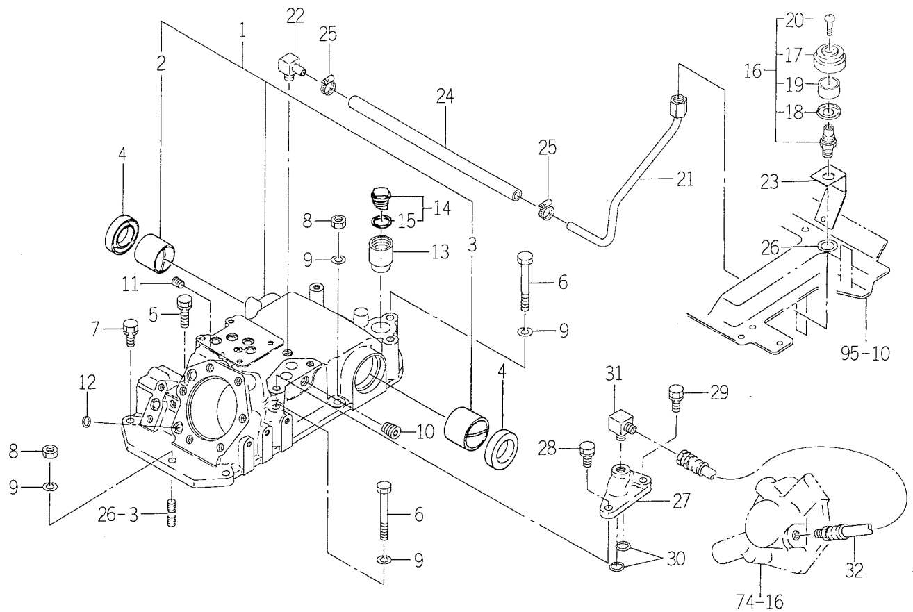
FIG. 72 CYLINDER CASE SYSTEM (TK529)
