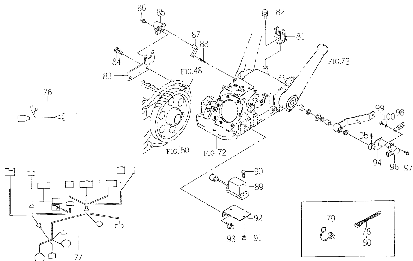
FIG.104 ELC. SYSTEM (4/5)
