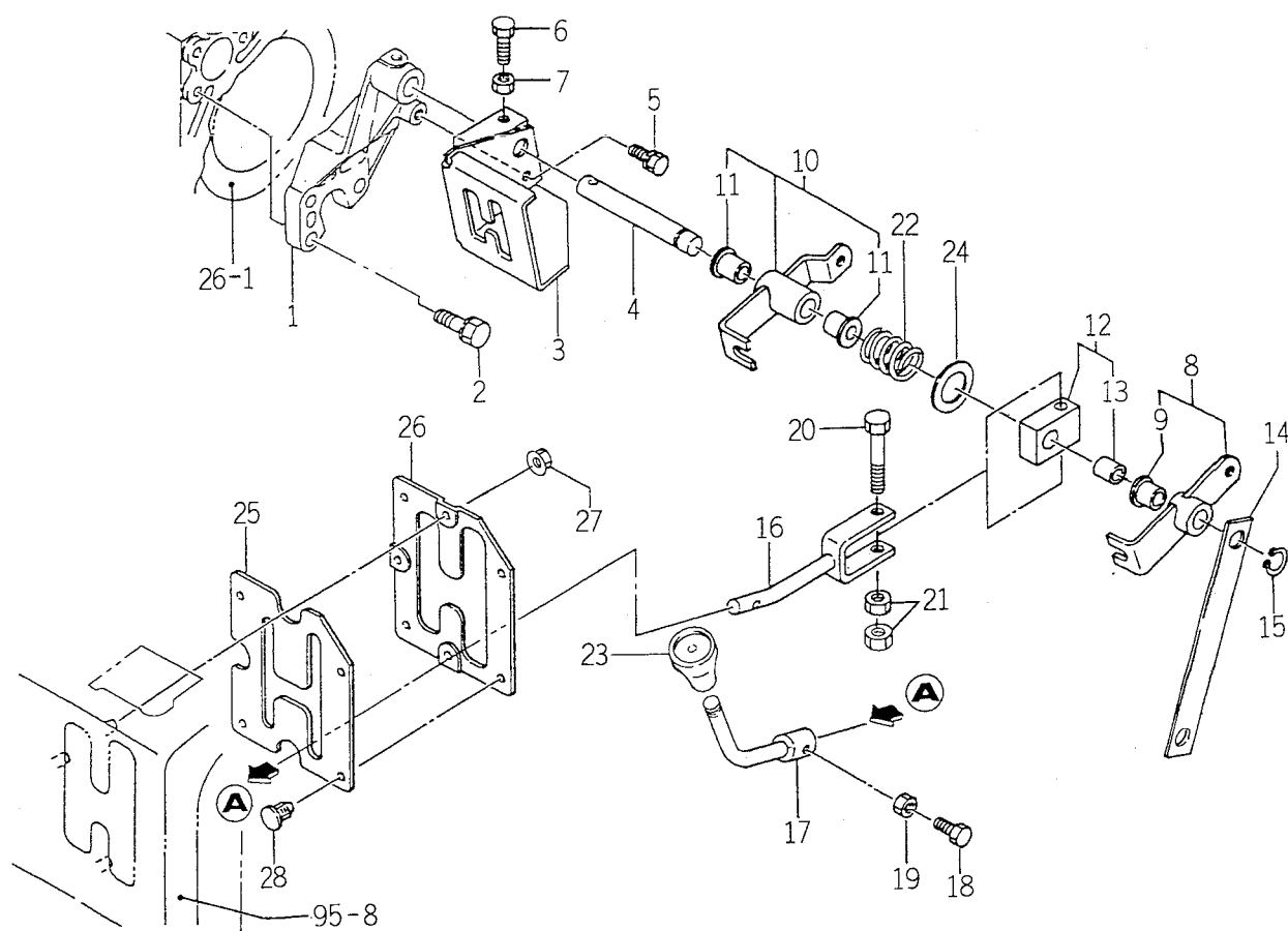
FIG. 41 PTO LEVER SYSTEM (TK533)
