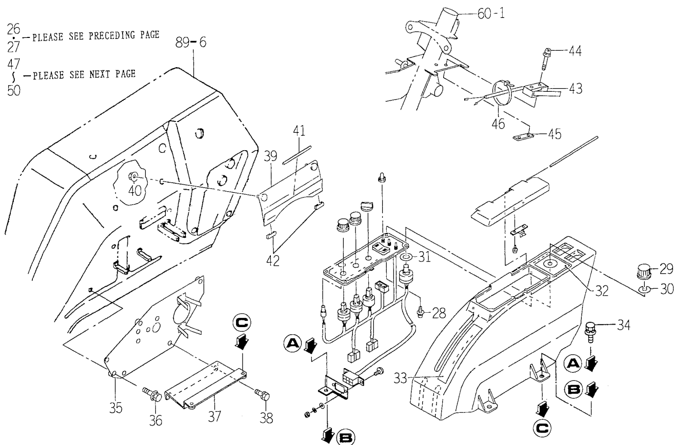
FIG.104 ELC. SYSTEM (2/5)
