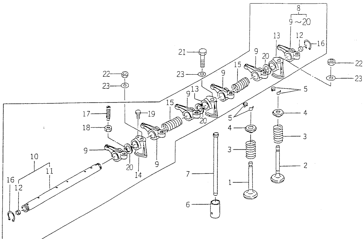
FIG. 11 VALVE
