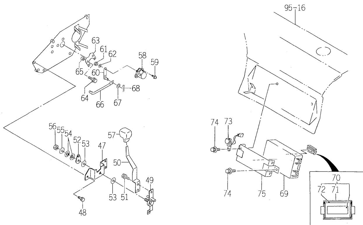
FIG.104 ELC. SYSTEM (3/5)
