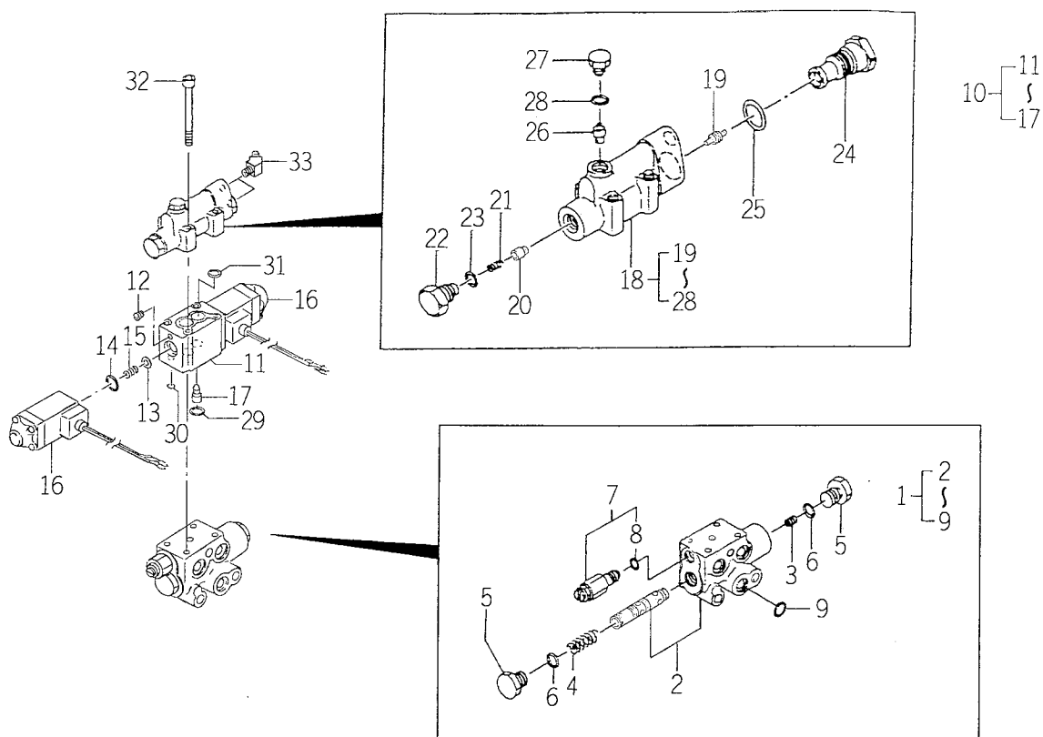
FIG. 117 COMPONENT PARTS FOR K200-019-000-00 ON Fig. 79
