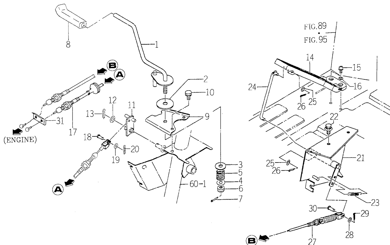
FIG. 7 ACCELERATOR SYSTEM (TK533)
