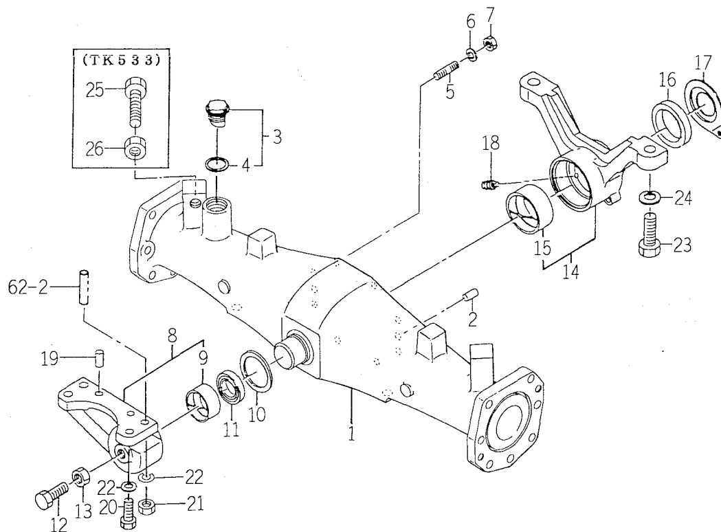
FIG. 66 AXLE HOUSING SYSTEM
