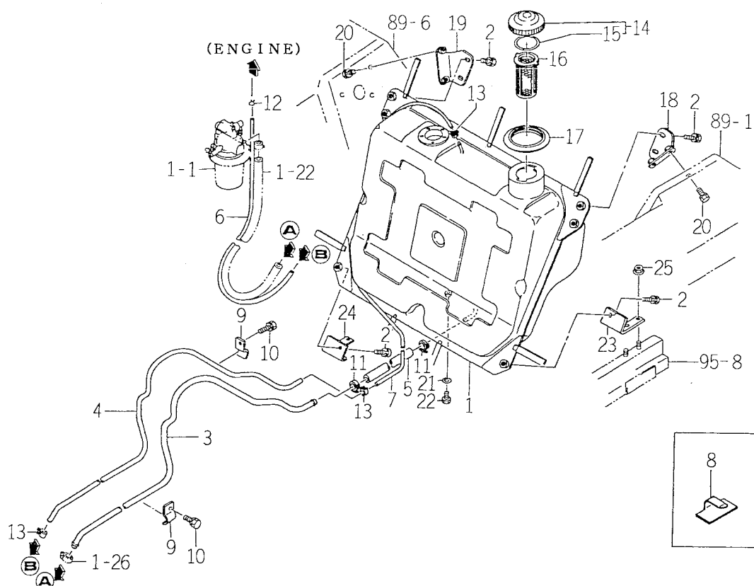
FIG. 5 FUEL TANK SYSTEM
