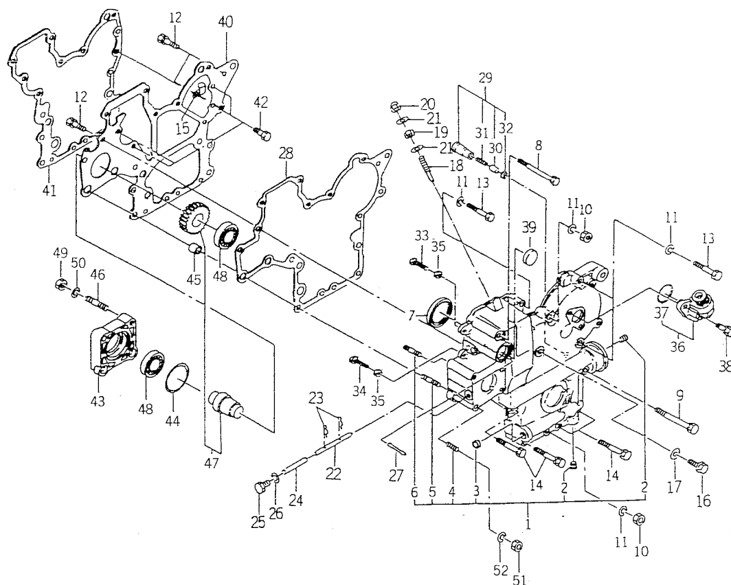
FIG. 9 TIMING GEAR CASE
