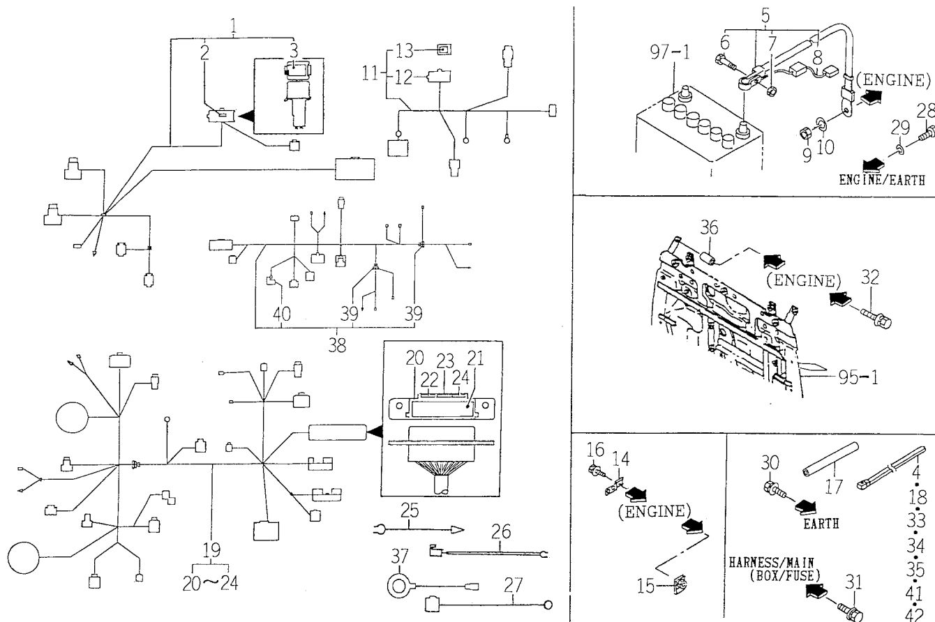
FIG.103 HARNESS SYSTEM
