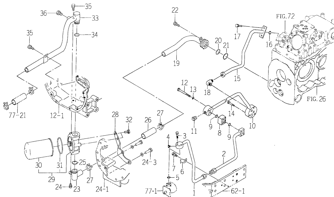
FIG. 75 PIPING SYSTEM (A) (TK529)
