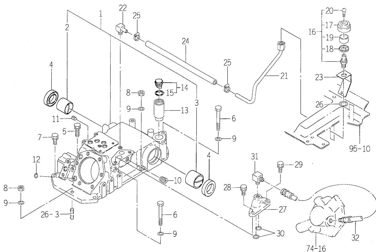
FIG. 71 CYLINDER CASE SYSTEM (TK533)
