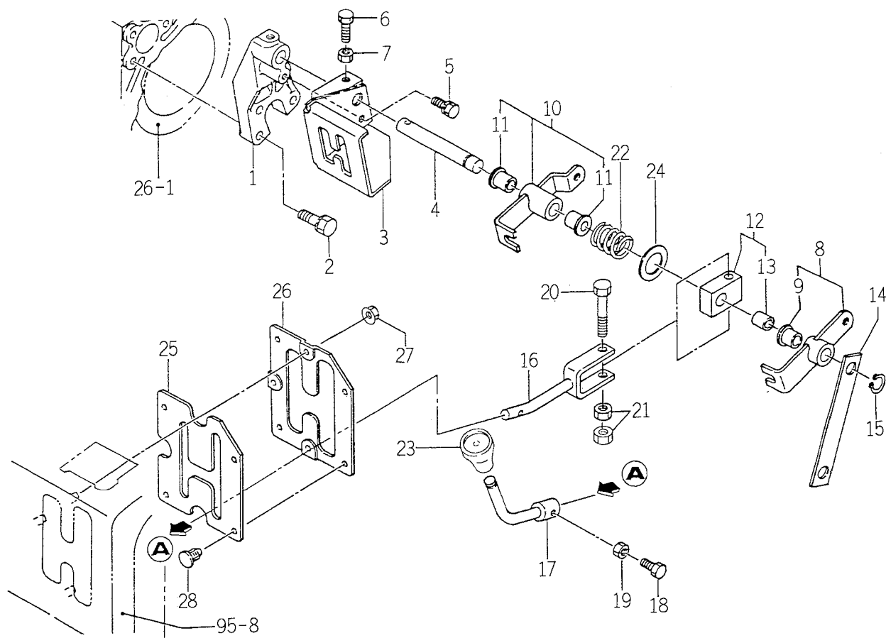
FIG. 40 PTO LEVER SYSTEM (TK529)
