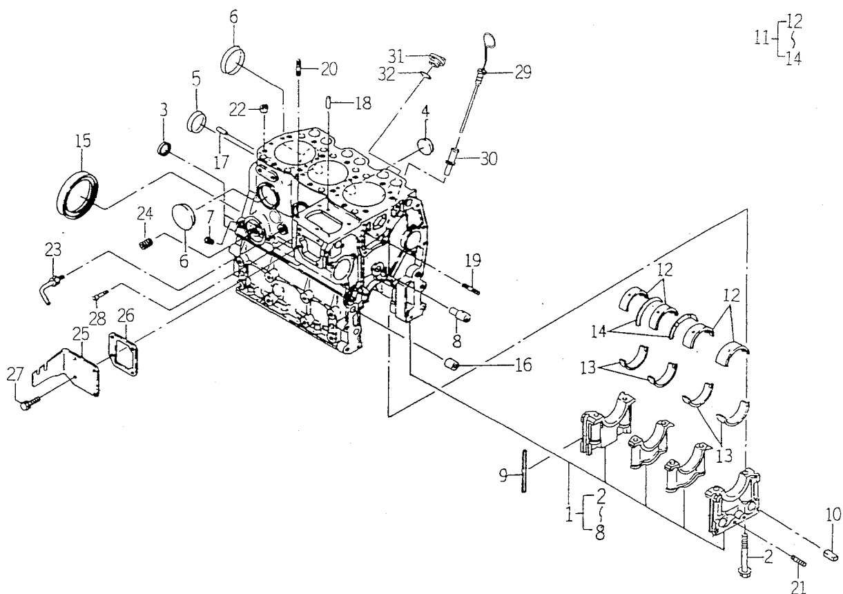
FIG. 5 CYLINDER BLOCK
