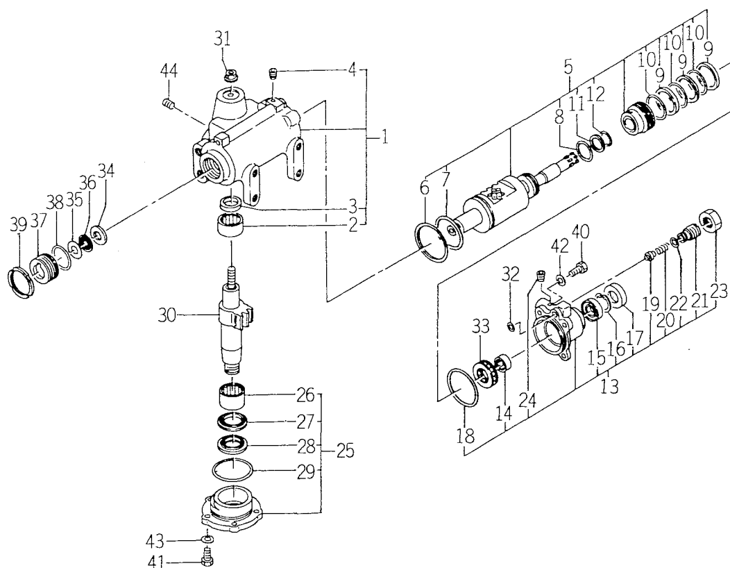
FIG. 118 COMPONENT PARTS FOR 1560-407-260-50 ON Fig. 61
