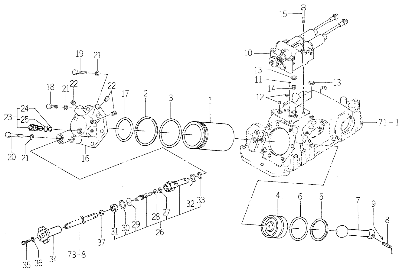
FIG. 74 CYLINDER SYSTEM
