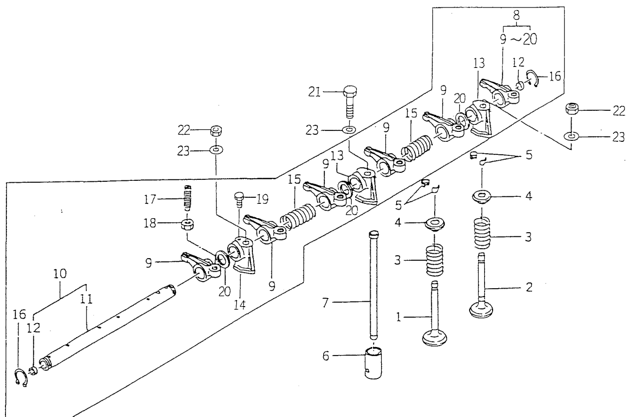
FIG. 11 VALVE
