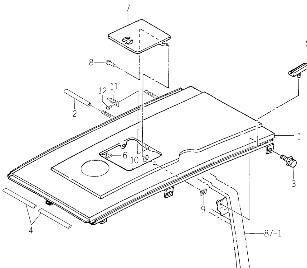
FIG. 86 HOOD SYSTEM
