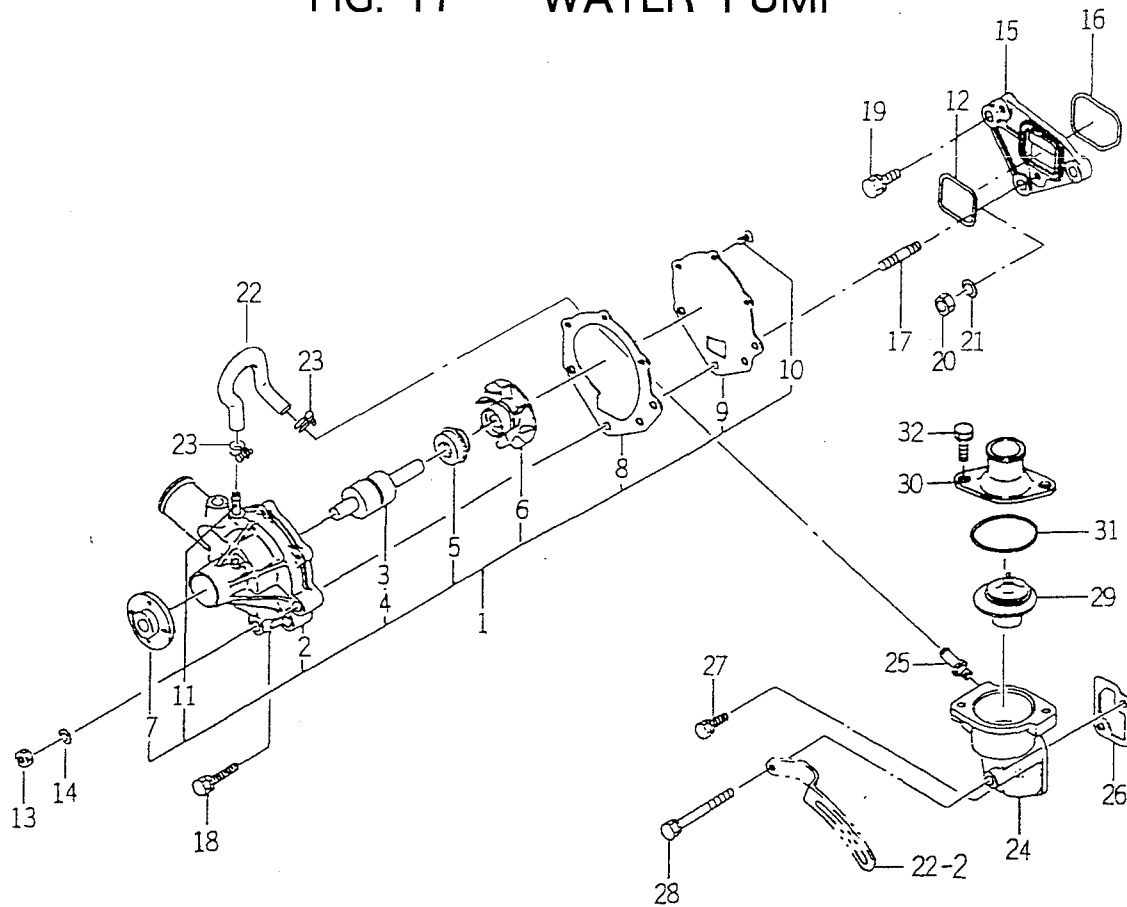
FIG. 17 WATER PUMP
