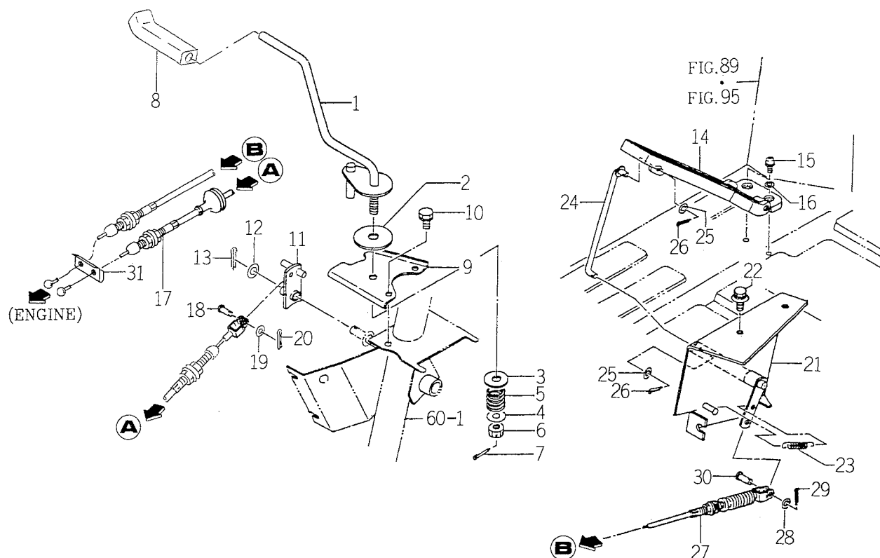
FIG. 7 ACCELERATOR SYSTEM (TK533)
