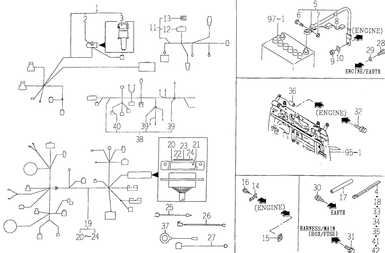
FIG.103 HARNESS SYSTEM
