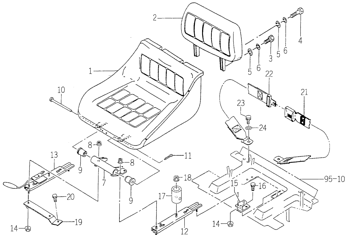
FIG. 91 SEAT SYSTEM
