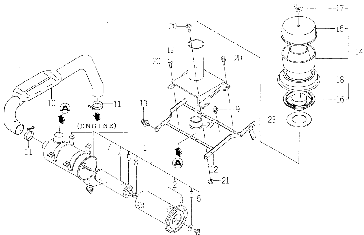
FIG. 2 AIR CLEANER SYSTEM
