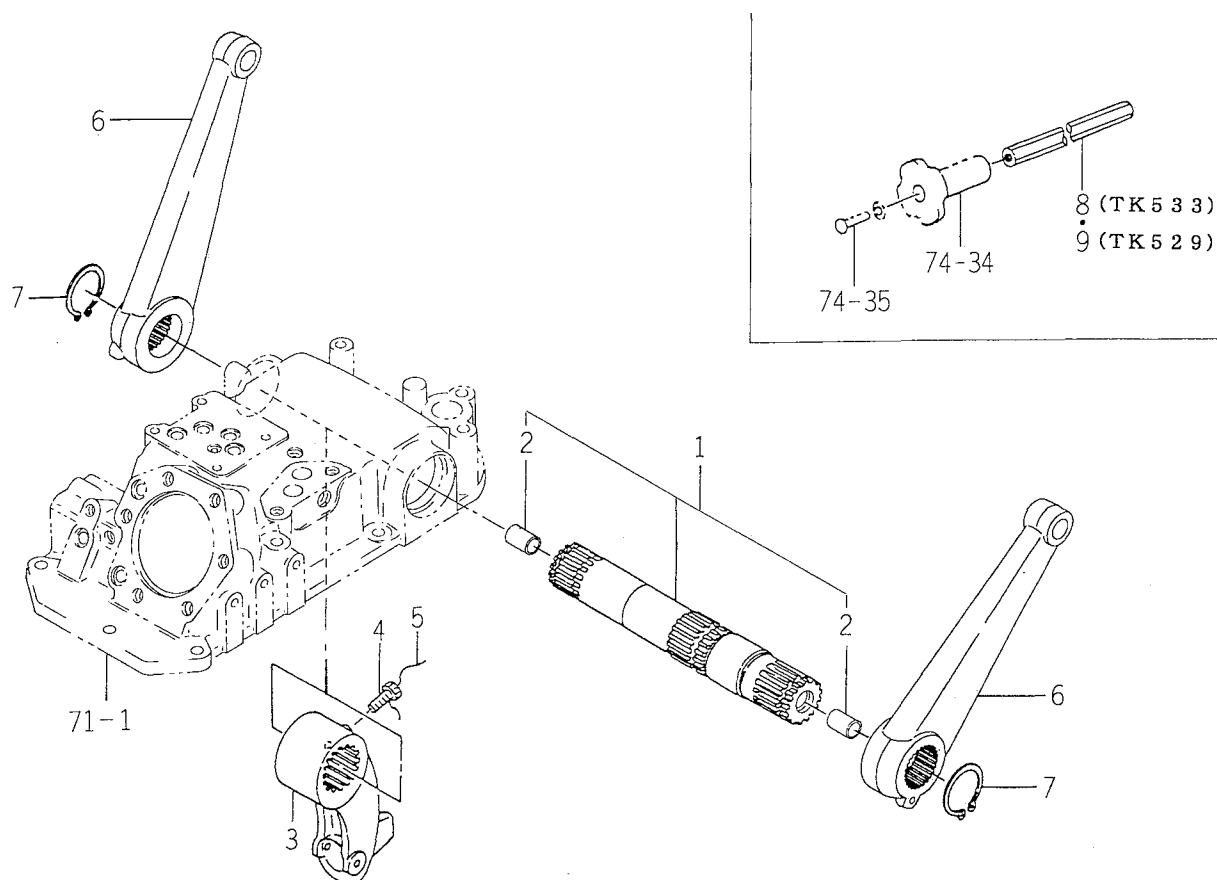
FIG. 73 LIFT ARM SYSTEM
