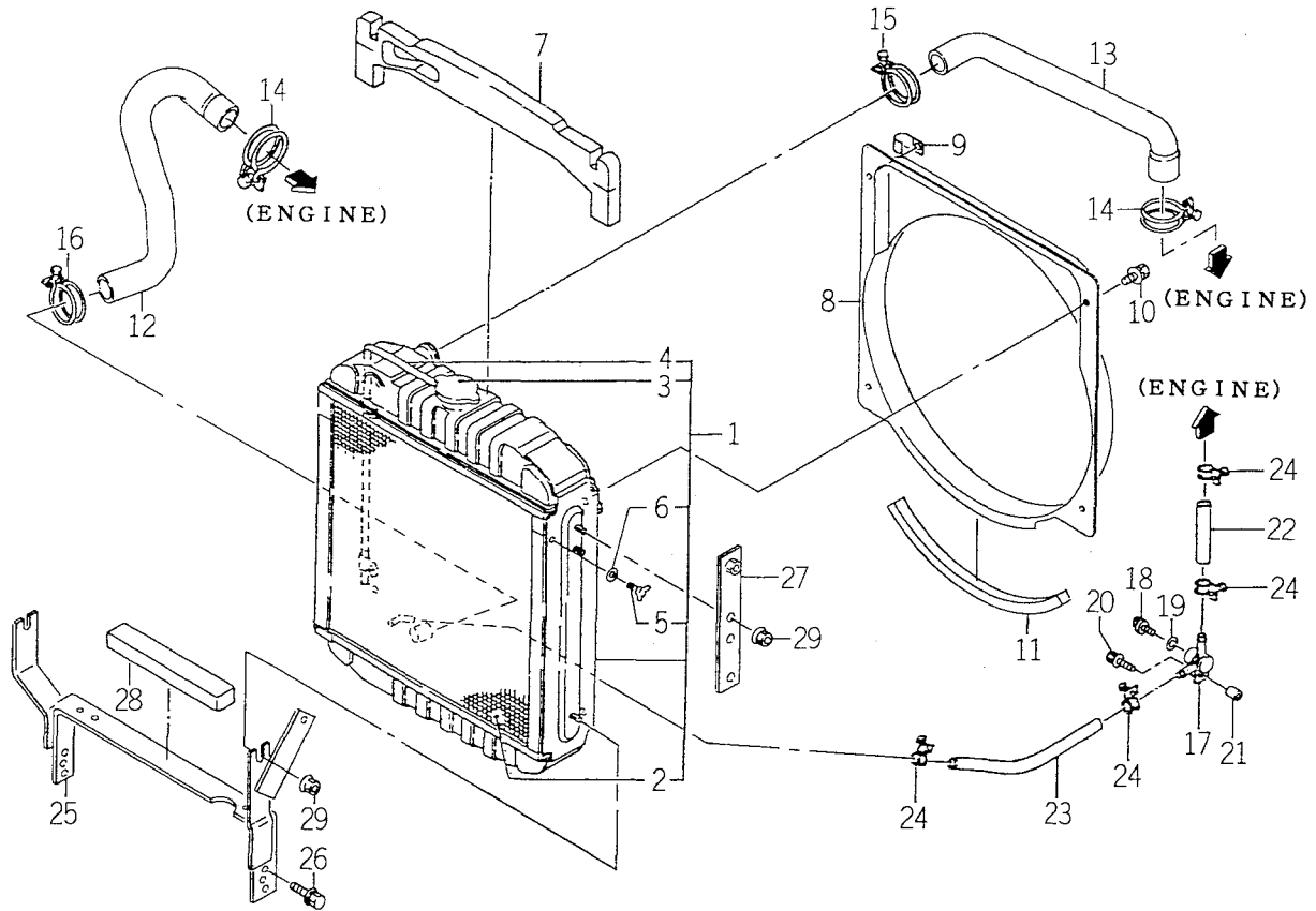
FIG. 3 RADIATOR SYSTEM
