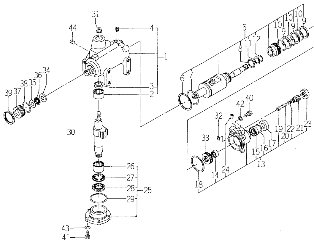
FIG. 118 COMPONENT PARTS FOR 1560-407-260-50 ON Fig. 61
