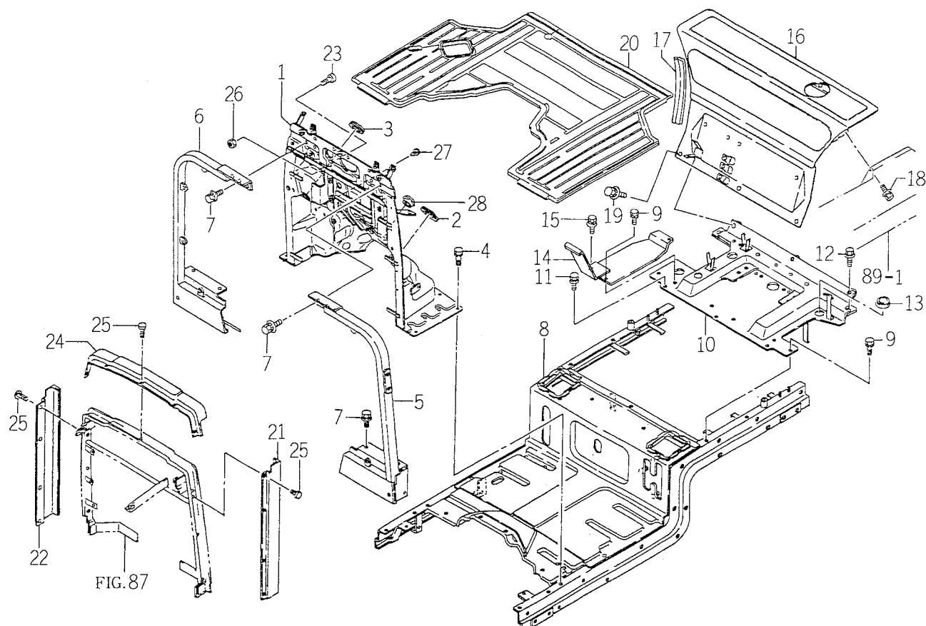
FIG. 95 FLOOR SYSTEM
