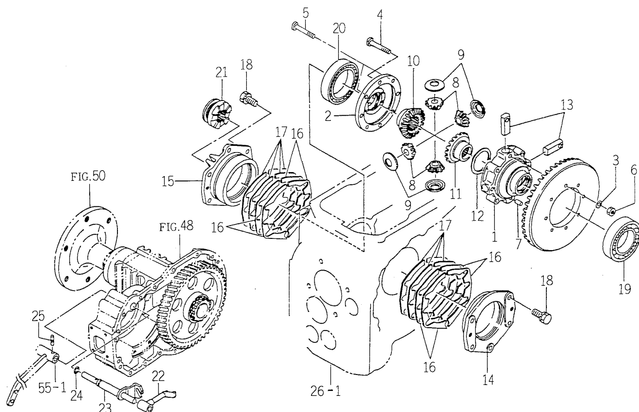
FIG. 47 DIFFERENTIAL GEAR SYSTEM
