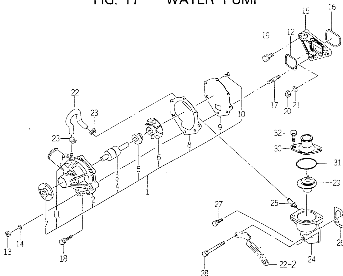
FIG. 17 WATER PUMP
