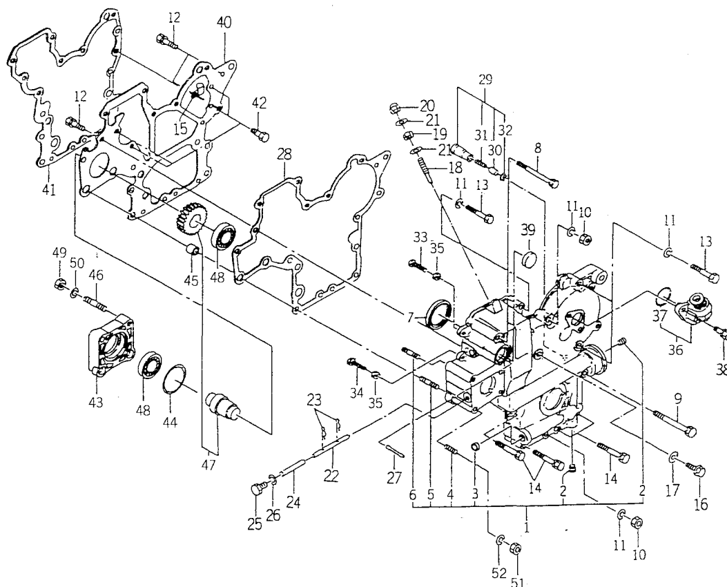
FIG. 9 TIMING GEAR CASE
