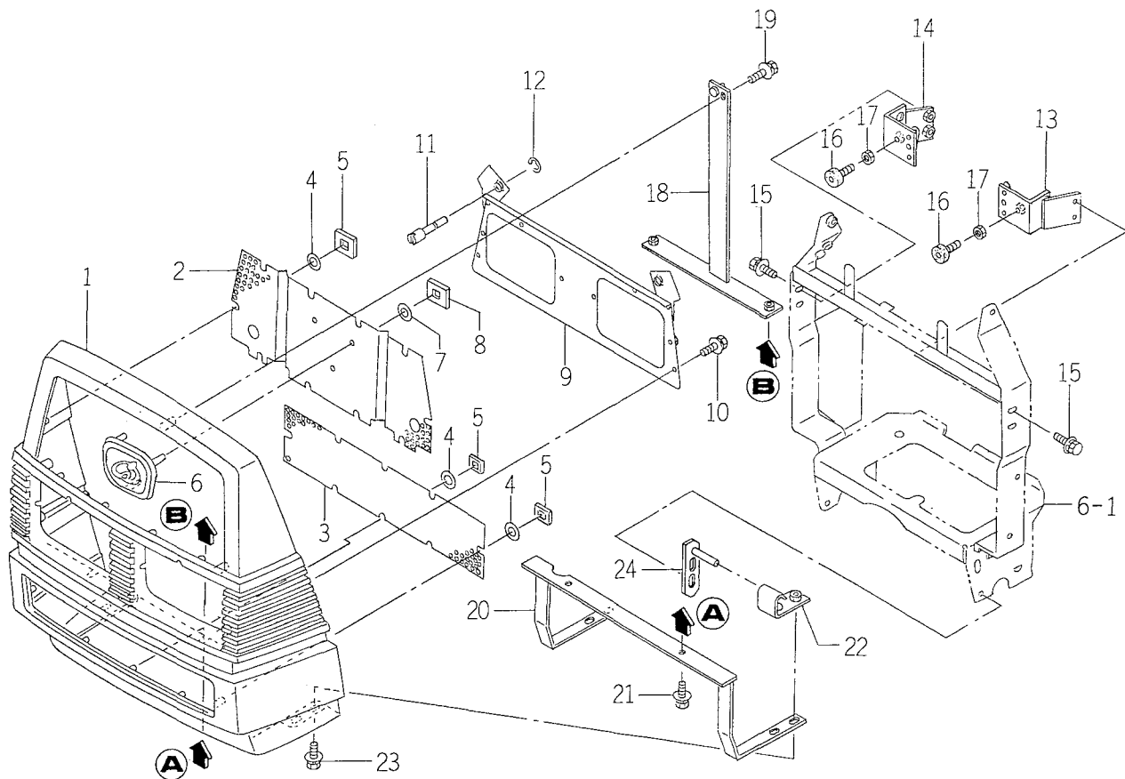
FIG. 85 GRILLE SYSTEM
