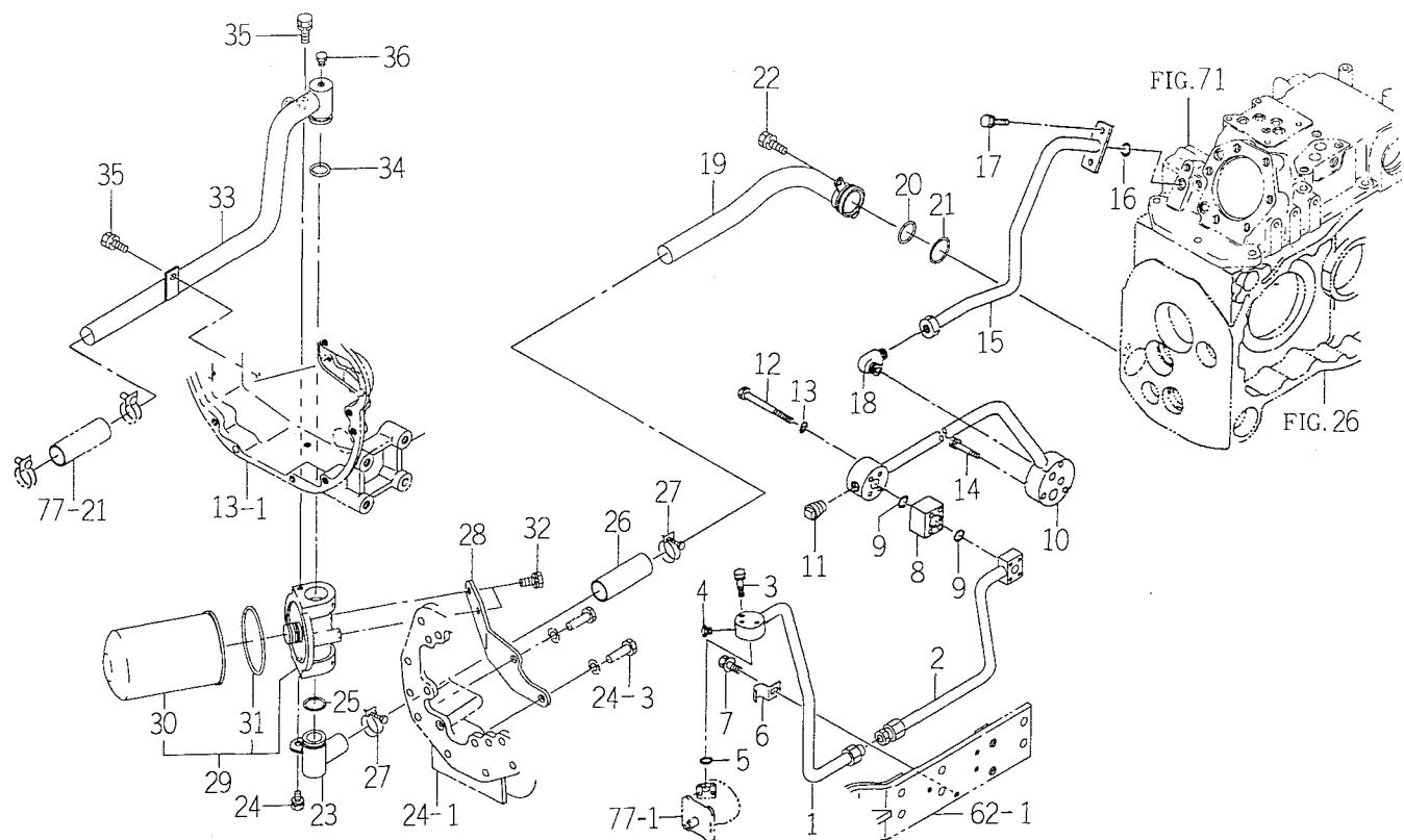
FIG. 76 PIPING SYSTEM (A) (TK533)
