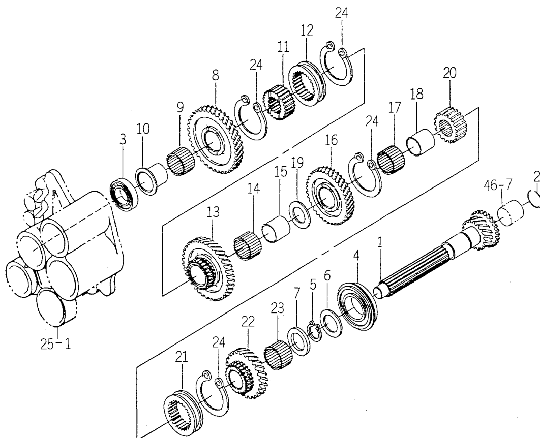
FIG. 15 CHANGE GEAR SYSTEM
