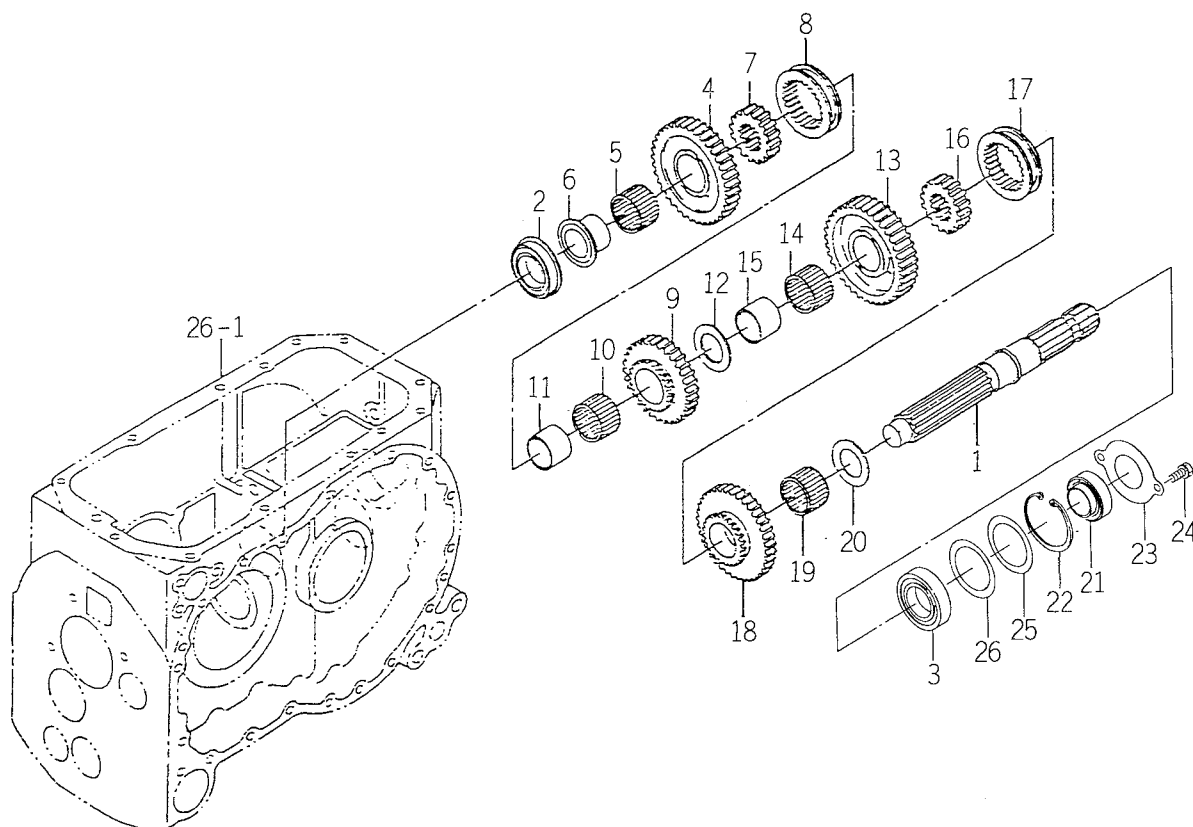
FIG. 33 PTO CHANGE GEAR SYSTEM
