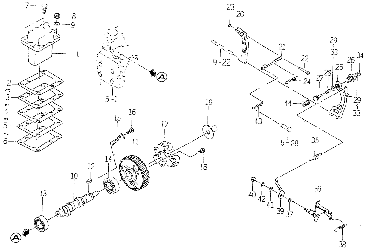
FIG. 20 INJECTION PUMP
