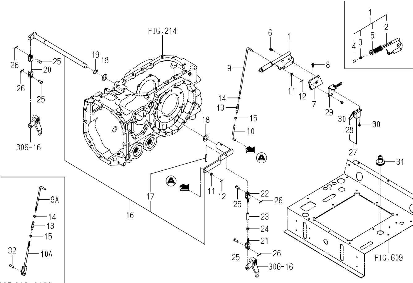
FIG.308 LEVER(BRAKE/PARKING)SYSTEM
