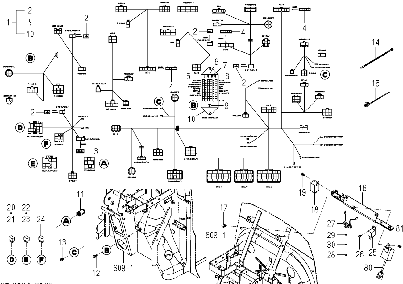
FIG.612 ELC.(MAIN)SYSTEM(1/3)
