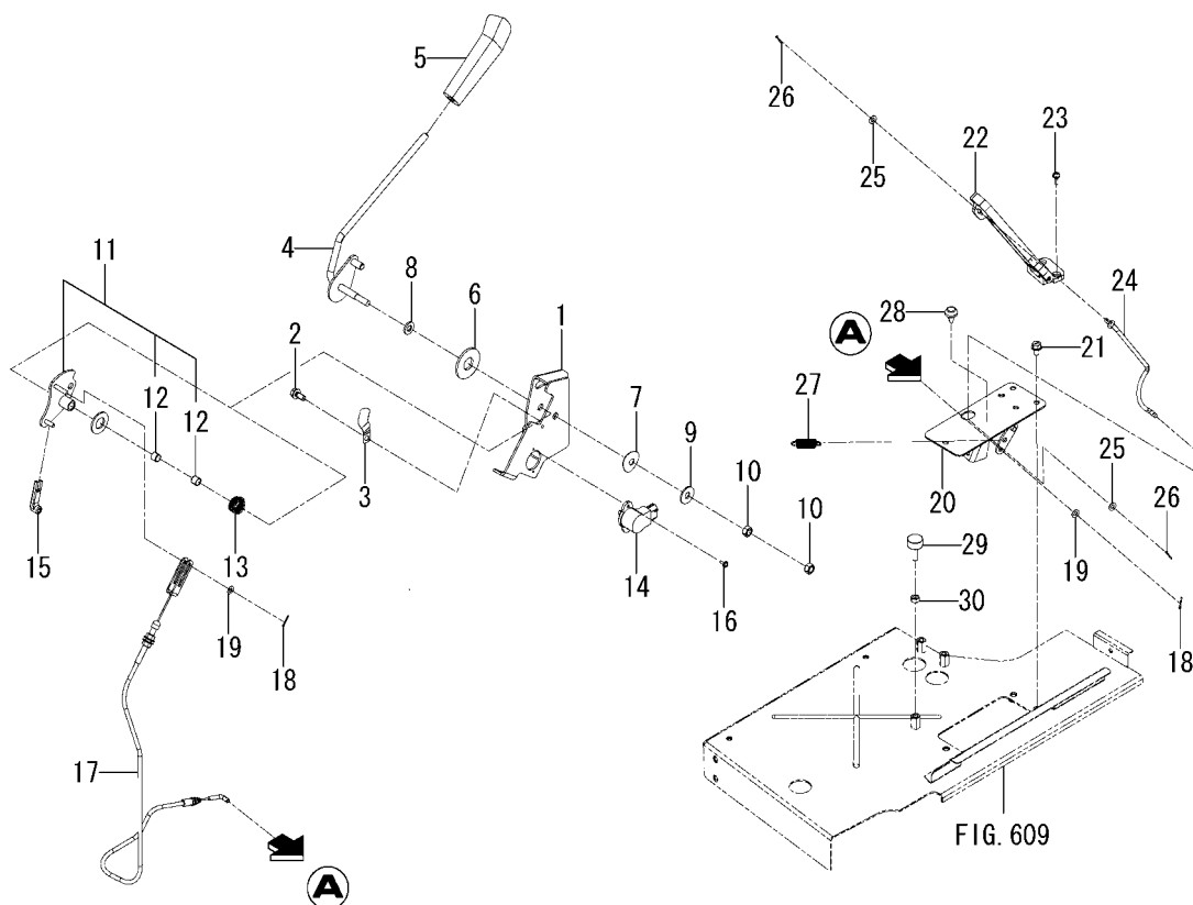
FIG.106 ACCELERATOR SYSTEM
