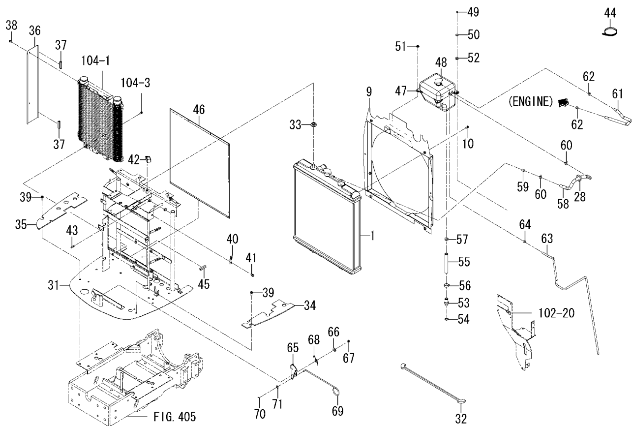
FIG.101 RADIATOR SYSTEM(2/2)
