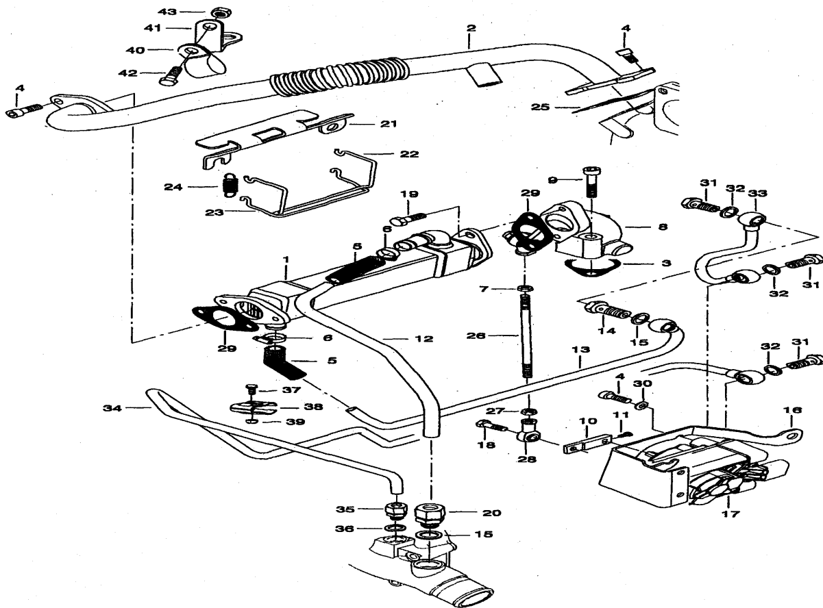
FIG.014 EGR PARTS
