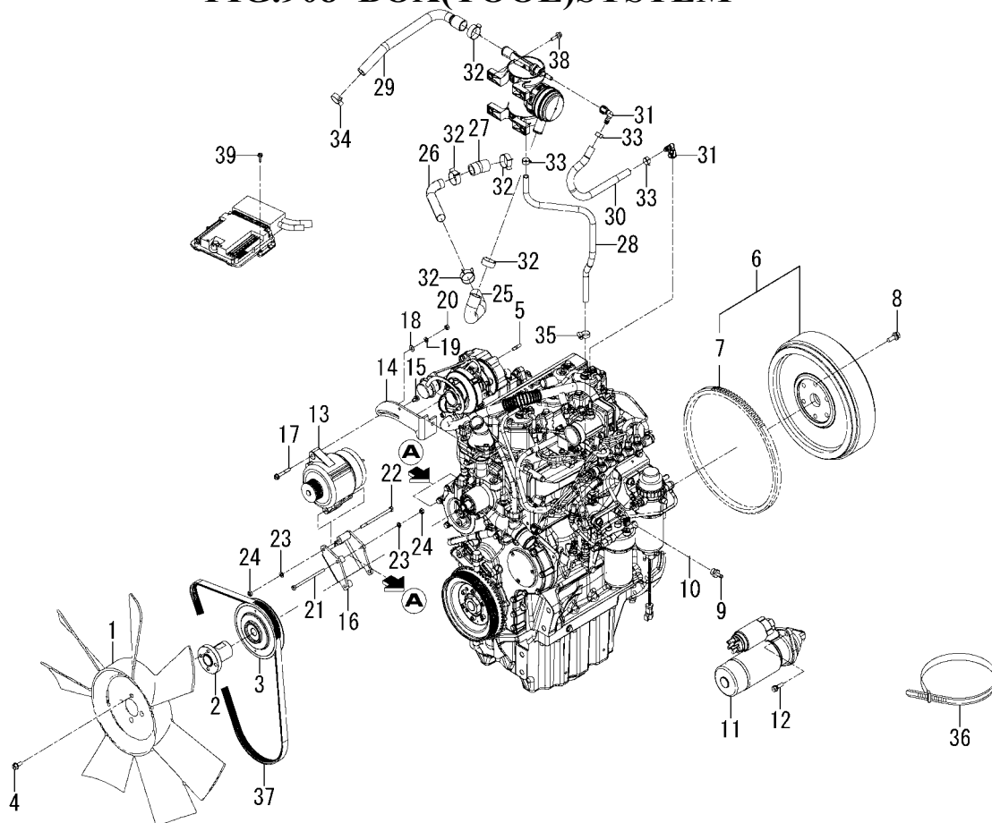
FIG.908 BOX(TOOL)SYSTEM
