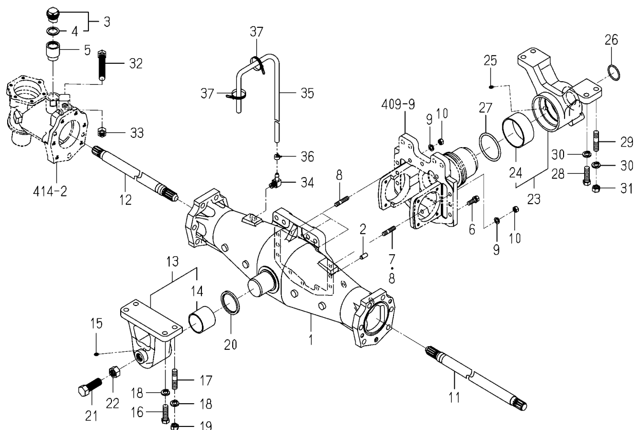
FIG.411 HOUSING(AXLE/FRONT)SYSTEM(8080)
