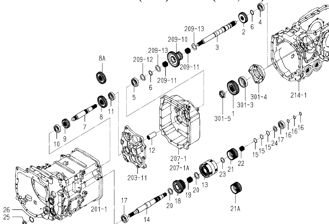
FIG.210 GEAR(4WD)SYSTEM(8090,8100)
