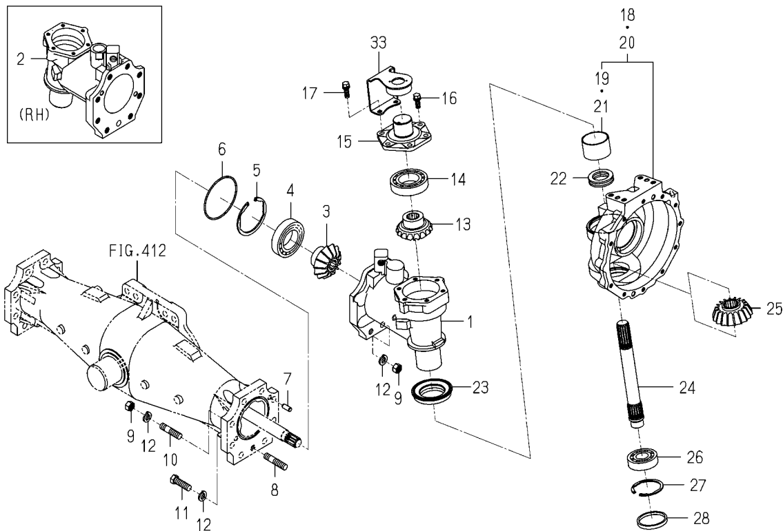
FIG.413 CASE(1/2) (GEAR/FINAL/FRONT)SYSTEM (8090,8100)
