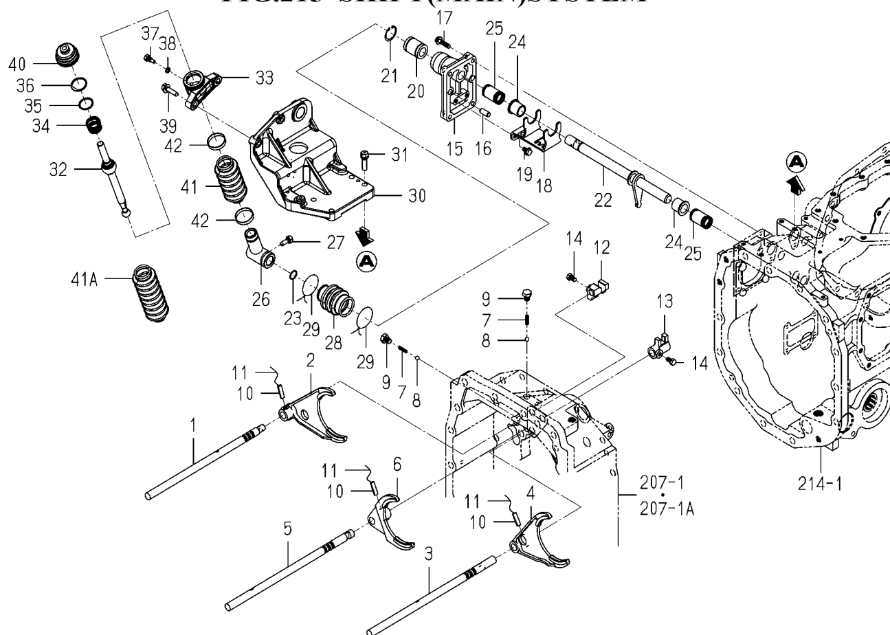
FIG.215 SHIFT(MAIN)SYSTEM
