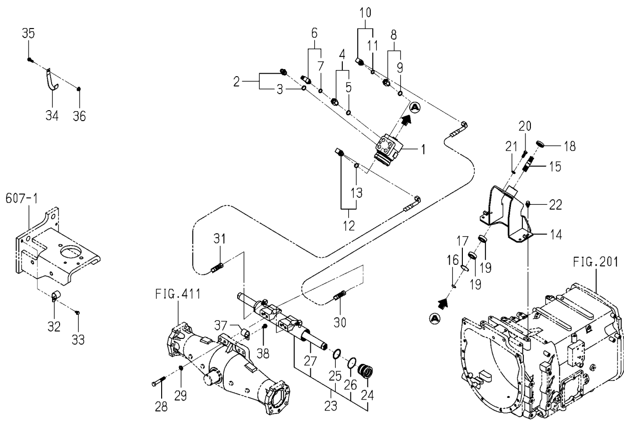
FIG.403 CONTROLLER(STEERING)SYSTEM(8080)
