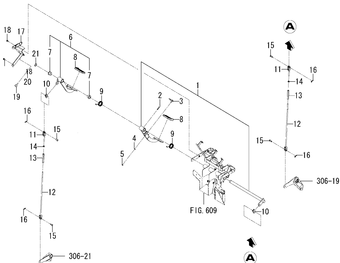
FIG.307 PEDAL(BRAKE)SYSTEM
