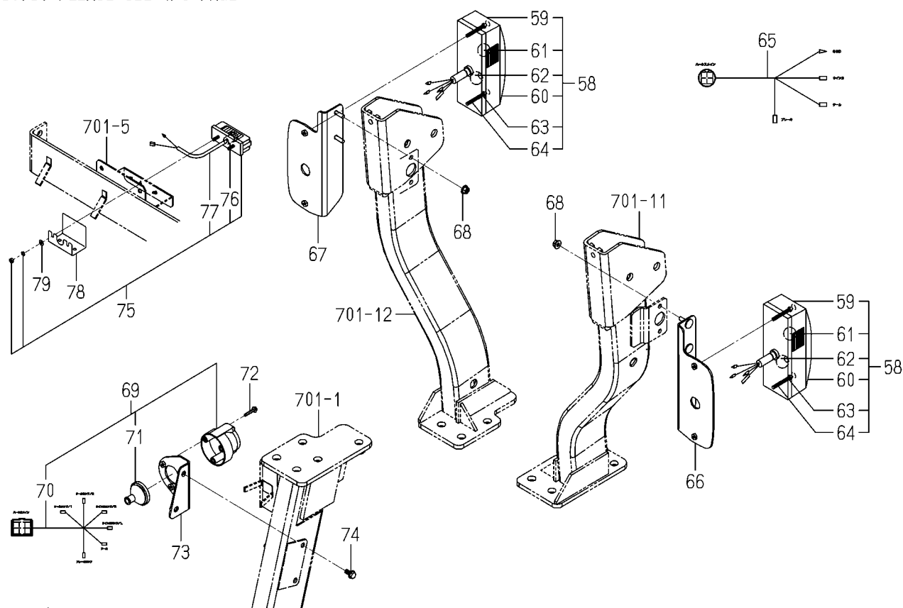
FIG.612 ELC.(MAIN)SYSTEM(3/3)
