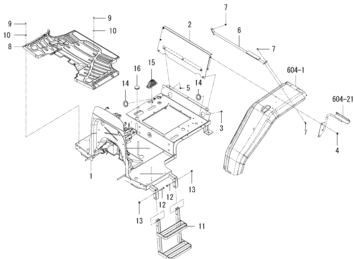
FIG.609 FLOOR(REAR)SYSTEM
