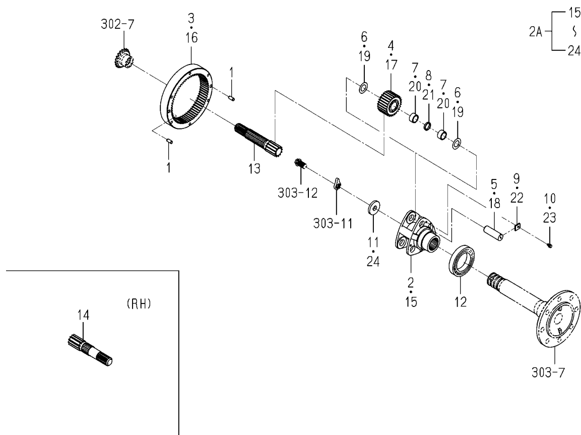
FIG.304 GEAR(FINAL/REAR)SYSTEM
