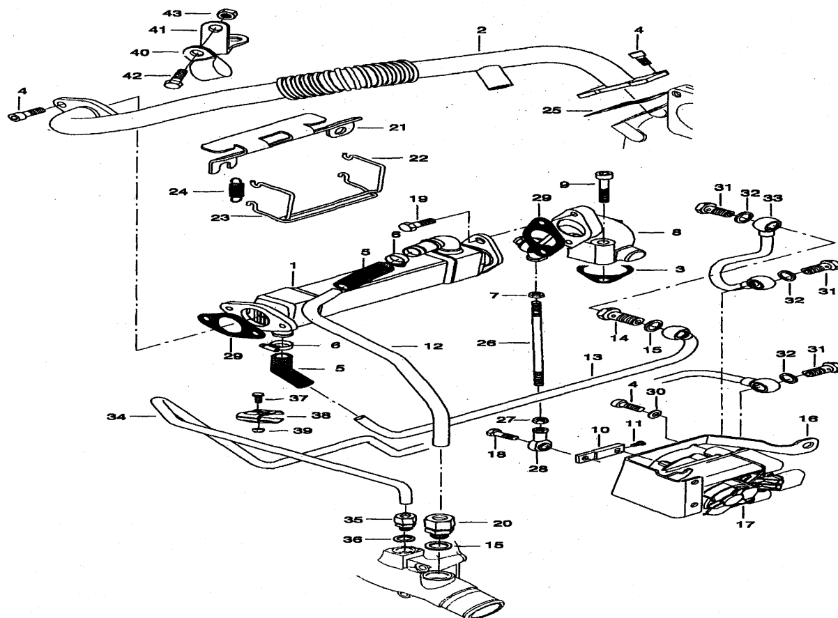
FIG.014 EGR PARTS
