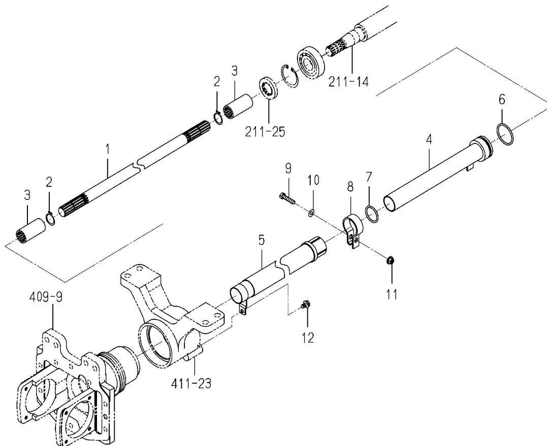
FIG.407 SHAFT(DRIVE/FRONT)SYSTEM(8080)
