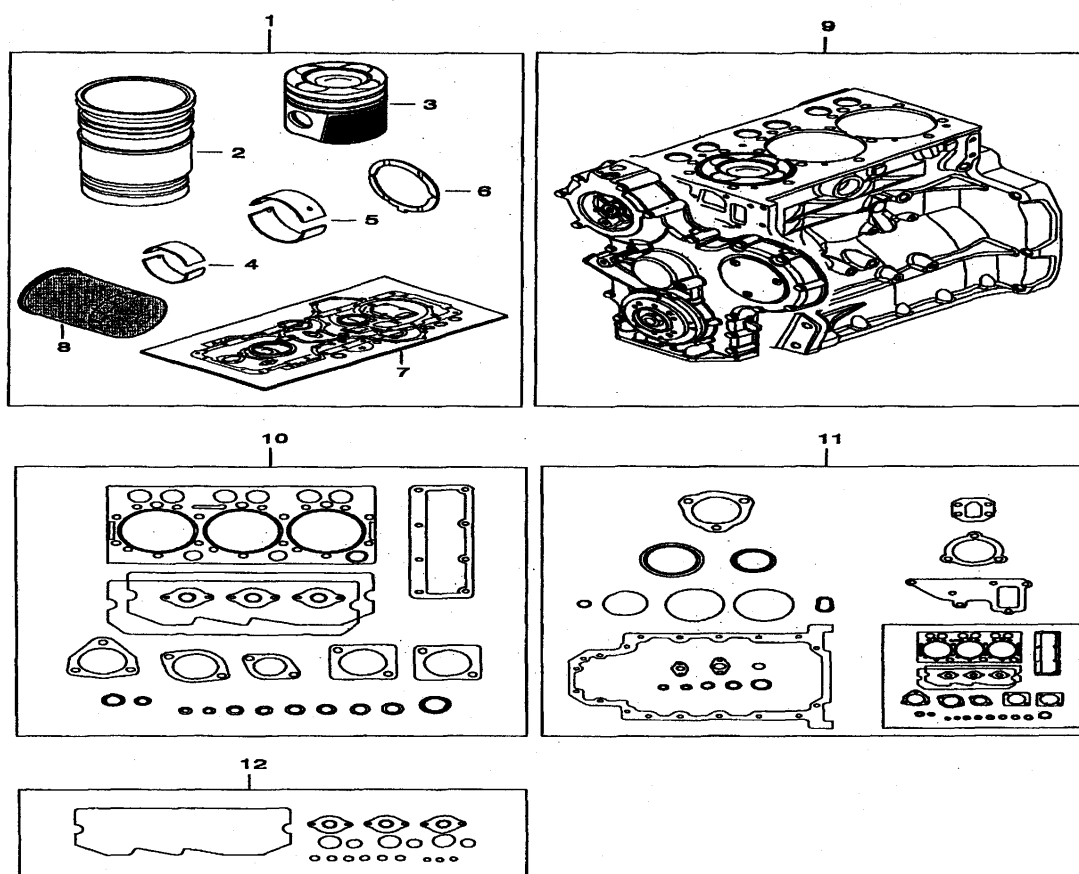
FIG.016 ENGINE OVERHAUL PARTS
