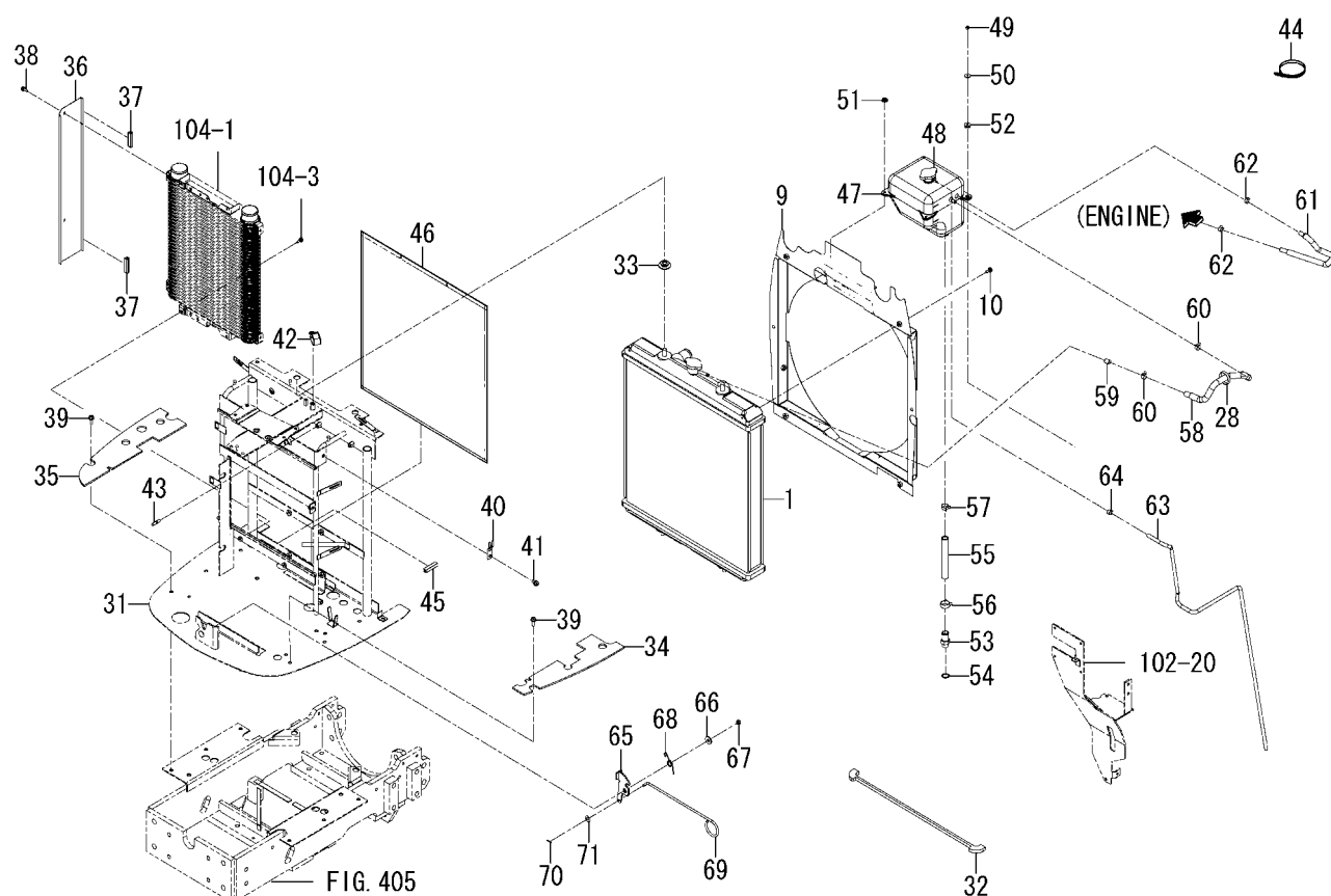
FIG.101 RADIATOR SYSTEM(2/2)
