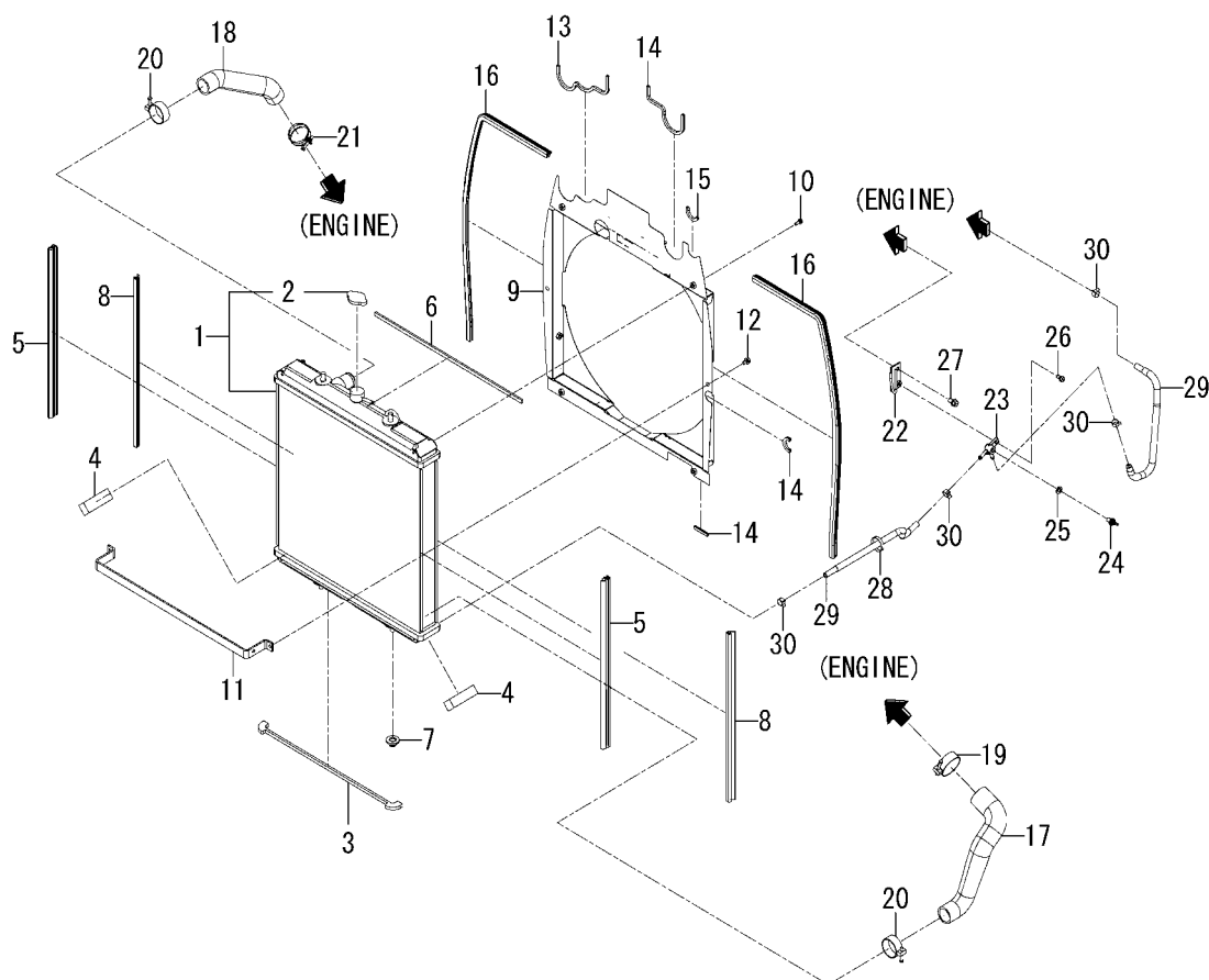
FIG.101 RADIATOR SYSTEM(1/2)
