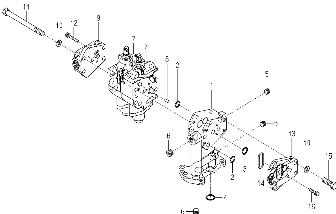
FIG.S04 COMPONENT PARTS FOR K211-099-000-10 ON Fig.505
