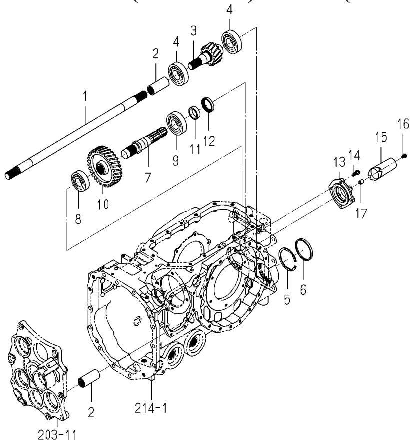
FIG.213 GEAR(PTO/REAR)SYSTEM(D TYPE)
