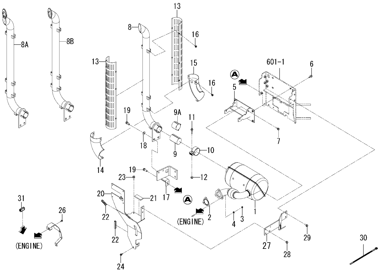
FIG.102 MUFFLER SYSTEM
