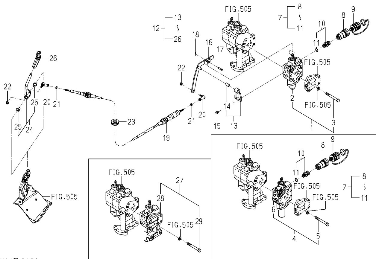
FIG.P05 VALVE(STD ETC), COUPLER&LEVER SYSTEM(OPTION)
