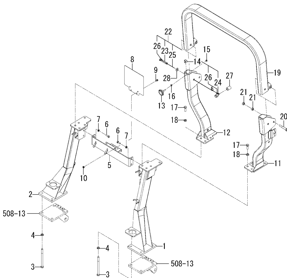
FIG.701 ROPS SYSTEM
