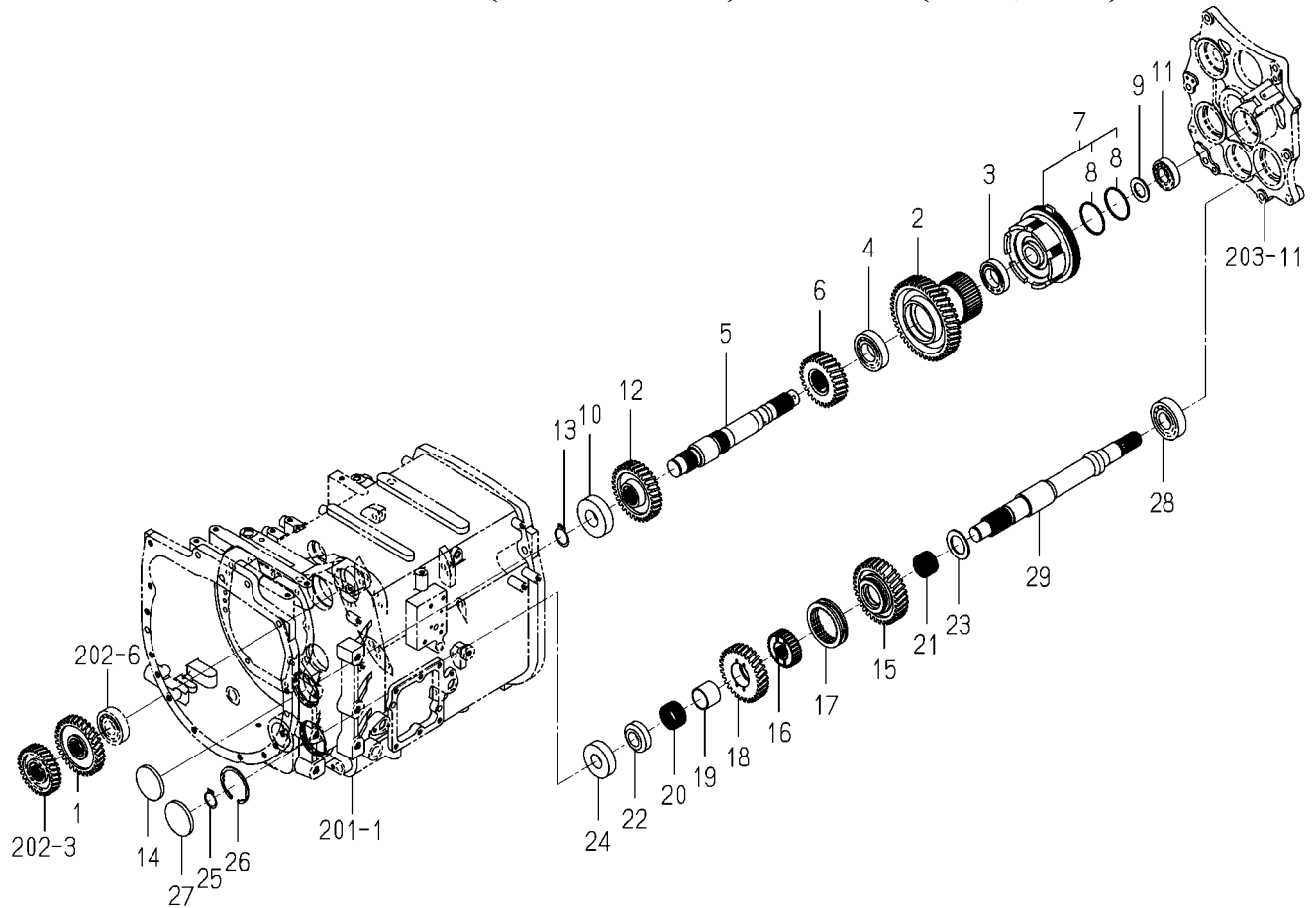
FIG.205 GEAR(PTO/INPUT)SYSTEM(8090,8100)
