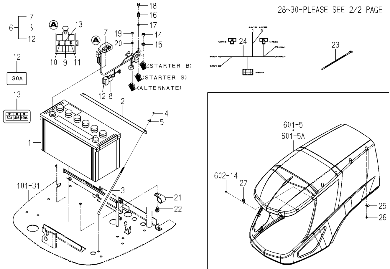
FIG.610 ELC.(FRONT)SYSTEM(1/2)
