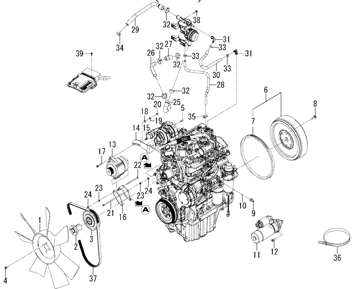
FIG.908 BOX(TOOL)SYSTEM
