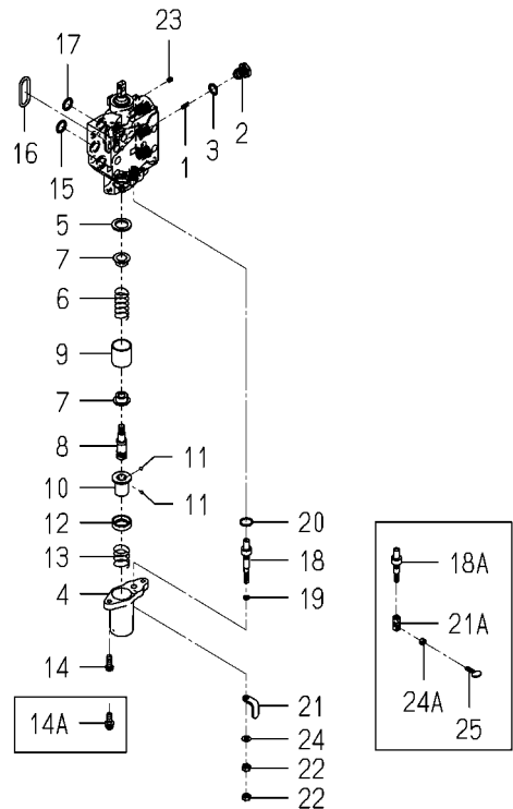
FIG.S03 COMPONENT PARTS FOR K211-075-500-60 ON Fig.P05
