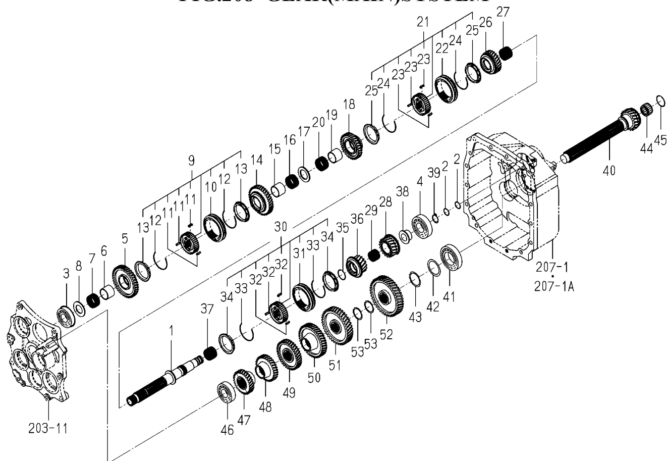
FIG.208 GEAR(MAIN)SYSTEM
