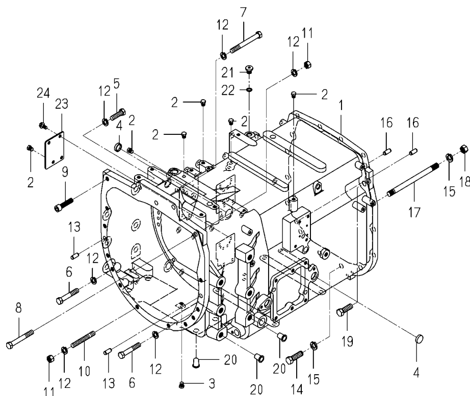
FIG.201 CASE(TRANSMISSION/FRONT)SYSTEM
