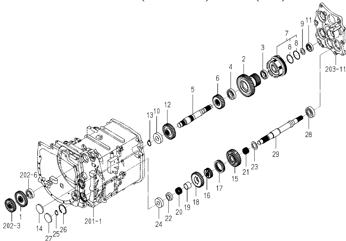
FIG.206 GEAR(PTO/INPUT)SYSTEM(8080)
