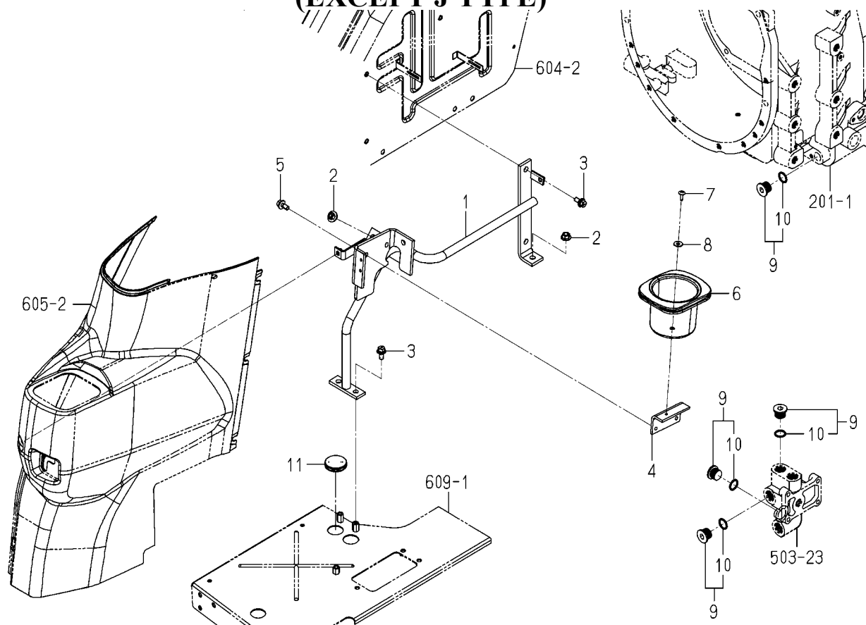
FIG.506 FRAME(GUIDE/LEVER)SYSTEM (EXCEPT J TYPE)
