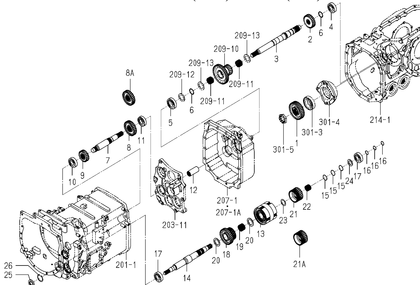
FIG.211 GEAR(4WD)SYSTEM(8080)
