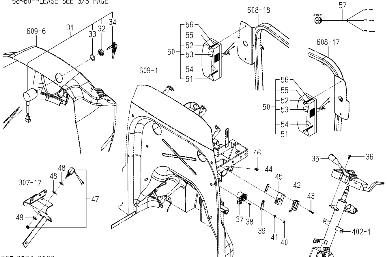
FIG.612 ELC.(MAIN)SYSTEM(2/3)
