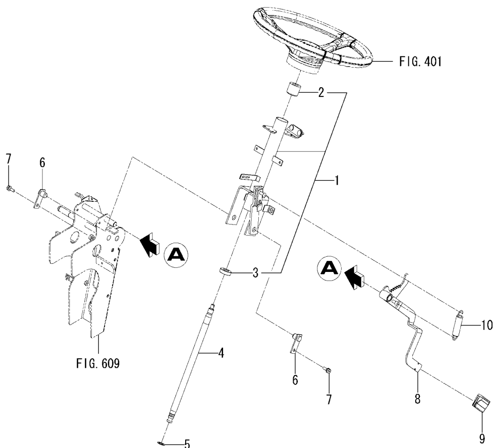
FIG.402 COLUMN(STEERING)SYSTEM
