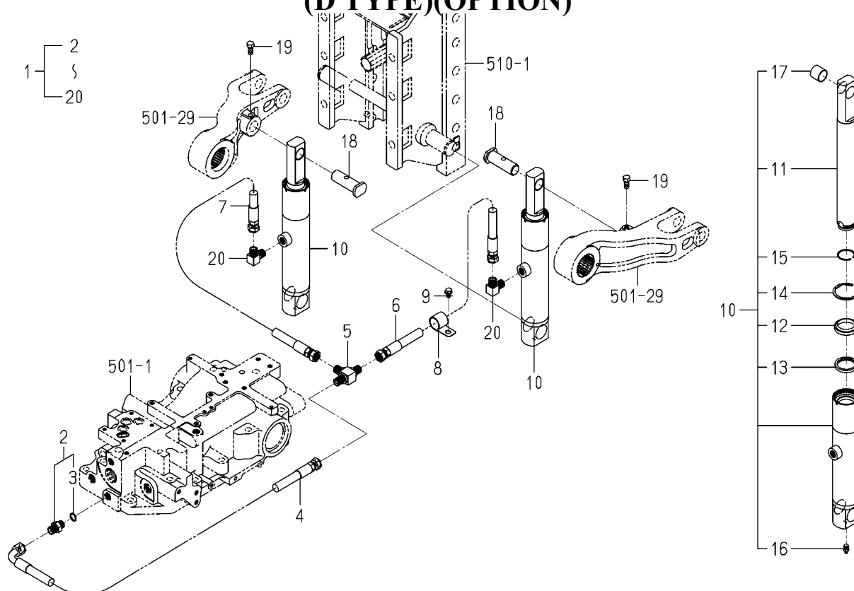
FIG.P04 CYLINDER(ASSIST/E4D)ASSY (D TYPE)(OPTION)
