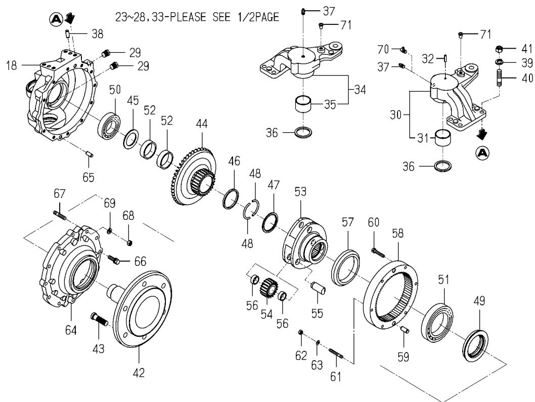
FIG.413 CASE(2/2) (GEAR/FINAL/FRONT)SYSTEM (8090,8100)
