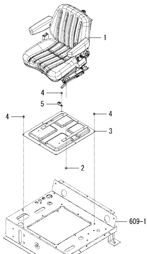
FIG.606 SEAT SYSTEM
