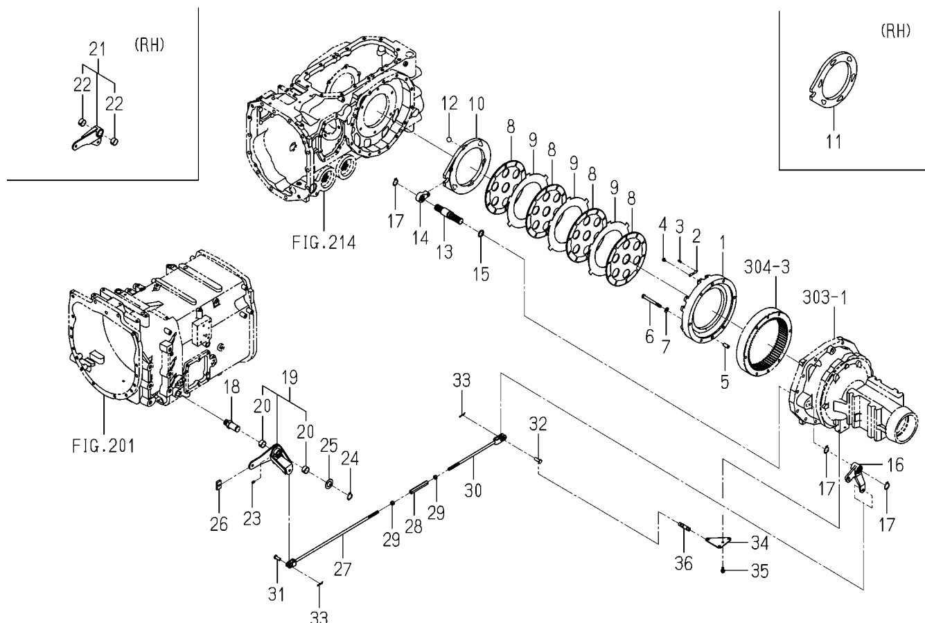
FIG.306 BRAKE SYSTEM
