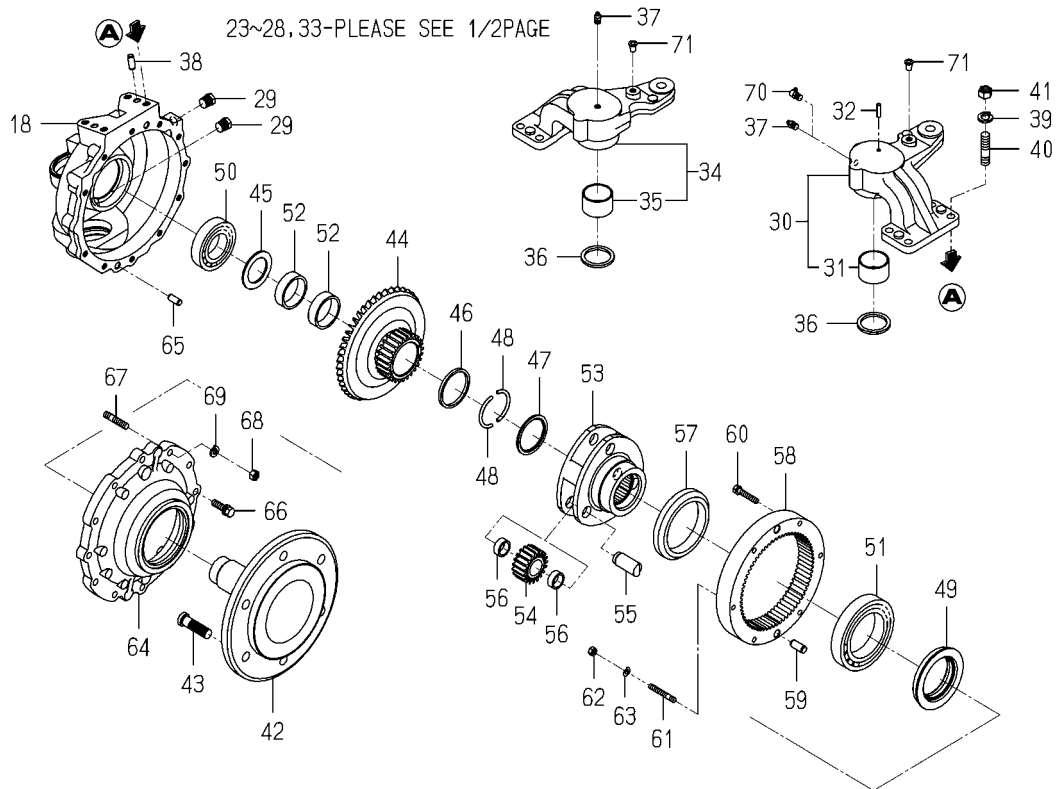
FIG.413 CASE(2/2) (GEAR/FINAL/FRONT)SYSTEM (8090,8100)
