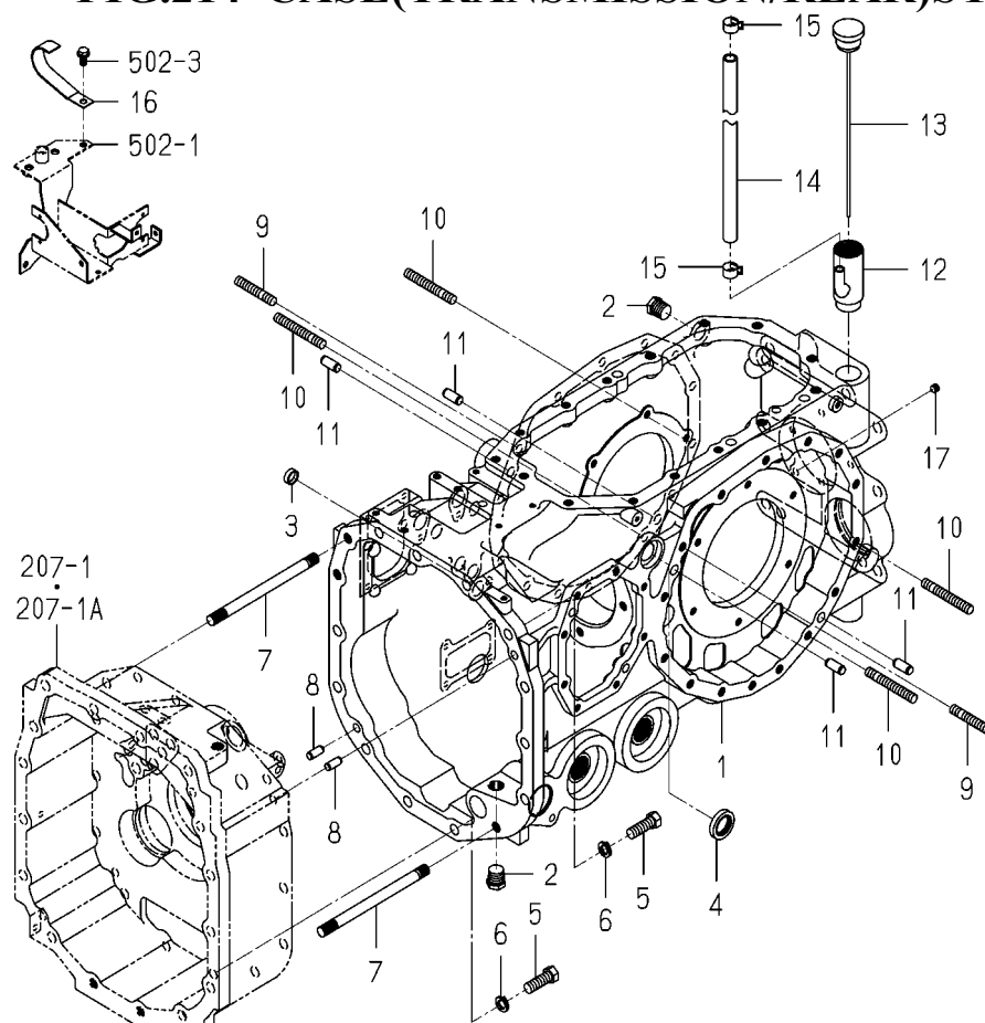
FIG.214 CASE(TRANSMISSION/REAR)SYSTEM
