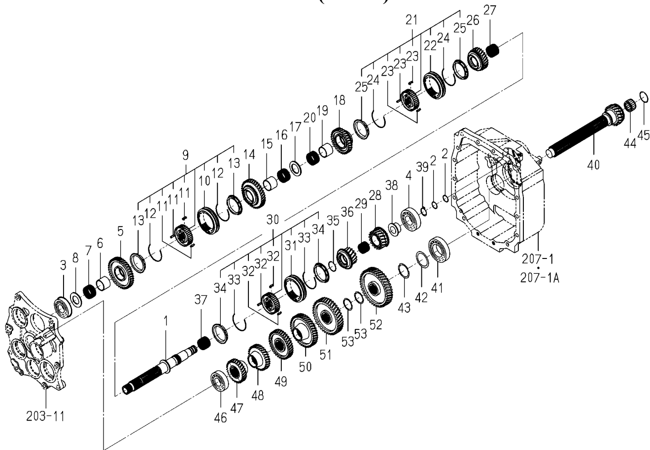
FIG.208 GEAR(MAIN)SYSTEM
