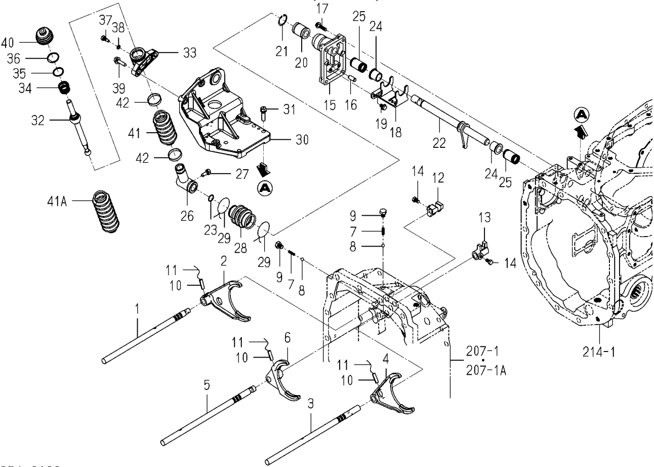
FIG.215 SHIFT(MAIN)SYSTEM
