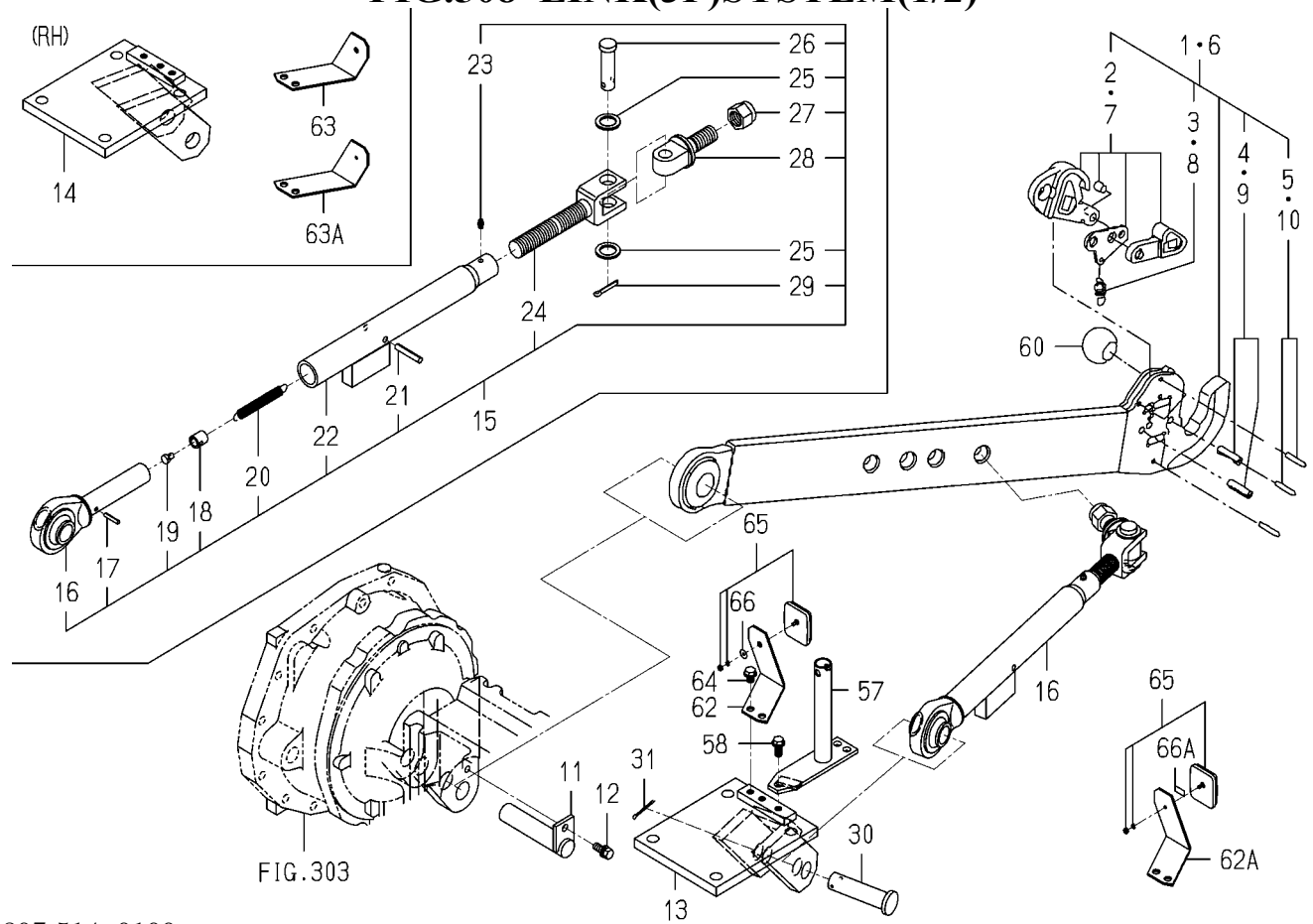
FIG.508 LINK(3P)SYSTEM(1/2)
