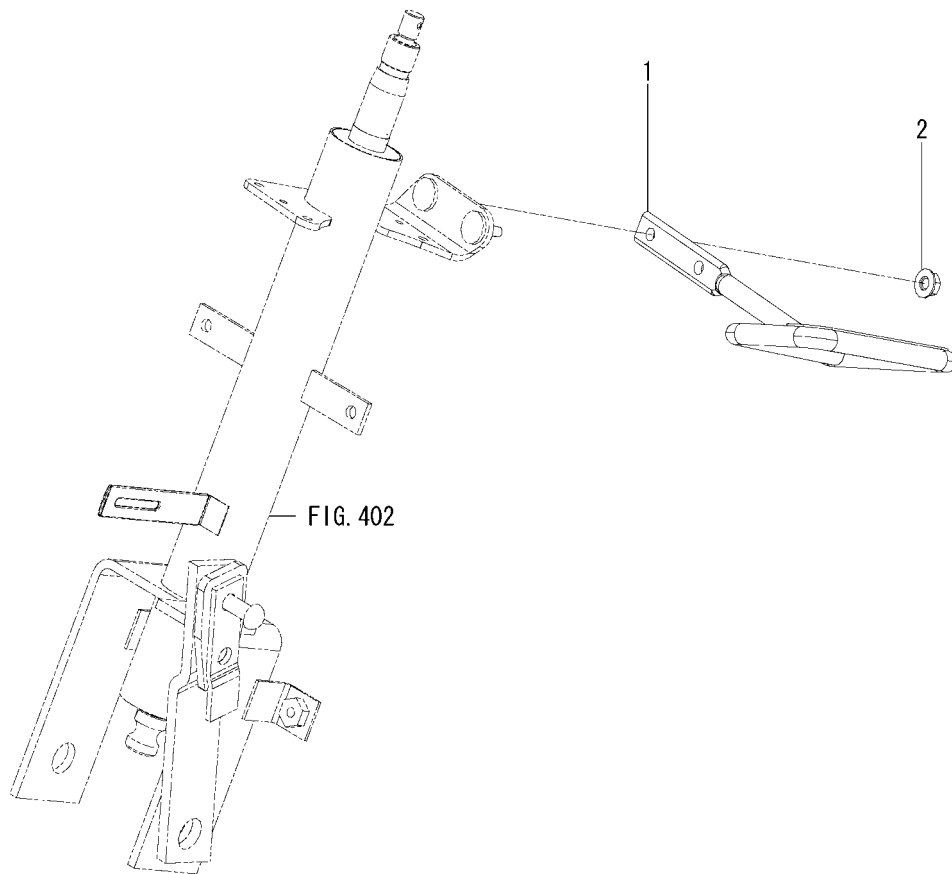
FIG.218 GUIDE(LEVER/REVERSE)SYSTEM
