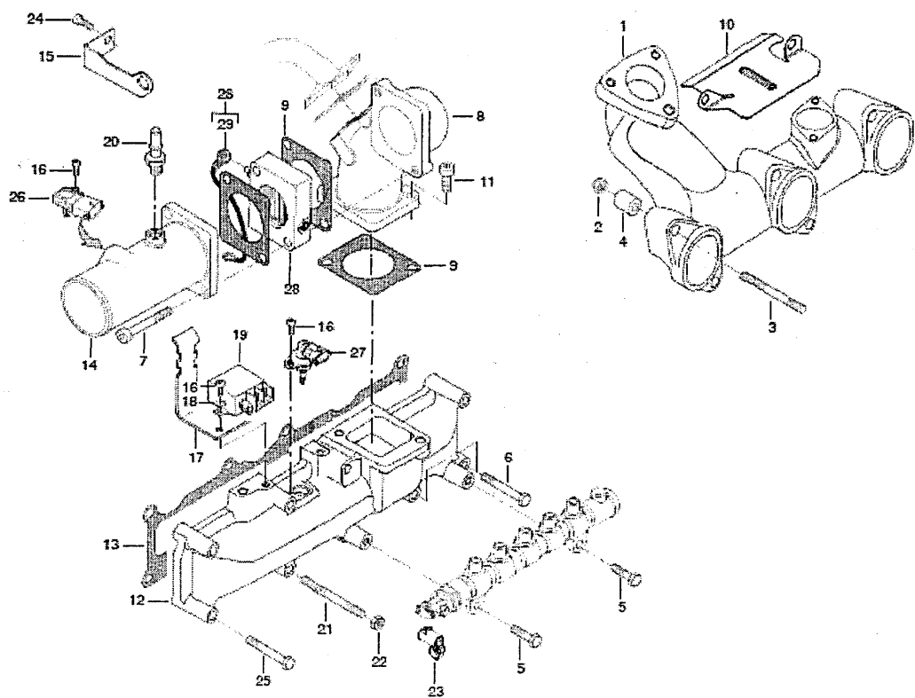
FIG.006 INLET&EXHAUST MANIFOLD
