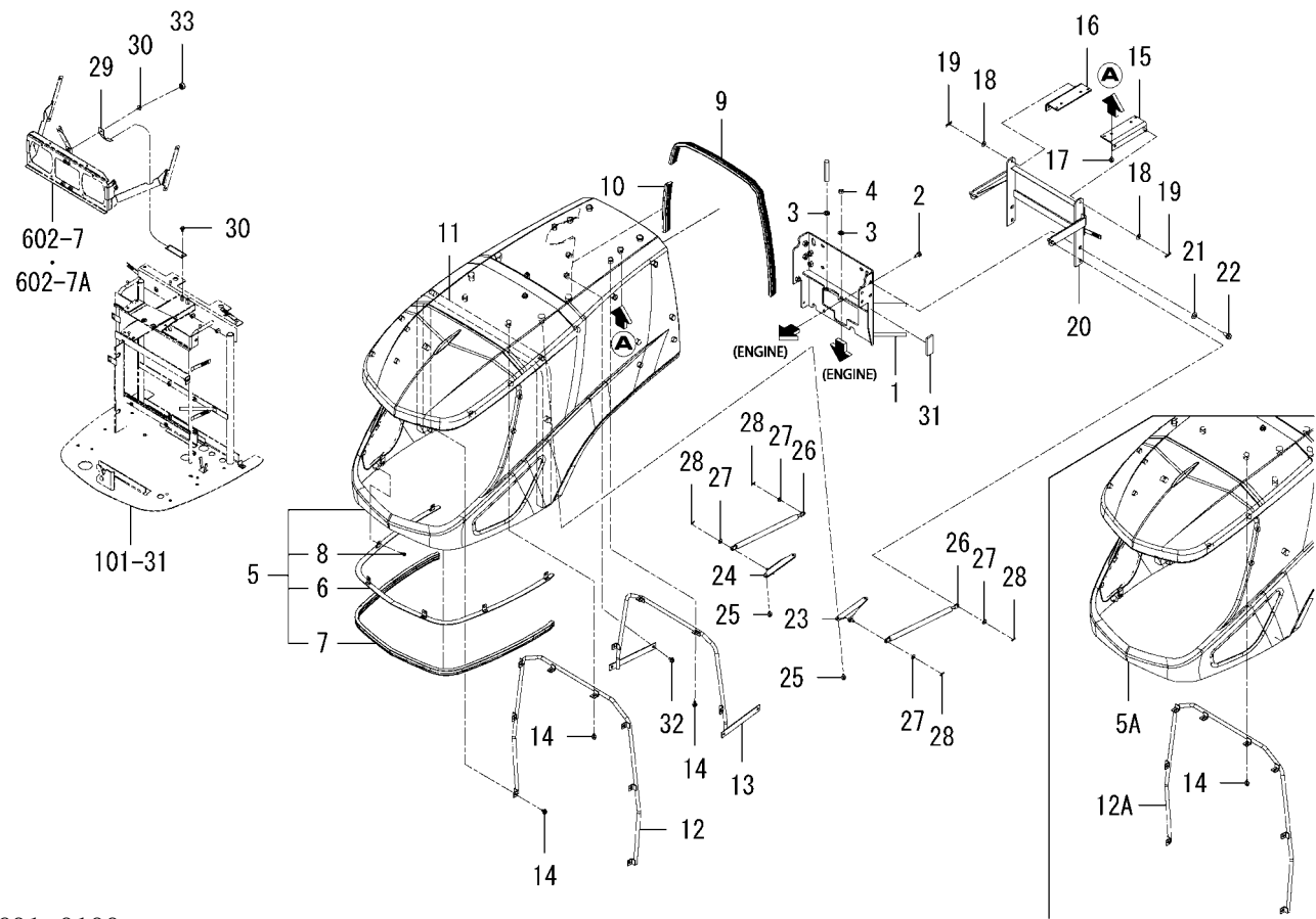
FIG.601 HOOD SYSTEM
