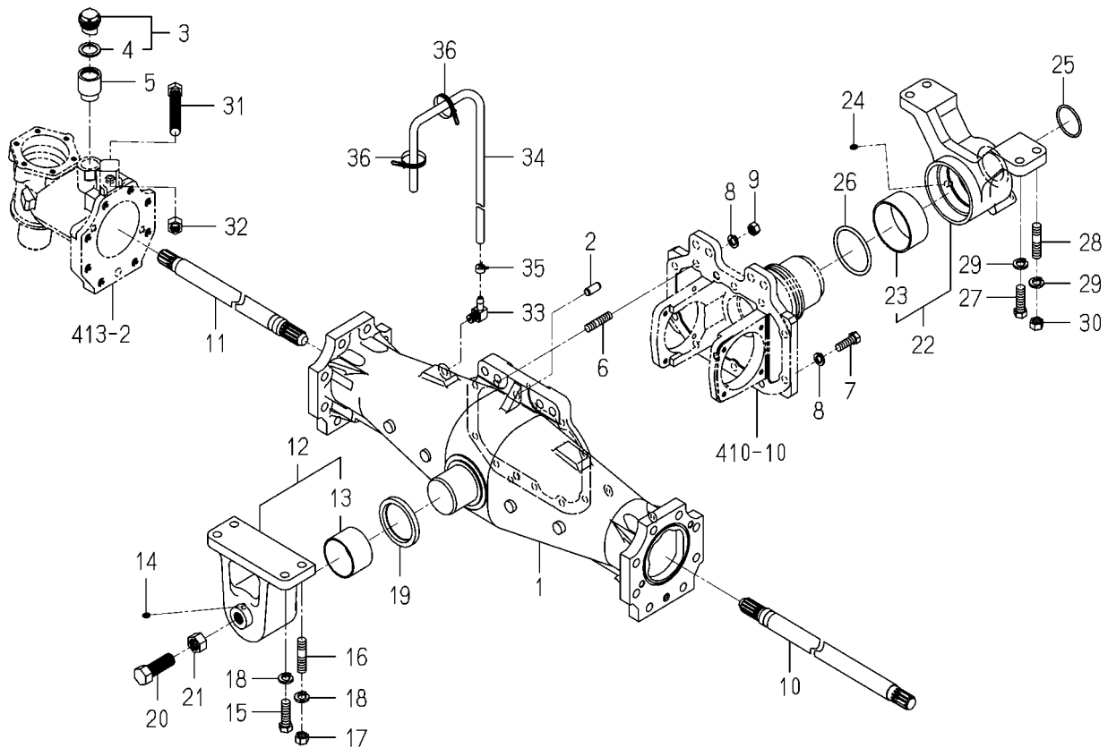
FIG.412 HOUSING(AXLE/FRONT)SYSTEM(8090,8100)
