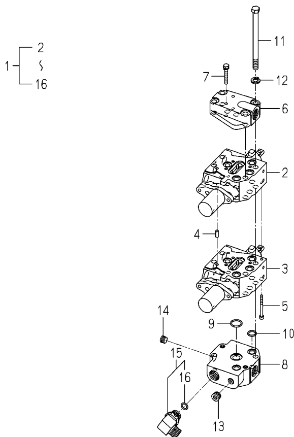
FIG.S06 COMPONENT PARTS FOR 1800-512-300-20 ON Fig.507,P06
