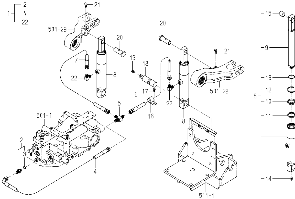
FIG.P03 CYLINDER(ASSIST/E4)ASSY (EXCEPT D TYPE)(OPTION)
