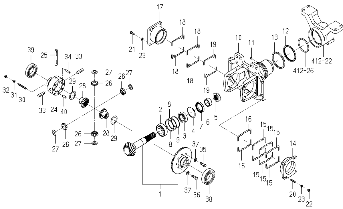
FIG.410 CASE (DIFFERENTIAL GEAR/FRONT)SYSTEM (8090,8100)
