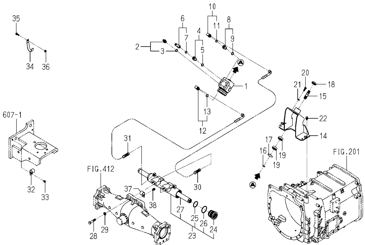
FIG.404 CONTROLLER (STEERING)SYSTEM(8090,8100)
