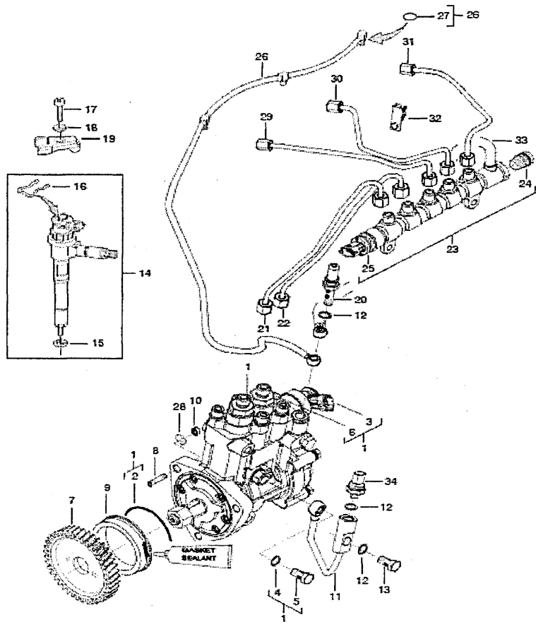
FIG.012 FUEL PUMP
