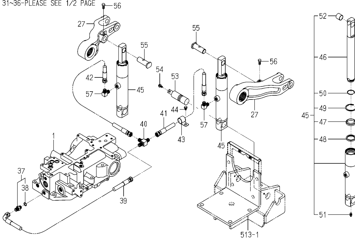
FIG.502 CASE(CYLINDER)SYSTEM(2/2) (EXCEPT 8090,8100-D TYPE)
