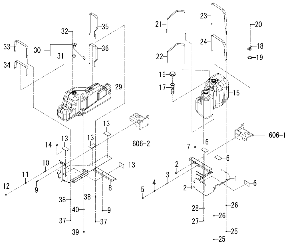
FIG.105 TANK(FUEL)SYSTEM(1/2)
