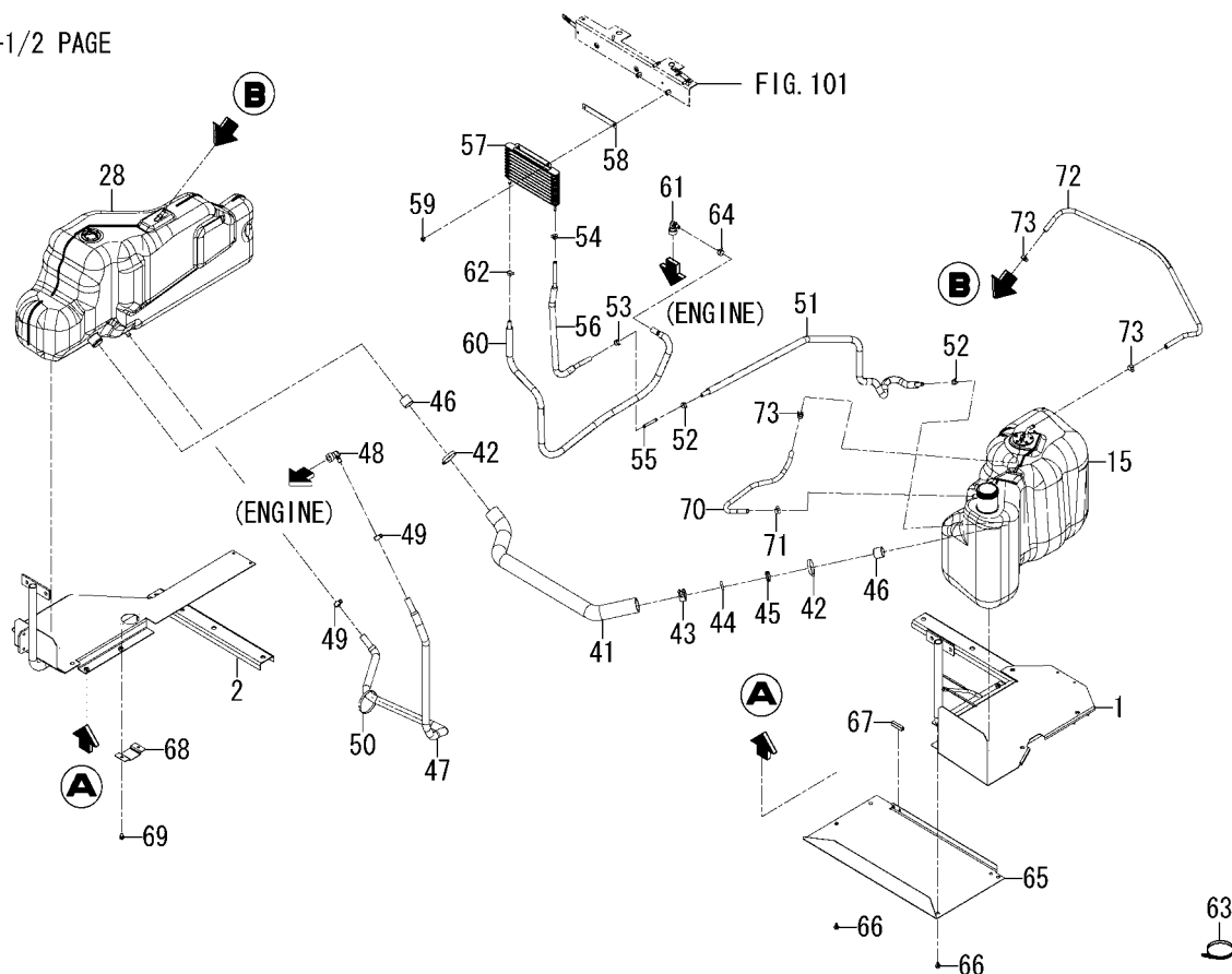
FIG.105 TANK(FUEL)SYSTEM(2/2)
