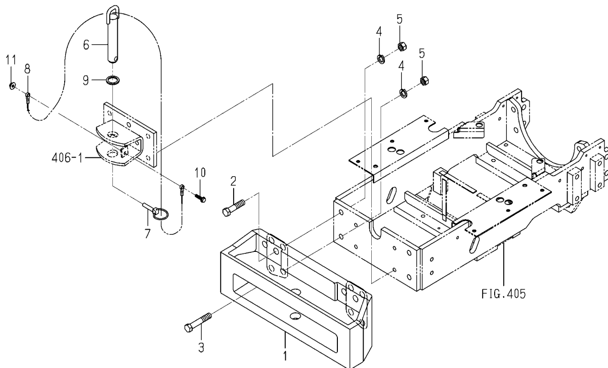
FIG.P02 HITCH(WEIGHT),BOLT&PIN SYSTEM (OPTION)
