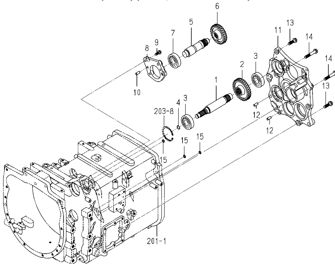
FIG.205 GEAR(POWER HIGH-LOW)SYSTEM (8080)(8090,8100-P TYPE)
