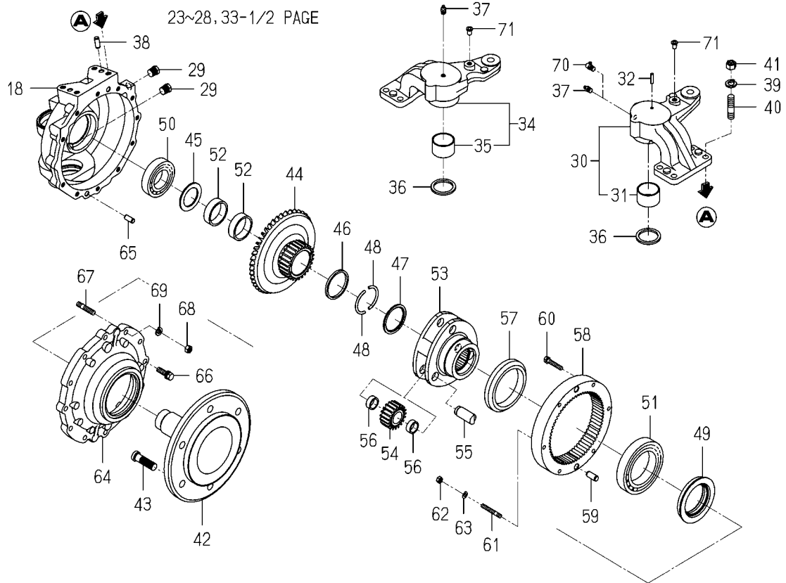
FIG.413 CASE(2/2) (GEAR/FINAL/FRONT)SYSTEM(8090,8100)
