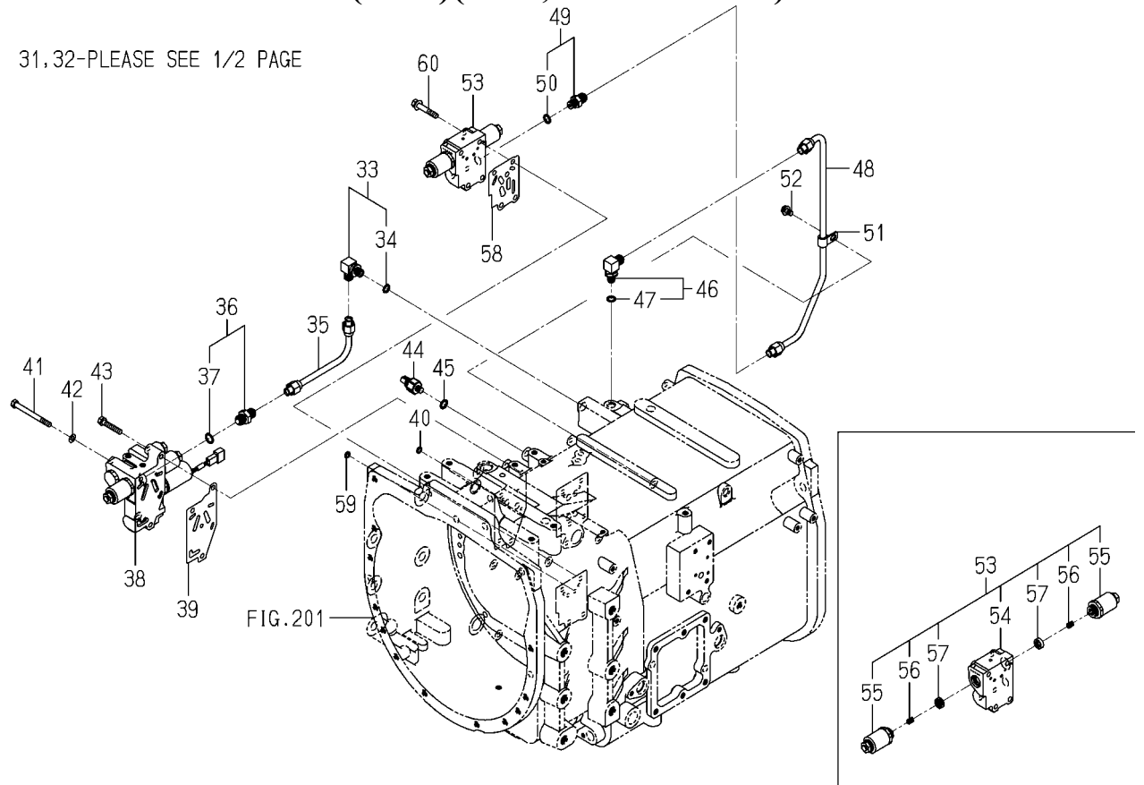
FIG.506 PIPING(SUB)SYSTEM(2/2) (8080)(8090,8100-P TYPE)
