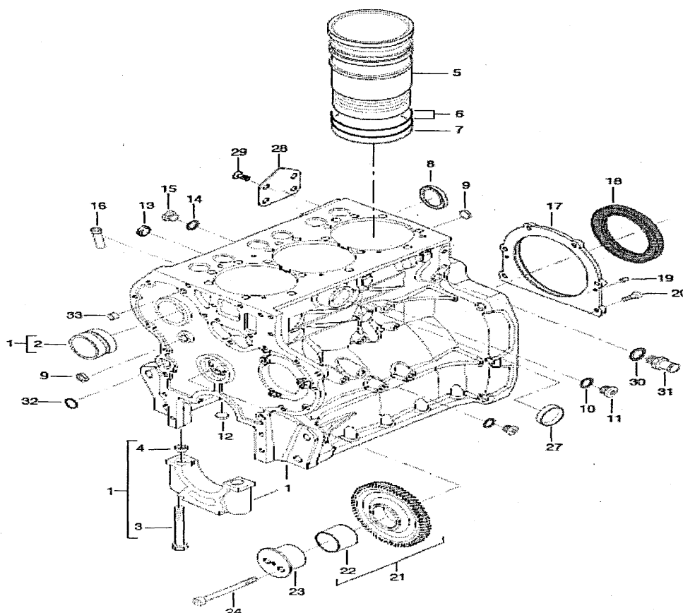
FIG.001 CYLINDER BLOCK
