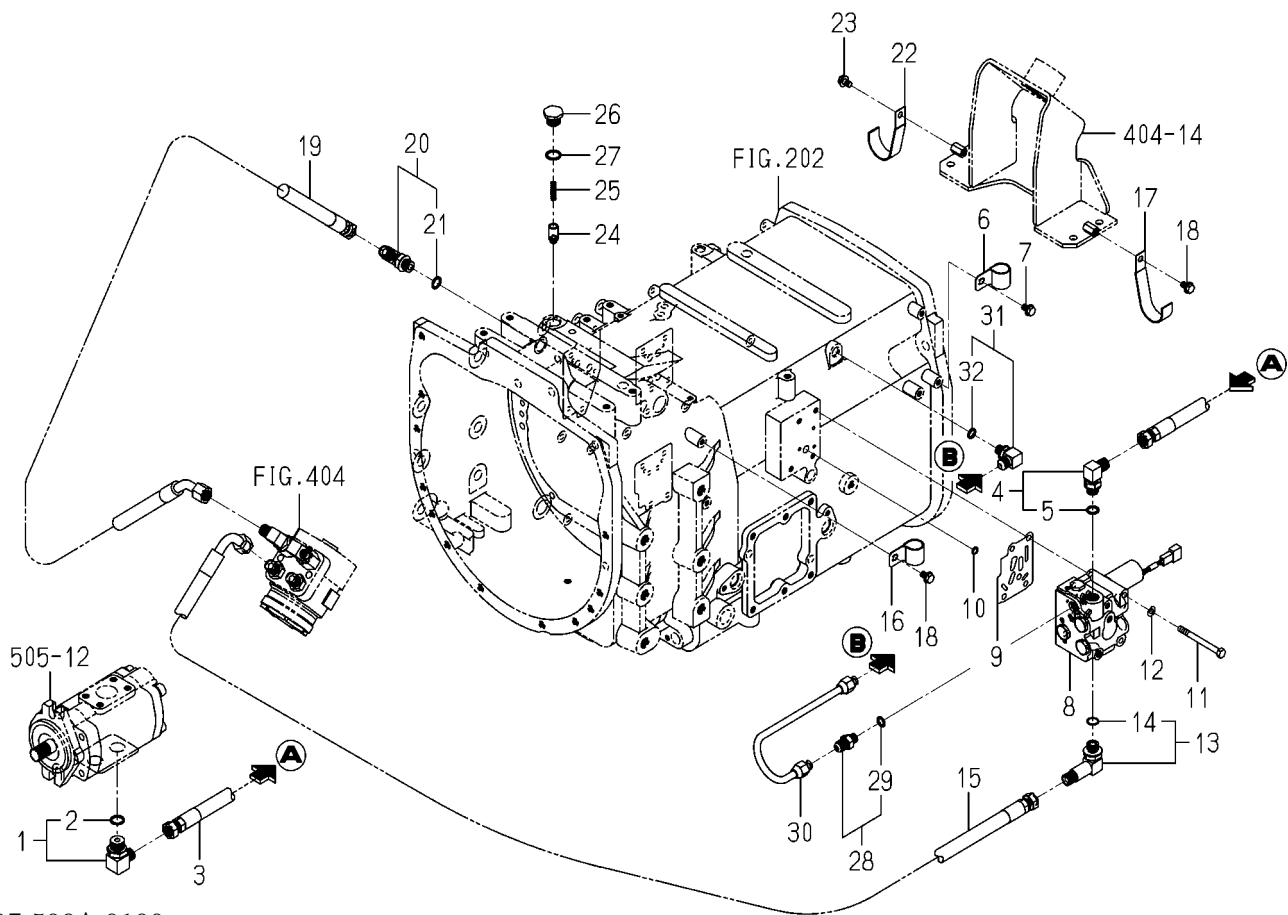
FIG.507 PIPING(SUB)SYSTEM(8090,8100-P1 TYPE)(1/2)
