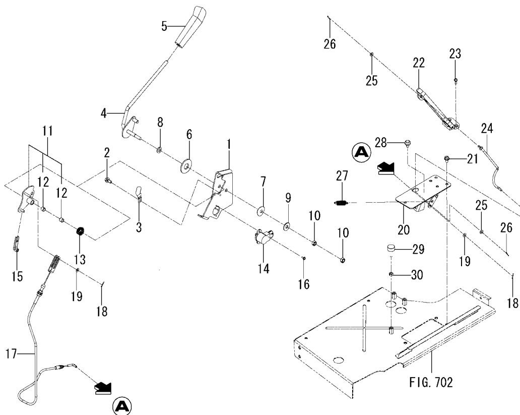
FIG.106 ACCELERATOR SYSTEM
