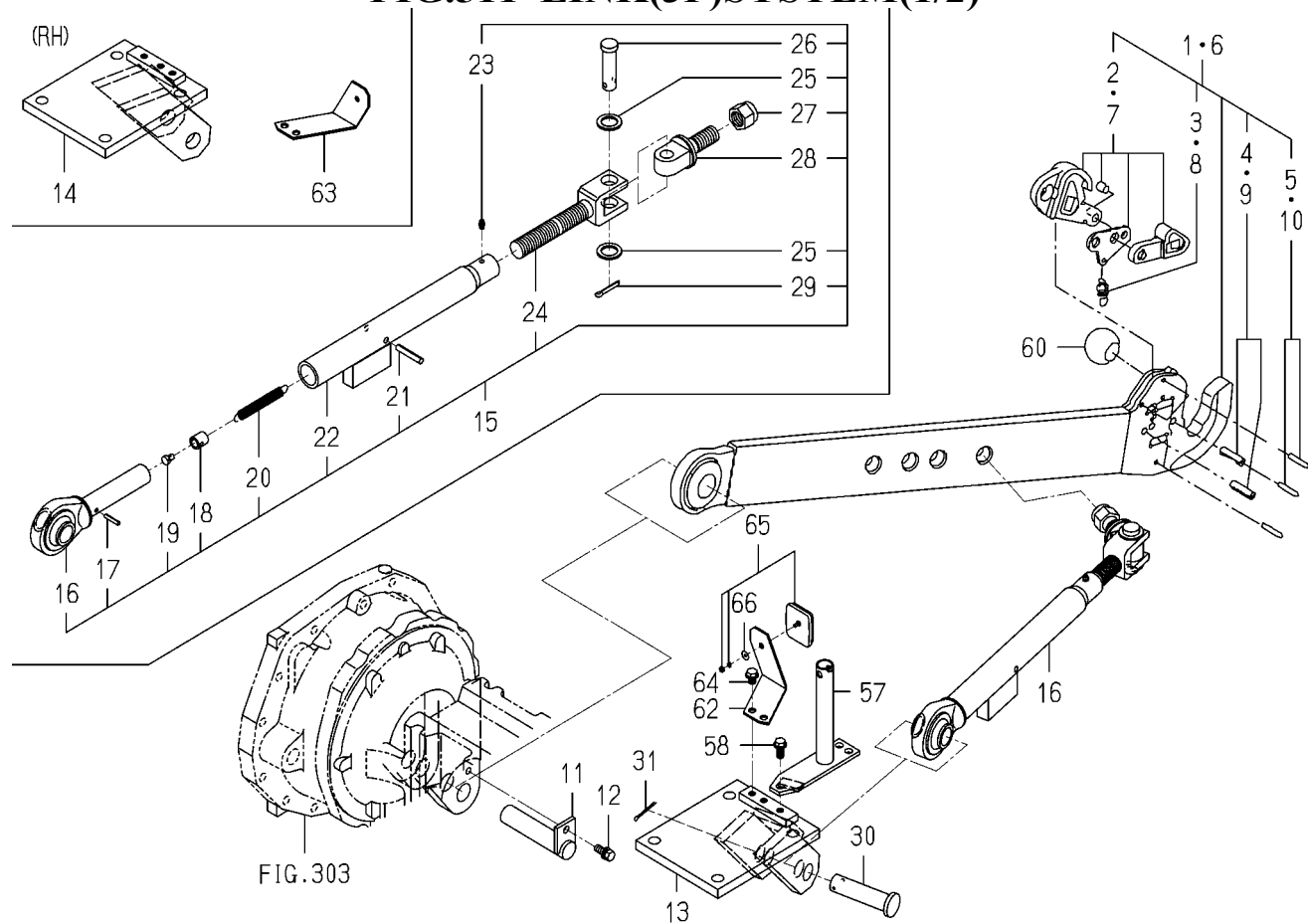
FIG.511 LINK(3P)SYSTEM(1/2)
