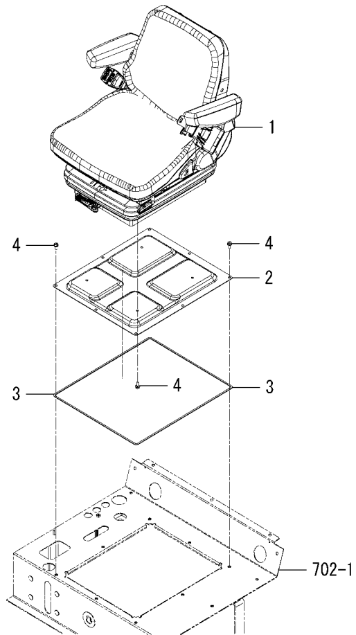
FIG.605 SEAT SYSTEM
