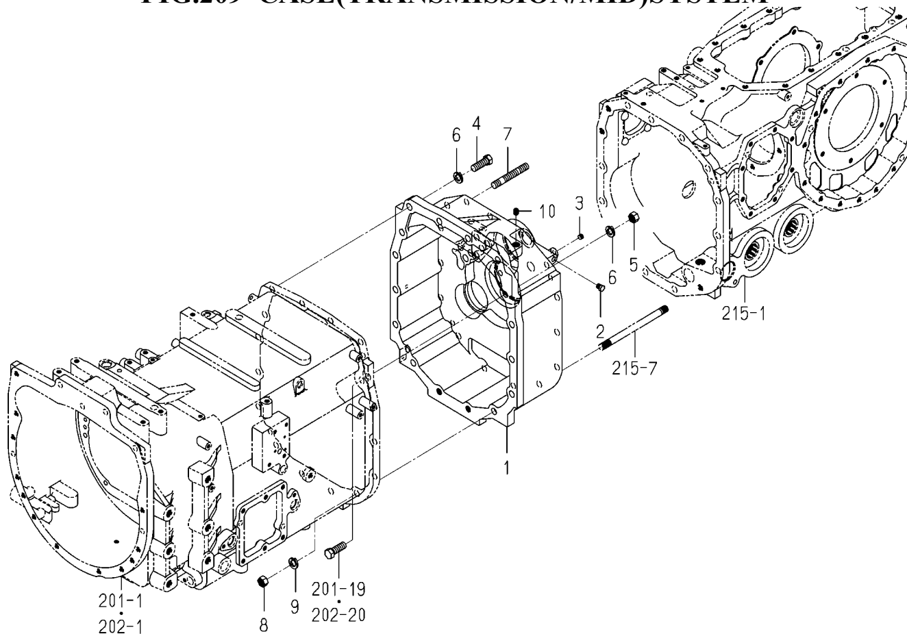
FIG.209 CASE(TRANSMISSION/MID)SYSTEM
