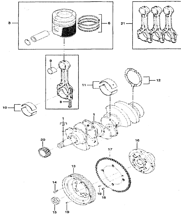
FIG.003 CRANKSHAFT
