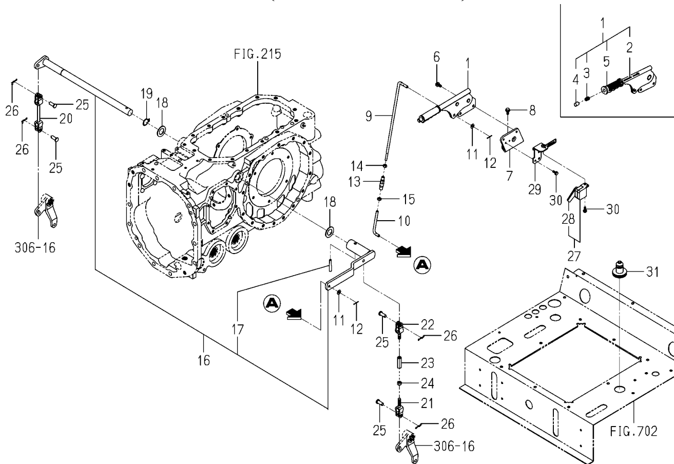
FIG.308 LEVER(BRAKE/PARKING)SYSTEM
