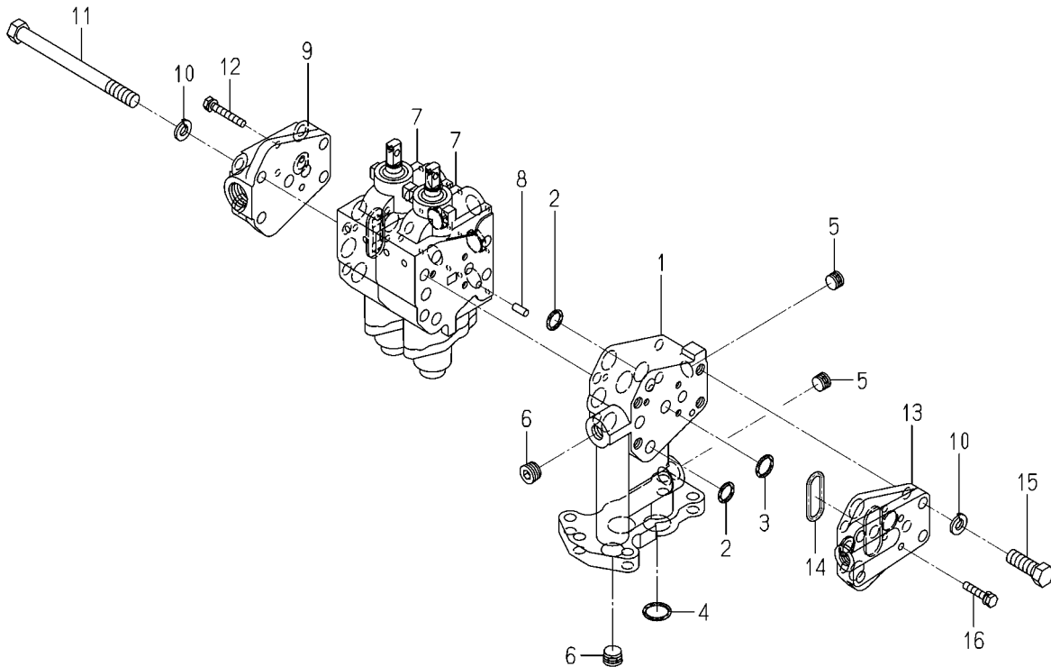
FIG.S04 COMPONENT PARTS FOR K211-099-000-10 ON Fig.508
