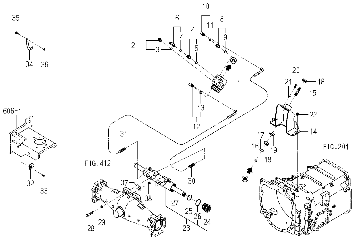
FIG.404 CONTROLLER(STEERING)SYSTEM (8090,8100)
