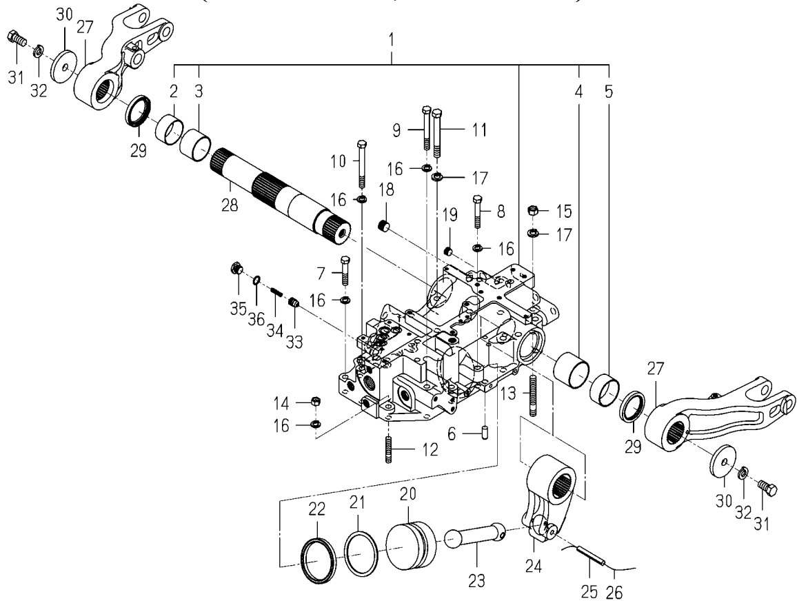
FIG.502 CASE(CYLINDER)SYSTEM(1/2) (EXCEPT 8090,8100-D TYPE)
