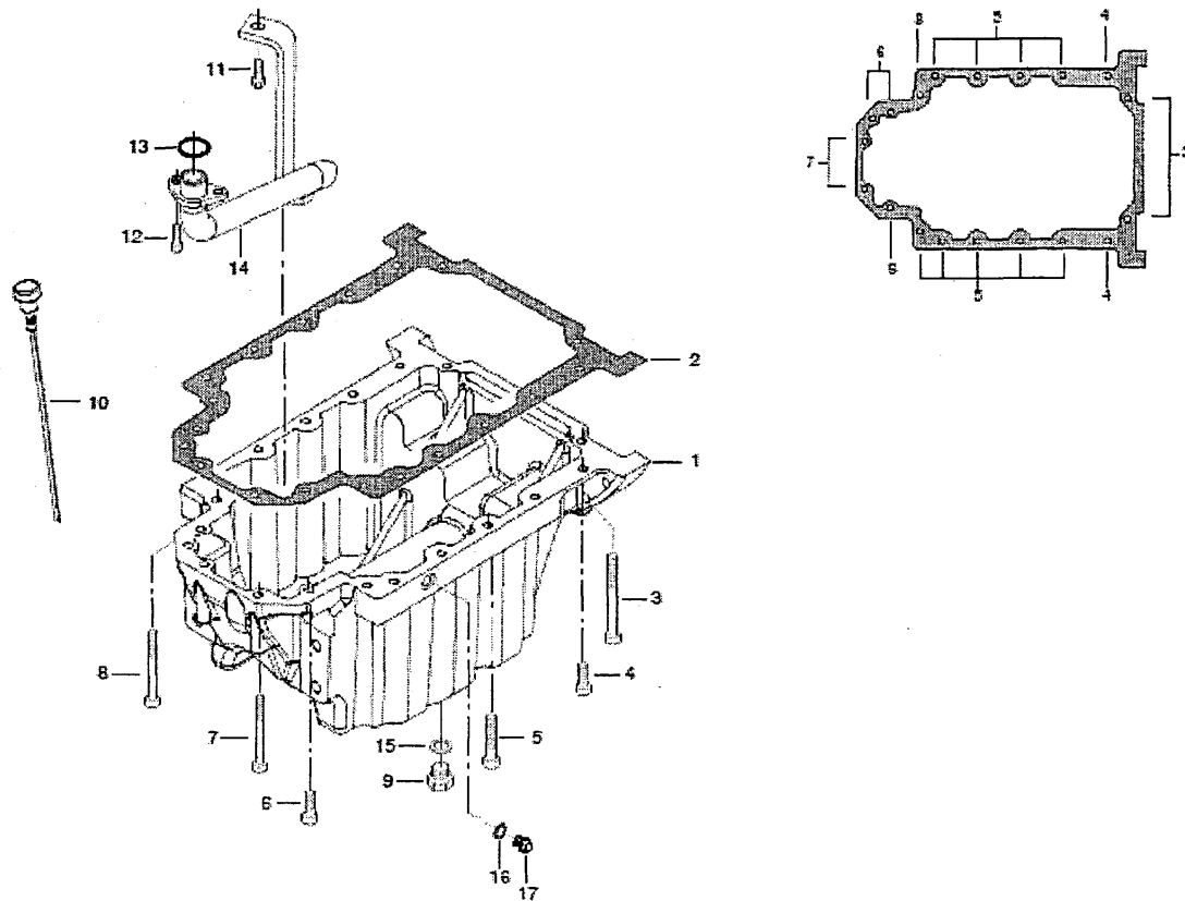
FIG.008 OIL SUMP
