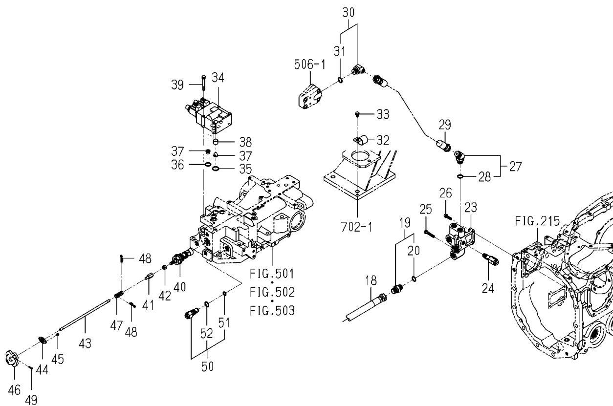
FIG.505 PIPING(MAIN)SYSTEM(2/3)
