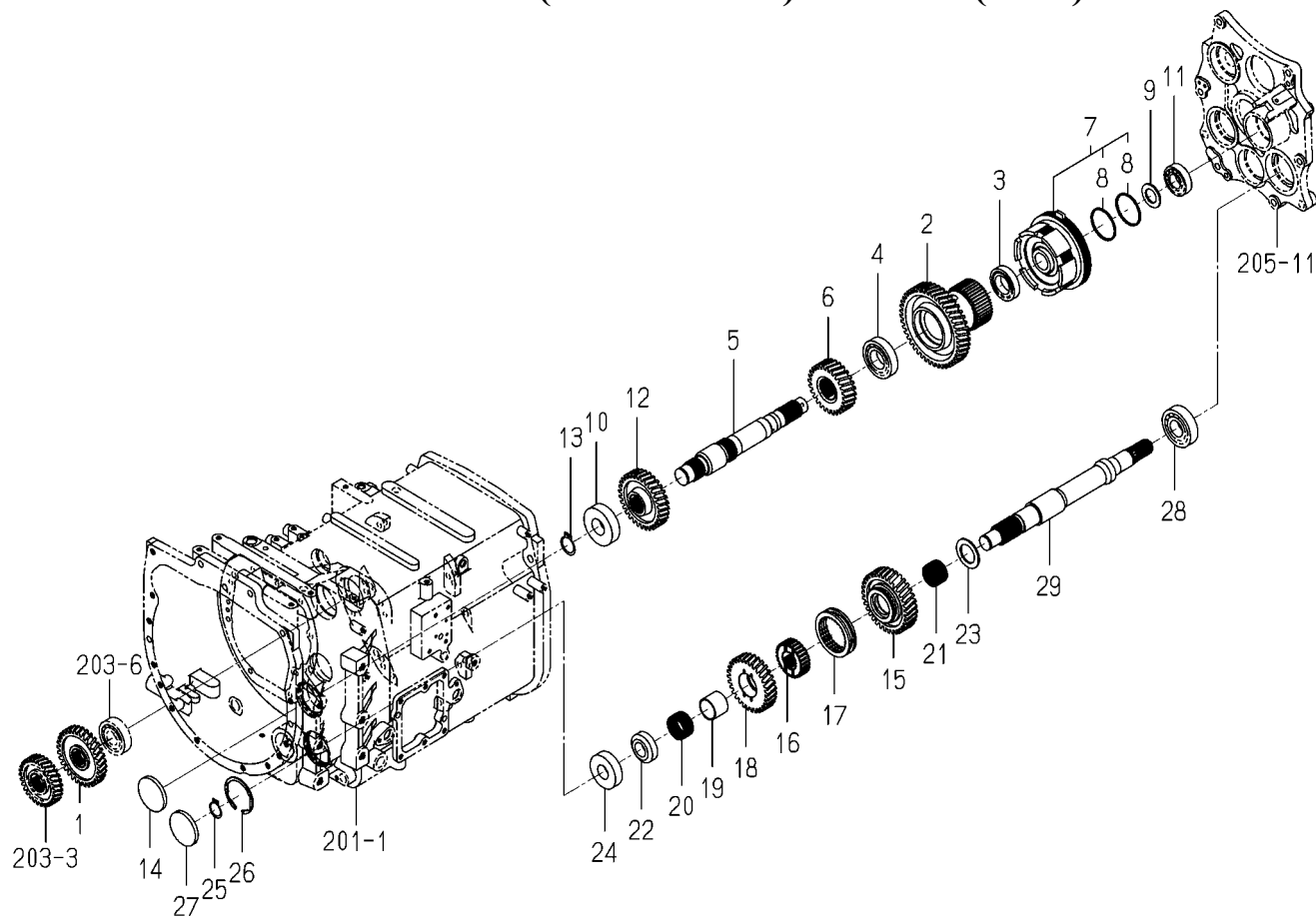
FIG.208 GEAR(PTO/INPUT)SYSTEM(8080)
