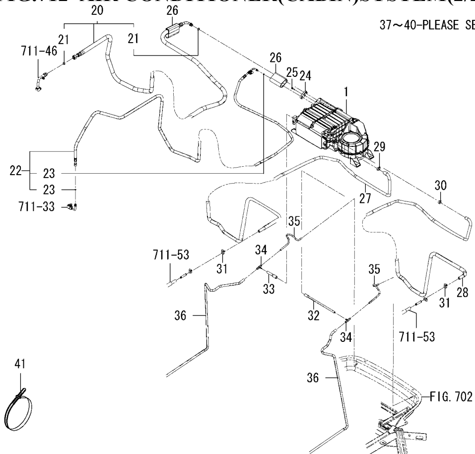
FIG.712 AIR CONDITIONER(CABIN)SYSTEM(2/2)
