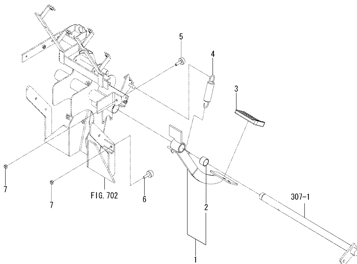
FIG.108 PEDAL(CLUTCH)SYSTEM
