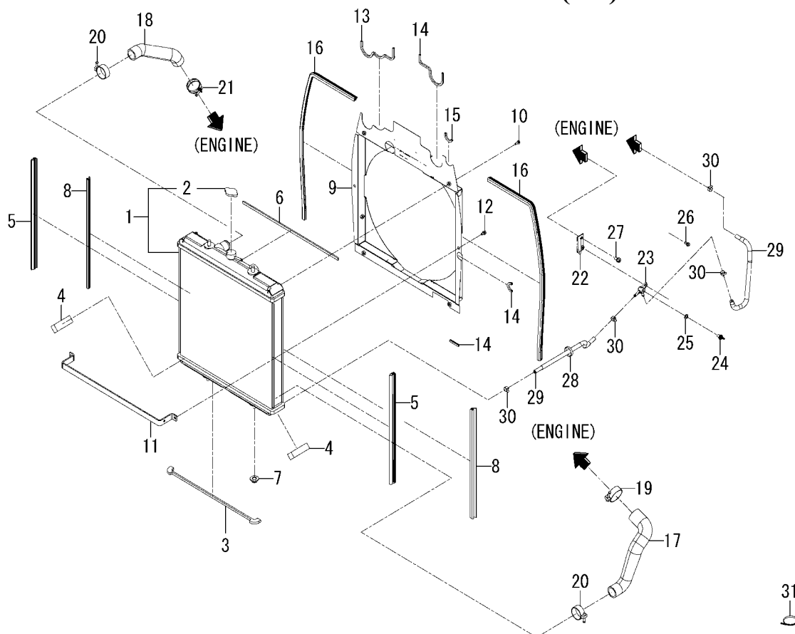
FIG.101 RADIATOR SYSTEM(1/2)
