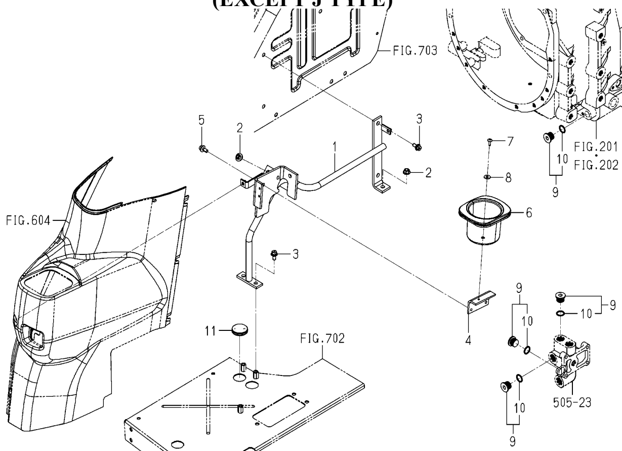
FIG.510 FRAME(GUIDE/LEVER)SYSTEM (EXCEPT J TYPE)
