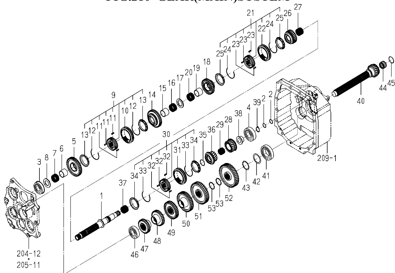
FIG.210 GEAR(MAIN)SYSTEM
