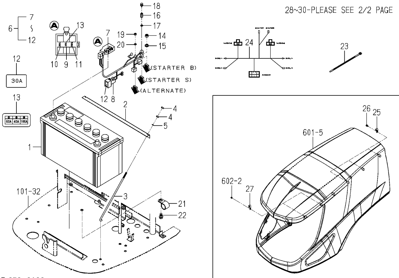
FIG.609 ELC.(FRONT)SYSTEM(1/2)
