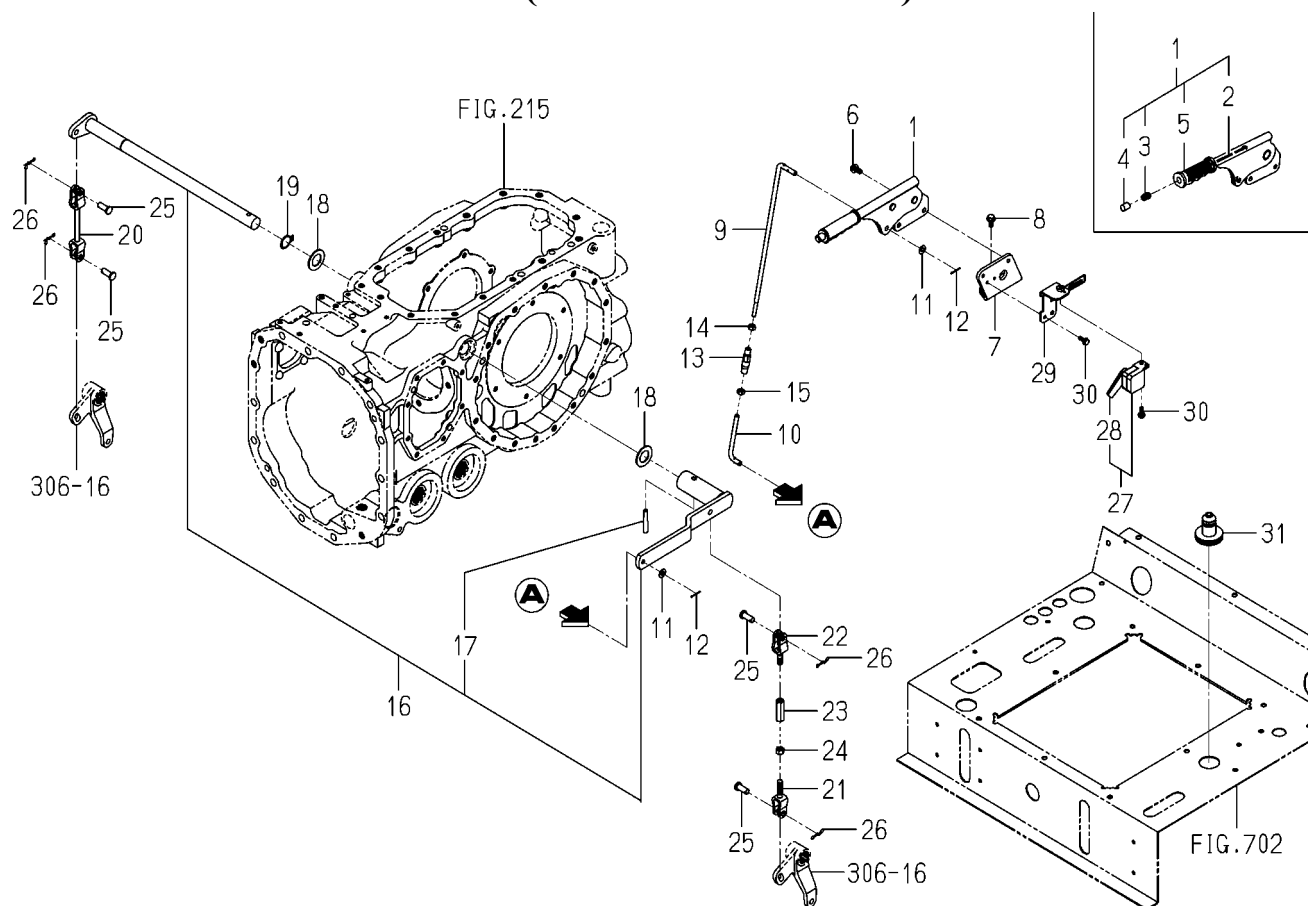
FIG.308 LEVER(BRAKE/PARKING)SYSTEM
