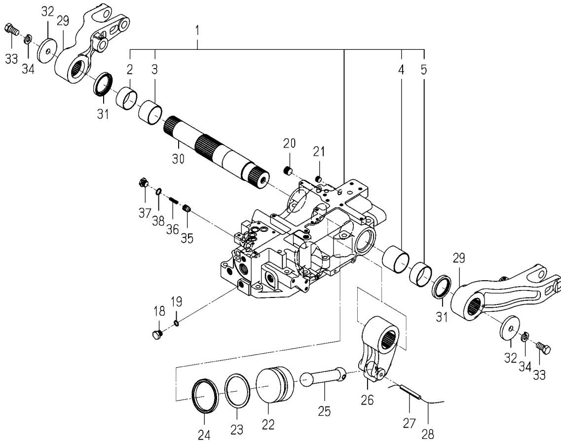
FIG.501 CASE(CYLINDER)SYSTEM(8080)(2/2)
