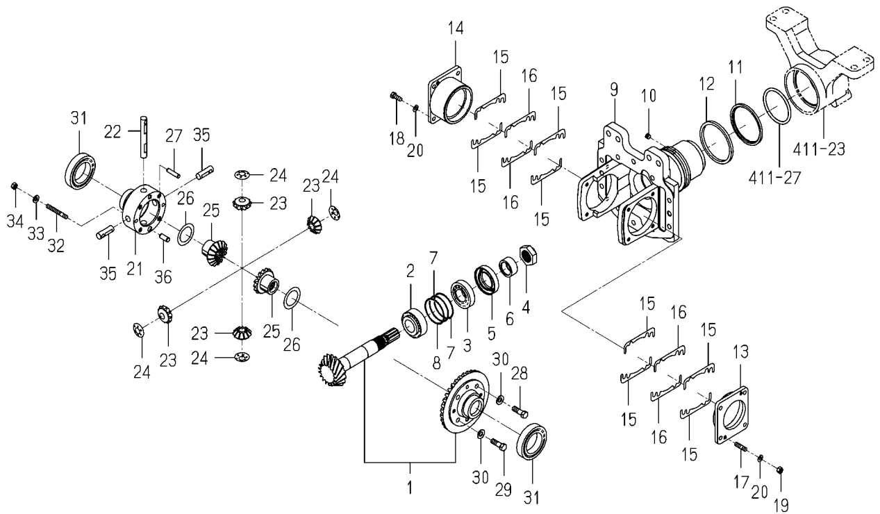
FIG.409 CASE (DIFFERENTIAL GEAR/FRONT)SYSTEM(8080)
