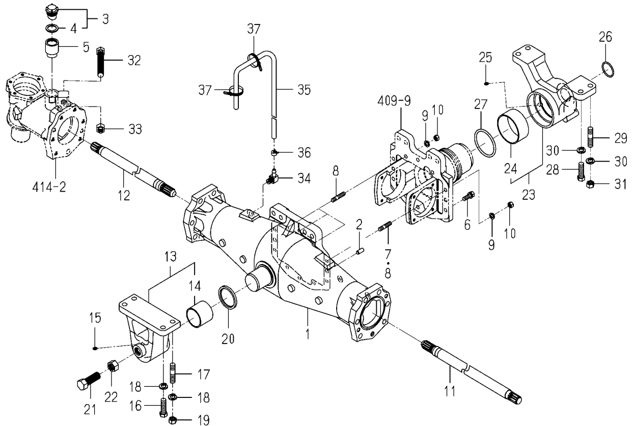
FIG.411 HOUSING(AXLE/FRONT)SYSTEM(8080)
