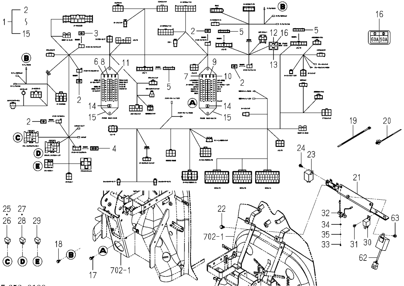
FIG.611 ELC.(MAIN)SYSTEM(1/2)
