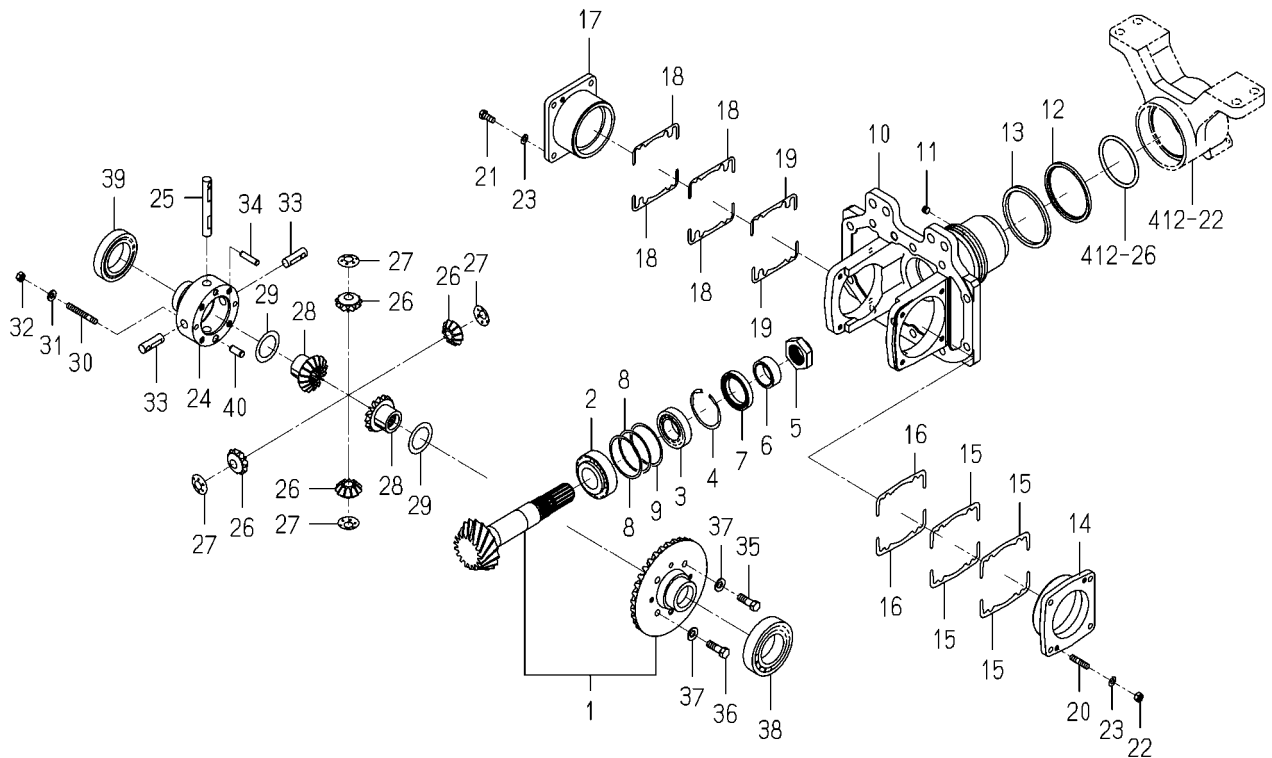
FIG.410 CASE (DIFFERENTIAL GEAR/FRONT)SYSTEM(8090,8100)
