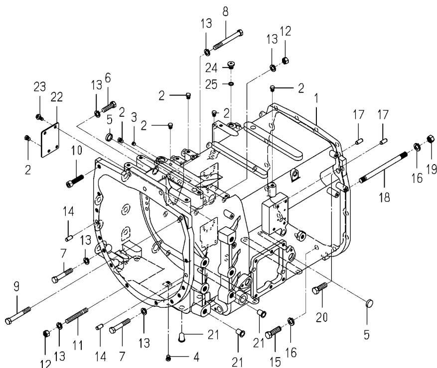
FIG.202 CASE(TRANSMISSION/FRONT)SYSTEM (8090,8100-P1 TYPE)
