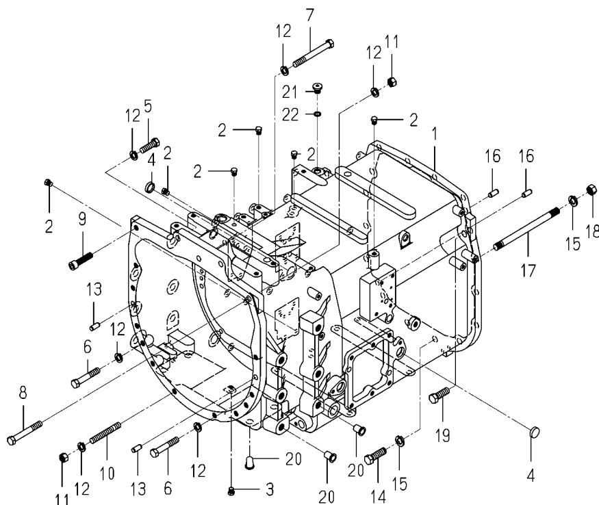
FIG.201 CASE(TRANSMISSION/FRONT)SYSTEM (8080)(8090,8100-P TYPE)
