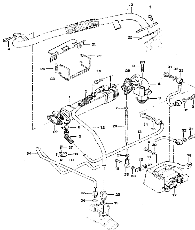
FIG.014 EGR PARTS
