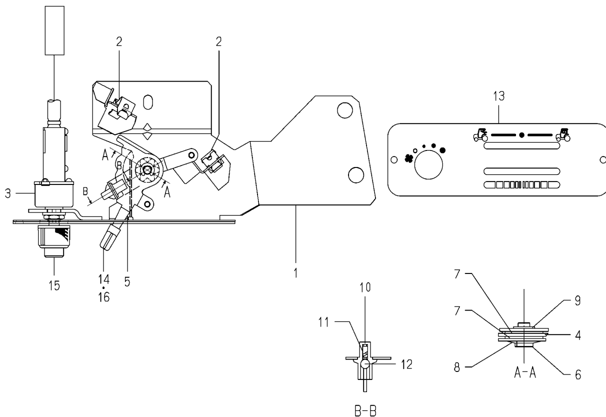
FIG.S09 COMPONENT PARTS FOR 1800-782-400-00 ON Fig.712
