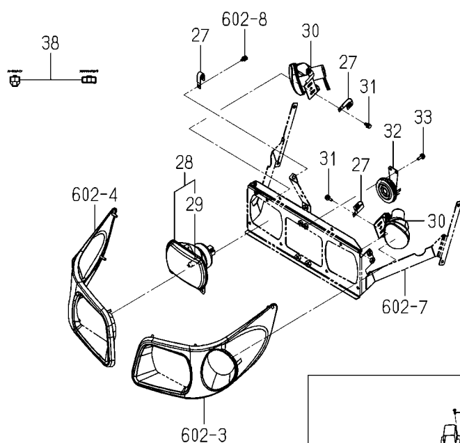
FIG.609 ELC.(FRONT)SYSTEM(2/2)
