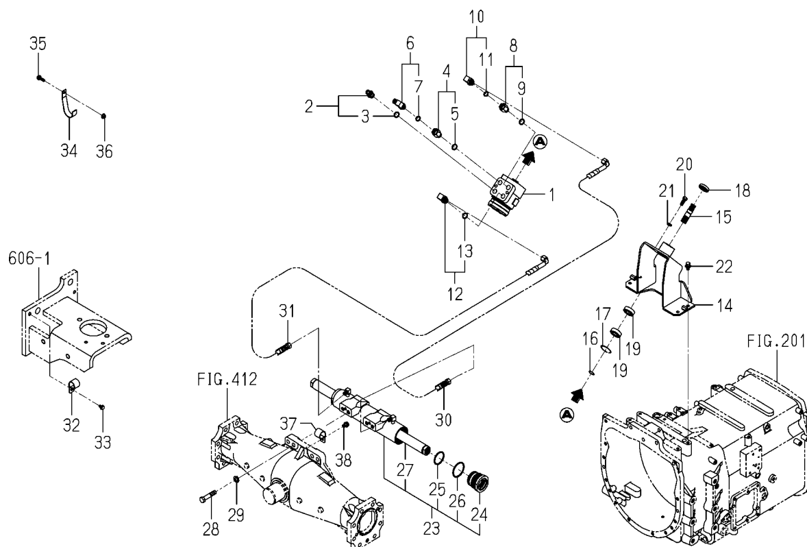
FIG.404 CONTROLLER(STEERING)SYSTEM (8090,8100)
