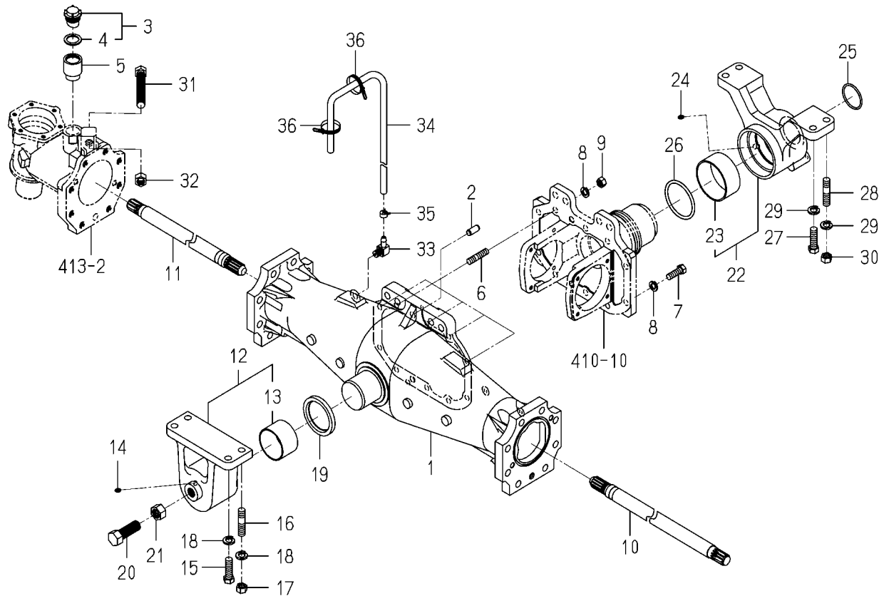
FIG.412 HOUSING(AXLE/FRONT)SYSTEM(8090,8100)
