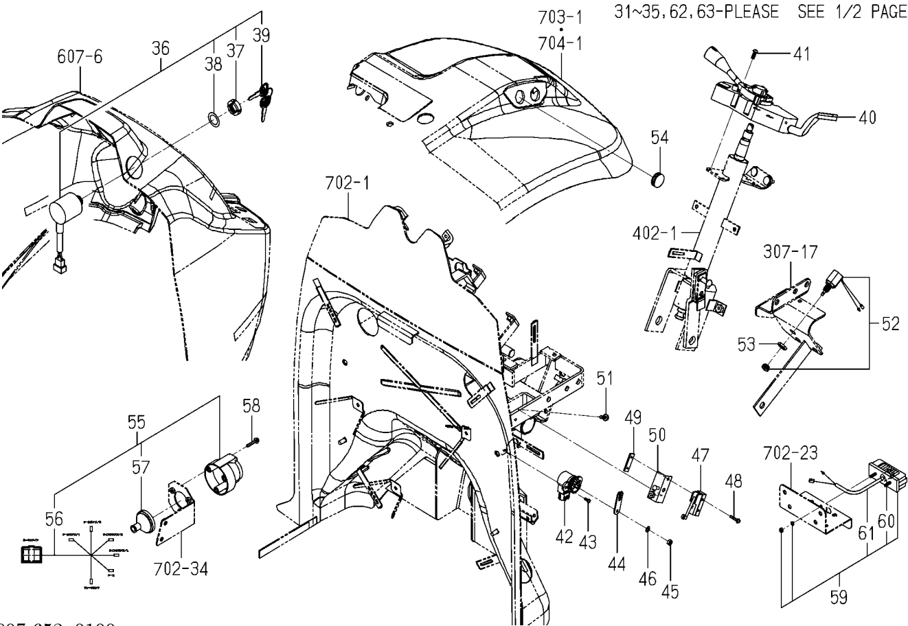
FIG.611 ELC.(MAIN)SYSTEM(2/2)
