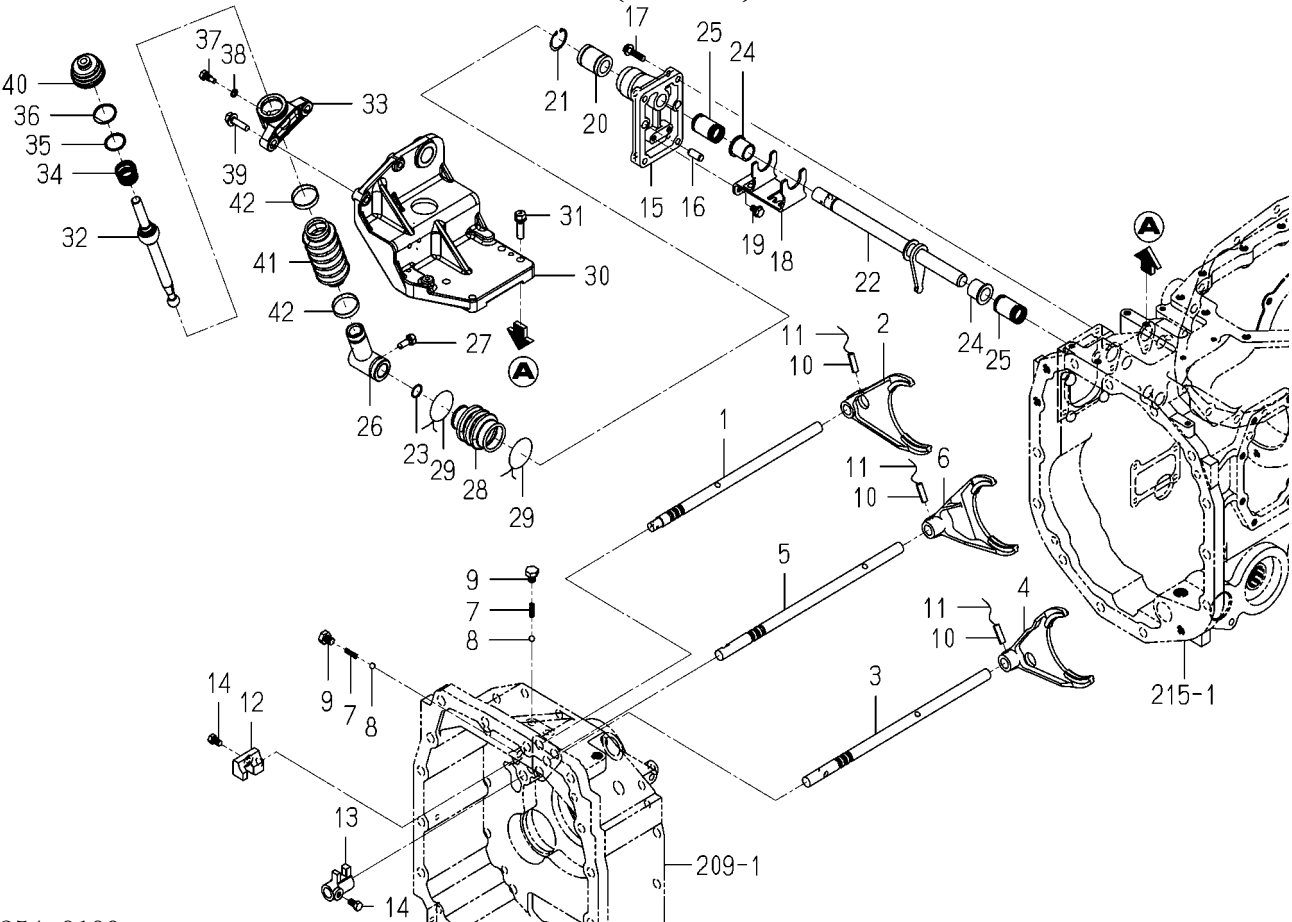
FIG.216 SHIFT(MAIN)SYSTEM
