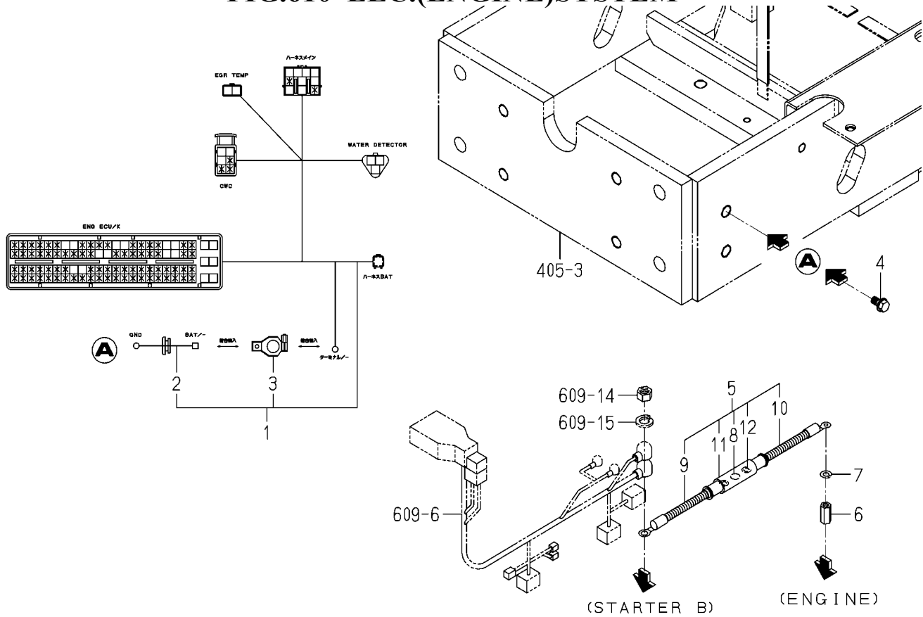
FIG.610 ELC.(ENGINE)SYSTEM
