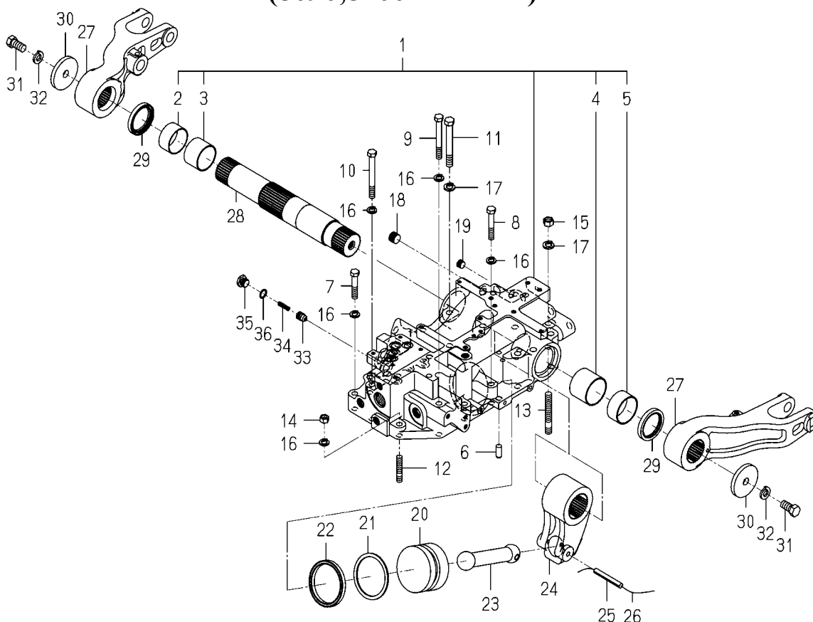
FIG.503 CASE(CYLINDER)SYSTEM(1/2) (8090,8100-D TYPE)
