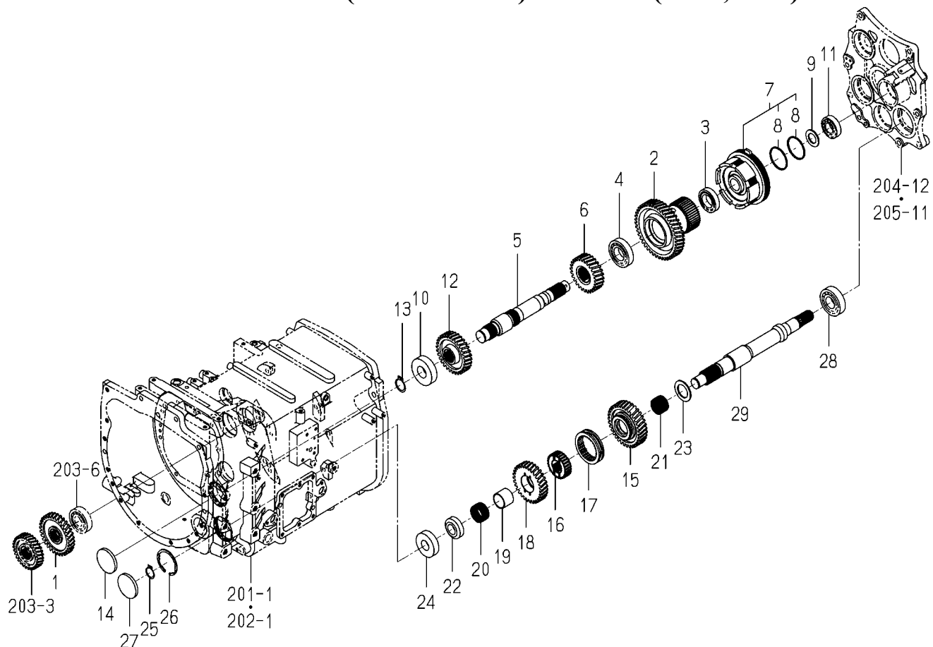
FIG.207 GEAR(PTO/INPUT)SYSTEM(8090,8100)
