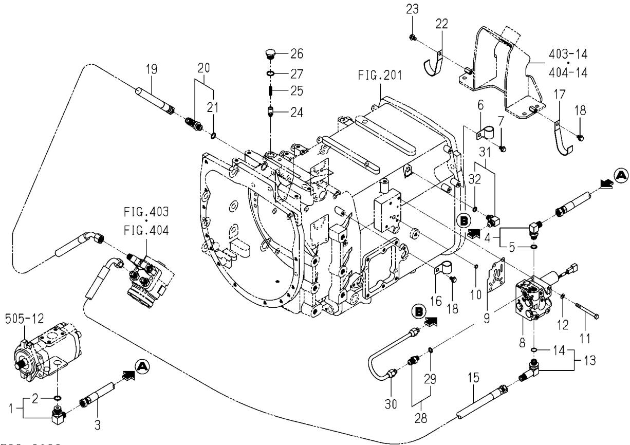
FIG.506 PIPING(SUB)SYSTEM(1/2) (8080)(8090,8100-P TYPE)
