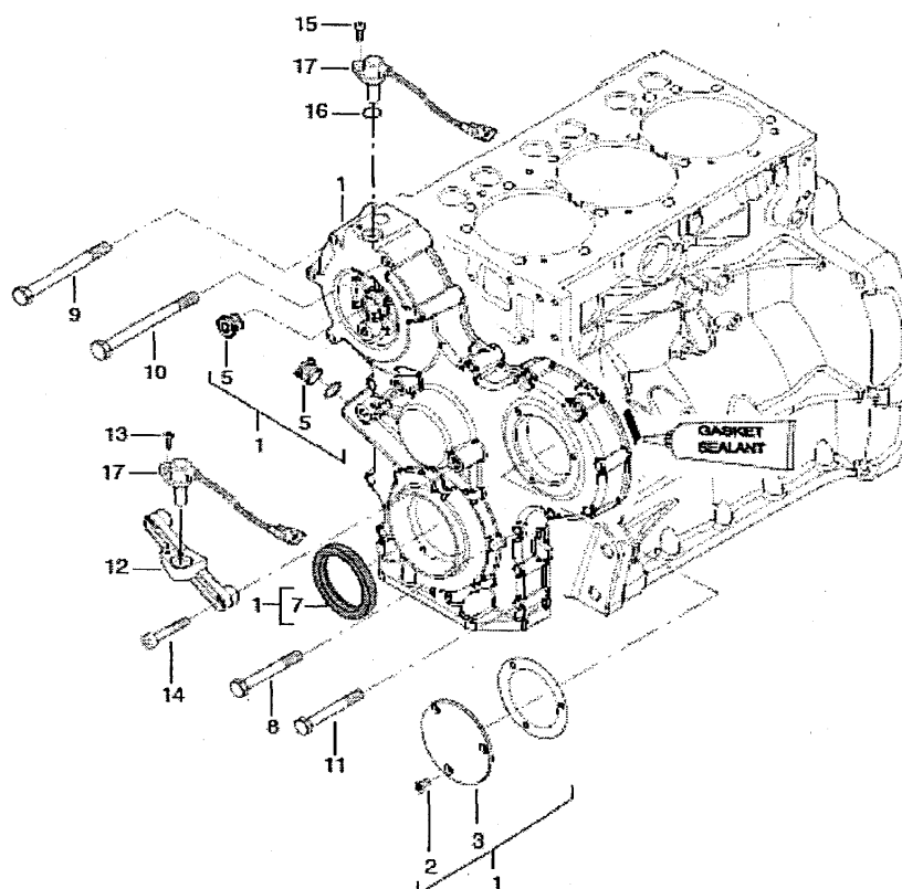
FIG.002 GEAR HOUSING
