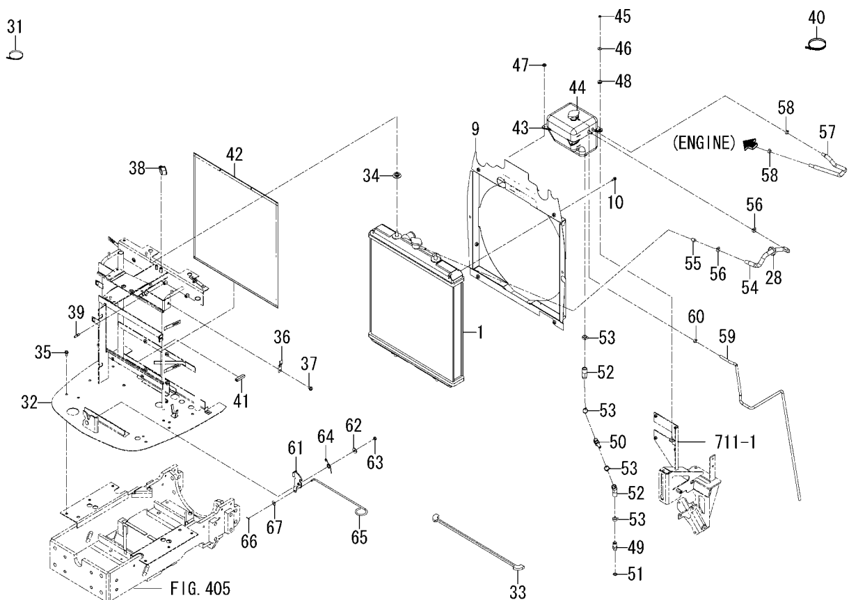
FIG.101 RADIATOR SYSTEM(2/2)
