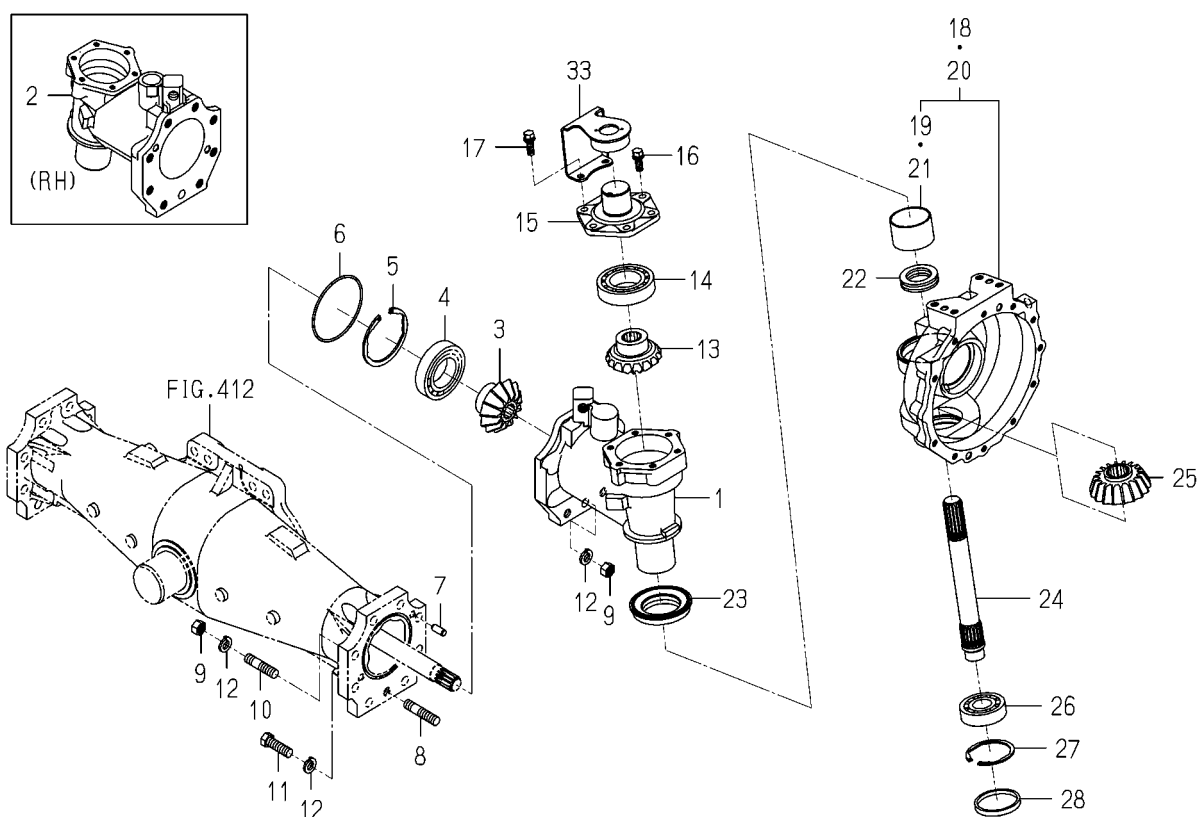
FIG.413 CASE(1/2) (GEAR/FINAL/FRONT)SYSTEM(8090,8100)
