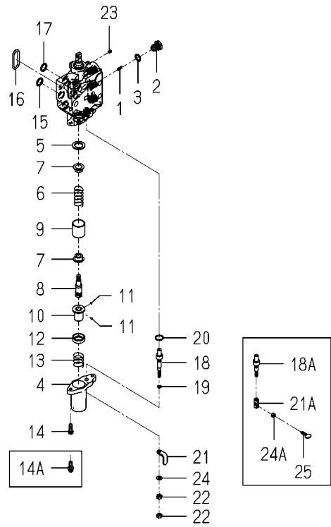
FIG.S03 COMPONENT PARTS FOR K211-075-500-60 ON Fig.P05
