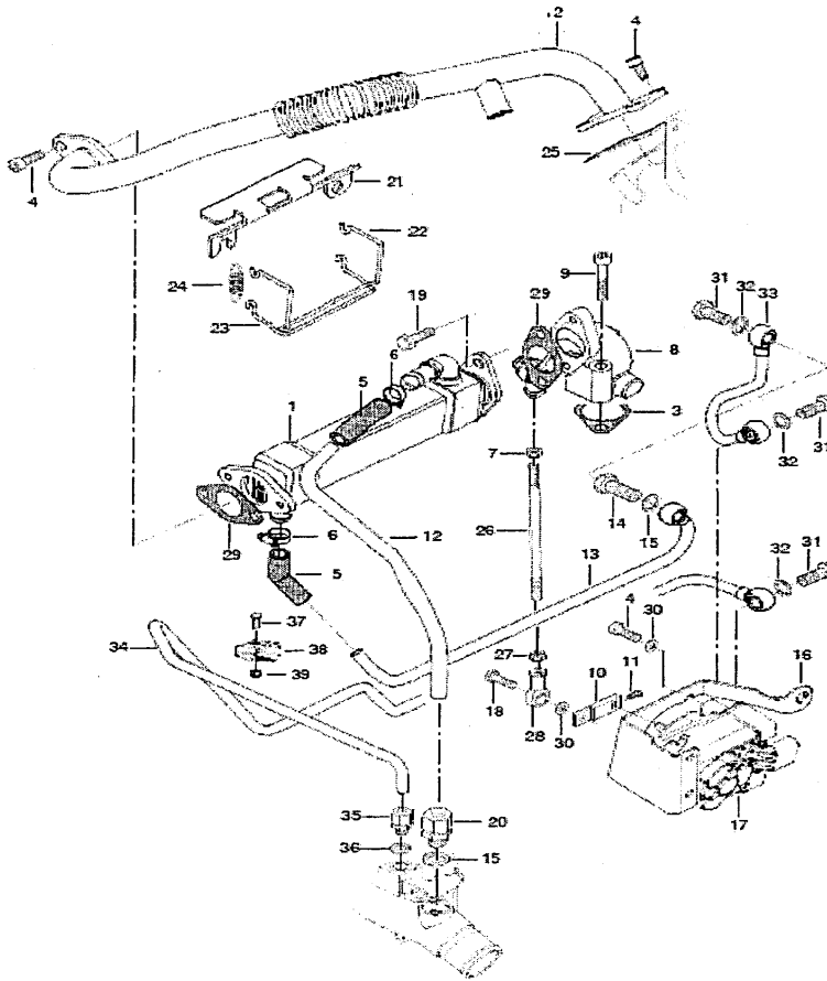
FIG.014 EGR PARTS
