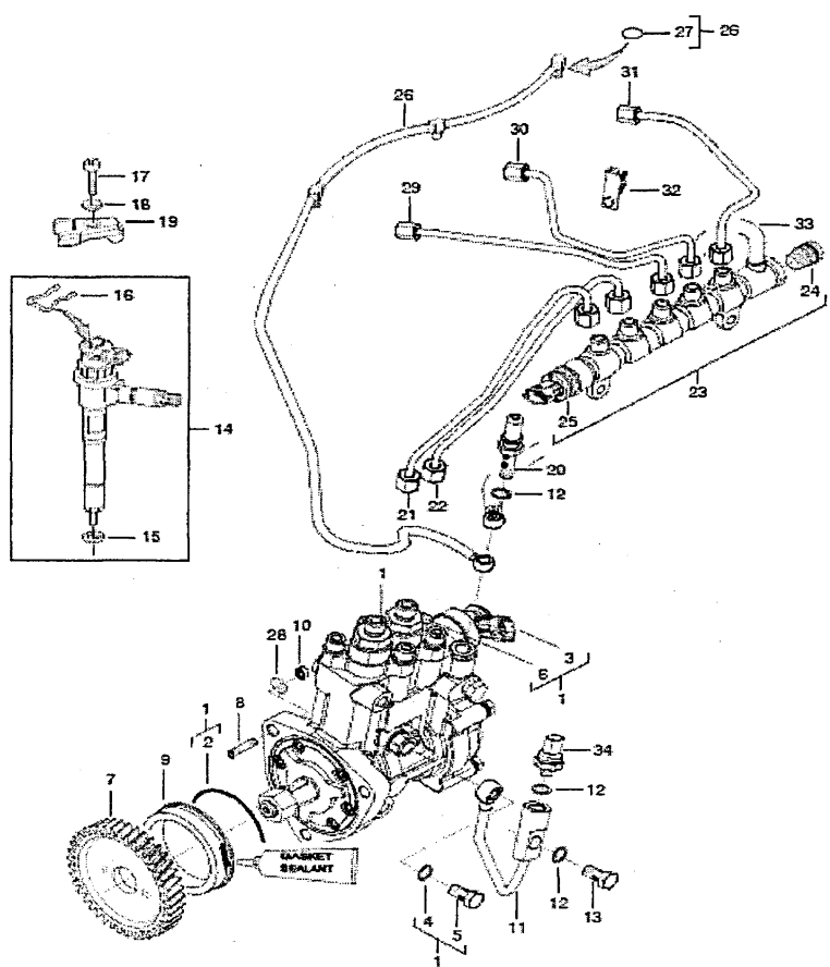
FIG.012 FUEL PUMP
