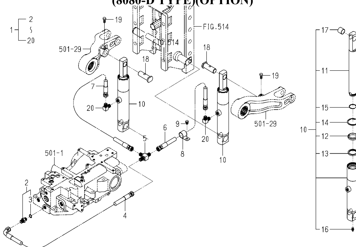
FIG.P04 CYLINDER(ASSIST/E4D)ASSY (8080-D TYPE)(OPTION)
