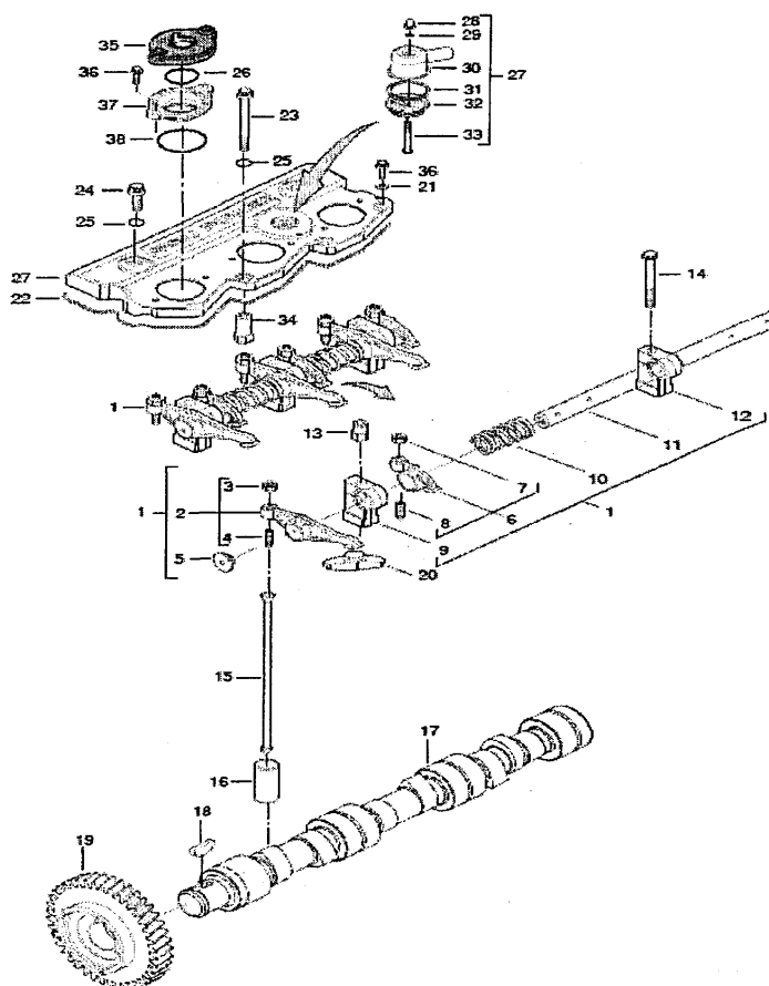
FIG.004 VALVE MECHANISM
