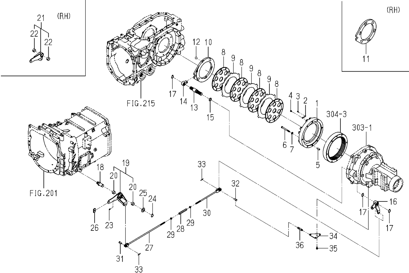
FIG.306 BRAKE SYSTEM
