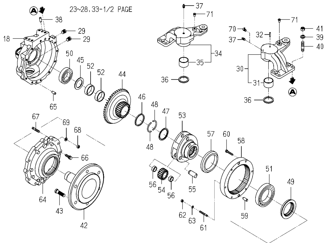
FIG.413 CASE(2/2) (GEAR/FINAL/FRONT)SYSTEM(8090,8100)
