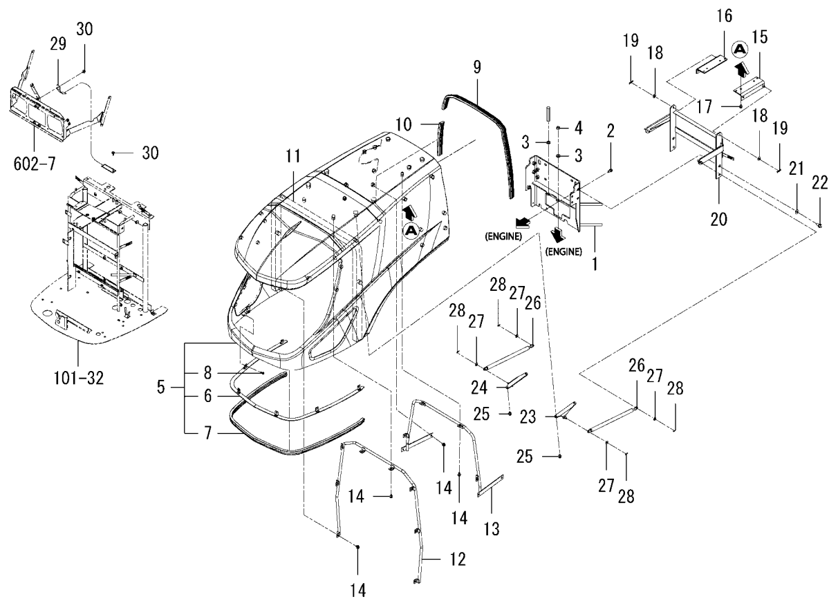
FIG.601 HOOD SYSTEM
