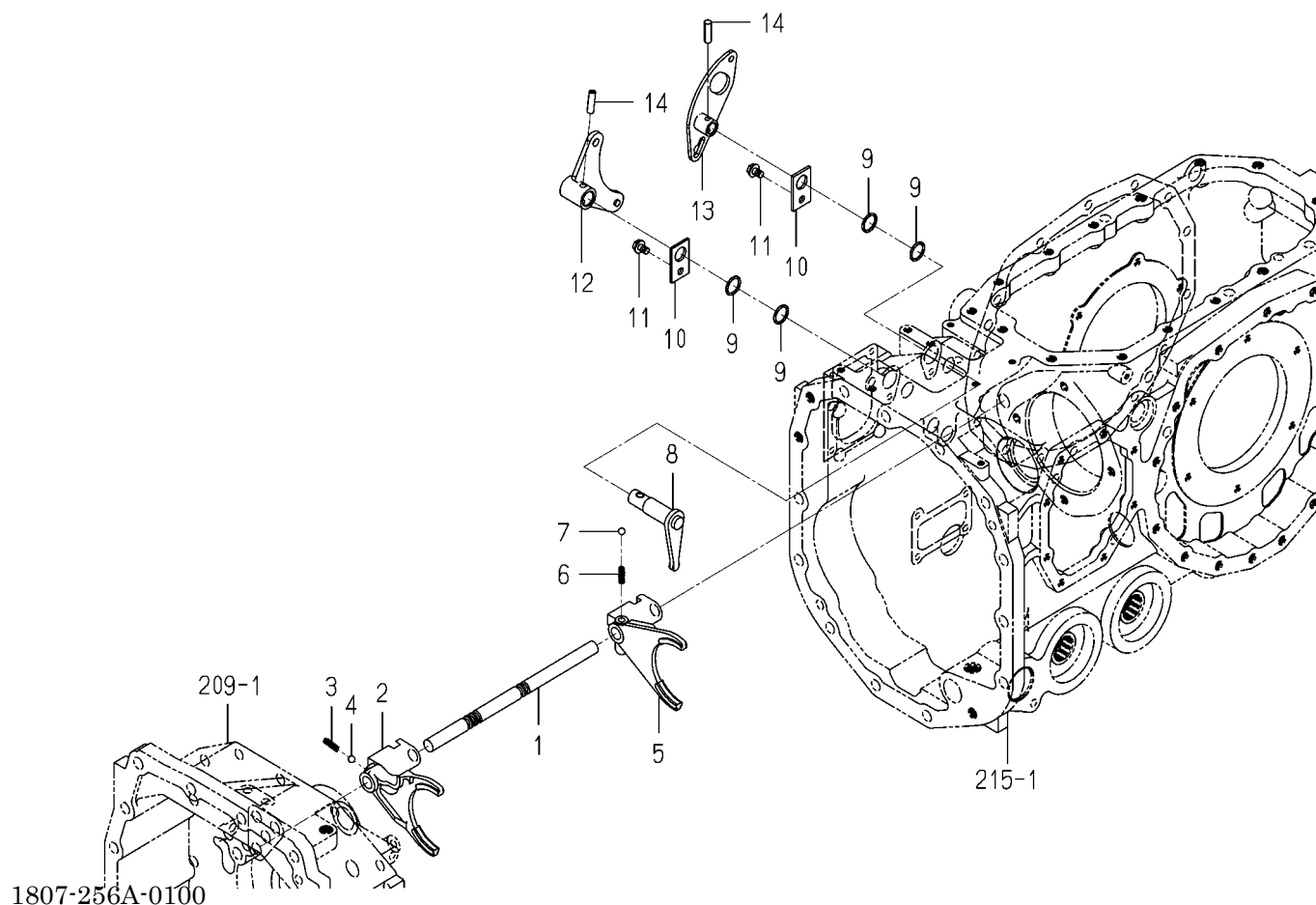
FIG.217 SHIFT(RANGE)SYSTEM
