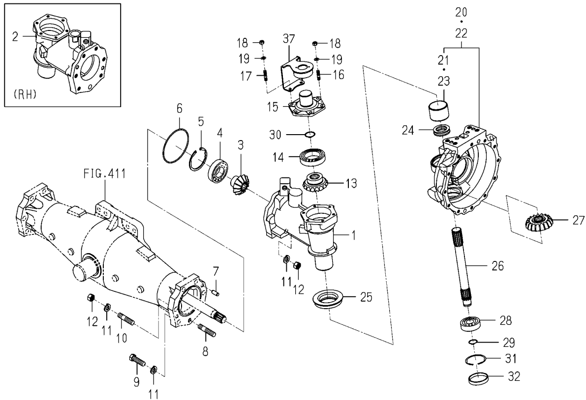
FIG.414 CASE(1/2) (GEAR/FINAL/FRONT)SYSTEM(8080)
