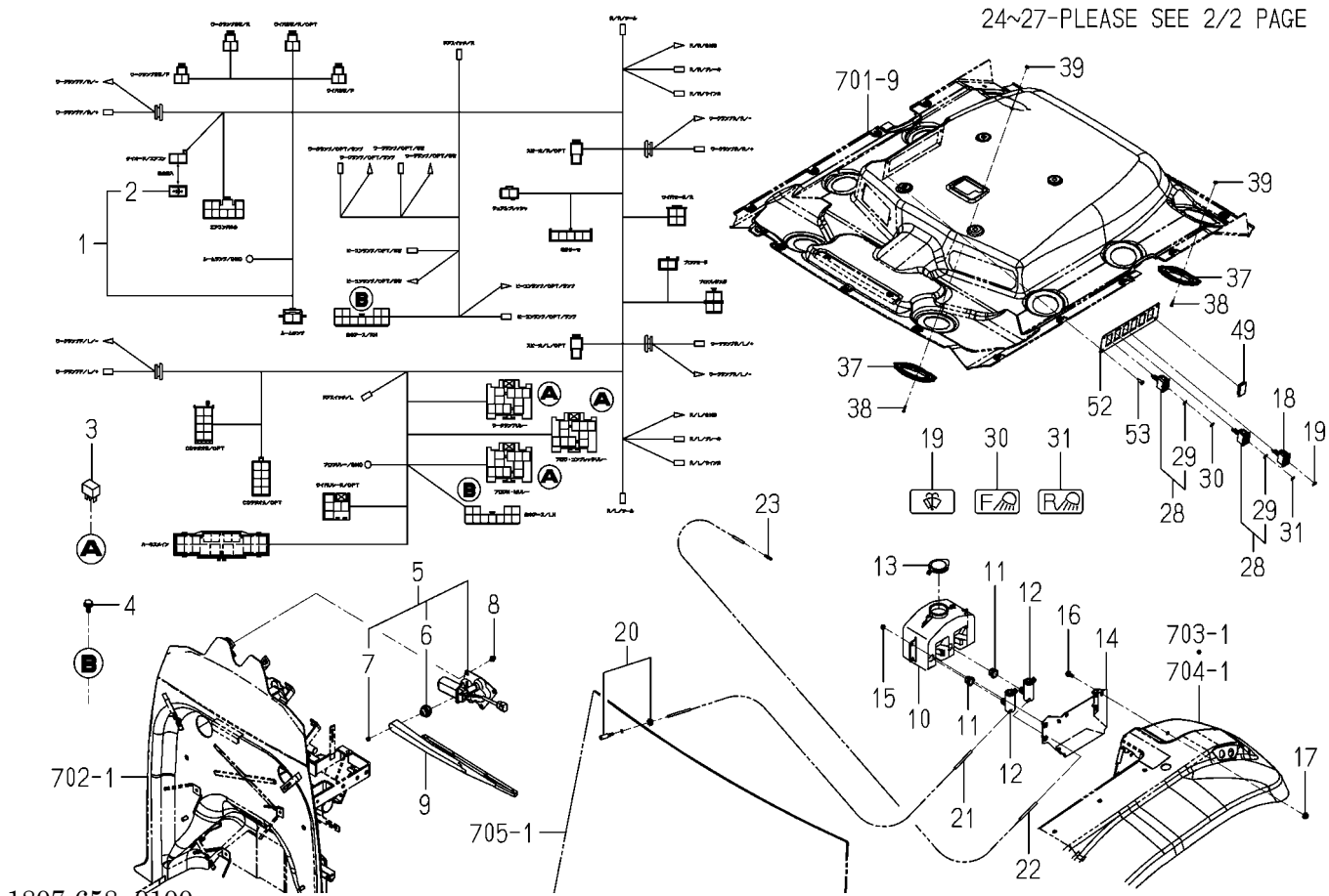
FIG.614 ELC.(CABIN)SYSTEM(1/2)
