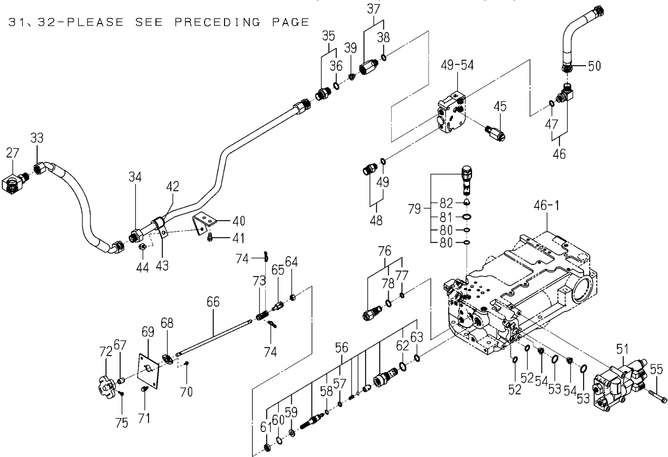
FIG. 48 PIPING (MAIN) SYSTEM(2/2)
