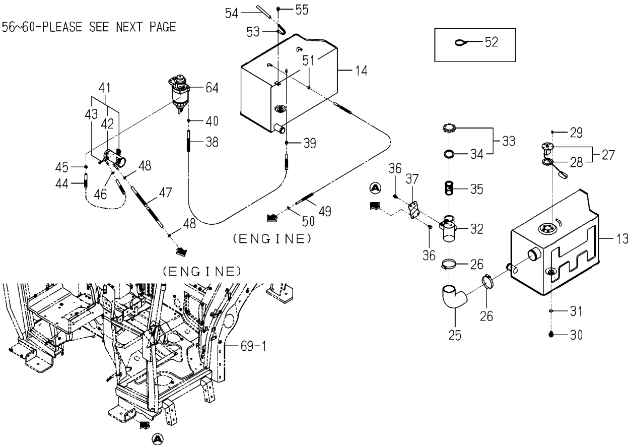
FIG. 4 TANK (FUEL) SYSTEM(2/3)
