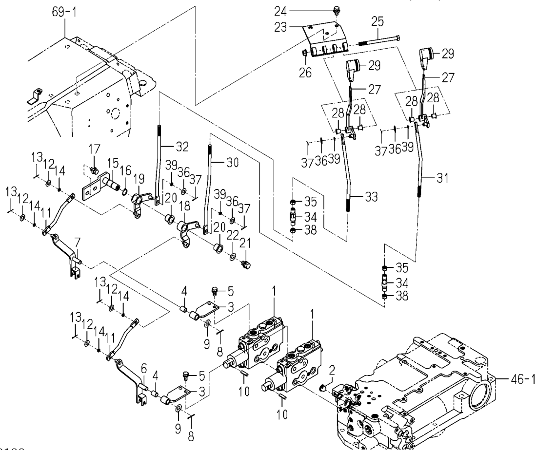
FIG. 50 SUB CONTROL SYSTEM(1/2)
