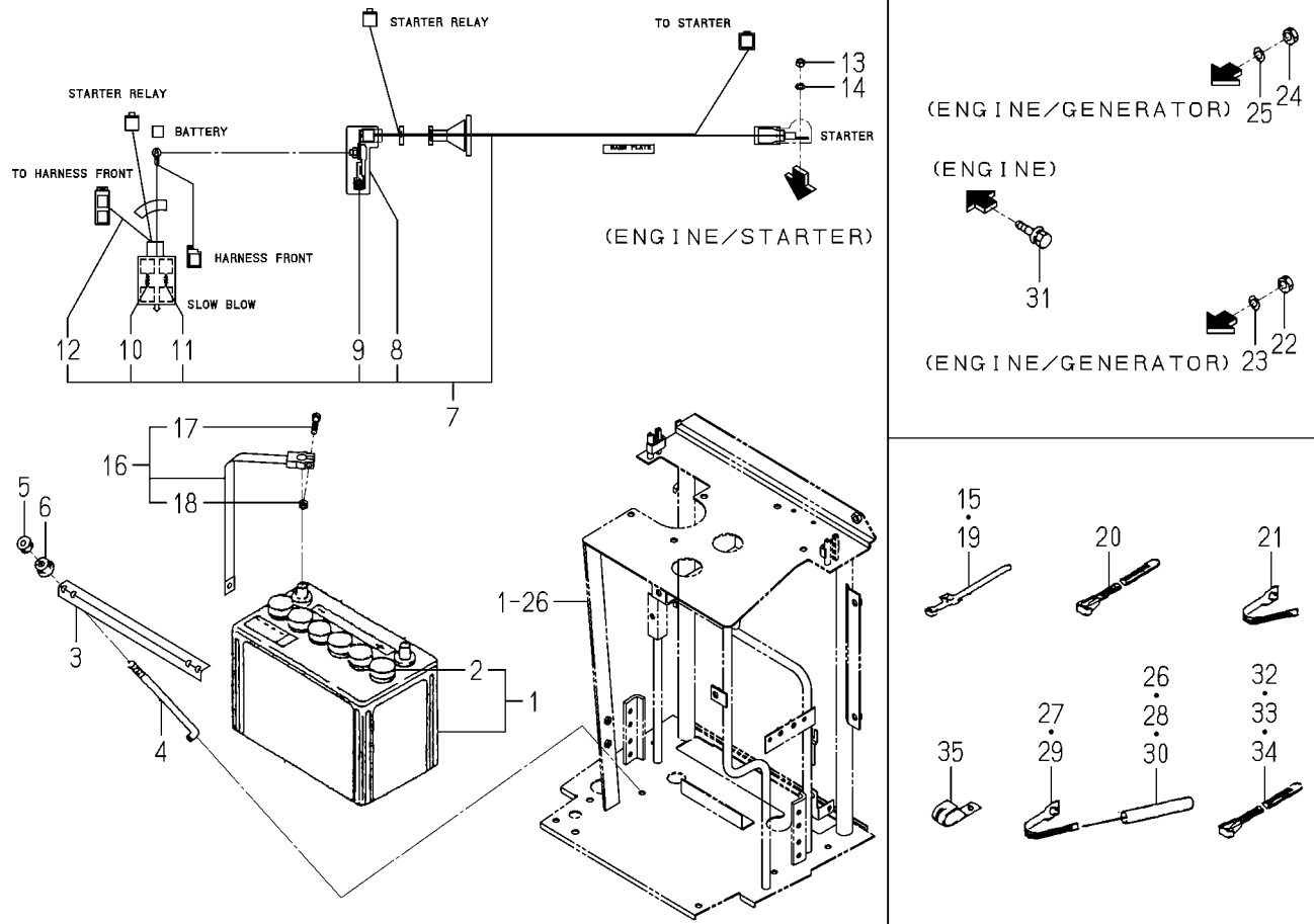
FIG. 62 ELC. SYSTEM (FRONT)(1/3)
