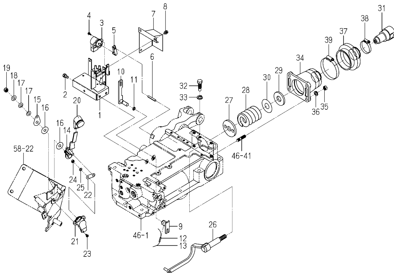
FIG. 47 CONTROL SYSTEM
