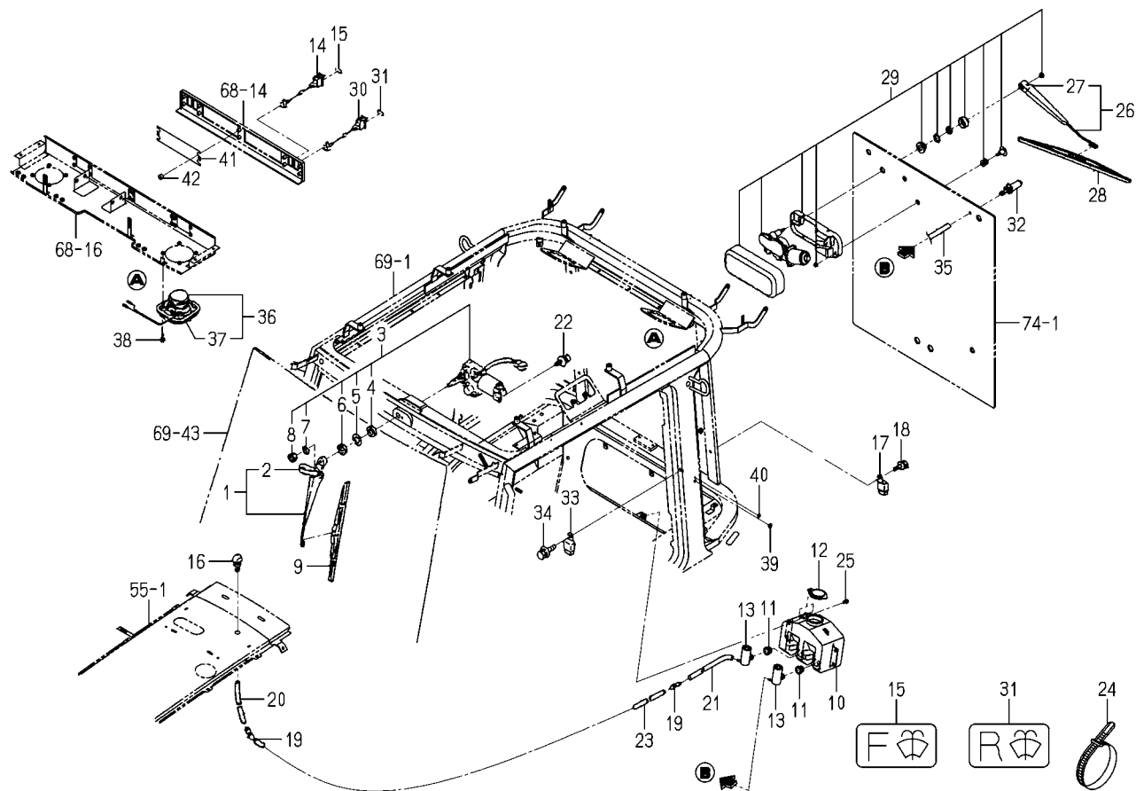
FIG. 66 ELC. SYSTEM (CABIN)(1/2)
