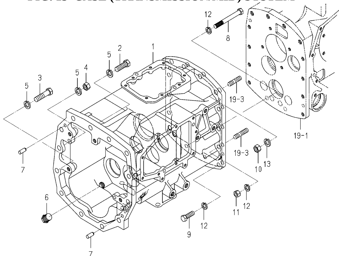
FIG. 15 CASE (TRANSMISSION/MID) SYSTEM
