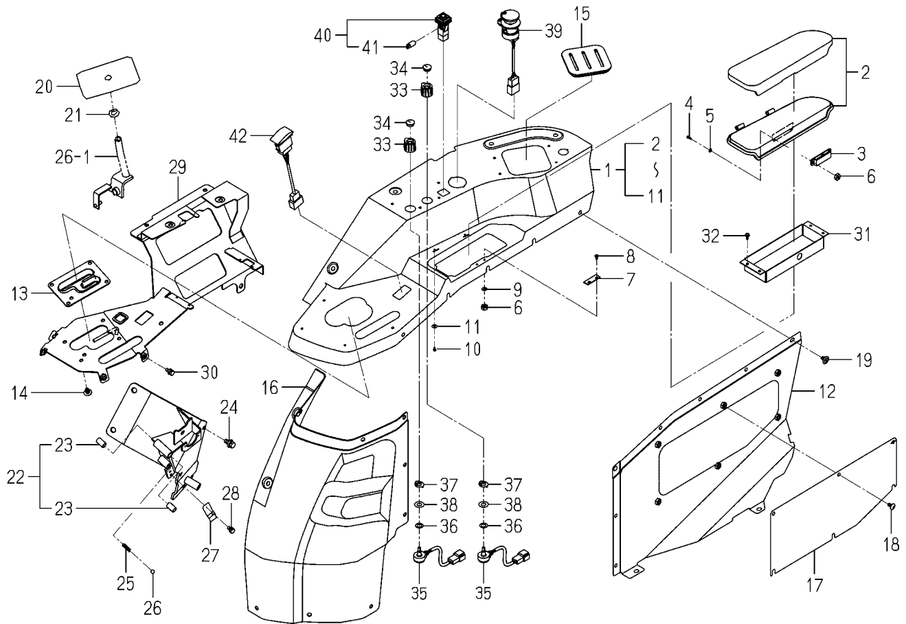
FIG. 58 LEVER GUIDE SYSTEM
