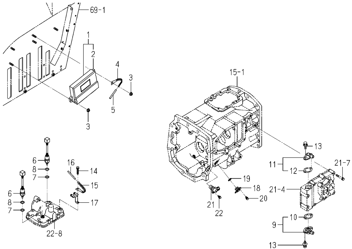
FIG. 67 ELC. SYSTEM
