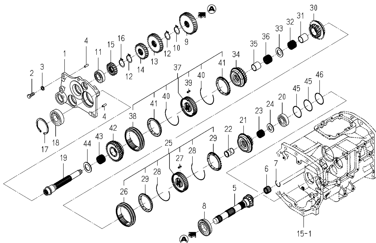
FIG. 16 GEAR (MAIN) SYSTEM
