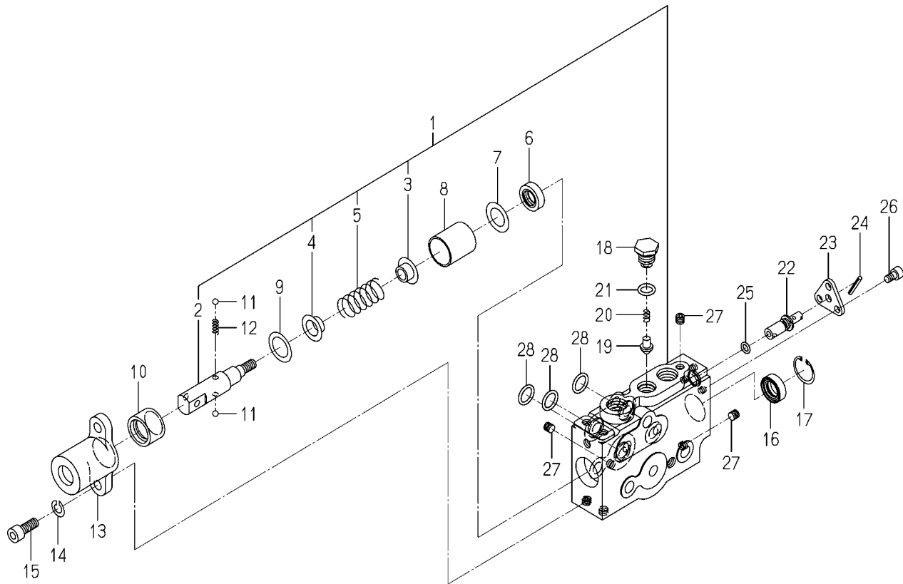
FIG. 91 COMPONENT PARTS FOR 1640-530-600-10 ON Fig.85
