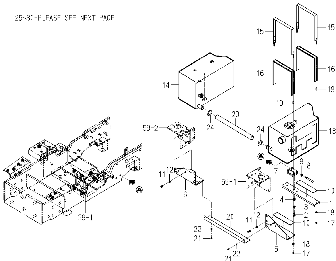
FIG. 4 TANK (FUEL) SYSTEM(1/3)
