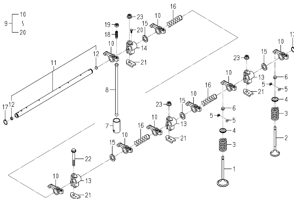
FIG. 12 VALVE
