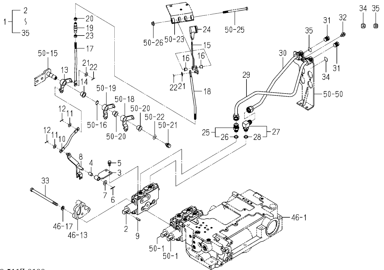
FIG. 85 SUB CONTROL (3) SYSTEM (OPTION)
