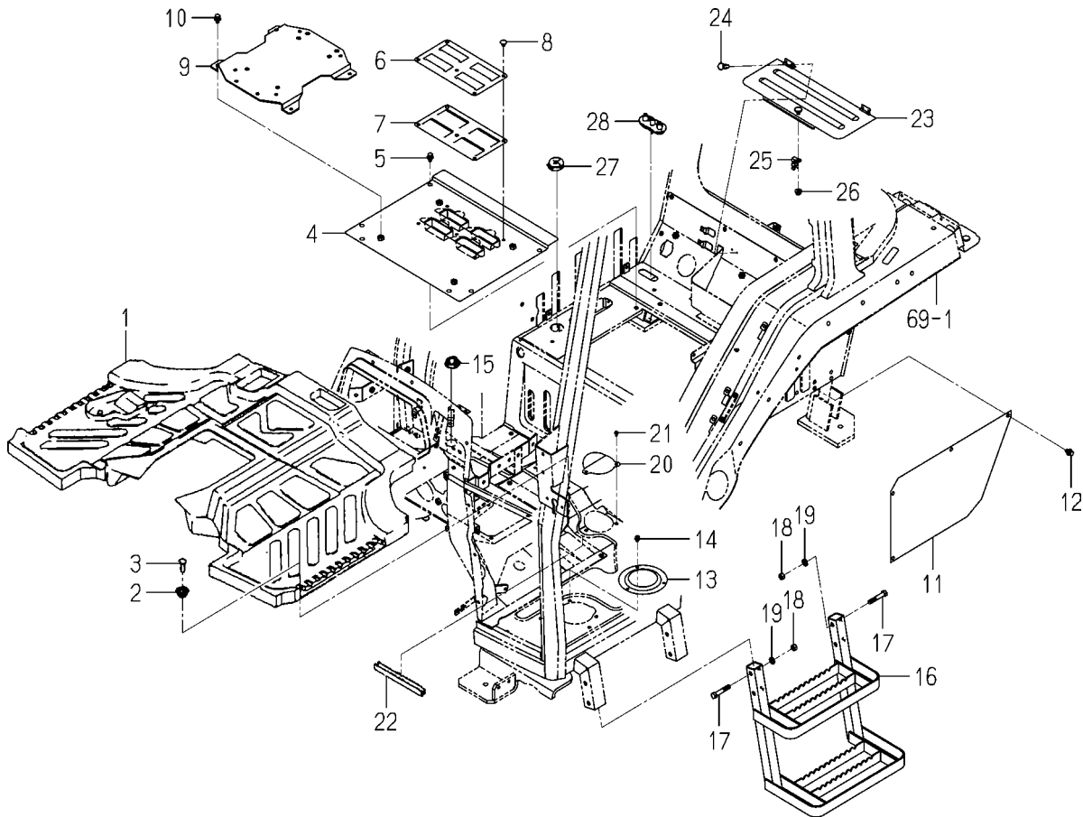
FIG. 61 FLOOR (REAR) SYSTEM
