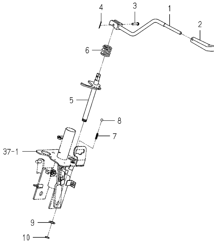
FIG. 25 LEVER (REVERSE) SYSTEM
