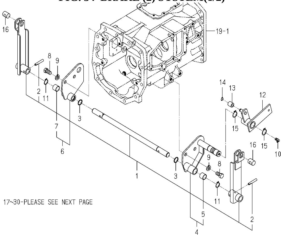
FIG. 34 BRAKE (2) SYSTEM(1/2)
