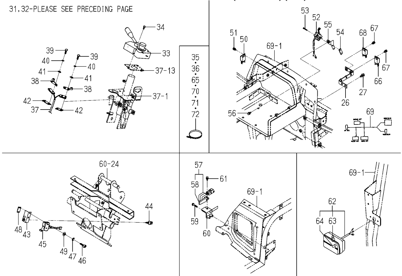
FIG. 63 ELC. SYSTEM (PANEL)(2/2)
