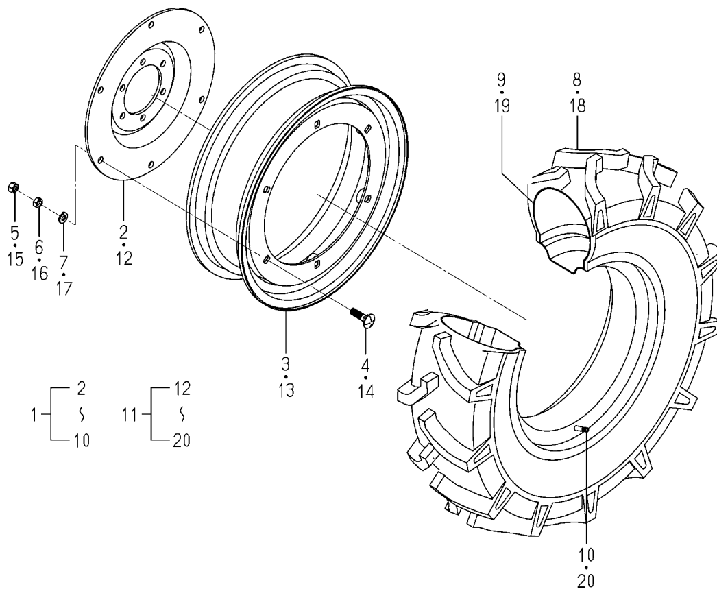
FIG. 84 WHEEL (FRONT) SYSTEM (OPTION)
