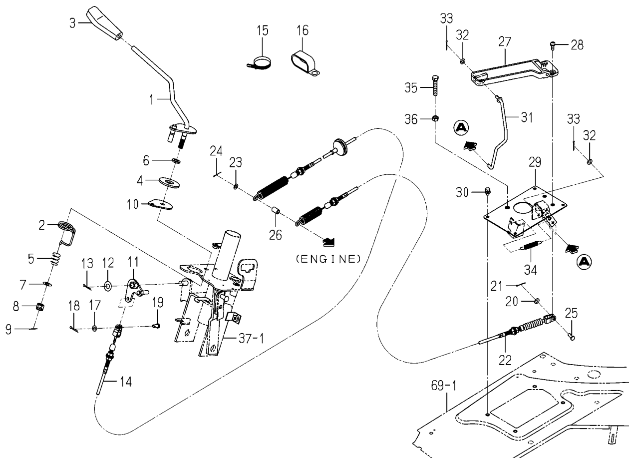
FIG. 5 ACCELERATOR SYSTEM
