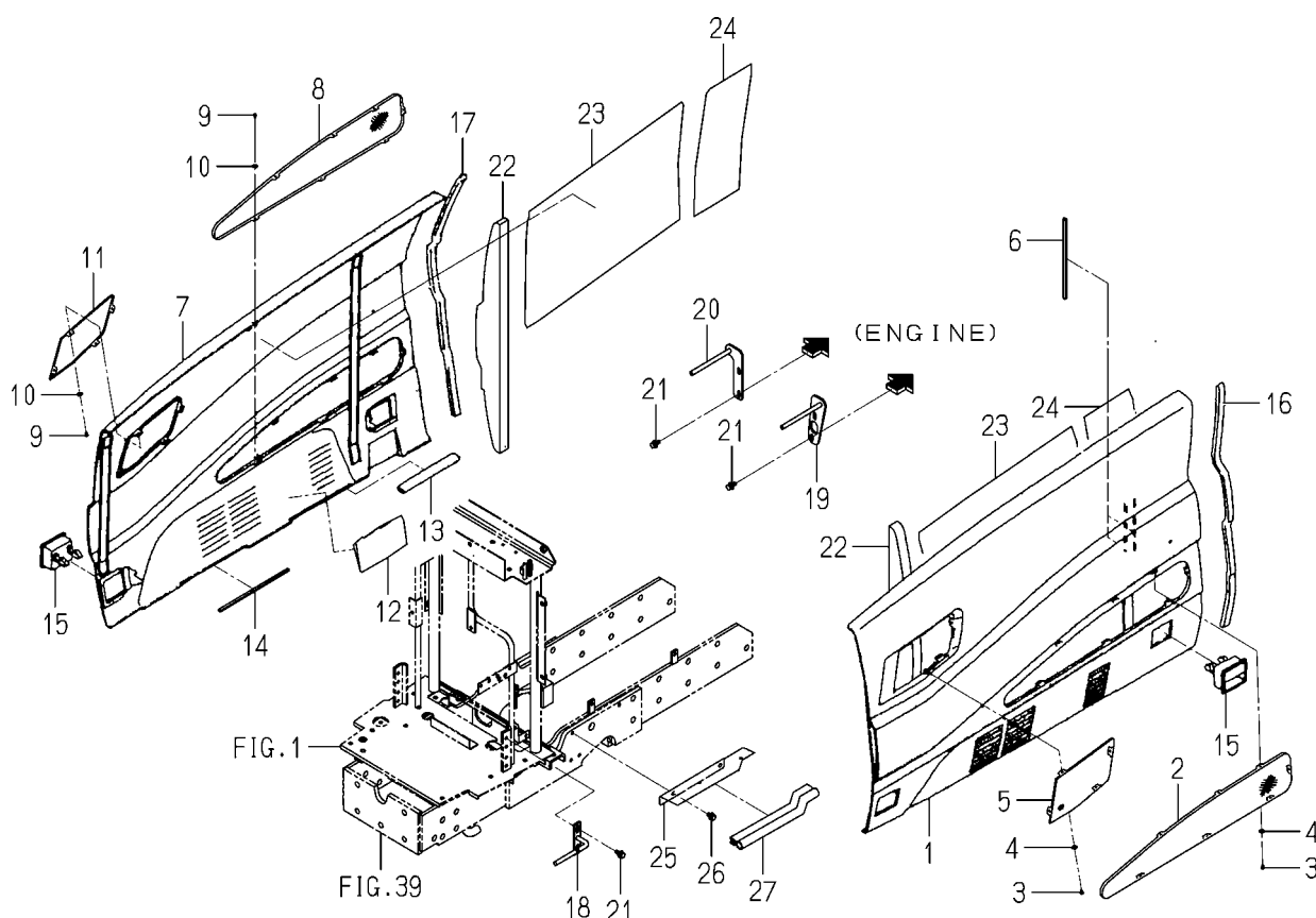
FIG. 57 COVER (SIDE) SYSTEM
