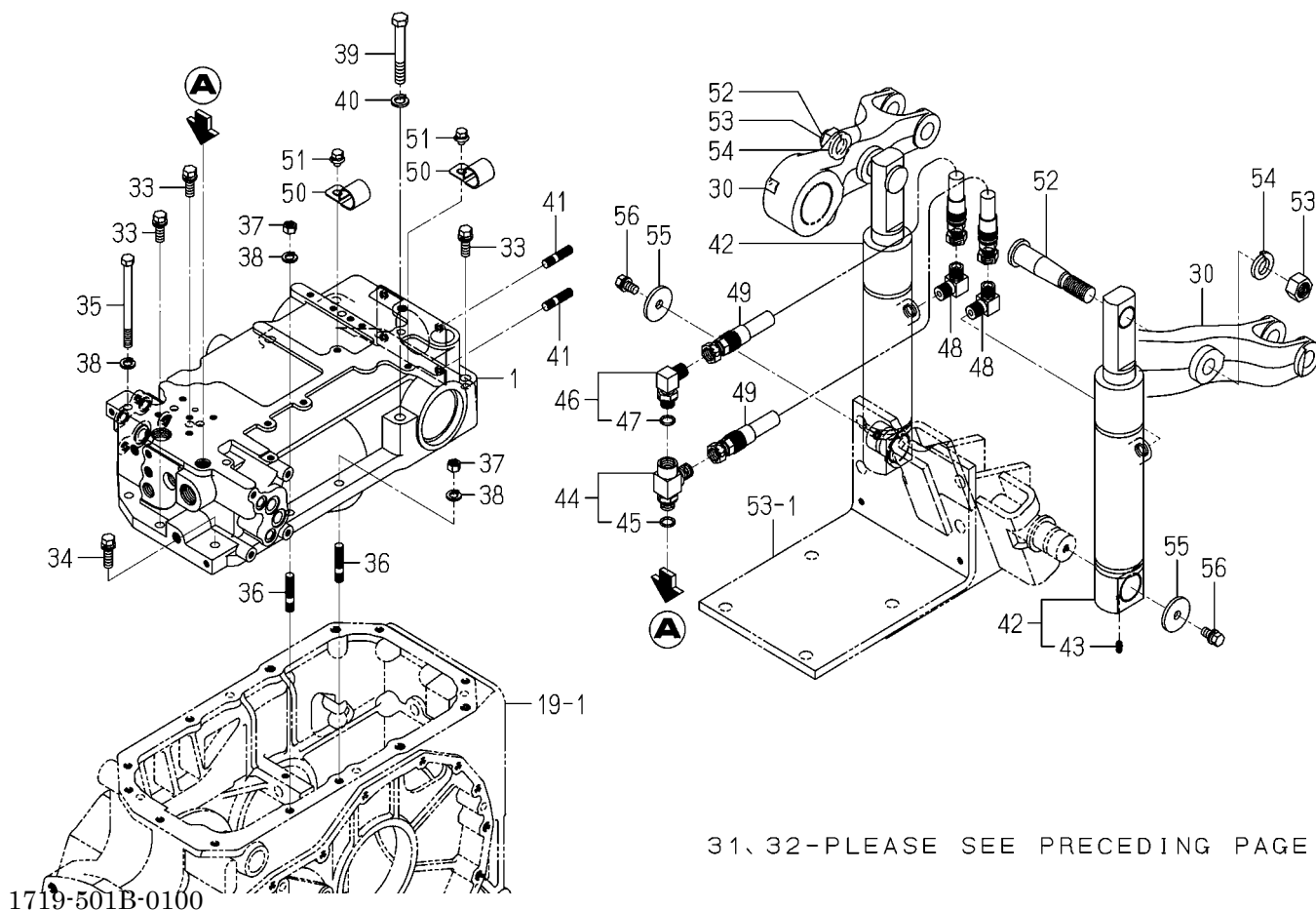
FIG. 46 CASE (CYLINDER) SYSTEM(2/2)
