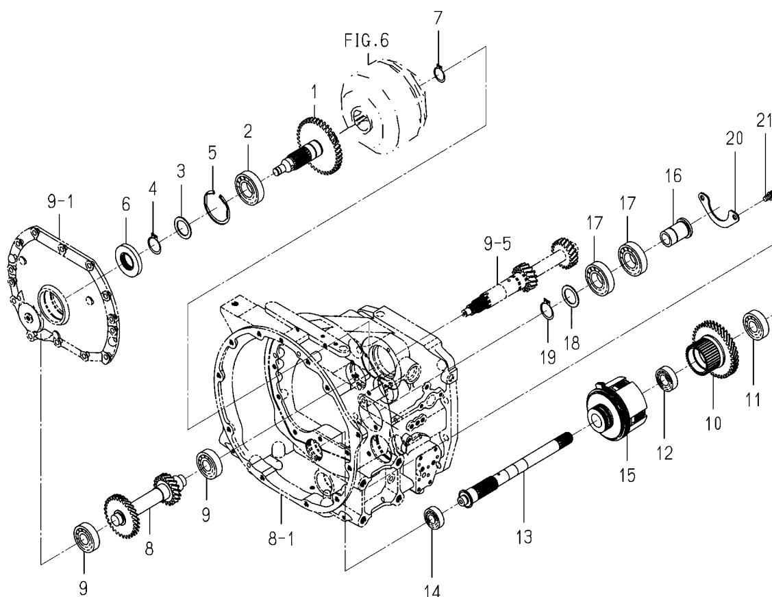
FIG. 10 GEAR (PTO) SYSTEM
