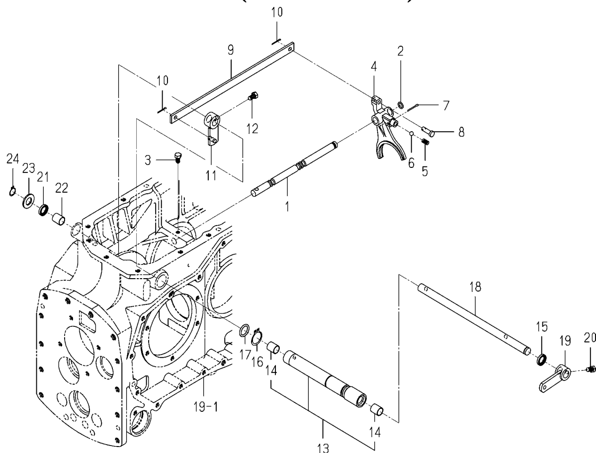
FIG. 24 FORK (SHIFT/PTO/2ND) SYSTEM
