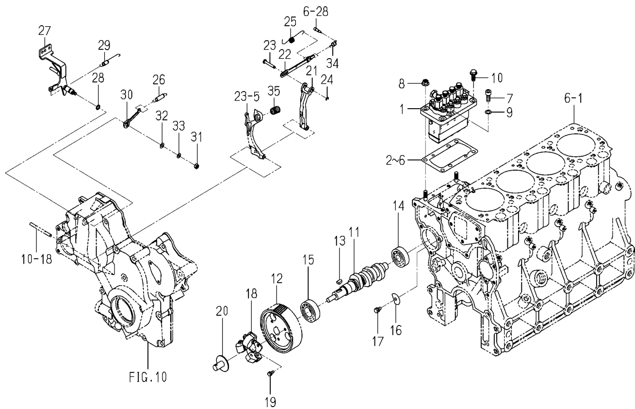
FIG. 21 INJECTION PUMP
