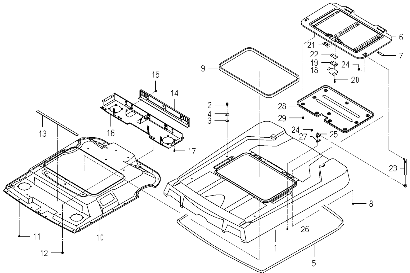
FIG. 68 ROOF SYSTEM
