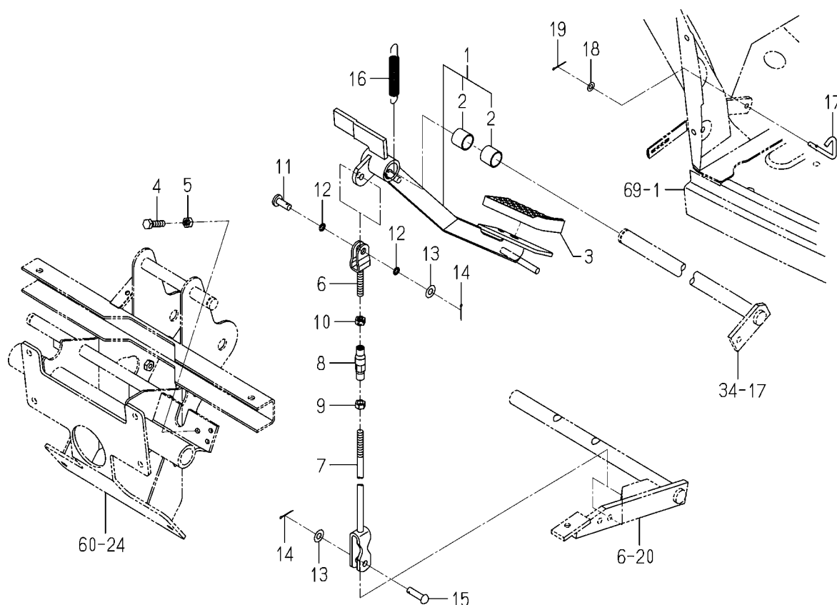
FIG. 7 PEDAL (CLUTCH) SYSTEM
