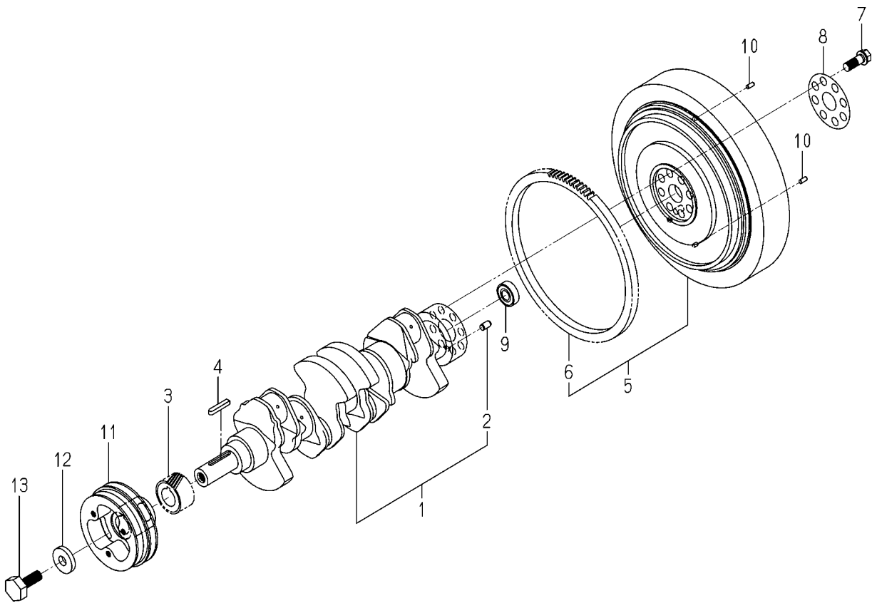
FIG. 16 CRANK SHAFT
