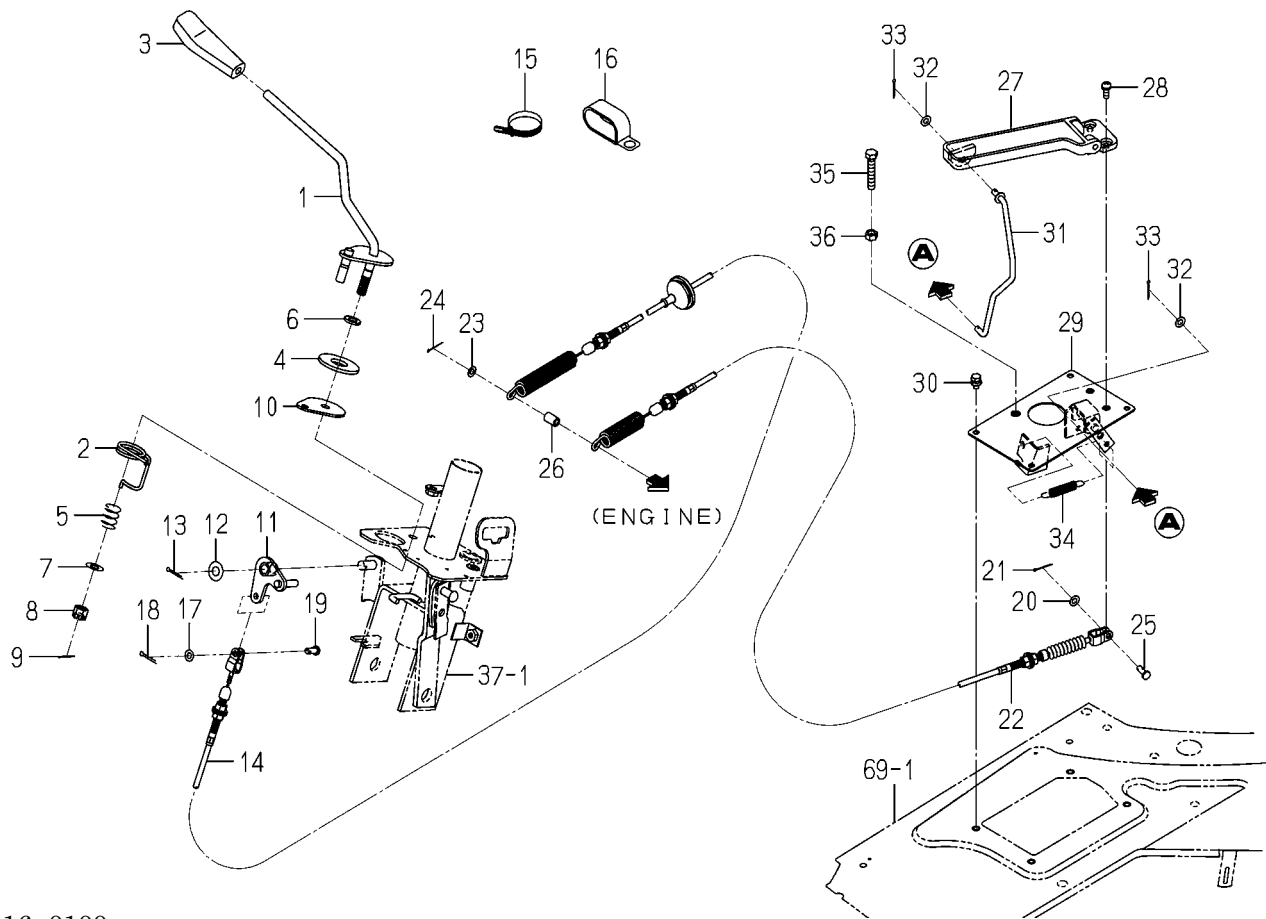
FIG. 5 ACCELERATOR SYSTEM
