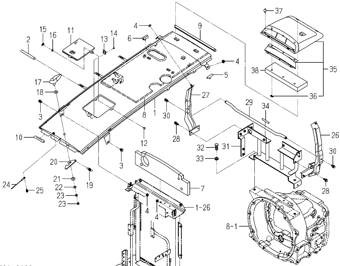
FIG. 55 HOOD SYSTEM
