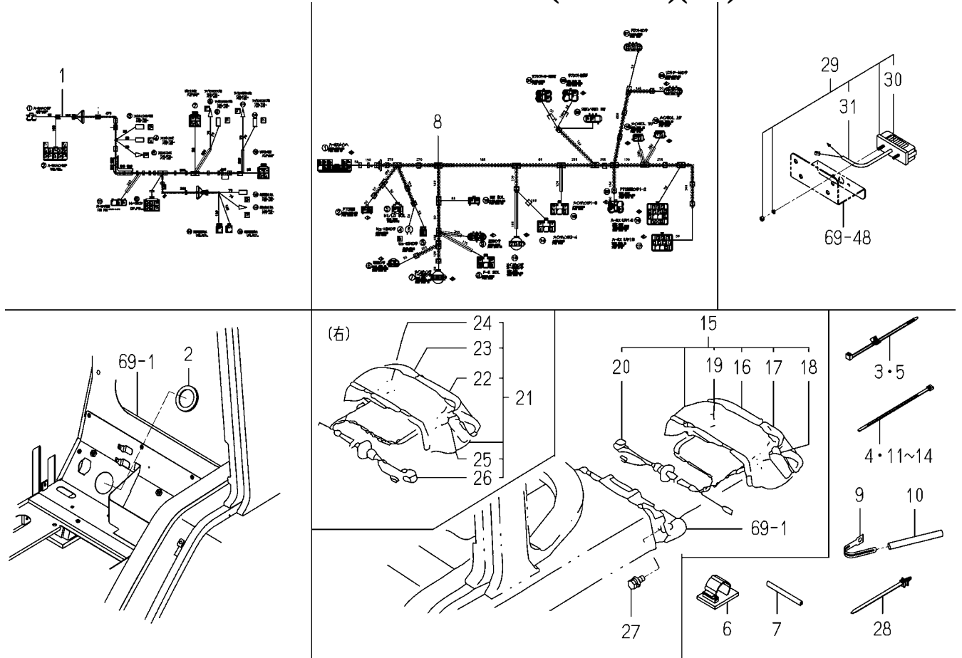
FIG. 64 ELC. SYSTEM (FLOOR)(1/2)
