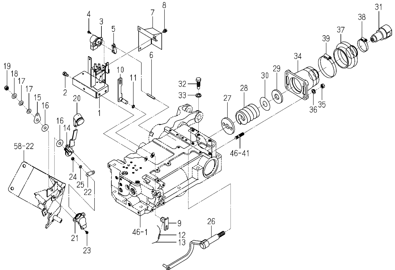
FIG. 47 CONTROL SYSTEM
