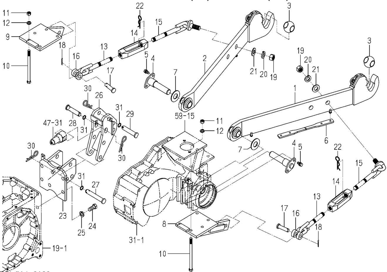
FIG. 51 LINK (3P) SYSTEM(1/2)
