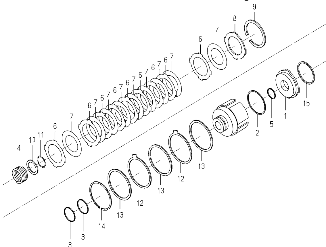
FIG. 93 COMPONENT PARTS FOR 1719-209-200-20 ON Fig.10
