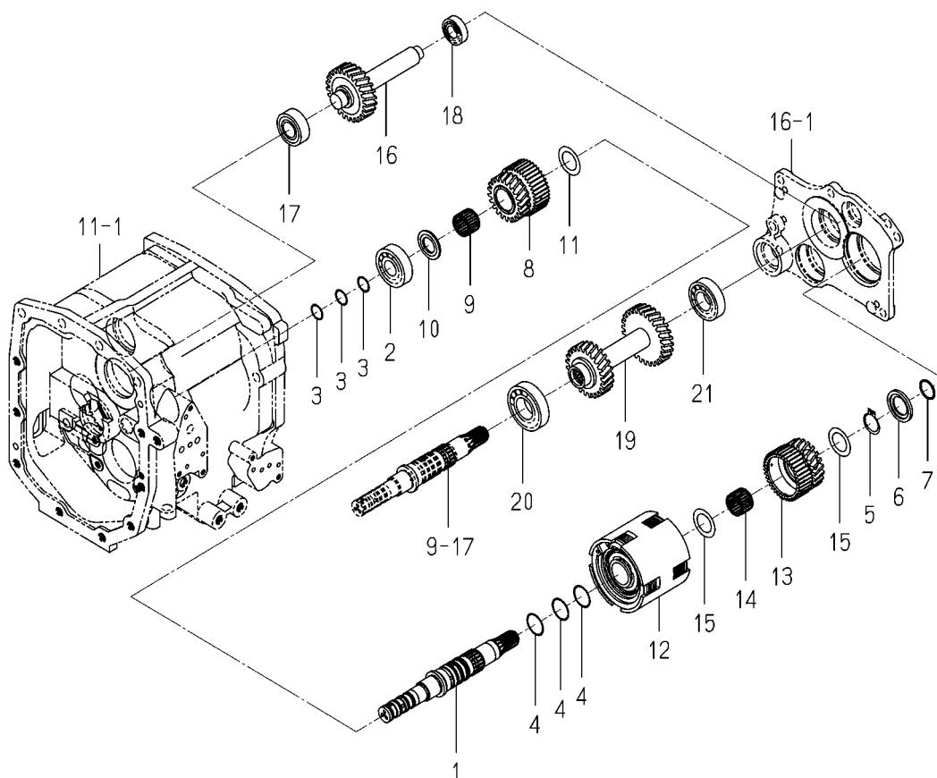
FIG. 12 GEAR (REVERSE) SYSTEM
