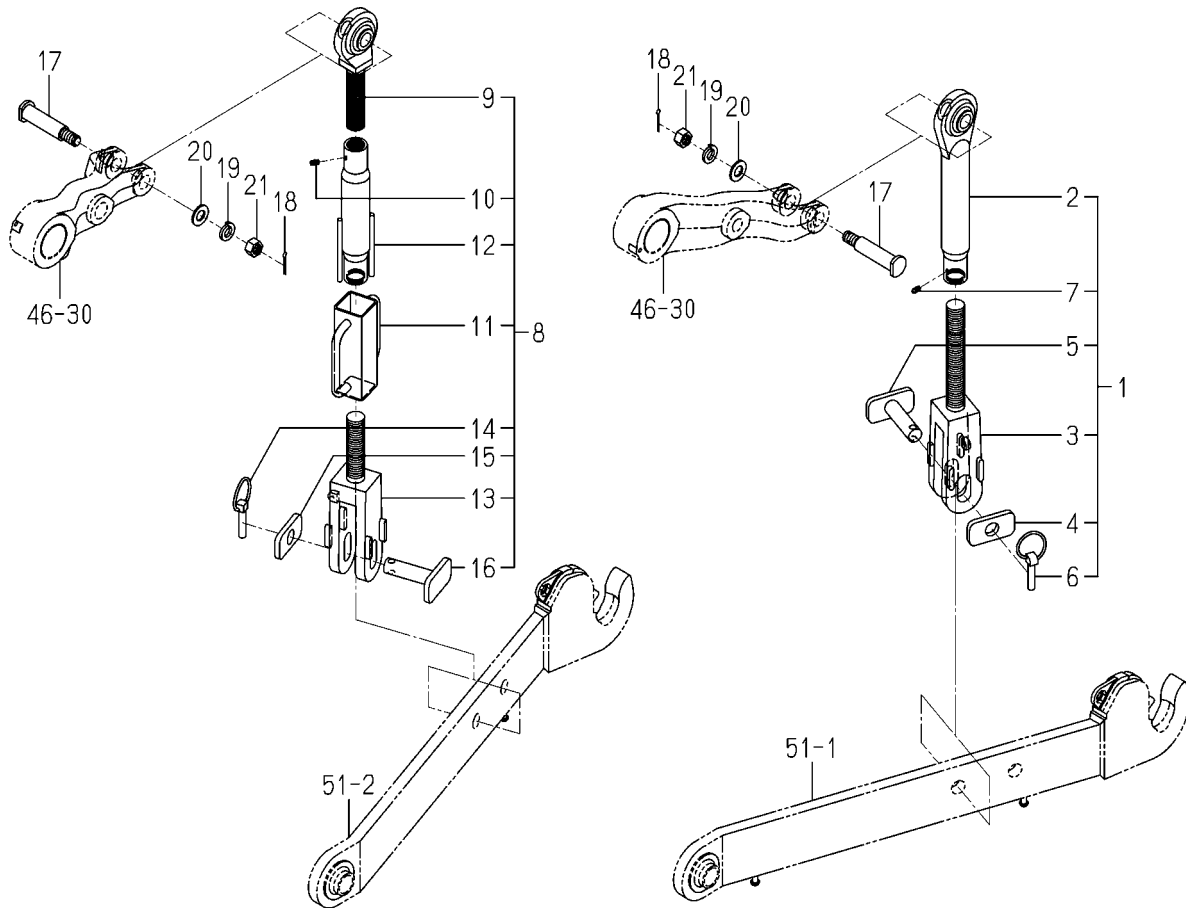
FIG. 52 ROD (LIFT) SYSTEM
