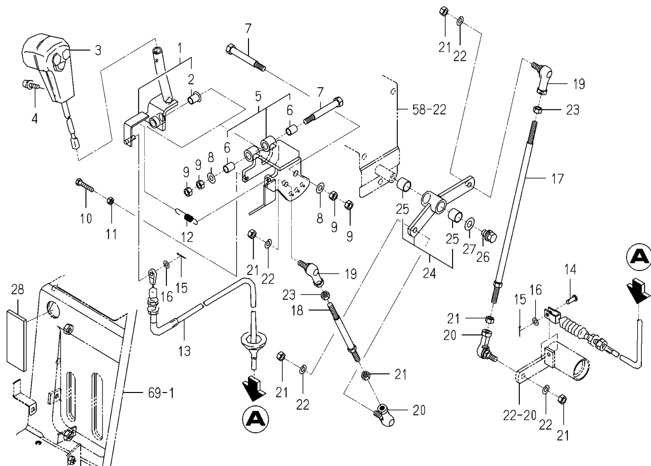
FIG. 26 LEVER (SHIFT/SUB) SYSTEM
