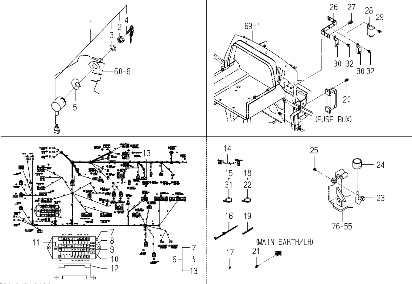
FIG. 63 ELC. SYSTEM (PANEL)(1/2)
