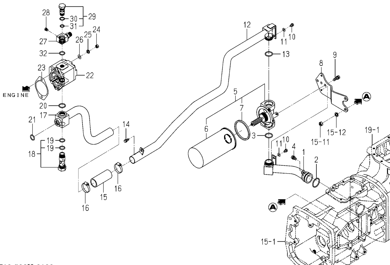
FIG. 48 PIPING (MAIN) SYSTEM(1/2)
