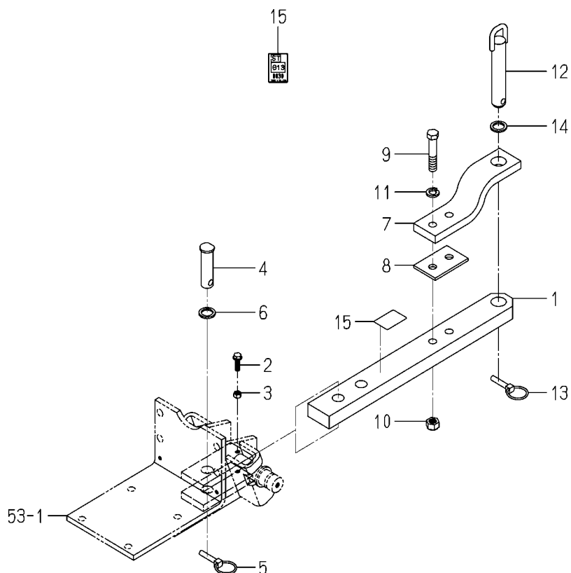
FIG. 54 DRAW BAR SYSTEM
