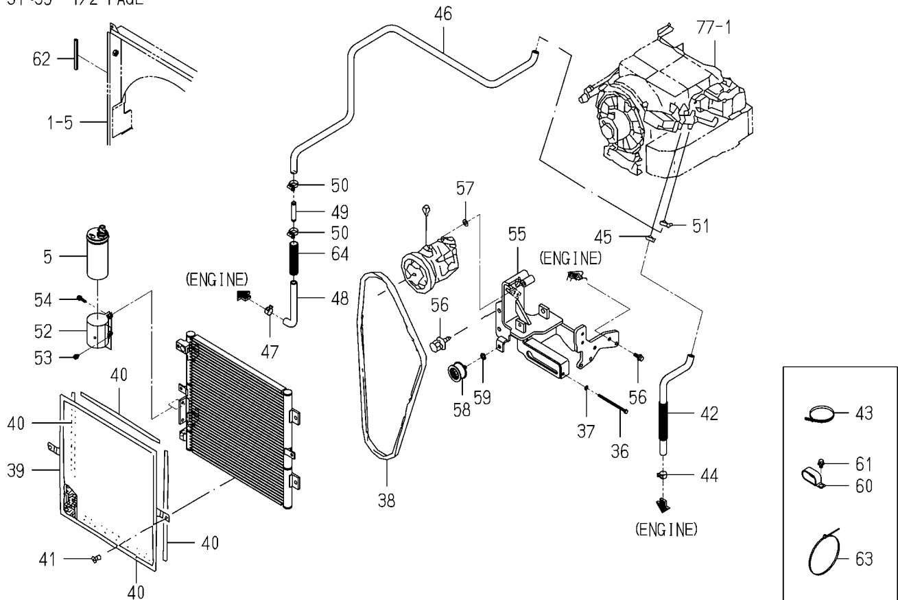
FIG. 76 AIR CONDITIONER (ENGINE) SYSTEM(2/2)
