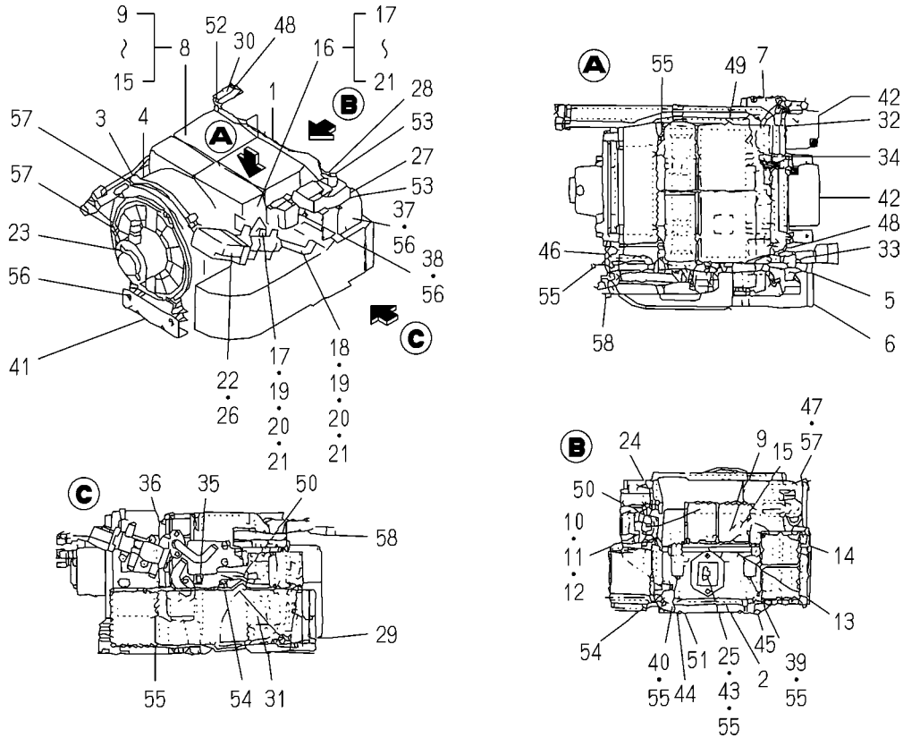
FIG. 96 COMPONENT PARTS FOR 1719-782-510-00 ON Fig.77
