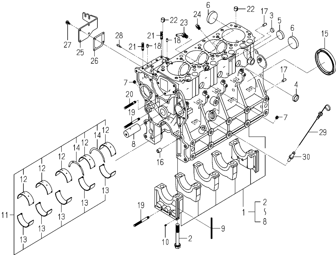
FIG. 6 CYLINDER BLOCK(1/2)
