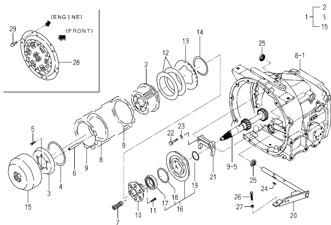
FIG. 6 CLUTCH (MAIN) SYSTEM
