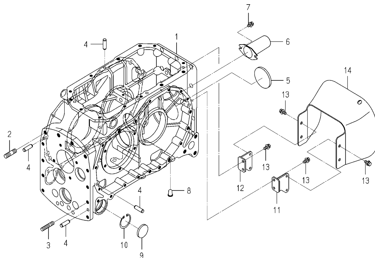
FIG. 19 CASE (TRANSMISSION/REAR) SYSTEM
