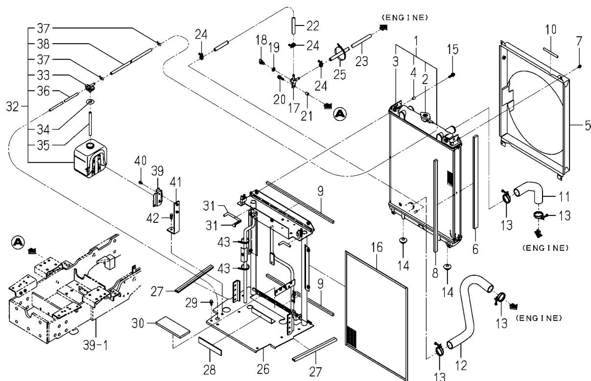
FIG. 1 RADIATOR SYSTEM
