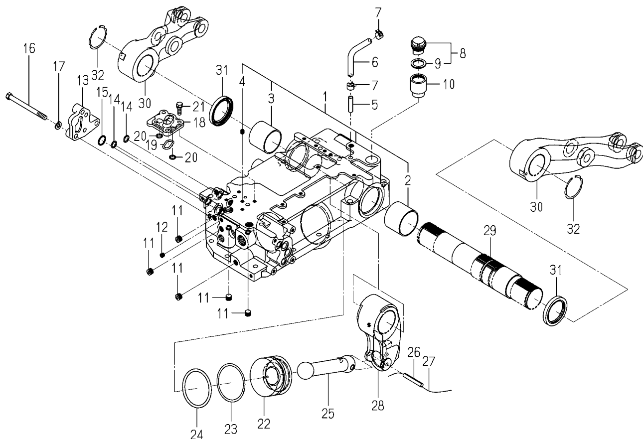
FIG. 46 CASE (CYLINDER) SYSTEM(1/2)
