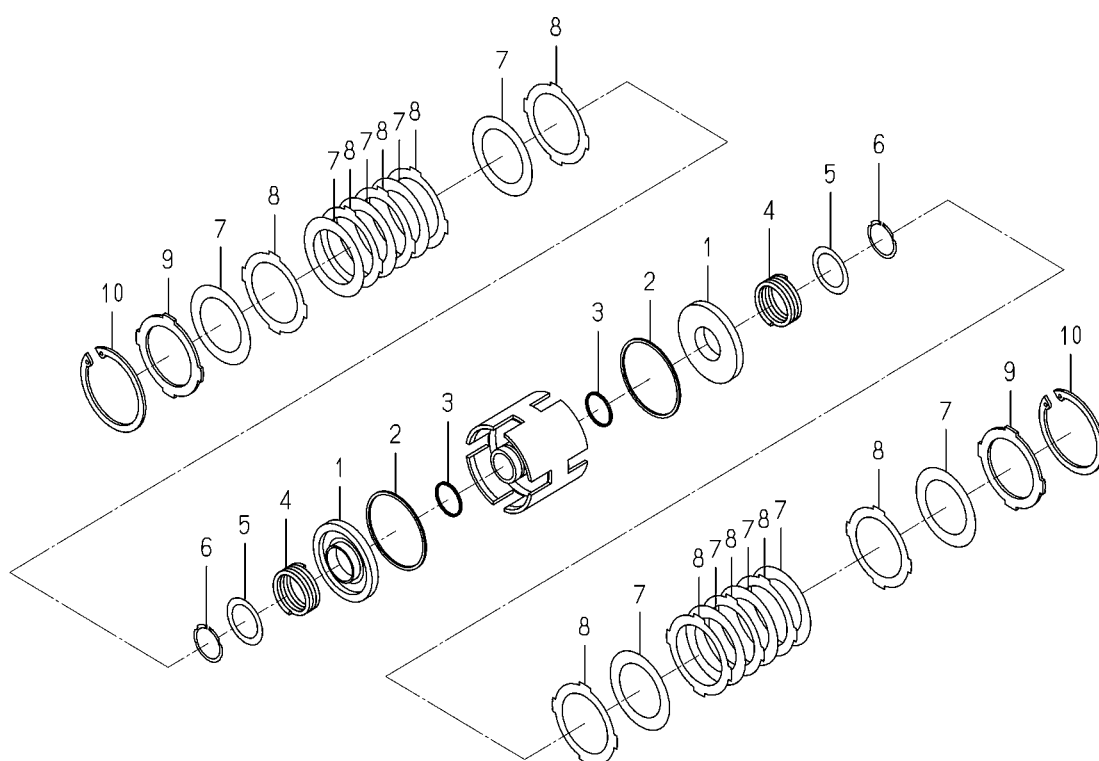
FIG. 92 COMPONENT PARTS FOR 1719-205-220-10 ON Fig.9,12
