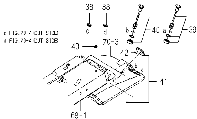
FIG. 64 ELC. SYSTEM (FLOOR)(2/2)
