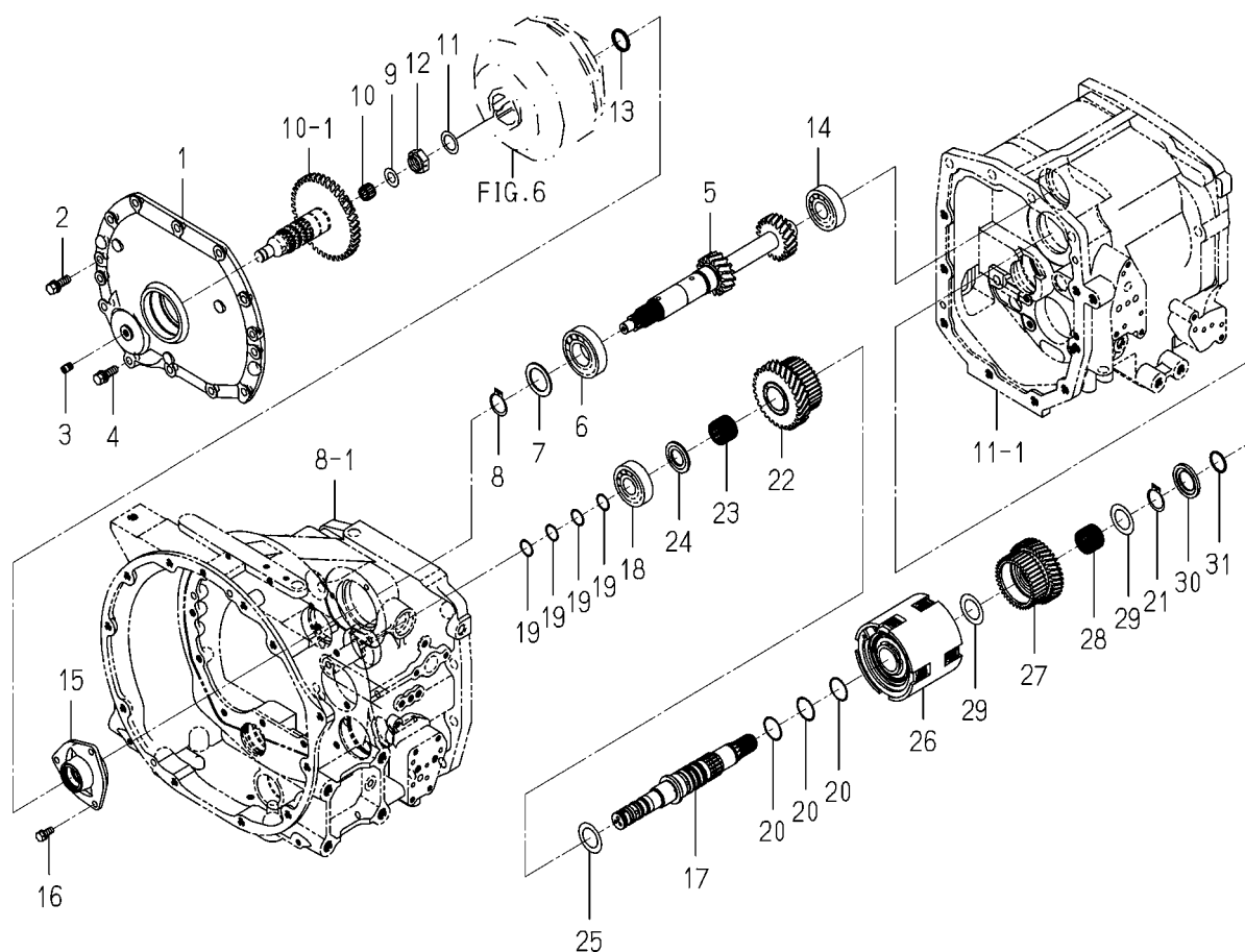
FIG. 9 GEAR (H-L) SYSTEM
