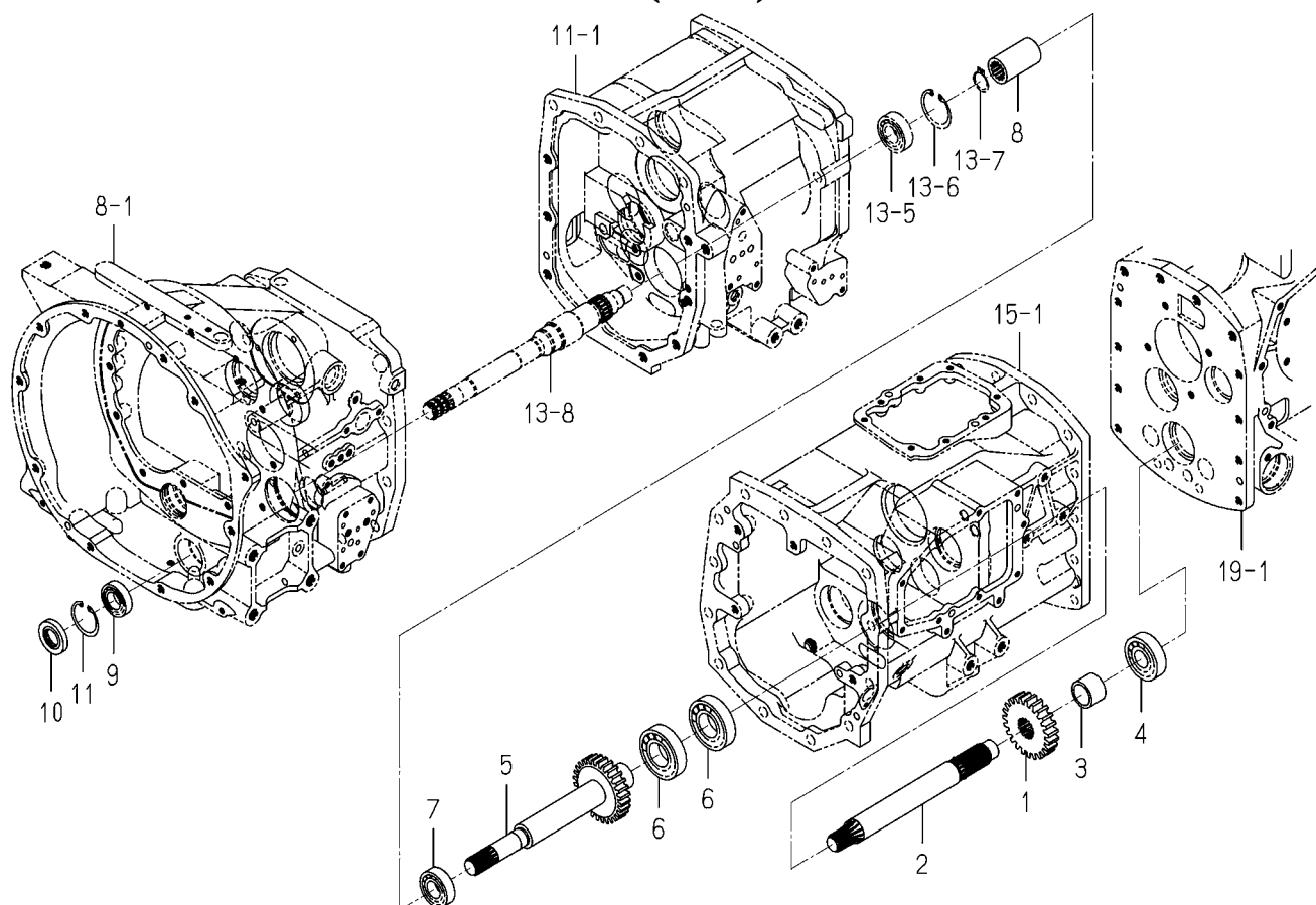
FIG. 18 GEAR (4WD) SYSTEM
