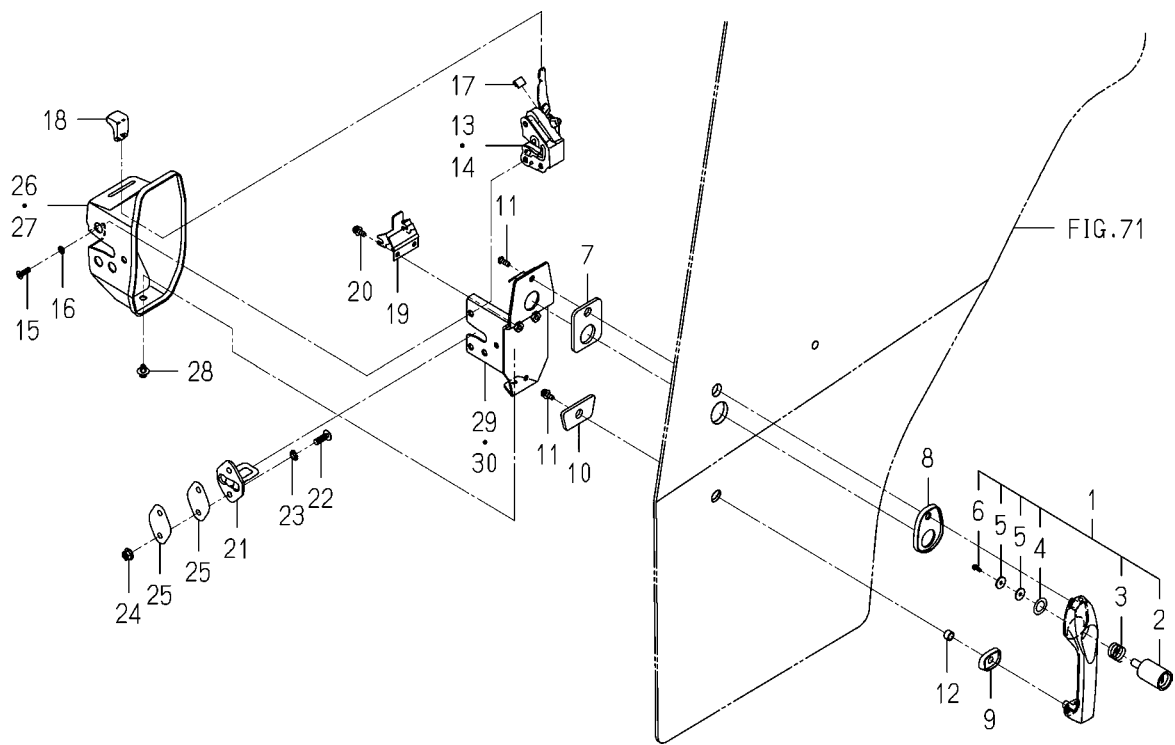
FIG. 72 LOCK (DOOR) SYSTEM
