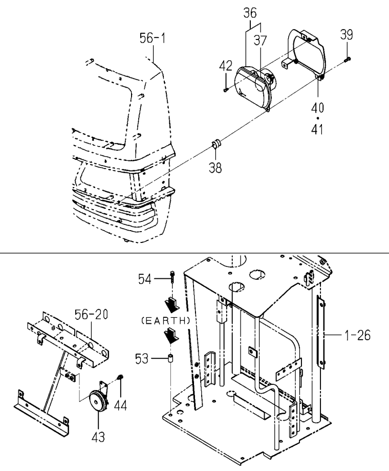
FIG. 62 ELC. SYSTEM (FRONT)(2/3)
