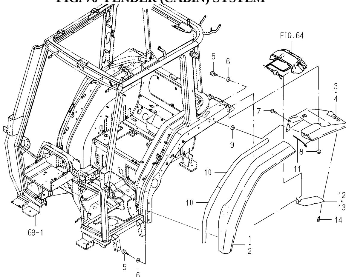
FIG. 70 FENDER (CABIN) SYSTEM
