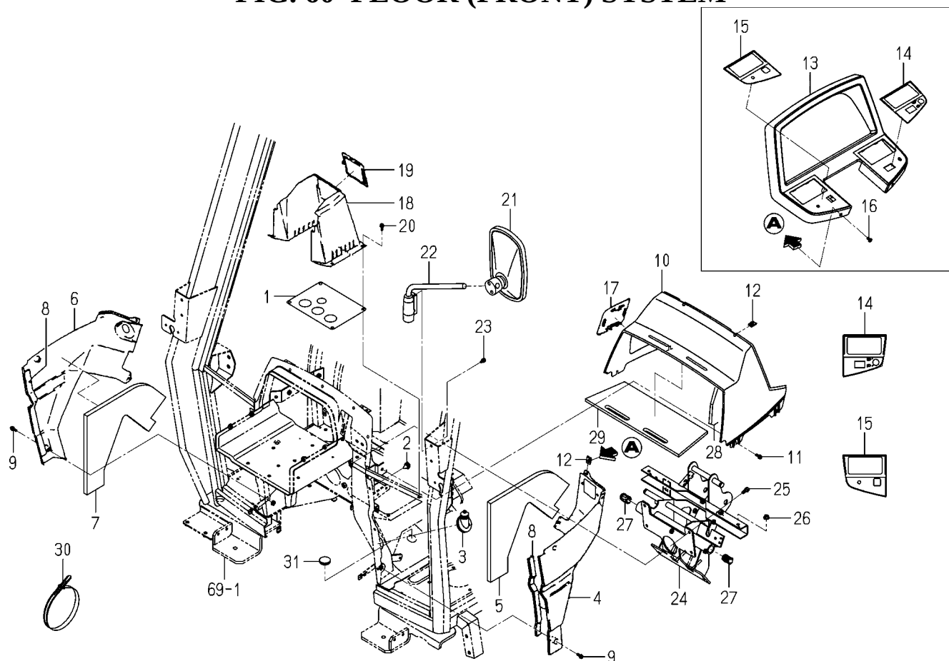
FIG. 60 FLOOR (FRONT) SYSTEM
