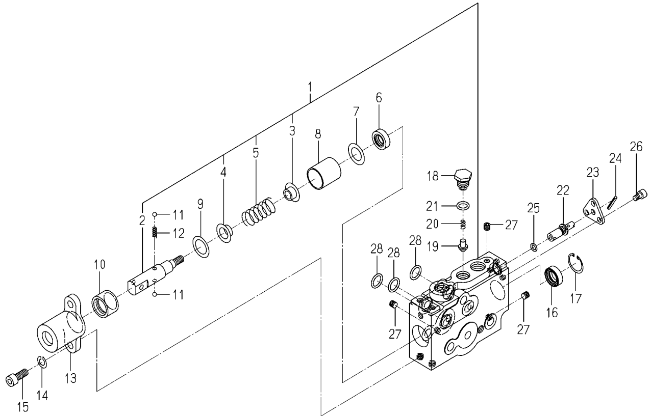
FIG. 94 COMPONENT PARTS FOR 1719-511-350-00 ON Fig.50
