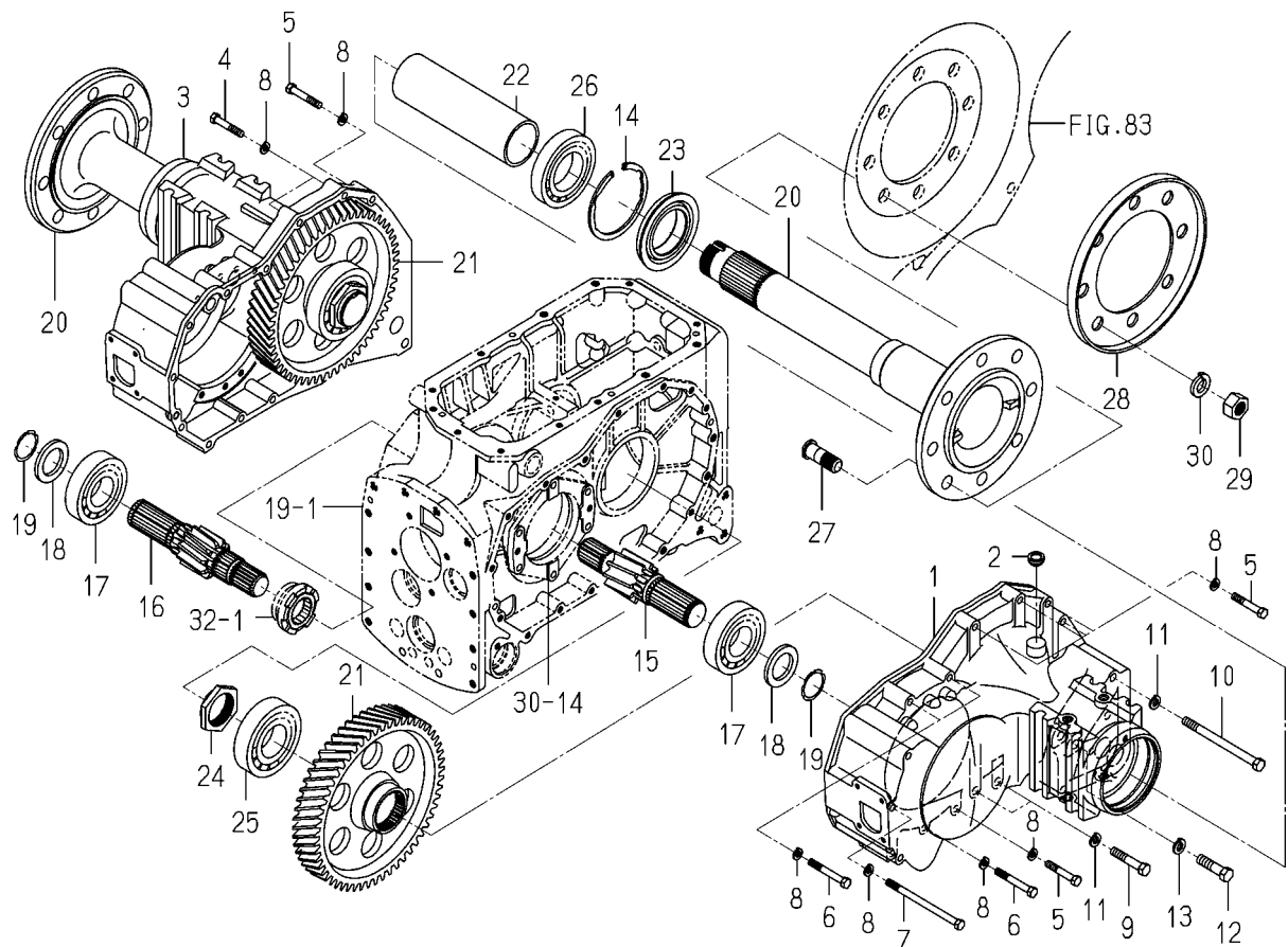
FIG. 31 HOUSING (AXLE/REAR) SYSTEM
