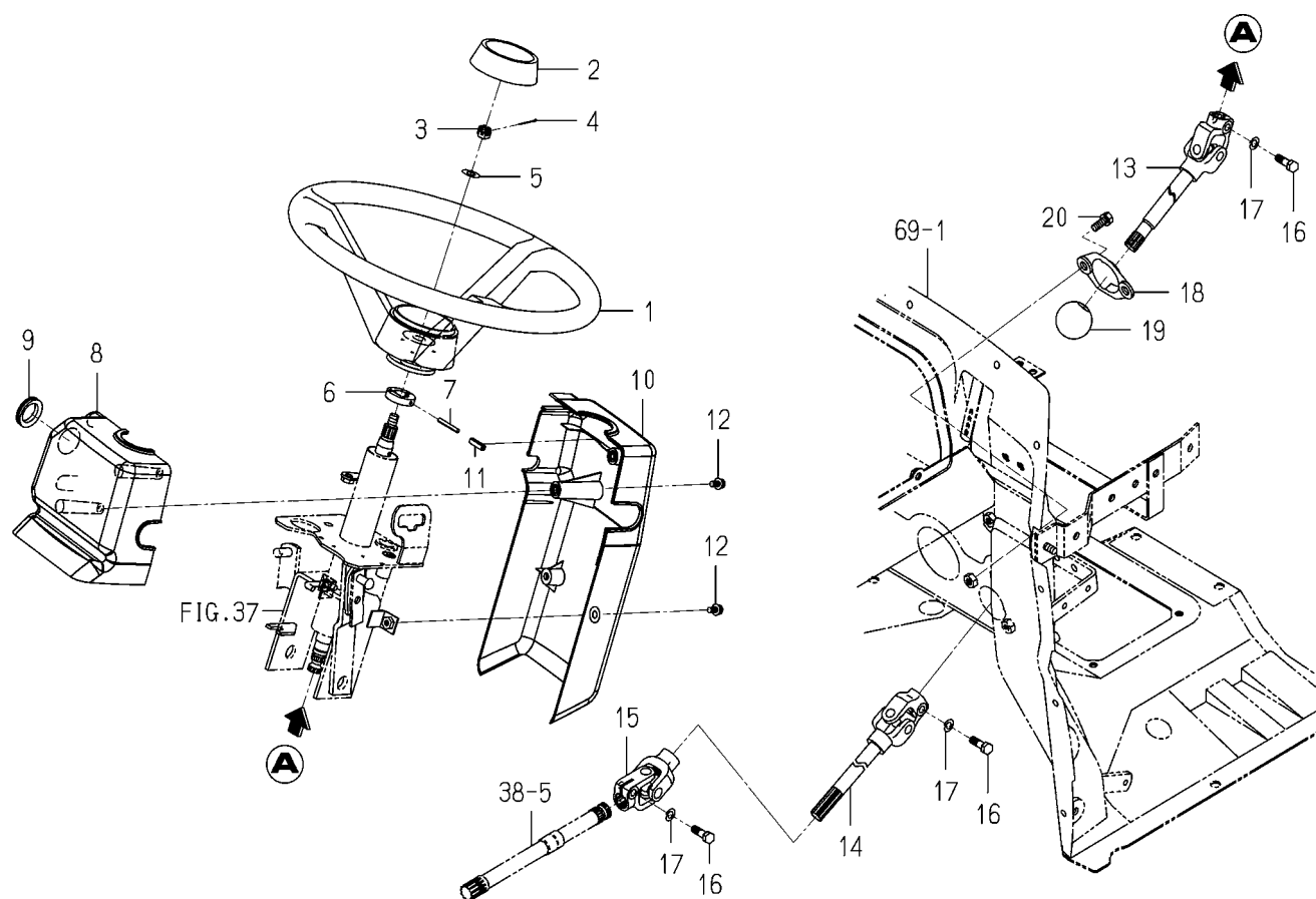
FIG. 36 WHEEL (STEERING) SYSTEM
