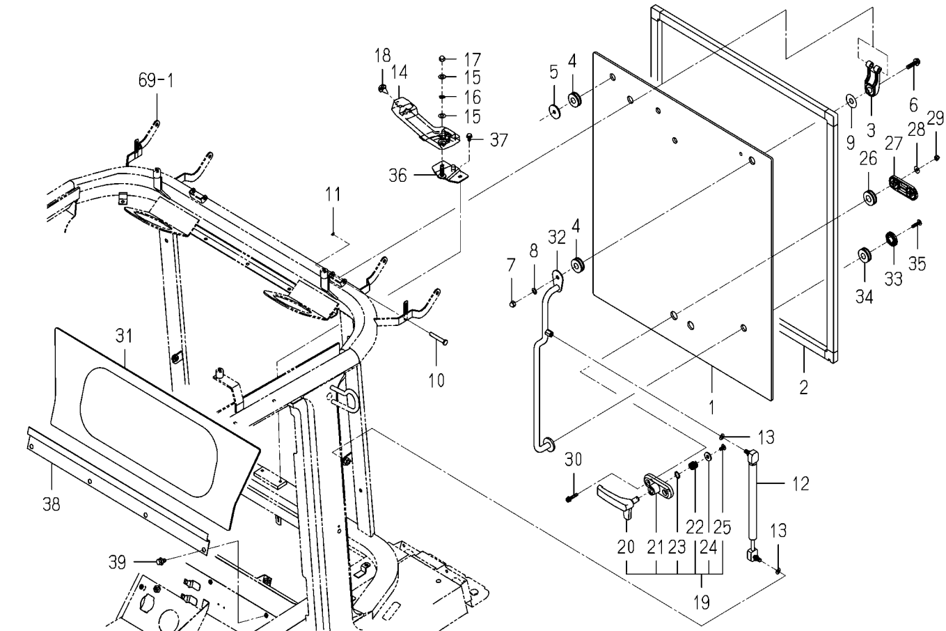
FIG. 74 GLASS (REAR) SYSTEM
