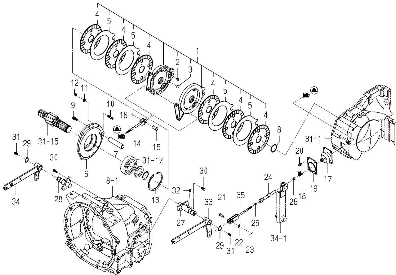
FIG. 33 BRAKE (1) SYSTEM
