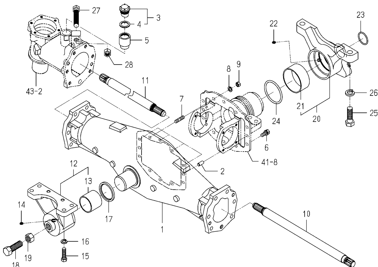
FIG. 42 HOUSING (AXLE) SYSTEM
