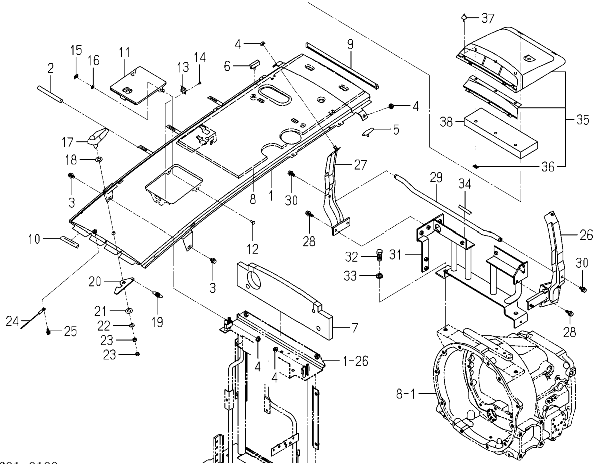
FIG. 55 HOOD SYSTEM
