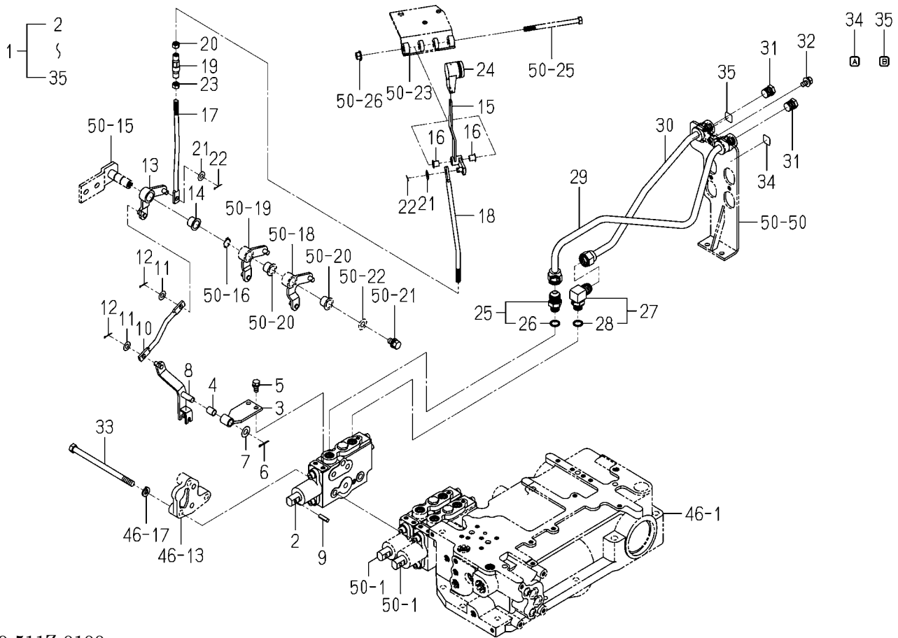
FIG. 85 SUB CONTROL (3) SYSTEM (OPTION)
