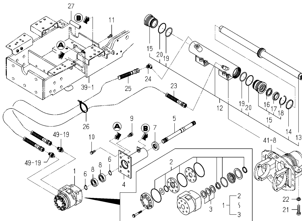
FIG. 38 STEERING (POWER) SYSTEM
