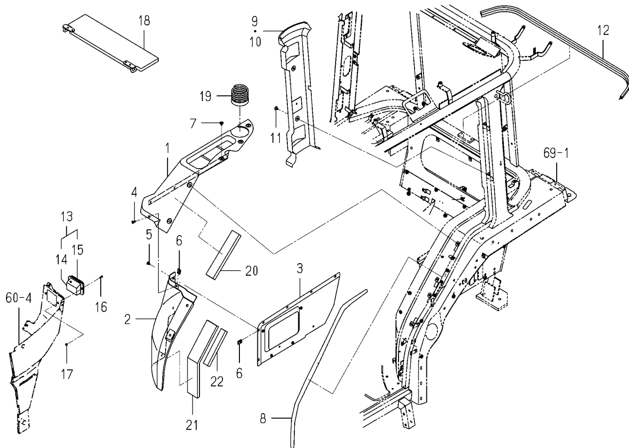
FIG. 75 INTERIOR SYSTEM
