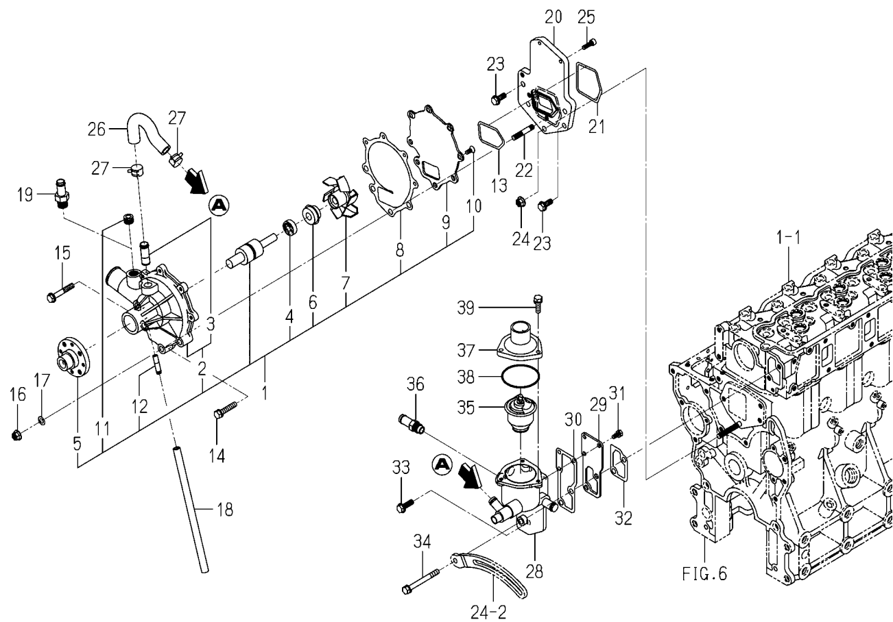
FIG. 18 WATER PUMP
