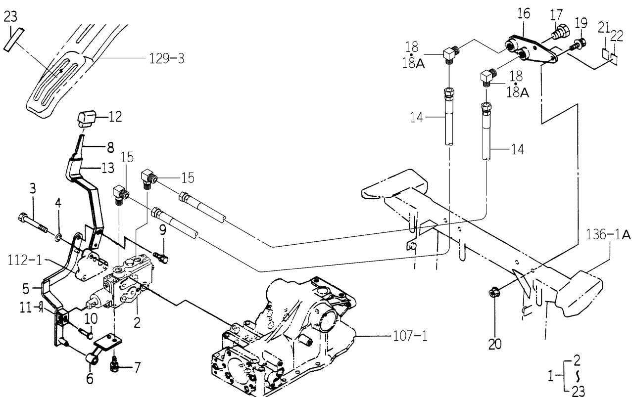
FIG.182 VALVE (STACK/R1) SET (EXCEPT W TYPE-OPTION)
