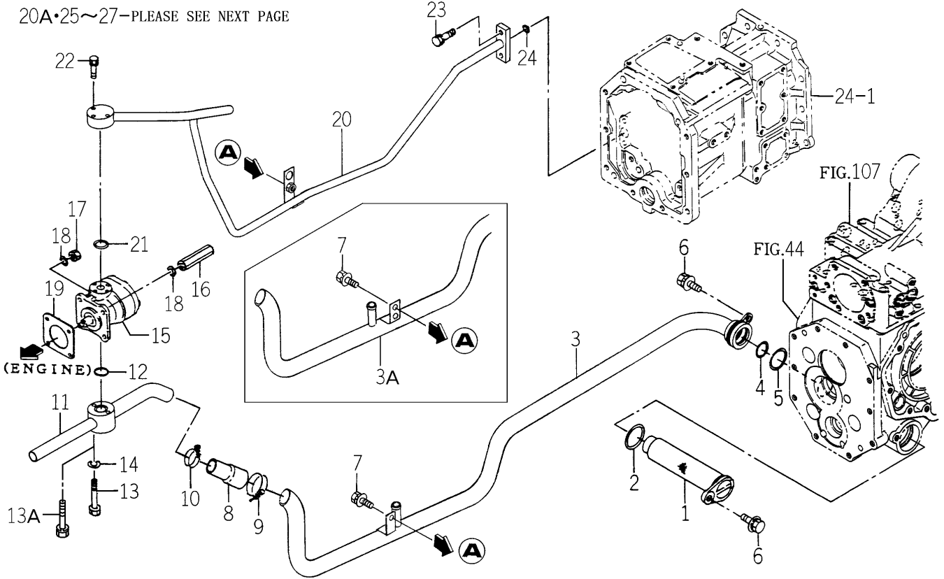
FIG.115 PIPING SYSTEM (EXCEPT H TYPE)(1/2)
