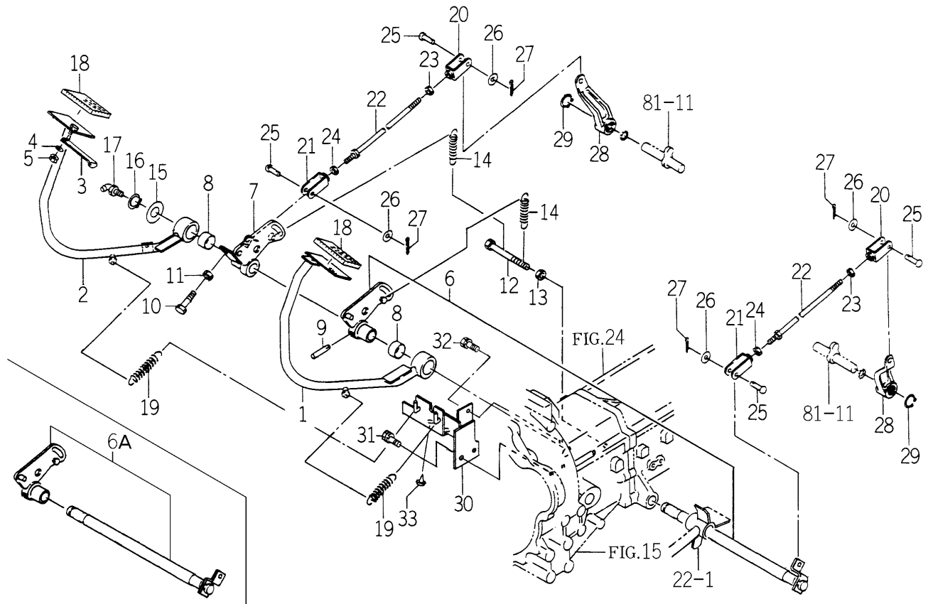
FIG. 83 PEDAL (BRAKE) SYSTEM (EXCEPT H TYPE)
