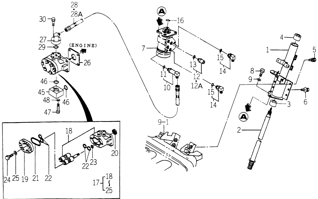
FIG. 87 STEERING (ORBIT) SYSTEM(1/2) (EXCEPT H TYPE)
