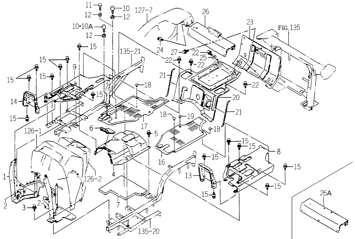
FIG.138 FLOOR SYSTEM (H TYPE-TH4260H-No.1~11006/ 4290H-1~10476/4330H-1~11256)
