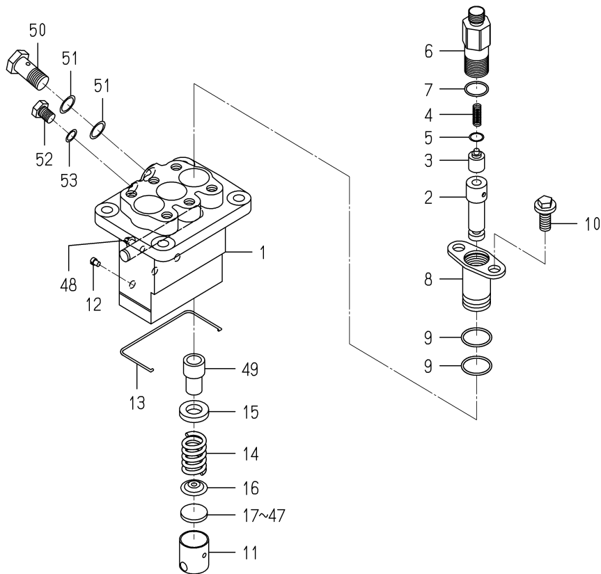
FIG. 30 COMPONENT PARTS FOR 6215-600-078-10 ON Fig.22
