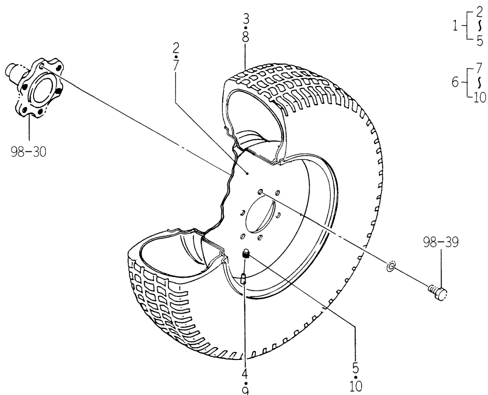
FIG.179 FRONT WHEEL (TURF/9.75I-12) SYSTEM (EXCEPT H TYPE-OPTION)
