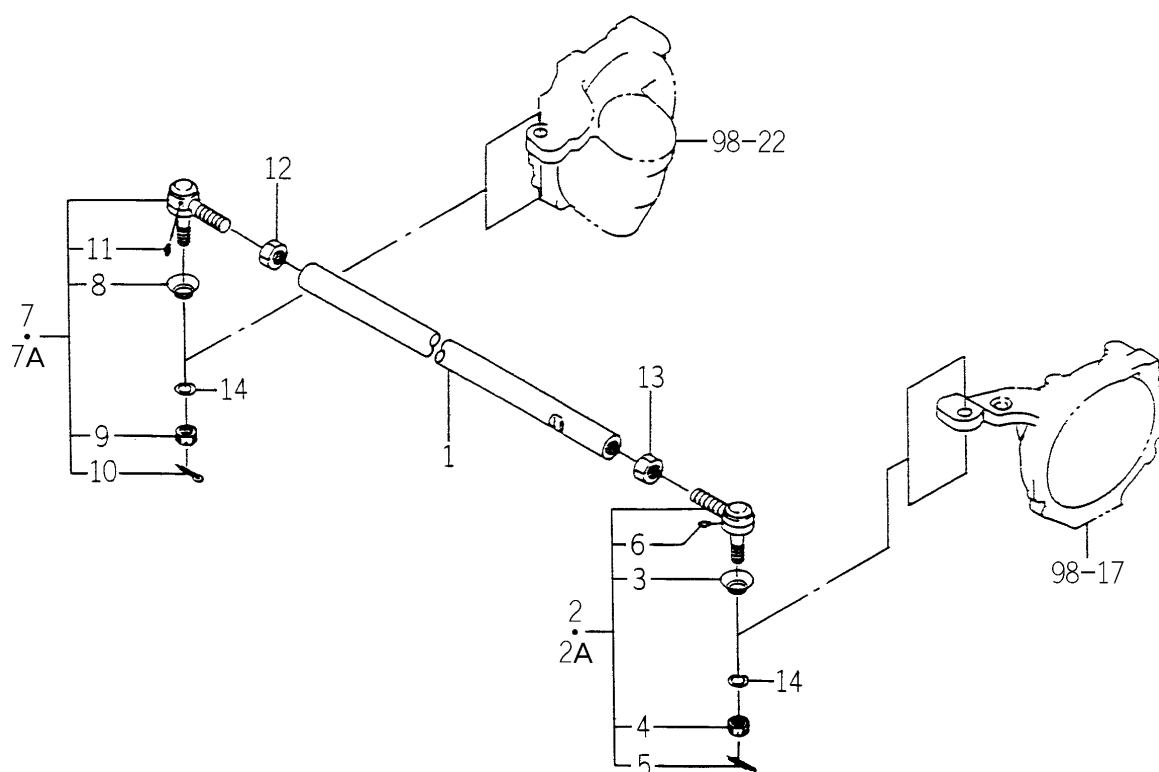
FIG.102 TIE ROD SYSTEM (EXCEPT H TYPE)
