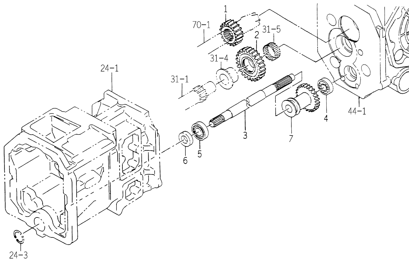
FIG. 39 4WD GEAR SYSTEM (EXCEPT H TYPE)
