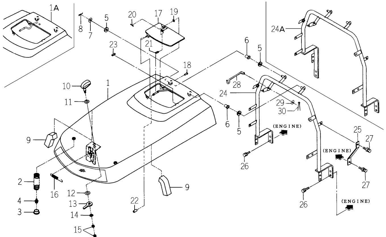
FIG.124 HOOD SYSTEM(1/2)
