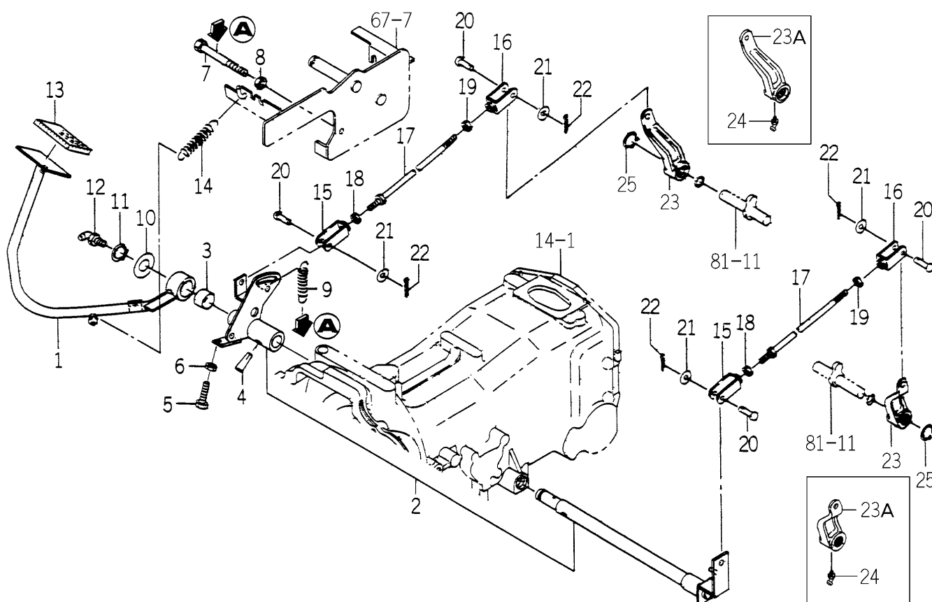
FIG. 82 PEDAL (BRAKE) SYSTEM (H TYPE)
