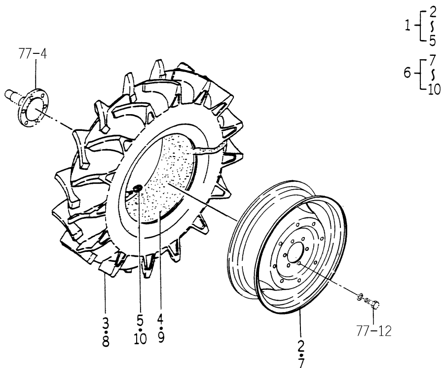
FIG.173 REAR WHEEL (9.5-24) SYSTEM (EXCEPT H TYPE-OPTION)
