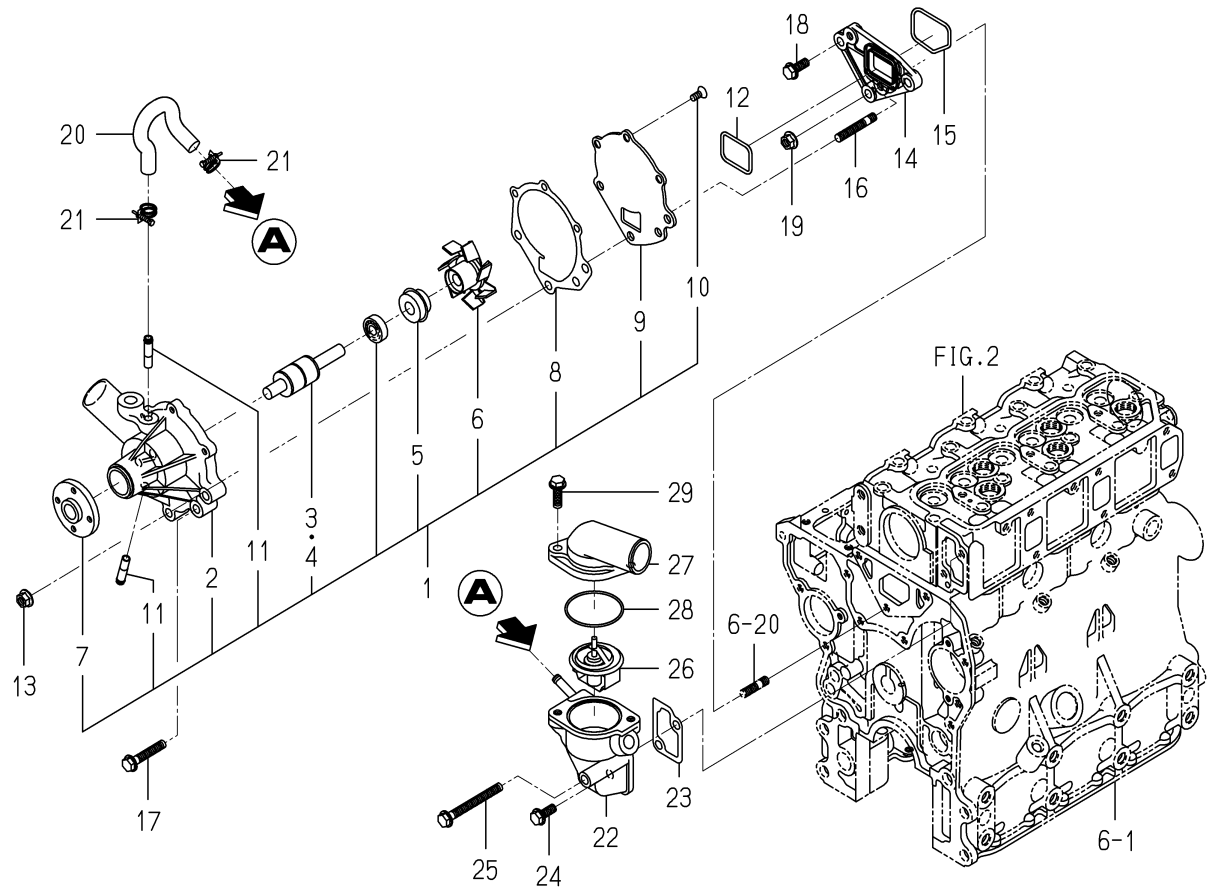
FIG. 18 WATER PUMP
