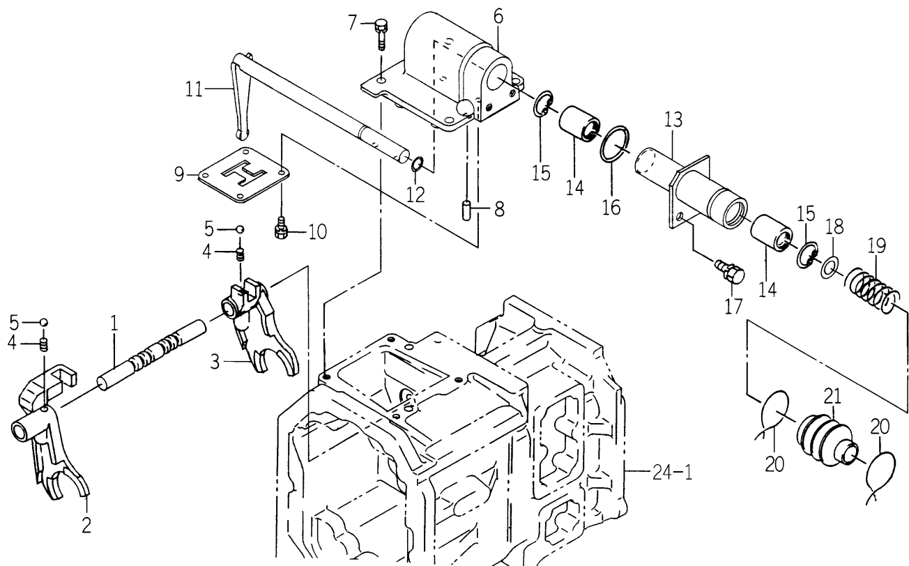
FIG. 35 MAIN CHANGE SYSTEM (EXCEPT H TYPE)
