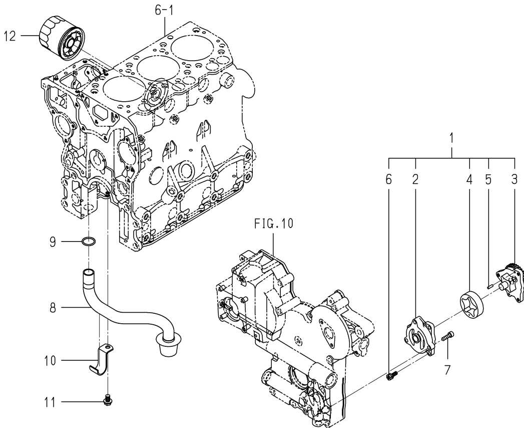
FIG. 17 OIL PUMP
