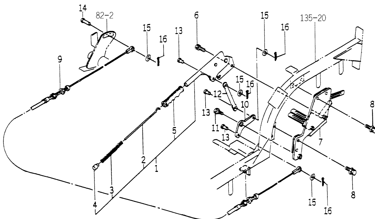
FIG. 84 BRAKE (PARKING) SYSTEM
