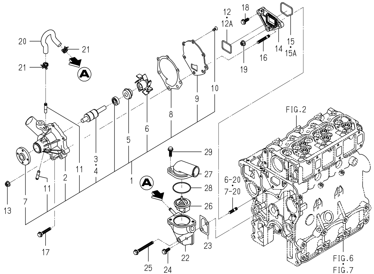
FIG. 22 WATER PUMP
