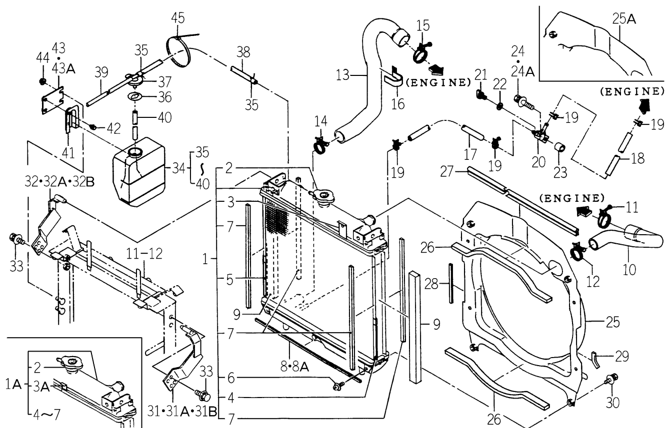
FIG. 1 RADIATOR SYSTEM
