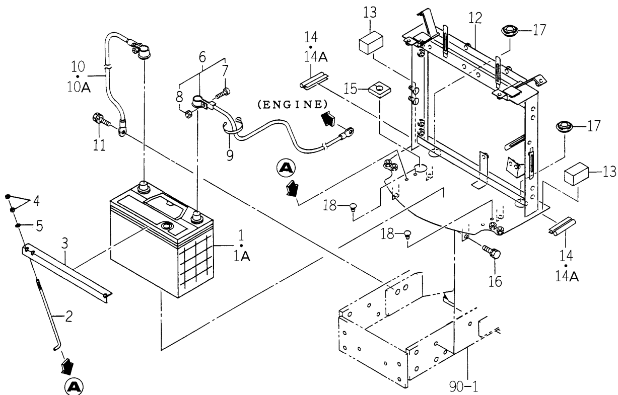
FIG. 11 BATTERY SYSTEM (EXCEPT H TYPE)
