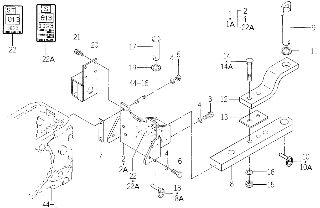
FIG.185 HITCH (DRAW BAR) SET (H TYPE EXCEPT R-OPTION)
