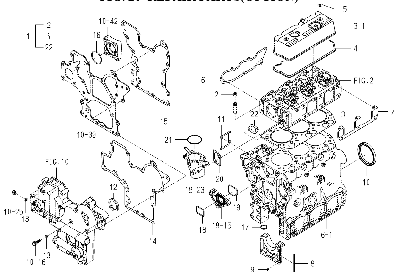
FIG. 26 REPAIR PARTS(OPTION)
