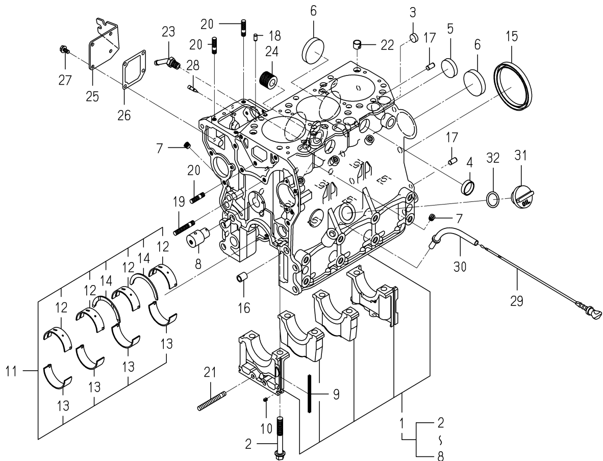
FIG. 6 CYLINDER BLOCK
