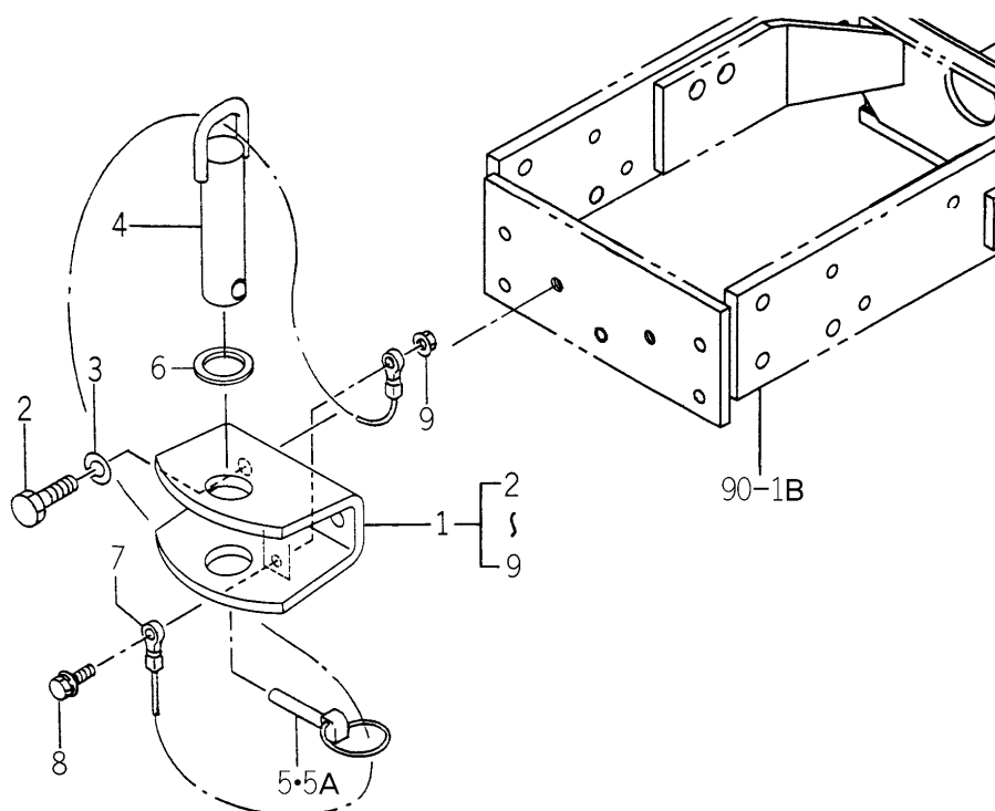
FIG.177 HITCH (FRONT) SET (EXCEPT R TYPE-OPTION)
