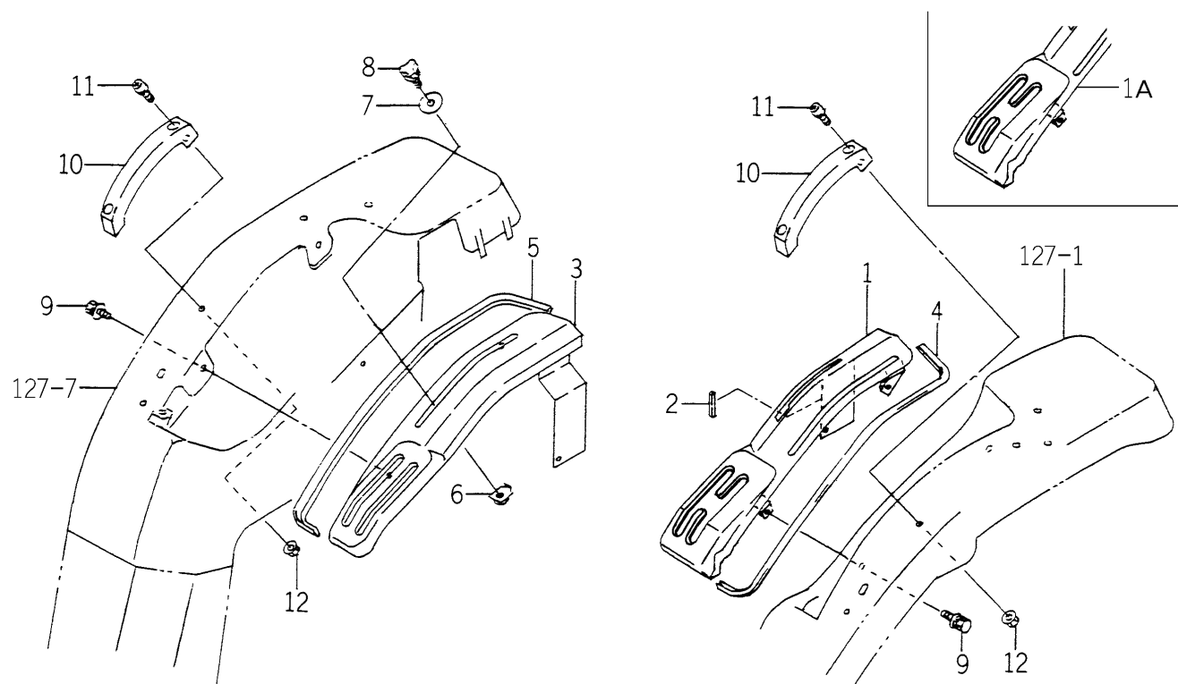
FIG.129 GUIDE (LEVER) SYSTEM (EXCEPT H TYPE)
