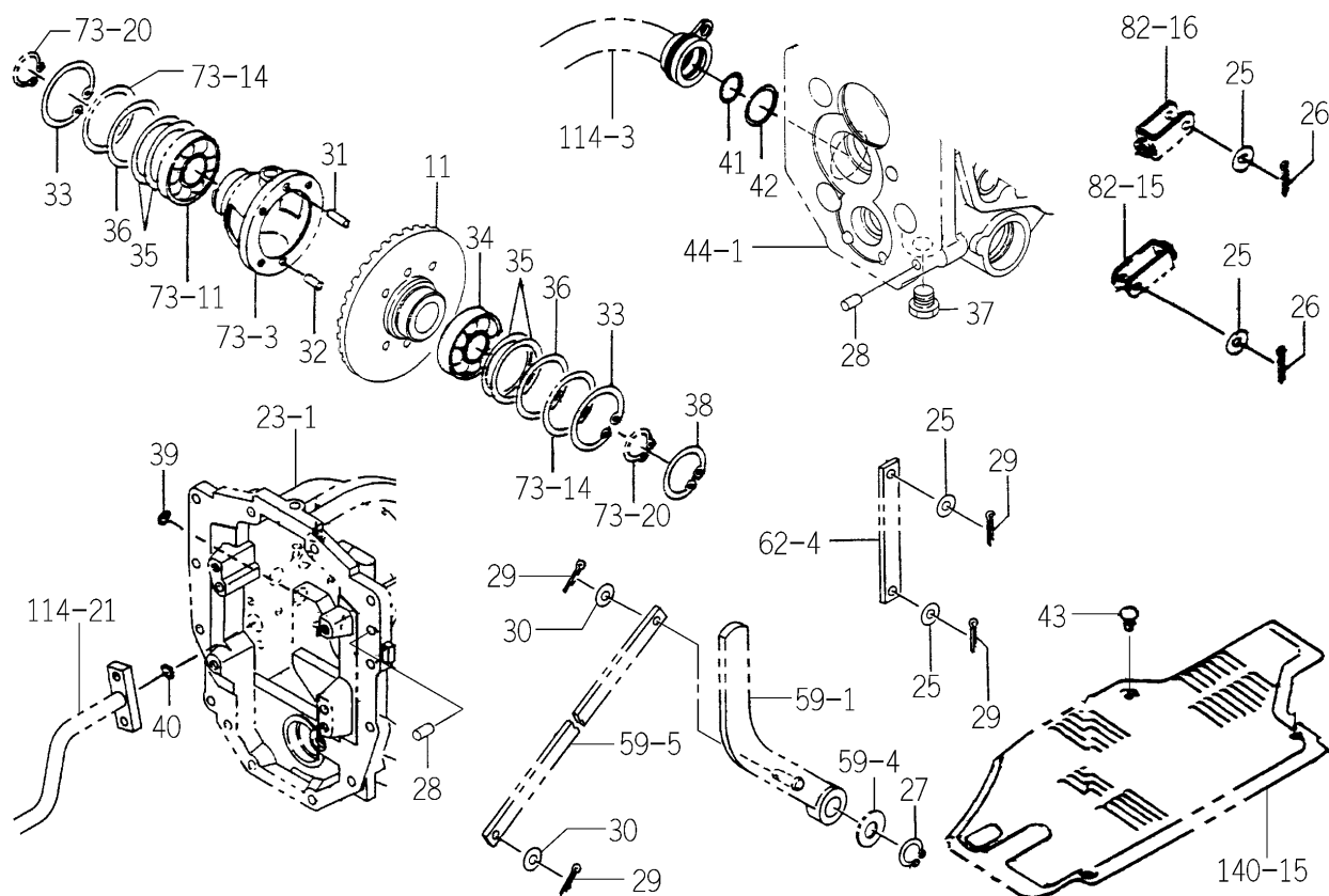
FIG.166 GEAR (SUB) SYSTEM(2/2) (H TYPE EXCEPT W-REPAIR)
