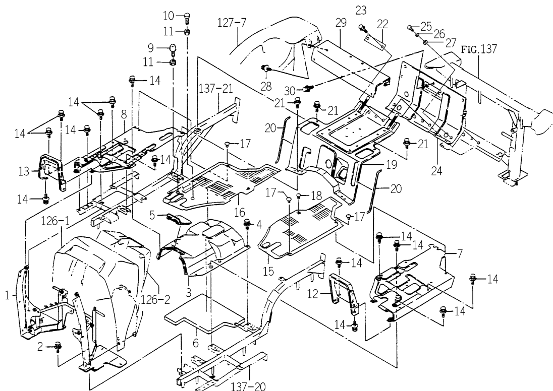
FIG.140 FLOOR SYSTEM (H TYPE-TH4260H-No.11007~/ 4290H-10477~/4330H-11257~)
