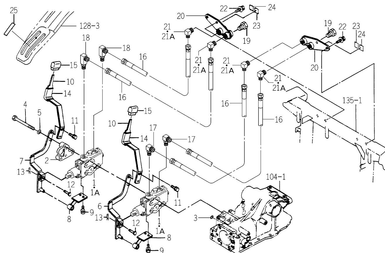
FIG.113 VALVE (STACK/R2) SYSTEM (W TYPE)
