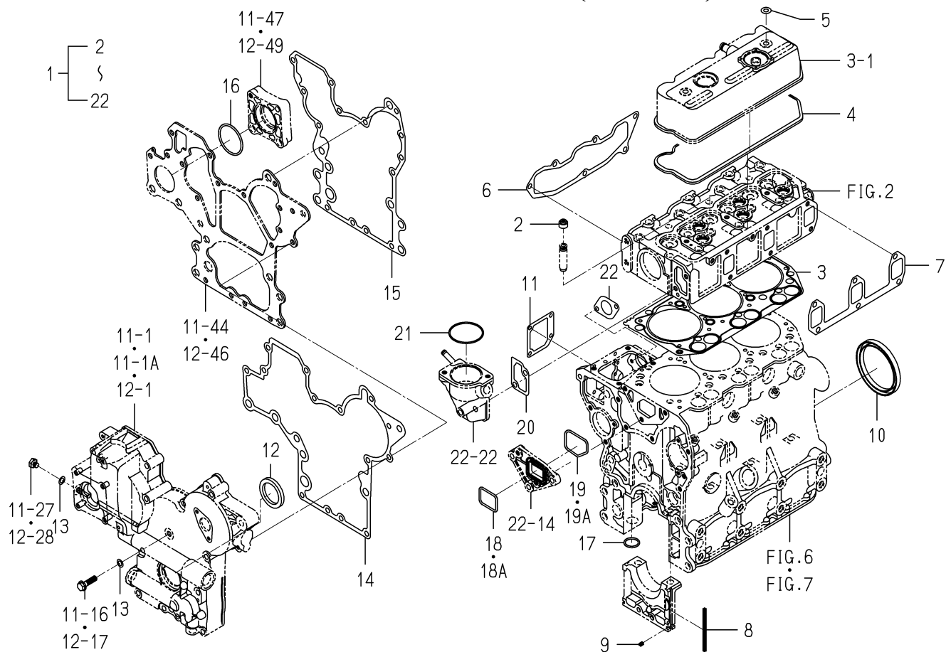
FIG. 33 REPAIR PARTS(OPTION)
