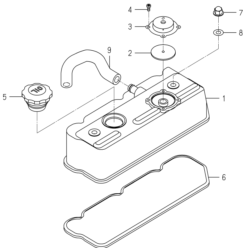
FIG. 3 CYLINDER HEAD COVER
