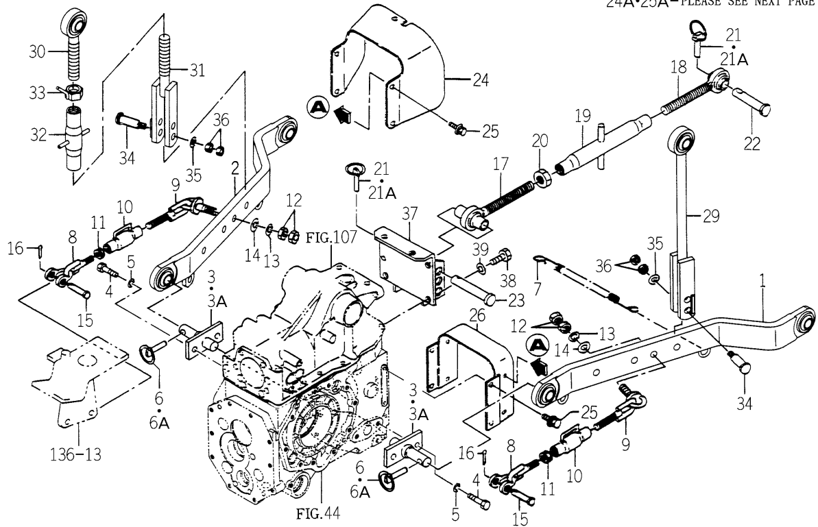
FIG.118 LINK (3P) SYSTEM (EXCEPT(1/2) H TYPE-No.1~)(H TYPE-4260H-10823~/ 4290H-10464~/4330H-10977~)
