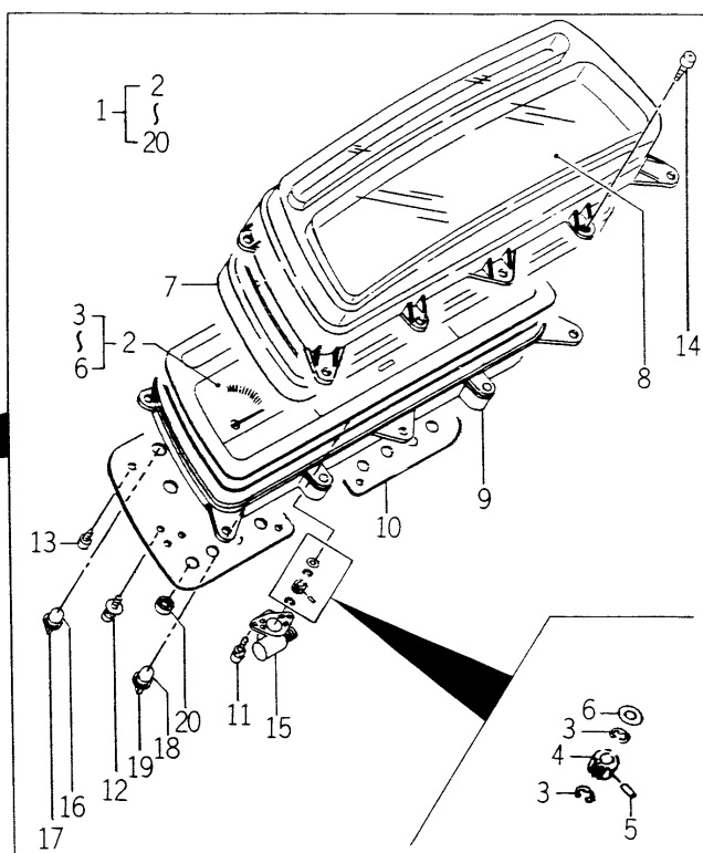
FIG.145 PANEL SYSTEM(D,R TYPE EXCEPT W-No.1~) (EXCEPT D,R TYPE/W TYPE-TH4260H-No. 1~11000/4290H-1~10472/4330H-1~11243)
