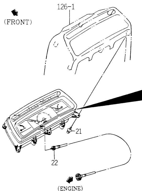
FIG.145 PANEL SYSTEM(D,R TYPE EXCEPT W-No.1~) (EXCEPT D,R TYPE/W TYPE-TH4260H-No. 1~11000/4290H-1~10472/4330H-1~11243)
