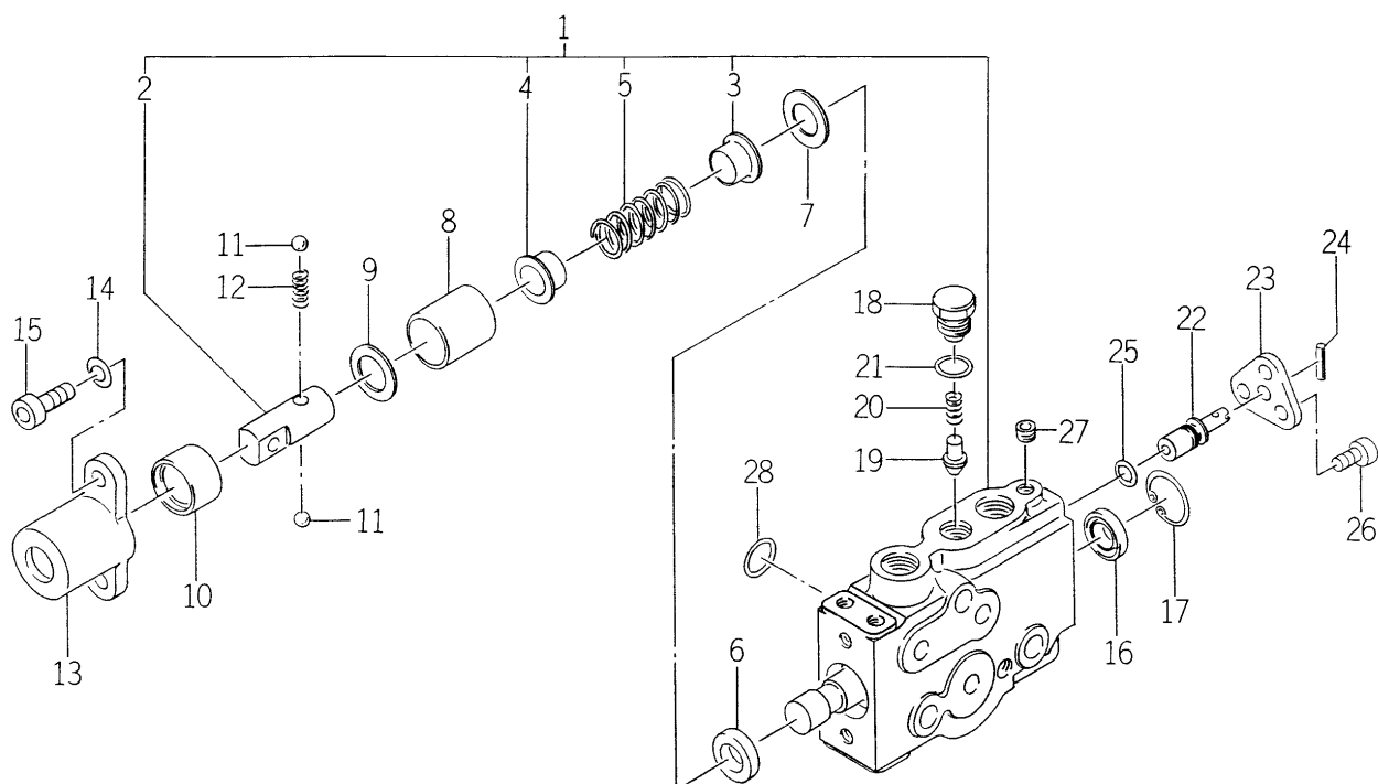
FIG.199 COMPONENT PARTS FOR 1719-511-350-00 ON Fig.113
