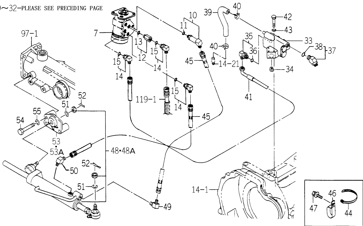
FIG. 86 STEERING (ORBIT) SYSTEM (H TYPE)(2/2)
