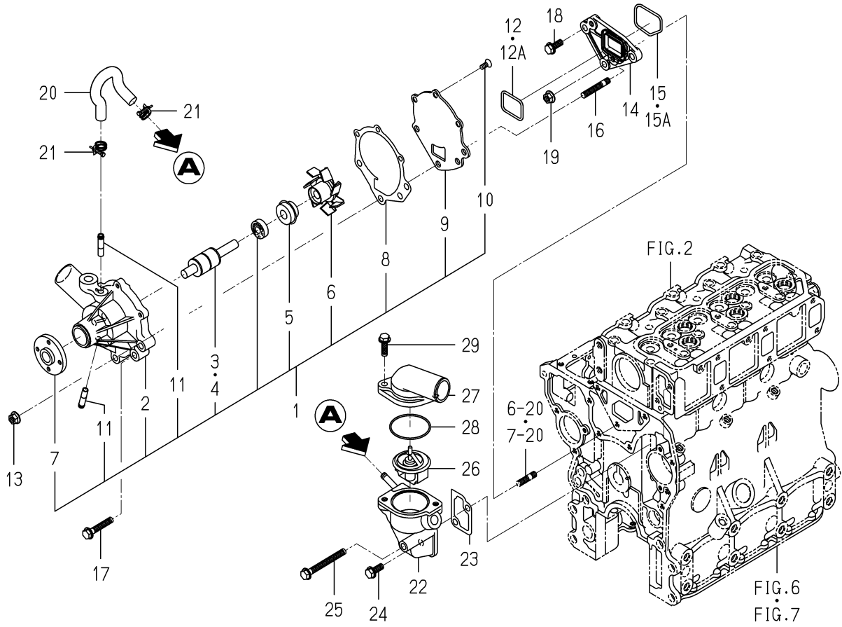
FIG. 22 WATER PUMP
