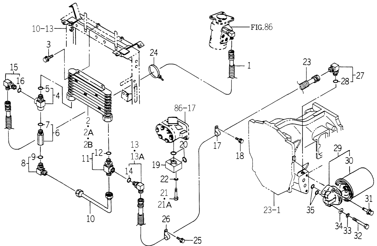
FIG.119 PIPING (COOLER) SYSTEM (H TYPE)
