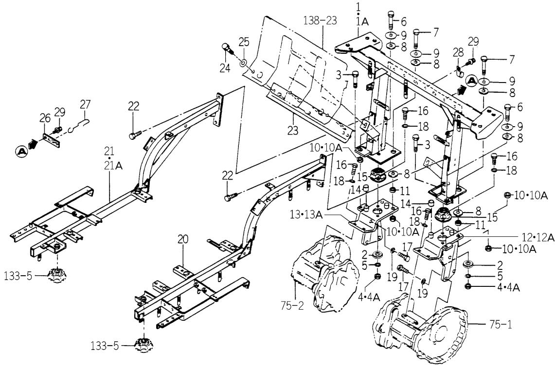
FIG.135 MOUNT (REAR) SYSTEM (H TYPE-TH4260H-No.1~11006/ 4290H-1~10476/4330H-1~11256)
