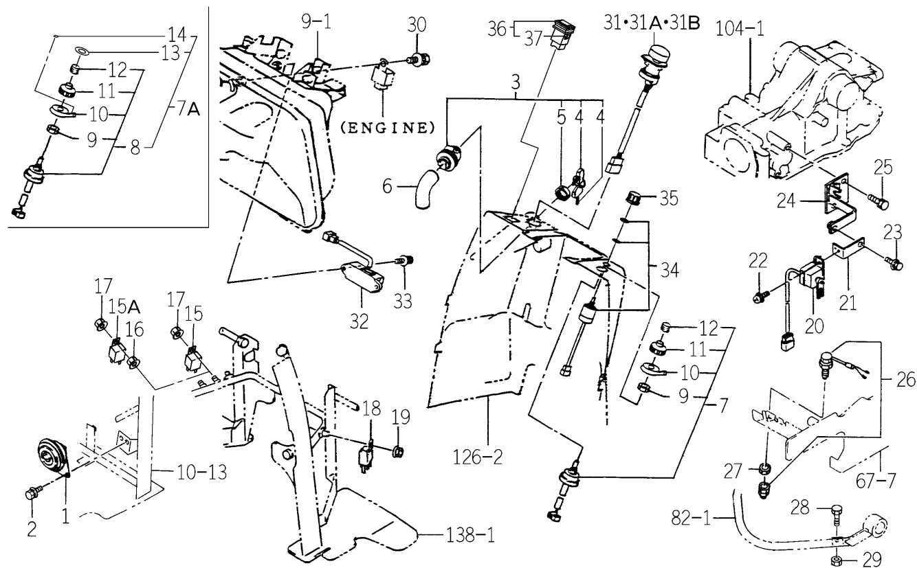
FIG.147 SWITCH SYSTEM (H TYPE)
