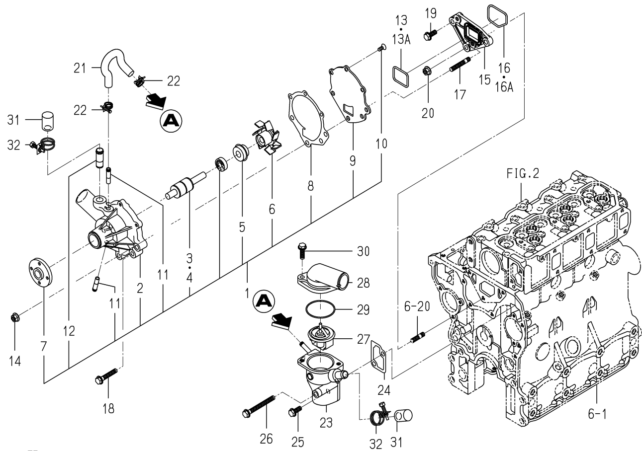
FIG. 19 WATER PUMP
