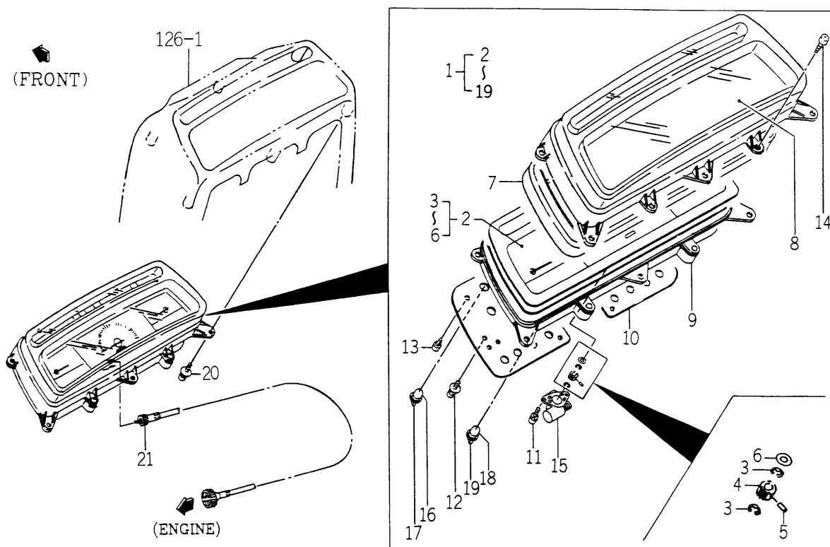
FIG.146 PANEL SYSTEM(EXCEPT D,R TYPE/ W TYPE-TH4260H-No.11001~/ 4290H-10473~/4330H-11244~)
