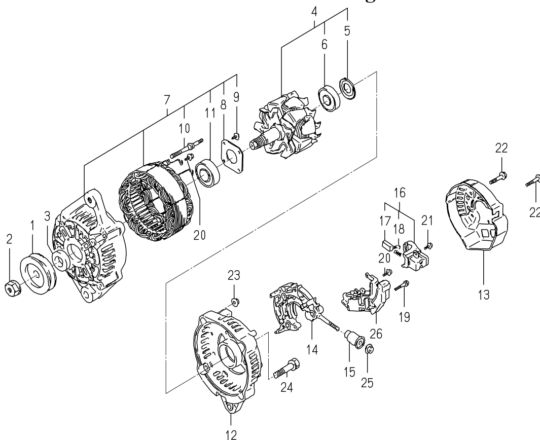
FIG. 37 COMPONENT PARTS FOR 6281-200-021-00 ON Fig.30
