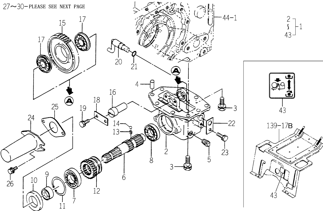
FIG.169 MID PTO SET(1/2) (EXCEPT M TYPE-OPTION)
