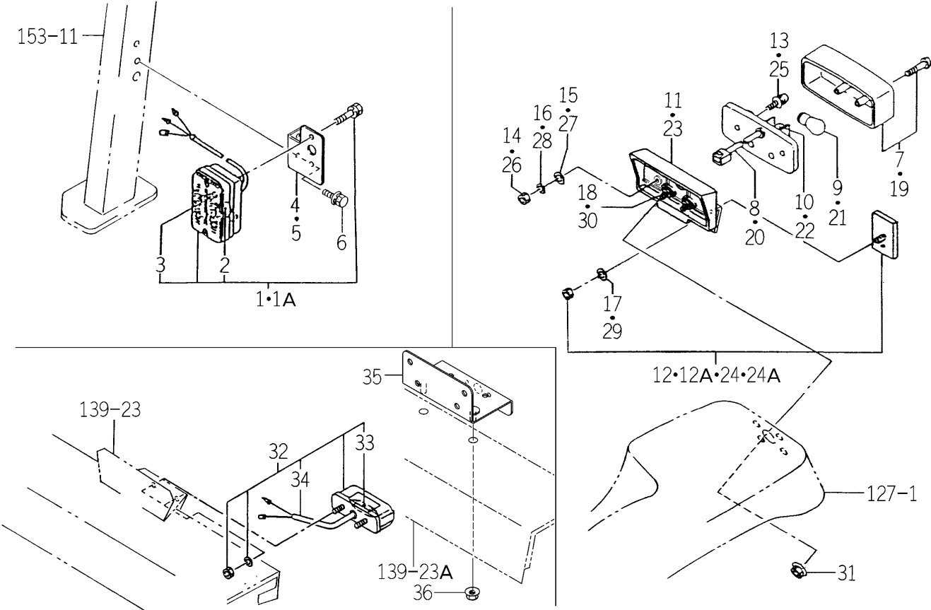
FIG.144 LAMP SYSTEM (EXCEPT H TYPE)
