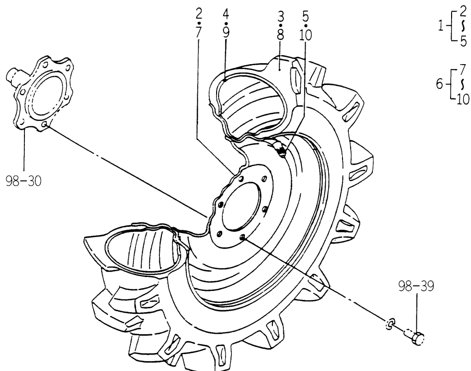
FIG.181 FRONT WHEEL SYSTEM (EXCEPT H TYPE-OPTION)
