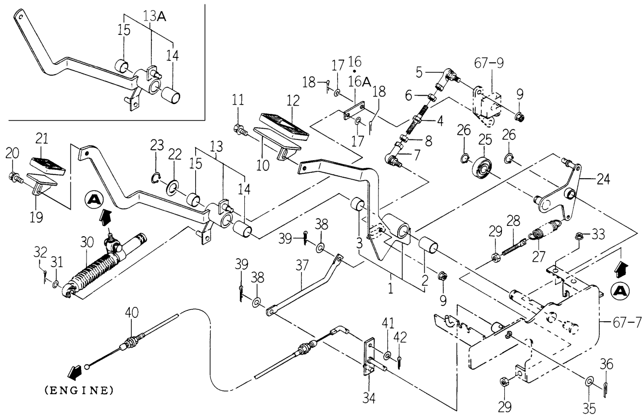
FIG. 69 PEDAL (HST) SYSTEM (H TYPE)
