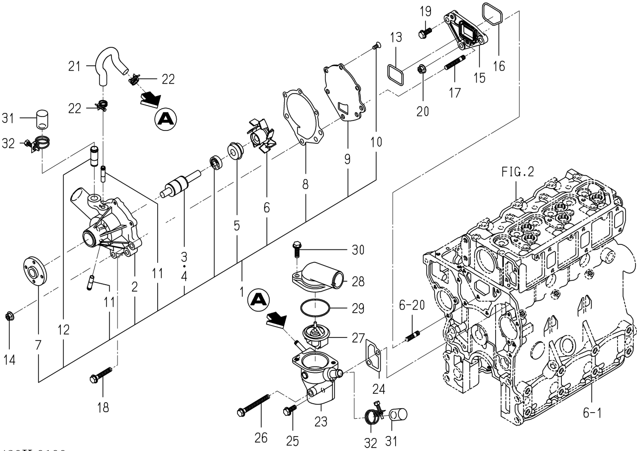
FIG. 18 WATER PUMP
