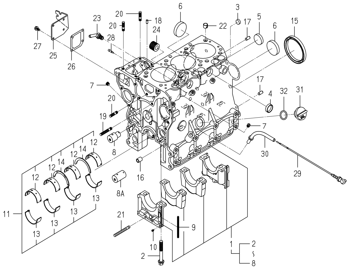
FIG. 7 CYLINDER BLOCK
