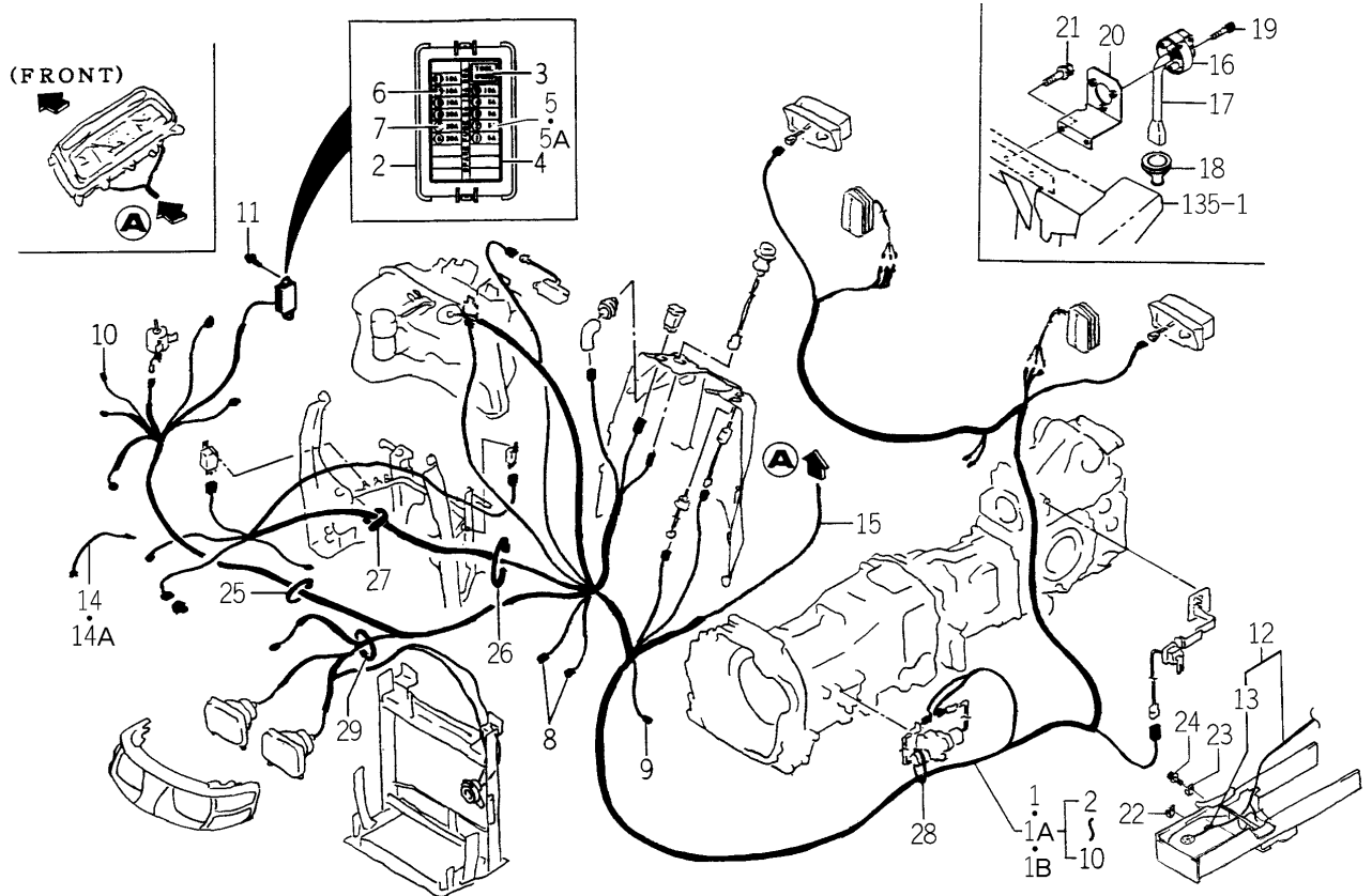
FIG.150 HARNESS SYSTEM (TH4290,4330-H TYPE)
