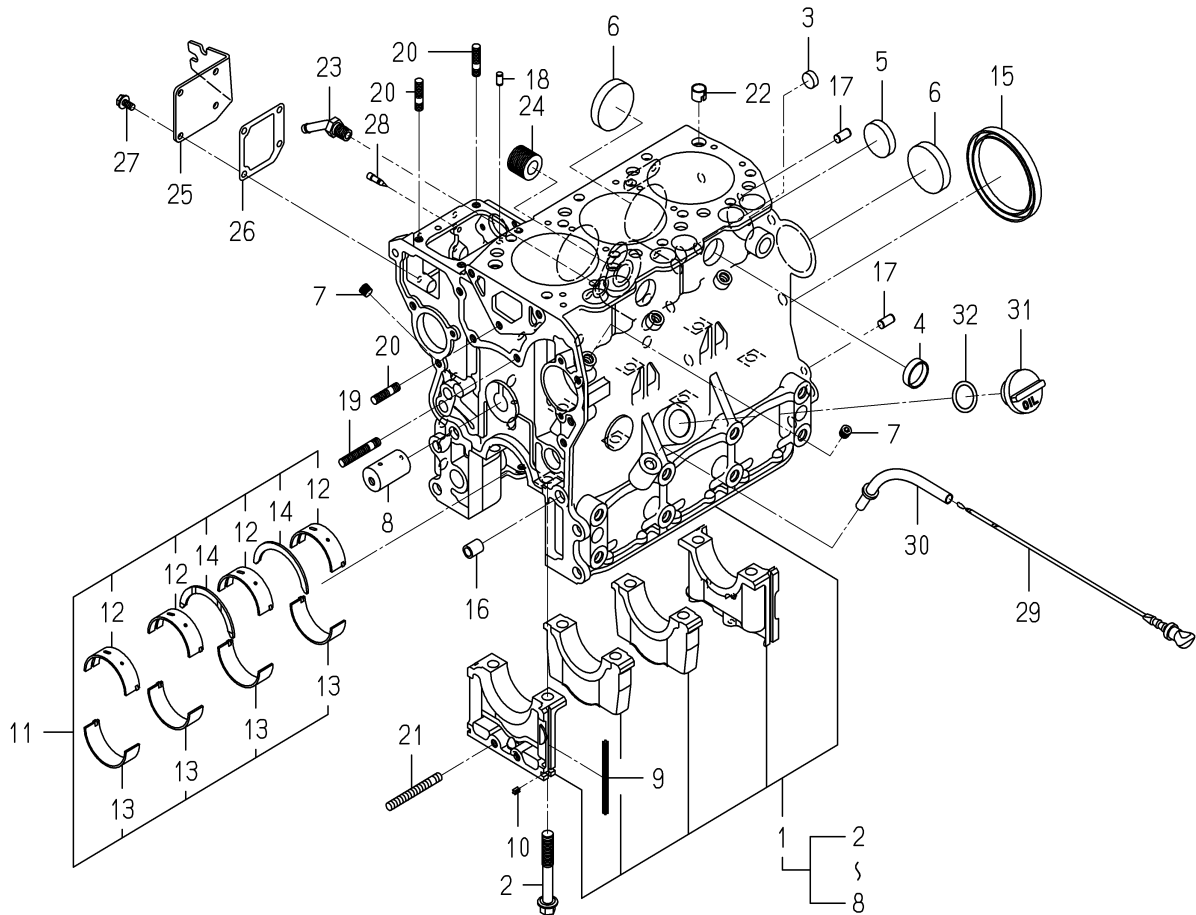
FIG. 6 CYLINDER BLOCK
