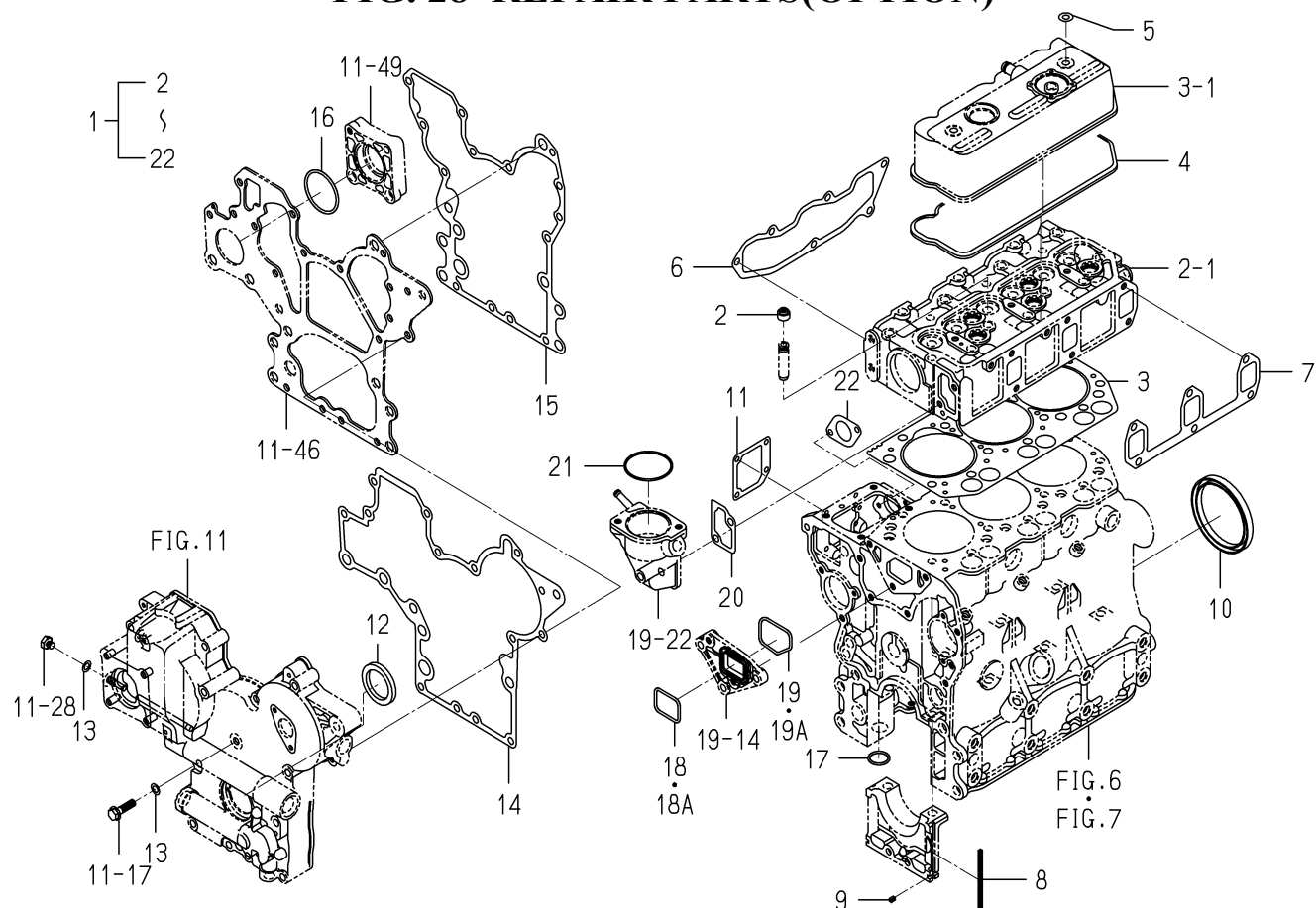
FIG. 28 REPAIR PARTS(OPTION)
