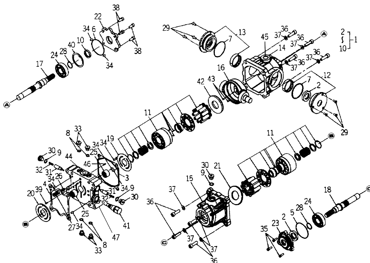
FIG.201 COMPONENT PARTS FOR 1740-202-500-00 ON Fig.25
