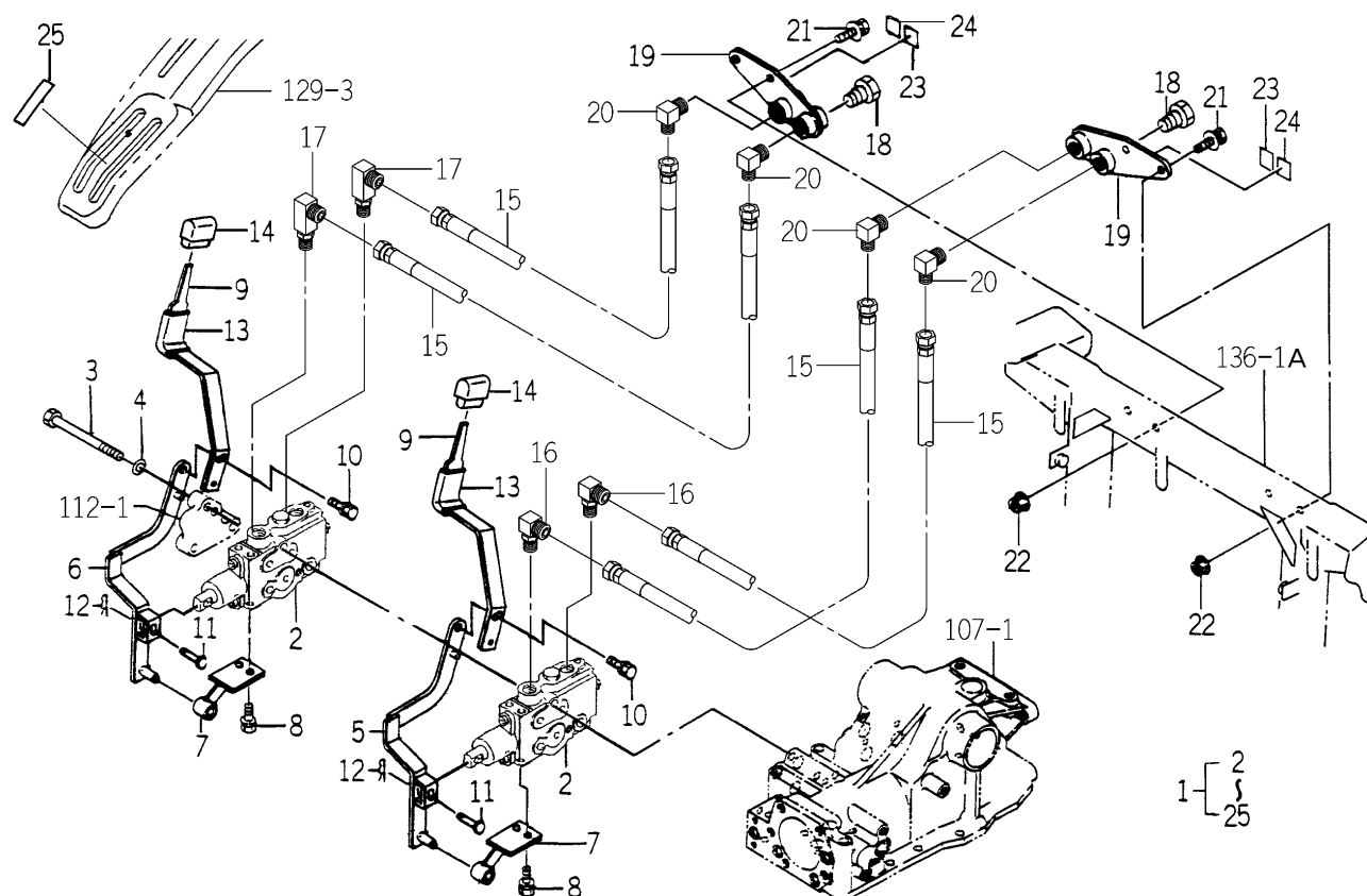
FIG.184 VALVE (STACK/R2) SET (EXCEPT W TYPE-OPTION)
