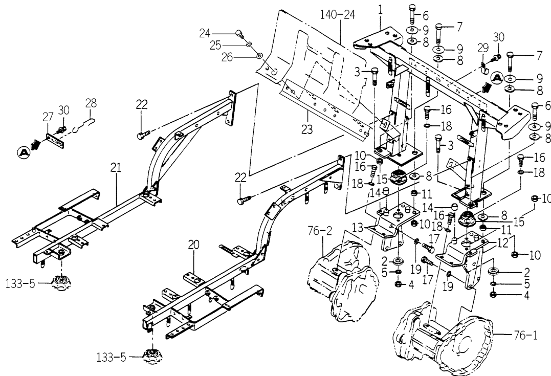
FIG.137 MOUNT (REAR) SYSTEM (H TYPE-TH4260H-No.11007~/ 4290H-10477~/4330H-11257~)
