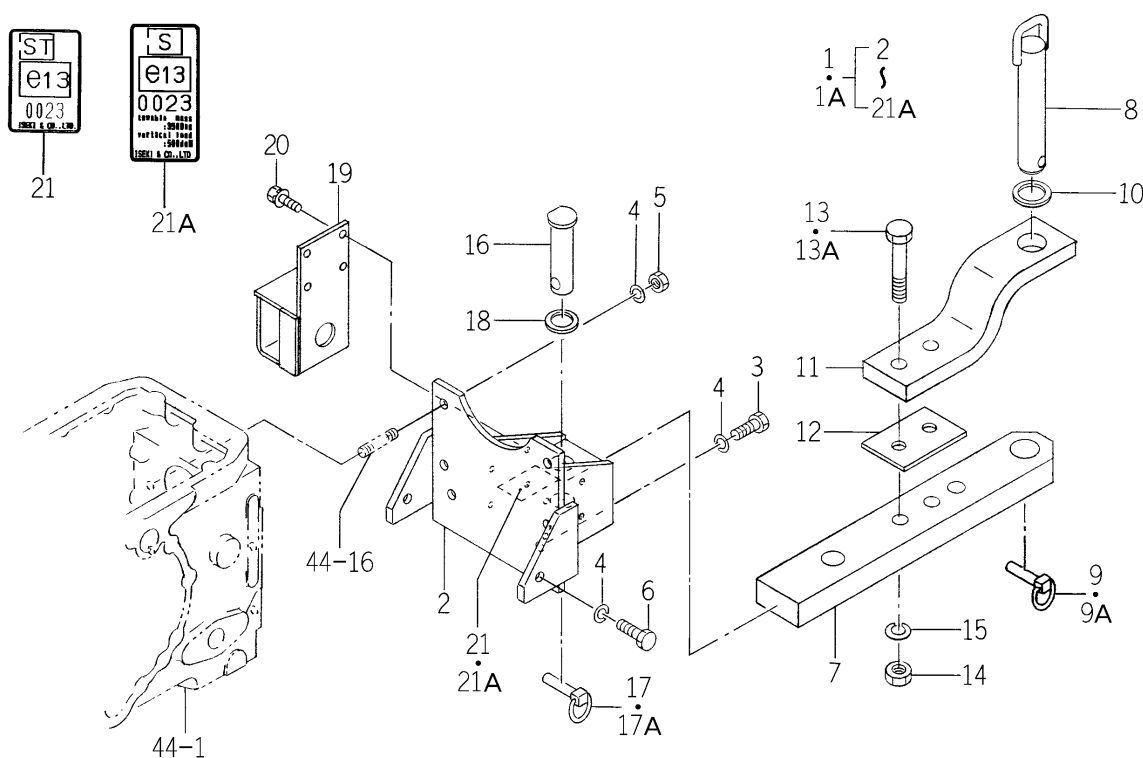
FIG.122 HITCH(DRAW BAR)SET(R TYPE EXCEPT H-STD/EXCEPT H,R-OPT-1~)(H TYPE- OPT4260H-10823~/4290H-10464~/4330H-10977~)
