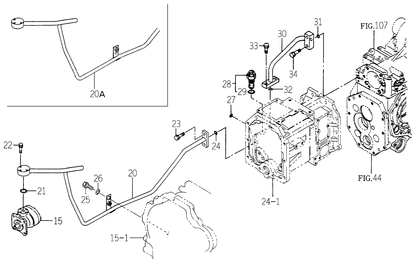
FIG.115 PIPING SYSTEM (EXCEPT H TYPE)(2/2)
