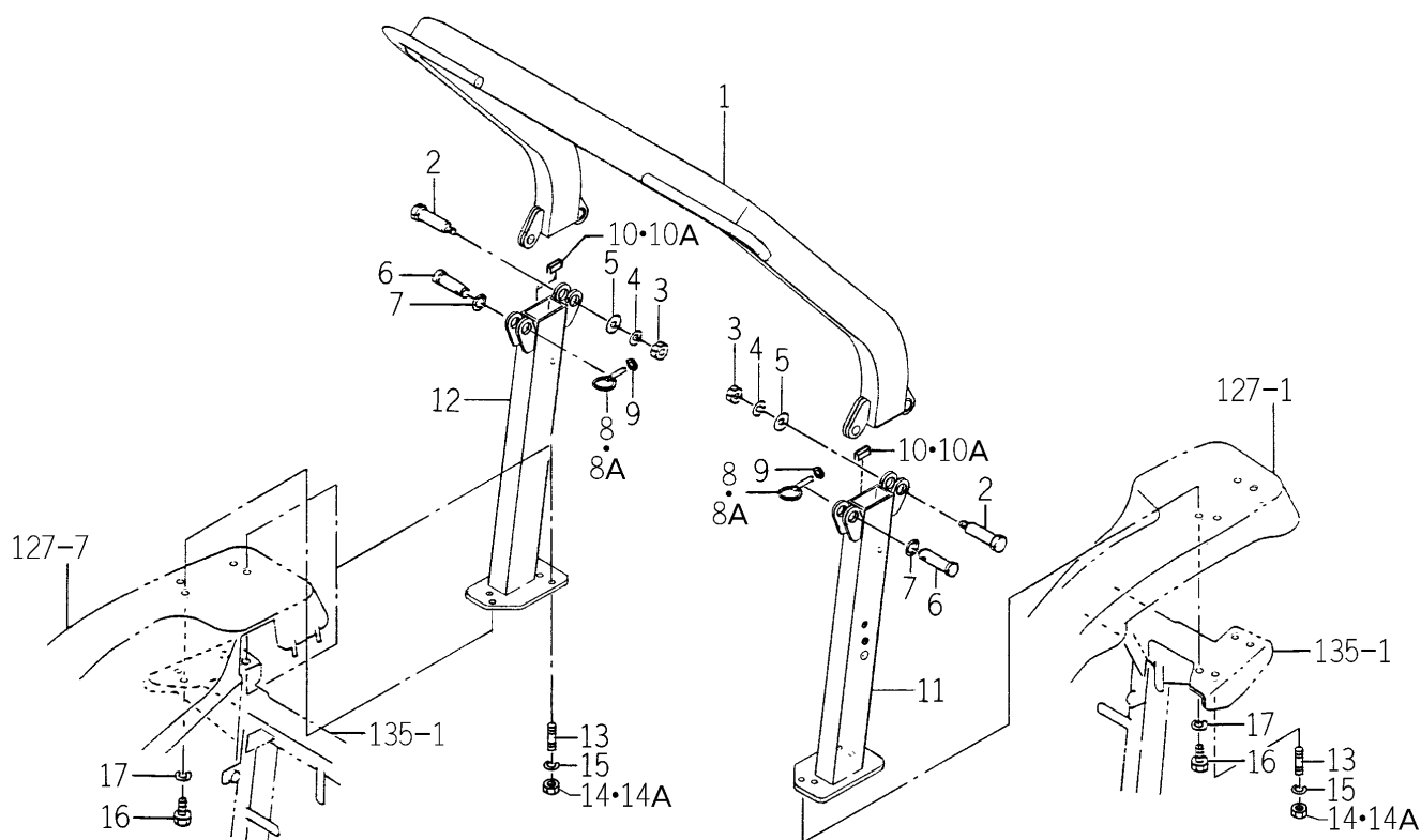
FIG.153 ROPS SYSTEM (R TYPE)
