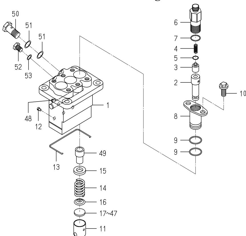
FIG. 30 COMPONENT PARTS FOR 6215-600-078-10 ON Fig.22
