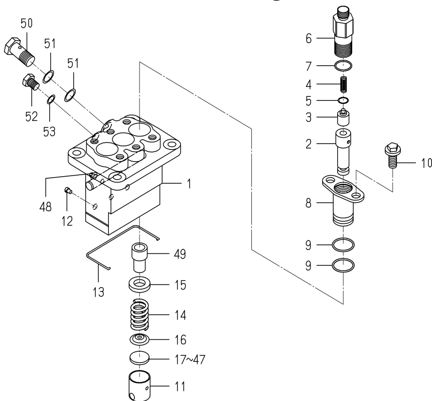
FIG. 35 COMPONENT PARTS FOR 6215-600-078-10 ON Fig.25
