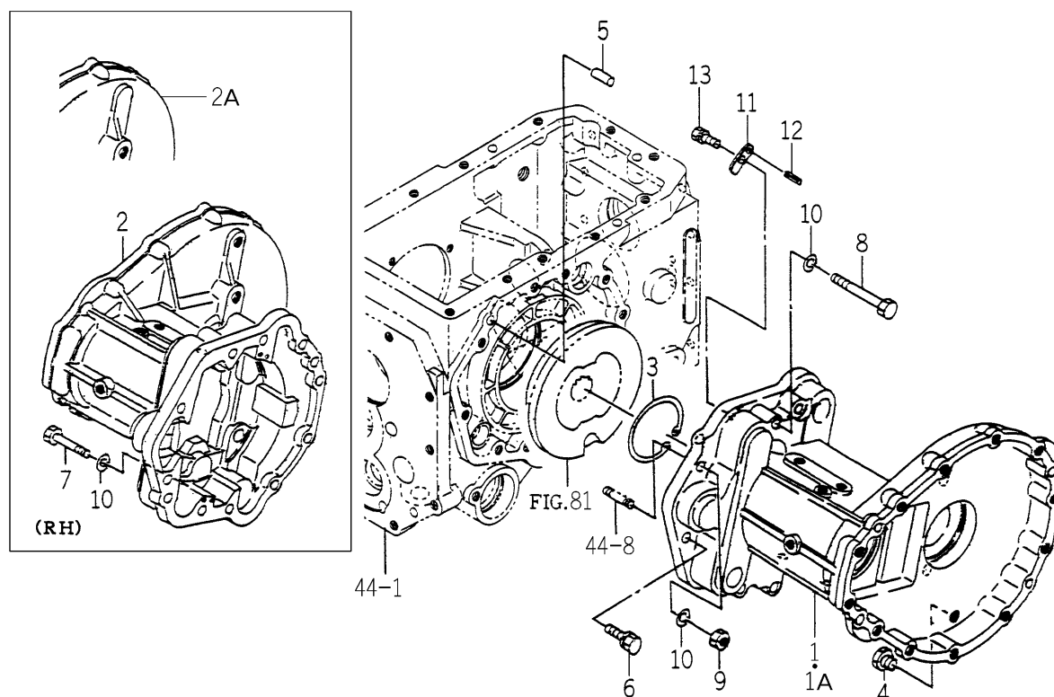
FIG. 76 REAR AXLE HOUSING SYSTEM (EXCEPT H TYPE-No.1~)(H TYPE-4260H-10823~/ 4290H-10464~/4330H-10977~)
