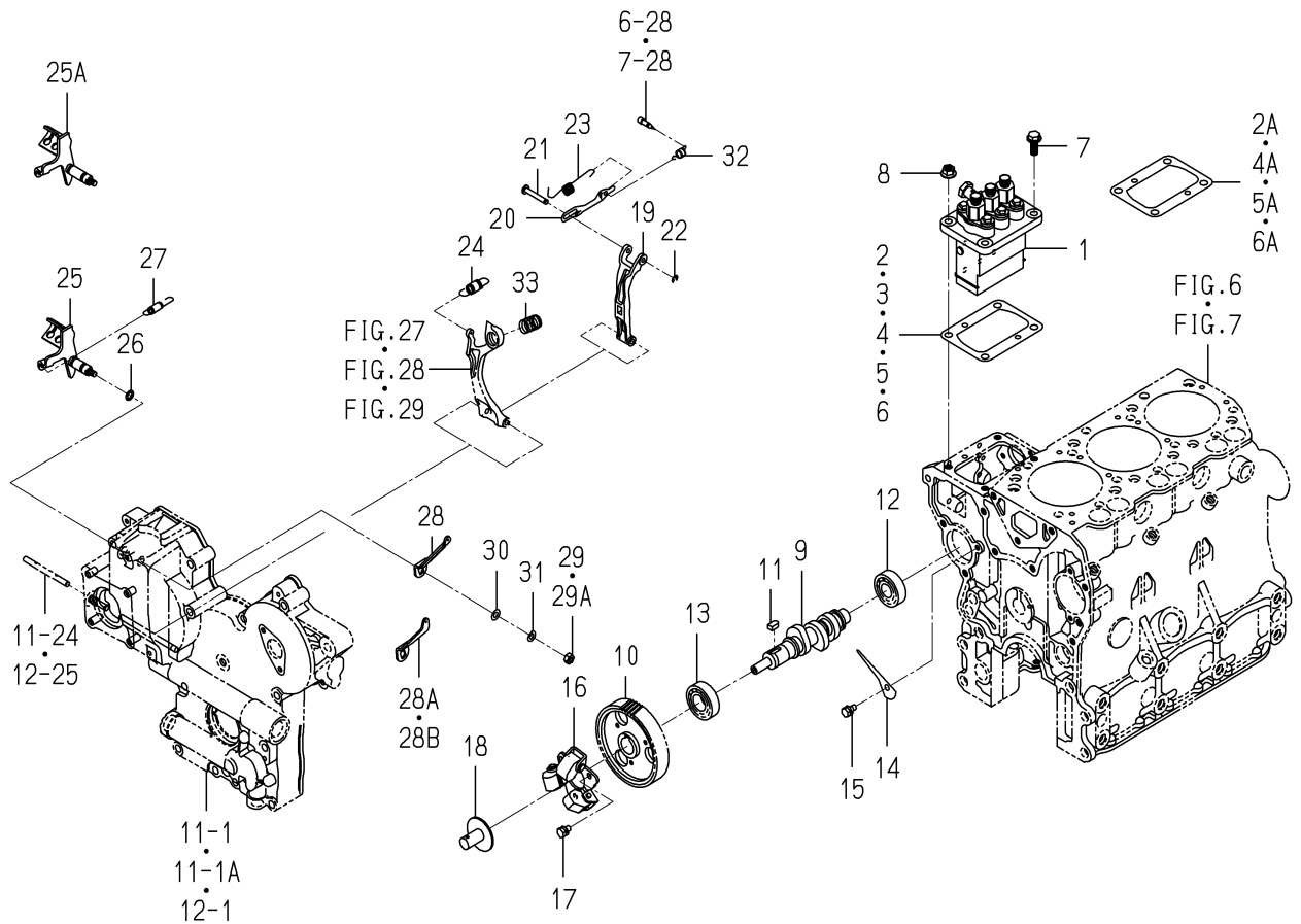
FIG. 25 INJECTION PUMP
