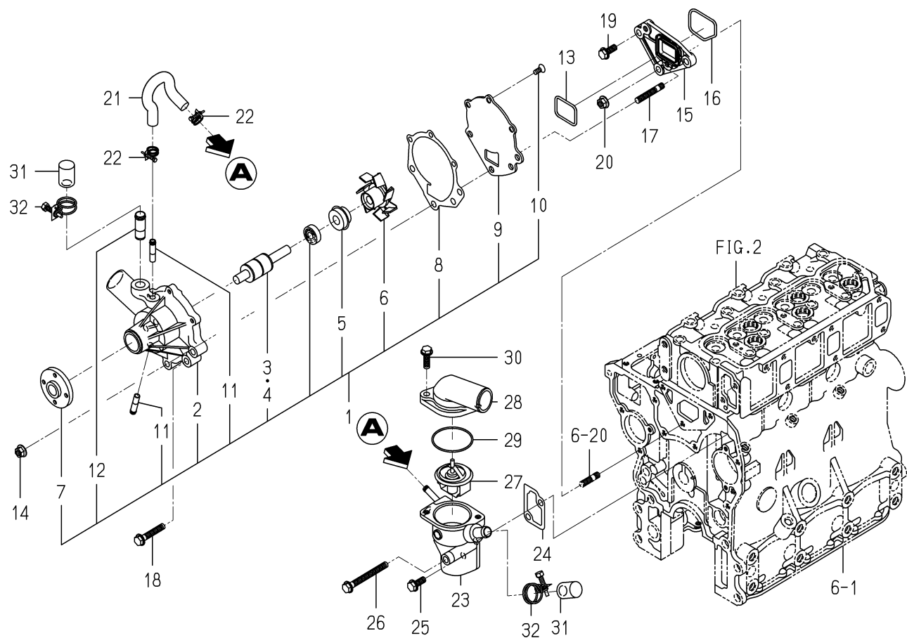
FIG. 18 WATER PUMP
