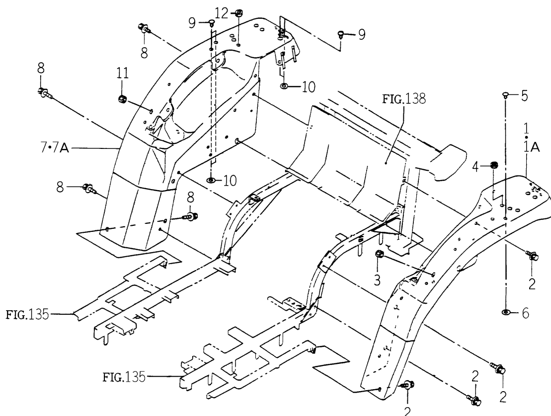
FIG.127 FENDER SYSTEM
