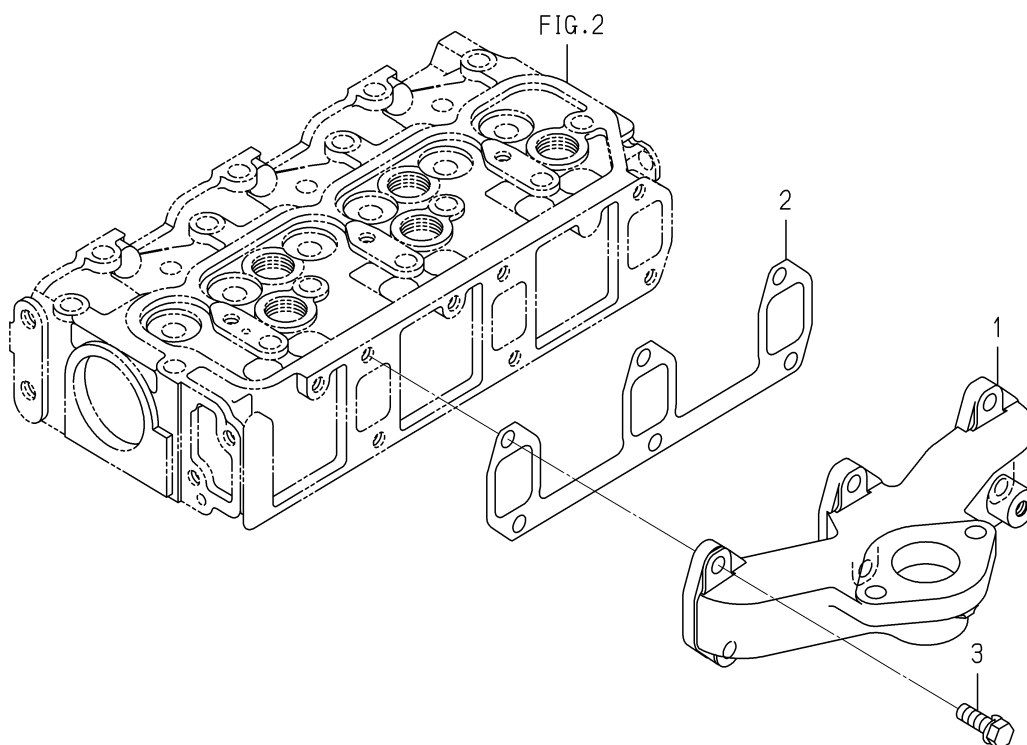
FIG. 5 EXHAUST MANIFOLD
