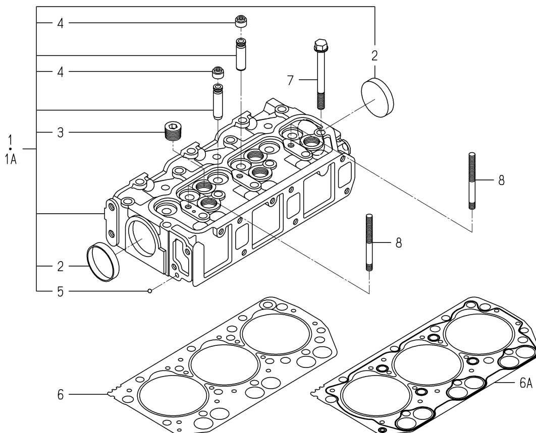
FIG. 2 CYLINDER HEAD
