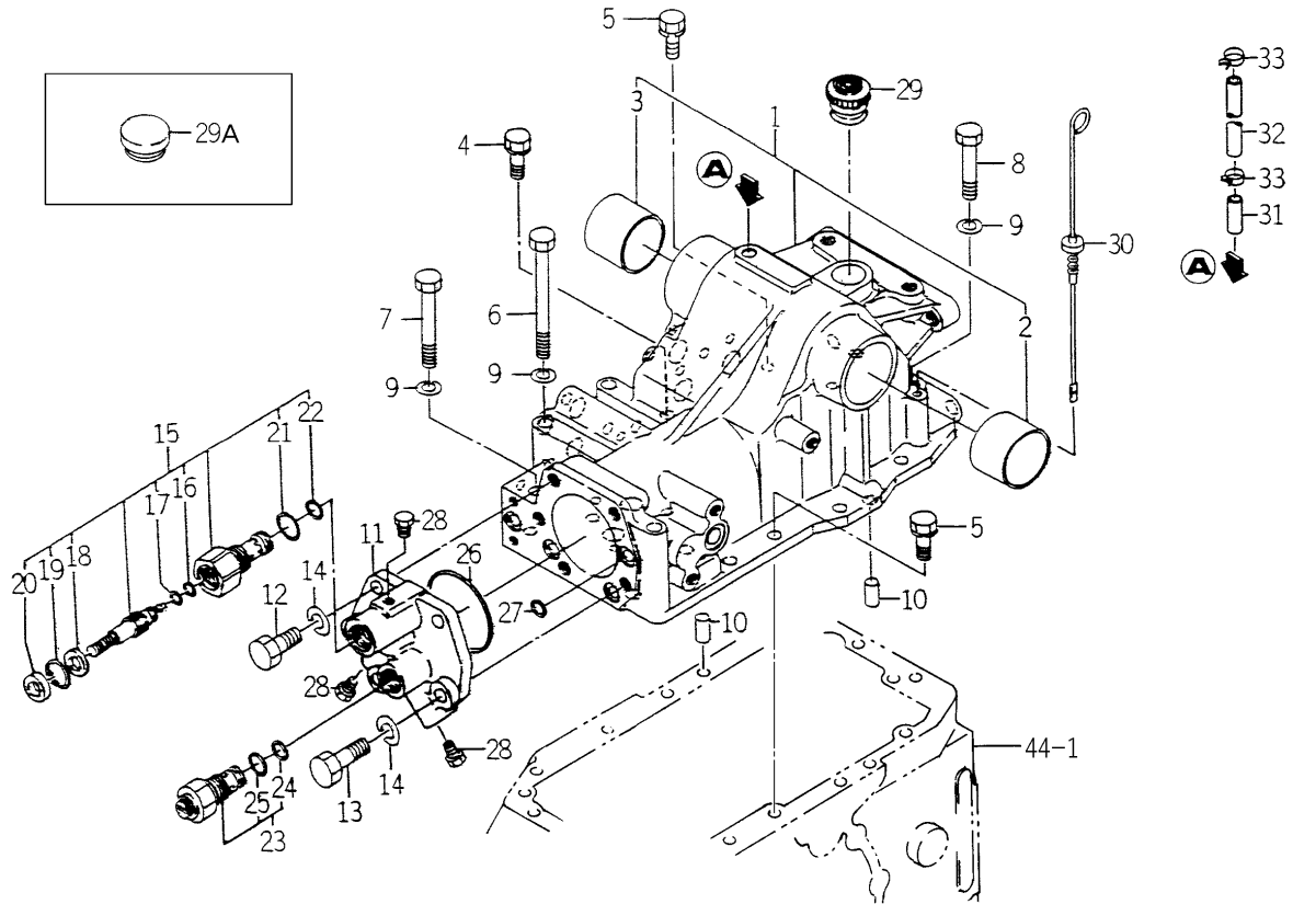
FIG.107 CASE (CYLINDER) SYSTEM (EXCEPT H TYPE)
