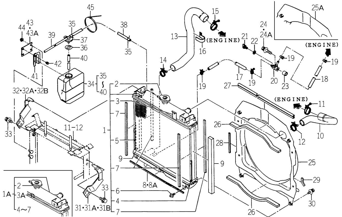
FIG. 1 RADIATOR SYSTEM
