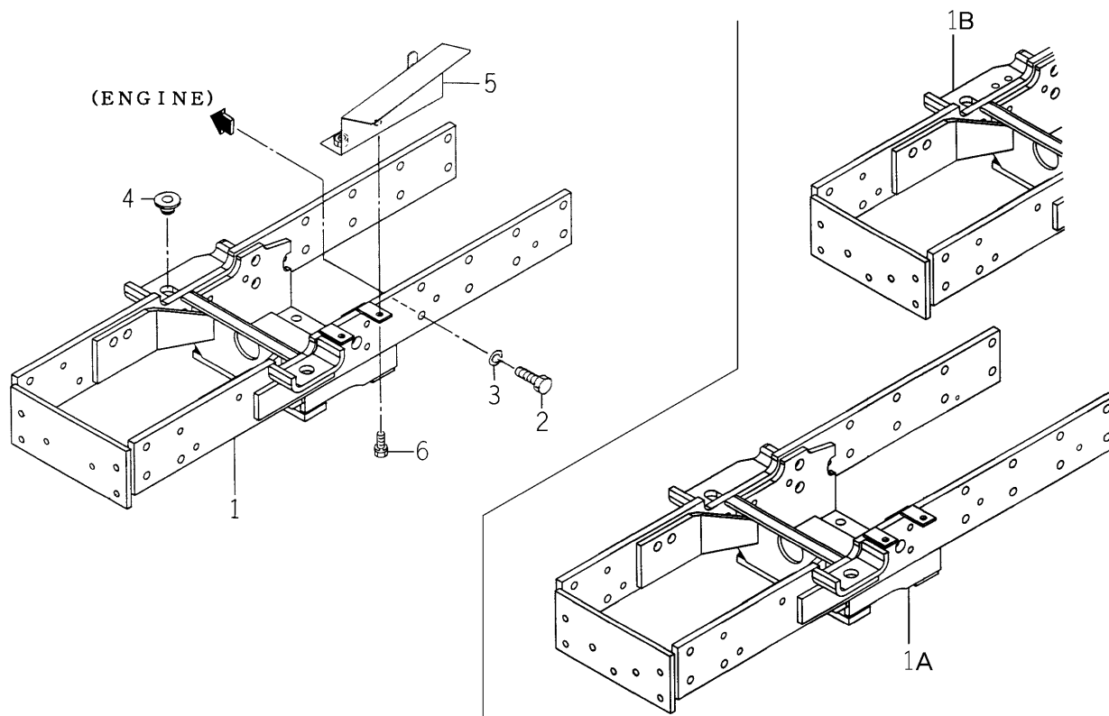
FIG. 90 BRACKET (AXLE) SYSTEM (TH4260-EXCEPT H TYPE)
