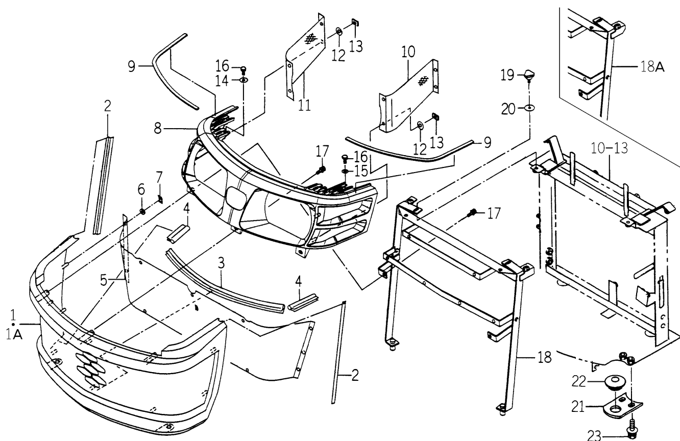
FIG.125 GRILLE SYSTEM
