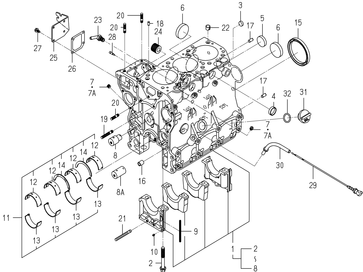
FIG. 6 CYLINDER BLOCK
