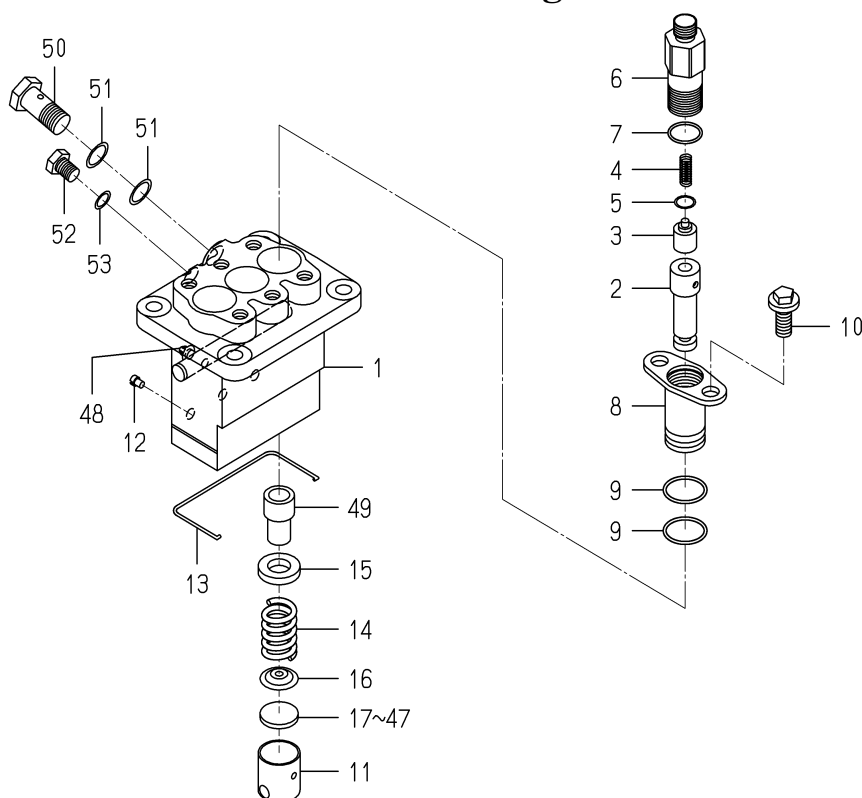
FIG. 28 COMPONENT PARTS FOR 6215-600-078-10 ON Fig.22
