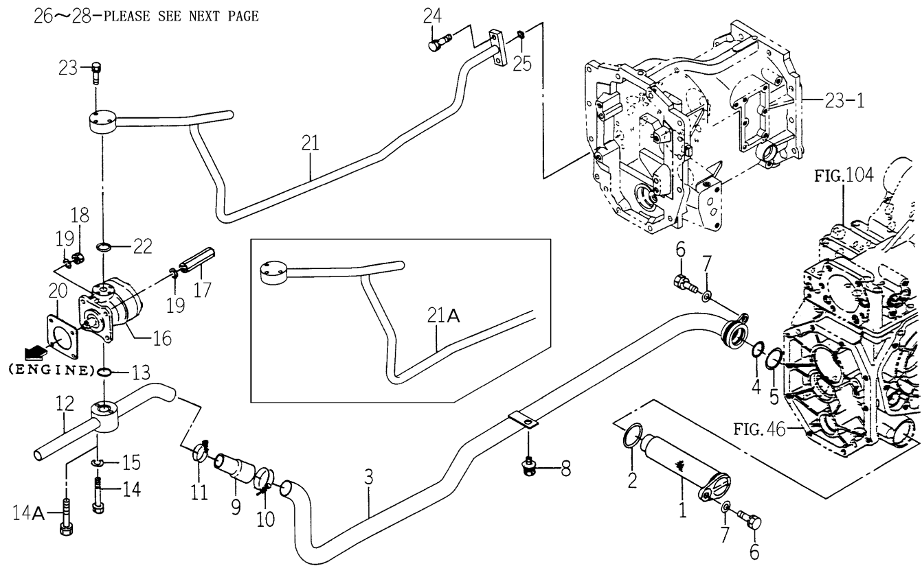
FIG.114 PIPING SYSTEM (H TYPE)(1/2)
