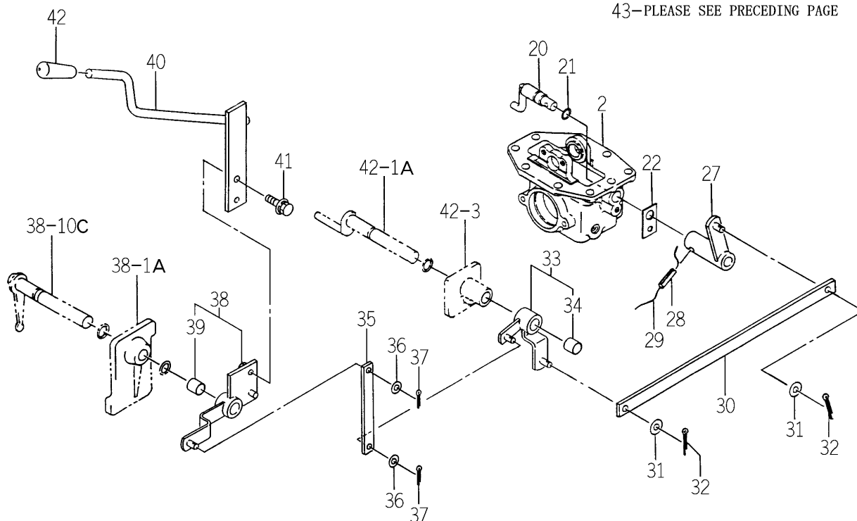
FIG.169 MID PTO SET(2/2) (EXCEPT M TYPE-OPTION)
