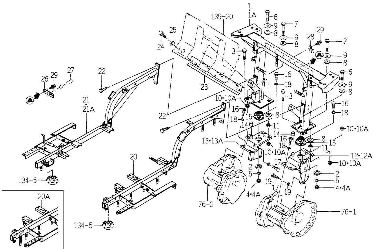
FIG.136 MOUNT (REAR) SYSTEM (EXCEPT H TYPE)
