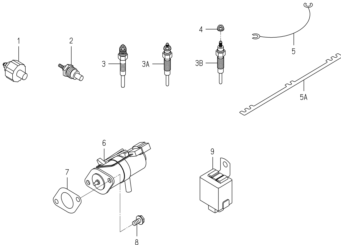
FIG. 31 ELECTRIC (2)
