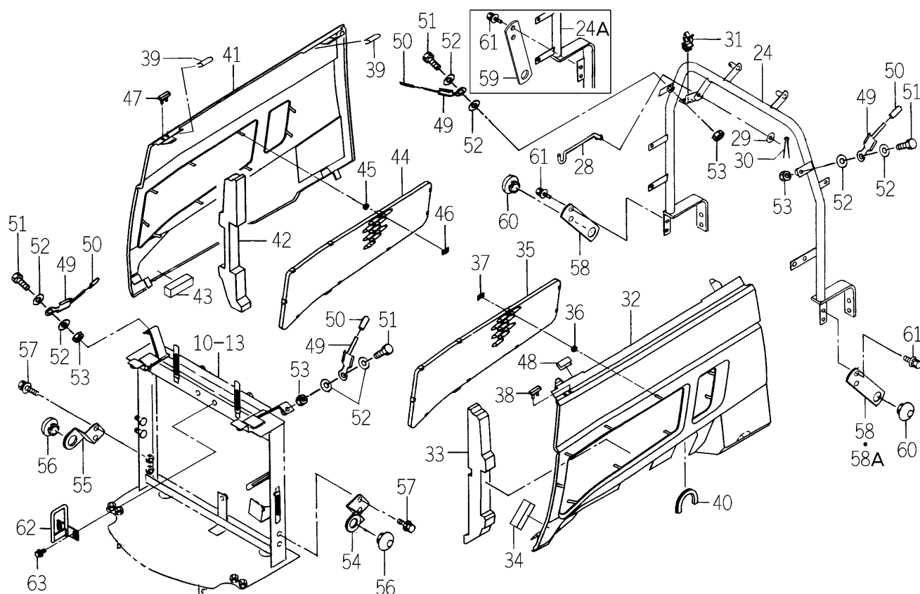
FIG.124 HOOD SYSTEM(2/2)
