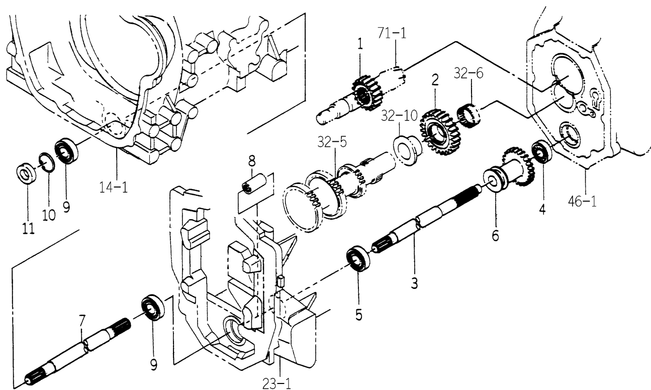
FIG. 40 4WD GEAR SYSTEM (H TYPE)
