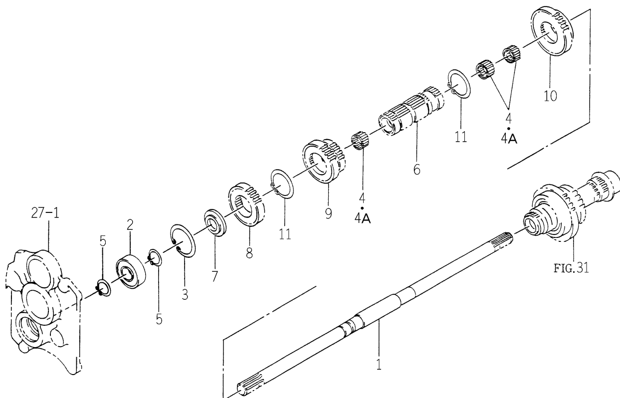
FIG. 28 MAIN CHANGE GEAR SYSTEM (EXCEPT H TYPE)
