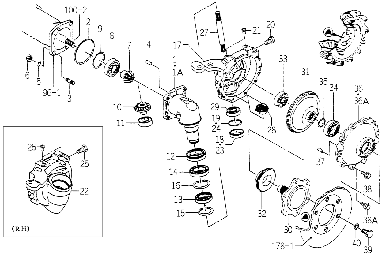
FIG. 98 FINAL GEAR CASE SYSTEM
