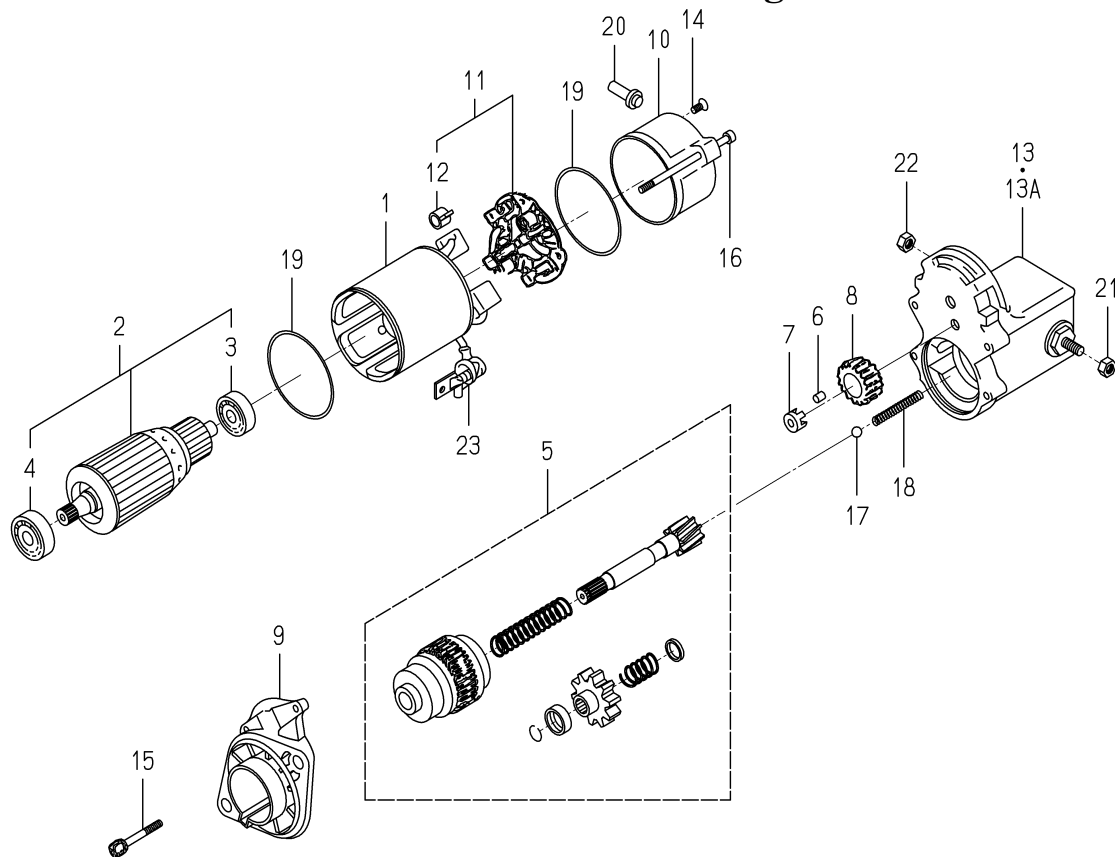
FIG. 31 COMPONENT PARTS FOR 6281-100-002-30 ON Fig.25
