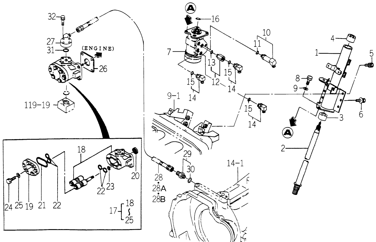
FIG. 86 STEERING (ORBIT) SYSTEM (H TYPE)(1/2)
