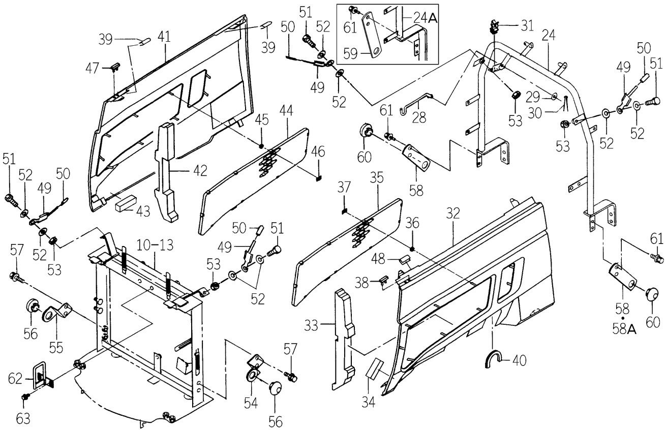
FIG.124 HOOD SYSTEM(2/2)
