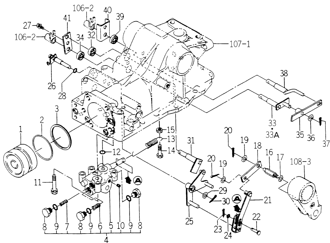
FIG.109 CYLINDER SYSTEM
