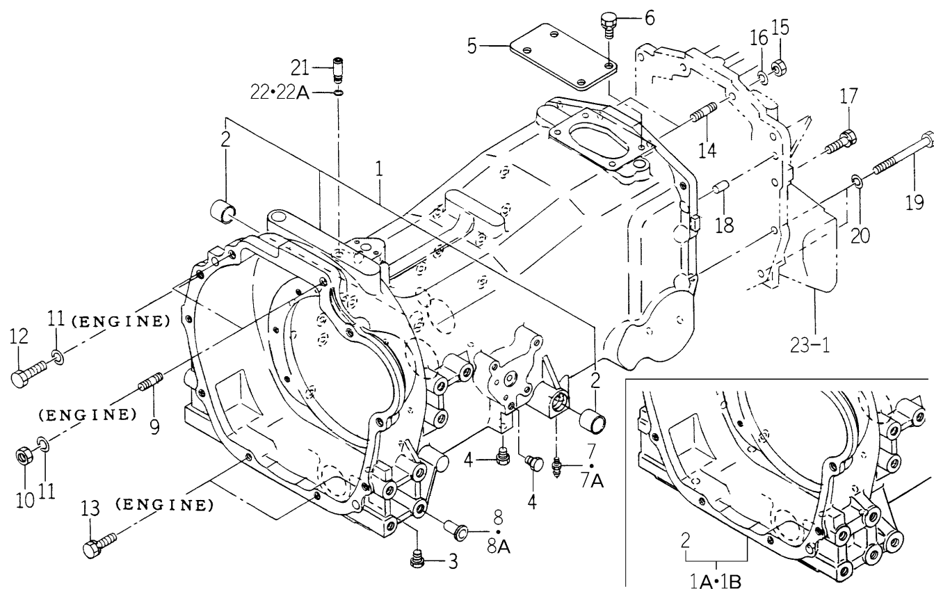
FIG. 14 FRONT MISSION CASE SYSTEM (H TYPE)
