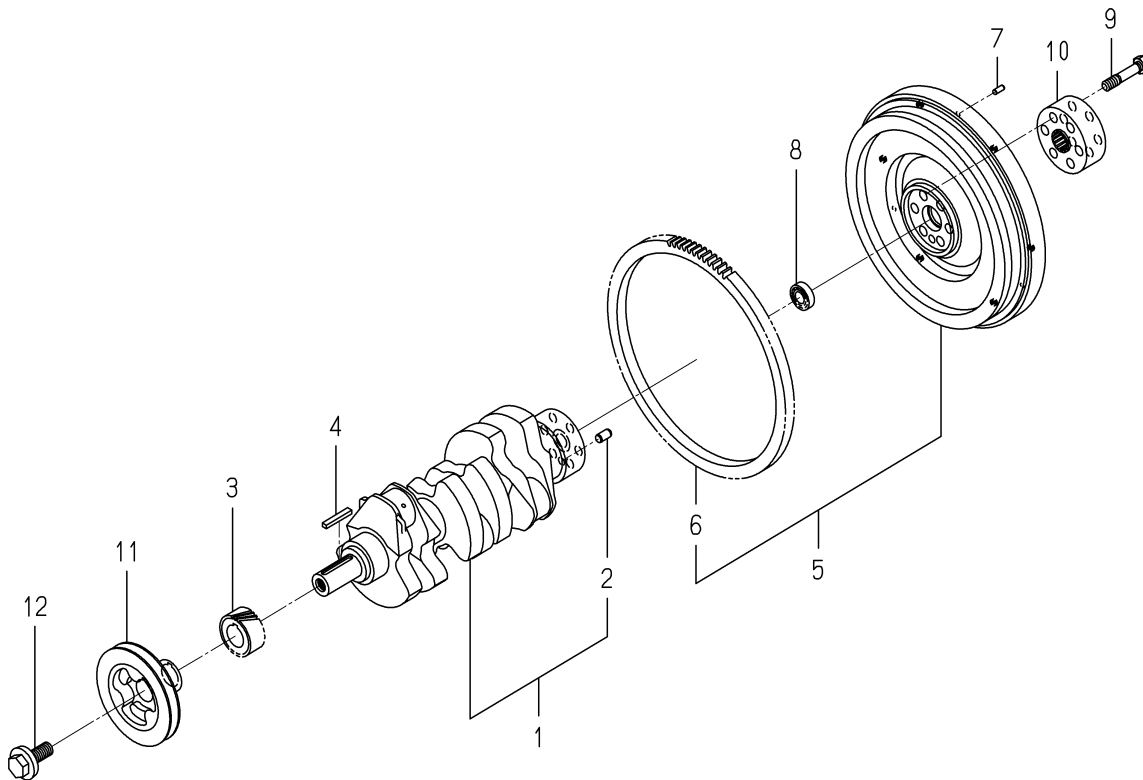
FIG. 16 CRANK SHAFT
