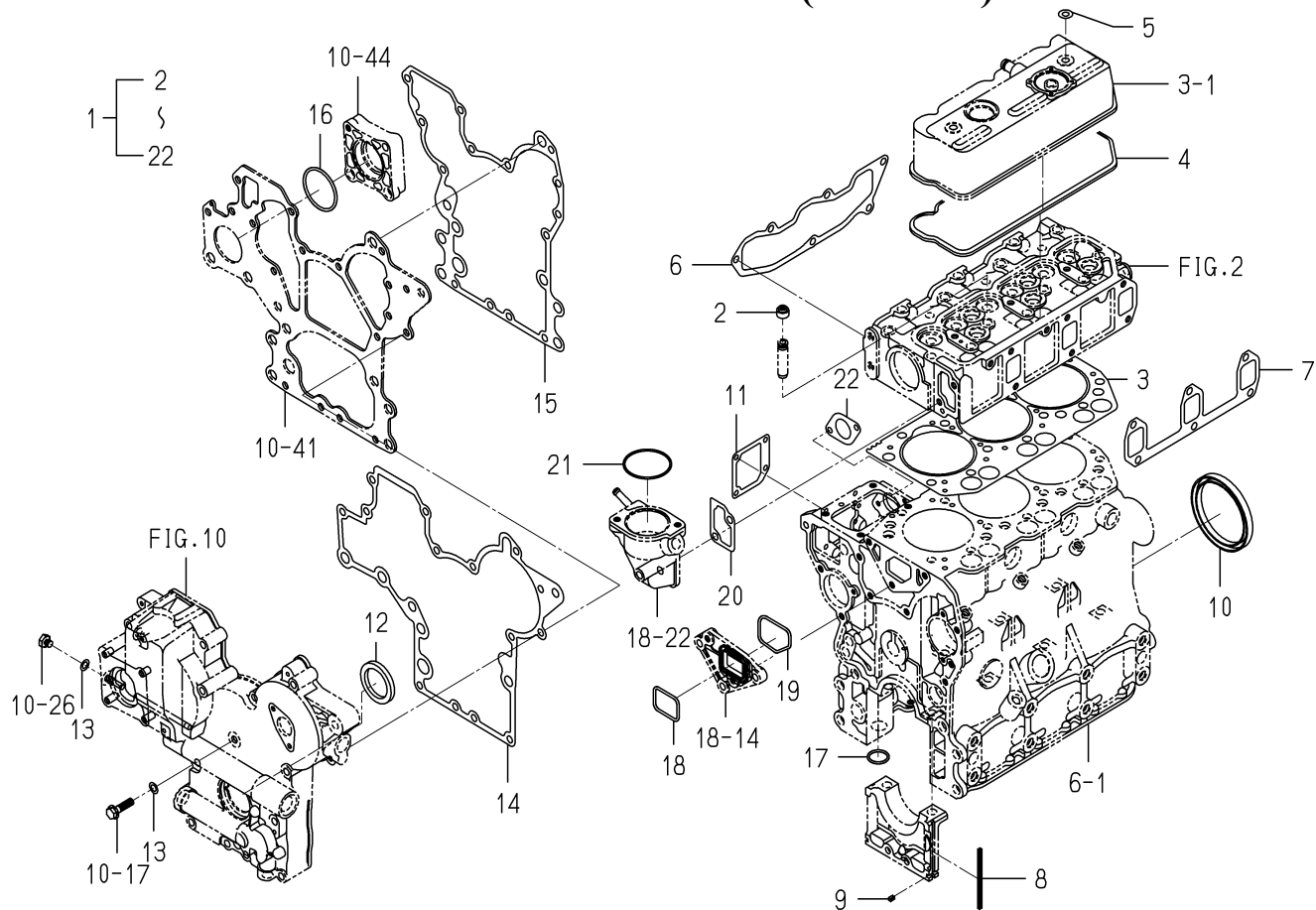
FIG. 27 REPAIR PARTS(OPTION)
