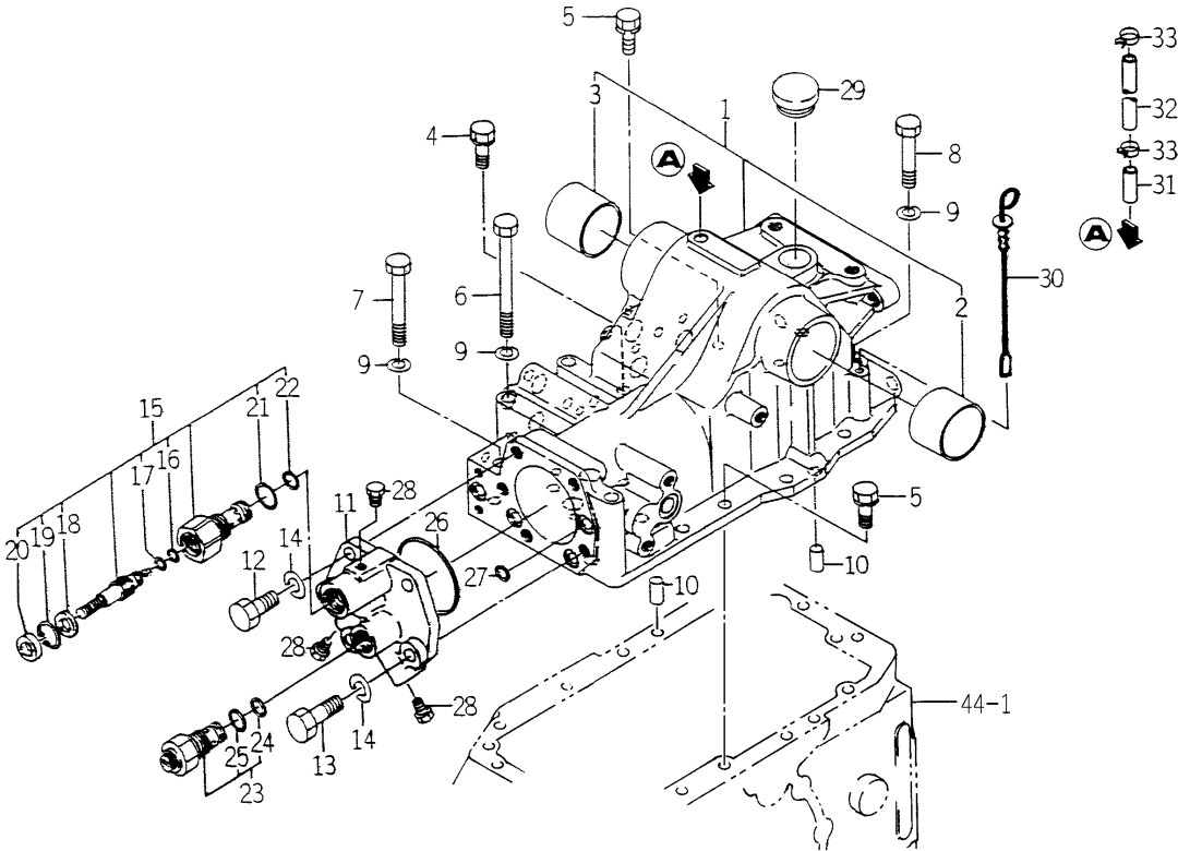
FIG.105 CASE (CYLINDER) SYSTEM (H TYPE-TH4260H-No.10823~/ 4290H-10464~/4330H-10977~)
