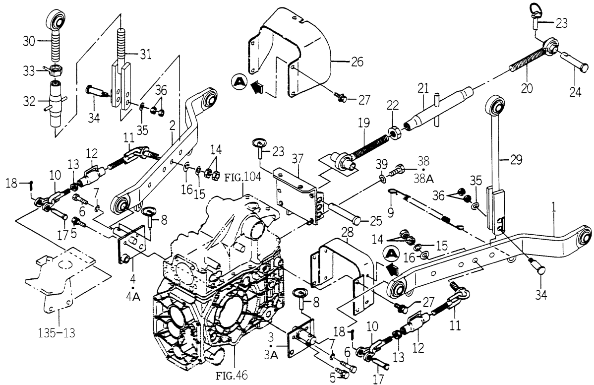
FIG.117 LINK (3P) SYSTEM (H TYPE-TH4260H-No.1~10822/ 4290H-1~10463/4330H-1~10976)
