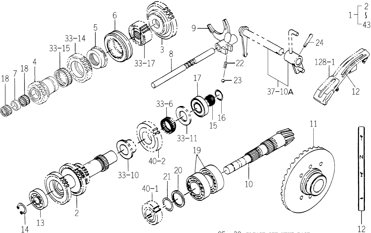
FIG.166 GEAR (SUB) SYSTEM(1/2) (H TYPE EXCEPT W-REPAIR)
