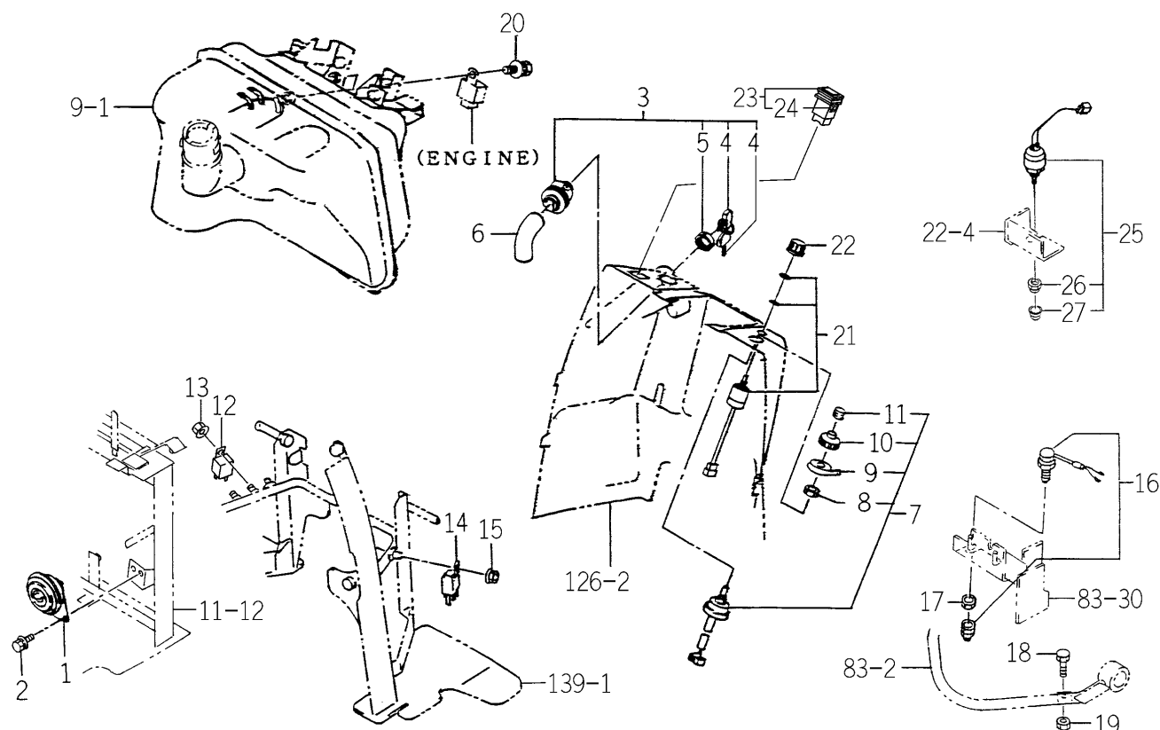
FIG.148 SWITCH SYSTEM (EXCEPT H TYPE)
