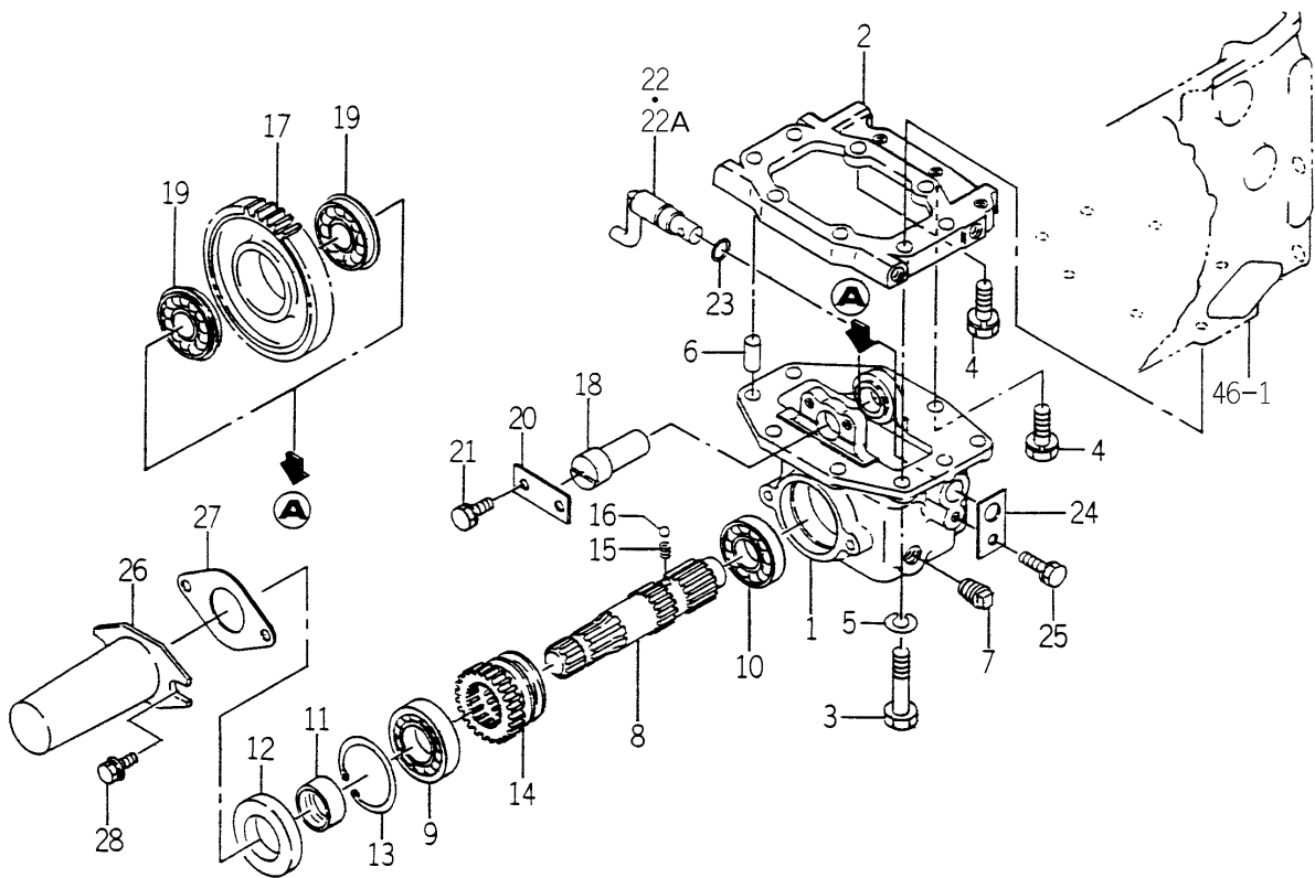
FIG. 53 MID PTO SYSTEM (H TYPE-TH4260H-No.1~10822/ 4290H-1~10463/4330H-1~10976)
