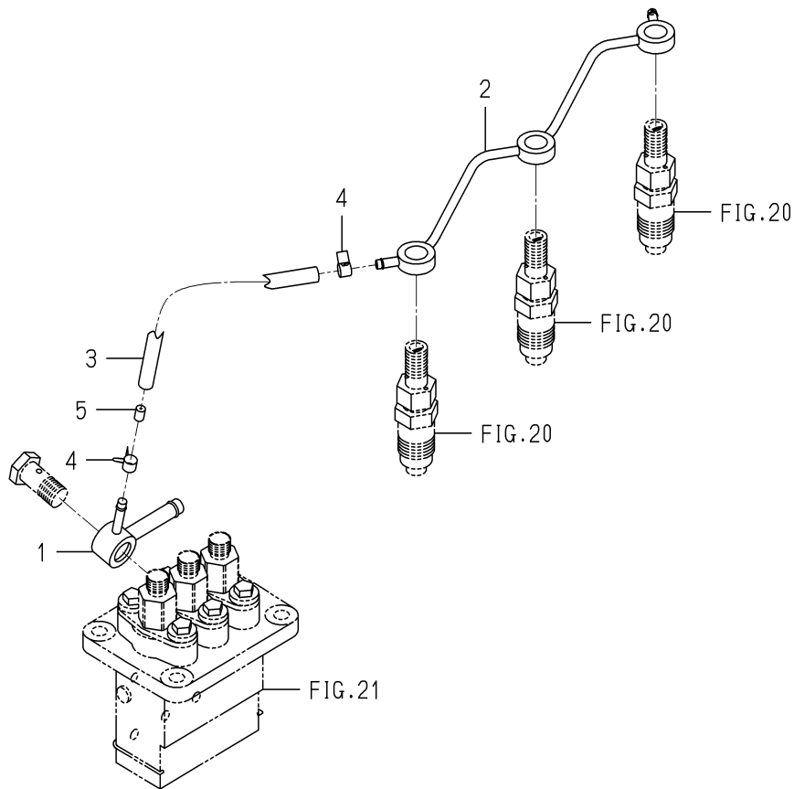
FIG. 22 FUEL PIPE
