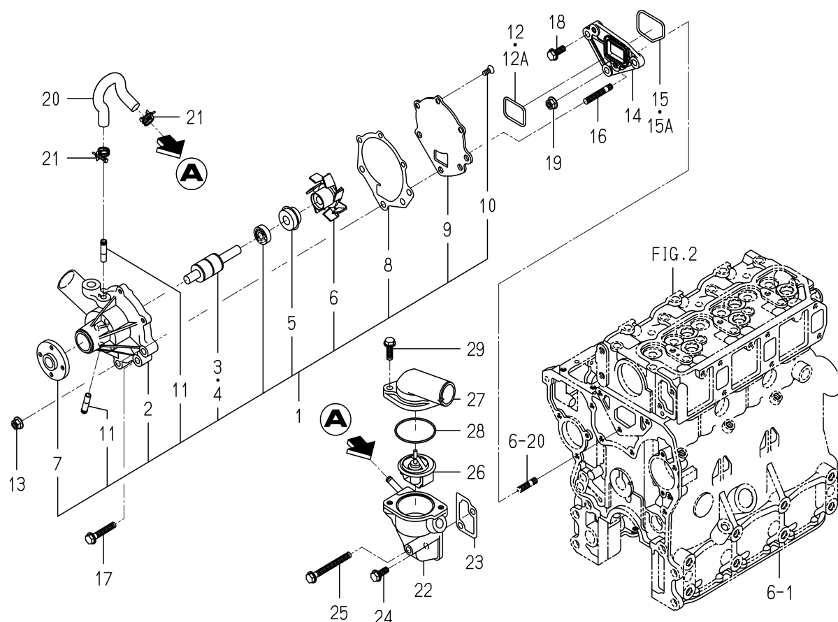
FIG. 18 WATER PUMP
