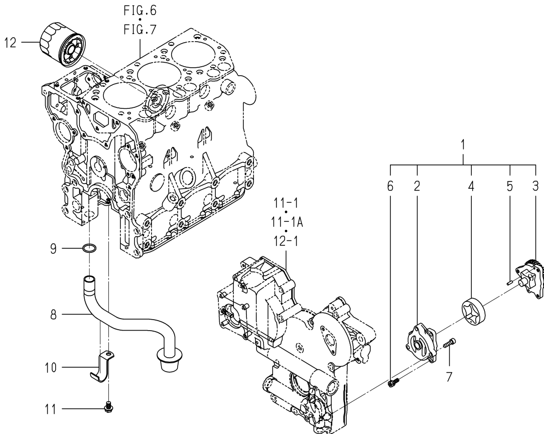
FIG. 21 OIL PUMP
