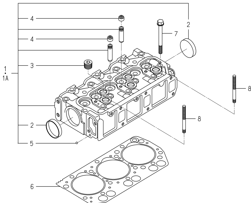
FIG. 2 CYLINDER HEAD
