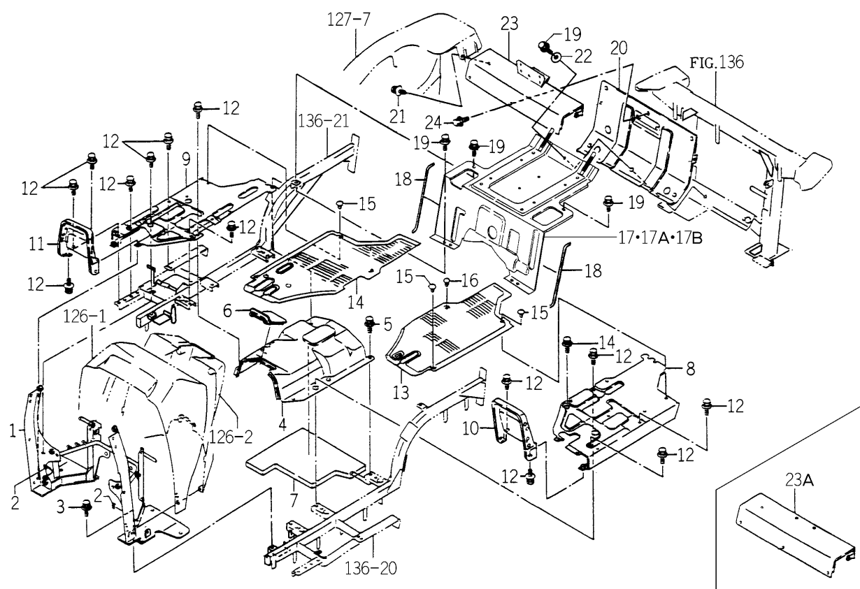
FIG.139 FLOOR SYSTEM (EXCEPT H TYPE)
