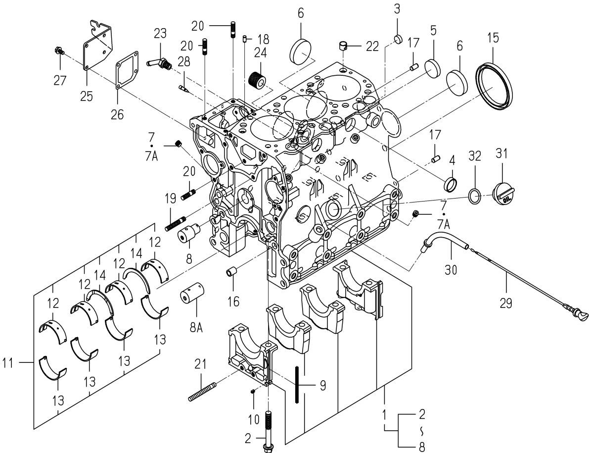
FIG. 7 CYLINDER BLOCK
