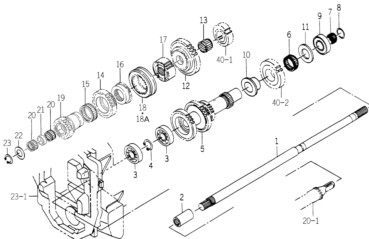
FIG. 33 SUB COUNTER GEAR SYSTEM (H TYPE-TH4260H-No.10224~/ 4290H-10185~/4330H-10218~)
