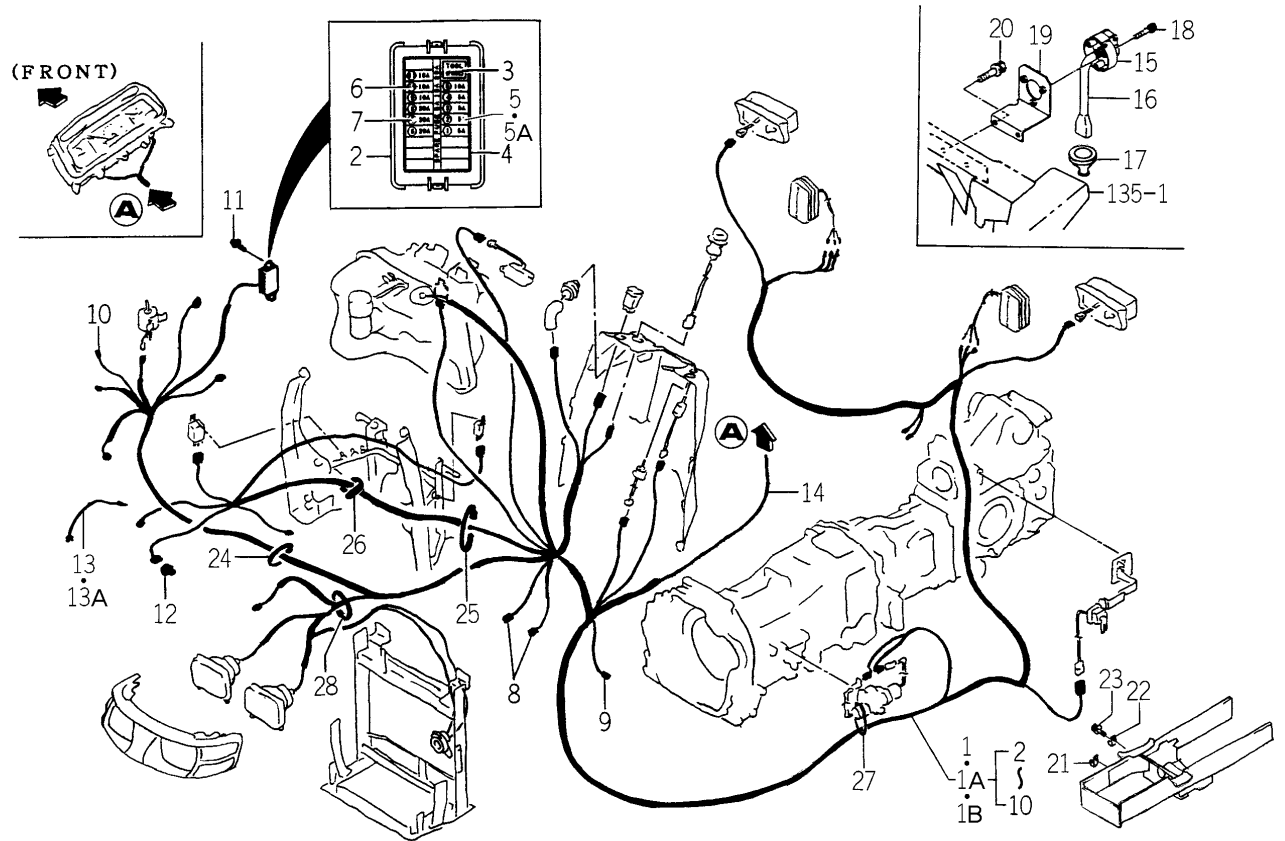
FIG.149 HARNESS SYSTEM (TH4260-H TYPE)
