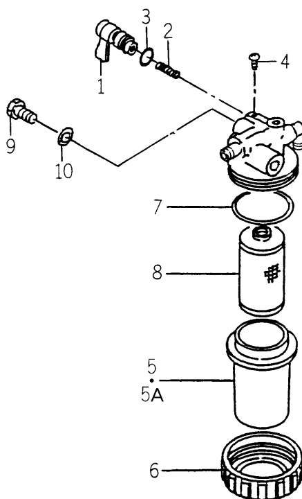
FIG.196 COMPONENT PARTS FOR 1588-105-220-00 ON Fig.5,6
