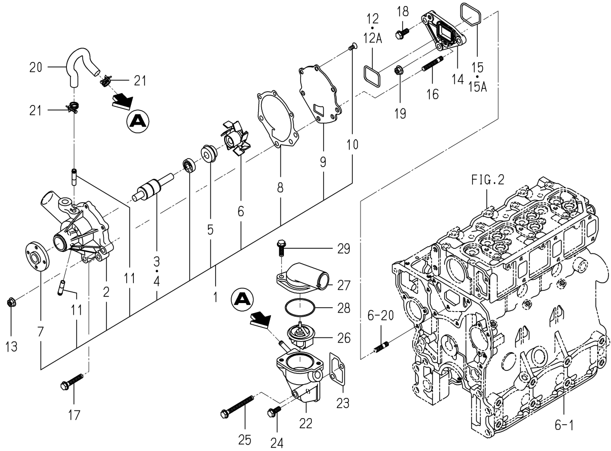
FIG. 18 WATER PUMP
