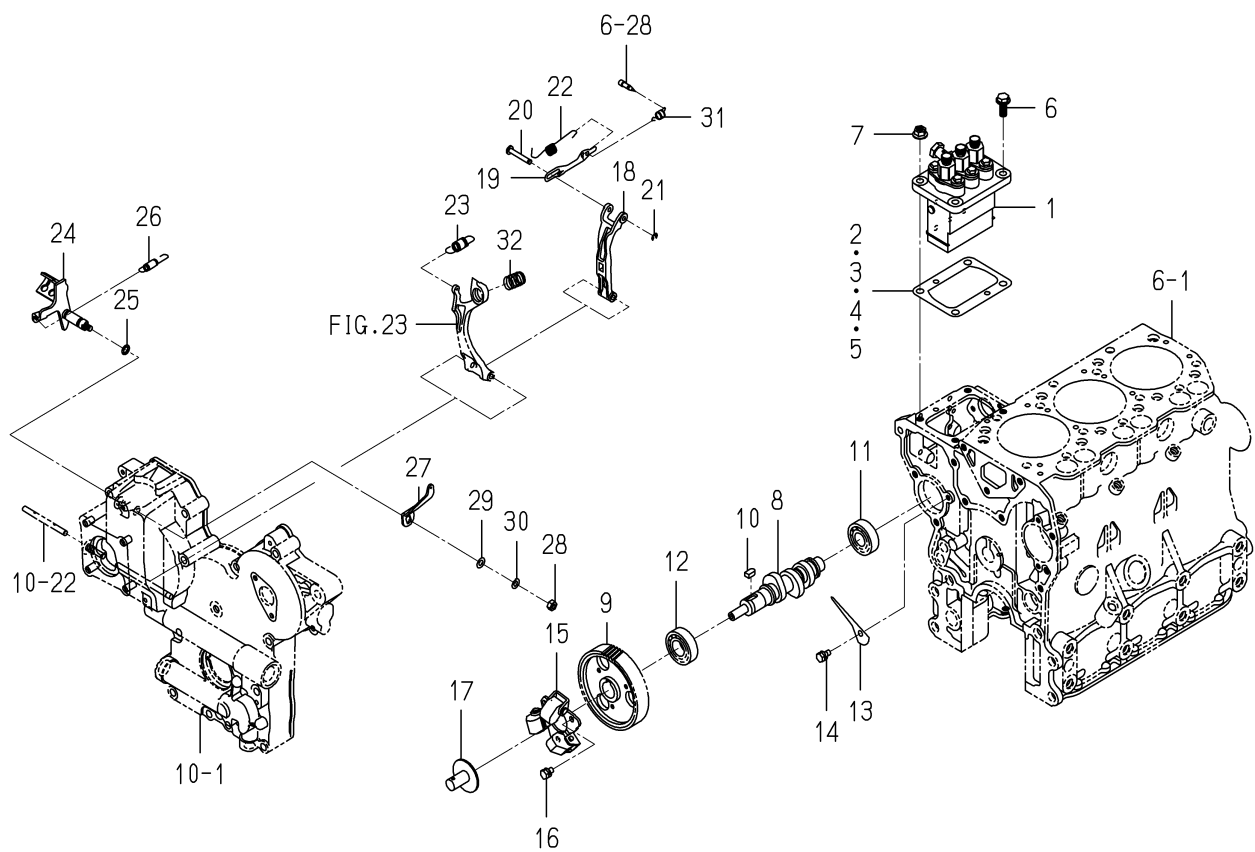
FIG. 21 INJECTION PUMP
