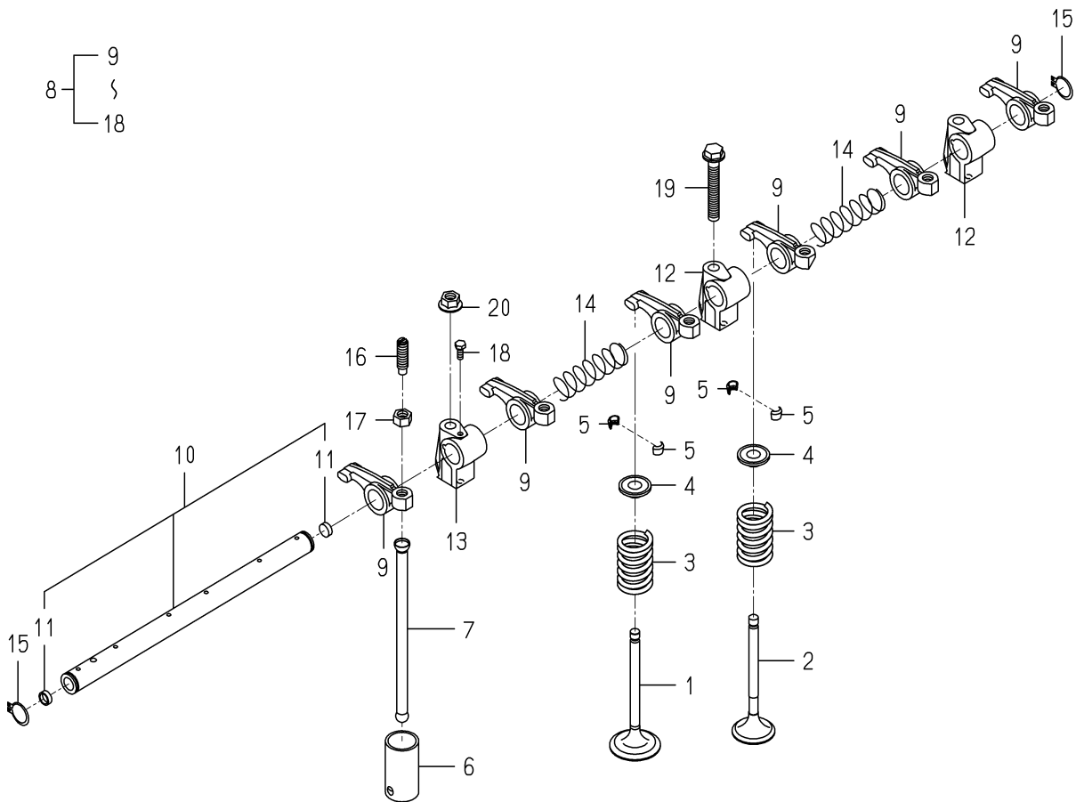
FIG. 12 VALVE
