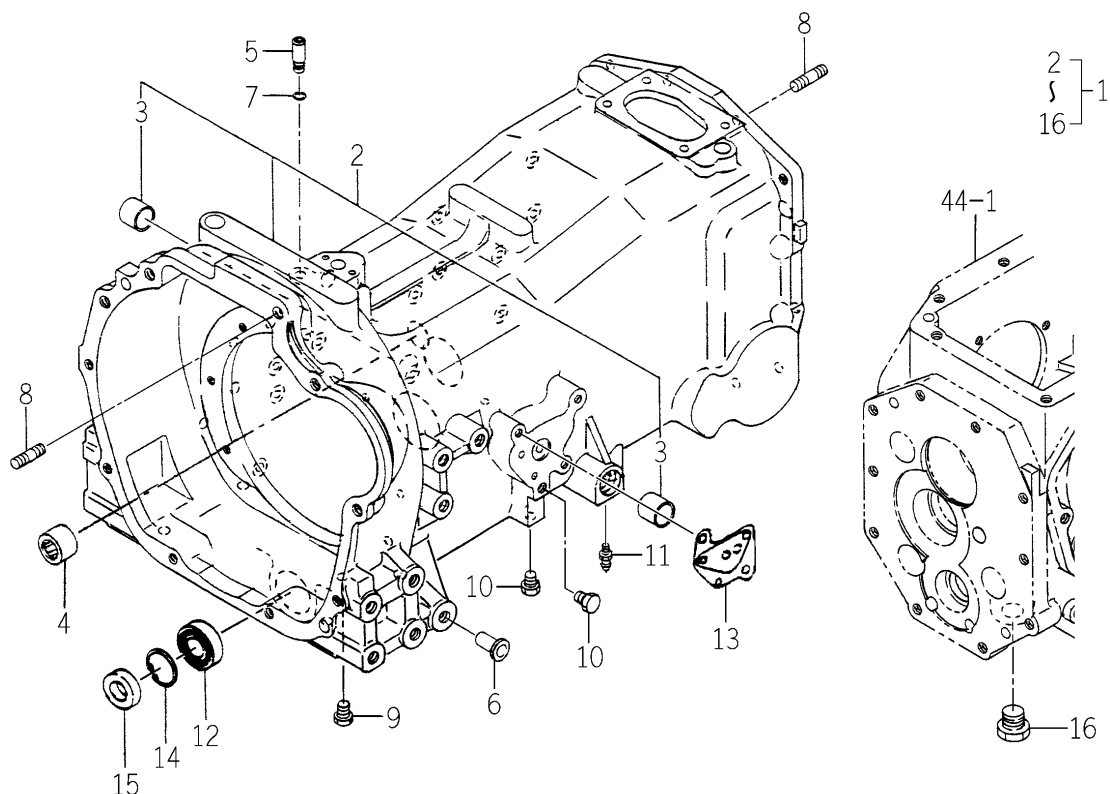
FIG.165 CASE (TRANSMISSION/FRONT) SYSTEM (H TYPE-REPAIR)
