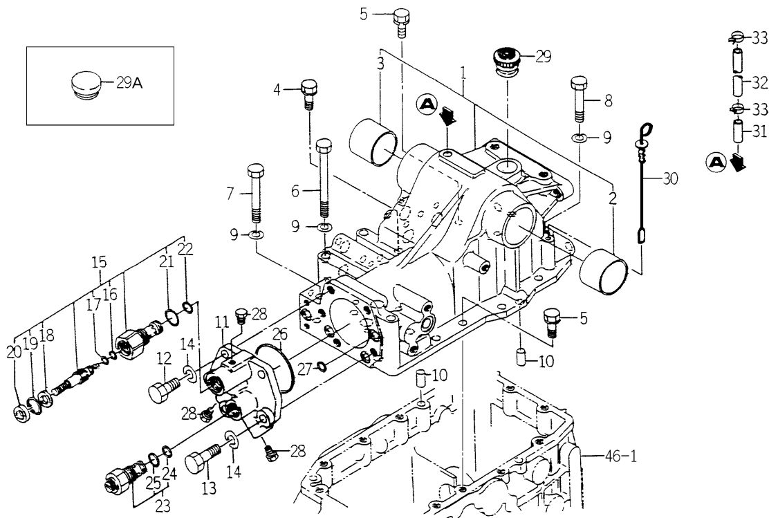
FIG.104 CASE (CYLINDER) SYSTEM (H TYPE-TH4260H-No.1~10822/ 4290H-1~10464/4330H-1~10976)
