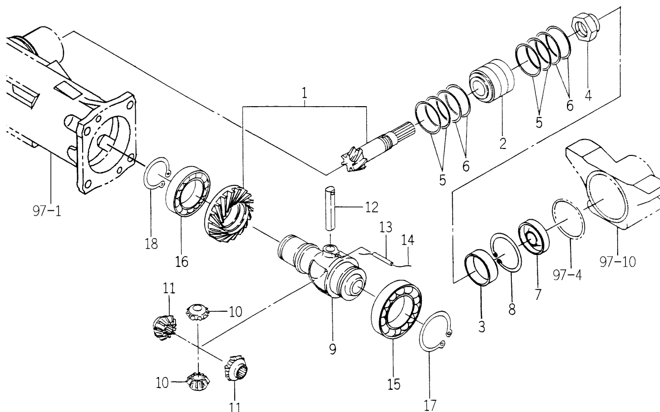
FIG. 95 BEVEL CASE SYSTEM (H TYPE)
