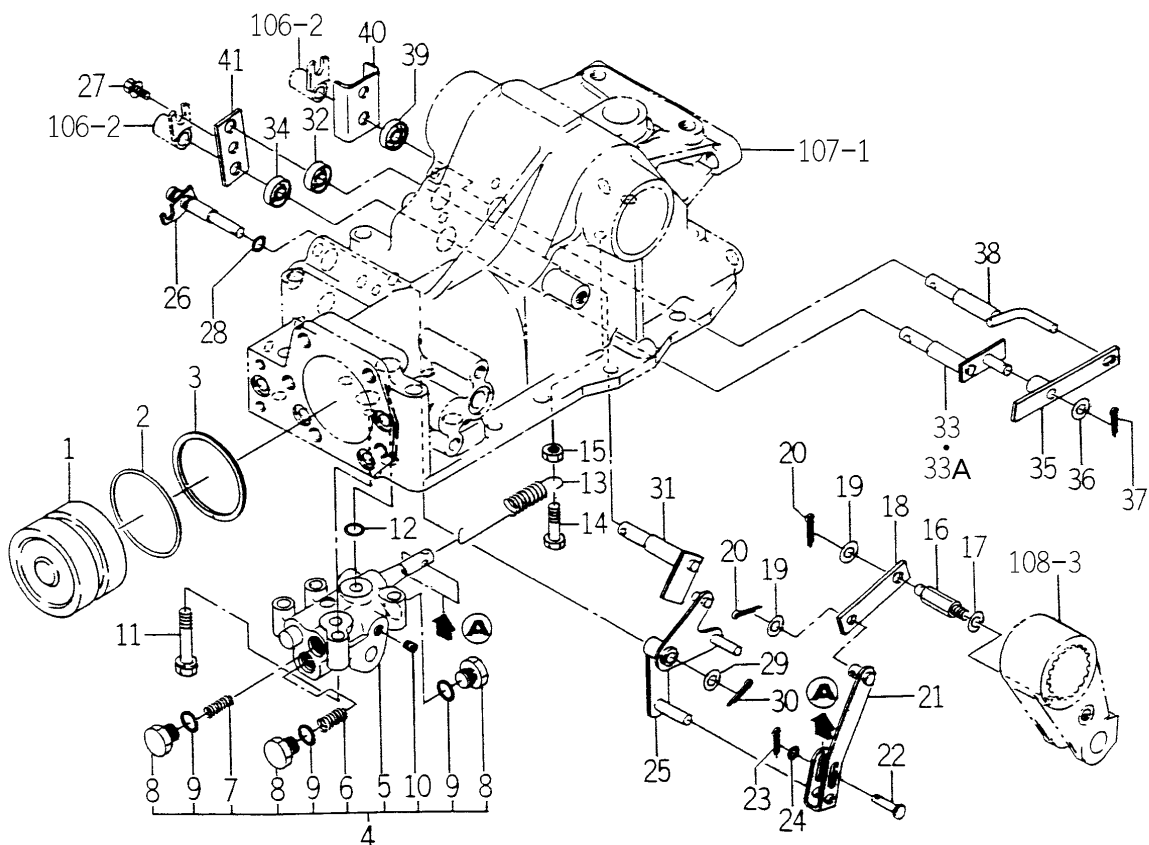
FIG.109 CYLINDER SYSTEM
