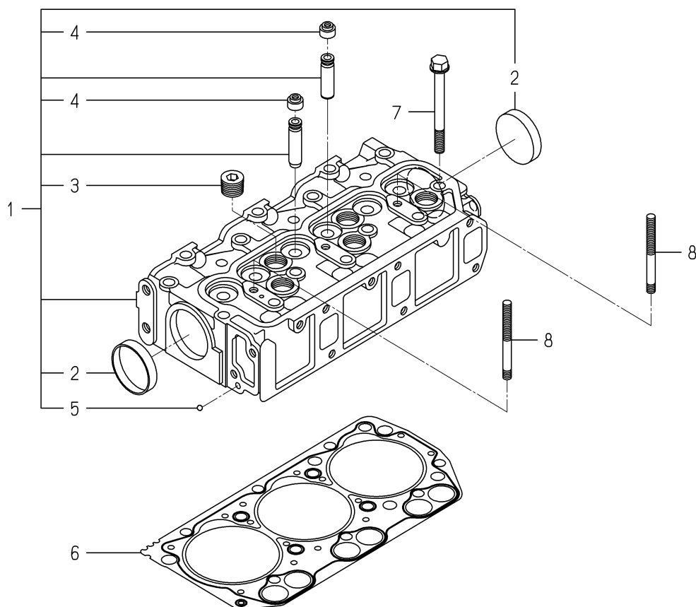
FIG. 2 CYLINDER HEAD
