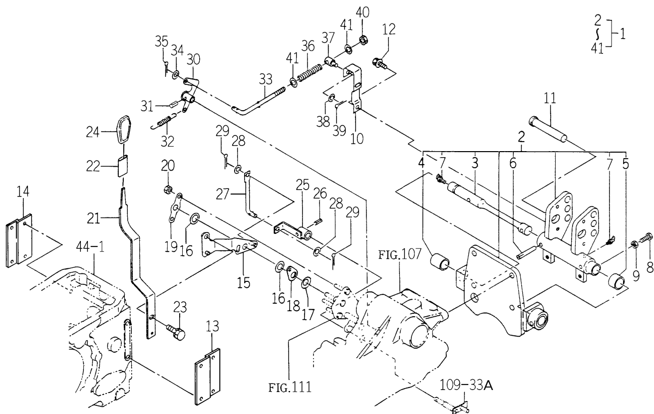
FIG.188 DRAFT SET (OPTION)
