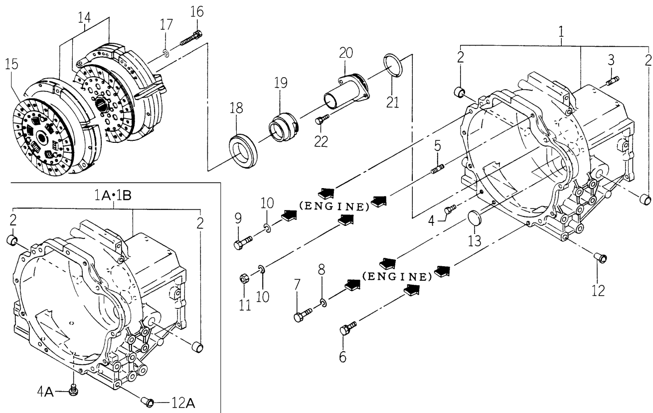
FIG. 15 DUAL CLUTCH SYSTEM (EXCEPT H TYPE)
