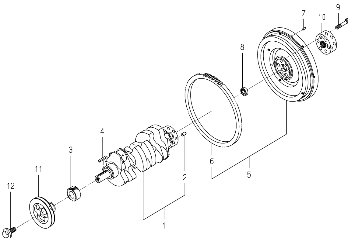
FIG. 16 CRANK SHAFT
