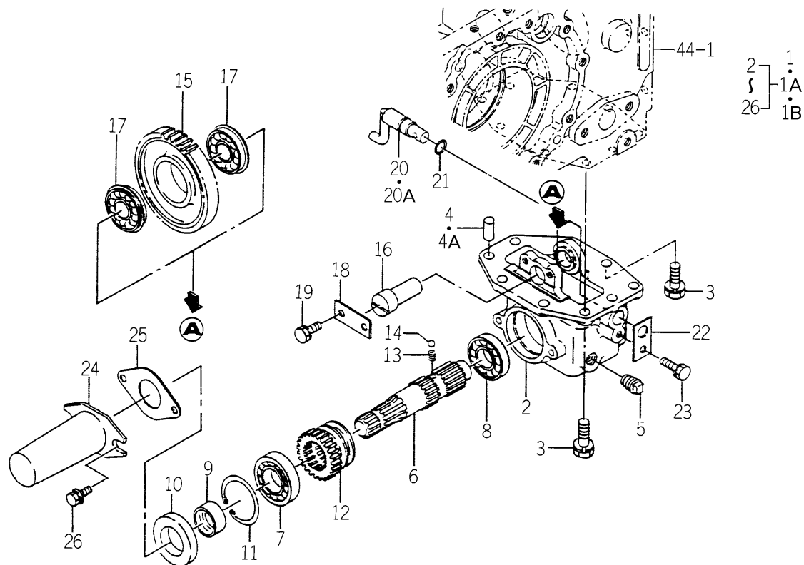
FIG. 55 MID PTO SYSTEM(M TYPE EXCEPT H-STD/ EXCEPT M TYPE-REP-1~)(H TYPE-STD- 4260H-10823~/4290H-10464~/4330H-10977~)
