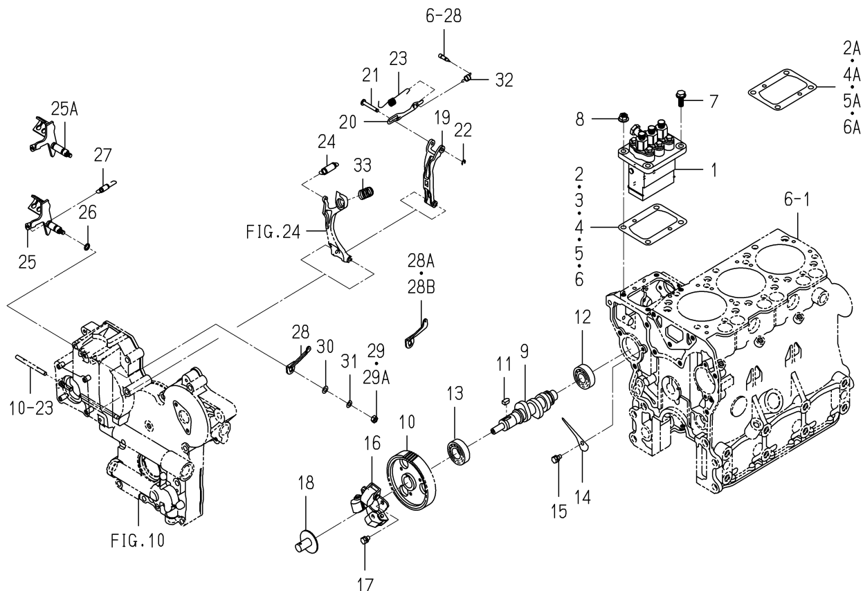
FIG. 22 INJECTION PUMP
