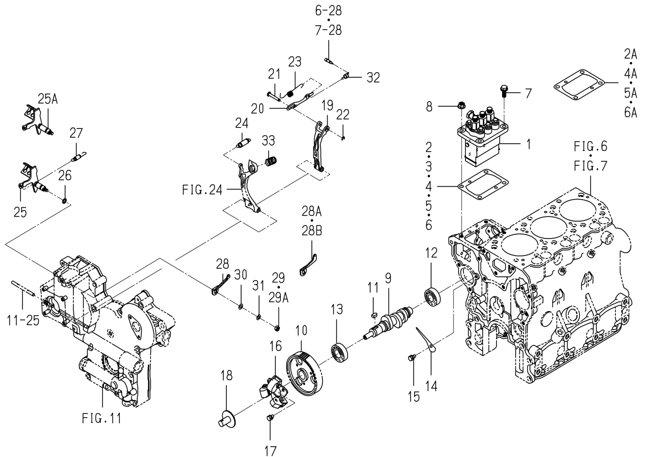
FIG. 22 INJECTION PUMP
