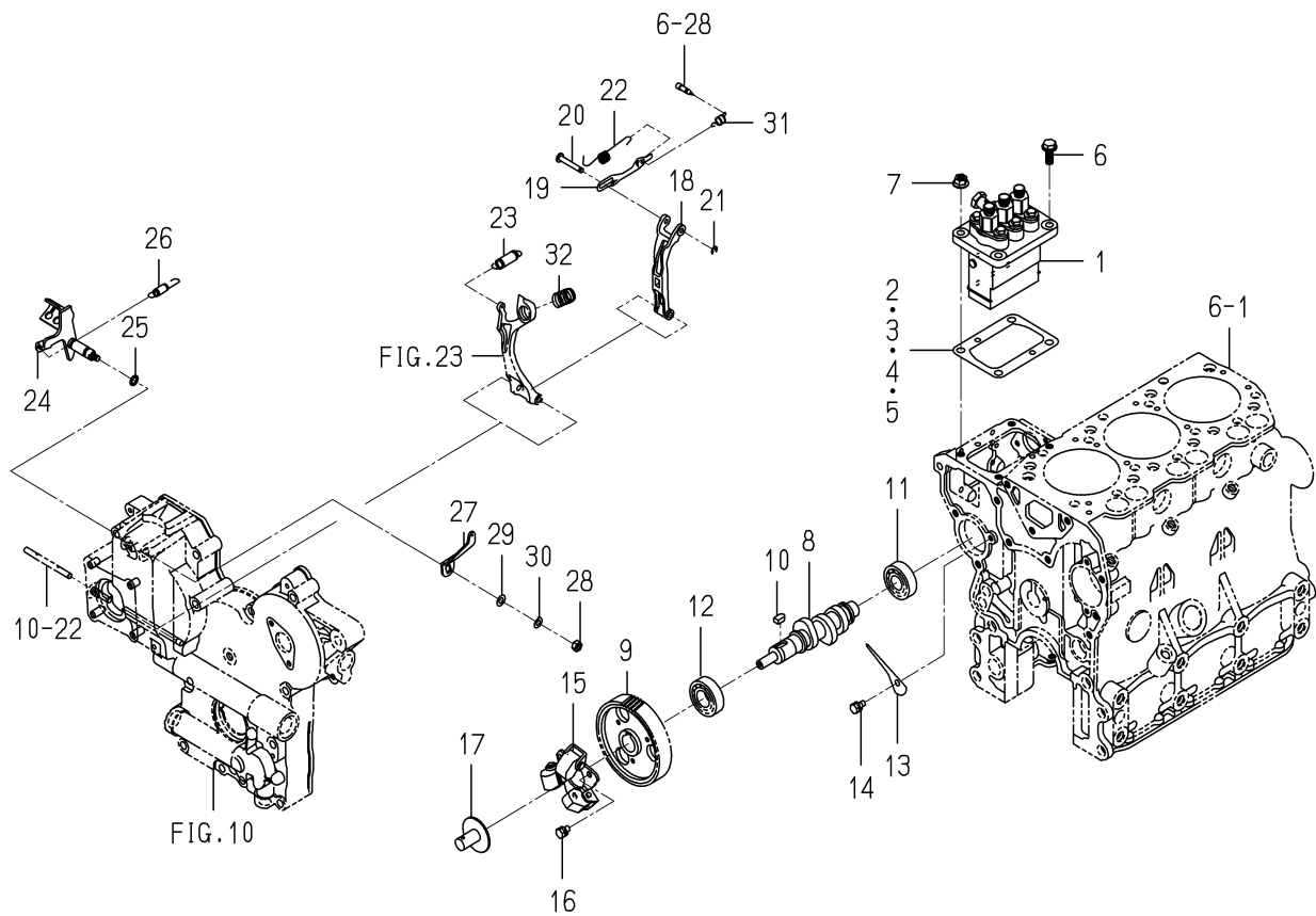
FIG. 21 INJECTION PUMP
