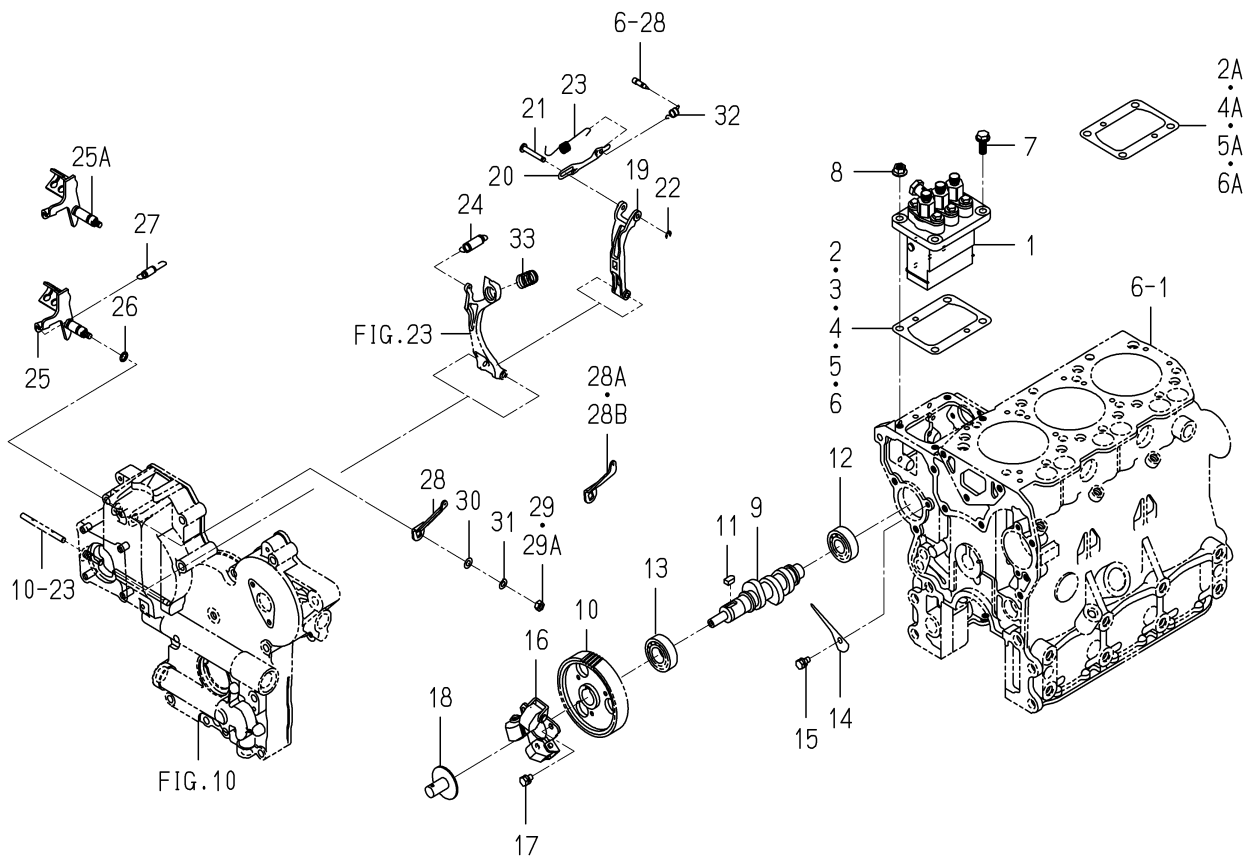
FIG. 21 INJECTION PUMP
