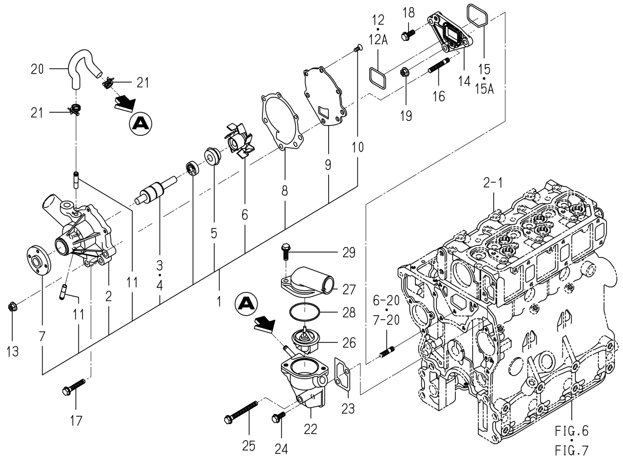
FIG. 19 WATER PUMP
