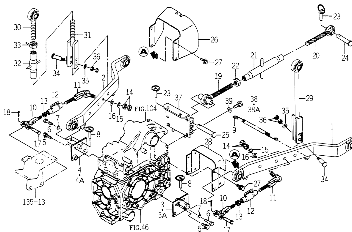
FIG.117 LINK (3P) SYSTEM (H TYPE-TH4260H-No.1~10822/ 4290H-1~10463/4330H-1~10976)
