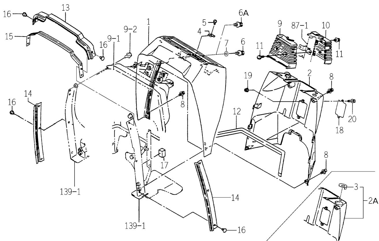
FIG.126 COVER (STEERING) SYSTEM
