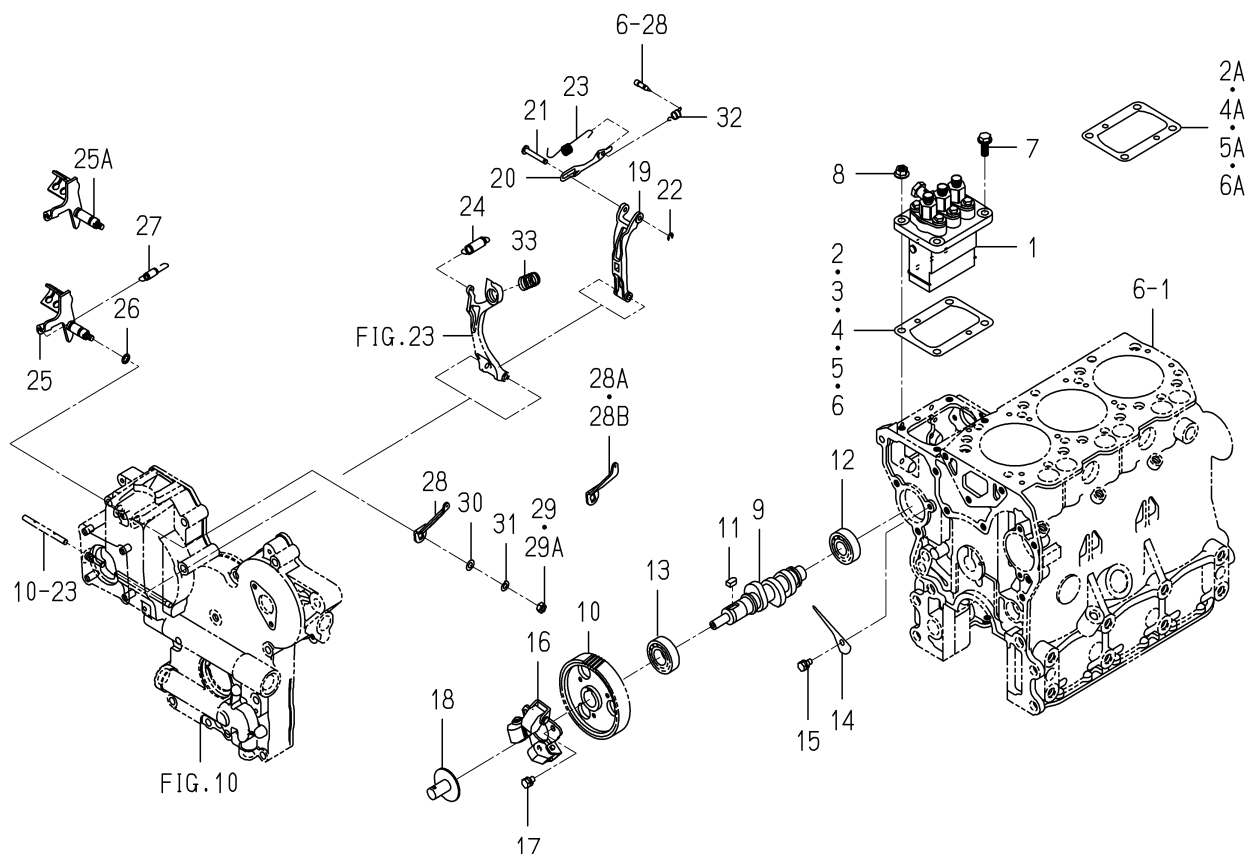
FIG. 21 INJECTION PUMP
