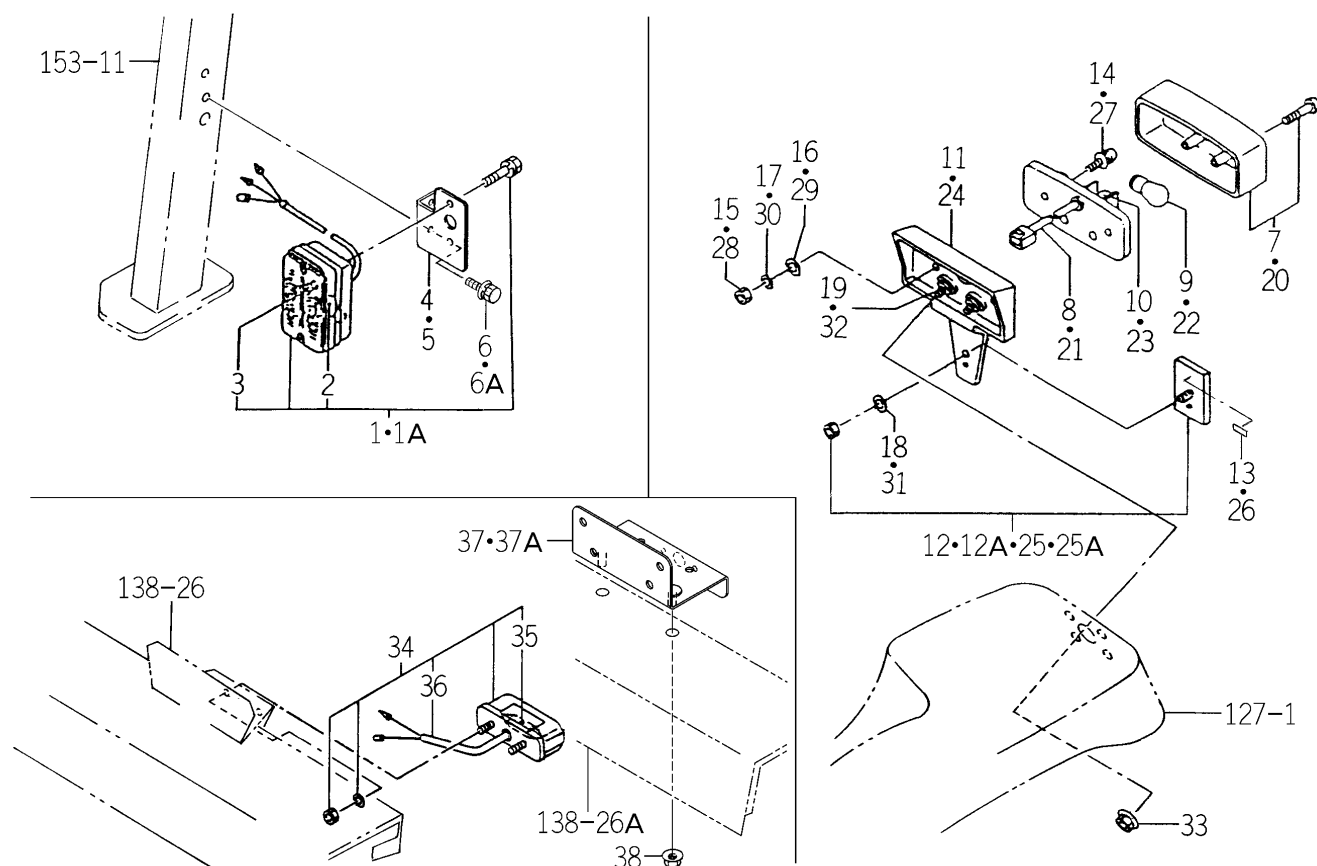
FIG.143 LAMP SYSTEM (H TYPE)
