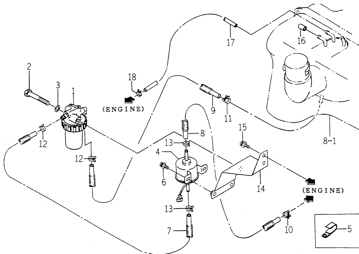
FIG. 5 FILTER (FUEL) SYSTEM (TH4260)
