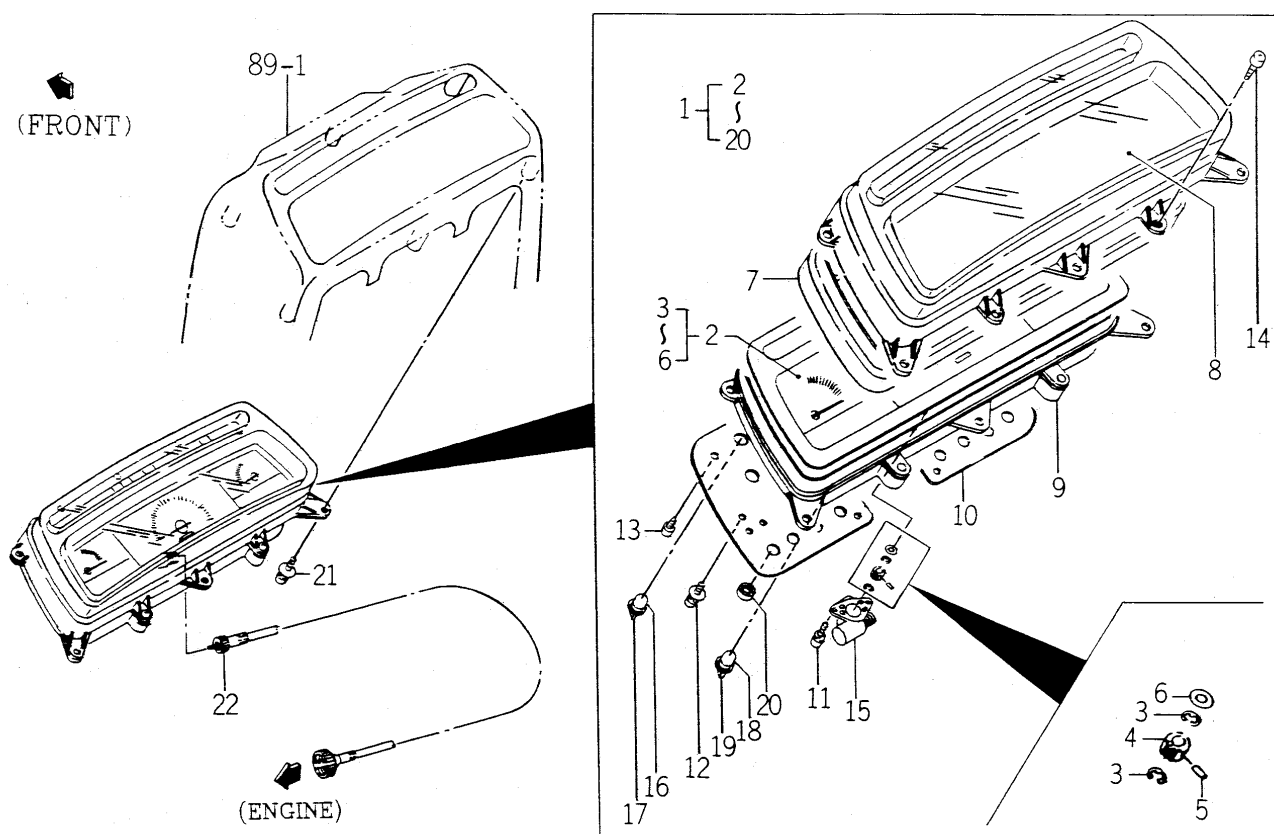
FIG.104 PANEL SYSTEM
