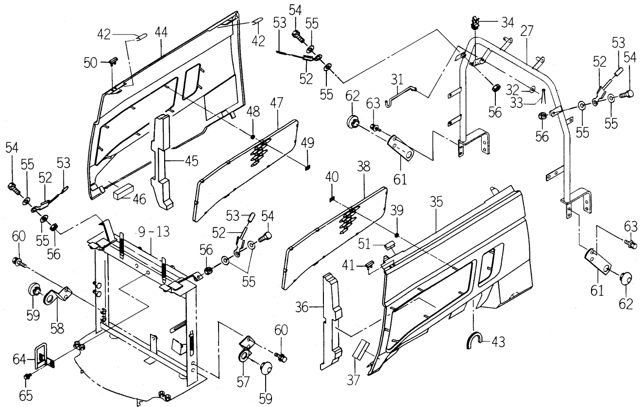
FIG. 87 HOOD SYSTEM(2/2)
