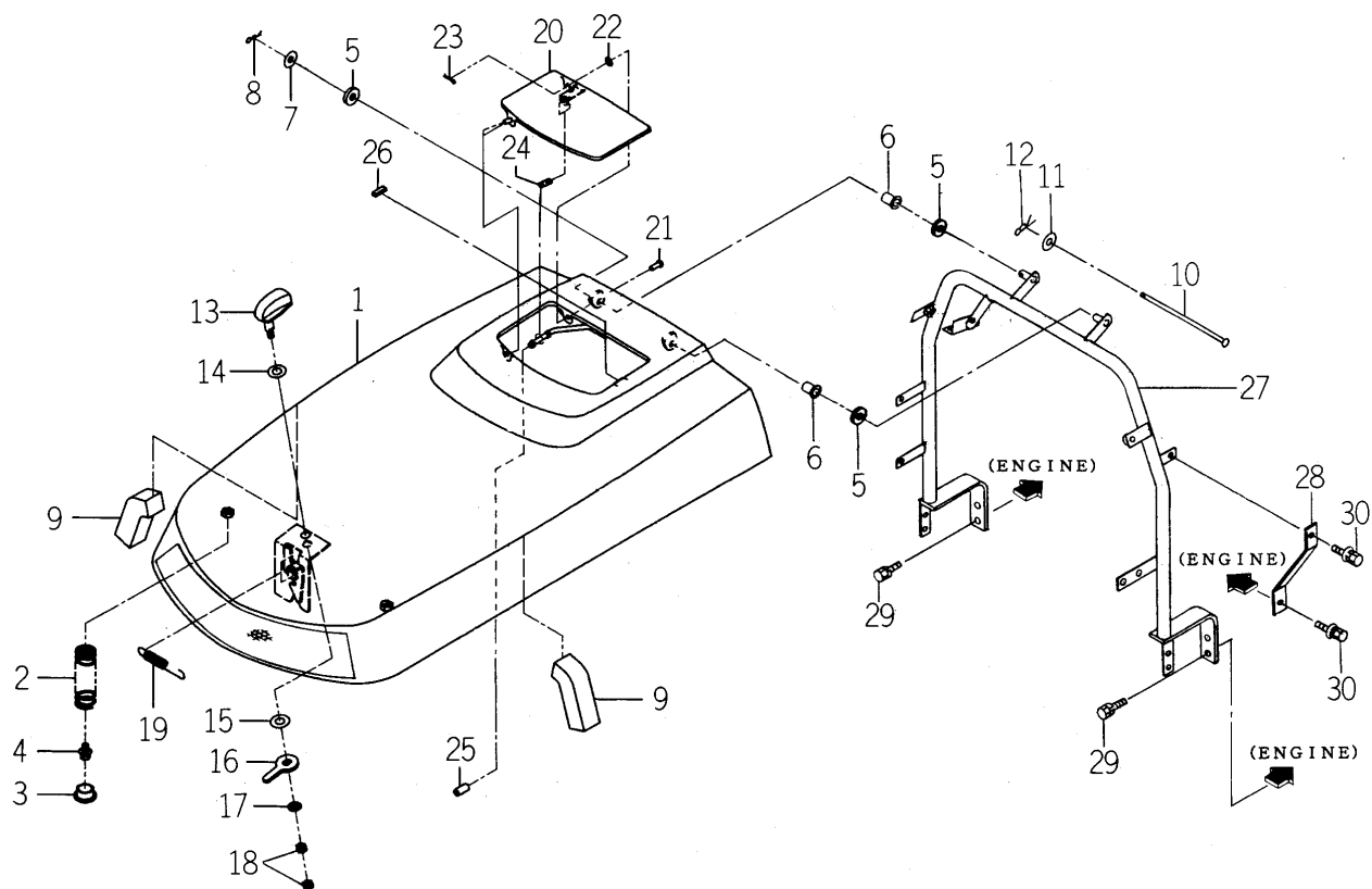
FIG. 87 HOOD SYSTEM(1/2)
