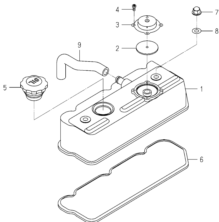
FIG. 2 CYLINDER HEAD COVER
