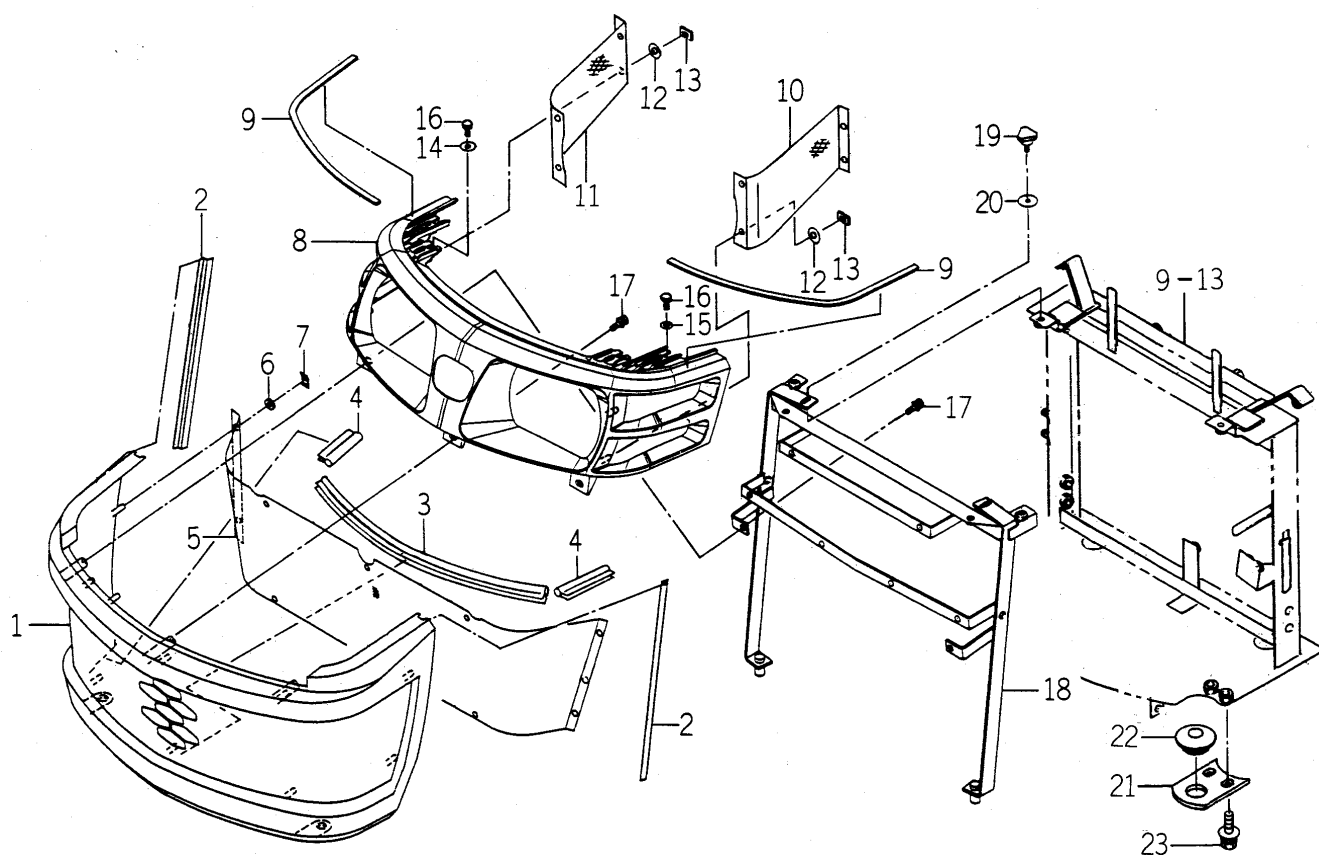
FIG. 88 GRILLE SYSTEM
