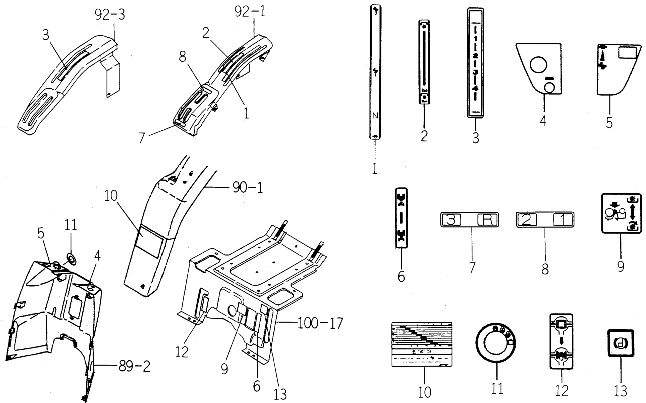
FIG.114 LABEL (EXCEPT H TYPE)
