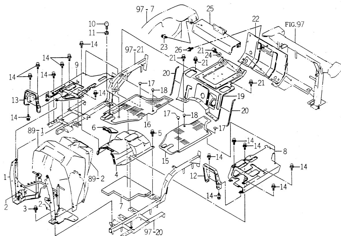
FIG. 99 FLOOR SYSTEM (H TYPE)
