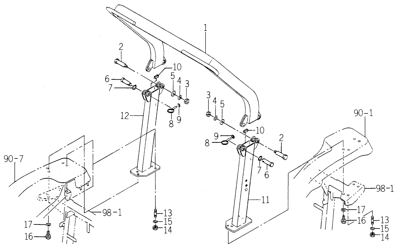
FIG.111 ROPS SYSTEM (R TYPE)
