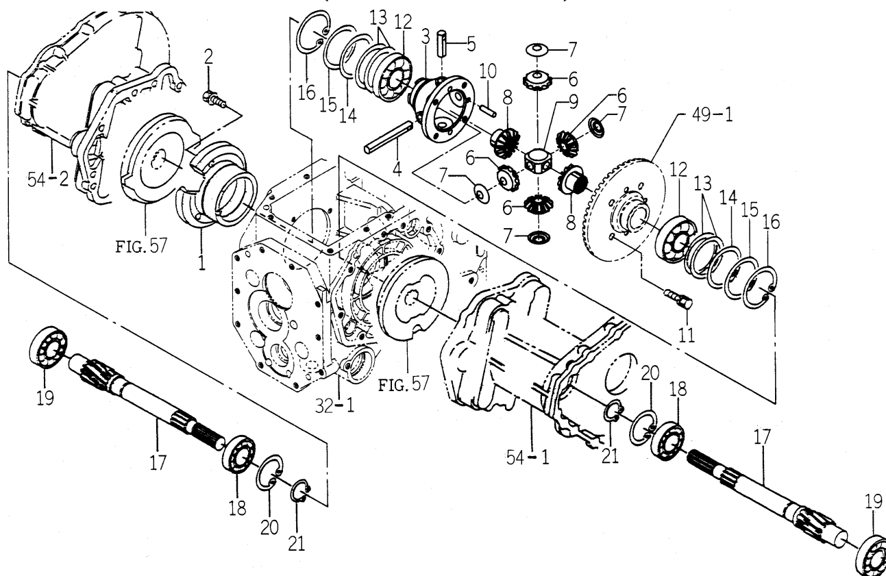
FIG. 52 DIFFERENTIAL CASE SYSTEM (EXCEPT H TYPE)
