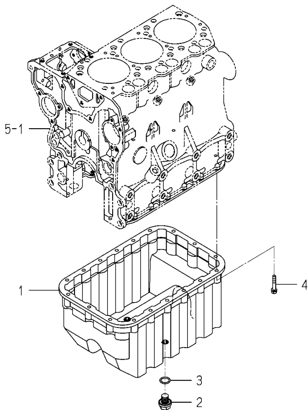
FIG. 7 OIL PAN
