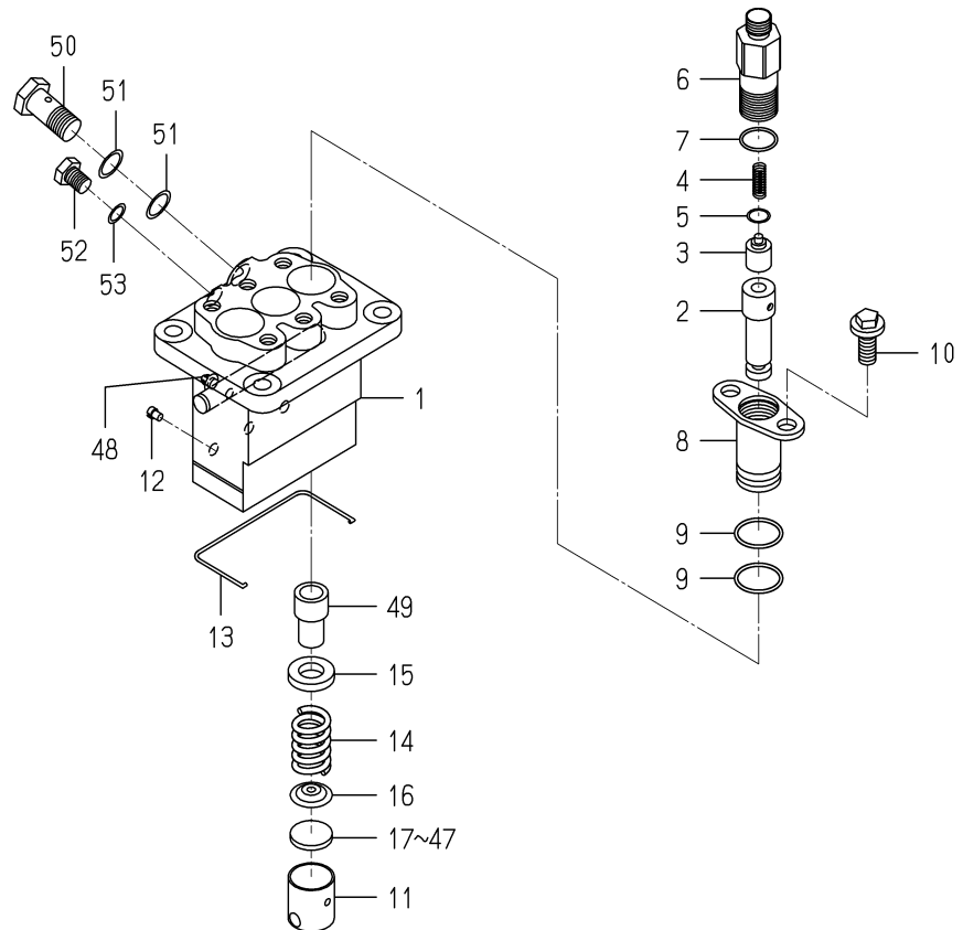
FIG. 27 COMPONENT PARTS FOR 6215-600-104-20 ON Fig.20
