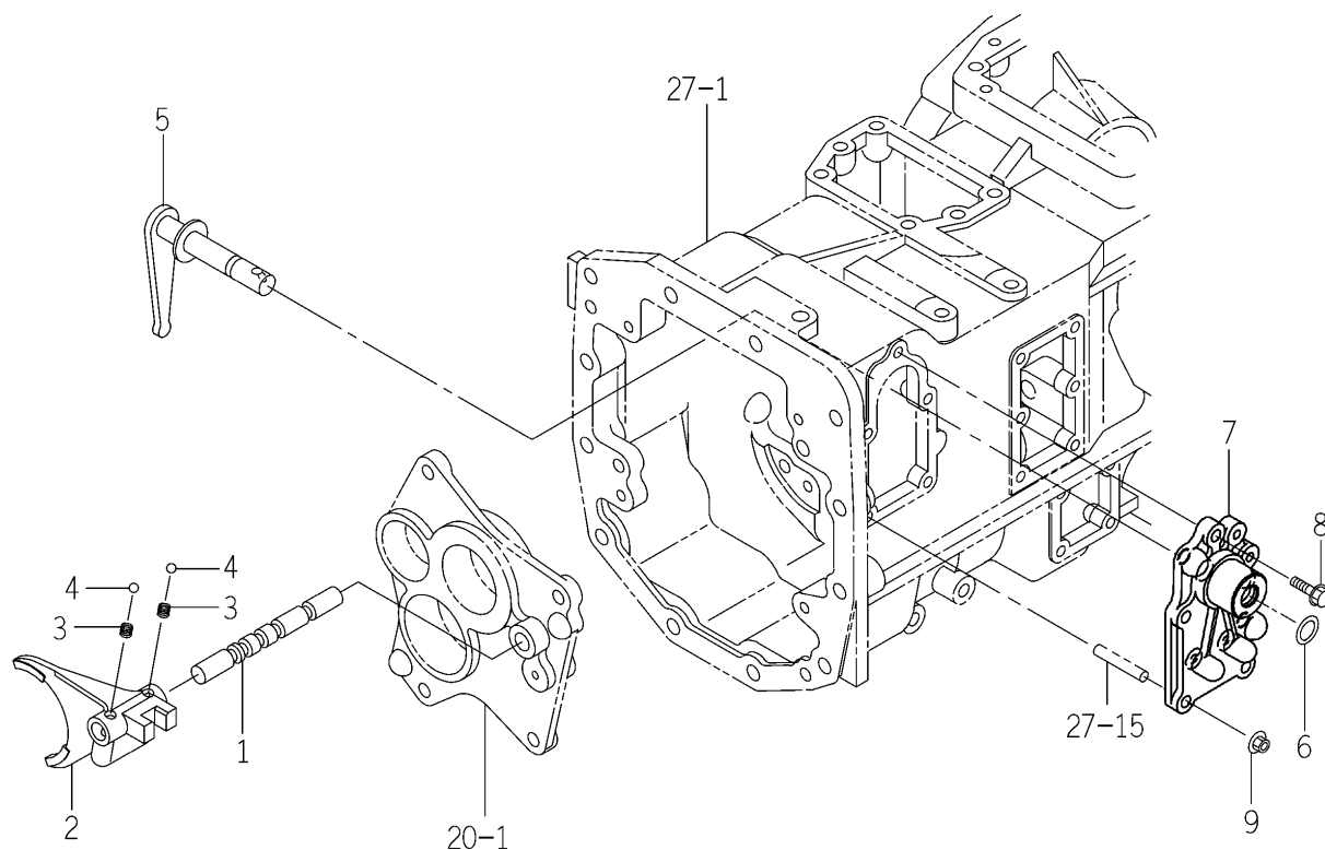
FIG. 30 FORK (SHIFT/MAIN) SYSTEM (EXCEPT S TYPE)
