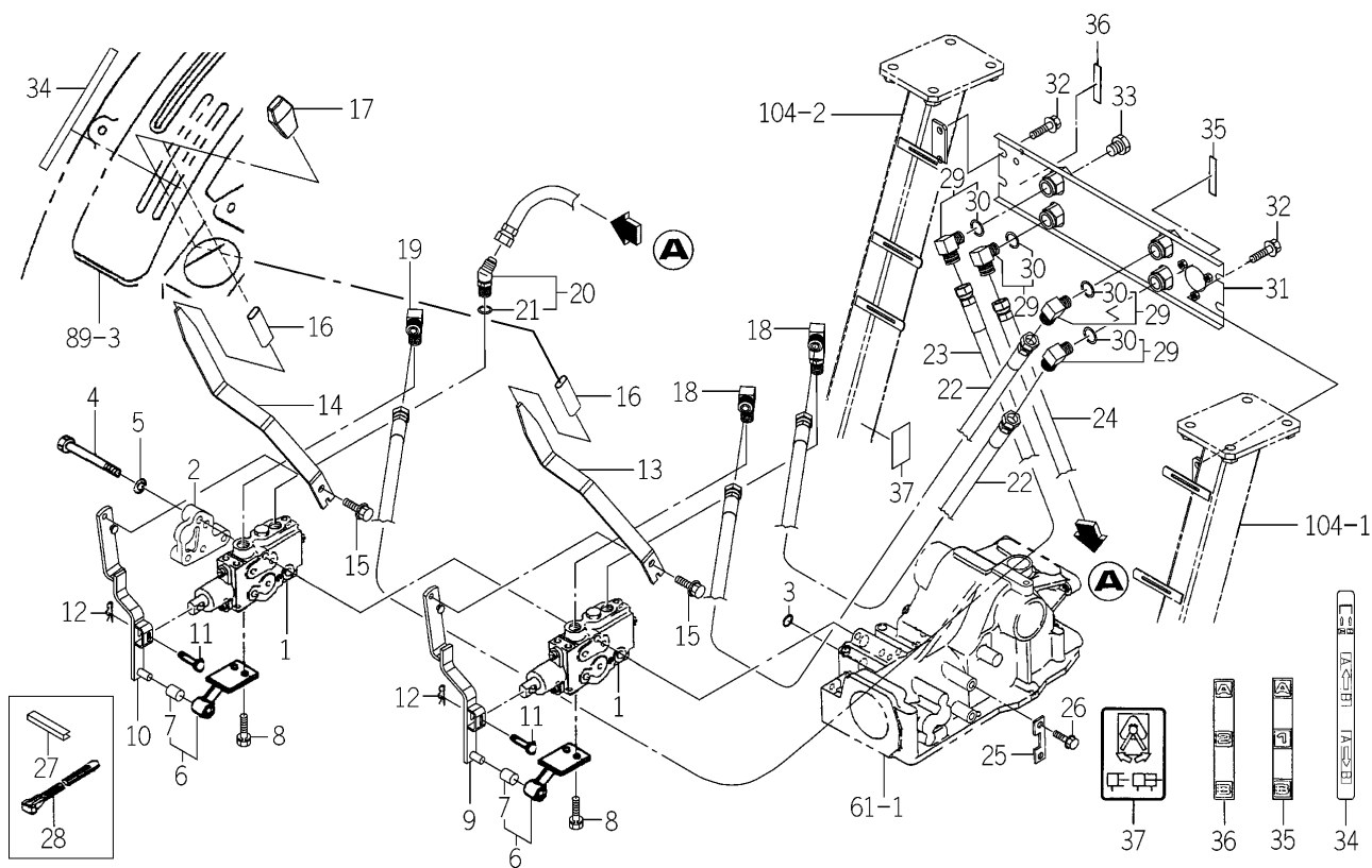
FIG. 71 VALVE (REMOTE/2R) SYSTEM (WR TYPE)
