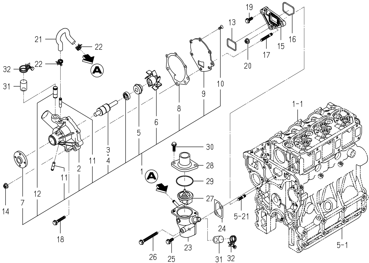
FIG. 17 WATER PUMP
