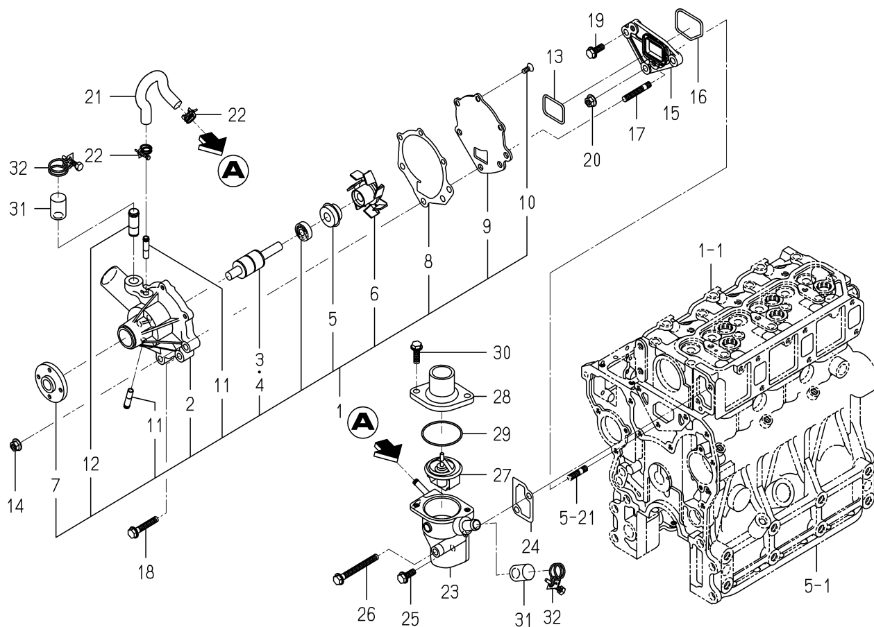
FIG. 17 WATER PUMP
