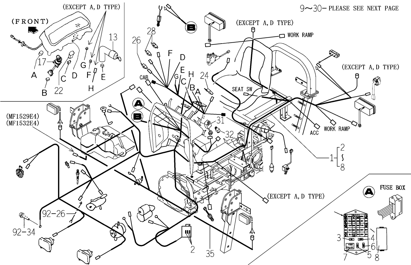
FIG. 94 ELC. SYSTEM (MAIN) (A,D TYPE)(1/2)
