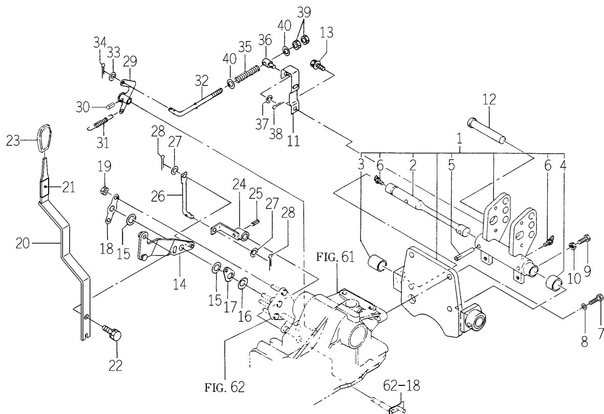
FIG. 64 MECHANICAL LINK (DRAFT) SYSTEM (A TYPE)
