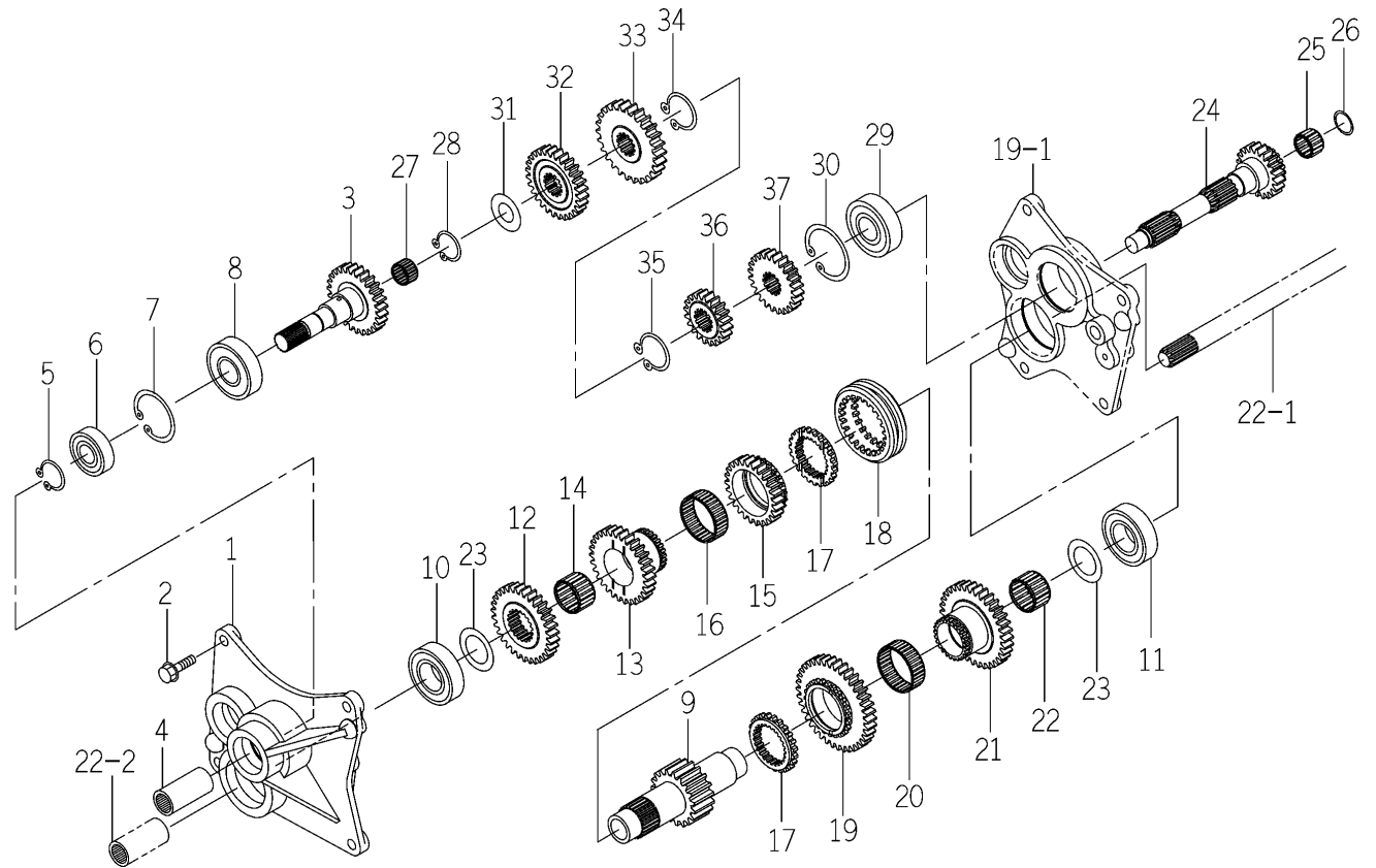
FIG. 17 GEAR (MAIN) SYSTEM (SK TYPE)
