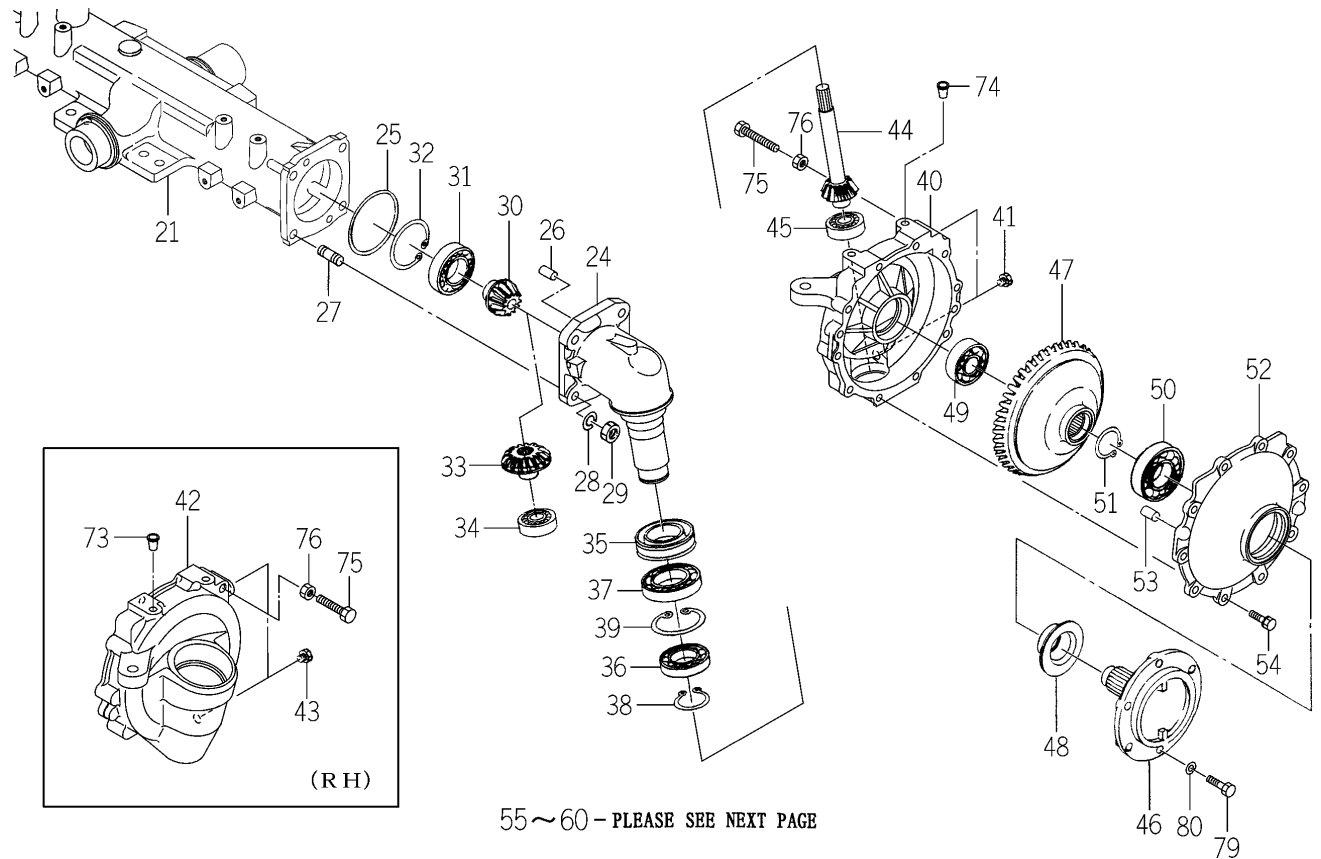
FIG. 55 FRONT AXLE SET (V TYPE)(2/3)
