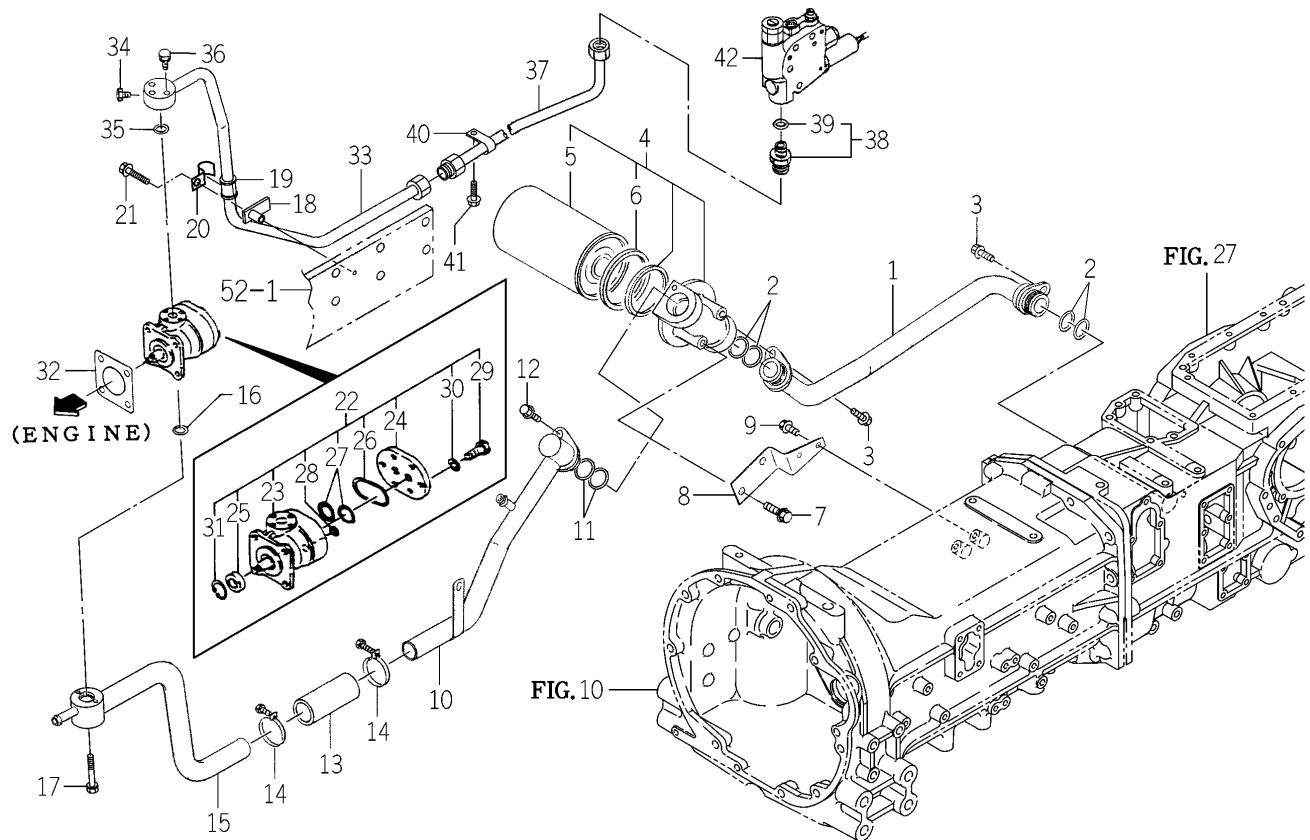
FIG. 68 HYD. SYSTEM (MAIN) (K TYPE)(1/2)
