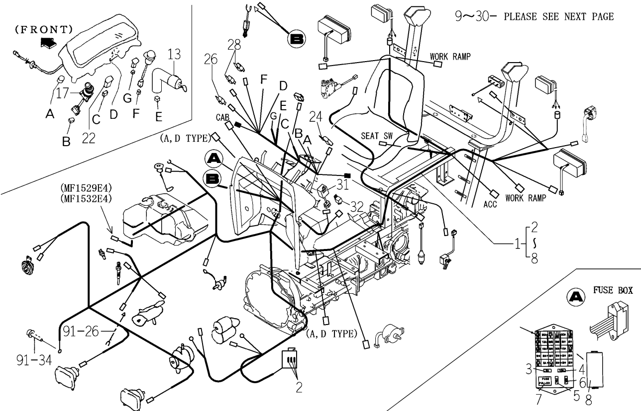
FIG. 93 ELC. SYSTEM (MAIN)(1/2) (EXCEPT A,D TYPE)
