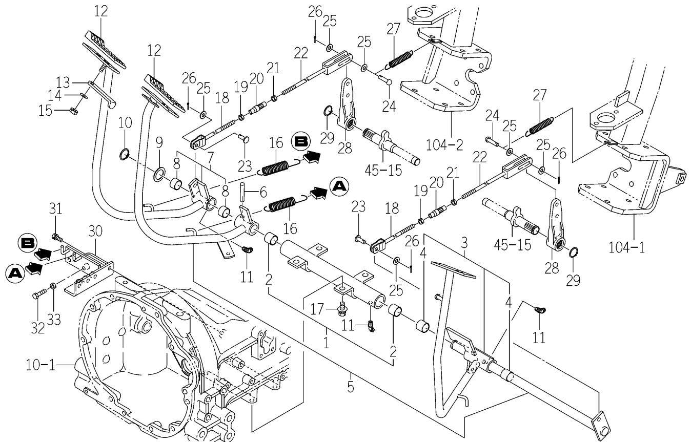
FIG. 46 PEDAL (BRAKE) SYSTEM
