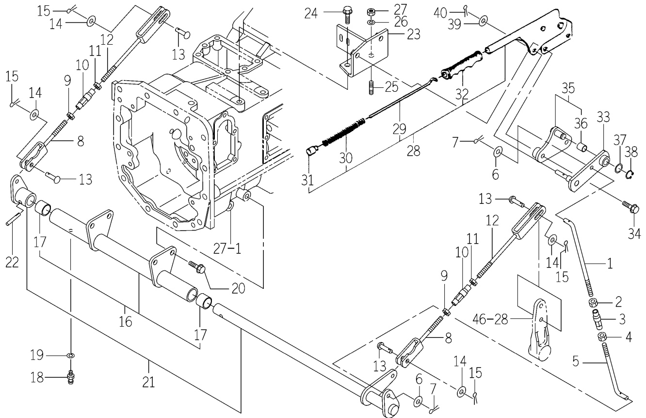
FIG. 47 BRAKE (PARKING) SYSTEM
