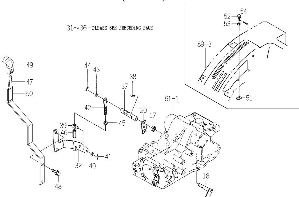
FIG. 62 MECHANICAL LINK (POSITION) SYSTEM(2/2) (A TYPE)
