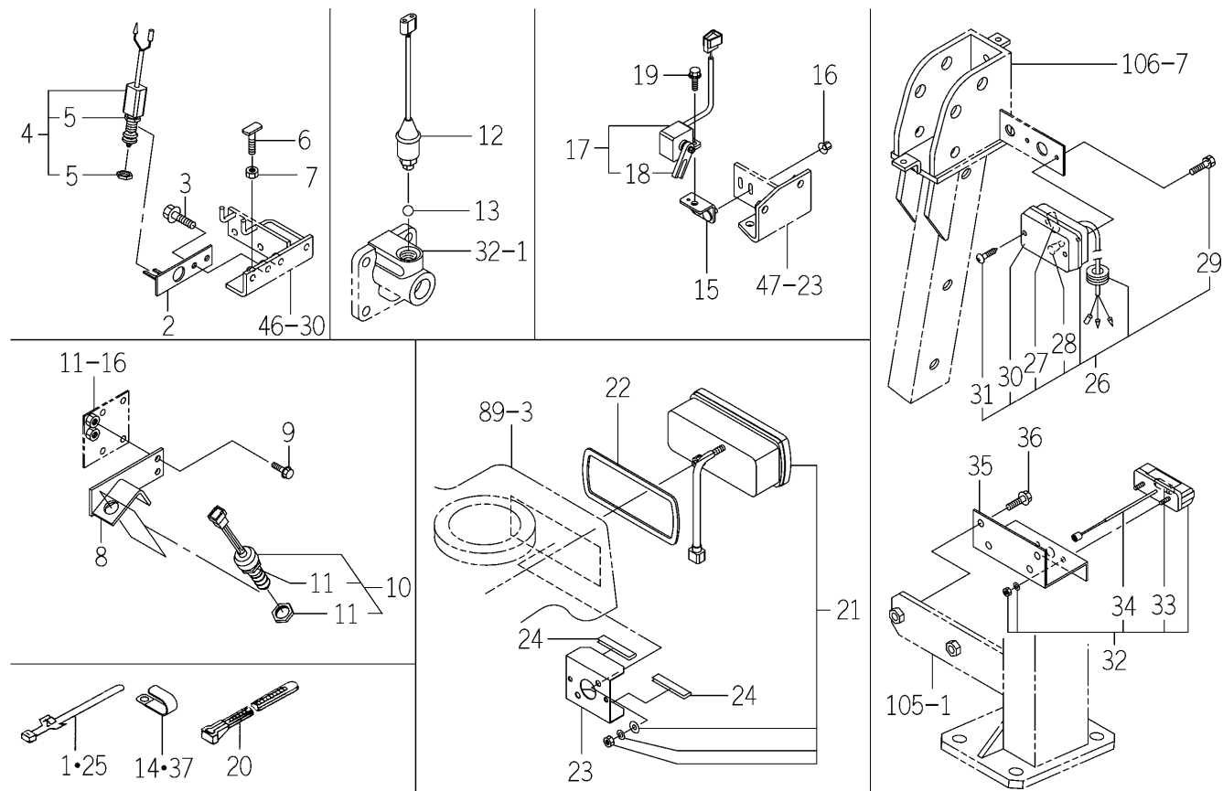
FIG. 98 ELC. SYSTEM (REAR) (A TYPE EXCEPT S)
