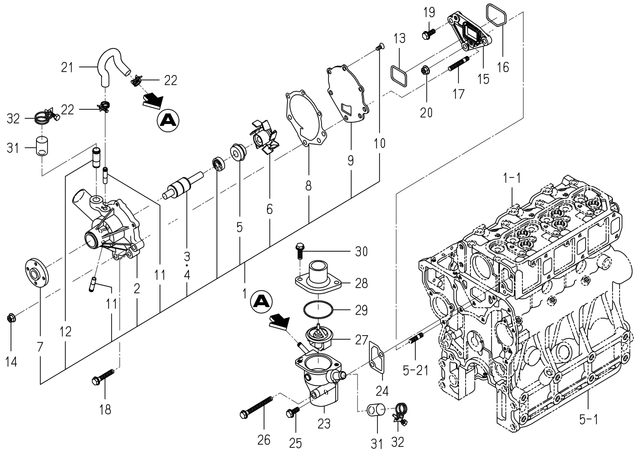
FIG. 17 WATER PUMP
