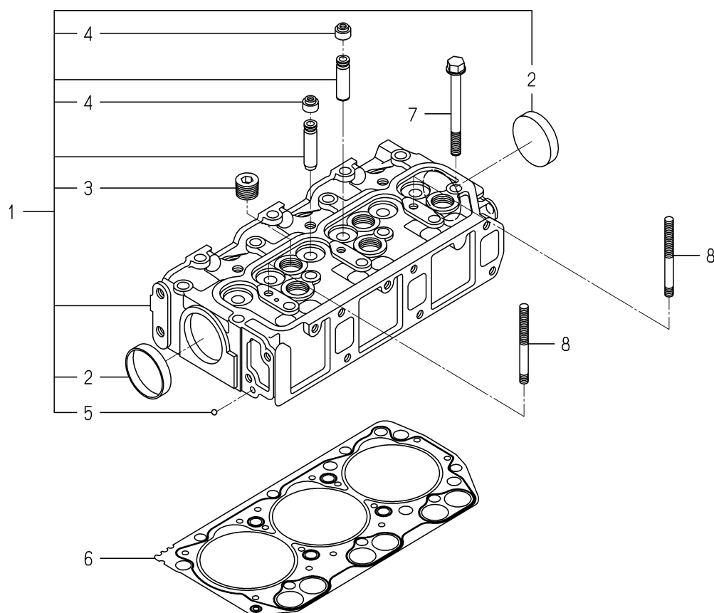
FIG. 1 CYLINDER HEAD
