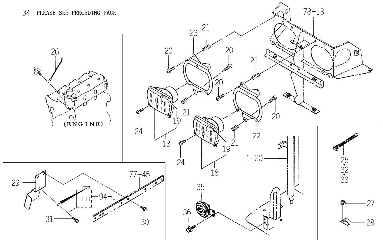
FIG. 92 ELC. SYSTEM (FRONT)(2/2) (EXCEPT K TYPE)
