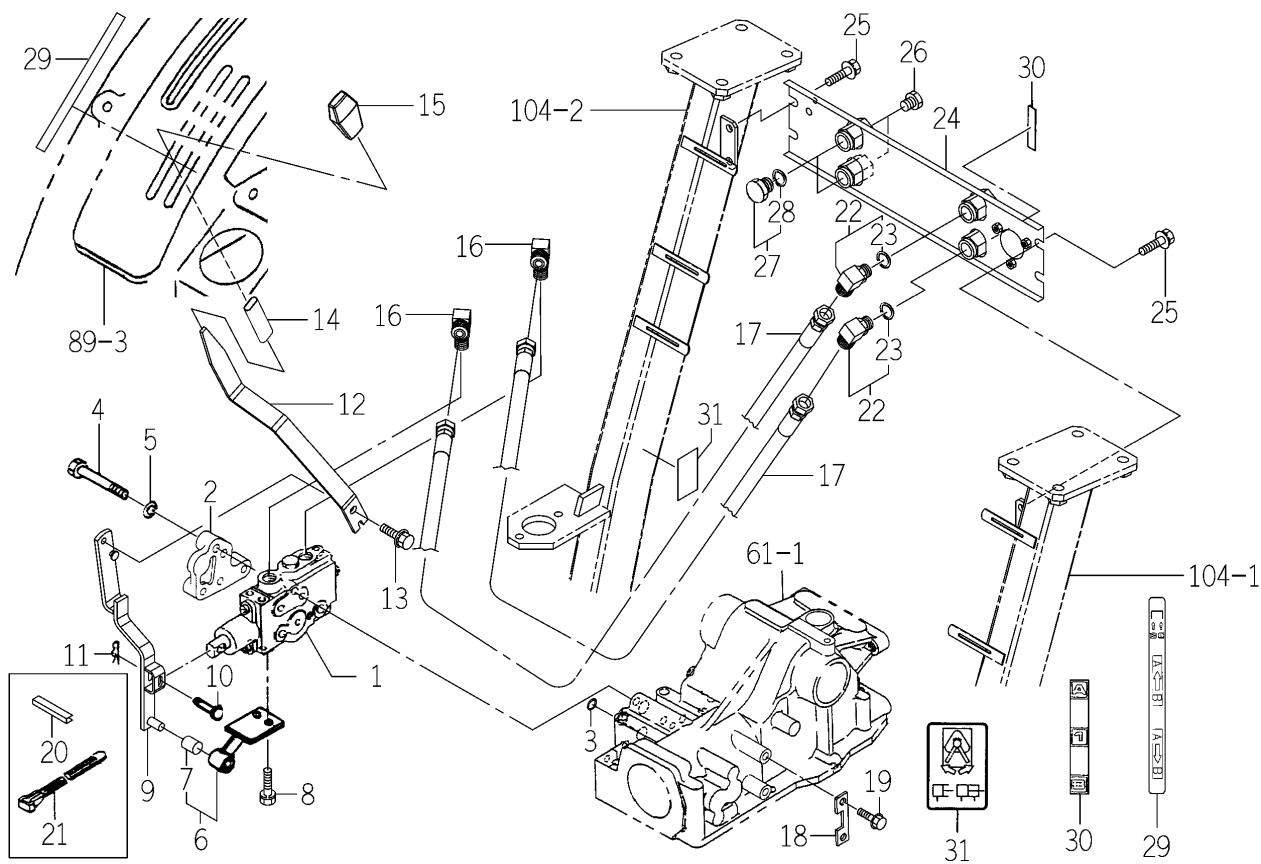
FIG. 70 VALVE (REMOTE/1R) SYSTEM (V TYPE)
