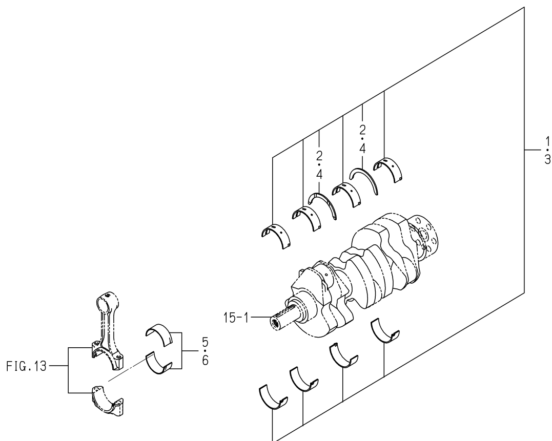
FIG. 6 BEARING/UNDER SIZE (OPTION)
