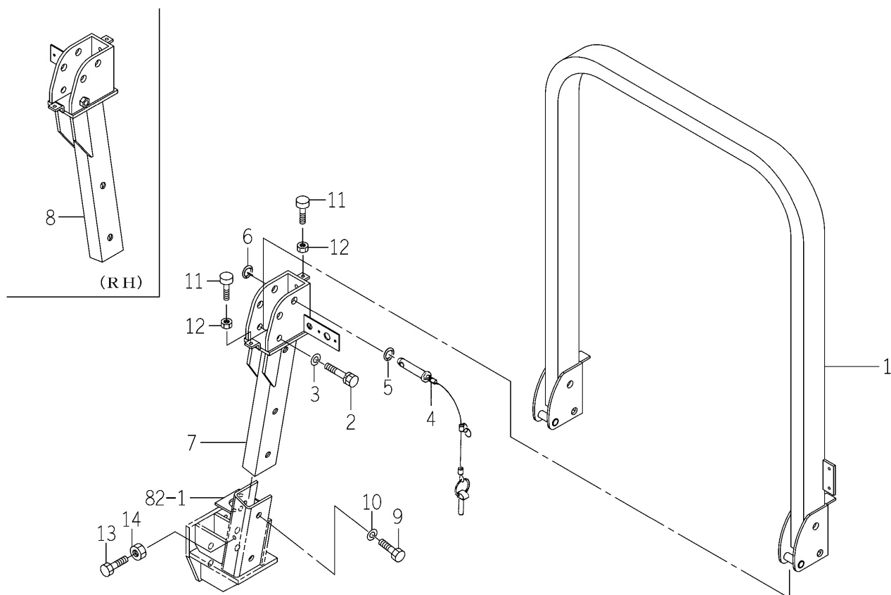
FIG.106 FRAME (MID) SYSTEM (A TYPE)
