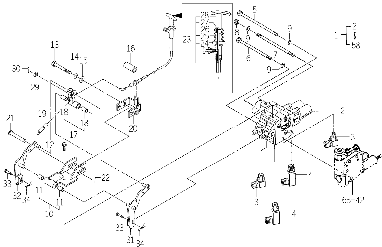
FIG.128 JOY STICK SYSTEM (EXCEPT D TYPE)(1/2) (OPTION)
