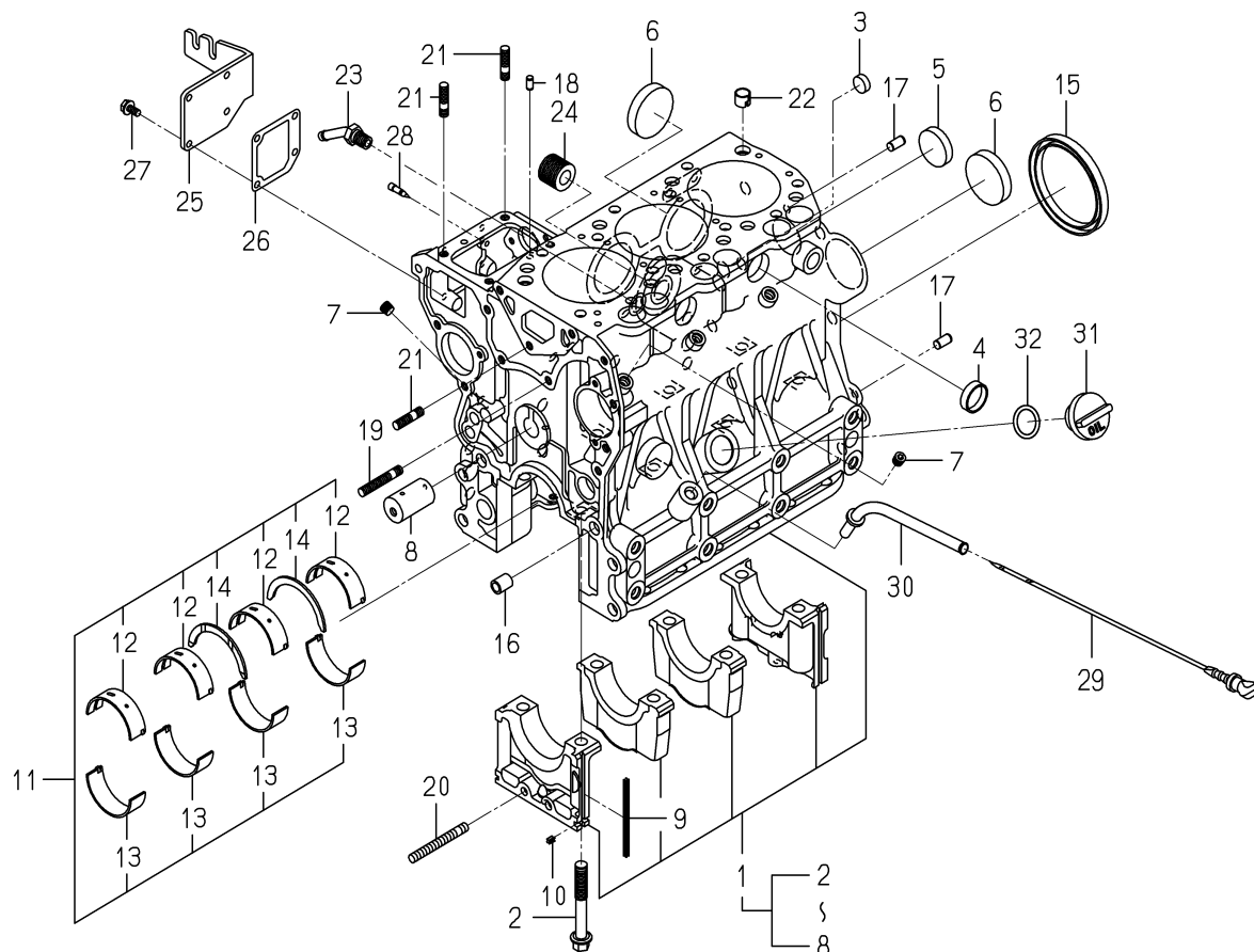
FIG. 5 CYLINDER BLOCK
