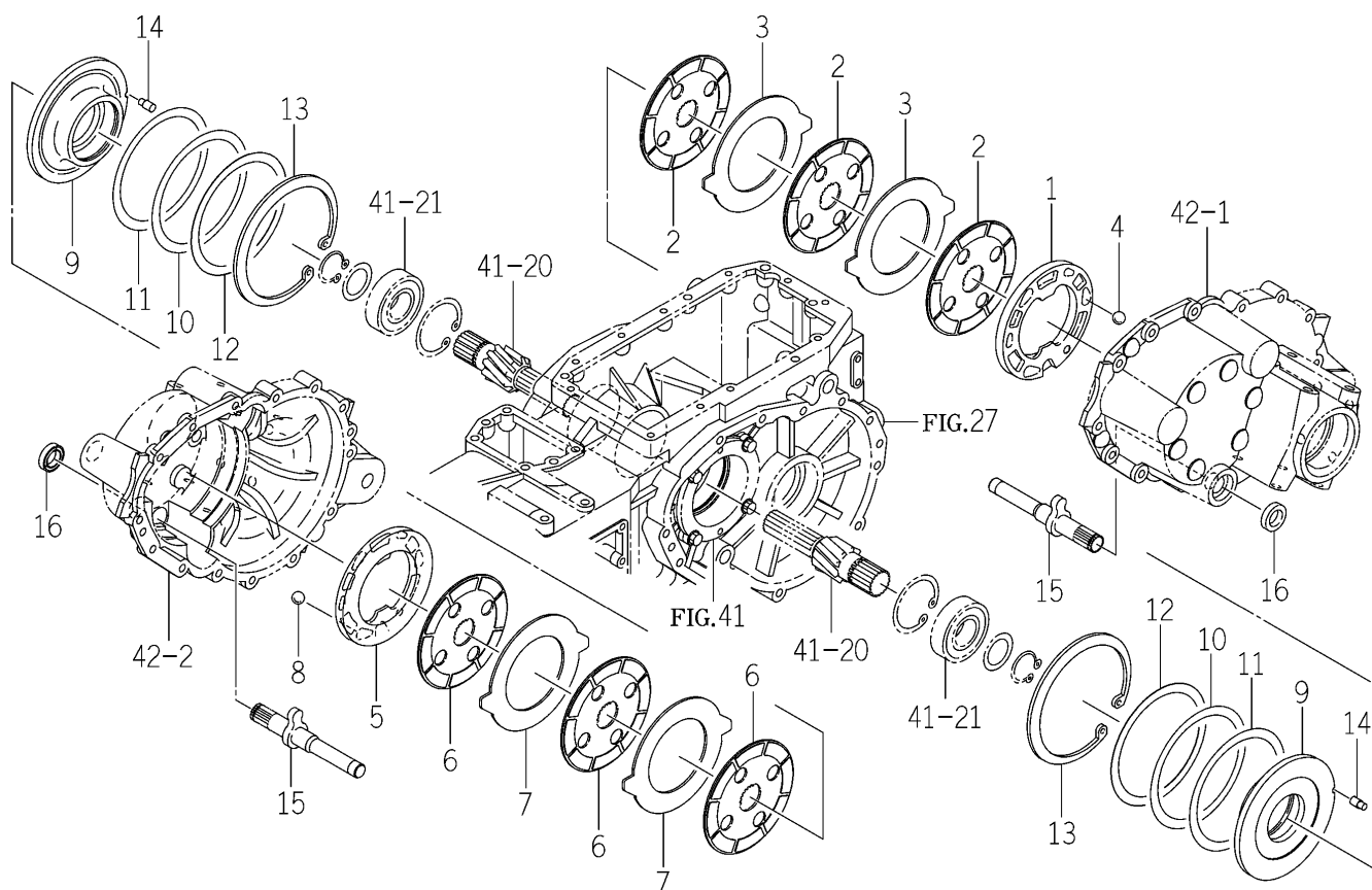
FIG. 45 BRAKE SYSTEM
