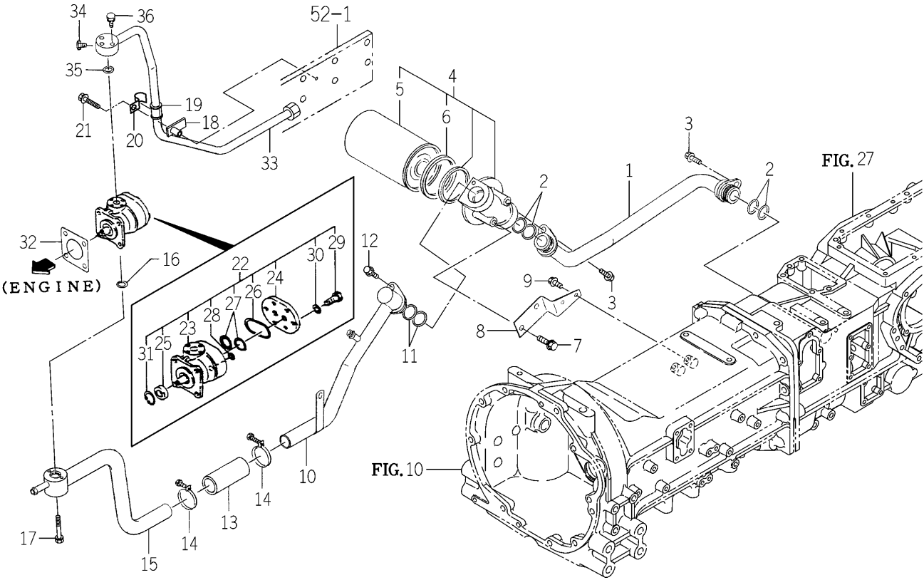
FIG. 66 HYD. SYSTEM (MAIN) (EXCEPT K TYPE)(1/2)
