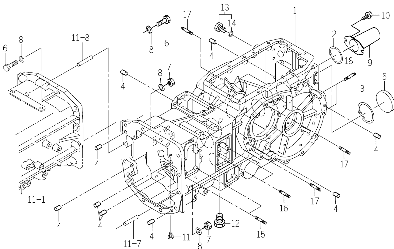
FIG. 27 CASE (TRANSMISSION/REAR) SYSTEM
