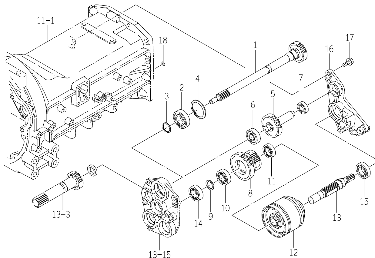
FIG. 15 GEAR (PTO) SYSTEM (K TYPE)
