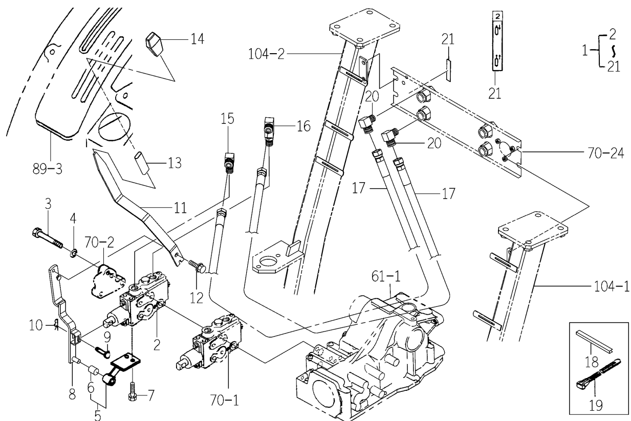
FIG.129 VALVE (REMOTE/PLUS) SYSTEM (V TYPE) (OPTION)
