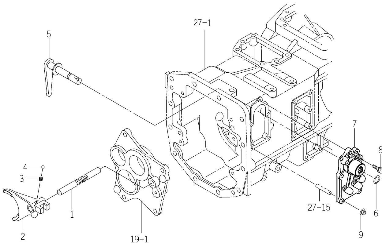
FIG. 29 FORK (SHIFT/MAIN) SYSTEM (S TYPE)
