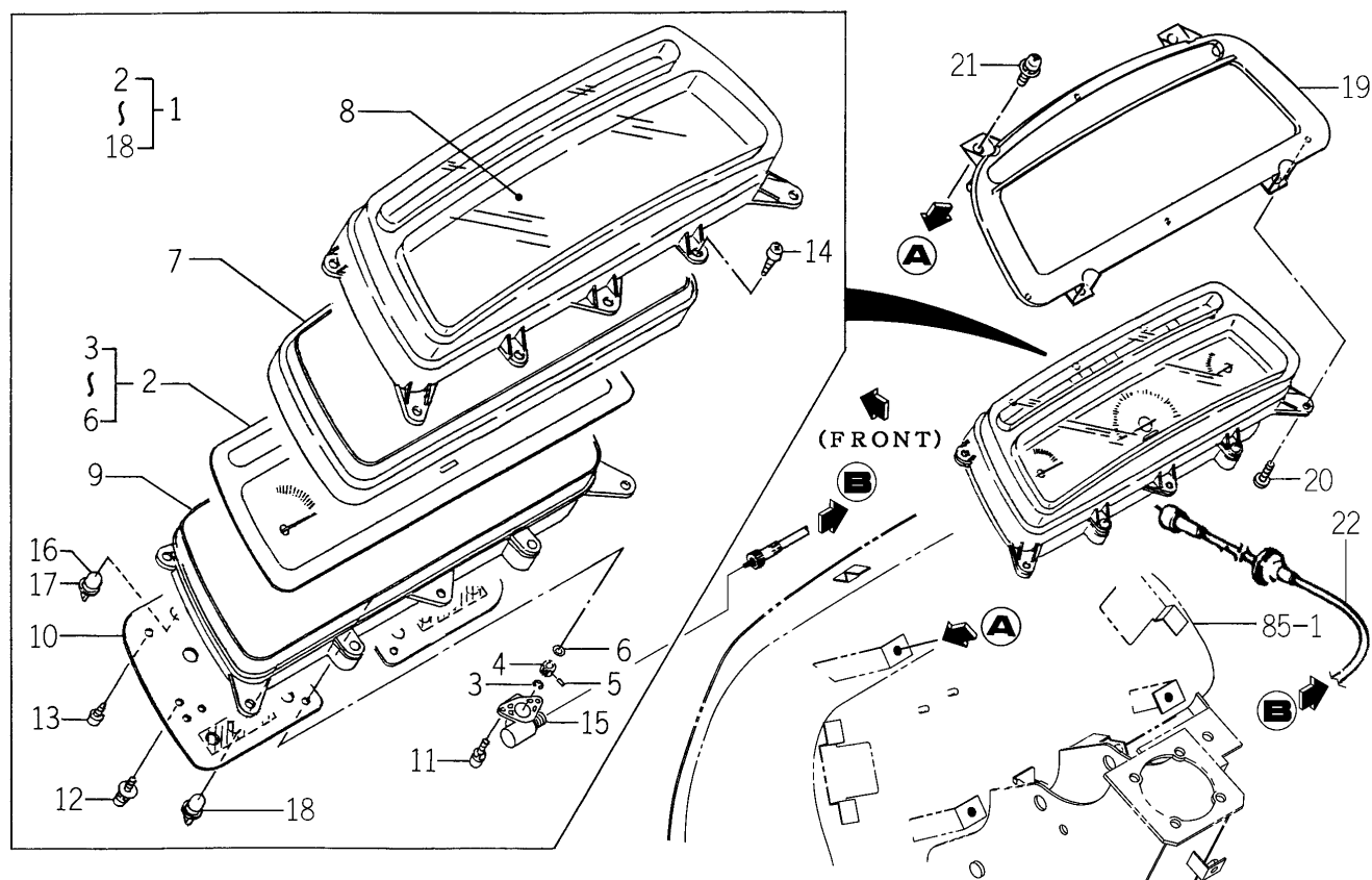
FIG.100 METER PANEL SYSTEM
