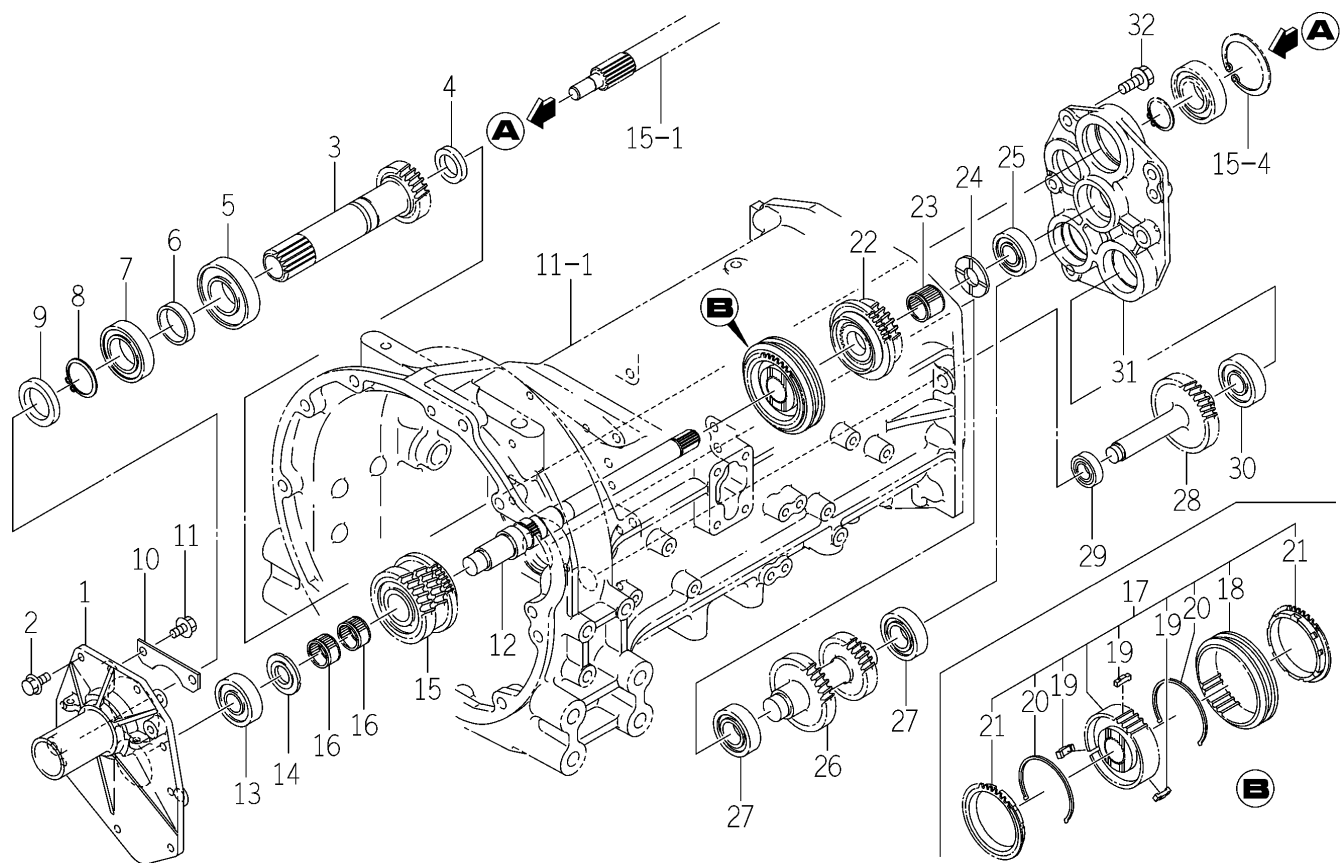
FIG. 14 GEAR (INPUT) SYSTEM (SK TYPE)
