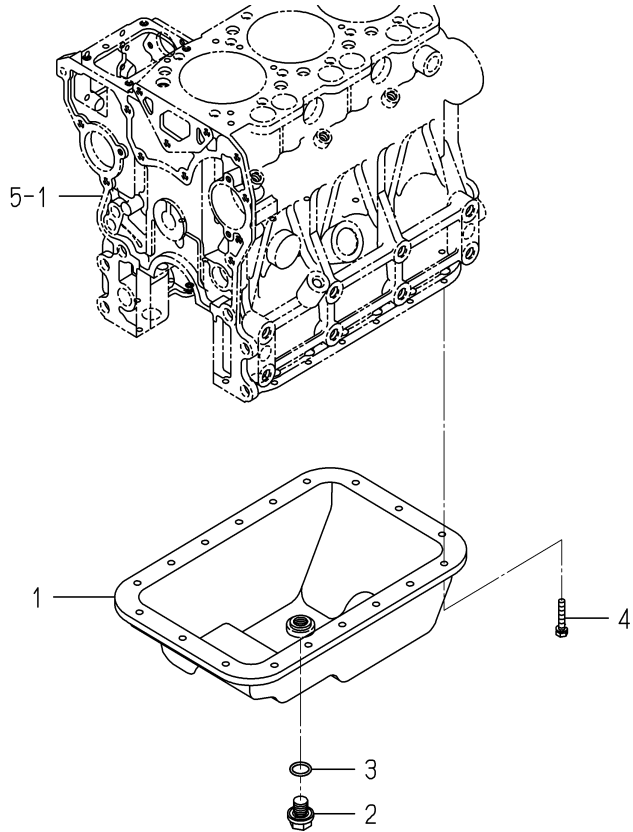
FIG. 7 OIL PAN
