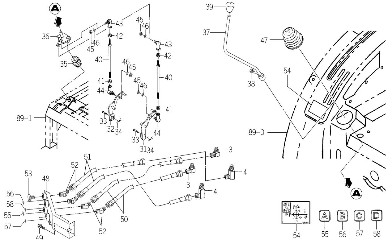
FIG.128 JOY STICK SYSTEM (EXCEPT D TYPE)(2/2) (OPTION)
