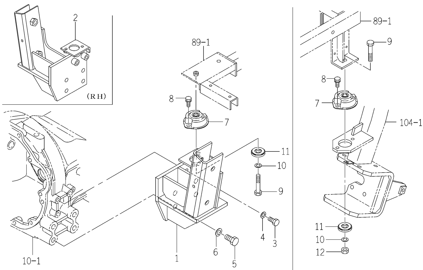
FIG. 82 MOUNT SYSTEM (A TYPE)
