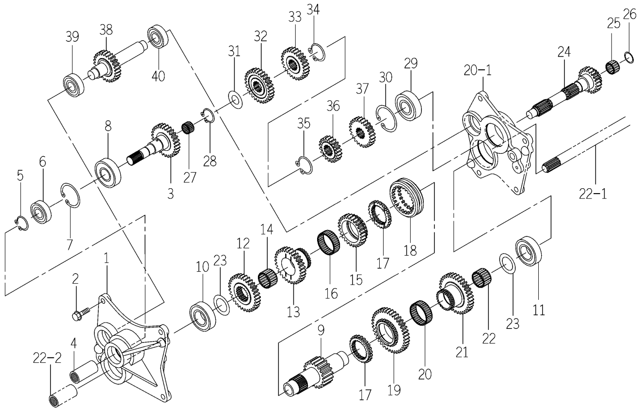
FIG. 16 GEAR (MAIN) SYSTEM (K TYPE EXCEPT S)
