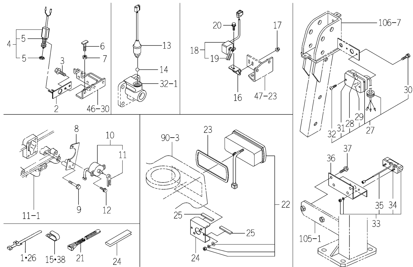
FIG. 99 ELC. SYSTEM (REAR) (SA TYPE)
