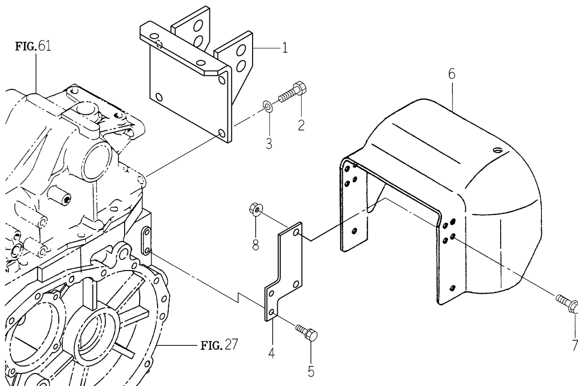
FIG. 74 TOP LINK BRACKET SYSTEM (EXCEPT A TYPE)
