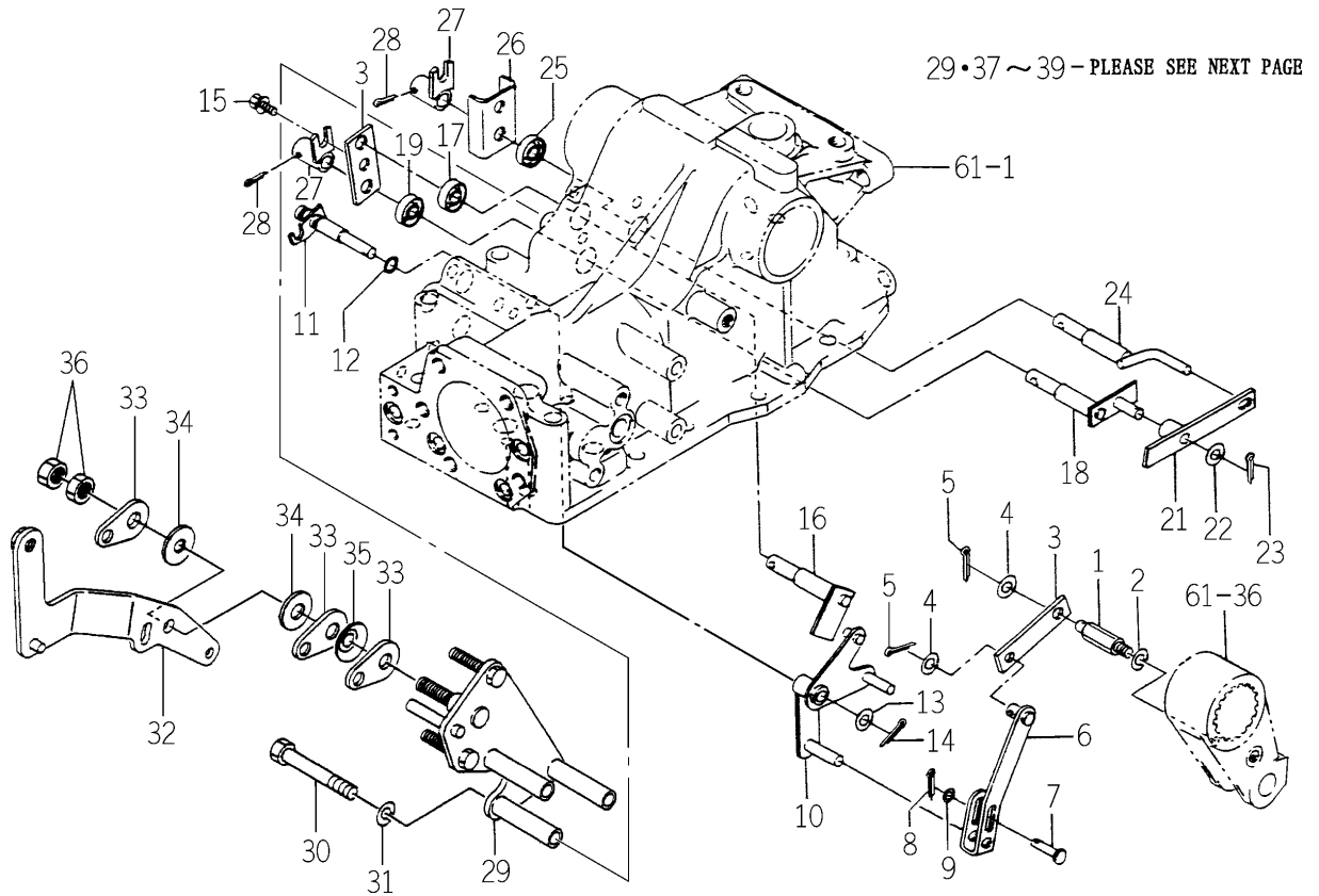
FIG. 62 MECHANICAL LINK (POSITION) SYSTEM(1/2) (A TYPE)
