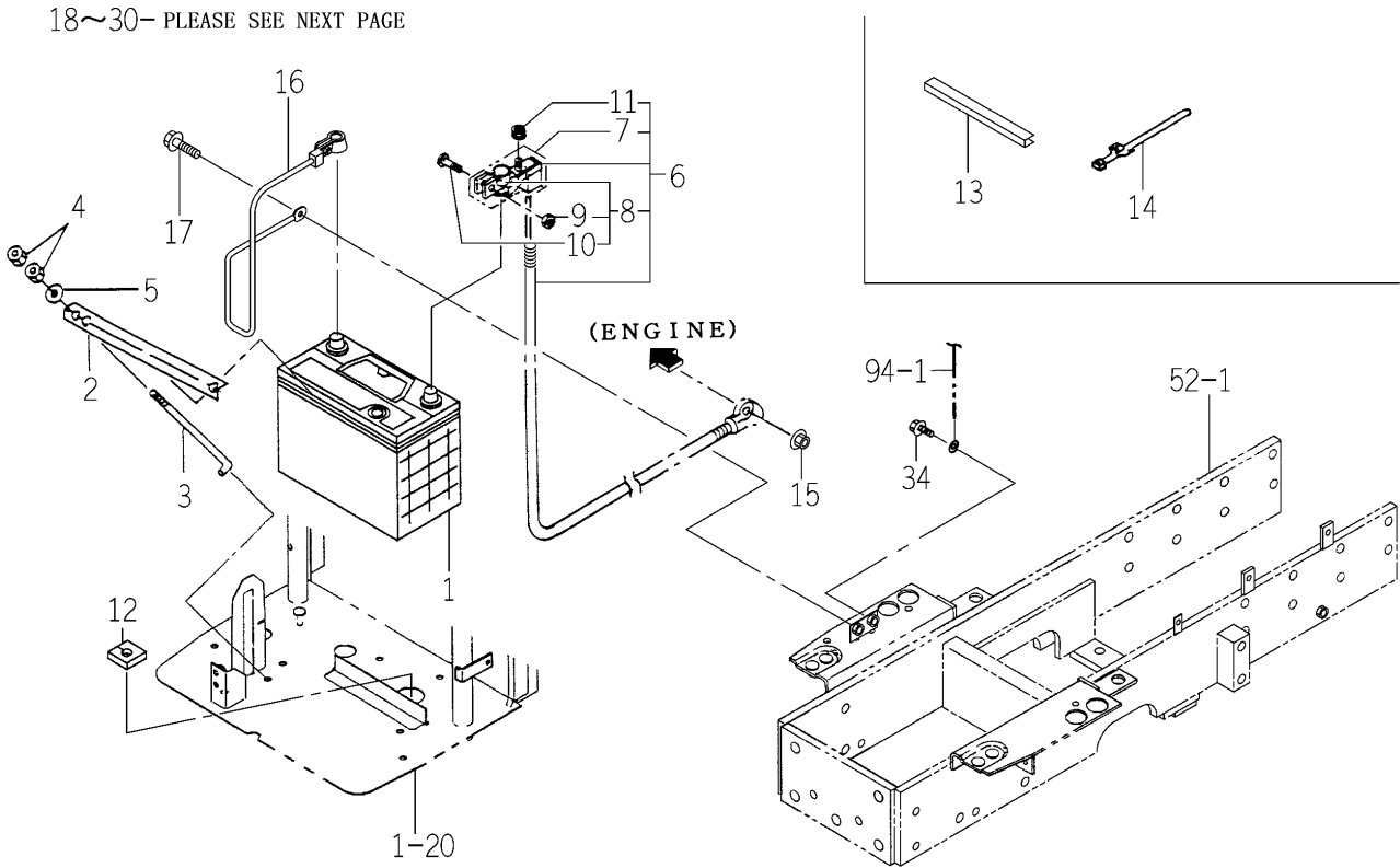
FIG. 92 ELC. SYSTEM (FRONT)(1/2) (EXCEPT K TYPE)
