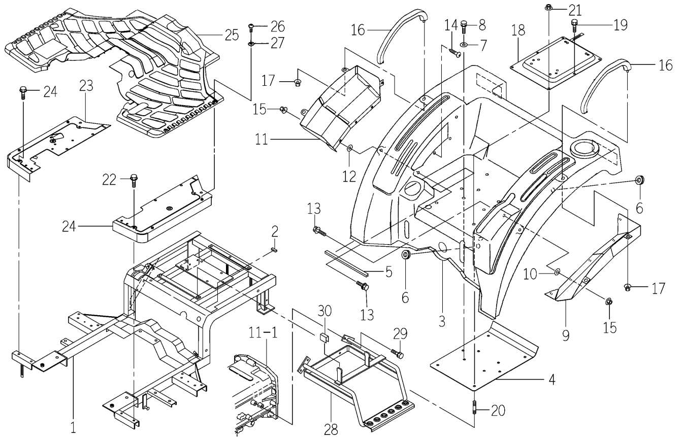
FIG. 90 FLOOR (REAR) SYSTEM (S TYPE)
