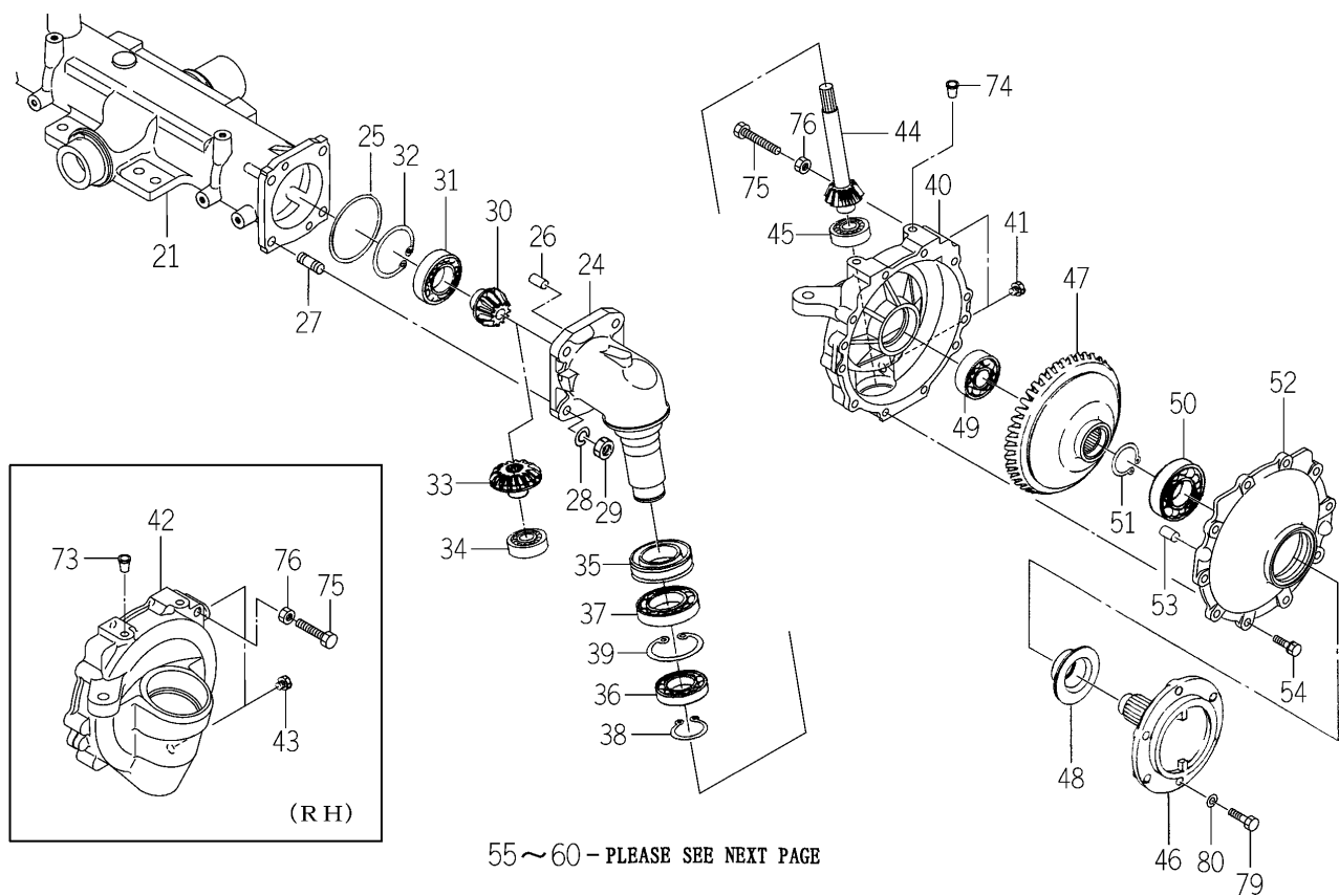
FIG. 56 FRONT AXLE SET (M TYPE)(2/3)
