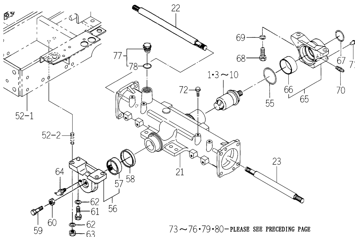
FIG. 55 FRONT AXLE SET (V TYPE)(3/3)
