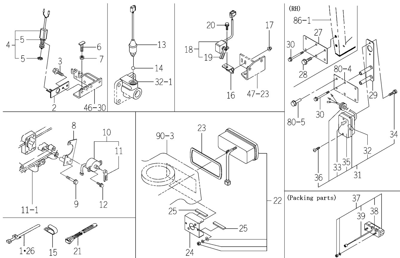
FIG. 97 ELC. SYSTEM (REAR) (D TYPE)
