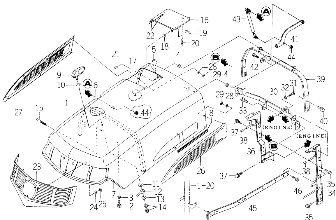
FIG. 77 HOOD SYSTEM
