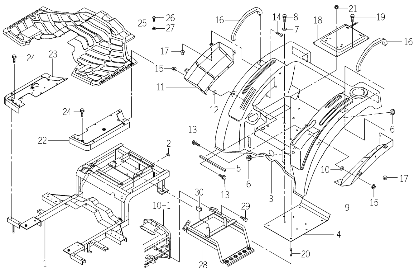
FIG. 89 FLOOR (REAR) SYSTEM (EXCEPT S TYPE)
