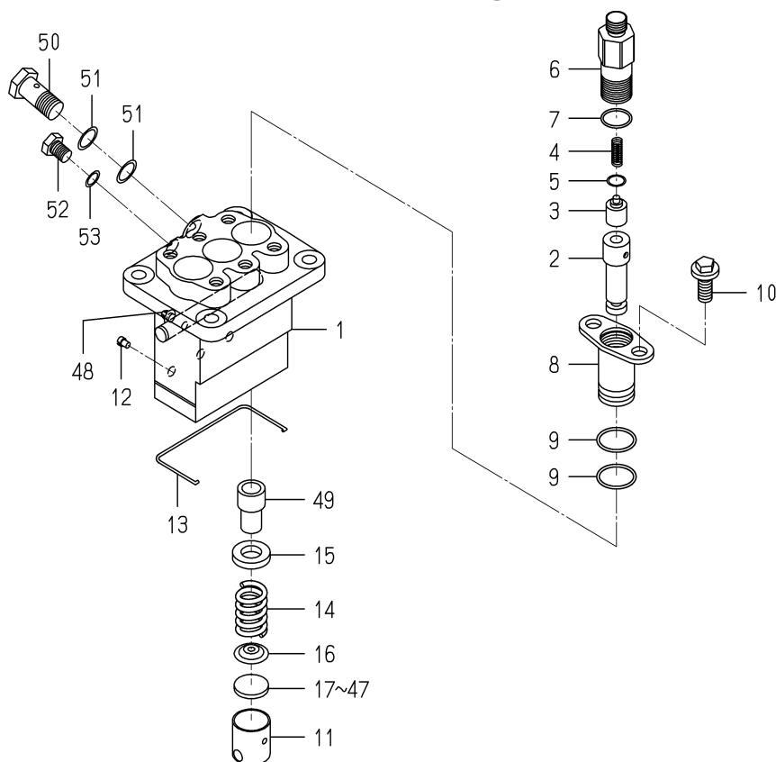
FIG. 27 COMPONENT PARTS FOR 6215-600-104-20 ON Fig.20
