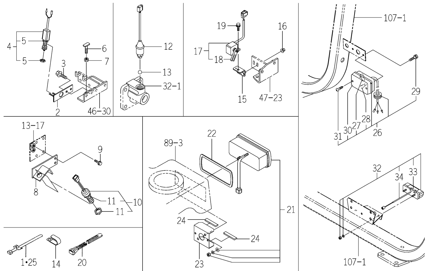
FIG. 95 ELC. SYSTEM (REAR) (EXCEPT S,A TYPE)
