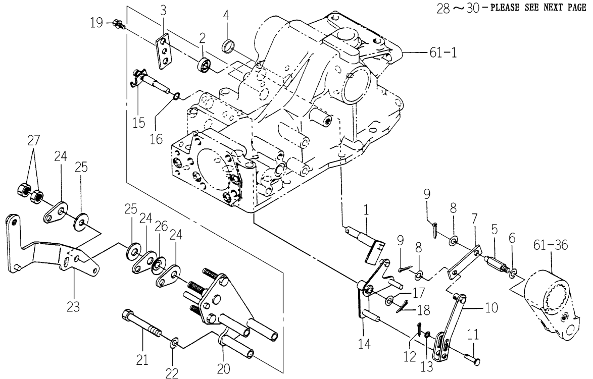
FIG. 63 MECHANICAL LINK (POSITION) SYSTEM(1/2) (EXCEPT A TYPE)
