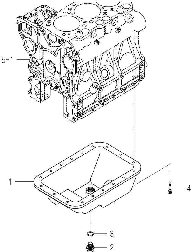
FIG. 7 OIL PAN
