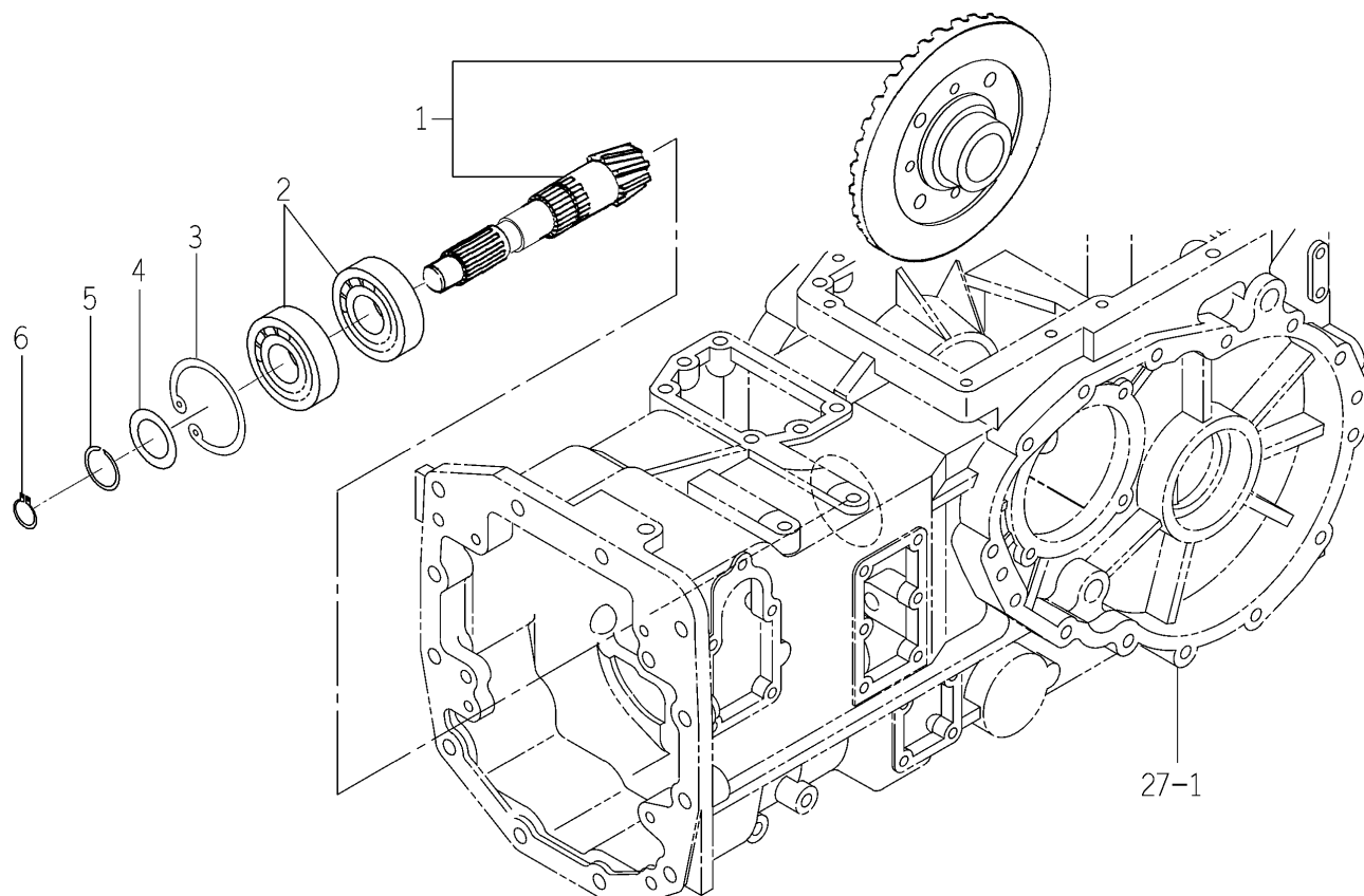
FIG. 40 PINION (DRIVE) SYSTEM
