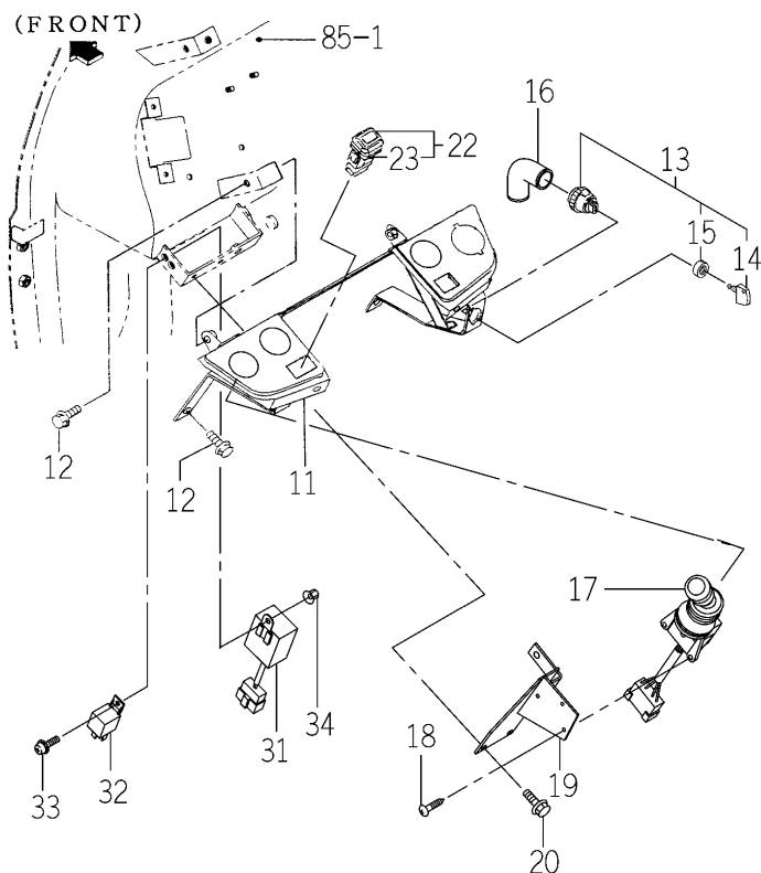
FIG. 93 ELC. SYSTEM (MAIN)(2/2) (EXCEPT A,D TYPE)
