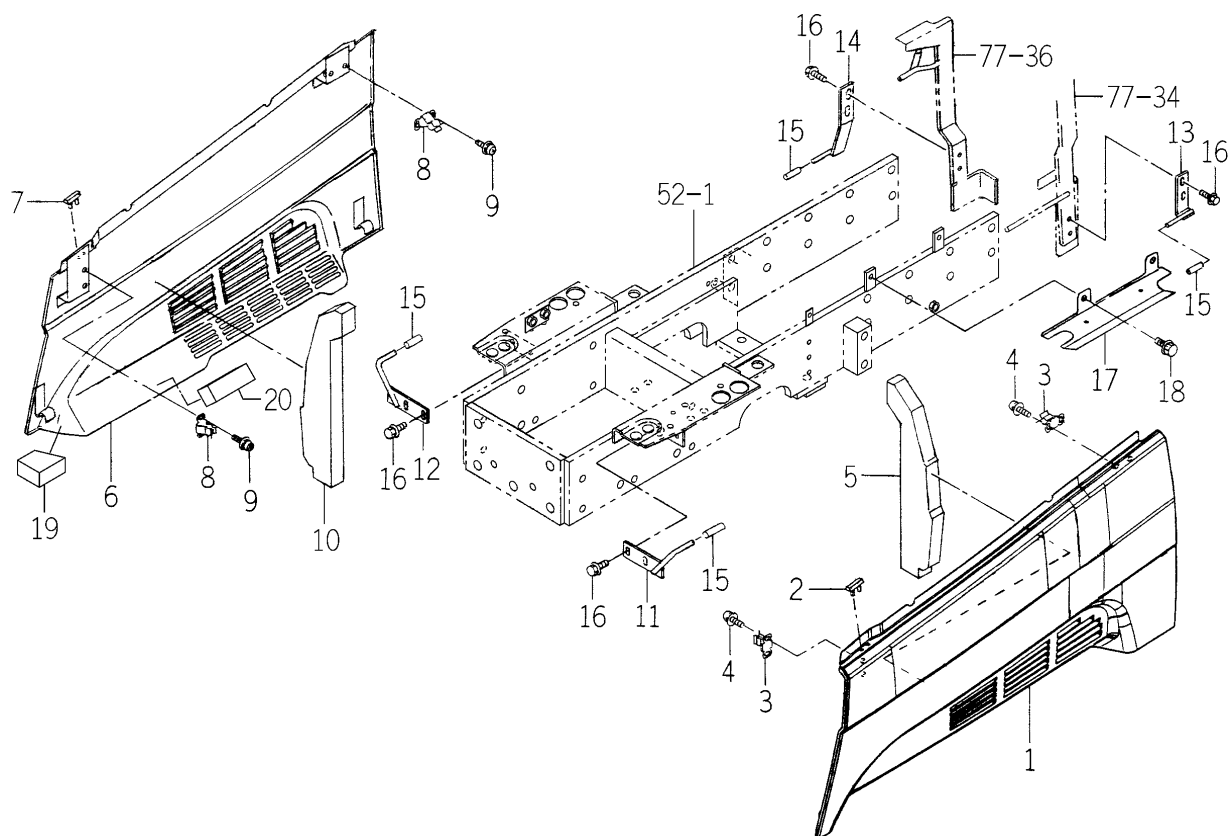
FIG. 79 COVER (SIDE) SYSTEM
