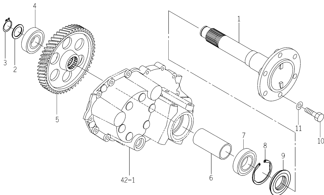
FIG. 43 SHAFT (WHEEL/REAR) SYSTEM
