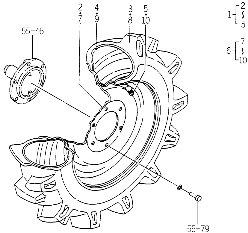
FIG.123 FRONT WHEEL (4WD) SYSTEM (OPTION)
