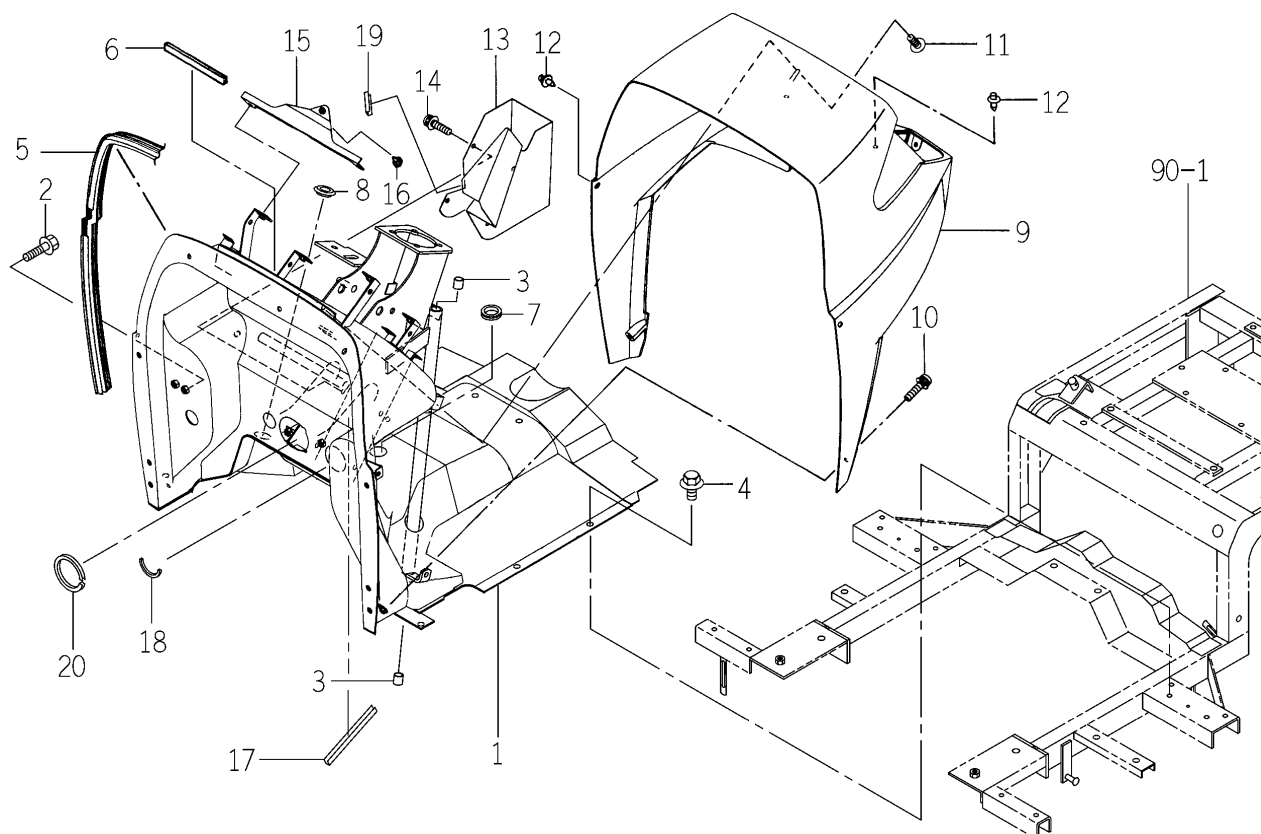
FIG. 88 DASHBOARD SYSTEM (SA TYPE)
