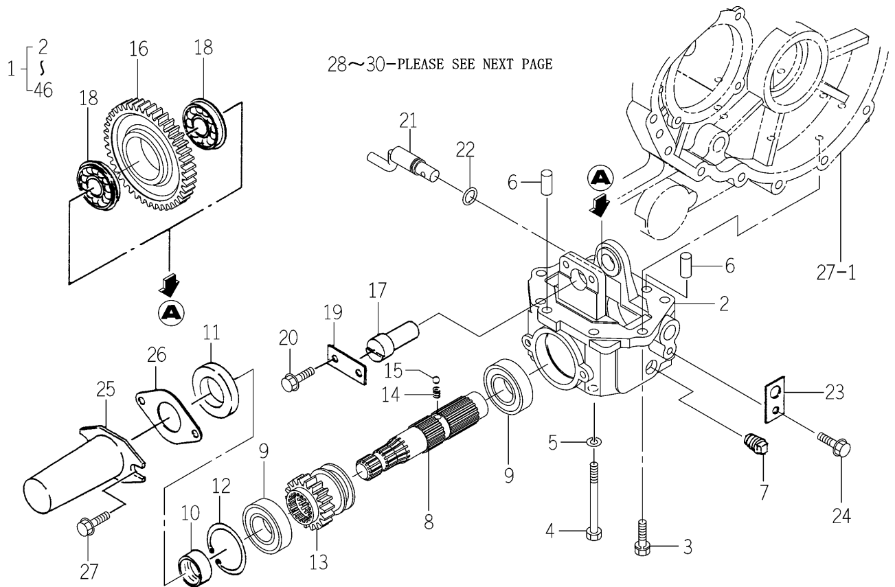
FIG. 25 MID PTO SYSTEM (M TYPE)(1/2)
