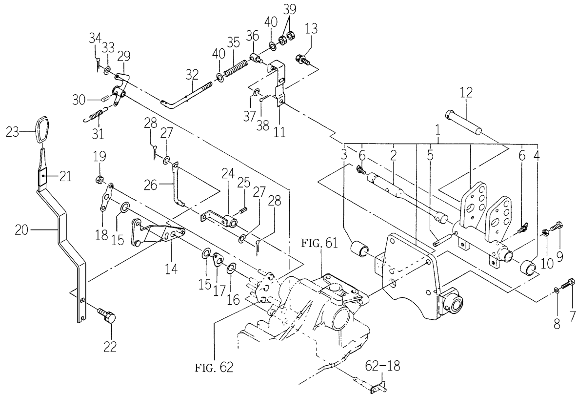
FIG. 64 MECHANICAL LINK (DRAFT) SYSTEM (A TYPE)
