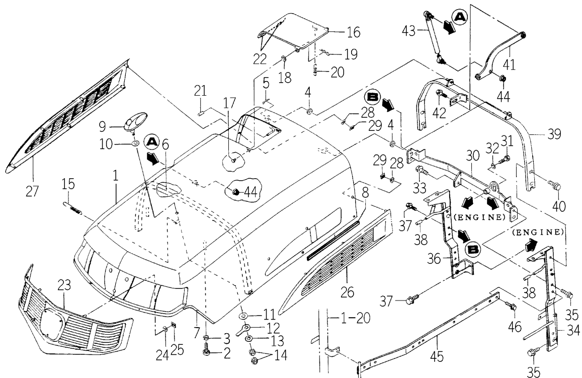
FIG. 77 HOOD SYSTEM
