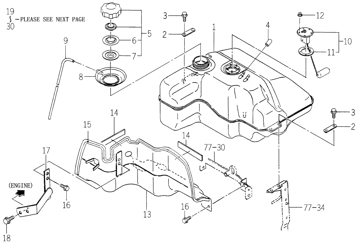
FIG. 4 FUEL SYSTEM(1/2)
