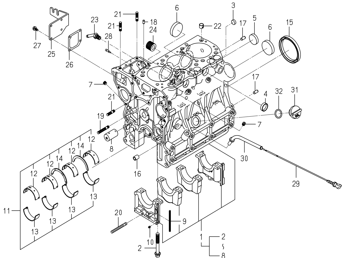
FIG. 5 CYLINDER BLOCK
