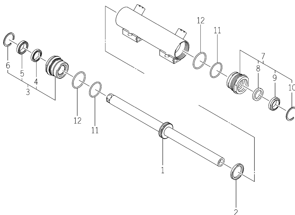
FIG.136 COMPONENT PARTS FOR 1772-407-300-00 ON Fig.51
