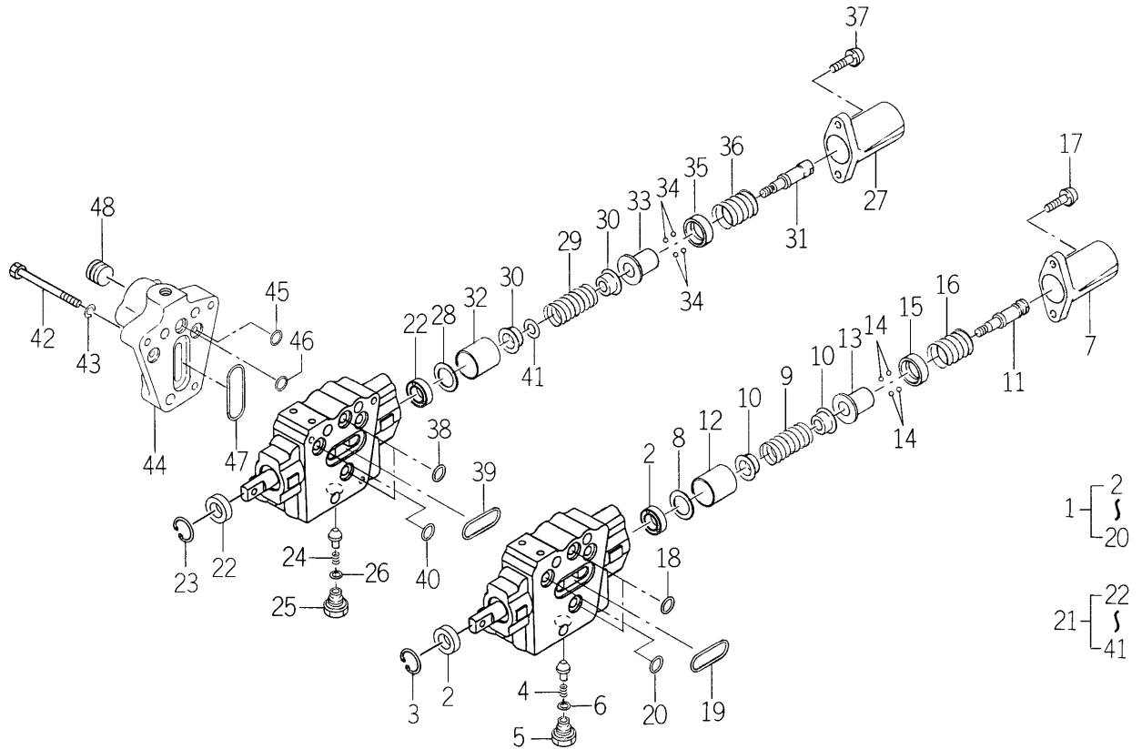
FIG.132 COMPONENT PARTS FOR K211-086-000-00 ON Fig.128
