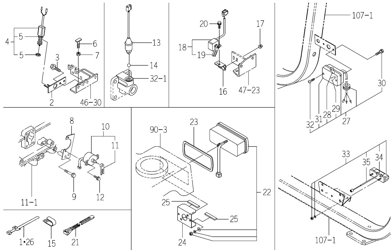
FIG. 96 ELC. SYSTEM (REAR) (S TYPE EXCEPT A,D)
