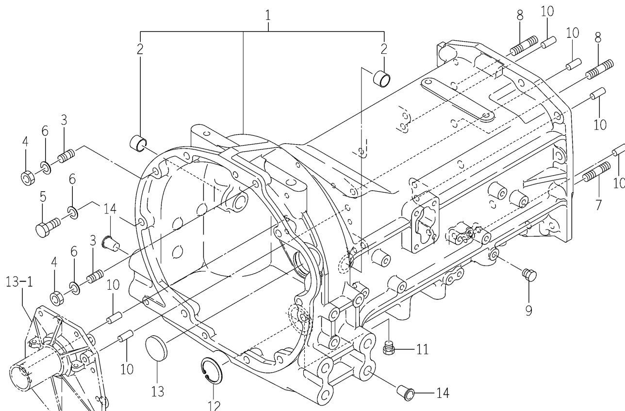
FIG. 11 CASE (TRANSMISSION/FRONT) SYSTEM (K TYPE)
