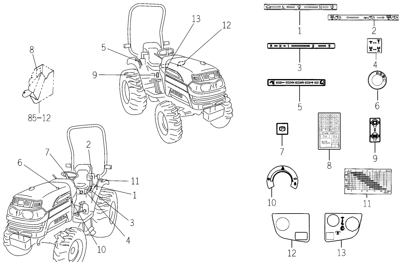
FIG.110 LABEL (CONTROL) (K TYPE EXCEPT S)
