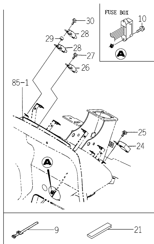
FIG. 93 ELC. SYSTEM (MAIN)(2/2) (EXCEPT A,D TYPE)
