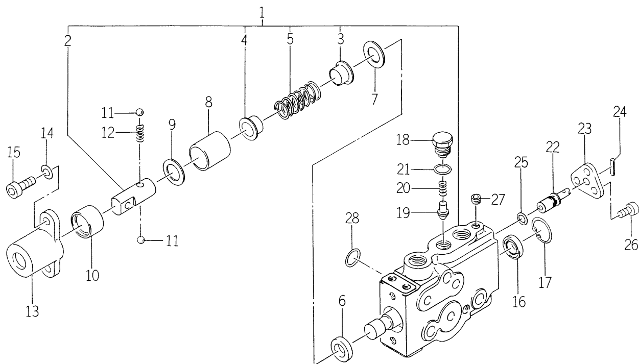
FIG.134 COMPONENT PARTS FOR 1719-511-350-00 ON Fig.70,71
