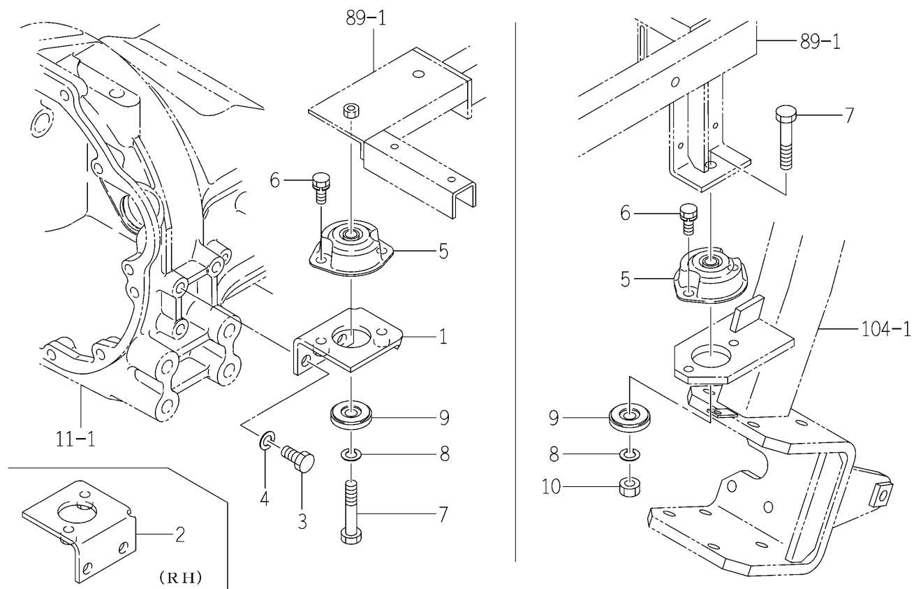
FIG. 83 MOUNT SYSTEM (EXCEPT A,D TYPE)
