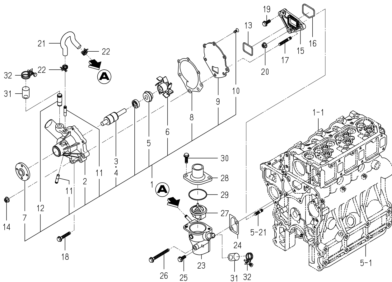
FIG. 17 WATER PUMP
