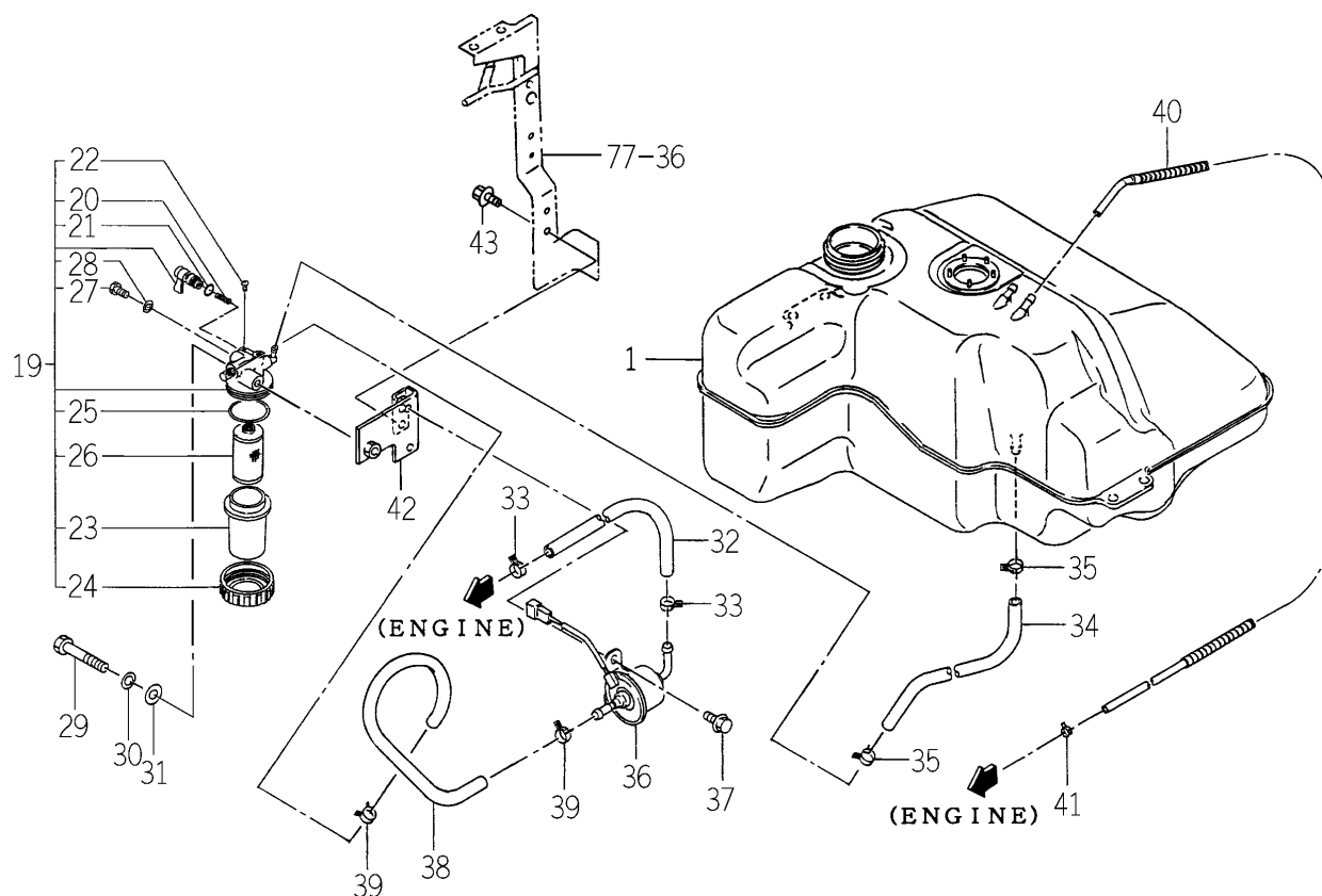
FIG. 4 FUEL SYSTEM(2/2)
