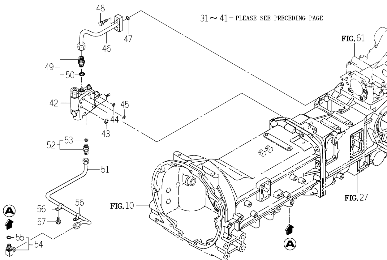
FIG. 68 HYD. SYSTEM (MAIN) (K TYPE)(2/2)
