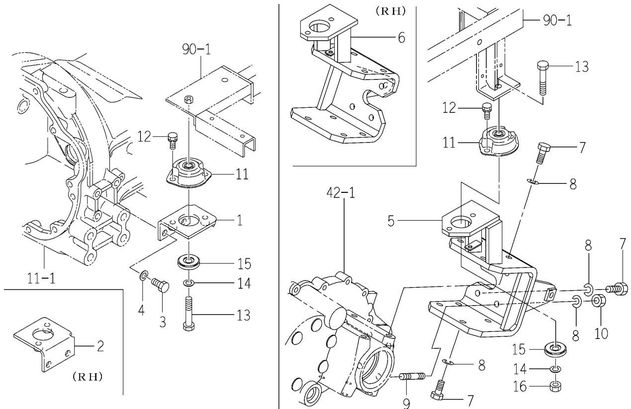
FIG. 84 MOUNT SYSTEM (D TYPE)
