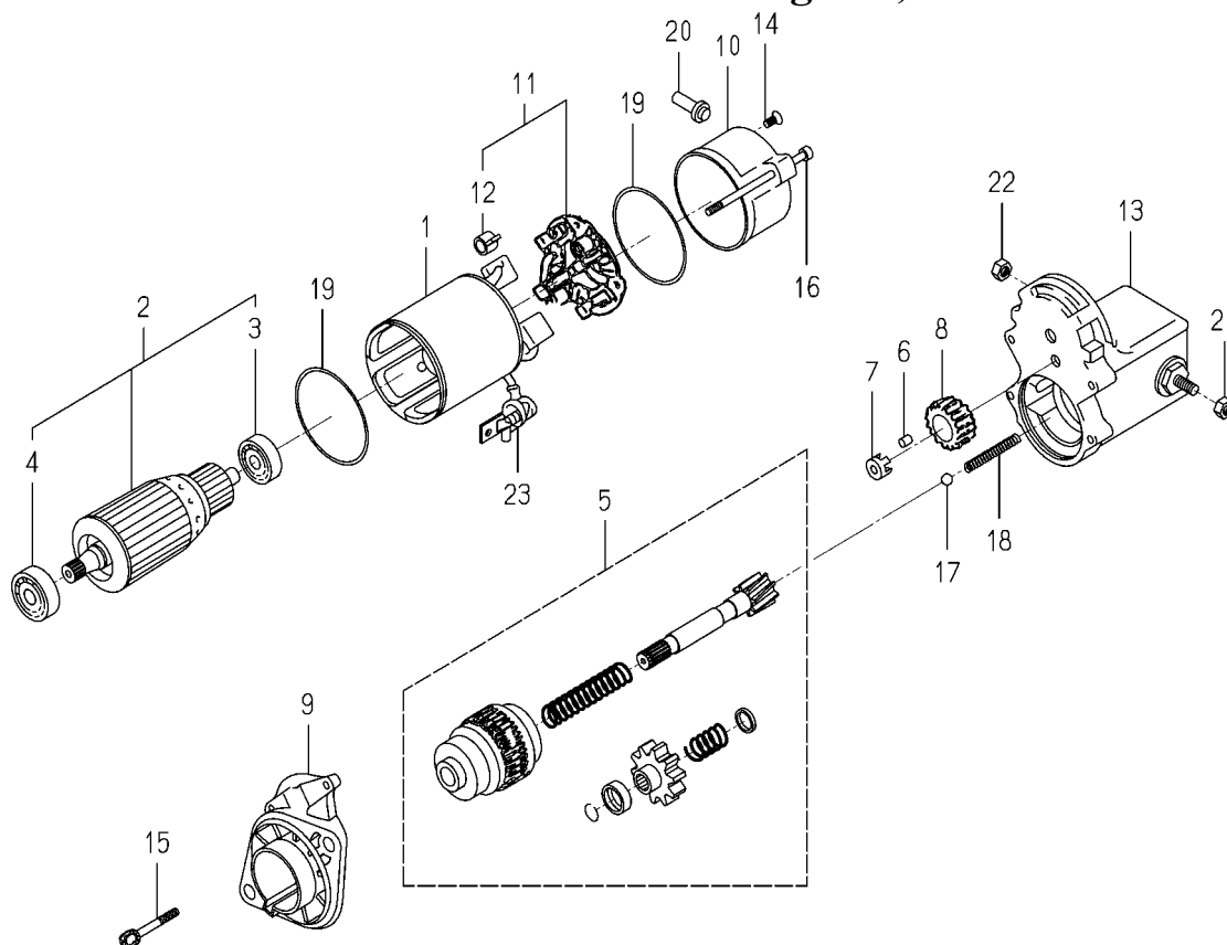
FIG. 34 COMPONENT PARTS FOR 6281-100-007-40 ON Fig.028,029
