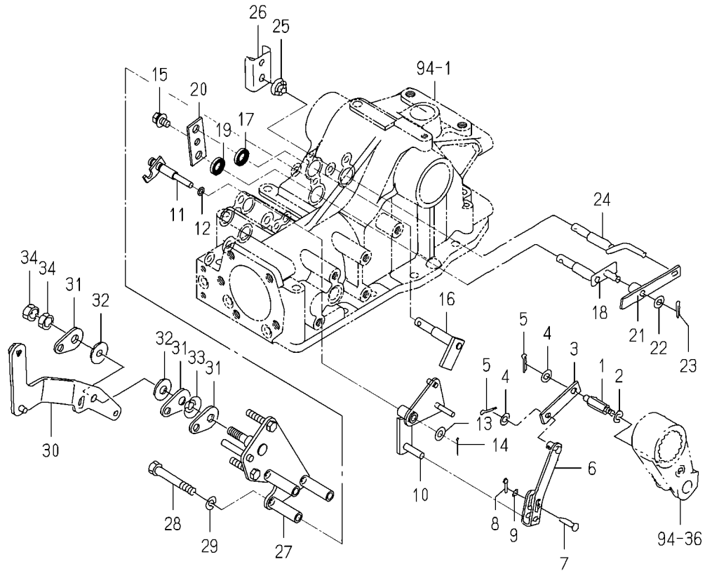
FIG. 96 LEVER(POSITION)SYSTEM(1/2) (V,J TYPE)
