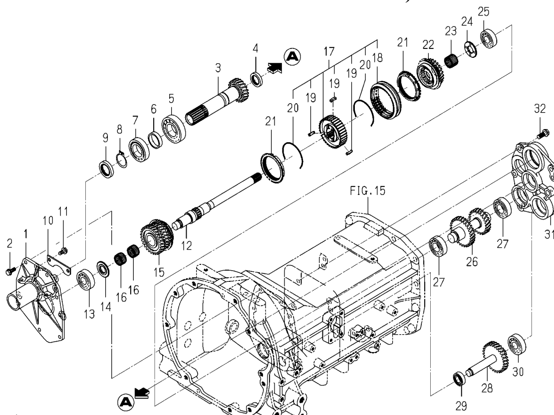
FIG. 18 GEAR(INPUT)SYSTEM (4295 TYPE EXCEPT H,V/ 4335 TYPE EXCEPT H)
