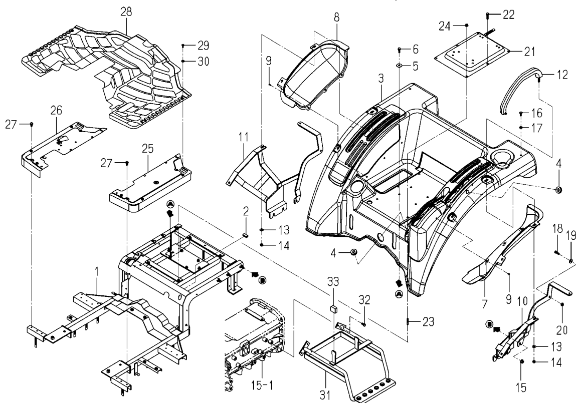
FIG.133 FLOOR(REAR)SYSTEM (4295 TYPE EXCEPT H,V/ 4335 TYPE EXCEPT H)
