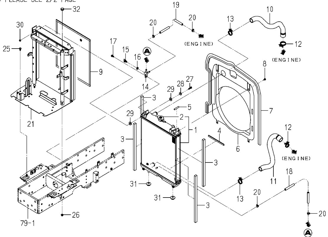
FIG. 3 RADIATOR SYSTEM(1/2) (4295,4335-H TYPE)
