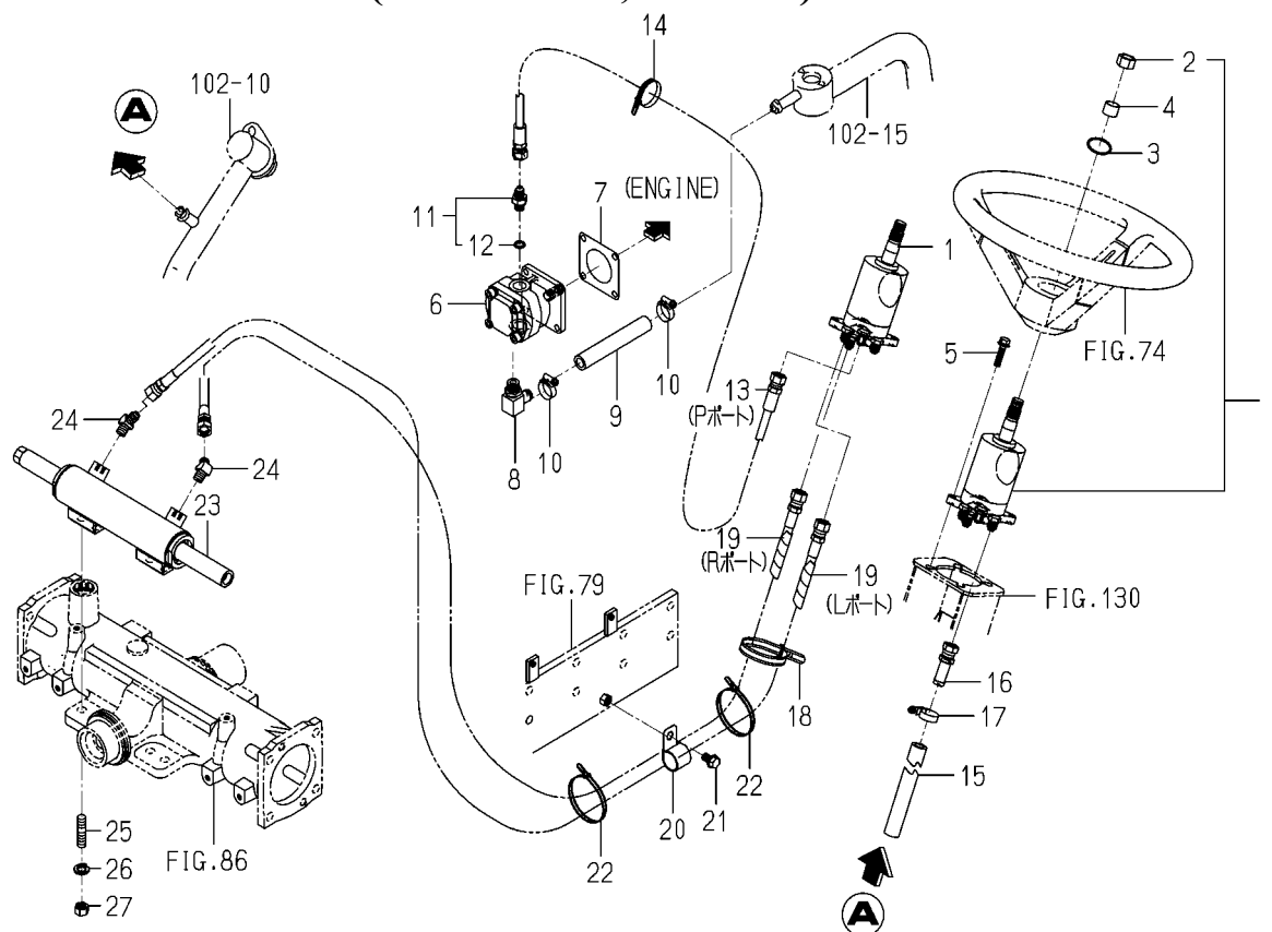
FIG. 77 CONTROLLER(STEERING)SYSTEM (EXCEPT H,V TYPE)
