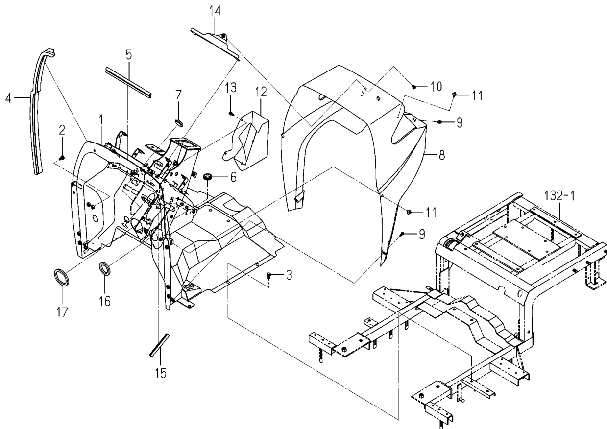
FIG.129 PANEL(DASH)SYSTEM(4295-V TYPE)
