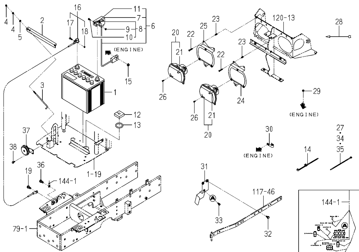
FIG.140 ELC.(FRONT)SYSTEM (G TYPE EXCEPT H)
