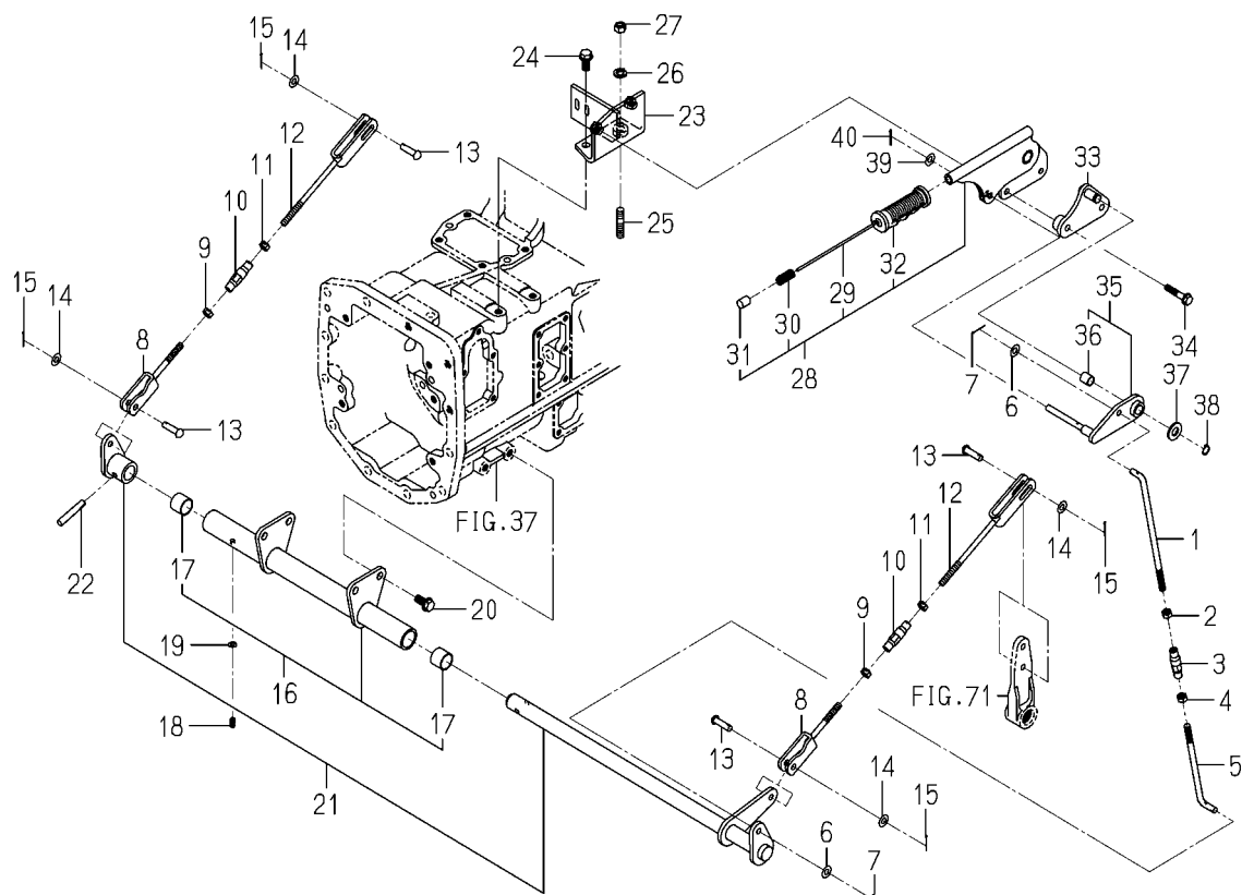
FIG. 72 LEVER(BRAKE/PARKING)SYSTEM (EXCEPT H TYPE)
