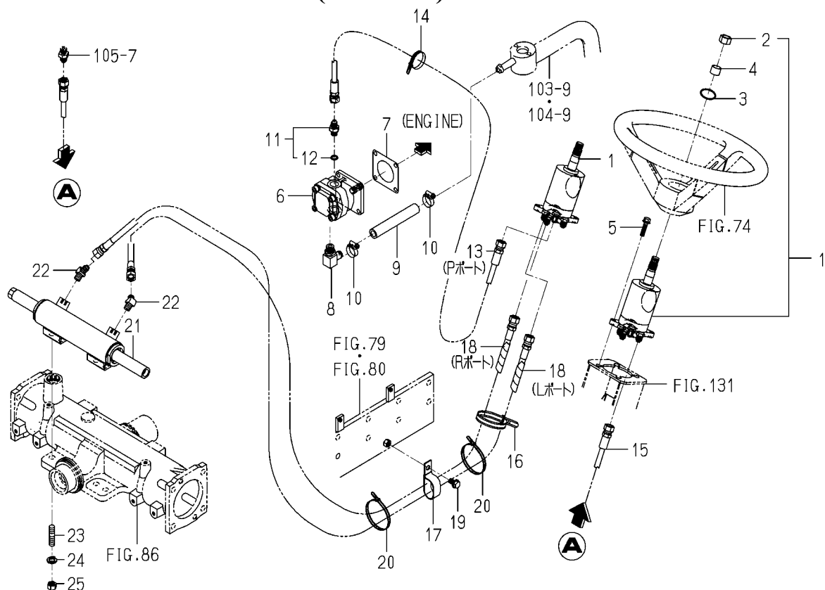
FIG. 78 CONTROLLER(STEERING)SYSTEM (H TYPE)
