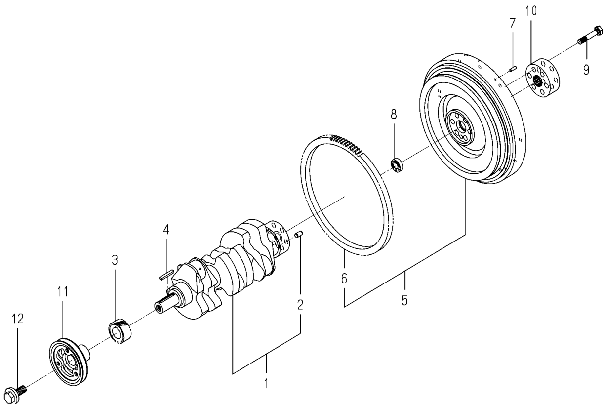
FIG. 17 CRANK SHAFT
