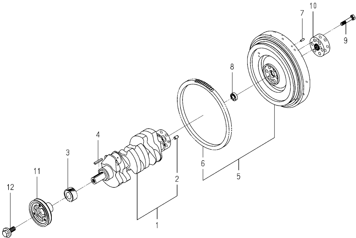
FIG. 17 CRANK SHAFT
