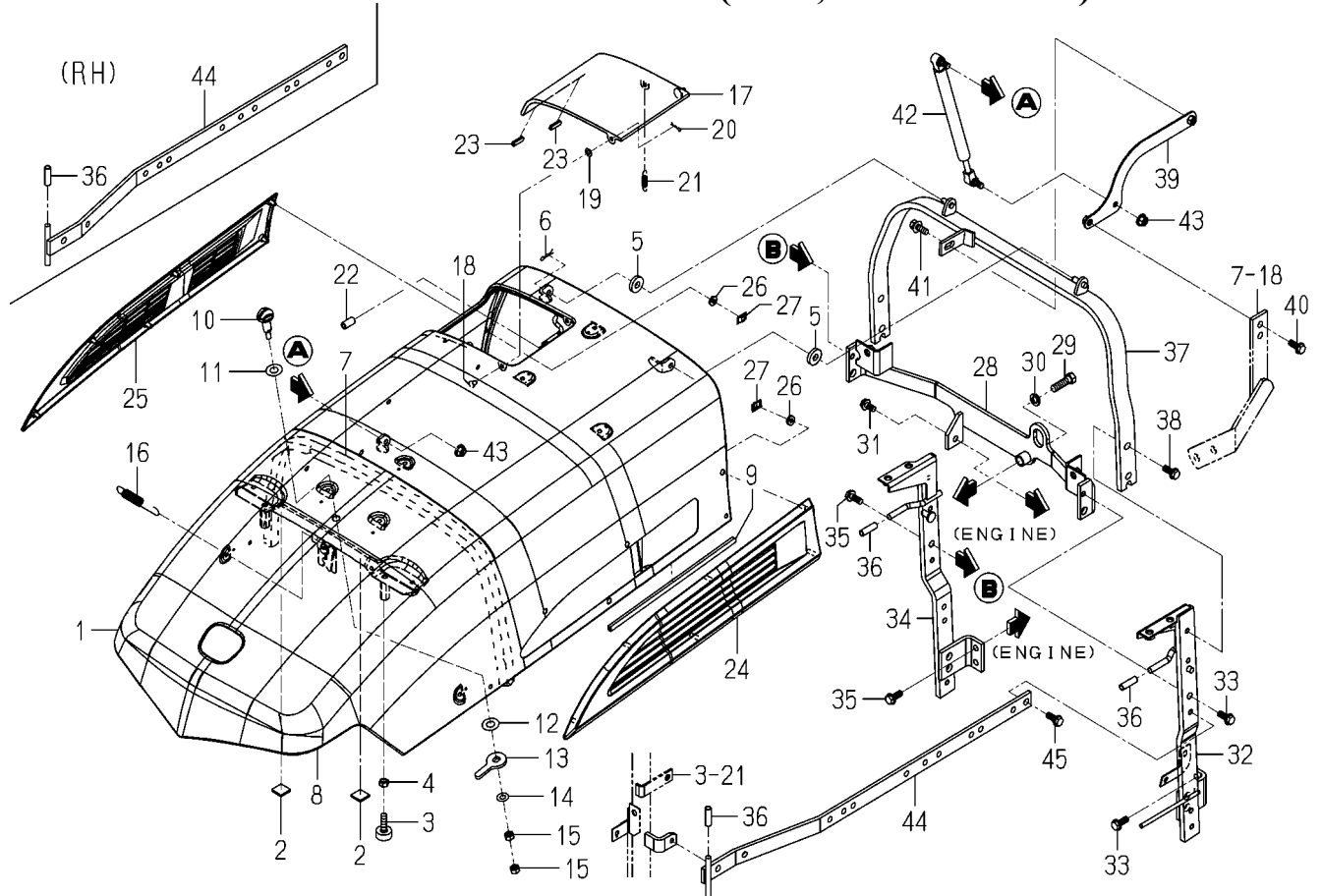
FIG.119 HOOD SYSTEM(4295,4335-H TYPE)
