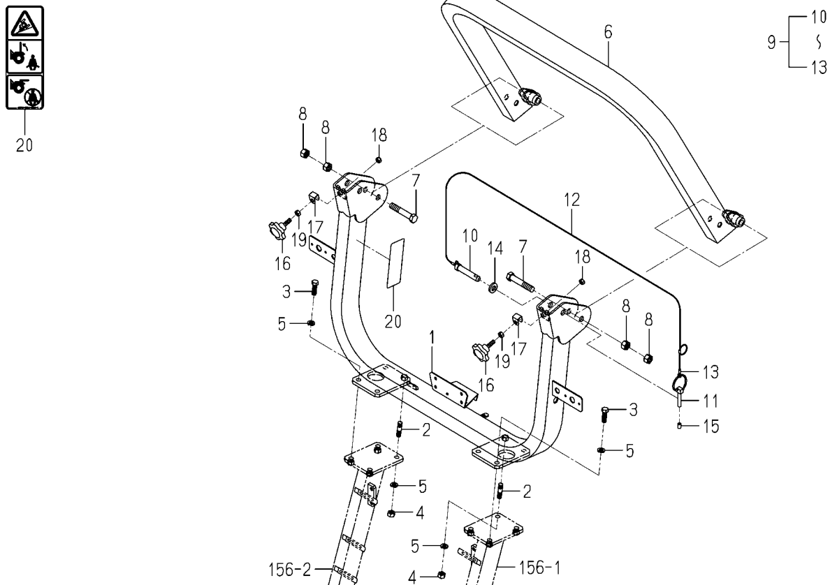
FIG.159 FRAME(REAR/UPPER)SYSTEM (A,C TYPE)
