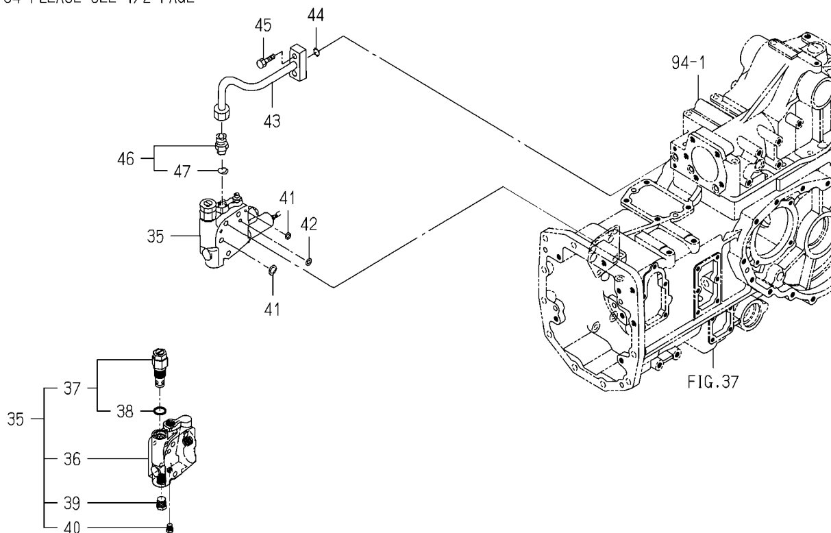
FIG.100 PIPING(MAIN)SYSTEM(2/2) (4295-V TYPE)
