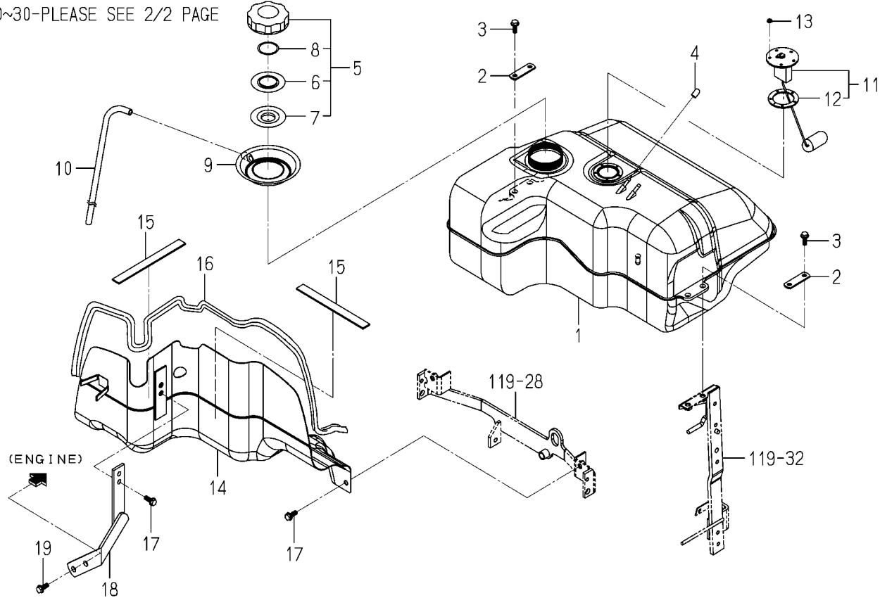
FIG. 7 FUEL SYSTEM(4295,4335-H TYPE)(1/2)
