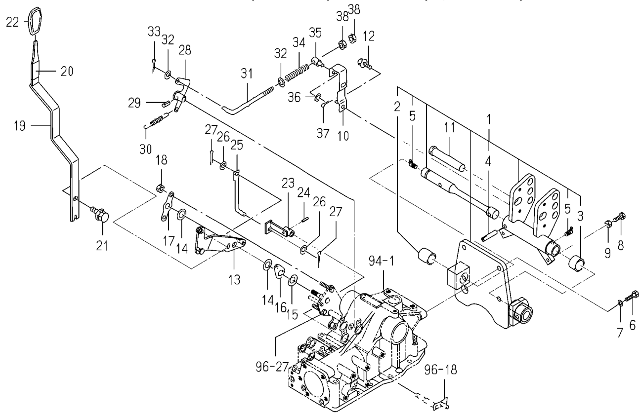
FIG. 99 LEVER(DRAFT)SYSTEM(V,J TYPE)
