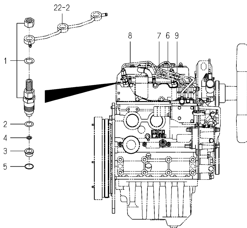
FIG. 20 INJECTION NOZZLE
