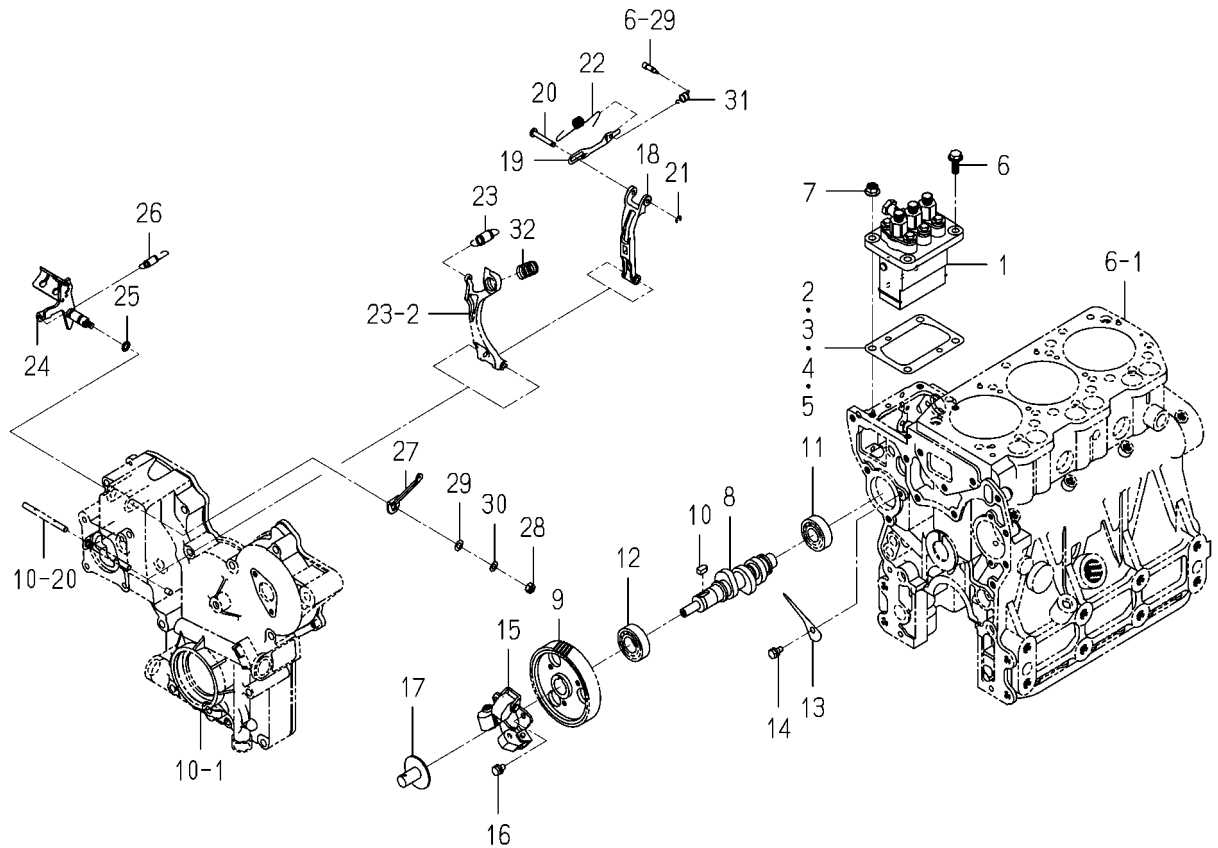
FIG. 21 INJECTION PUMP
