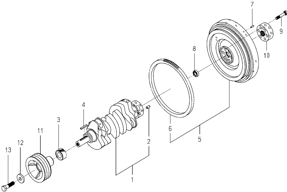
FIG. 16 CRANK SHAFT
