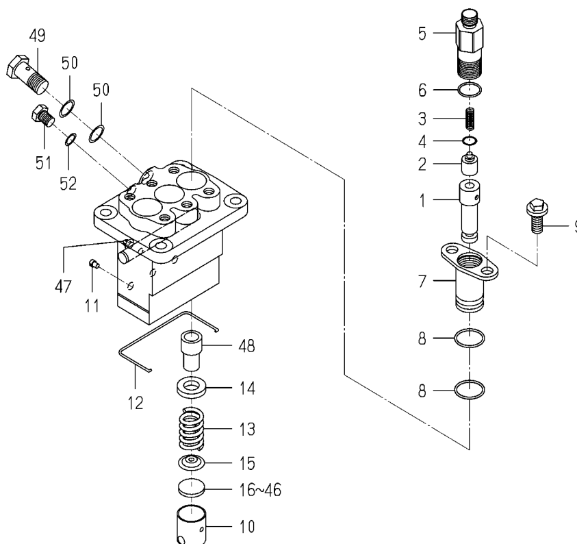
FIG. 33 COMPONENT PARTS FOR 6215-600-104-20 ON Fig.025
