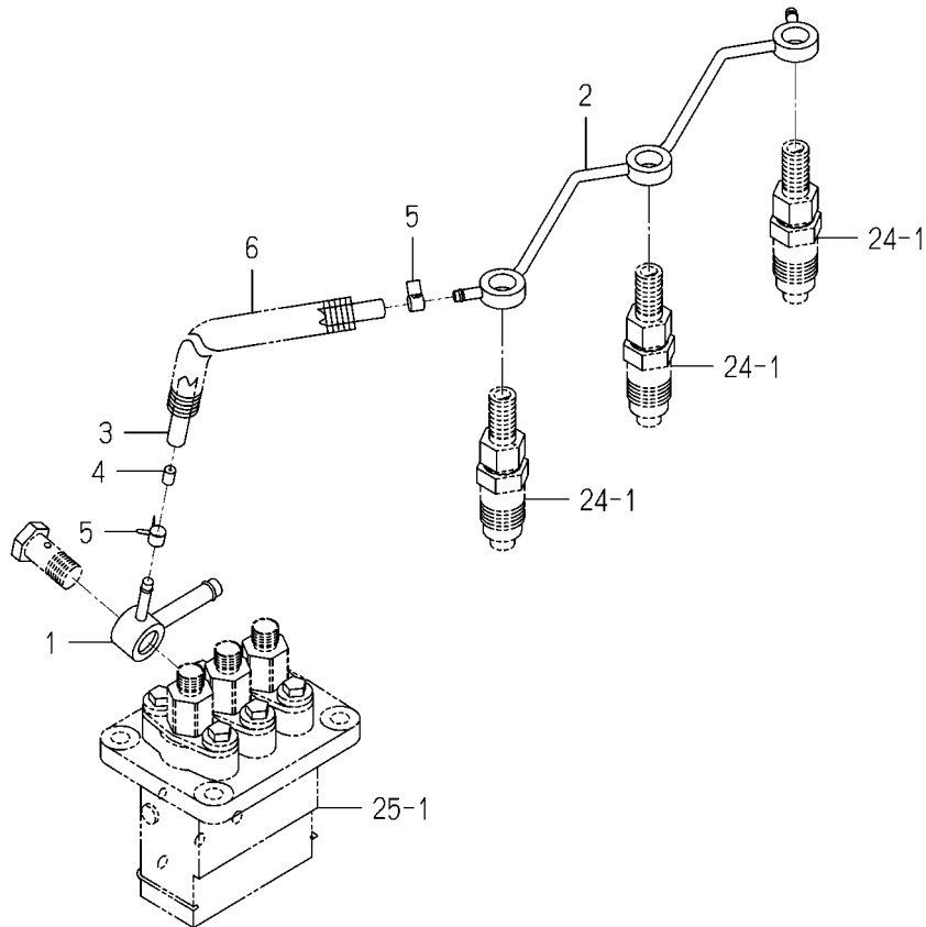
FIG. 26 FUEL PIPE
