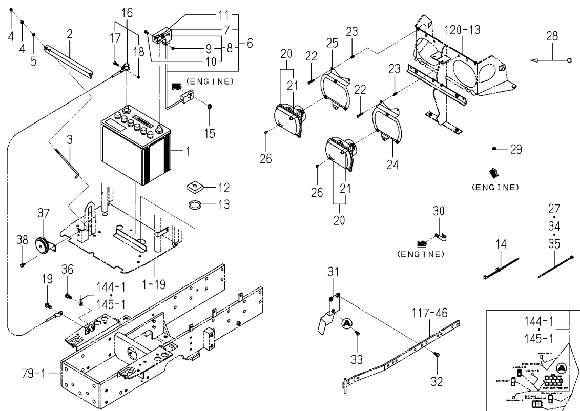
FIG.139 ELC.(FRONT)SYSTEM (4295 TYPE EXCEPT H,V/ 4335 TYPE EXCEPT H,G)
