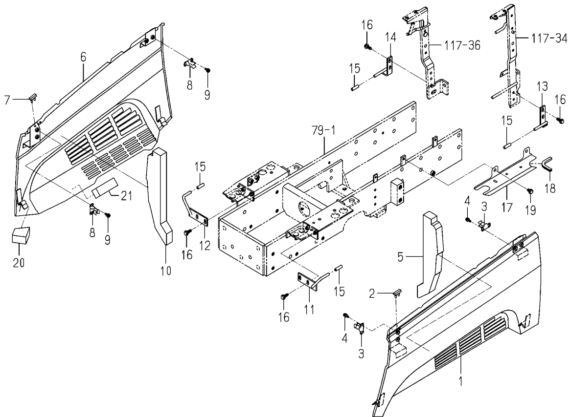
FIG.123 COVER(SIDE)SYSTEM (4295,4335 TYPE EXCEPT H)
