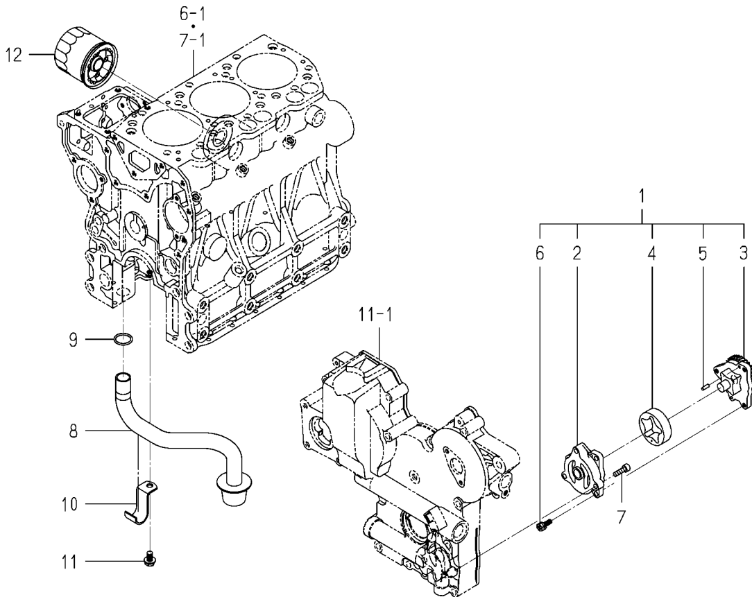
FIG. 19 OIL PUMP
