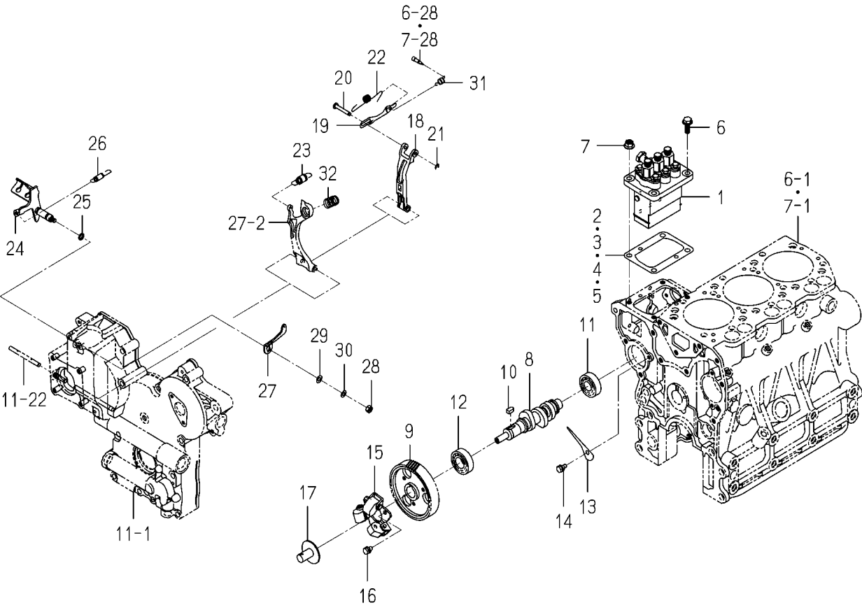
FIG. 25 INJECTION PUMP
