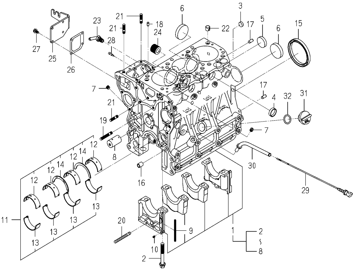
FIG. 7 CYLINDER BLOCK
