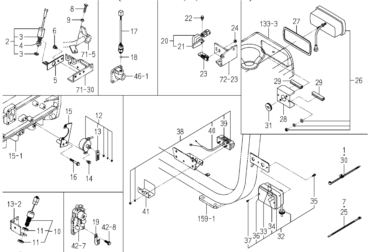
FIG.146 ELC.(REAR)SYSTEM (EXCEPT H,V,JA TYPE)
