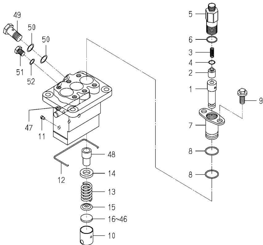
FIG. 32 COMPONENT PARTS FOR 6215-600-104-20 ON Fig.024
