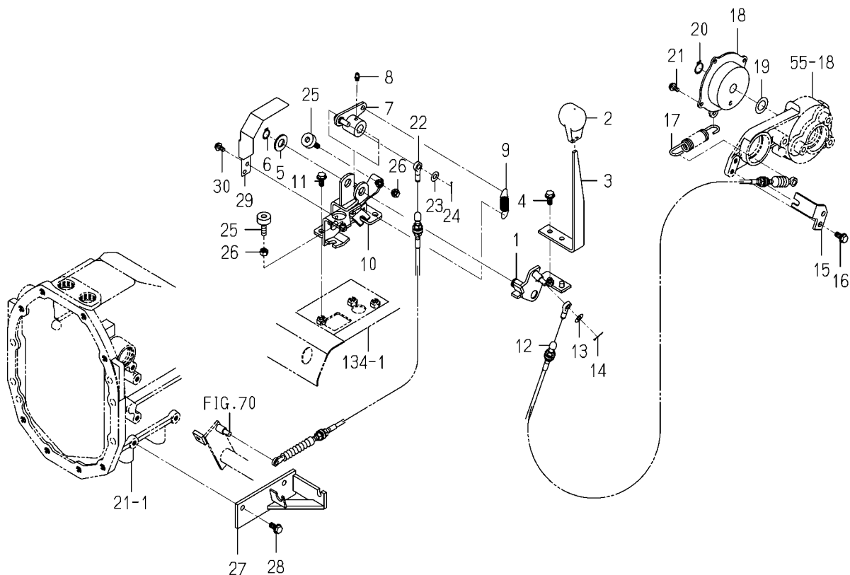
FIG. 56 AUTO CRUISE SYSTEM (H TYPE EXCEPT C)
