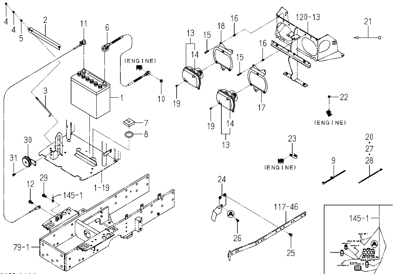
FIG.141 ELC.(FRONT)SYSTEM(4295-V TYPE)
