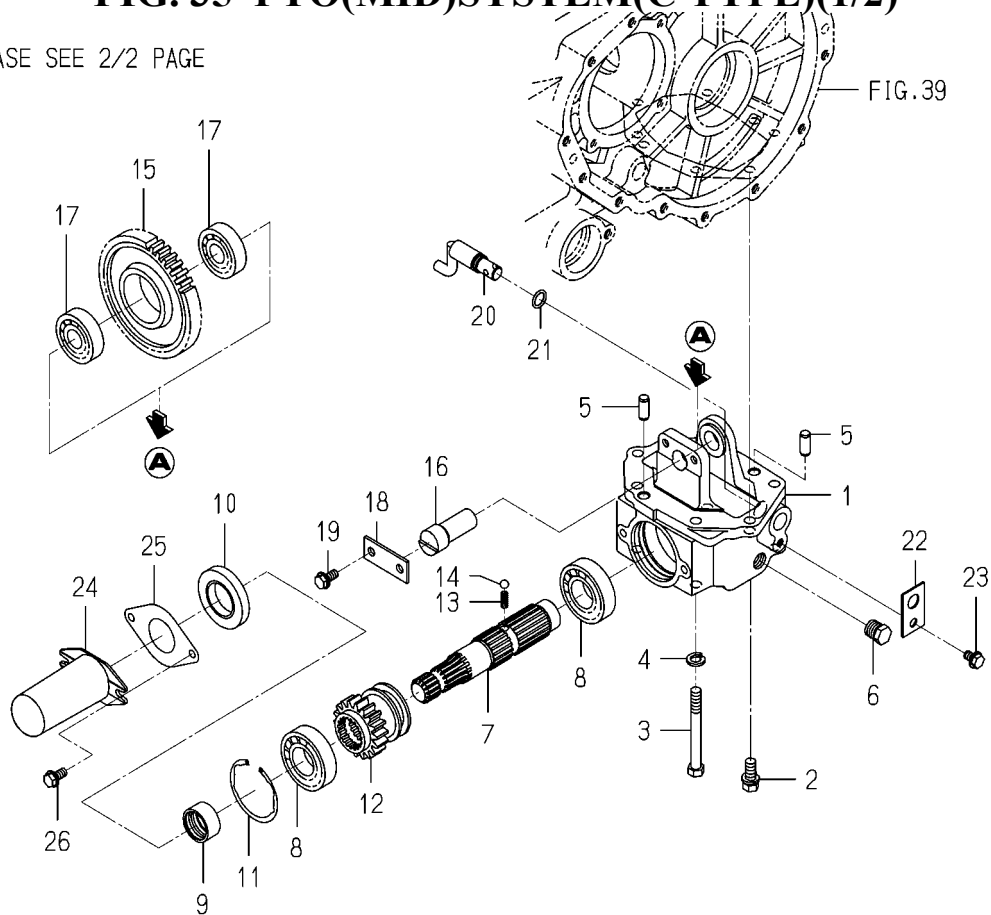
FIG. 35 PTO(MID)SYSTEM(C TYPE)(1/2)
