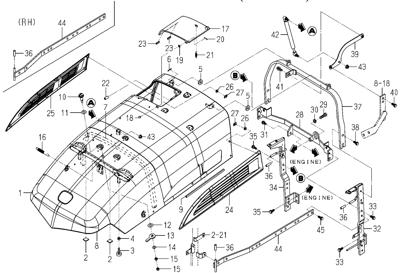
FIG.118 HOOD SYSTEM(4365 TYPE)
