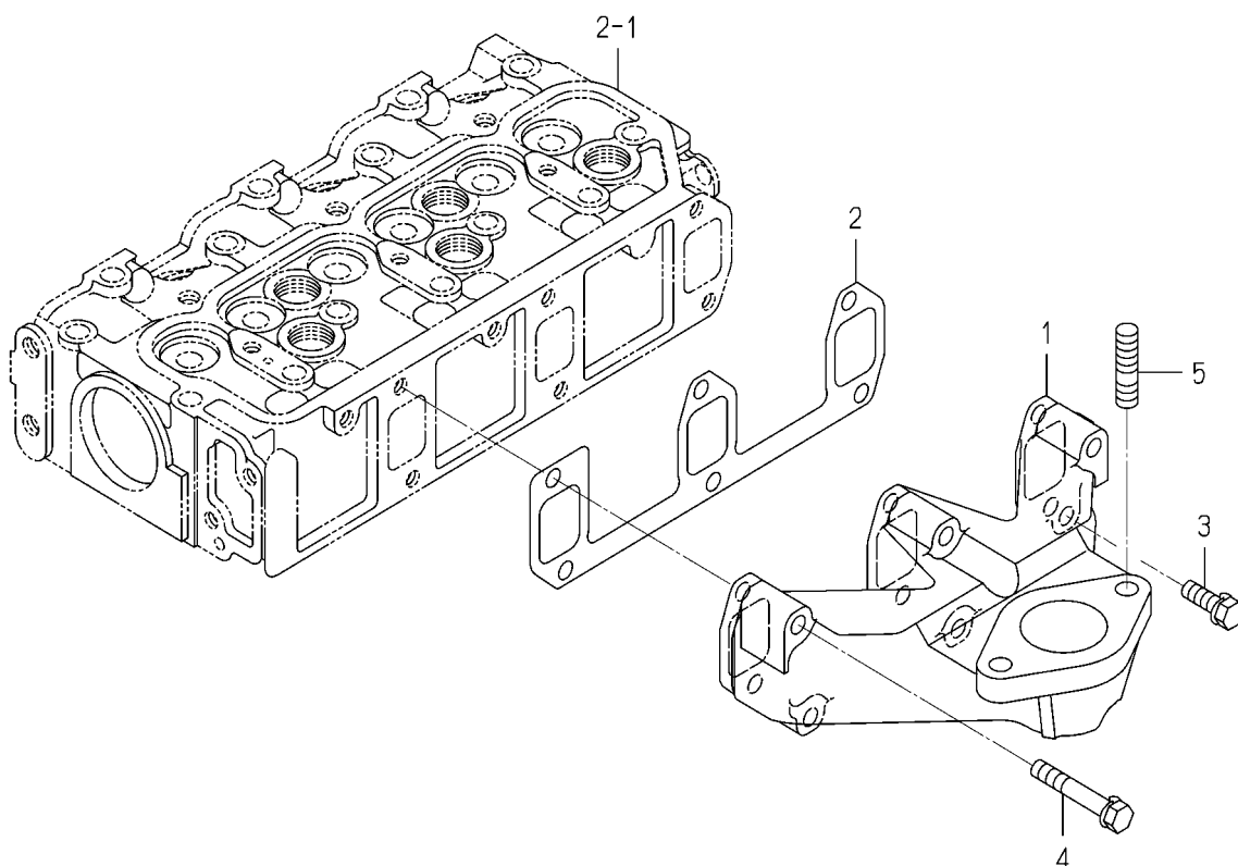
FIG. 5 EXHAUST MANIFOLD
