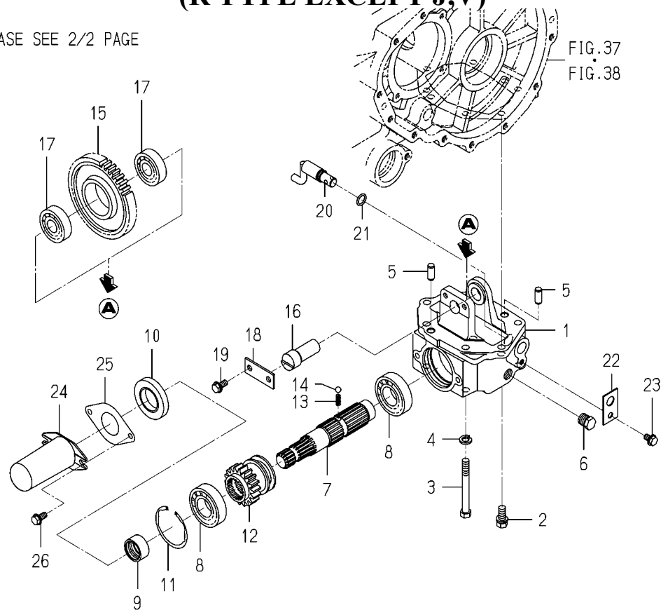
FIG. 36 PTO(MID)SYSTEM(1/2) (R TYPE EXCEPT J,V)
