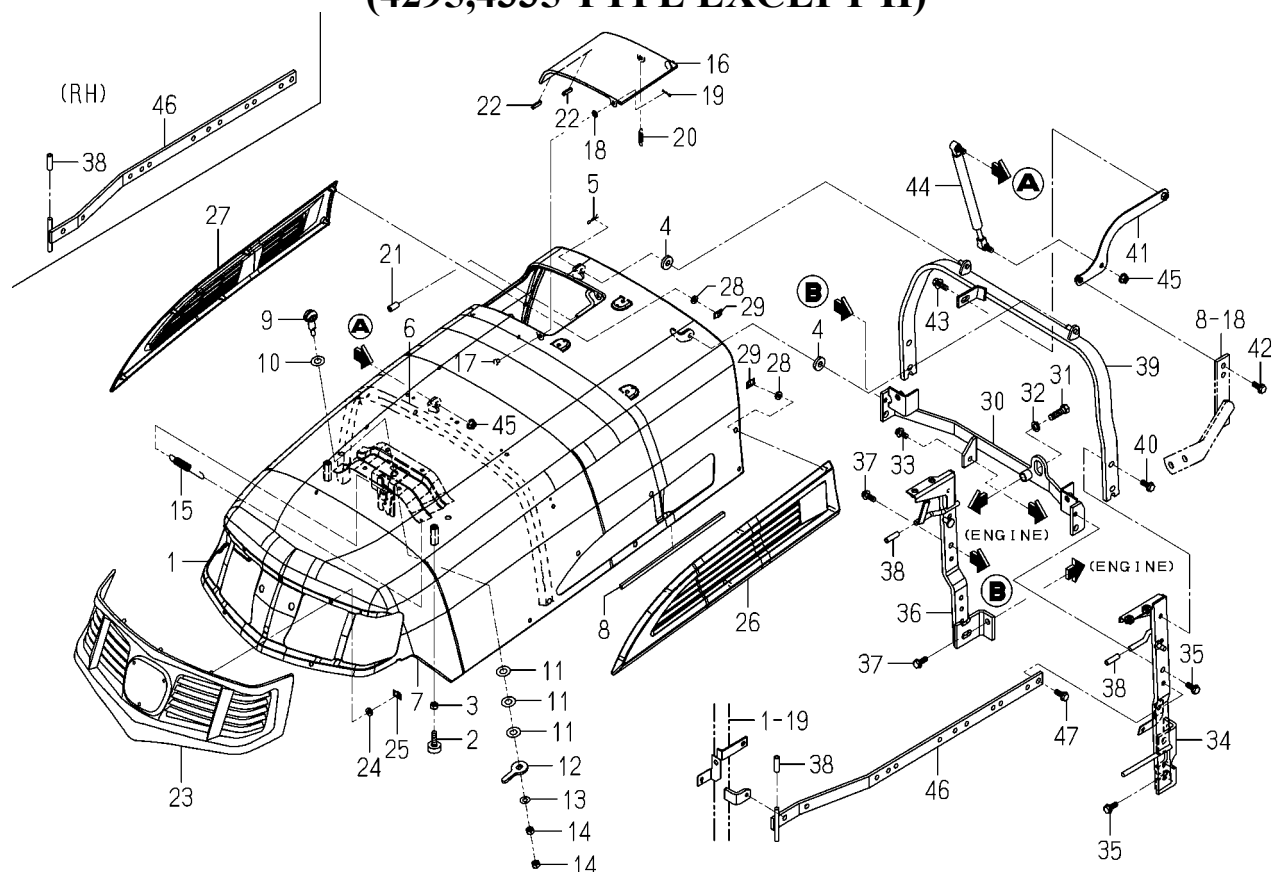
FIG.117 HOOD SYSTEM (4295,4335 TYPE EXCEPT H)
