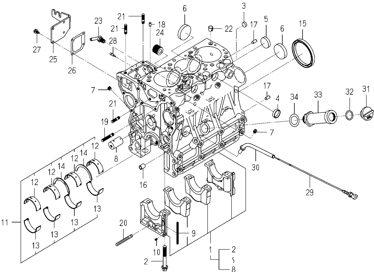
FIG. 7 CYLINDER BLOCK
