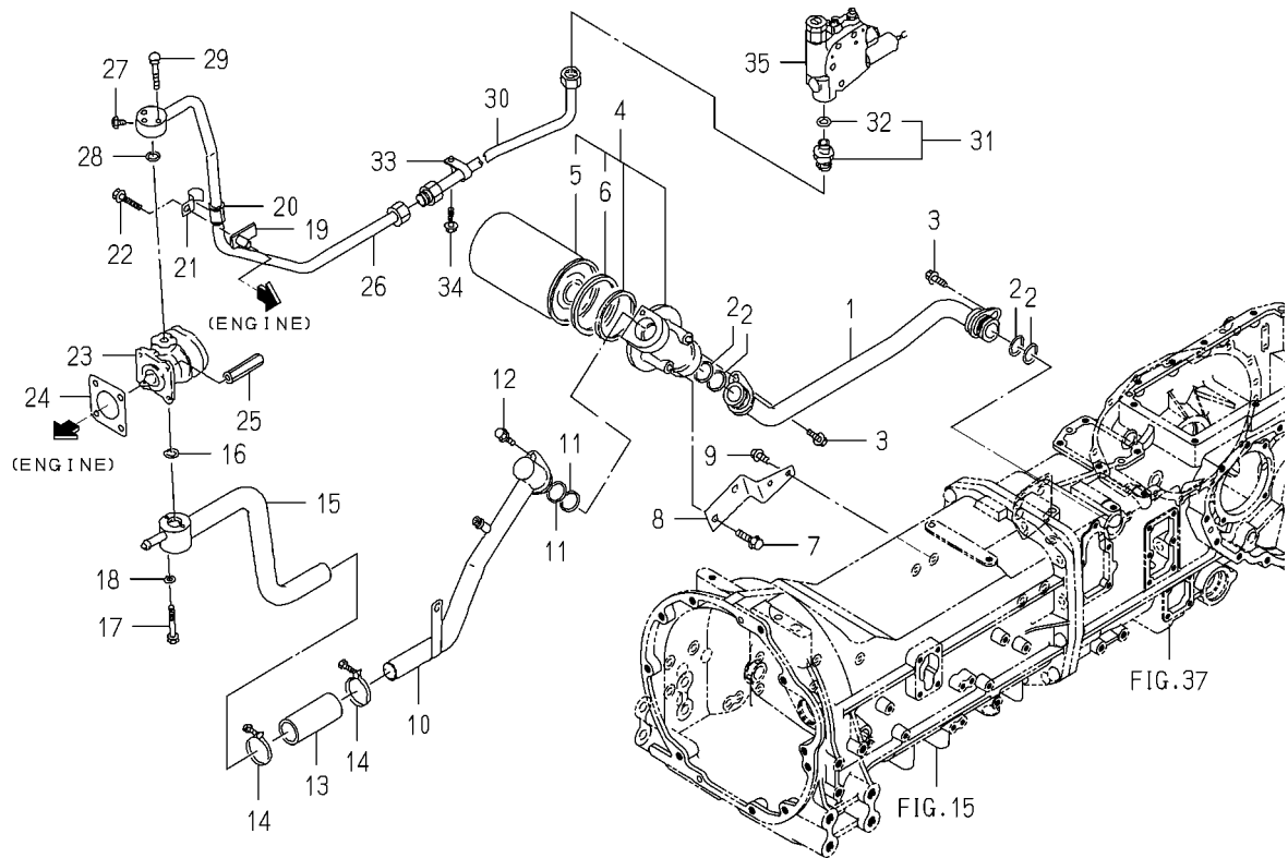
FIG.102 PIPING(MAIN)SYSTEM(1/2) (4295 TYPE EXCEPT H,V/ 4335 TYPE EXCEPT H)
