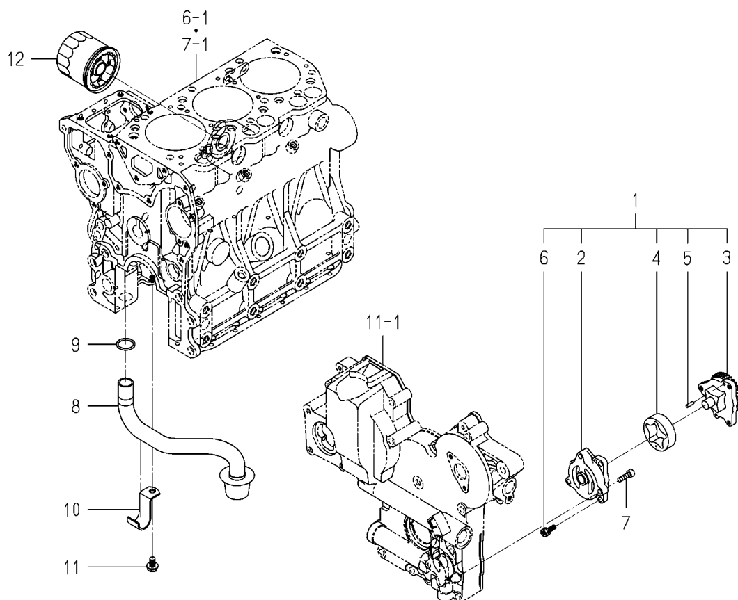
FIG. 20 OIL PUMP
