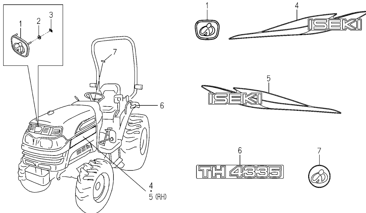
FIG.160 ORNAMENT(4335 TYPE EXCEPT H)
