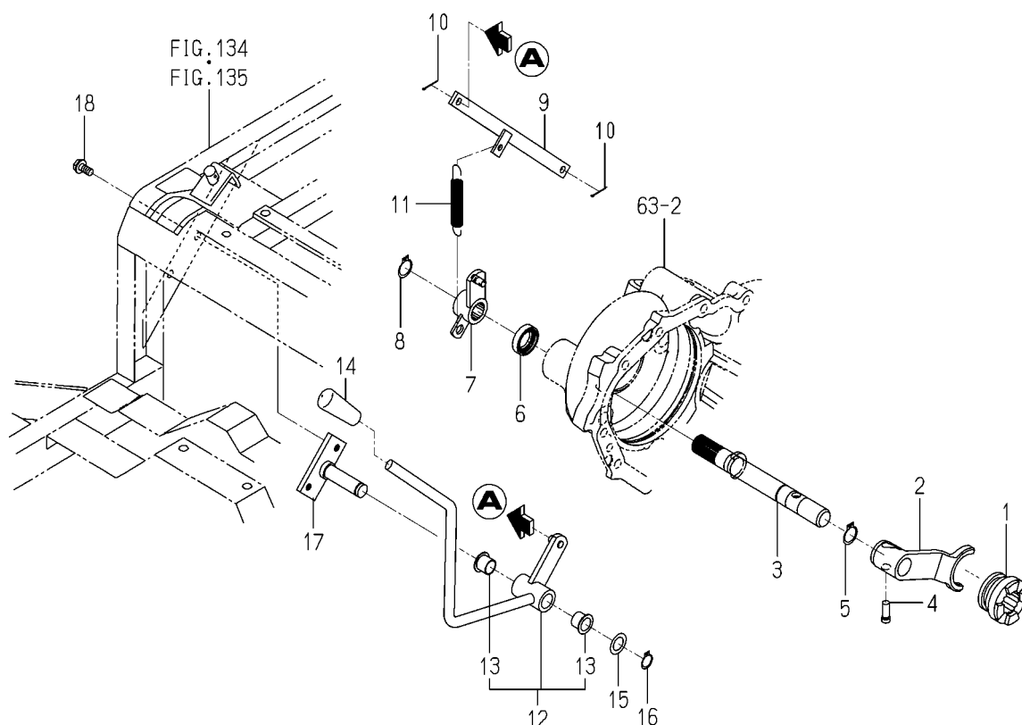
FIG. 67 CLUTCH(DIFFERENTIAL GEAR)SYSTEM (H TYPE)
