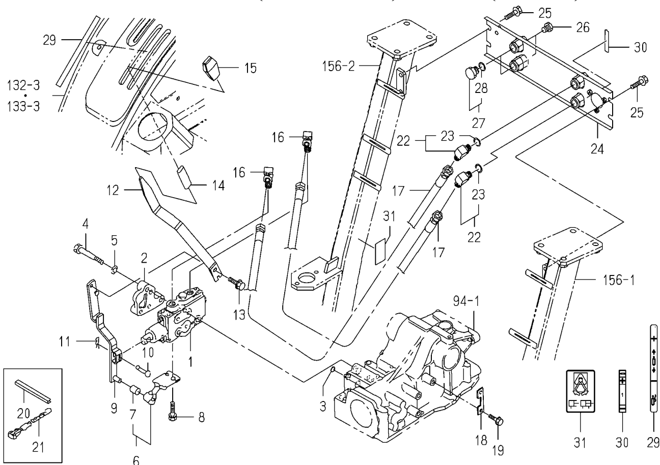
FIG.108 VALVE(REMOTE/1R)SYSTEM(V TYPE)
