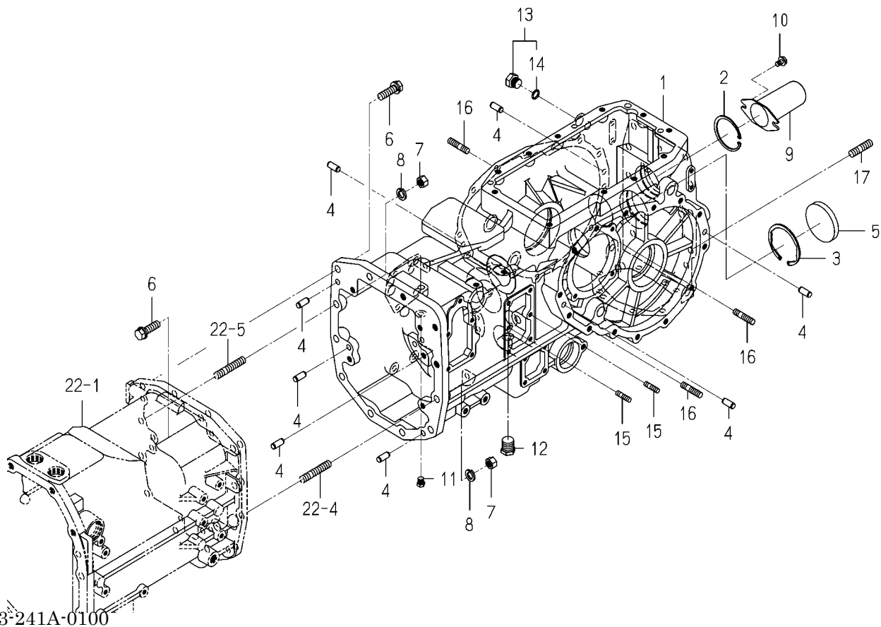
FIG. 38 CASE(TRANSMISSION/REAR)SYSTEM (HR TYPE)
