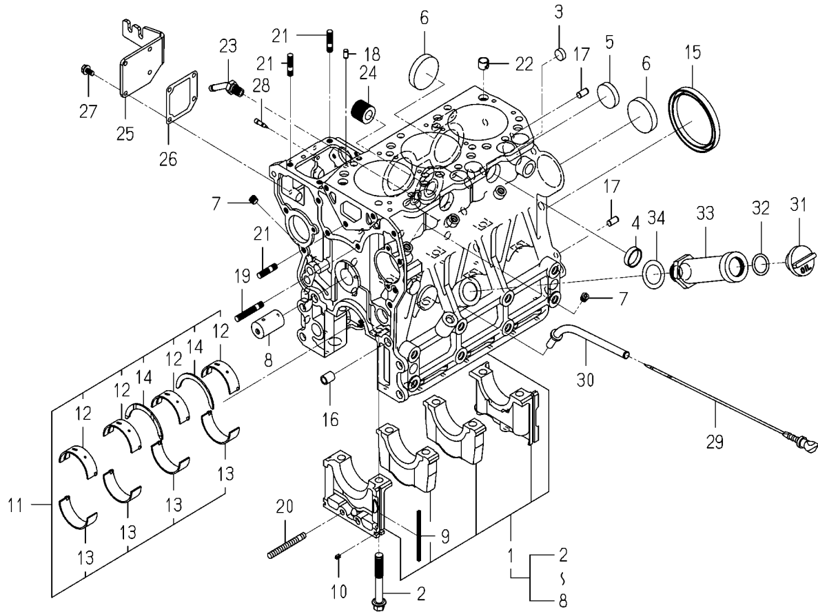
FIG. 6 CYLINDER BLOCK
