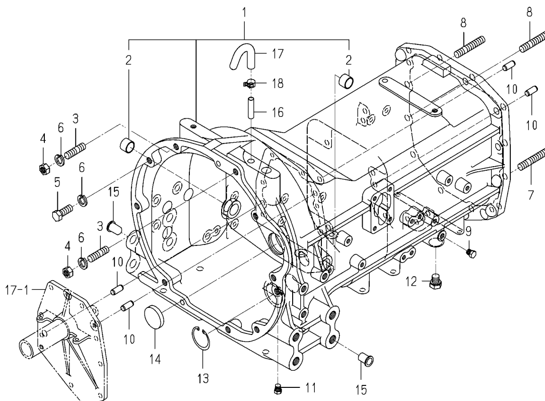
FIG. 14 CASE(TRANSMISSION/FRONT)SYSTEM (4295-V TYPE)
