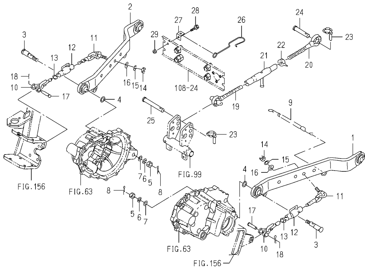
FIG.110 LINK(3P)SYSTEM (V TYPE,J TYPE EXCEPT M)
