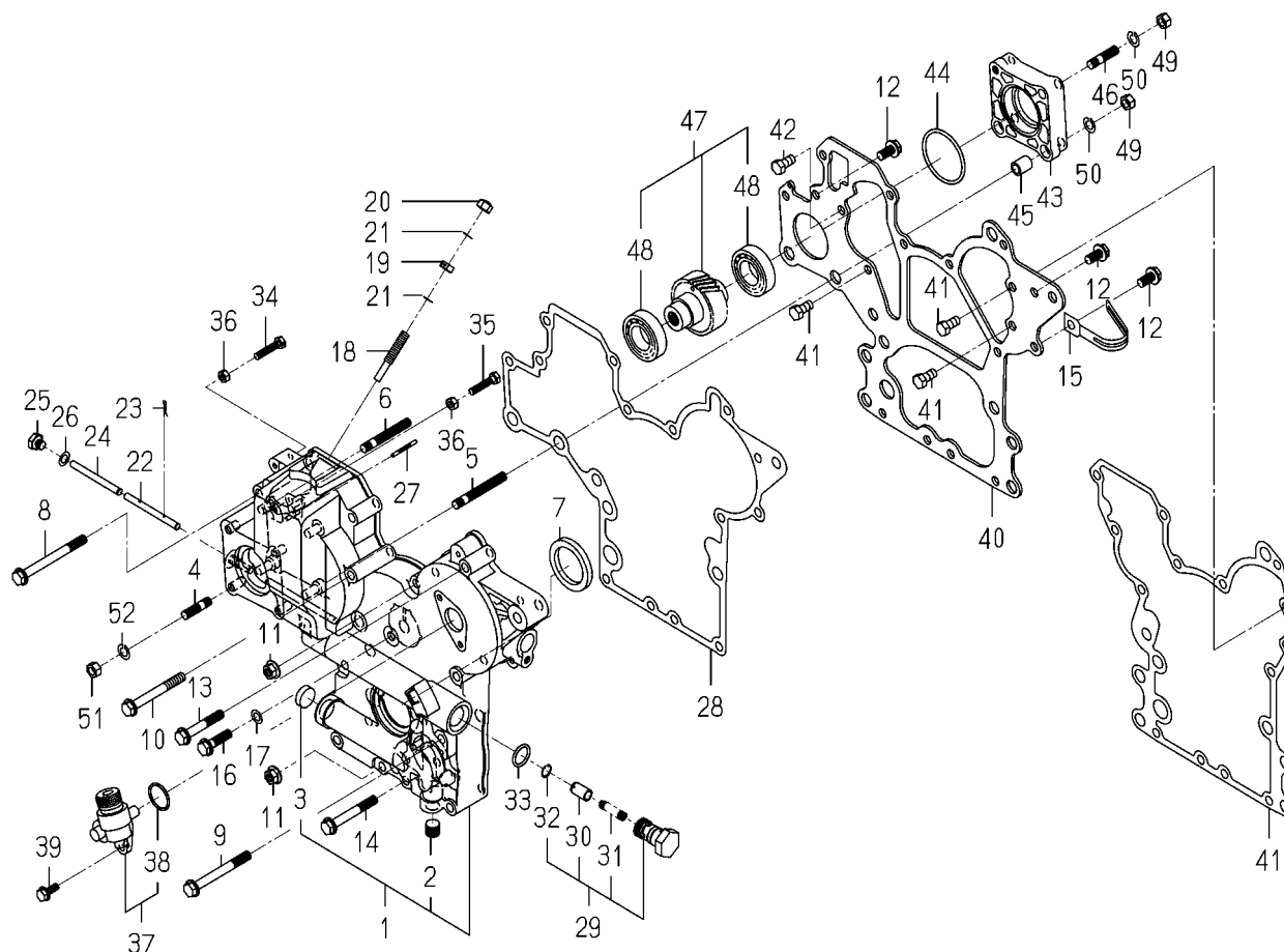
FIG. 11 TIMING GEAR CASE
