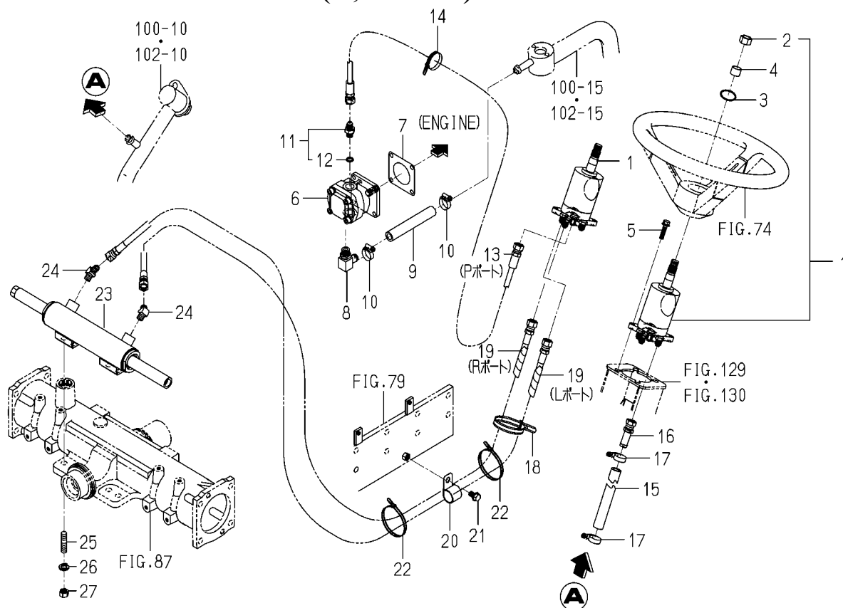
FIG. 76 CONTROLLER(STEERING)SYSTEM (V,J TYPE)
