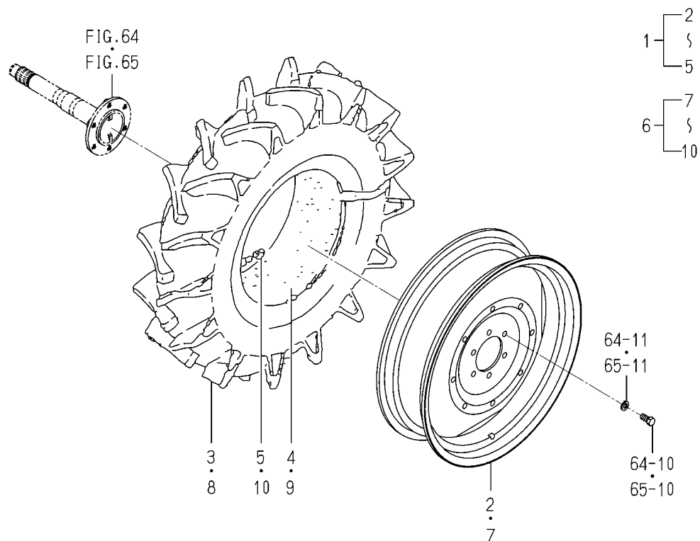
FIG.179 WHEEL(REAR/AGR/9.5-24)SYSTEM (OPTION)
