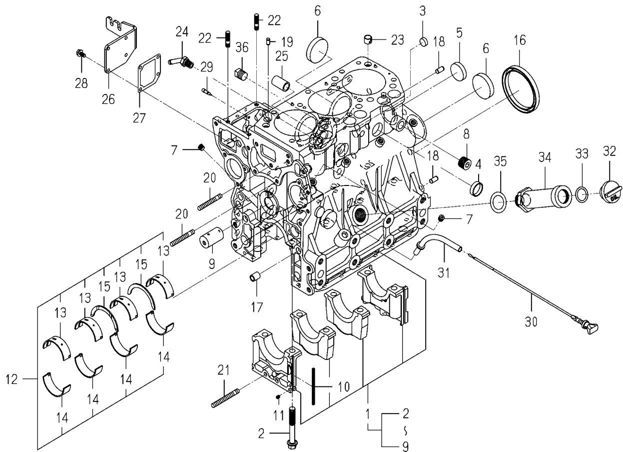
FIG. 6 CYLINDER BLOCK
