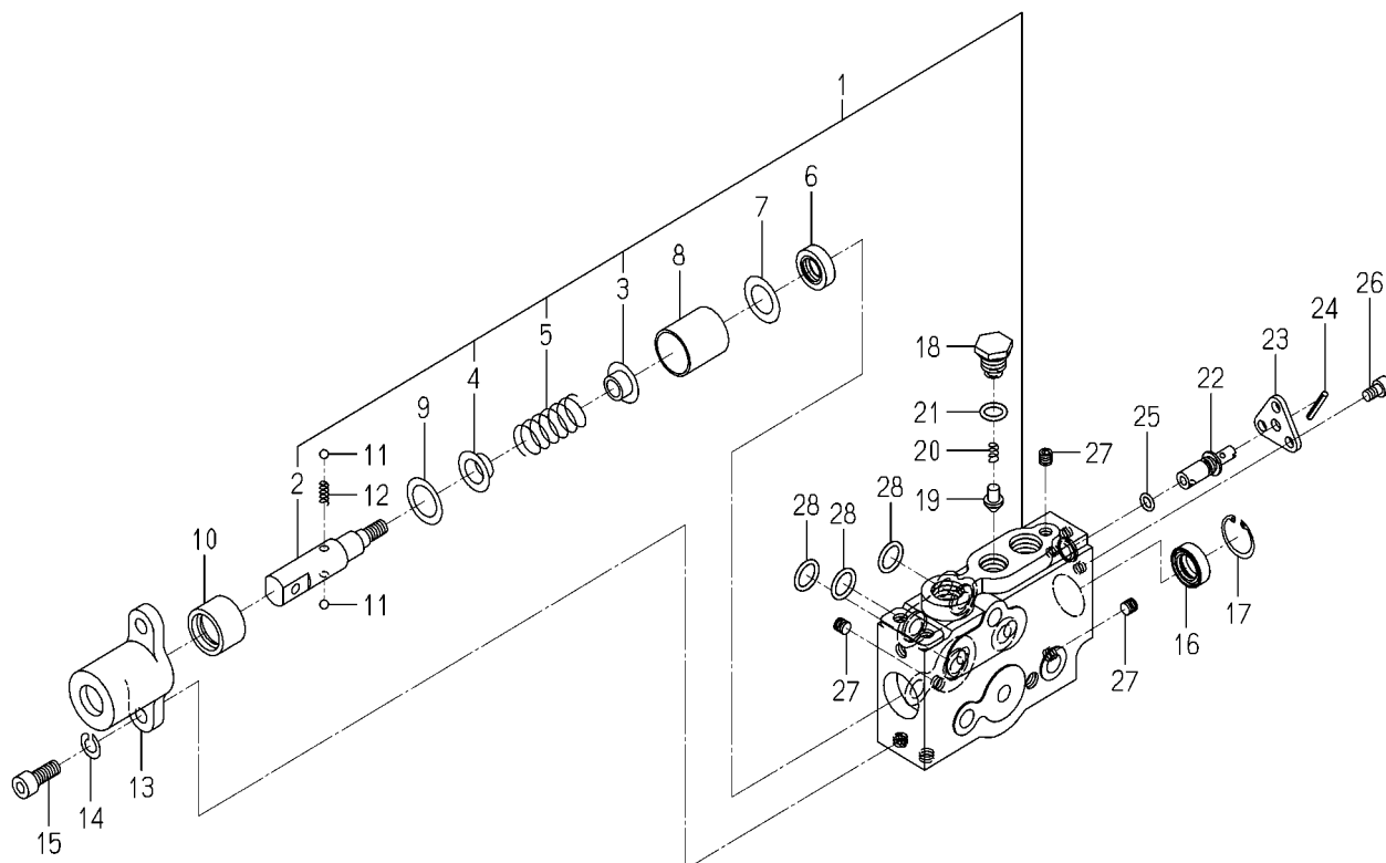
FIG.202 COMPONENT PARTS FOR 1719-511-350-00 ON Fig.108,109
