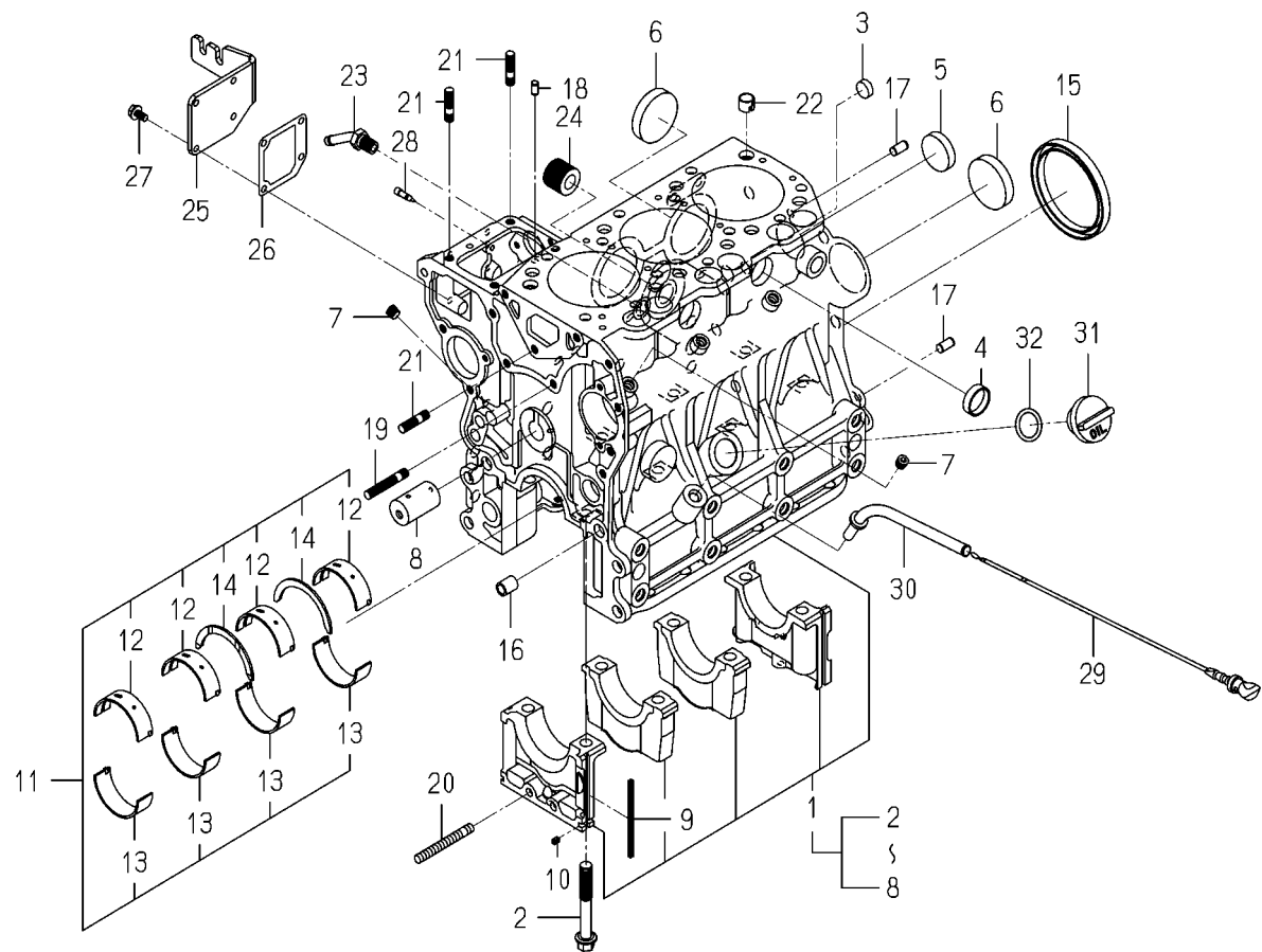
FIG. 6 CYLINDER BLOCK
