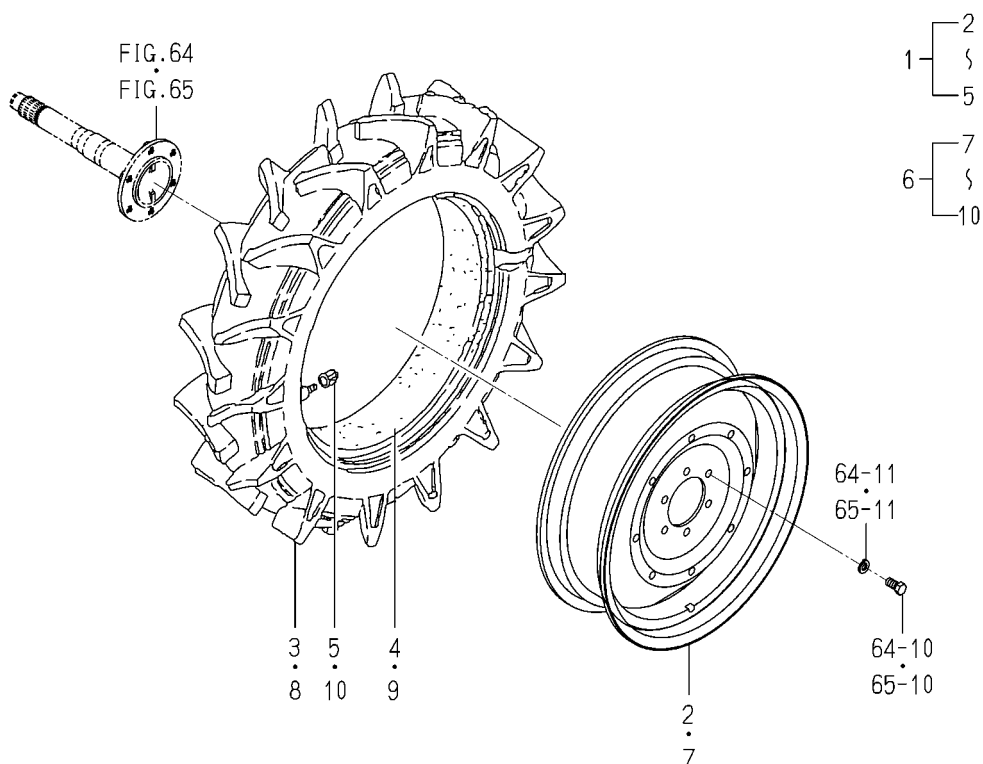
FIG.182 WHEEL(REAR/AGR/9.5-22)SYSTEM (OPTION)
