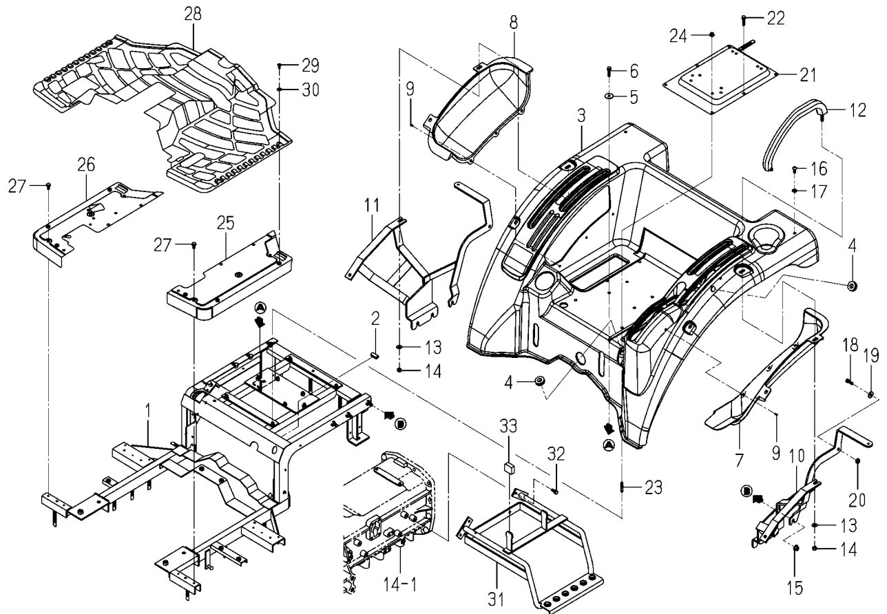
FIG.132 FLOOR(REAR)SYSTEM(4295-V TYPE)
