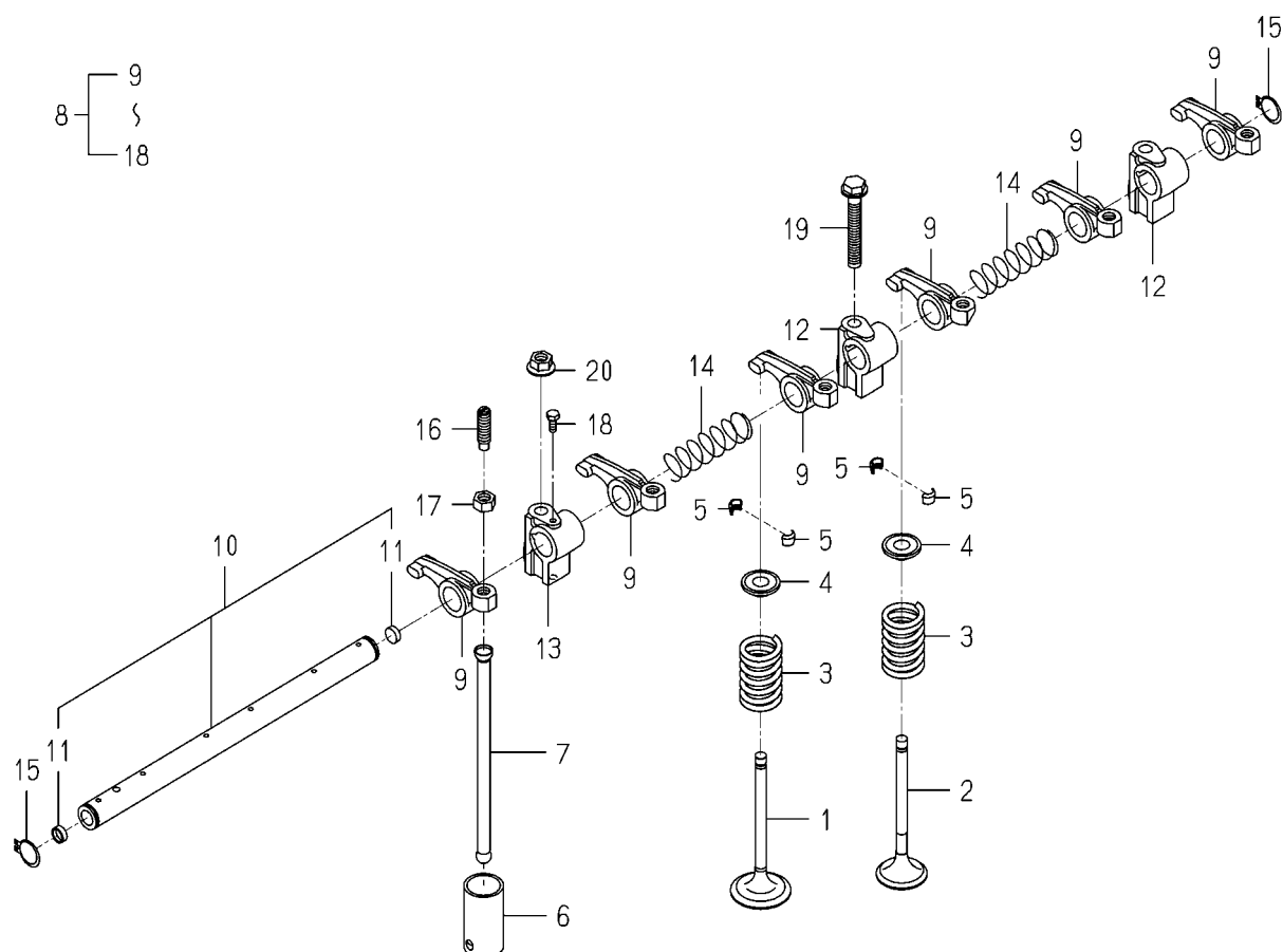
FIG. 13 VALVE
