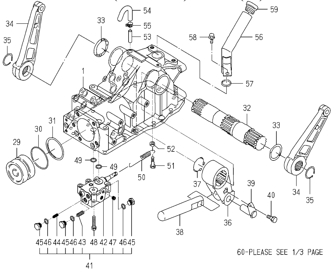
FIG. 94 CASE(CYLINDER)SYSTEM(2/3)
