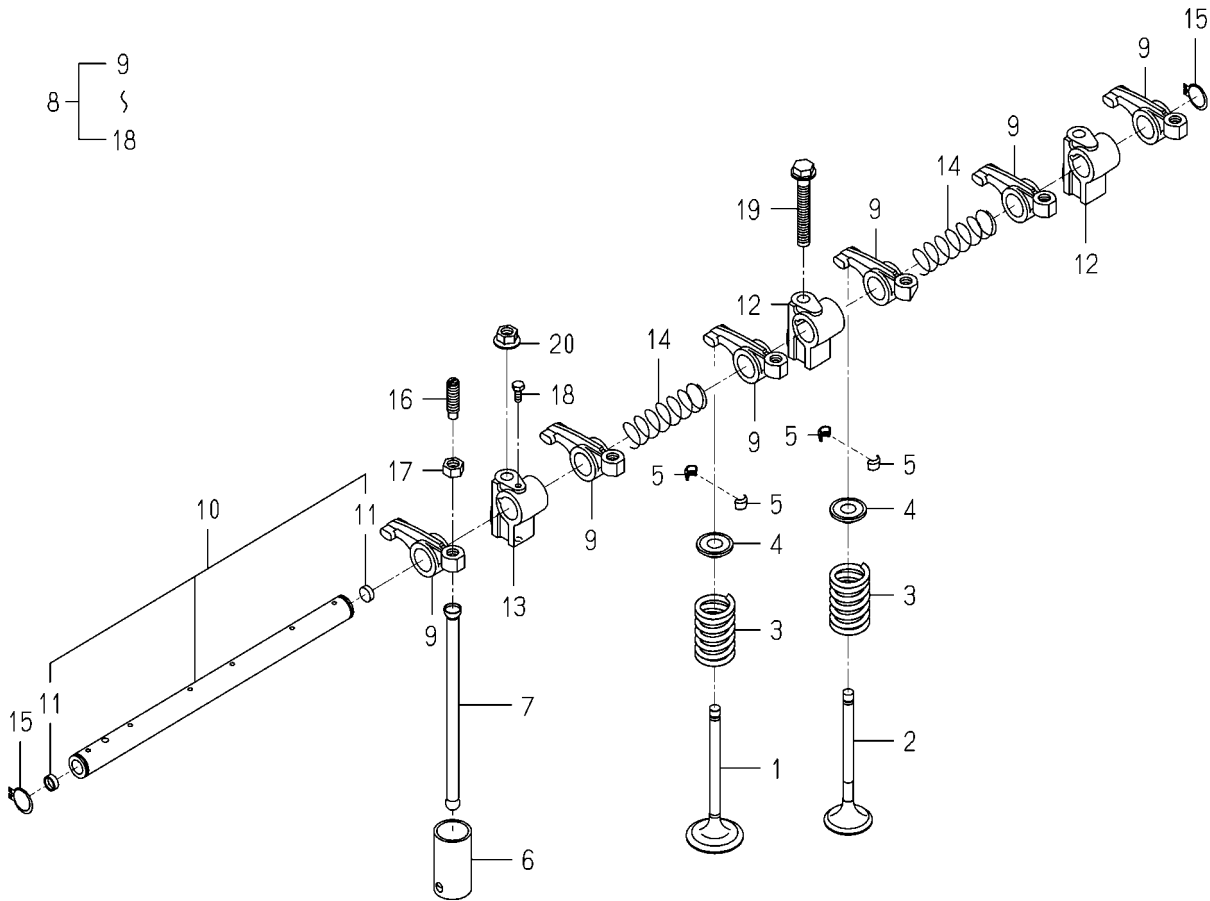
FIG. 13 VALVE
