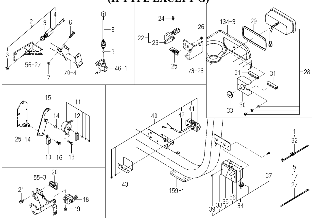
FIG.149 ELC.(REAR)SYSTEM (H TYPE EXCEPT G)
