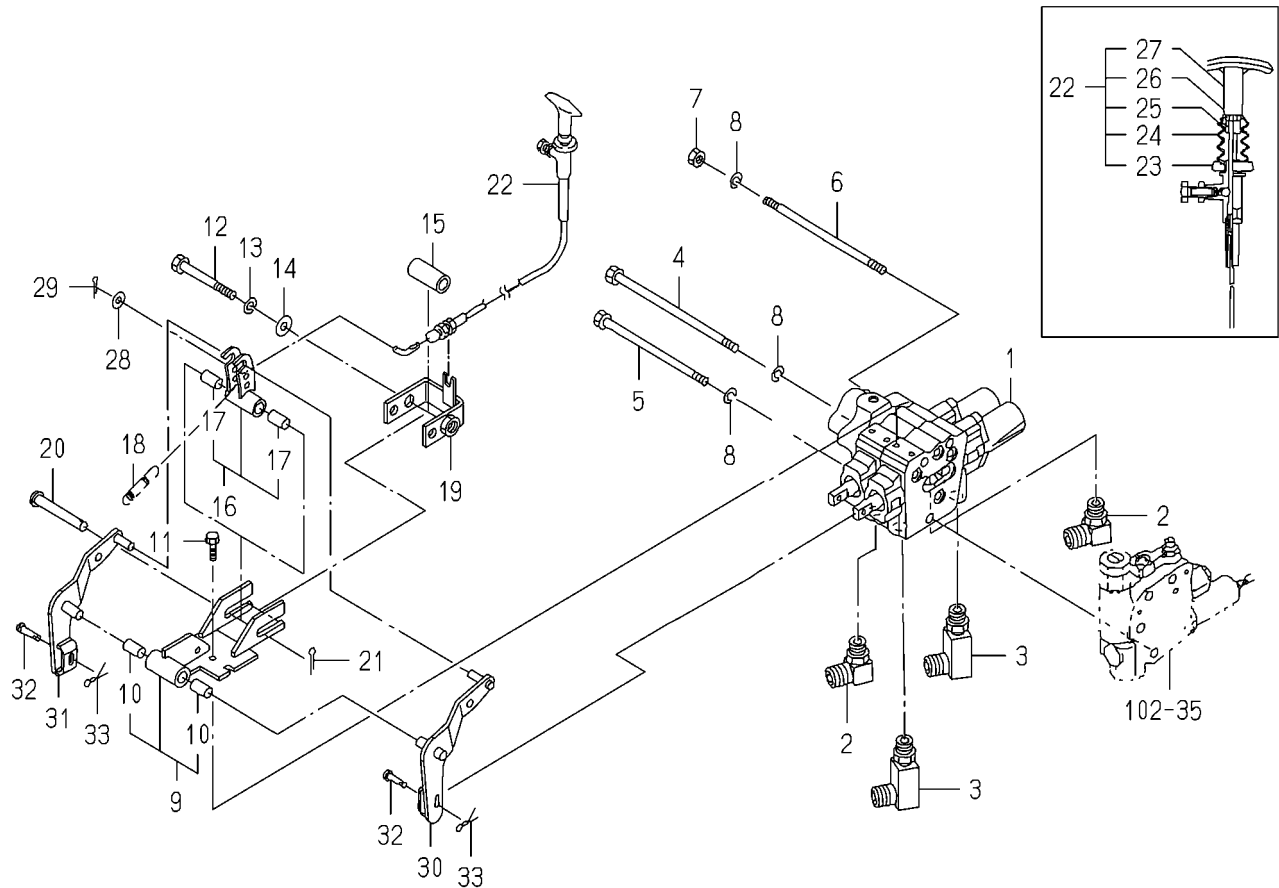
FIG.107 JOY STICK SYSTEM(4335-J TYPE)(1/2)
