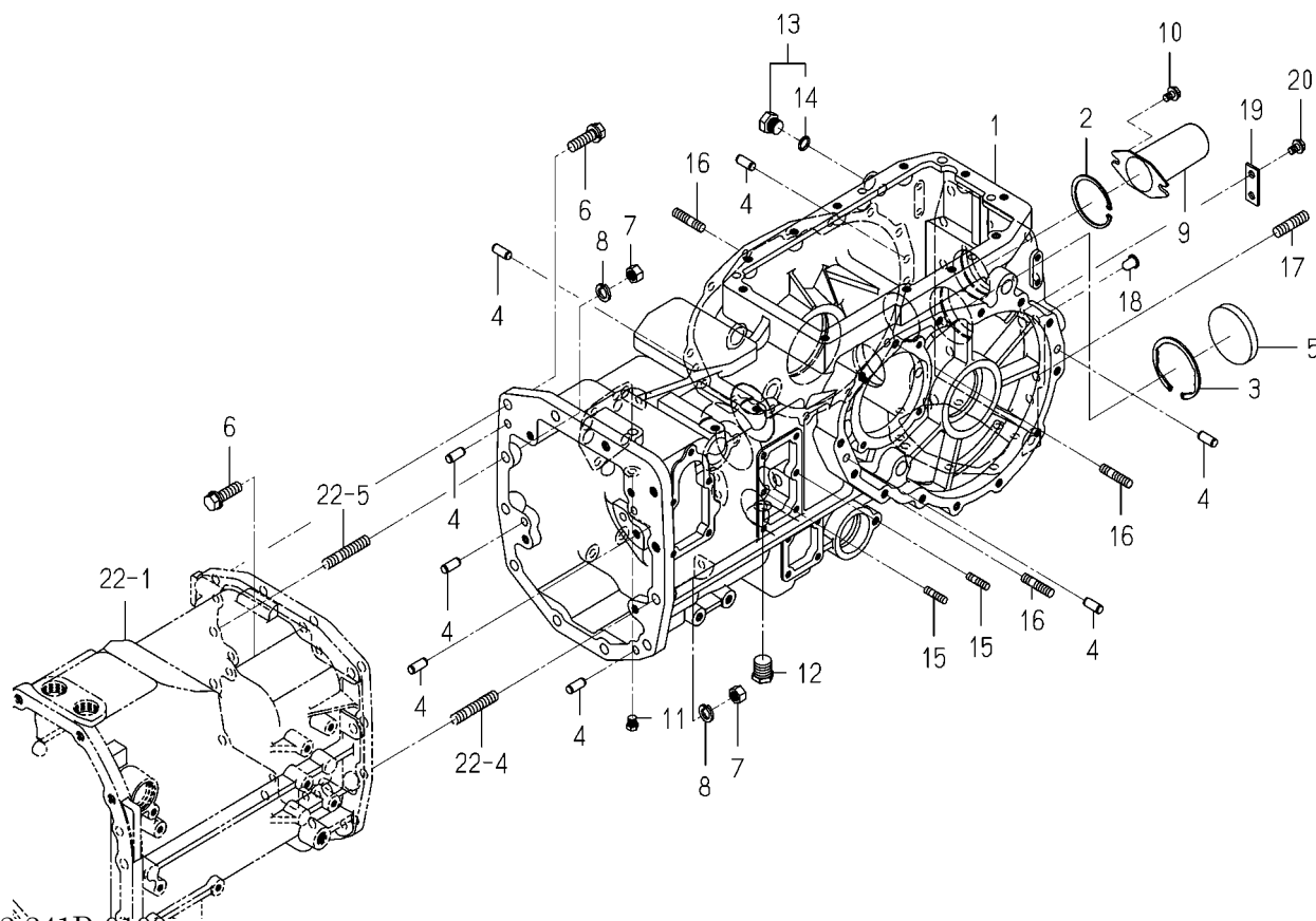
FIG. 39 CASE(TRANSMISSION/REAR)SYSTEM (C TYPE)
