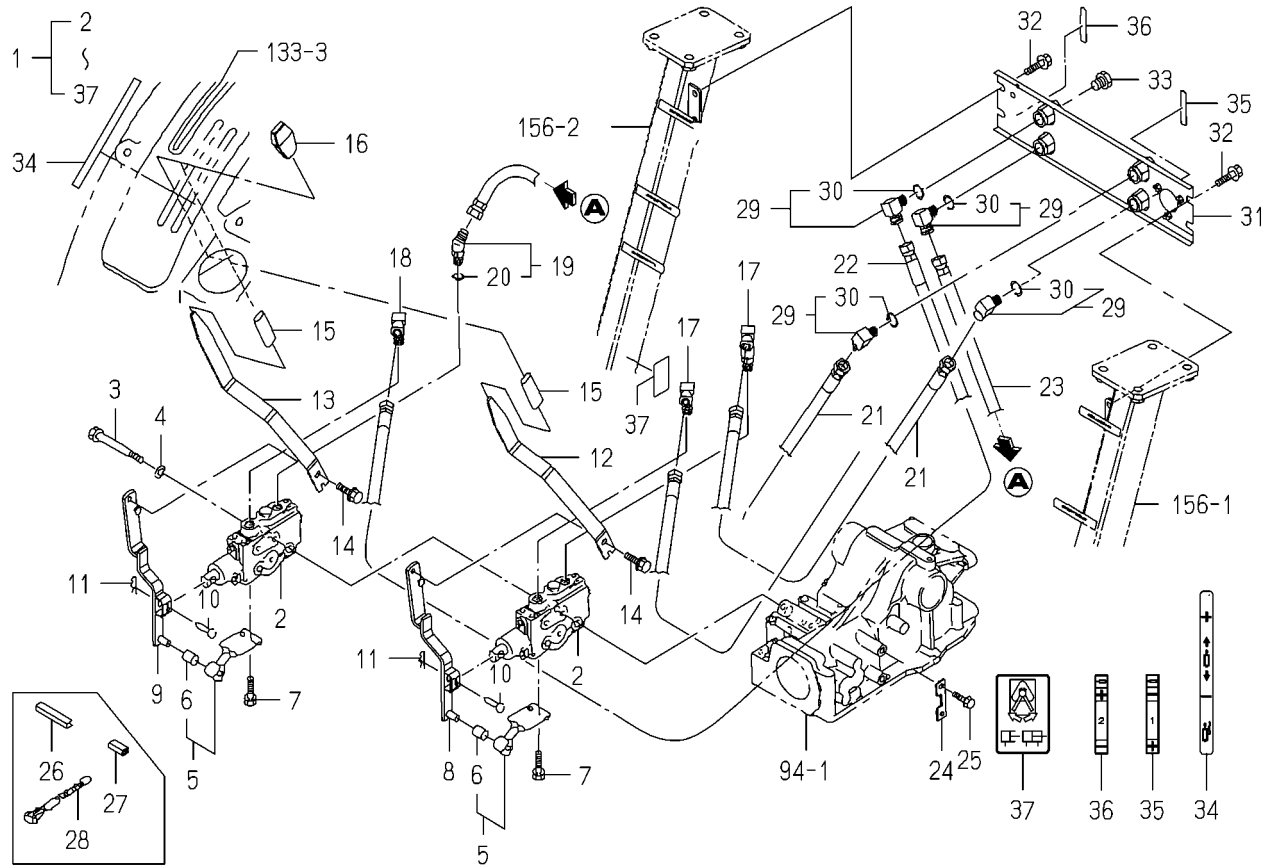
FIG.190 VALVE(REMOTE/2ND/3)SET (J TYPE)(OPTION)
