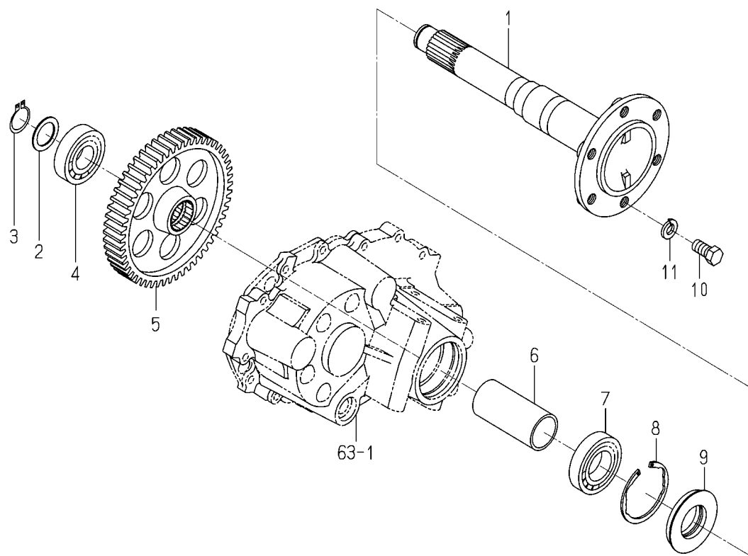
FIG. 65 SHAFT(WHEEL/REAR)SYSTEM(H TYPE)
