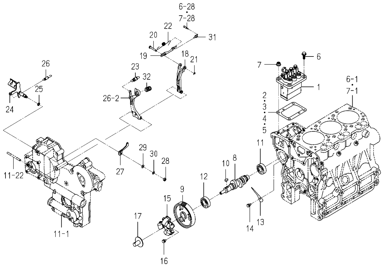
FIG. 24 INJECTION PUMP
