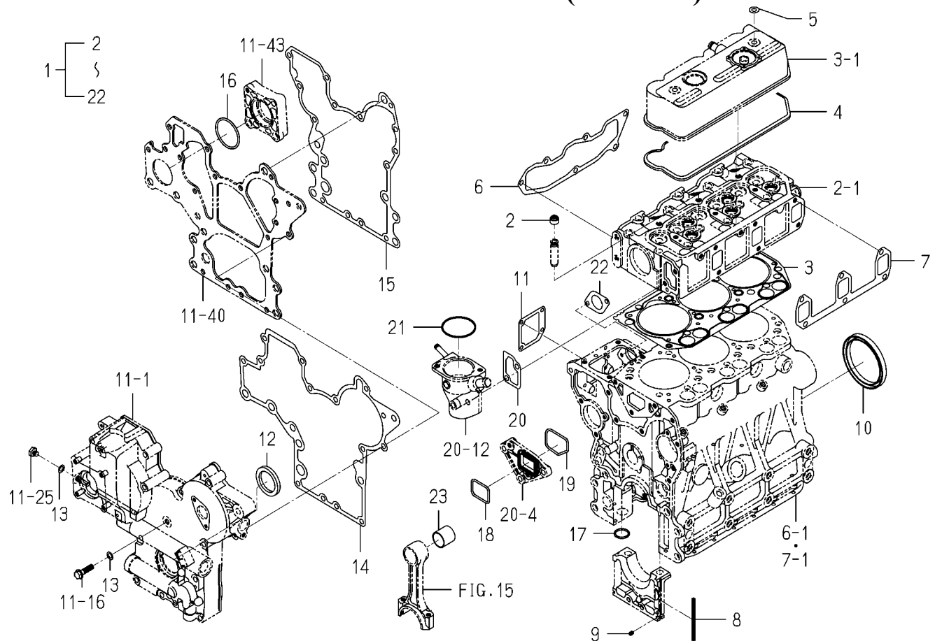
FIG. 30 REPAIR PARTS(OPTION)
