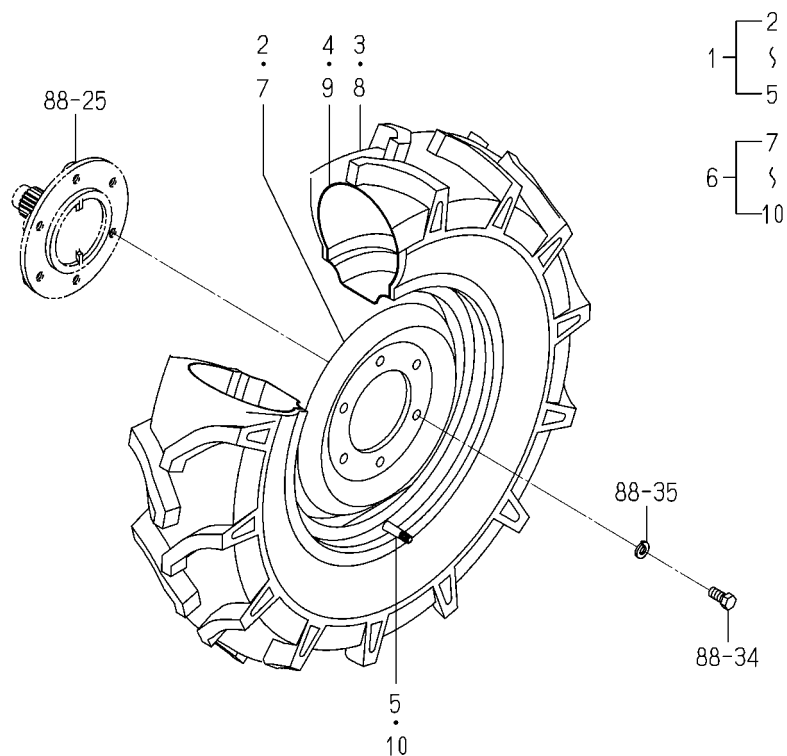
FIG.187 WHEEL(FRONT/AGR/7-14)SYSTEM (OPTION)
