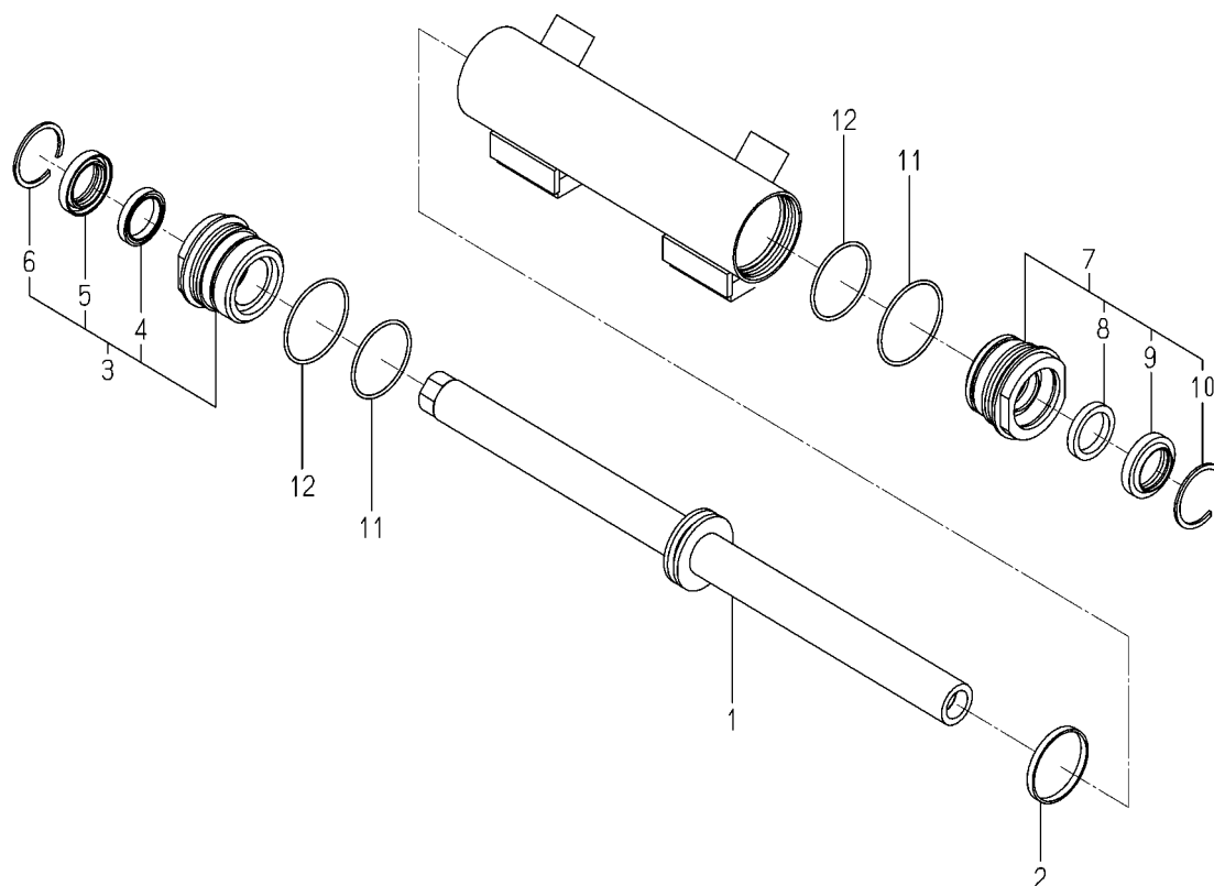
FIG.204 COMPONENT PARTS FOR 1772-407-300-10 ON Fig.77,78
