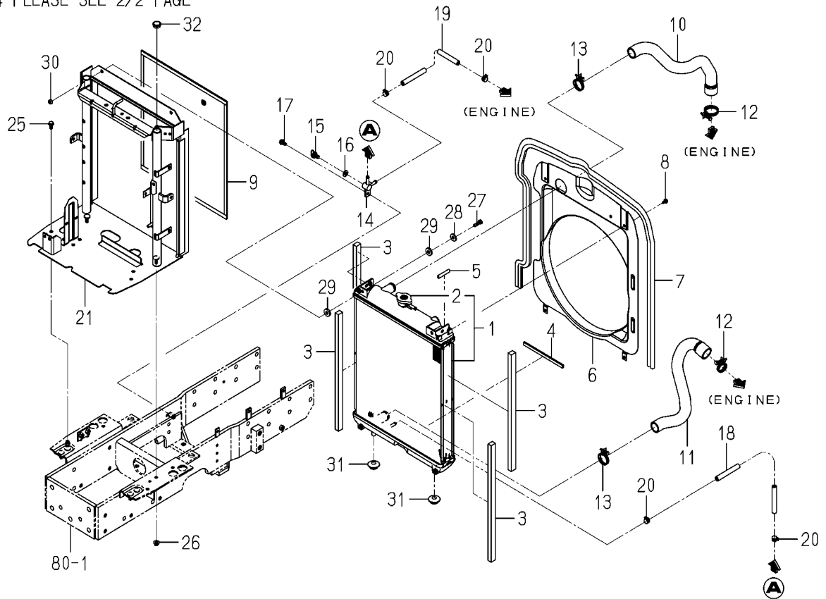
FIG. 2 RADIATOR SYSTEM(4365 TYPE)(1/2)
