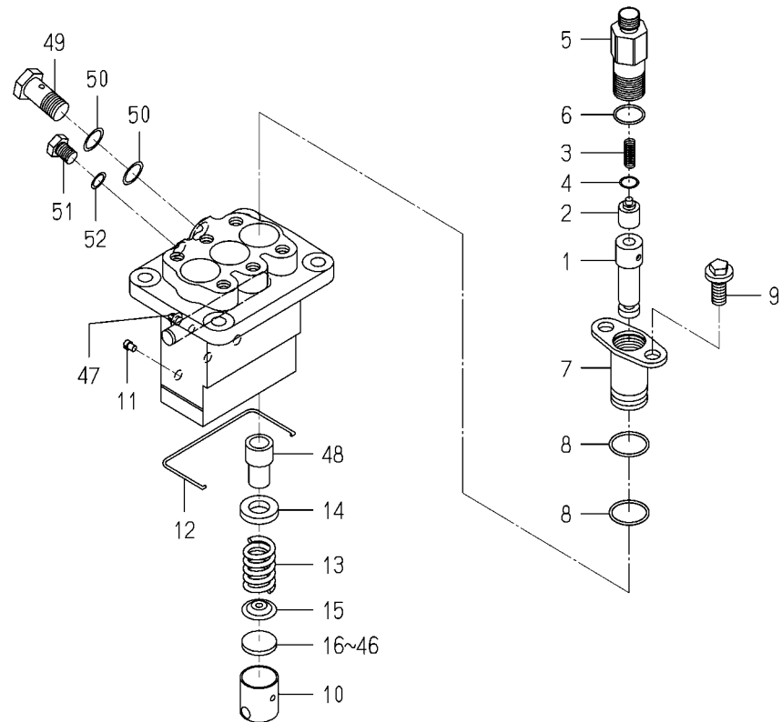
FIG. 30 COMPONENT PARTS FOR 6215-600-104-20 ON Fig.021
