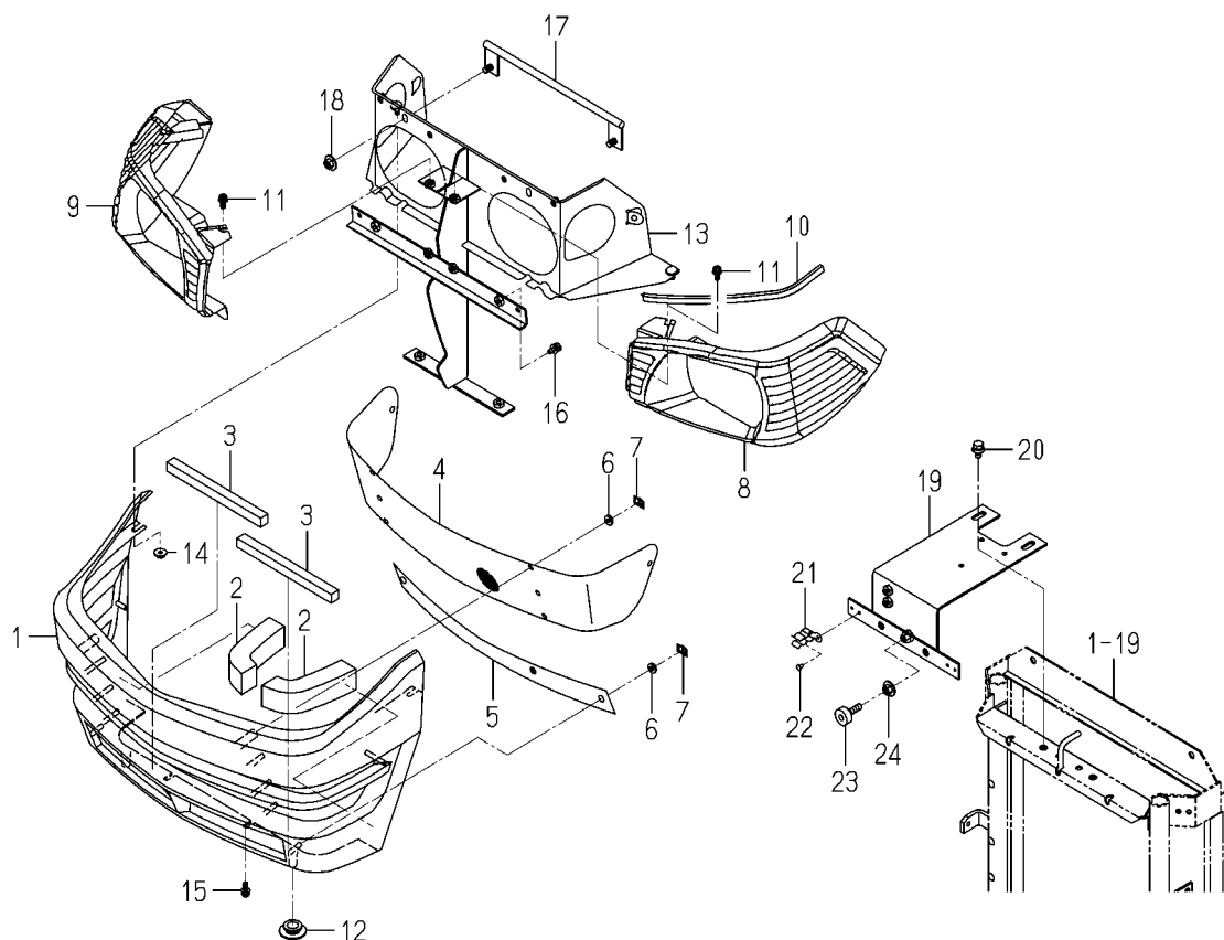
FIG.120 GRILLE SYSTEM (4295,4335 TYPE EXCEPT H)
