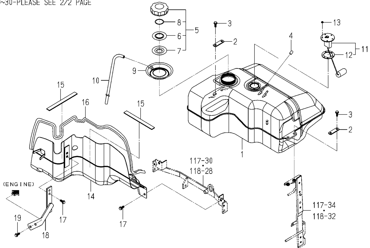
FIG. 8 FUEL SYSTEM(1/2) (4295,4335 TYPE EXCEPT H/4365 TYPE)
