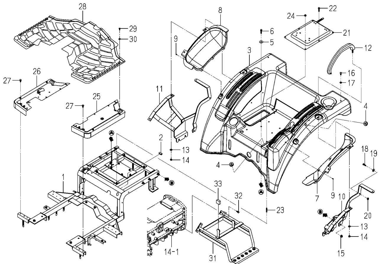
FIG.132 FLOOR(REAR)SYSTEM(4295-V TYPE)
