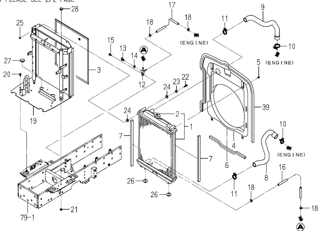
FIG. 1 RADIATOR SYSTEM(1/2) (EXCEPT H TYPE)
