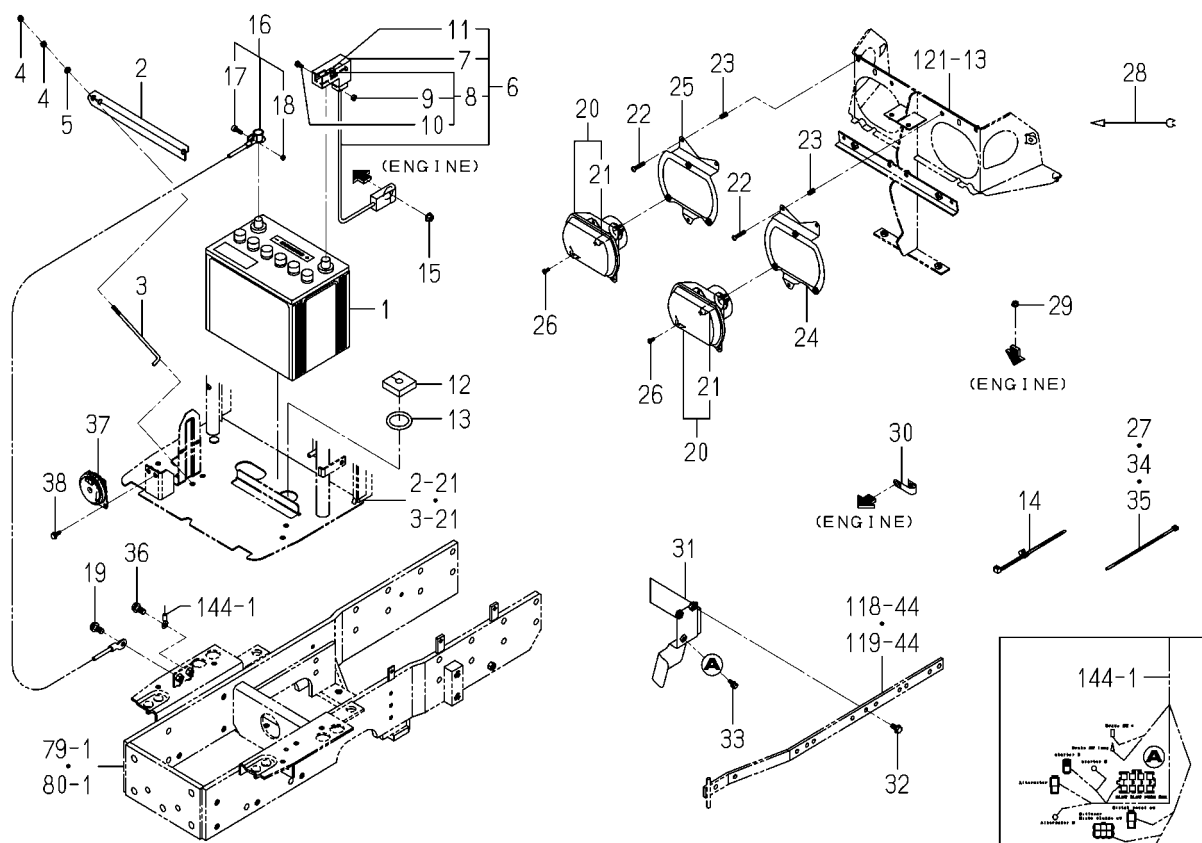
FIG.142 ELC.(FRONT)SYSTEM (H TYPE EXCEPT G)
