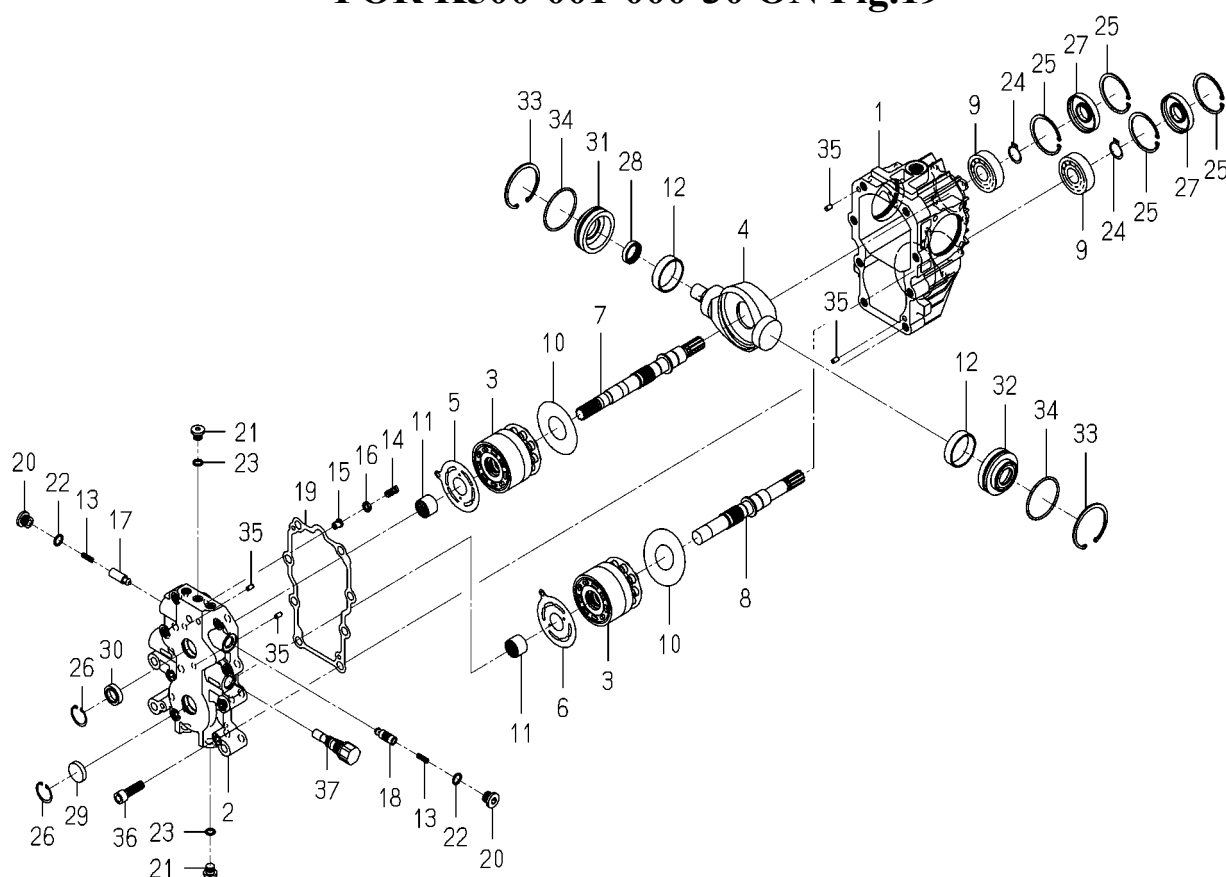
FIG.199 COMPONENT PARTS FOR K500-001-000-30 ON Fig.19
