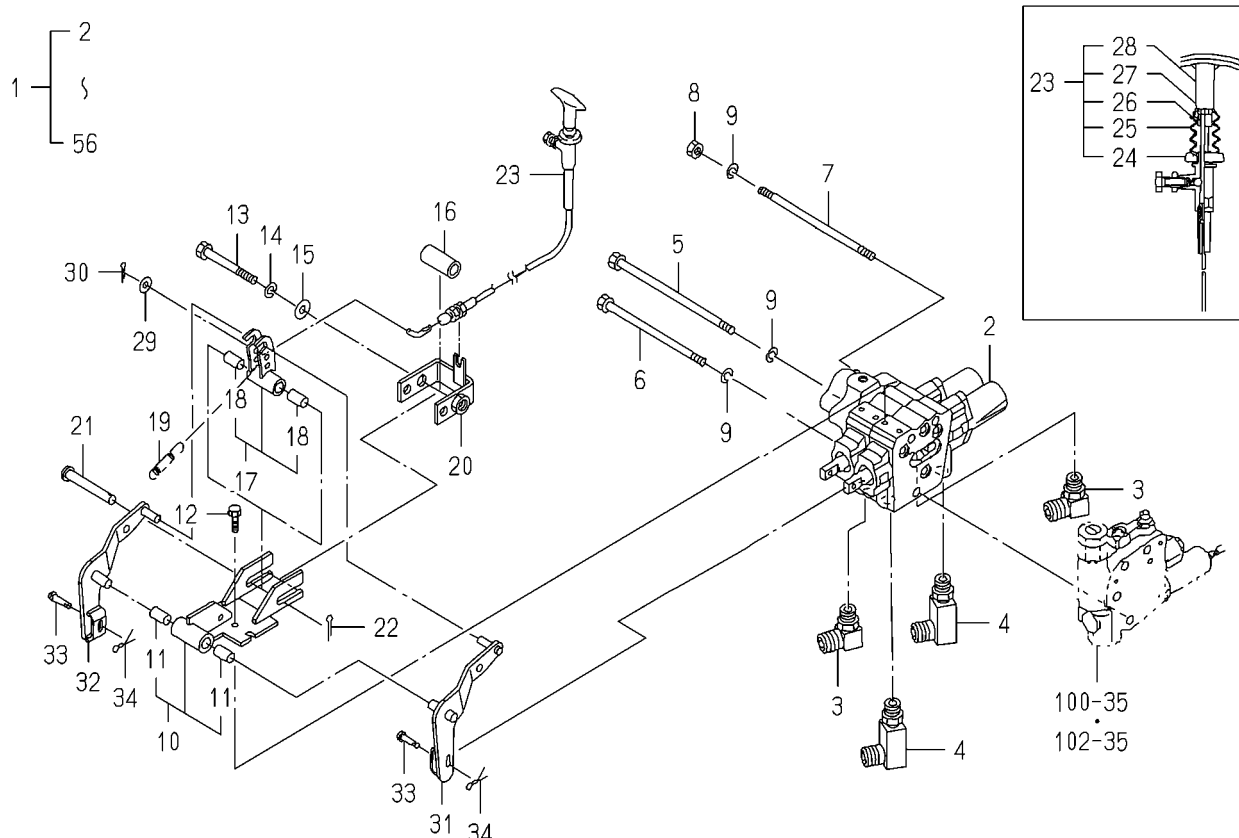
FIG.188 JOY STICK(E4)SET(1/2) (EXCEPT H TYPE)(OPTION)
