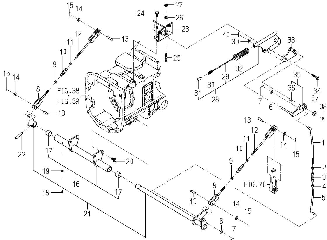
FIG. 73 LEVER(BRAKE/PARKING)SYSTEM (H TYPE)
