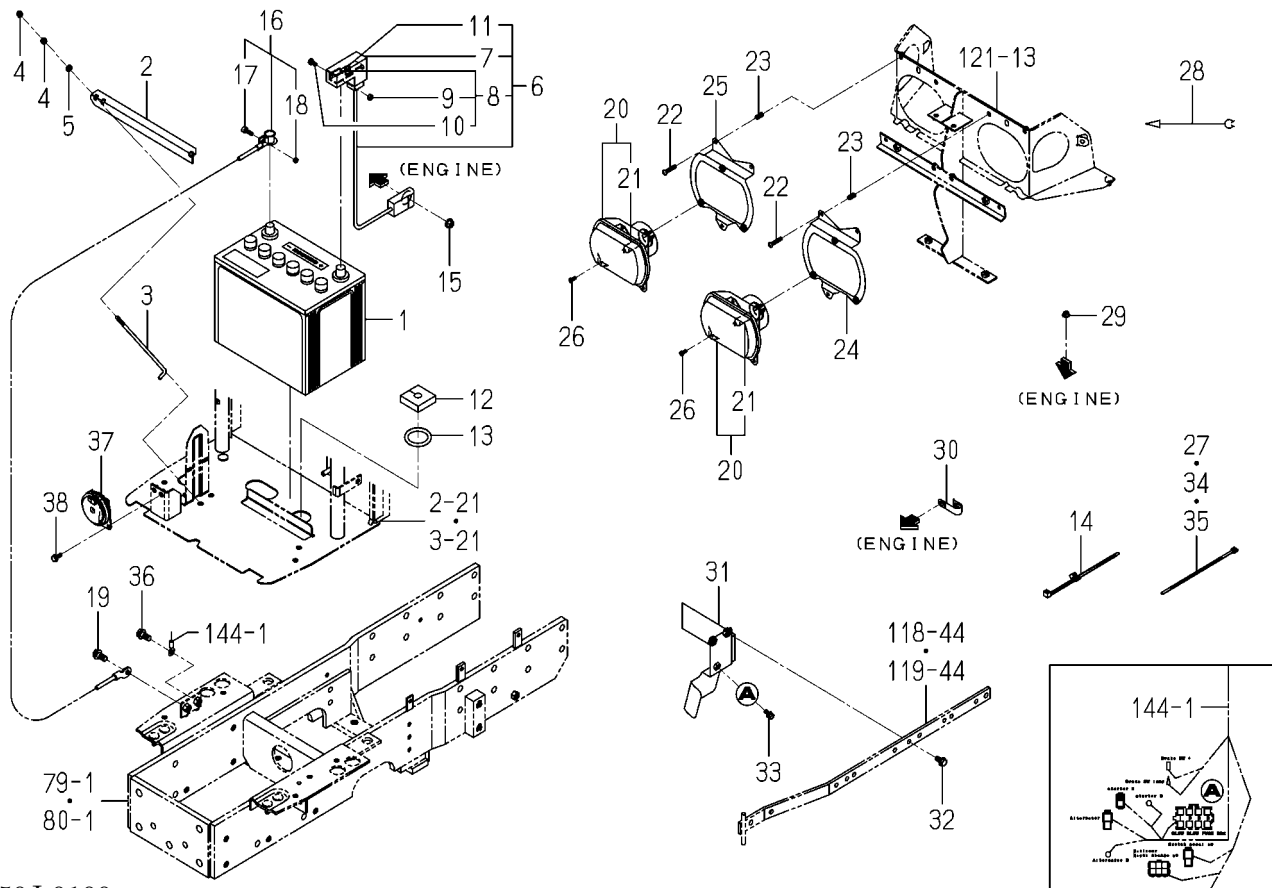
FIG.143 ELC.(FRONT)SYSTEM(HG TYPE)
