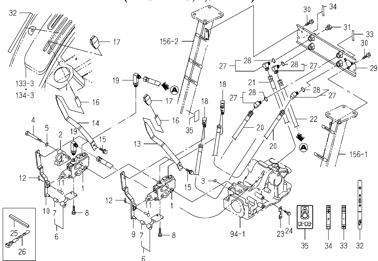
FIG.109 VALVE(REMOTE/2R)SYSTEM (EXCEPT C,V,J TYPE)
