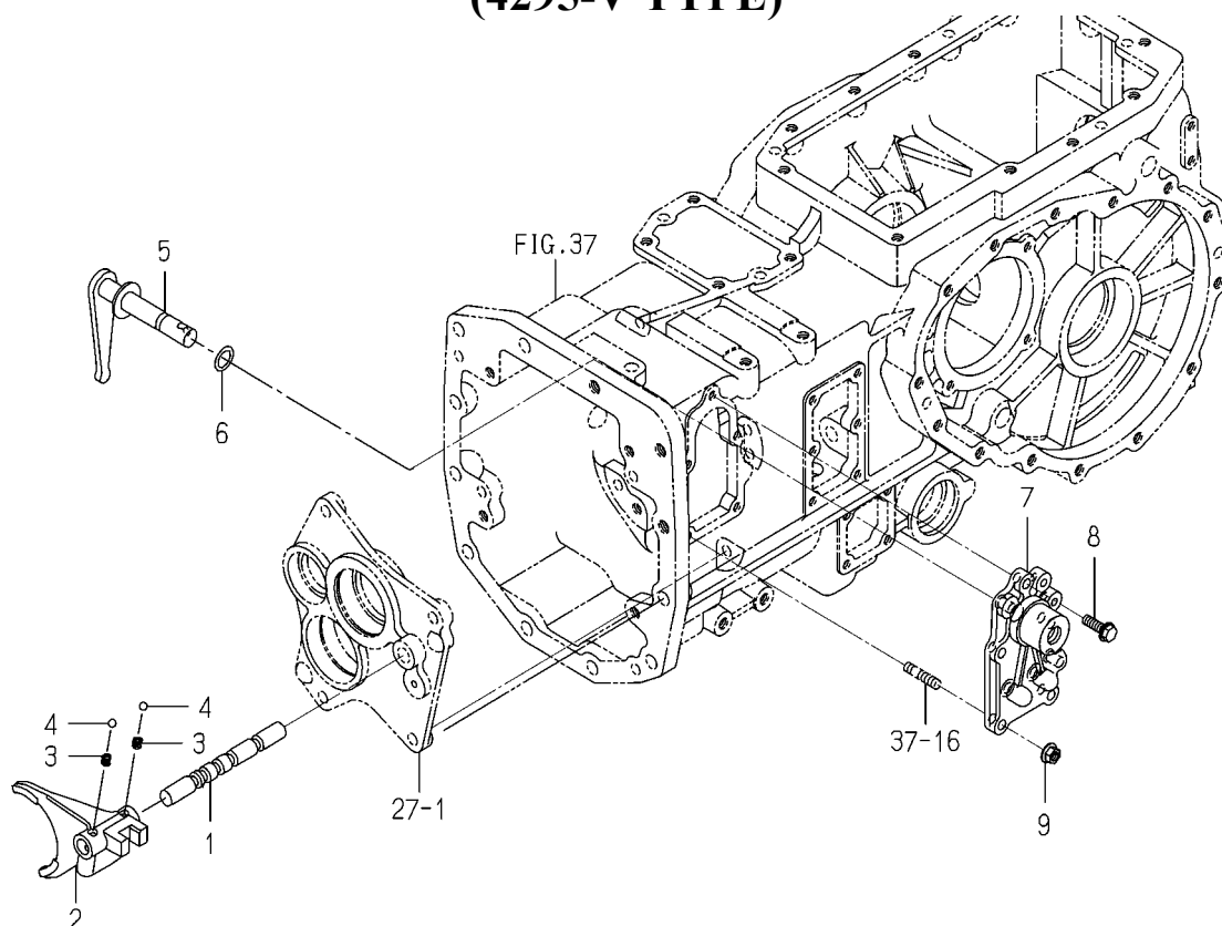
FIG. 43 FORK(SHIFT/MAIN)SYSTEM (4295-V TYPE)
