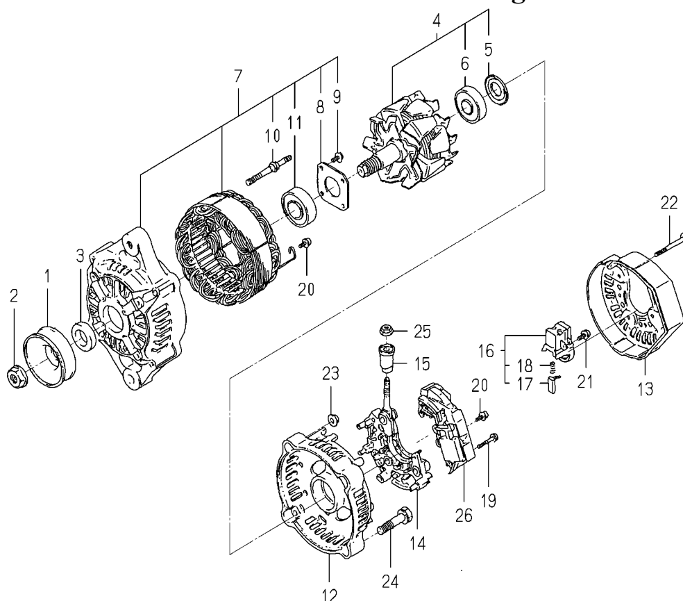
FIG. 33 COMPONENT PARTS FOR 6281-200-020-00 ON Fig.024
