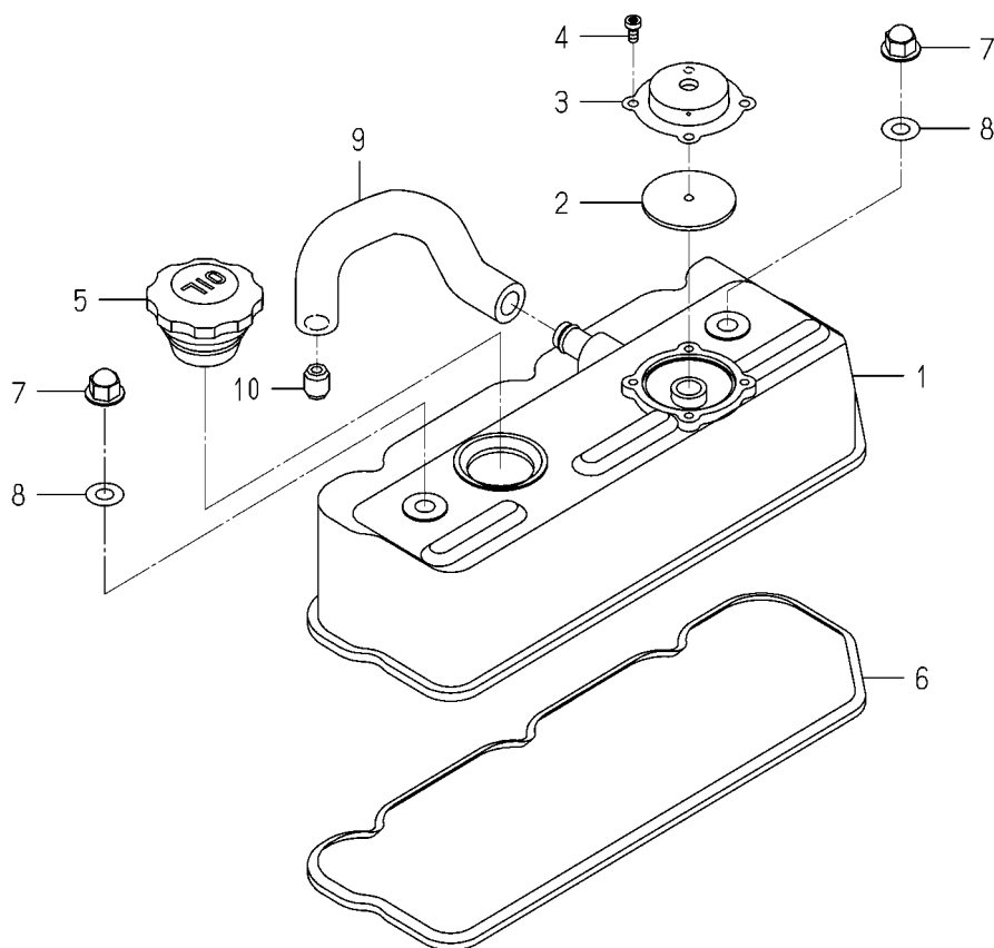
FIG. 3 CYLINDER HEAD COVER
