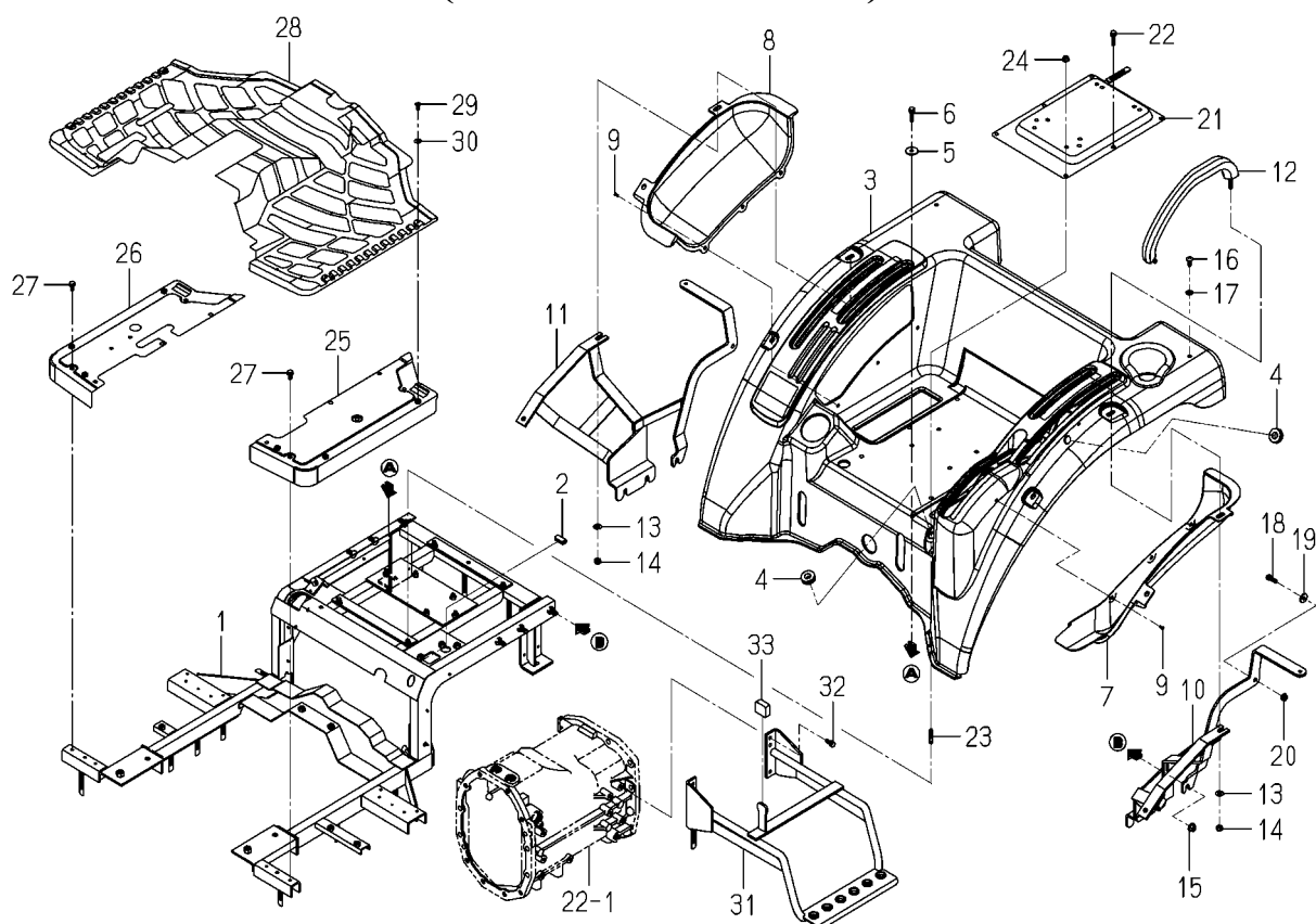
FIG.134 FLOOR(REAR)SYSTEM (H TYPE EXCEPT C)
