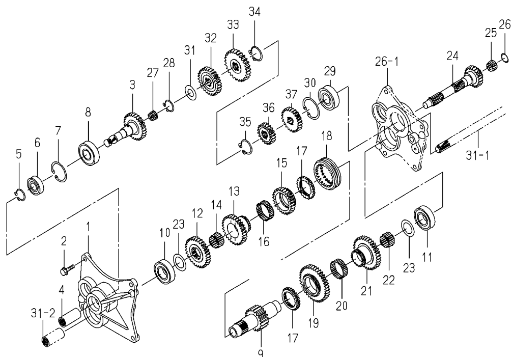
FIG. 23 GEAR(MAIN)SYSTEM (4295 TYPE EXCEPT H,V/ 4335 TYPE EXCEPT H)
