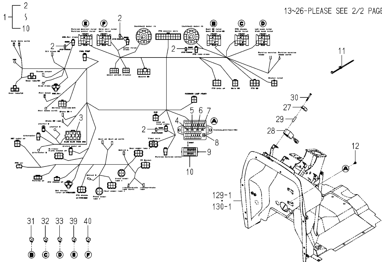
FIG.145 ELC.(MAIN)SYSTEM(V,JA TYPE)(1/2)
