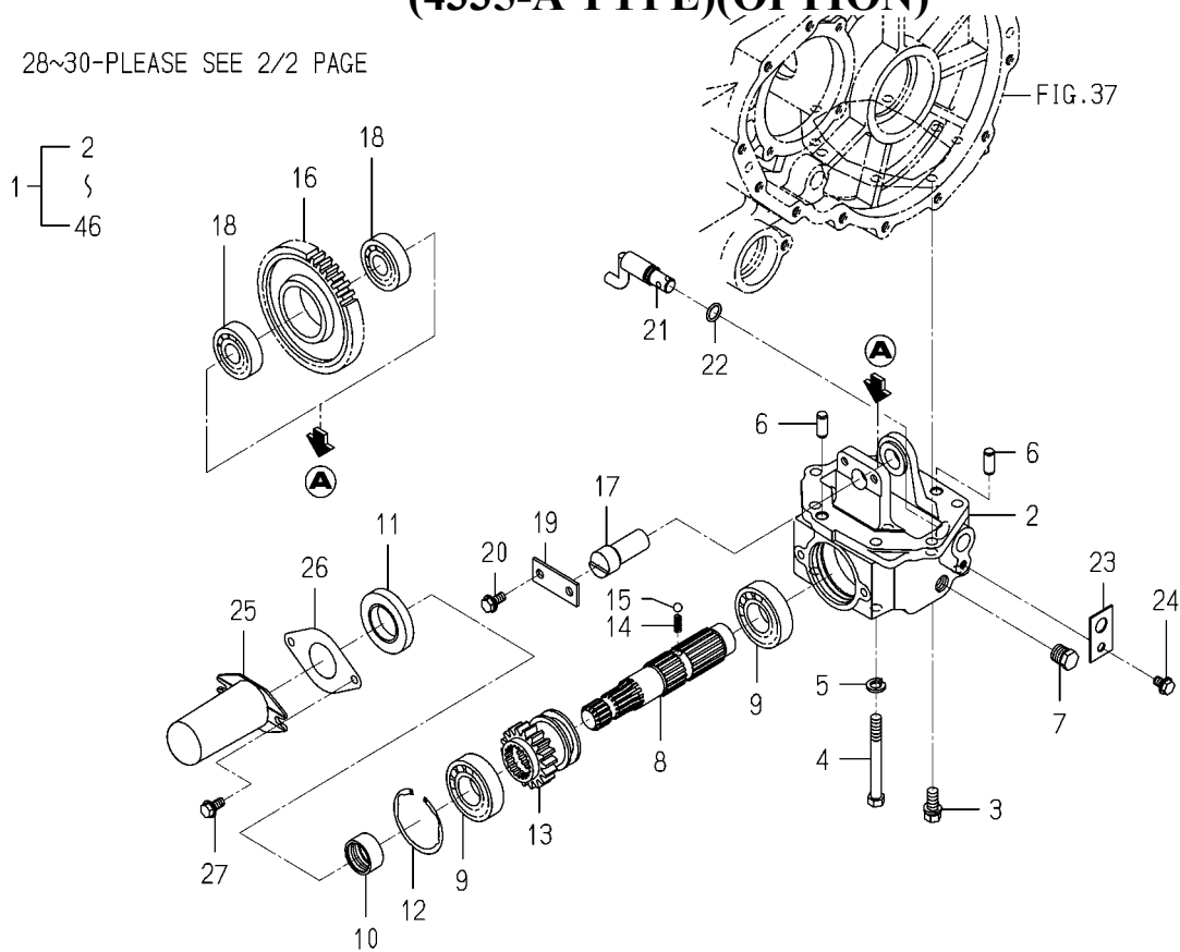
FIG.176 PTO(MID)SET(1/2) (4335-A TYPE)(OPTION)
