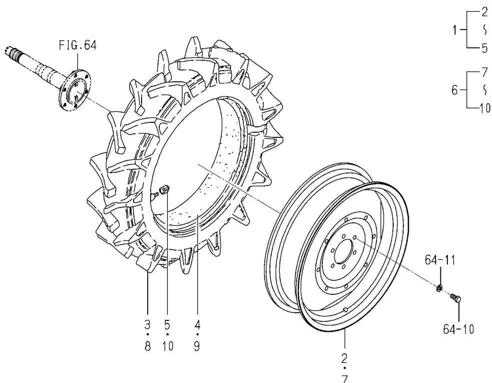
FIG.180 WHEEL(REAR/AGR/11.2-24)SYSTEM (V,J TYPE)(OPTION)
