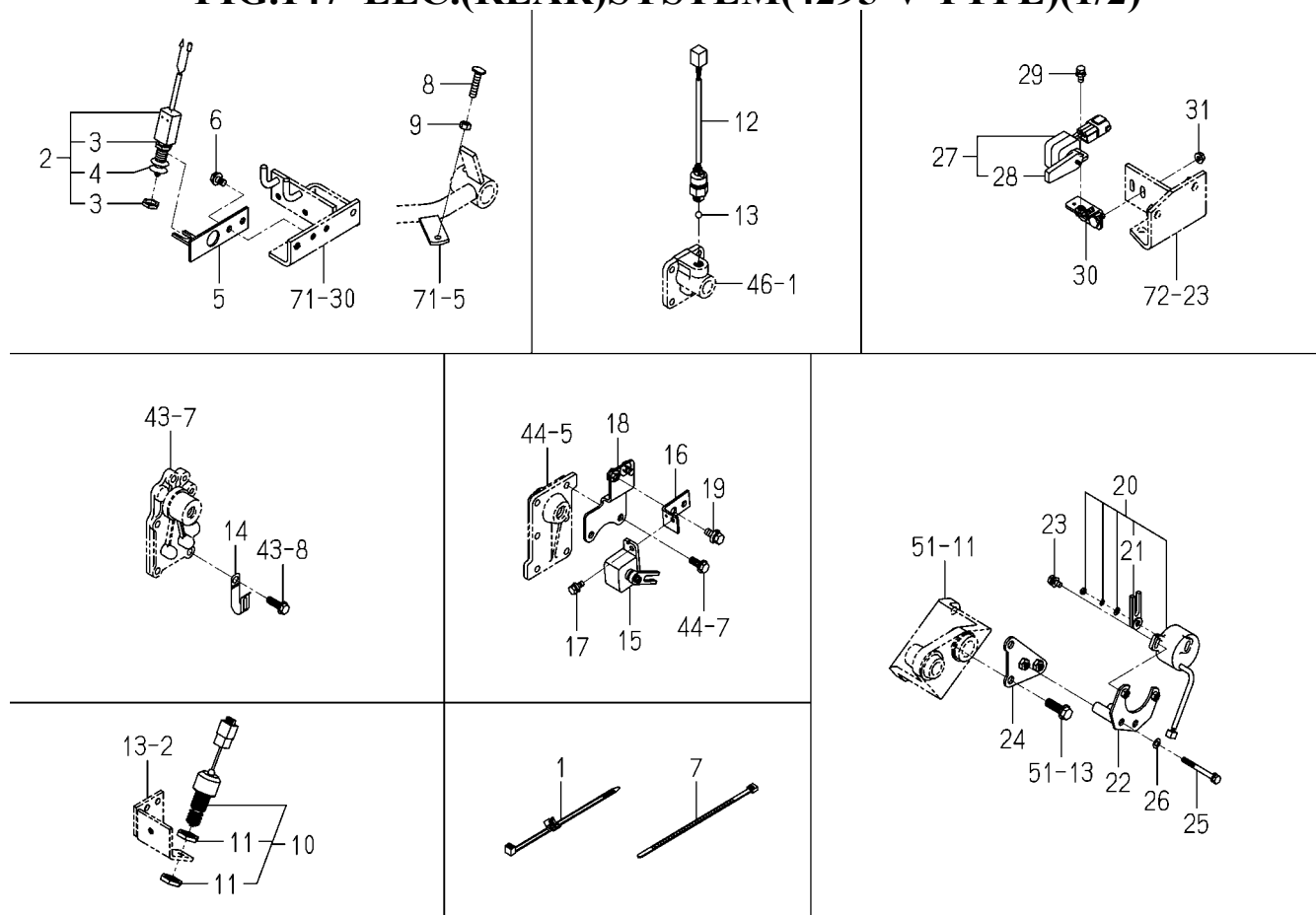
FIG.147 ELC.(REAR)SYSTEM(4295-V TYPE)(1/2)
