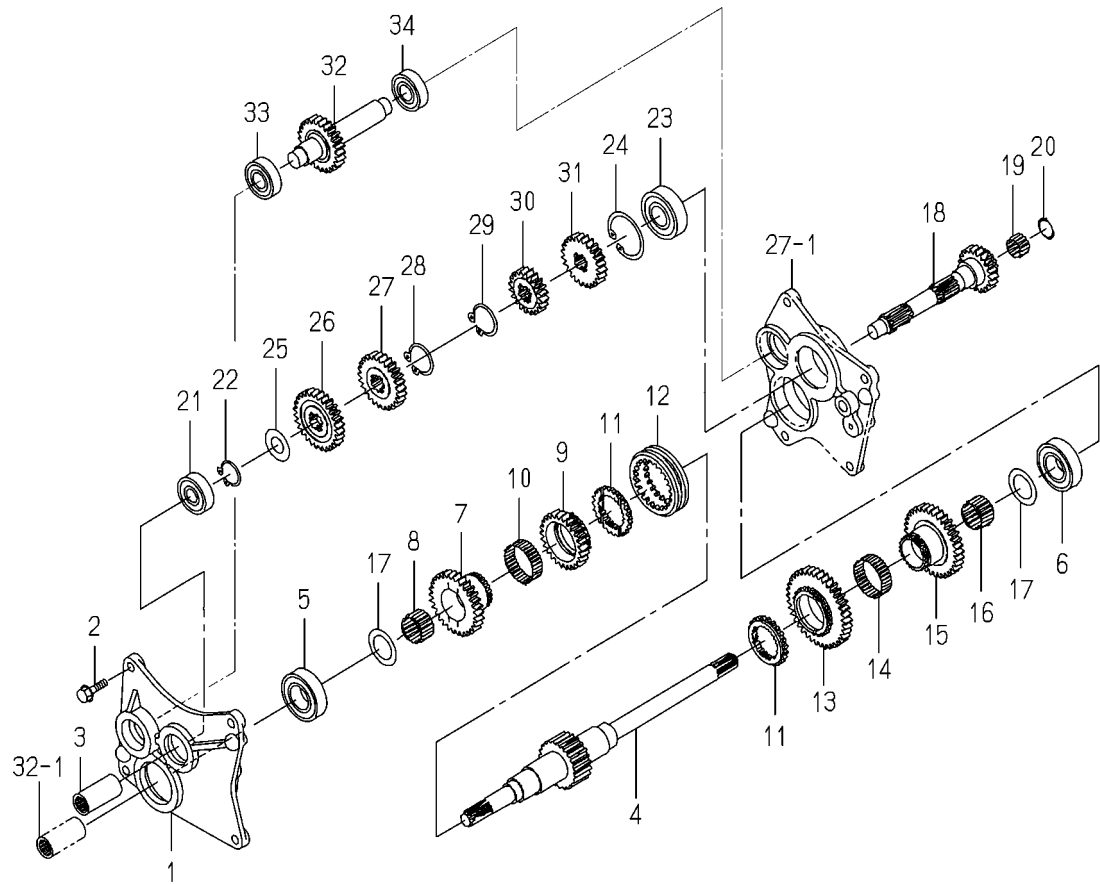
FIG. 24 GEAR(MAIN)SYSTEM(4295-V TYPE)
