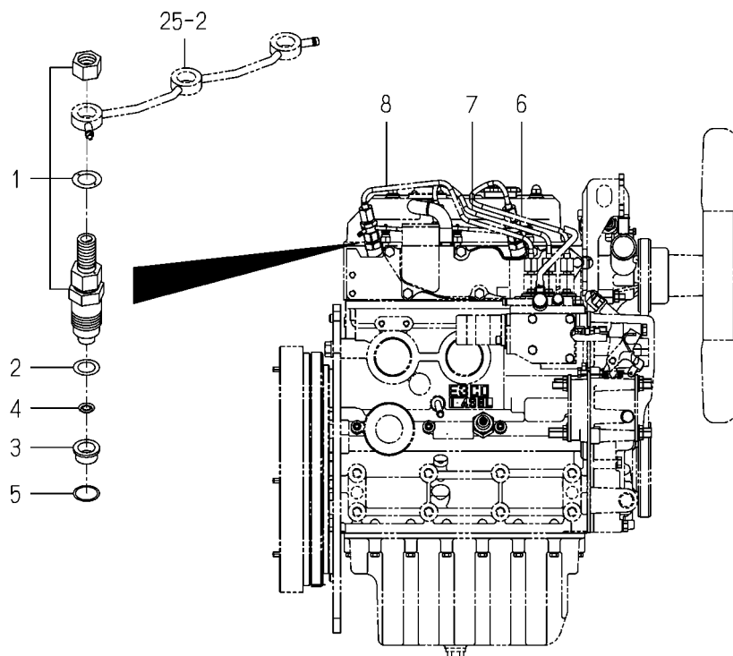
FIG. 23 INJECTION NOZZLE
