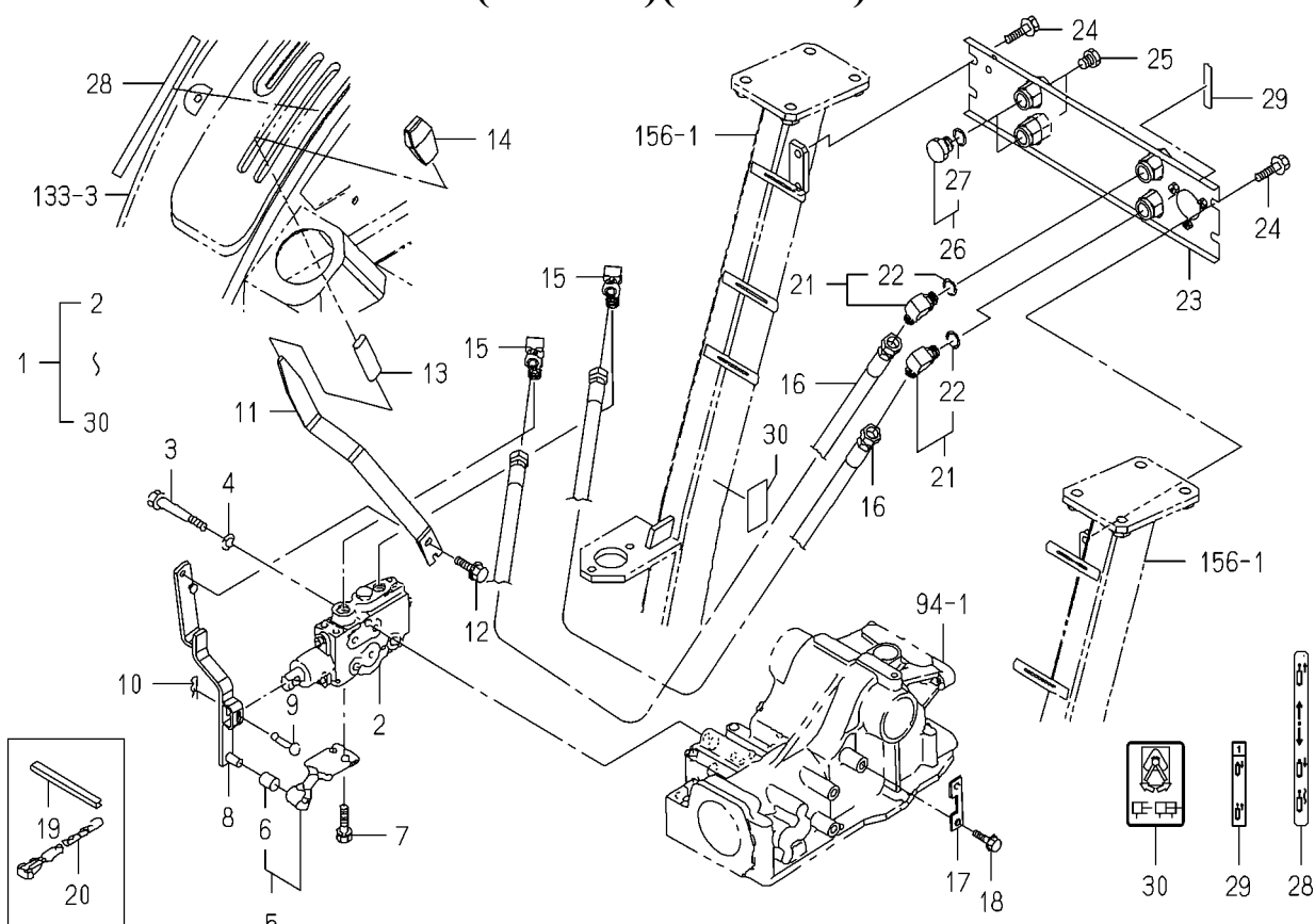
FIG.191 VALVE(REMOTE/1ST)SET (J TYPE)(OPTION)
