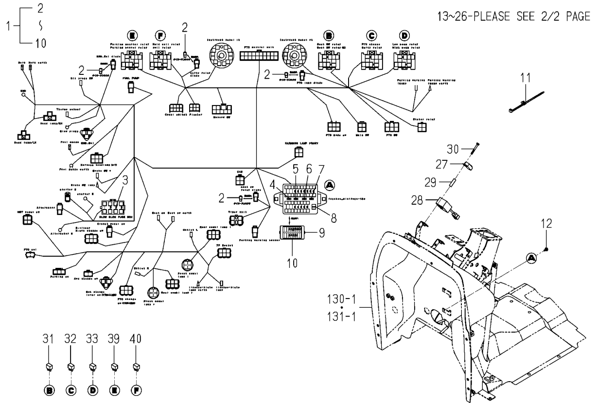
FIG.144 ELC.(MAIN)SYSTEM(1/2) (EXCEPT V,JA TYPE)
