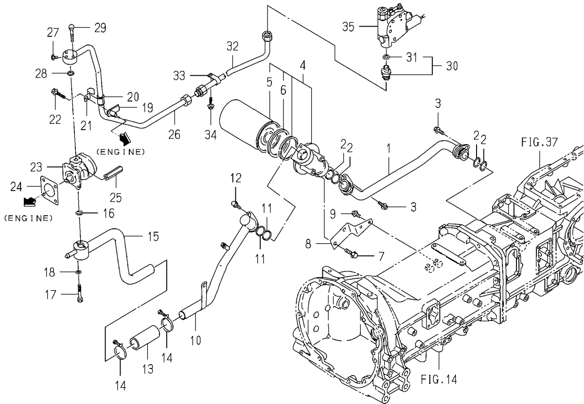
FIG.100 PIPING(MAIN)SYSTEM(1/2) (4295-V TYPE)
