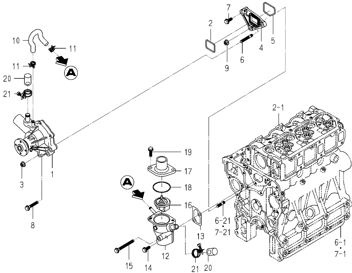
FIG. 21 WATER PUMP
