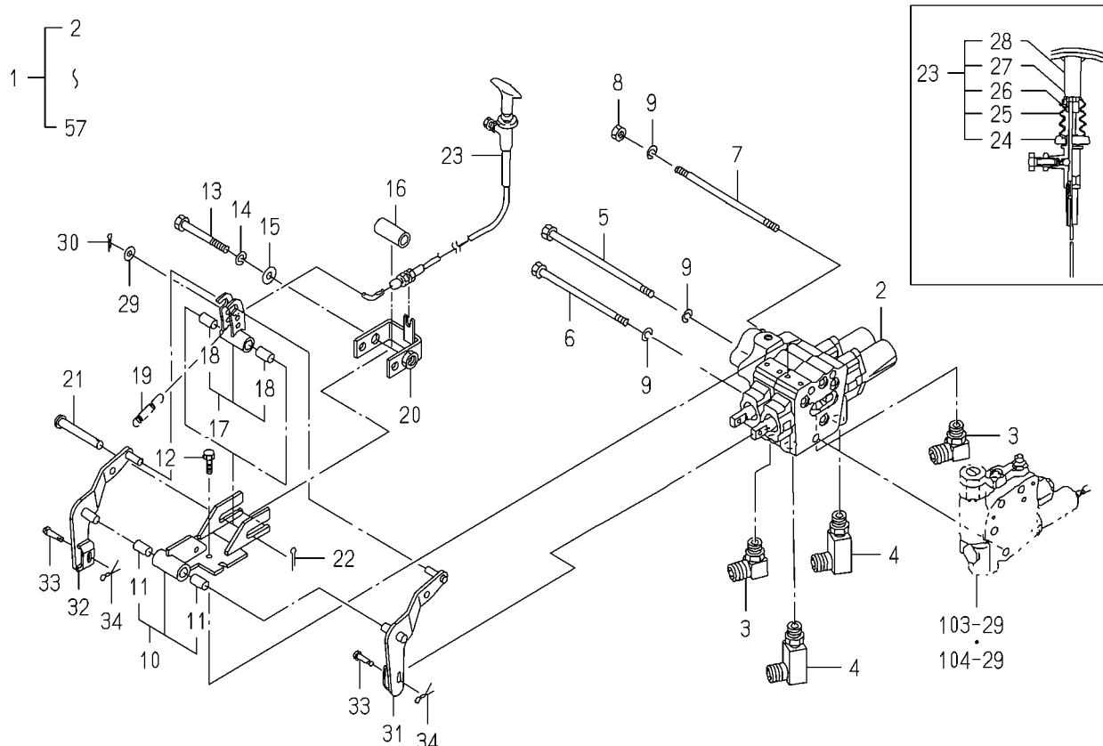
FIG.189 JOY STICK(H/E4)SET(1/2) (H TYPE EXCEPT C)(OPTION)
