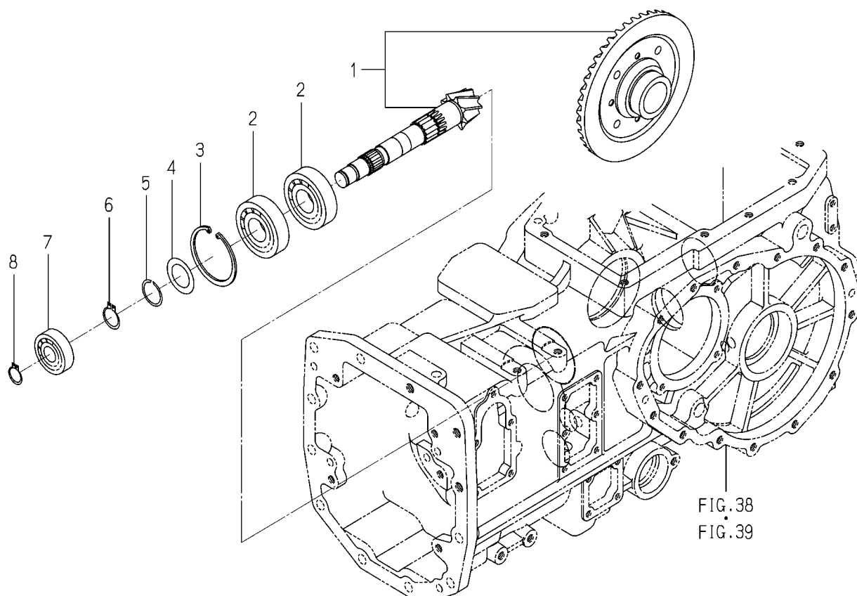
FIG. 60 PINION(DRIVE/REAR)SYSTEM(H TYPE)
