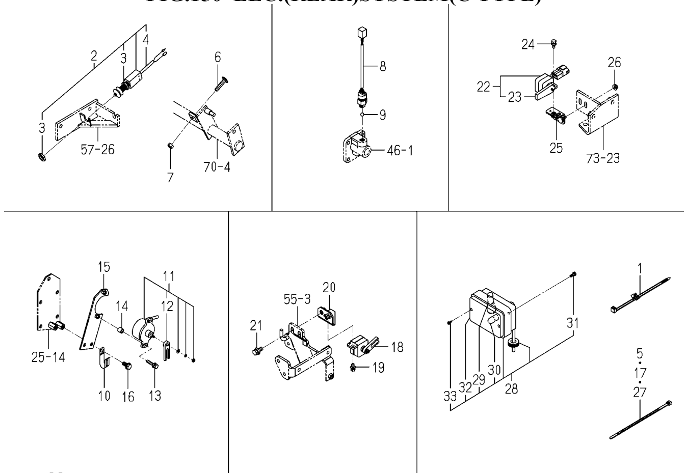
FIG.150 ELC.(REAR)SYSTEM(C TYPE)
