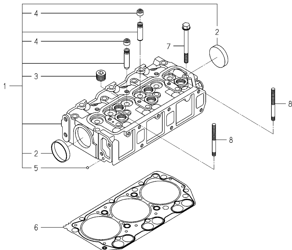
FIG. 2 CYLINDER HEAD
