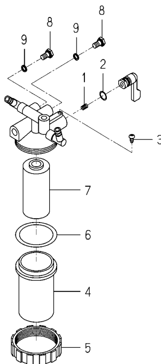
FIG.201 COMPONENT PARTS FOR 1672-105-210-00 ON Fig.7,8
