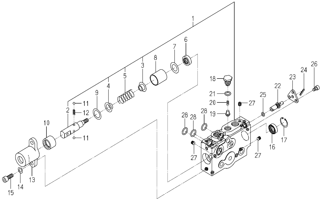
FIG.200 COMPONENT PARTS FOR 1640-530-600-10 ON Fig.2
