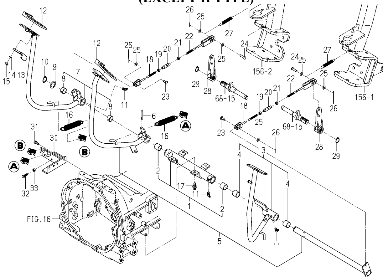
FIG. 71 PEDAL(BRAKE)SYSTEM (EXCEPT H TYPE)
