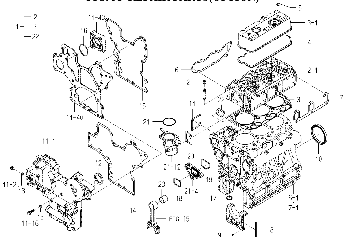
FIG. 31 REPAIR PARTS(OPTION)
