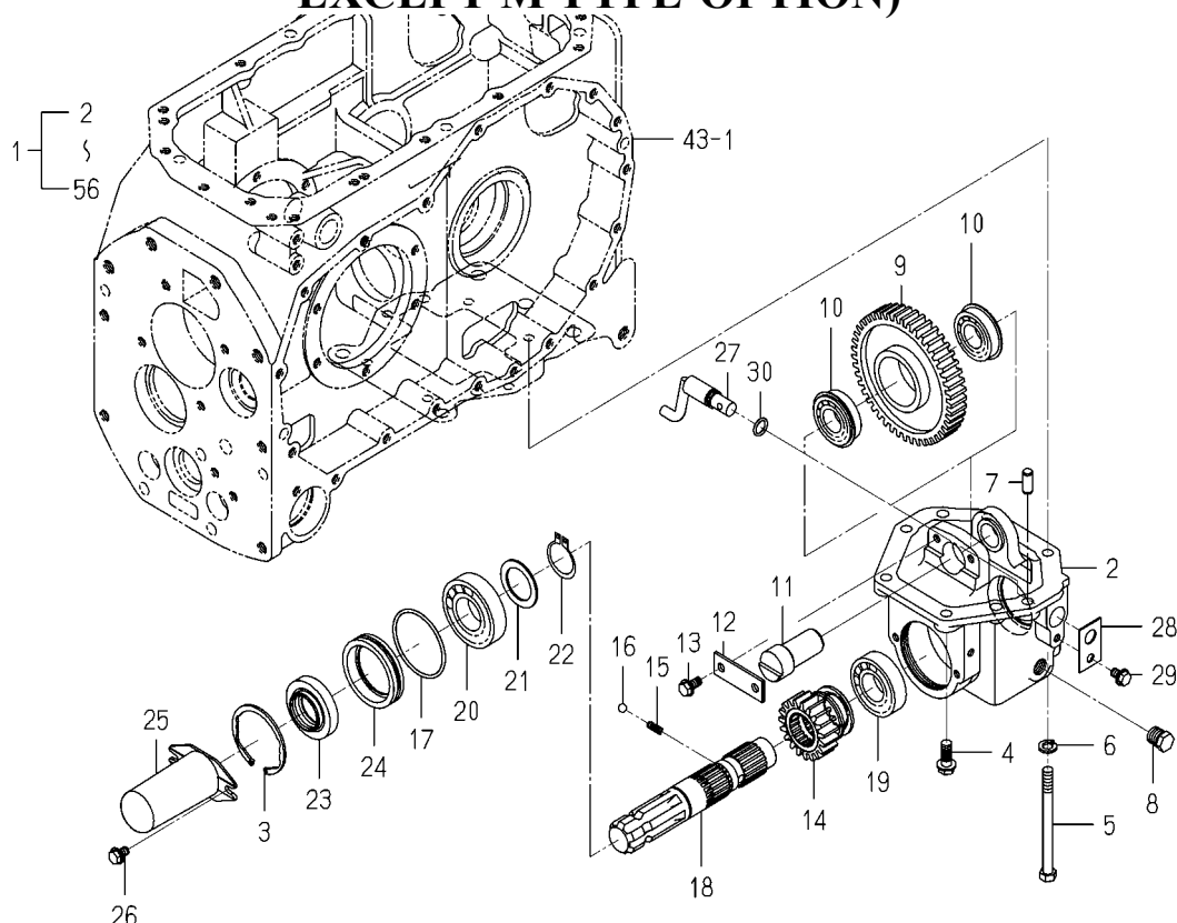
FIG. 40 PTO(MID)SYSTEM(1/2) (6675-M TYPE-STANDARD/ EXCEPT M TYPE-OPTION)
