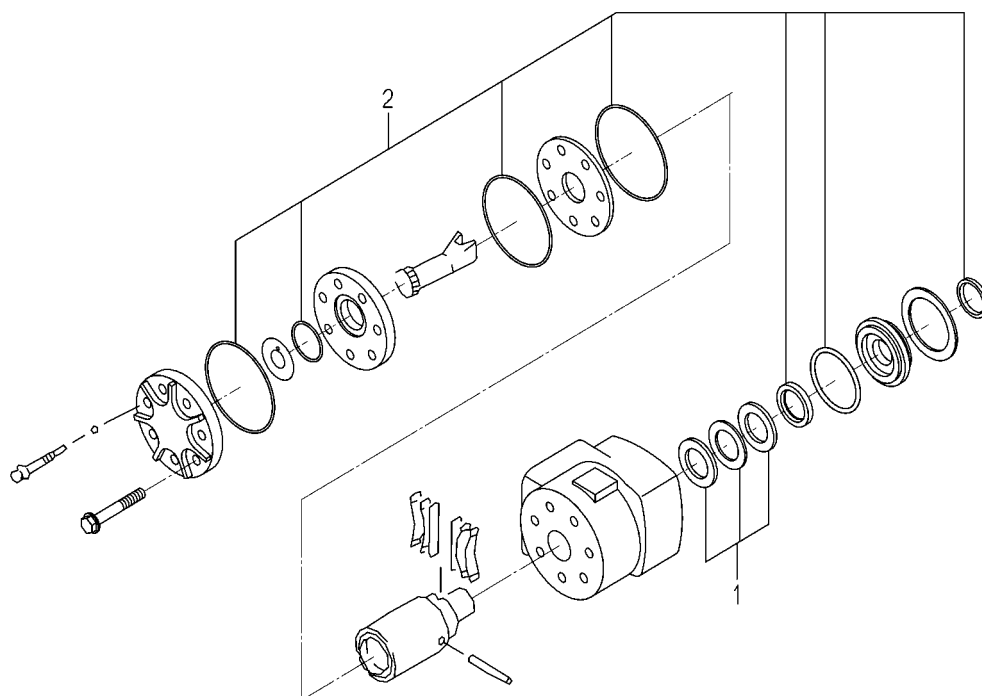
FIG.197 COMPONENT PARTS FOR 1646-407-670-20 ON FIG.80,81
