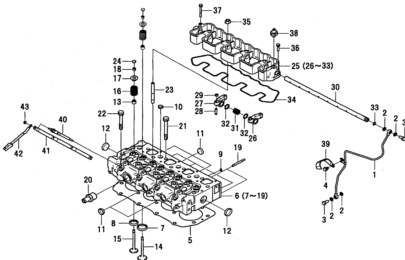
FIG.004 CYLINDER HEAD/ROCKER ARM
