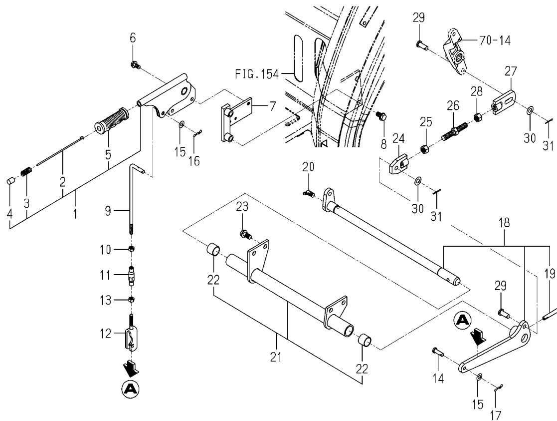
FIG. 76 LEVER(BRAKE/PARKING)SYSTEM (6675H,6625H TYPE)
