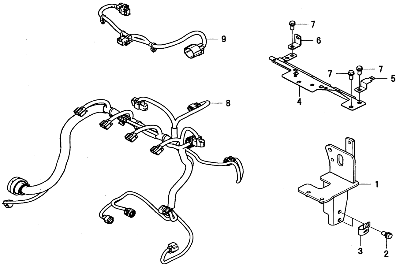
FIG.013 HARNESS WIRE
