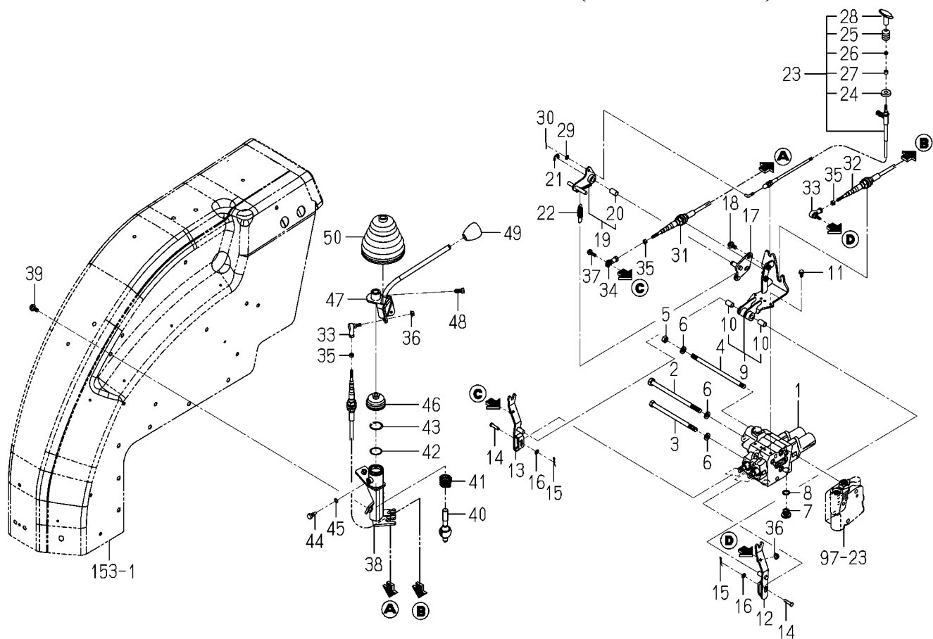
FIG.104 JOY STICK SYSTEM(6675-D TYPE)
