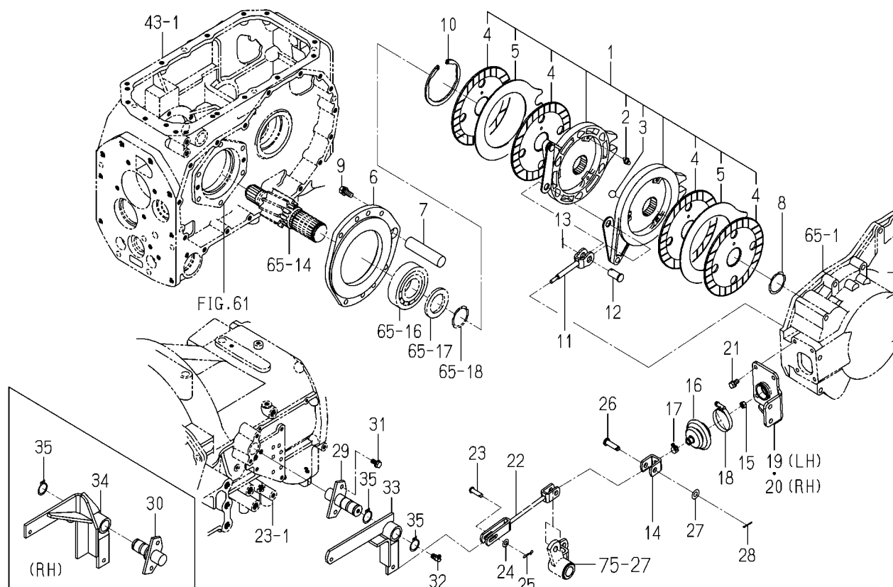
FIG. 71 LEVER(BRAKE/PARKING)SYSTEM (6675 TYPE)
