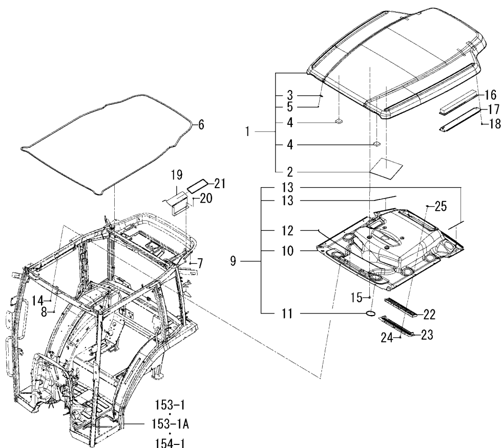
FIG.151 ROOF(CABIN)SYSTEM(M TYPE)
