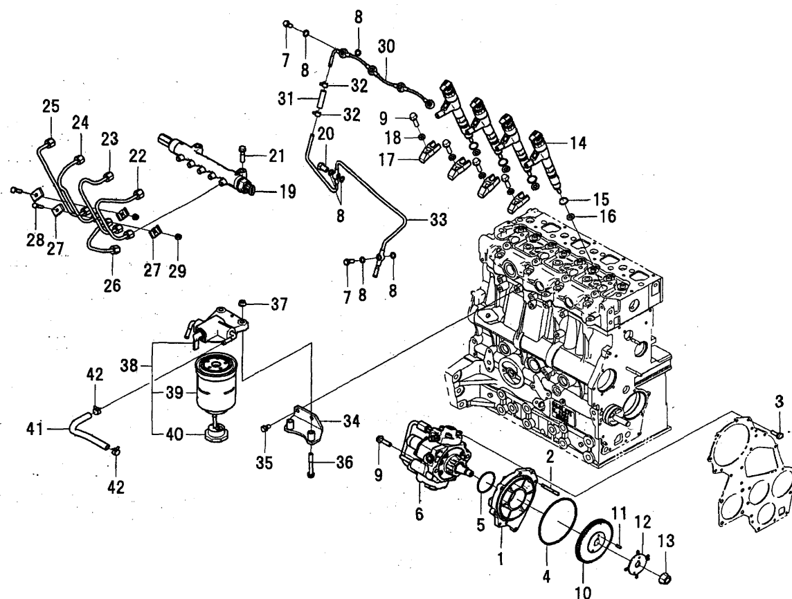
FIG.009 INJECTOR/HP PUMP/FUEL FILTER
