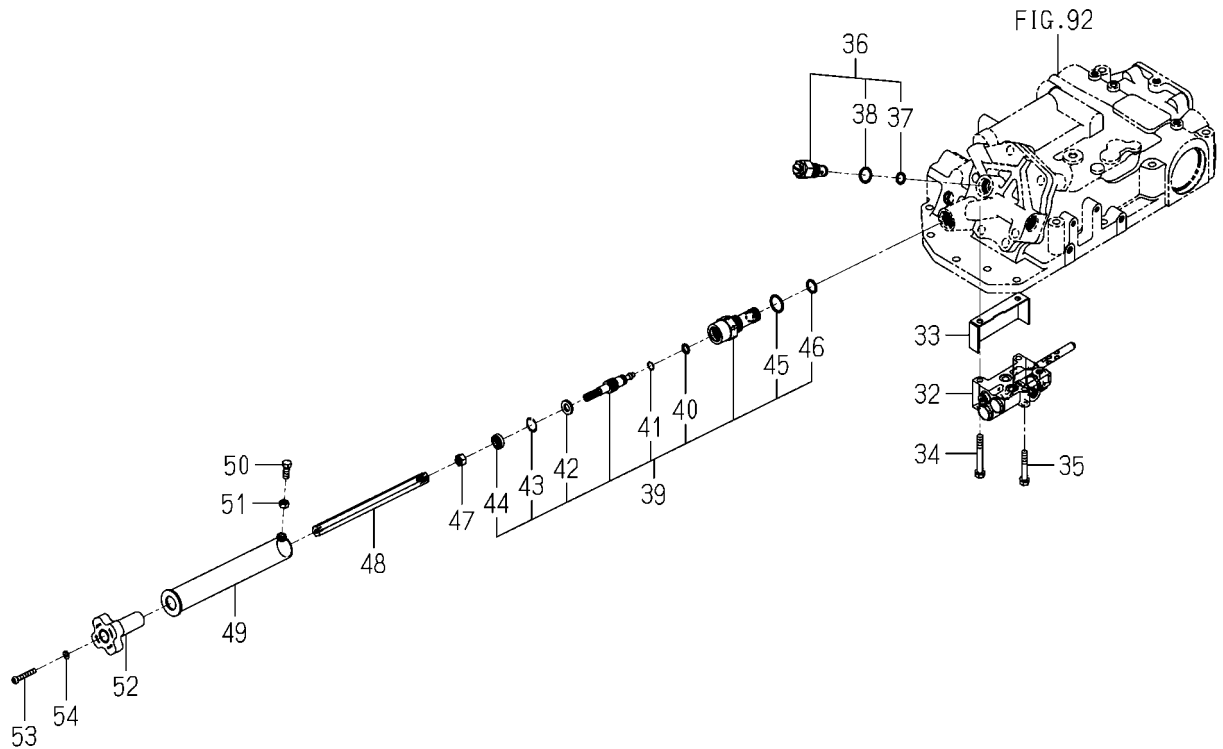
FIG. 97 PIPING(MAIN)SYSTEM(6675 TYPE)(2/2)
