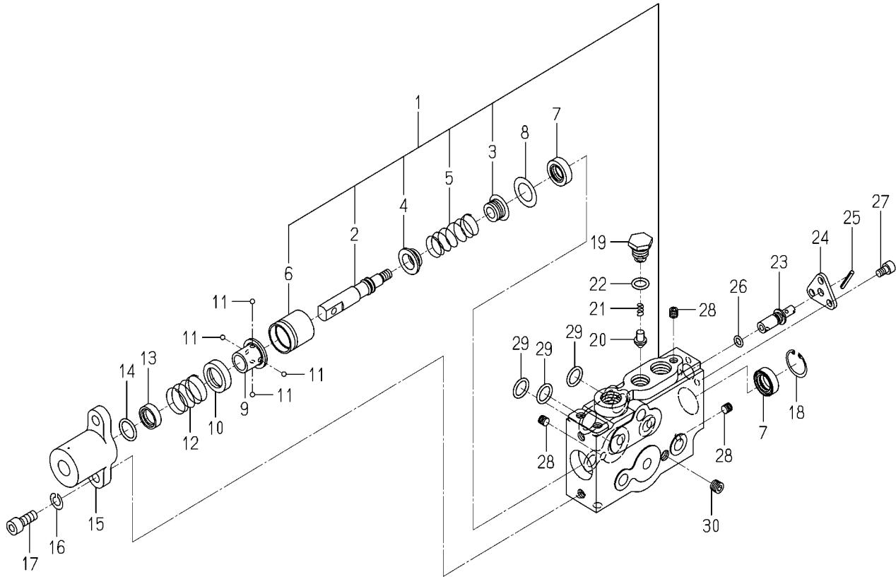
FIG.202 COMPONENT PARTS FOR 1801-512-300-10 ON FIG.107,108
