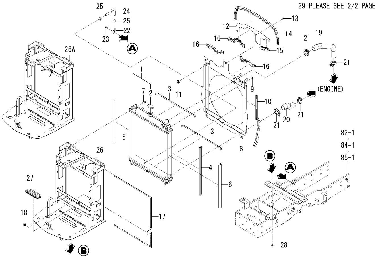
FIG. 4 RADIATOR SYSTEM(1/2)
