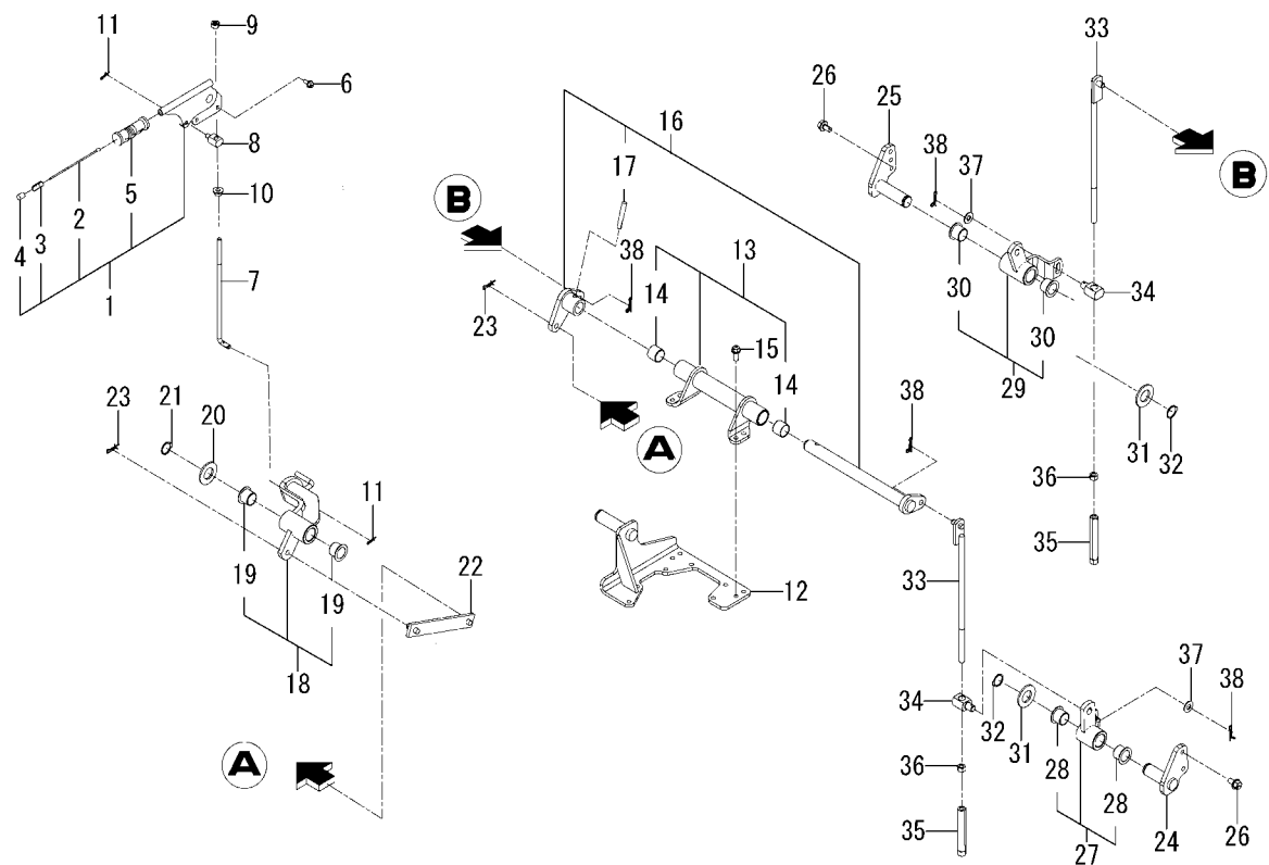
FIG. 75 LEVER(BRAKE/PARKING)SYSTEM (6675 TYPE)
