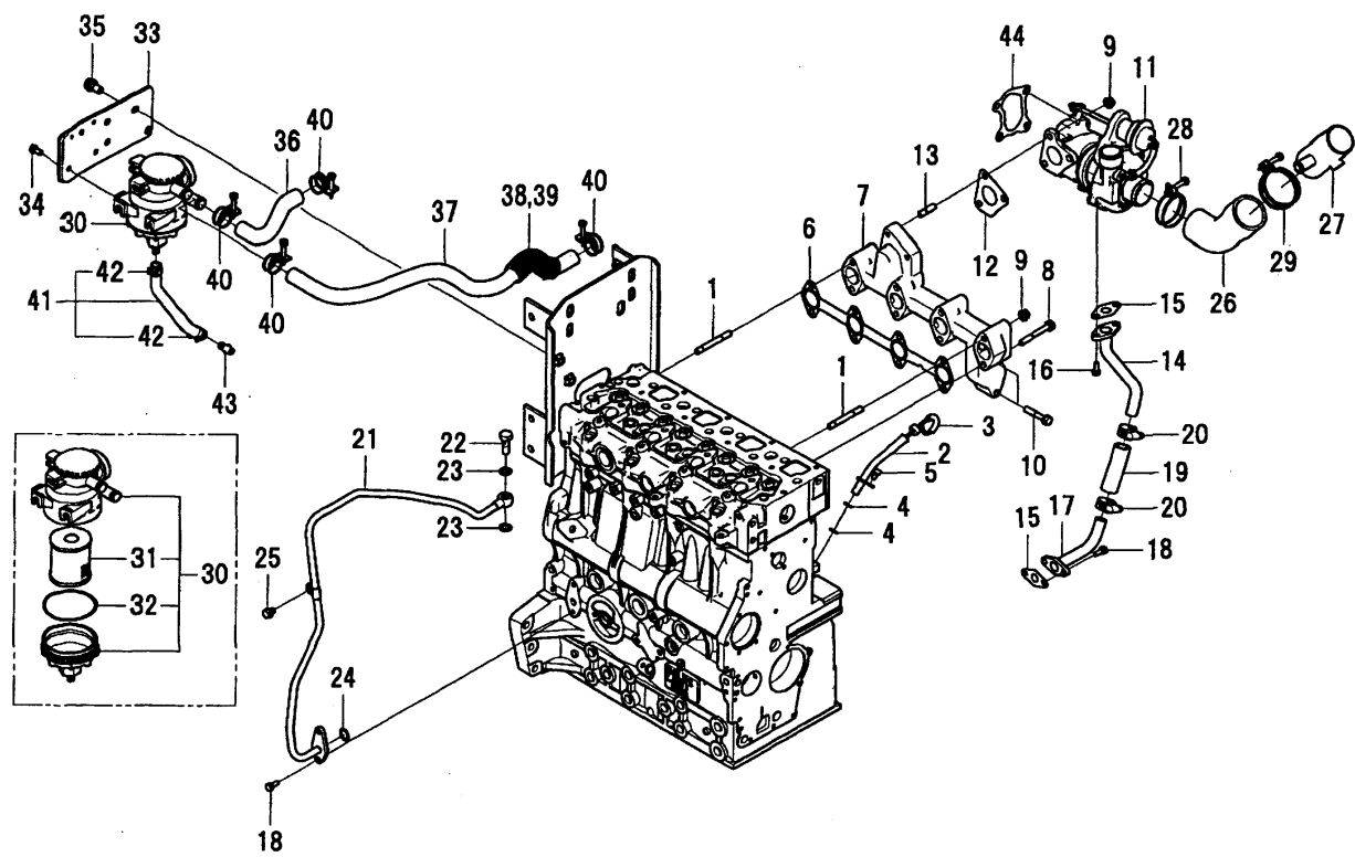
FIG.006 EXHAUST MANIFOLD/ TURBO CHARGER/OMS
