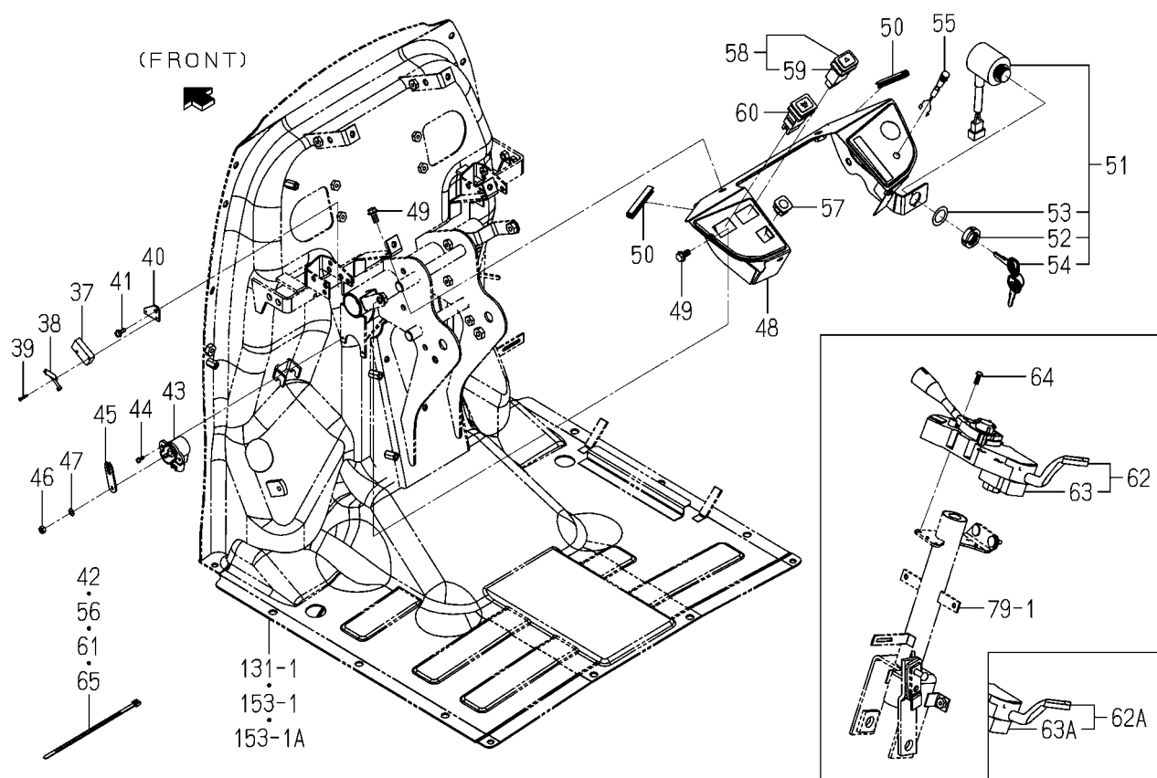
FIG.138 ELC.(MAIN)SYSTEM(6675 TYPE)(2/2)
