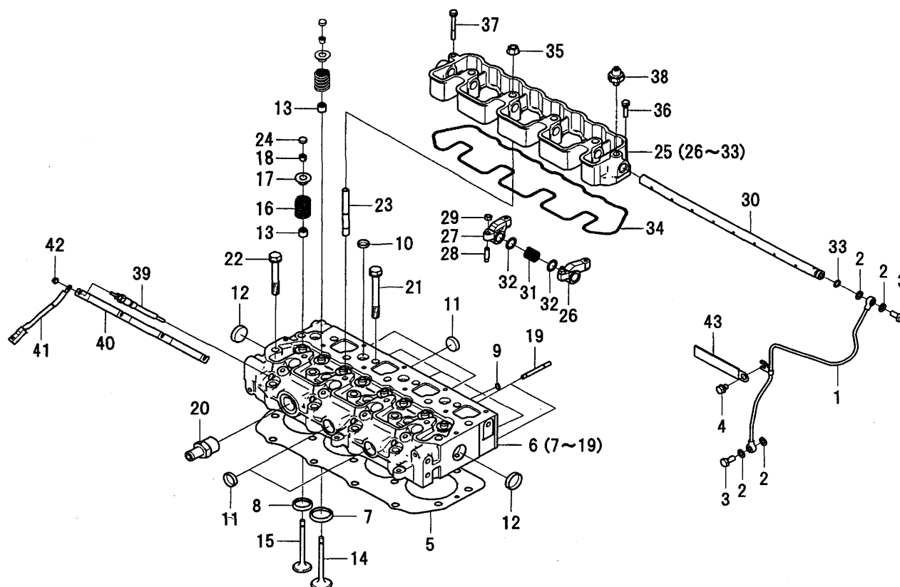
FIG.004 CYLINDER HEAD/ROCKER ARM
