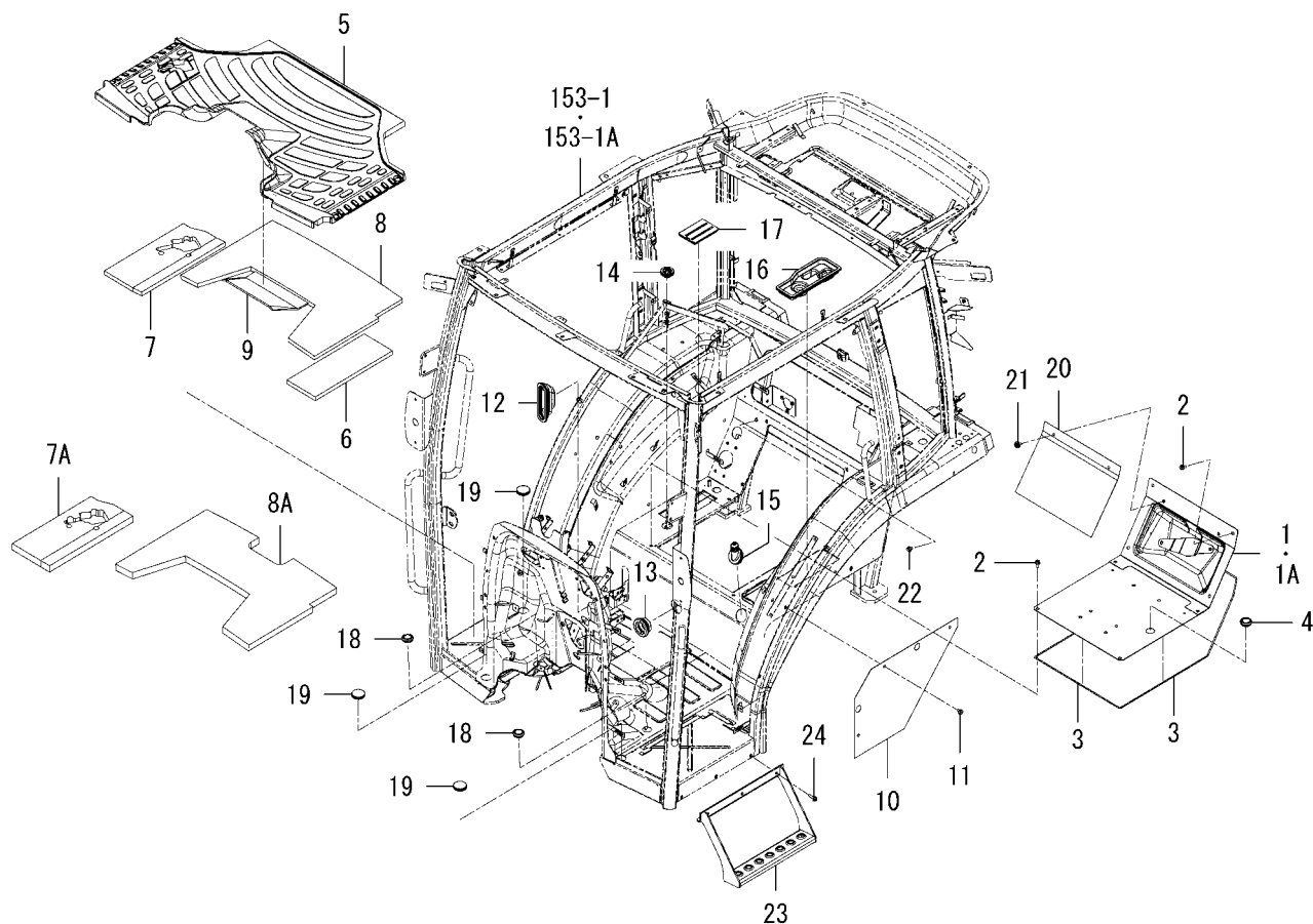
FIG.134 FLOOR(REAR)SYSTEM(6675-M TYPE)
