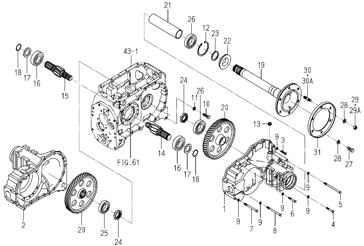
FIG. 65 HOUSING(AXLE/REAR)SYSTEM (6675 TYPE)
