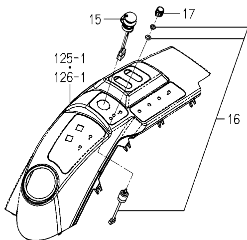
FIG.145 CONTROL SYSTEM(6675 TYPE)
