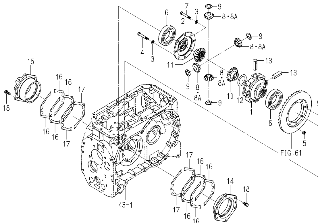
FIG. 63 CASE(DIFFERENTIAL/REAR)SYSTEM (6675 TYPE)
