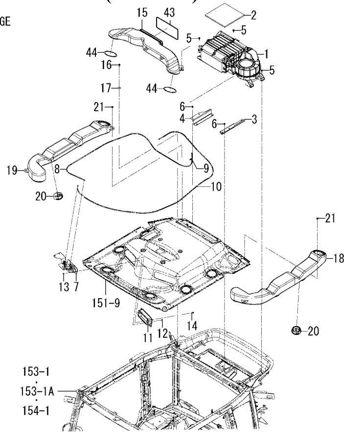
FIG.162 AIR CONDITIONER(CABIN)SYSTEM(1/2) (M TYPE)
