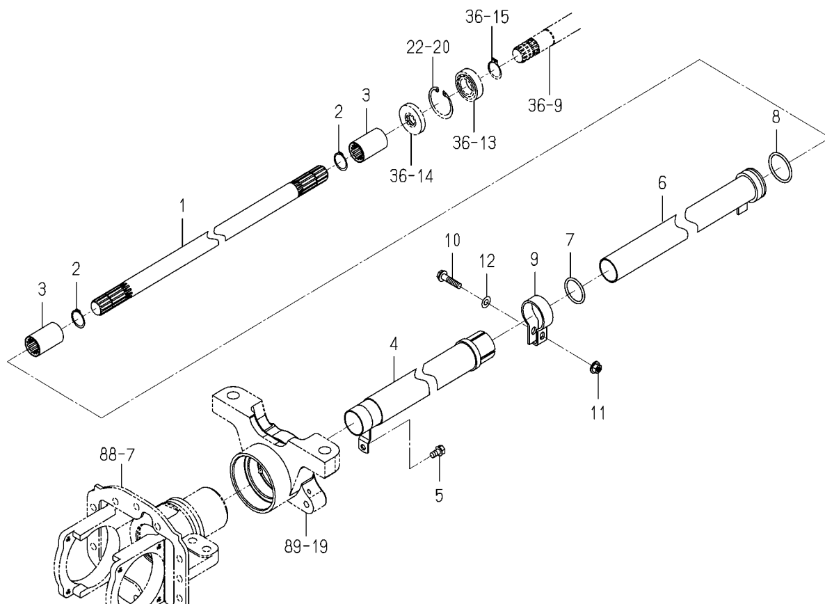
FIG. 87 SHAFT(DRIVE/FRONT)SYSTEM (6675H,6625H TYPE)
