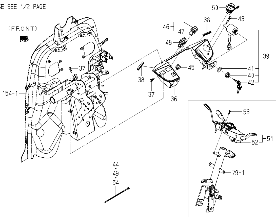
FIG.139 ELC.(MAIN)SYSTEM(2/2) (6675H,6625H TYPE)
