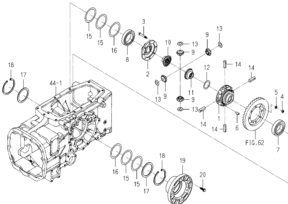
FIG. 64 CASE(DIFFERENTIAL/REAR)SYSTEM (6675H,6625H TYPE)
