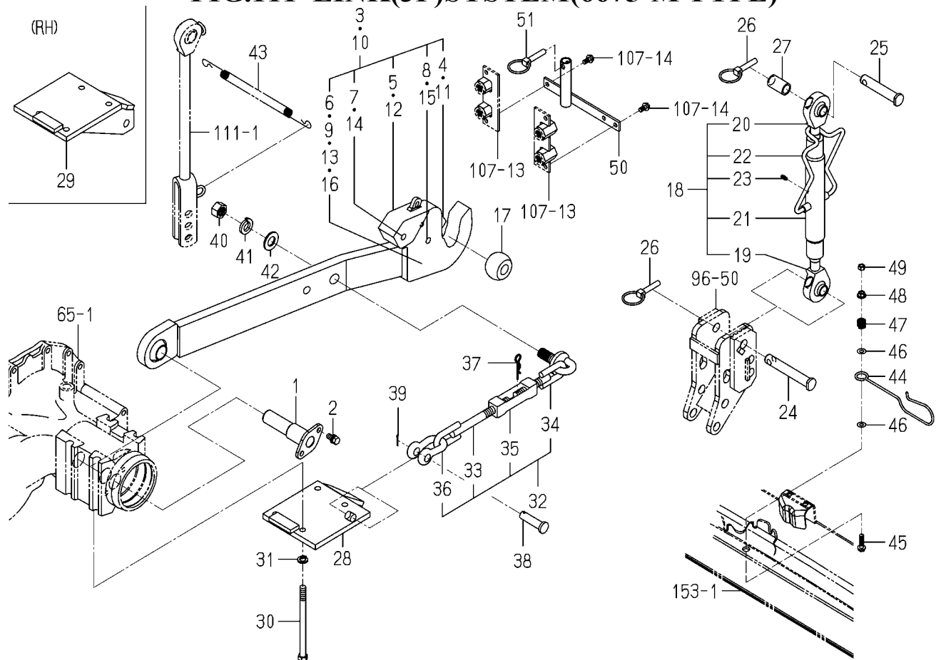
FIG.111 LINK(3P)SYSTEM(6675-M TYPE)
