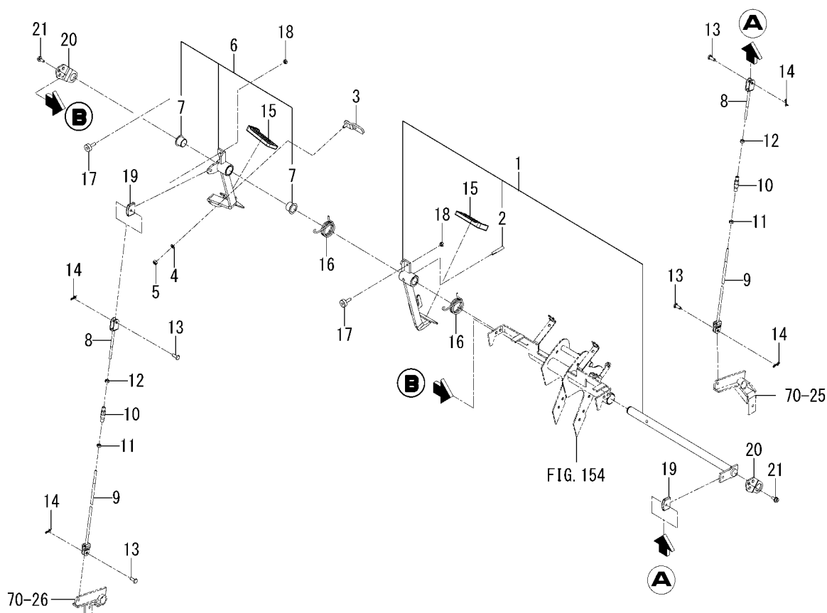
FIG. 74 PEDAL(BRAKE)SYSTEM (6675H,6625H TYPE)
