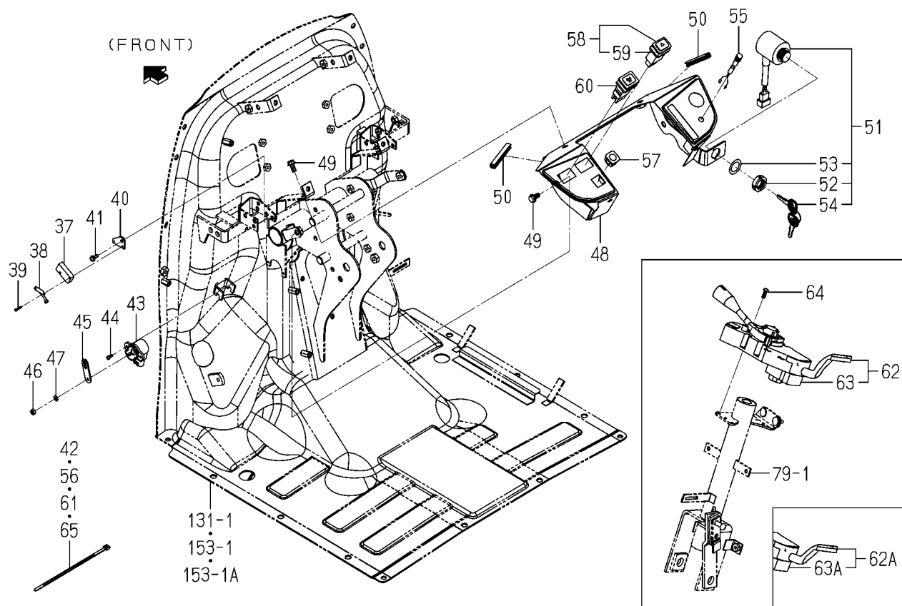
FIG.138 ELC.(MAIN)SYSTEM(6675 TYPE)(2/2)
