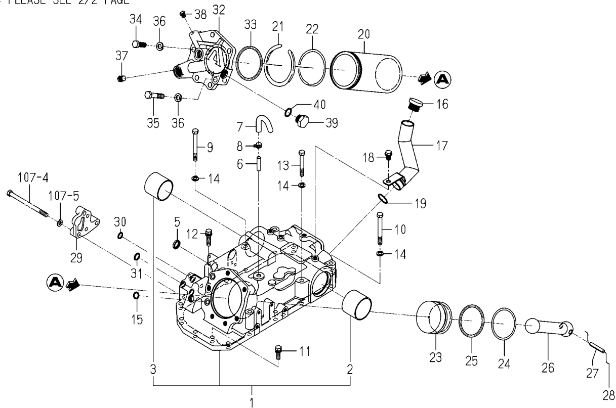
FIG. 92 CASE(CYLINDER)SYSTEM(1/2) (6675 TYPE)
