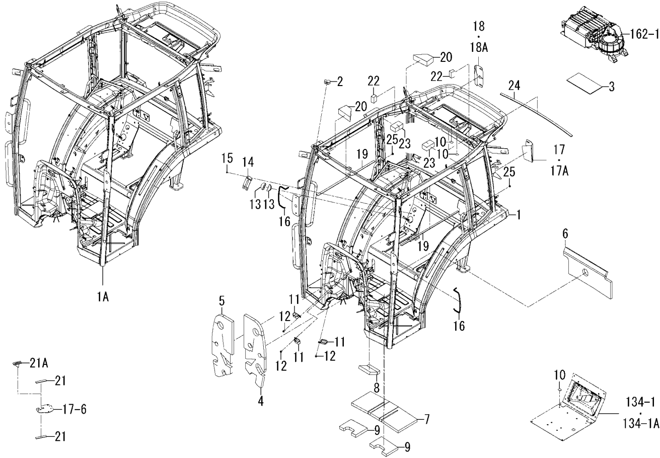
FIG.153 FRAME(CABIN)SYSTEM(M TYPE)
