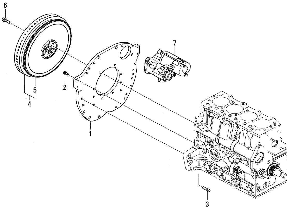
FIG.003 FLYWHEEL/REAR PLATE/STARTER
