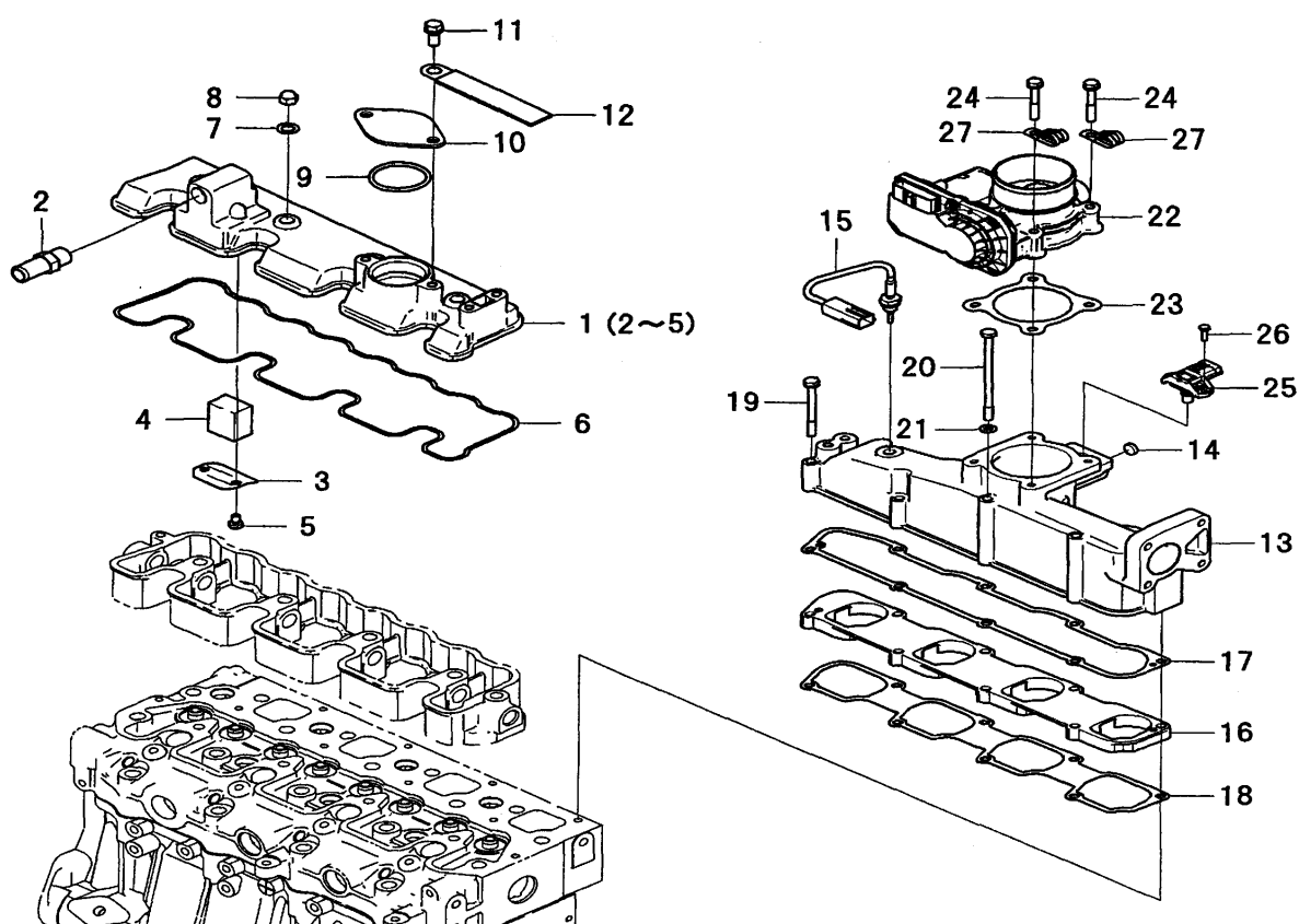
FIG.005 HEAD COVER
