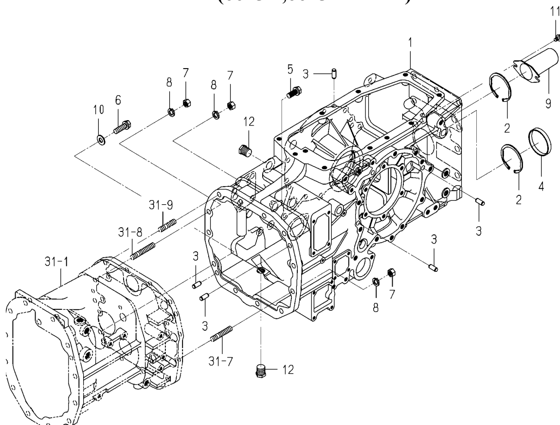
FIG. 44 CASE(TRANSMISSION)SYSTEM (6675H,6625H TYPE)
