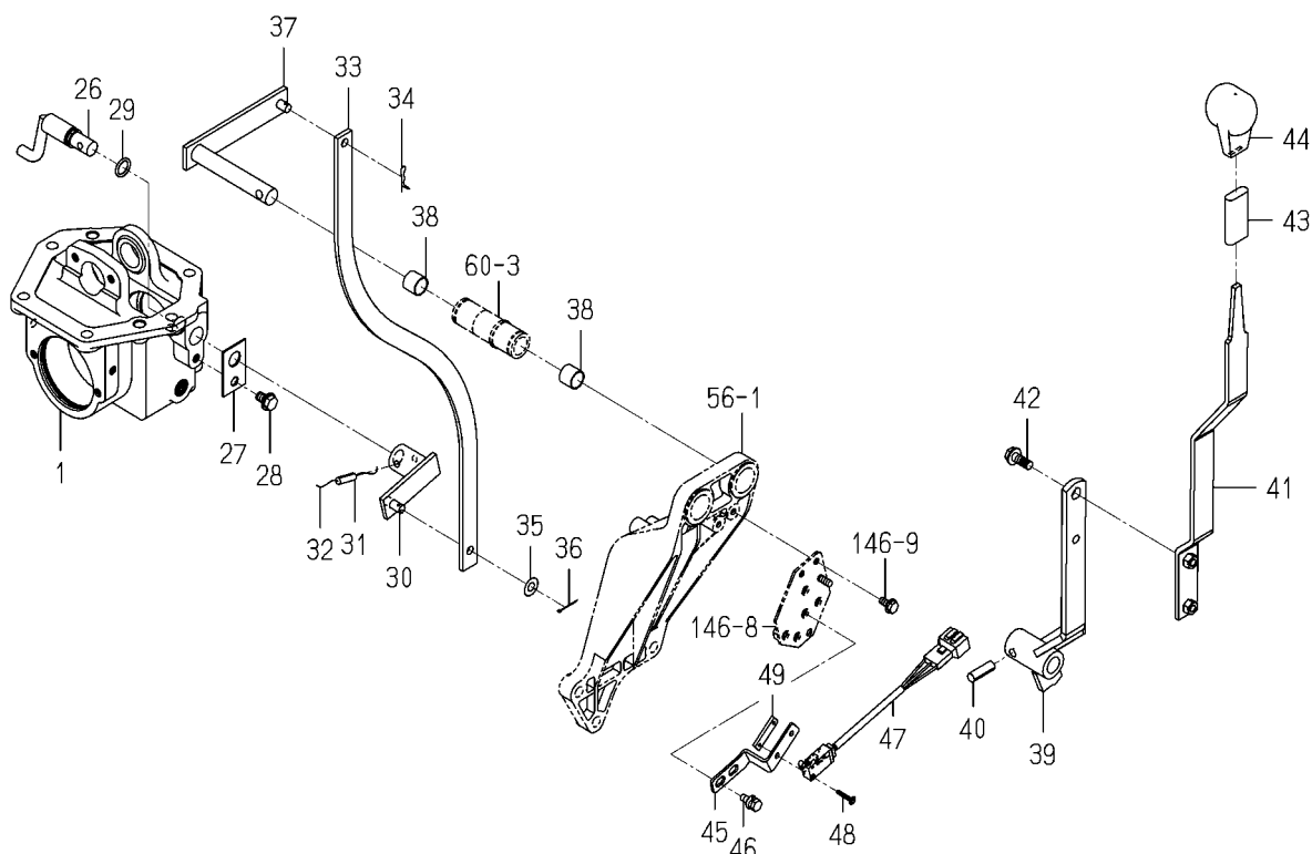
FIG. 42 PTO(MID)SYSTEM(2/2) (6675H,6625H TYPE)
