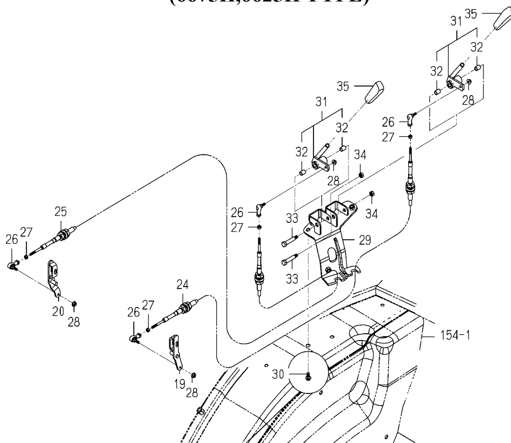
FIG.108 VALVE(REMOTE/2R)SET SYSTEM(2/2) (6675H,6625H TYPE)
