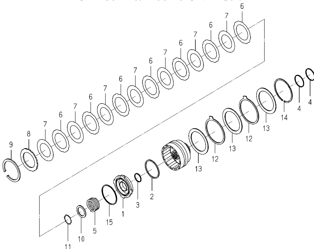
FIG.203 COMPONENT PARTS FOR 1802-209-200-10 ON FIG.29
