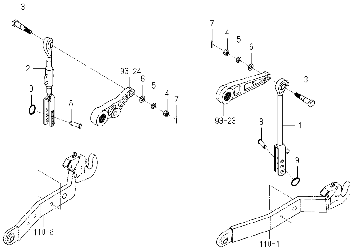
FIG.112 ROD(LIFT)SYSTEM(6675H,6625H TYPE)
