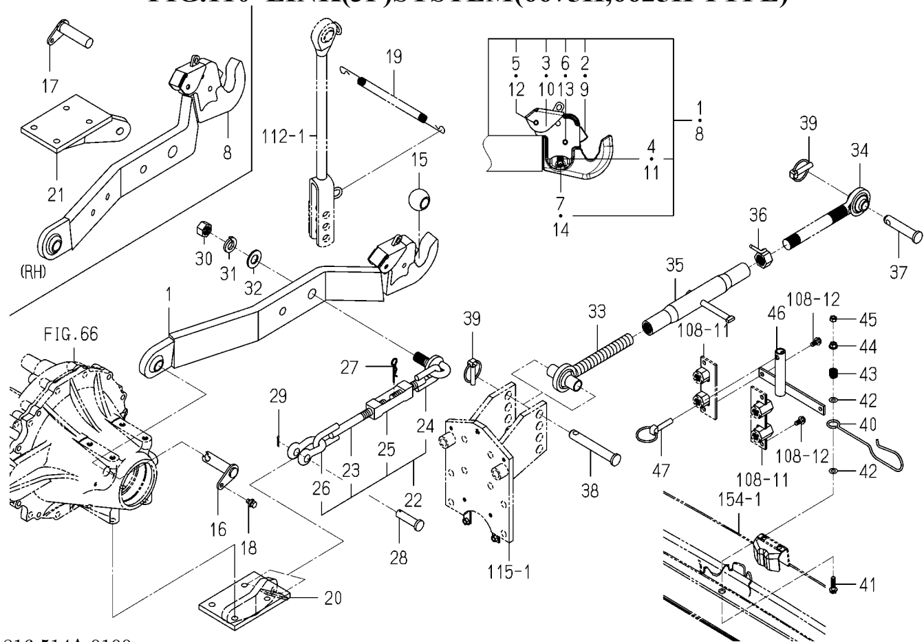
FIG.110 LINK(3P)SYSTEM(6675H,6625H TYPE)
