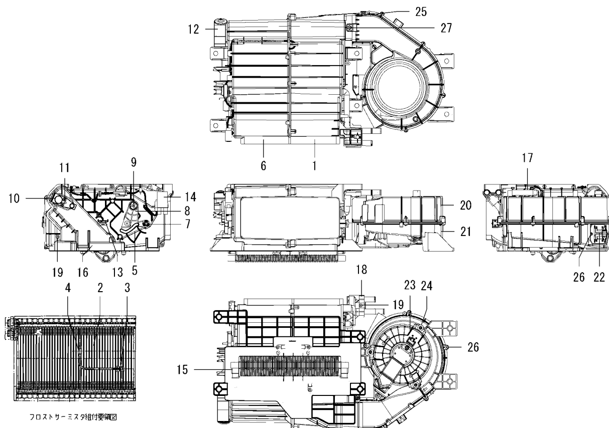
FIG.200 COMPONENT PARTS FOR 1792-782-600-20 ON FIG.162
