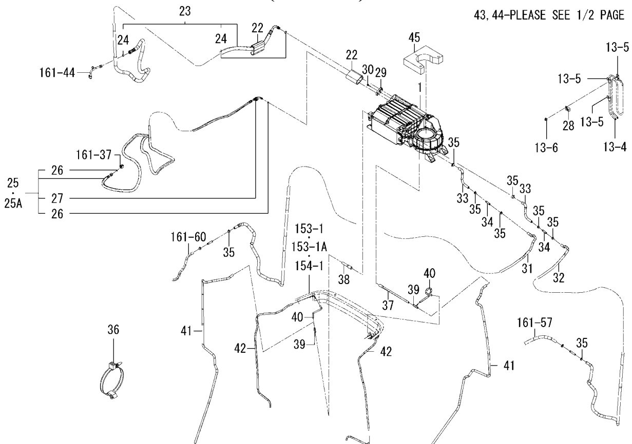
FIG.162 AIR CONDITIONER(CABIN)SYSTEM(2/2) (M TYPE)
