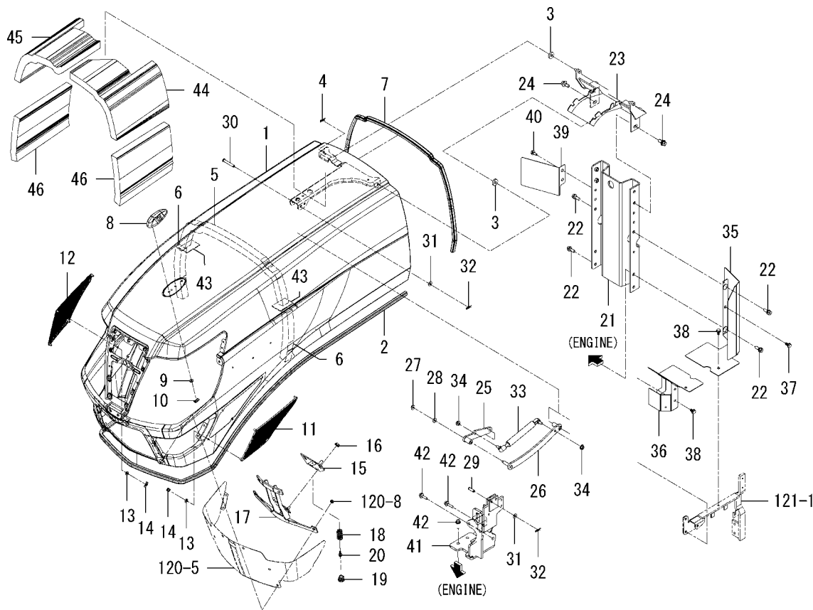
FIG.118 HOOD(LONG)SYSTEM (6675 TYPE EXCEPT M)
