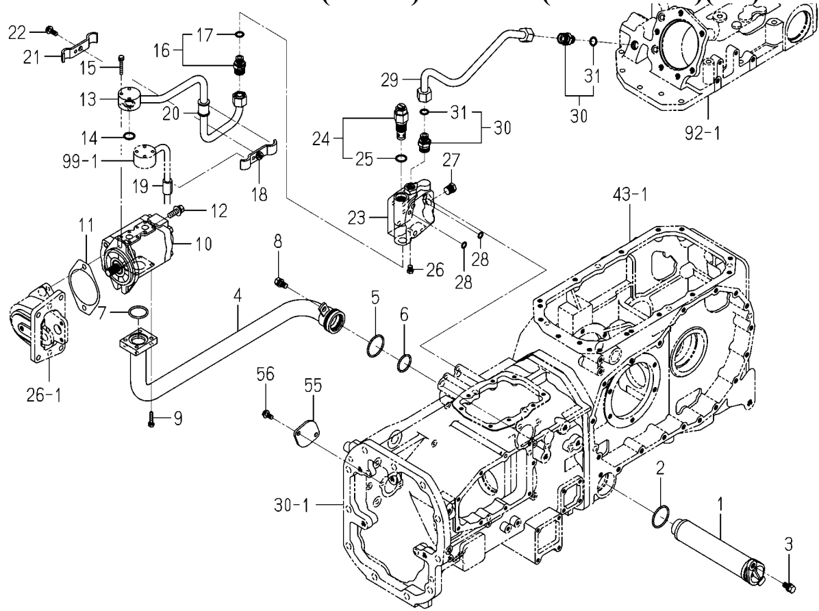
FIG. 97 PIPING(MAIN)SYSTEM(6675 TYPE)(1/2)
