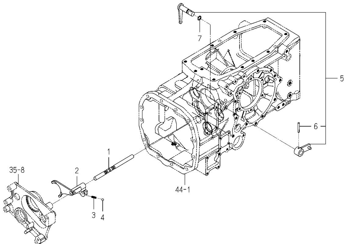
FIG. 46 FORK(SHIFT/CHANGE/SUB)SYSTEM (6675H,6625H TYPE)
