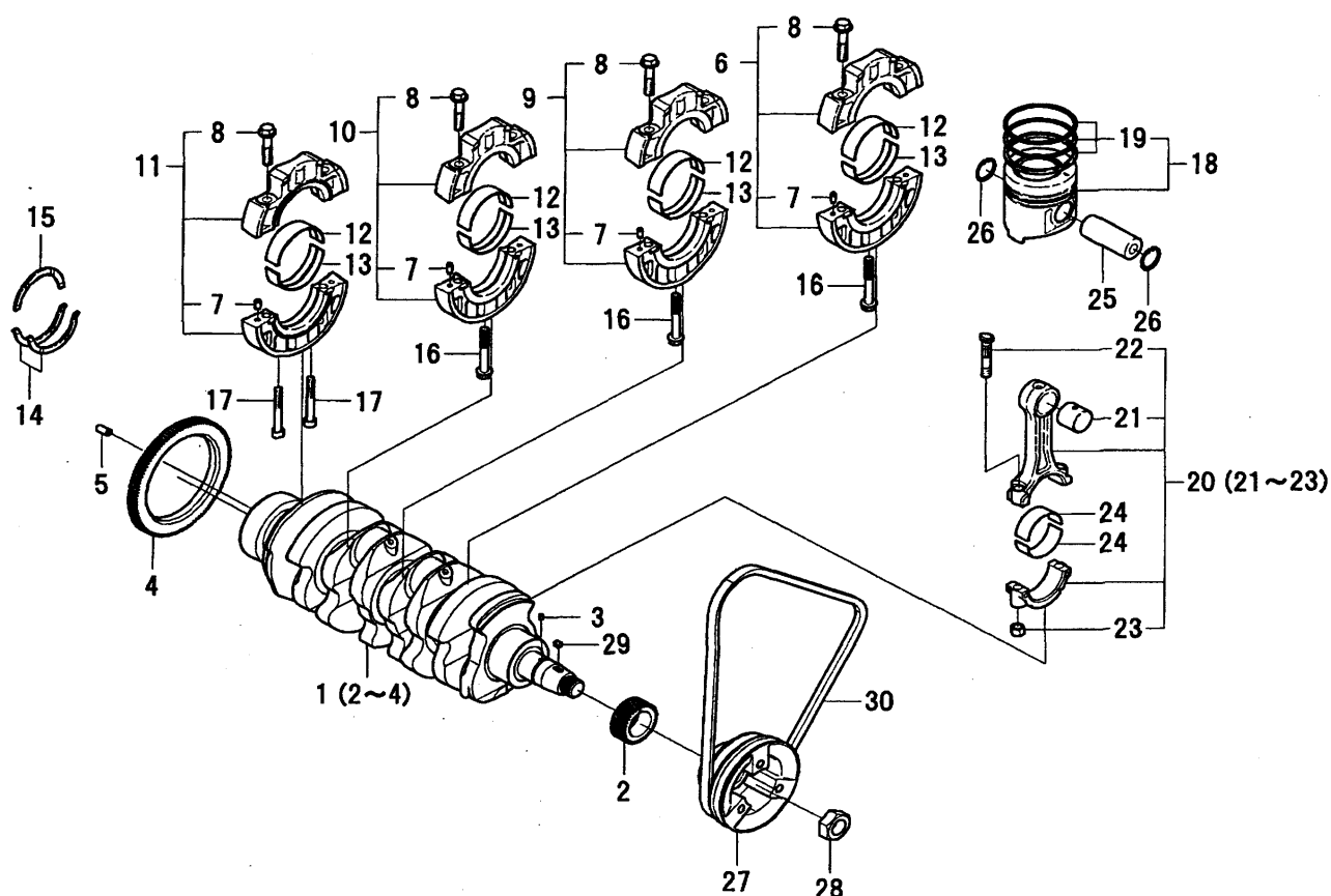
FIG.002 CRANKSHAFT/PISTON
