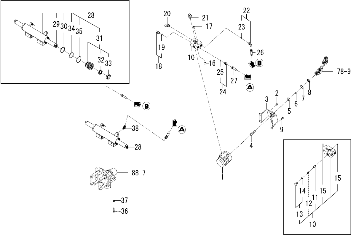
FIG. 81 STEERING(POWER)SYSTEM (6675H,6625H TYPE)
