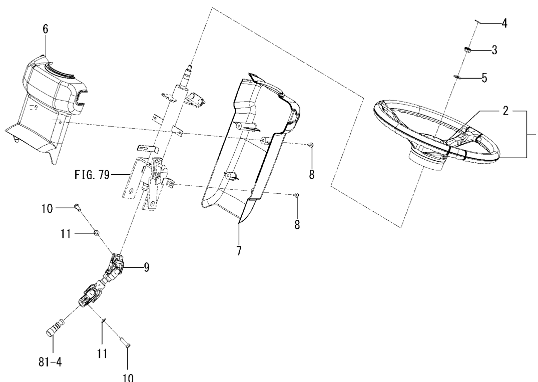
FIG. 78 WHEEL(STEERING)SYSTEM (6675H,6625H TYPE)
