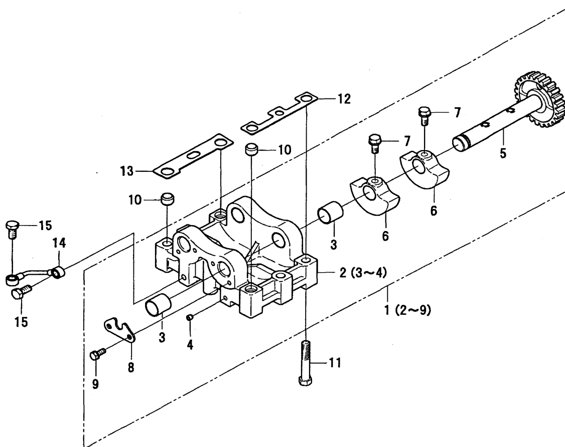
FIG.012 BALANCER
