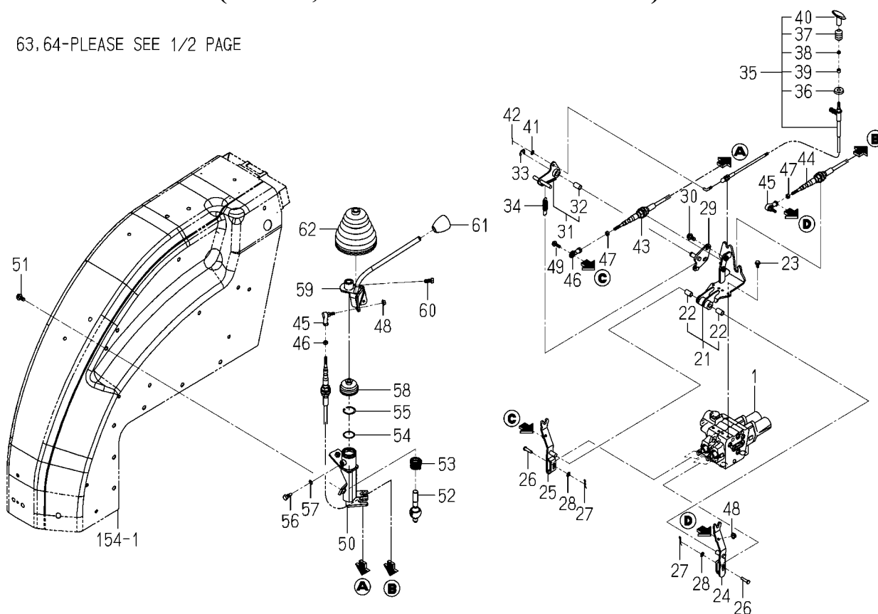
FIG.106 JOY STICK SYSTEM(2/2) (6675H,6625H TYPE EXCEPT D)
