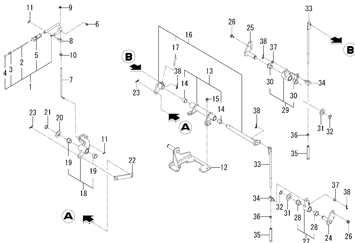
FIG. 75 LEVER(BRAKE/PARKING)SYSTEM (6675 TYPE)
