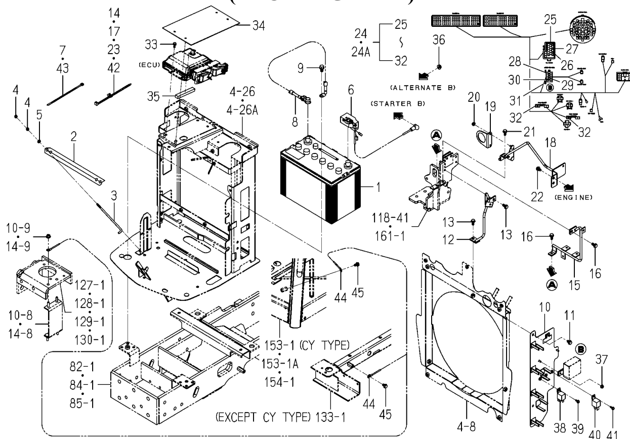
FIG.136 ELC.(FRONT)SYSTEM(1/2) (EXCEPT G TYPE)
