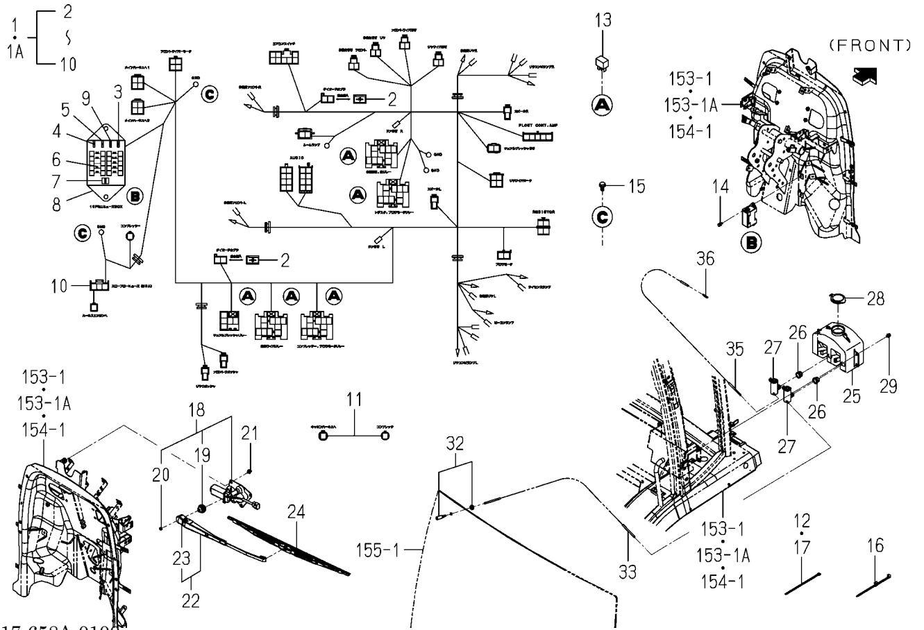
FIG.144 ELC.(CABIN)SYSTEM(M TYPE)(1/2)
