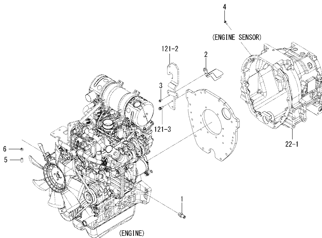
FIG. 3 ENGINE(PARTS)SYSTEM (6675H,6625H TYPE)
