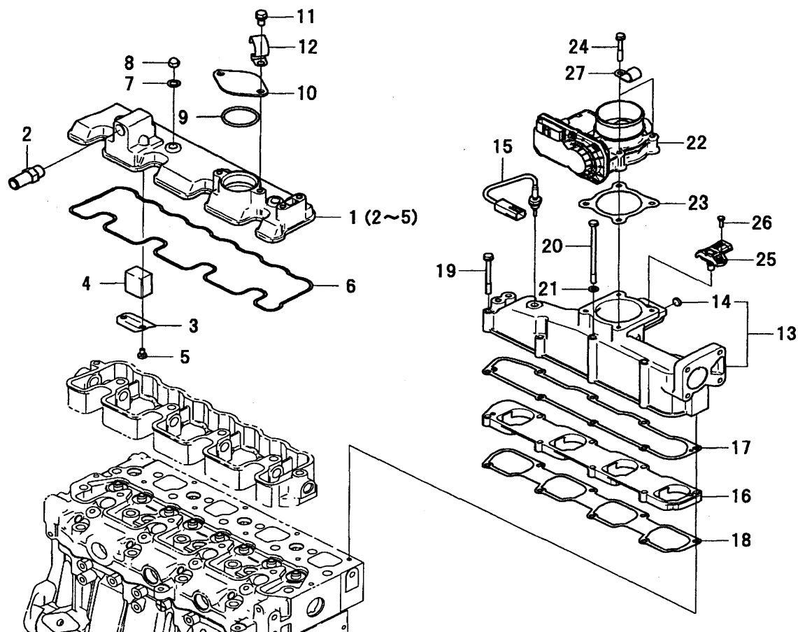
FIG.005 HEAD COVER
