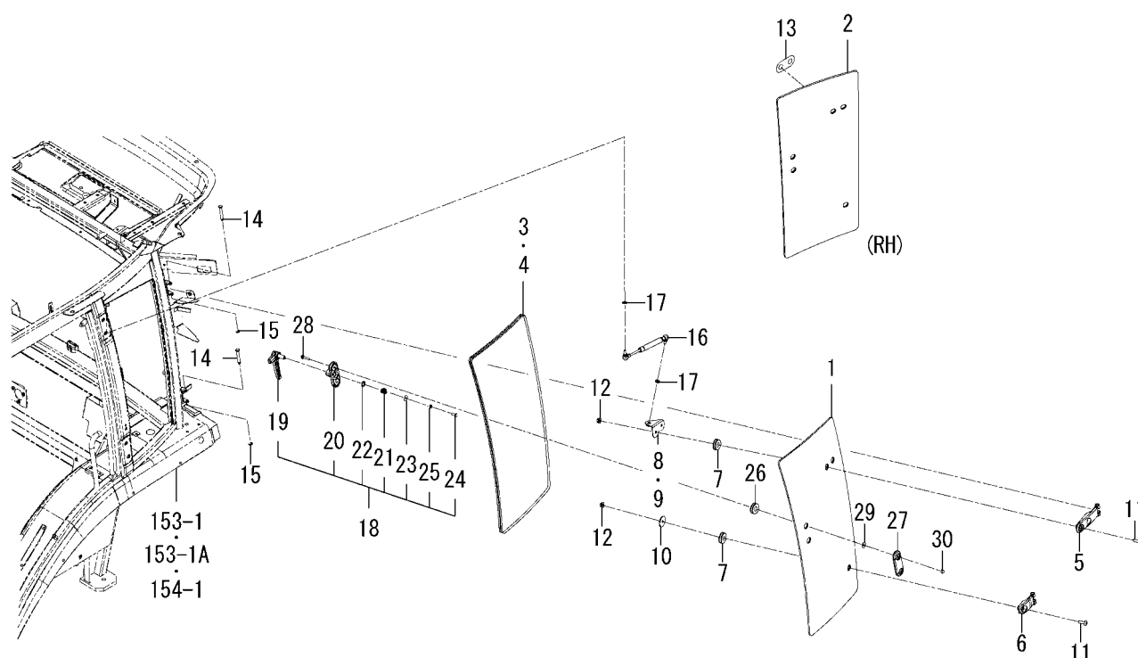
FIG.158 GLASS(SIDE/CABIN)SYSTEM(M TYPE)
