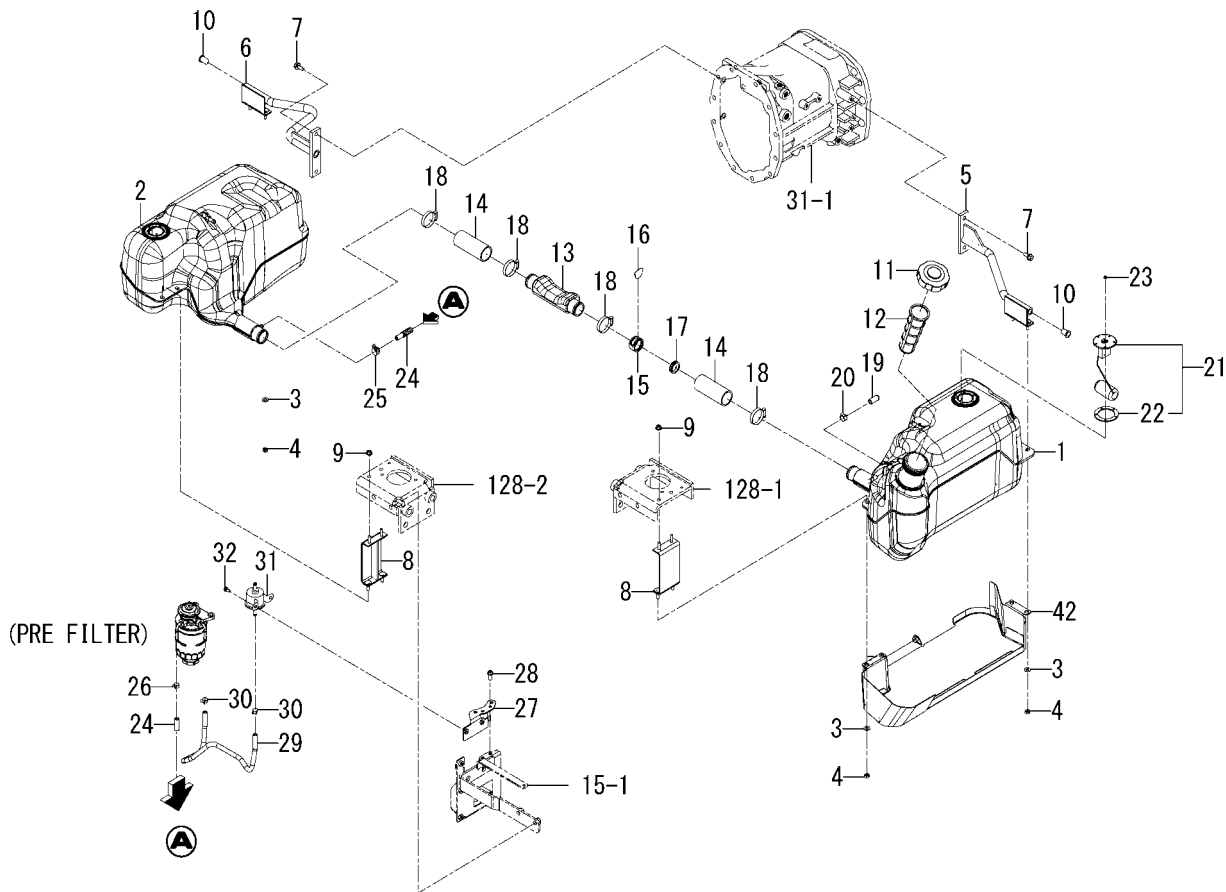
FIG. 14 TANK(FUEL)SYSTEM(1/2)
