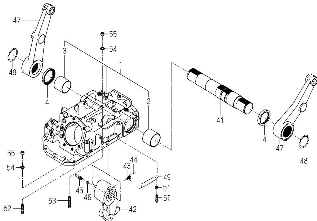
FIG. 92 CASE(CYLINDER)SYSTEM(2/2) (6675 TYPE)
