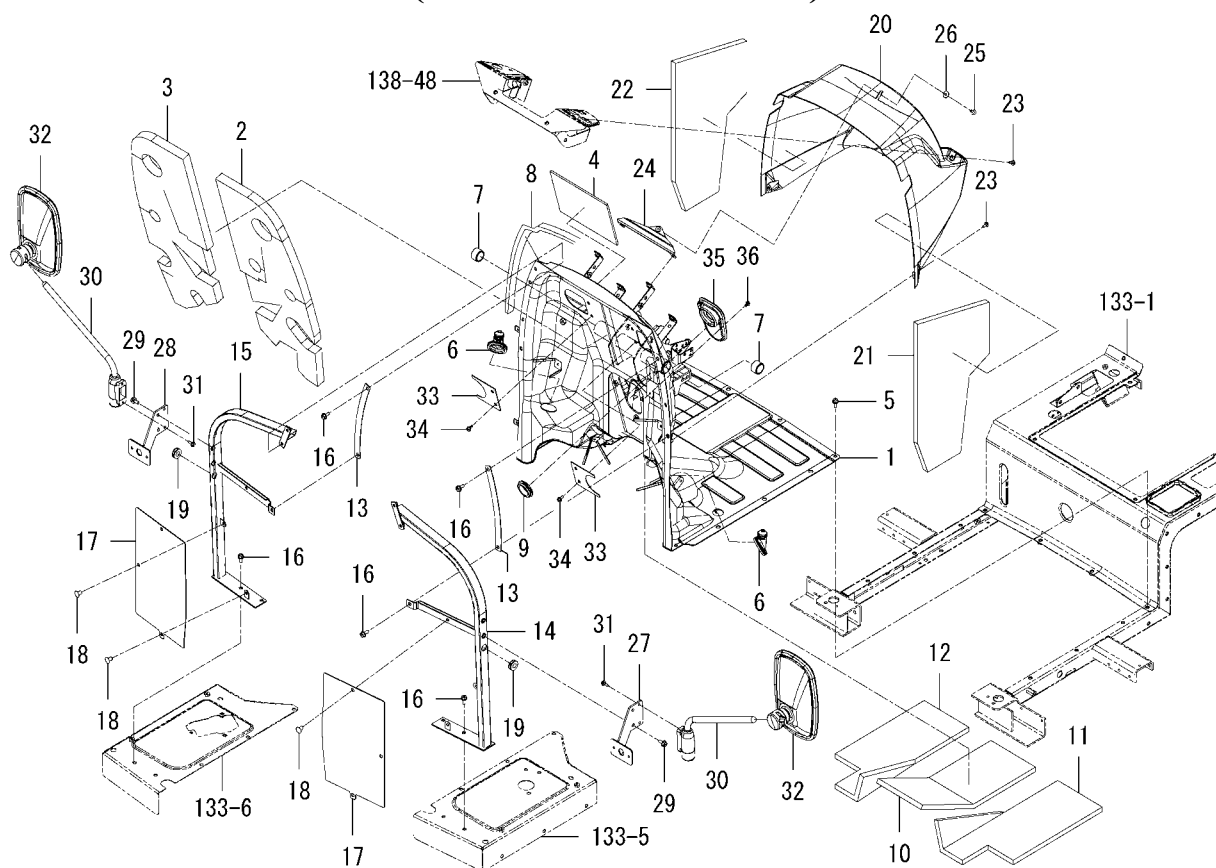
FIG.131 FLOOR(FRONT)SYSTEM (6675 TYPE M TYPE)
