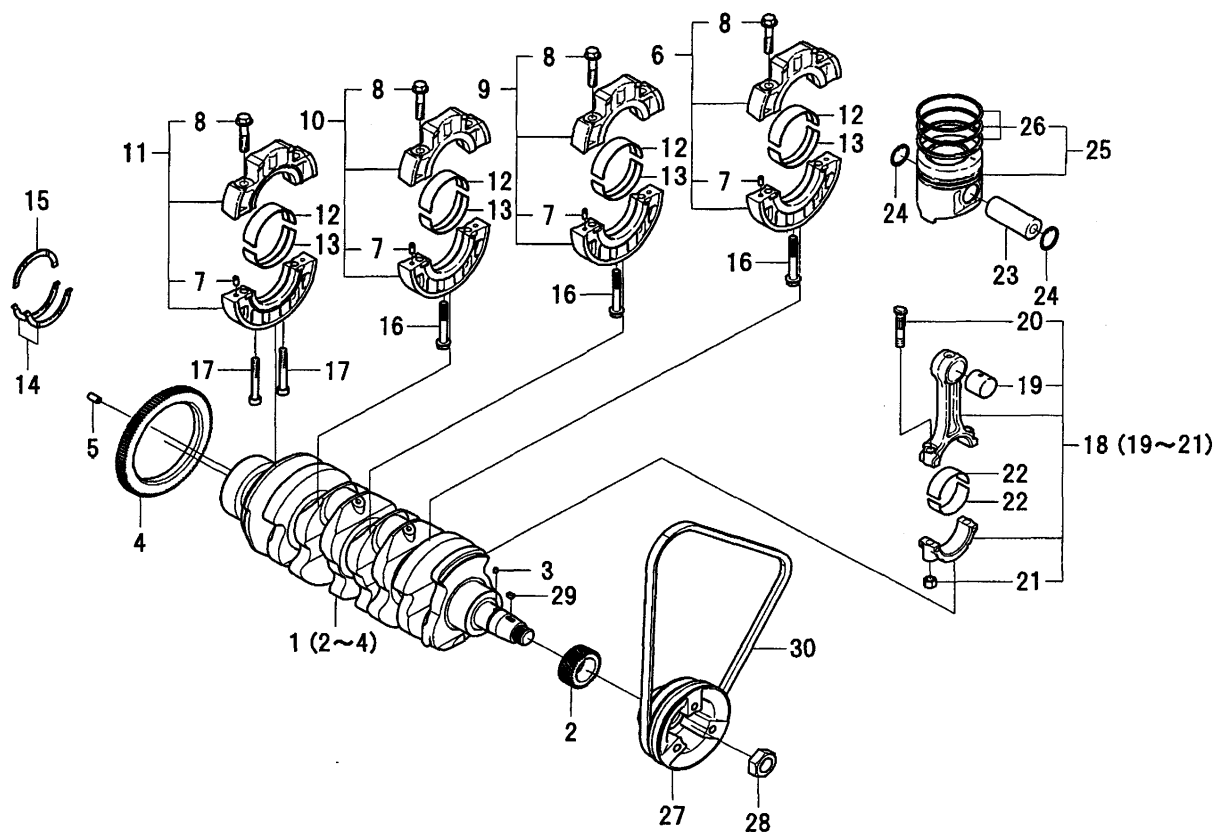
FIG.002 CRANKSHAFT/PISTON
