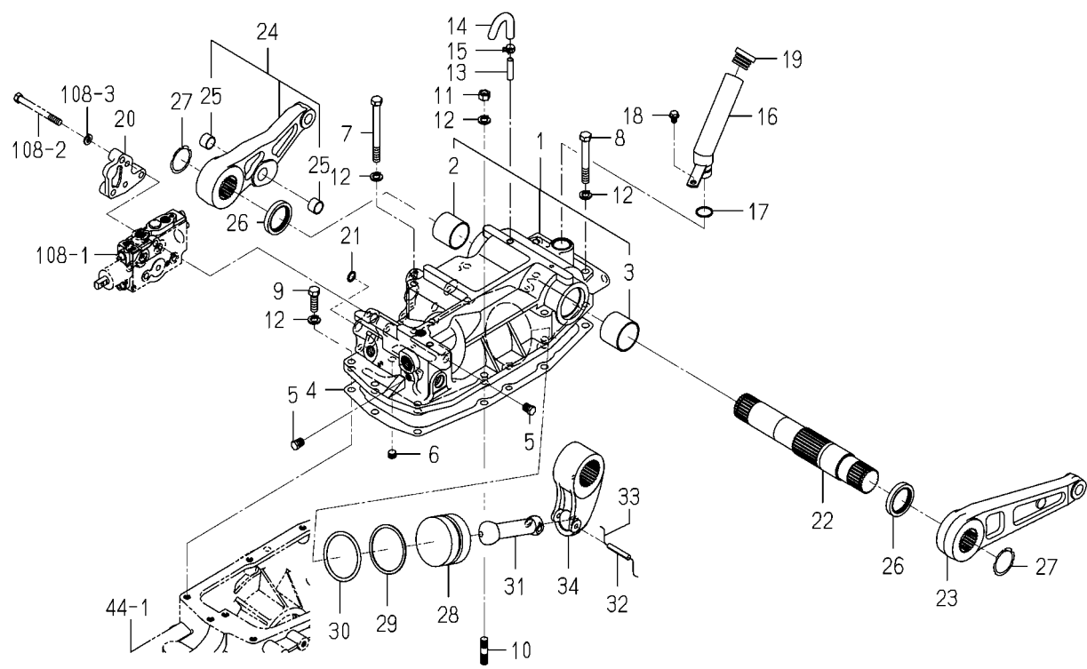
FIG. 93 CASE(CYLINDER)SYSTEM(1/2) (6675H,6625H TYPE)
