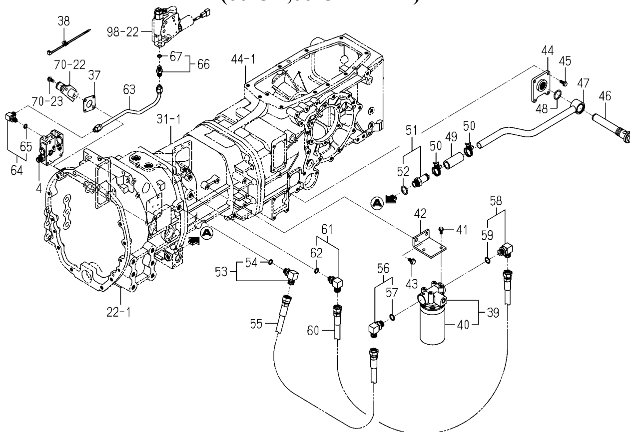
FIG.100 PIPING(SUB)SYSTEM(3/3) (6675H,6625H TYPE)
