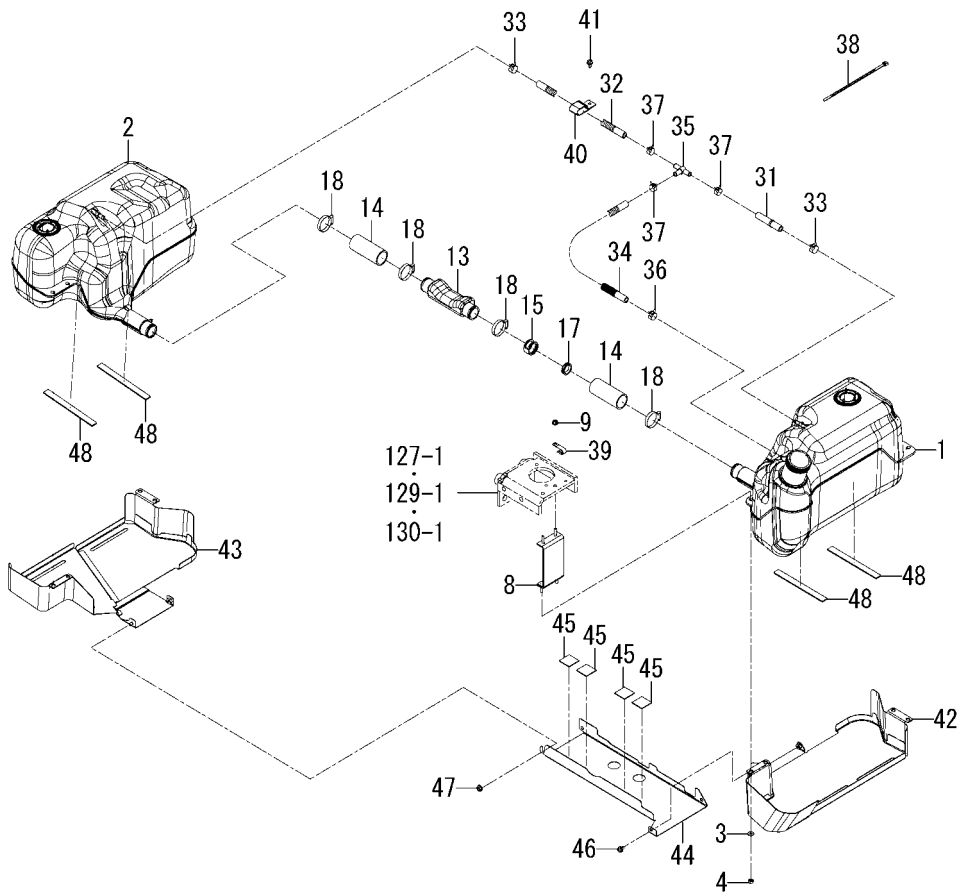
FIG. 10 TANK(FUEL)SYSTEM(6675 TYPE)(2/2)
