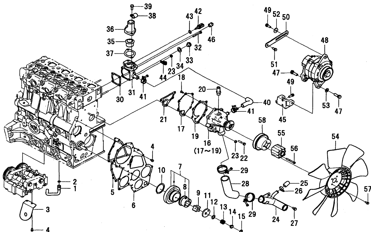
FIG.007 OIL PUMP/WATER PUMP/ THERMOSTAT CASE/ALTERNATOR
