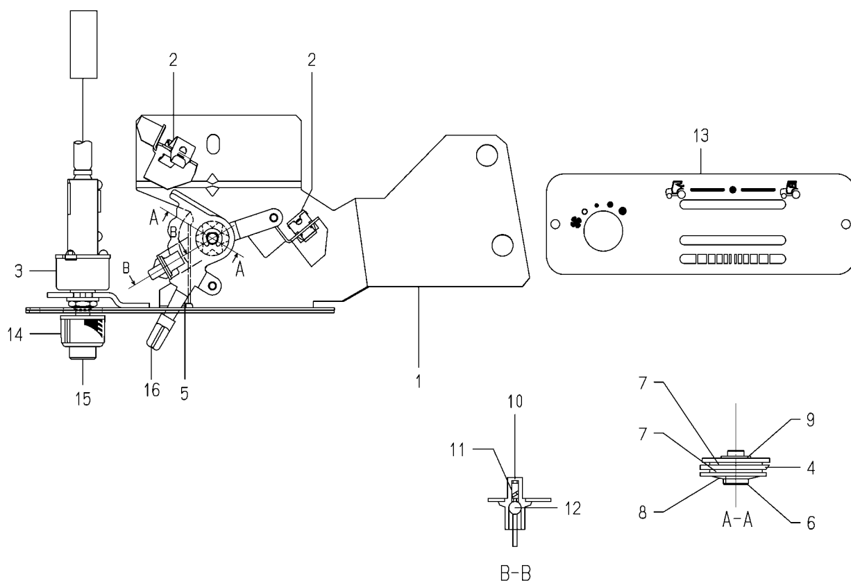
FIG.201 COMPONENT PARTS FOR 1800-782-400-20 ON FIG.162
