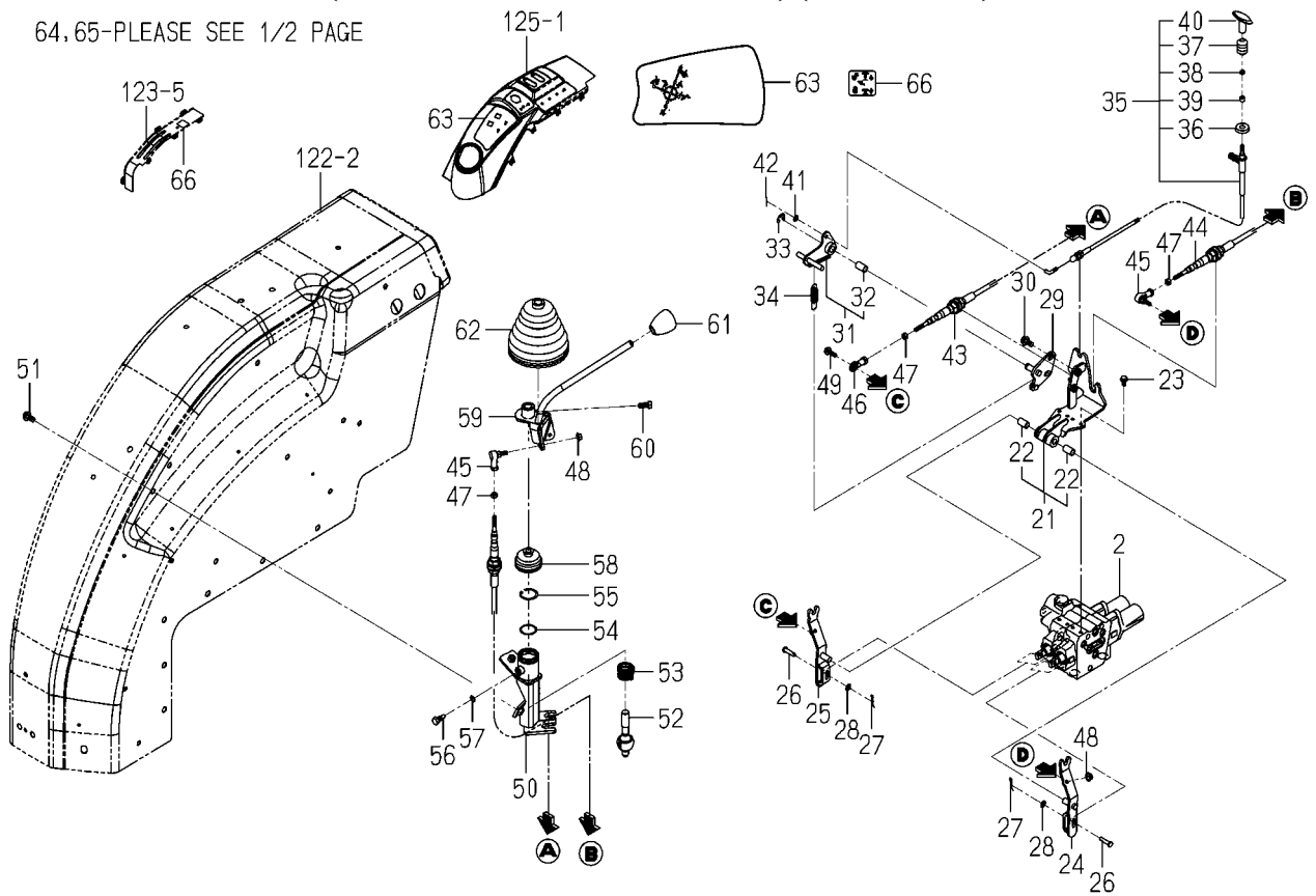
FIG.182 JOYSTICK(E4/5)SET(2/2) (6675 TYPE EXCEPT J)(OPTION)
