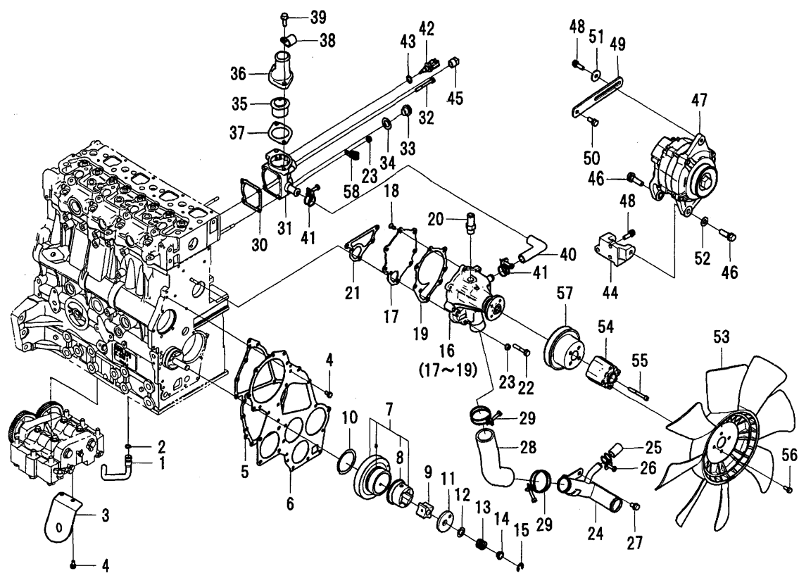
FIG.007 OIL PUMP/WATER PUMP/ THERMOSTAT CASE/ALTERNATOR
