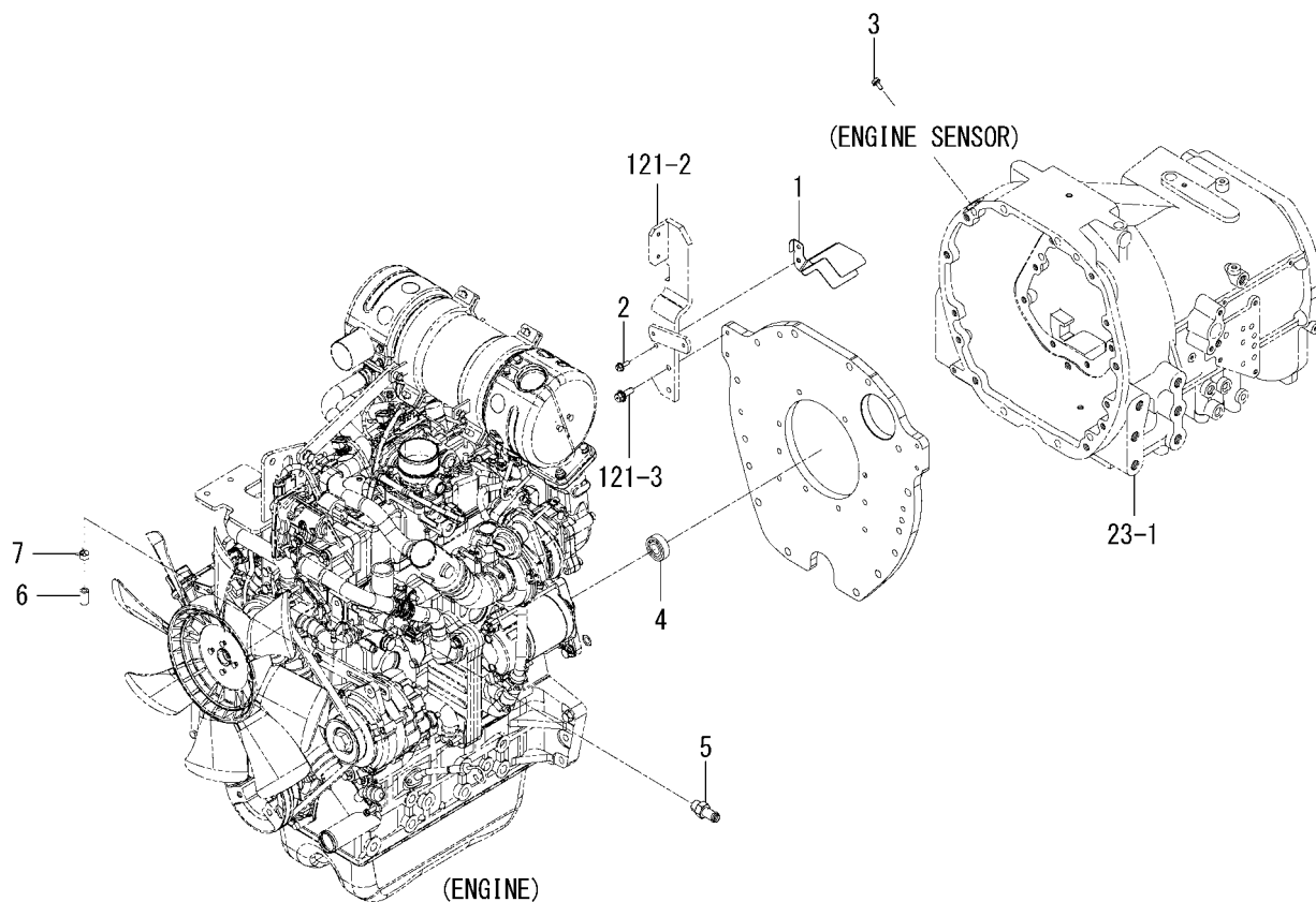
FIG. 2 ENGINE(PARTS)SYSTEM(6675-M TYPE)
