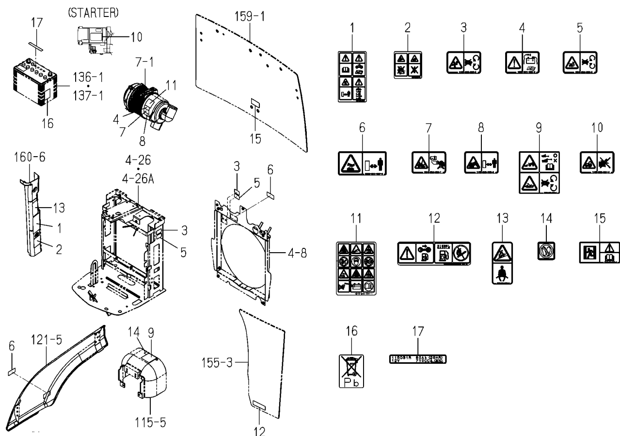
FIG.172 LABEL(CAUTION)(6675H,6625H TYPE)
