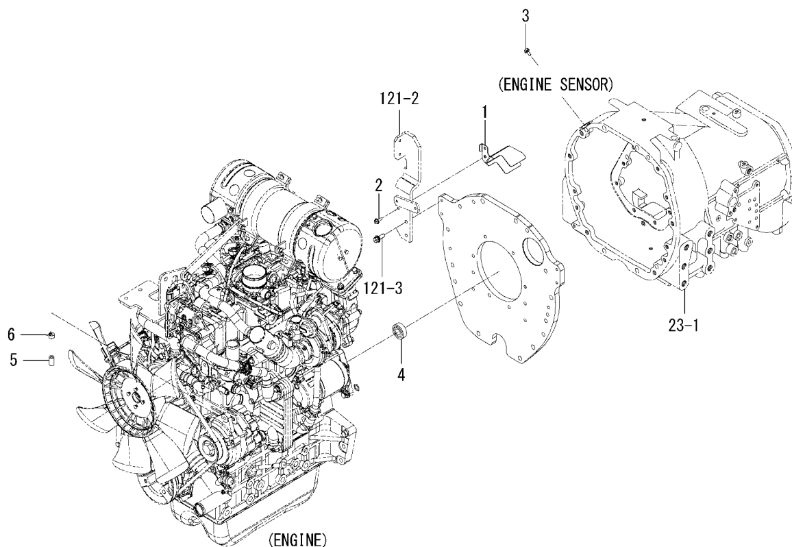
FIG. 1 ENGINE(PARTS)SYSTEM (6675 TYPE EXCEPT M)
