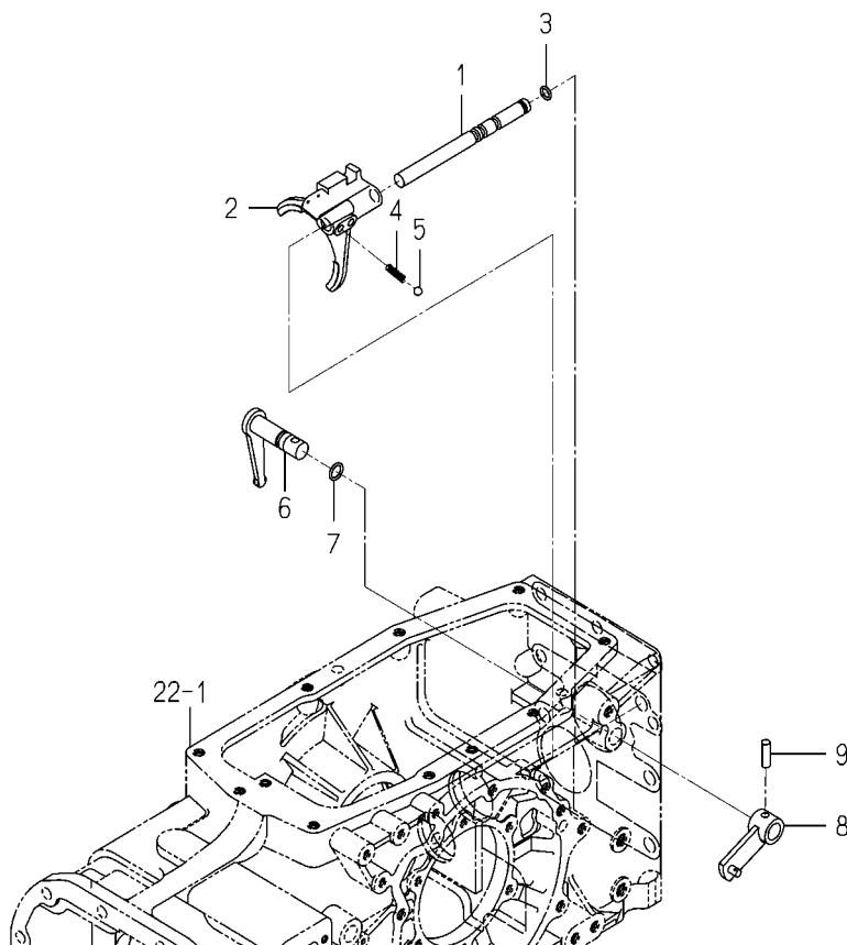
FIG. 50 FORK(SHIFT/PTO)SYSTEM (6675H,6625H TYPE)
