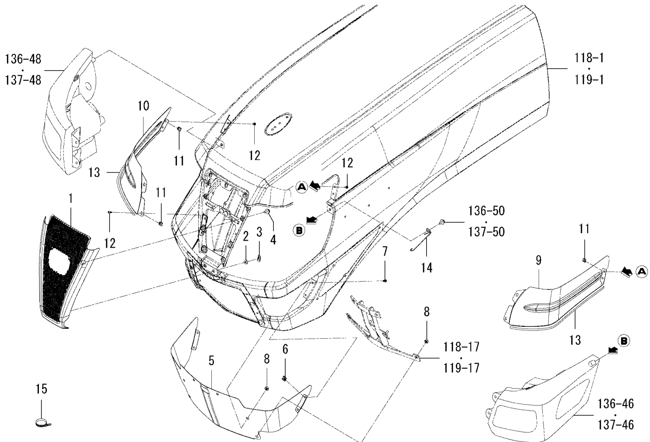
FIG.120 GRILLE SYSTEM
