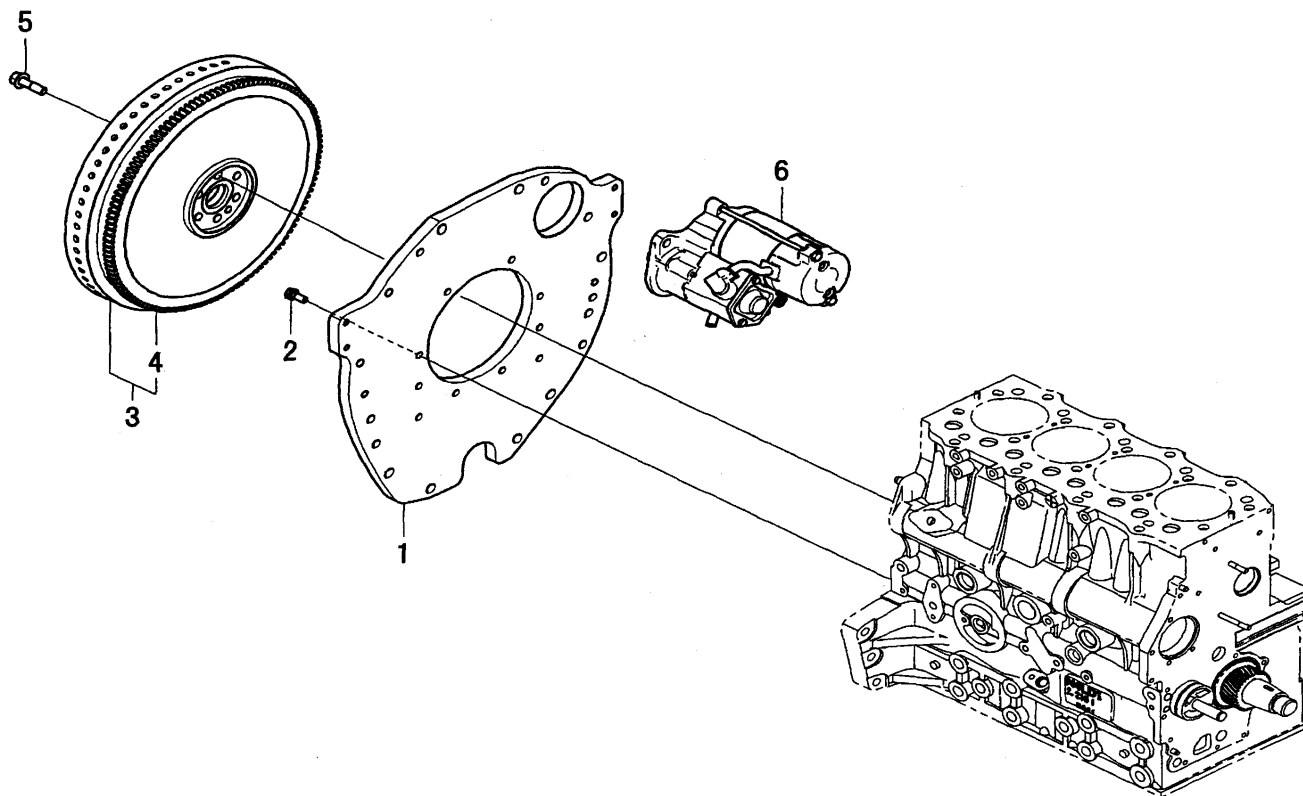
FIG.003 FLYWHEEL/REAR PLATE/STARTER
