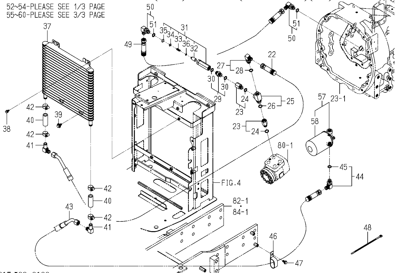
FIG. 99 PIPING(SUB)SYSTEM(6675 TYPE)(2/3)
