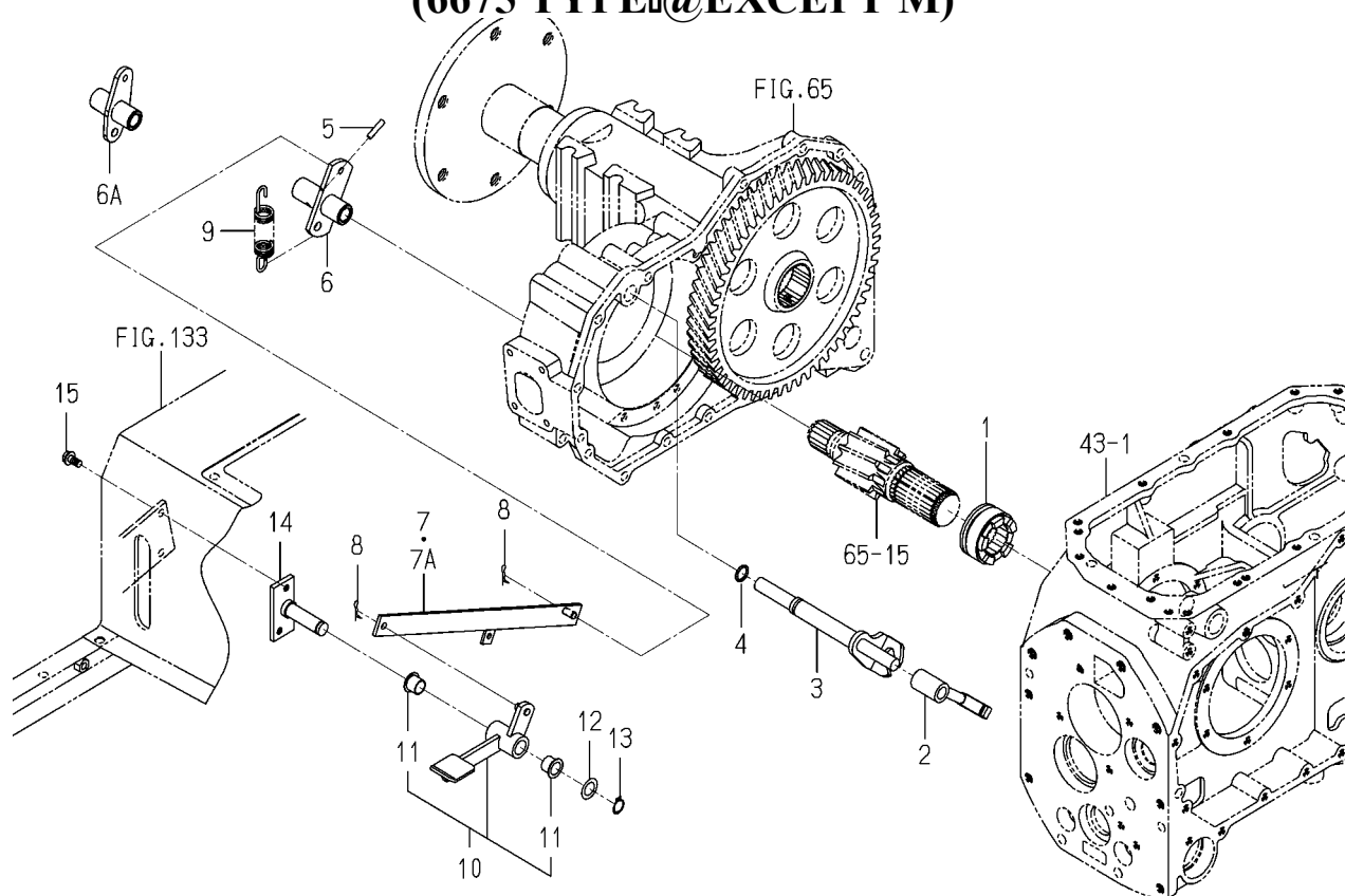
FIG. 67 PEDAL(DIFF-LOCK)SYSTEM (6675 TYPE@EXCEPT M)
