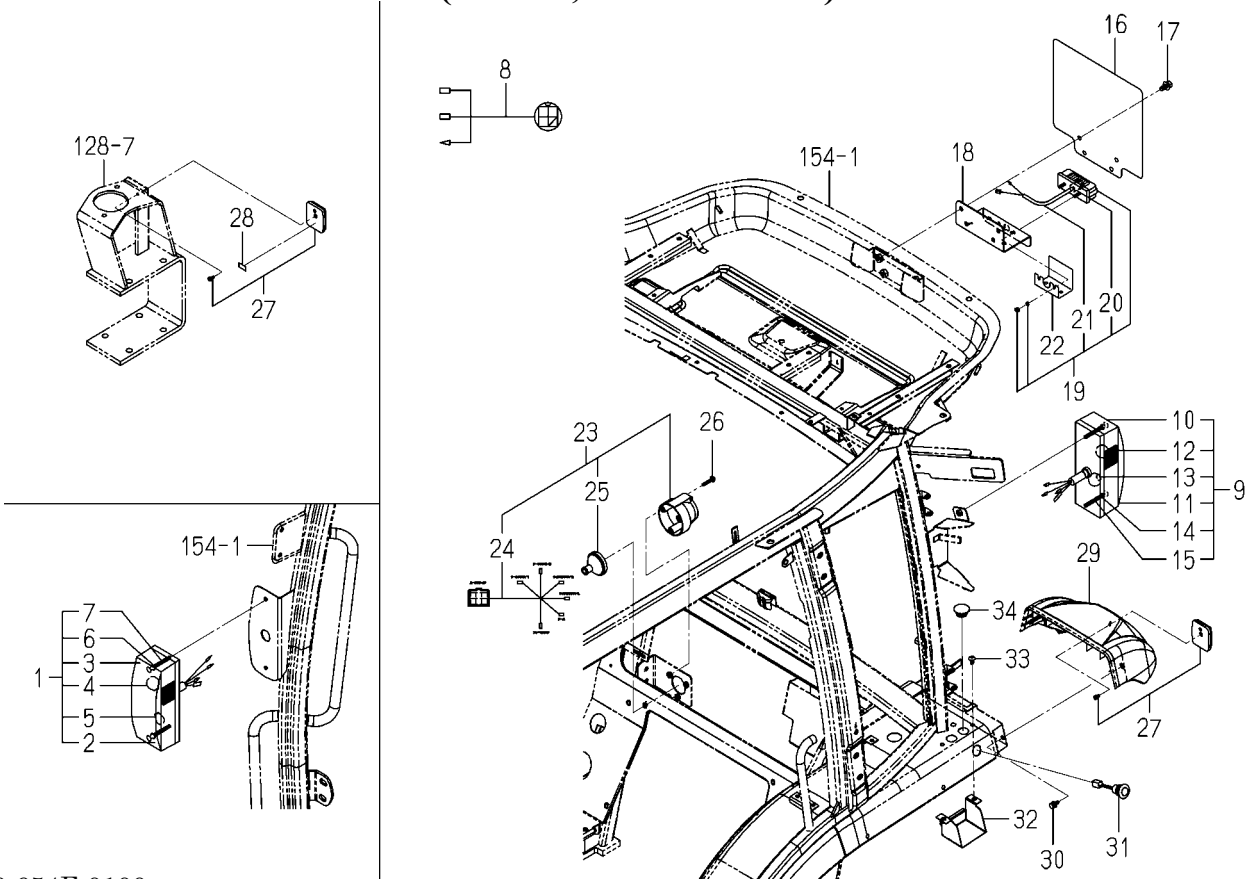
FIG.142 ELC.(FLOOR)SYSTEM(1/2) (6675H,6625H TYPE)
