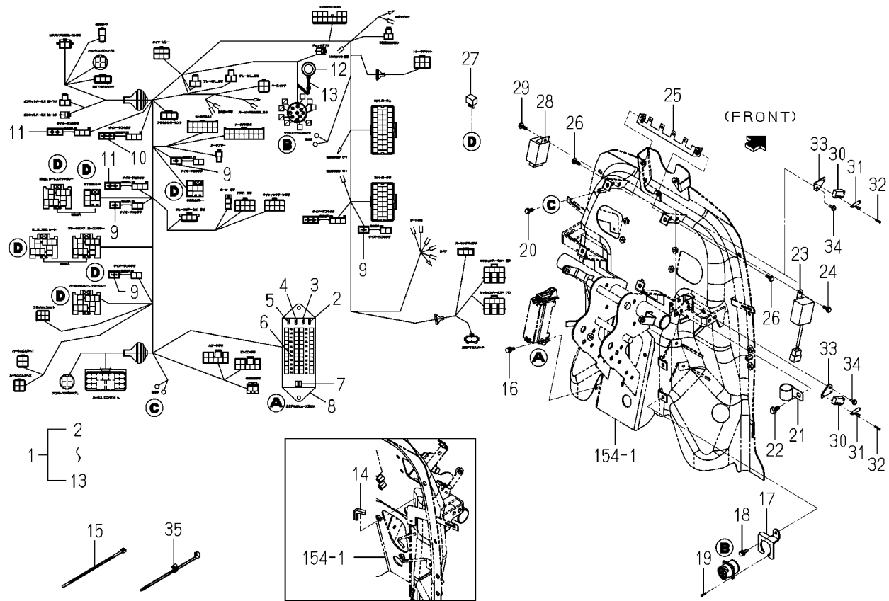
FIG.139 ELC.(MAIN)SYSTEM(1/2) (6675H,6625H TYPE)
