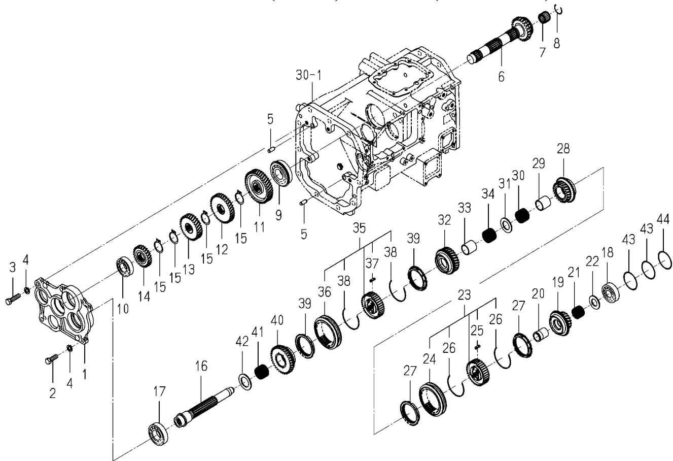
FIG. 32 GEAR(MAIN)SYSTEM(6675 TYPE)
