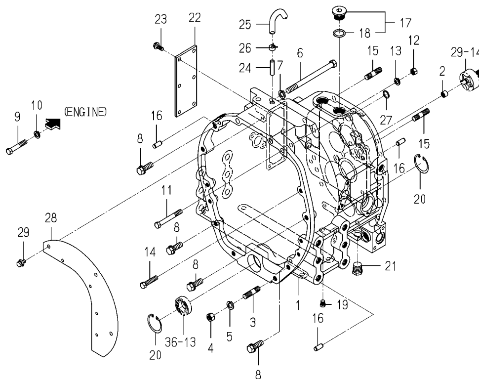
FIG. 22 CASE(TRANSMISSION)SYSTEM (6675H,6625H TYPE)
