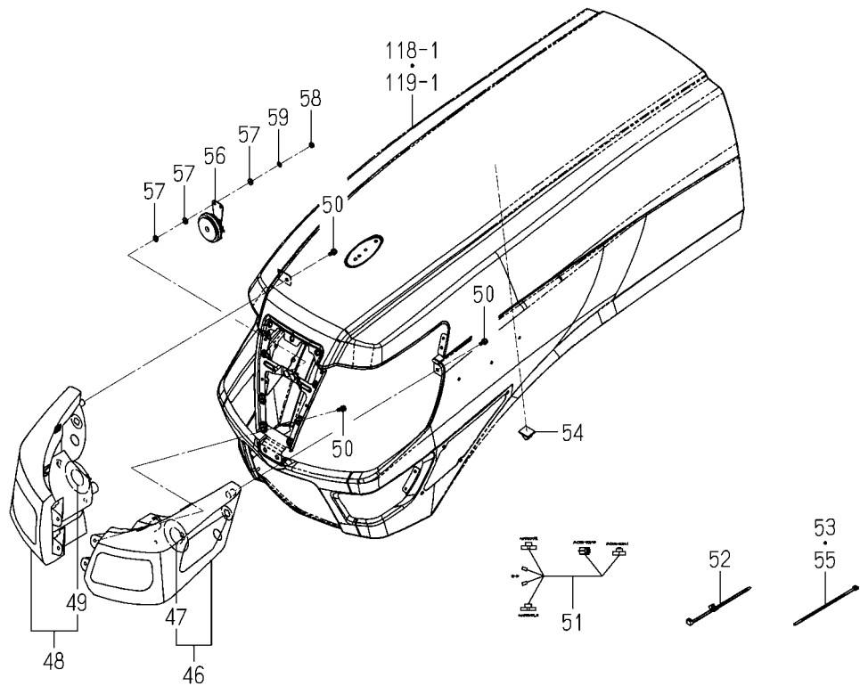
FIG.136 ELC.(FRONT)SYSTEM(2/2) (EXCEPT G TYPE)
