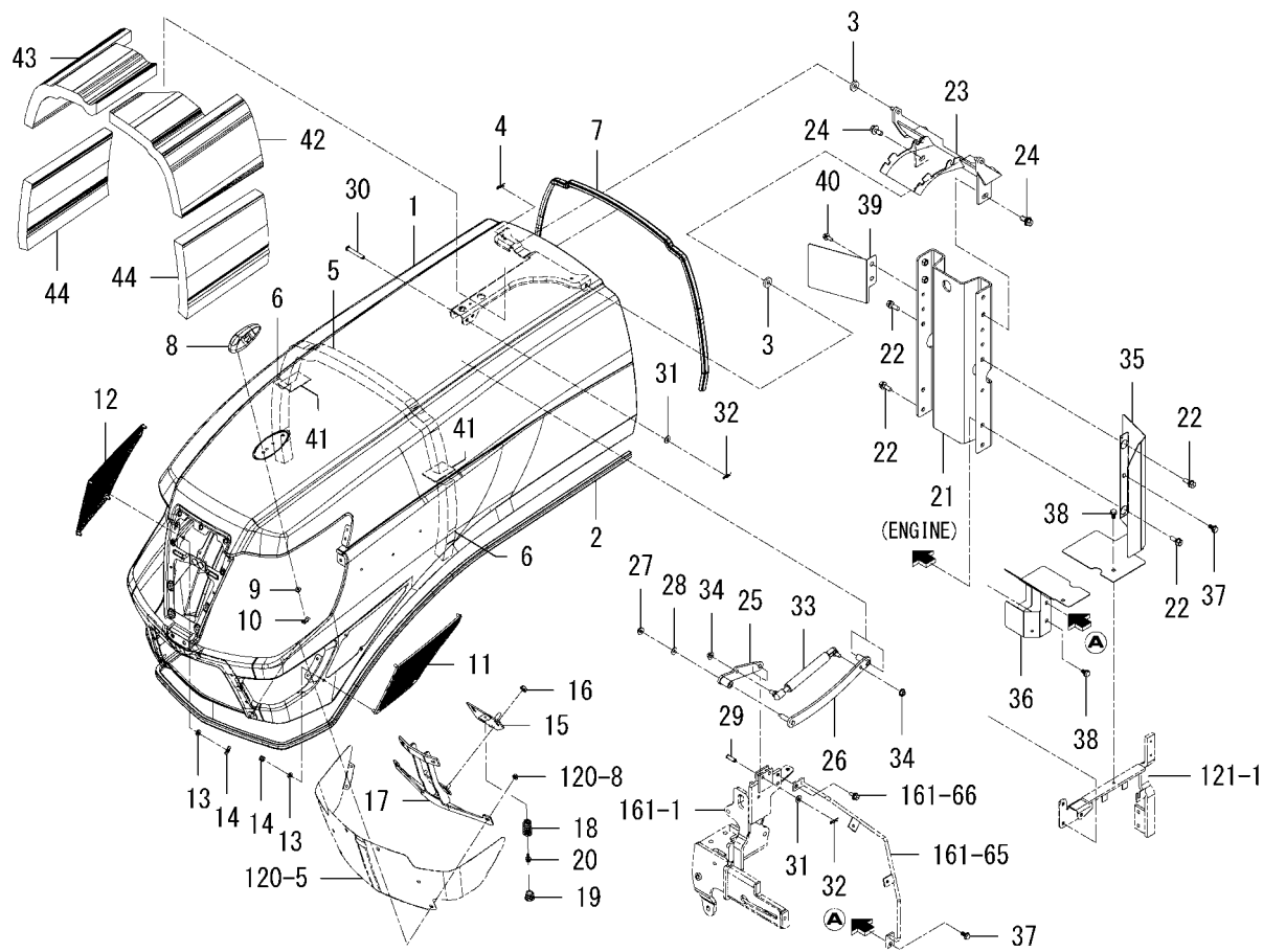
FIG.119 HOOD(LONG)SYSTEM(6675-M TYPE)
