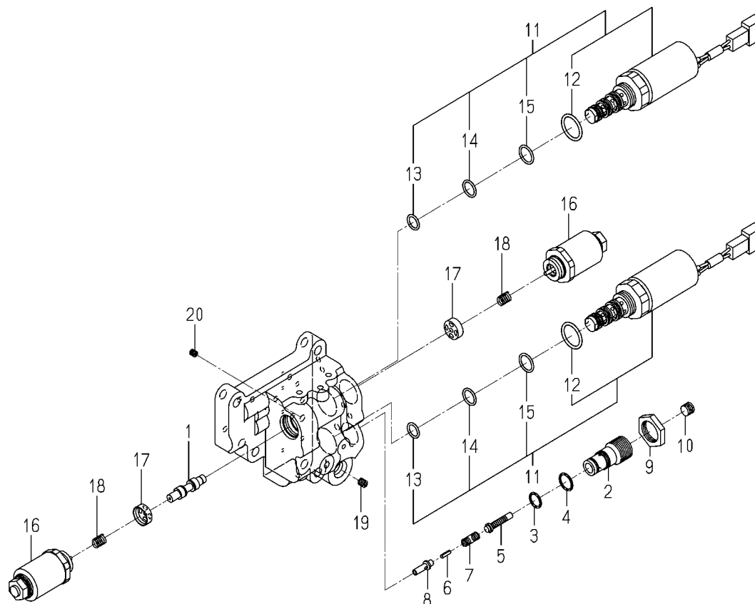
FIG.192 COMPONENT PARTS FOR K200-251-000-20 ON FIG.99
