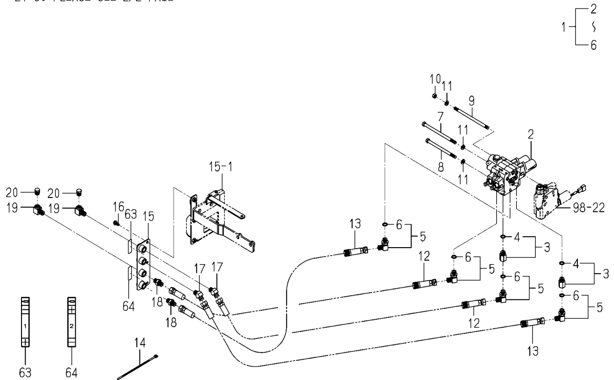
FIG.106 JOY STICK SYSTEM(1/2) (6675H,6625H TYPE EXCEPT D)
