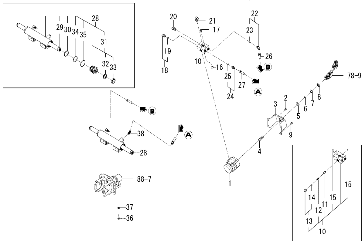
FIG. 81 STEERING(POWER)SYSTEM (6675H,6625H TYPE)
