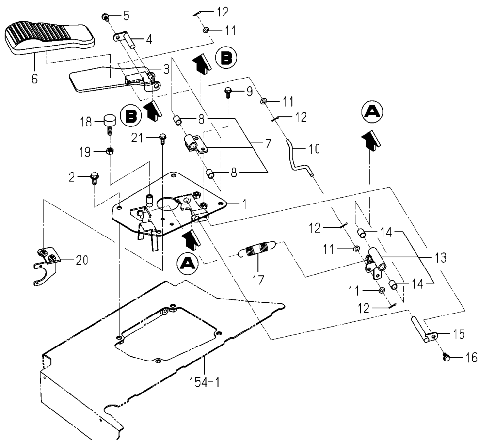
FIG. 18 PEDAL(HST)SYSTEM(6675H,6625H TYPE)
