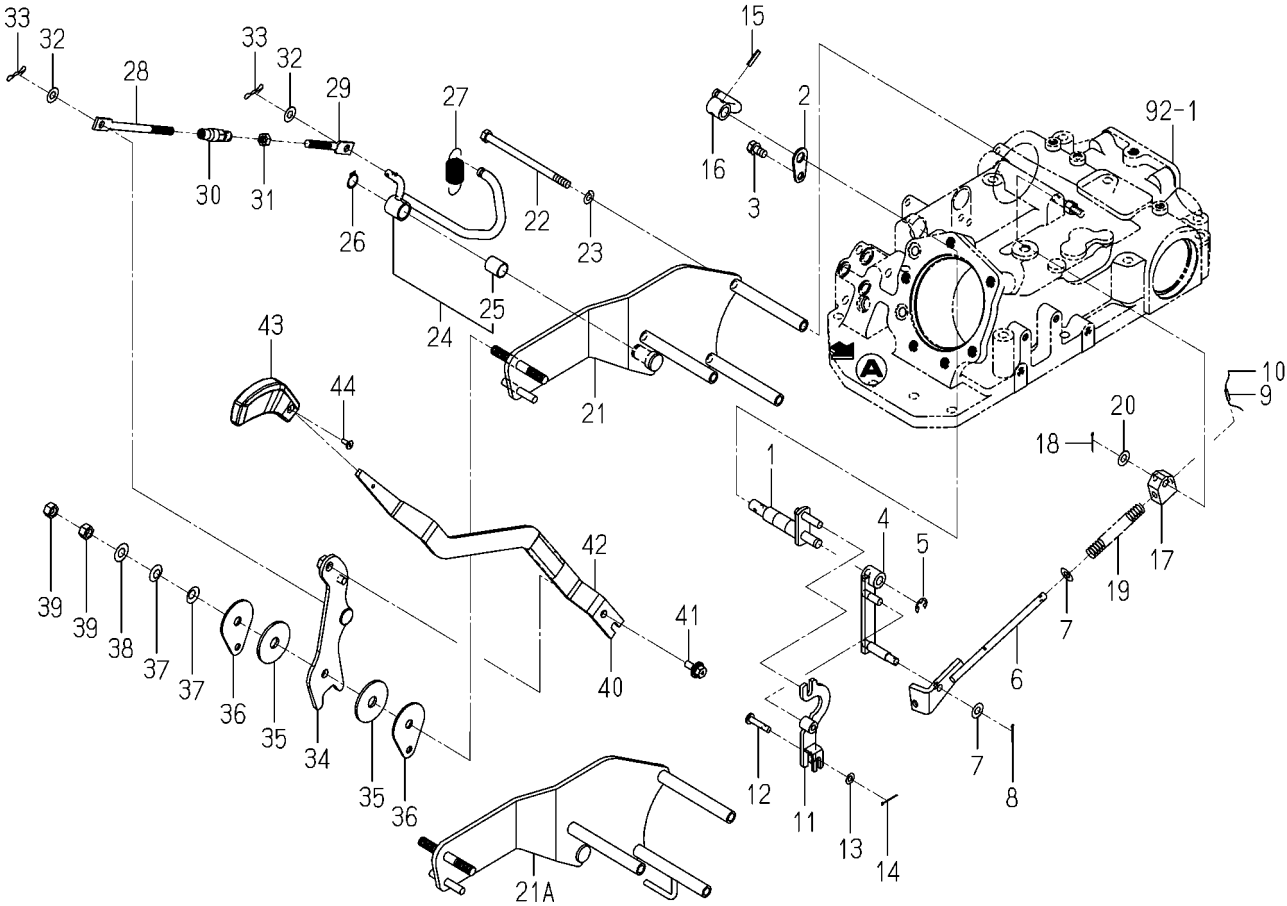
FIG. 94 LEVER(POSITION)SYSTEM(6675 TYPE)
