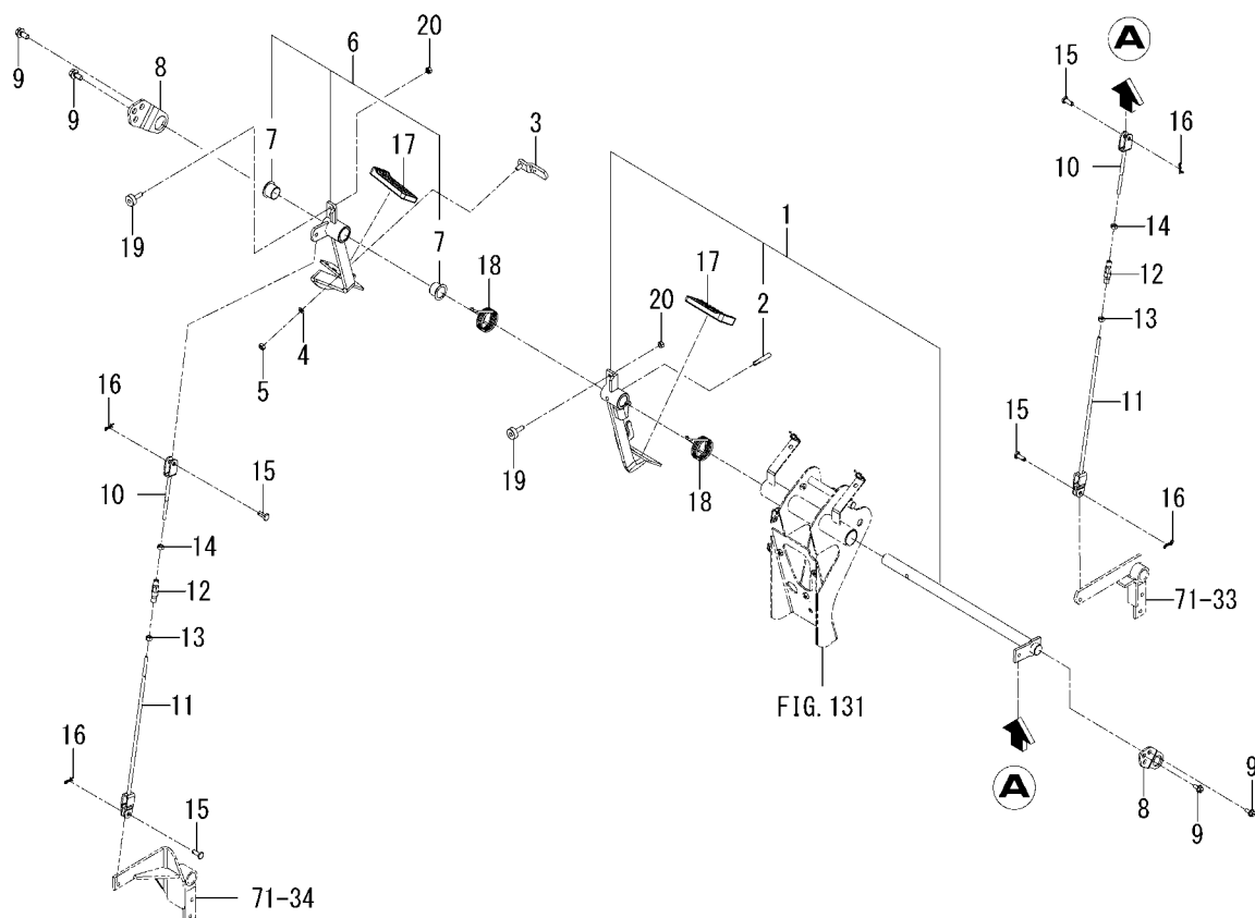
FIG. 72 PEDAL(BRAKE)SYSTEM (6675 TYPE EXCEPT M)
