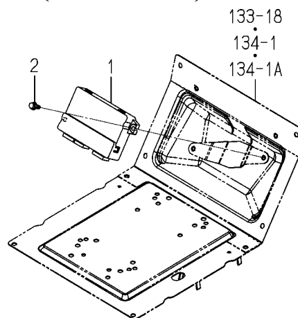
FIG.145 CONTROL SYSTEM(6675 TYPE)
