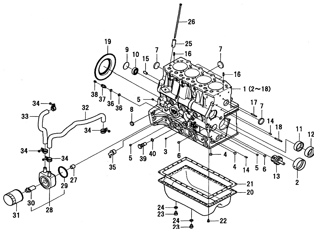
FIG.001 CYLINDER BLOCK/OIL PAN
