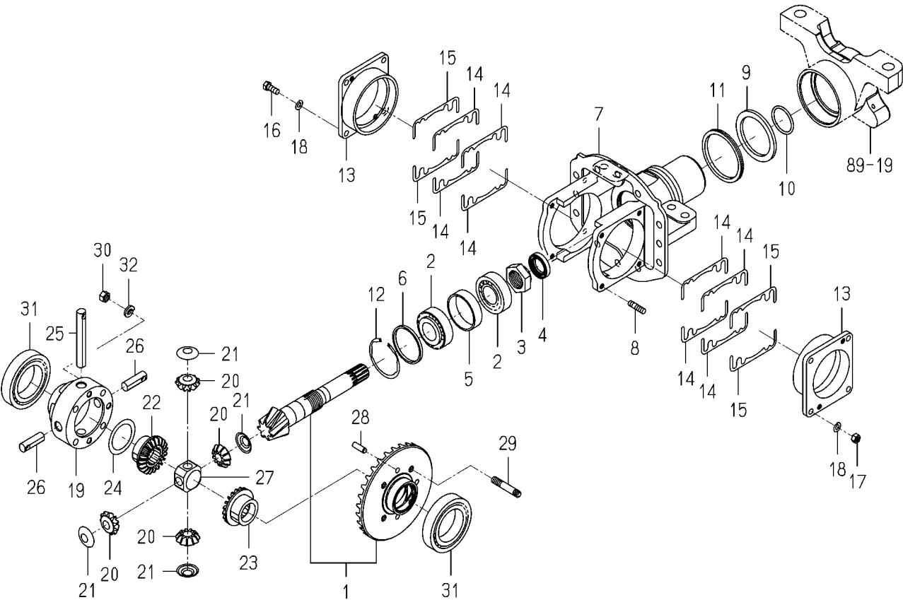
FIG. 88 CASE(DIFFERENTIAL/FRONT)SYSTEM
