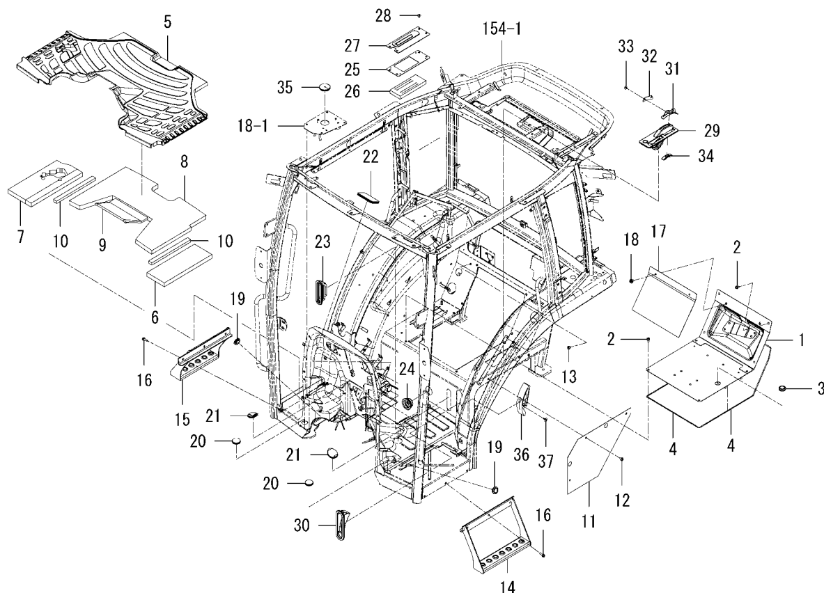
FIG.135 FLOOR(REAR)SYSTEM (6675H,6625H TYPE)
