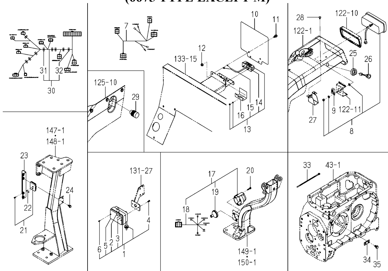
FIG.140 ELC.(FLOOR)SYSTEM (6675 TYPE EXCEPT M)
