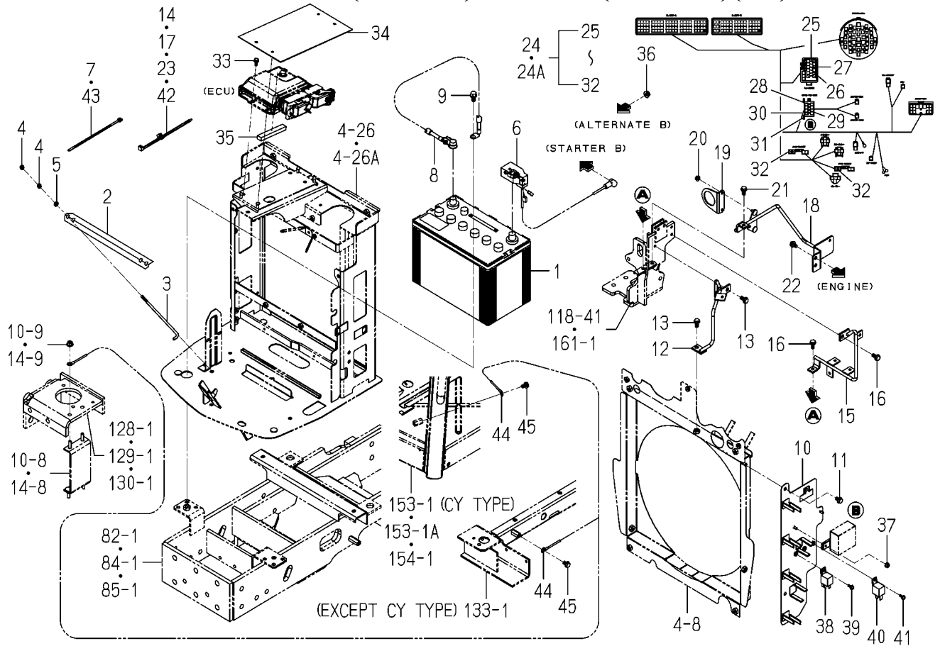
FIG.137 ELC.(FRONT)SYSTEM(G TYPE)(1/2)
