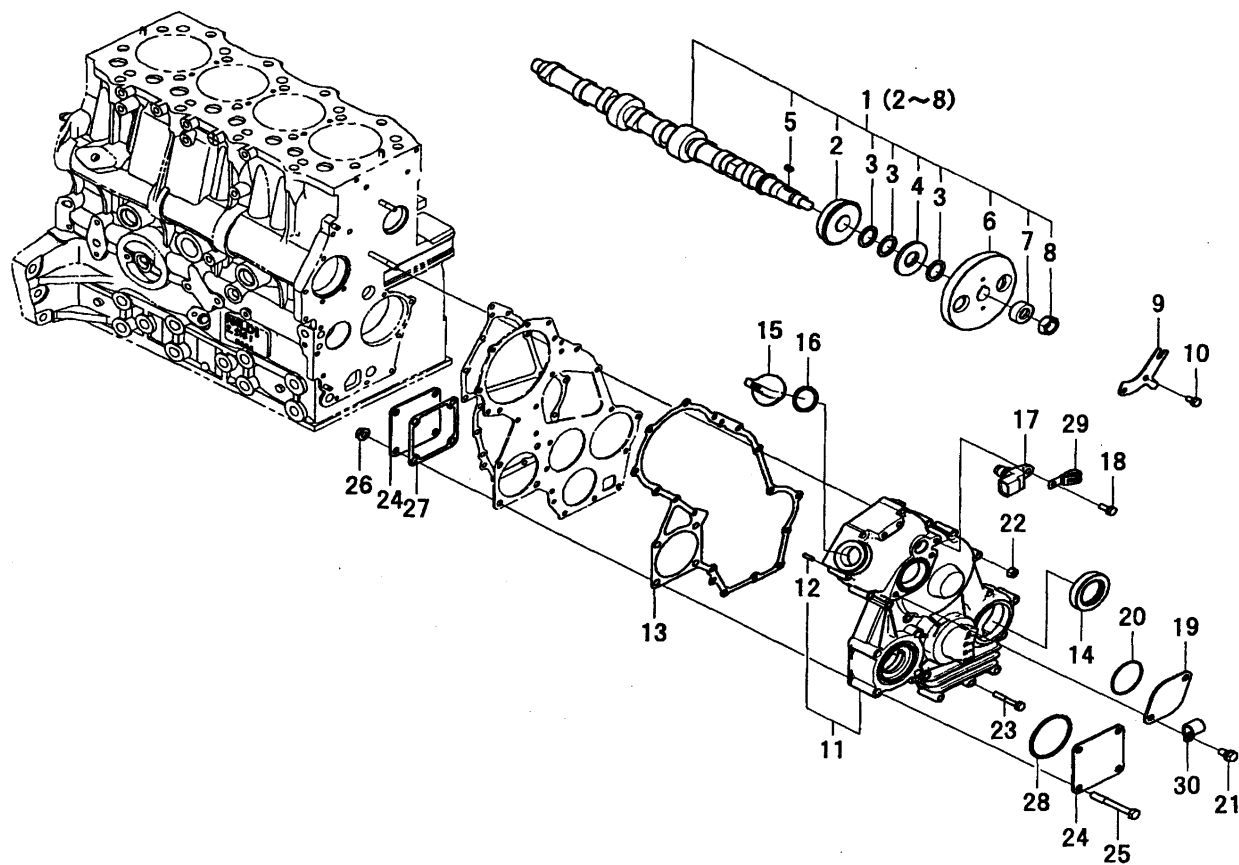
FIG.008 TIMING GEAR CASE/CAMSHAFT
