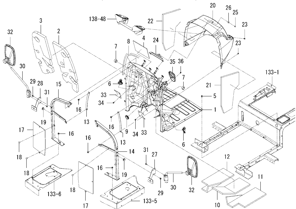
FIG.131 FLOOR(FRONT)SYSTEM (6675 TYPE M TYPE)
