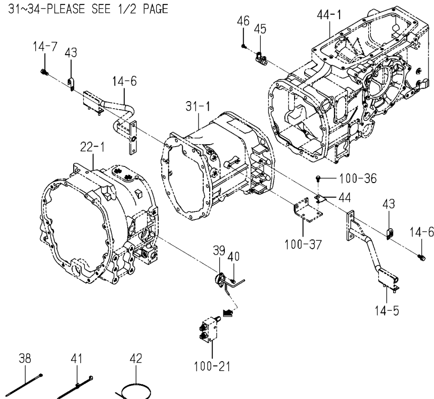
FIG.142 ELC.(FLOOR)SYSTEM(2/2) (6675H,6625H TYPE)
