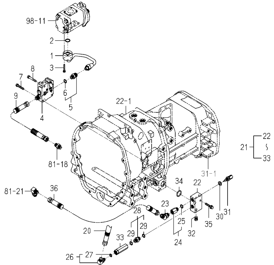
FIG.100 PIPING(SUB)SYSTEM(1/3) (6675H,6625H TYPE)
