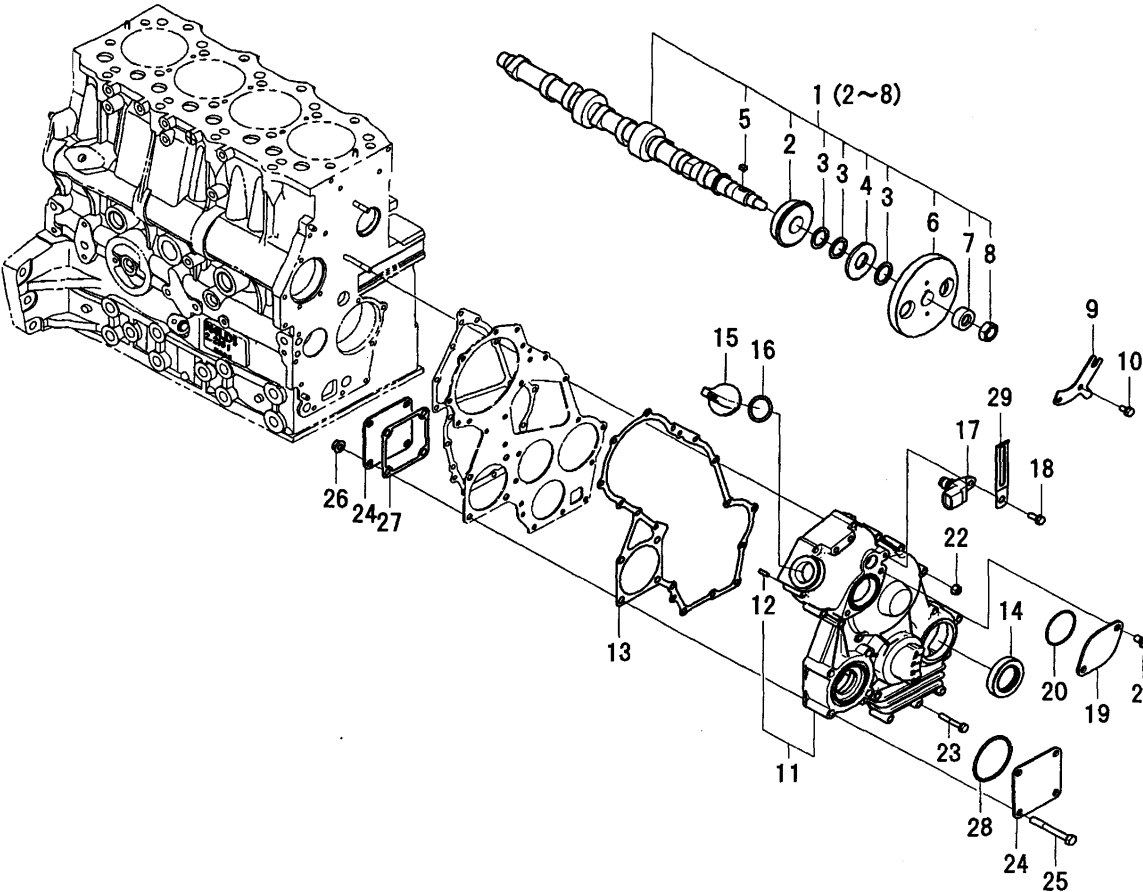
FIG.008 TIMING GEAR CASE/CAMSHAFT
