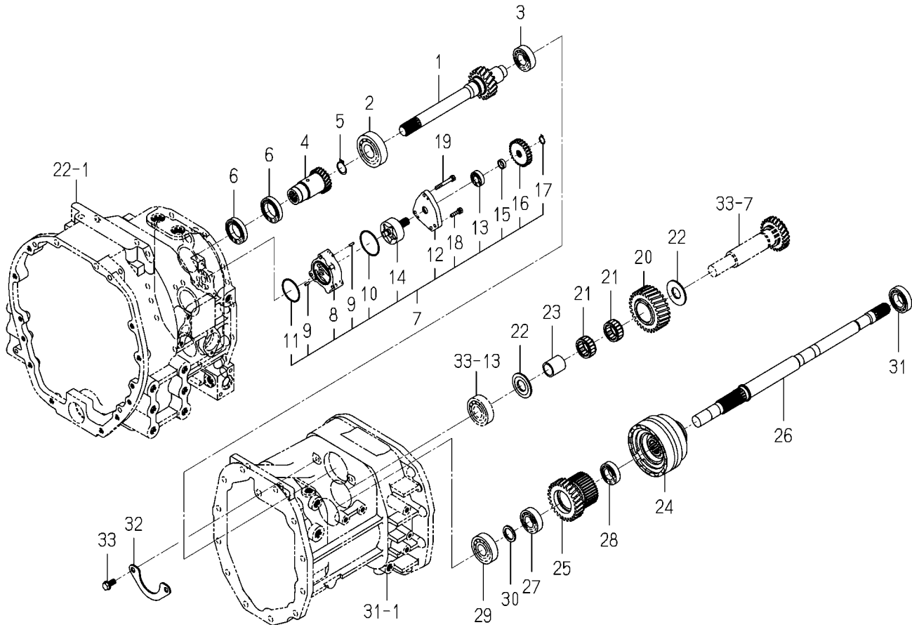
FIG. 29 GEAR(PTO)SYSTEM(6675H,6625H TYPE)
