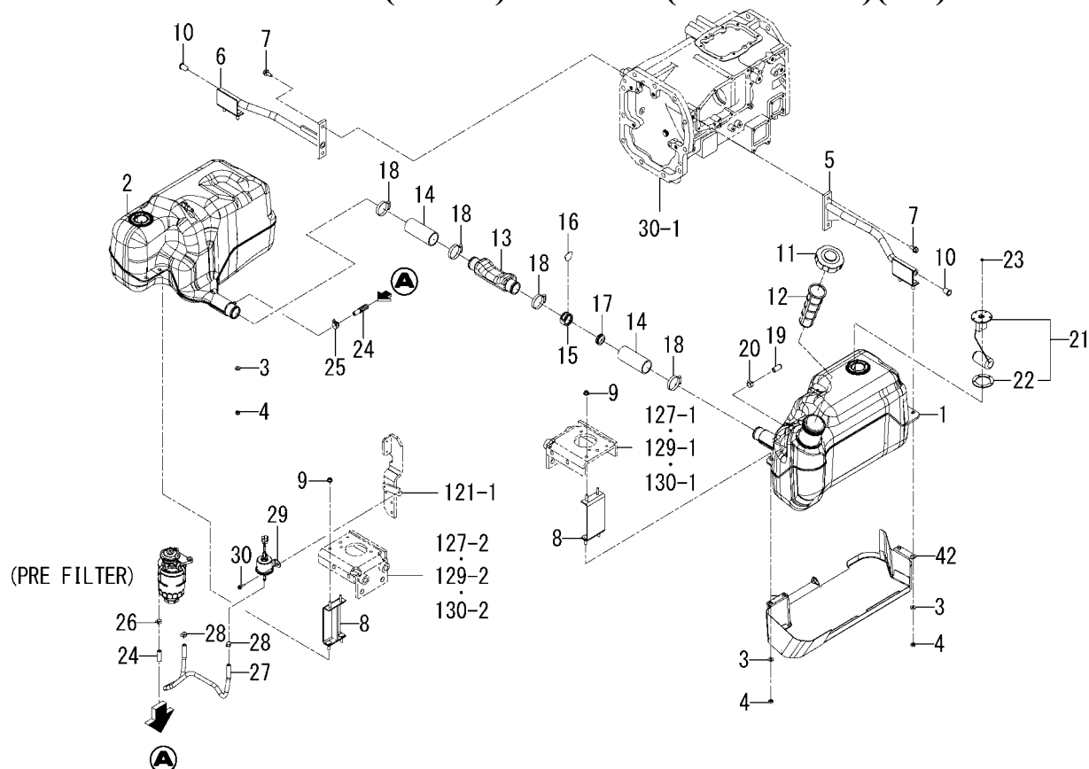
FIG. 10 TANK(FUEL)SYSTEM(6675 TYPE)(1/2)
