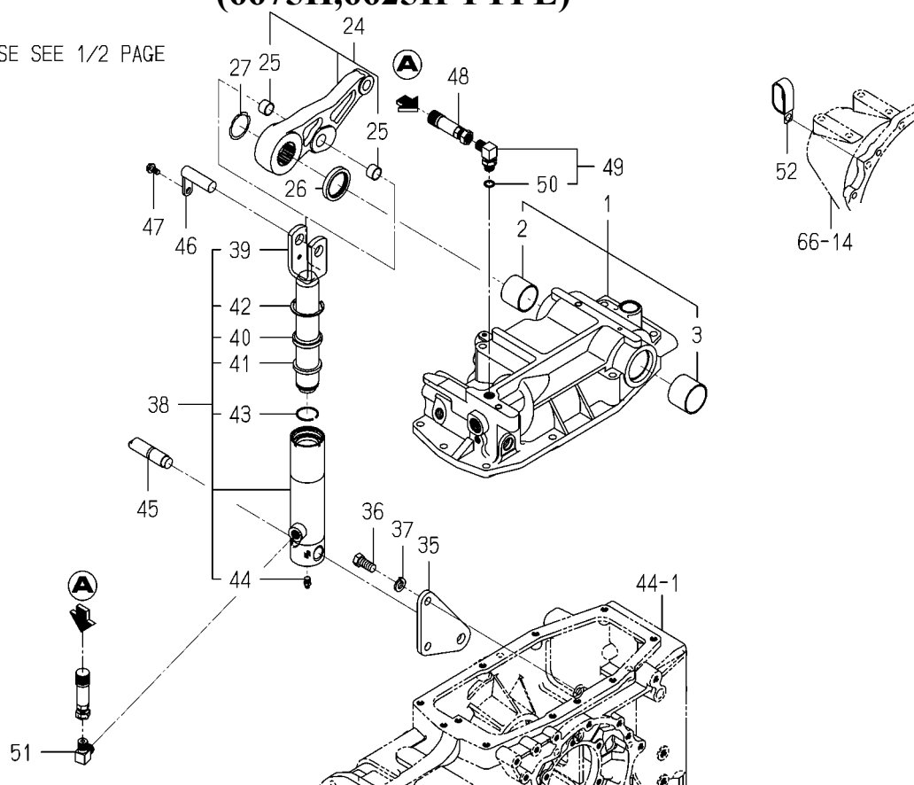
FIG. 93 CASE(CYLINDER)SYSTEM(2/2) (6675H,6625H TYPE)
