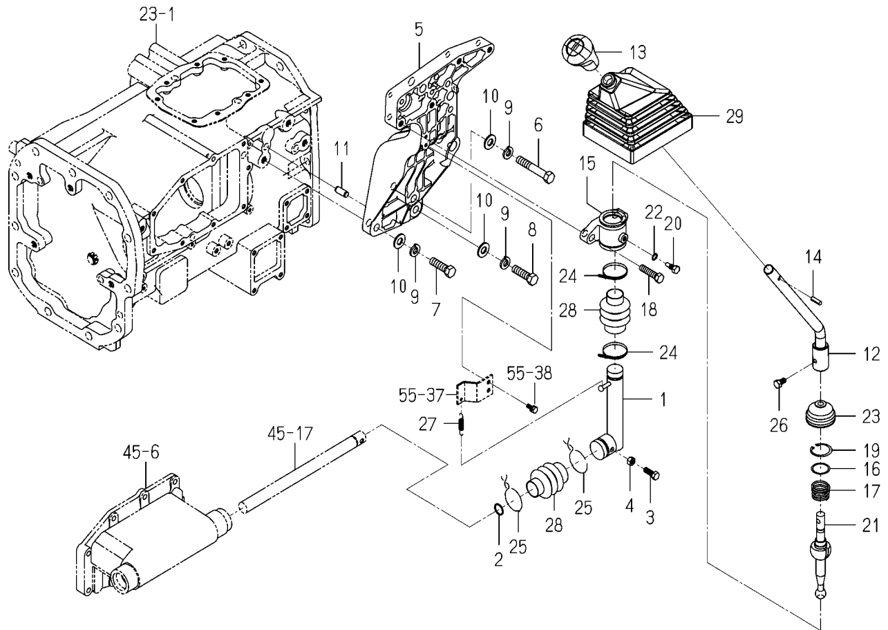
FIG. 54 LEVER(MAIN)SYSTEM(6675 TYPE)
