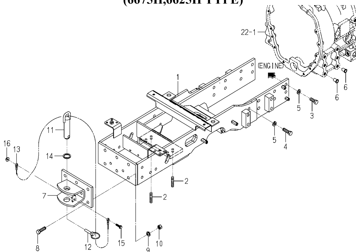
FIG. 85 BRACKET(AXLE)SYSTEM (6675H,6625H TYPE)
