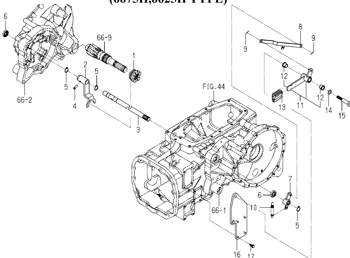
FIG. 69 PEDAL(DIFF-LOCK)SYSTEM (6675H,6625H TYPE)
