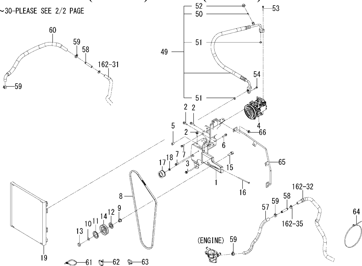
FIG.161 AIR CONDITIONER(1/2) (ENGINE)SYSTEM(M TYPE)
