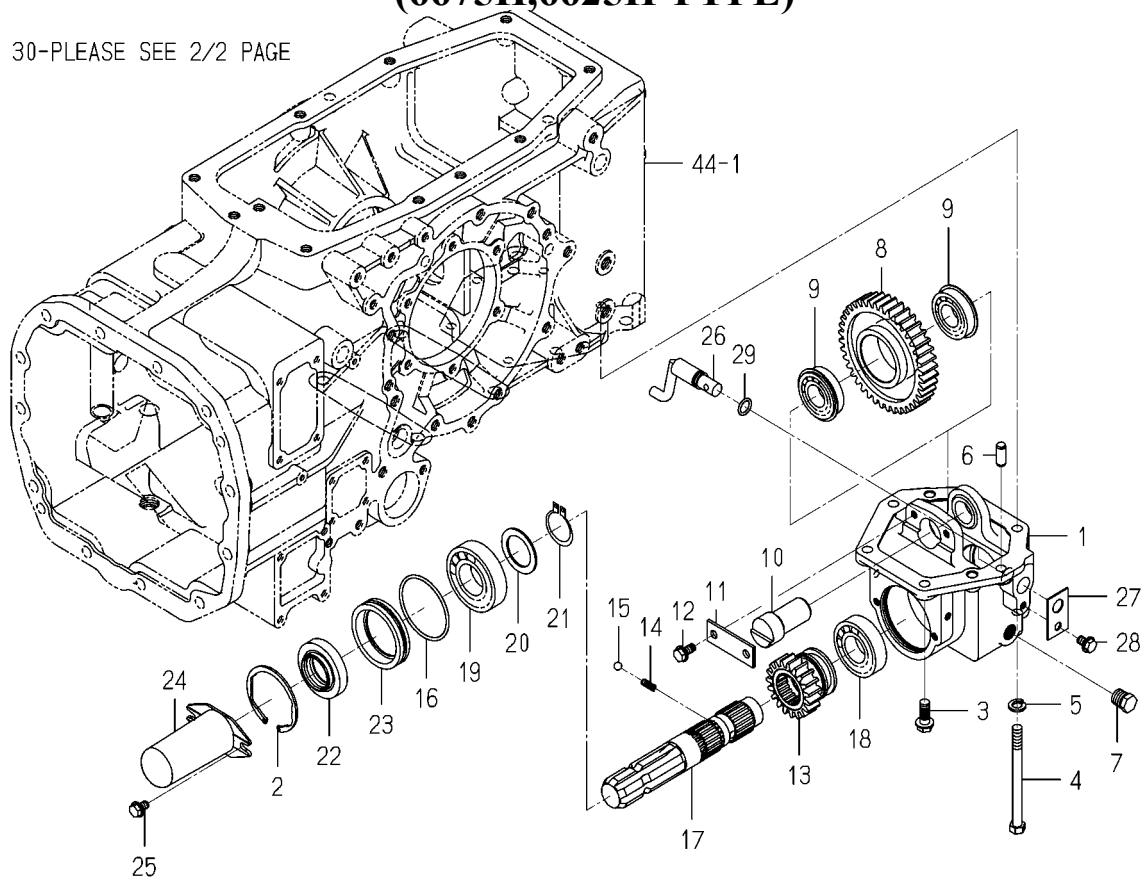
FIG. 42 PTO(MID)SYSTEM(1/2) (6675H,6625H TYPE)
