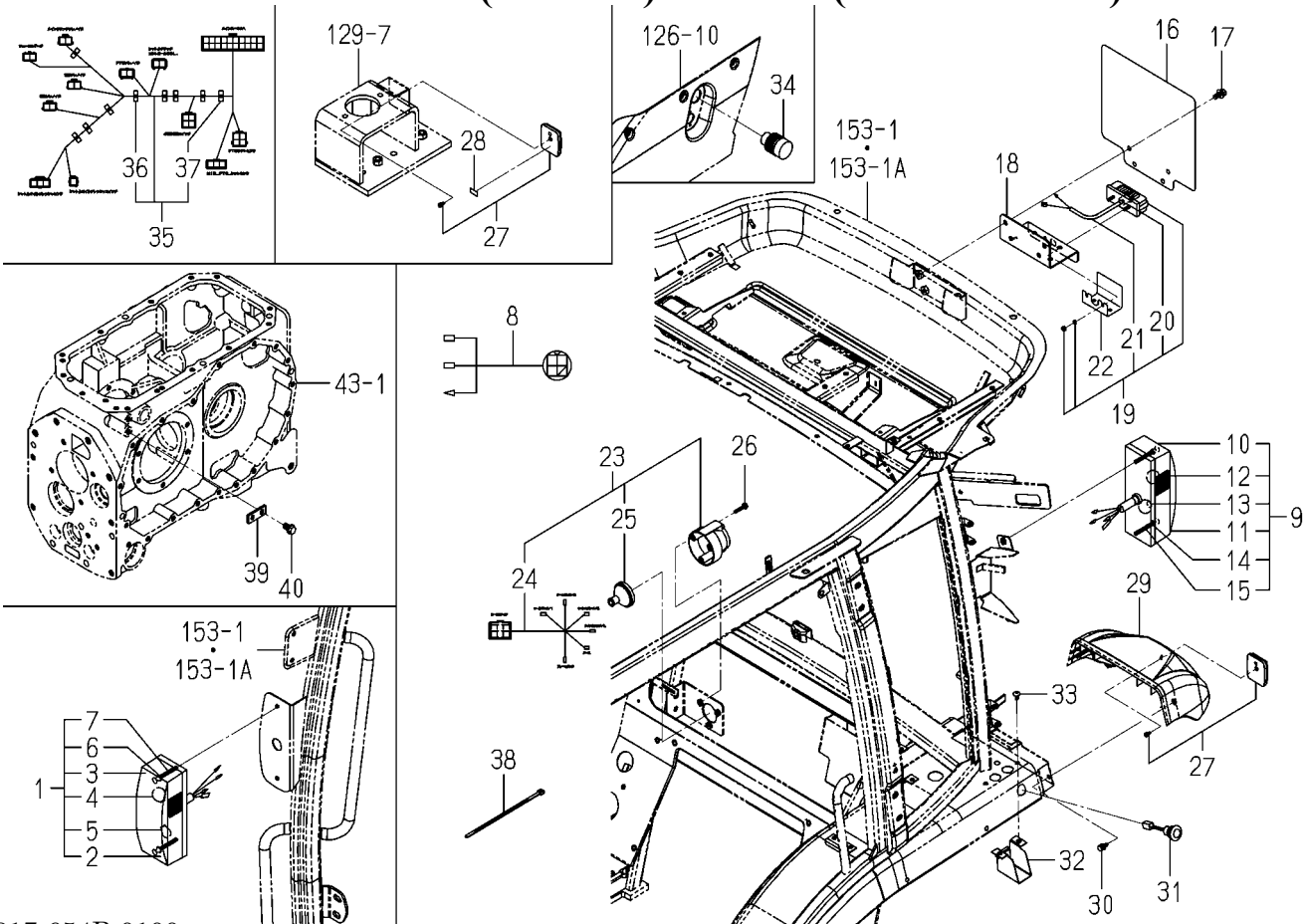
FIG.141 ELC.(FLOOR)SYSTEM(6675-M TYPE)
