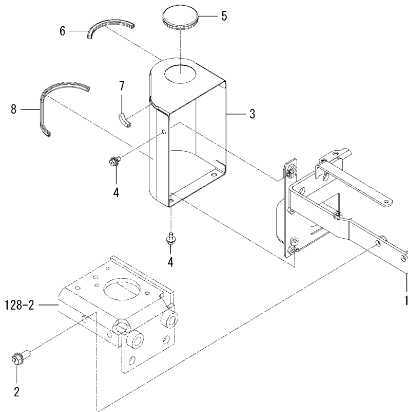
FIG. 15 BRACKET(FILTER)SYSTEM (6675H,6625H TYPE)
