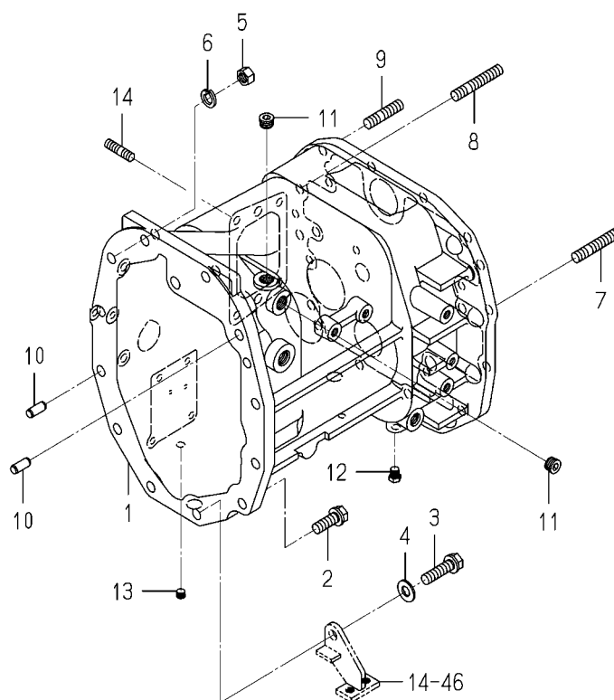
FIG. 31 CASE(TRANSMISSION)SYSTEM (6675H,6625H TYPE)
