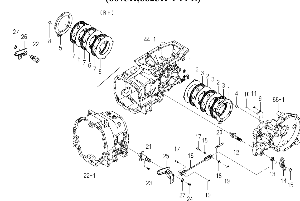
FIG. 70 LEVER(BRAKE/PARKING)SYSTEM (6675H,6625H TYPE)
