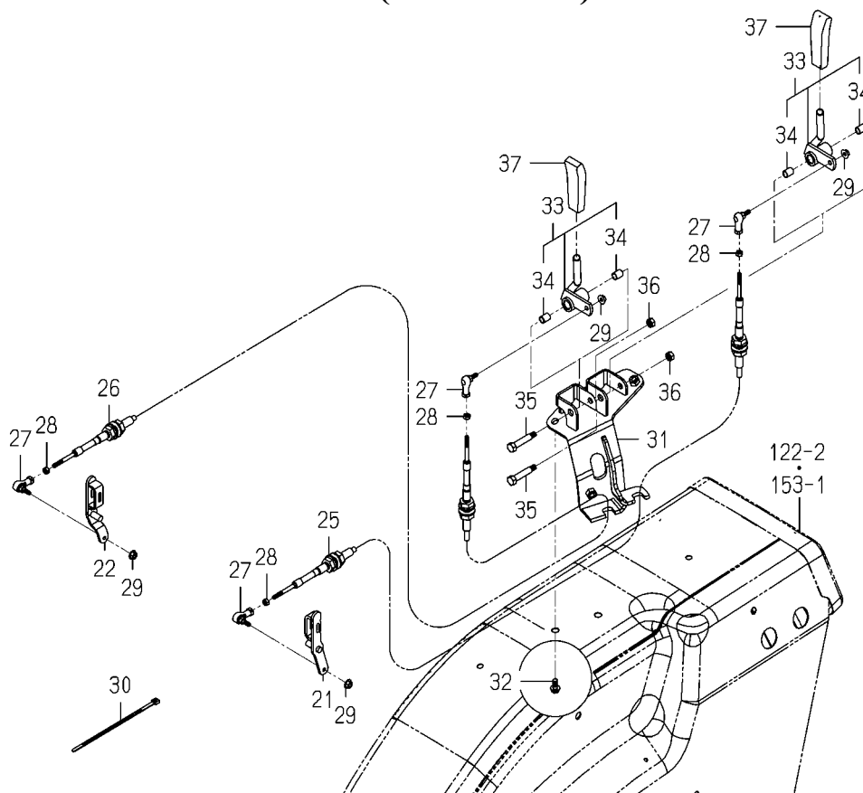
FIG.107 VALVE(REMOTE/2R)SET SYSTEM(2/2) (6675 TYPE)
