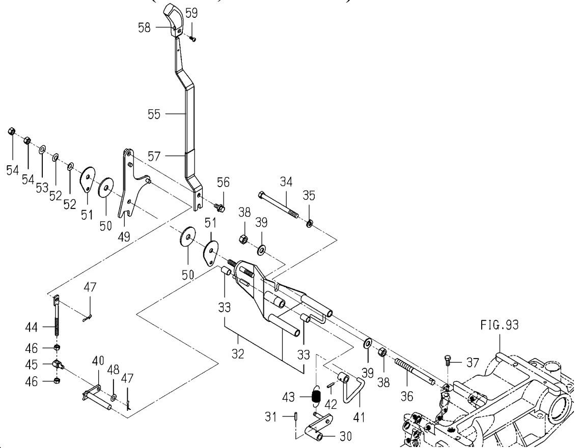
FIG. 95 LEVER(POSITION)SYSTEM(2/2) (6675H,6625H TYPE)
