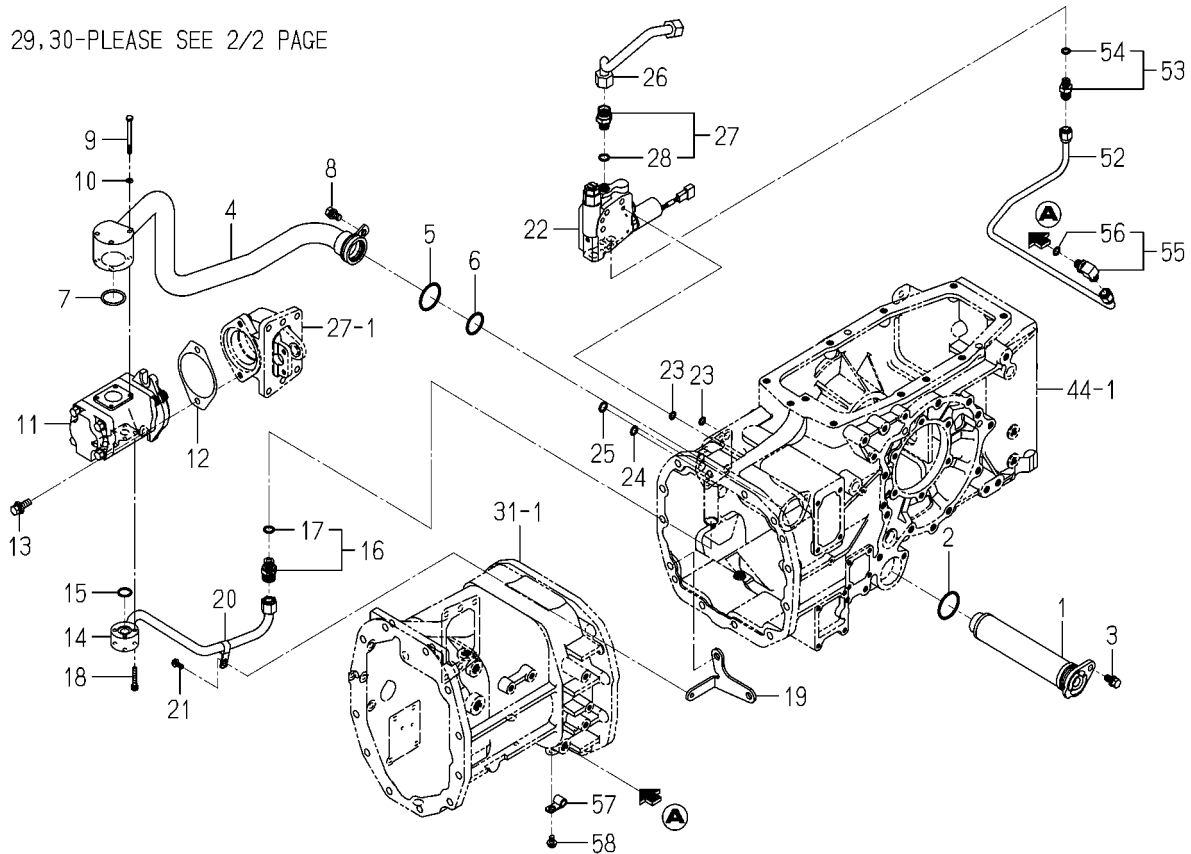
FIG. 98 PIPING(MAIN)SYSTEM(1/2) (6675H,6625H TYPE)
