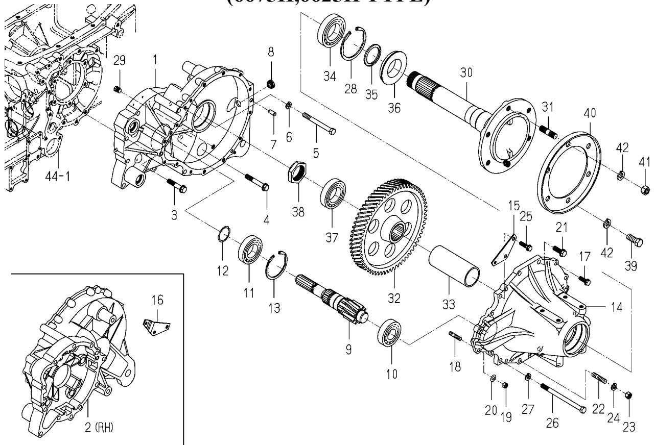
FIG. 66 HOUSING(AXLE/REAR)SYSTEM (6675H,6625H TYPE)
