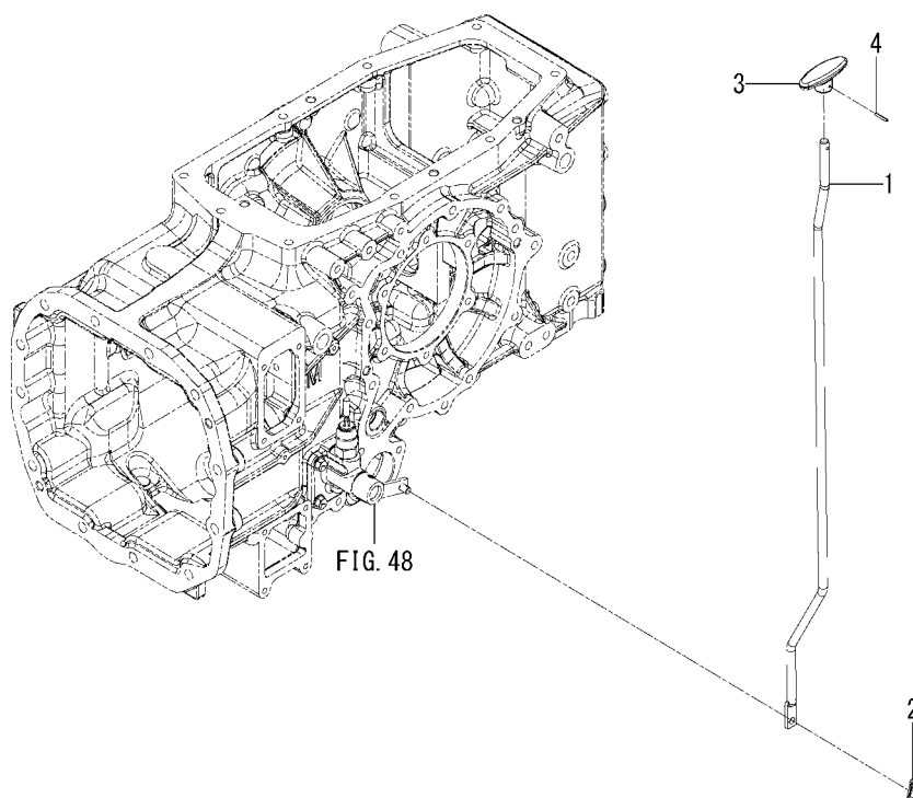
FIG. 57 LEVER(4WD)SYSTEM (6675H,6625H TYPE)
