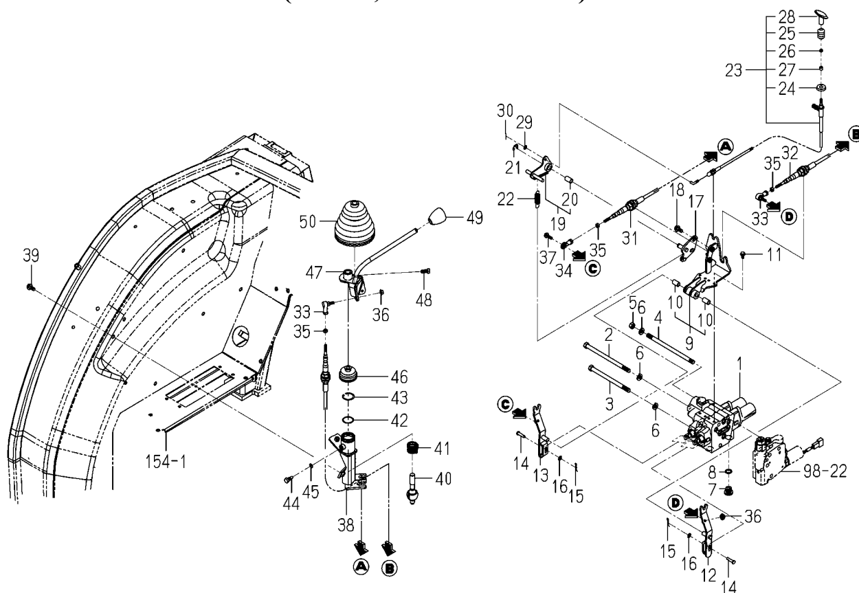
FIG.101 JOY STICK SYSTEM (6675H,6625H-D TYPE)
