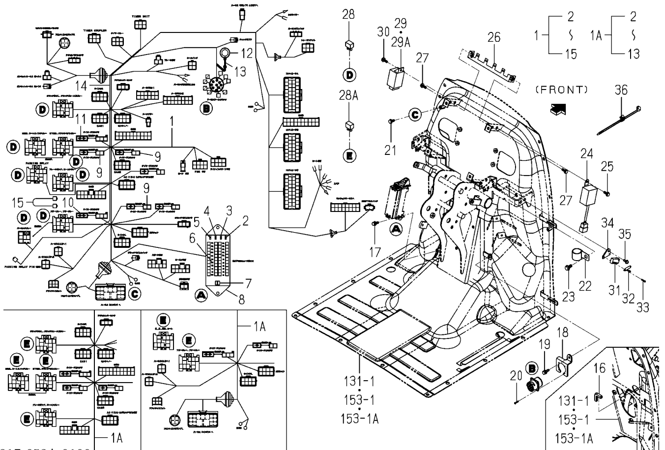
FIG.138 ELC.(MAIN)SYSTEM(6675 TYPE)(1/2)
