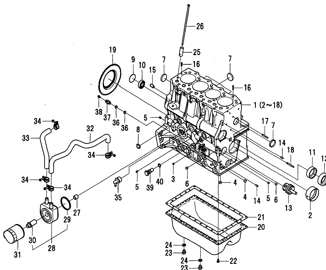
FIG.001 CYLINDER BLOCK/OIL PAN
