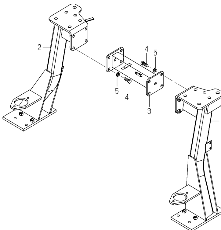
FIG.147 FRAME(REAR)SYSTEM (6675 TYPE EXCEPT M,A)
