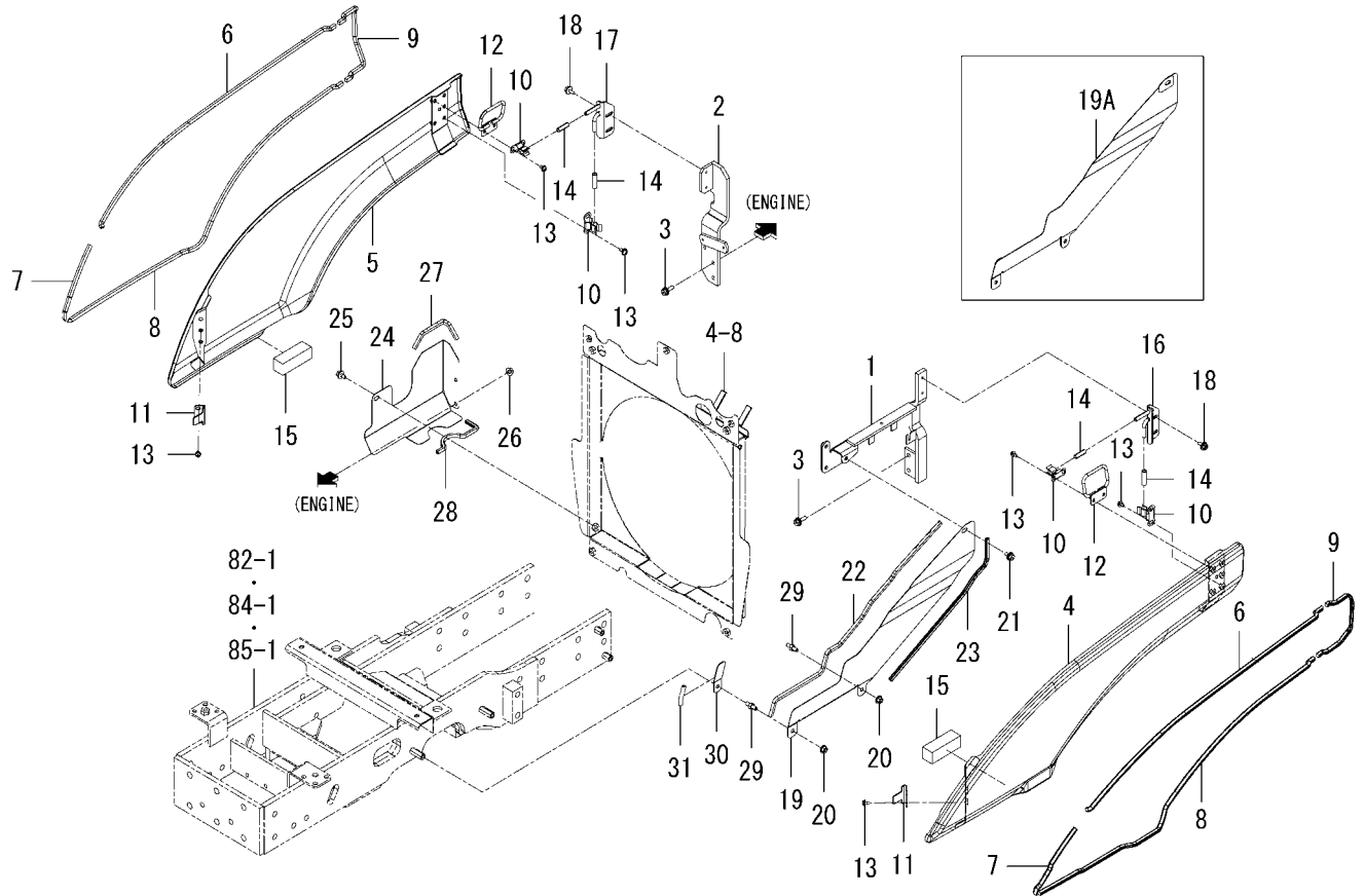
FIG.121 COVER(SIDE)SYSTEM
