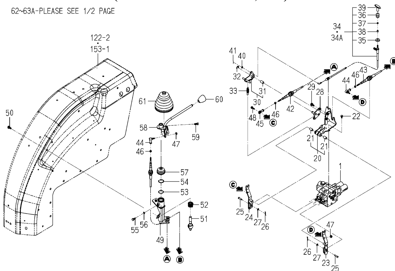
FIG.102 JOY STICK SYSTEM(2/2) (6675 TYPE EXCEPT D,JRA)
