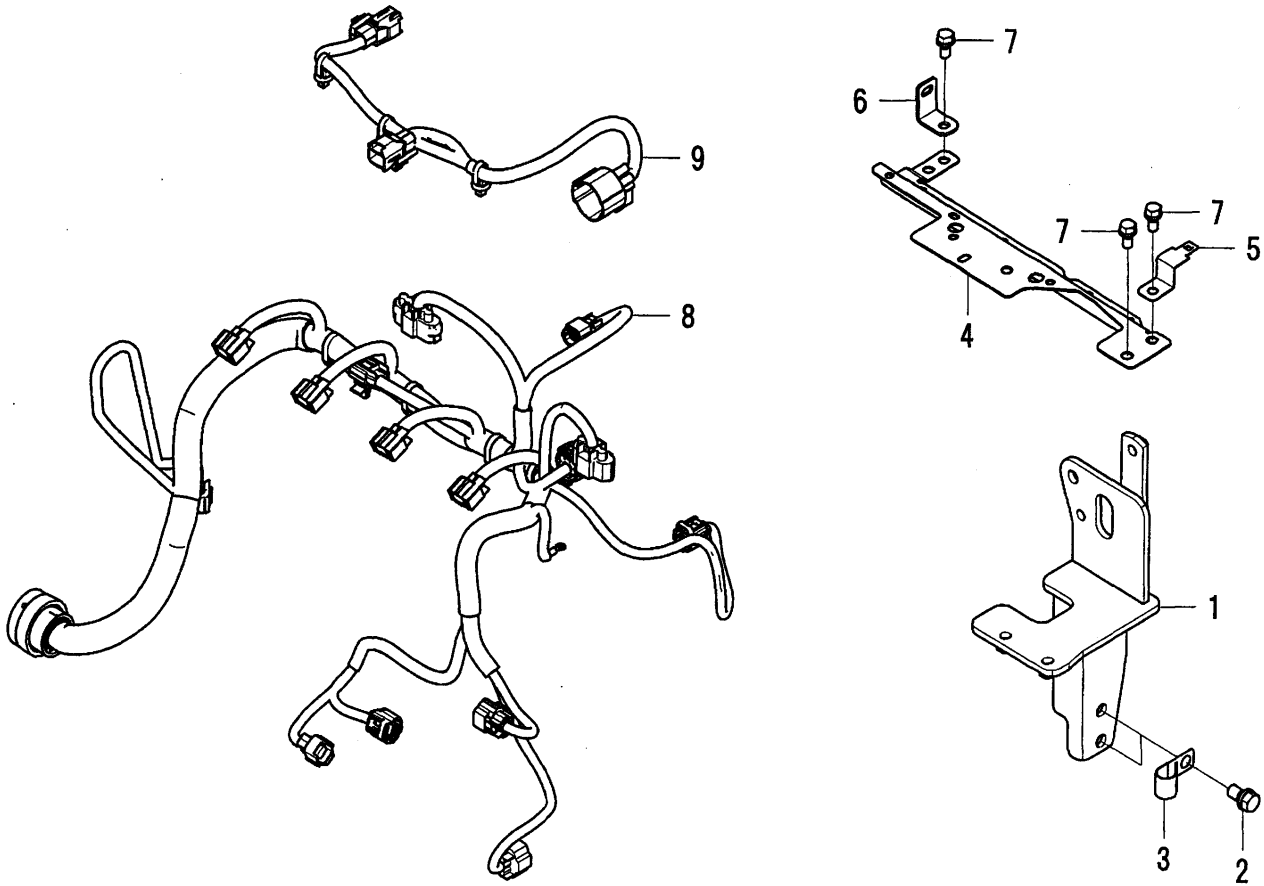
FIG.013 HARNESS WIRE
