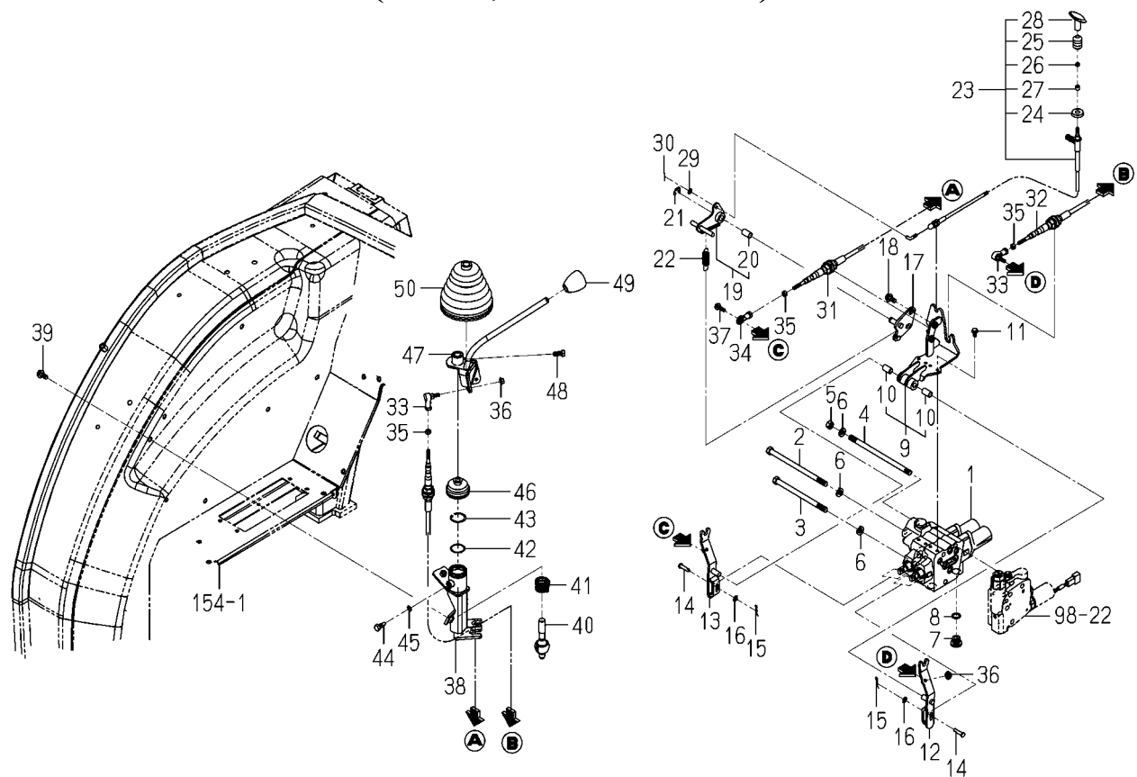
FIG.101 JOY STICK SYSTEM (6675H,6625H-D TYPE)
