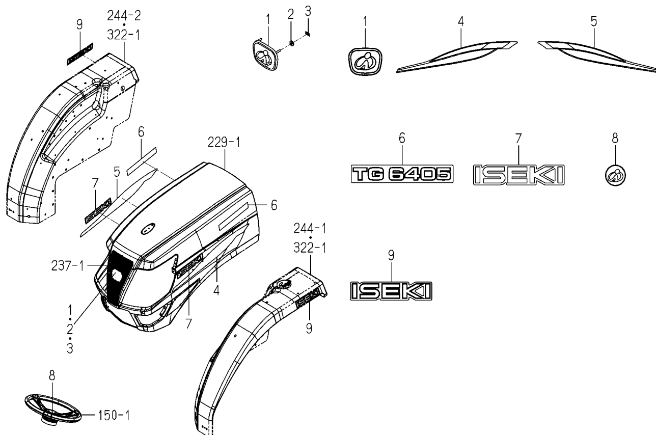
FIG.337 ORNAMENT(6405H TYPE)
