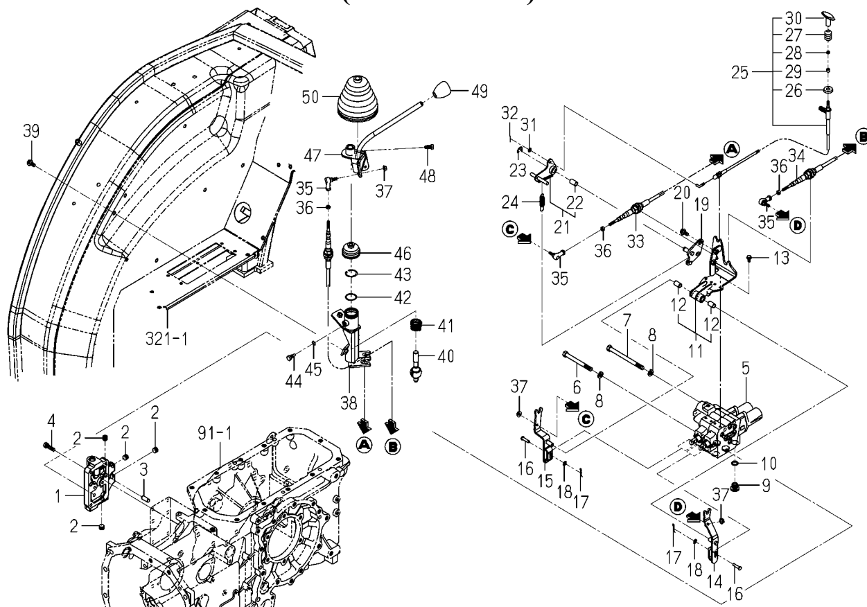
FIG.202 JOY STICK VALVE SYSTEM (6495-D TYPE)
