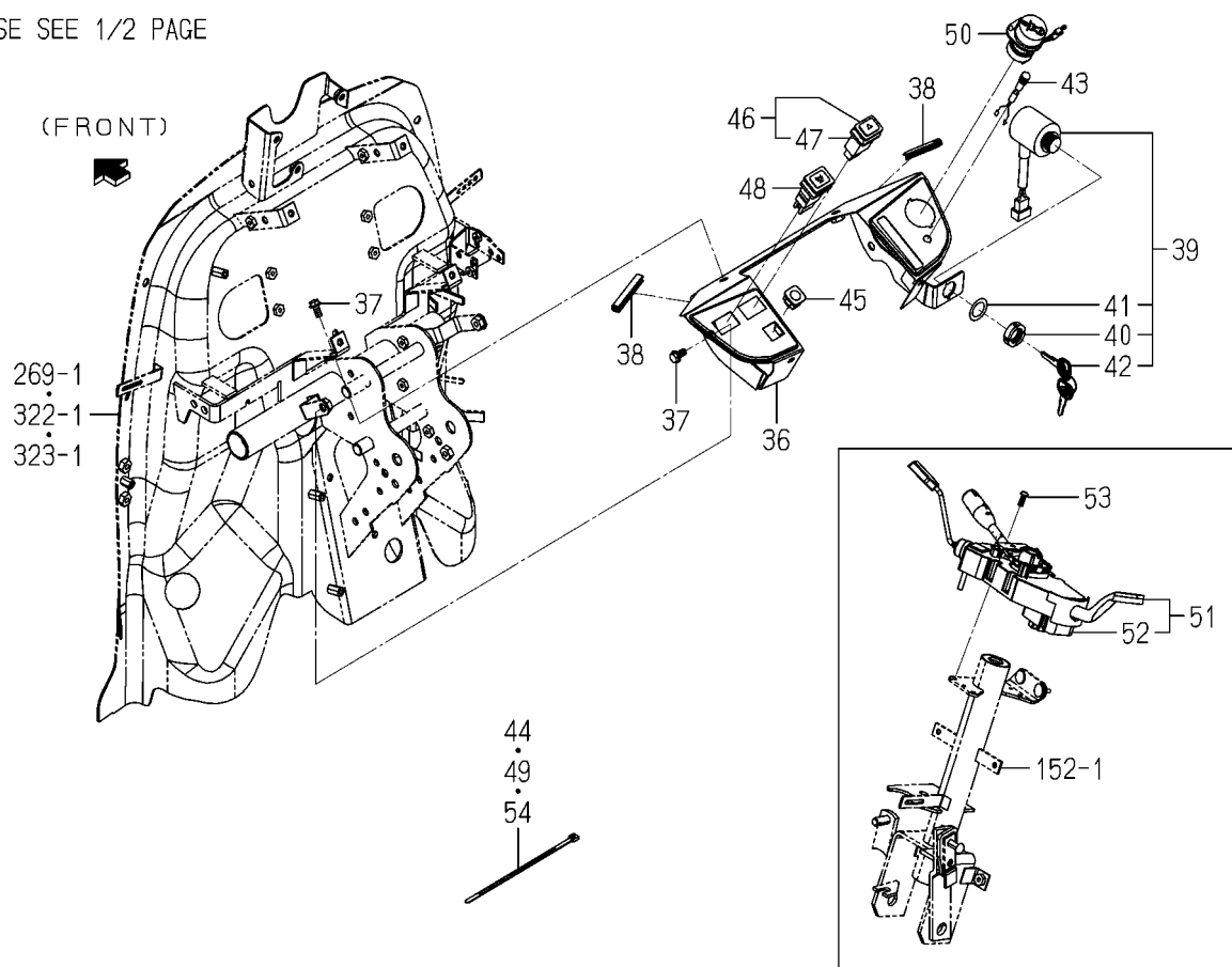
FIG.291 ELC.(MAIN)SYSTEM(H TYPE)(2/2)
