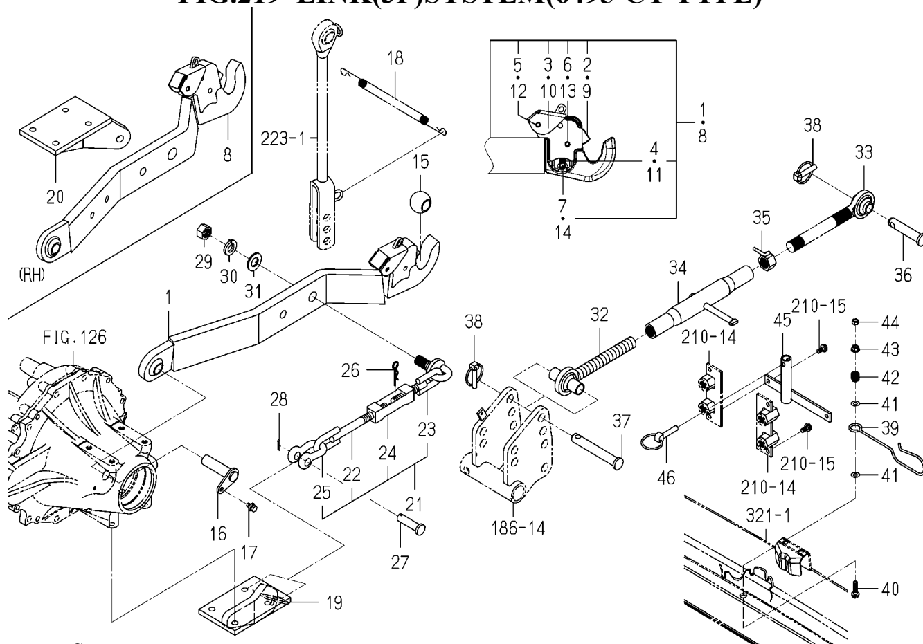
FIG.219 LINK(3P)SYSTEM(6495-CY TYPE)
