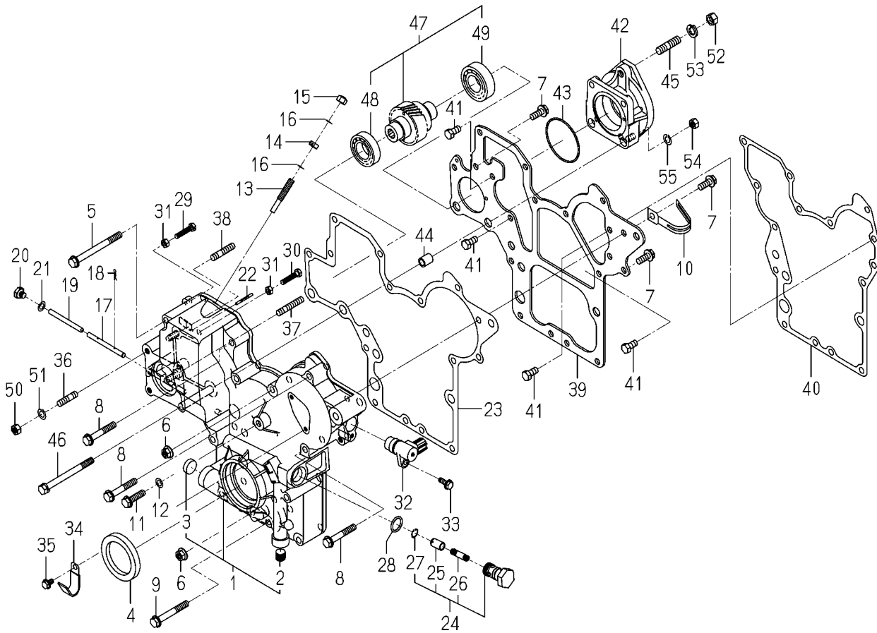
FIG. 17 TIMING GEAR CASE
