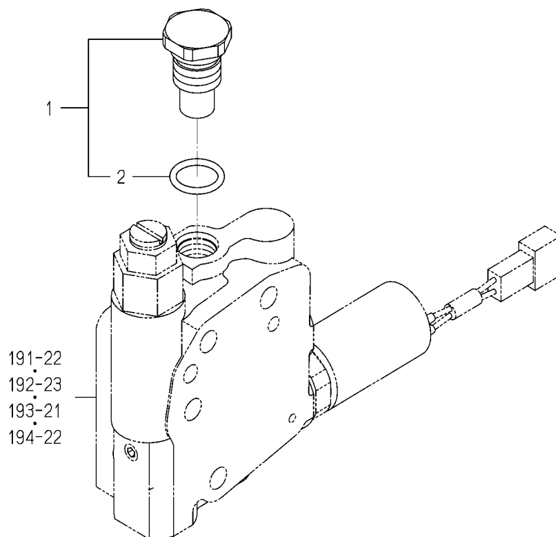
FIG.366 PLUG(M18)ASSY(SD,H TYPE)(OPTION)
