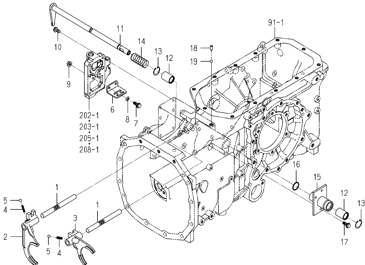
FIG. 98 FORK(SHIFT/SUB)SYSTEM(G TYPE)
