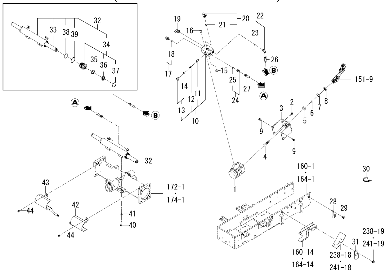
FIG.154 STEERING(POWER)SYSTEM (6375-G TYPE/6405H TYPE)
