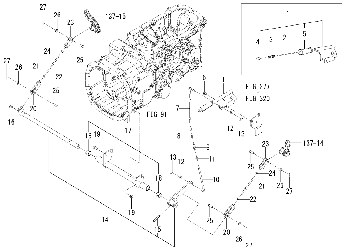
FIG.147 LEVER(BRAKE/PARKING)SYSTEM (6375-G TYPE)
