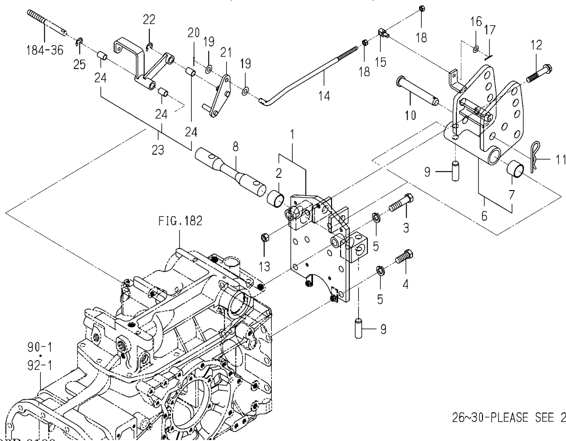
FIG.188 LEVER(DRAFT)SYSTEM(1/2) (6495-SD TYPE)
