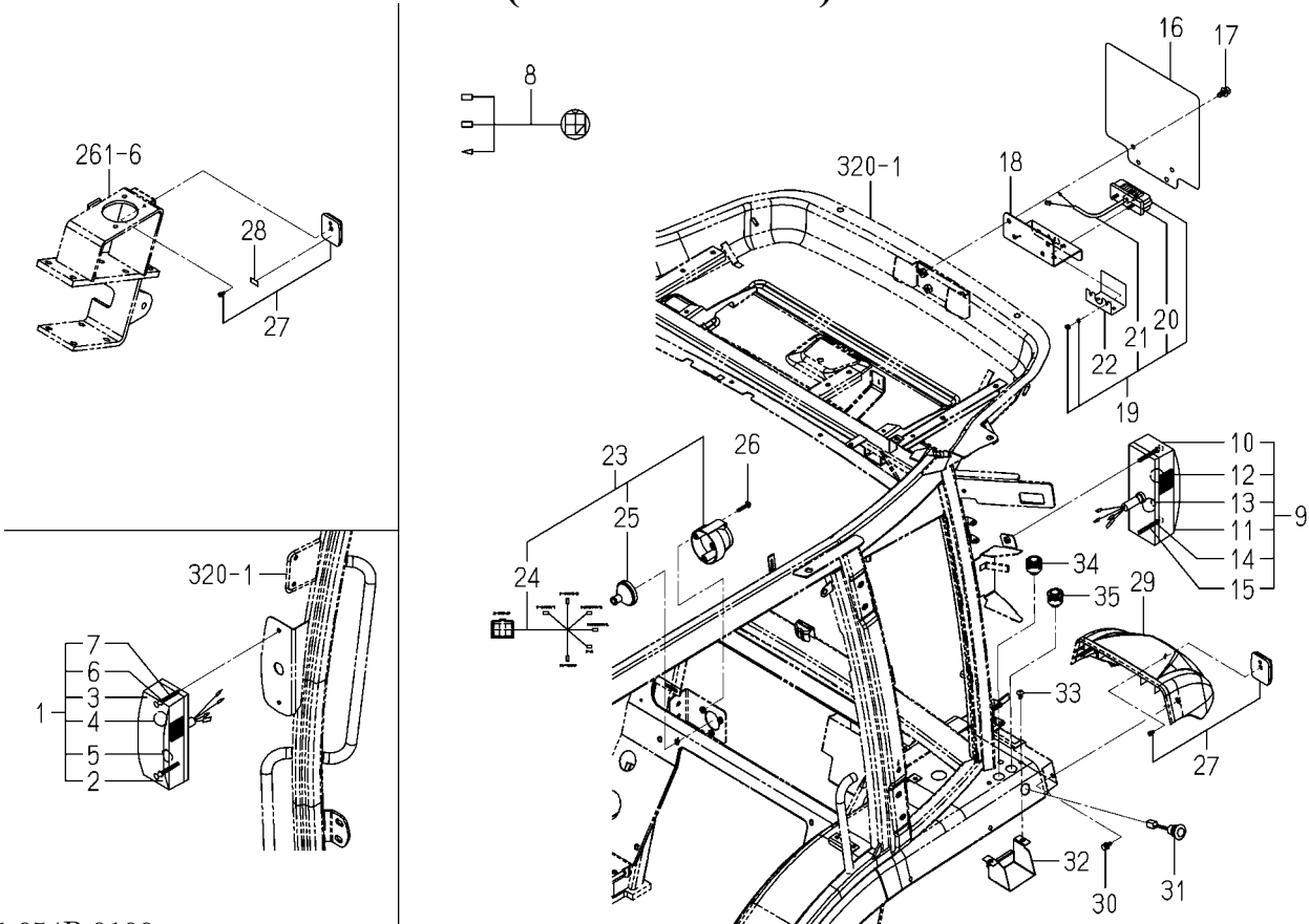
FIG.301 ELC.(FLOOR)SYSTEM(1/2) (6375-CY TYPE)
