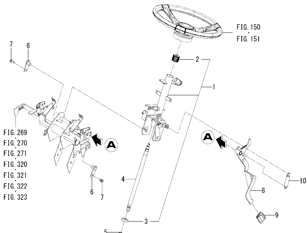
FIG.152 COLUMN(STEERING)SYSTEM (G,H TYPE)
