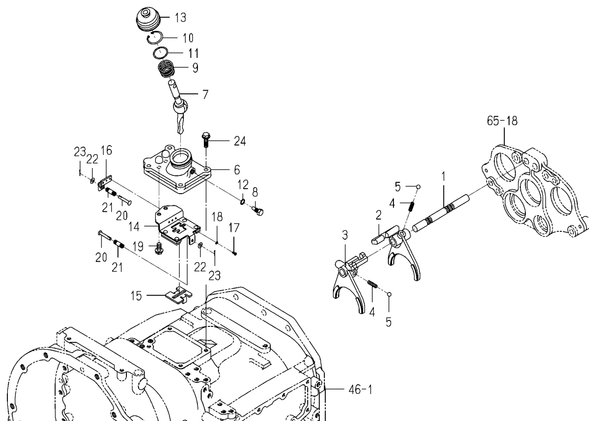
FIG.101 FORK(SHIFT/PTO)SYSTEM (6375-G TYPE)
