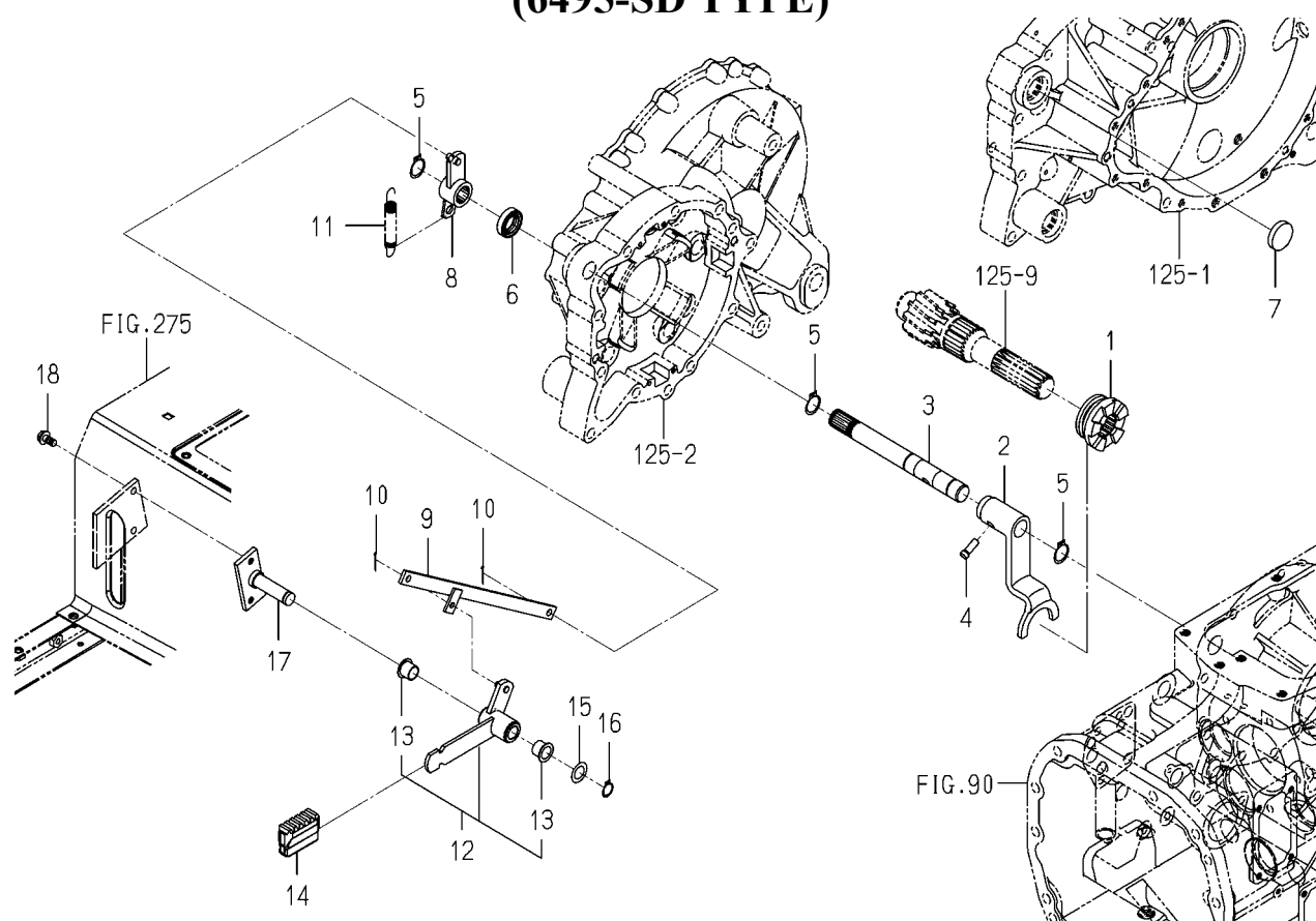
FIG.128 CLUTCH(DIFF-LOCK)SYSTEM (6495-SD TYPE)
