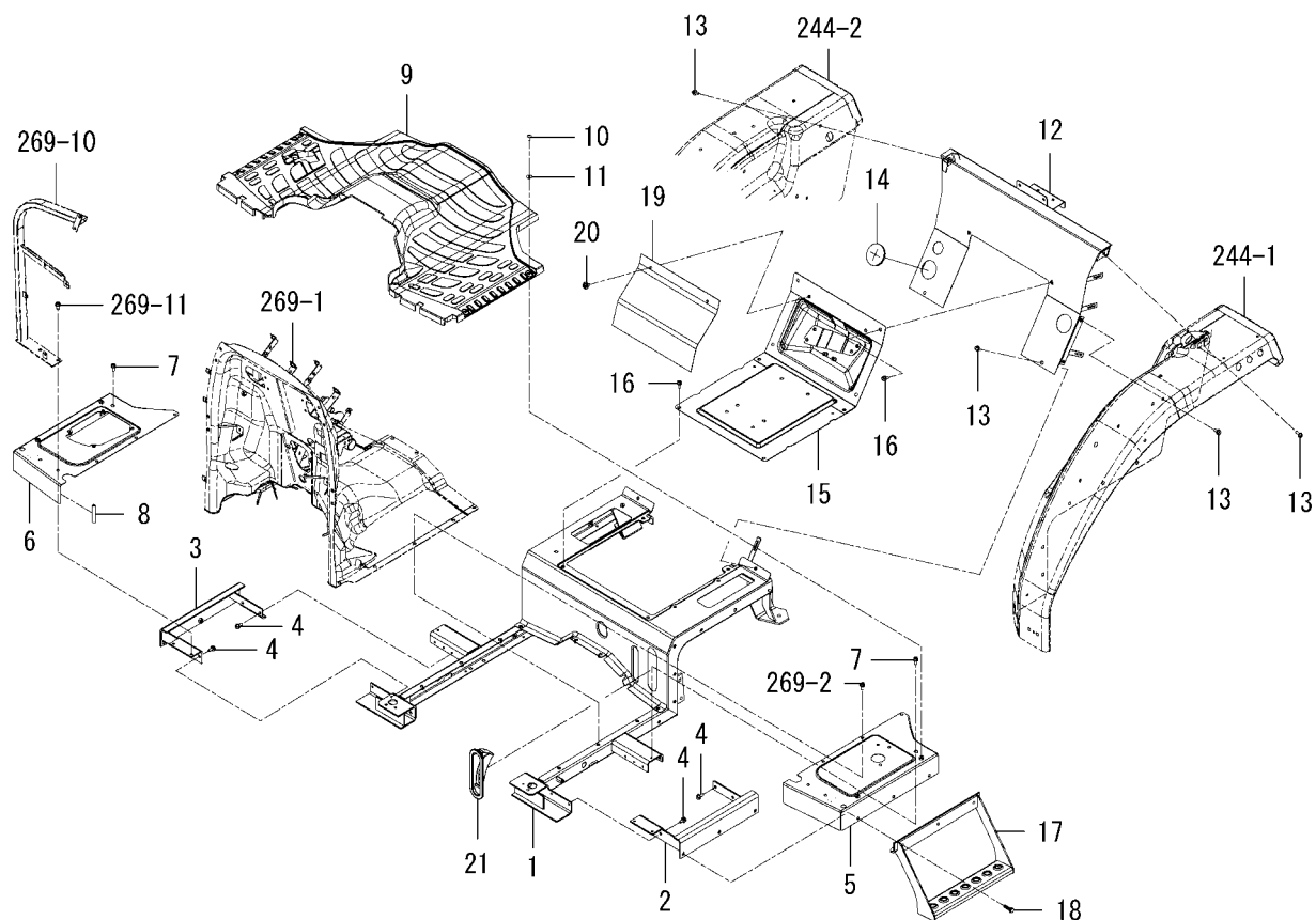
FIG.276 FLOOR(REAR)SYSTEM(6405H-R TYPE)
