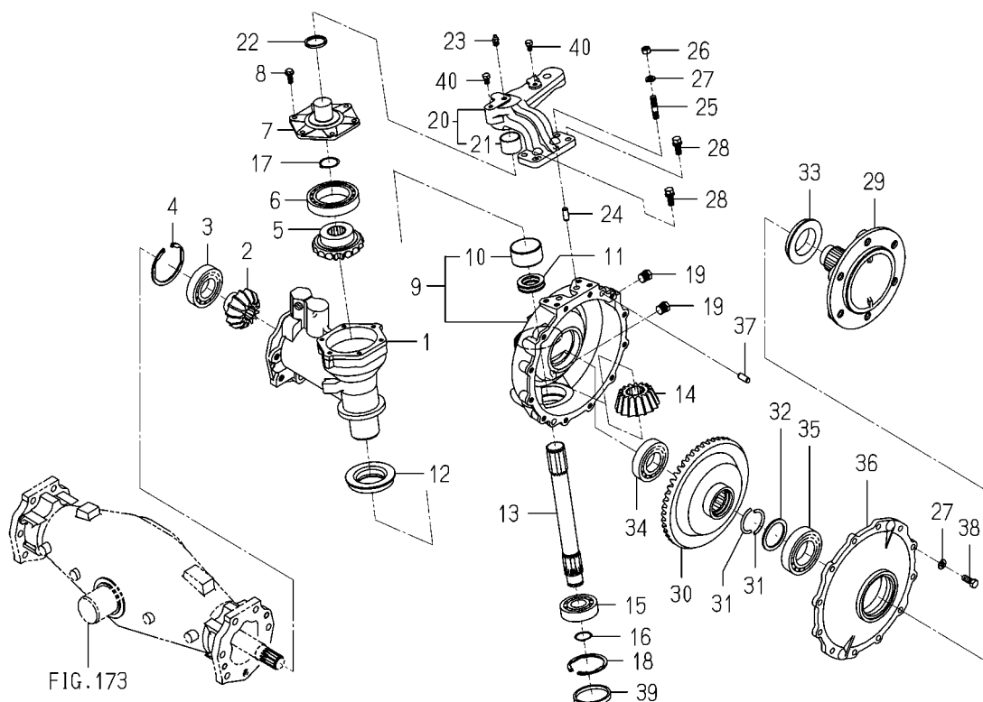
FIG.175 CASE(GEAR/FRONT)SYSTEM(1/2) (6495 TYPE/6495H TYPE)
