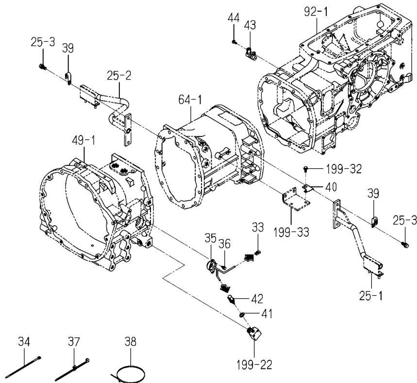
FIG.297 ELC.(FLOOR)SYSTEM(2/2) (6495H-R TYPE)
