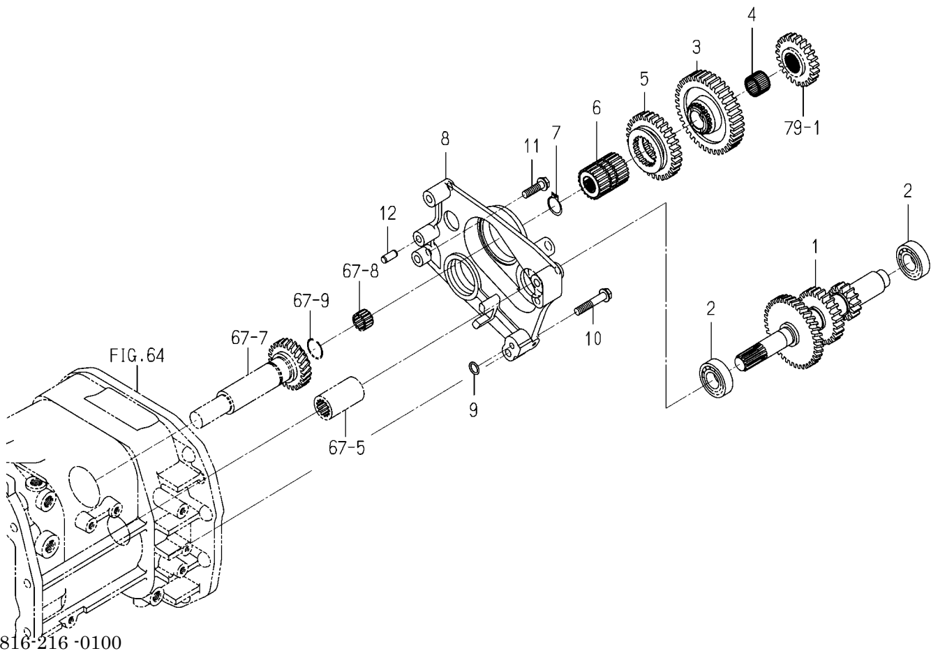
FIG. 74 GEAR(SUB)SYSTEM(6495-H TYPE)
