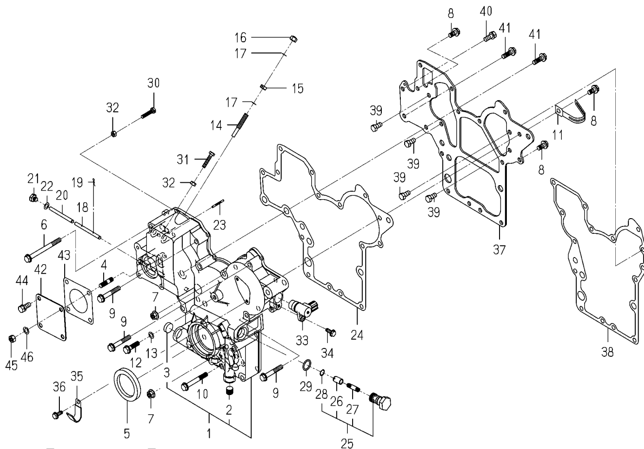
FIG. 14 TIMING GEAR CASE
