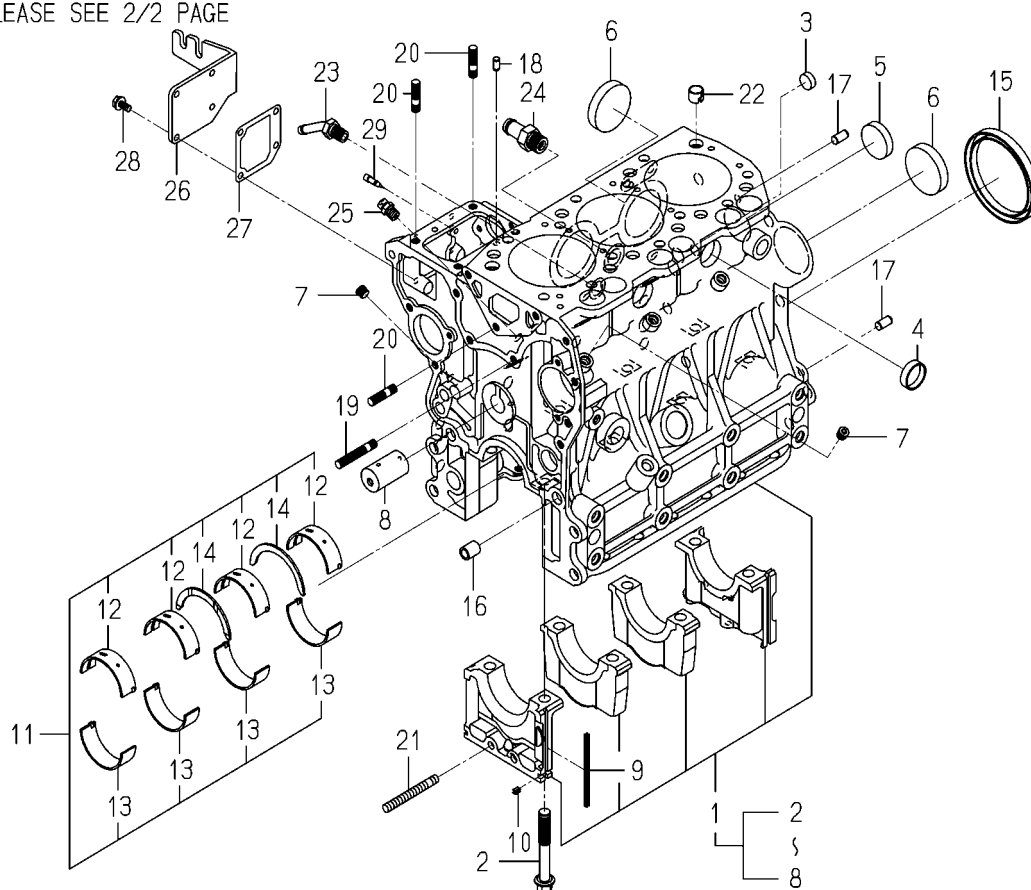
FIG. 7 CYLINDER BLOCK(1/2)
