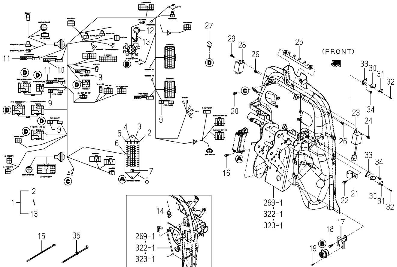
FIG.291 ELC.(MAIN)SYSTEM(H TYPE)(1/2)
