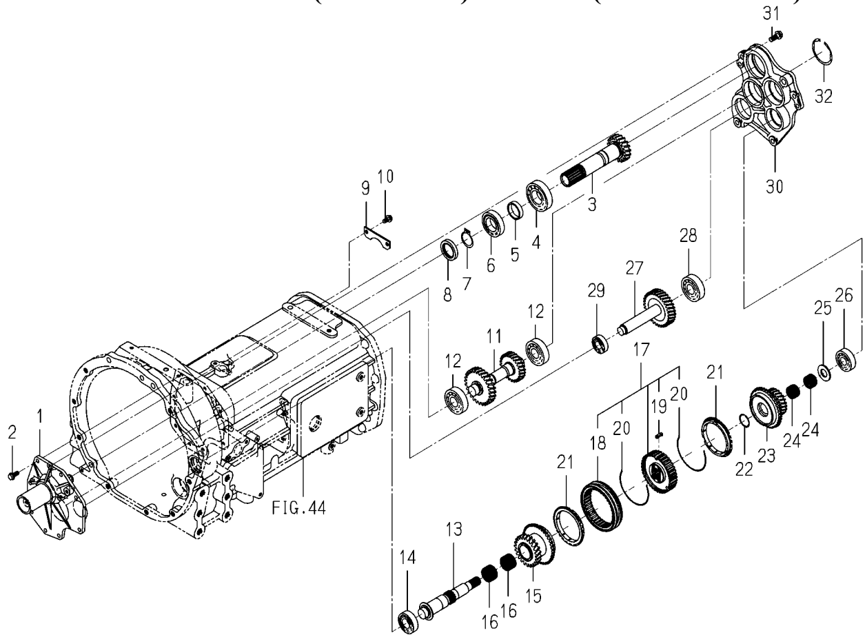
FIG. 52 GEAR(REVERSE)SYSTEM(6375-SD TYPE)
