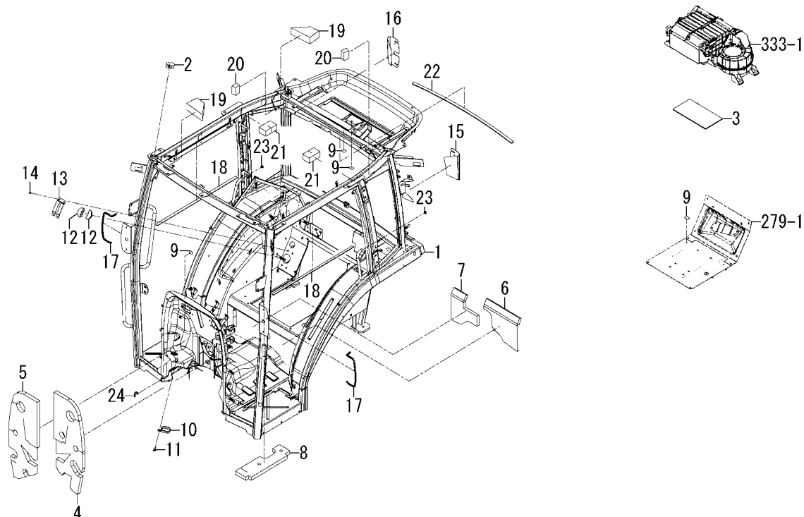
FIG.320 FLAME SYSTEM(6375-CY TYPE)
