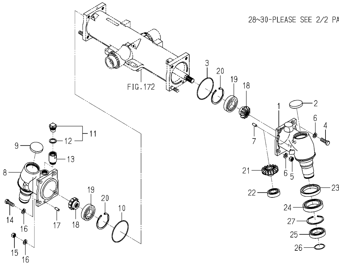
FIG.176 CASE(GEAR/FRONT)SYSTEM(1/2) (6375 TYPE/6405H TYPE)
