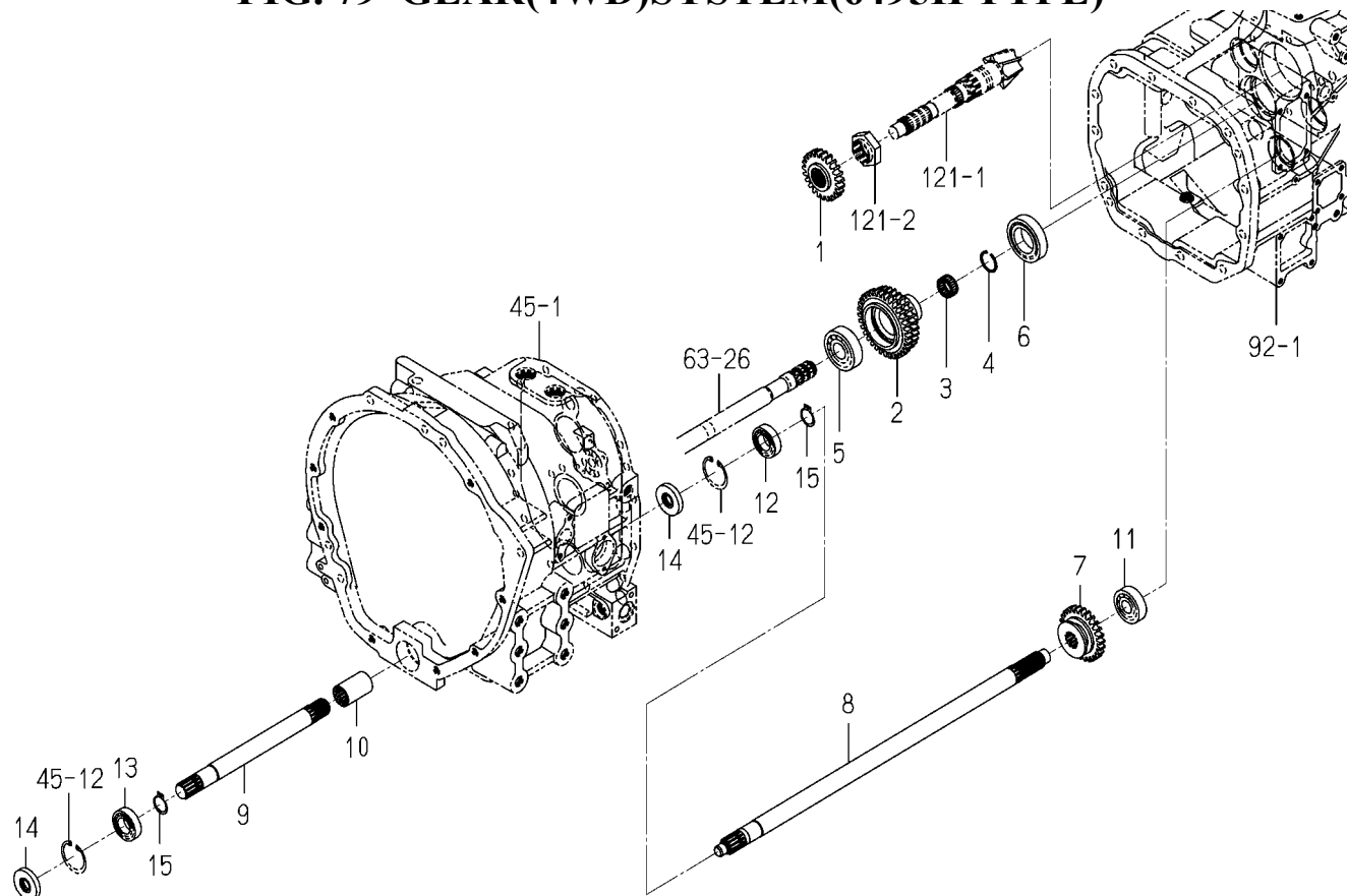
FIG. 79 GEAR(4WD)SYSTEM(6495H TYPE)
