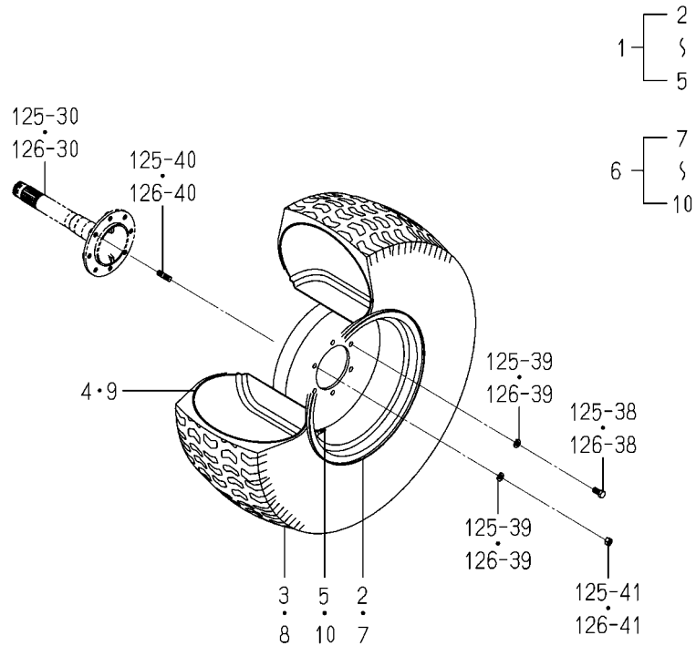
FIG.356 WHEEL(REAR/TURF/475/65D-20)ASSY (6495 TYPE EXCEPT A/6495H TYPE)(OPTION)
