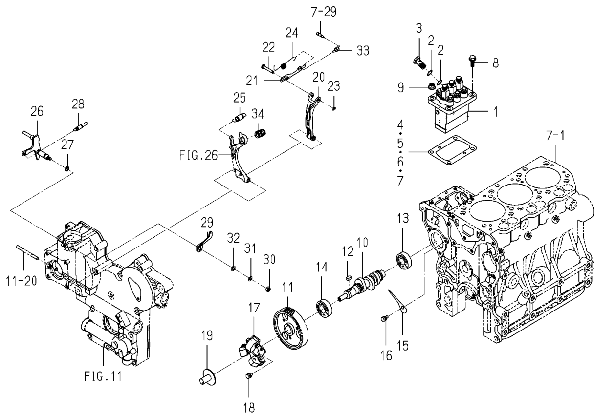
FIG. 24 INJECTION PUMP
