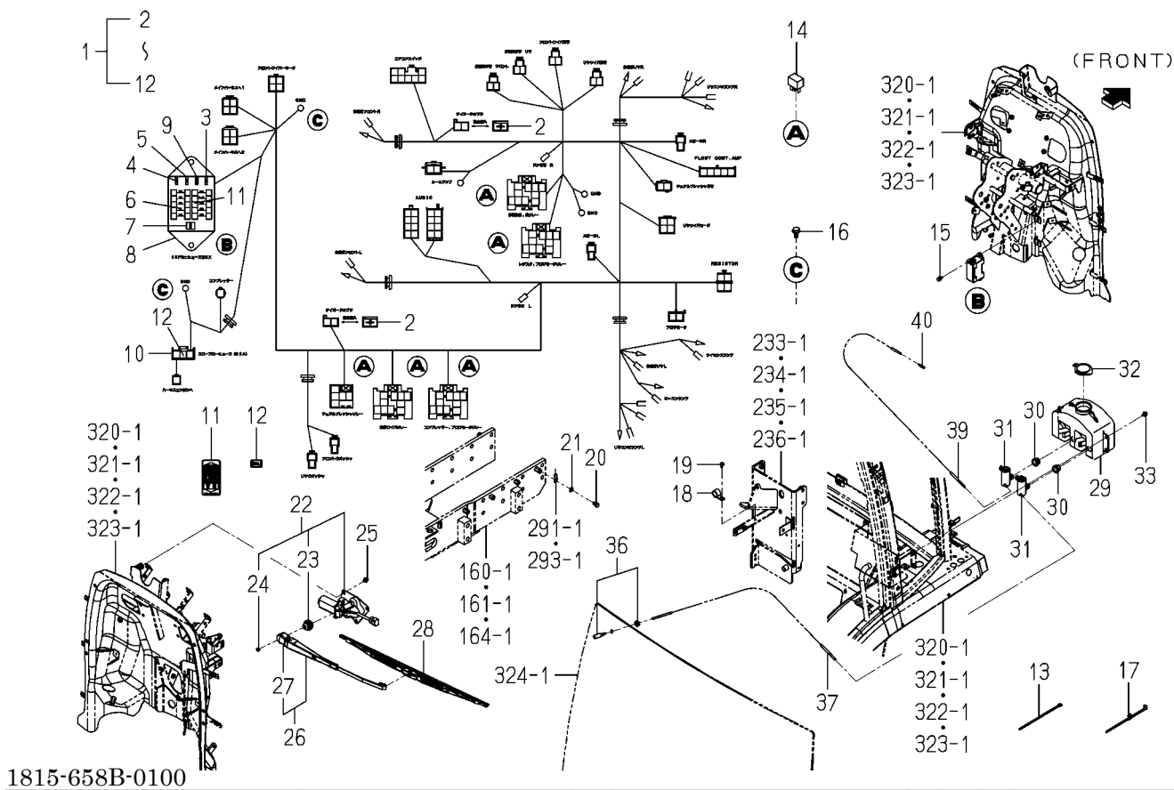
FIG.304 ELC.(CABIN)SYSTEMM(1/2) (EXCEPT CY TYPE)
