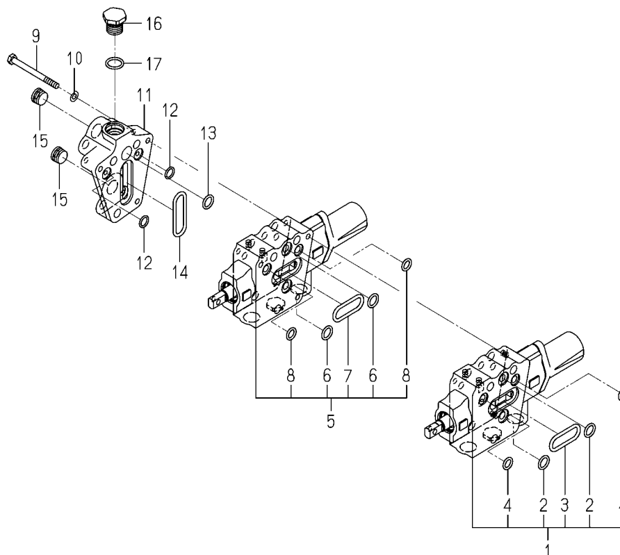
FIG.383 COMPONENT PARTS FOR K211-104-000-10 ON FIG.201,204,206,207
