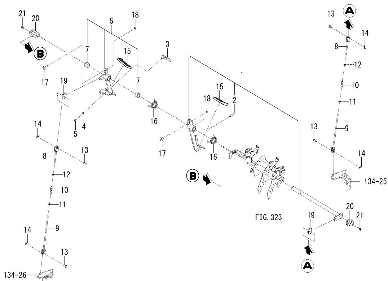
FIG.145 PEDAL(BRAKE)SYSTEM(6495H TYPE)
