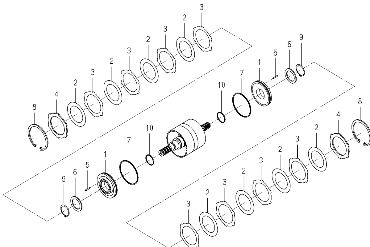
FIG.395 COMPONENT PARTS FOR 1792-215-700-00 ON FIG.70
