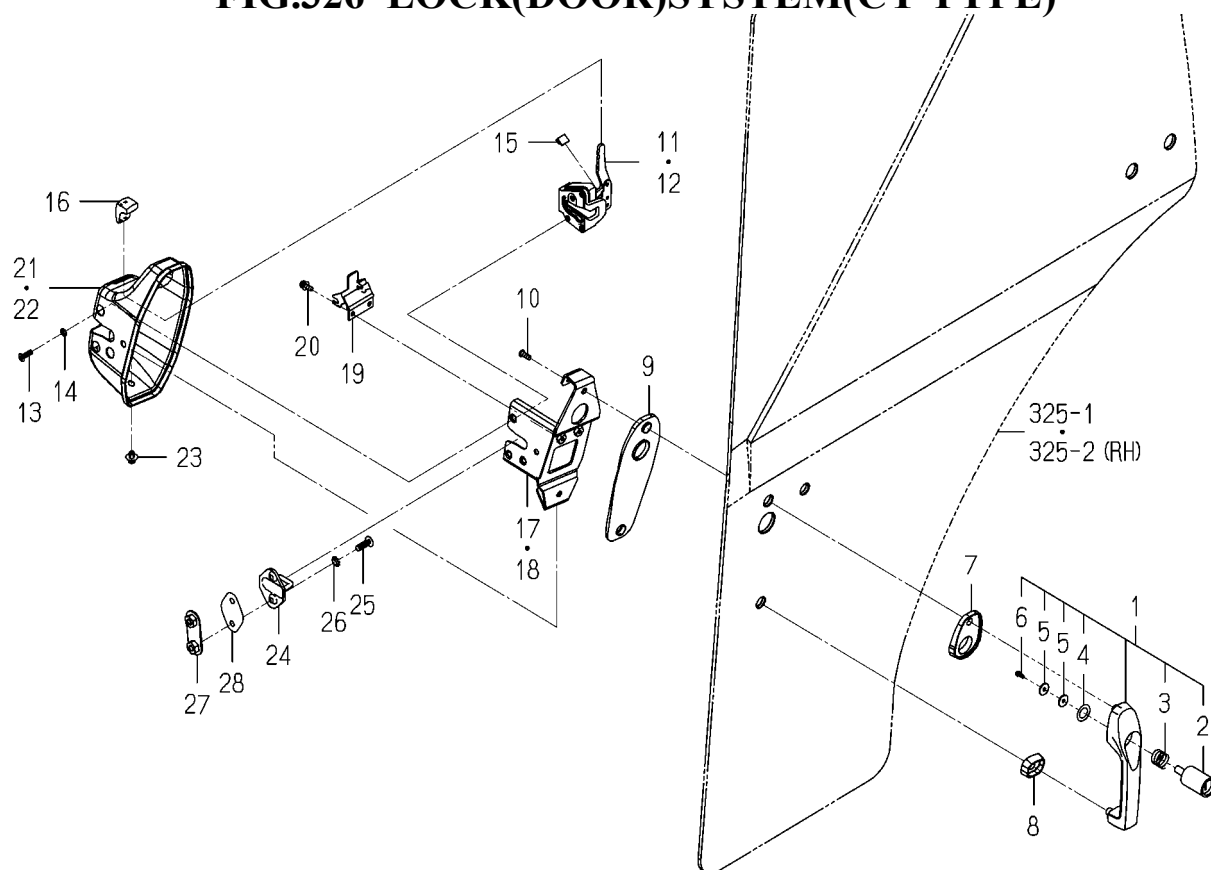
FIG.326 LOCK(DOOR)SYSTEM(CY TYPE)
