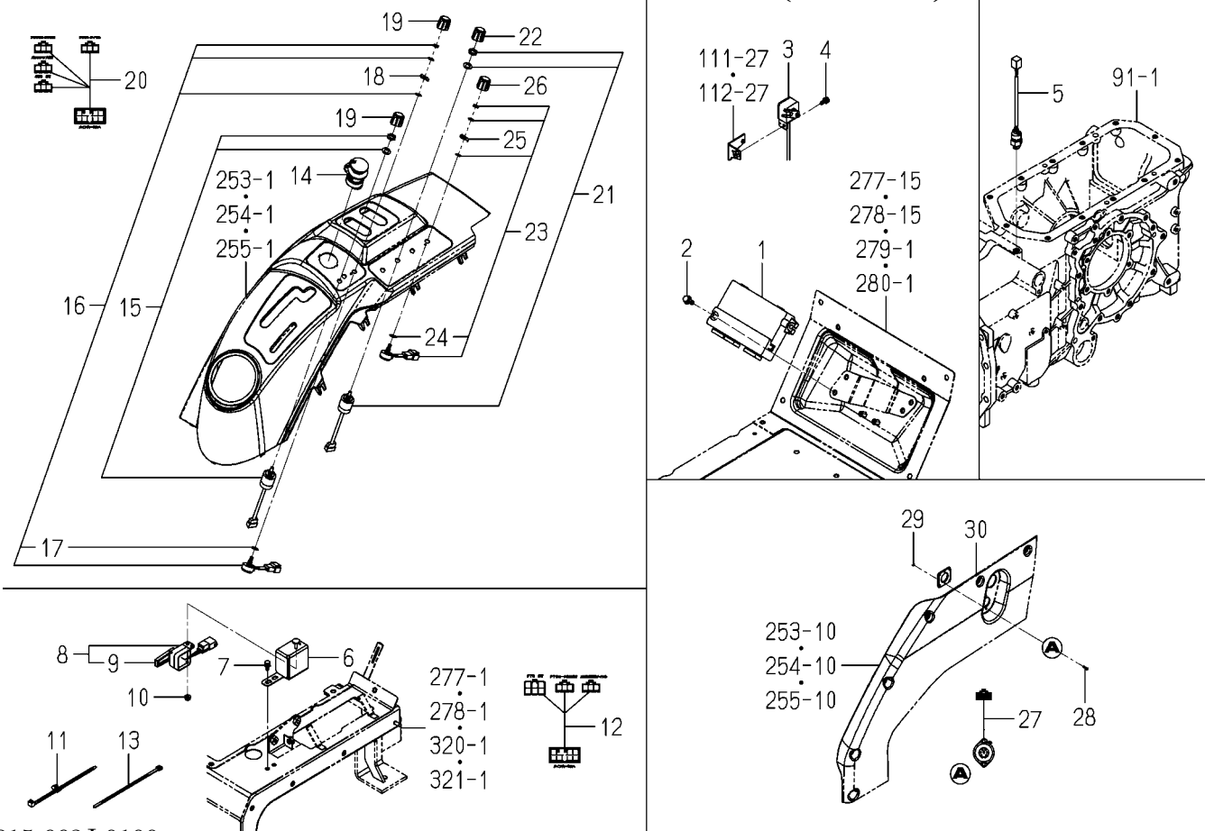
FIG.307 CONTROL SYSTEM(G TYPE)
