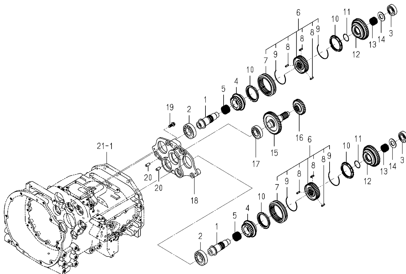
FIG. 65 GEAR(MAIN)SYSTEM(6375-G TYPE)
