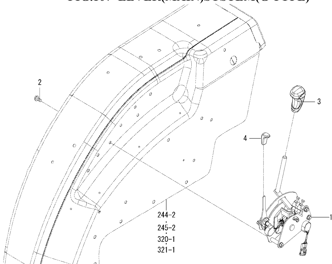
FIG.107 LEVER(MAIN)SYSTEM(G TYPE)
