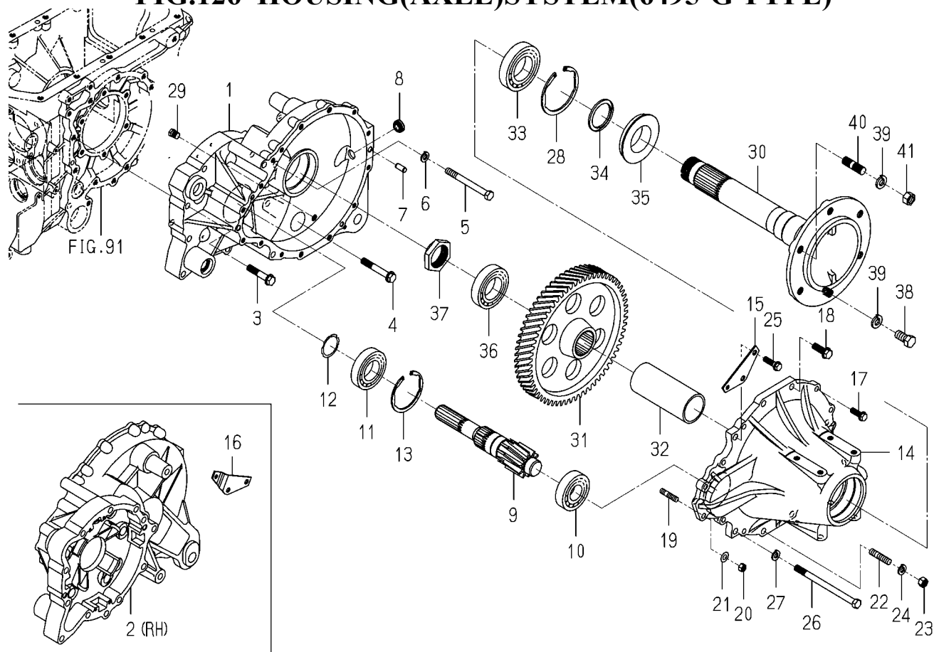
FIG.126 HOUSING(AXLE)SYSTEM(6495-G TYPE)
