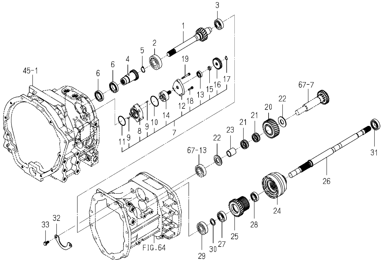
FIG. 63 GEAR(PTO)SYSTEM(6495H TYPE)
