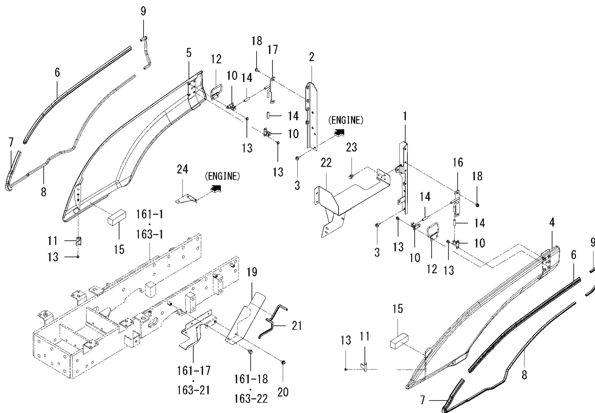
FIG.239 COVER(SIDE)SYSTEM (6495-SD TYPE/6495H TYPE)
