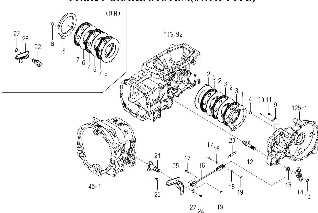
FIG.134 BRAKE SYSTEM(6495H TYPE)
