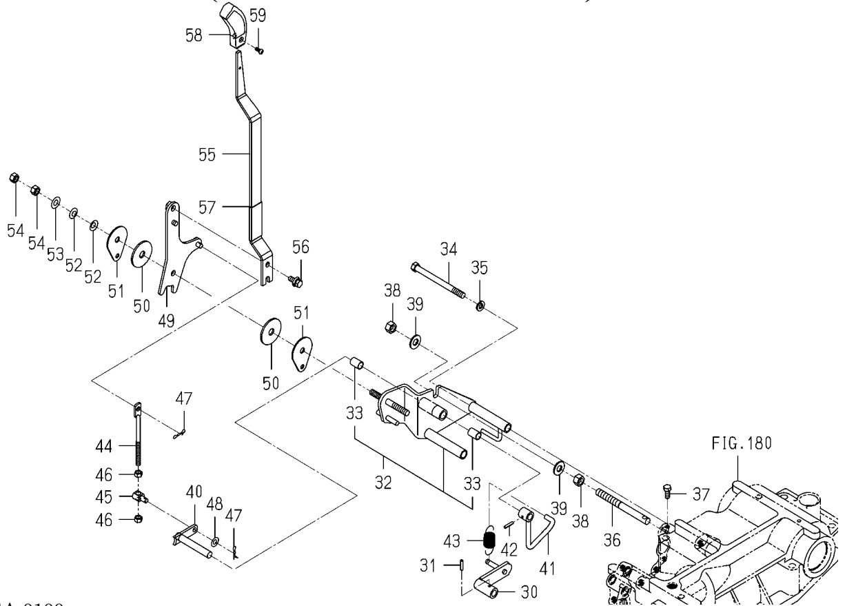
FIG.183 LEVER(POSITION)SYSTEM(2/2) (6375-SD TYPE/6405H TYPE)
