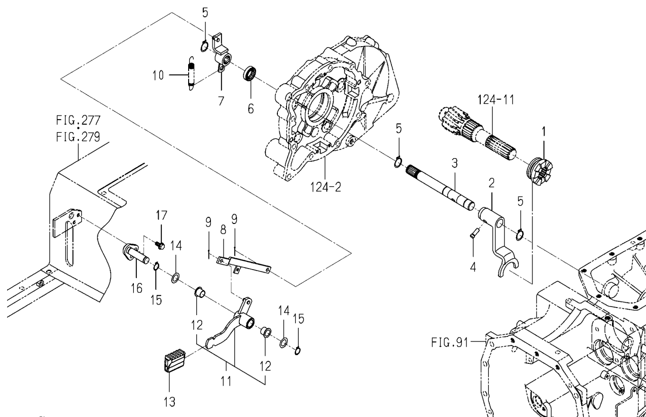
FIG.131 CLUTCH(DIFF-LOCK)SYSTEM (6375-G TYPE)
