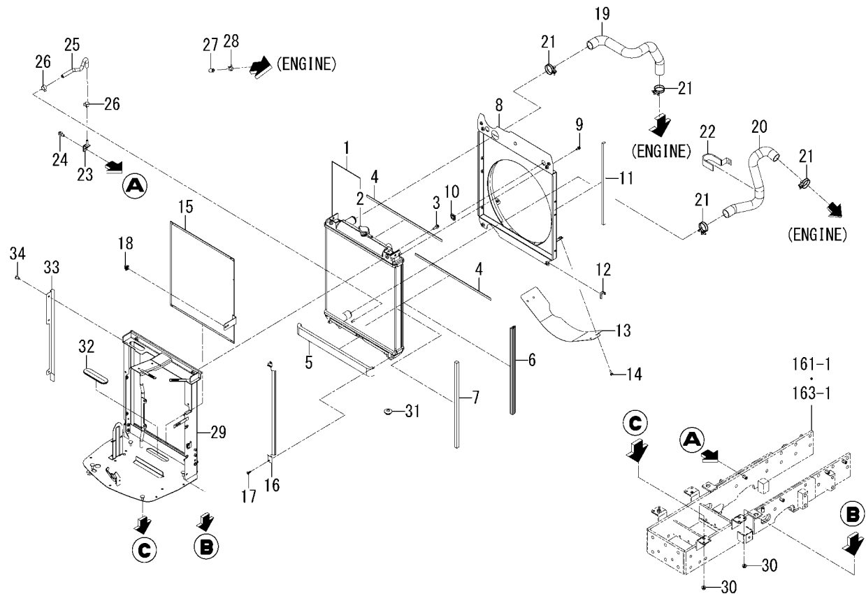
FIG. 3 RADIATOR SYSTEM(1/2) (6495 TYPE/6495H TYPE)
