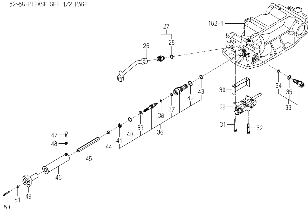
FIG.194 PIPING(MAIN)SYSTEM(2/2) (6495-H TYPE)
