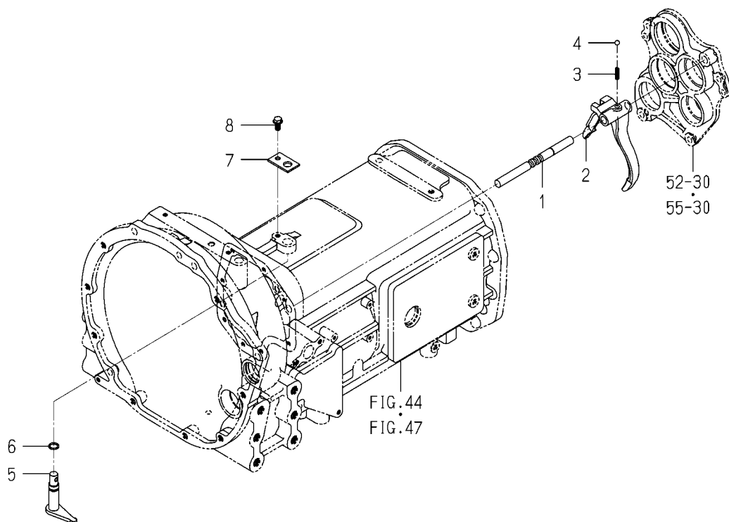
FIG. 93 FORK(SHIFT/REVERSE)SYSTEM (SD TYPE)
