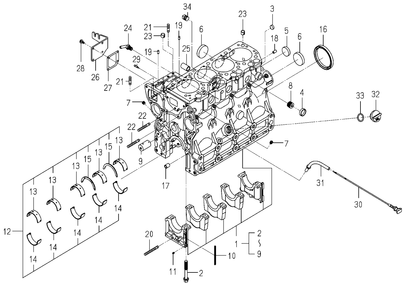
FIG. 9 CYLINDER BLOCK
