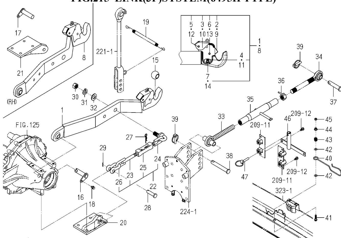
FIG.215 LINK(3P)SYSTEM(6495H TYPE)
