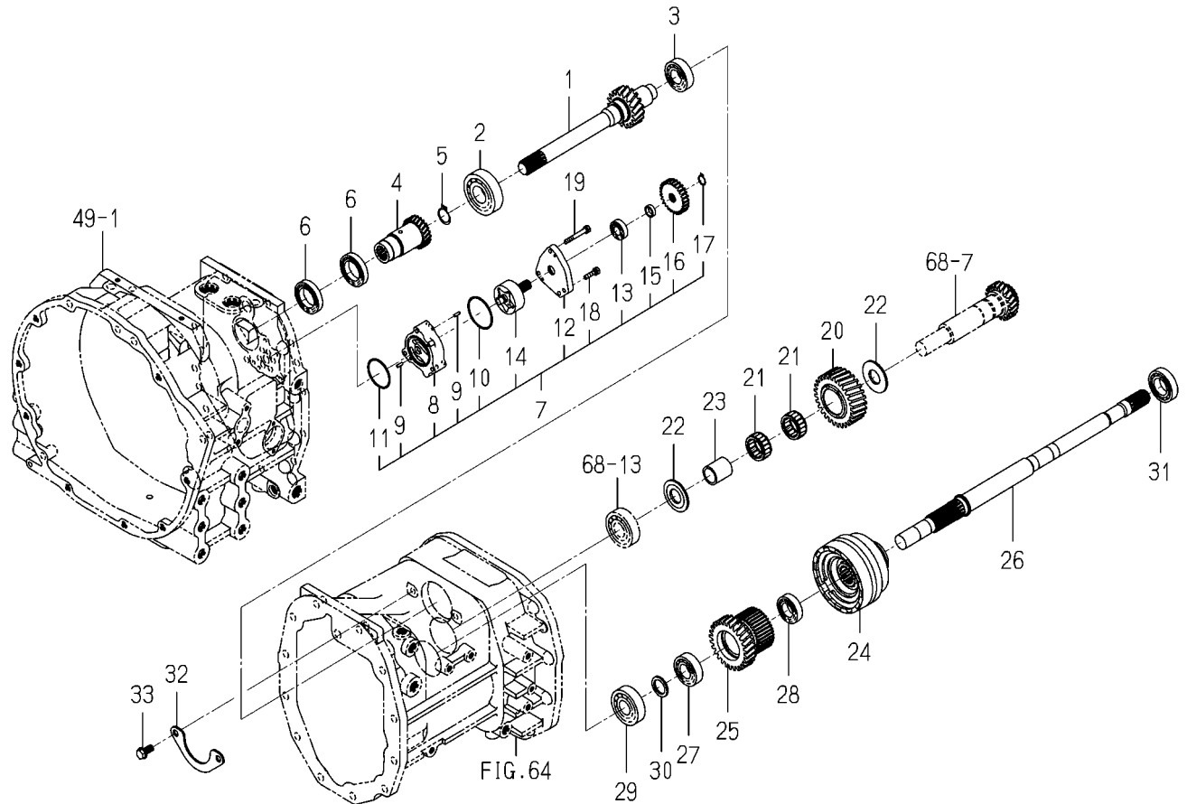
FIG. 60 GEAR(PTO)SYSTEM(6405H TYPE)
