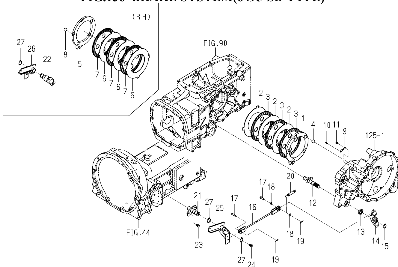
FIG.136 BRAKE SYSTEM(6495-SD TYPE)
