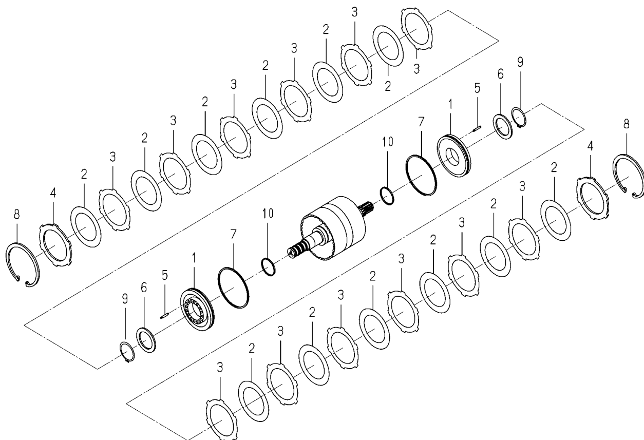
FIG.399 COMPONENT PARTS FOR 1796-215-700-00 ON FIG.71
