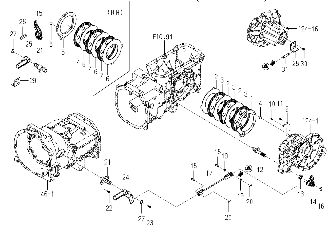
FIG.137 BRAKE SYSTEM(6375-G TYPE)
