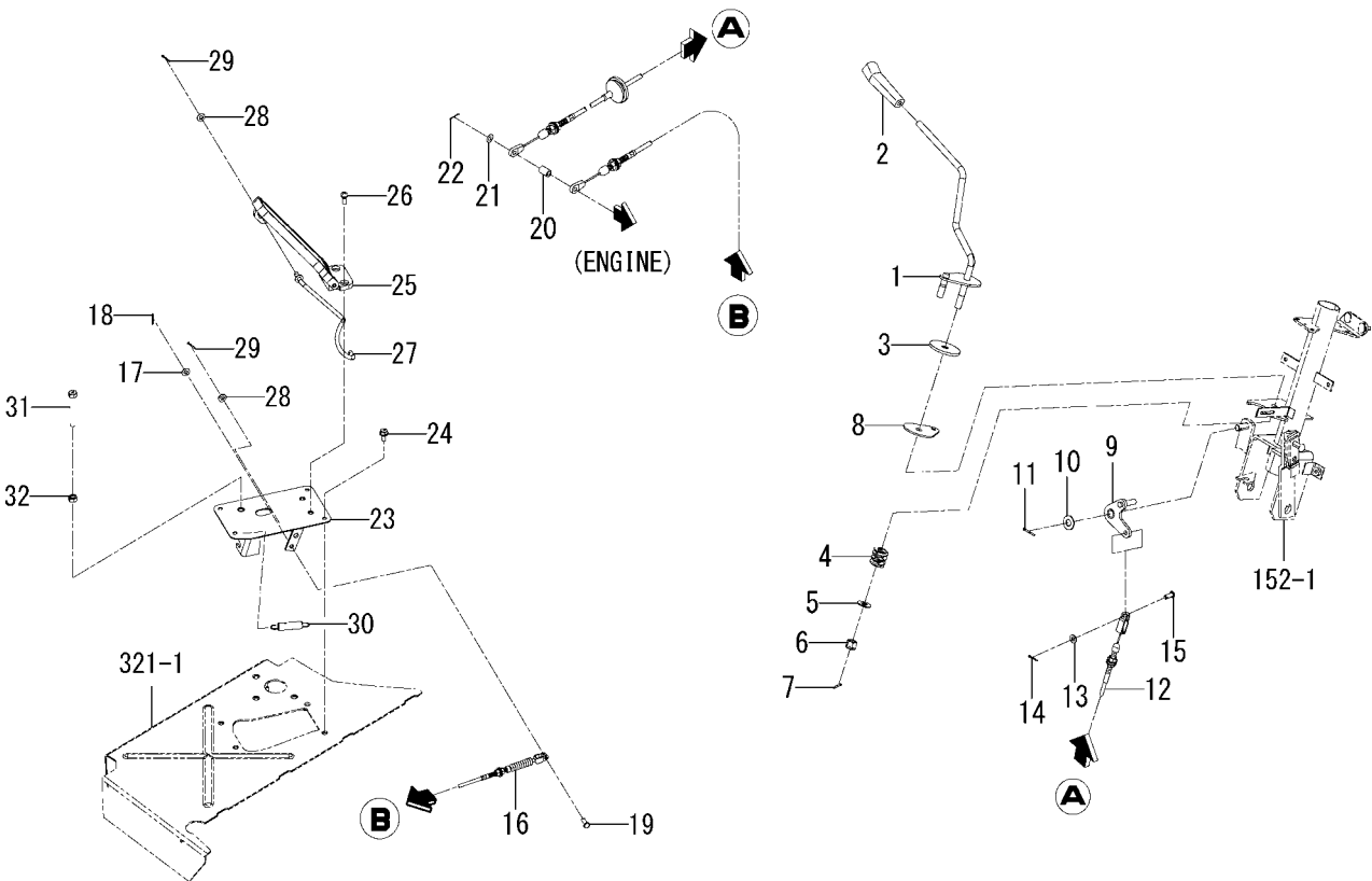
FIG. 34 ACCELERATOR SYSTEM(6495-CY TYPE)
