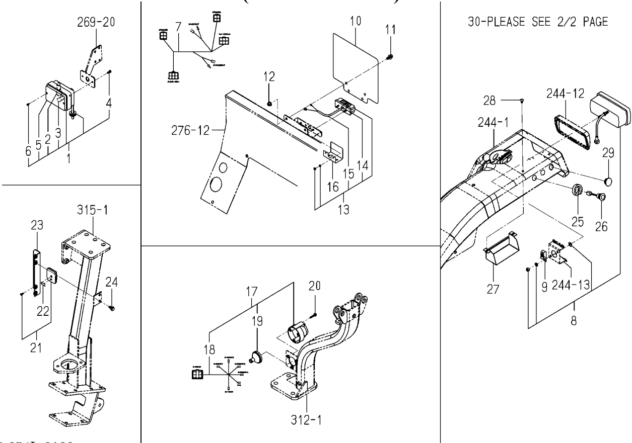
FIG.297 ELC.(FLOOR)SYSTEM(1/2) (6495H-R TYPE)
