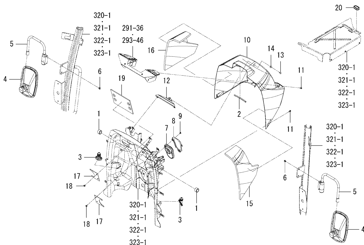
FIG.266 FLOOR(FRONT)SYSTEM(CY TYPE)
