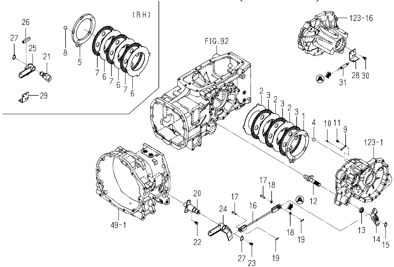
FIG.133 BRAKE SYSTEM(6405H TYPE)
