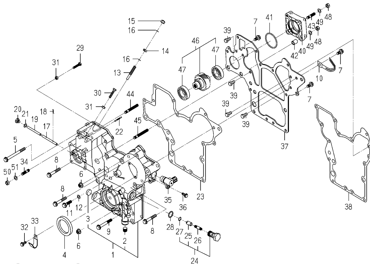
FIG. 13 TIMING GEAR CASE
