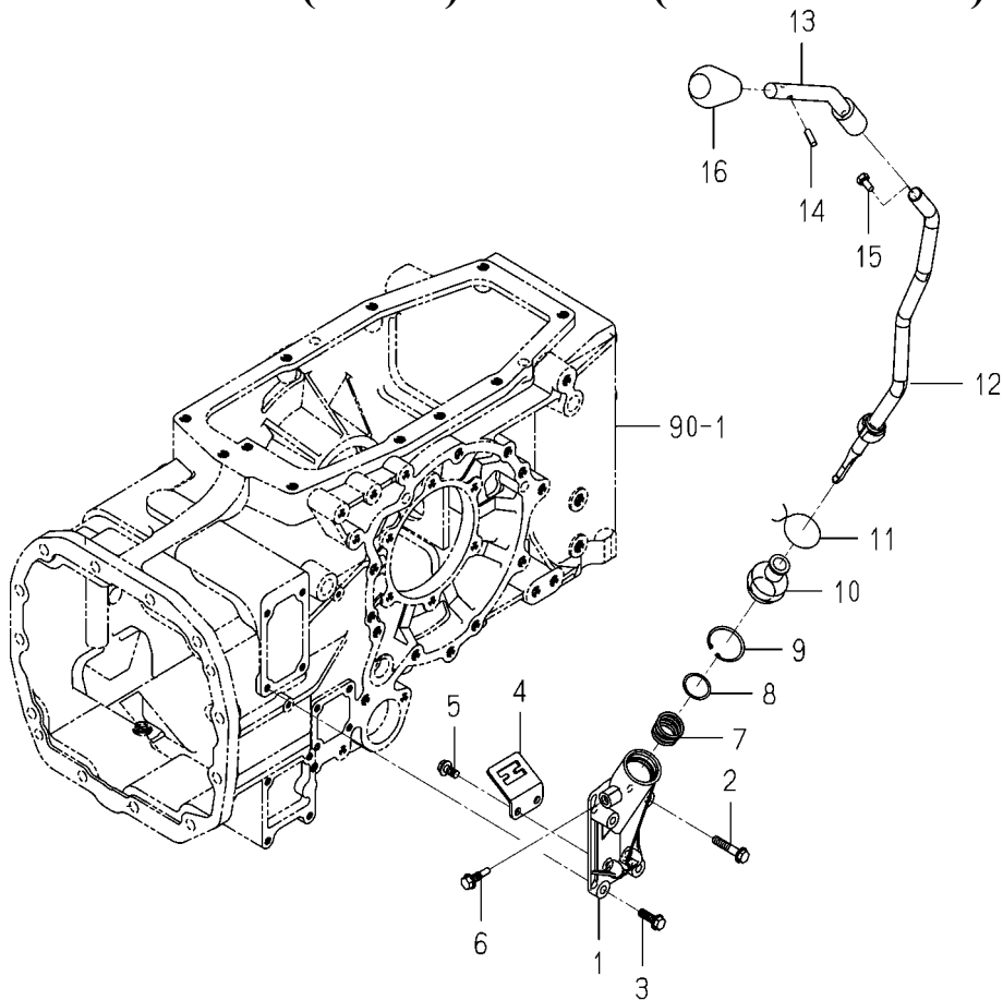
FIG.108 LEVER(MAIN)SYSTEM(6495-SD TYPE)
