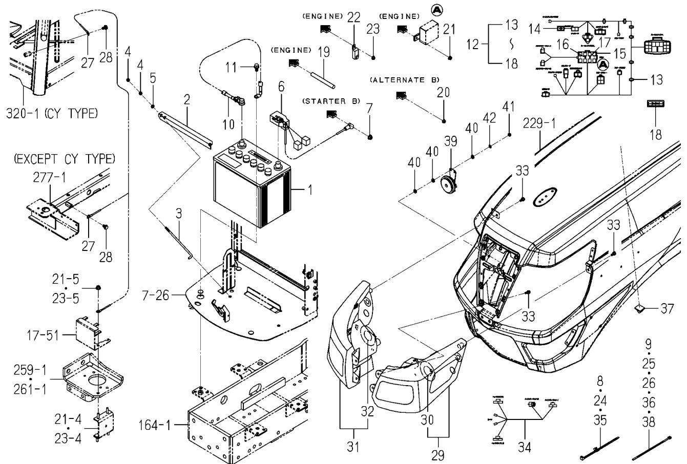
FIG.289 ELC.(FRONT)SYSTEM(6375-E4G TYPE)
