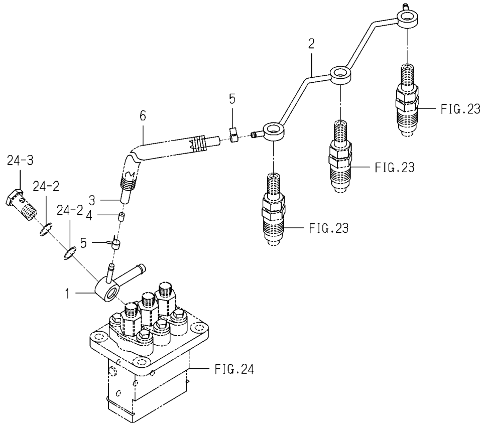
FIG. 25 FUEL PIPE
