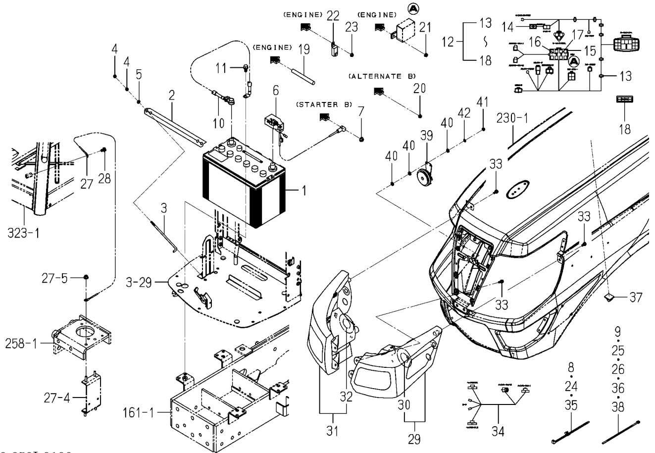
FIG.286 ELC.(FRONT)SYSTEM(6495H-G TYPE)
