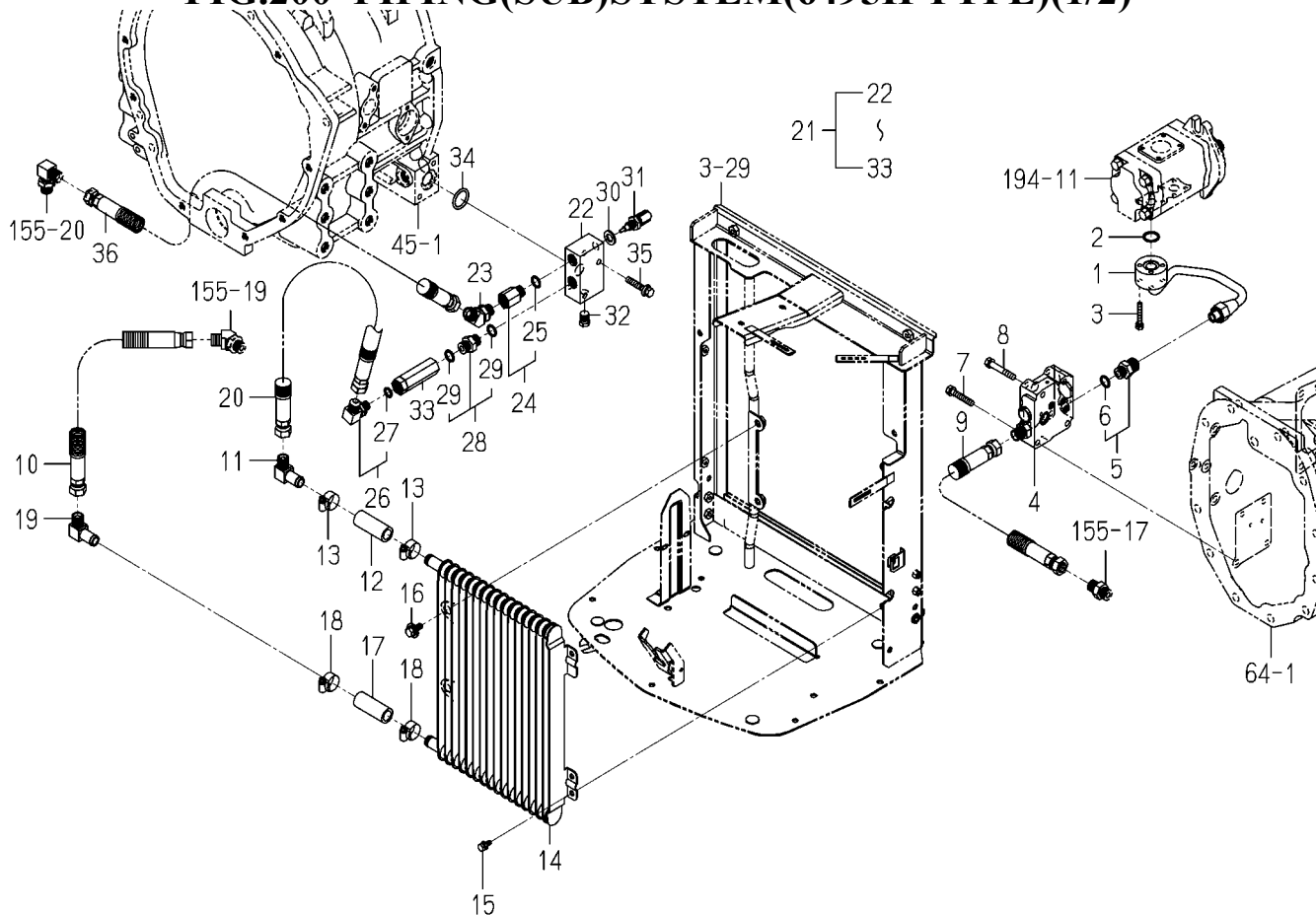
FIG.200 PIPING(SUB)SYSTEM(6495H TYPE)(1/2)
