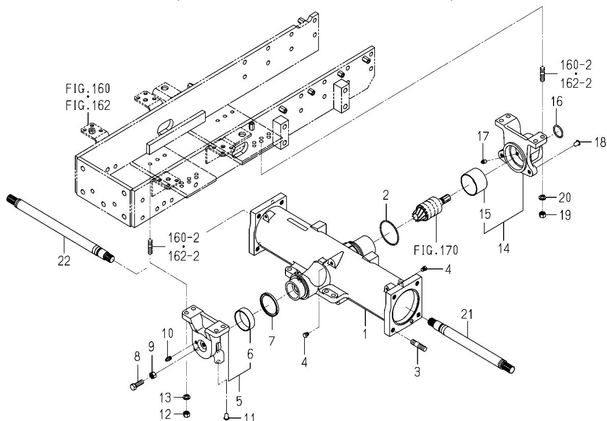
FIG.172 HOUSING(AXLE/FRONT)SYSTEM (6375-SD TYPE/6405H TYPE)
