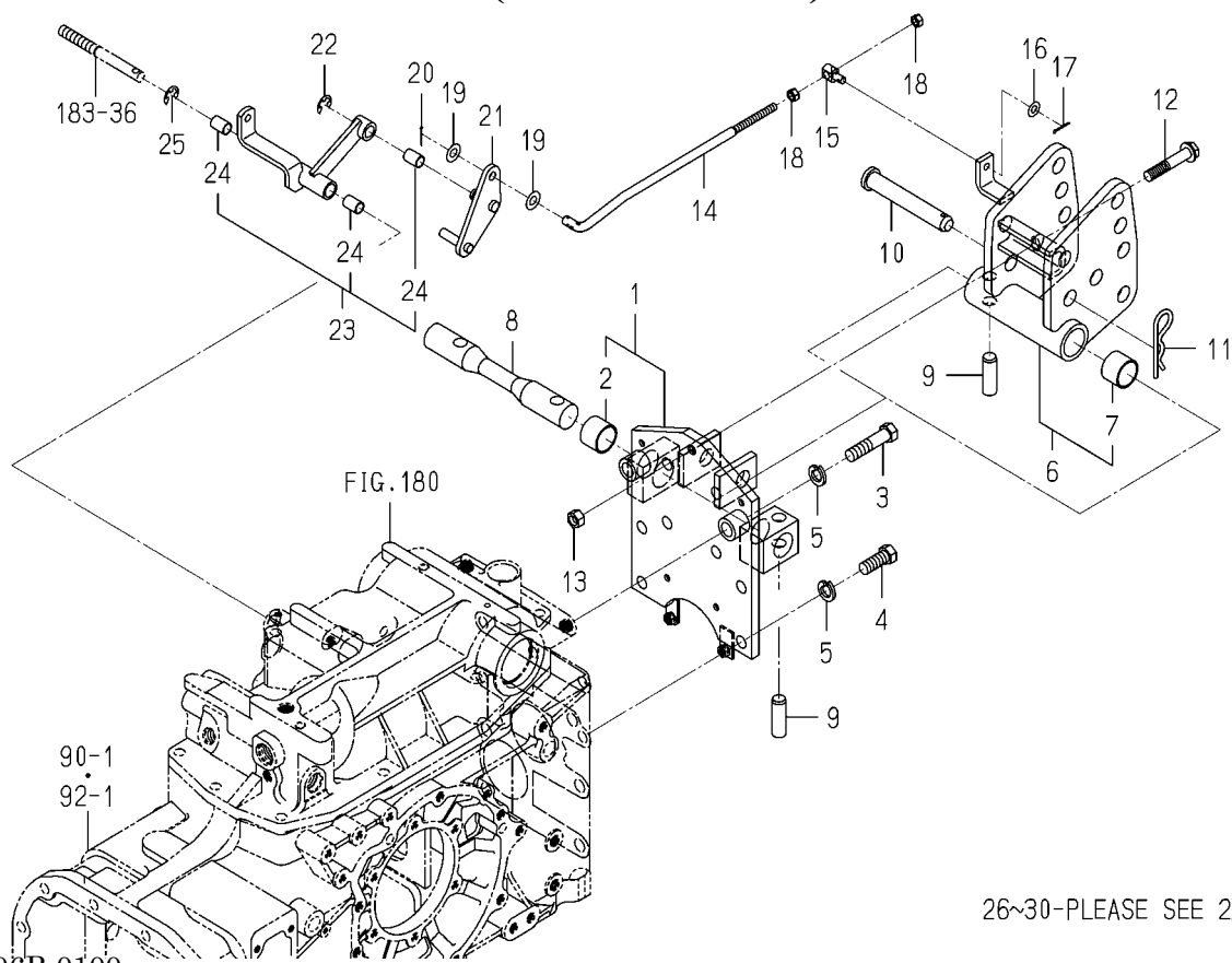
FIG.187 LEVER(DRAFT)SYSTEM(1/2) (6375-SD TYPE)
