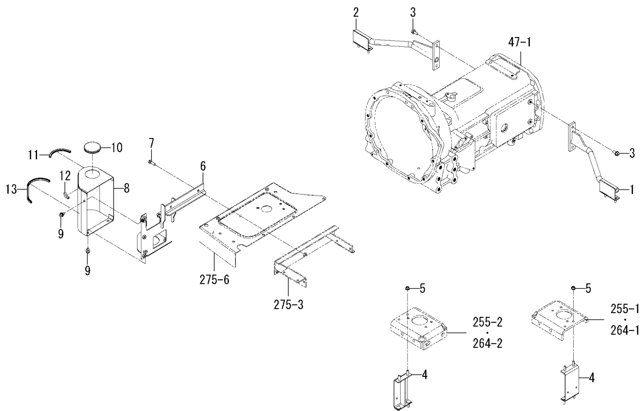
FIG. 20 STAY(TANK)SET SYSTEM(6495-SD TYPE)
