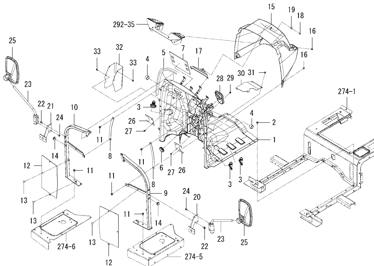
FIG.267 PANEL(DASH)SYSTEM(6375-SD TYPE)
