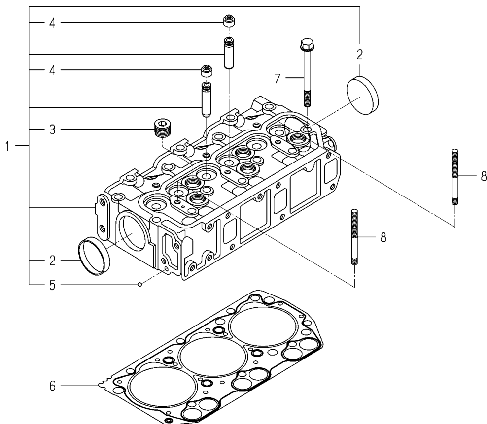
FIG. 2 CYLINDER HEAD
