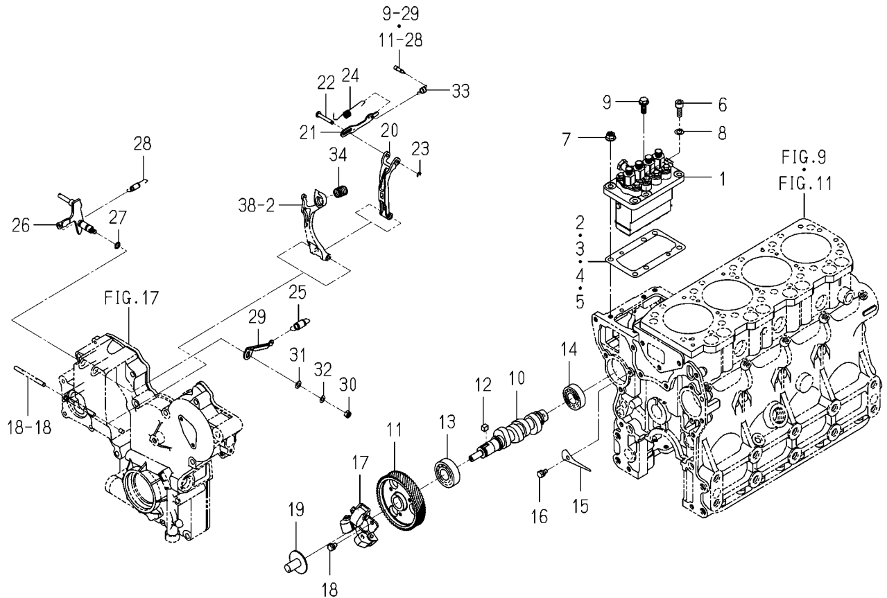
FIG. 36 INJECTION PUMP
