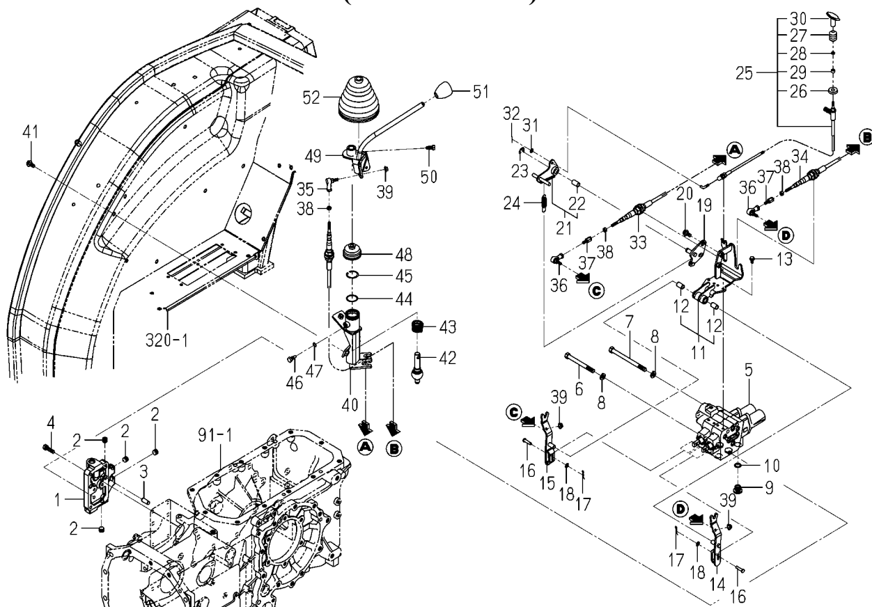
FIG.205 JOY STICK VALVE SYSTEM (6375-D TYPE)
