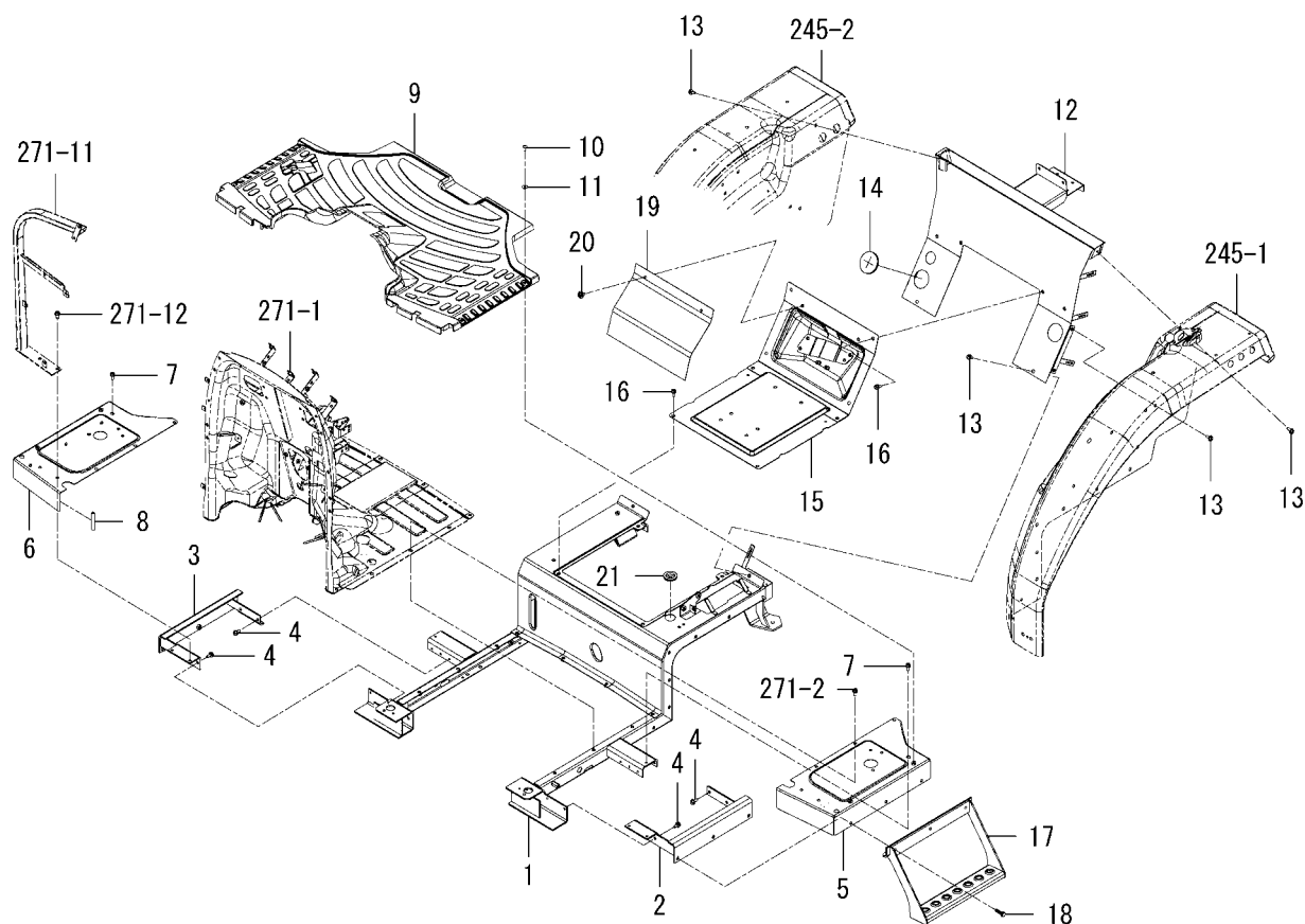
FIG.278 FLOOR(REAR)SYSTEM(6495-GR TYPE)
