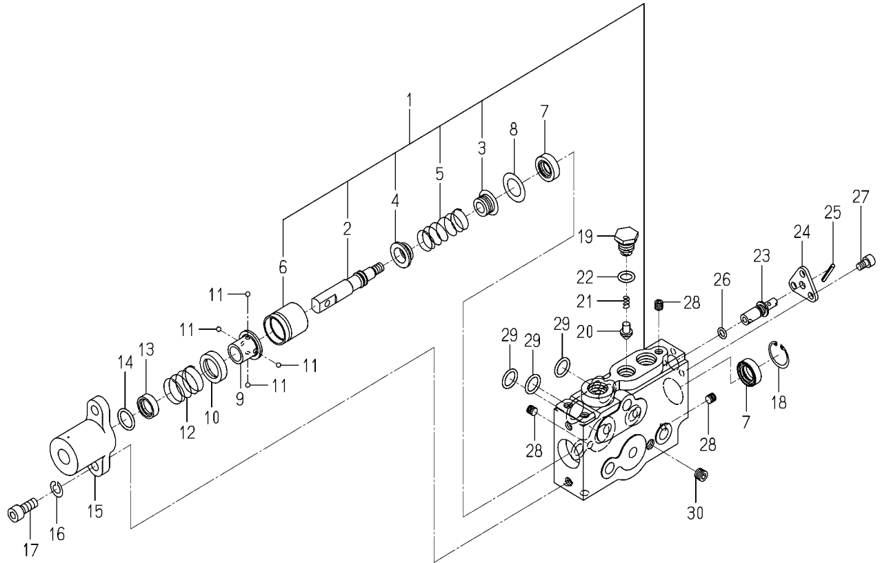
FIG.403 COMPONENT PARTS FOR 1801-512-300-10 ON FIG.209
