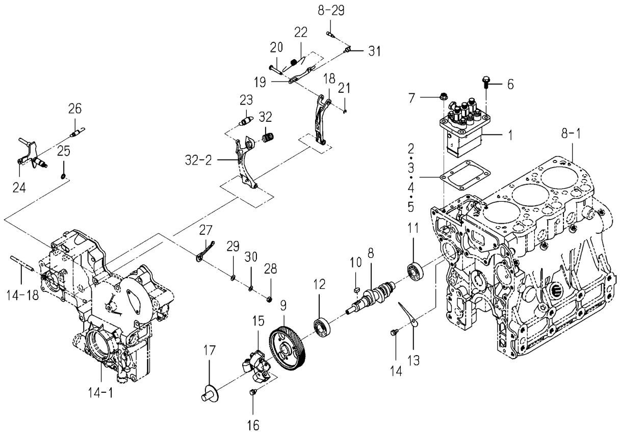
FIG. 29 INJECTION PUMP
