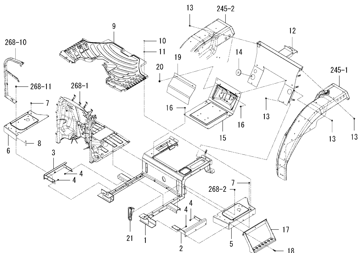
FIG.275 FLOOR(REAR)SYSTEM(6495-SD TYPE)
