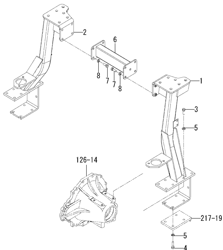
FIG.317 FLAME(LOWER)SYSTEM(6495-SD TYPE)
