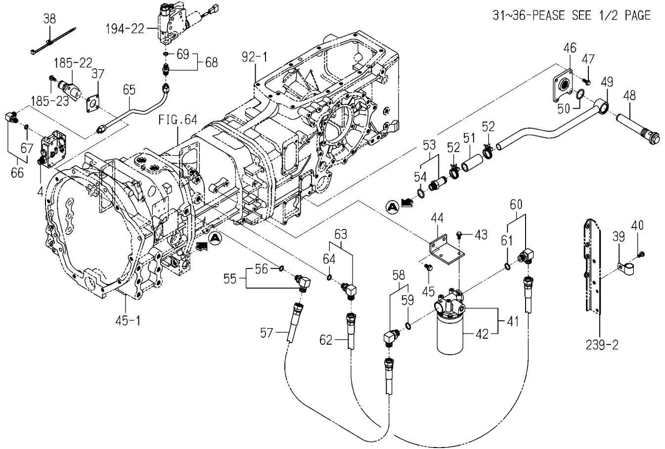
FIG.200 PIPING(SUB)SYSTEM(6495H TYPE)(2/2)
