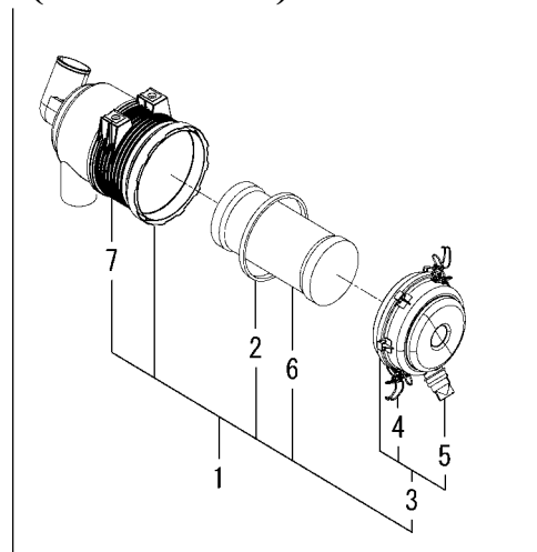
FIG. 13 CLEANER(AIR)SYSTEM(6375 TYPE)
