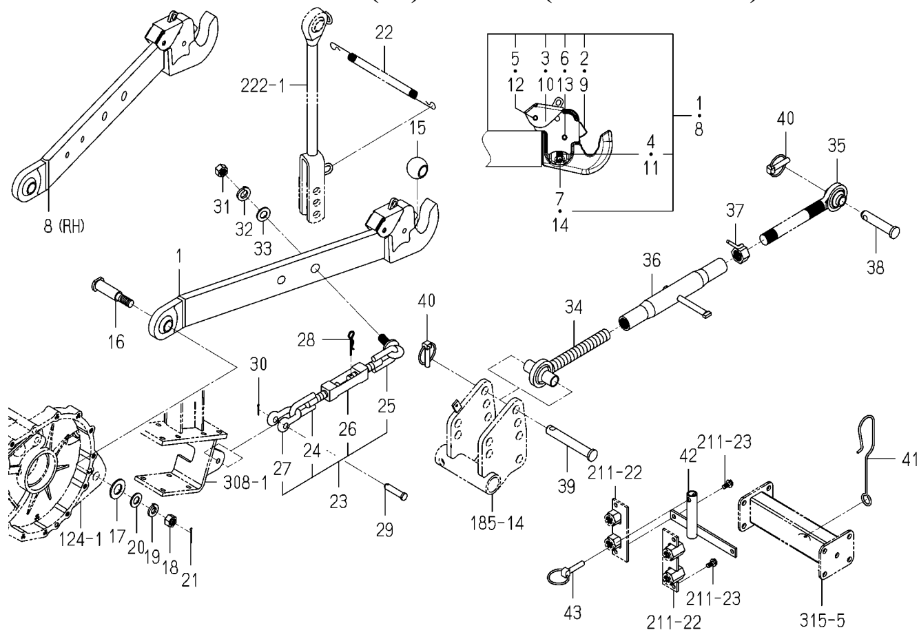
FIG.216 LINK(3P)SYSTEM(6375-GR TYPE)
