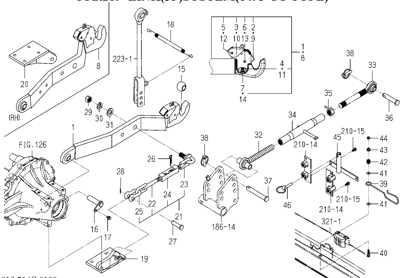
FIG.219 LINK(3P)SYSTEM(6495-CY TYPE)
