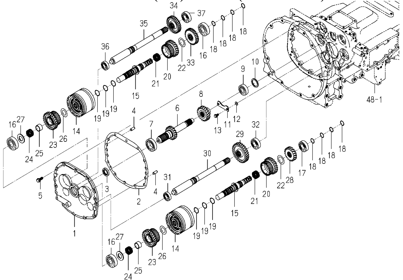
FIG. 51 GEAR(H/L)SYSTEM(6495-G TYPE)
