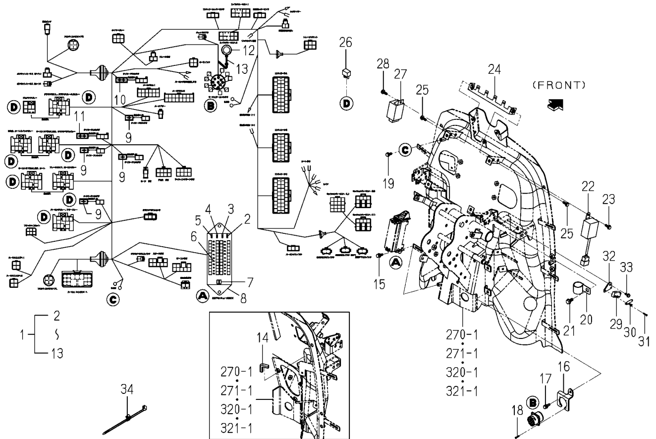
FIG.293 ELC.(MAIN)SYSTEM(G TYPE)(1/2)
