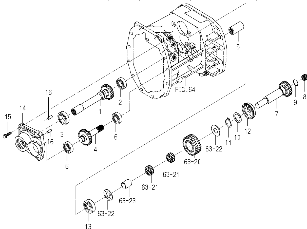
FIG. 67 GEAR(MAIN)SYSTEM(6495-H TYPE)
