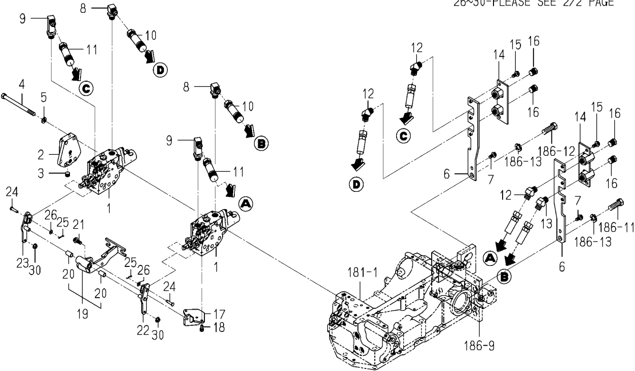
FIG.210 VALVE(REMOTE/2)SET SYSTEM(1/2) (6495-G TYPE)
