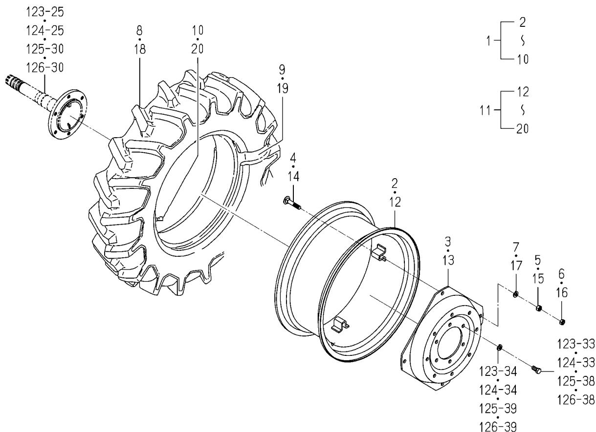
FIG.353 WHEEL(REAR/24XW11)ASSY(OPTION)
