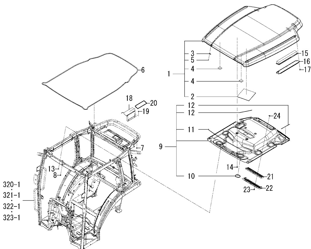
FIG.318 ROOF SYSTEM(CY TYPE)
