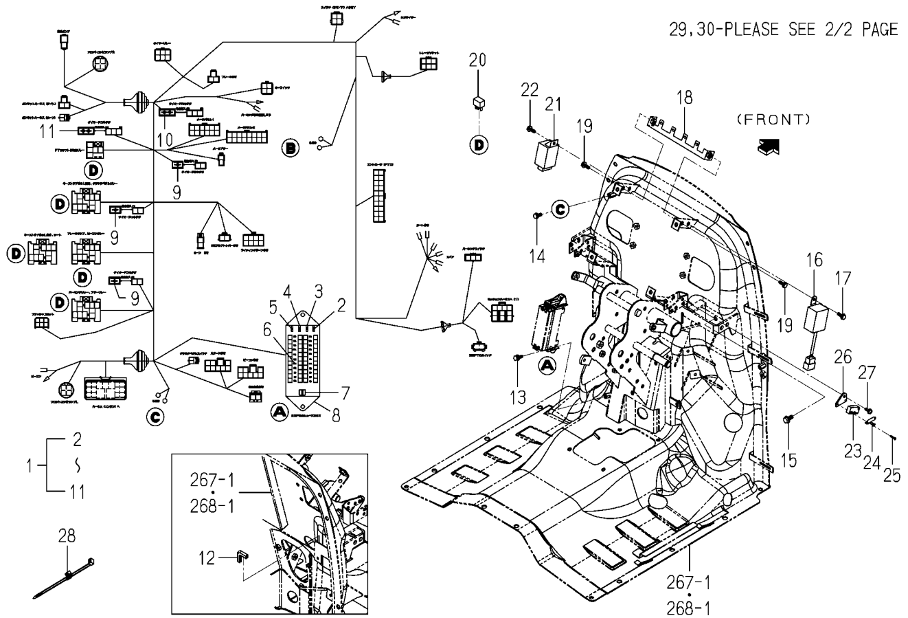
FIG.292 ELC.(MAIN)SYSTEM(SD TYPE)(1/2)
