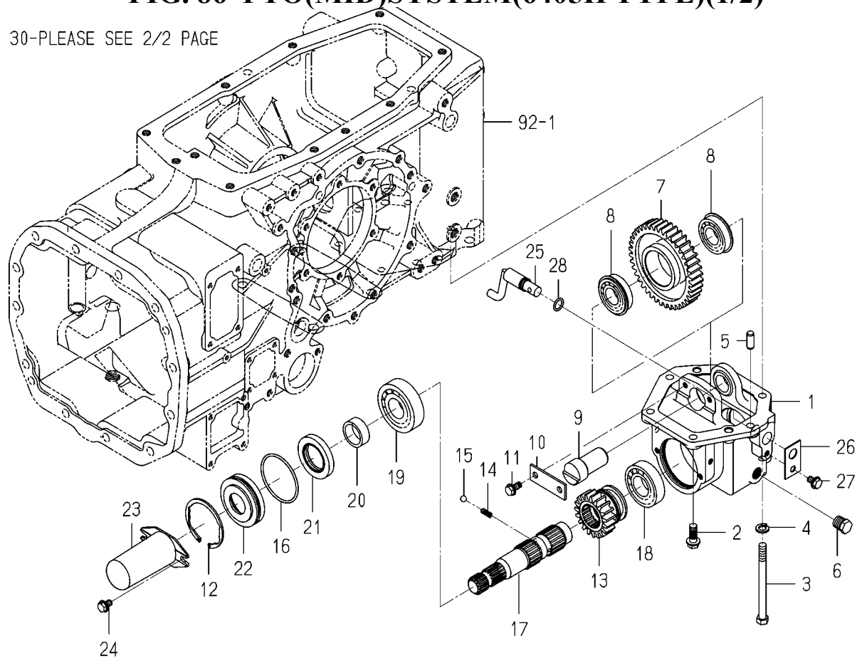
FIG. 86 PTO(MID)SYSTEM(6405H TYPE)(1/2)
