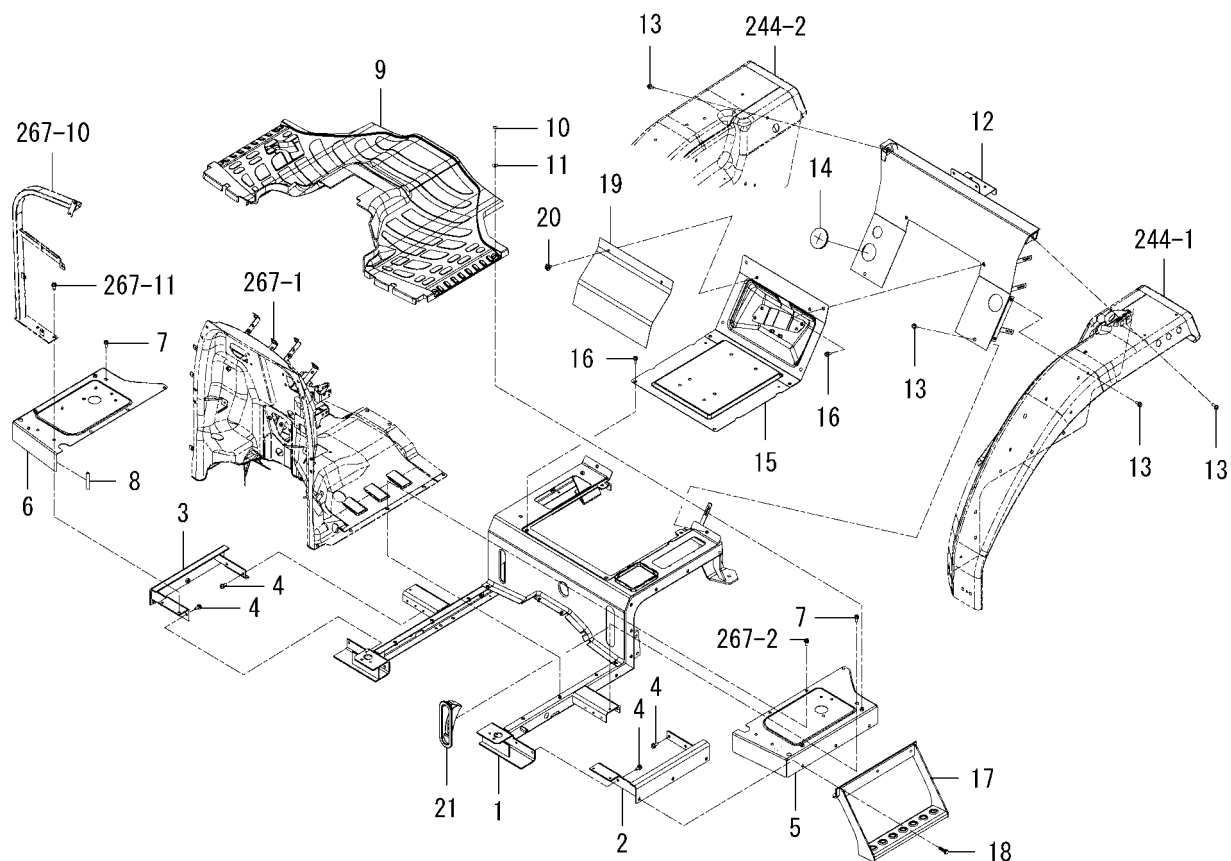
FIG.274 FLOOR(REAR)SYSTEM(6375-SD TYPE)
