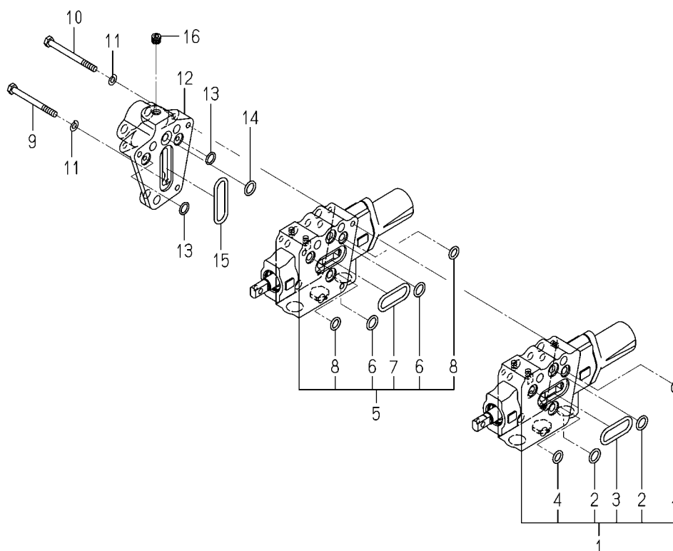
FIG.385 COMPONENT PARTS FOR K211-109-000-10 ON FIG.202,203,205,208
