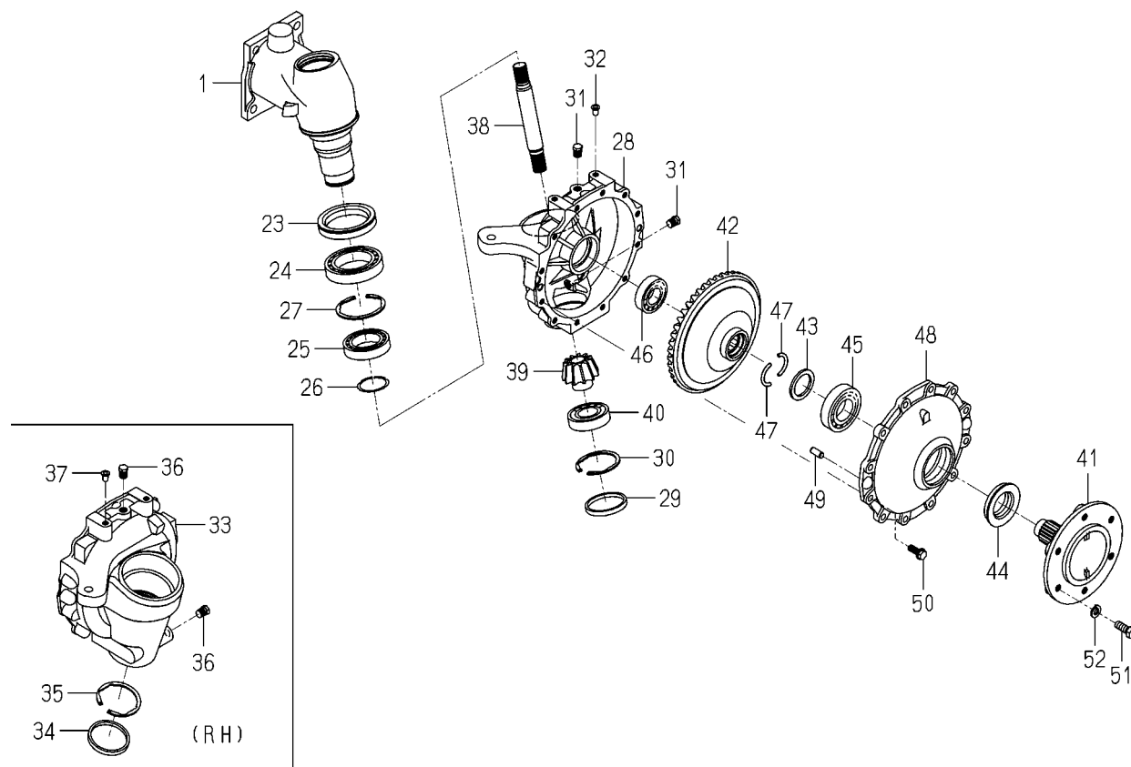
FIG.176 CASE(GEAR/FRONT)SYSTEM(2/2) (6375 TYPE/6405H TYPE)
