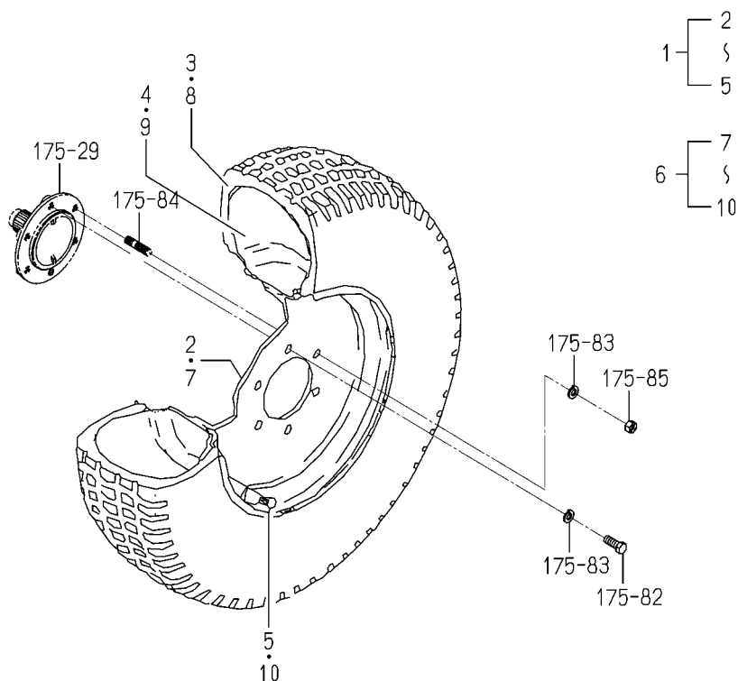
FIG.363 WHEEL(FRONT/TURF/7JAX15)ASSY (6495-SD TYPE EXCEPT A/6495H TYPE)(OPTION)
