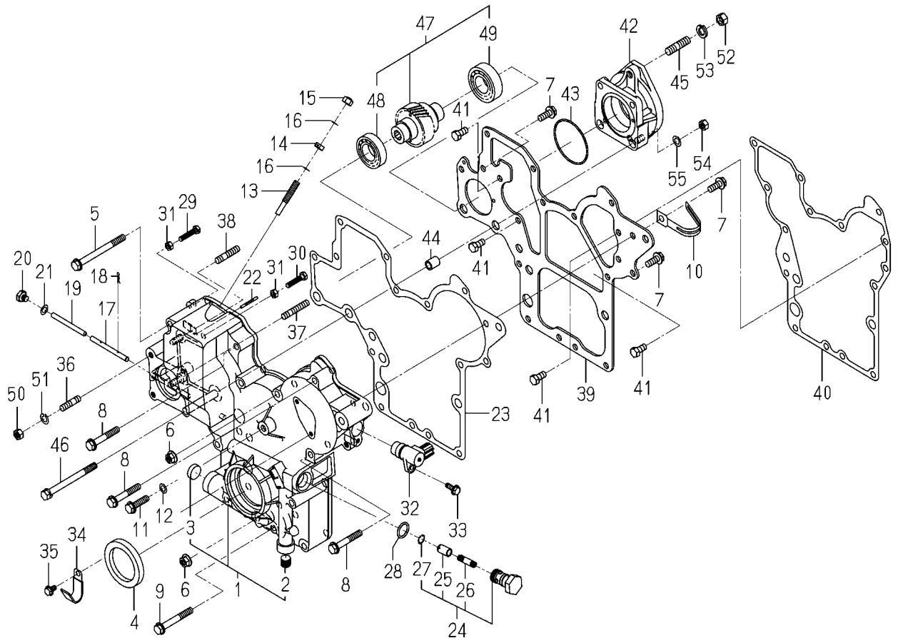
FIG. 17 TIMING GEAR CASE
