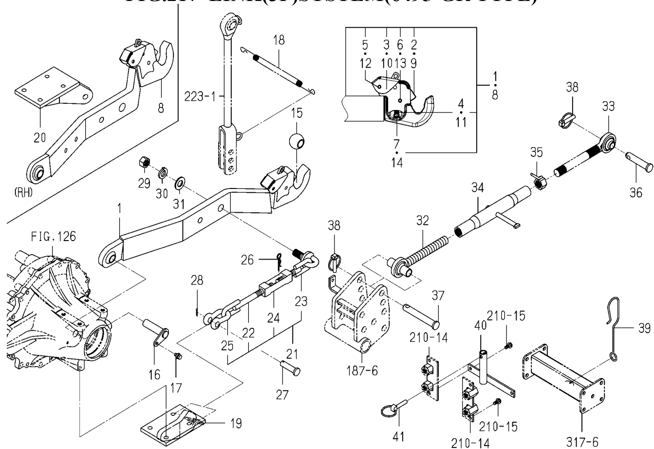
FIG.217 LINK(3P)SYSTEM(6495-GR TYPE)
