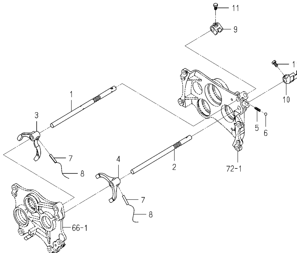
FIG. 94 FORK(SHIFT/MAIN)SYSTEM(SD TYPE)
