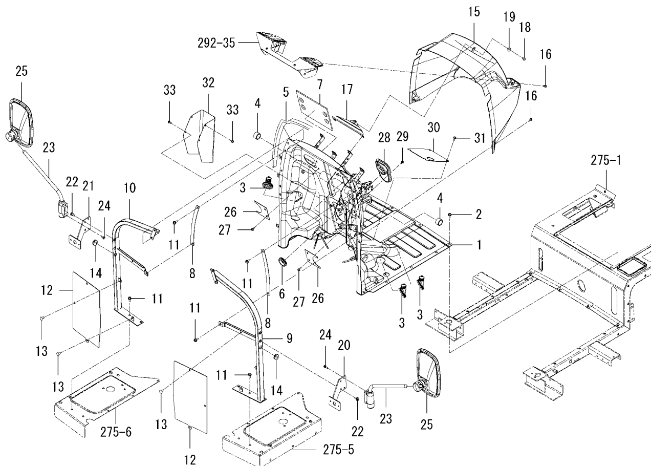
FIG.268 PANEL(DASH)SYSTEM(6495-SD TYPE)
