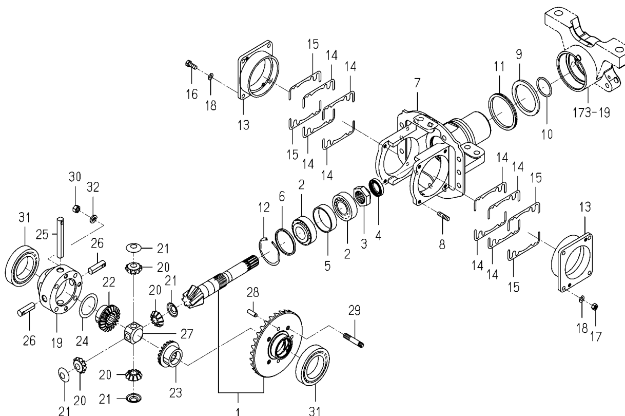
FIG.171 CASE(BEVEL)SYSTEM (6495 TYPE/6495H TYPE)
