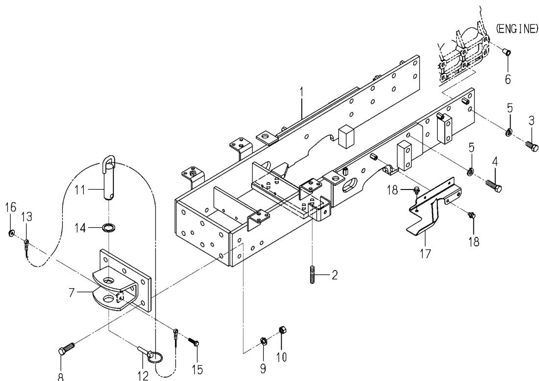
FIG.161 BRACKET(AXLE)SYSTEM (6495 TYPE/6495H TYPE)
