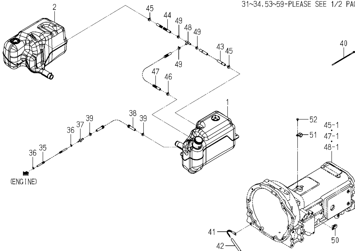
FIG. 18 TANK(FUEL)SYSTEM(2/2) (6495 TYPE/6495H TYPE)
