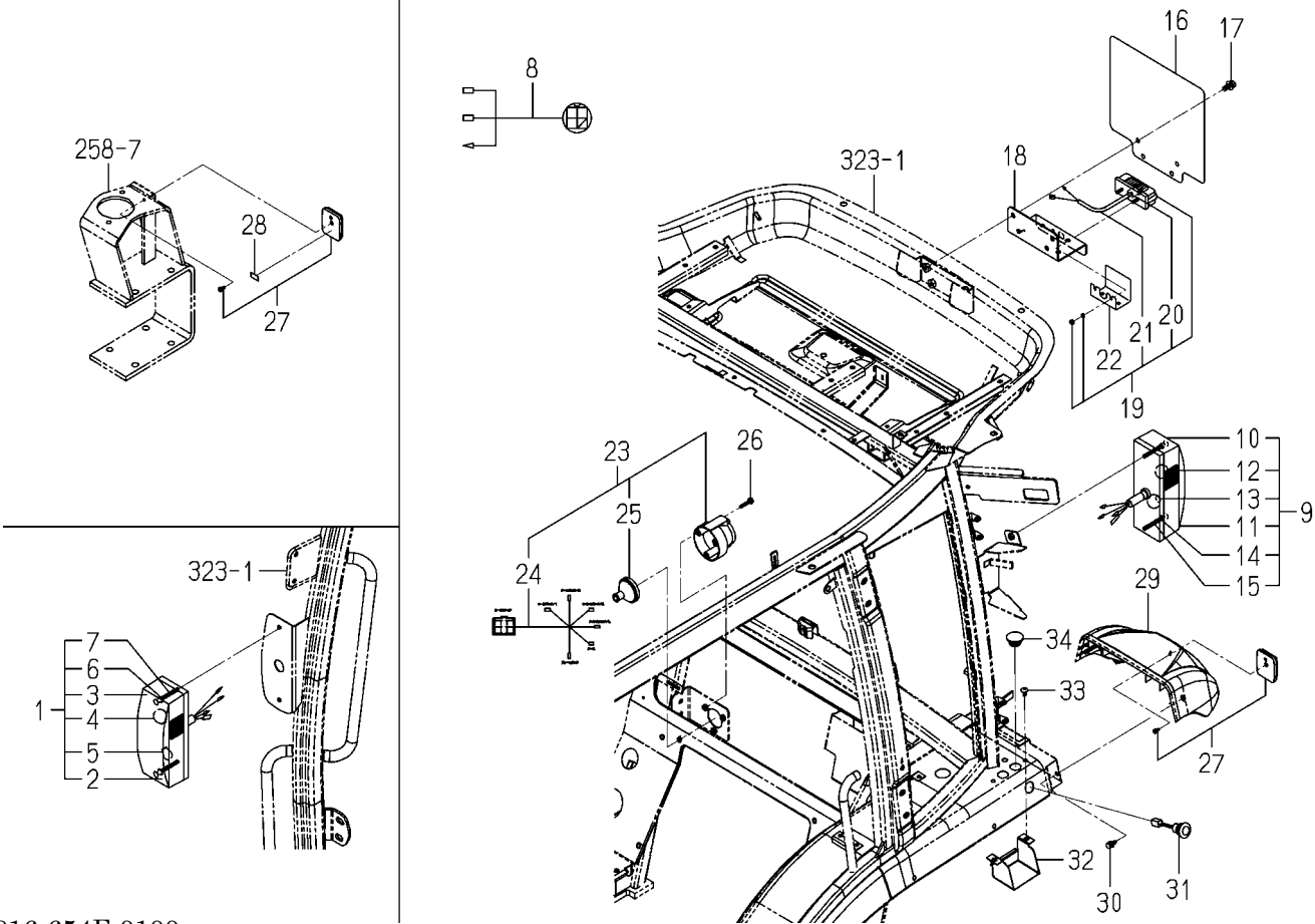
FIG.294 ELC.(FLOOR)SYSTEM(6495H TYPE)(1/2)
