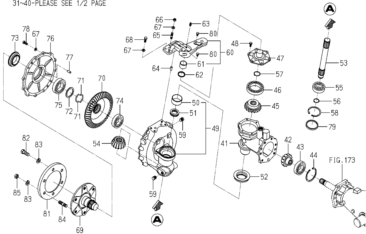
FIG.175 CASE(GEAR/FRONT)SYSTEM(2/2) (6495 TYPE/6495H TYPE)
