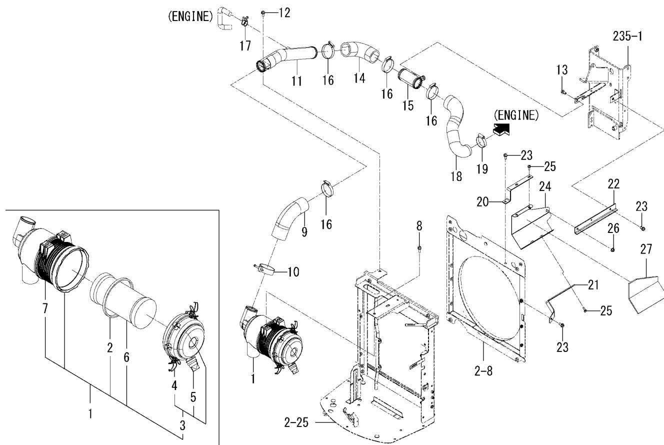
FIG. 15 CLEANER(AIR)SYSTEM(6405H TYPE)
