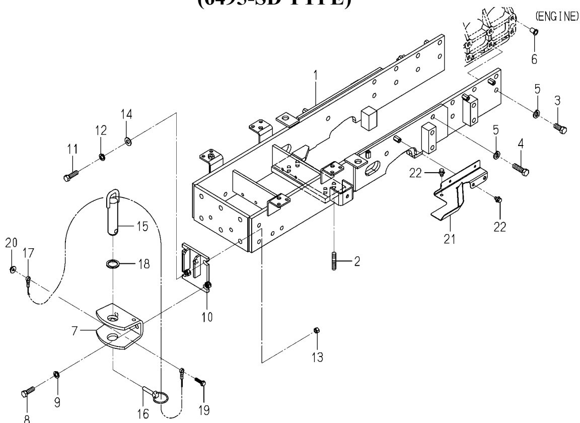
FIG.163 BRACKET(AXLE)SYSTEM (6495-SD TYPE)
