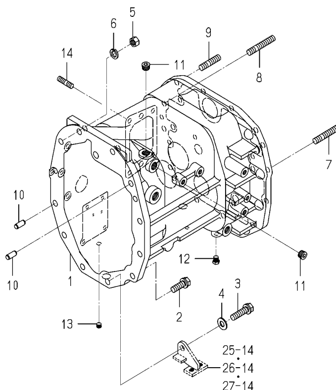
FIG. 64 CASE(TRANSMISSION/MID)SYSTEM (H TYPE)
