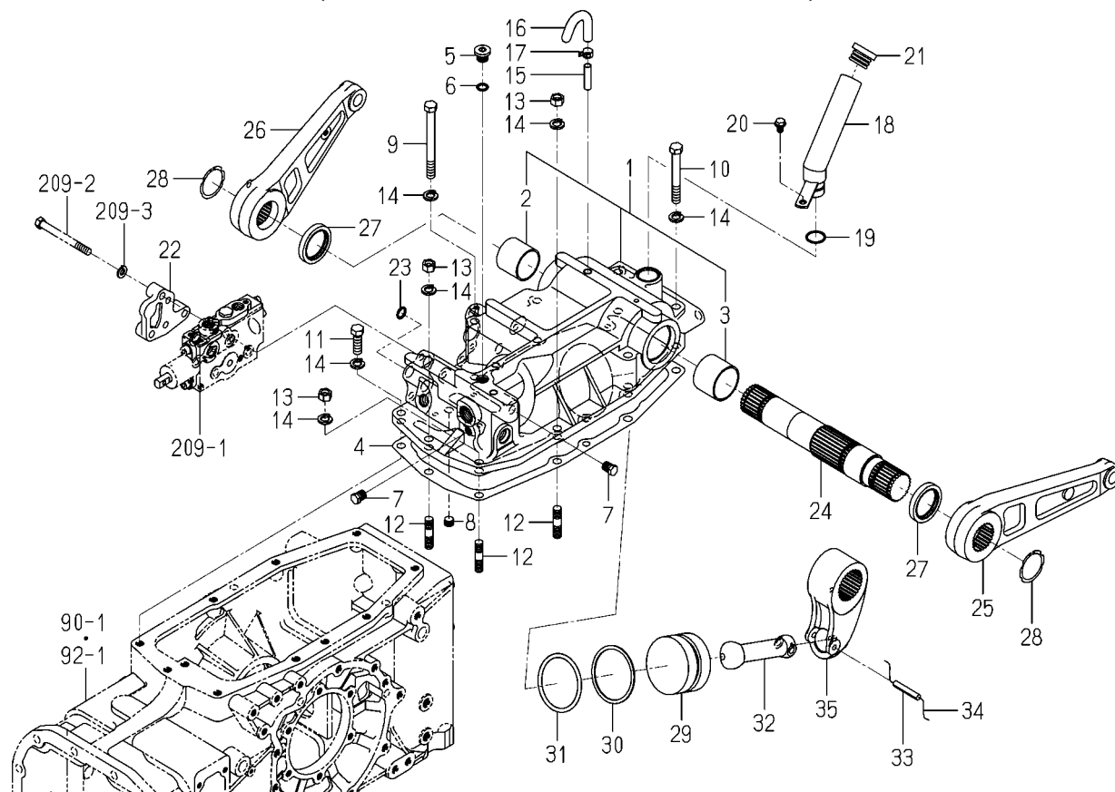
FIG.180 CASE(CYLINDER)SYSTEM (6375-SD TYPE/6405H TYPE)
