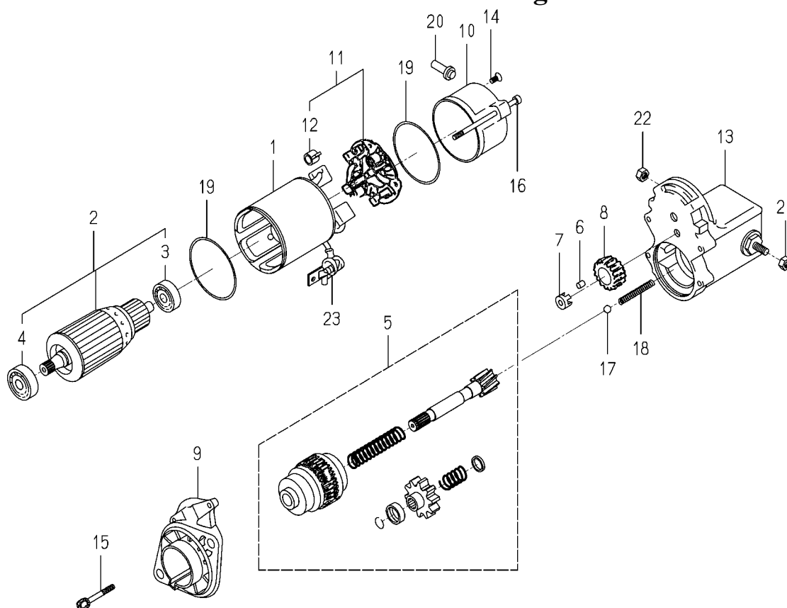
FIG. 31 COMPONENT PARTS FOR 6281-100-007-40 ON Fig.027
