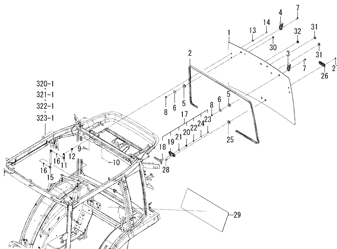
FIG.328 GLASS(REAR)SYSTEM(CY TYPE)
