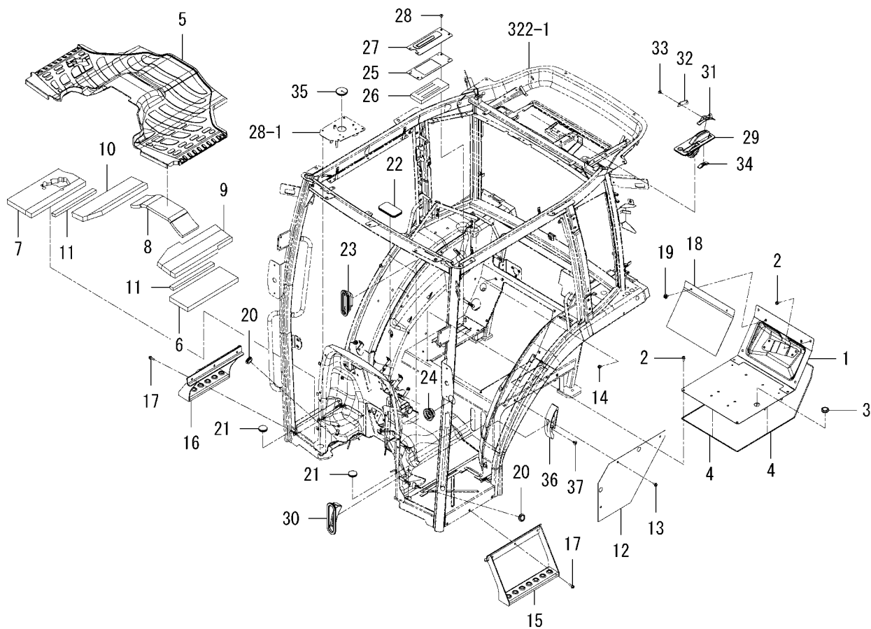
FIG.281 FLOOR(REAR)SYSTEM(6405H-CY TYPE)
