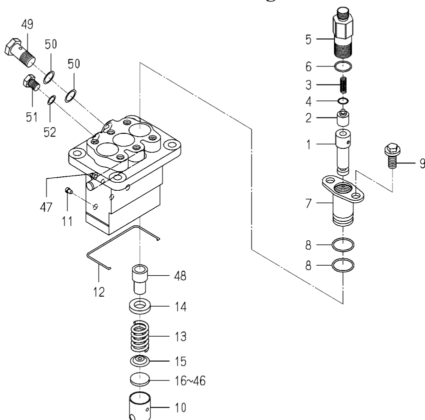
FIG. 39 COMPONENT PARTS FOR 6215-600-104-20 ON Fig.029
