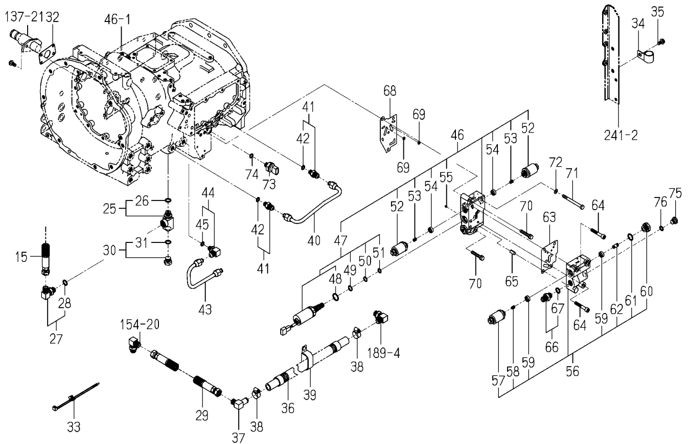
FIG.195 PIPING(SUB)SYSTEM(6375-G TYPE)(2/2)
