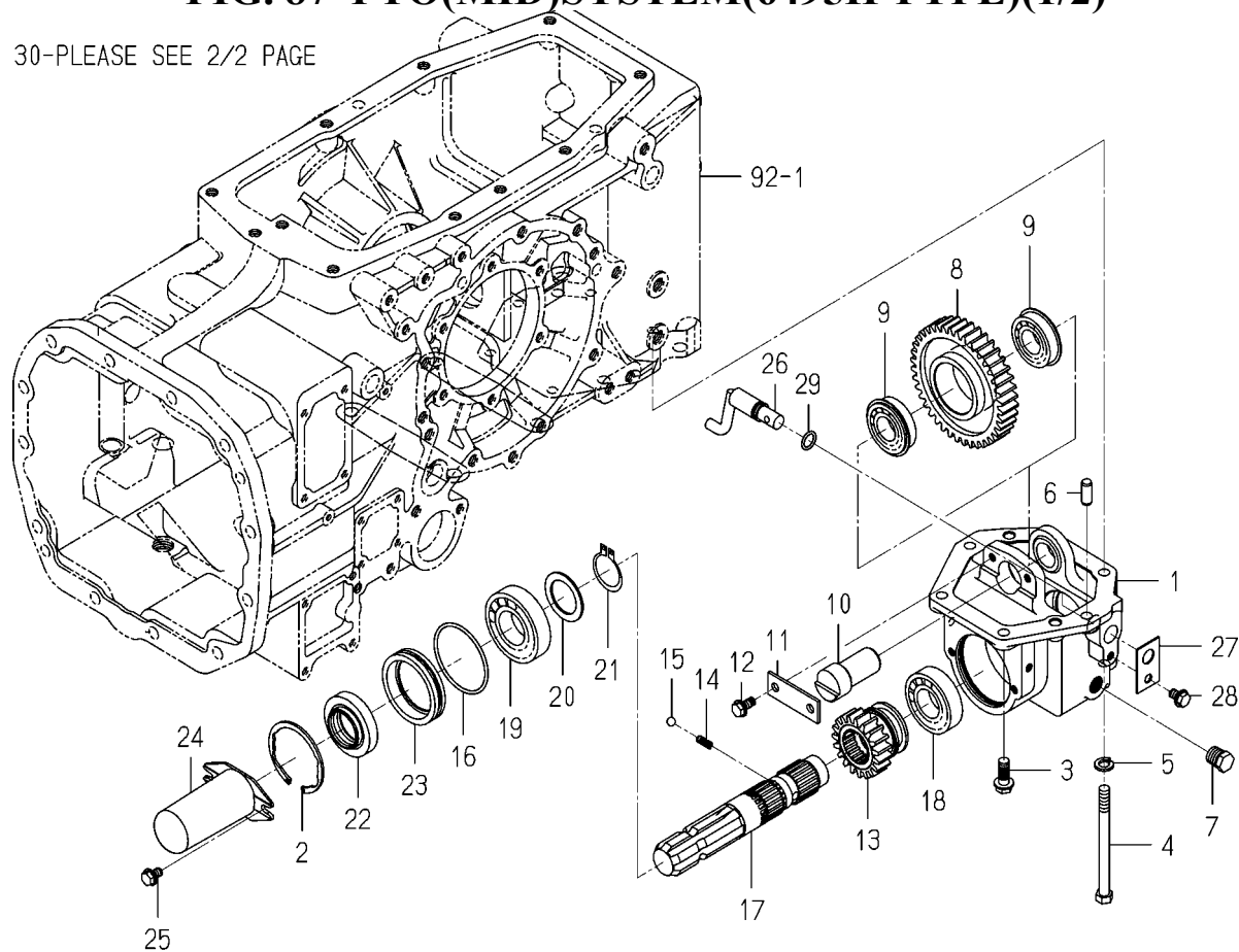
FIG. 87 PTO(MID)SYSTEM(6495H TYPE)(1/2)
