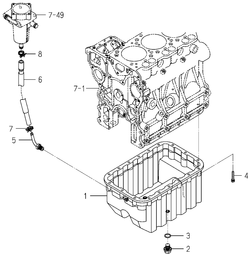
FIG. 9 OIL PAN
