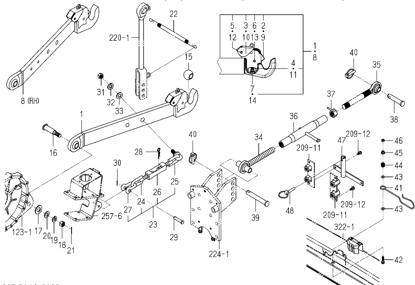
FIG.214 LINK(3P)SYSTEM(6405H-CY TYPE)
