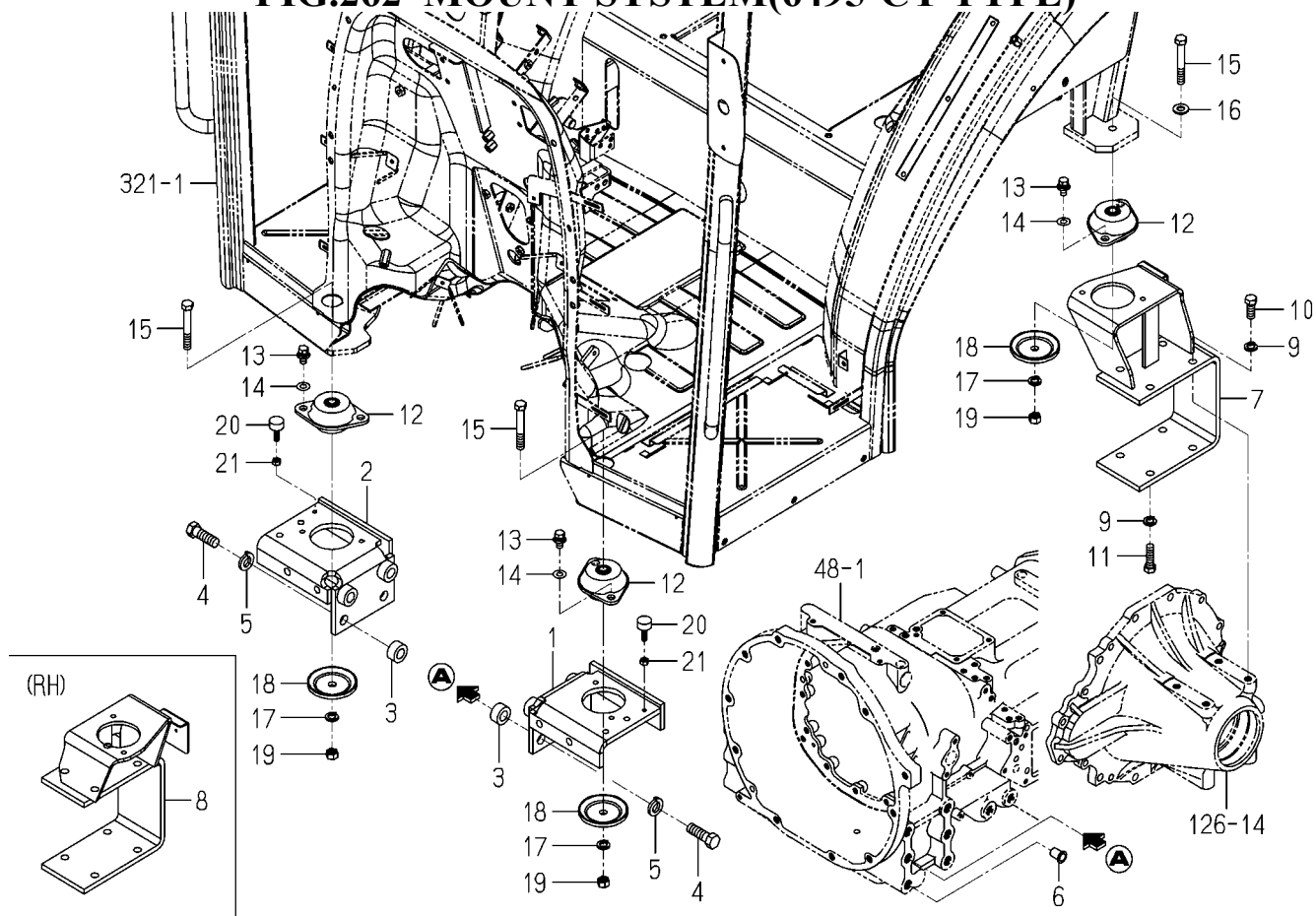
FIG.262 MOUNT SYSTEM(6495-CY TYPE)
