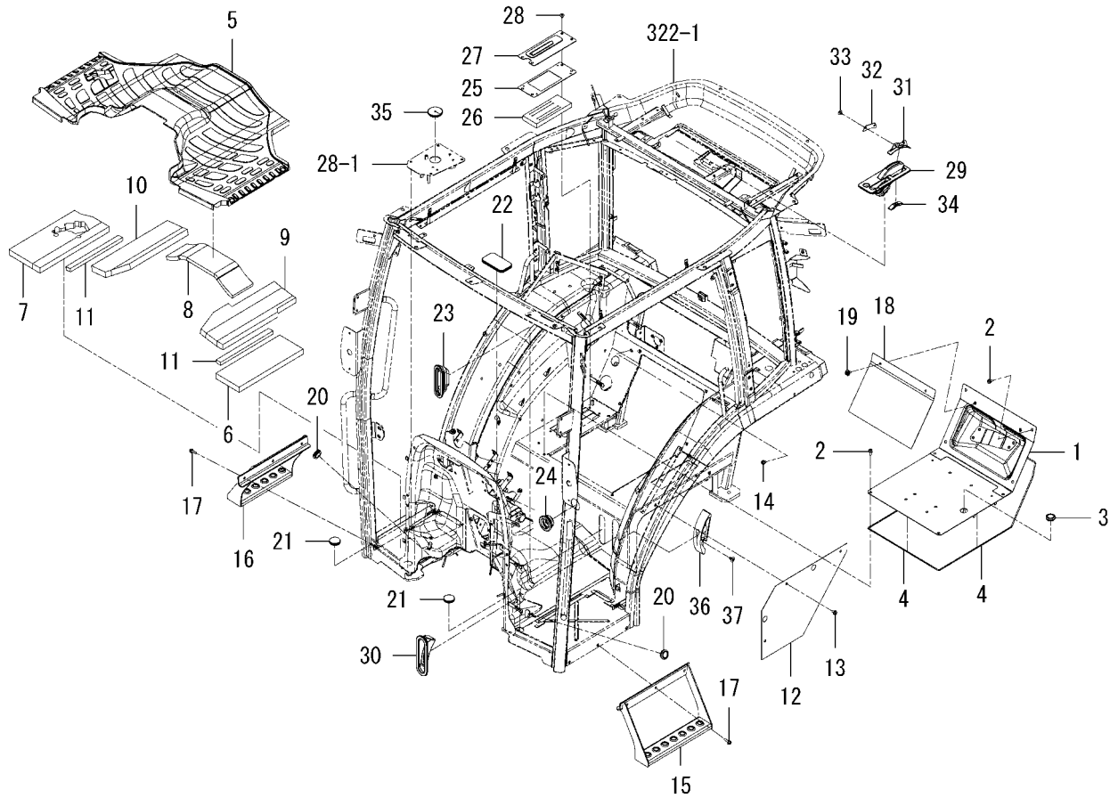
FIG.281 FLOOR(REAR)SYSTEM(6405H-CY TYPE)
