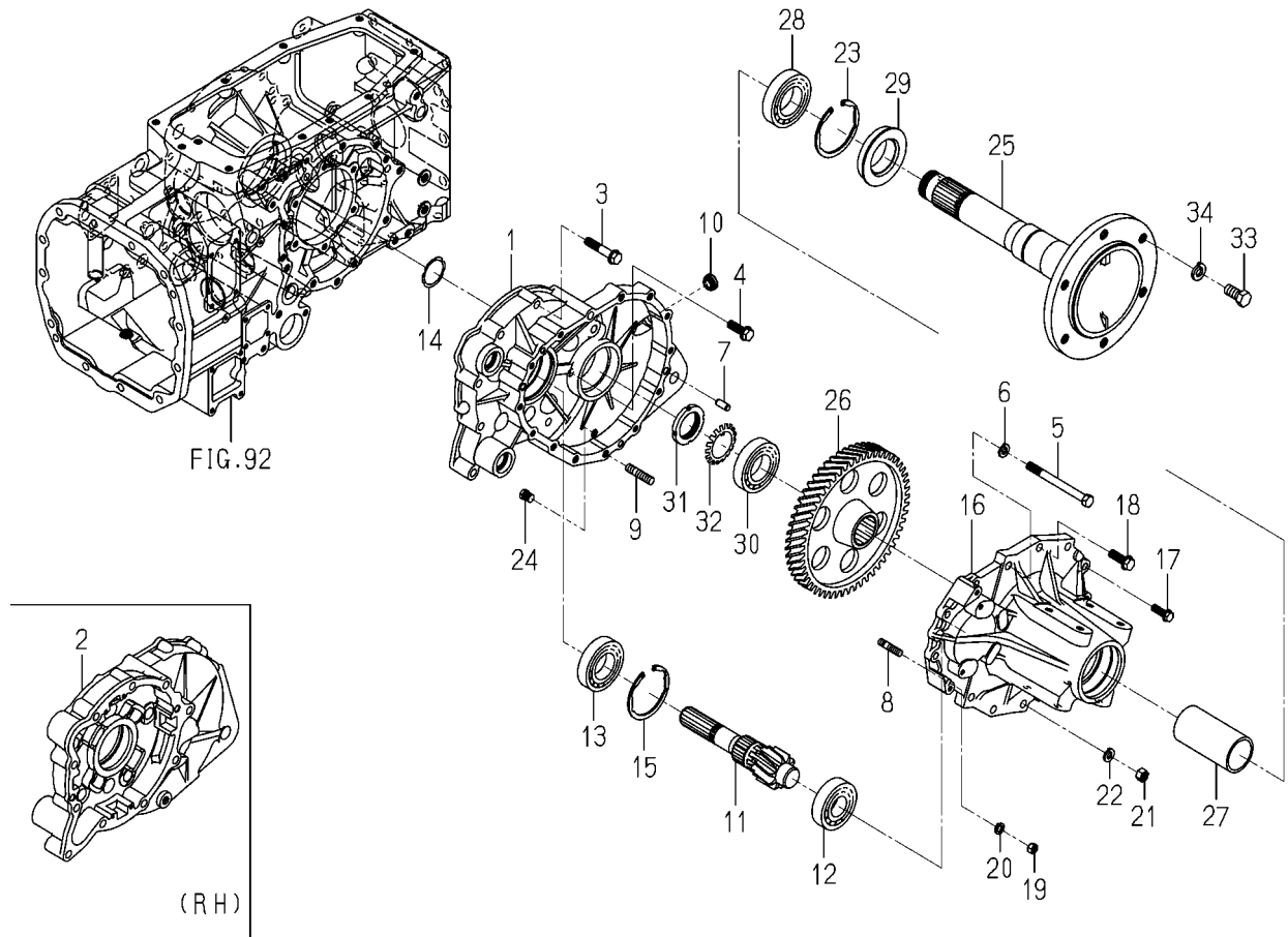
FIG.123 HOUSING(AXLE)SYSTEM(6405H TYPE)
