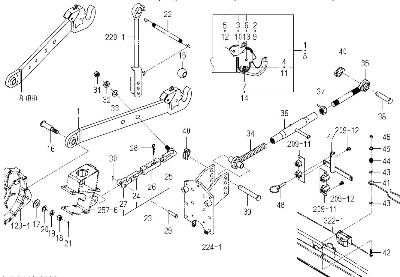
FIG.214 LINK(3P)SYSTEM(6405H-CY TYPE)
