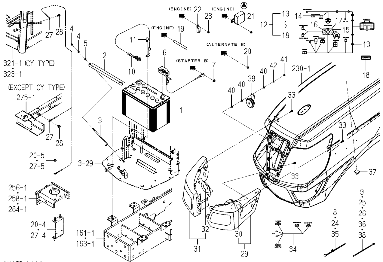
FIG.284 ELC.(FRONT)SYSTEM (6495-SD TYPE/6495H TYPE EXCEPT G)
