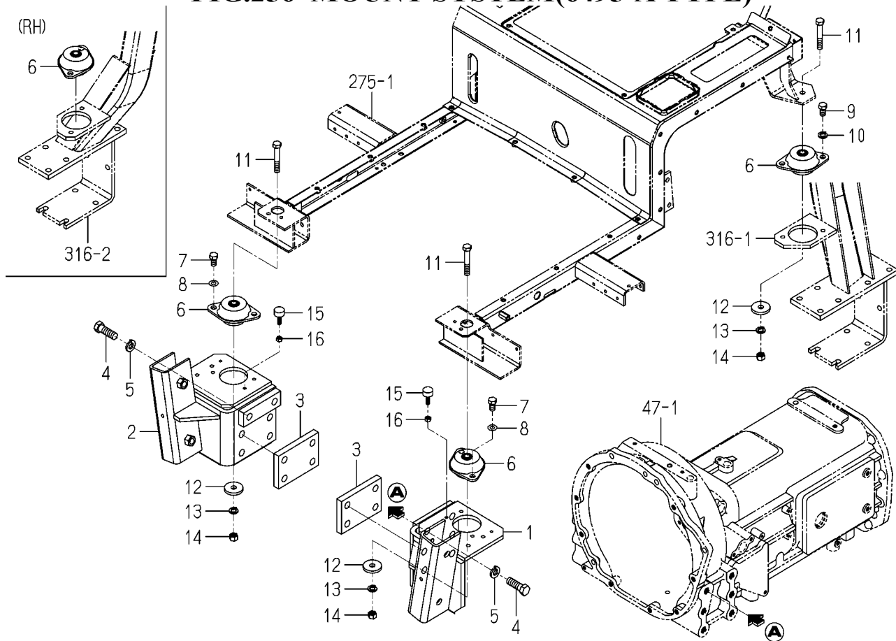
FIG.256 MOUNT SYSTEM(6495-A TYPE)
