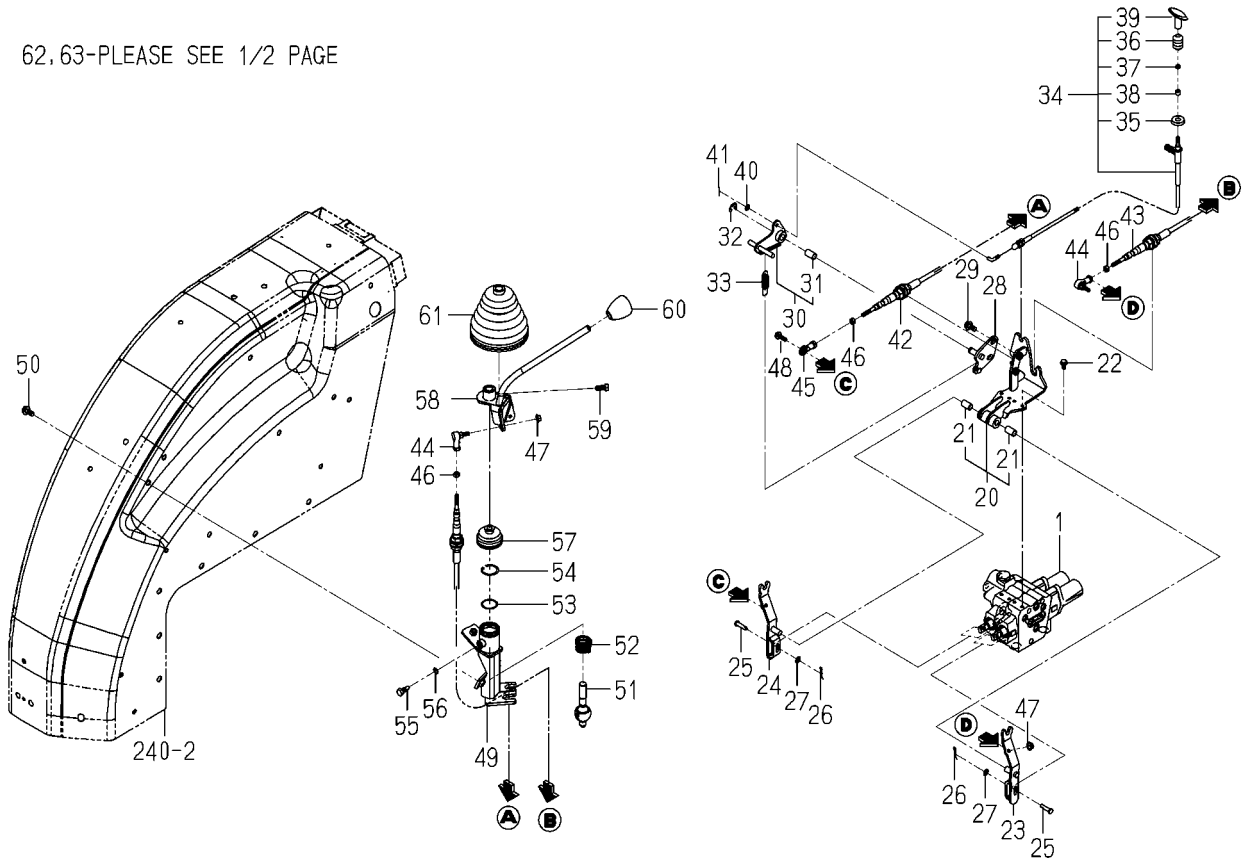
FIG.204 JOY STICK VALVE SYSTEM(2/2) (6495-SDA TYPE)
