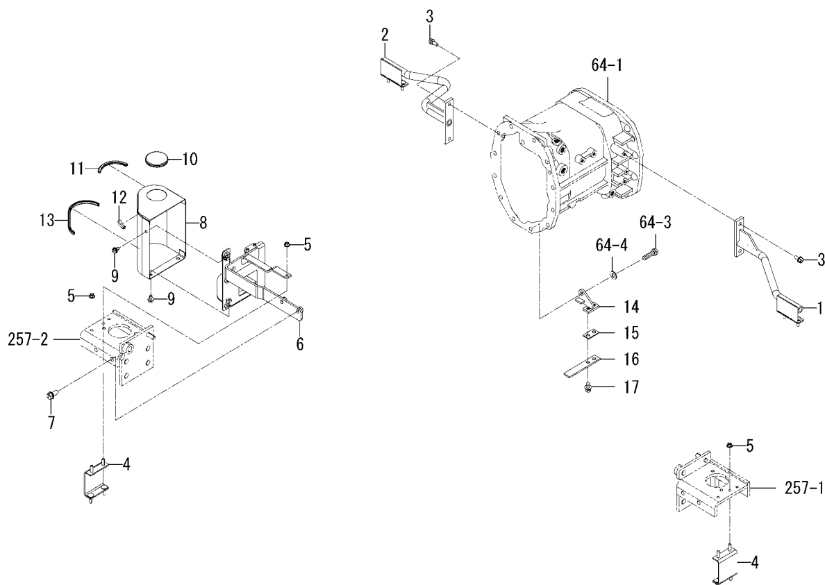
FIG. 26 STAY(TANK)SET SYSTEM (6405H-CY TYPE)
