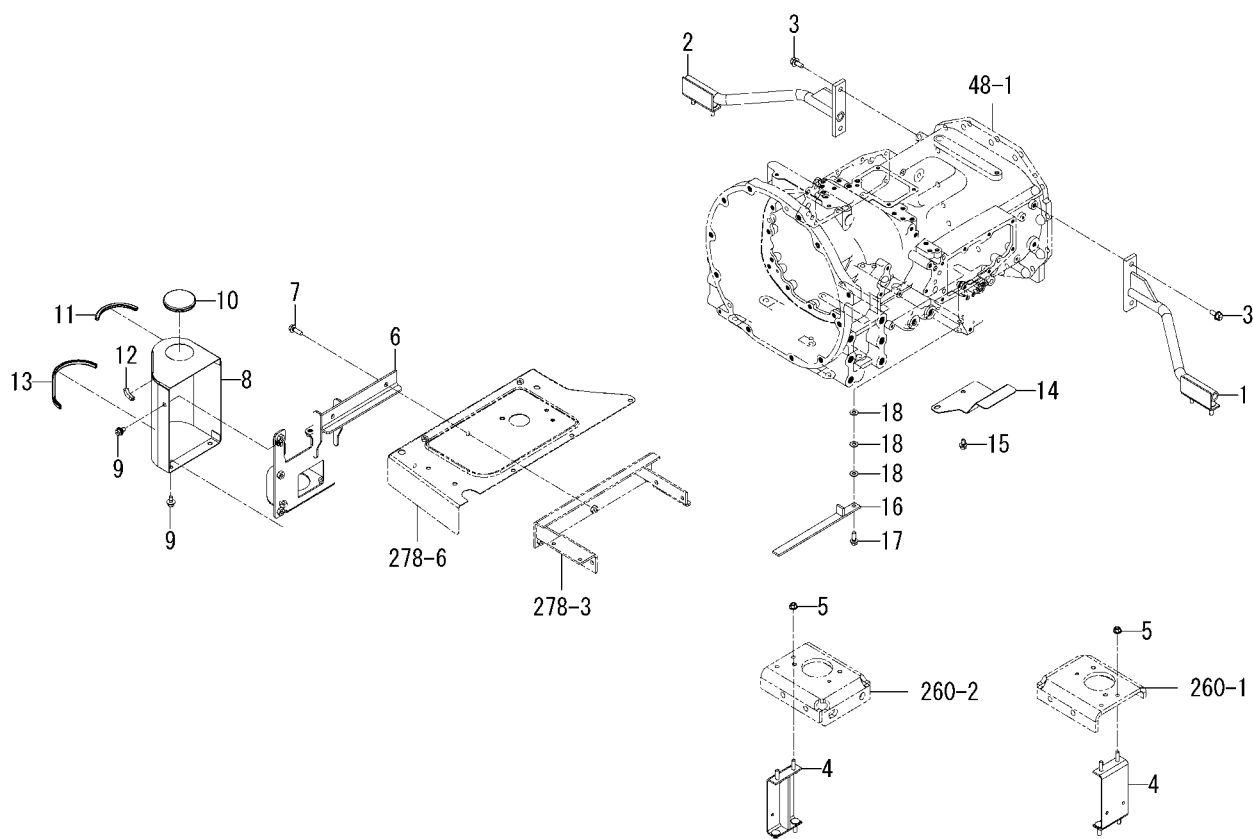
FIG. 22 STAY(TANK)SET SYSTEM (6495-GR TYPE)
