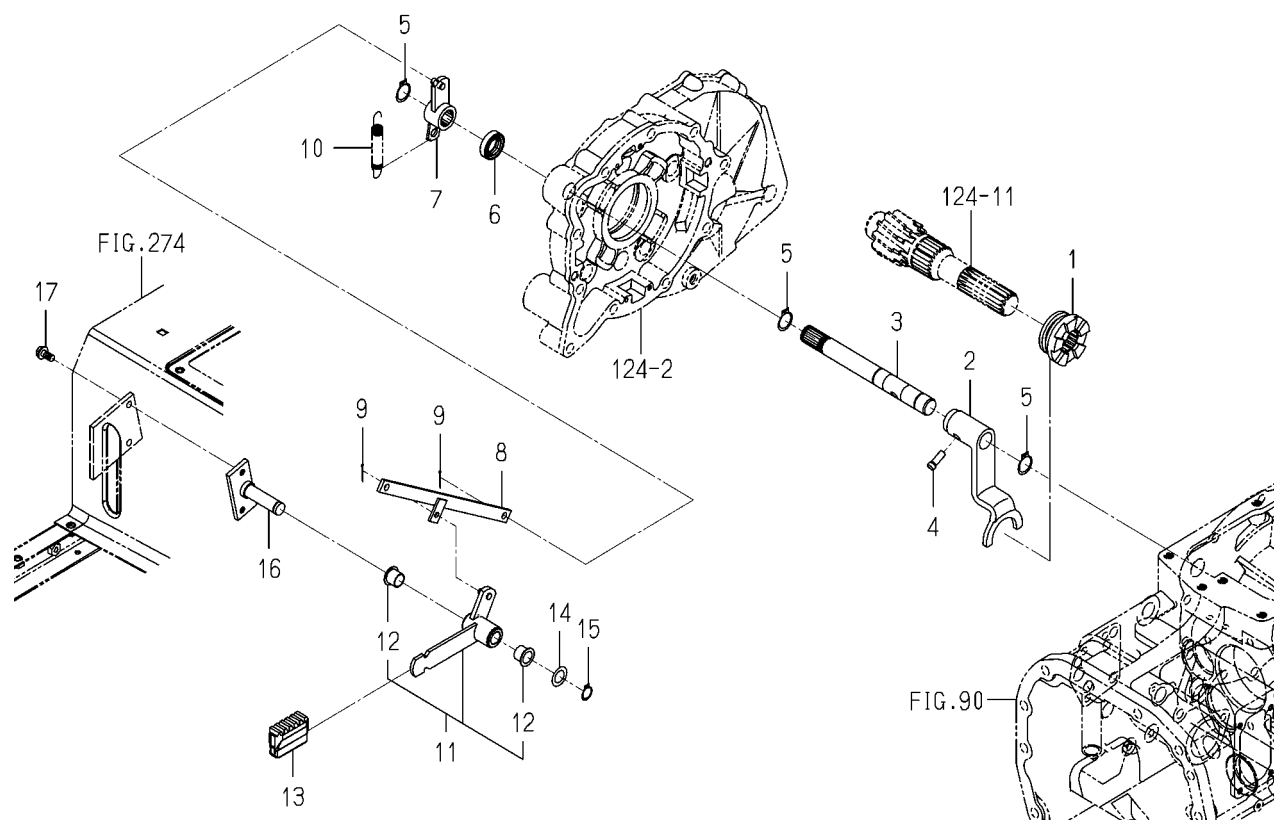
FIG.127 CLUTCH(DIFF-LOCK)SYSTEM (6375-SD TYPE)
