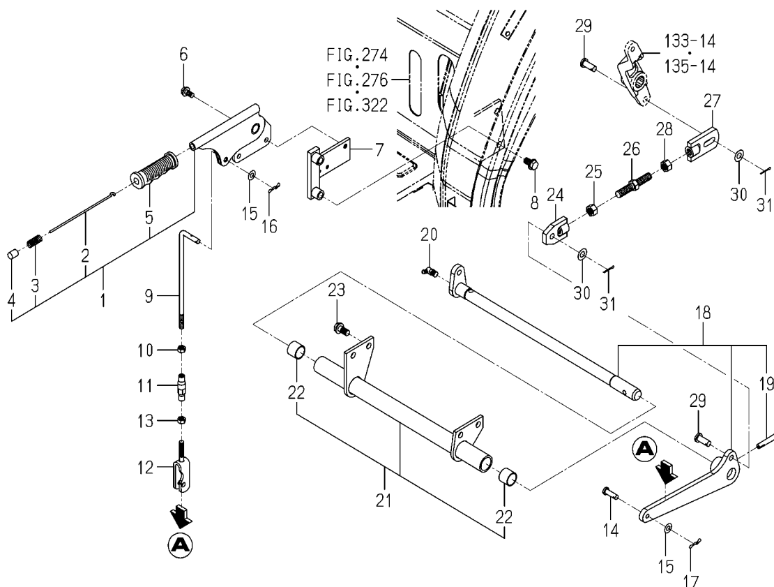
FIG.146 LEVER(BRAKE/PARKING)SYSTEM (6375-SD TYPE/6405H TYPE)
