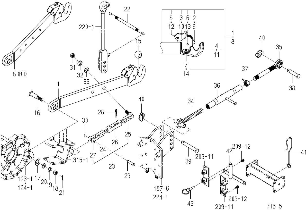
FIG.212 LINK(3P)SYSTEM (6375-SD TYPE/6405H-R TYPE)
