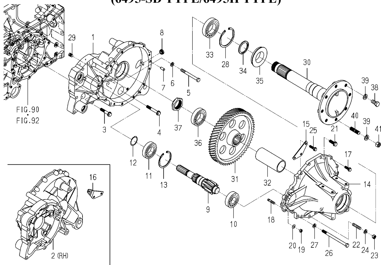
FIG.125 HOUSING(AXLE)SYSTEM (6495-SD TYPE/6495H TYPE)
