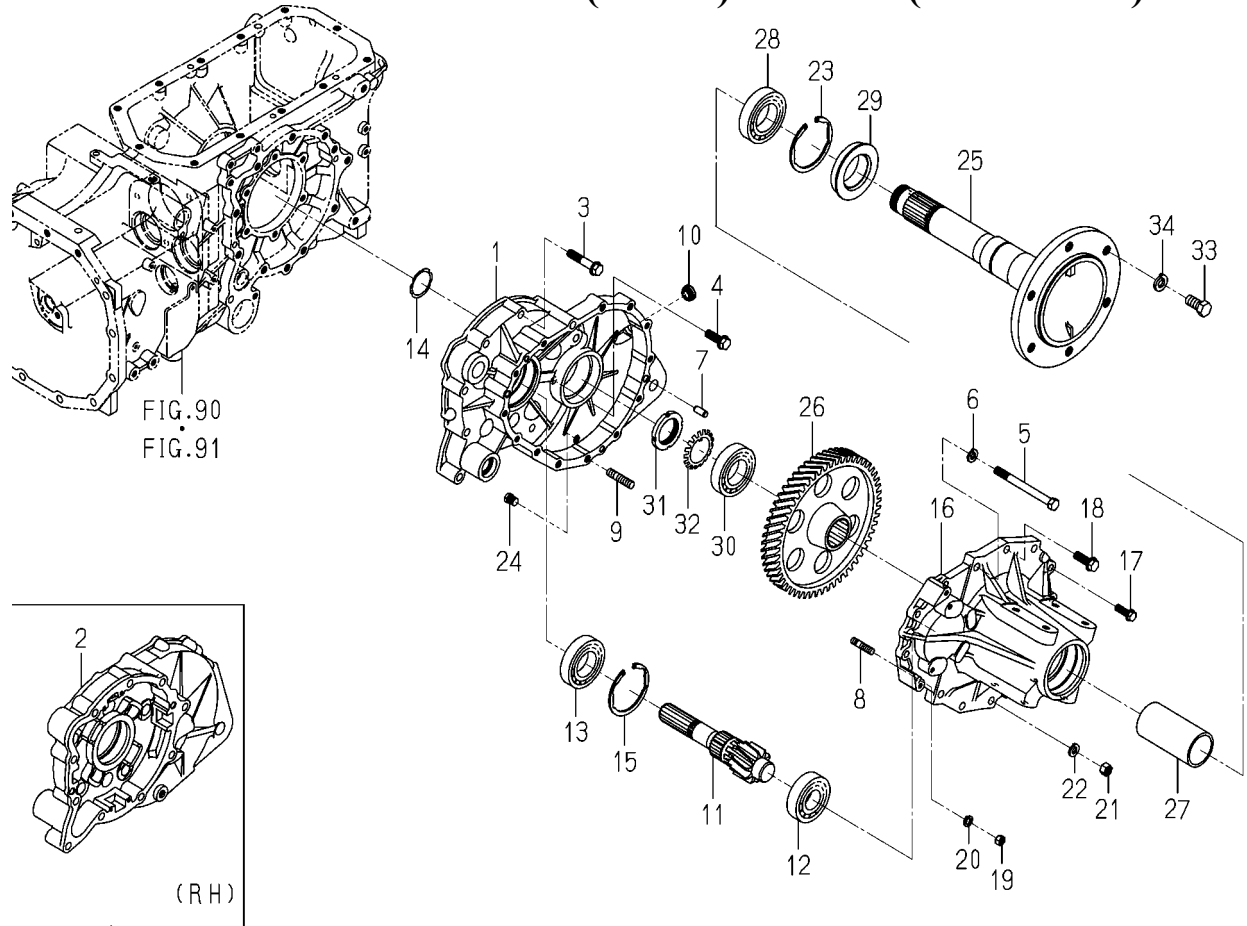
FIG.124 HOUSING(AXLE)SYSTEM(6375 TYPE)
