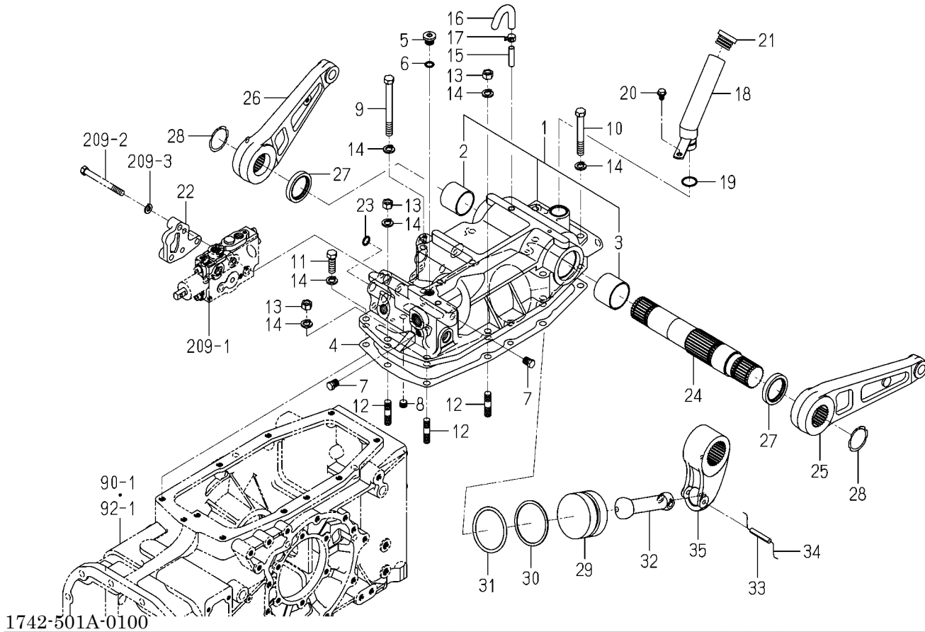
FIG.180 CASE(CYLINDER)SYSTEM (6375-SD TYPE/6405H TYPE)
