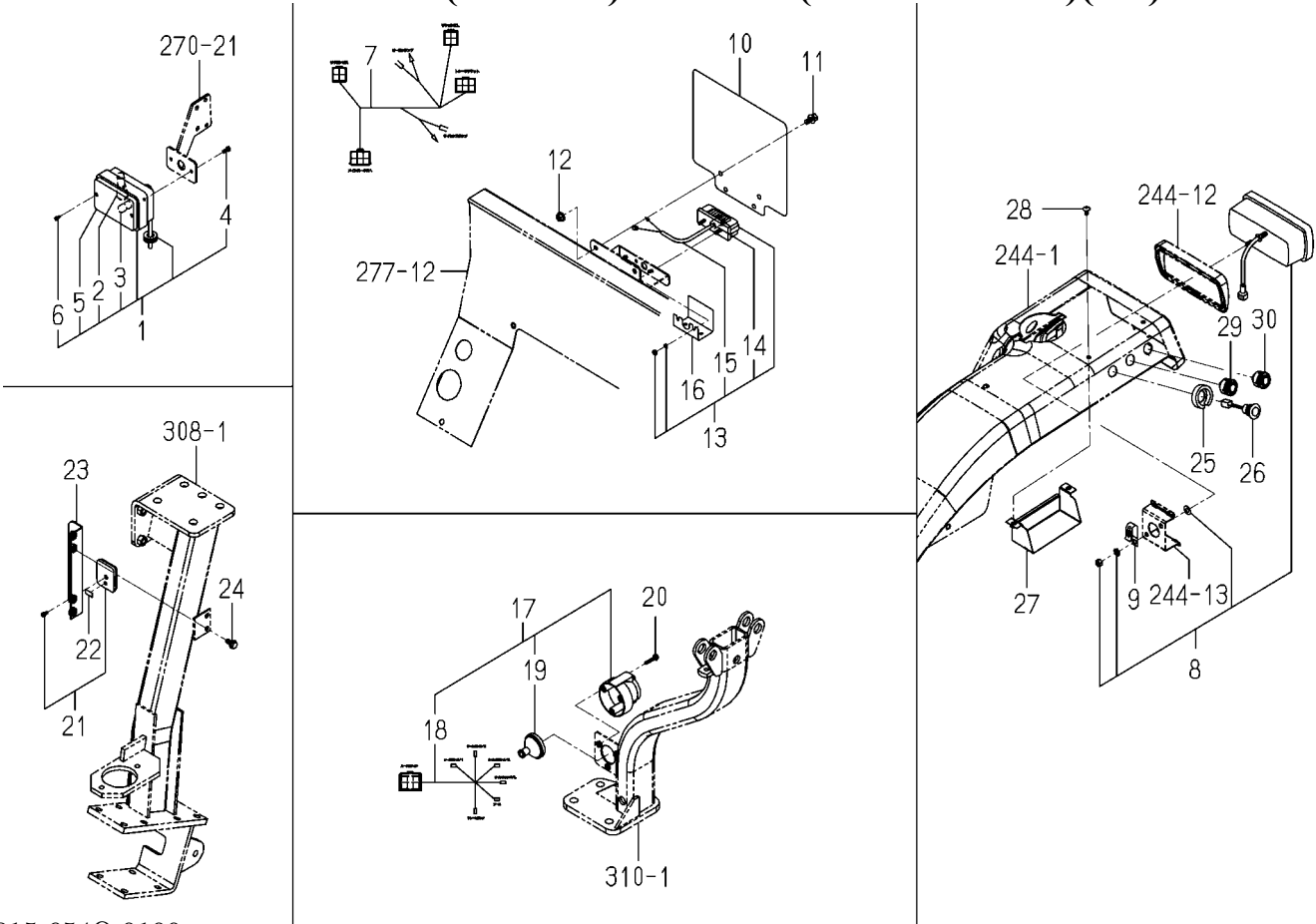
FIG.300 ELC.(FLOOR)SYSTEM(6375-R TYPE)(1/2)
