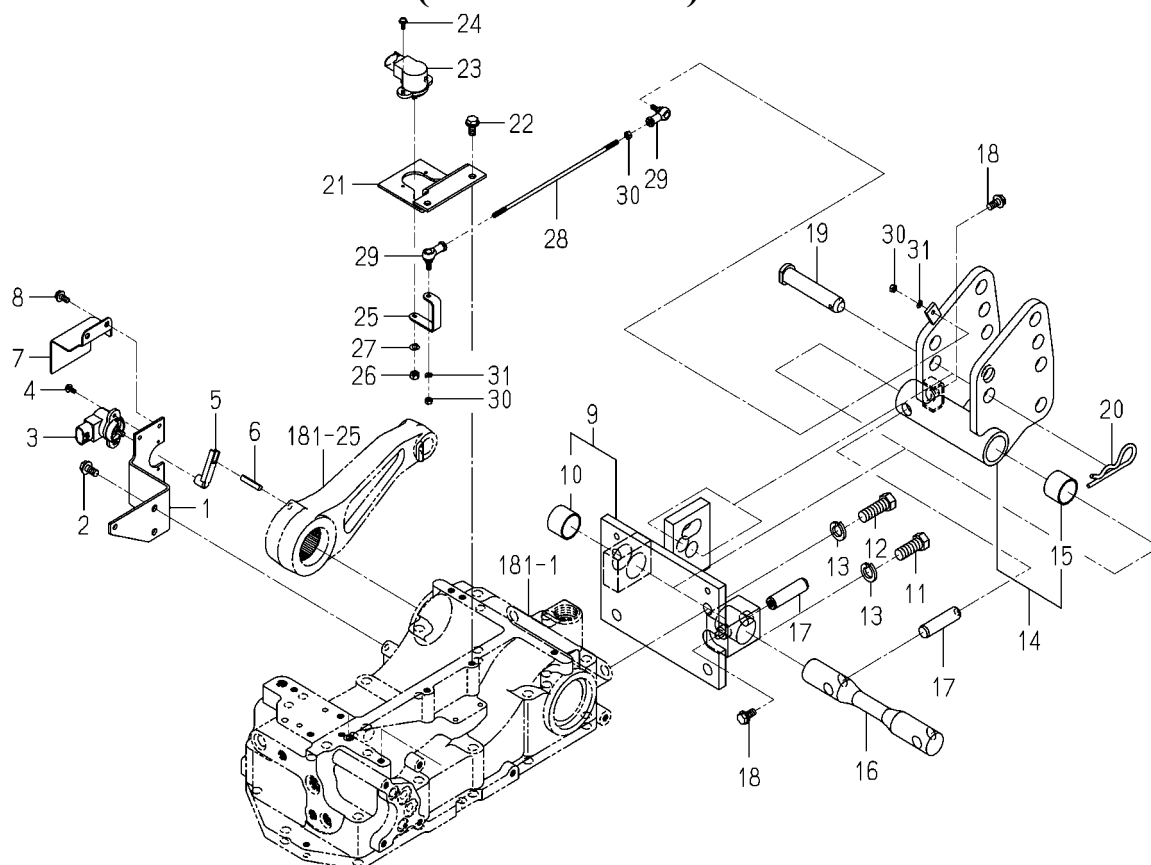
FIG.186 CONTROL(POSITION/DRAFT)SYSTEM (6495-G TYPE)
