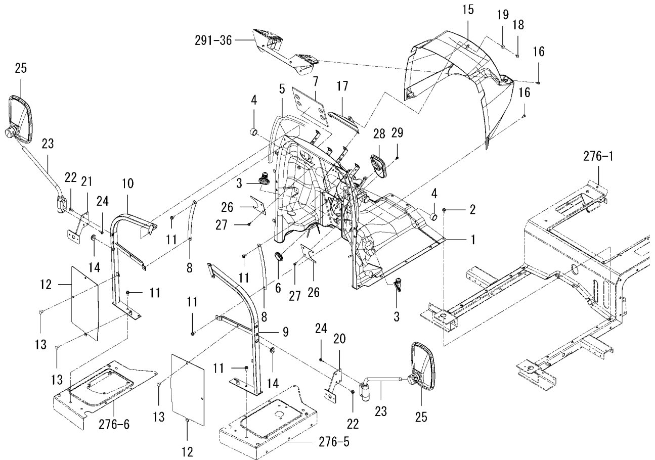
FIG.269 PANEL(DASH)SYSTEM(6405-R TYPE)
