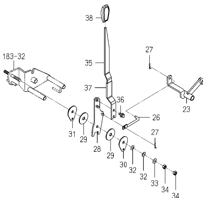
FIG.187 LEVER(DRAFT)SYSTEM(2/2) (6375-SD TYPE)
