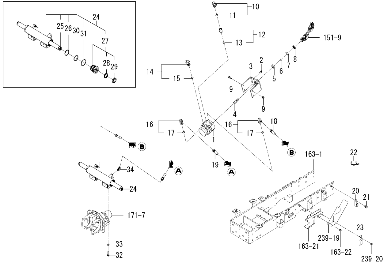
FIG.157 STEERING(POWER)SYSTEM (6495-SD TYPE)
