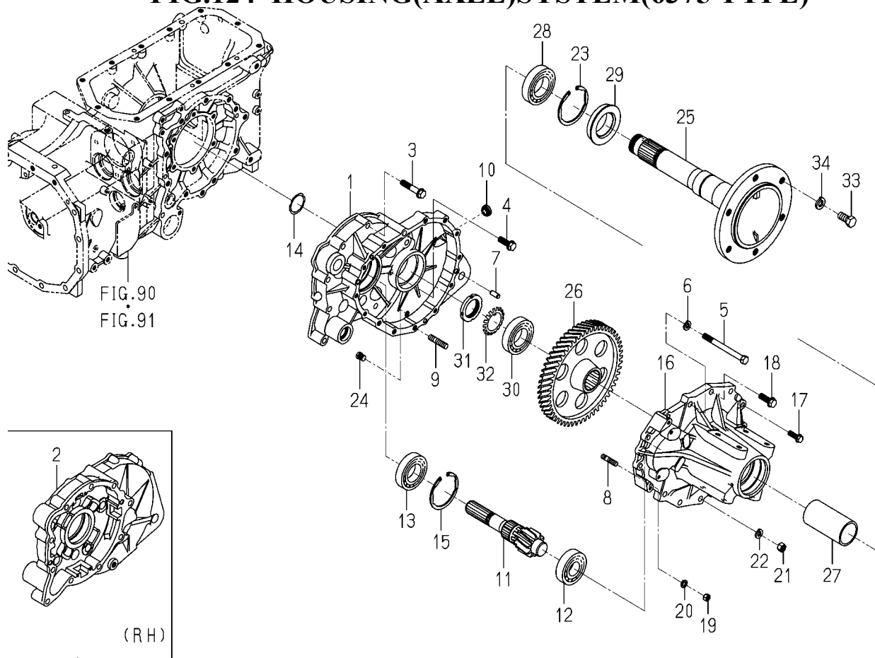
FIG.124 HOUSING(AXLE)SYSTEM(6375 TYPE)
