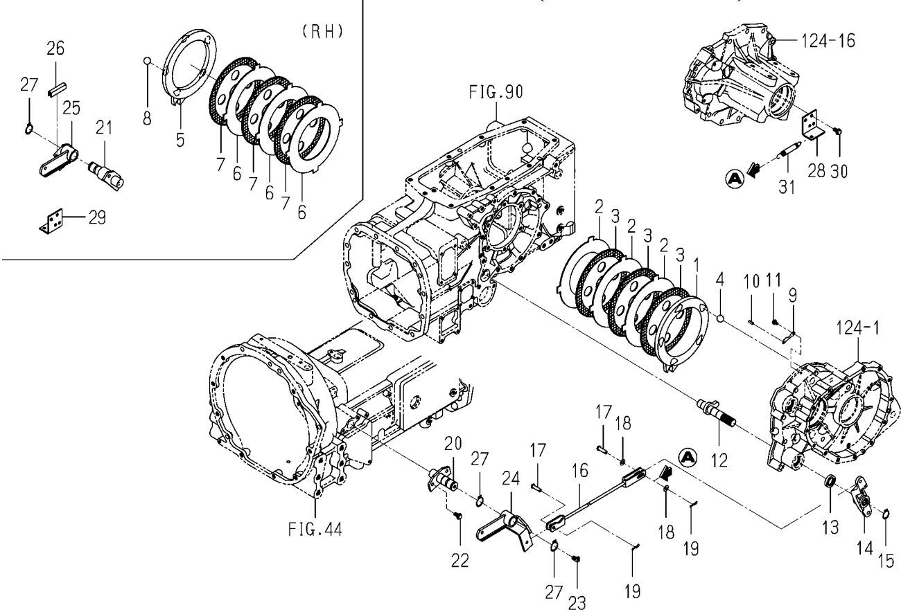
FIG.135 BRAKE SYSTEM(6375-SD TYPE)
