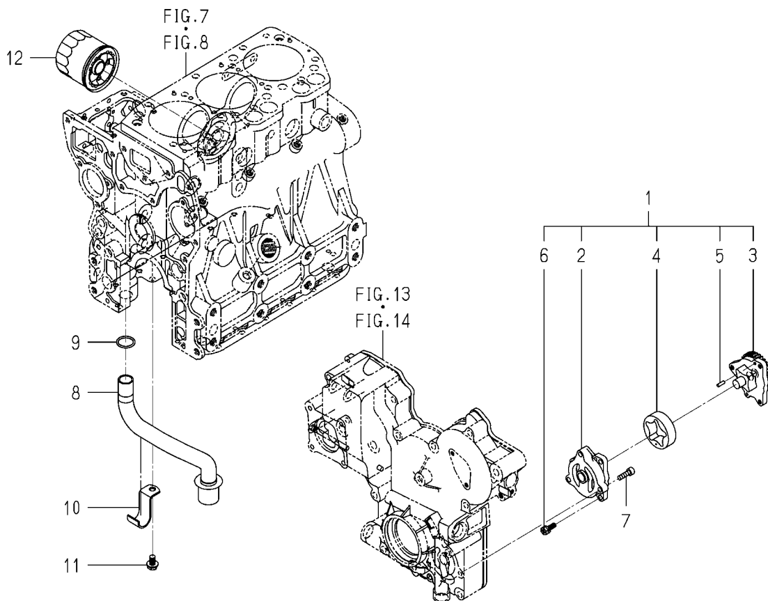
FIG. 24 OIL PUMP
