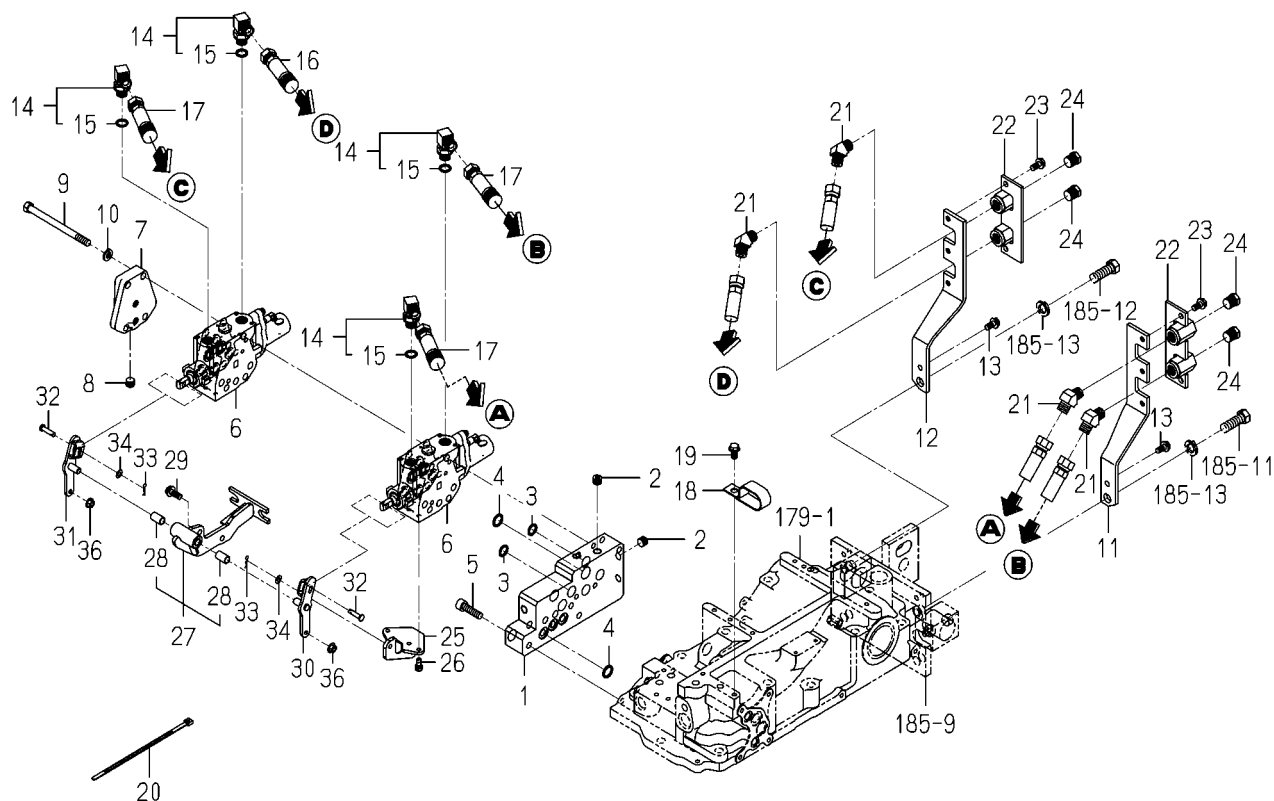
FIG.211 VALVE(REMOTE/2)SET SYSTEM(1/2) (6375-G TYPE)
