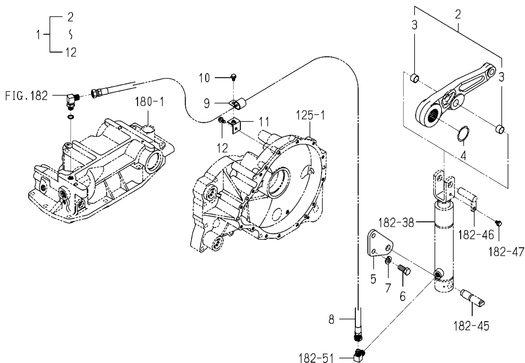
FIG.365 CYLINDER(SUB/LH)SET (6495-SD TYPE/6495H TYPE)(OPTION)
