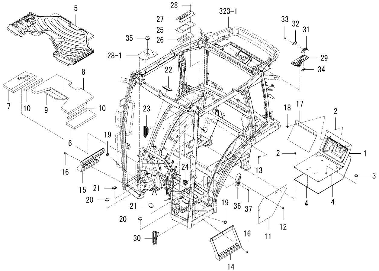
FIG.282 FLOOR(REAR)SYSTEM(6495H TYPE)
