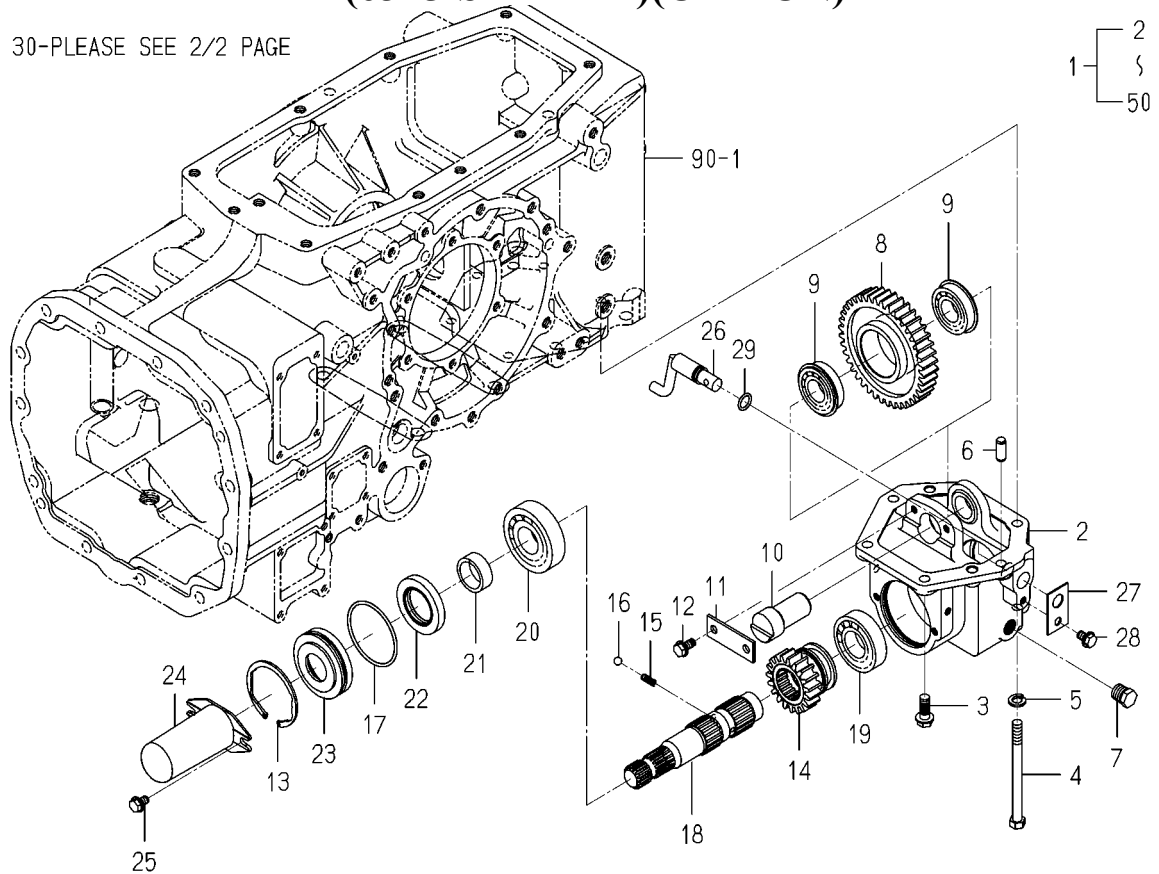
FIG.349 PTO(MID)SYSTEM(1/2) (6375-SD TYPE)(OPTION)
