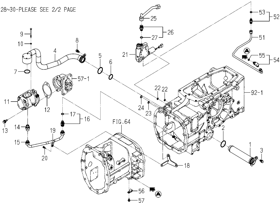
FIG.193 PIPING(MAIN)SYSTEM(1/2) (6405-H TYPE)
