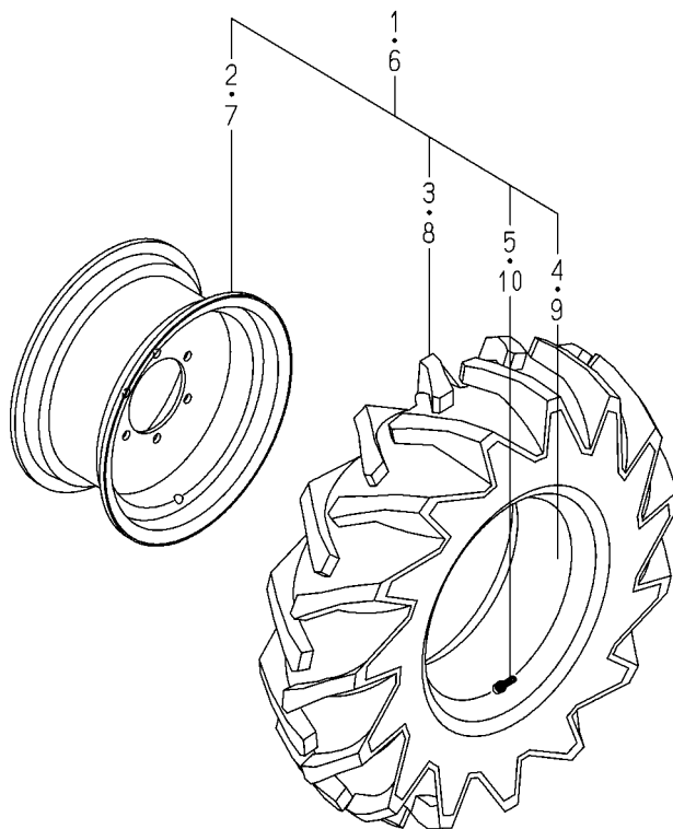
FIG.358 WHEEL(FRONT/9.5-16)ASSY (6495 TYPE/6495H TYPE)(OPTION)
