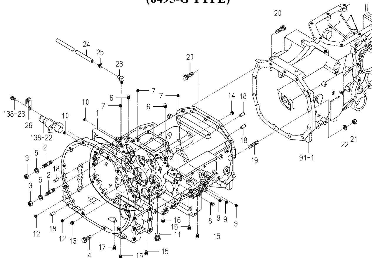
FIG. 48 CASE(TRANSMISSION)SYSTEM (6495-G TYPE)
