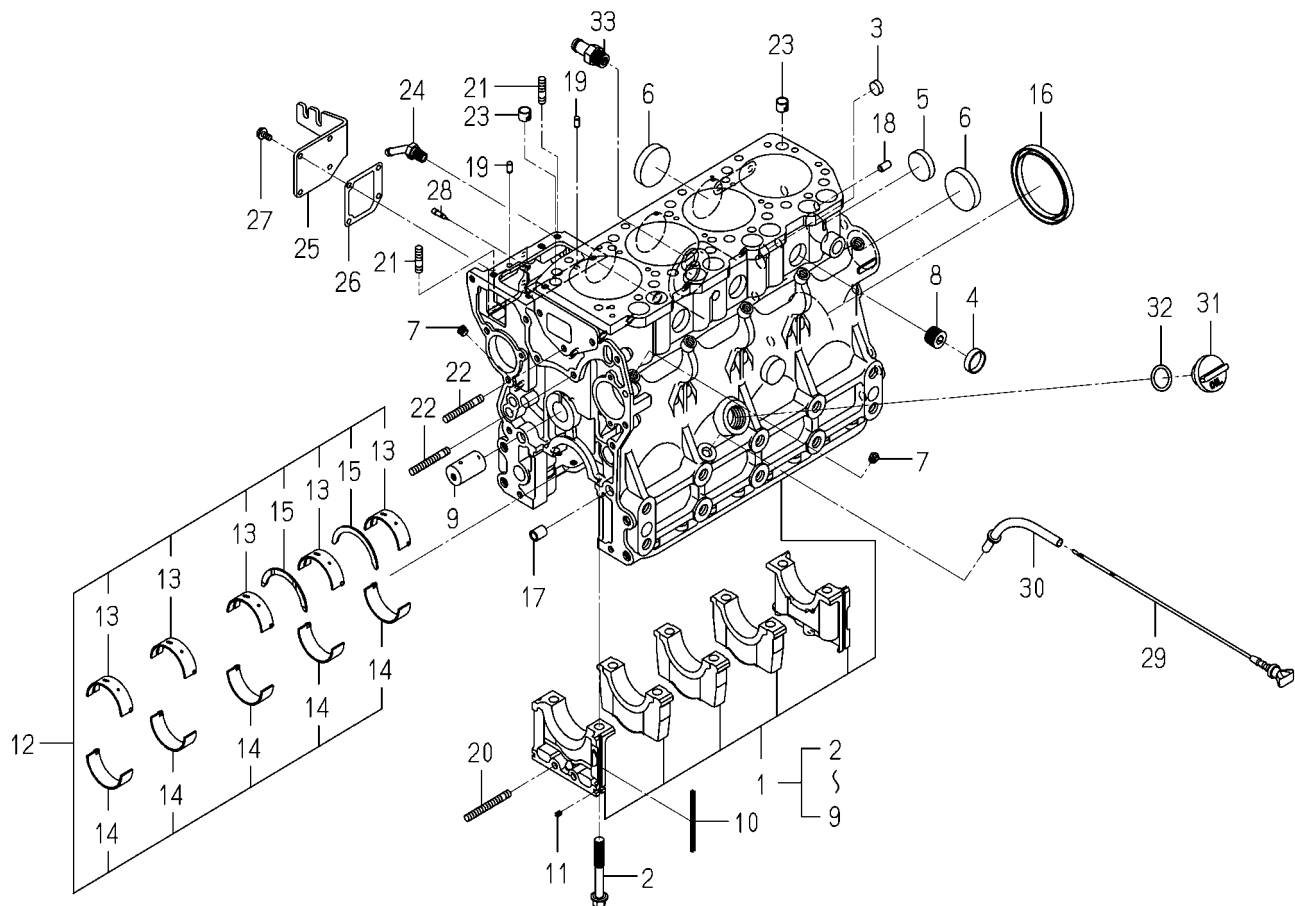
FIG. 11 CYLINDER BLOCK
