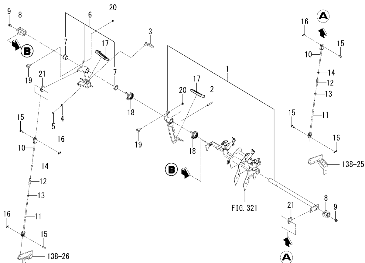
FIG.143 PEDAL(BRAKE)SYSTEM(6495-CY TYPE)
