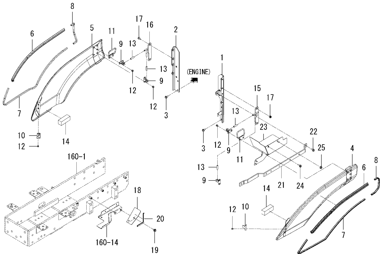
FIG.238 COVER(SIDE)SYSTEM(6405H TYPE)
