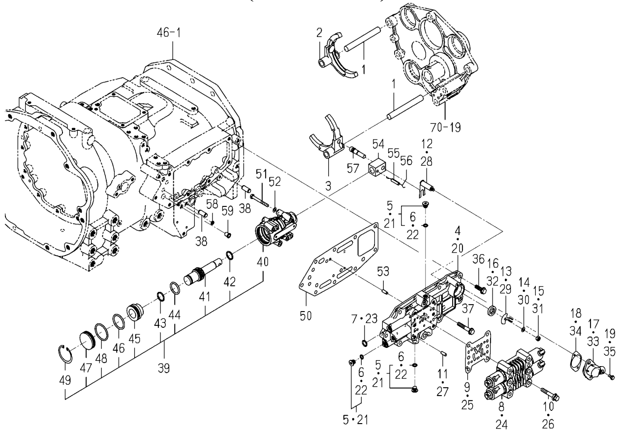
FIG. 95 FORK(SHIFT/MAIN)SYSTEM (6375-G TYPE)
