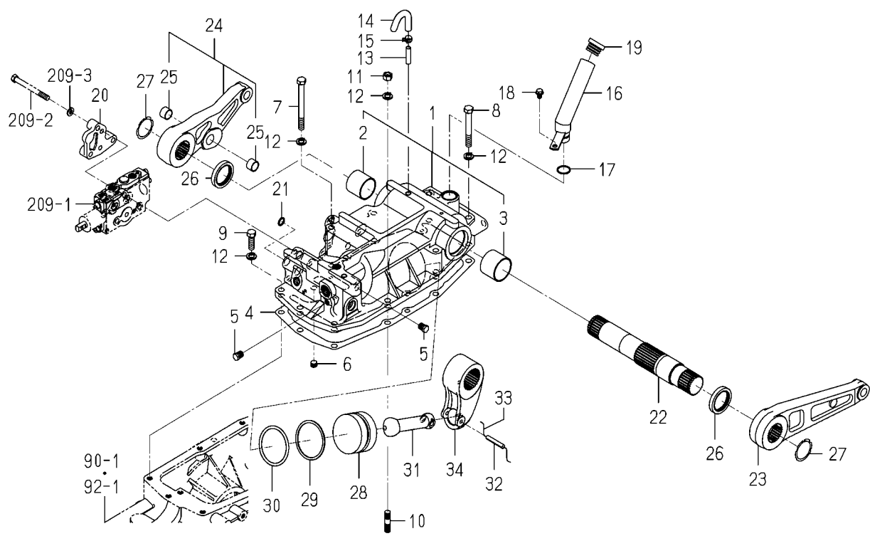
FIG.182 CASE(CYLINDER)SYSTEM(1/2) (6495-SD TYPE/6495H TYPE)
