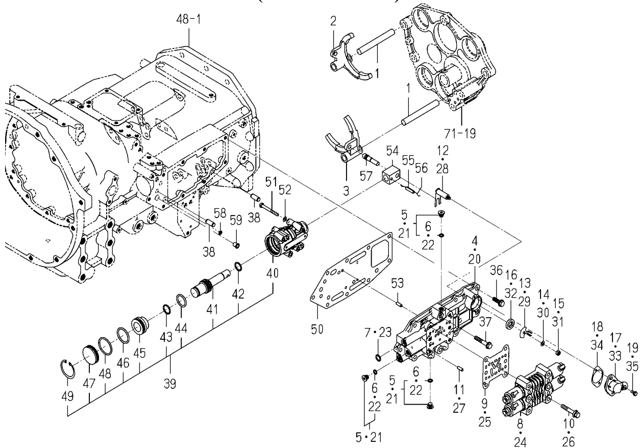
FIG. 96 FORK(SHIFT/MAIN)SYSTEM (6495-G TYPE)
