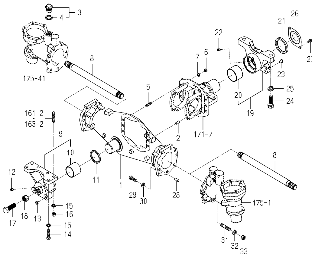
FIG.173 HOUSING(AXLE/FRONT)SYSTEM (6495 TYPE/6495H TYPE)
