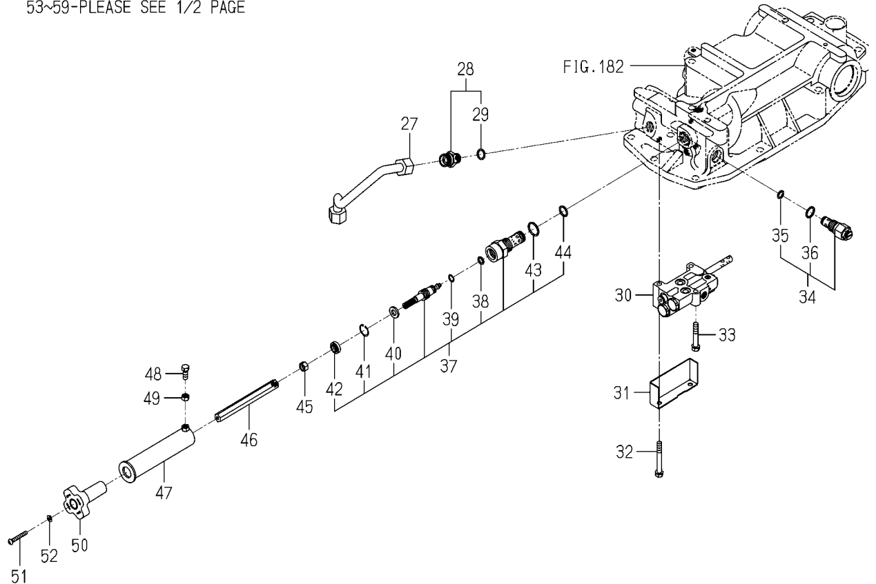
FIG.192 PIPING(MAIN)SYSTEM(2/2) (6495-H TYPE)
