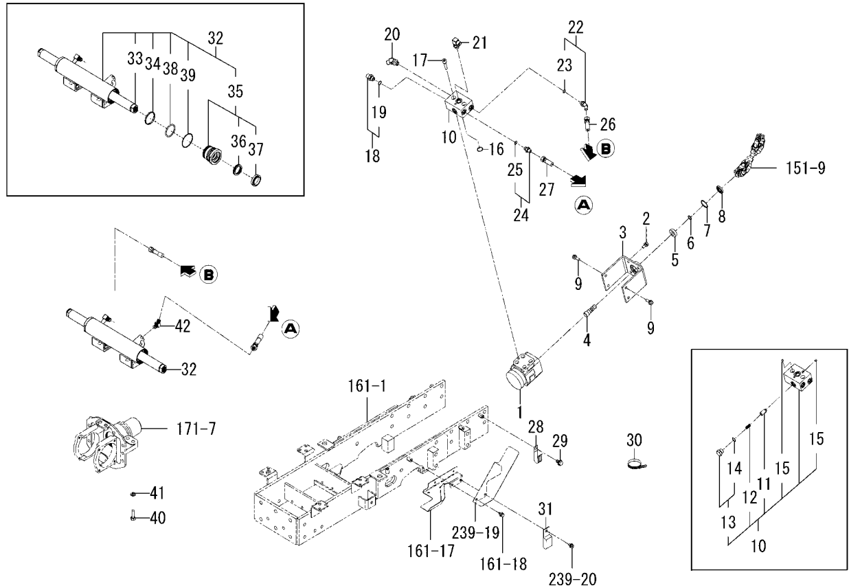
FIG.158 STEERING(POWER)SYSTEM (6495H TYPE)
