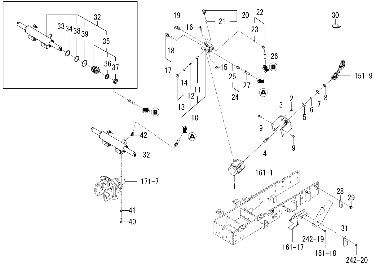
FIG.155 STEERING(POWER)SYSTEM (6495-G TYPE/6495H TYPE)
