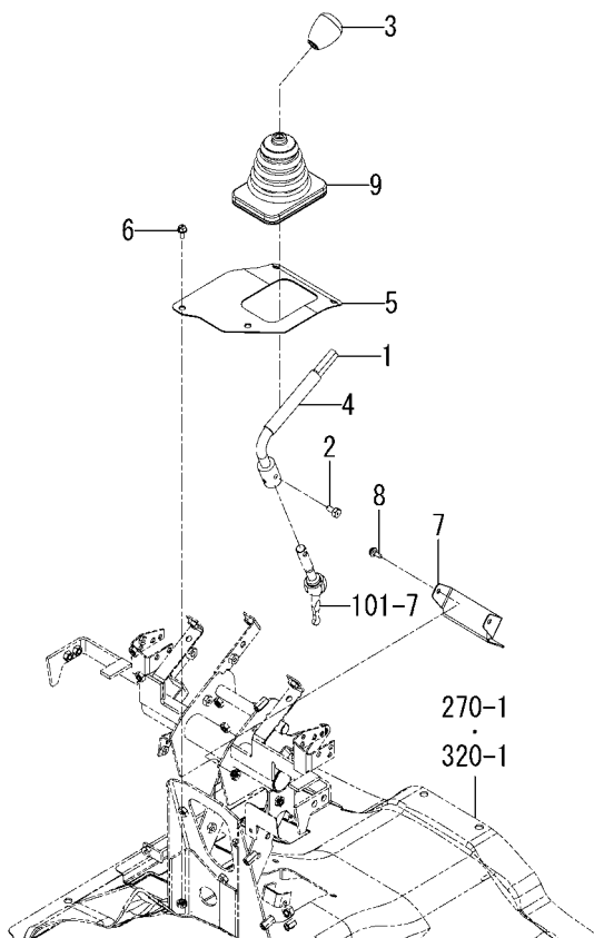
FIG.117 LEVER(PTO)SYSTEM(6375-G TYPE)
