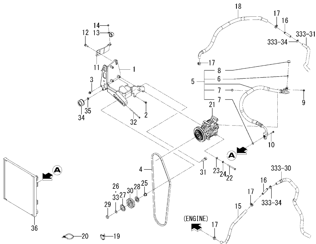
FIG.332 AIR CONDITIONER(1/2) (ENGINE)SYSTEM (6375-CY TYPE)
