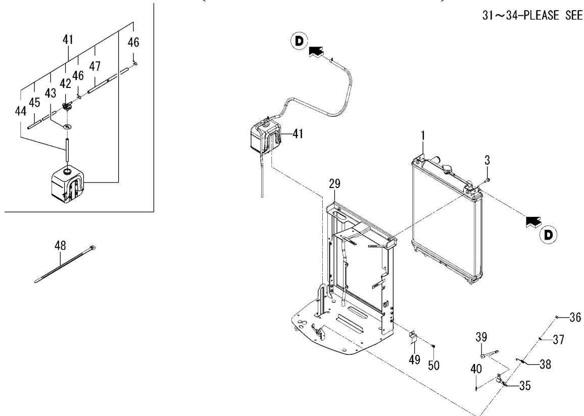
FIG. 3 RADIATOR SYSTEM(2/2) (6495 TYPE/6495H TYPE)
