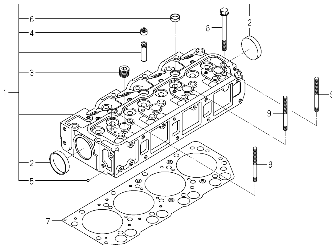
FIG. 4 CYLINDER HEAD
