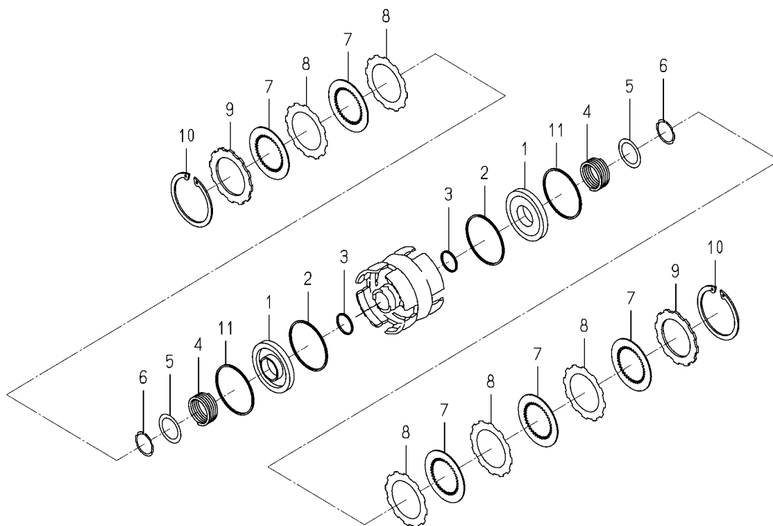
FIG.389 COMPONENT PARTS FOR 1729-218-310-20 ON FIG.80
