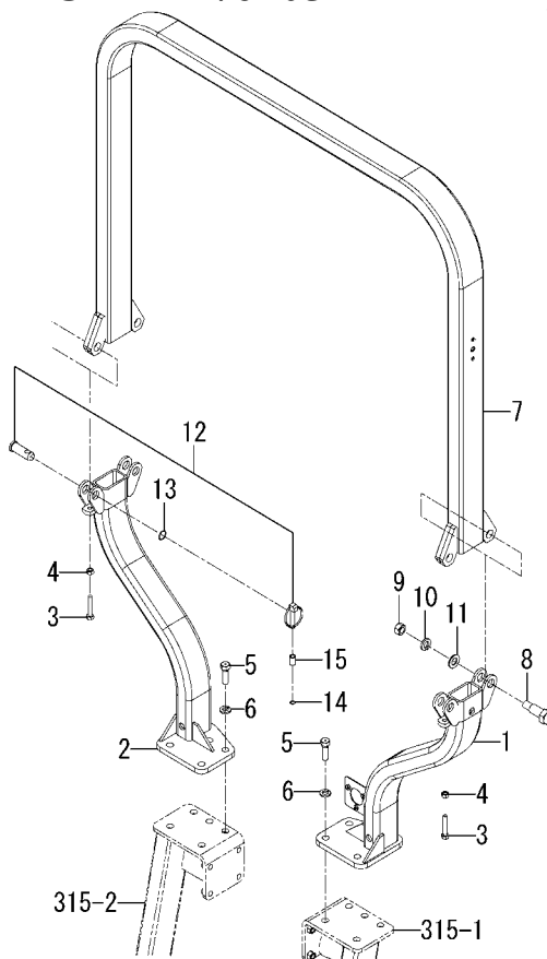
FIG.312 FLAME(UPPER)SYSTEM(6375-SD TYPE EXCEPT A/6405H-R TYPE)
