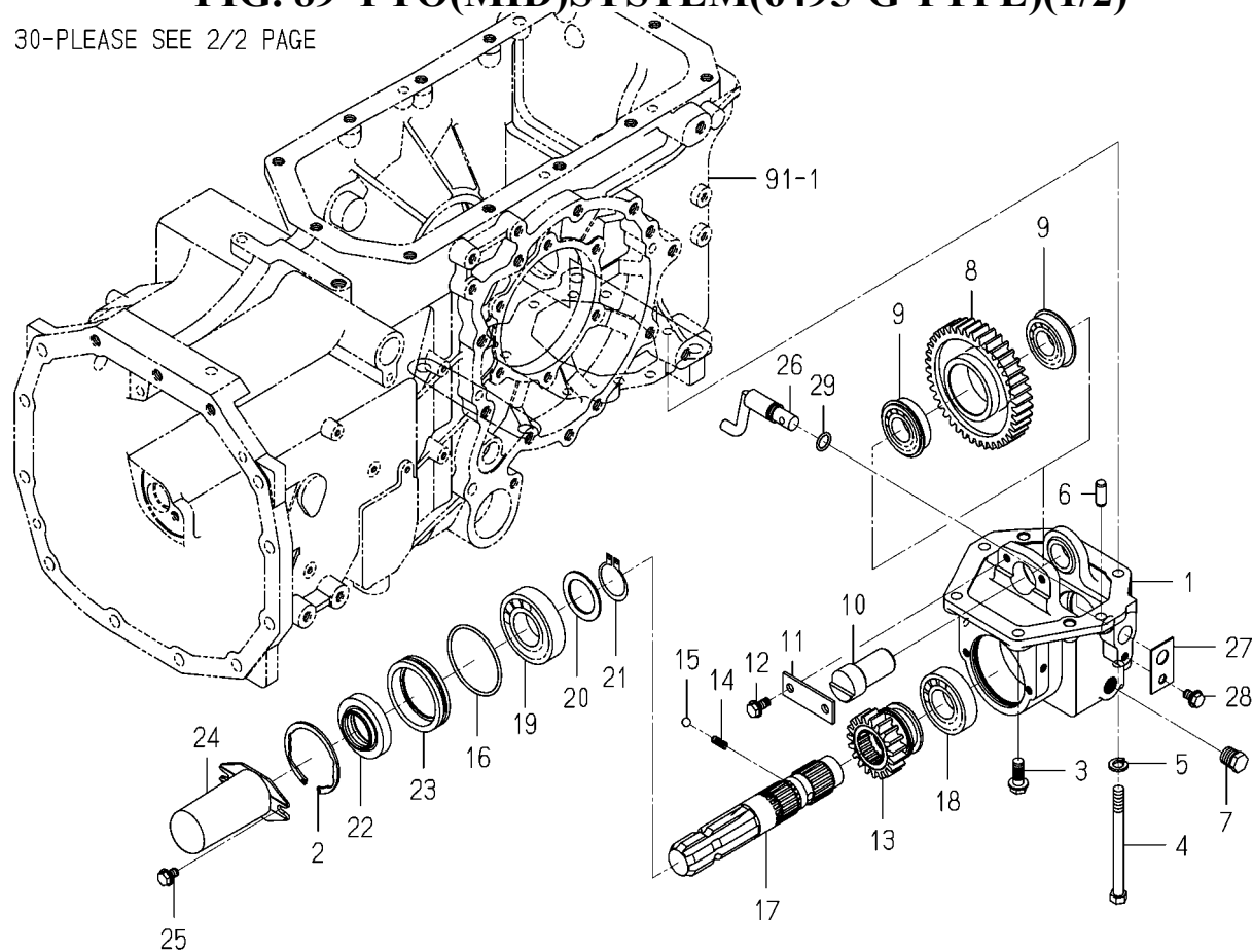
FIG. 89 PTO(MID)SYSTEM(6495-G TYPE)(1/2)
