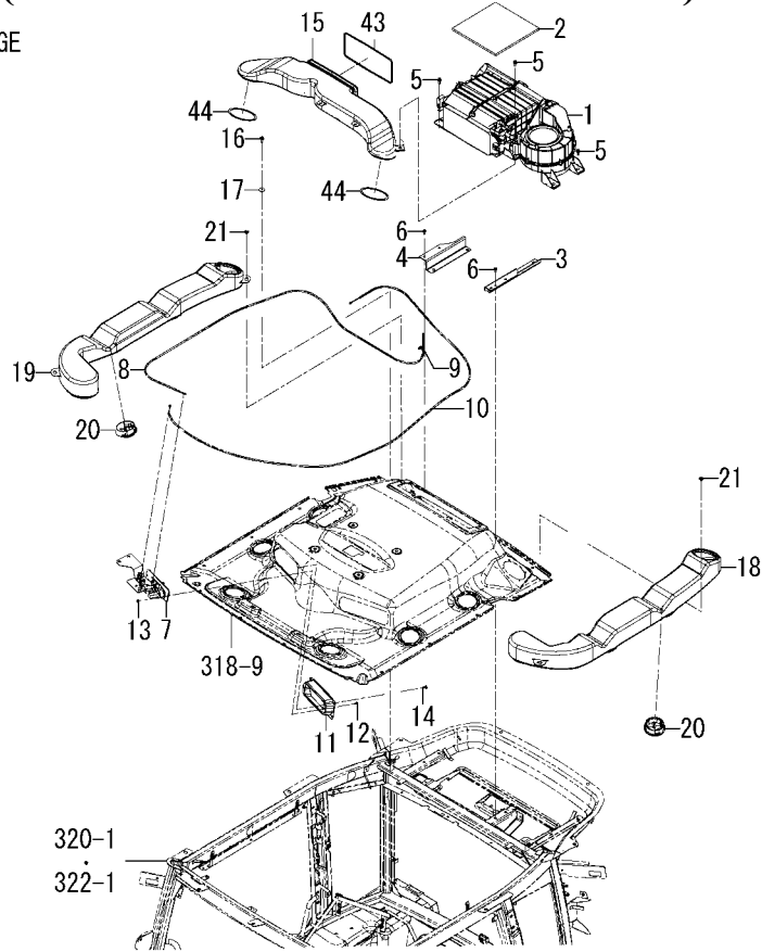
FIG.333 AIR CONDITIONER(CABIN)SYSTEM(1/2) (6375-CY TYPE/6405H-CY TYPE)
