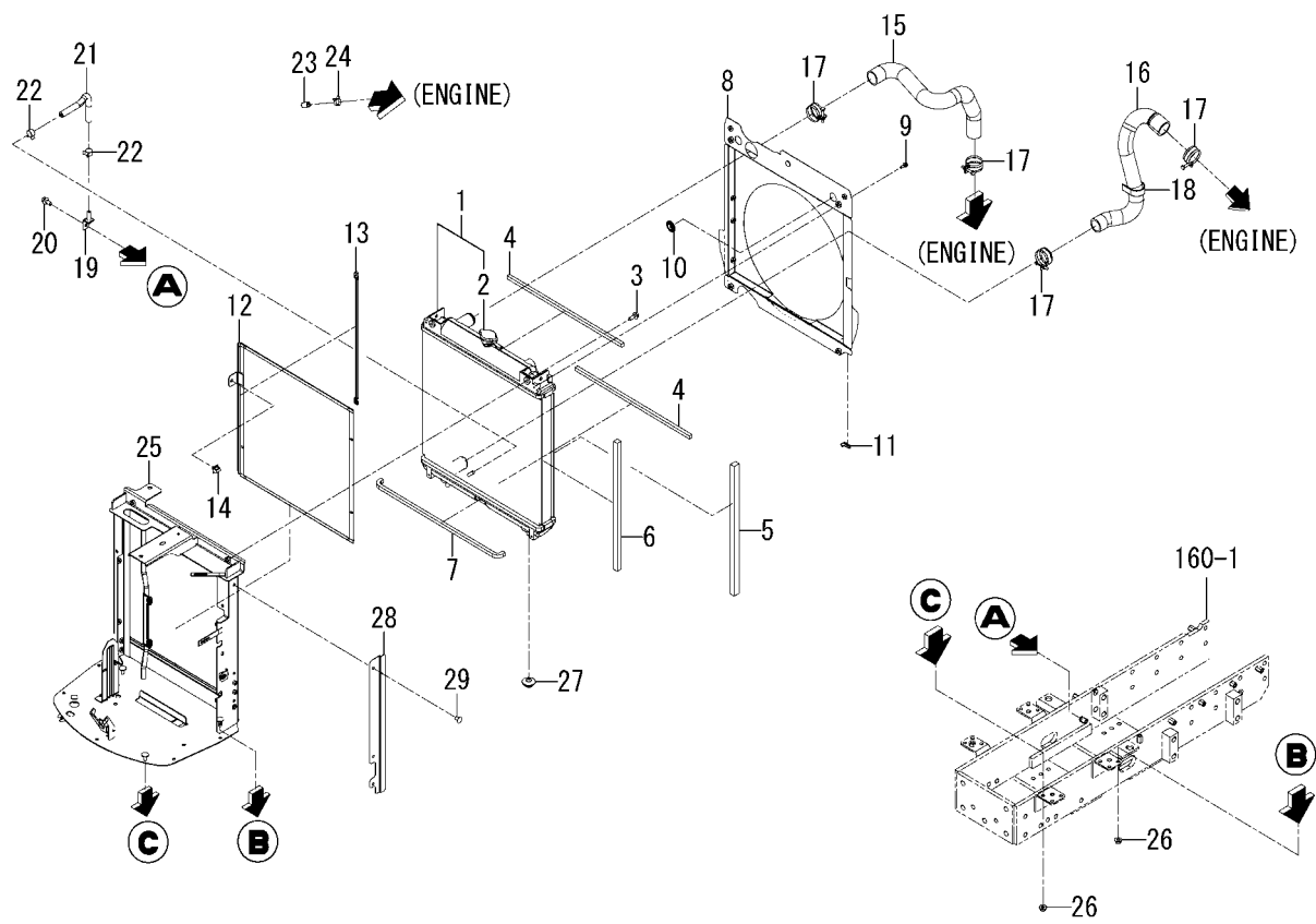
FIG. 2 RADIATOR SYSTEM(6405H TYPE)(1/2)
