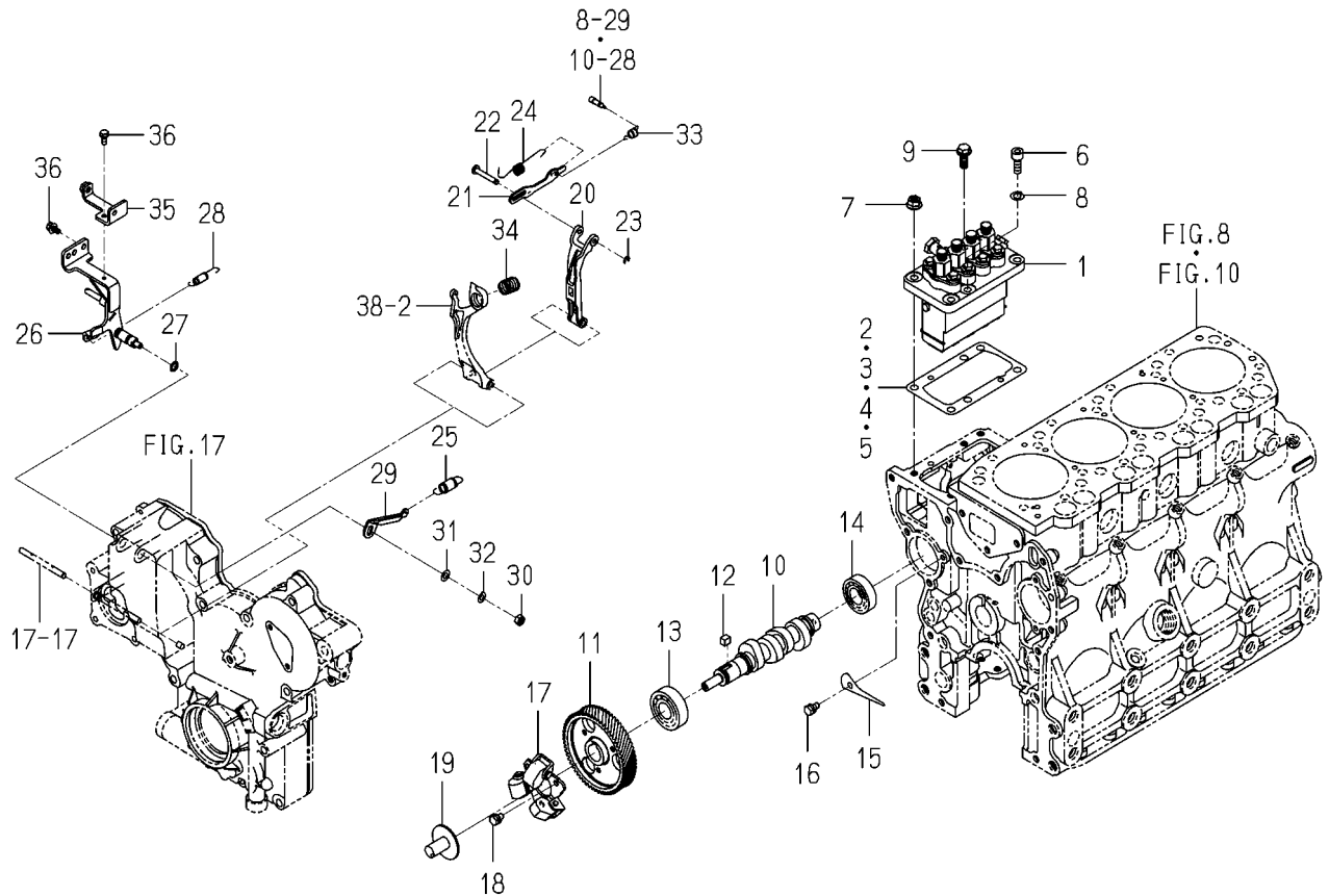
FIG. 35 INJECTION PUMP
