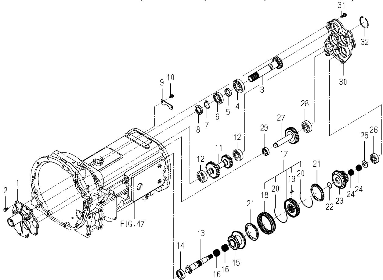
FIG. 55 GEAR(REVERSE)SYSTEM(6495-SD TYPE)
