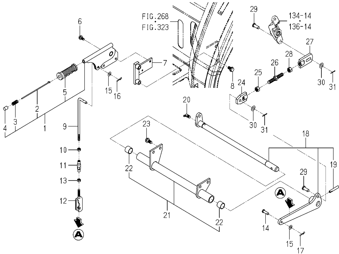
FIG.149 LEVER(BRAKE/PARKING)SYSTEM (6495-SD TYPE/6495H TYPE)
