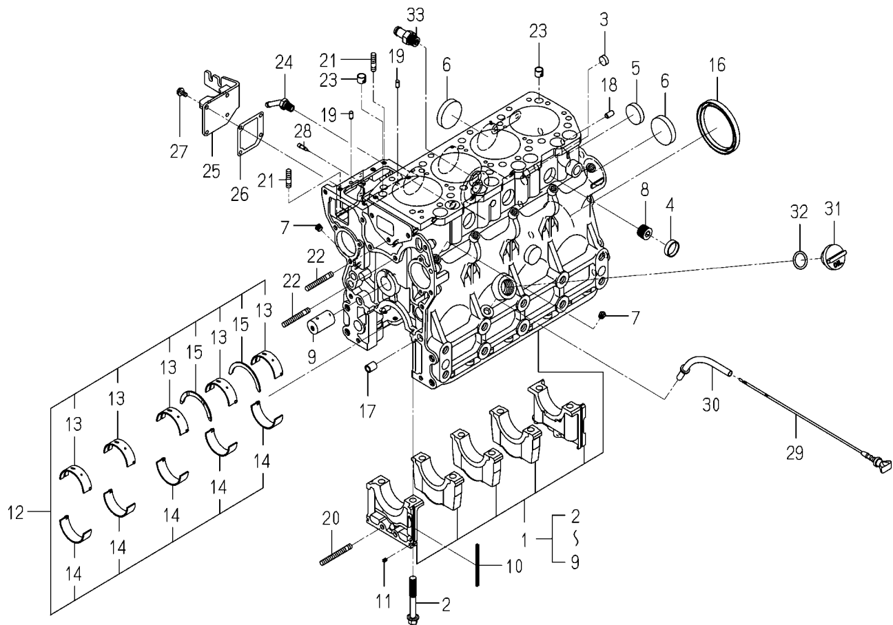
FIG. 10 CYLINDER BLOCK
