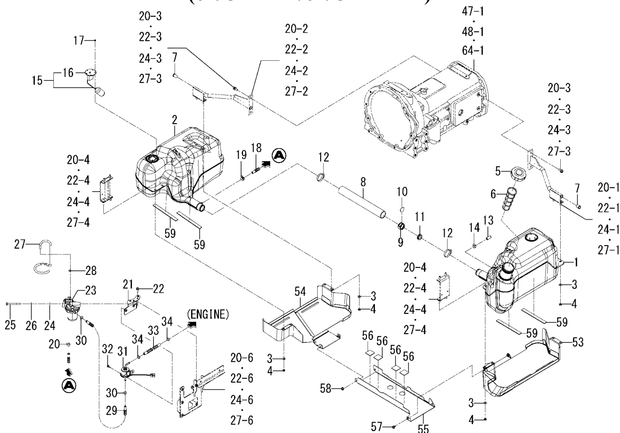
FIG. 18 TANK(FUEL)SYSTEM(1/2) (6495 TYPE/6495H TYPE)
