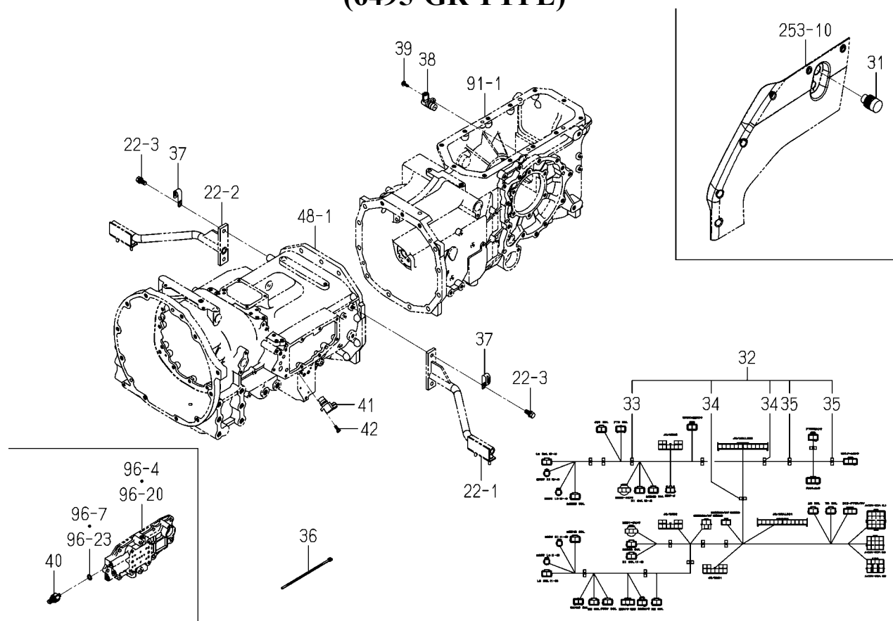
FIG.295 ELC.(FLOOR)SYSTEM(2/2) (6495-GR TYPE)
