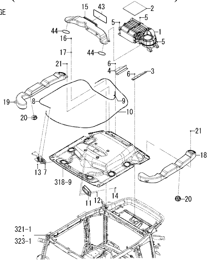
FIG.334 AIR CONDITIONER(CABIN)SYSTEM(1/2) (6495-CY TYPE/6495H TYPE)
