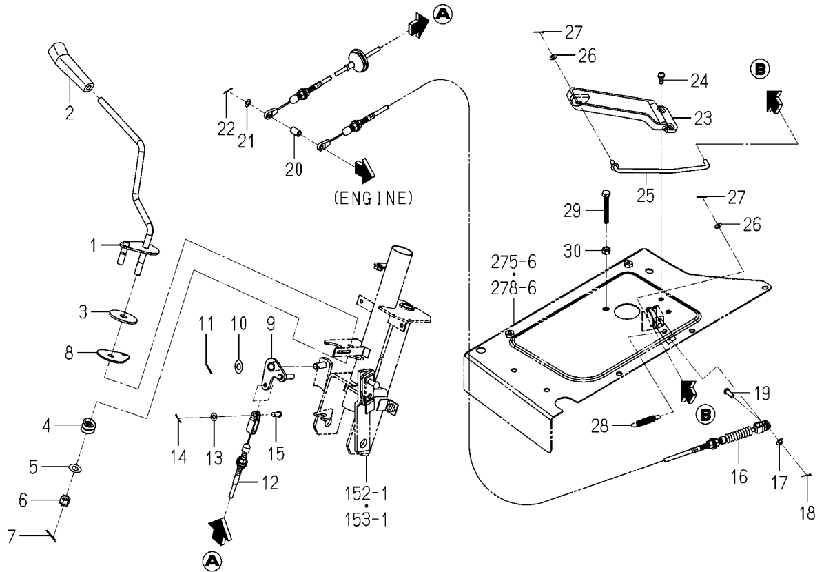
FIG. 30 ACCELERATOR SYSTEM(6495-R TYPE)
