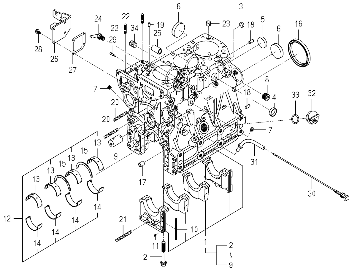
FIG. 7 CYLINDER BLOCK
