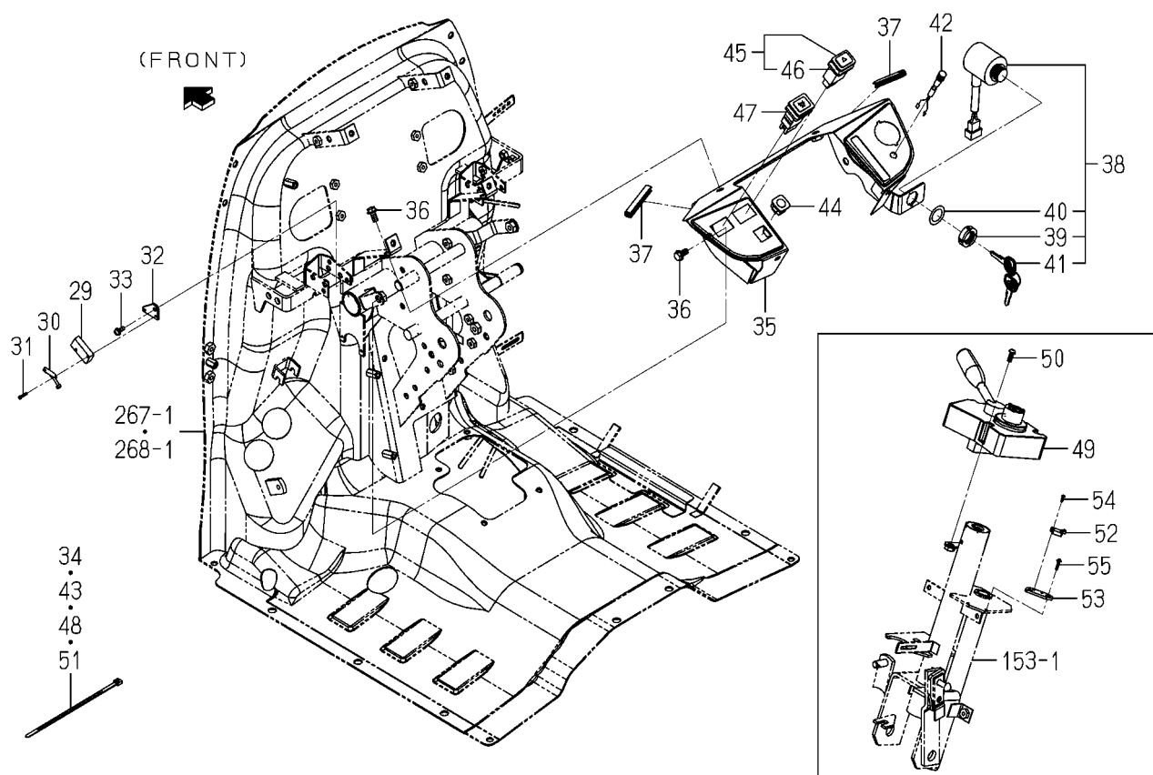
FIG.292 ELC.(MAIN)SYSTEM(SD TYPE)(2/2)
