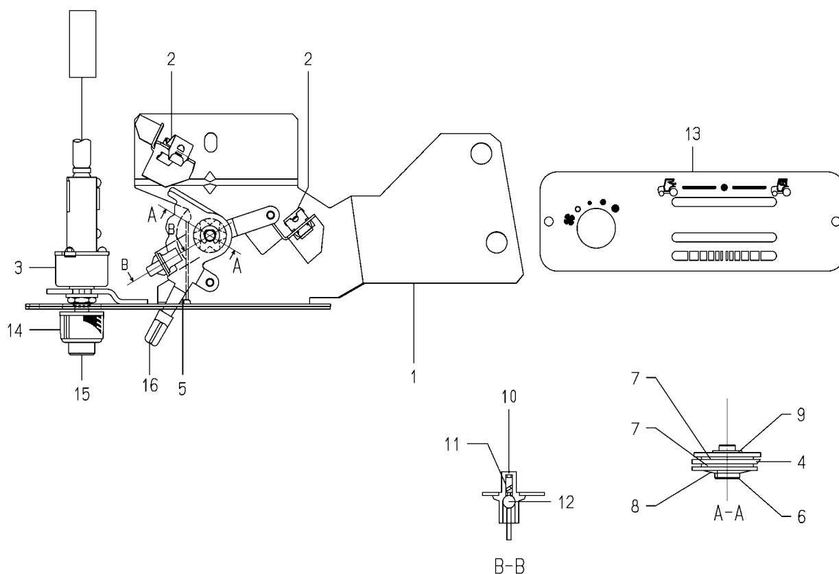
FIG.401 COMPONENT PARTS FOR 1800-782-400-20 ON FIG.333,334
