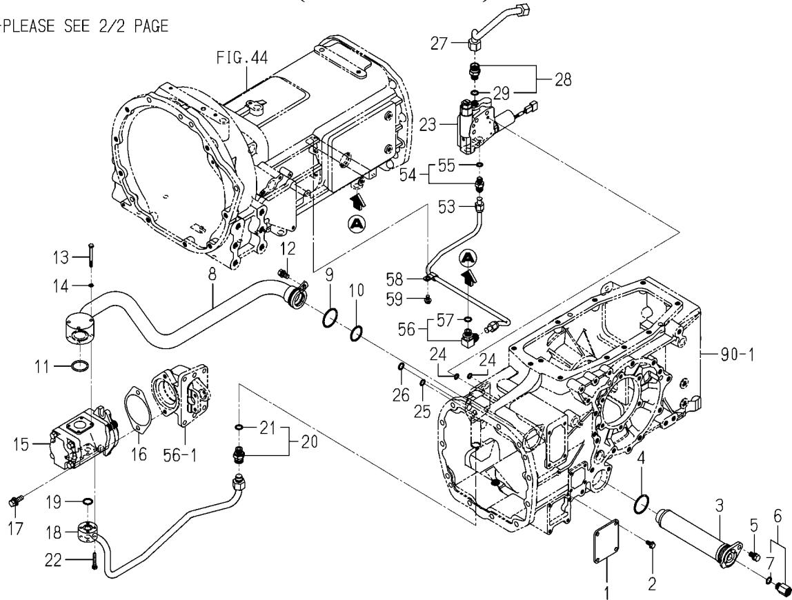
FIG.192 PIPING(MAIN)SYSTEM(1/2) (6495-H TYPE)
