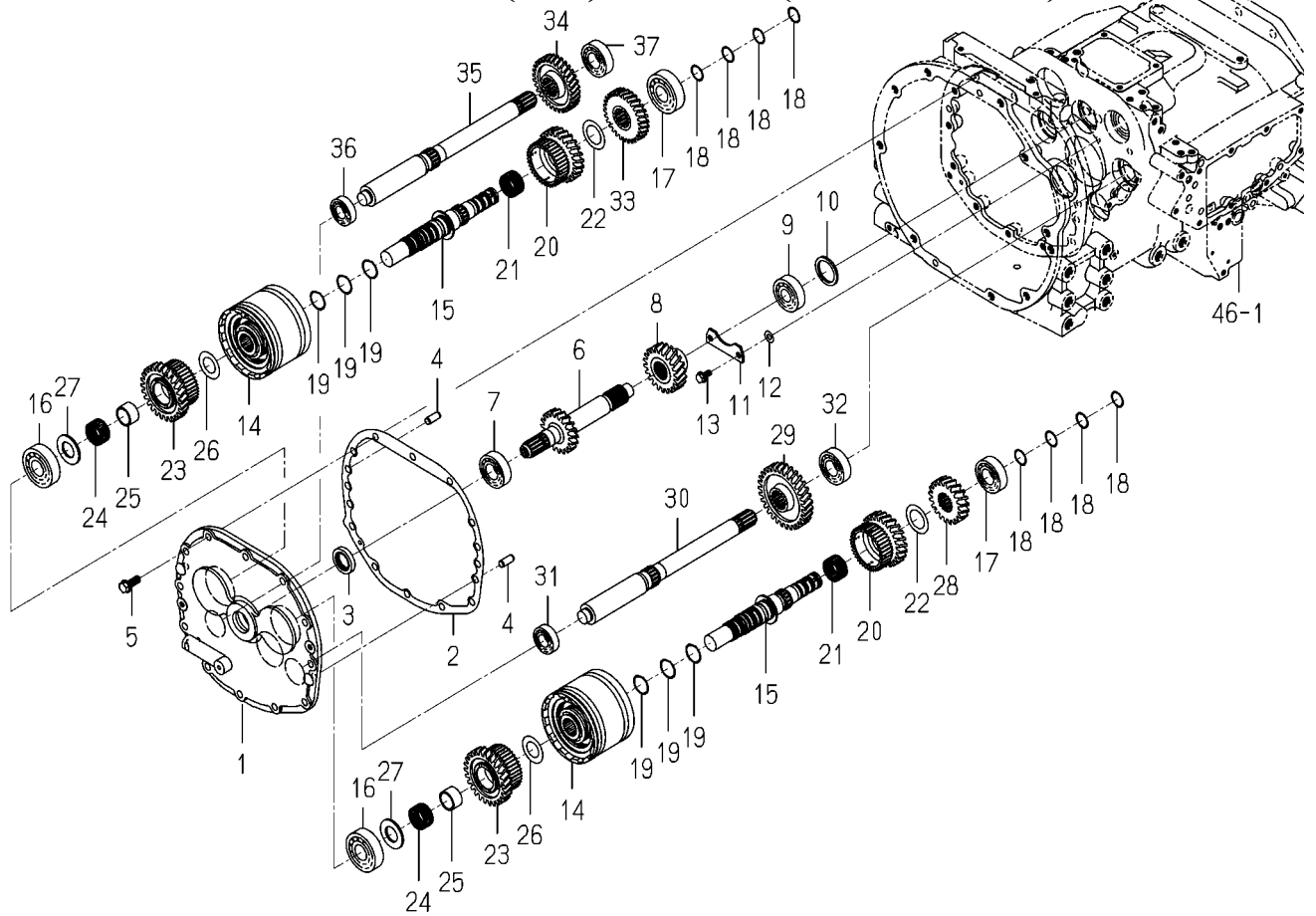
FIG. 50 GEAR(H/L)SYSTEM(6375-G TYPE)
