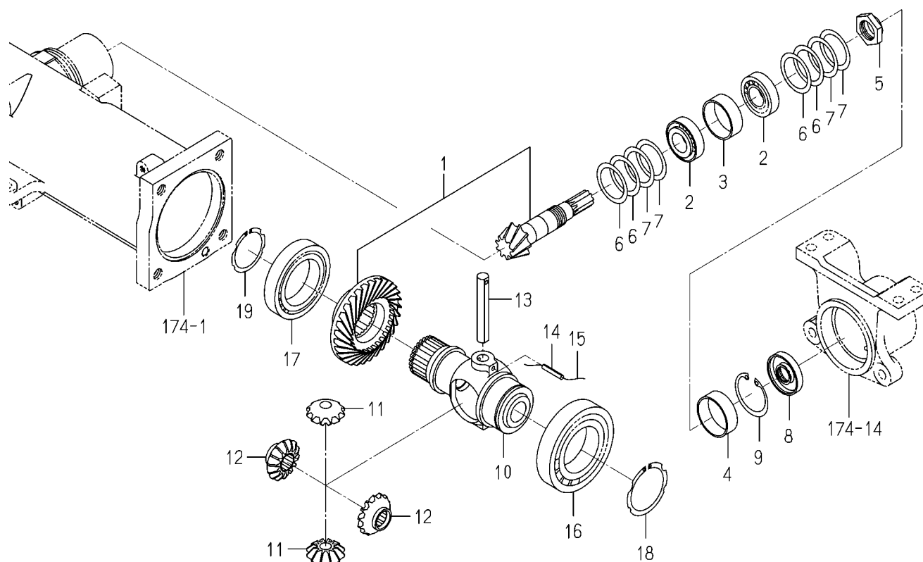
FIG.169 CASE(BEVEL)SYSTEM(6375-G TYPE)
