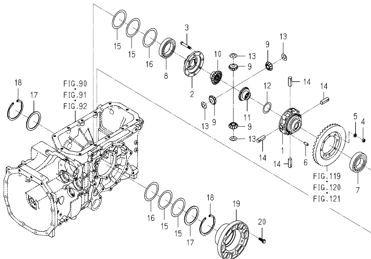
FIG.122 CASE(DIFFERENTIAL/REAR)SYSTEM
