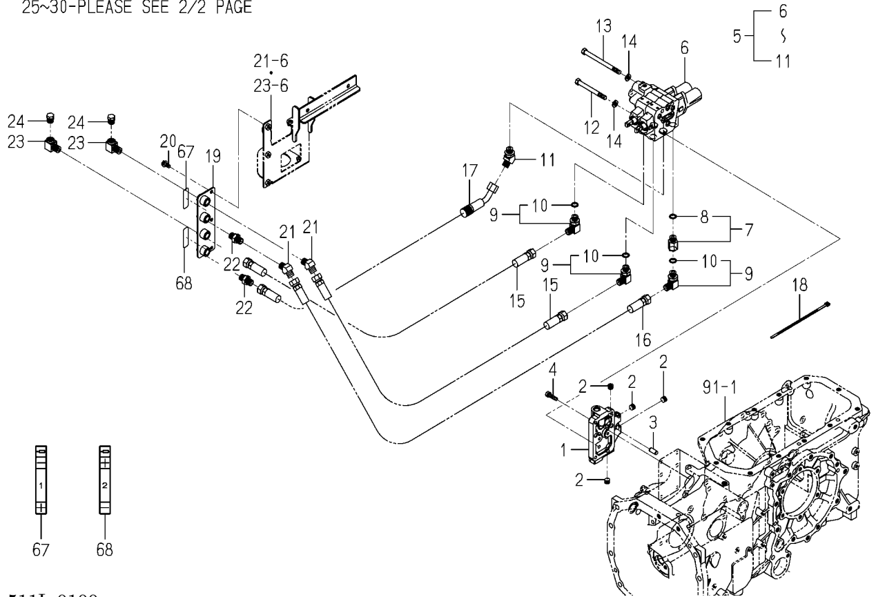
FIG.208 JOY STICK VALVE SYSTEM(1/2) (6375 TYPE EXCEPT D)
