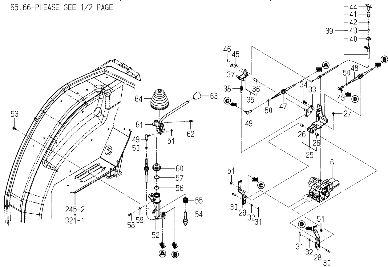
FIG.203 JOY STICK VALVE SYSTEM(2/2) (6495-G TYPE EXCEPT D)
