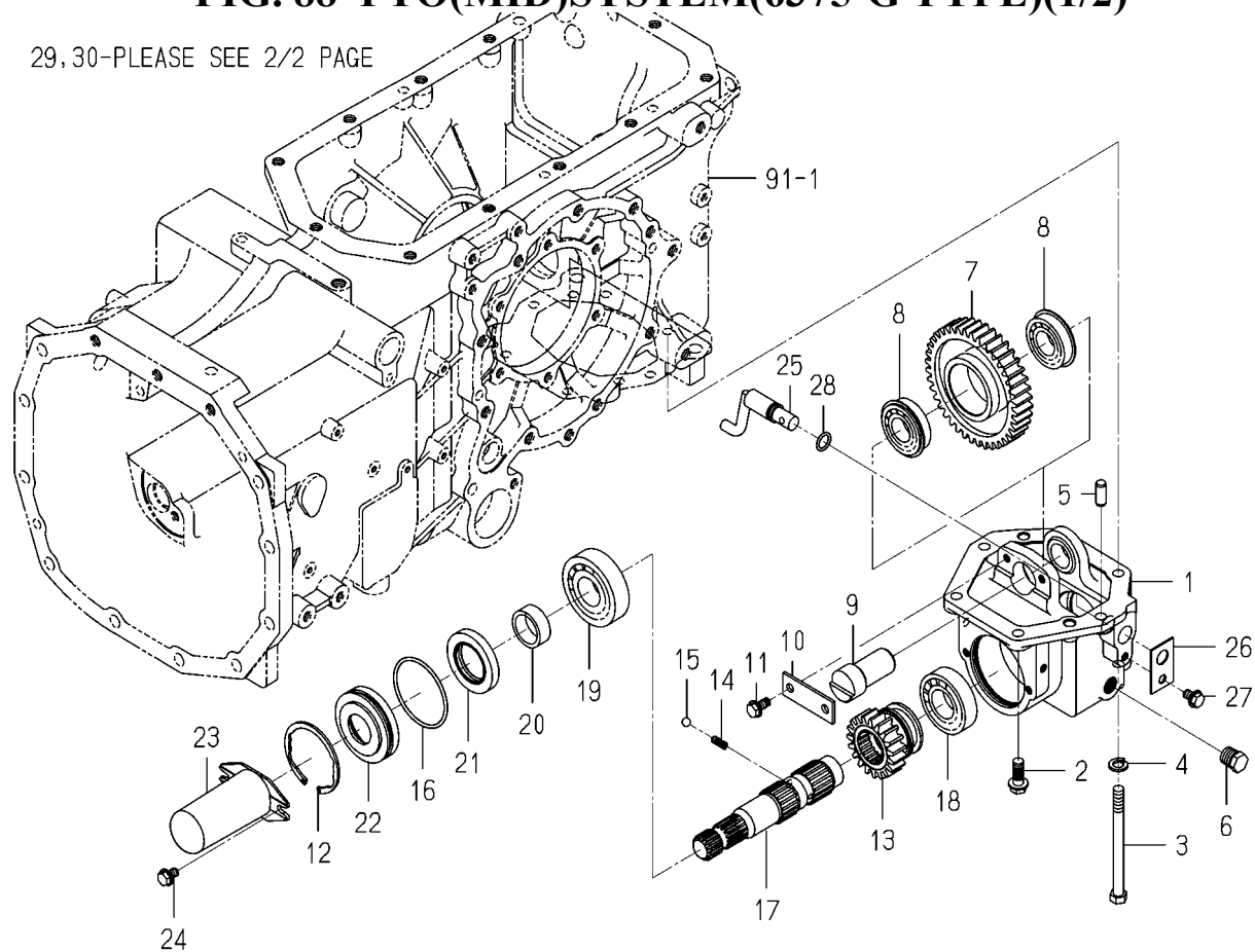
FIG. 88 PTO(MID)SYSTEM(6375-G TYPE)(1/2)
