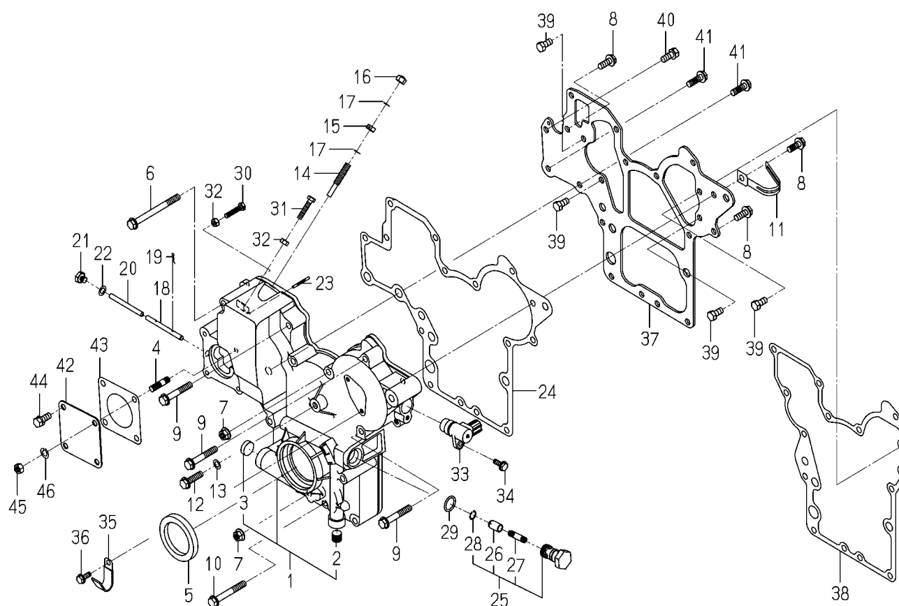
FIG. 18 TIMING GEAR CASE
