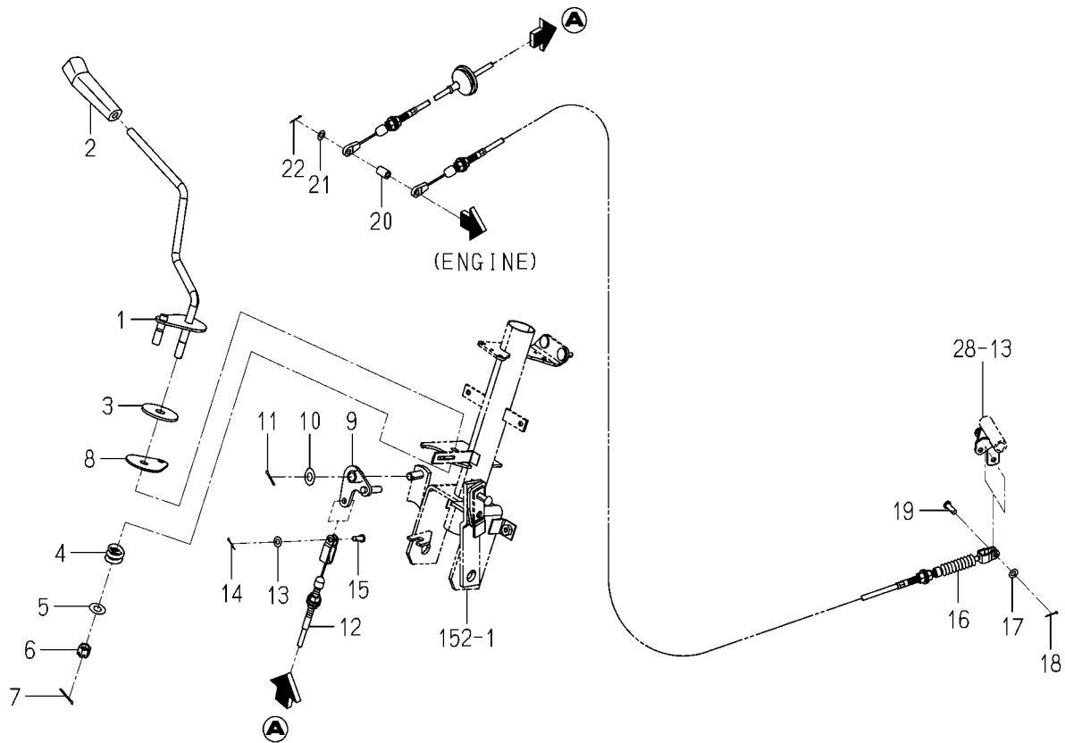
FIG. 31 ACCELERATOR SYSTEM(6405H TYPE)
