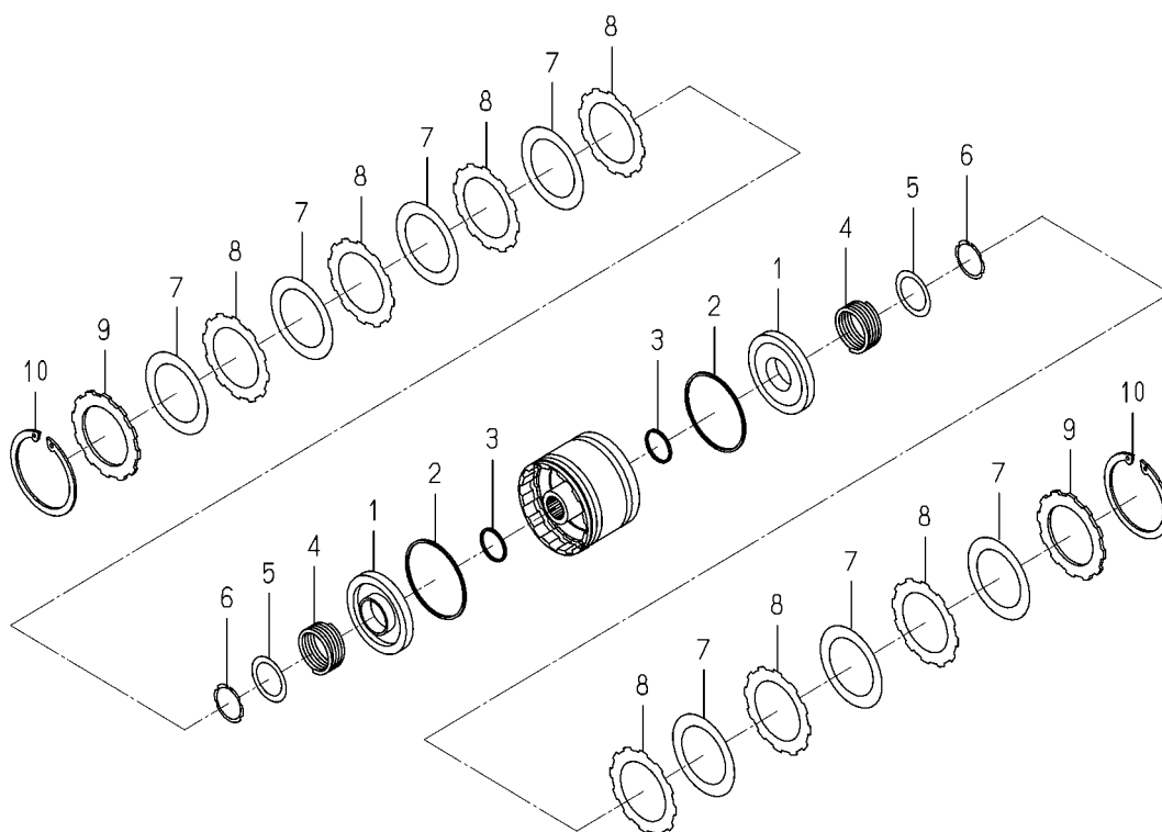
FIG.397 COMPONENT PARTS FOR 1796-203-300-00 ON FIG.51
