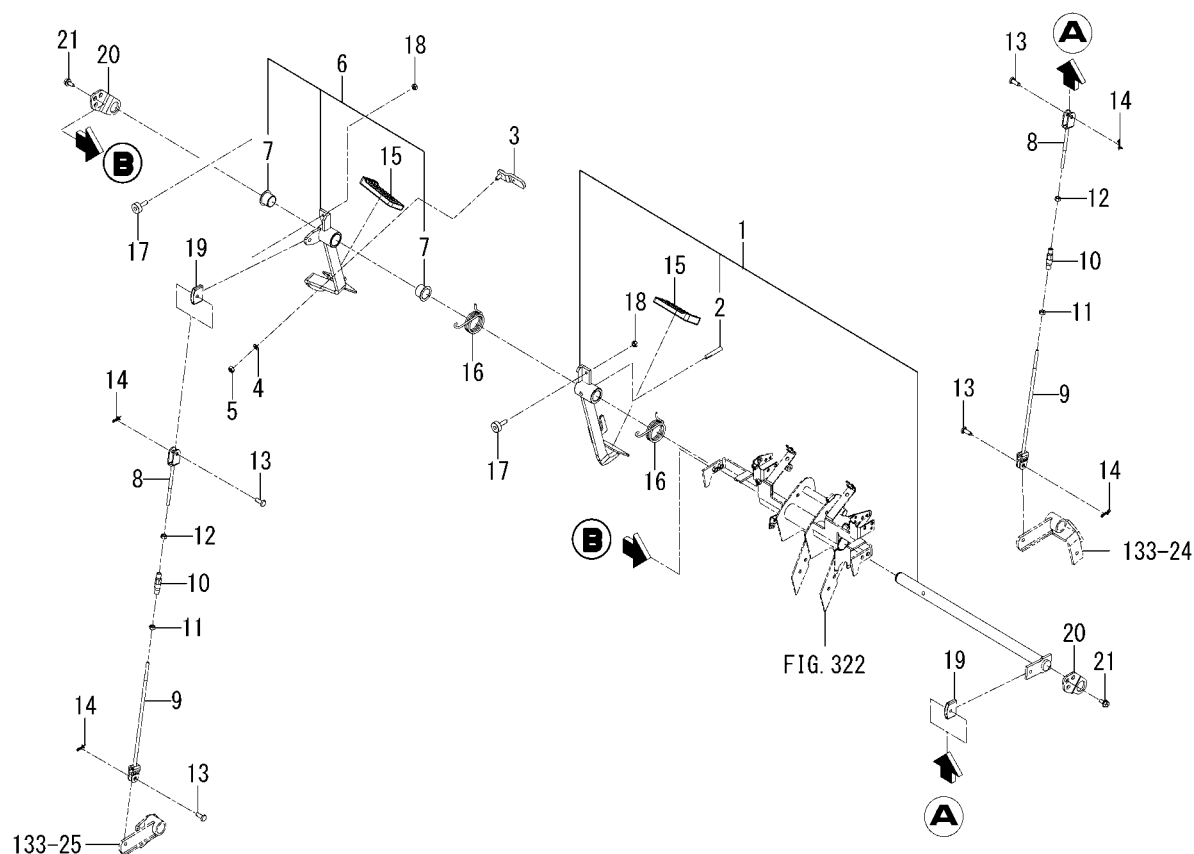
FIG.144 PEDAL(BRAKE)SYSTEM (6405H-CY TYPE)
