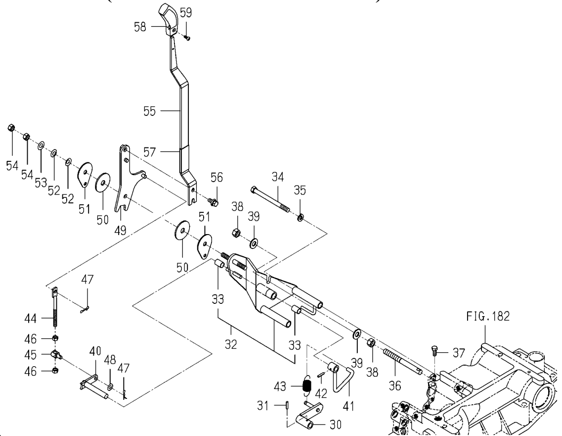
FIG.184 LEVER(POSITION)SYSTEM(2/2) (6495-SD TYPE/6495H TYPE)
