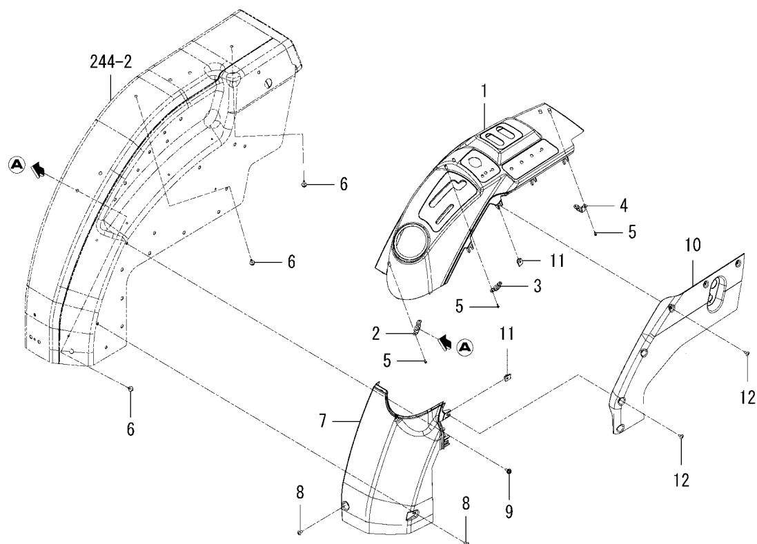
FIG.254 GUIDE(LEVER)SYSTEM(6375-GR TYPE)
