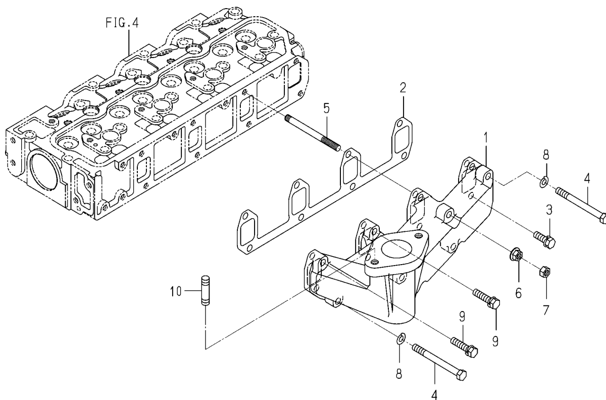
FIG. 7 EXHAUST MANIFOLD
