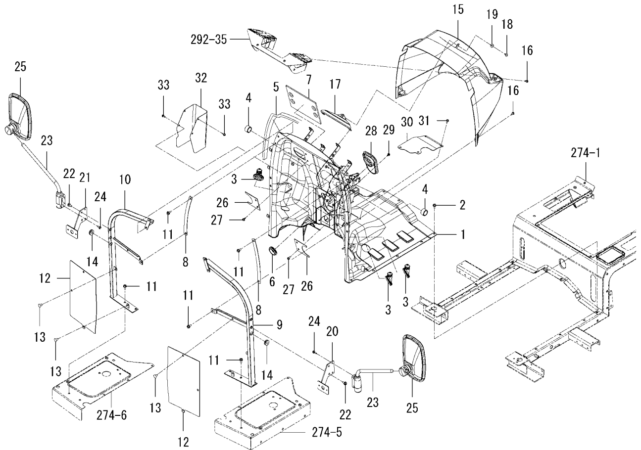
FIG.267 PANEL(DASH)SYSTEM(6375-SD TYPE)
