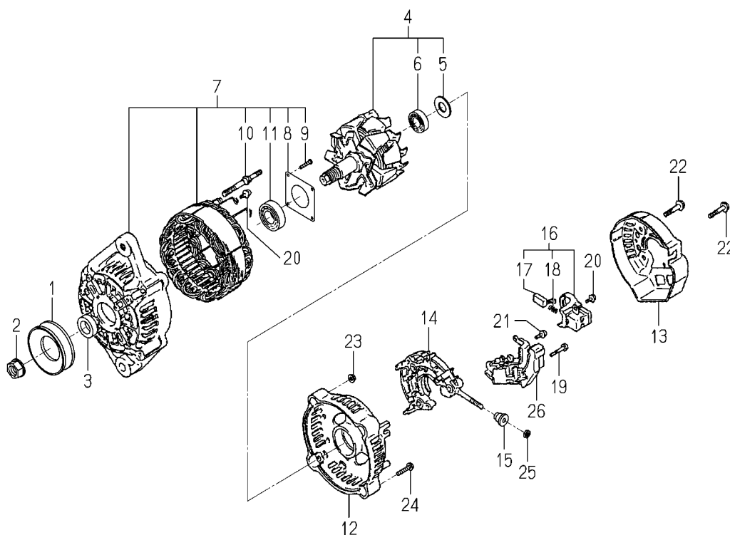
FIG. 46 COMPONENT PARTS FOR 6281-200-015-00 ON Fig.039
