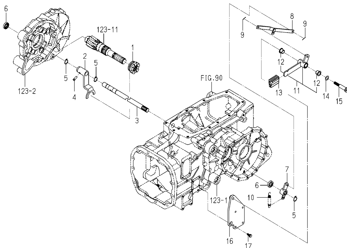
FIG.129 CLUTCH(DIFF-LOCK)SYSTEM (6405H TYPE)
