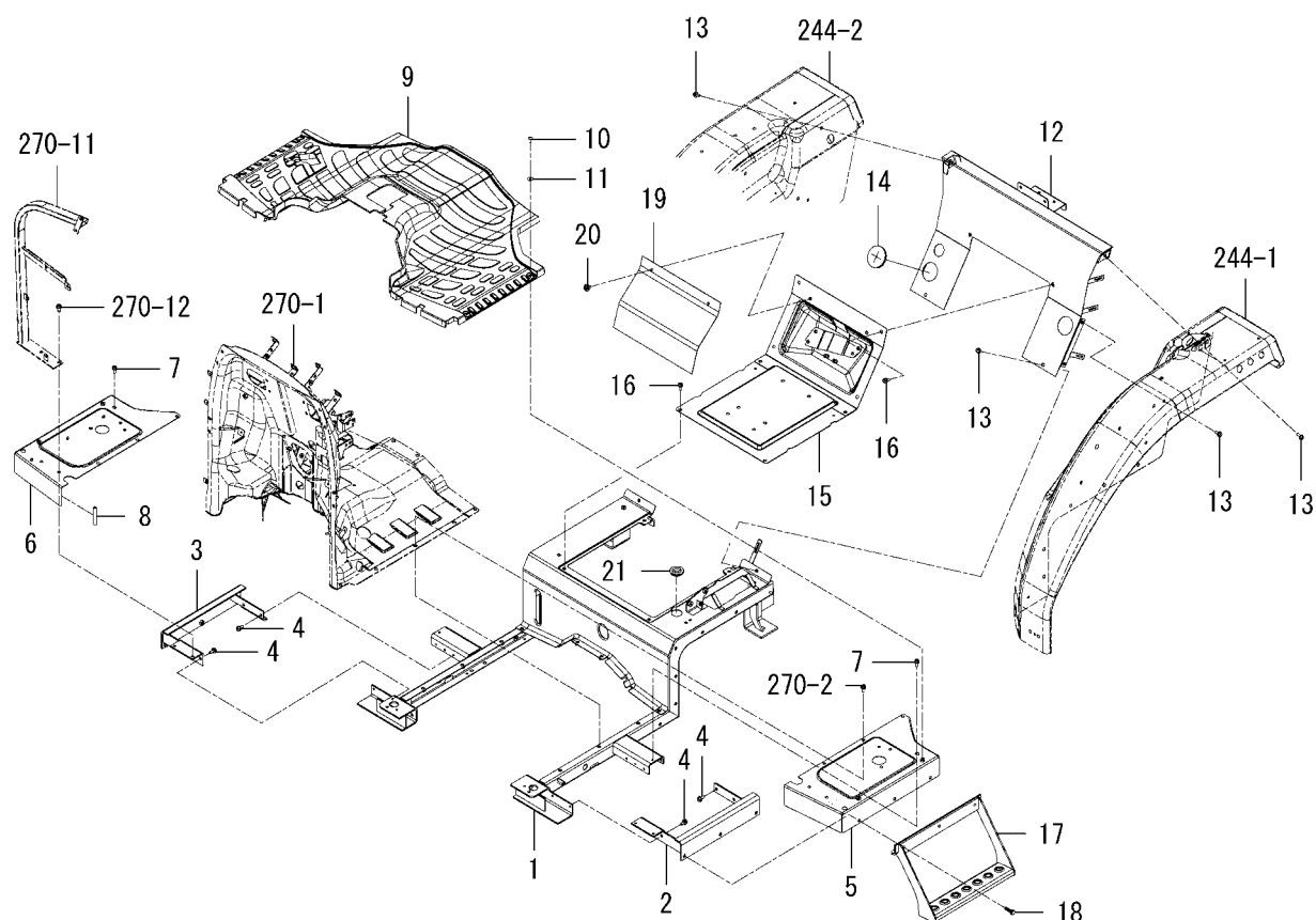
FIG.277 FLOOR(REAR)SYSTEM(6375-GR TYPE)
