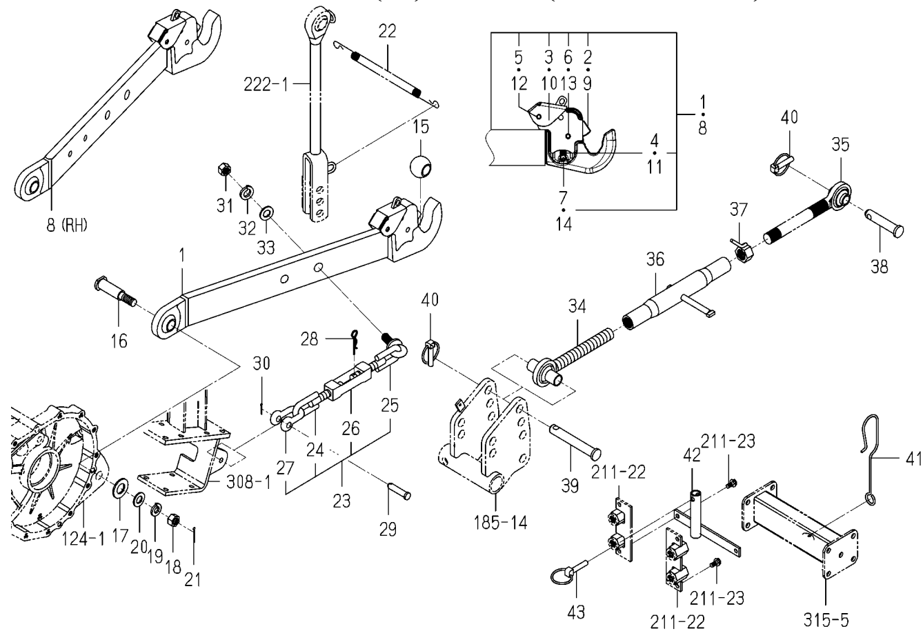
FIG.216 LINK(3P)SYSTEM(6375-GR TYPE)
