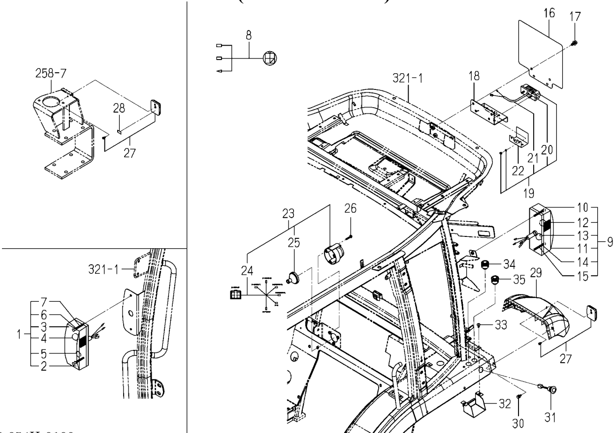
FIG.296 ELC.(FLOOR)SYSTEM(1/2) (6495-CY TYPE)
