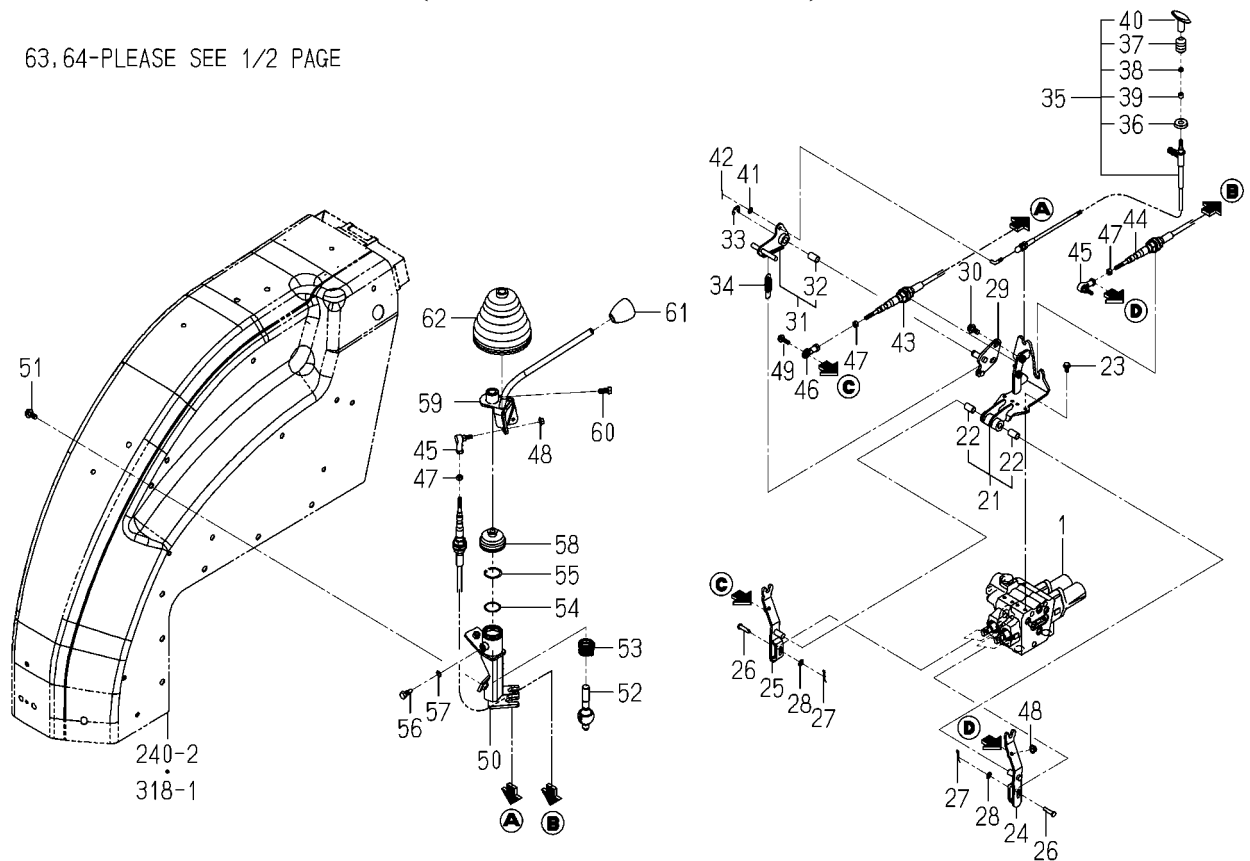
FIG.206 JOY STICK VALVE SYSTEM(2/2) (H TYPE EXCEPT D)
