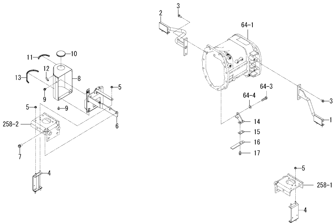
FIG. 27 STAY(TANK)SET SYSTEM(6495H TYPE)
