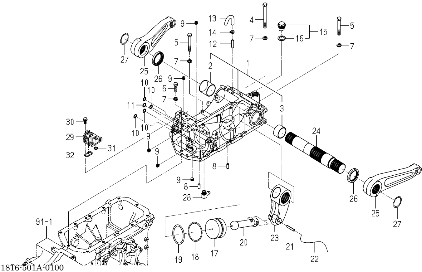
FIG.181 CASE(CYLINDER)SYSTEM(6495-G TYPE)
