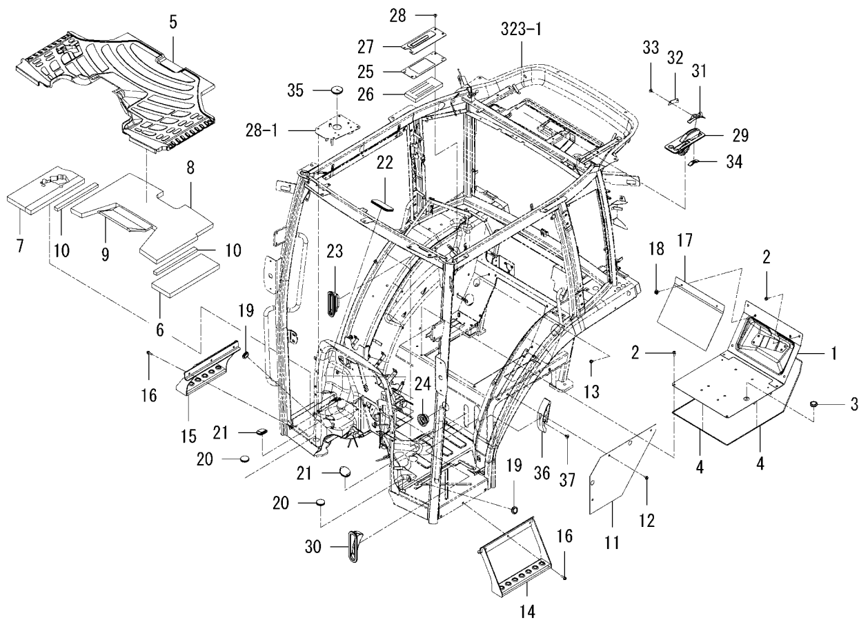
FIG.282 FLOOR(REAR)SYSTEM(6495H TYPE)
