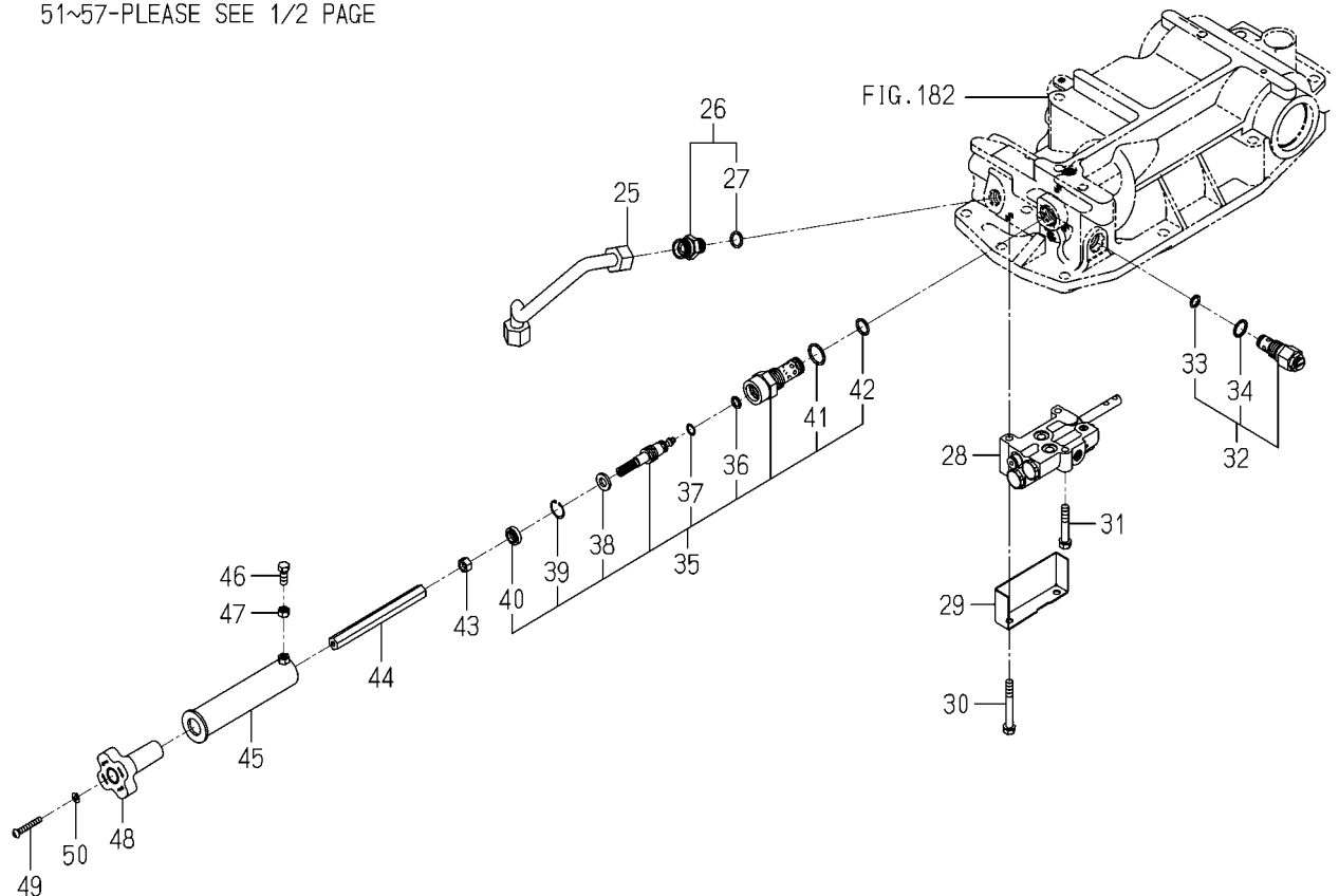
FIG.193 PIPING(MAIN)SYSTEM(2/2) (6405-H TYPE)
