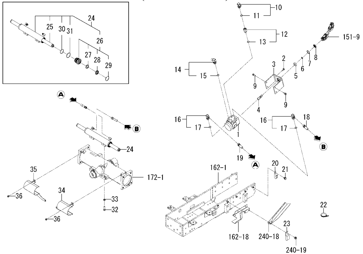
FIG.156 STEERING(POWER)SYSTEM (6375-SD TYPE)
