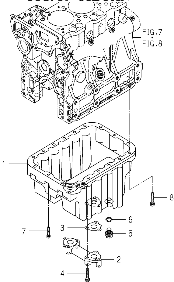
FIG. 10 OIL PAN
