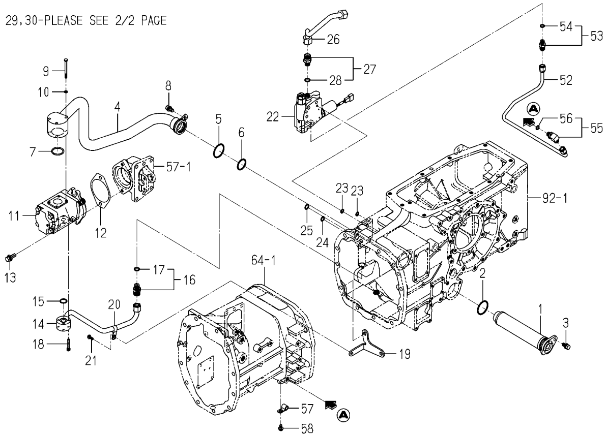
FIG.194 PIPING(MAIN)SYSTEM(1/2) (6495-H TYPE)
