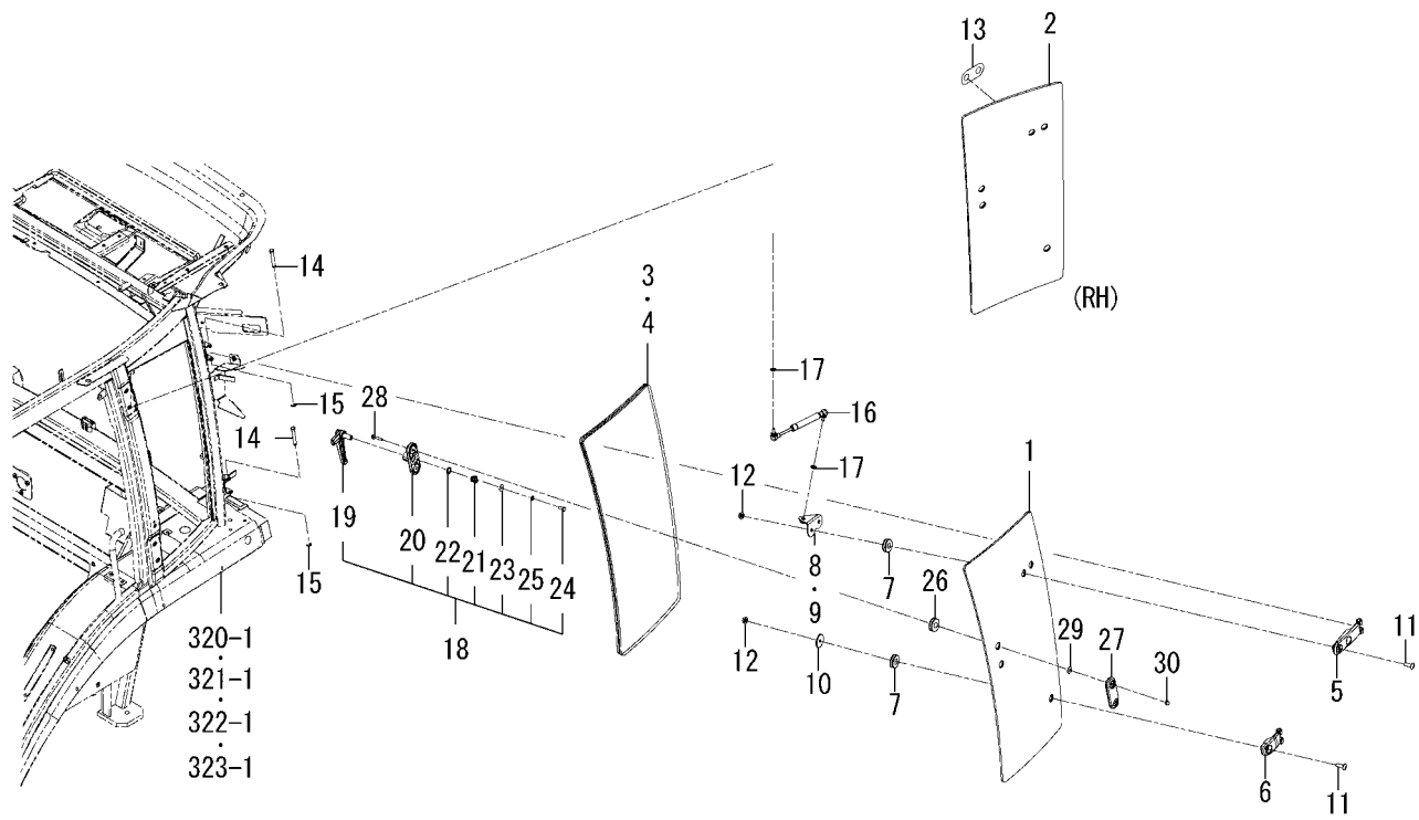
FIG.327 GLASS(SIDE)SYSTEM(CY TYPE)
