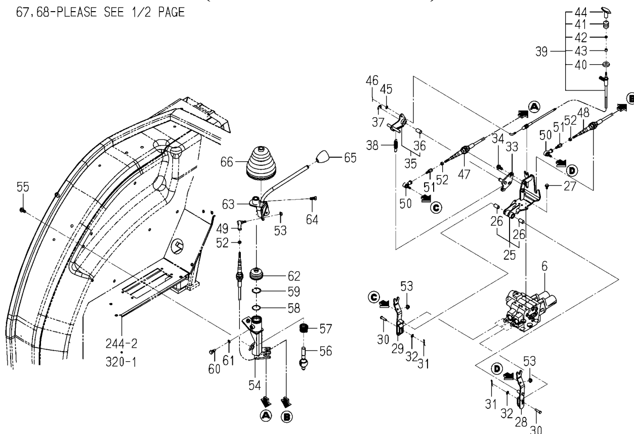
FIG.208 JOY STICK VALVE SYSTEM(2/2) (6375 TYPE EXCEPT D)
