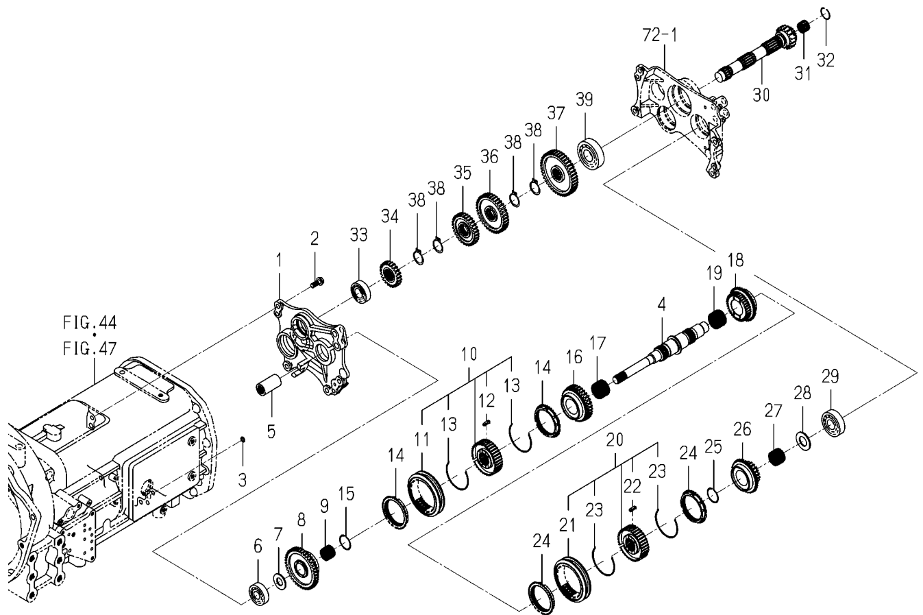
FIG. 66 GEAR(MAIN)SYSTEM(SD TYPE)
