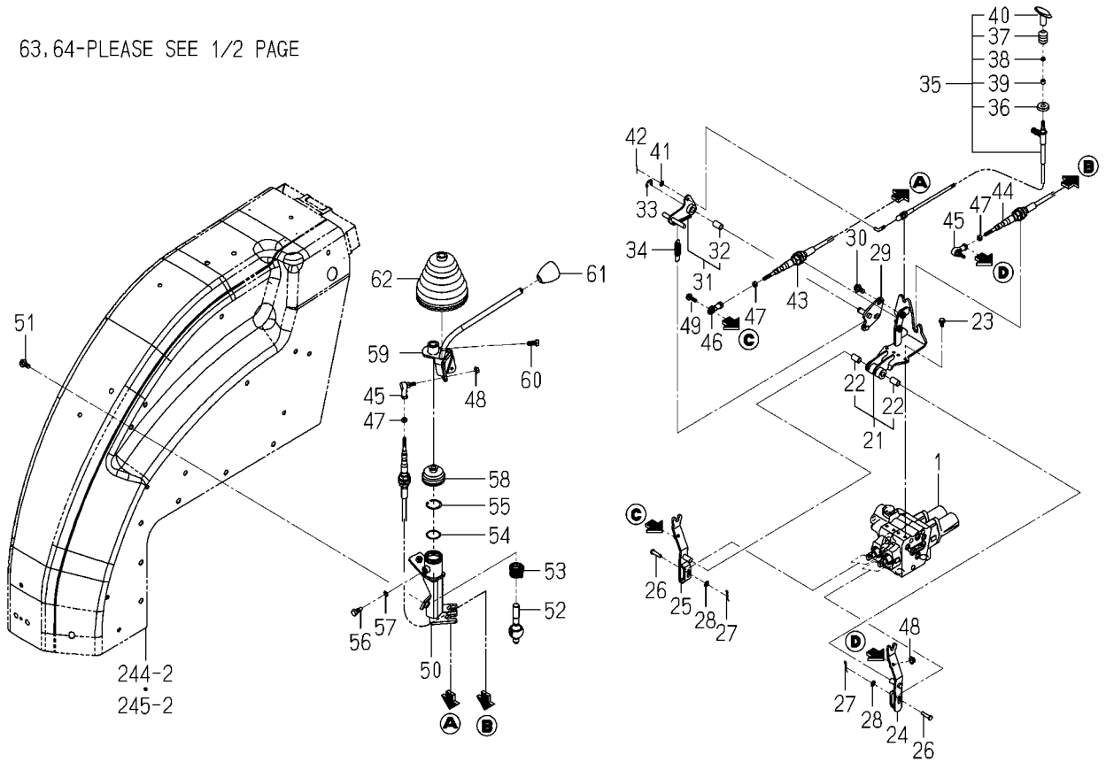
FIG.207 JOY STICK VALVE SYSTEM(2/2) (SD TYPE EXCEPT 6495-SDA)
