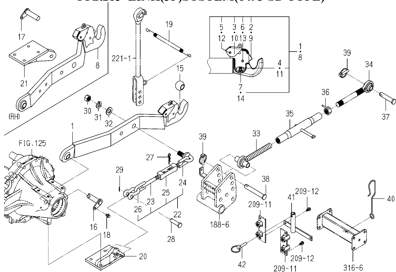
FIG.213 LINK(3P)SYSTEM(6495-SD TYPE)
