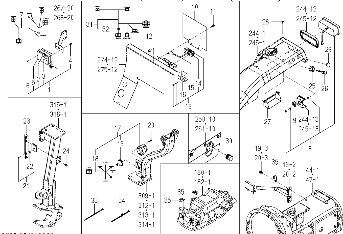
FIG.299 ELC.(FLOOR)SYSTEM(SD TYPE)
