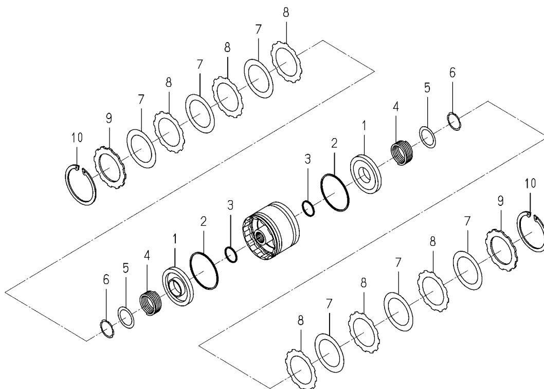
FIG.393 COMPONENT PARTS FOR 1792-203-300-00 ON FIG.50
