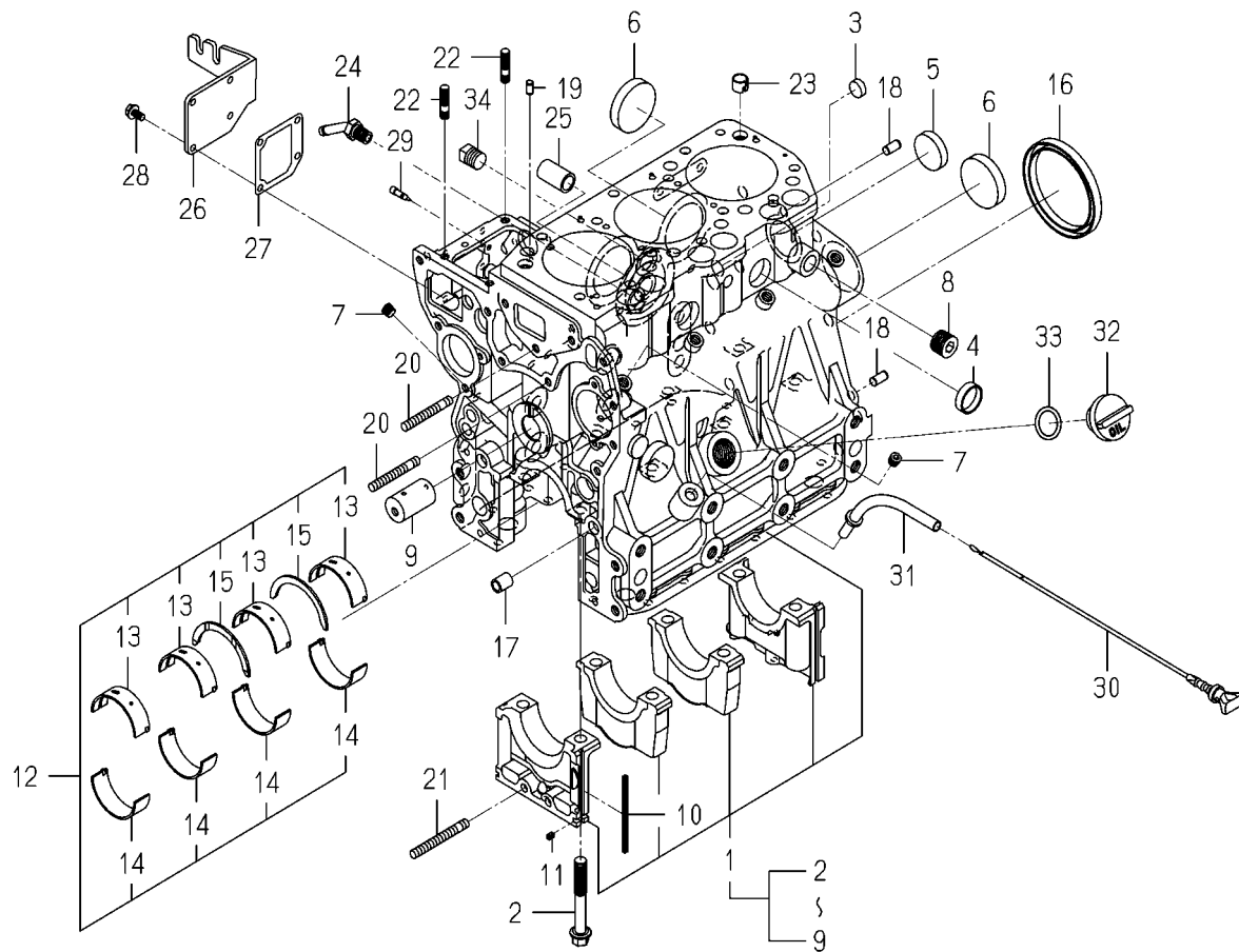
FIG. 8 CYLINDER BLOCK
