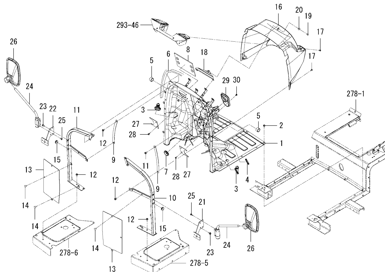
FIG.271 PANEL(DASH)SYSTEM(6495-GR TYPE)
