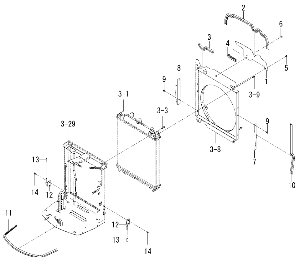
FIG. 5 RADIATOR SYSTEM (6495 TYPE/6495H TYPE)
