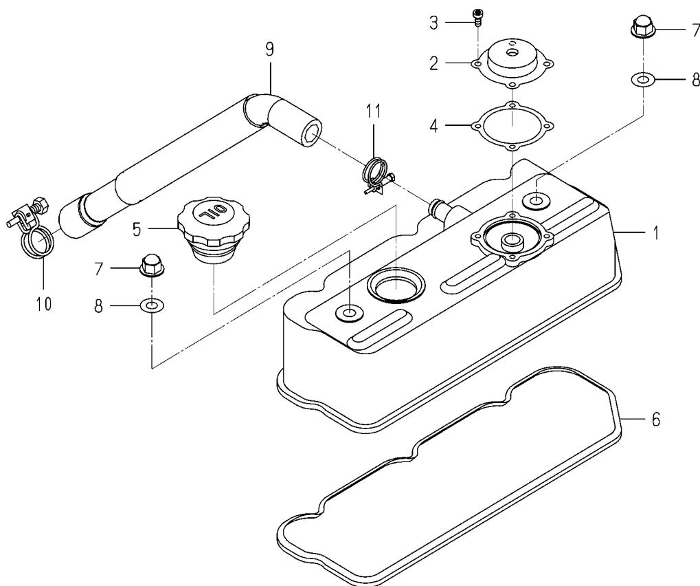
FIG. 3 CYLINDER HEAD COVER
