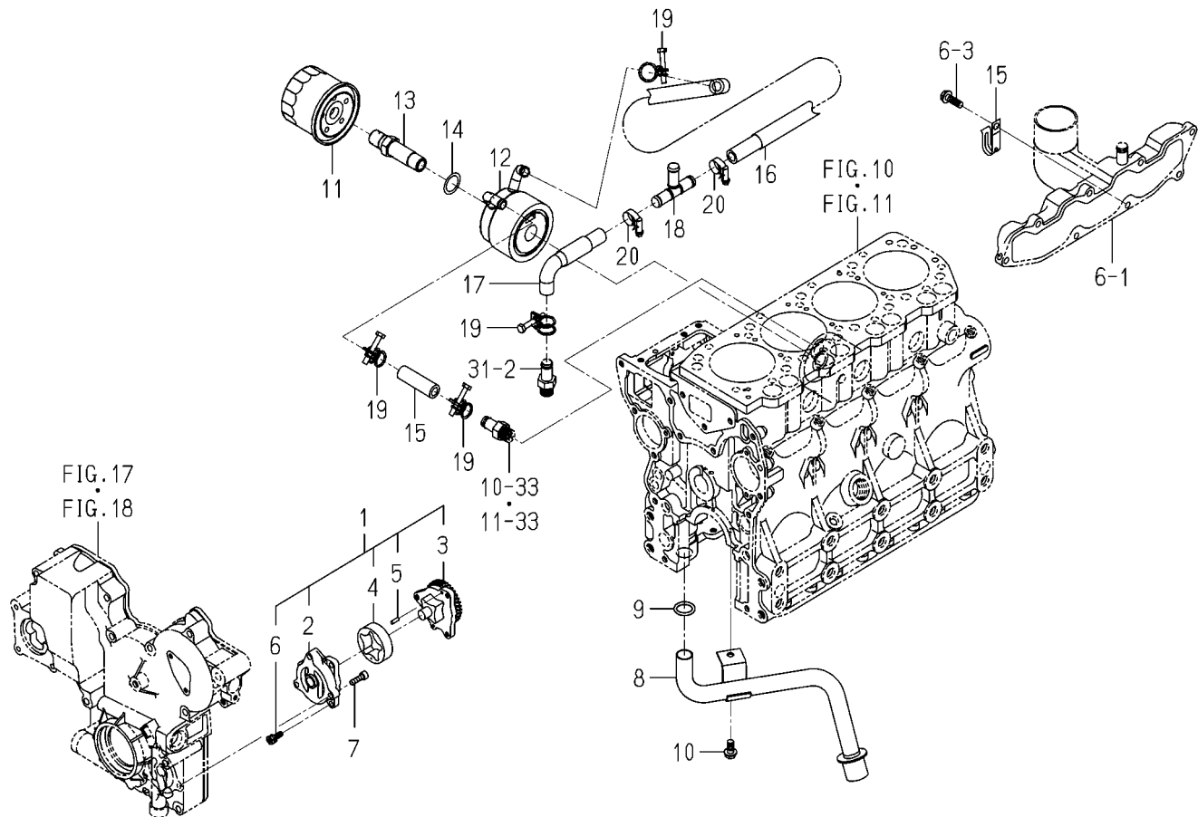
FIG. 30 OIL PUMP
