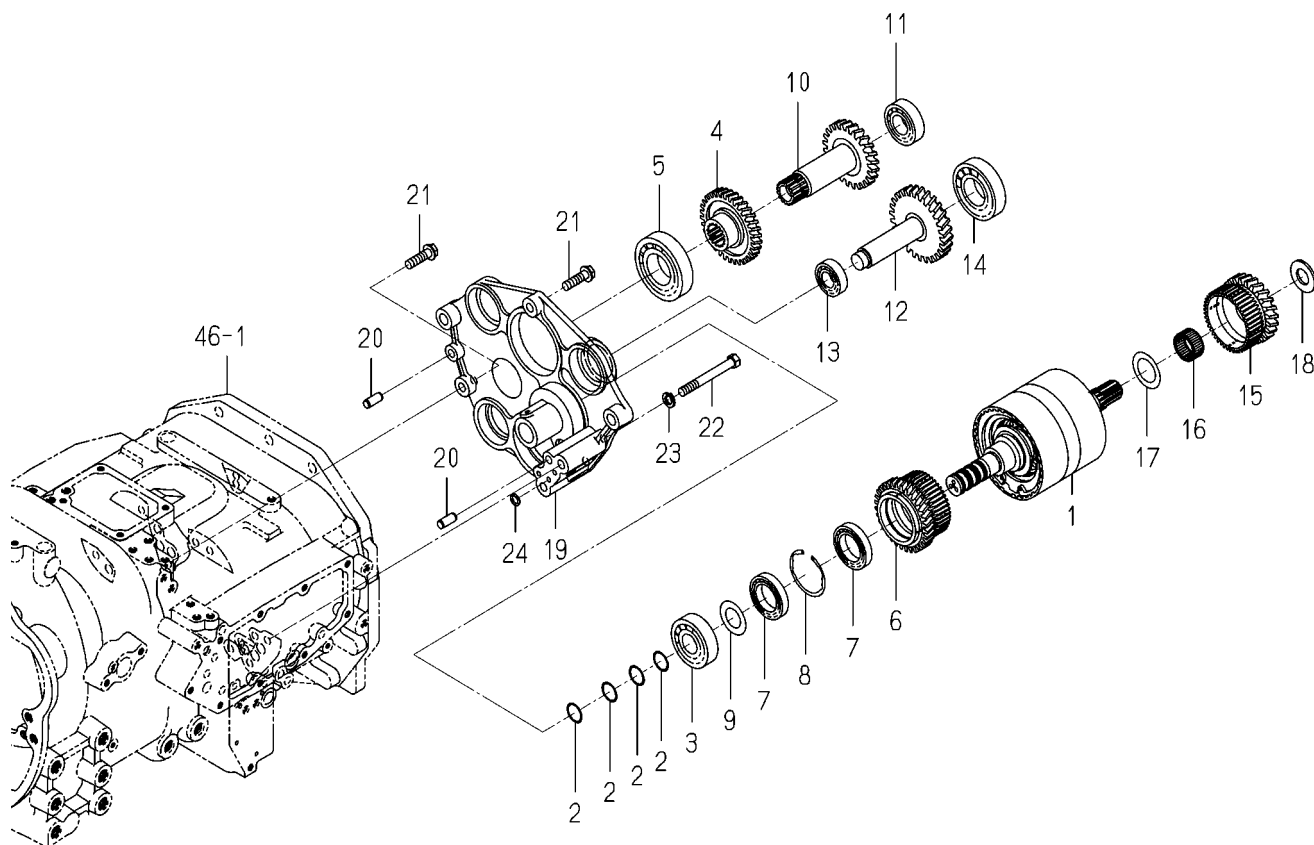
FIG. 70 GEAR(MAIN)SYSTEM(6375-G TYPE)
