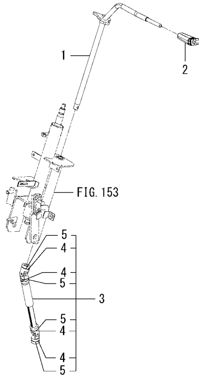
FIG.104 LEVER(REVERSE)SYSTEM (6495-SD TYPE)
