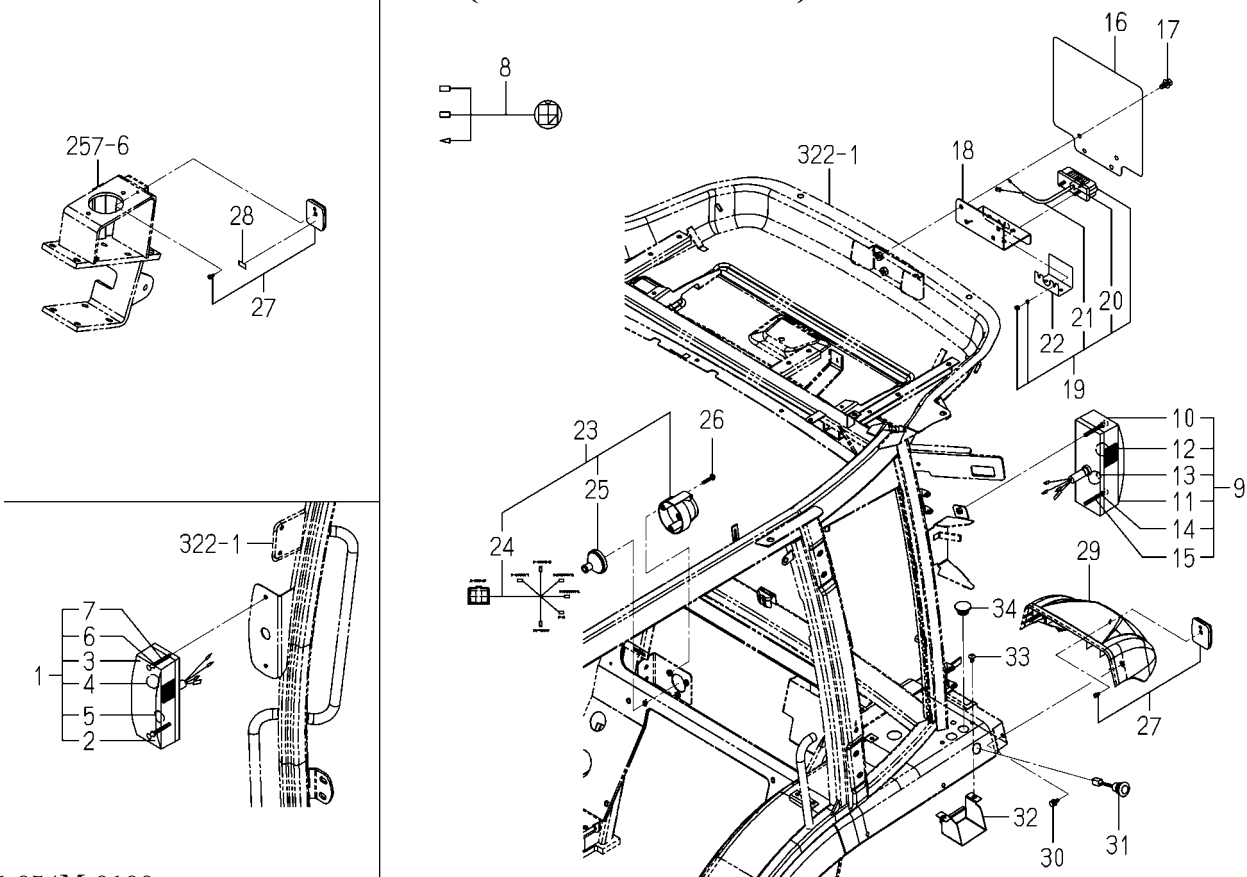
FIG.298 ELC.(FLOOR)SYSTEM(1/2) (6405H-CY TYPE)
