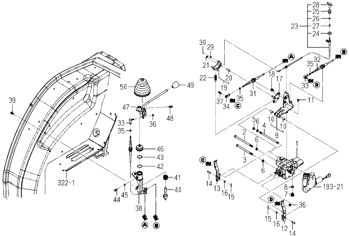
FIG.201 JOY STICK VALVE SYSTEM(HD TYPE)
