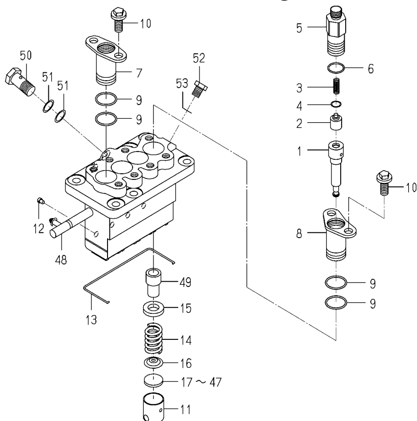
FIG. 44 COMPONENT PARTS FOR 6215-600-119-20 ON Fig.035,36
