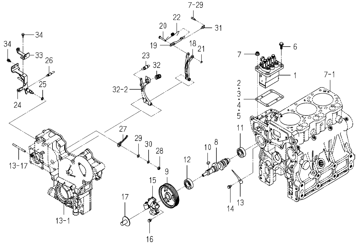
FIG. 30 INJECTION PUMP
