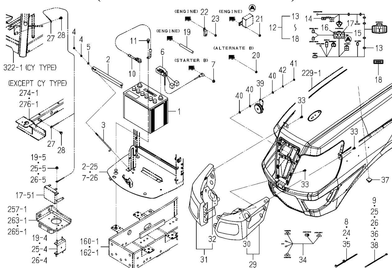
FIG.285 ELC.(FRONT)SYSTEM (6375-SDG TYPE/6405H-G TYPE)
