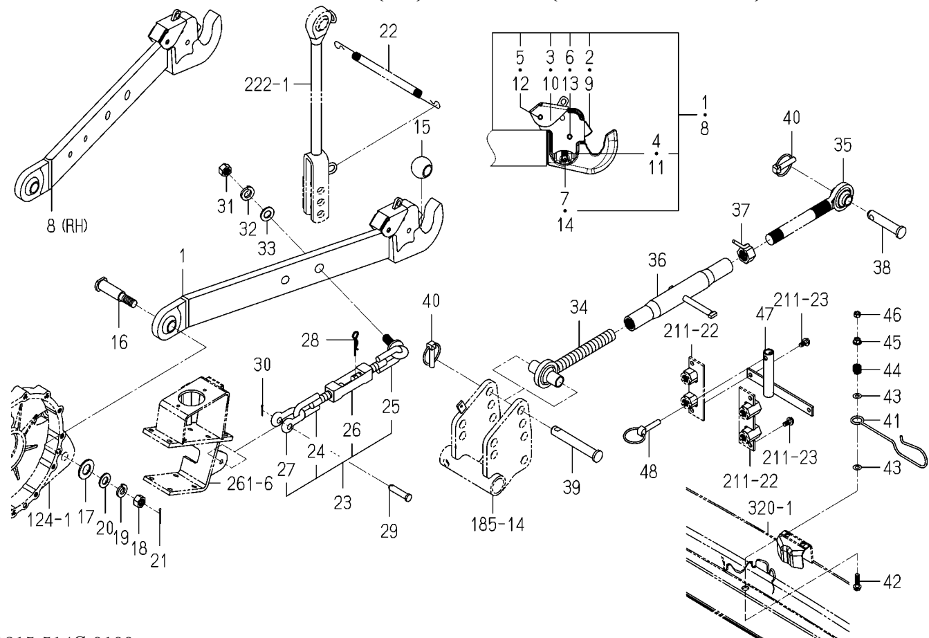
FIG.218 LINK(3P)SYSTEM(6375-CY TYPE)
