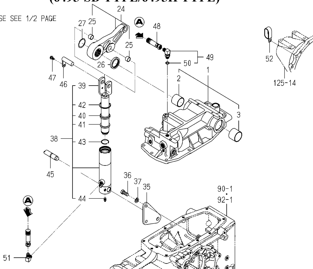
FIG.182 CASE(CYLINDER)SYSTEM(2/2) (6495-SD TYPE/6495H TYPE)
