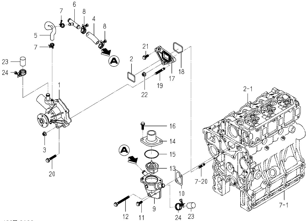
FIG. 20 WATER PUMP
