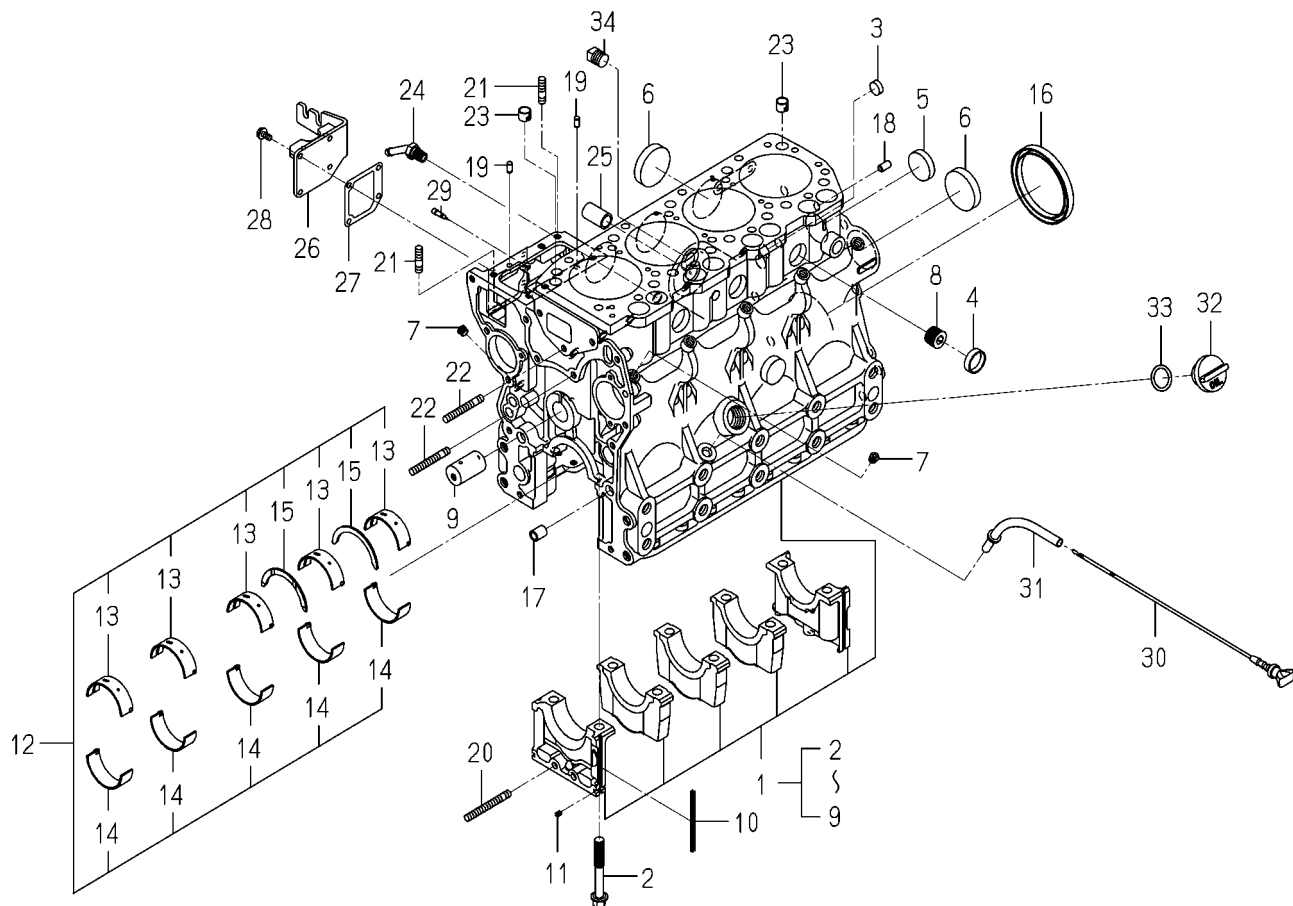
FIG. 8 CYLINDER BLOCK
