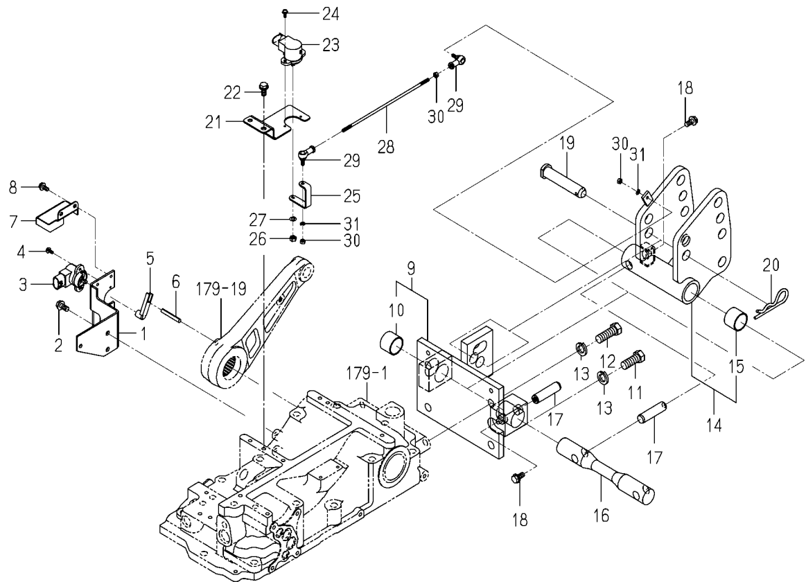
FIG.185 CONTROL(POSITION/DRAFT)SYSTEM (6375-G TYPE)
