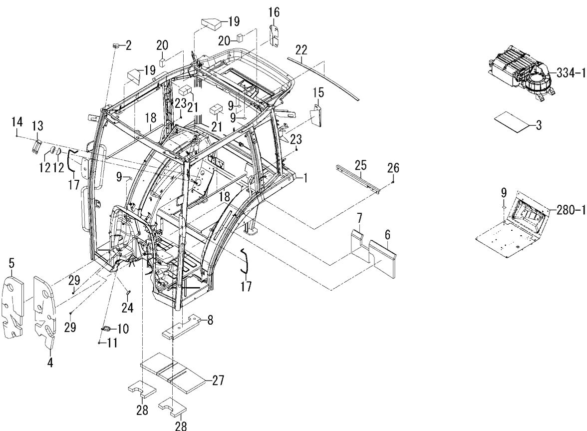
FIG.321 FLAME SYSTEM(6495-CY TYPE)
