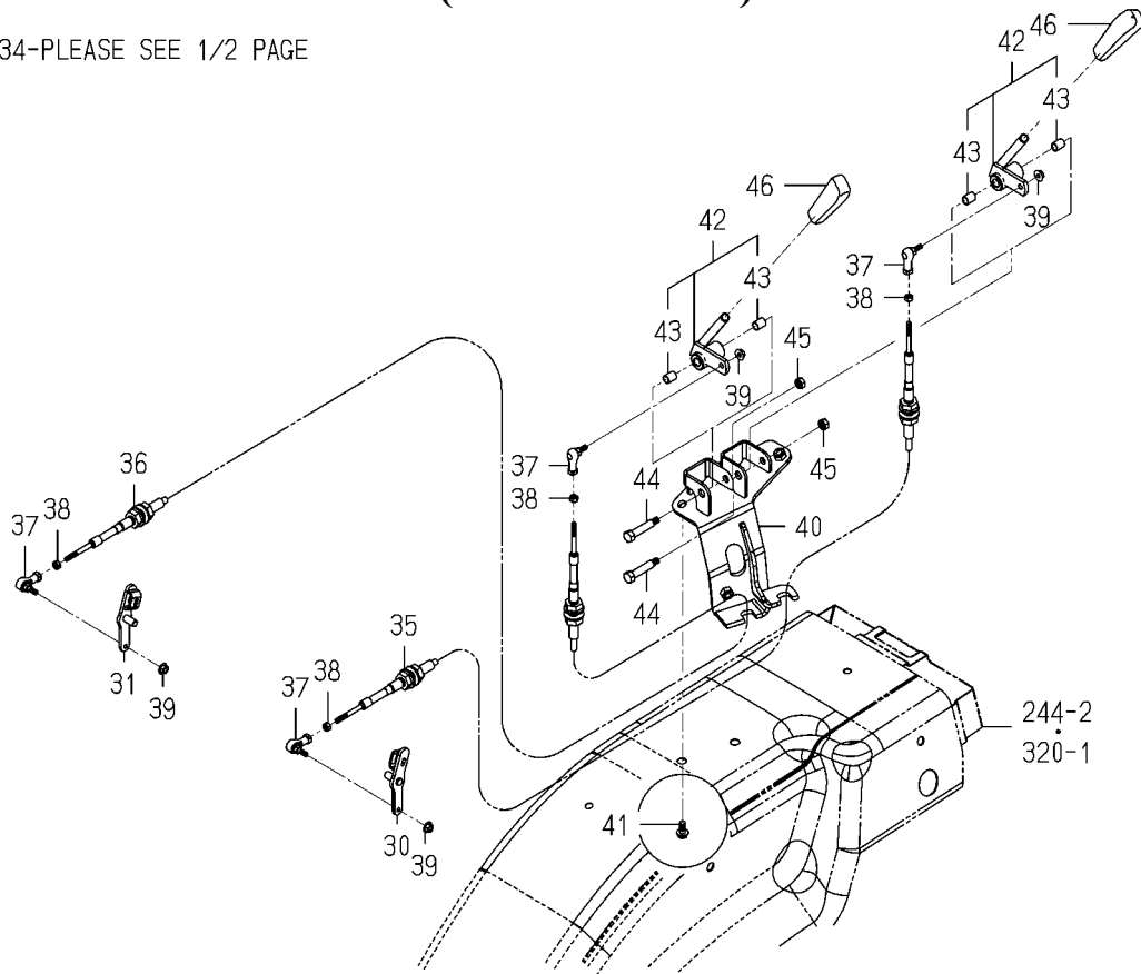
FIG.211 VALVE(REMOTE/2)SET SYSTEM(2/2) (6375-G TYPE)
