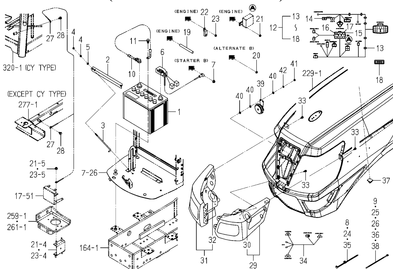
FIG.287 ELC.(FRONT)SYSTEM (6375-G TYPE EXCEPT E4G)
