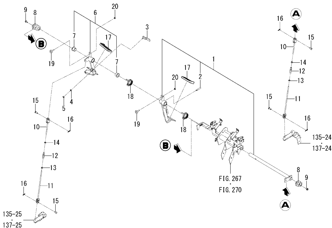
FIG.139 PEDAL(BRAKE)SYSTEM(6375-R TYPE)
