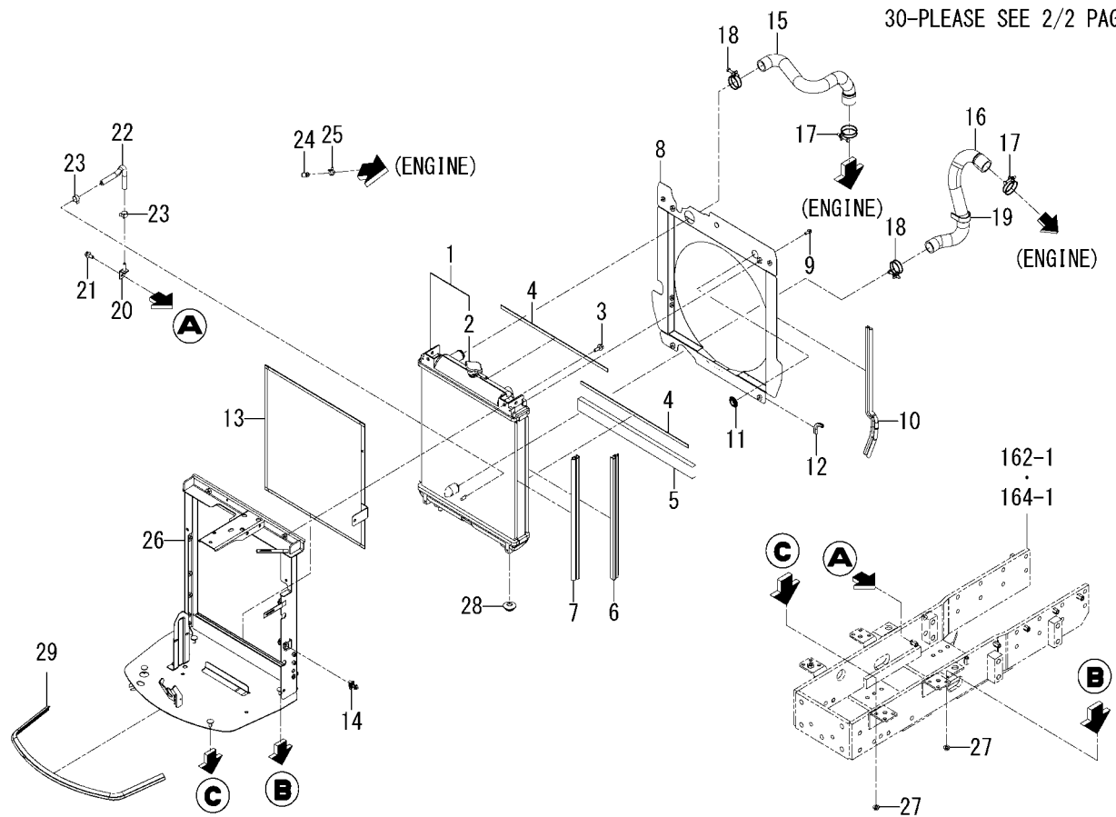
FIG. 7 RADIATOR SYSTEM(6375 TYPE)(1/2)
