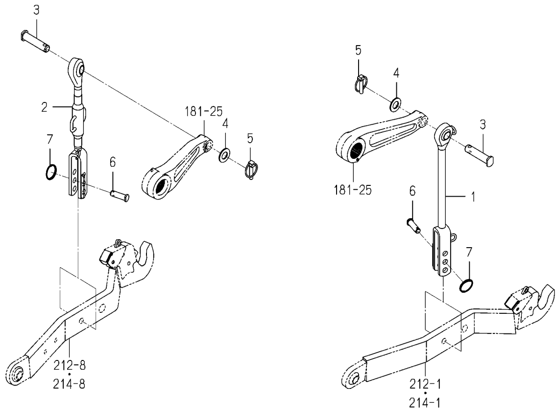
FIG.223 ROD(LIFT)SYSTEM(6495-G TYPE)
