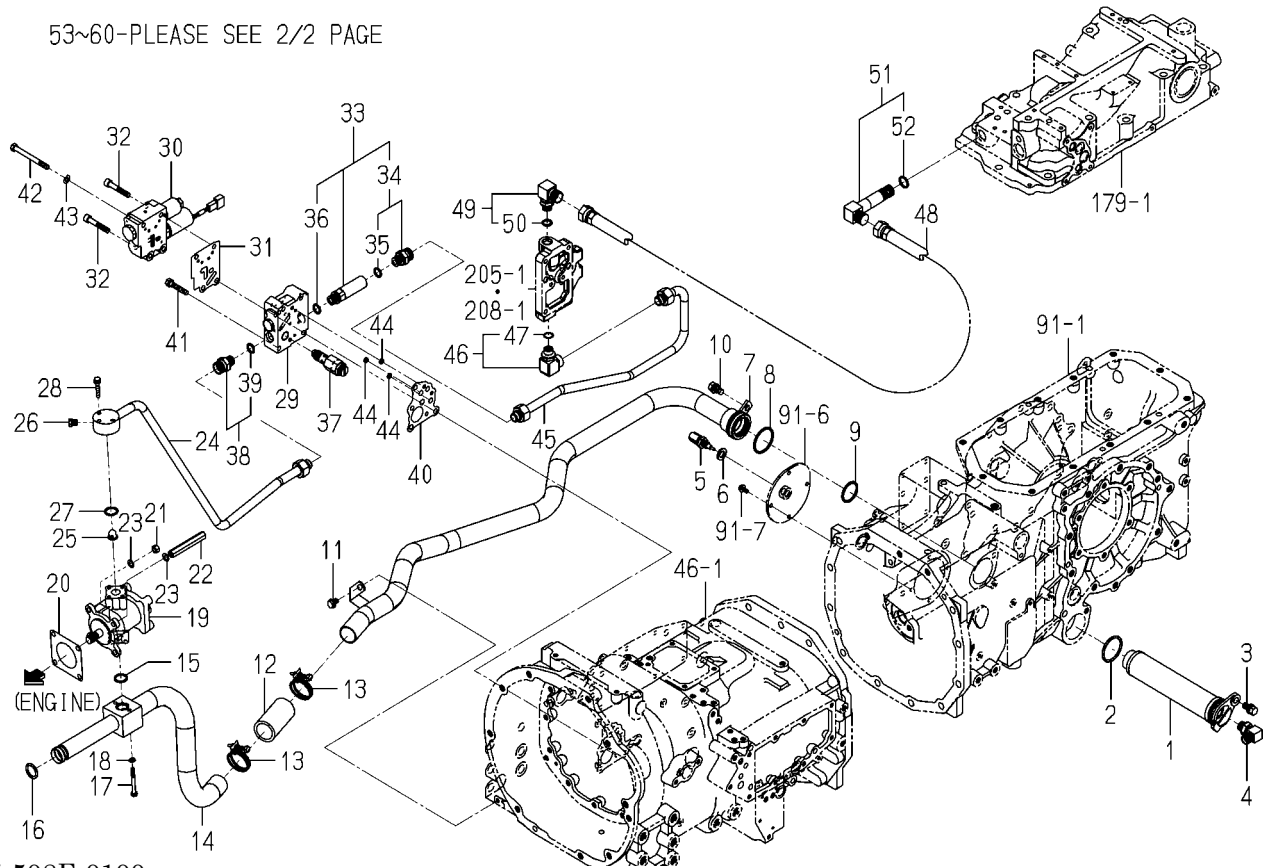
FIG.189 PIPING(MAIN)SYSTEM(1/2) (6375-G TYPE)
