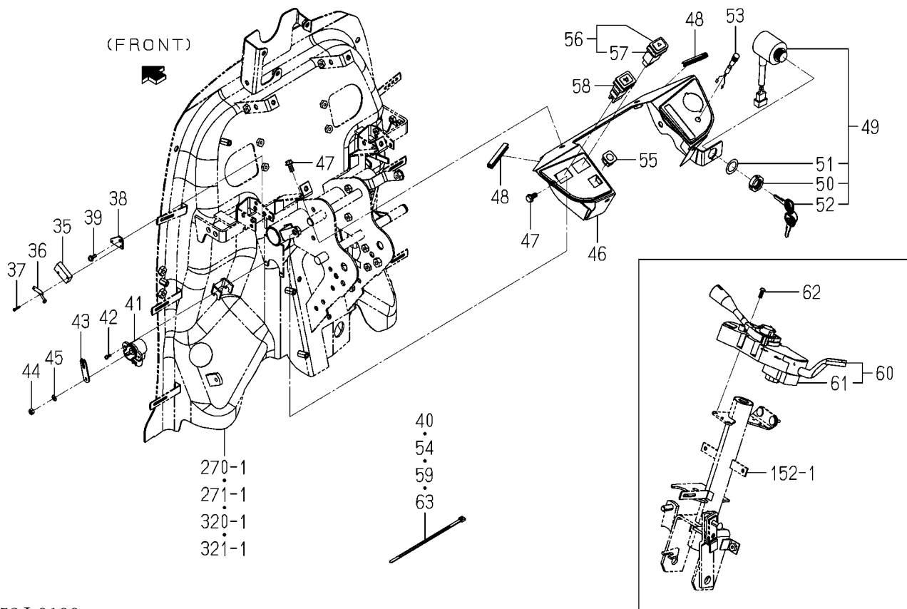
FIG.293 ELC.(MAIN)SYSTEM(G TYPE)(2/2)
