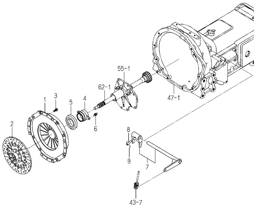
FIG. 37 CLUTCH(MAIN)SYSTEM(6495-SD TYPE)
