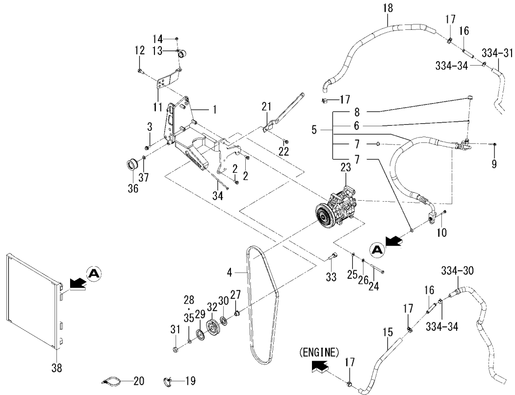
FIG.331 AIR CONDITIONER(1/2) (ENGINE)SYSTEM (6495H-CY TYPE/6495H TYPE)
