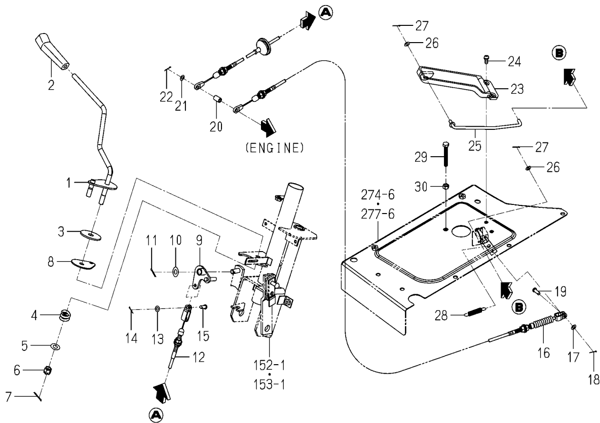
FIG. 29 ACCELERATOR SYSTEM(6375-R TYPE)
