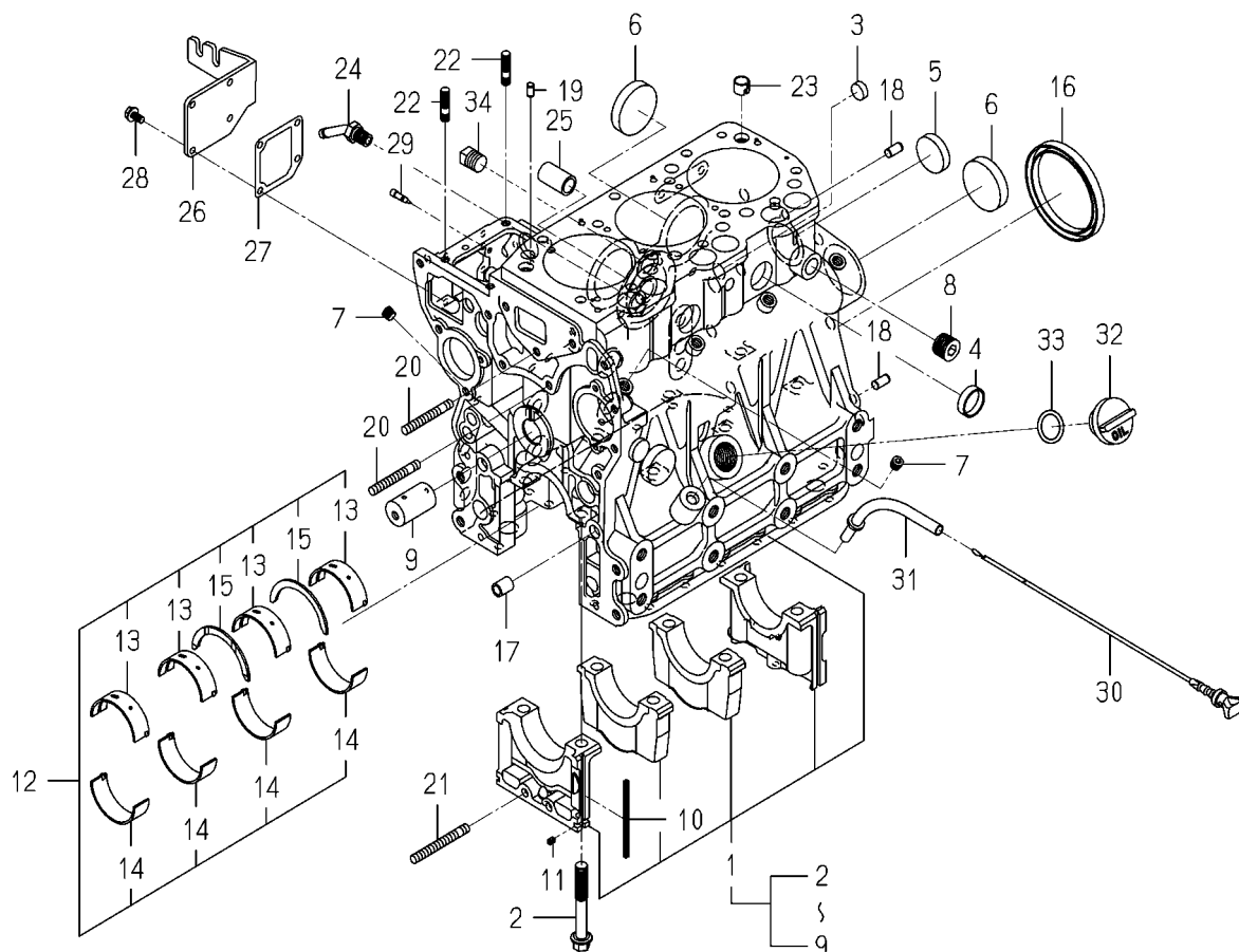
FIG. 8 CYLINDER BLOCK
