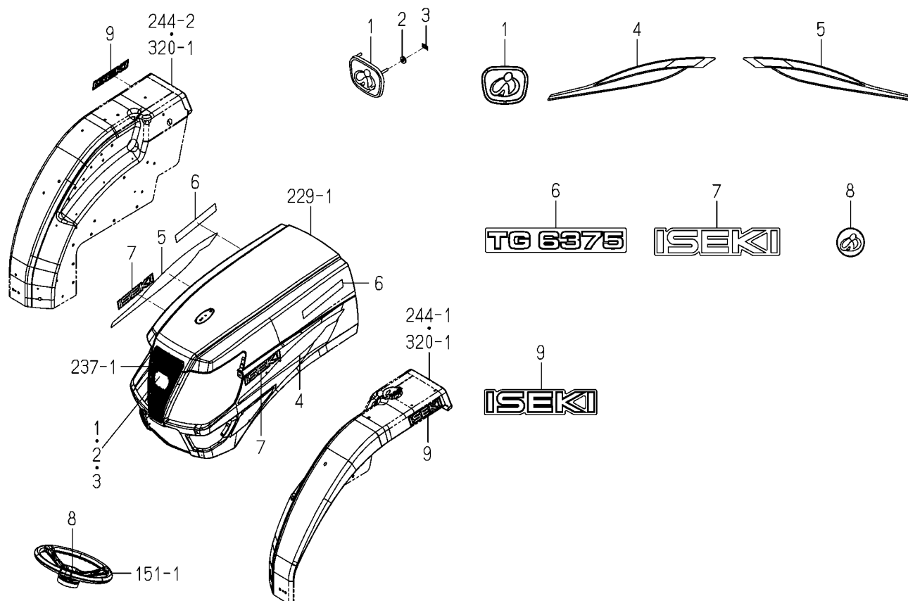
FIG.335 ORNAMENT(6375 TYPE)
