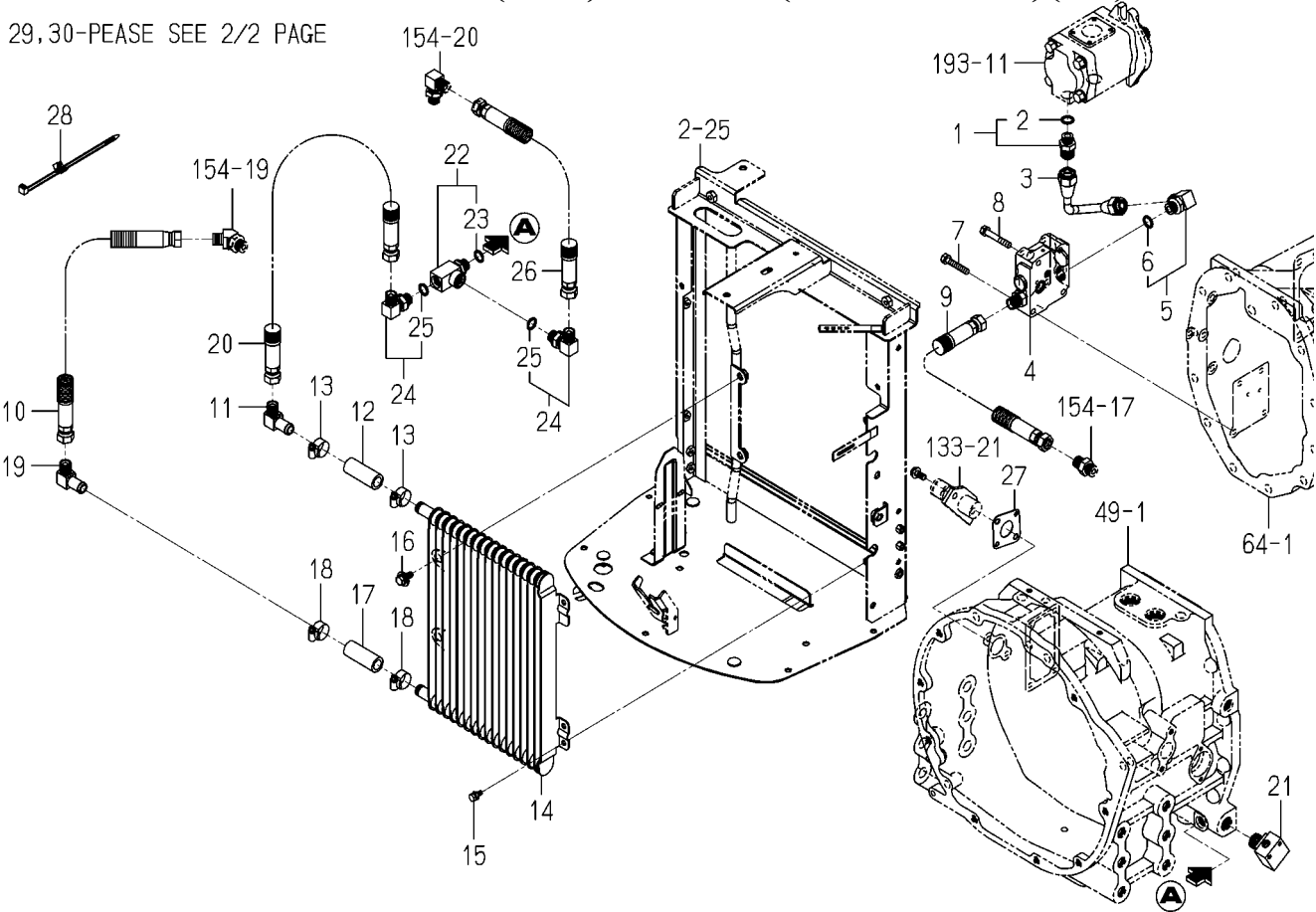
FIG.199 PIPING(SUB)SYSTEM(6405H TYPE)(1/2)
