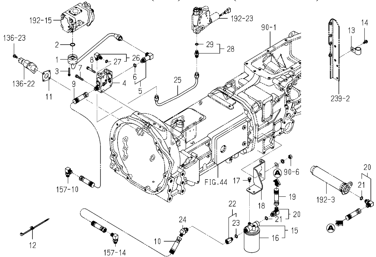
FIG.198 PIPING(SUB)SYSTEM(6495-SD TYPE)
