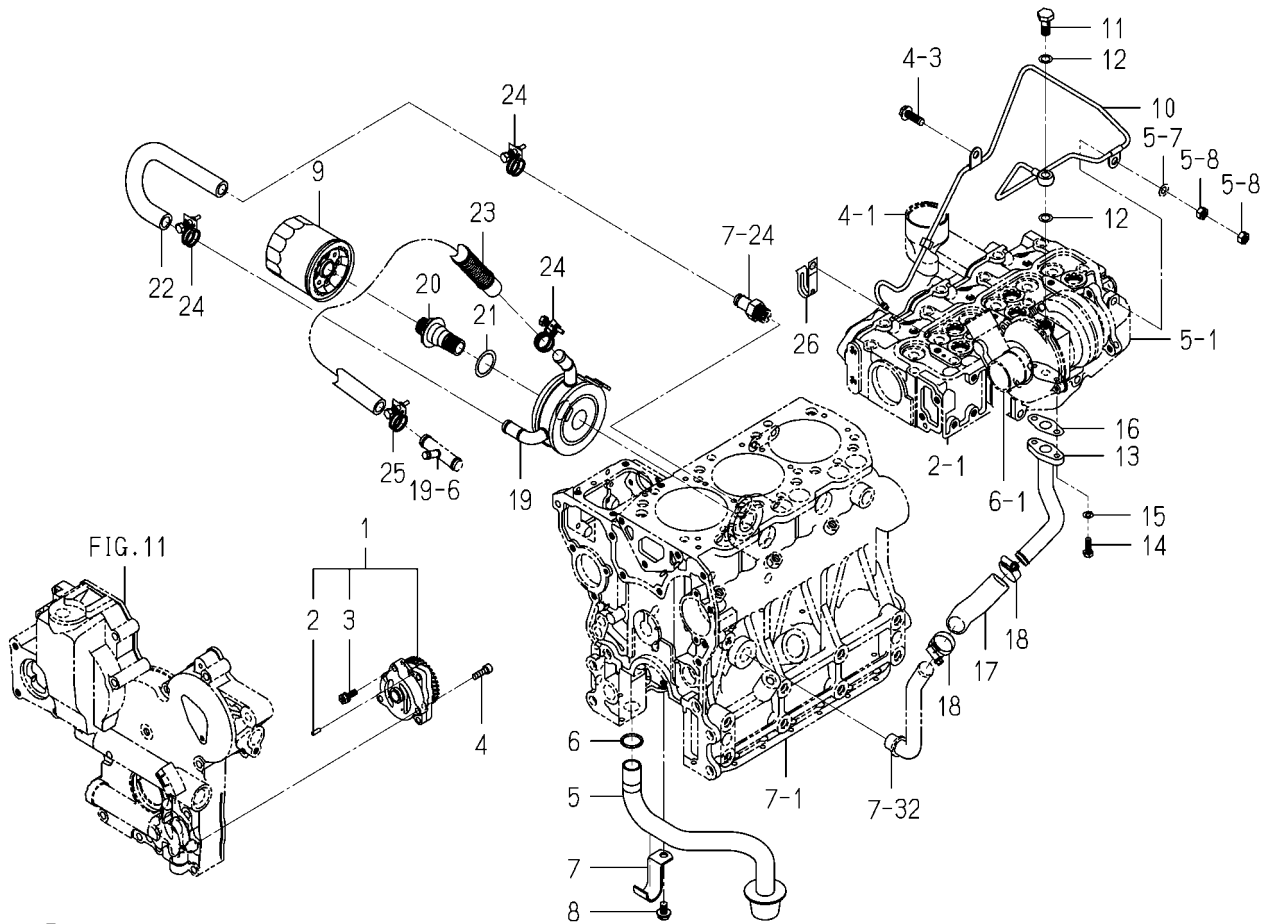
FIG. 18 OIL PUMP
