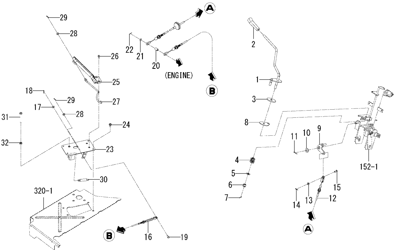
FIG. 33 ACCELERATOR SYSTEM(6375-CY TYPE)
