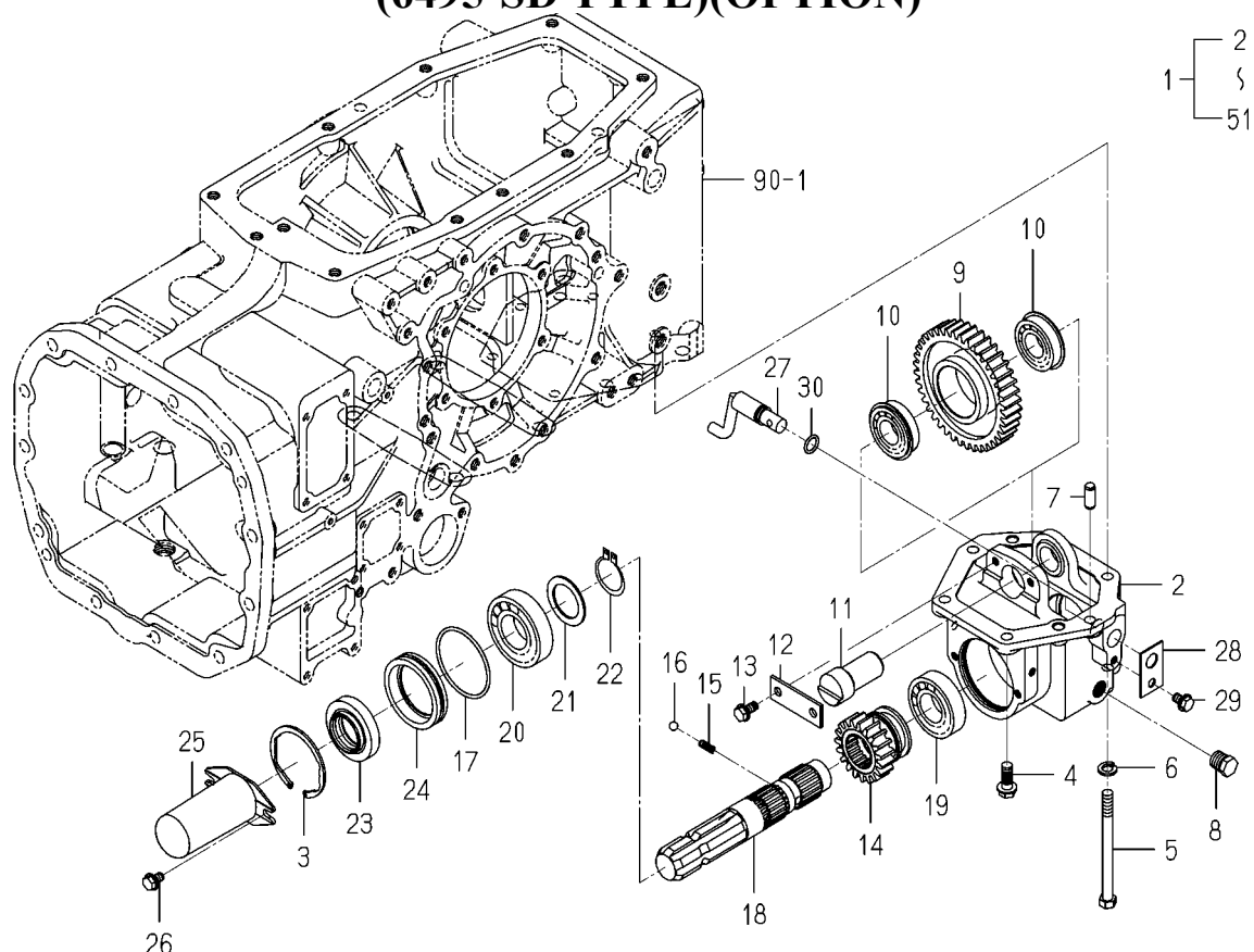
FIG.350 PTO(MID)SYSTEM(1/2) (6495-SD TYPE)(OPTION)
