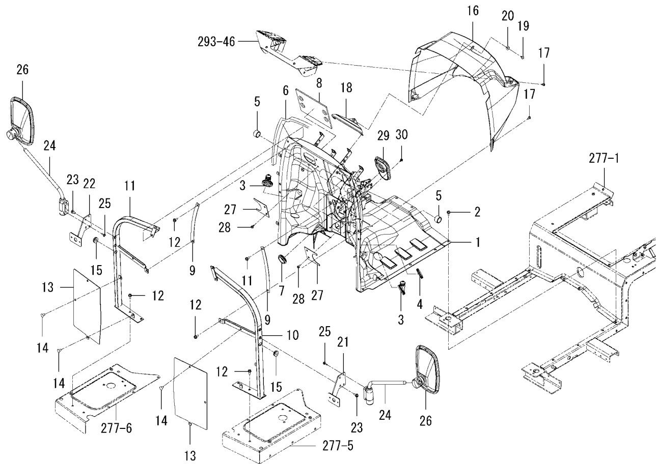
FIG.270 PANEL(DASH)SYSTEM(6375-GR TYPE)
