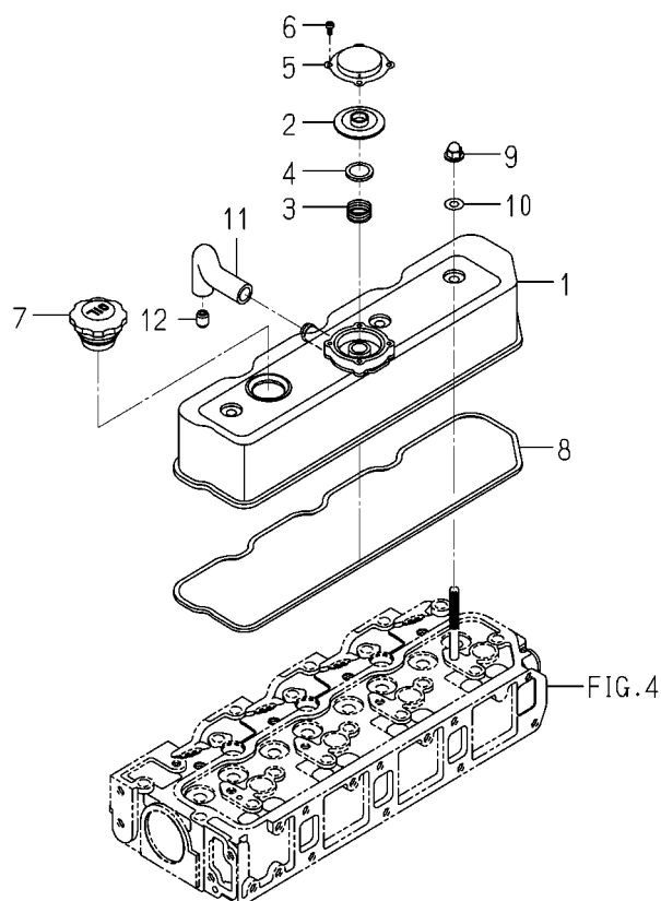
FIG. 5 CYLINDER HEAD COVER
