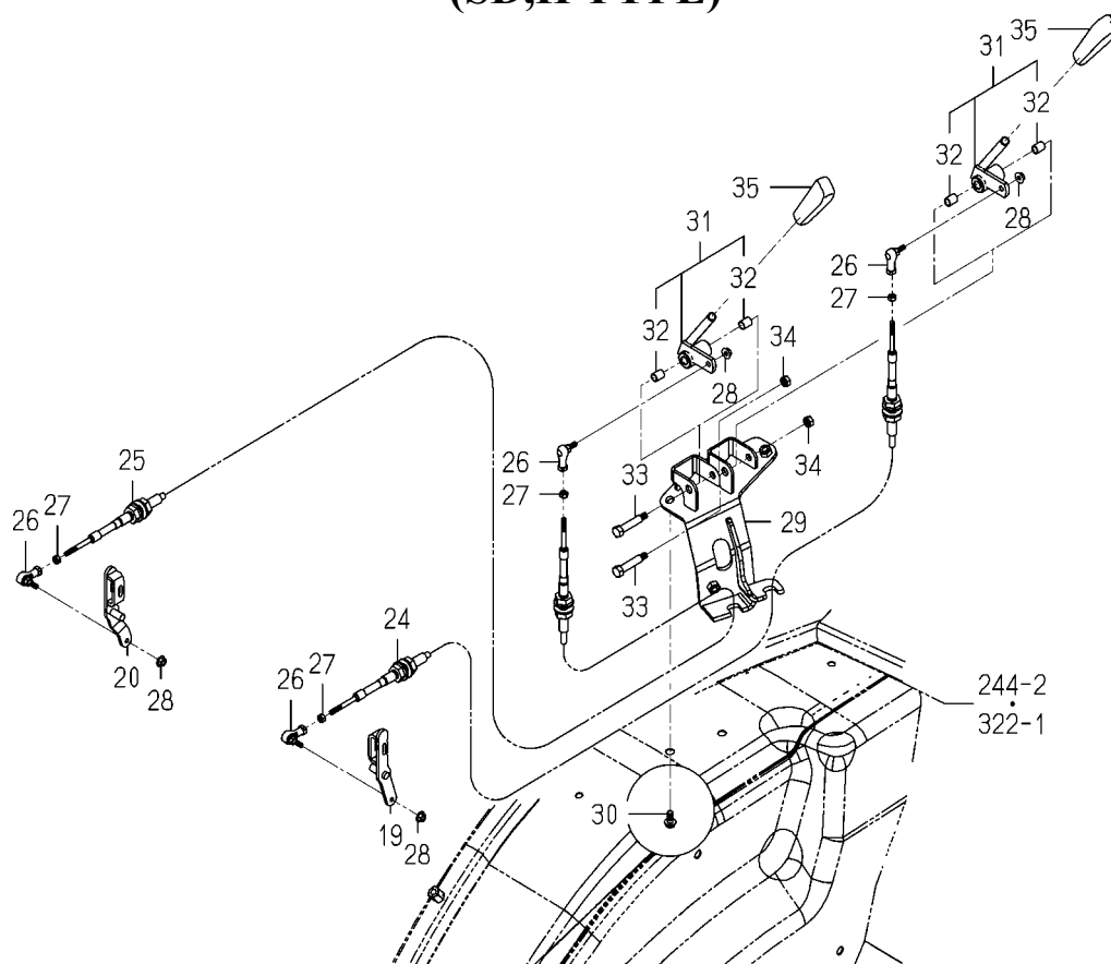
FIG.209 VALVE(REMOTE/2)SET SYSTEM(2/2) (SD,H TYPE)
