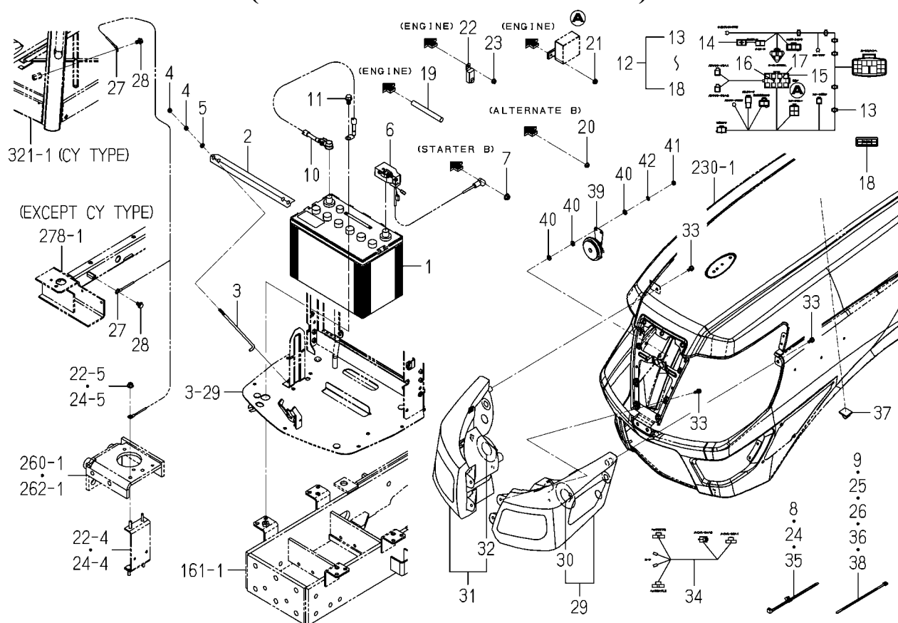
FIG.288 ELC.(FRONT)SYSTEM (6495-G TYPE EXCEPT E4G)
