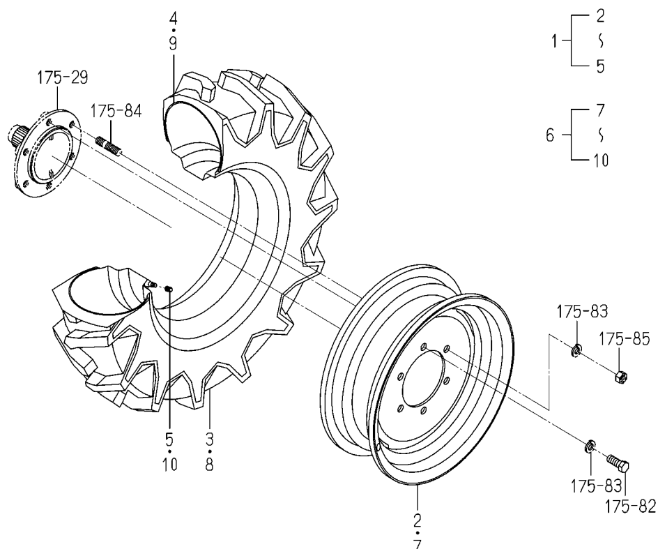
FIG.361 WHEEL(FRONT/AGR/8-16)ASSY (6495 TYPE/6495H TYPE)(OPTION)
