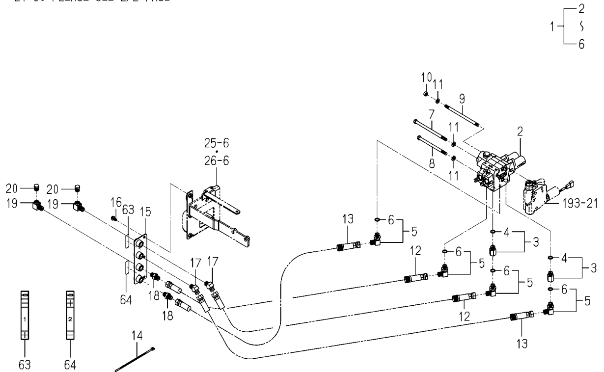
FIG.206 JOY STICK VALVE SYSTEM(1/2) (H TYPE EXCEPT D)
