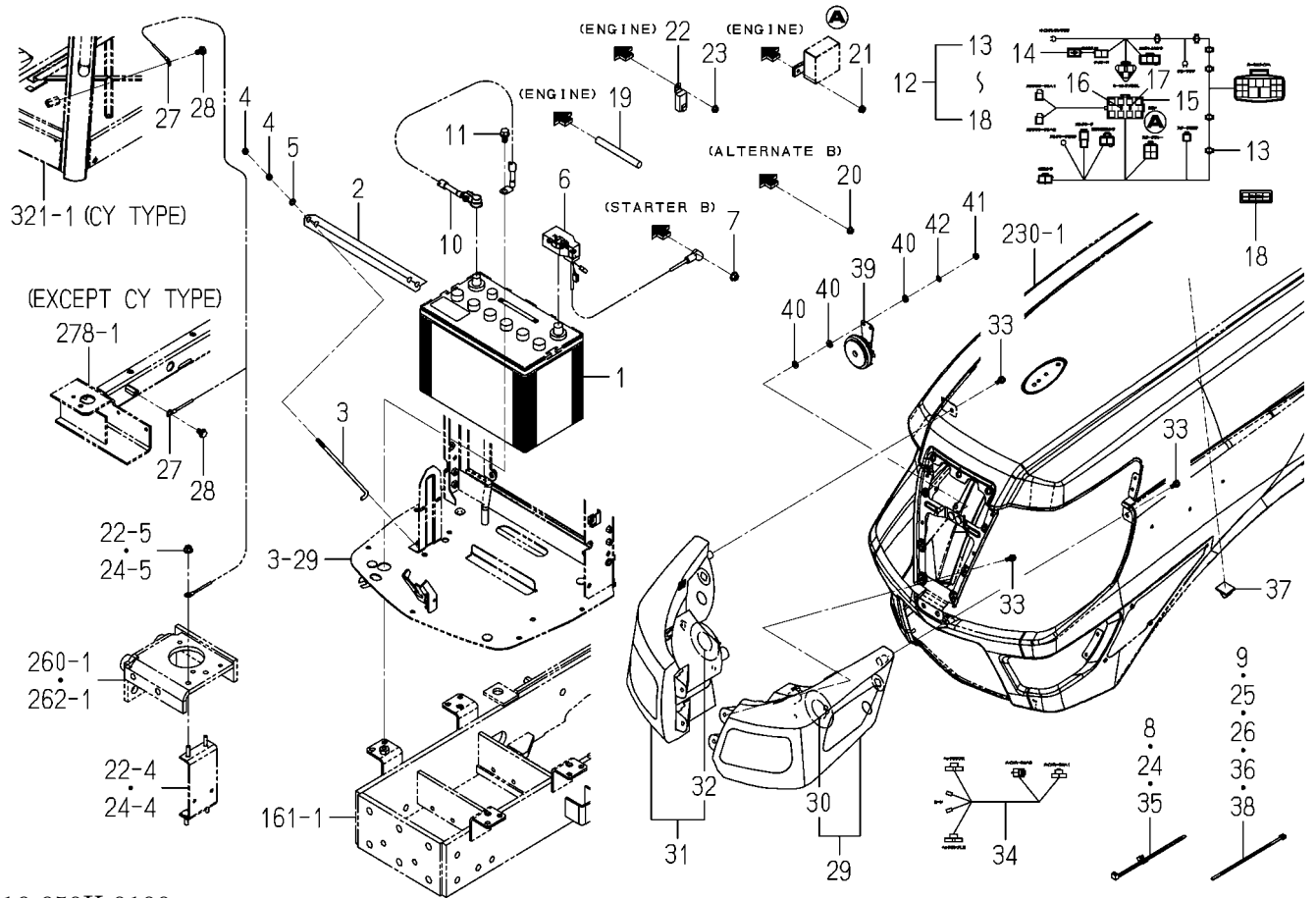
FIG.290 ELC.(FRONT)SYSTEM(6495-E4G TYPE)
