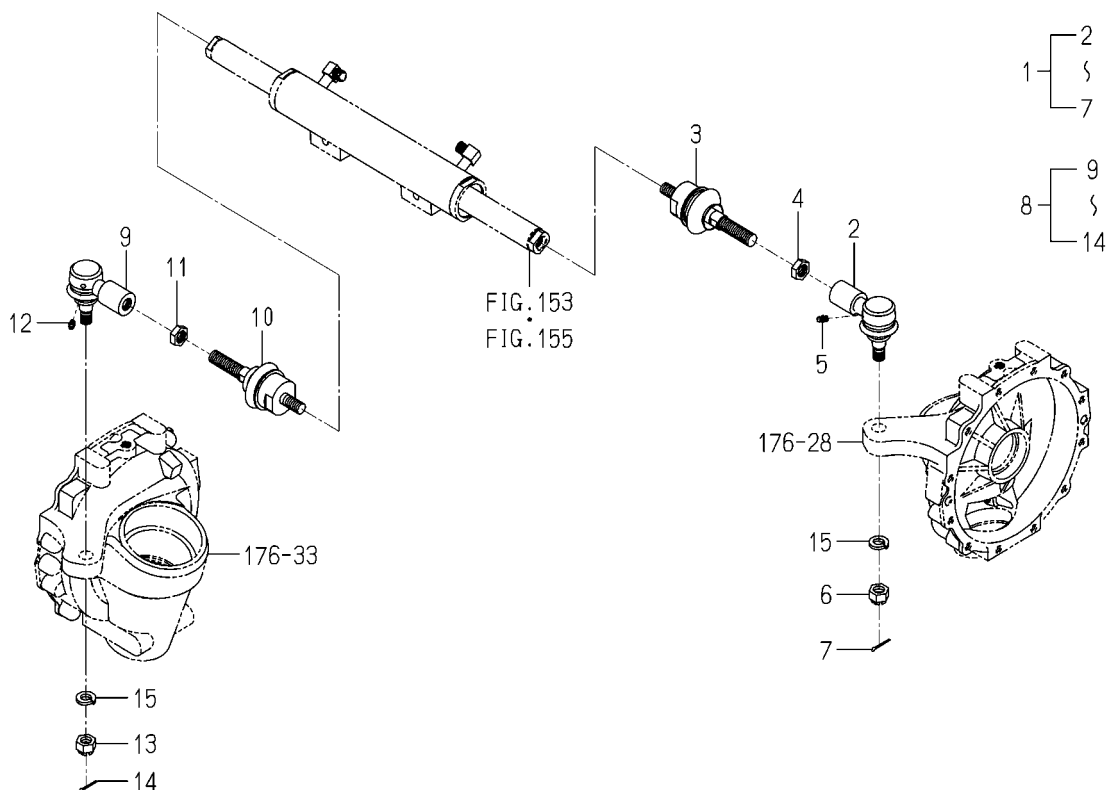
FIG.178 ROD(TIE)SYSTEM (6375 TYPE/6405H TYPE)
