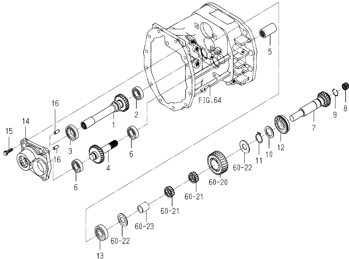
FIG. 68 GEAR(MAIN)SYSTEM(6405H TYPE)
