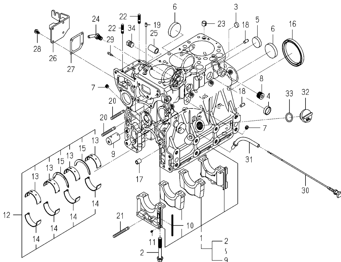
FIG. 7 CYLINDER BLOCK
