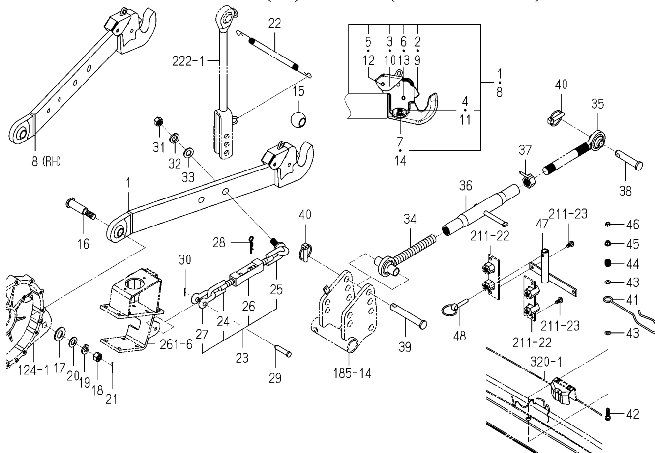
FIG.218 LINK(3P)SYSTEM(6375-CY TYPE)
