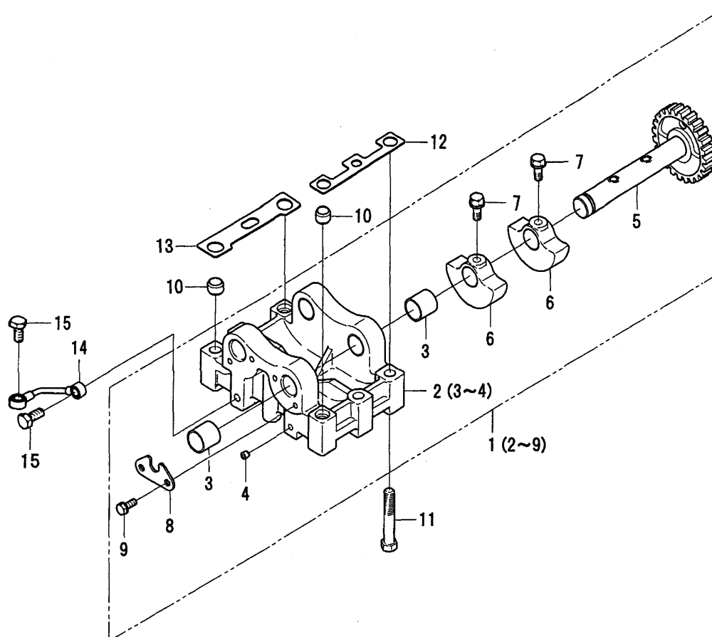
FIG.012 BALANCER
