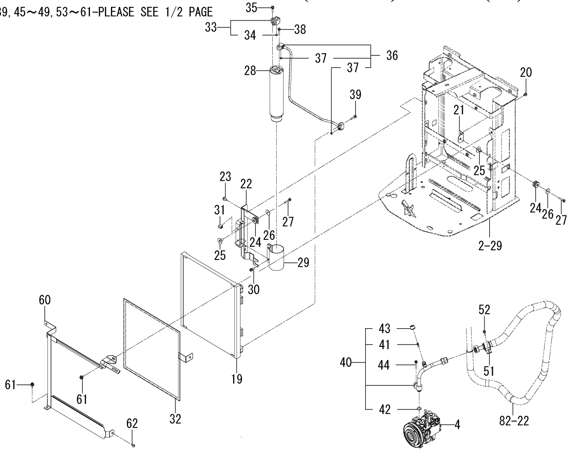
FIG. 81 AIR CONDITIONER(ENGINE)SYSTEM(2/2)
