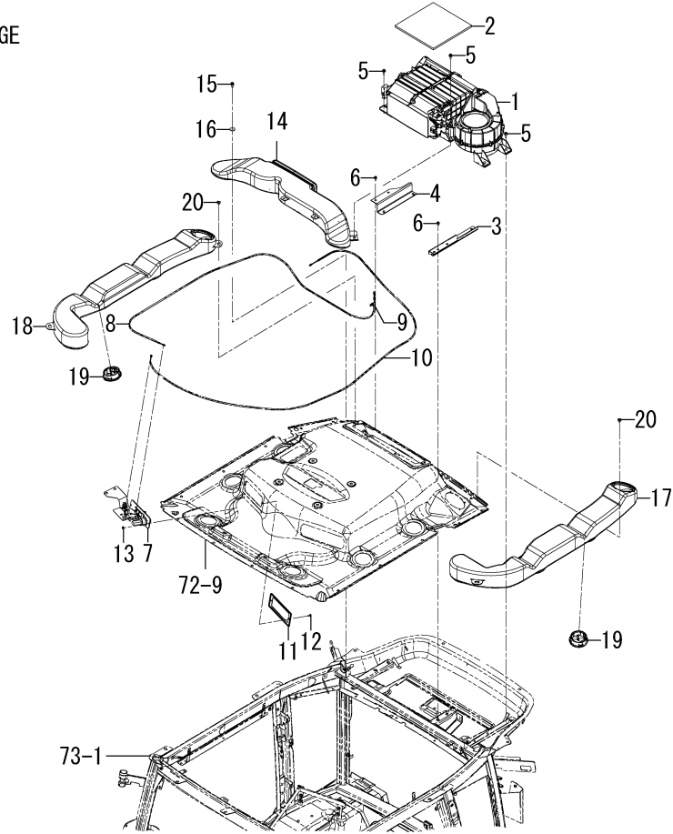
FIG. 82 AIR CONDITIONER(MANUAL)SYSTEM(1/2)
