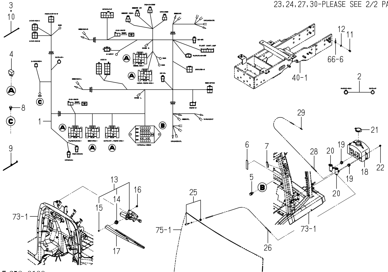
FIG. 69 ELC.(CABIN)SYSTEM(1/2)
