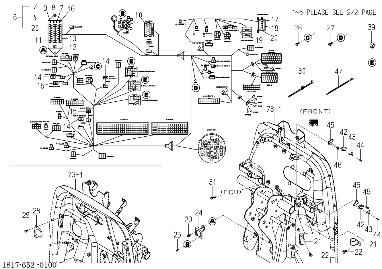
FIG. 66 ELC.(MAIN)SYSTEM(1/2)
