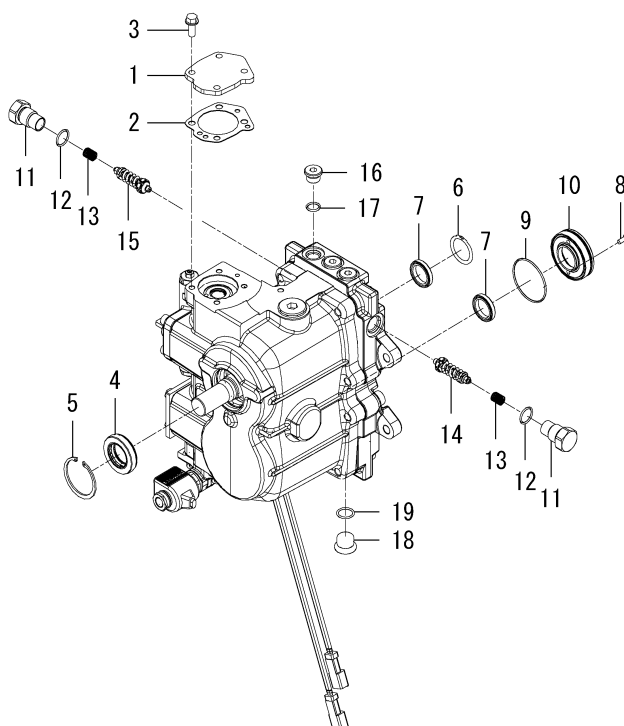
FIG.111 COMPONENT PARTS FOR 1816-203-500-00 ON FIG.13
