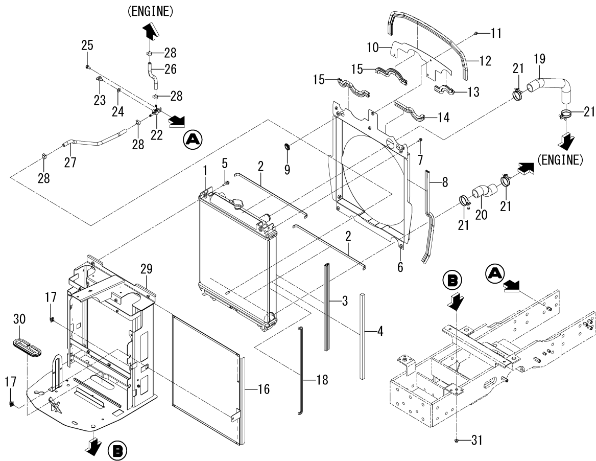
FIG. 2 RADIATOR SYSTEM(1/2)
