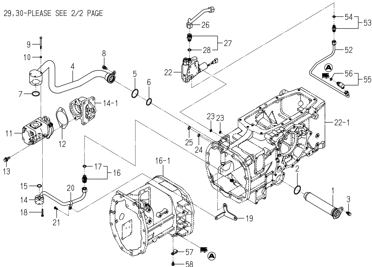
FIG. 48 PIPING(MAIN)SYSTEM(1/2)
