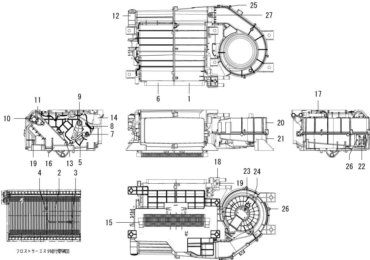
FIG.108 COMPONENT PARTS FOR 1792-782-600-20 ON FIG.82
