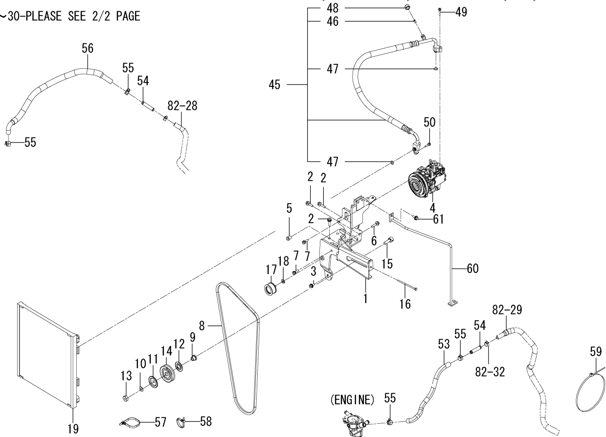
FIG. 81 AIR CONDITIONER(ENGINE)SYSTEM(1/2)
