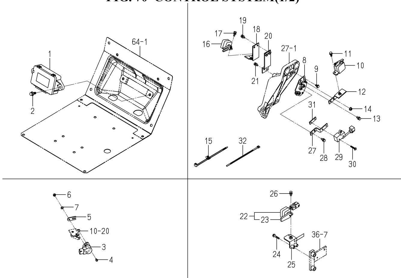
FIG. 70 CONTROL SYSTEM(1/2)
