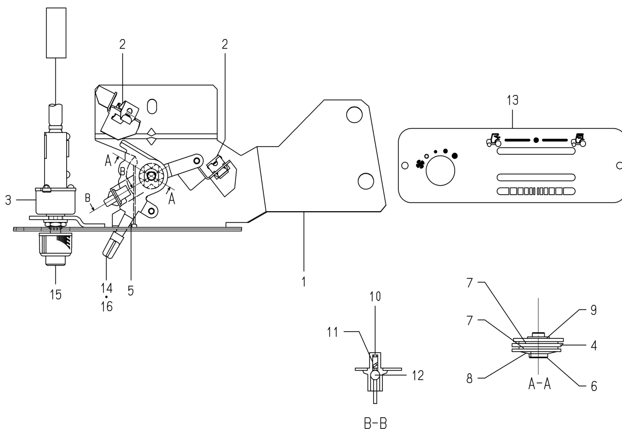
FIG.109 COMPONENT PARTS FOR 1800-782-400-10 ON FIG.82
