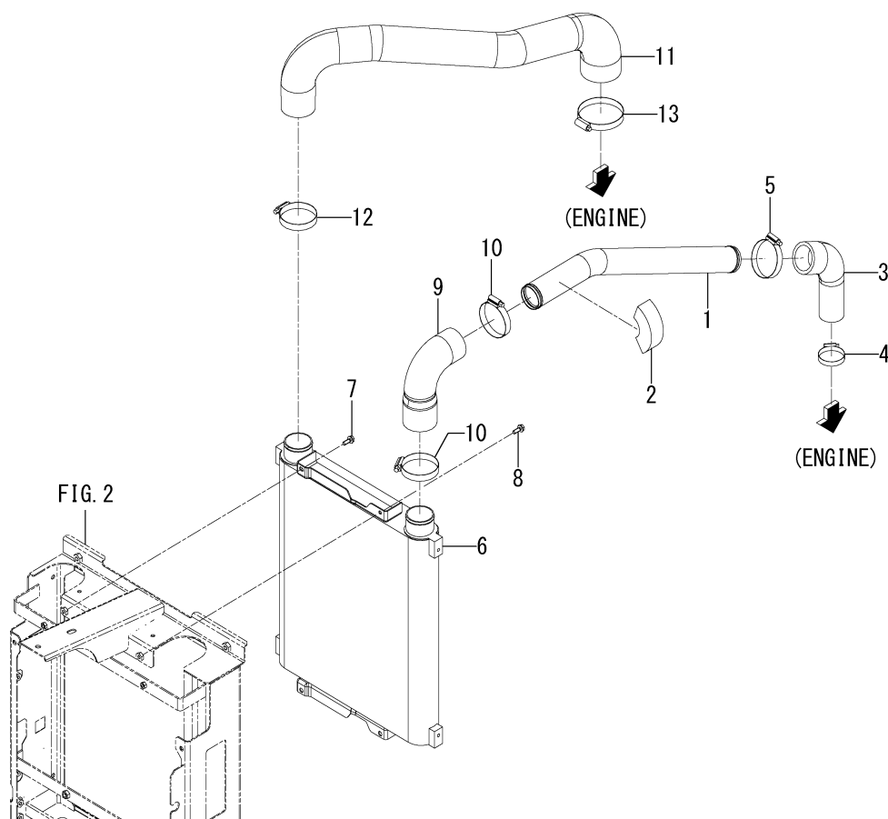
FIG. 5 INTERCOOLER SYSTEM
