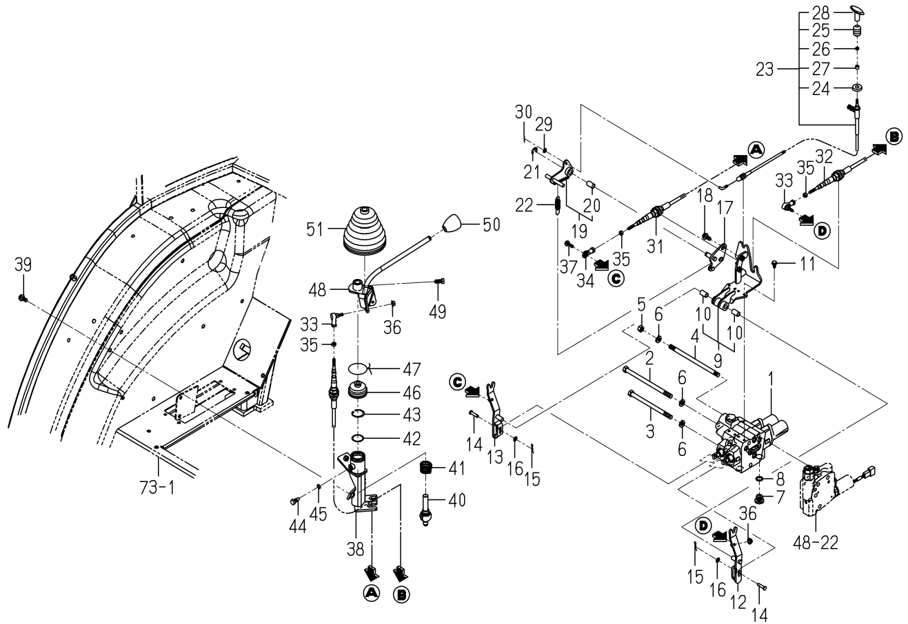
FIG. 51 JOY STICK VALVE SYSTEM(D TYPE)
