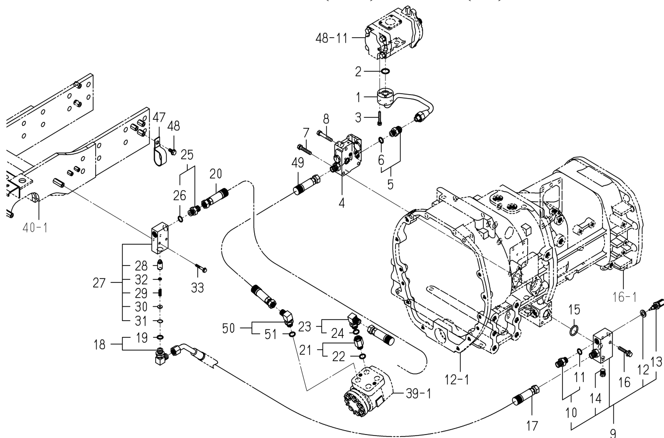
FIG. 49 PIPING(SUB)SYSTEM(1/3)
