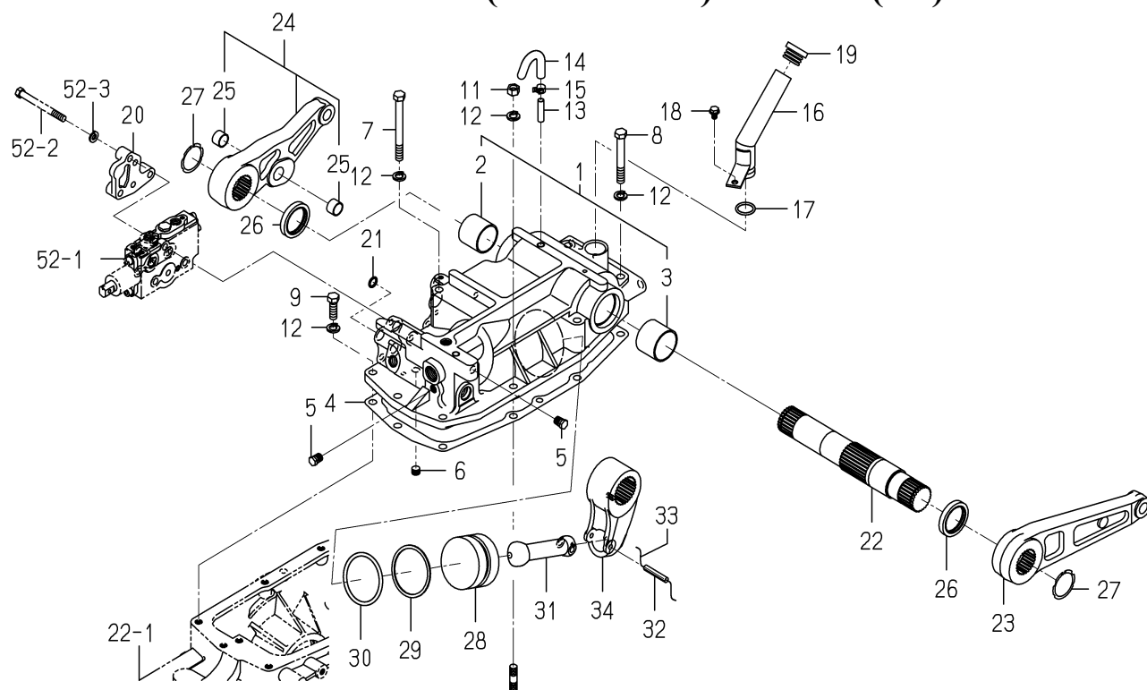
FIG. 46 CASE(CYLINDER)SYSTEM(1/2)
