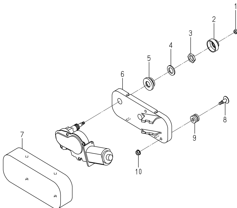
FIG.107 COMPONENT PARTS FOR 1757-658-370-10 ON FIG.97
