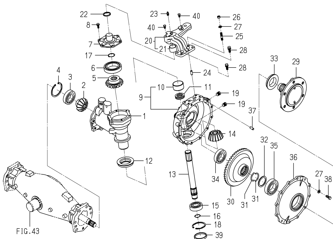
FIG. 44 CASE(GEAR/FINAL)SYSTEM(1/2)
