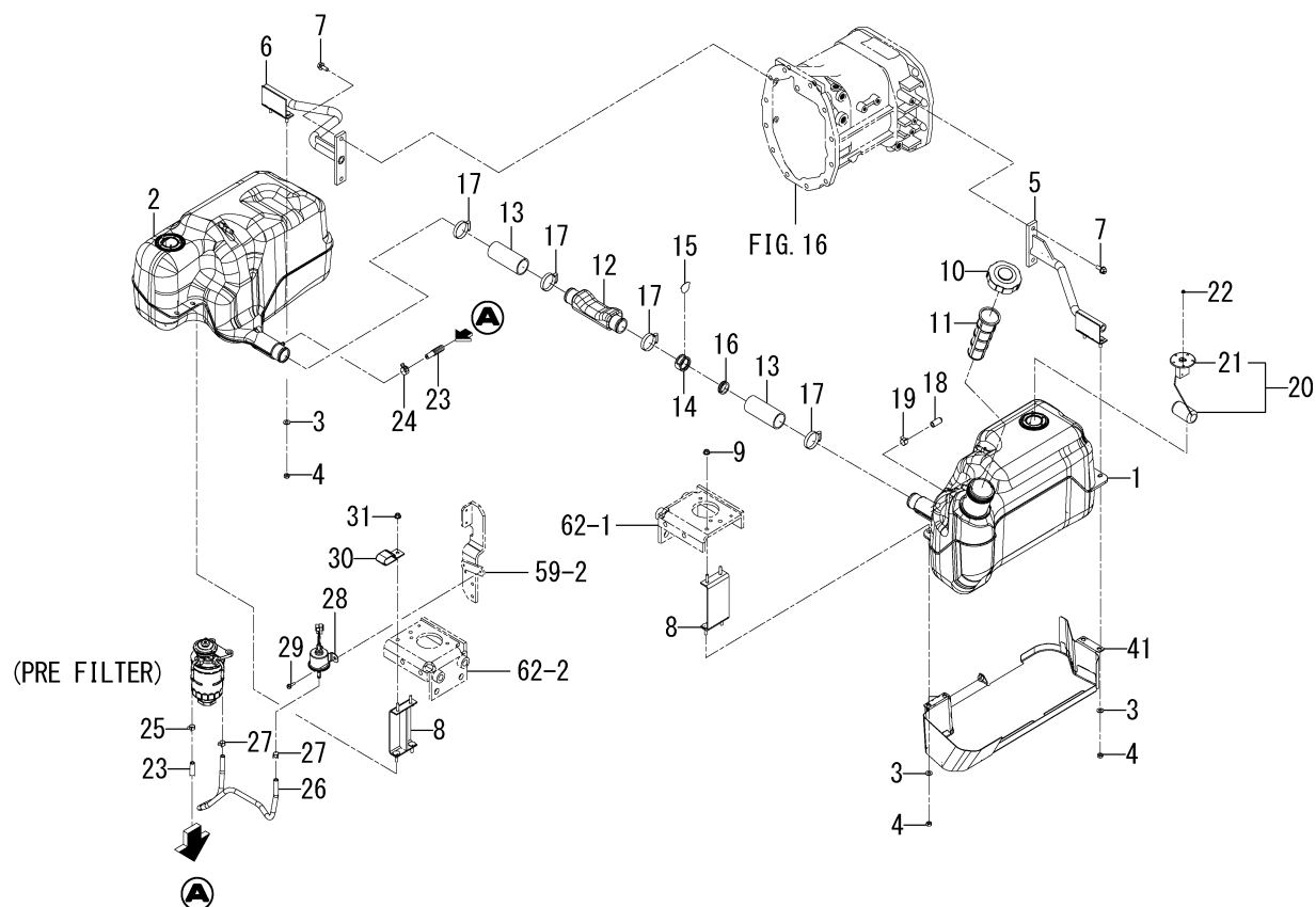
FIG. 6 TANK(FUEL)SYSTEM(1/2)
