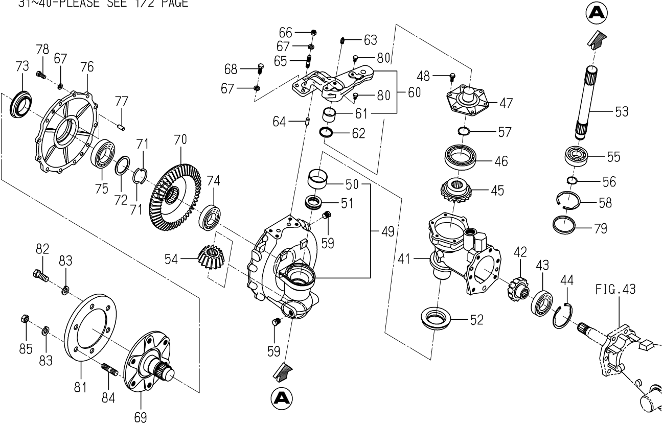
FIG. 44 CASE(GEAR/FINAL)SYSTEM(2/2)
