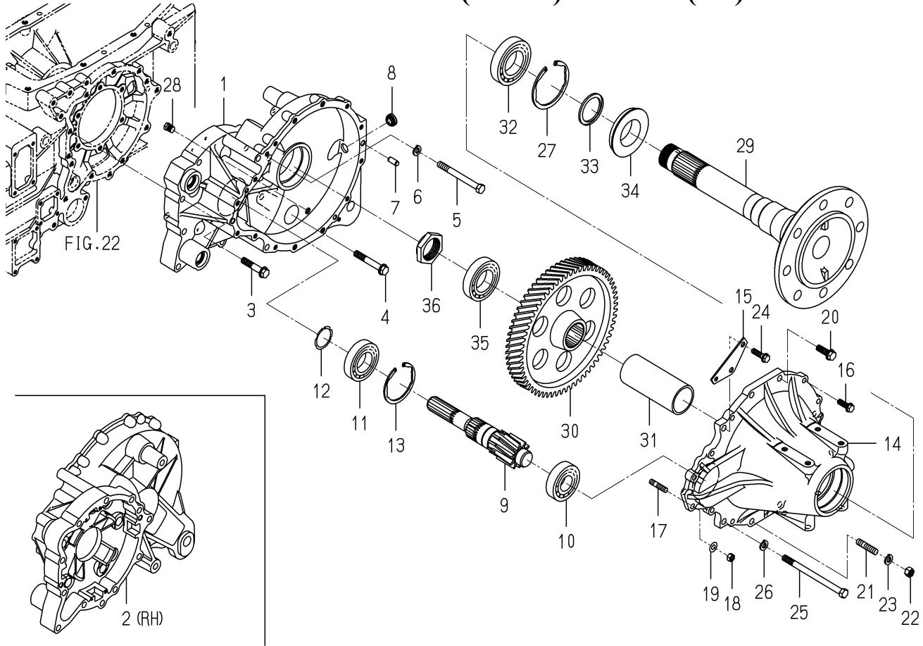
FIG. 32 HOUSING(AXLE)SYSTEM(1/2)
