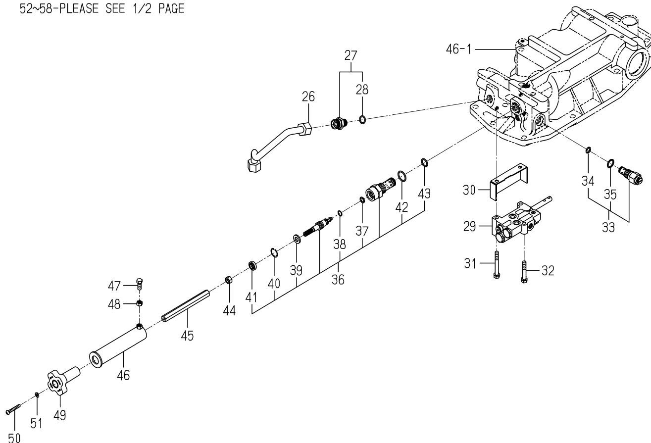
FIG. 48 PIPING(MAIN)SYSTEM(2/2)
