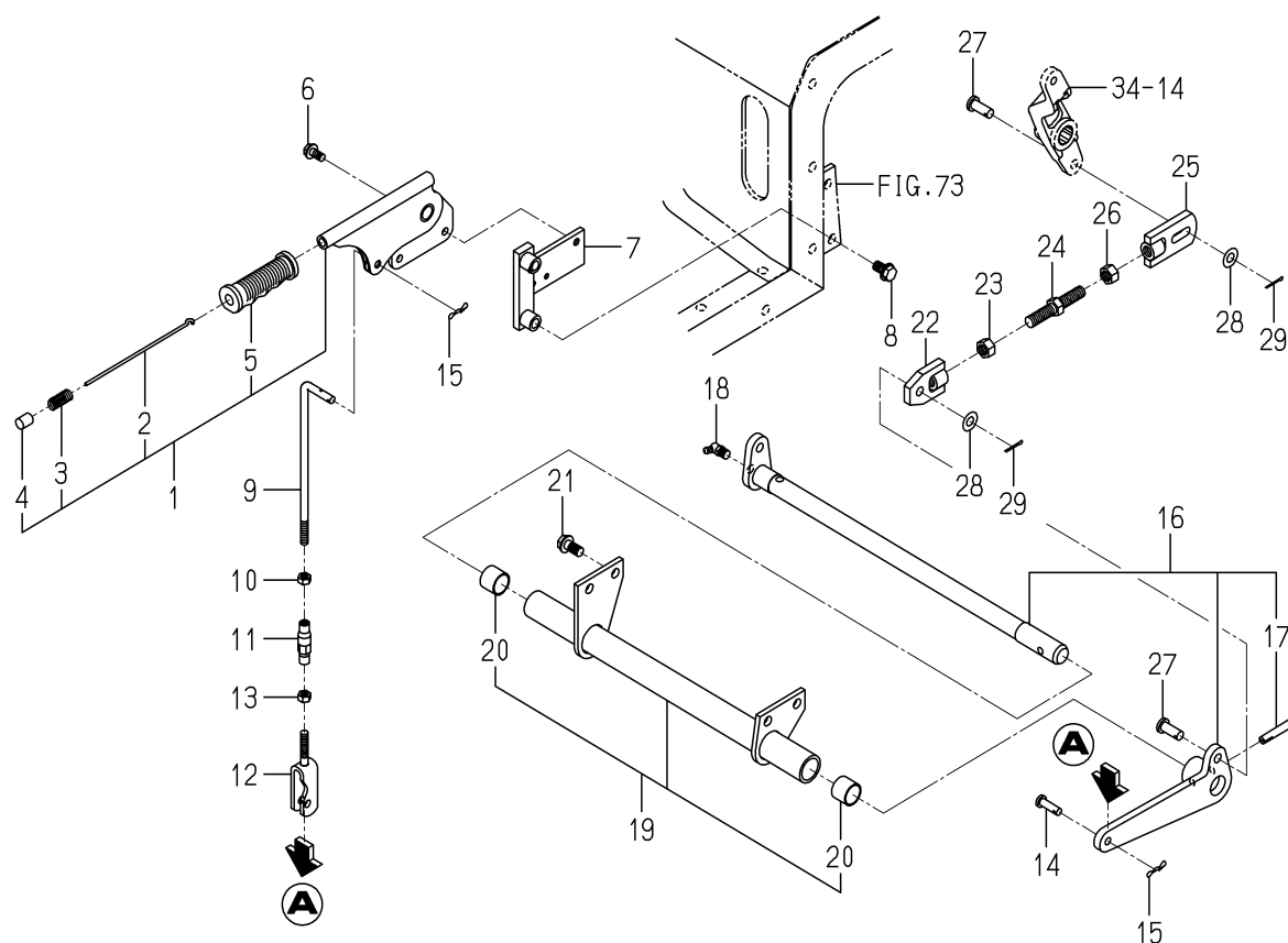
FIG. 36 LEVER(BRAKE/PARKING)SYSTEM
