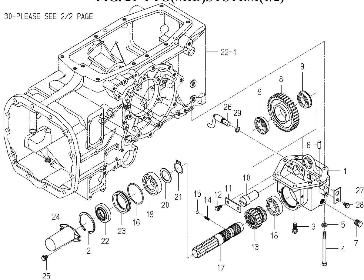
FIG. 21 PTO(MID)SYSTEM(1/2)
