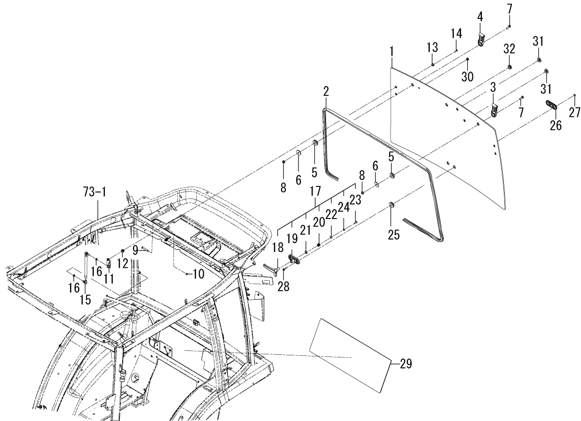
FIG. 79 GLASS(REAR)SYSTEM
