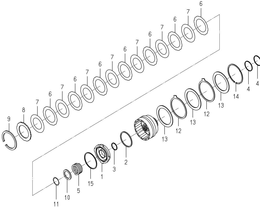
FIG.110 COMPONENT PARTS FOR 1802-209-200-00 ON FIG.15
