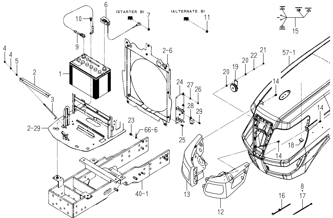
FIG. 65 ELC.(FRONT)SYSTEM
