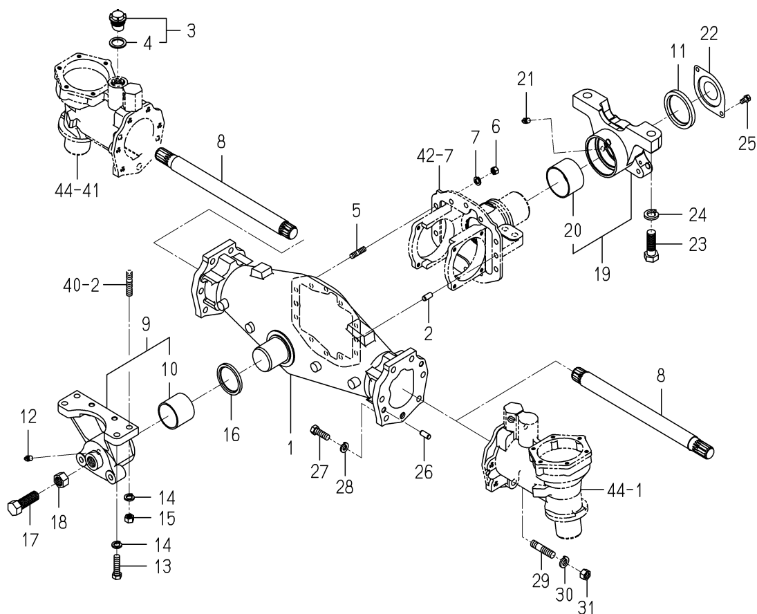
FIG. 43 HOUSING(AXLE)SYSTEM
