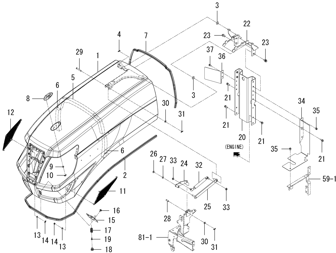
FIG. 57 HOOD SYSTEM
