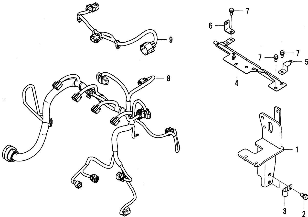
FIG.013 HARNESS WIRE
