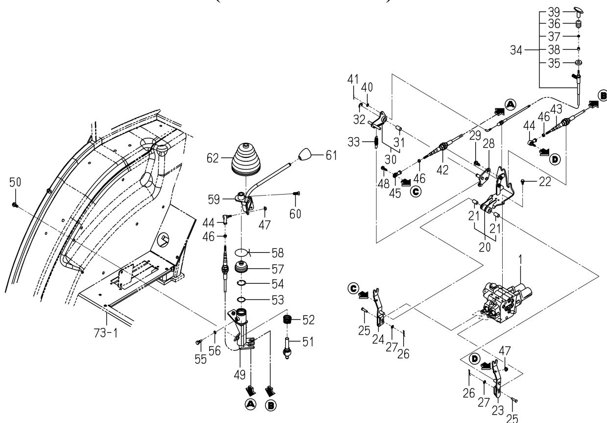
FIG. 50 JOY STICK VALVE SYSTEM(2/2) (ECXEPT D TYPE)
