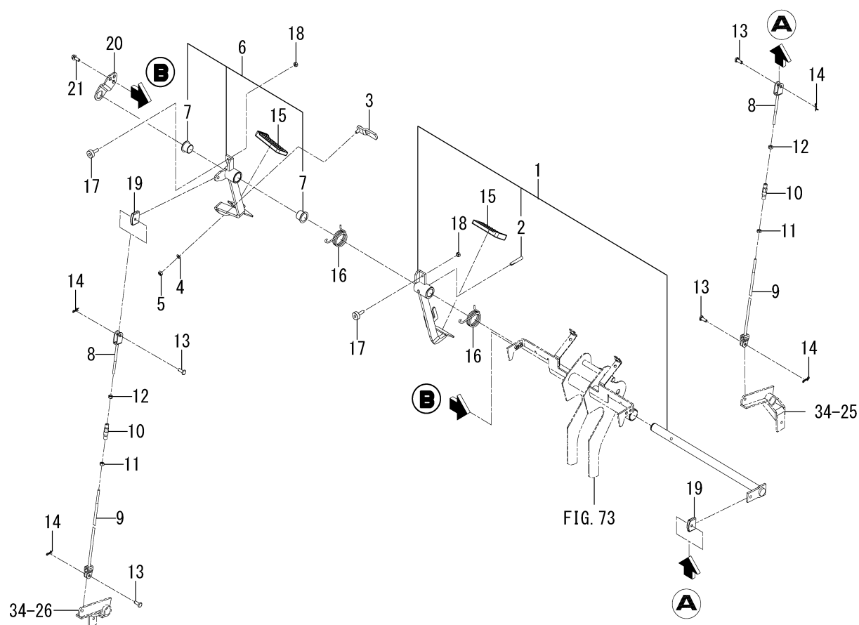
FIG. 35 PEDAL(BRAKE)SYSTEM
