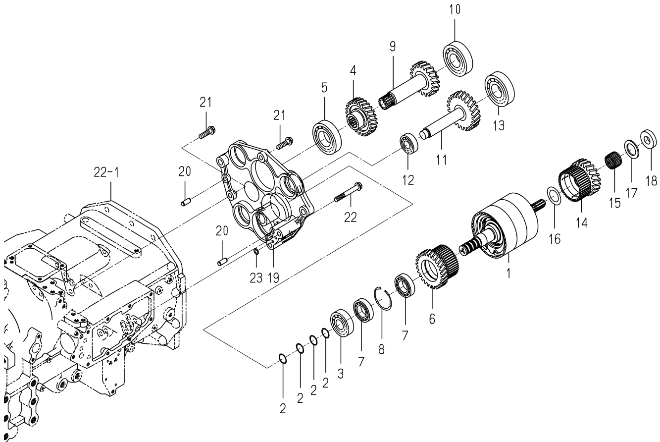
FIG. 30 GEAR(REVERSE)SYSTEM(6490 TYPE)
