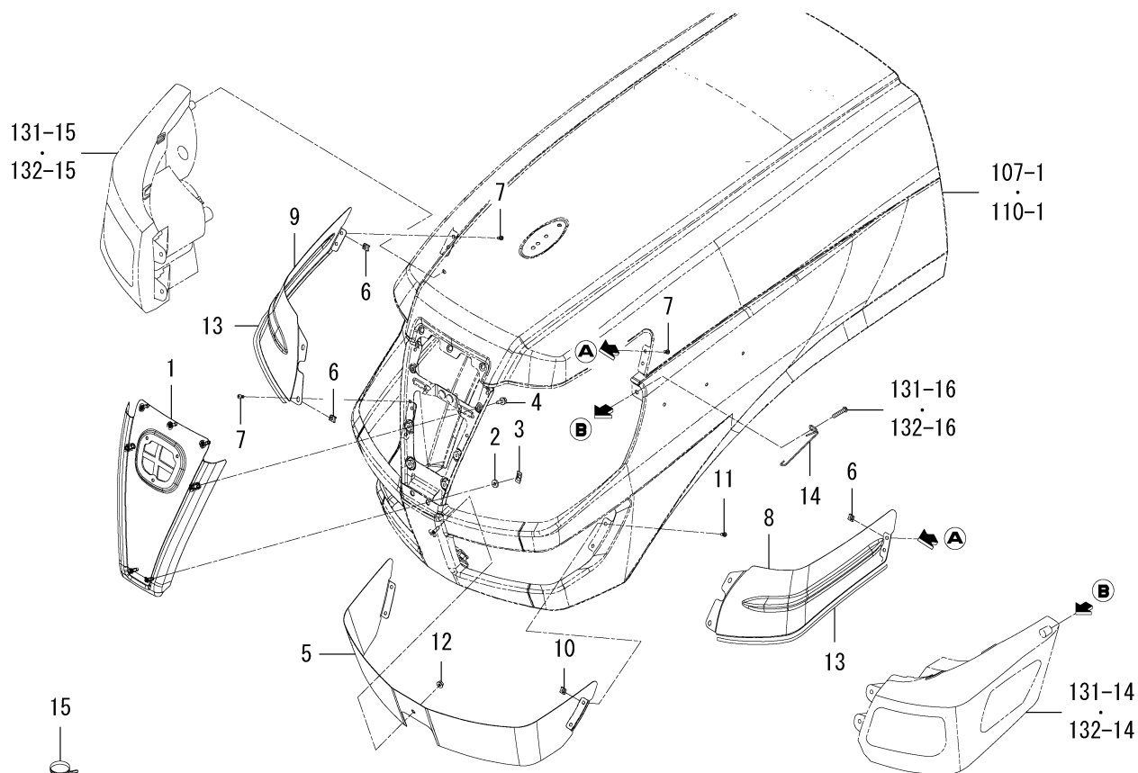
FIG.111 GRILLE SYSTEM
