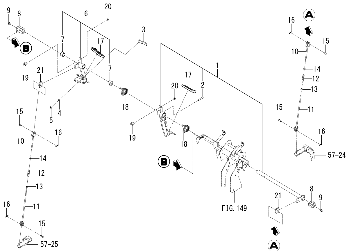
FIG. 61 PEDAL(BRAKE)SYSTEM(6370-CY TYPE)
