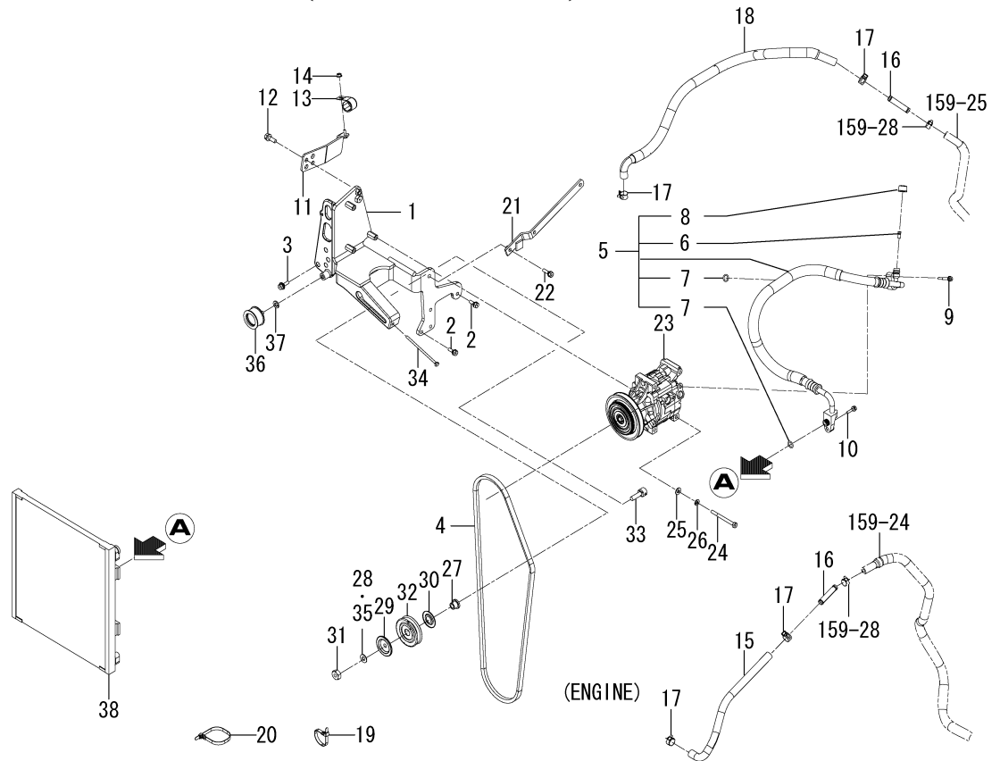
FIG.157 AIR CONDITIONER(ENGINE)SYSTEM(1/2) (6490-CY TYPE)
