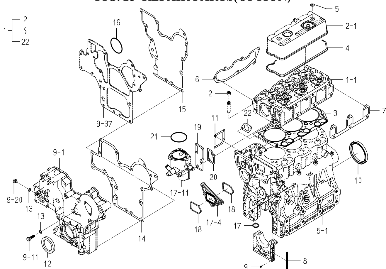
FIG. 25 REPAIR PARTS(OPTION)
