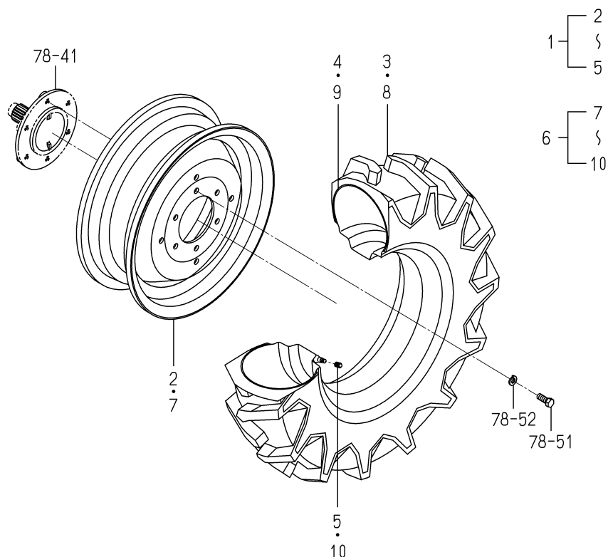
FIG.181 WHEEL(FRONT/AGR/7-16-4)ASSY (6370 TYPE)(OPTION)
