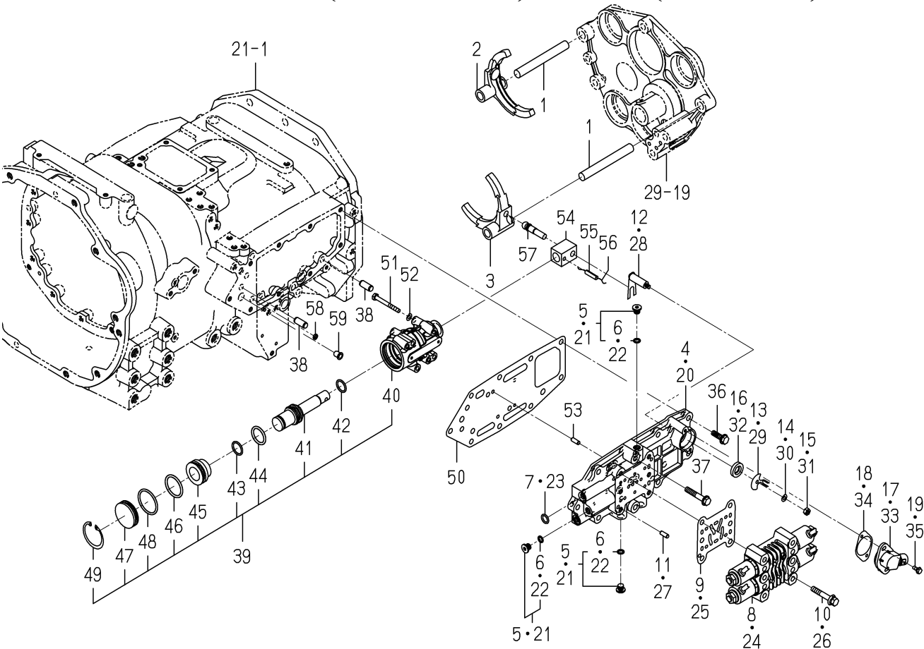
FIG. 39 FORK(SHIFT/MAIN)SYSTEM(6370 TYPE)
