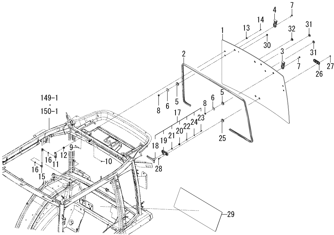
FIG.155 GLASS(REAR)SYSTEM(CY TYPE)
