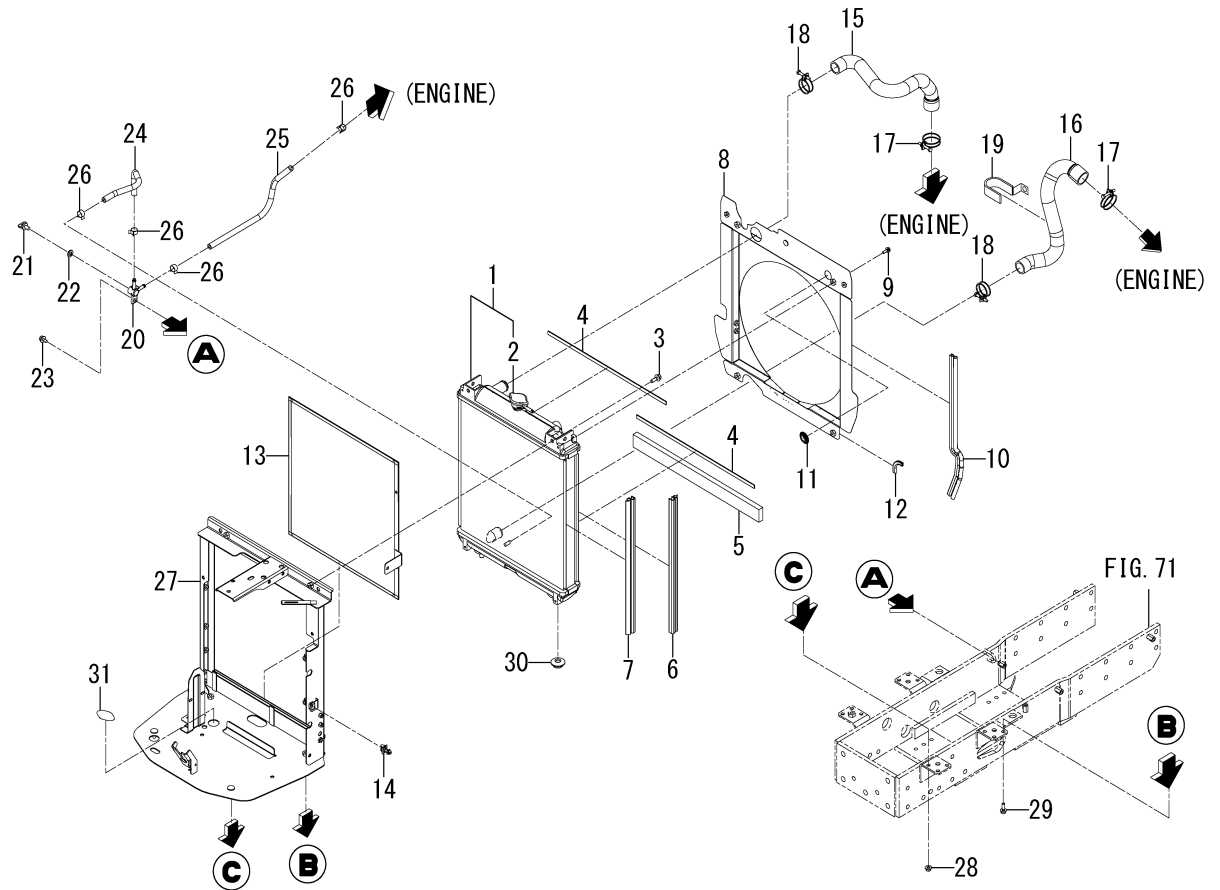
FIG. 1 RADIATOR SYSTEM(6370-CY TYPE)(1/2)
