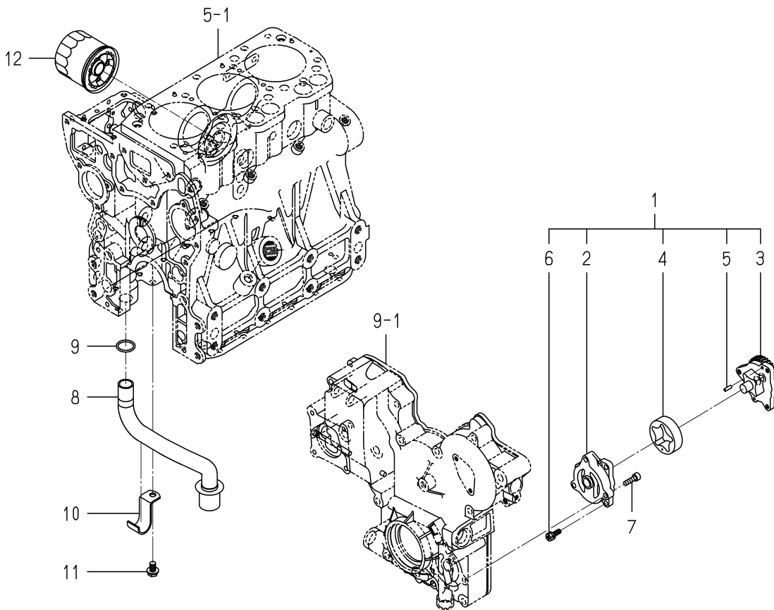
FIG. 16 OIL PUMP
