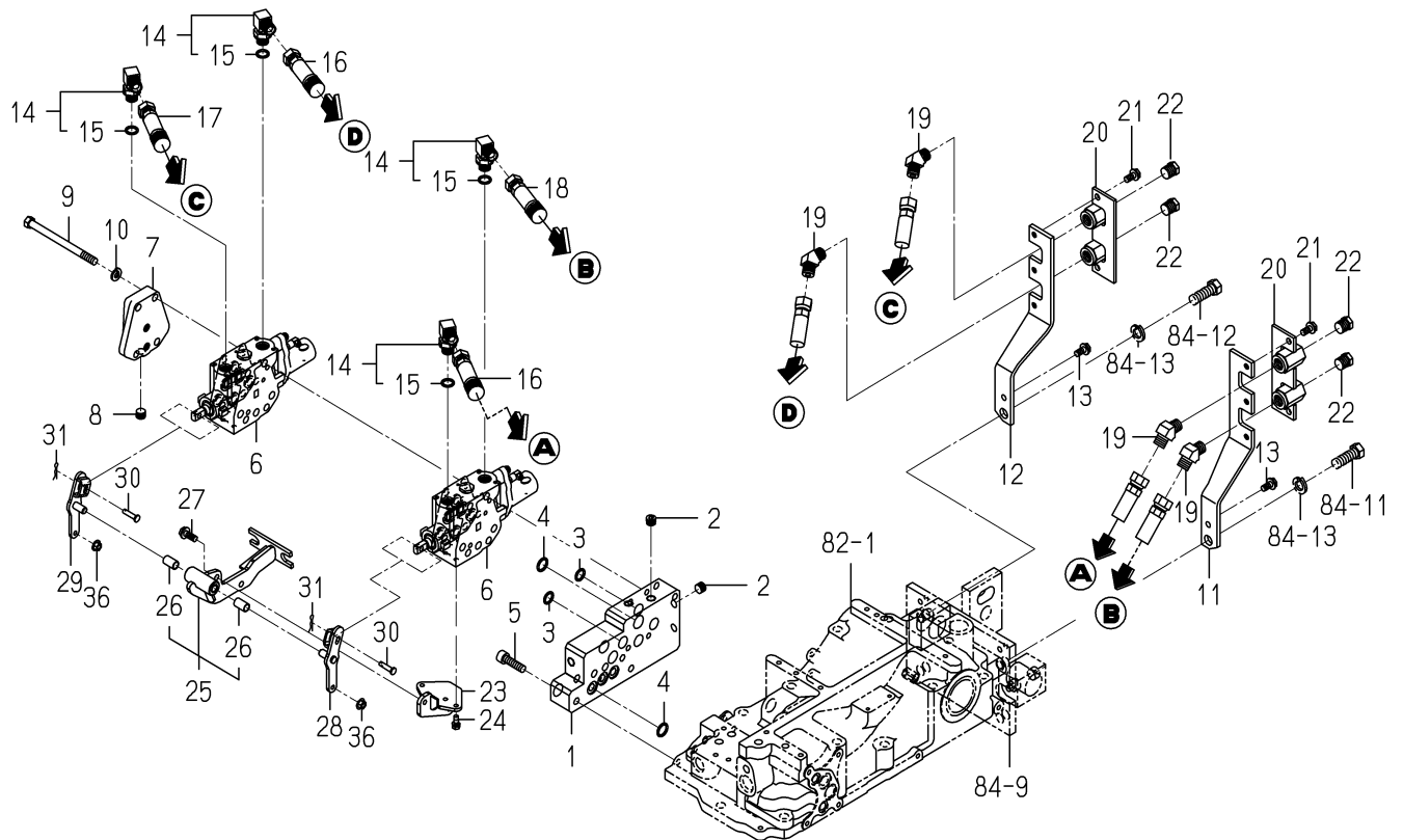
FIG. 96 VALVE(REMOTE/2)SET(6370 TYPE)(1/2)
