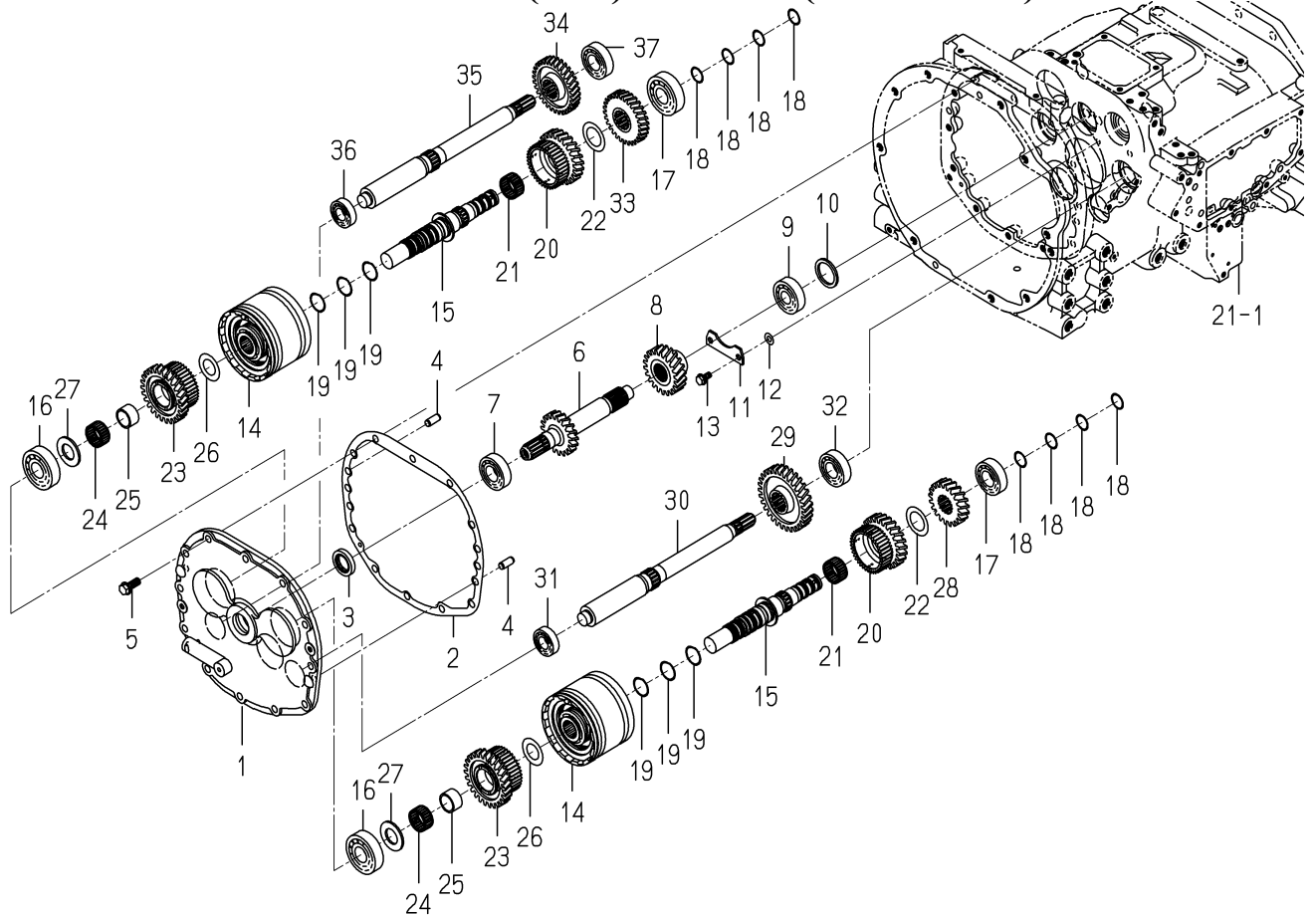
FIG. 23 GEAR(H/L)SYSTEM(6370 TYPE)
