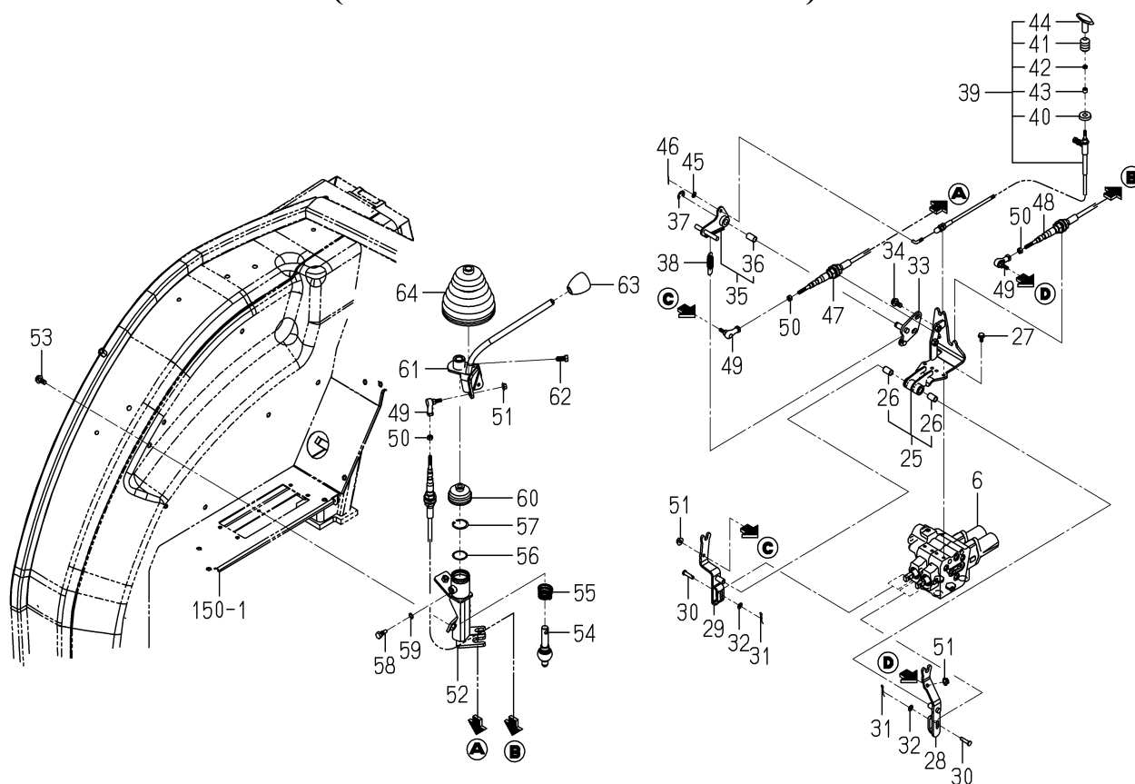
FIG. 90 JOY STICK VALVE SYSTEM(2/2) (6490-CY TYPE EXCEPT D)
