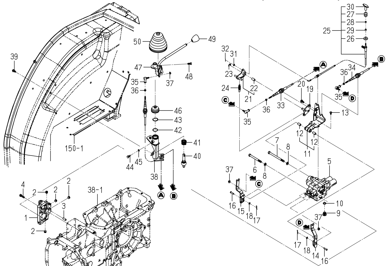
FIG. 91 JOY STICK VALVE SYSTEM(6490-D TYPE)
