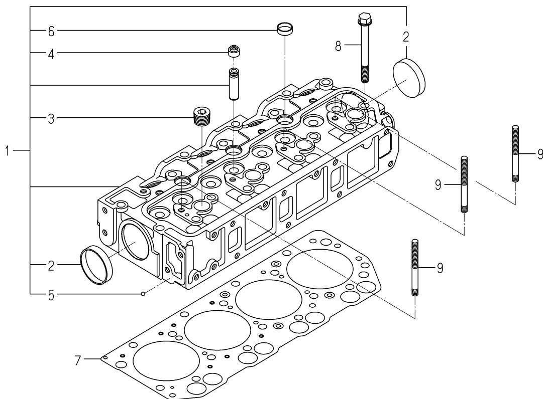
FIG. 1 CYLINDER HEAD
