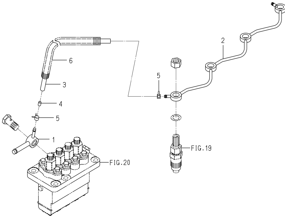
FIG. 21 FUEL PIPE
