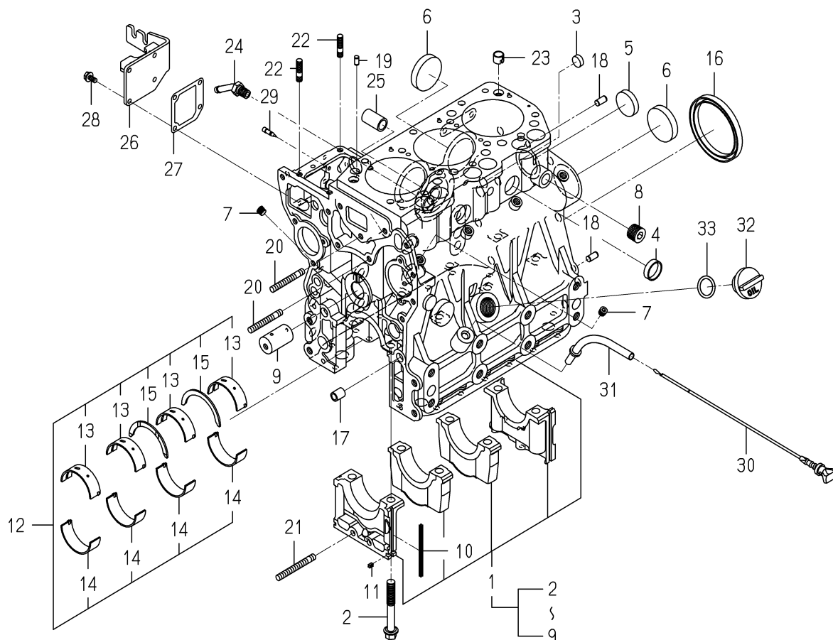
FIG. 5 CYLINDER BLOCK
