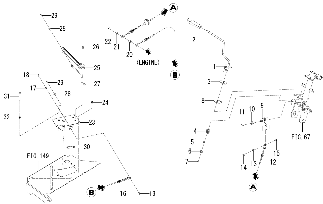
FIG. 17 ACCELERATOR SYSTEM(6370-CY TYPE)
