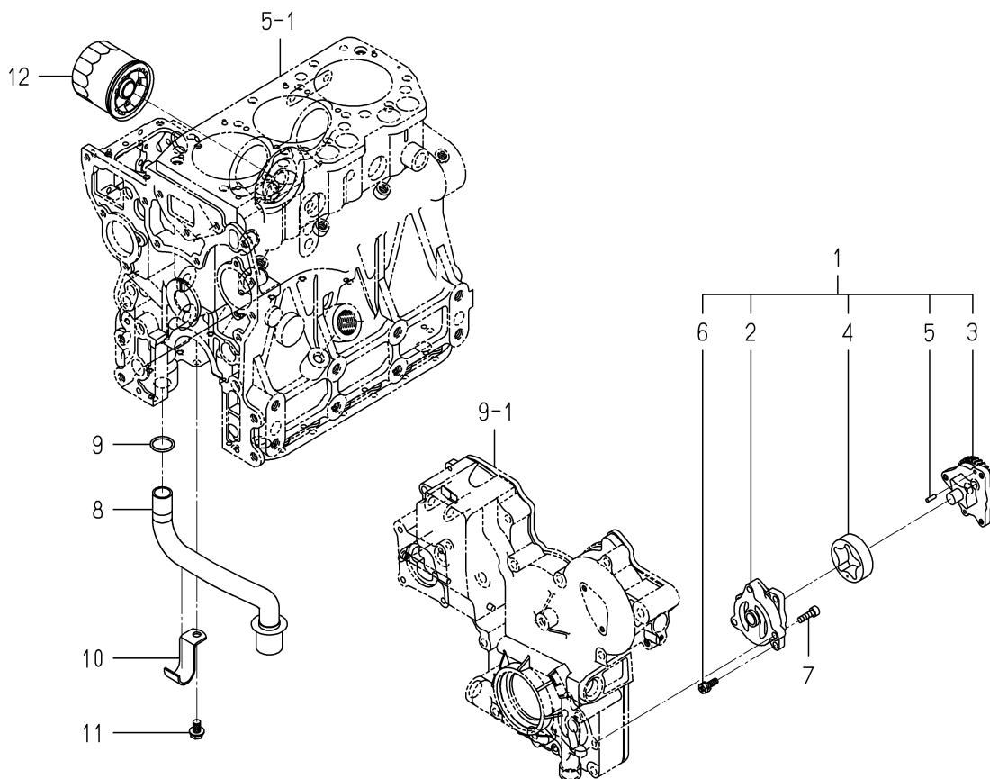
FIG. 16 OIL PUMP
