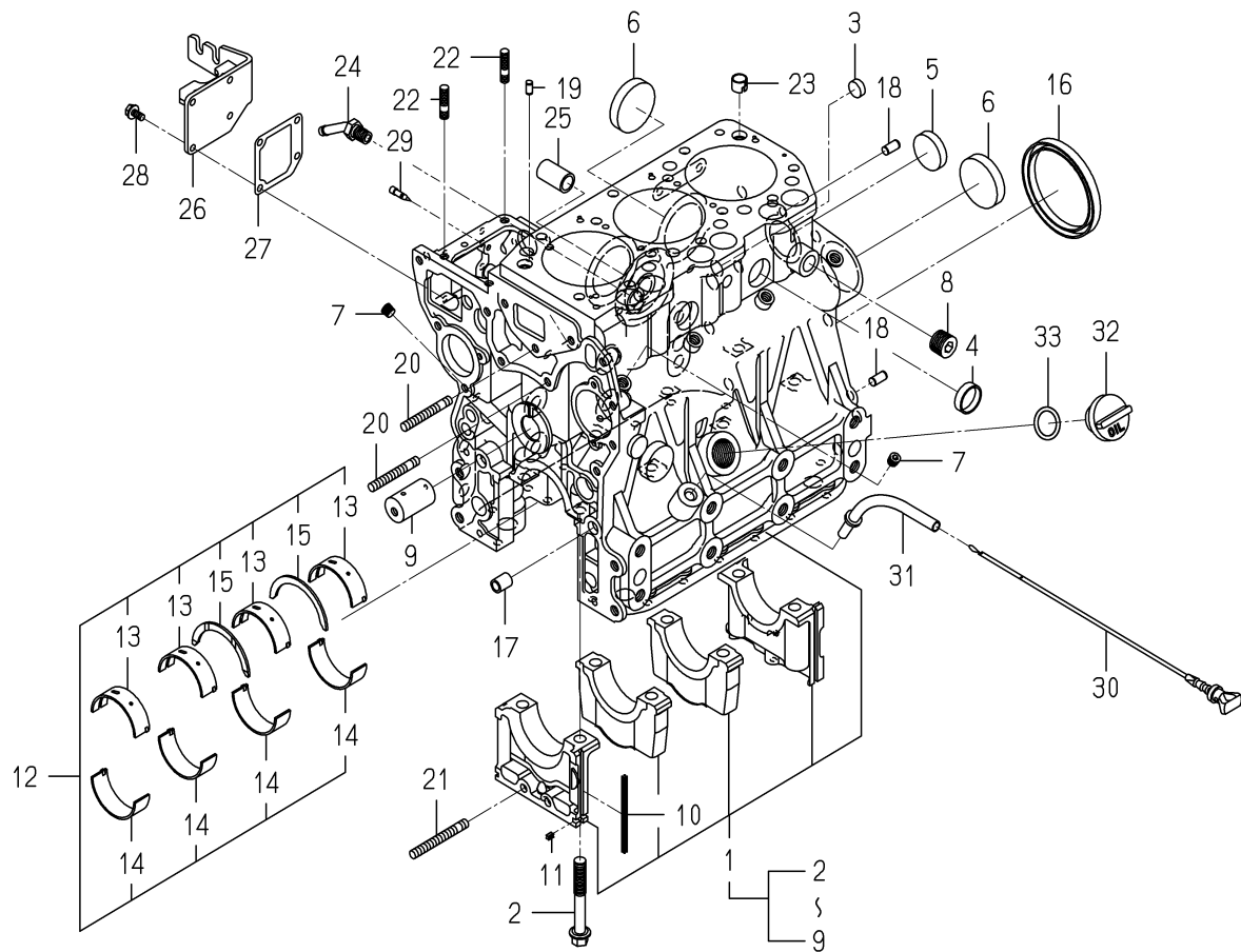
FIG. 5 CYLINDER BLOCK
