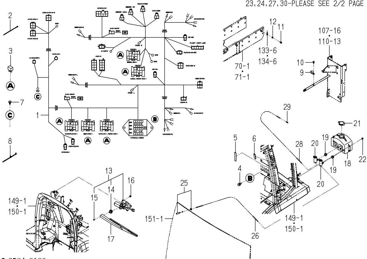
FIG.140 ELC.(CABIN)SYSTEM(CY TYPE)(1/2)
