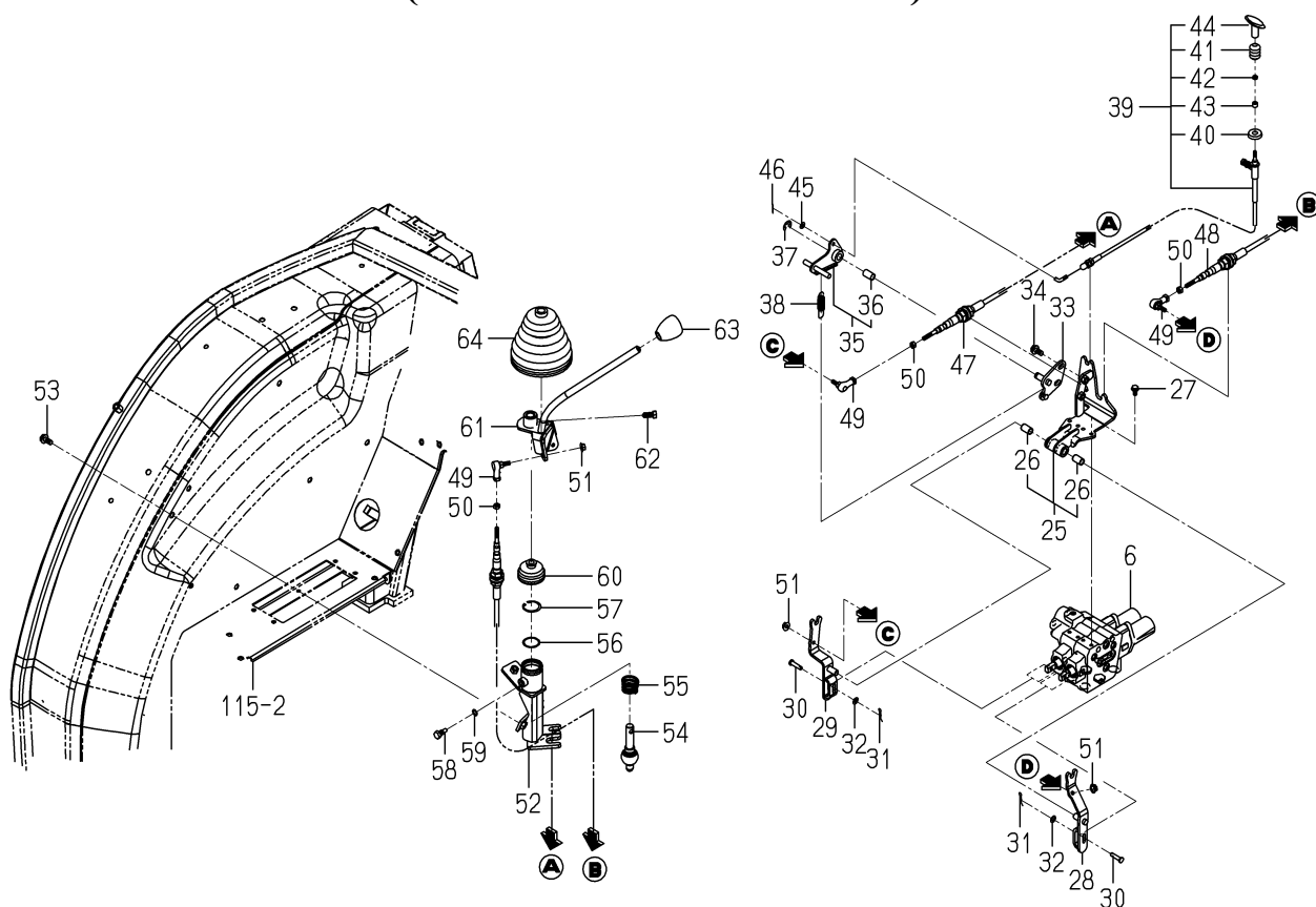
FIG. 92 JOY STICK VALVE SYSTEM(2/2) (6490-EXCEPT CY TYPE)
