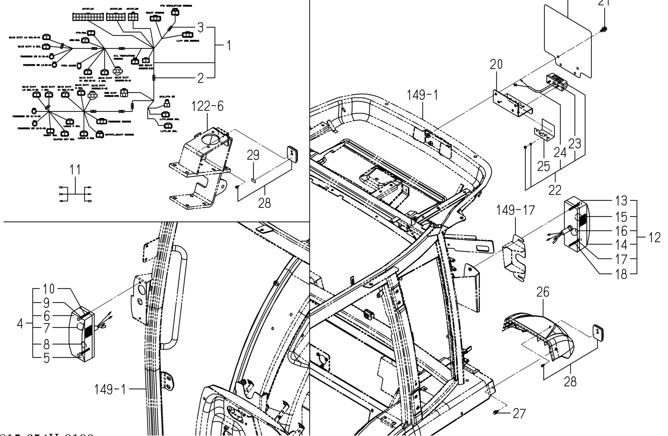
FIG.138 ELC.(FLOOR)SYSTEM(6370 TYPE)(1/2)
