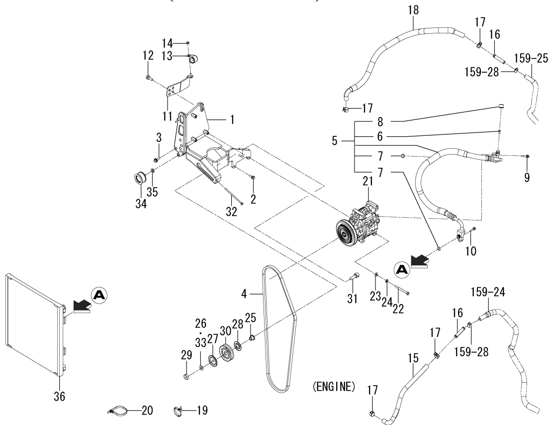
FIG.158 AIR CONDITIONER(ENGINE)SYSTEM(1/2) (6370-CY TYPE)
