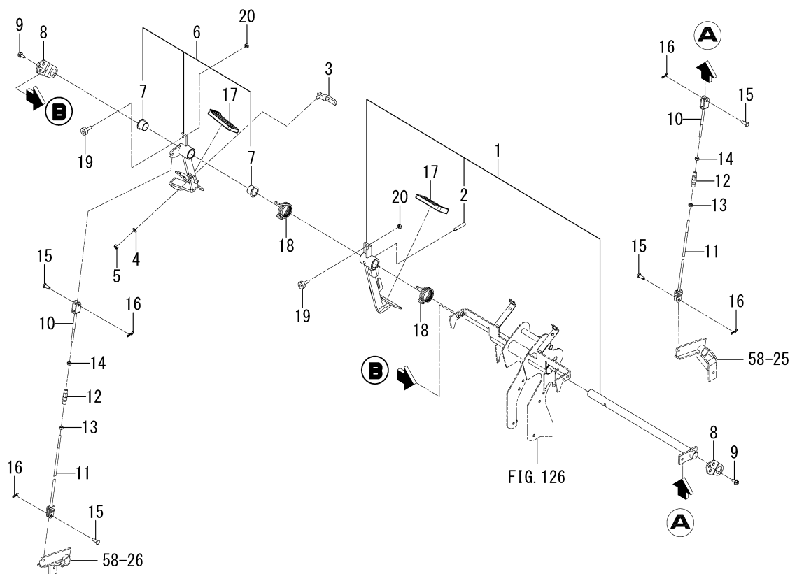
FIG. 60 PEDAL(BRAKE)SYSTEM (6490-EXCEPT CY TYPE)
