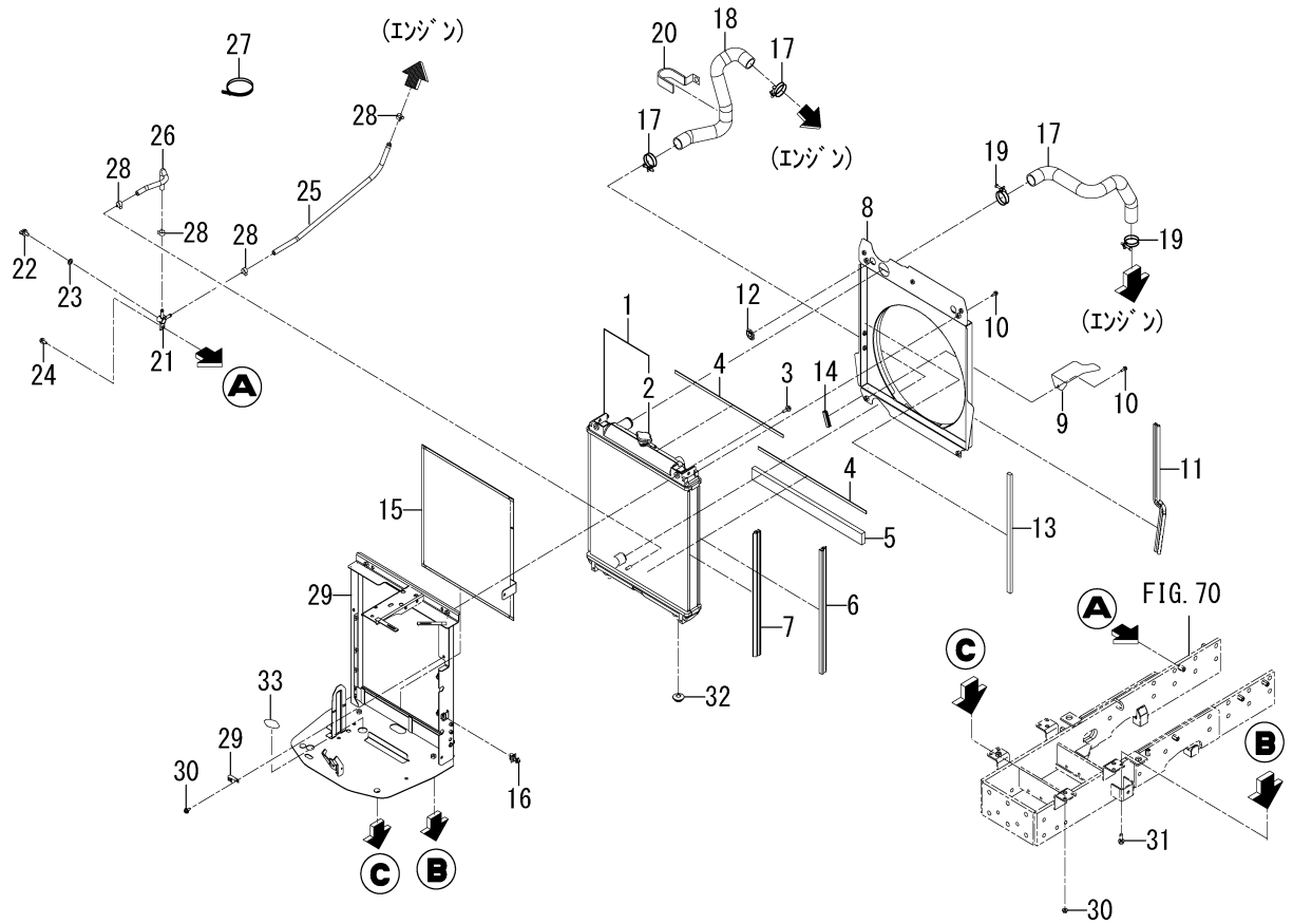
FIG. 3 RADIATOR SYSTEM(6490-CY TYPE)(1/2)
