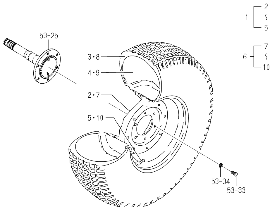
FIG.174 WHEEL(REAR/TURF/20XW11)ASSY (6370 TYPE)(OPTION)
