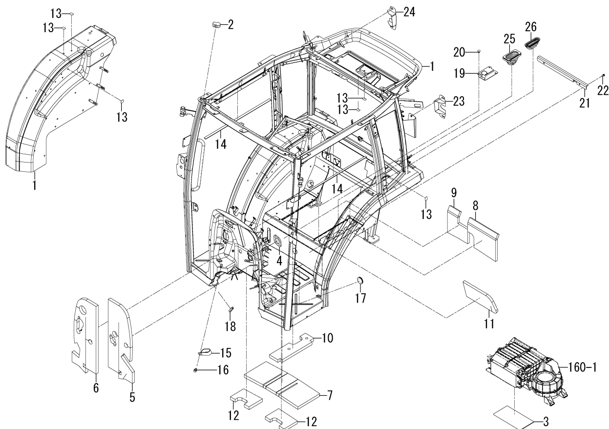
FIG.150 FLAME SYSTEM(6490-CY TYPE)
