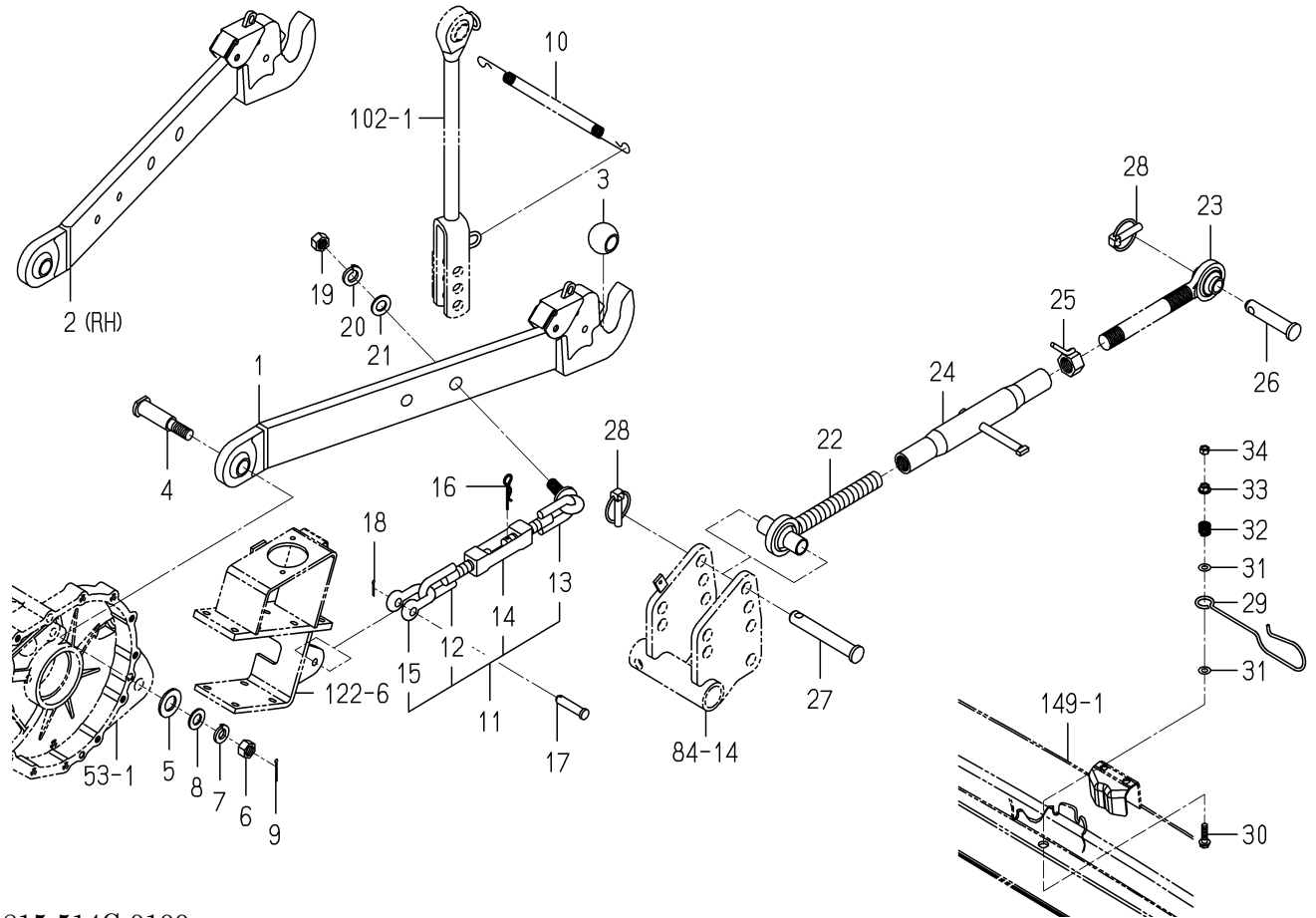
FIG.100 LINK(3P)SYSTEM(6370-CY TYPE)
