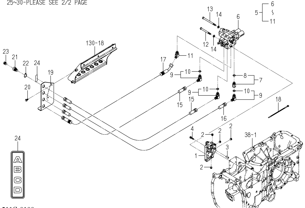
FIG. 93 JOY STICK VALVE SYSTEM(1/2) (6370-CY TYPE EXCEPT D)
