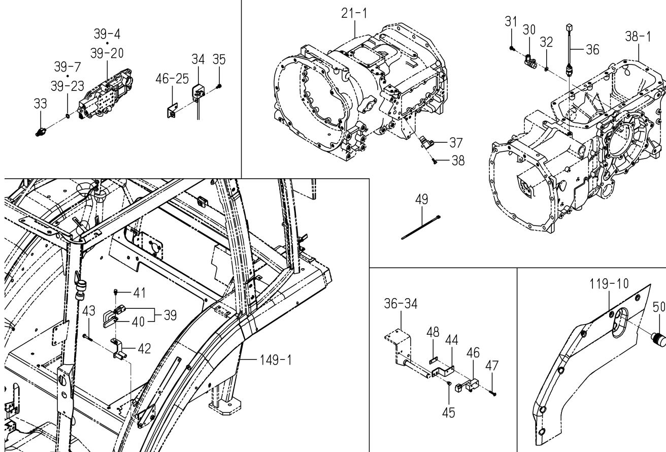
FIG.138 ELC.(FLOOR)SYSTEM(6370 TYPE)(2/2)
