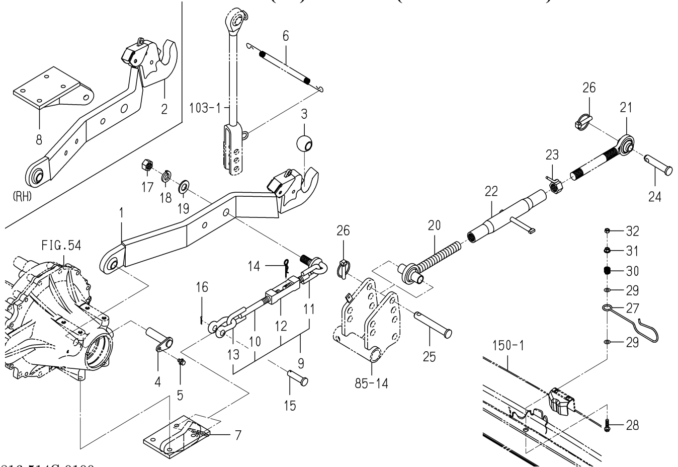
FIG.101 LINK(3P)SYSTEM(6490-CY TYPE)
