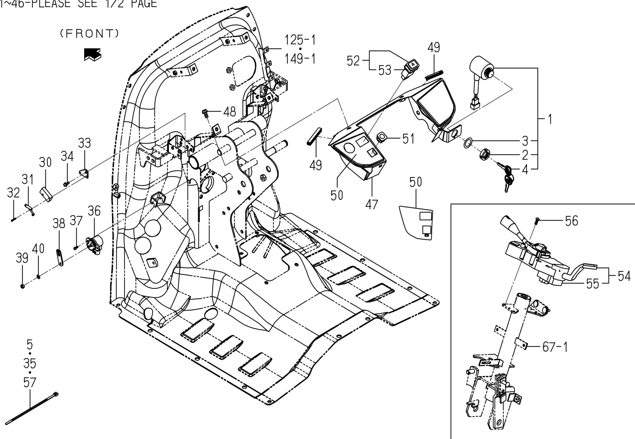
FIG.133 ELC.(MAIN)SYSTEM(6370 TYPE)(2/2)
