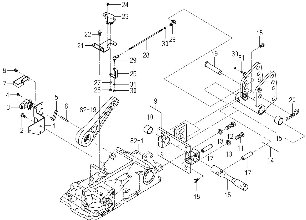
FIG. 84 CONTROL(POSITION&DRAFT)SYSTEM (6370 TYPE)
