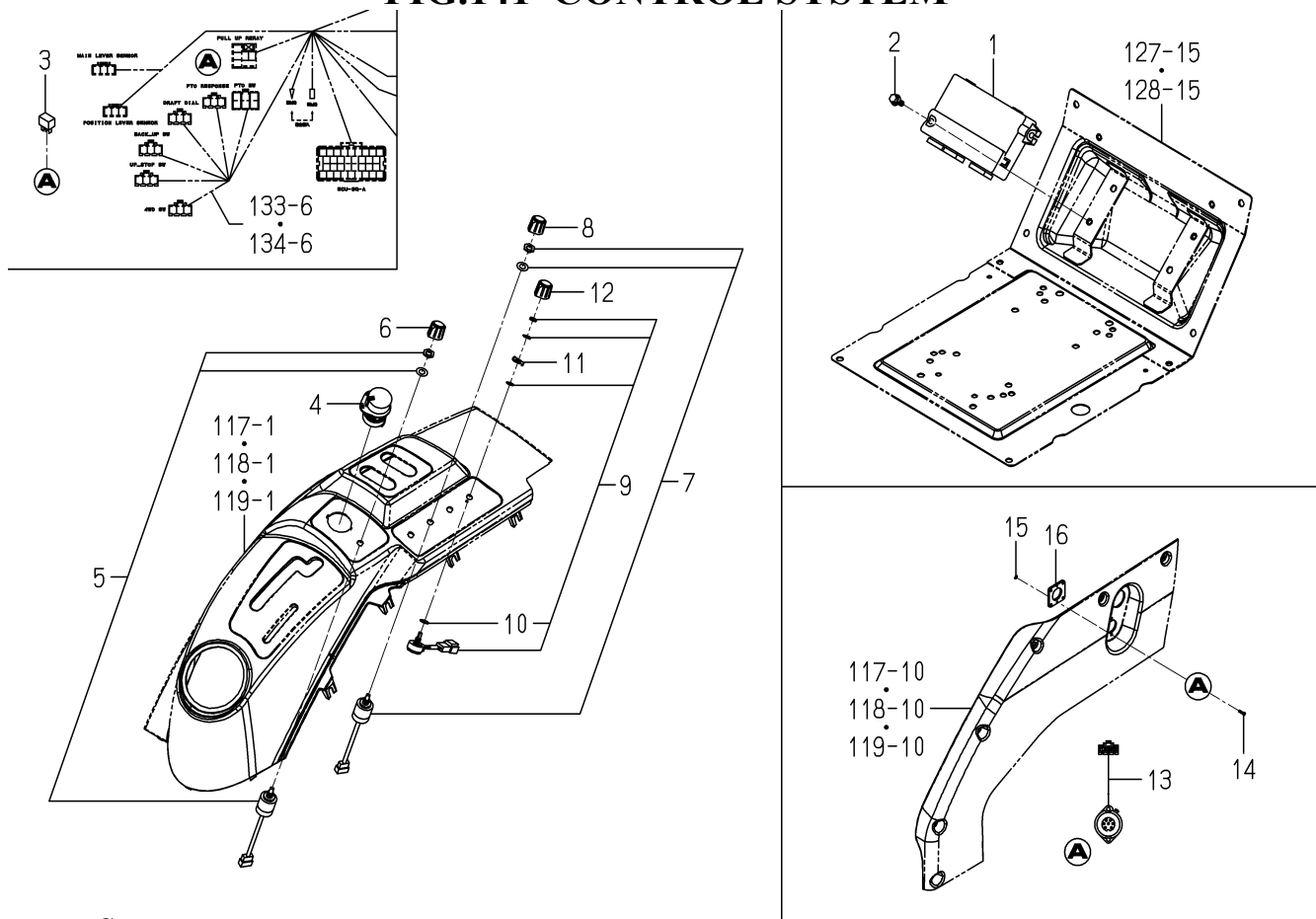
FIG.141 CONTROL SYSTEM
