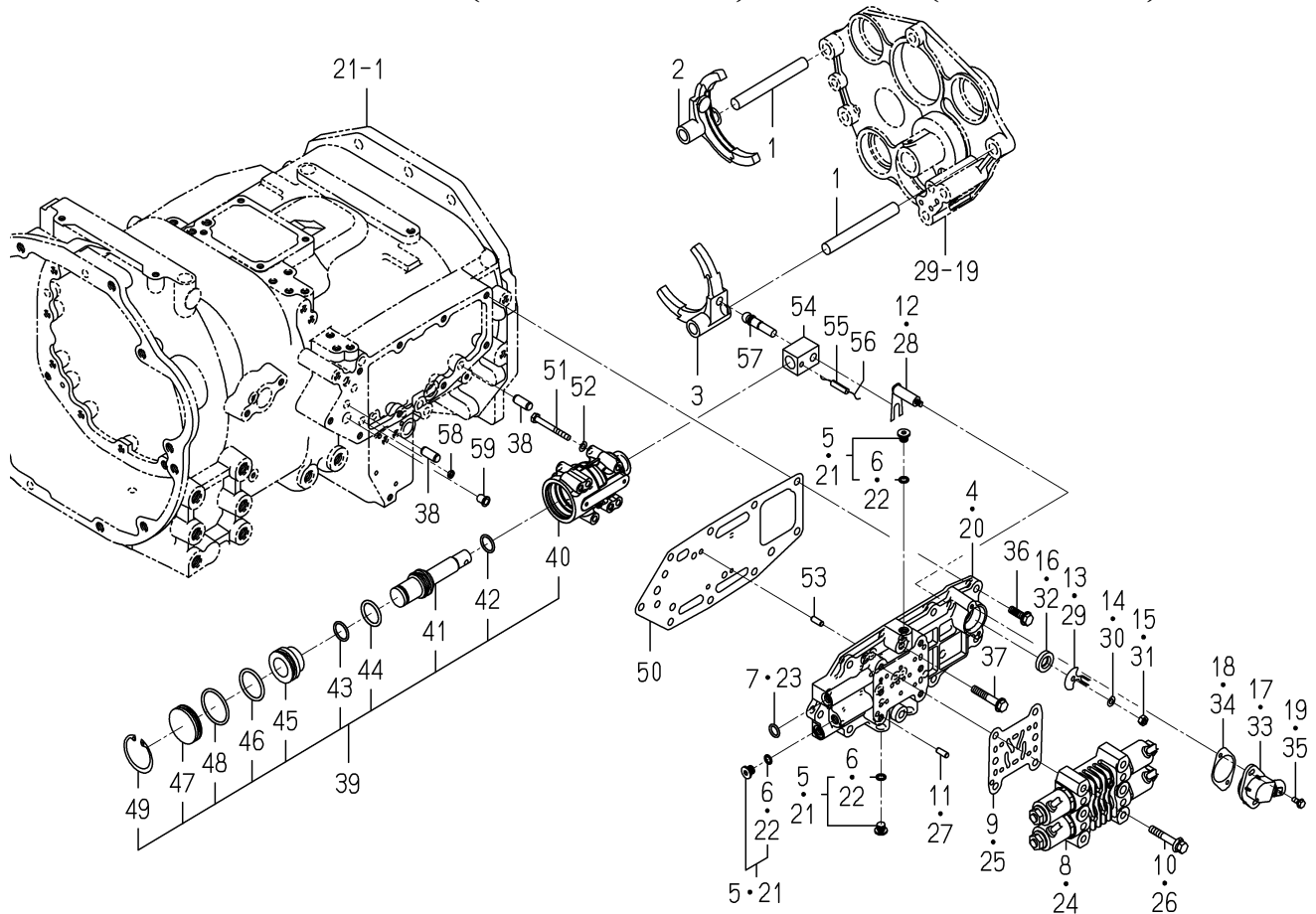
FIG. 39 FORK(SHIFT/MAIN)SYSTEM(6370 TYPE)
