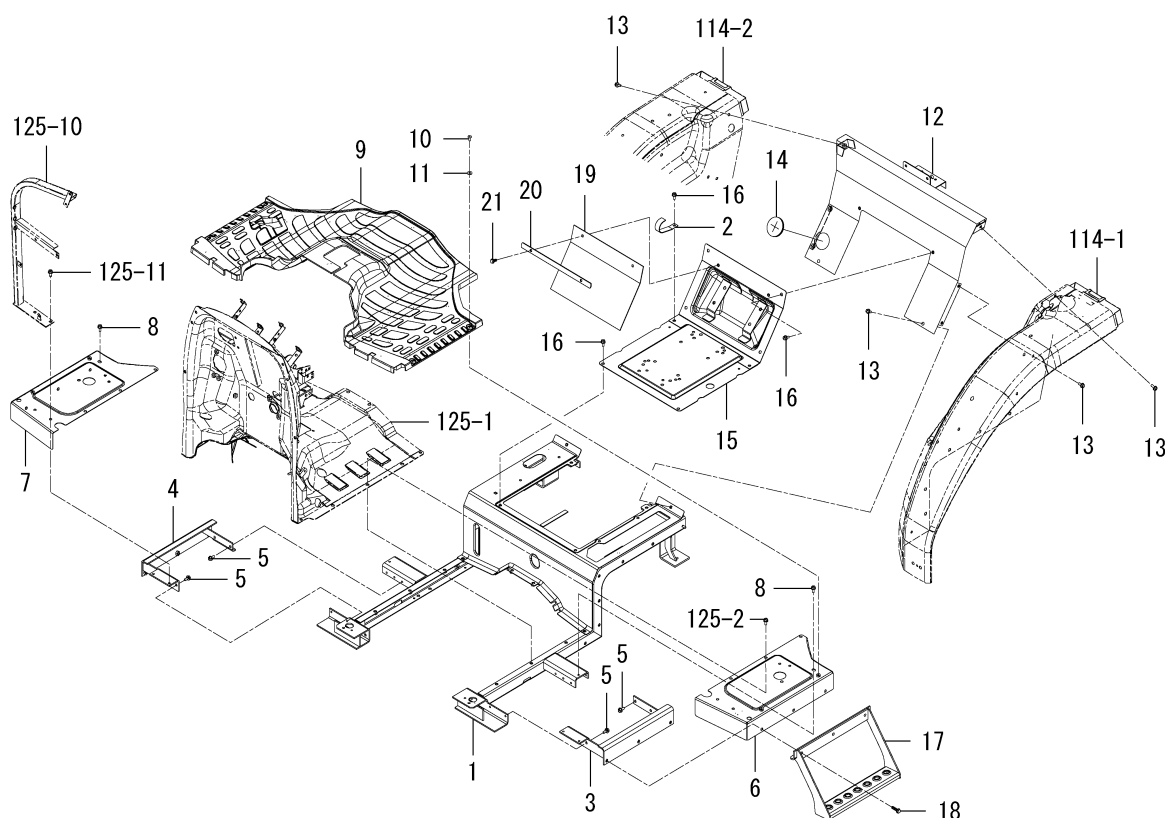
FIG.127 FLOOR(REAR)SYSTEM (6370-EXCEPT CY TYPE)
