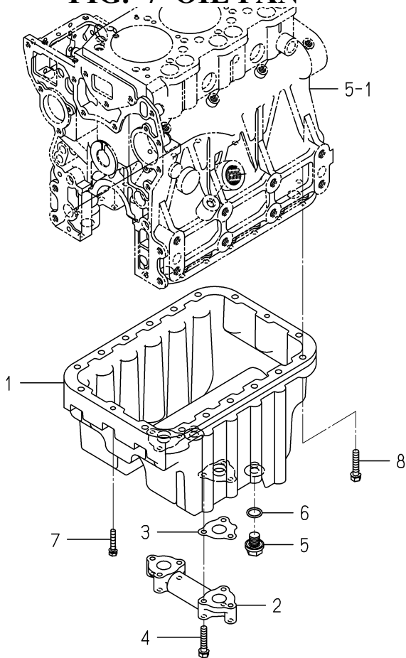
FIG. 7 OIL PAN
