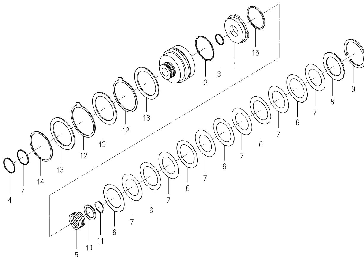
FIG.206 COMPONENT PARTS FOR 1796-209-300-00 ON FIG.26
