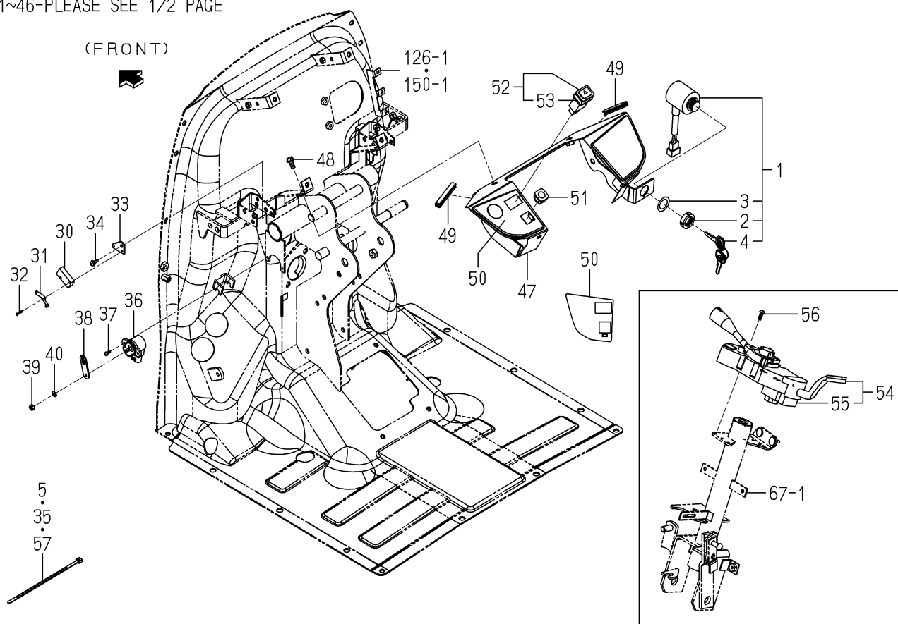
FIG.134 ELC.(MAIN)SYSTEM(6490 TYPE)(2/2)
