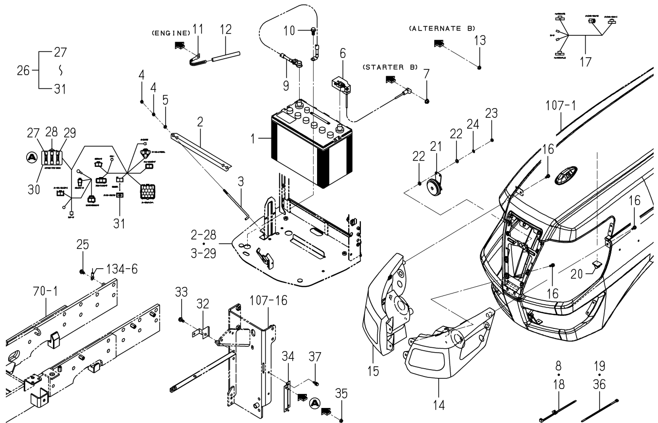
FIG.132 ELC.(FRONT)SYSTEM(6490 TYPE)
