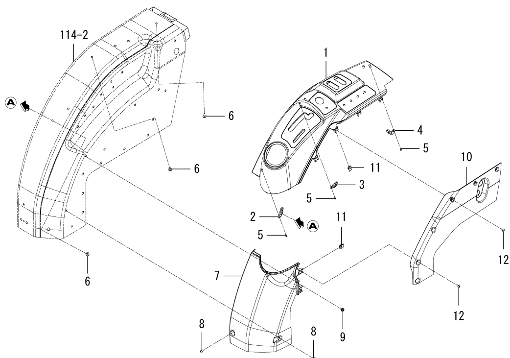
FIG.118 GUIDE(LEVER)SYSTEM (6370-EXCEPT CY TYPE)
