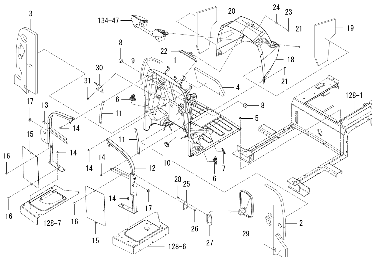
FIG.126 PANEL(DASH)SYSTEM (6490-EXCEPT CY TYPE)
