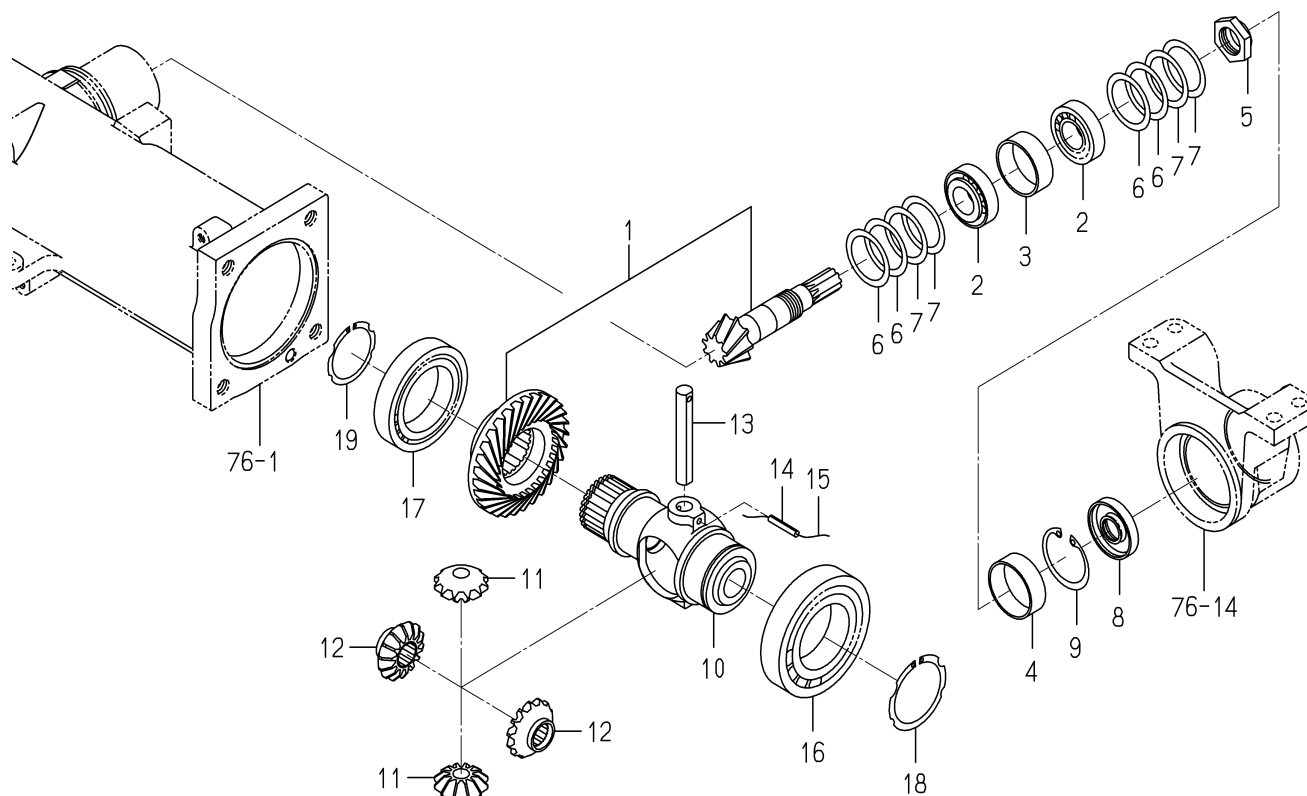
FIG. 74 CASE(BEVEL)SYSTEM(6370 TYPE)
