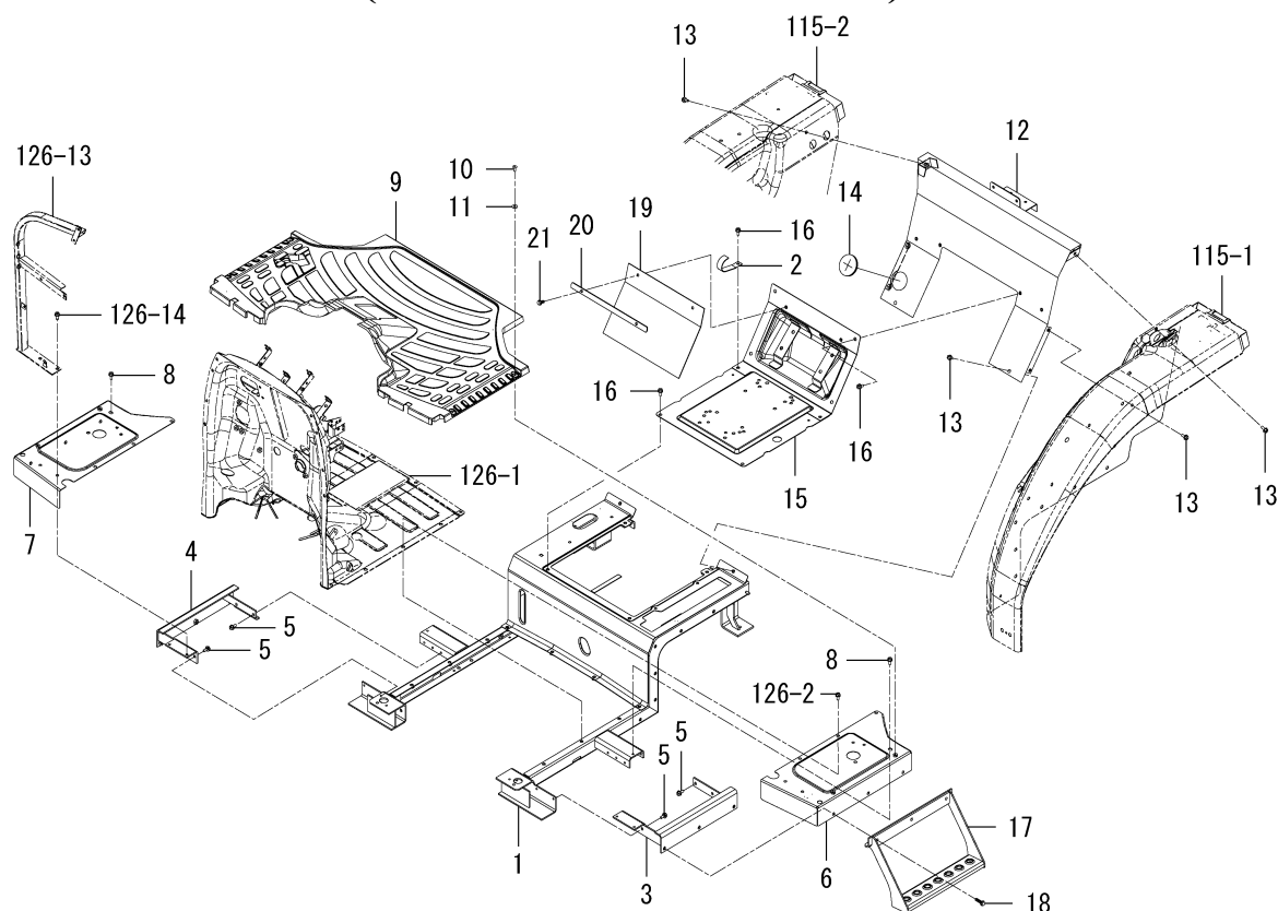
FIG.128 FLOOR(REAR)SYSTEM (6490-EXCEPT CY TYPE)
