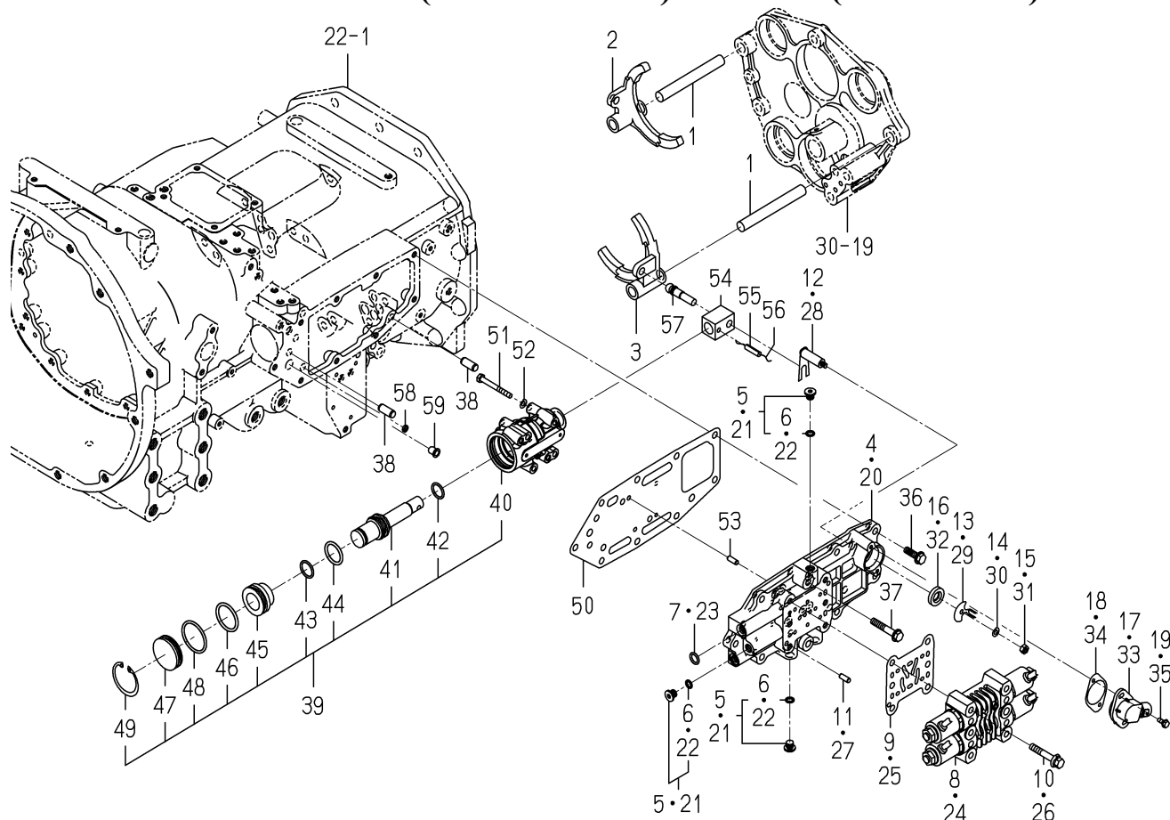
FIG. 40 FORK(SHIFT/MAIN)SYSTEM(6490 TYPE)
