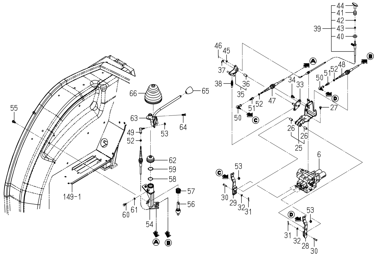
FIG. 93 JOY STICK VALVE SYSTEM(2/2) (6370-CY TYPE EXCEPT D)
