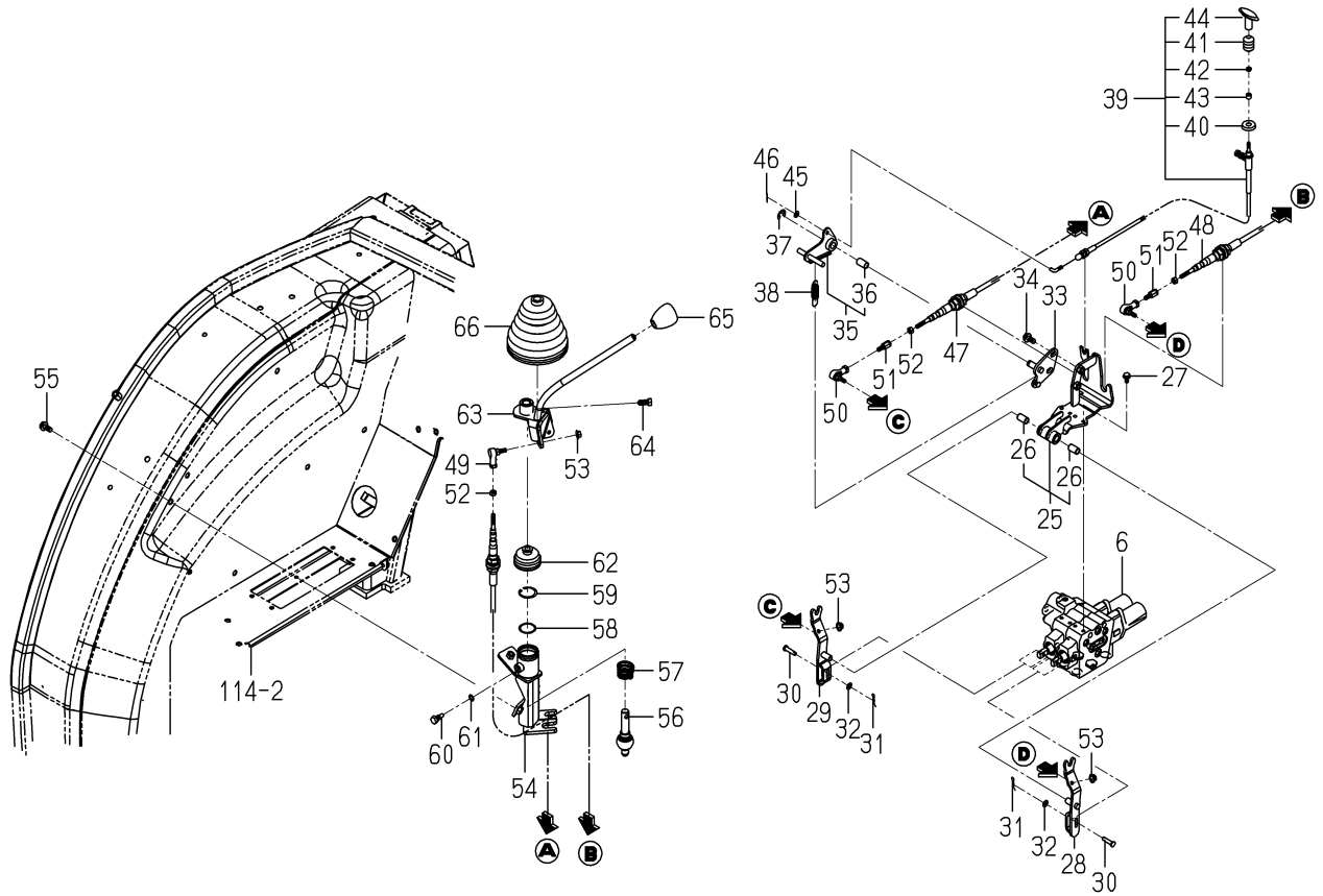
FIG. 94 JOY STICK VALVE SYSTEM(2/2) (6370-EXCEPT CY TYPE)
