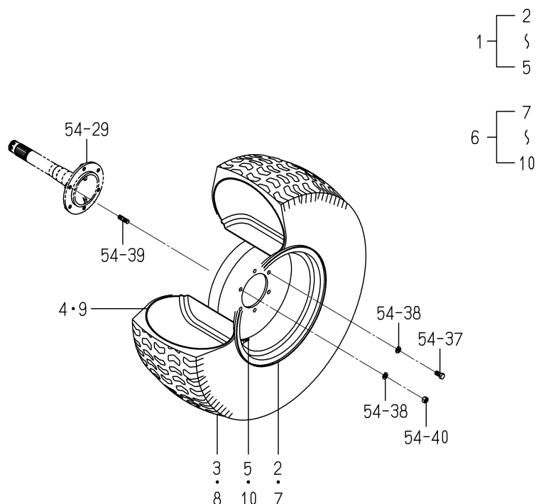
FIG.176 WHEEL(REAR/TURF/475/65D-20)ASSY (6490 TYPE)(OPTION)
