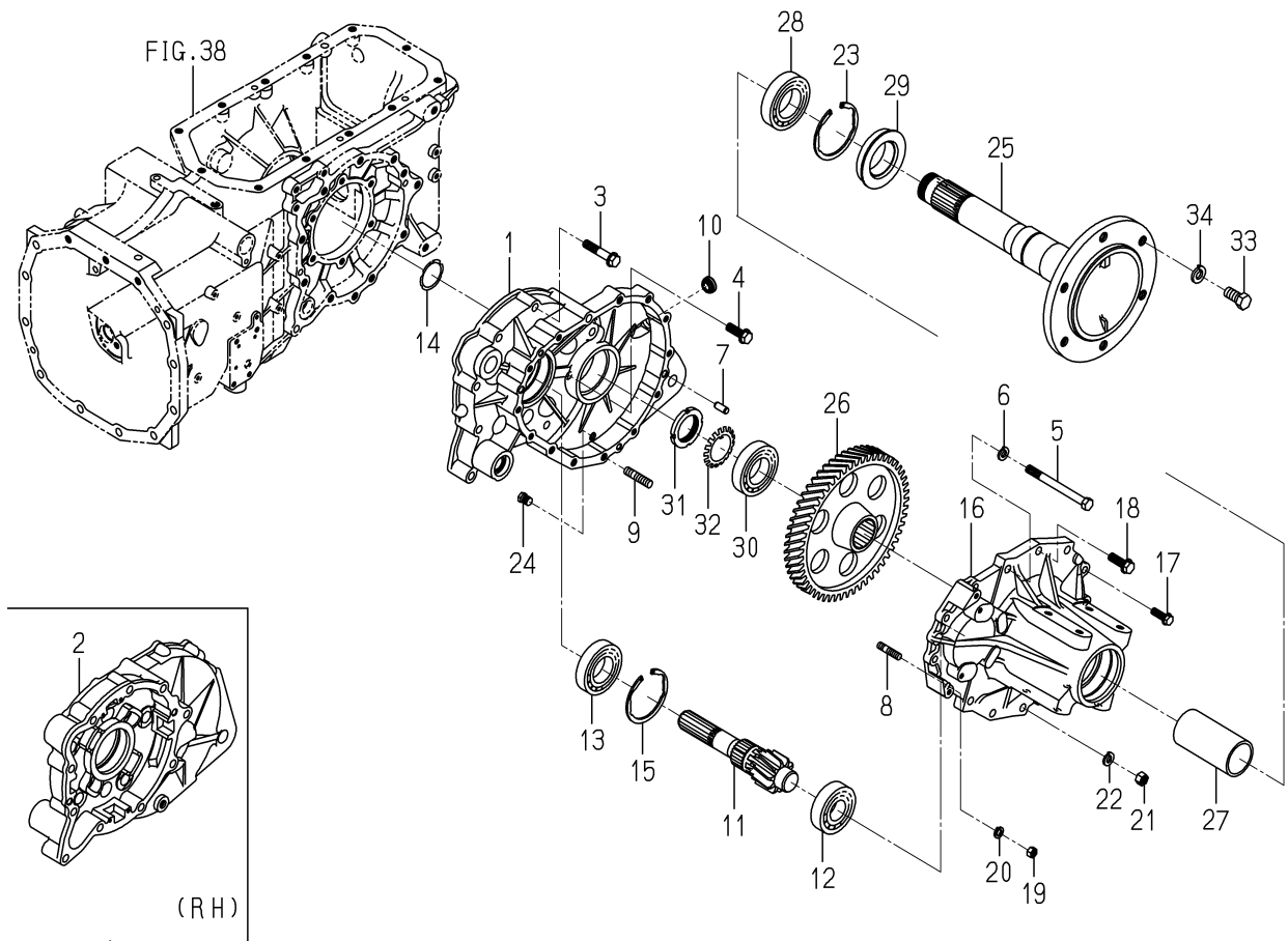
FIG. 53 HOUSING(AXLE)SYSTEM(6370 TYPE)
