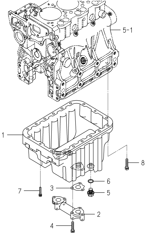
FIG. 7 OIL PAN
