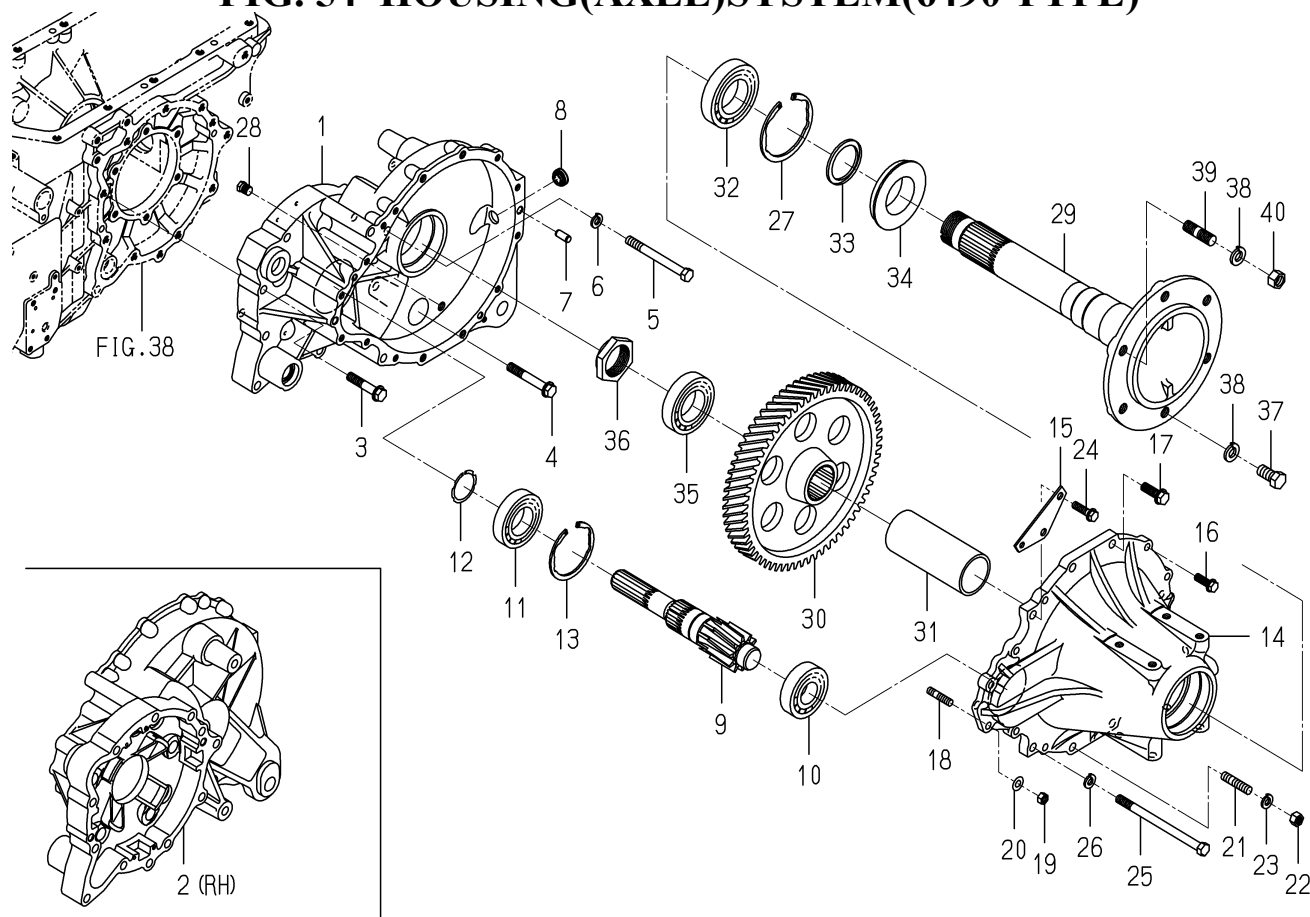
FIG. 54 HOUSING(AXLE)SYSTEM(6490 TYPE)
