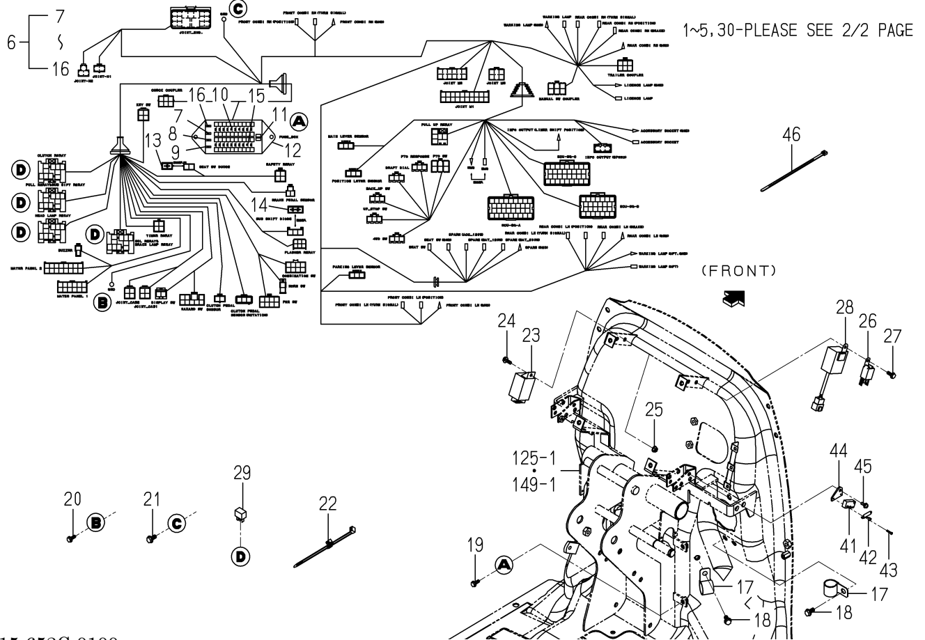
FIG.133 ELC.(MAIN)SYSTEM(6370 TYPE)(1/2)
