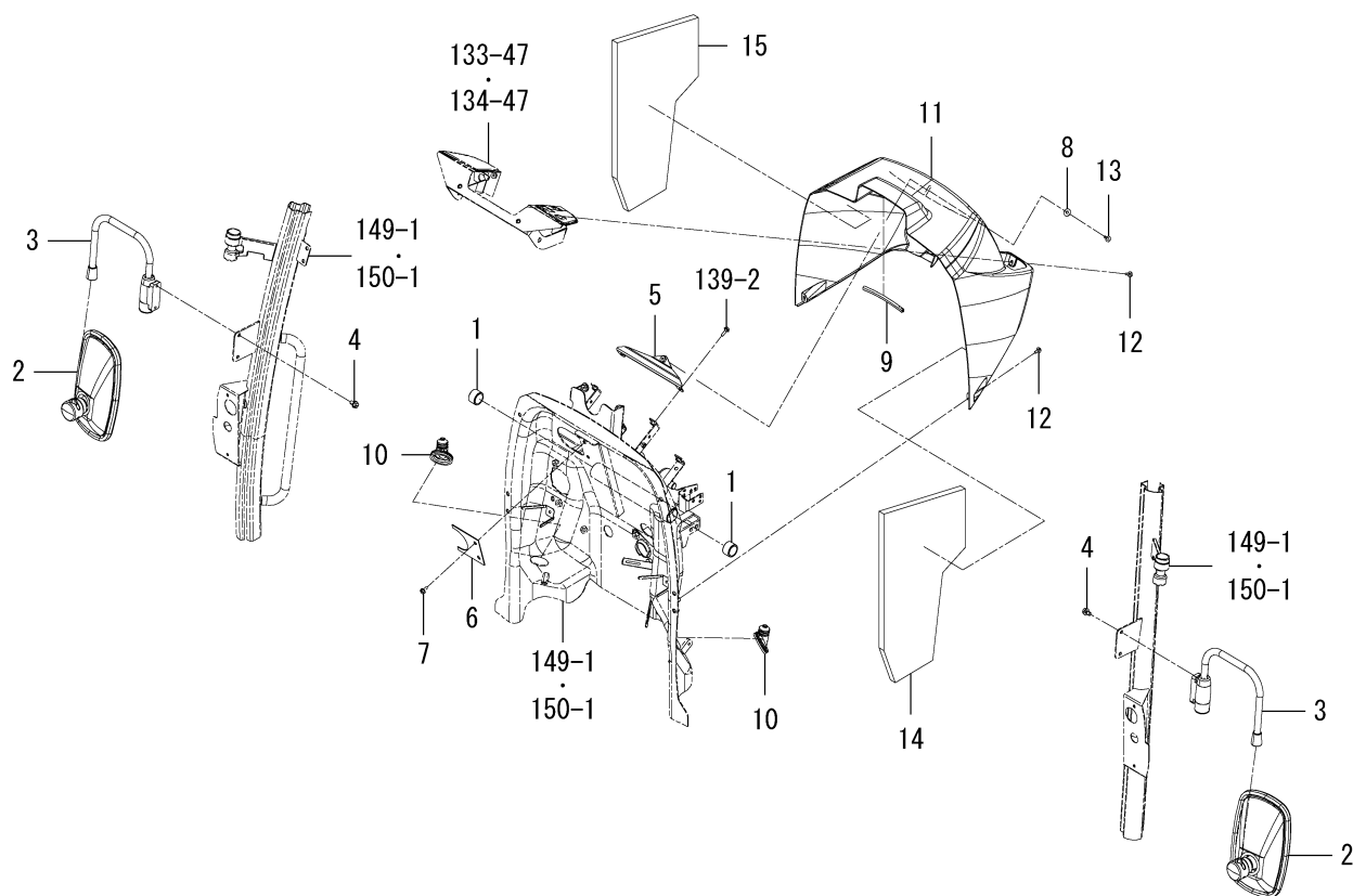
FIG.124 FLOOR(FRONT)SYSTEM(CY TYPE)
