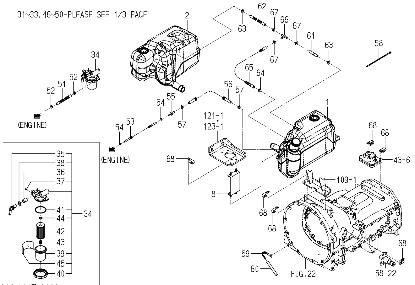
FIG. 12 TANK(FUEL)SYSTEM(6490 TYPE)(2/3)
