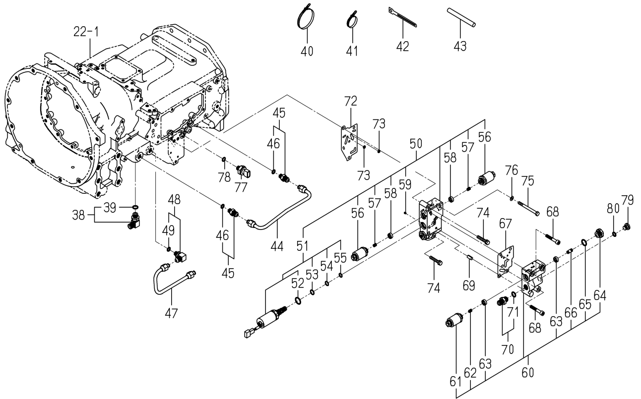
FIG. 89 PIPING(SUB)SYSTEM(6490 TYPE)(2/2)
