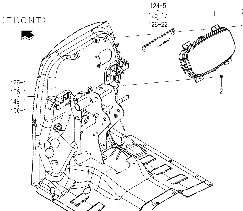
FIG.139 PANEL SYSTEM
