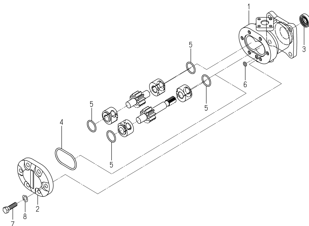
FIG.190 COMPONENT PARTS FOR K135-015-000-00 ON FIG.88,89
