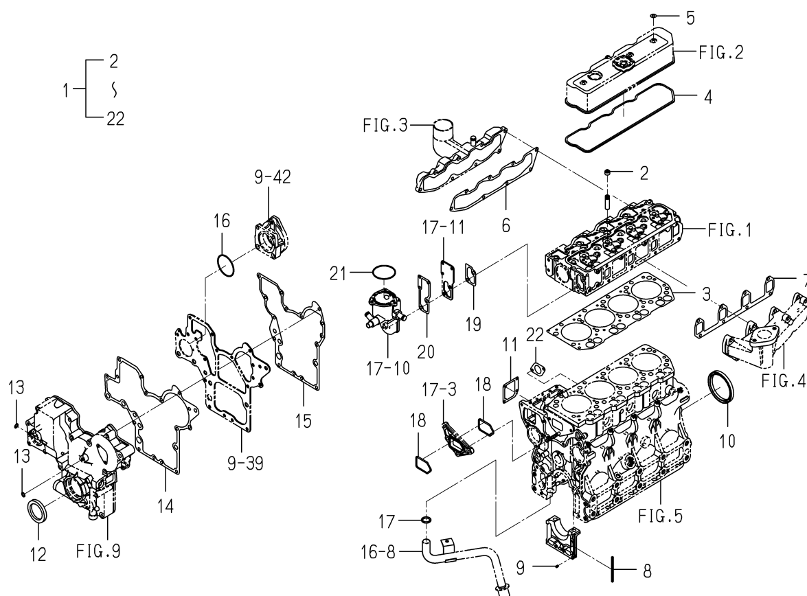
FIG. 25 REPAIR PARTS(OPTION)
