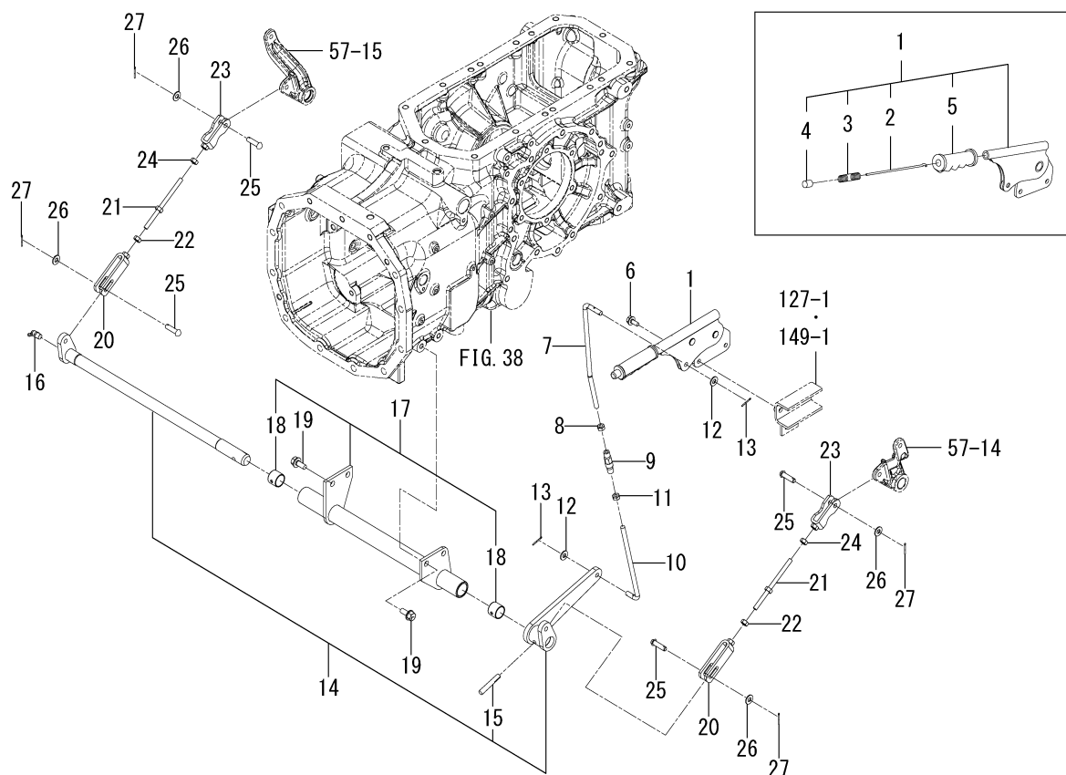
FIG. 63 LEVER(BRAKE/PARKING)SYSTEM (6370 TYPE)
