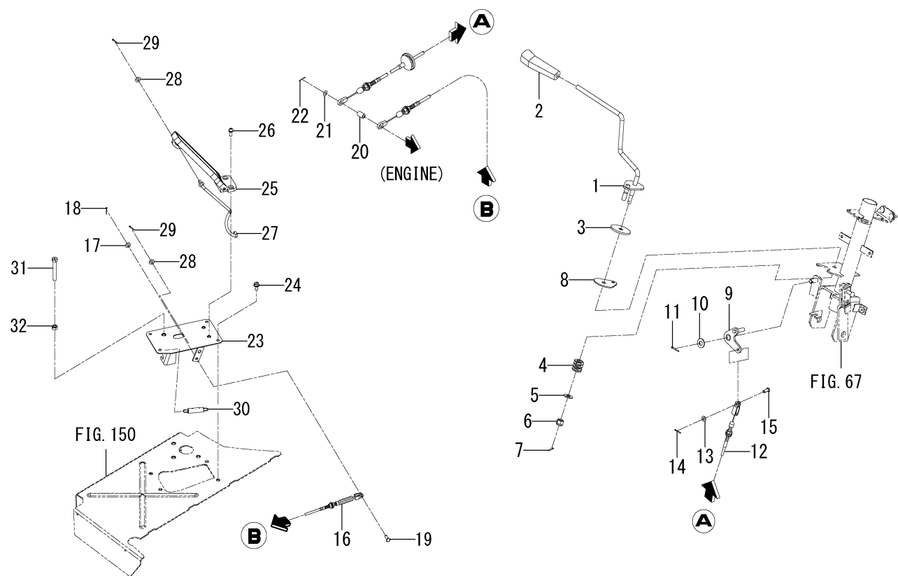
FIG. 16 ACCELERATOR SYSTEM(6490-CY TYPE)
