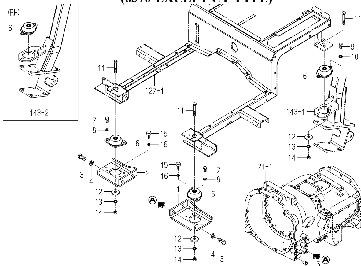
FIG.120 MOUNT(FRONT)SYSTEM (6370-EXCEPT CY TYPE)
