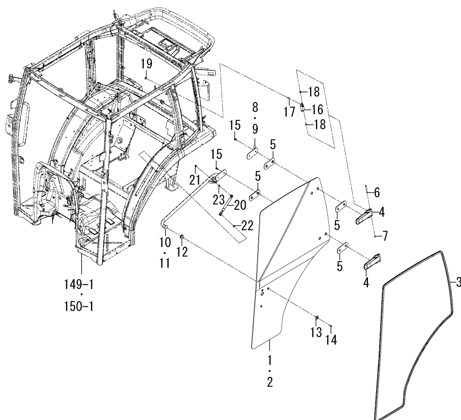
FIG.152 DOOR SYSTEM(CY TYPE)
