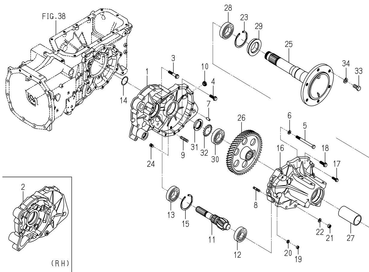
FIG. 53 HOUSING(AXLE)SYSTEM(6370 TYPE)
