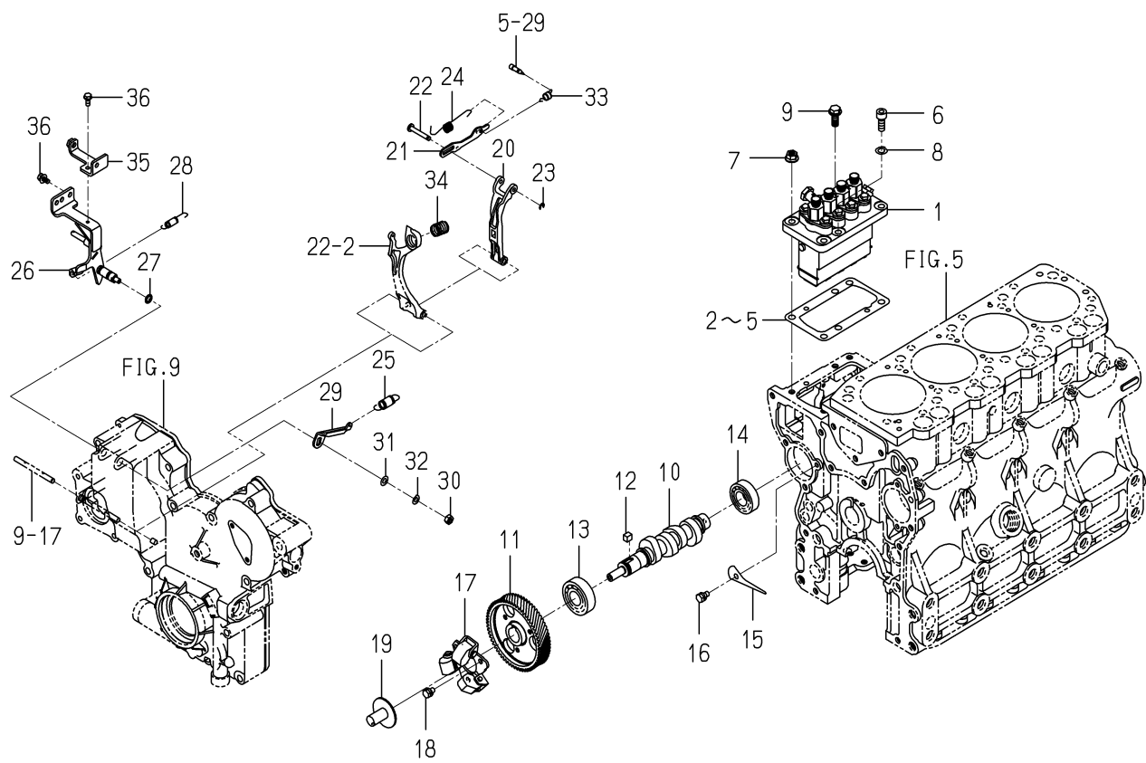
FIG. 20 INJECTION PUMP
