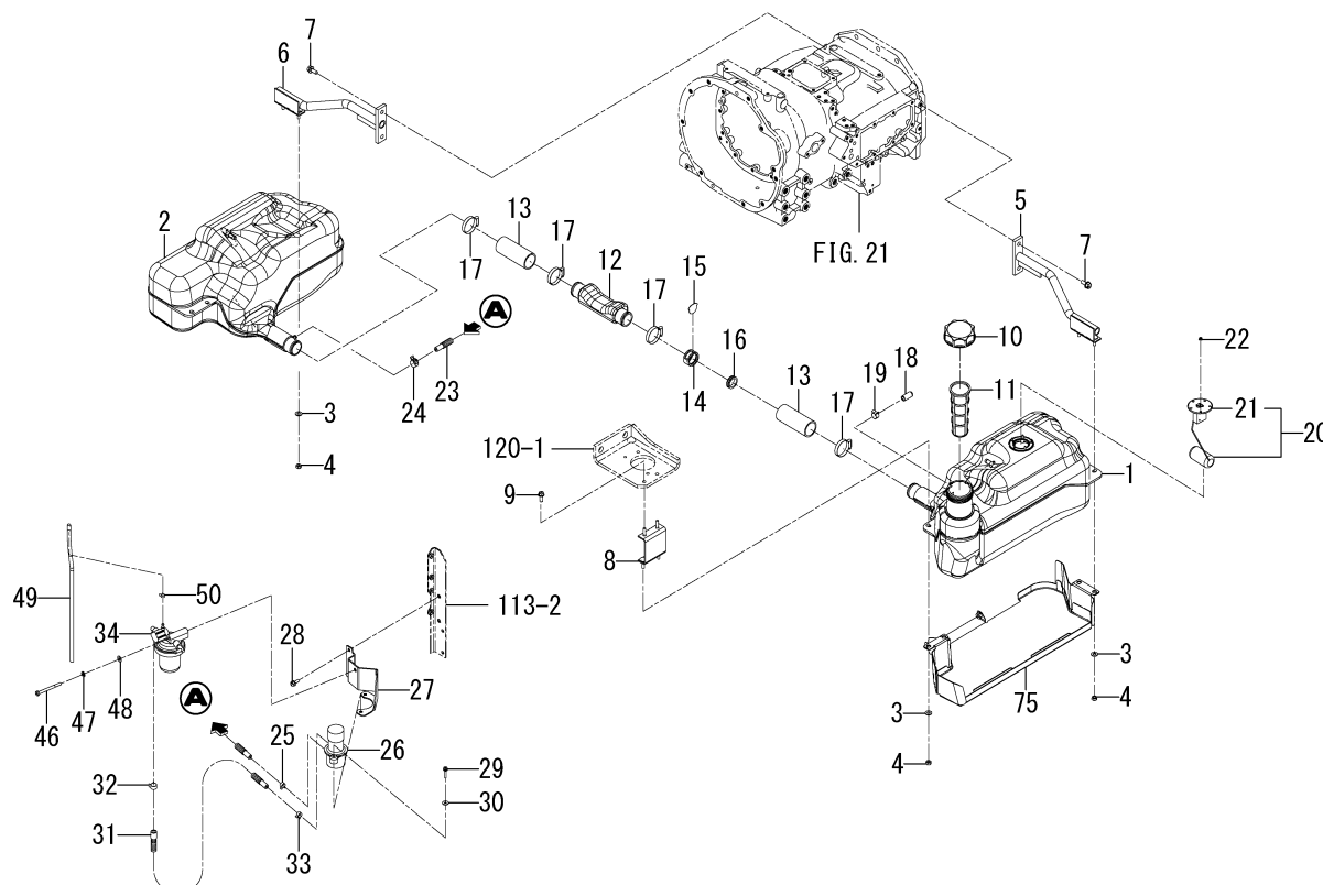
FIG. 11 TANK(FUEL)SYSTEM(1/3) (6370-EXCEPT CY TYPE)
