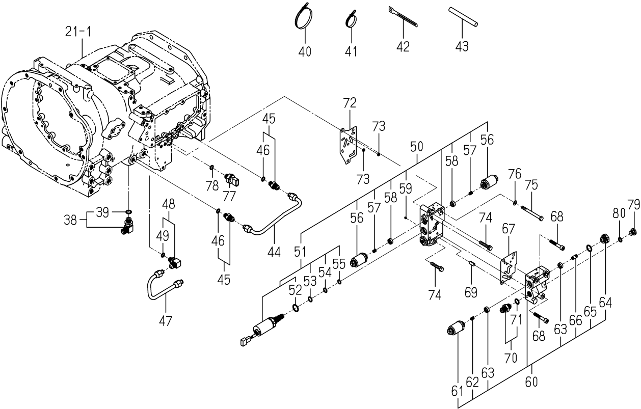
FIG. 88 PIPING(SUB)SYSTEM(6370 TYPE)(2/2)
