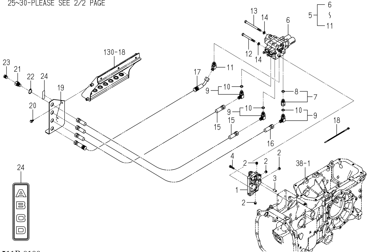
FIG. 90 JOY STICK VALVE SYSTEM(1/2) (6490-CY TYPE EXCEPT D)
