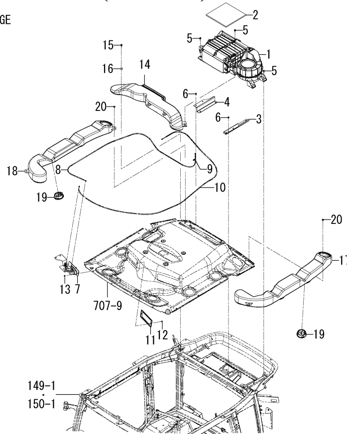
FIG.159 AIR CONDITIONER(CABIN)SYSTEM(1/2) (CY TYPE)
