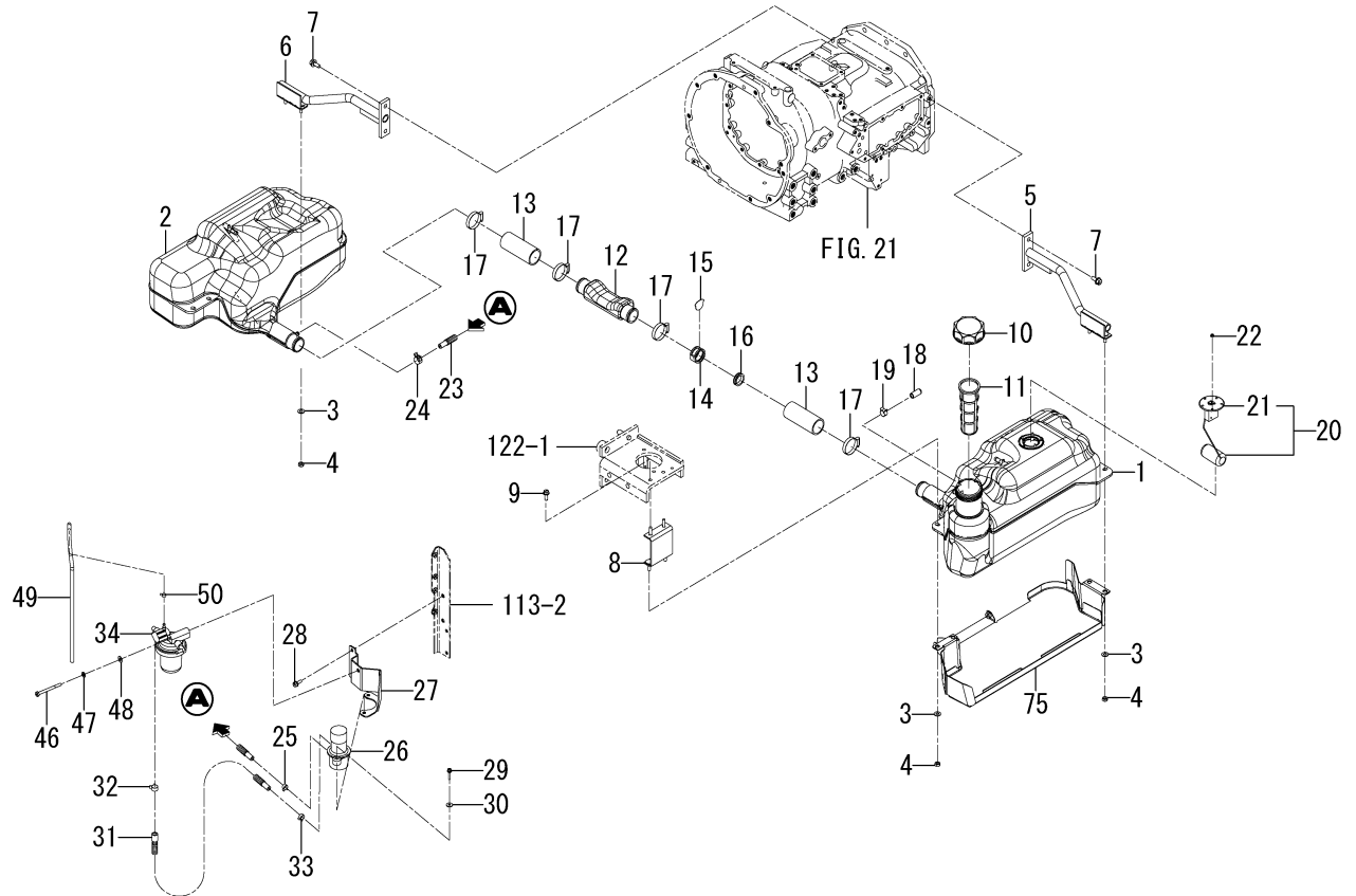
FIG. 13 TANK(FUEL)SYSTEM(6370-CY TYPE)(1/3)
