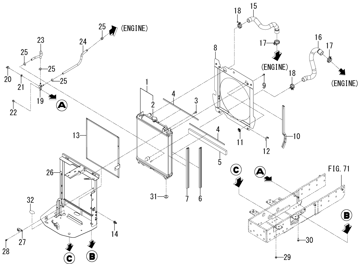
FIG. 4 RADIATOR SYSTEM(1/2) (6370-EXCEPT CY TYPE)
