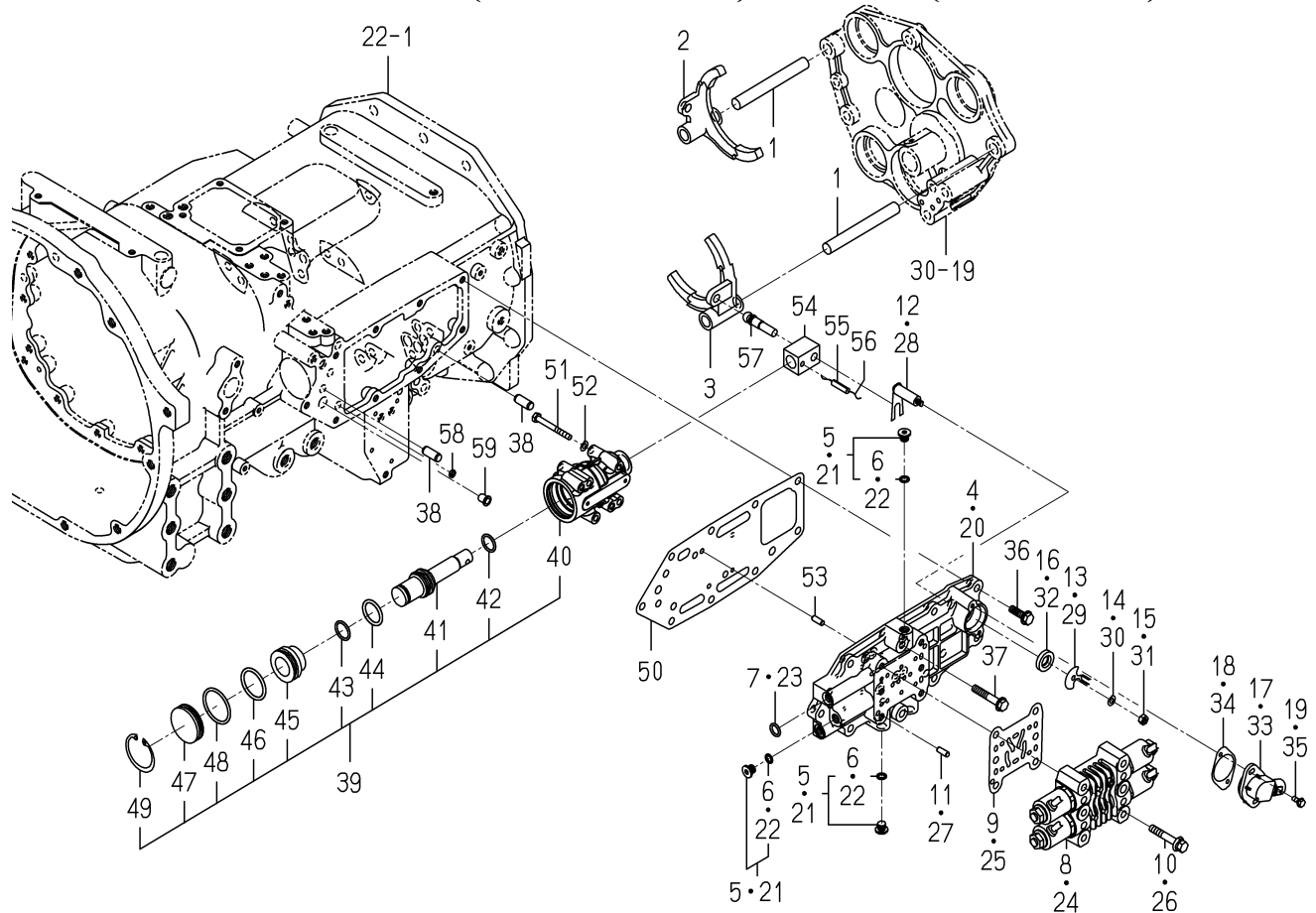
FIG. 40 FORK(SHIFT/MAIN)SYSTEM(6490 TYPE)
