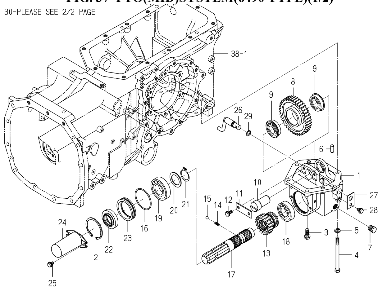
FIG. 37 PTO(MID)SYSTEM(6490 TYPE)(1/2)
