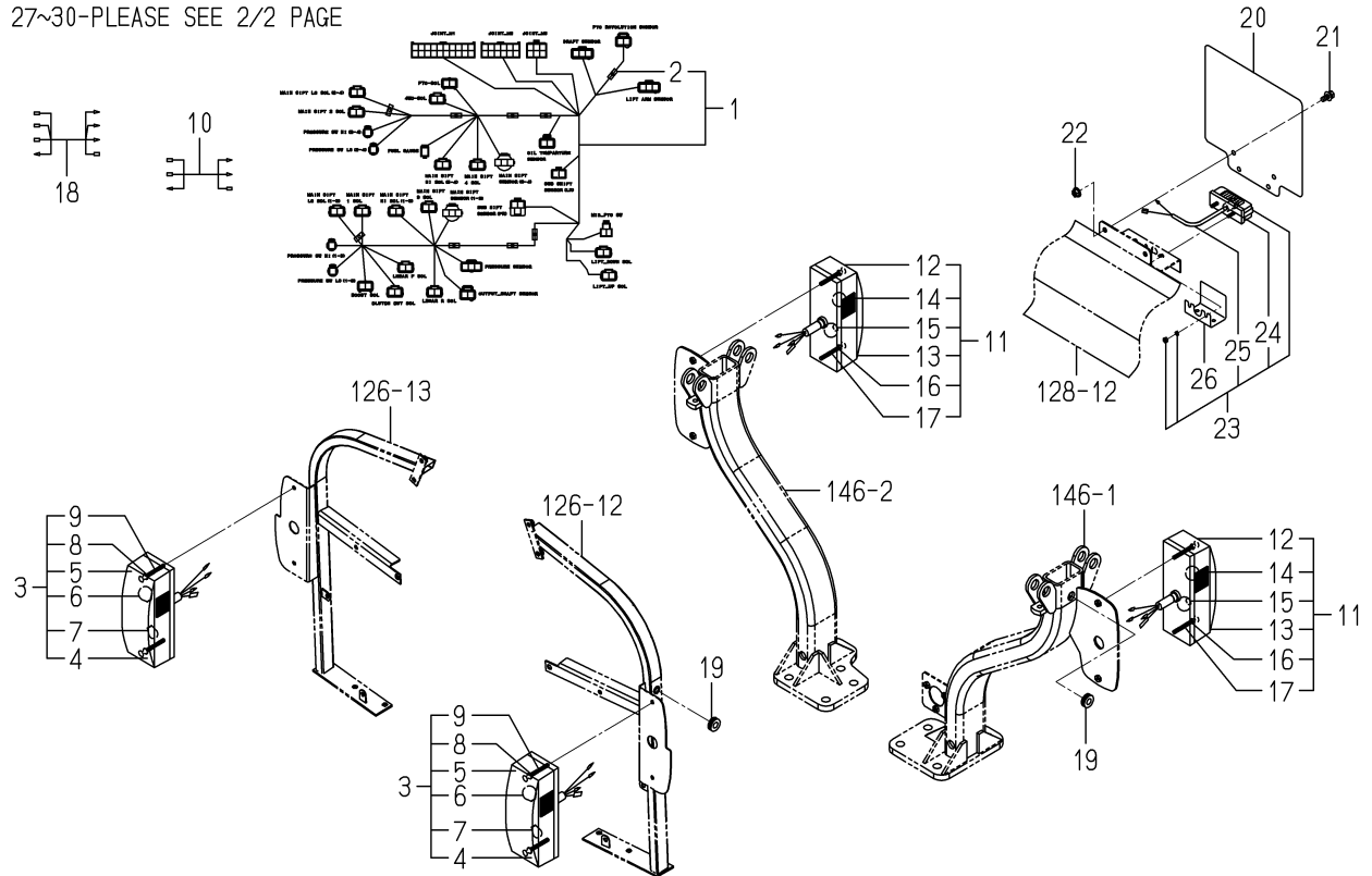
FIG.135 ELC.(FLOOR)SYSTEM(1/2) (6490-EXCEPT CY TYPE)
