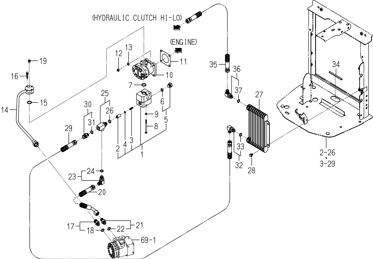
FIG. 89 PIPING(SUB)SYSTEM(6490 TYPE)(1/2)
