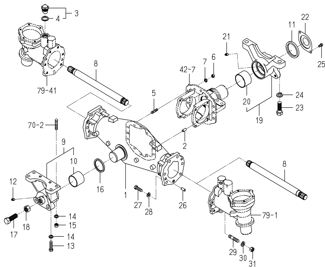
FIG. 77 HOUSING(AXLE/FRONT)SYSTEM(6490 TYPE)
