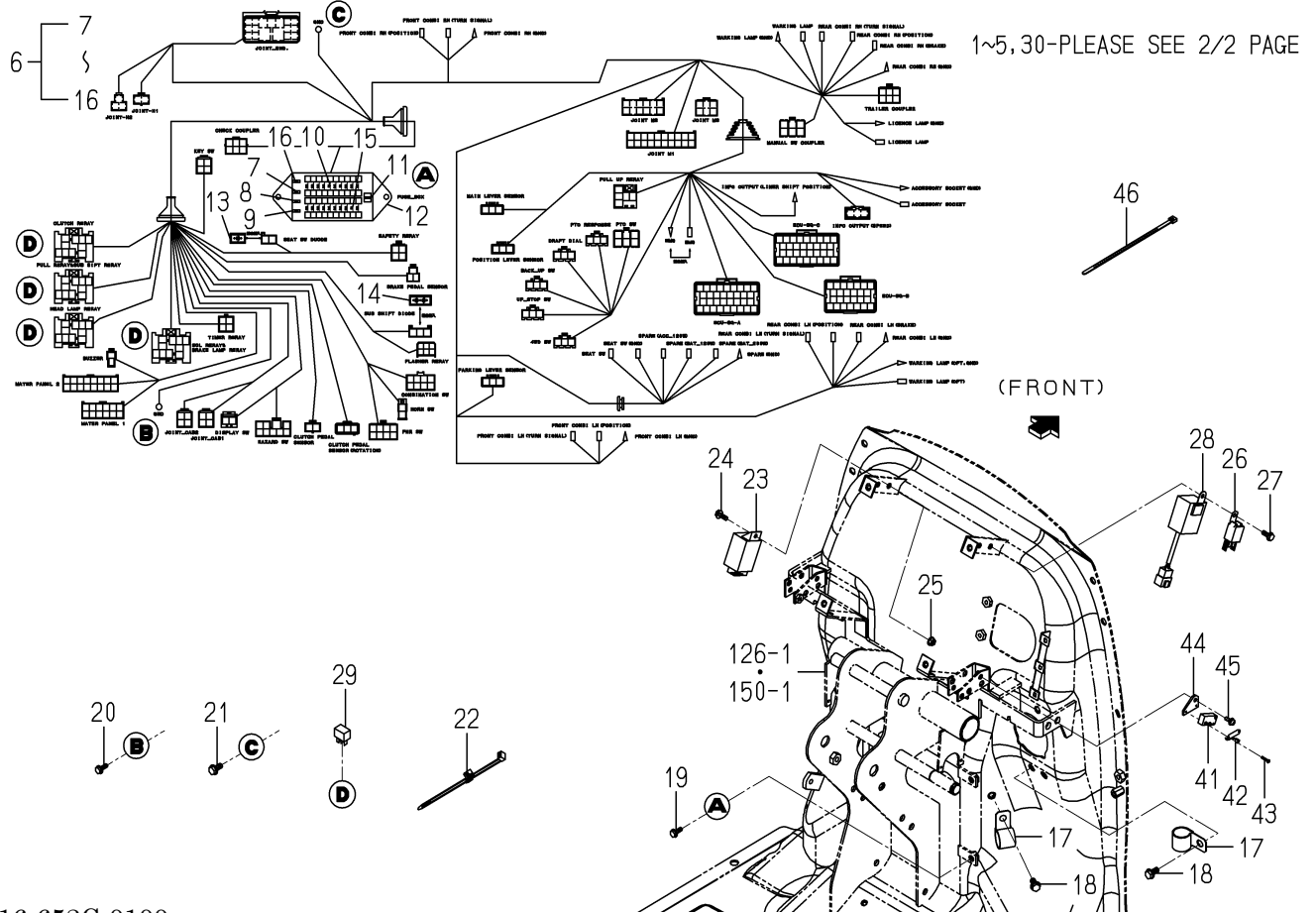
FIG.134 ELC.(MAIN)SYSTEM(6490 TYPE)(1/2)
