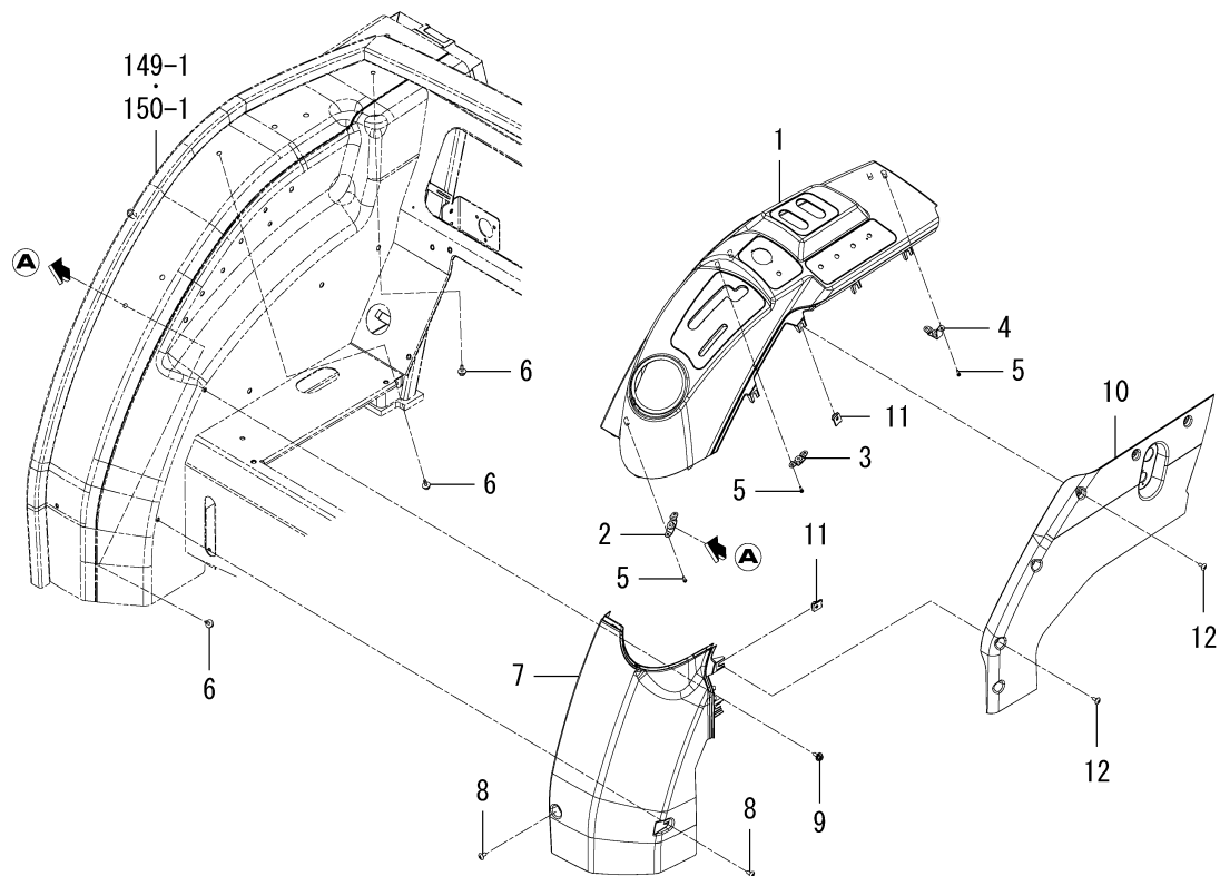
FIG.119 GUIDE(LEVER)SYSTEM(CY TYPE)
