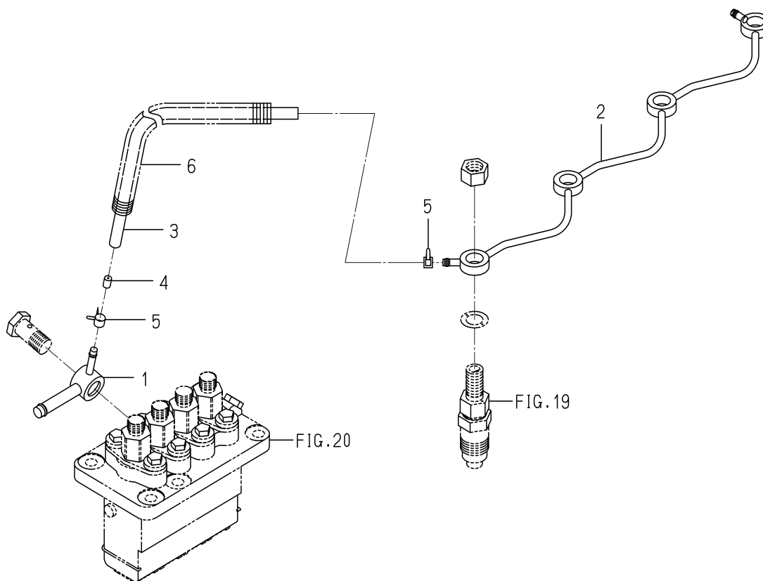
FIG. 21 FUEL PIPE
