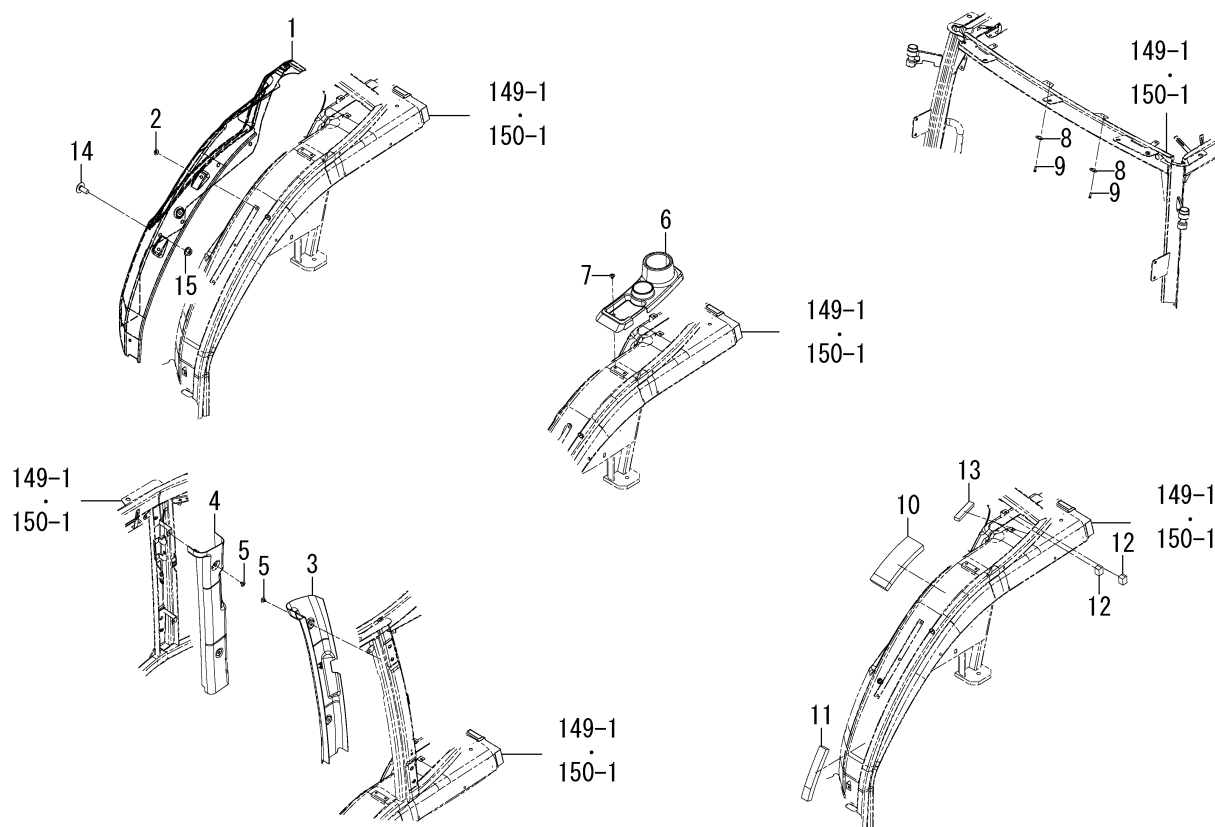
FIG.156 INTERIOR SYSTEM(CY TYPE)
