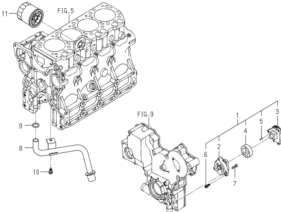
FIG. 16 OIL PUMP
