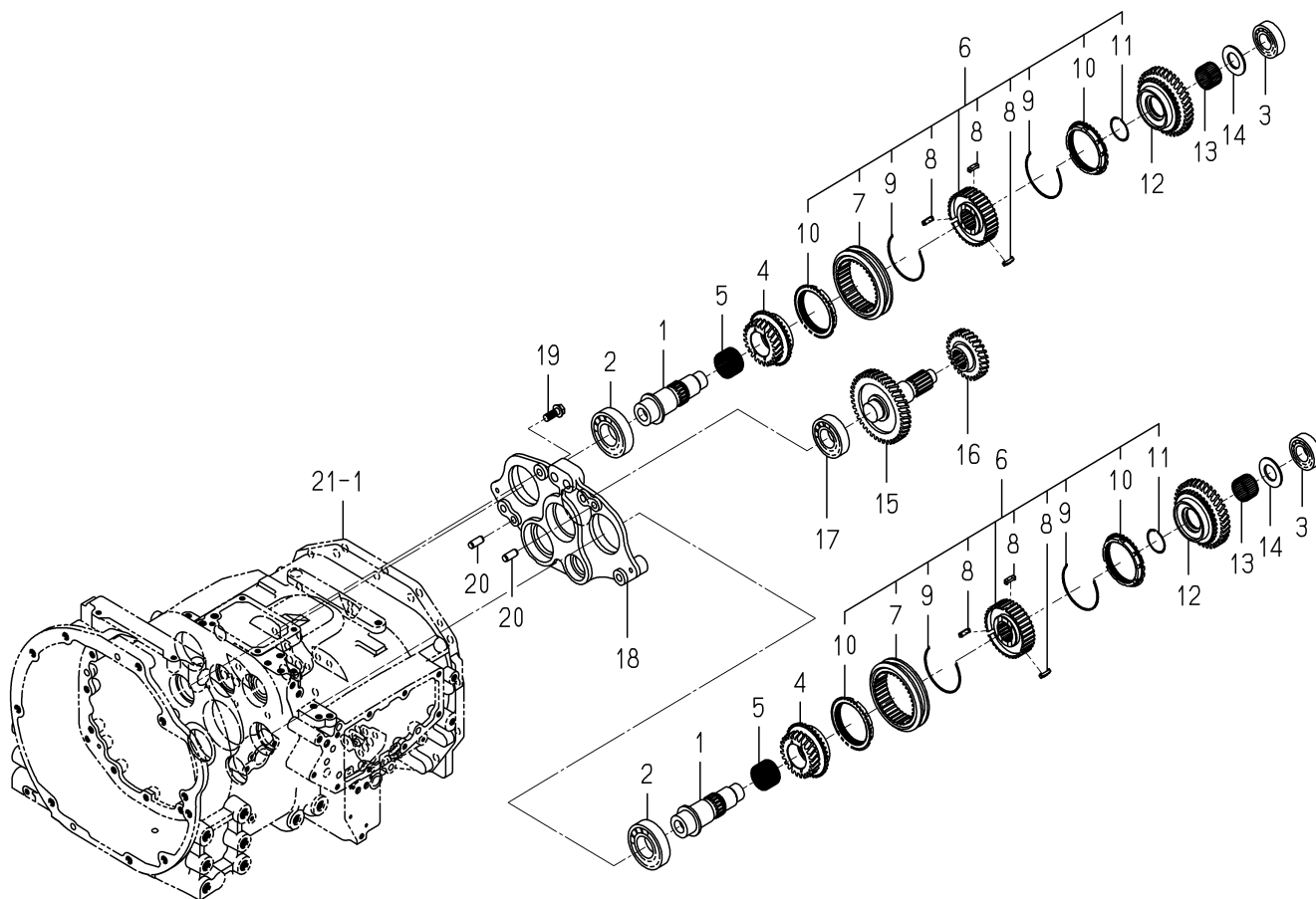
FIG. 27 GEAR(MAIN)SYSTEM(6370 TYPE)
