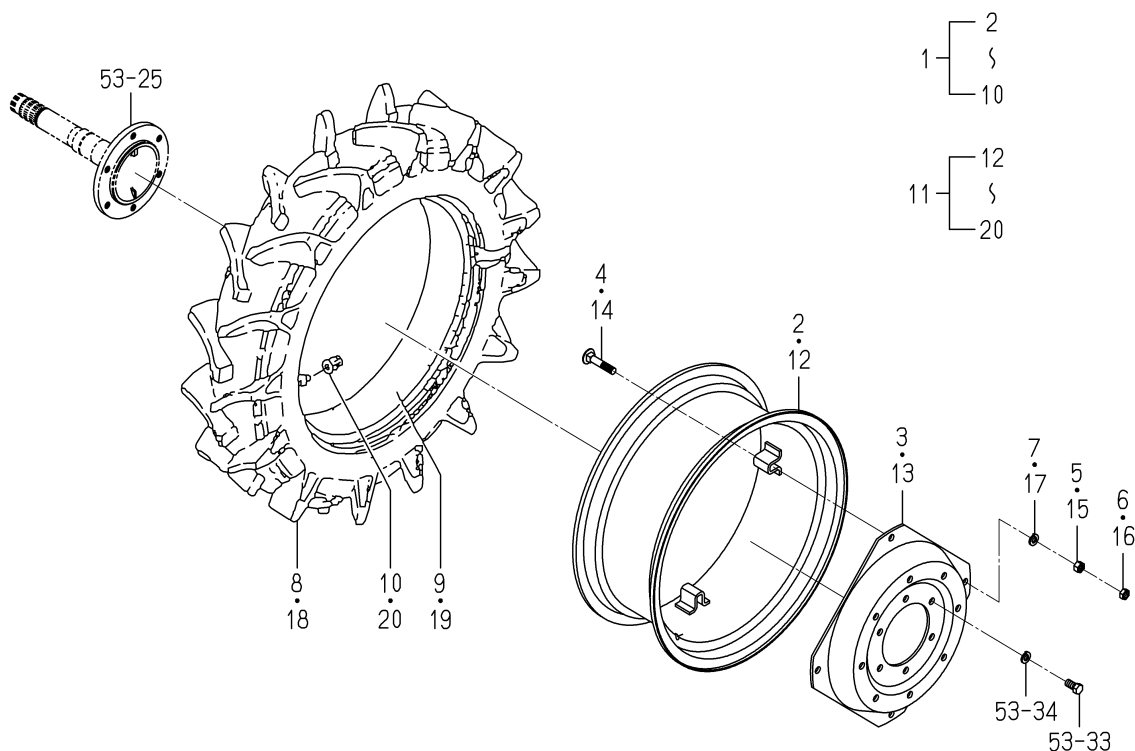
FIG.172 WHEEL(REAR/24XW10)ASSY (6370 TYPE)(OPTION)
