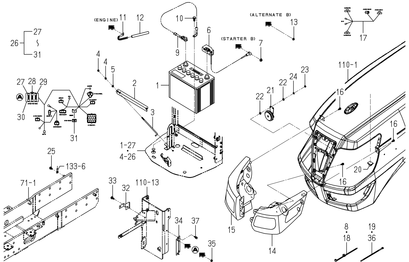
FIG.131 ELC.(FRONT)SYSTEM(6370 TYPE)
