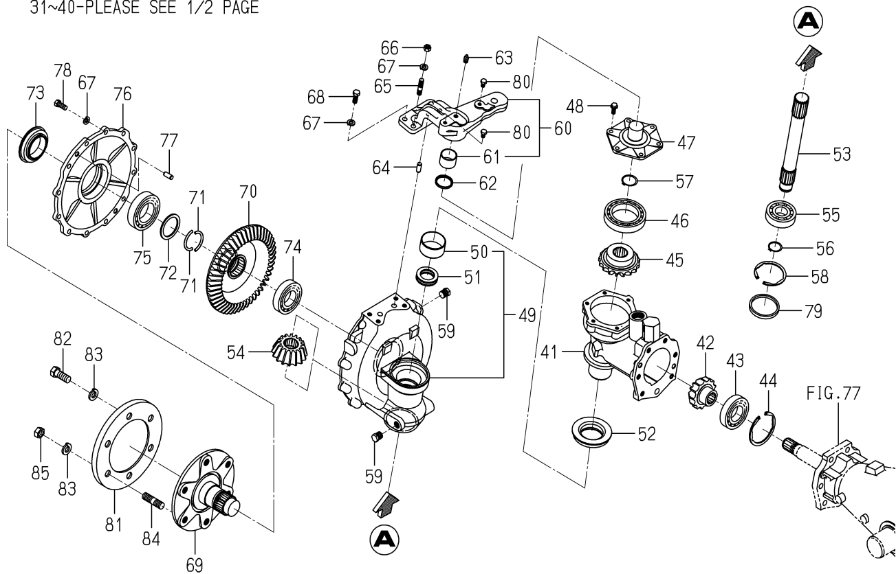
FIG. 79 CASE(GEAR/FINAL)SYSTEM(6490 TYPE)(2/2)
