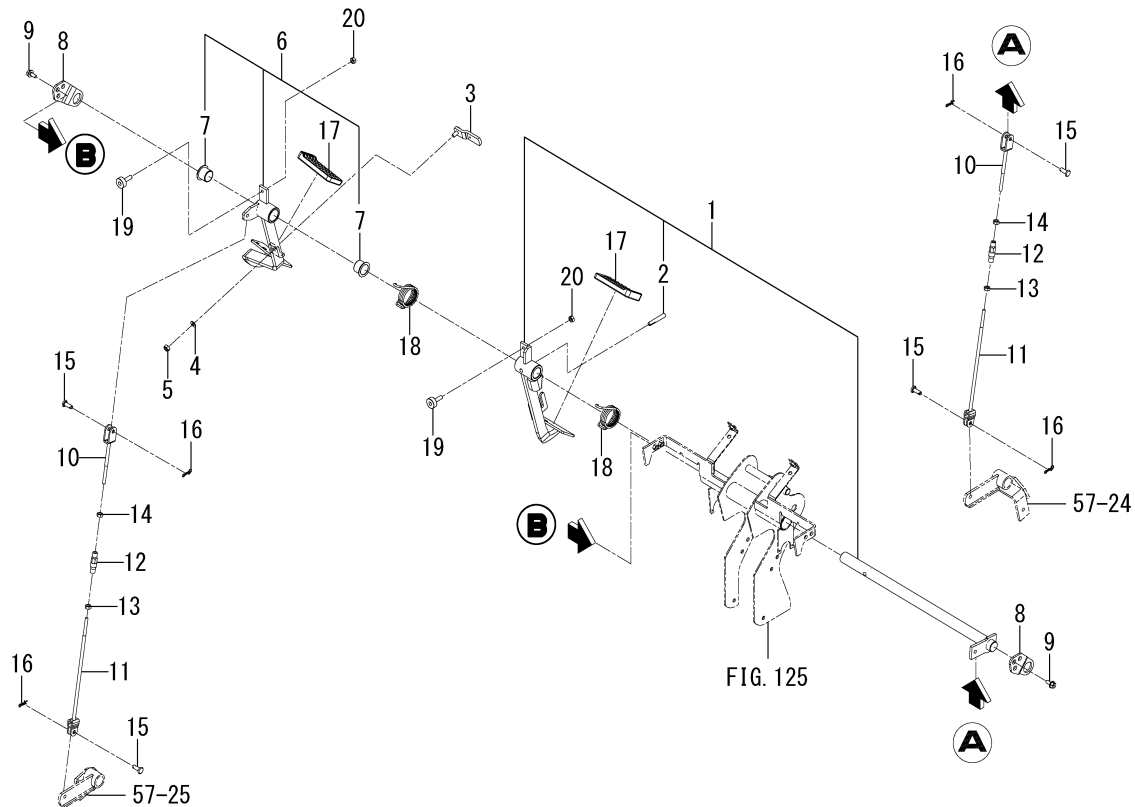
FIG. 59 PEDAL(BRAKE)SYSTEM (6370-EXCEPT CY TYPE)
