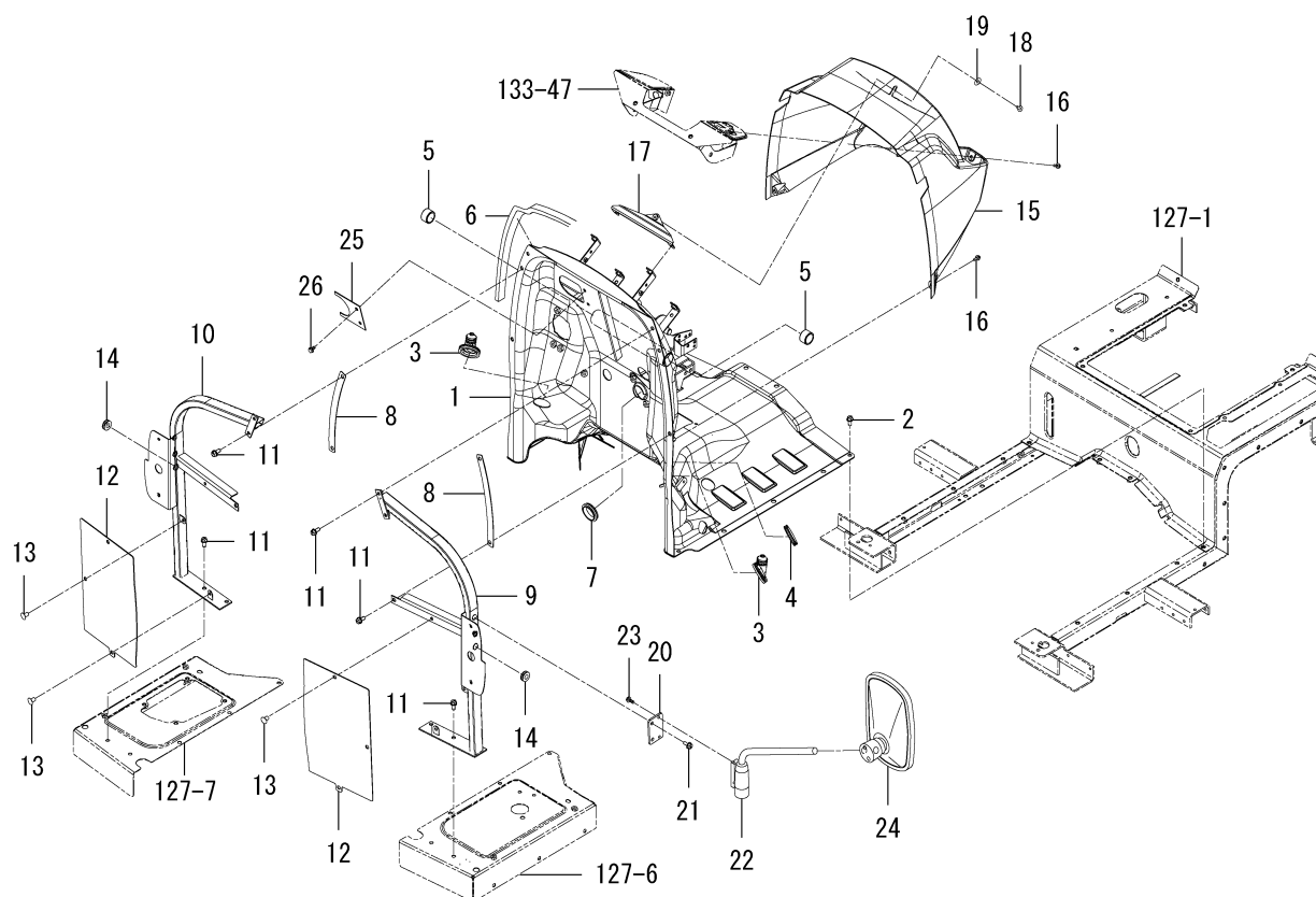
FIG.125 PANEL(DASH)SYSTEM (6370-EXCEPT CY TYPE)
