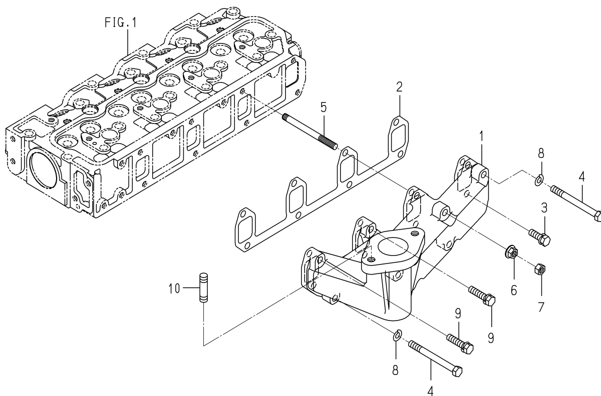
FIG. 4 EXHAUST MANIFOLD
