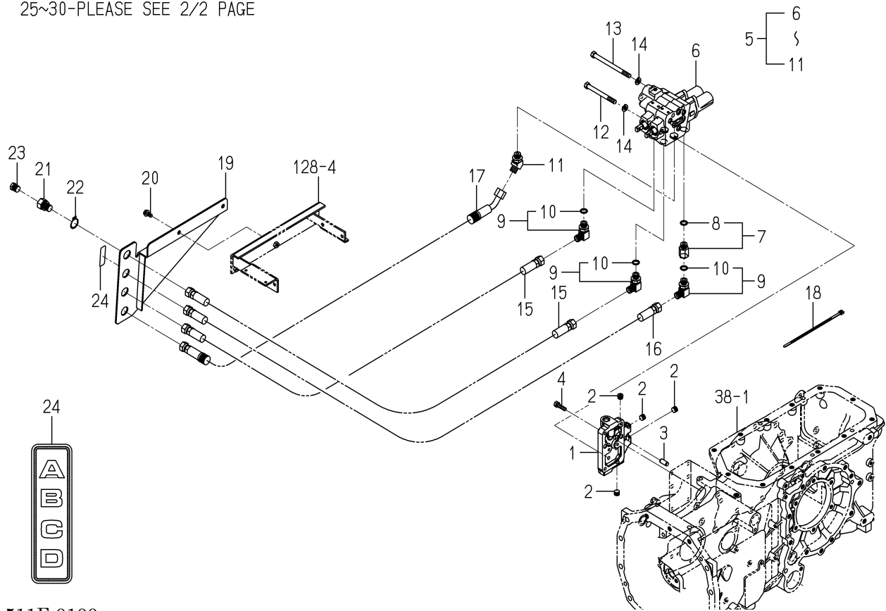
FIG. 92 JOY STICK VALVE SYSTEM(1/2) (6490-EXCEPT CY TYPE)
