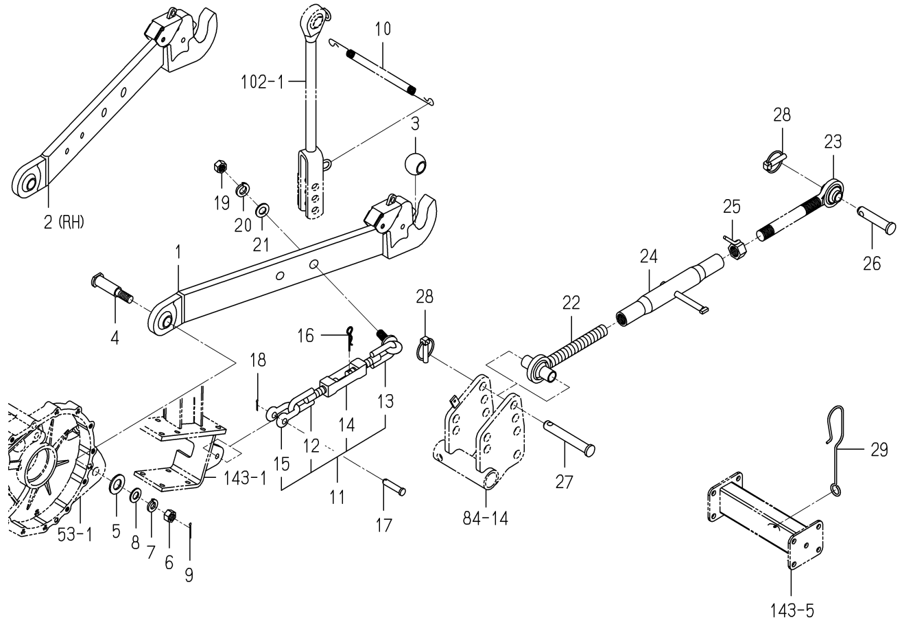
FIG. 98 LINK(3P)SYSTEM(6370-EXCEPT CY TYPE)
