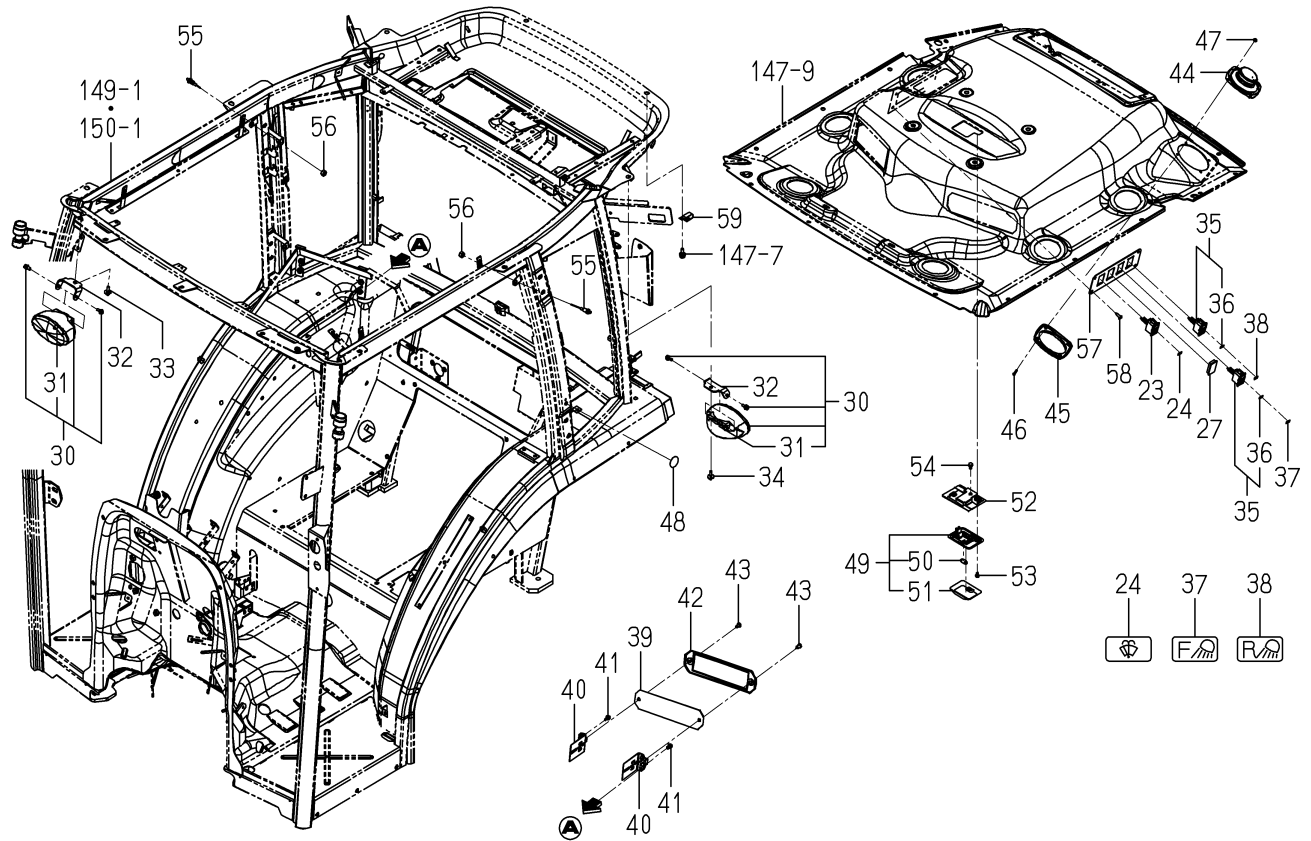
FIG.140 ELC.(CABIN)SYSTEM(CY TYPE)(2/2)
