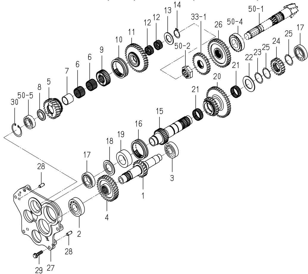
FIG. 31 GEAR(SUB)SYSTEM(6370 TYPE)
