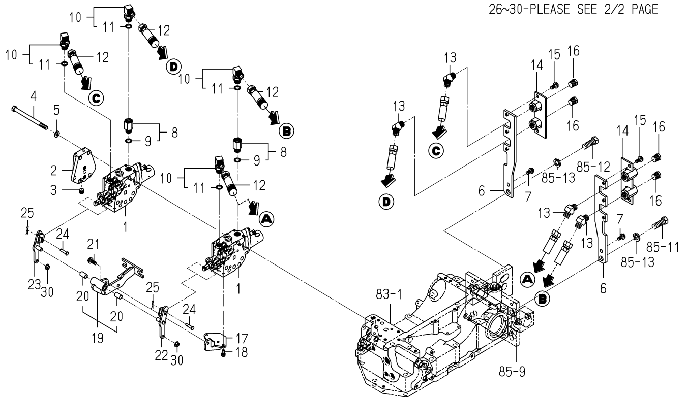
FIG. 97 VALVE(REMOTE/2)SET(6490 TYPE)(1/2)
