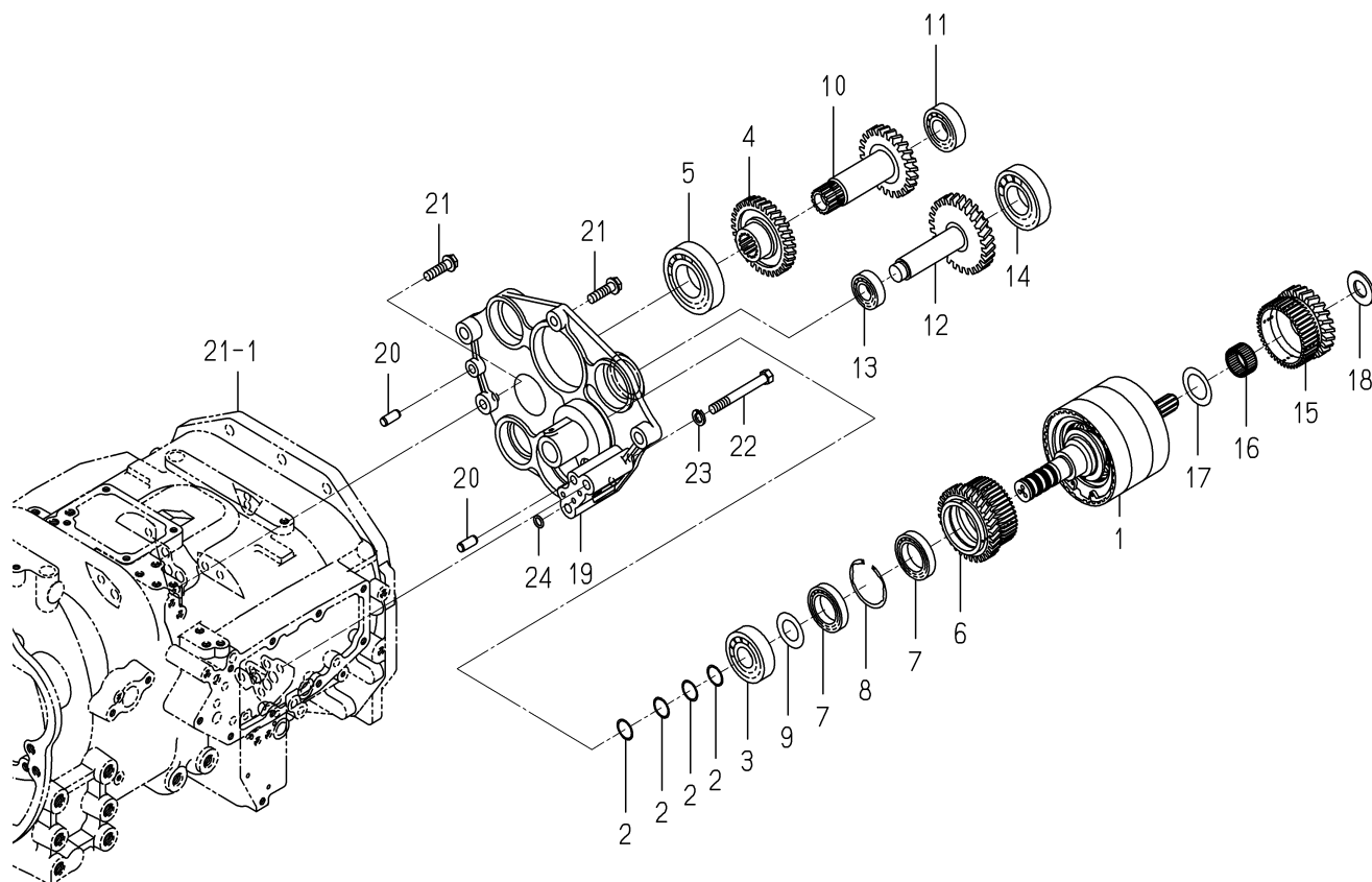
FIG. 29 GEAR(REVERSE)SYSTEM(6370 TYPE)
