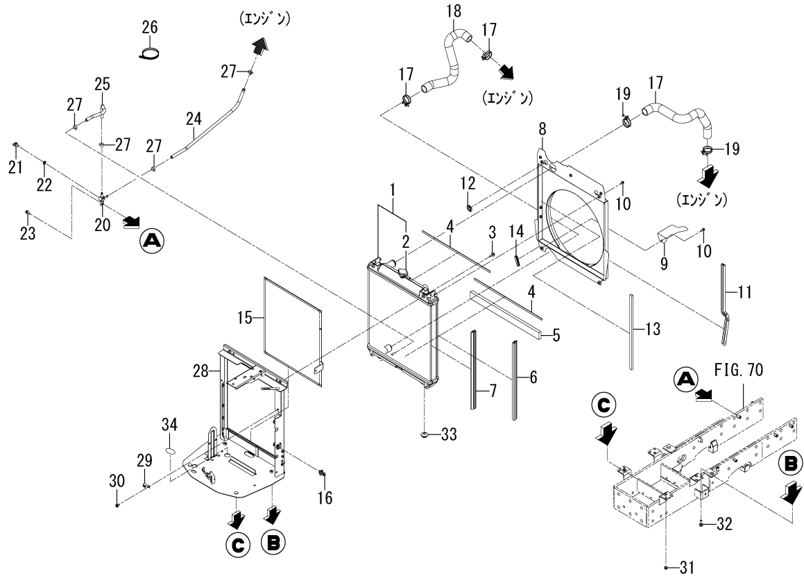
FIG. 2 RADIATOR SYSTEM(1/2) (6490-EXCEPT CY TYPE)
