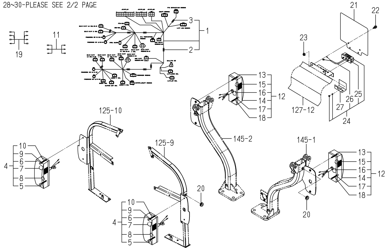
FIG.137 ELC.(FLOOR)SYSTEM(1/2) (6370-EXCEPT CY TYPE)
