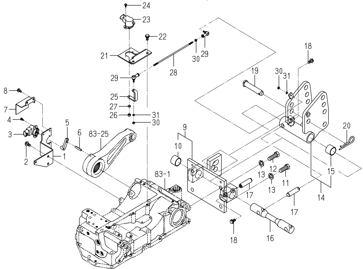
FIG. 85 CONTROL(POSITION&DRAFT)SYSTEM (6490 TYPE)
