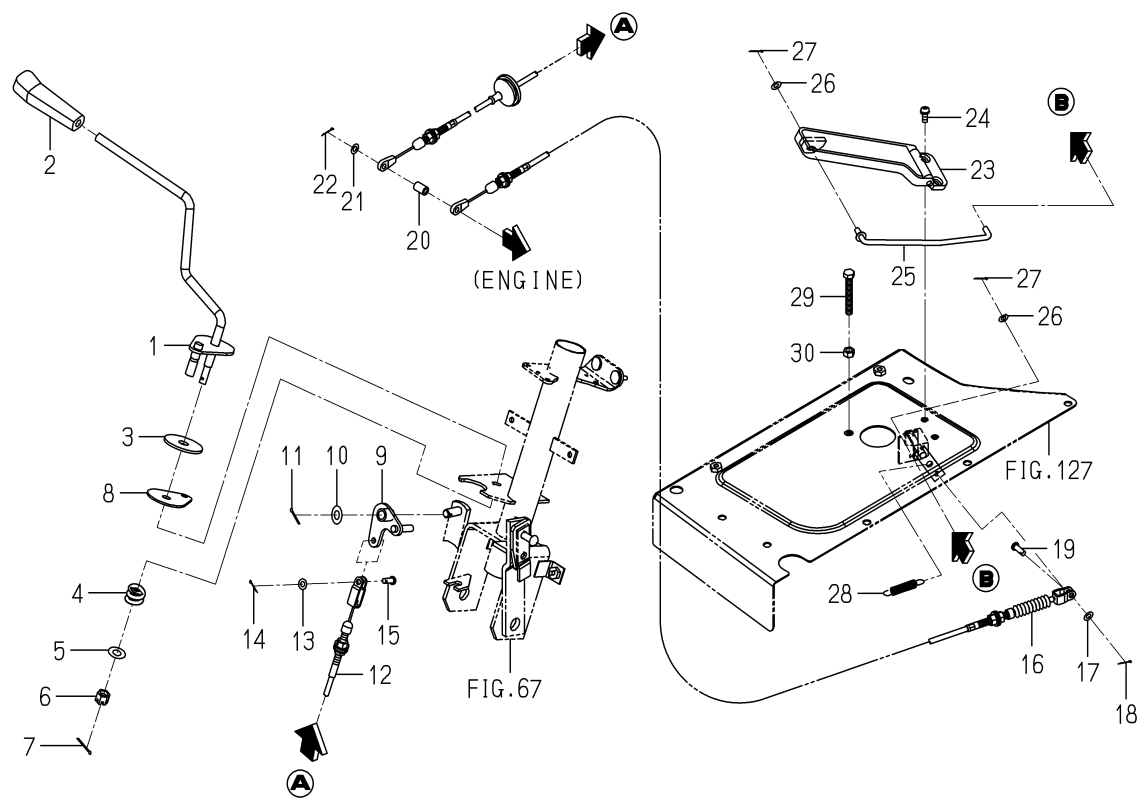
FIG. 14 ACCELERATOR SYSTEM (6370-EXCEPT CY TYPE)
