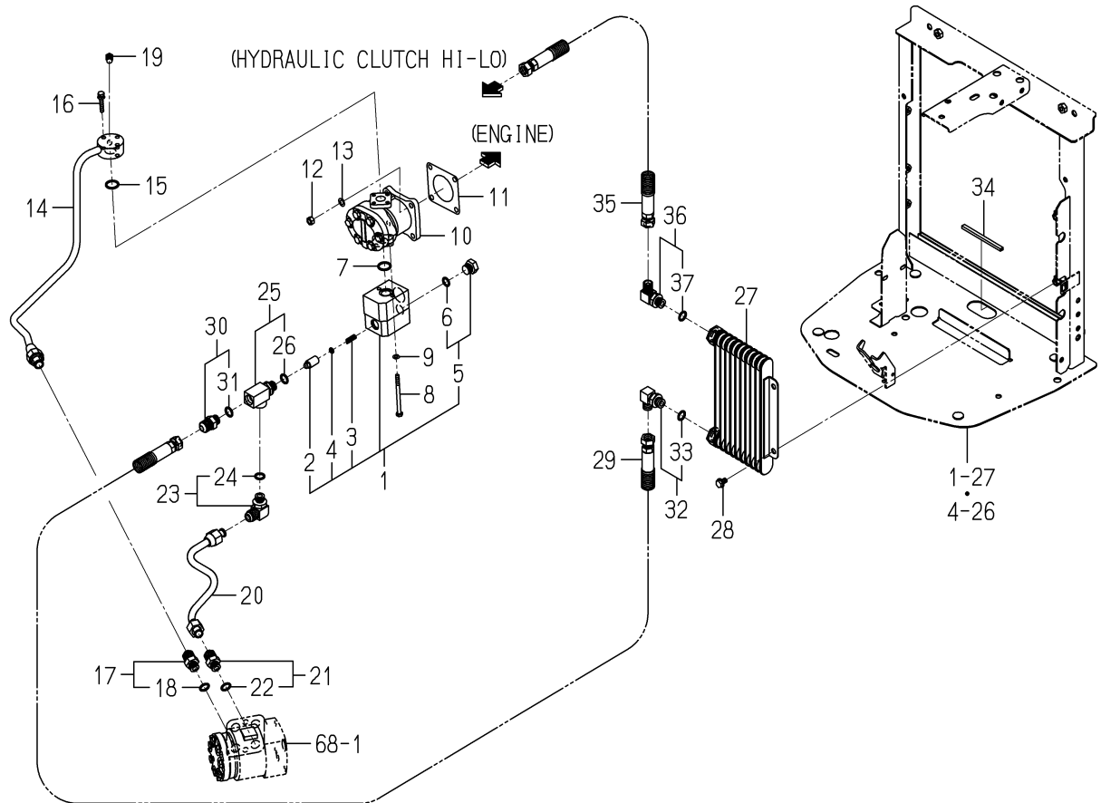
FIG. 88 PIPING(SUB)SYSTEM(6370 TYPE)(1/2)
