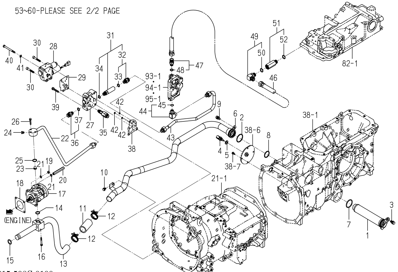
FIG. 86 PIPING(MAIN)SYSTEM(6370 TYPE)(1/2)
