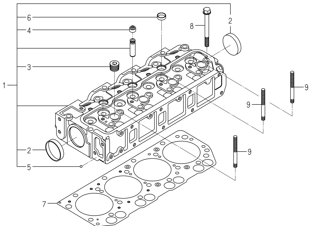
FIG. 1 CYLINDER HEAD
