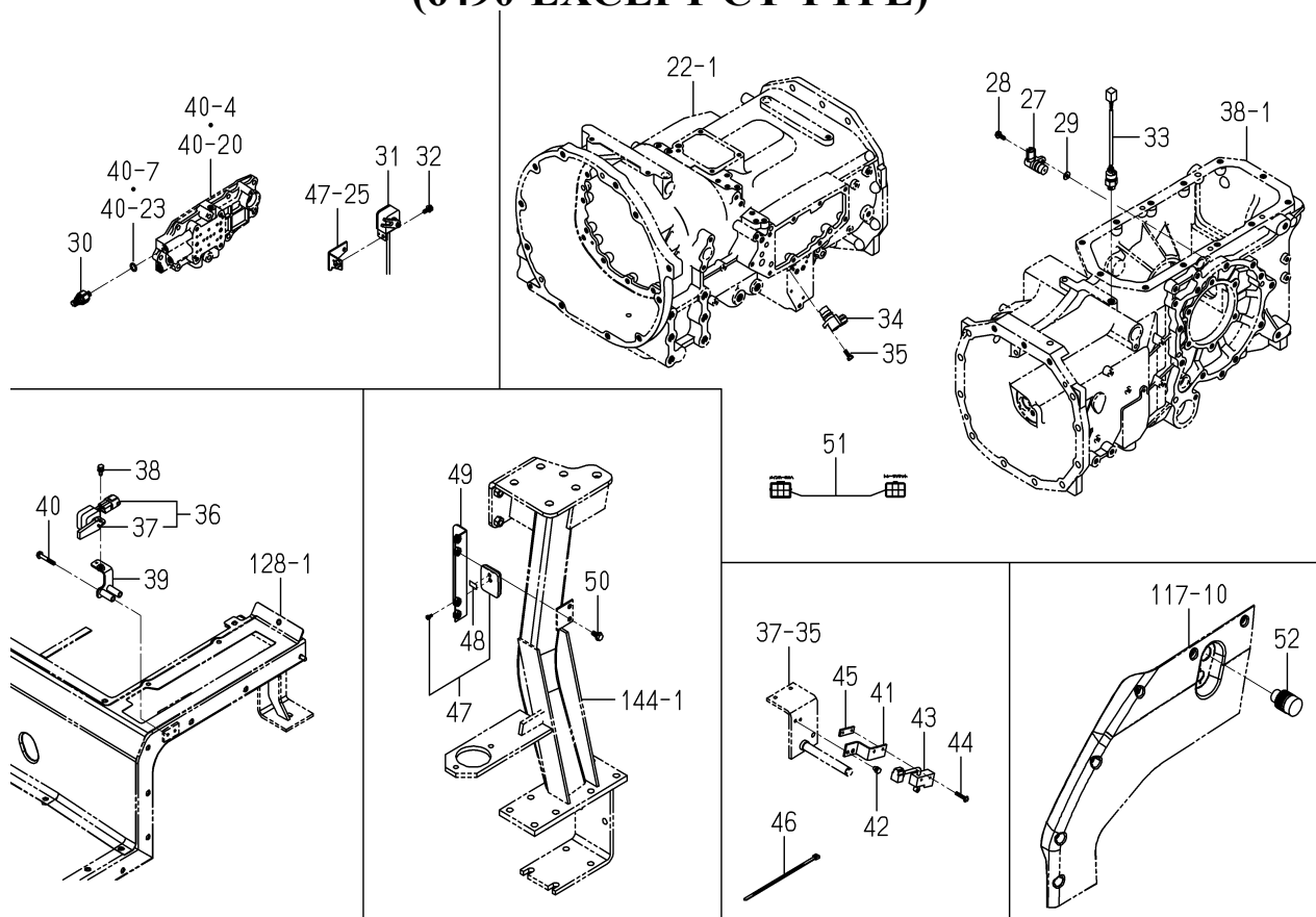
FIG.135 ELC.(FLOOR)SYSTEM(2/2) (6490-EXCEPT CY TYPE)
