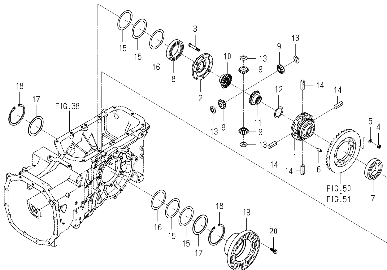
FIG. 52 CASE(DIFFERENTIAL/REAR)SYSTEM
