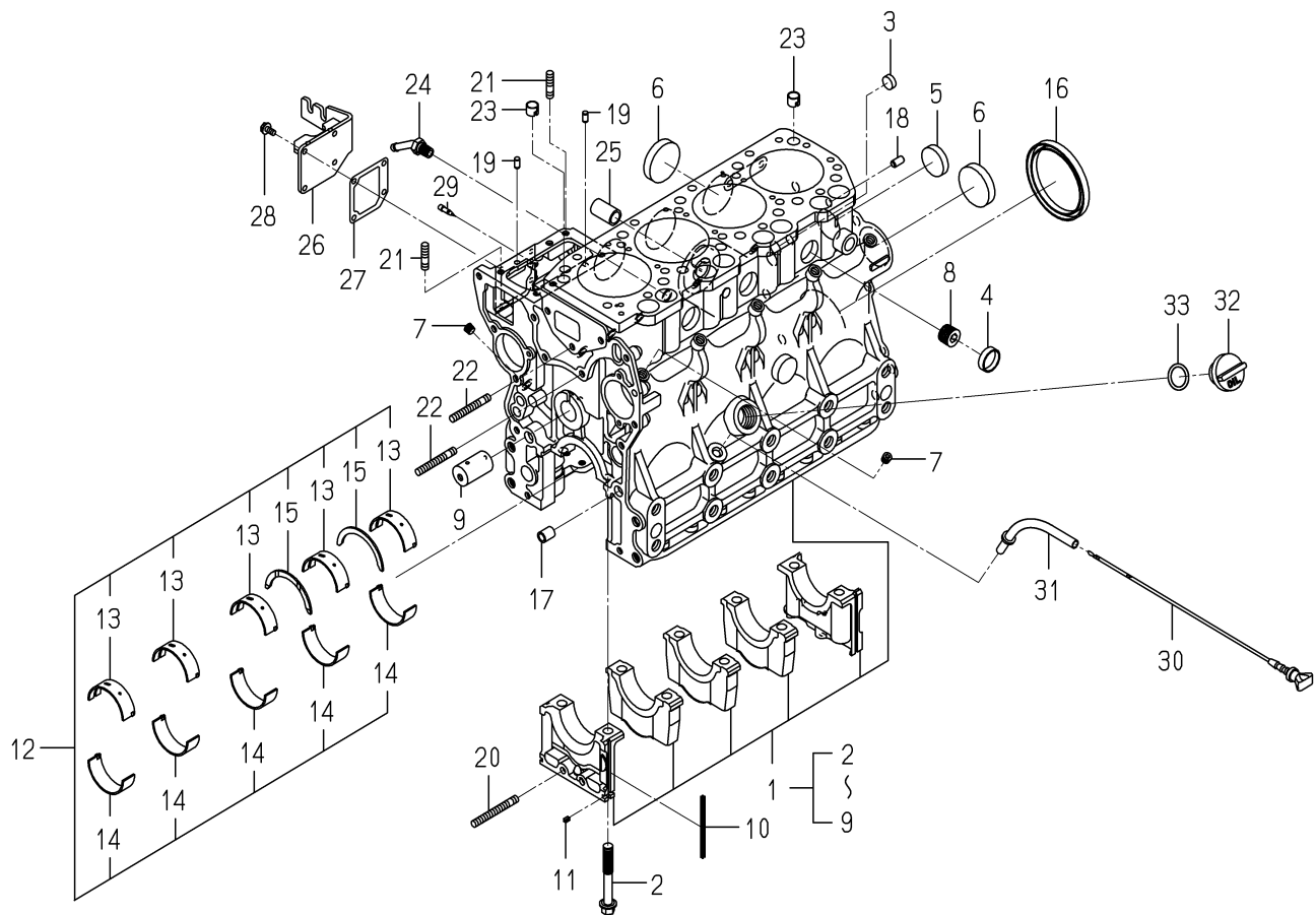
FIG. 5 CYLINDER BLOCK
