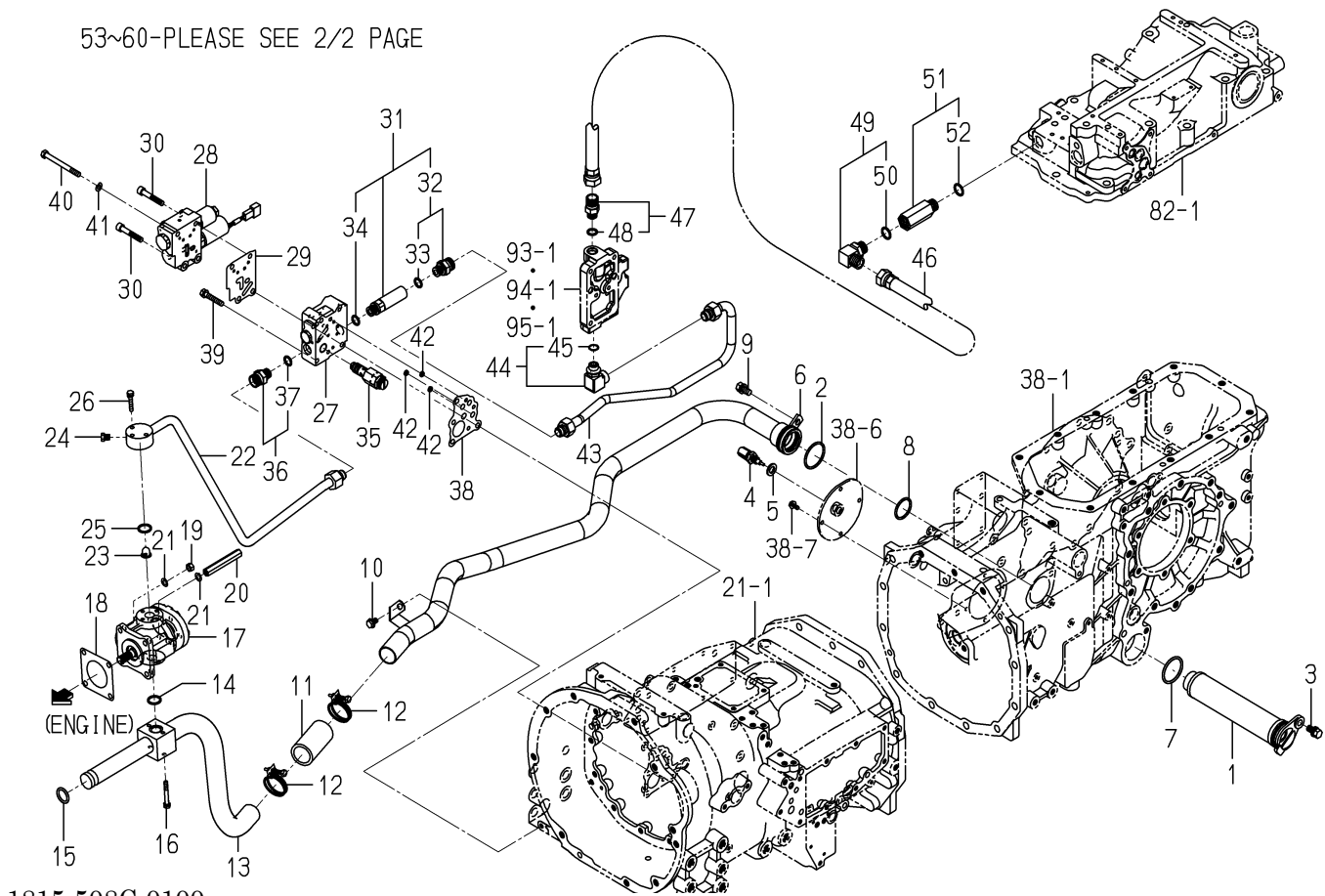
FIG. 86 PIPING(MAIN)SYSTEM(6370 TYPE)(1/2)
