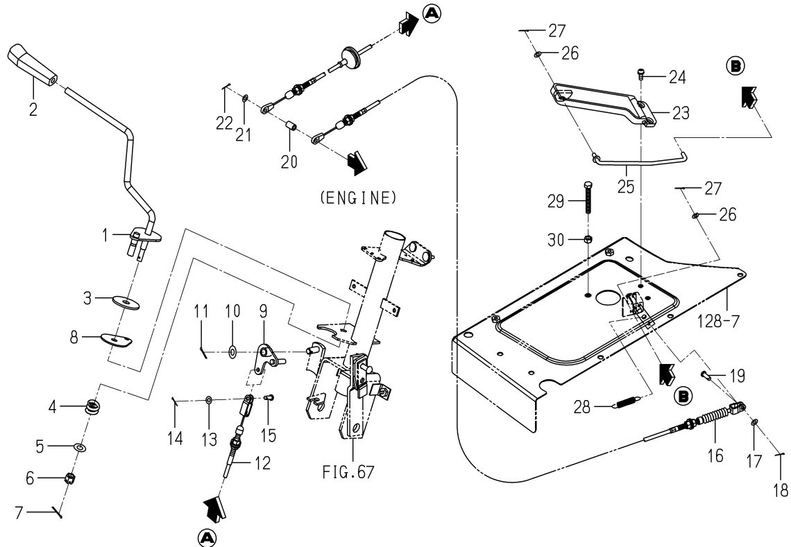
FIG. 15 ACCELERATOR SYSTEM (6490-EXCEPT CY TYPE)
