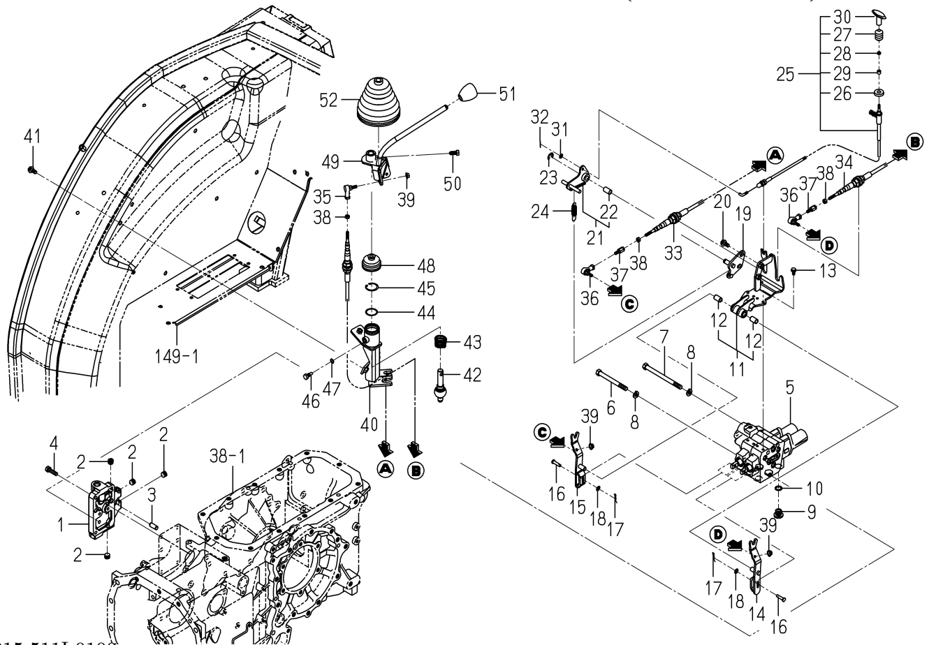
FIG. 95 JOY STICK VALVE SYSTEM(6370-D TYPE)
