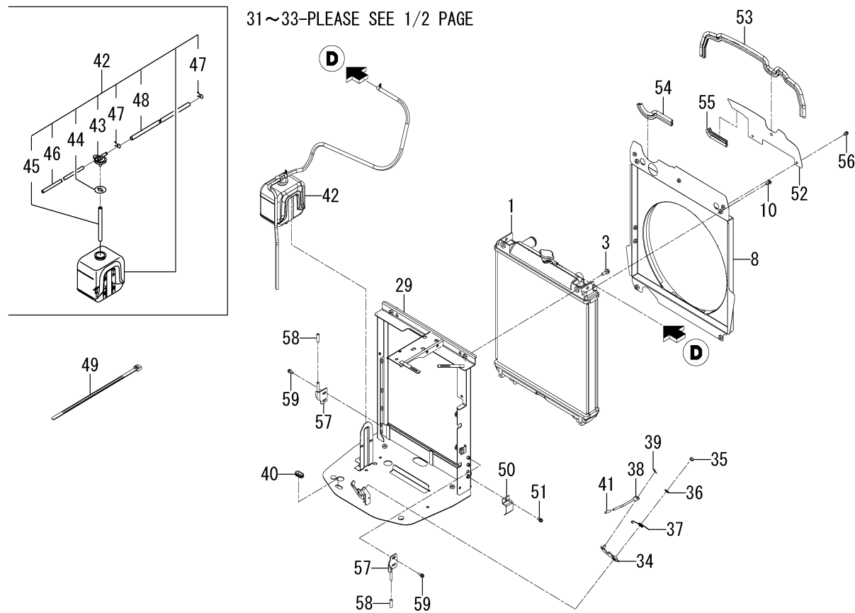
FIG. 3 RADIATOR SYSTEM(6490-CY TYPE)(2/2)
