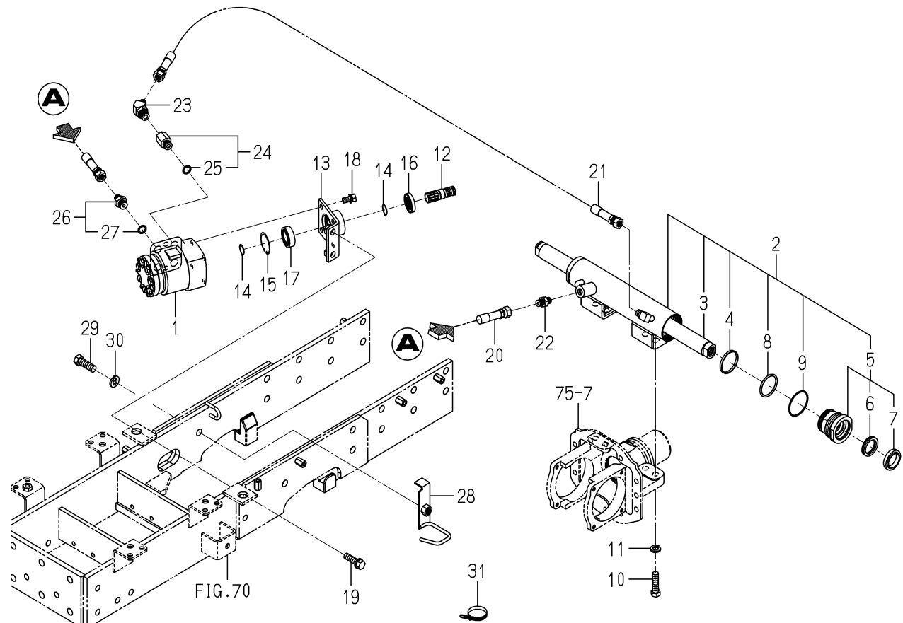
FIG. 69 STEERING(POWER)SYSTEM(6490 TYPE)
