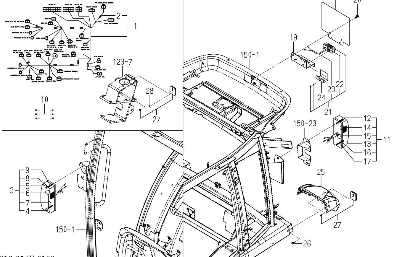
FIG.136 ELC.(FLOOR)SYSTEM(6490-CY TYPE)(1/2)
