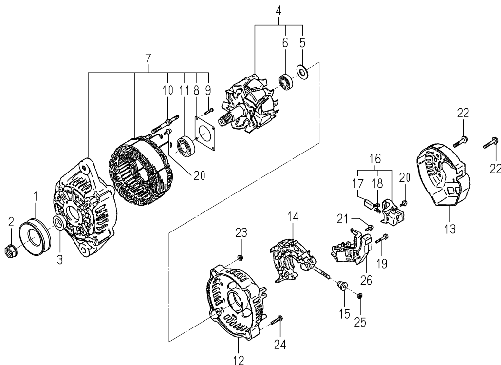
FIG. 29 COMPONENT PARTS FOR 6281-200-015-00 ON Fig.23
