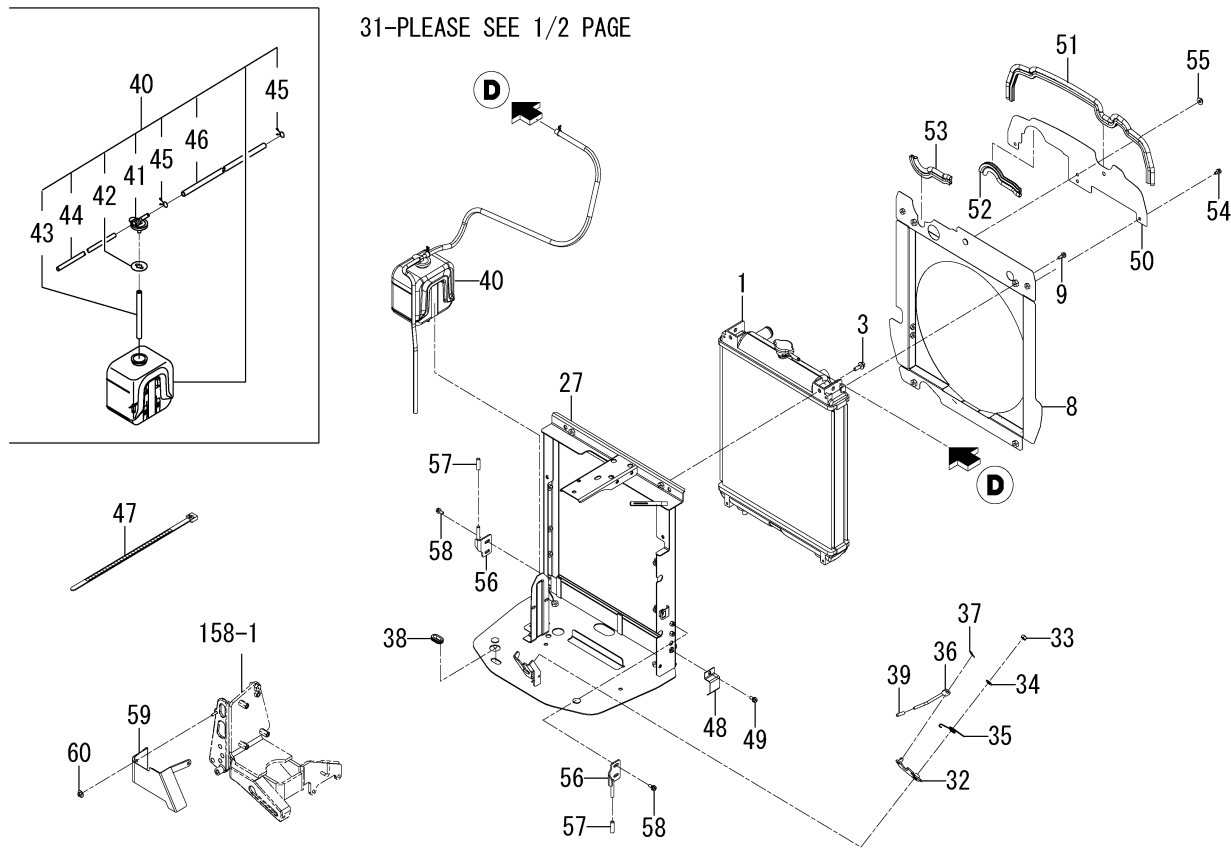
FIG. 1 RADIATOR SYSTEM(6370-CY TYPE)(2/2)
