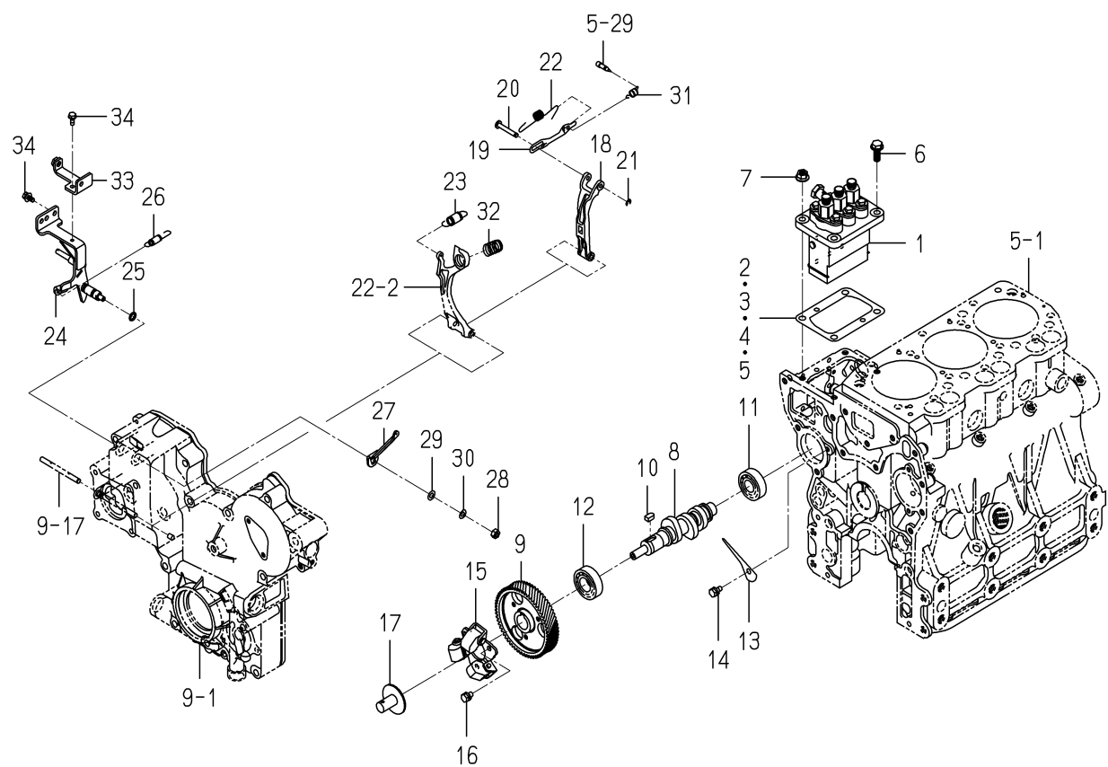
FIG. 20 INJECTION PUMP
