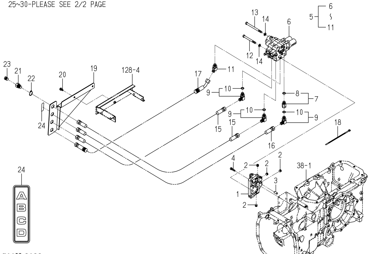
FIG. 94 JOY STICK VALVE SYSTEM(1/2) (6370-EXCEPT CY TYPE)
