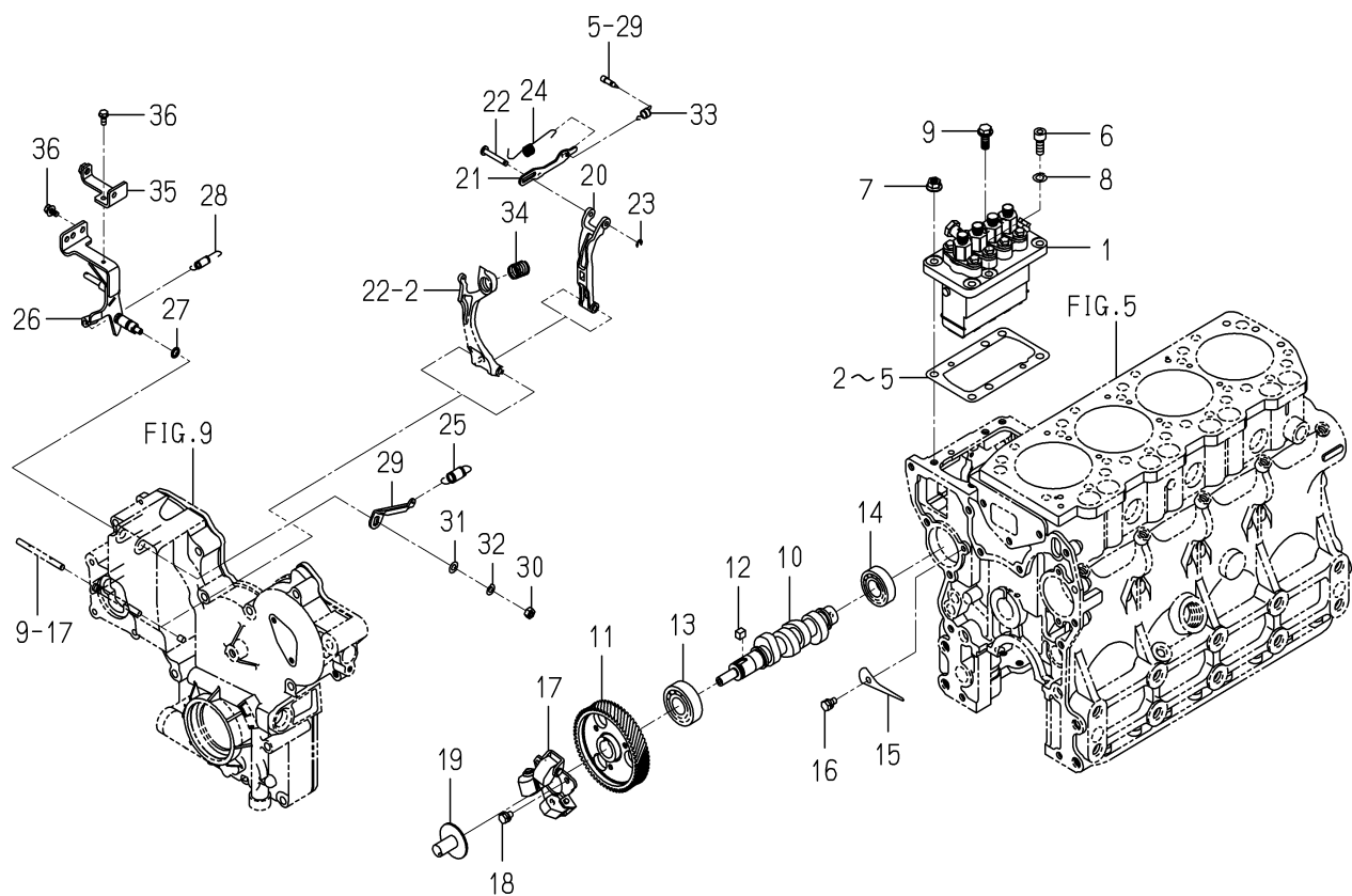
FIG. 20 INJECTION PUMP
