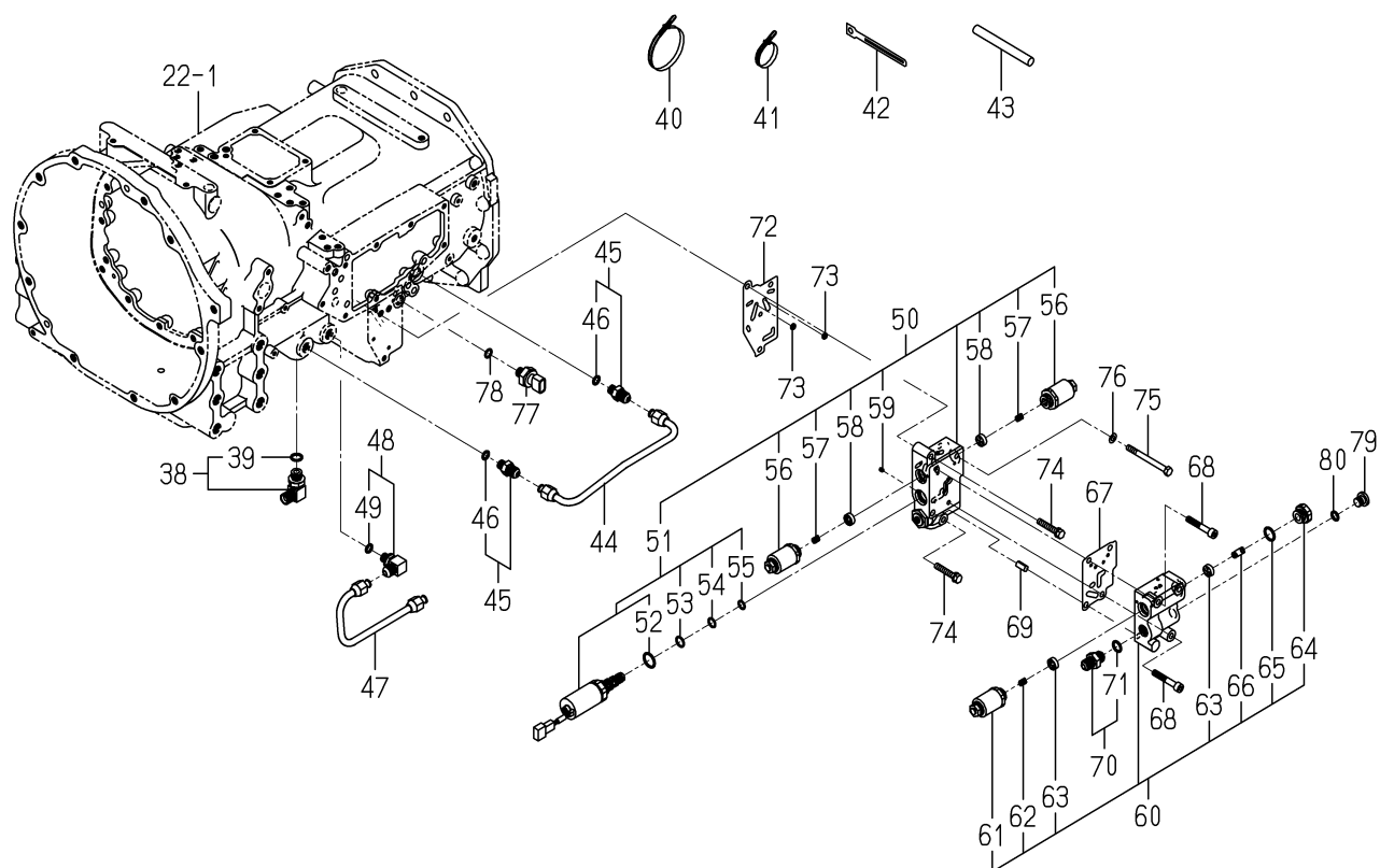
FIG. 89 PIPING(SUB)SYSTEM(6490 TYPE)(2/2)
