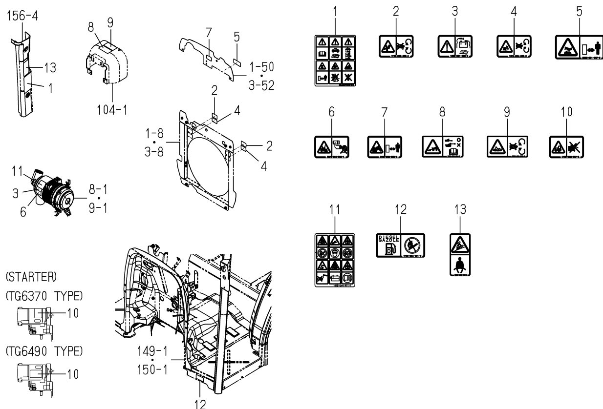
FIG.167 LABEL(CAUTION)(CY TYPE)
