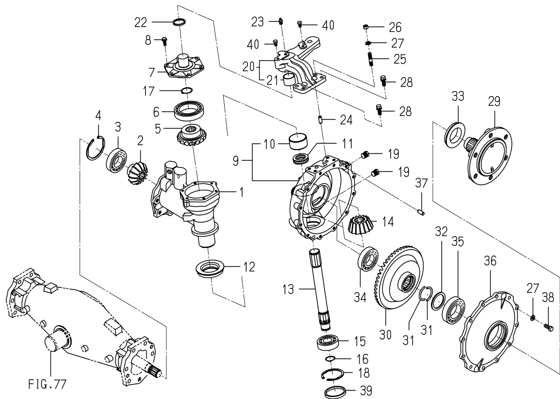
FIG. 79 CASE(GEAR/FINAL)SYSTEM(6490 TYPE)(1/2)
