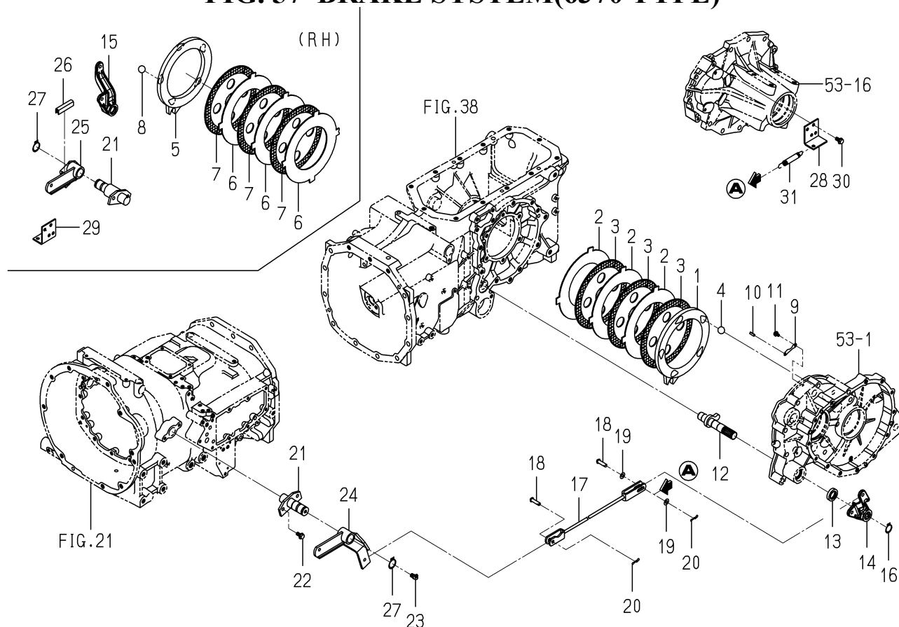
FIG. 57 BRAKE SYSTEM(6370 TYPE)
