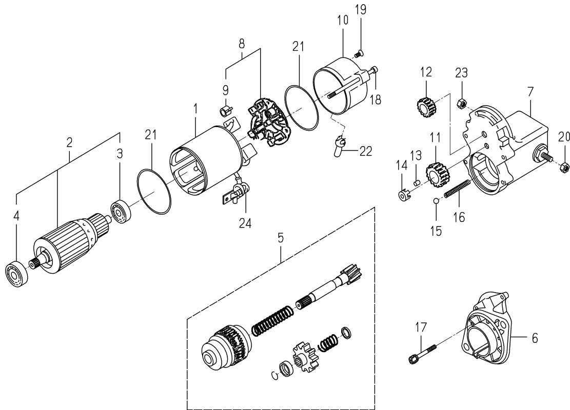
FIG. 28 COMPONENT PARTS FOR 6281-100-010-50 ON Fig.23
