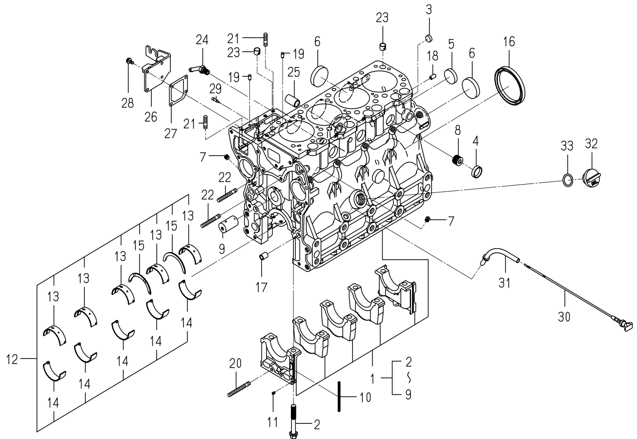
FIG. 5 CYLINDER BLOCK
