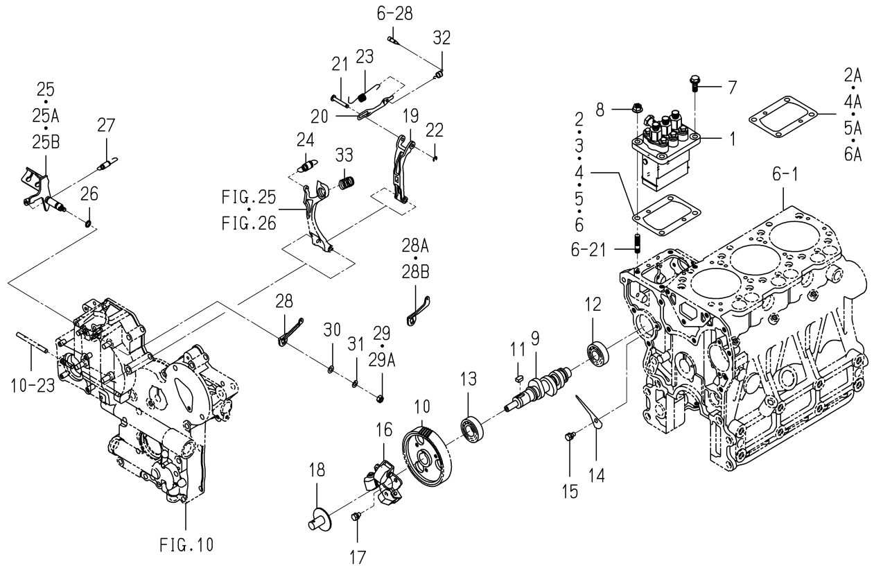
FIG. 23 INJECTION PUMP
