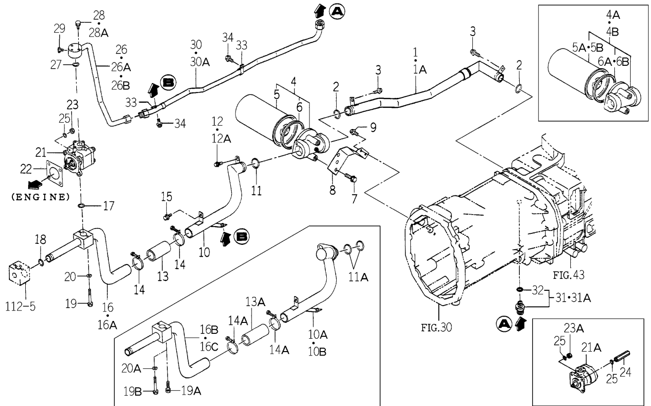
FIG.103 HYD. SYSTEM (MAIN)(1/2) (H TYPE EXCEPT H3-TG5390E4-No.1-774)
