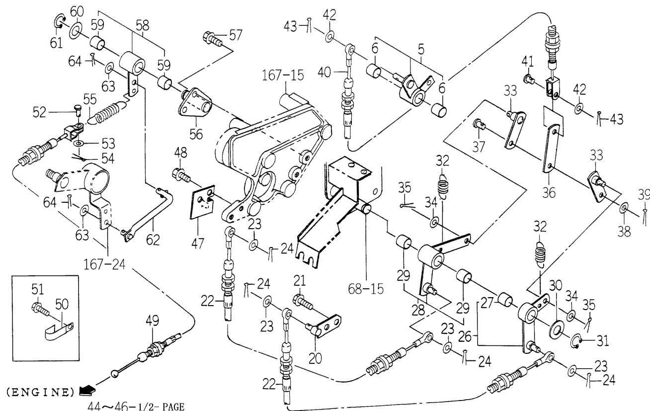
FIG.170 CRUISE CONTROL SYSTEM(2/2) (H TYPE EXCEPT H3)
