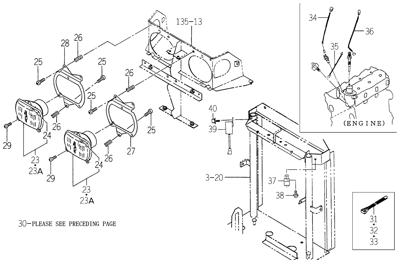
FIG.174 ELC. SYSTEM (FRONT) (E6 TYPE)(2/2)
