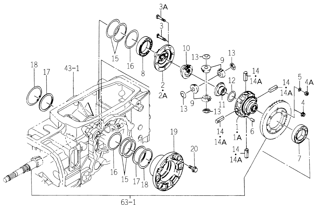
FIG. 64 DIFFERENTIAL GEAR SYSTEM
