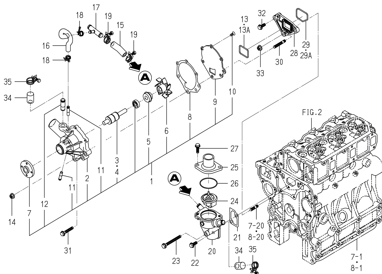
FIG. 21 WATER PUMP
