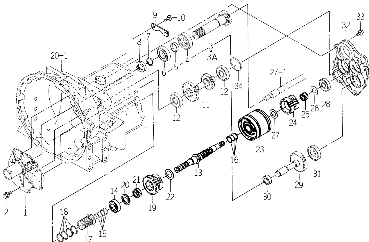
FIG. 24 GEAR (REVERSE) SYSTEM (P,Q TYPE)
