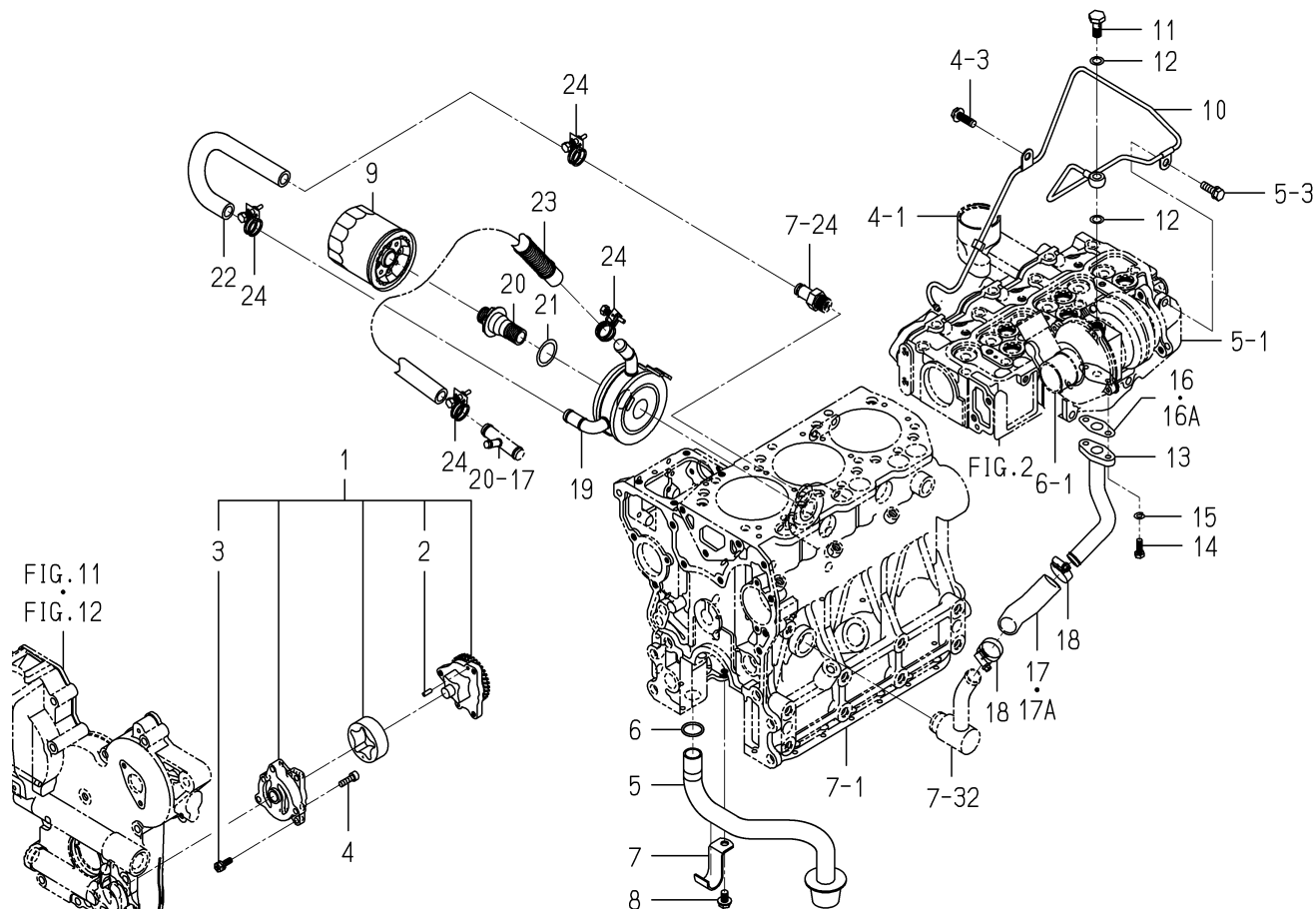
FIG. 19 OIL PUMP
