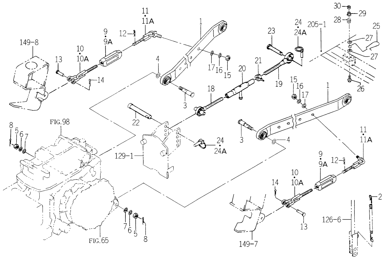
FIG.124 3P LINK SYSTEM (C TYPE)
