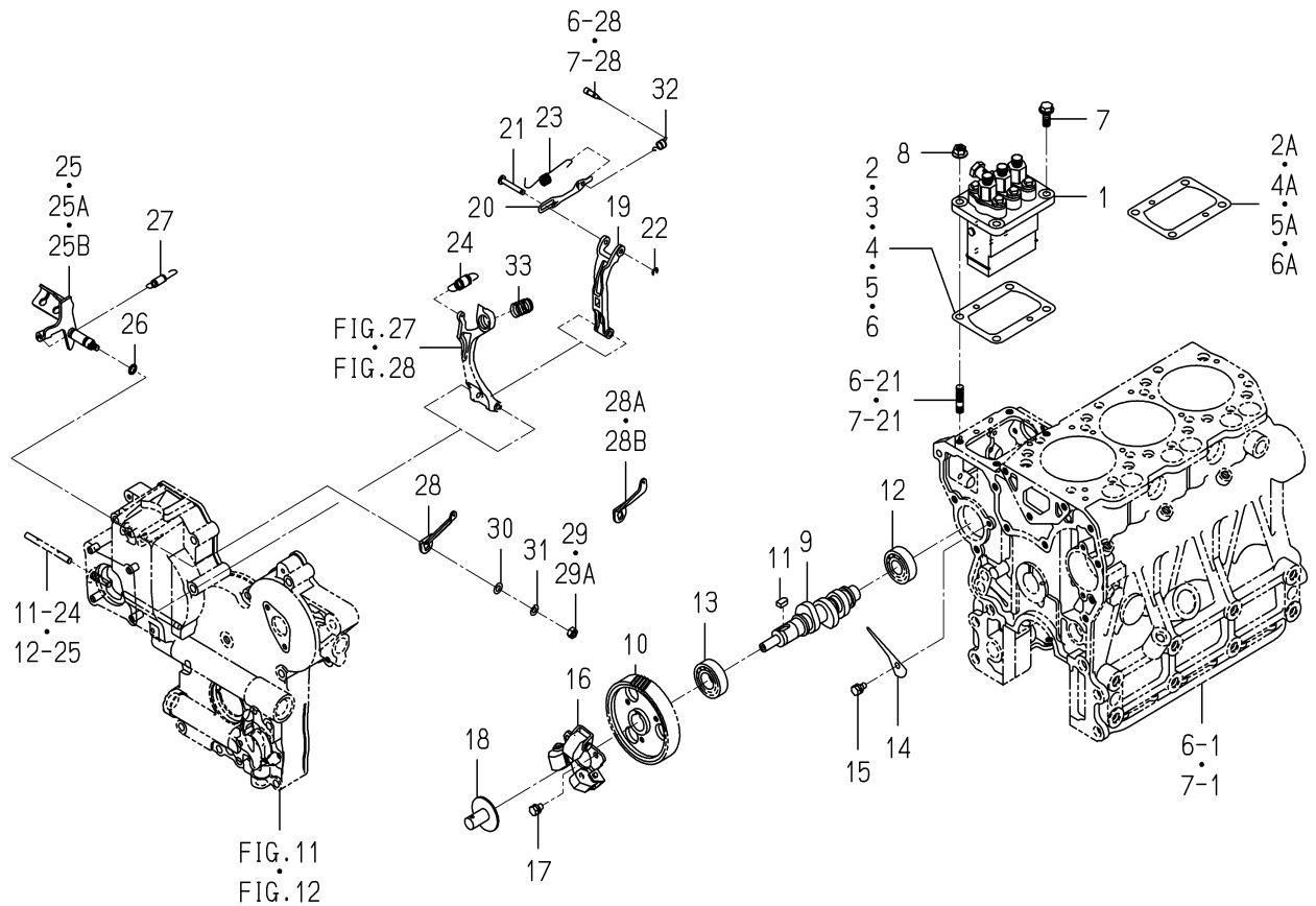
FIG. 25 INJECTION PUMP
