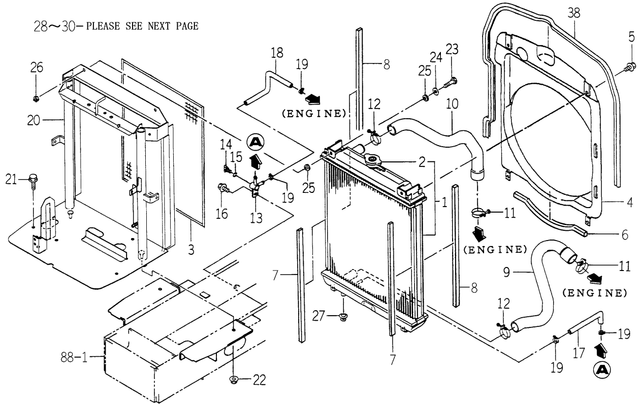
FIG. 4 RADIATOR SYSTEM(1/2) (HE6 TYPE-TG5390E6-No.878-)
