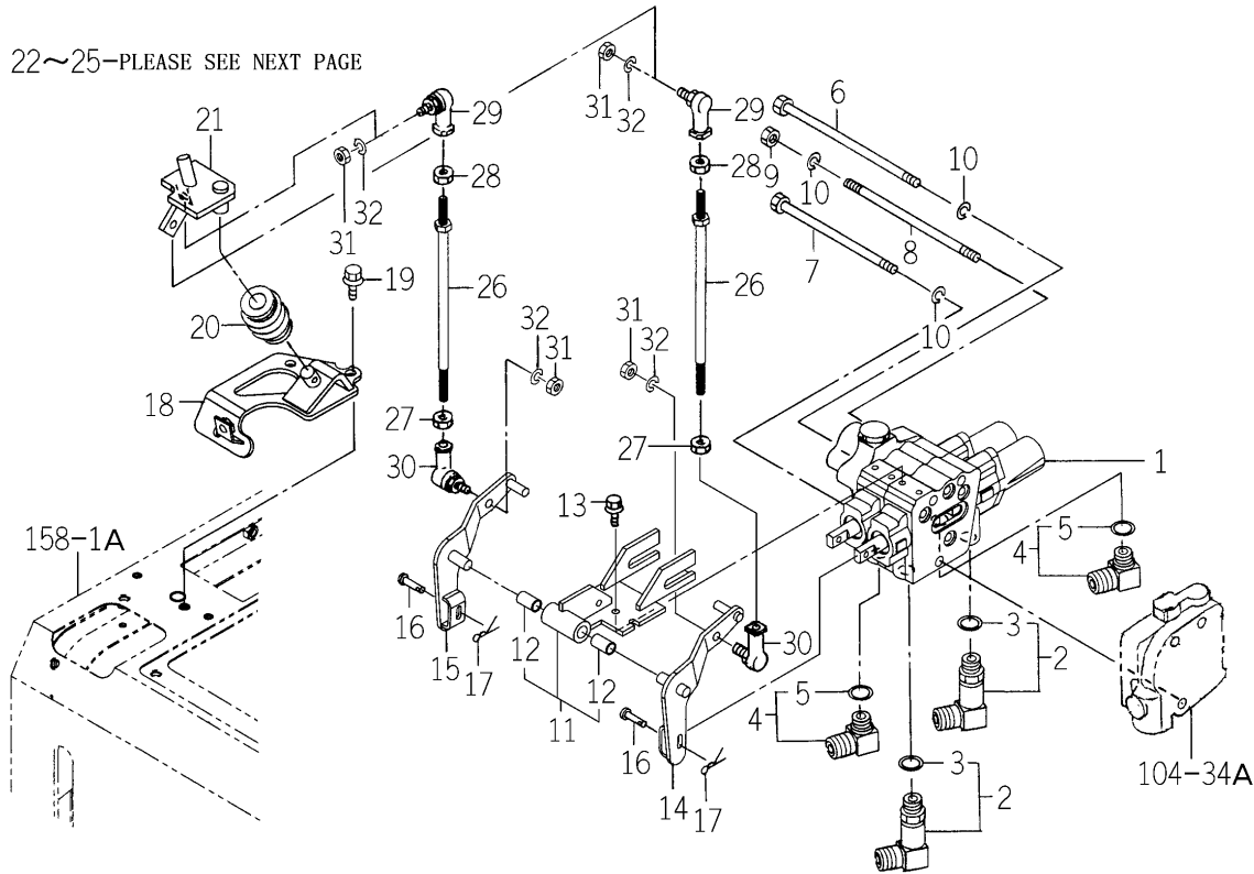
FIG.118 JOY STICK VALVE SET(1/3) (E6 TYPE-TG5330E6-No.567-/TG5390E6-No.882-)
