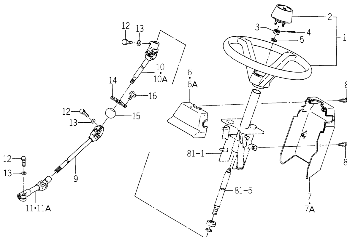
FIG. 80 WHEEL (STEERING) SYSTEM
