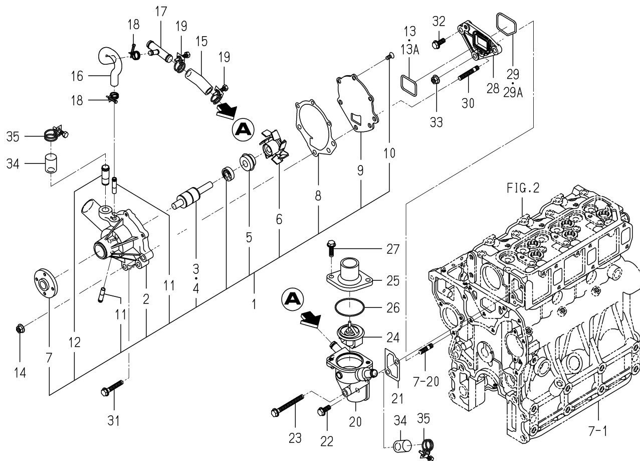
FIG. 20 WATER PUMP
