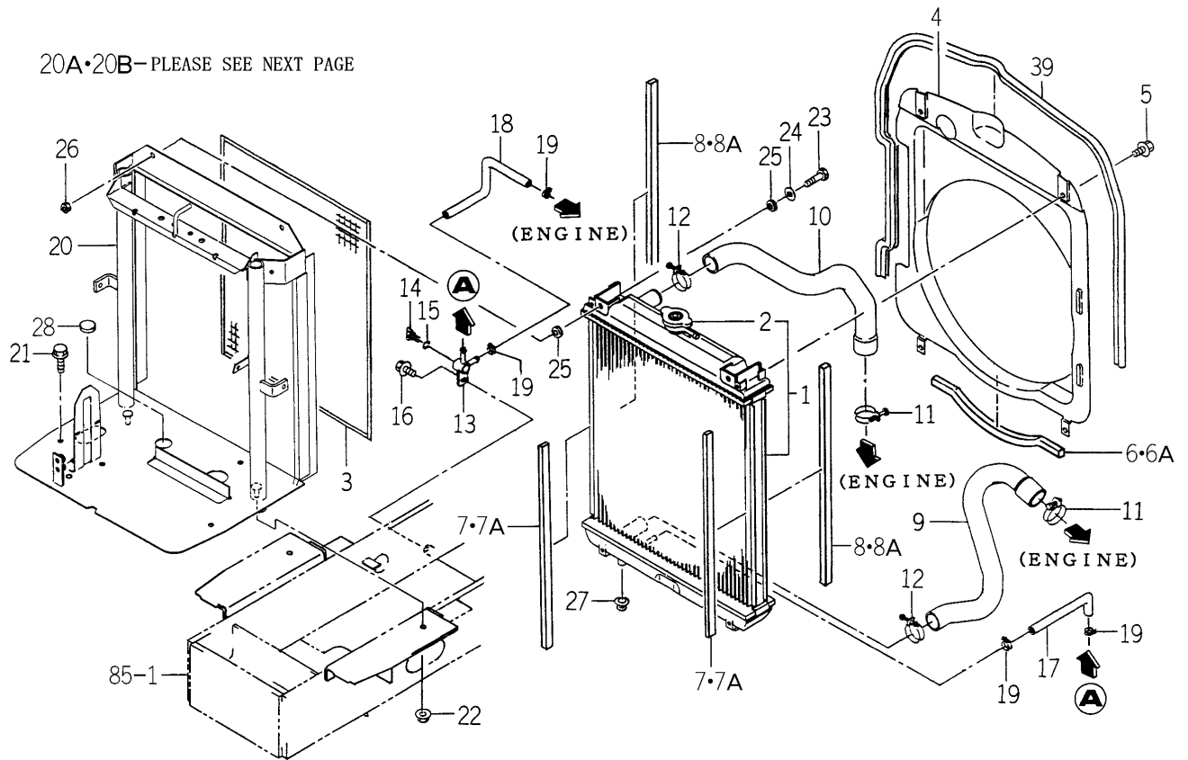
FIG. 1 RADIATOR SYSTEM (S TYPE)(1/2)
