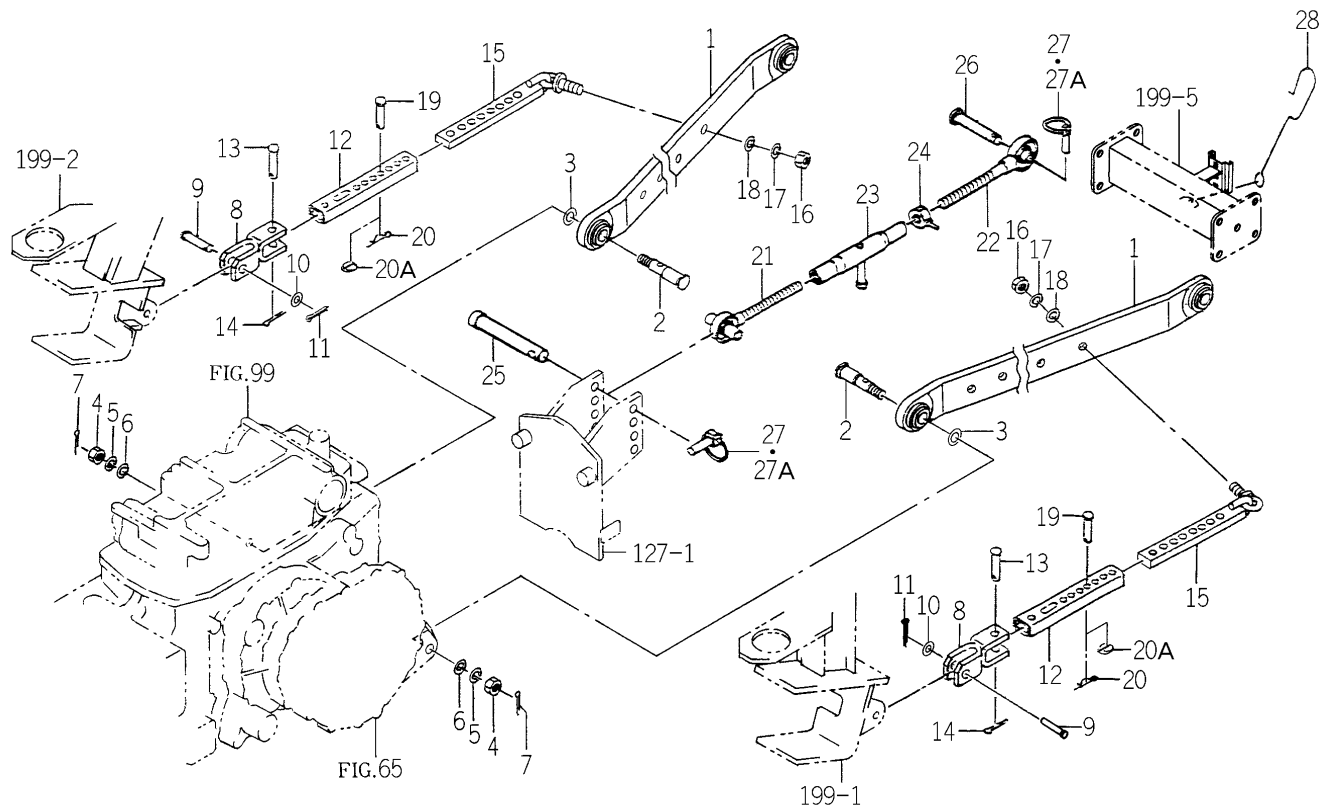
FIG.122 3P LINK SYSTEM (E6 TYPE)
