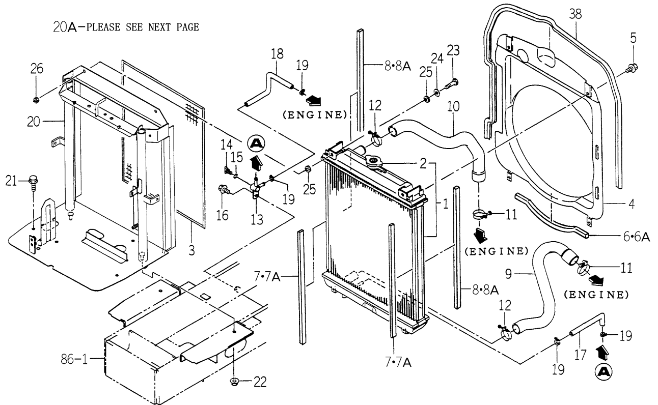
FIG. 2 RADIATOR SYSTEM(1/2) (HE4 TYPE-No.1-/HE6 TYPE-TG5390E6-No.1-877)
