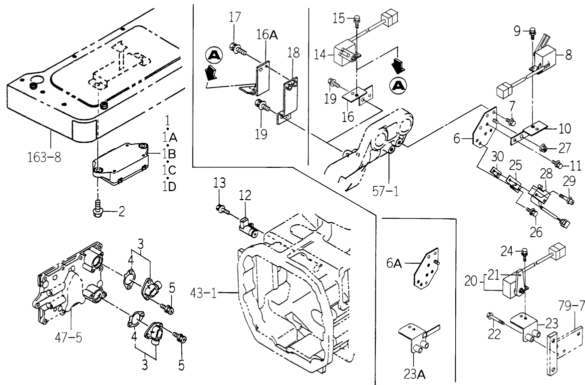
FIG.191 CONTROL SYSTEM(Q TYPE EXCEPT C-No.1-/QC TYPE-TG5330E4-No.1-81/ TG5390E4-No.1-270)
