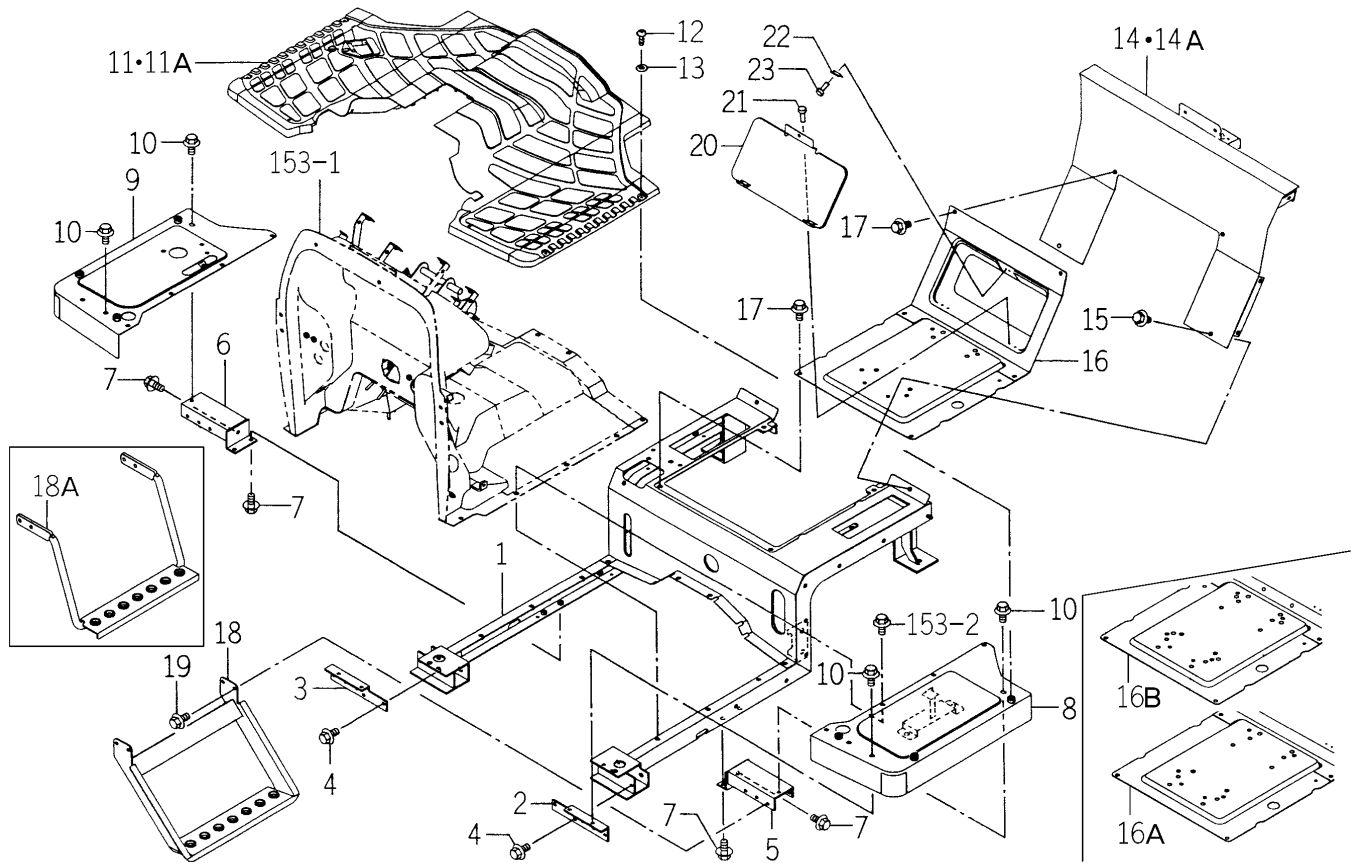
FIG.163 FLOOR (REAR) SYSTEM (Q TYPE EXCEPT C)
