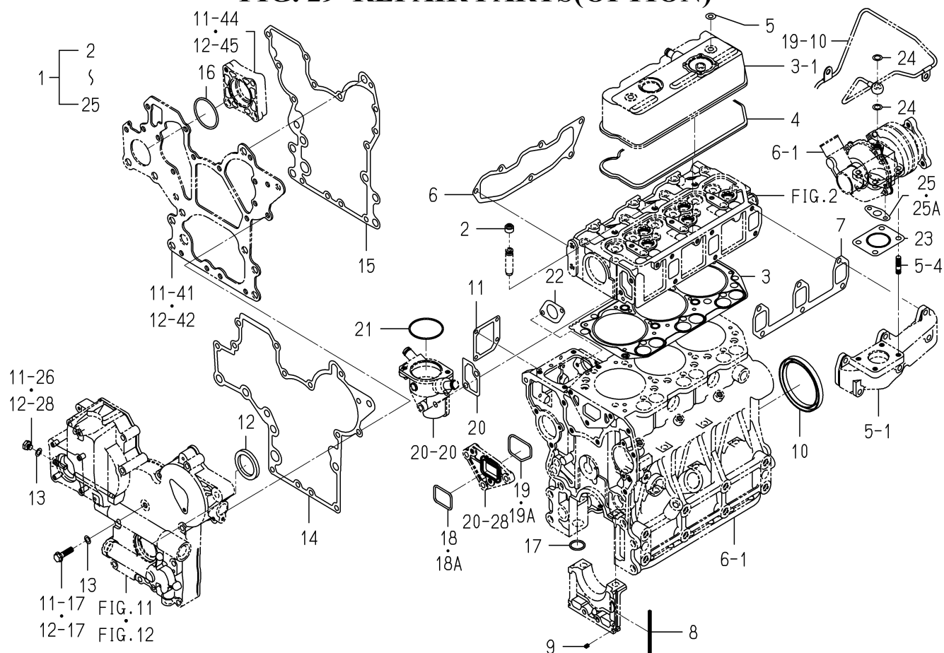
FIG. 29 REPAIR PARTS(OPTION)
