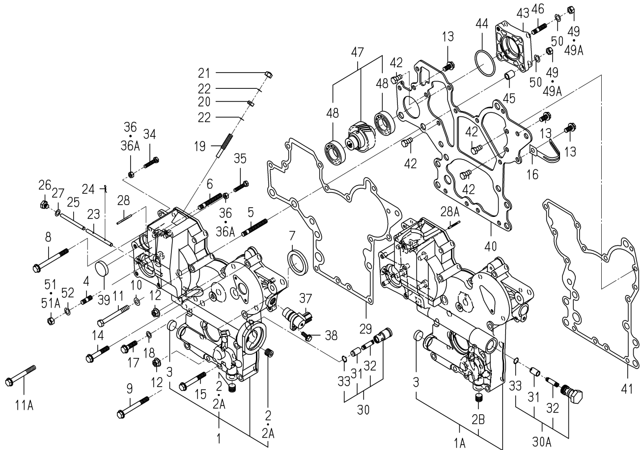
FIG. 11 TIMING GEAR CASE
