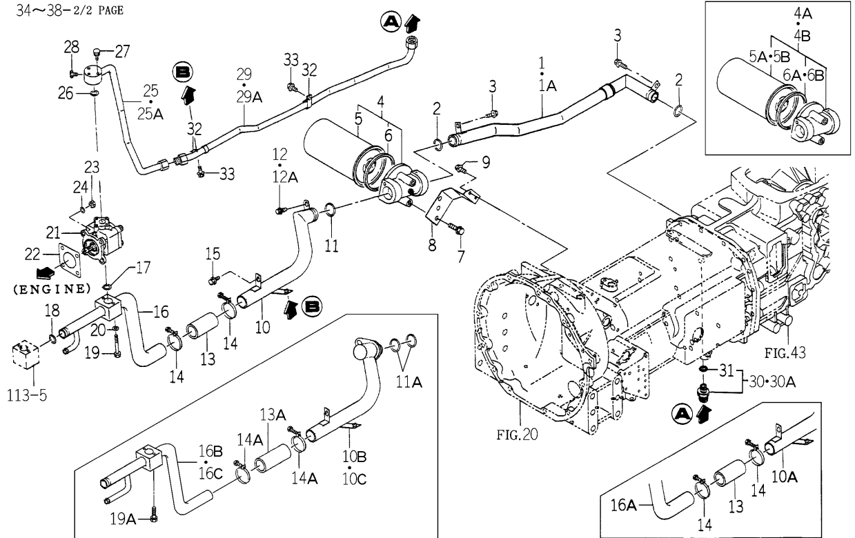
FIG.104 HYD. SYSTEM (MAIN) (P TYPE-No.1-/(1/2) Q TYPE-TG5330E4-No.1-443/ TG5390E4-No.1-777)
