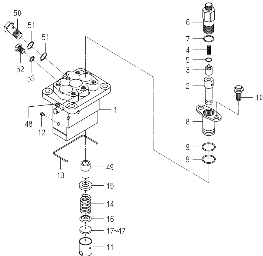
FIG. 34 COMPONENT PARTS FOR 6215-600-104-20 ON Fig.25
