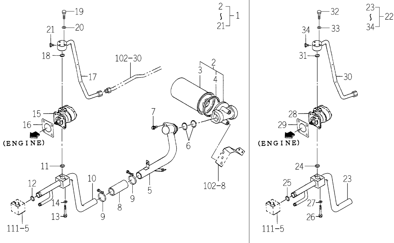
FIG.110 SUCTION SYSTEM (EXCEPT H TYPE-REPAIR)
