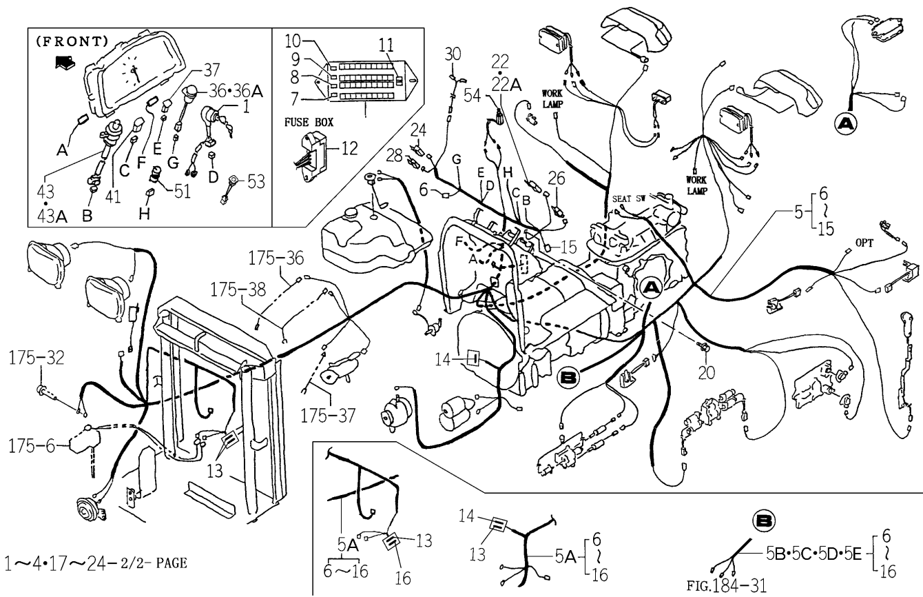
FIG.178 ELC. SYSTEM (MAIN) (Q TYPE)(1/2)
