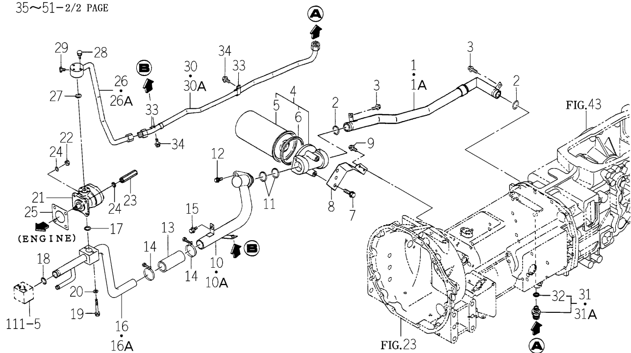
FIG.106 HYD. SYSTEM (MAIN)(1/2) (S TYPE-TG5330E4-No.440-/TG5390E4-No.776-)
