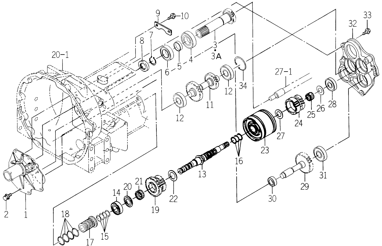
FIG. 24 GEAR (REVERSE) SYSTEM (P,Q TYPE)
