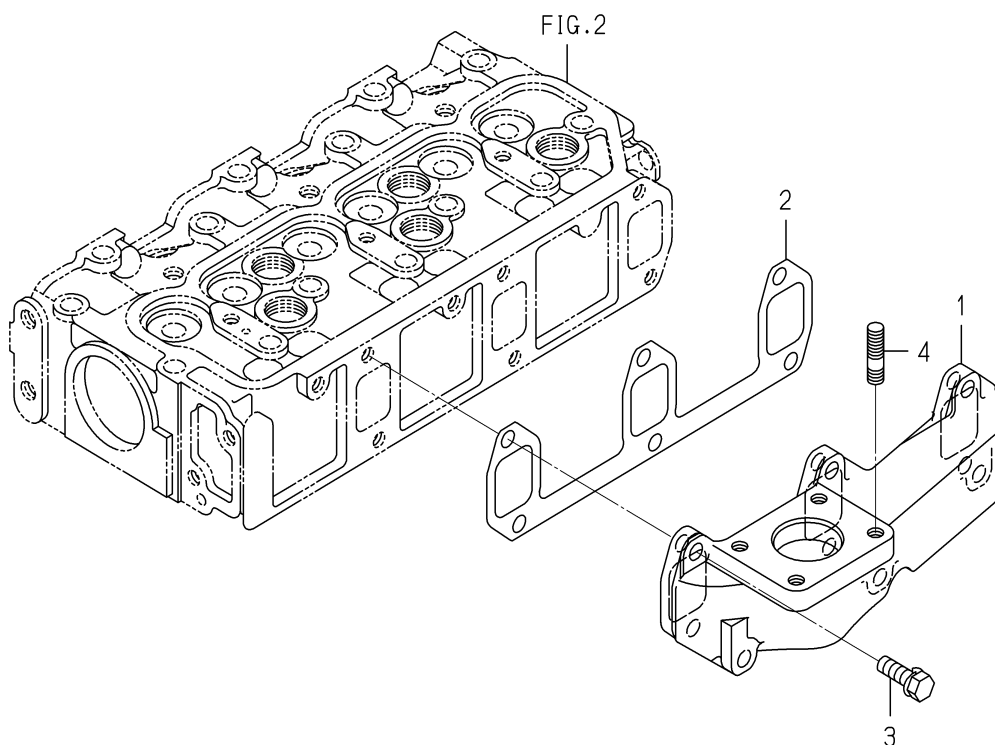
FIG. 5 EXHAUST MANIFOLD
