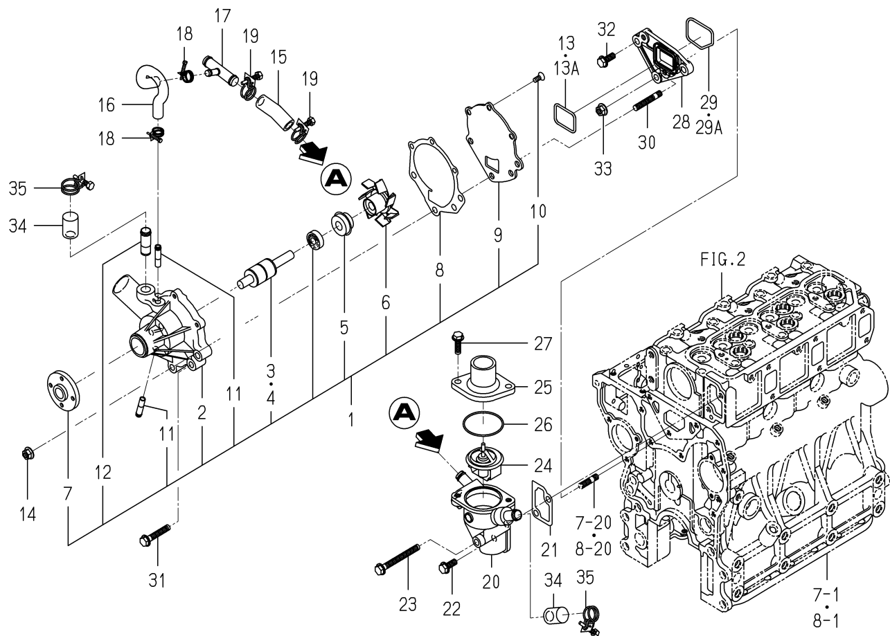
FIG. 21 WATER PUMP
