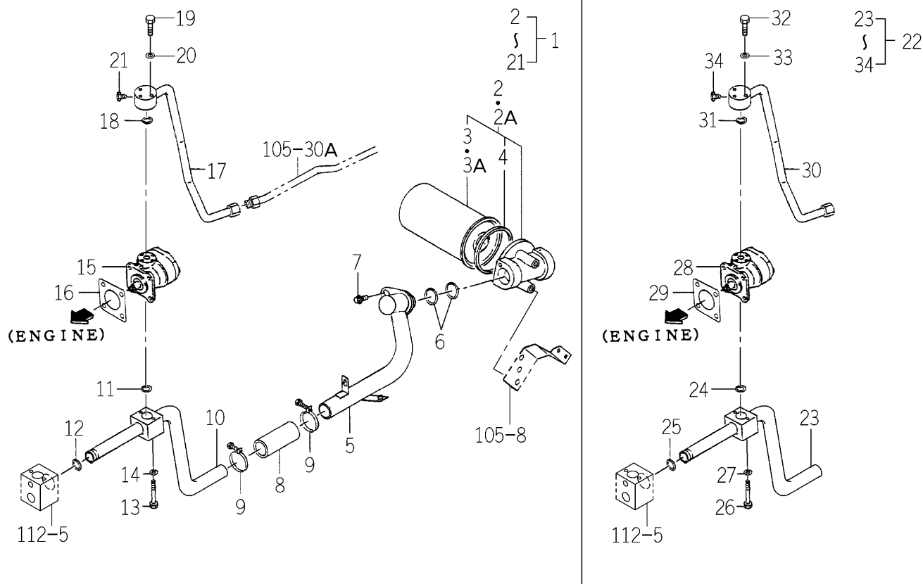
FIG.245 SUCTION SYSTEM (H TYPE-REPAIR)
