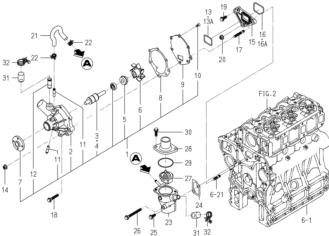
FIG. 20 WATER PUMP
