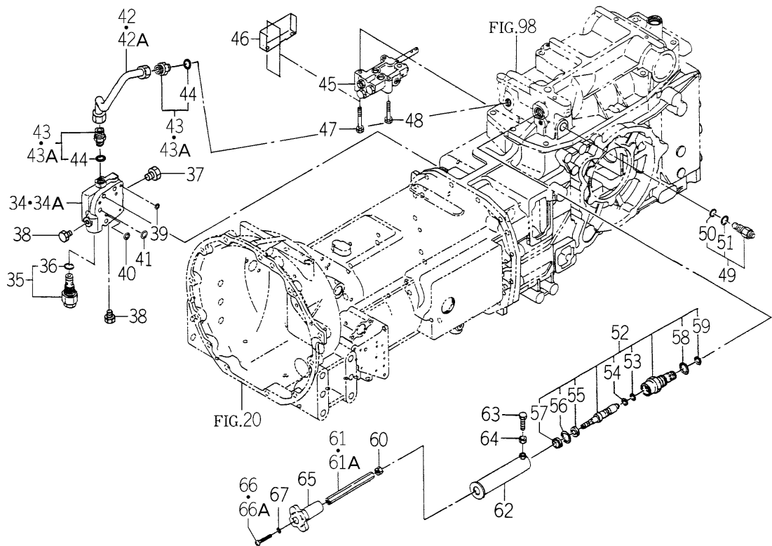
FIG.104 HYD. SYSTEM (MAIN) (P TYPE-No.1-/(2/2) Q TYPE-TG5330E4-No.1-443/ TG5390E4-No.1-777)
