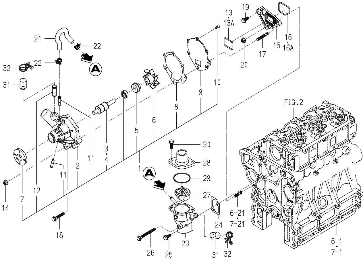
FIG. 22 WATER PUMP
