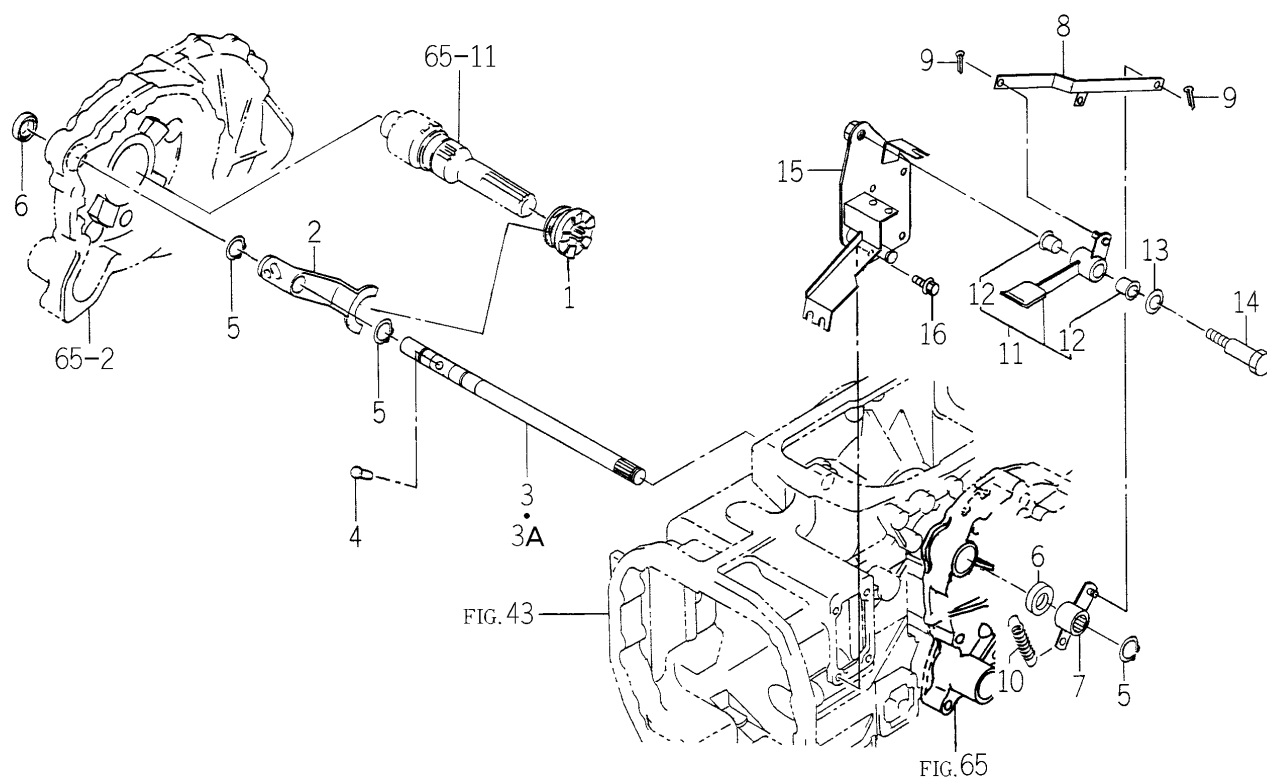
FIG. 68 DIFF-LOCK SYSTEM (H TYPE)
