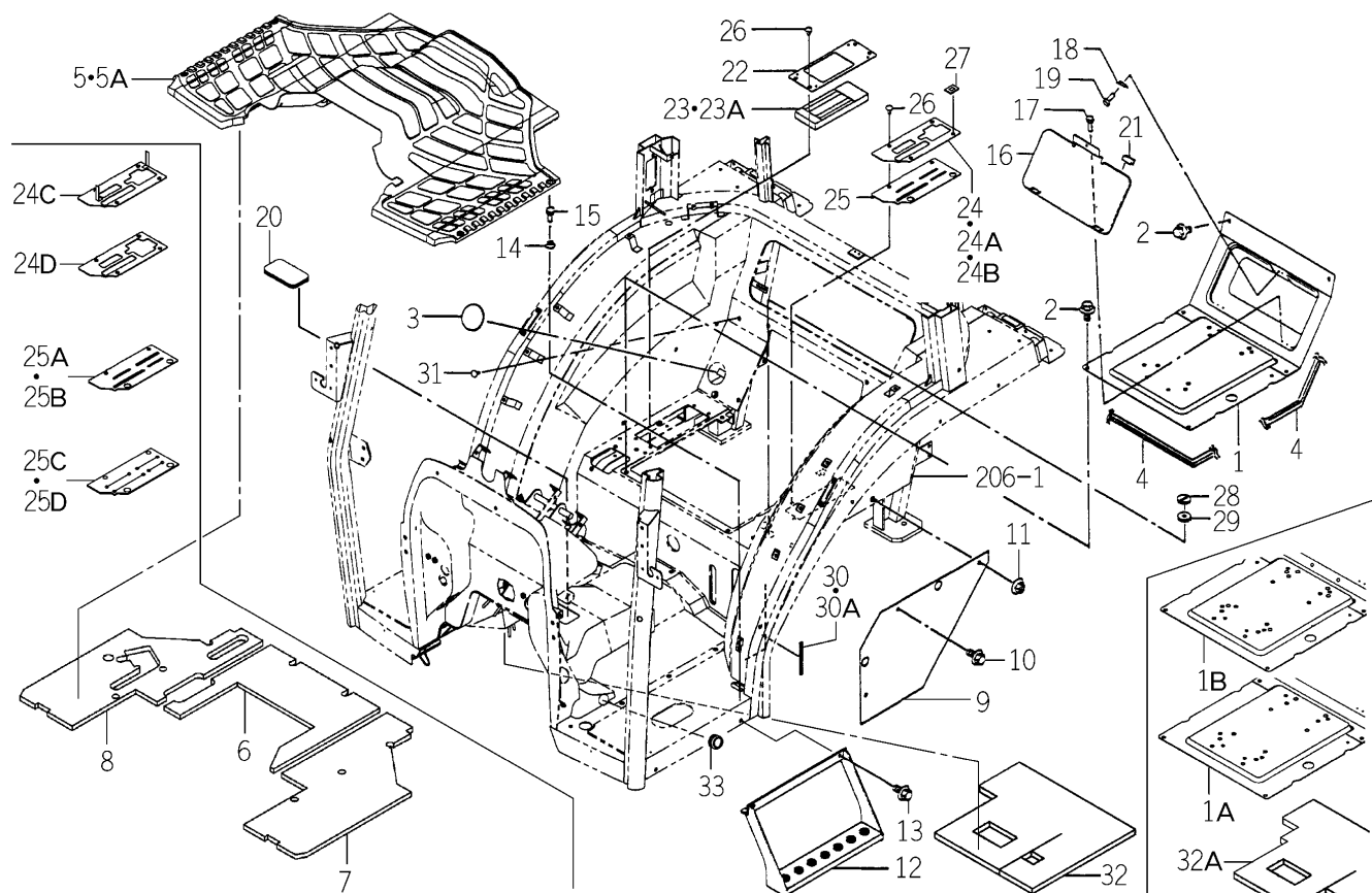
FIG.162 FLOOR (REAR) SYSTEM (HC TYPE)
