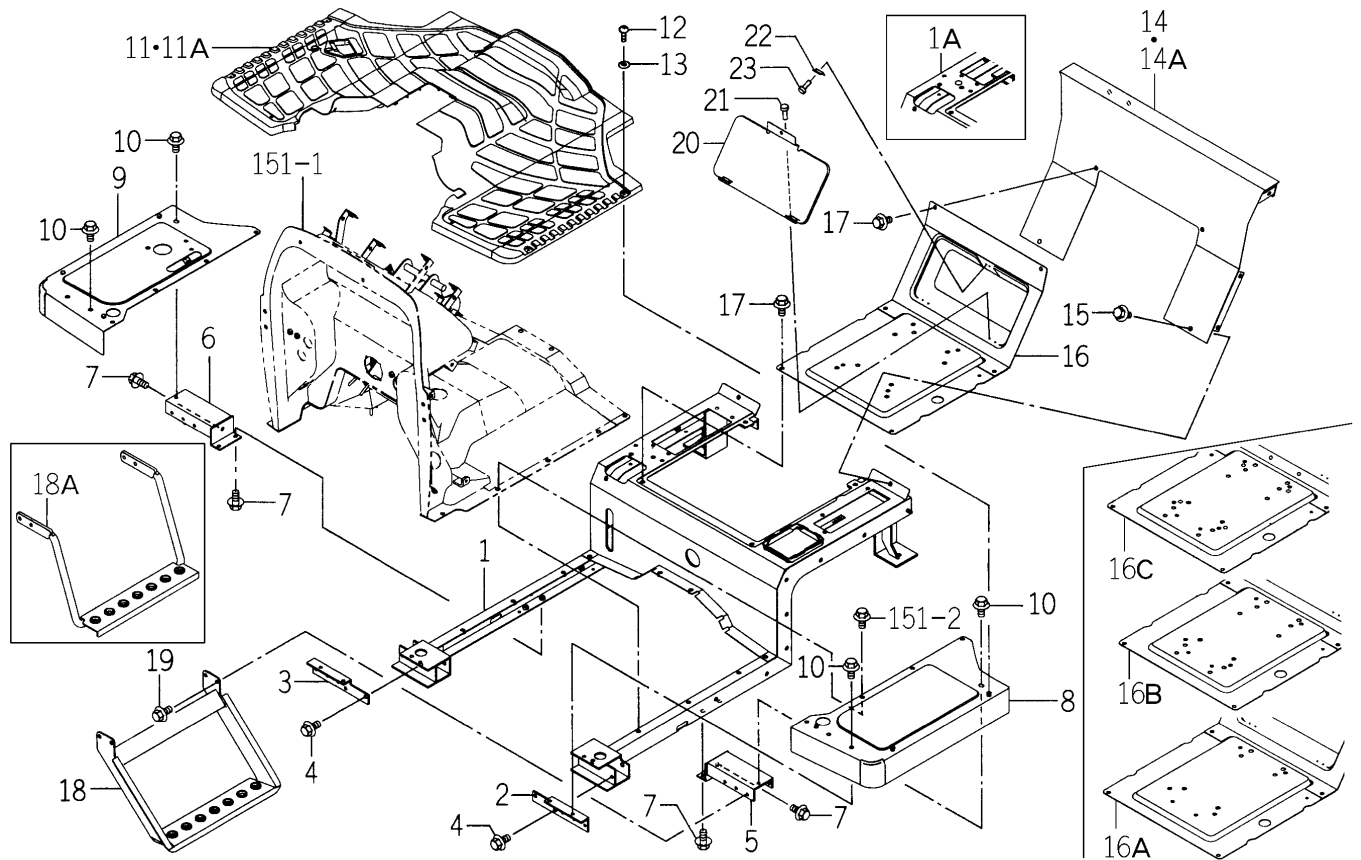
FIG.158 FLOOR (REAR) SYSTEM (P TYPE)
