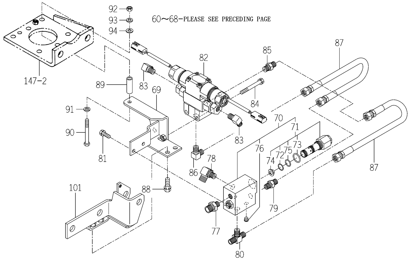
FIG.116 HYD. SYSTEM (SUB) (H3 TYPE)(3/4)
