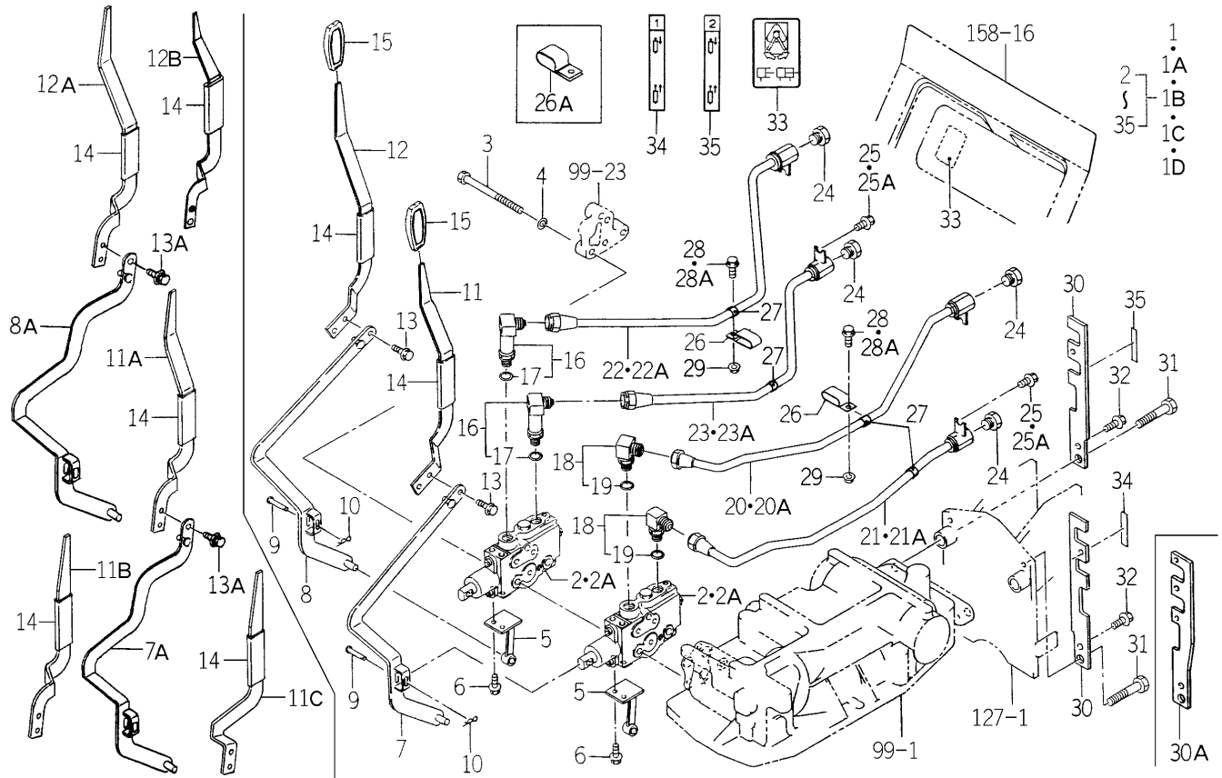
FIG.119 VALVE (REMOTE/2R) SET (E6 TYPE)
