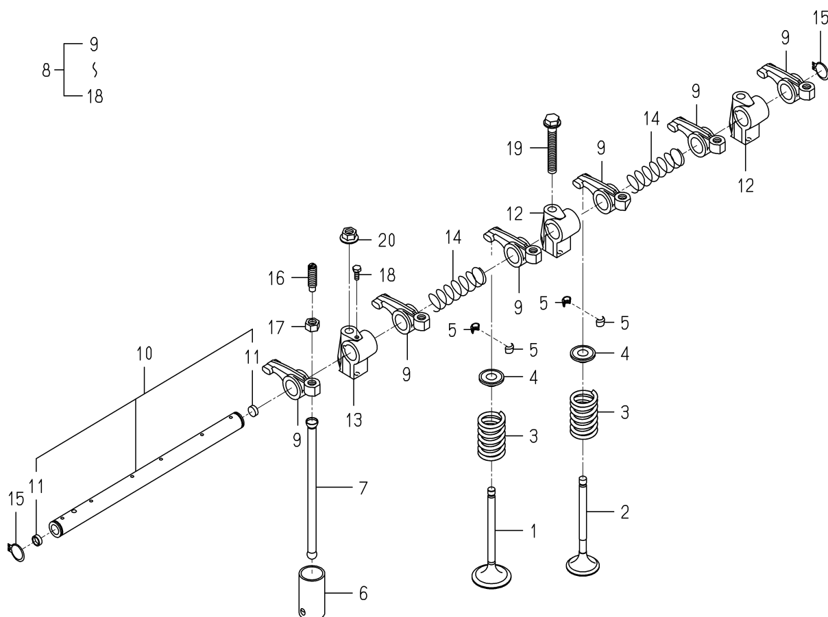
FIG. 14 VALVE
