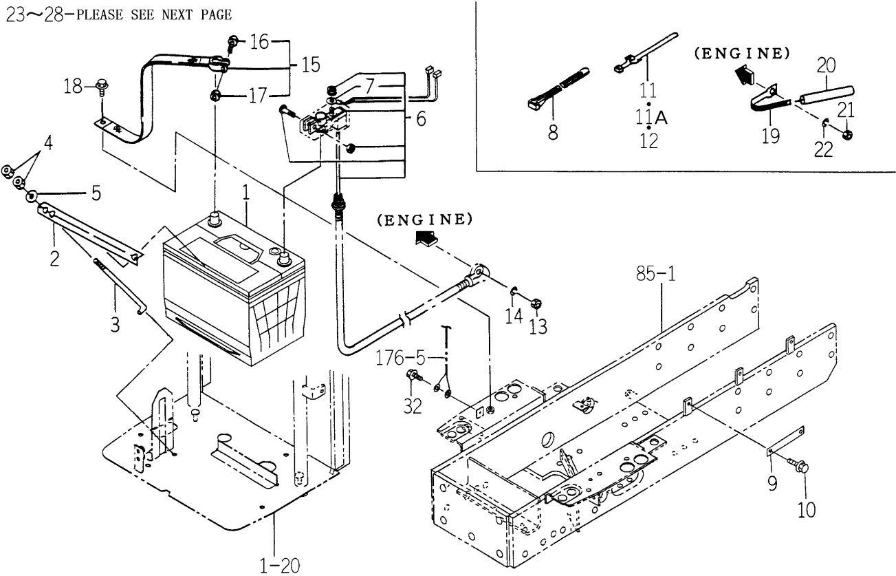
FIG.172 ELC. SYSTEM (FRONT) (S TYPE)(1/2)
