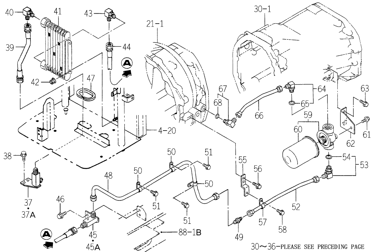
FIG.114 HYD. SYSTEM (SUB)(2/3) (HE6 TYPE-TG5390E6-No.878-)
