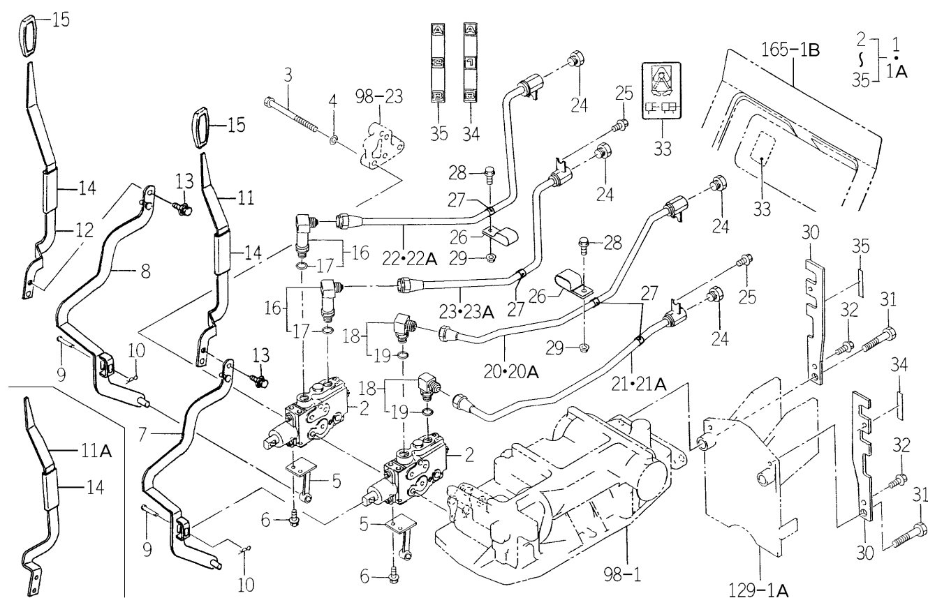
FIG.248 VALVE (REMOTE/2R) SET (C TYPE-OPTION)
