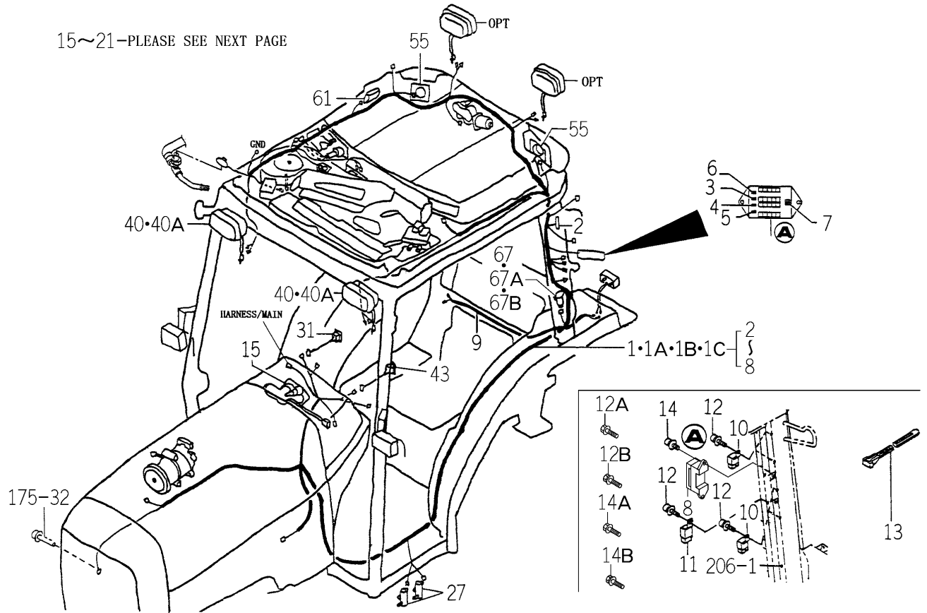
FIG.188 ELC. SYSTEM (C TYPE)(1/3)
