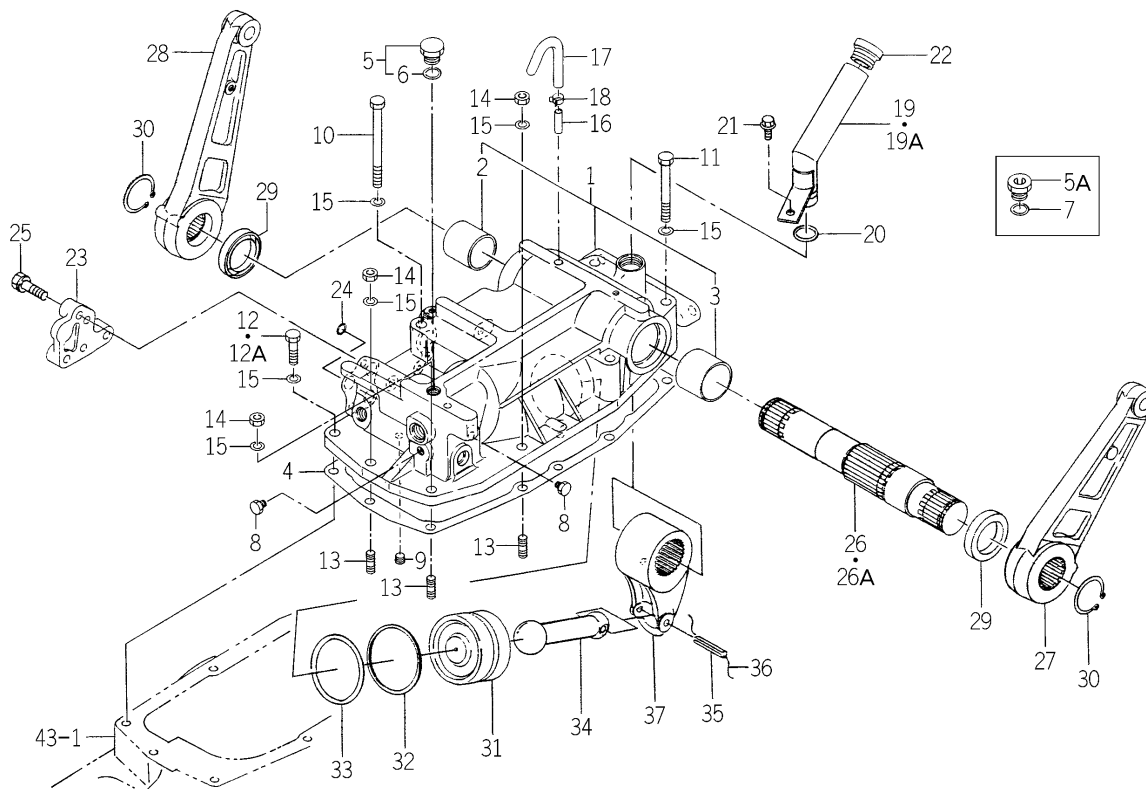
FIG. 98 CYLINDER CASE SYSTEM (EXCEPT W,A TYPE-No.1-/ A TYPE-TG5330E4-No.1-159/TG5390E4-No.1-519)
