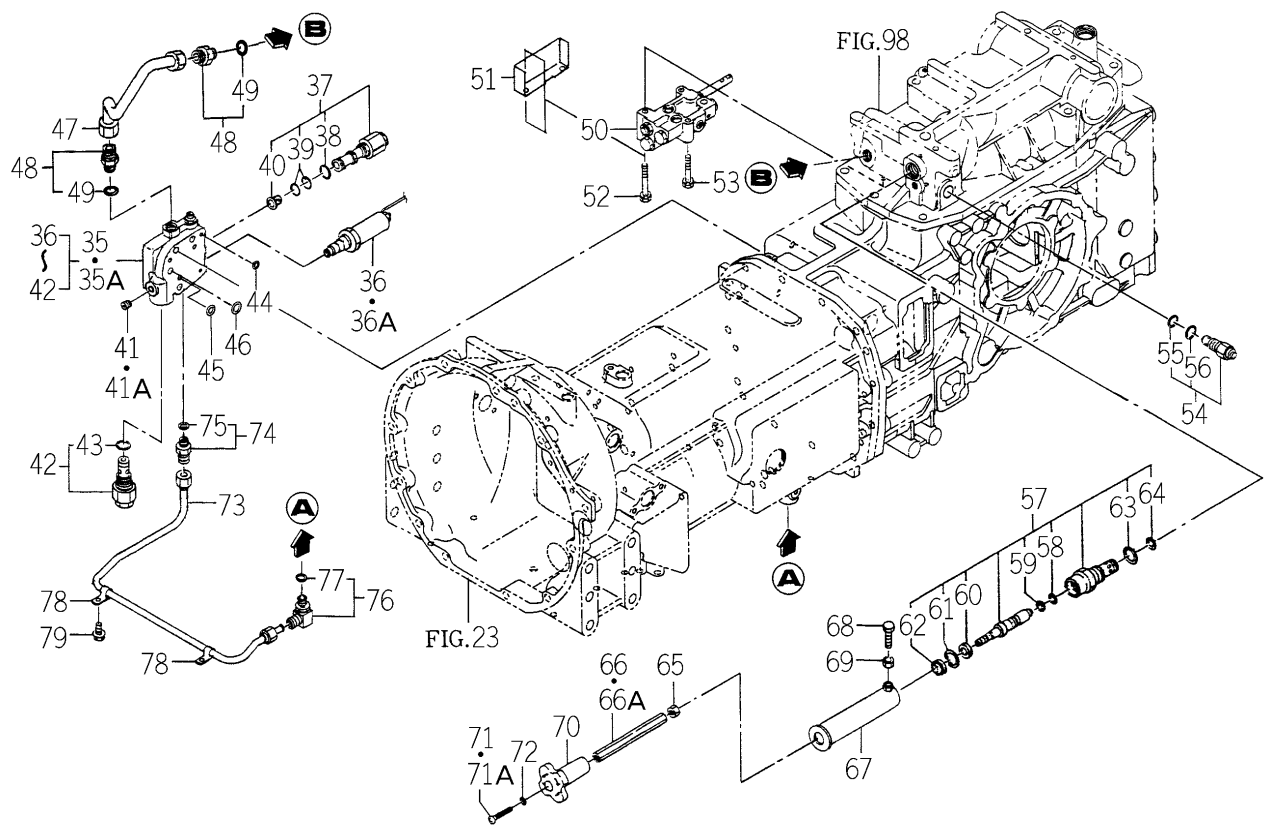
FIG.102 HYD. SYSTEM (MAIN)(2/2) (S TYPE-TG5330E4-No.1-439/TG5390E4-No.1-775)
