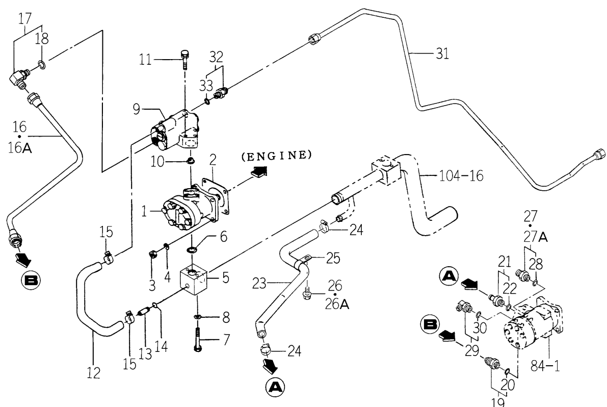
FIG.113 HYD. SYSTEM (SUB) (P TYPE)(1/2)
