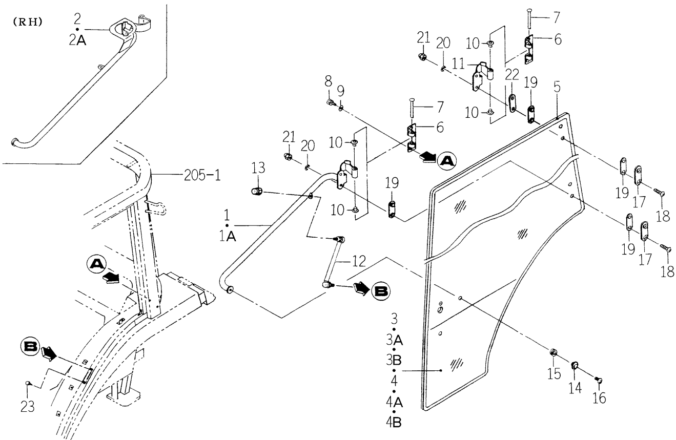
FIG.210 DOOR SYSTEM (C TYPE)
