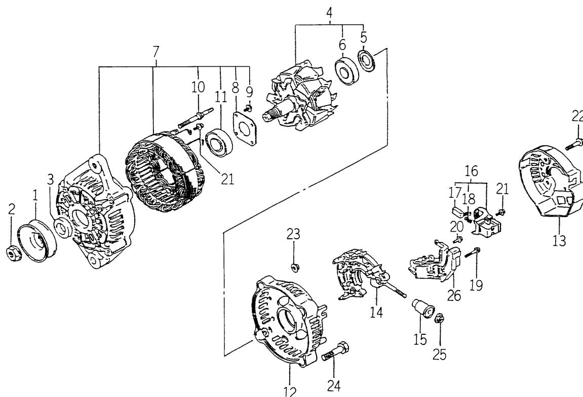
FIG.279 COMPONENT PARTS FOR 6281-200-015-00 ON Fig.254,255
