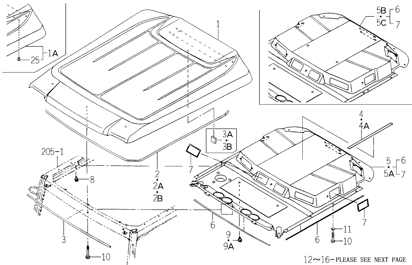
FIG.204 ROOF SYSTEM (C TYPE)(1/2)
