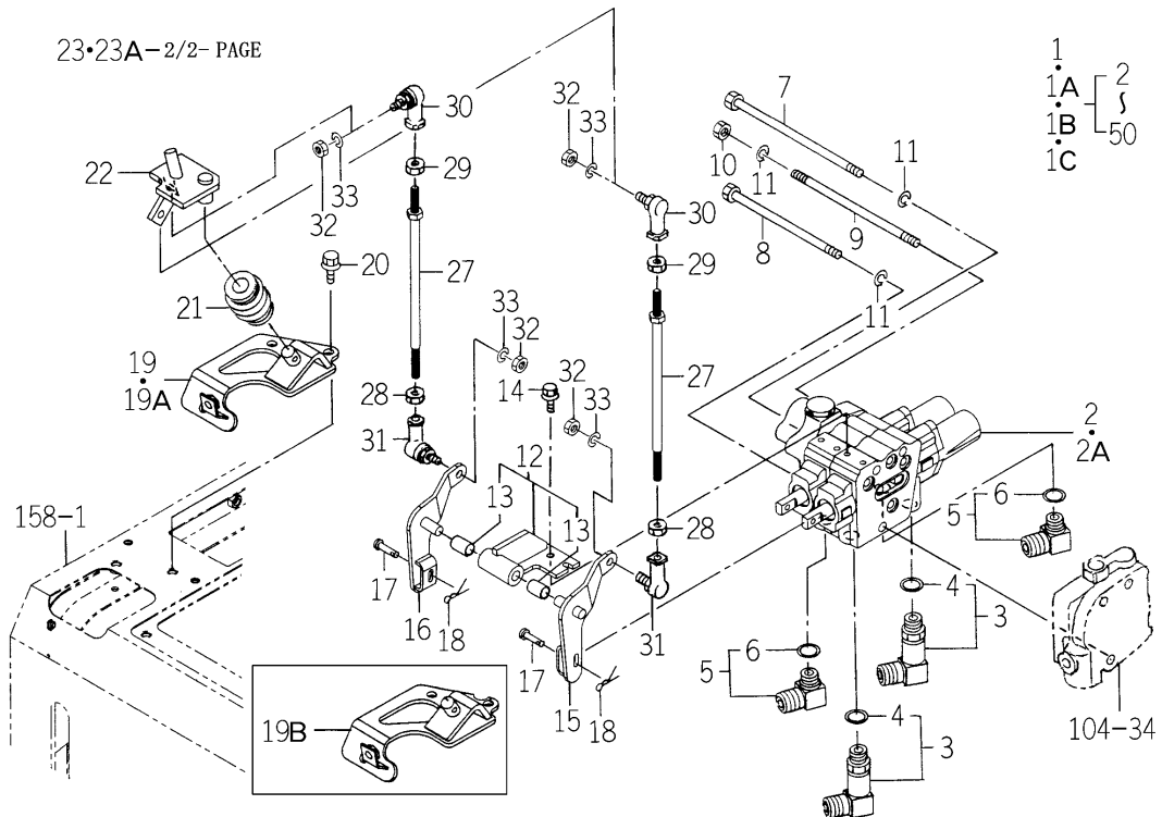
FIG.117 JOY STICK VALVE SET(E6 TYPE-STD-(1/2) TG5330E6-No.1-566/TG5390E6-No.1-881/ E4 TYPE EXCEPT A-OPTION-No.1-)
