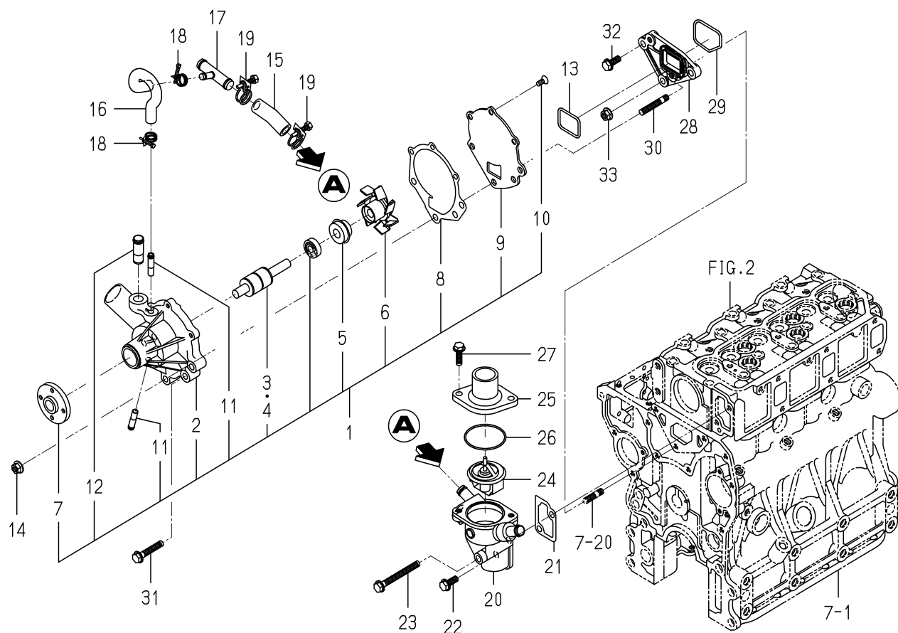
FIG. 20 WATER PUMP
