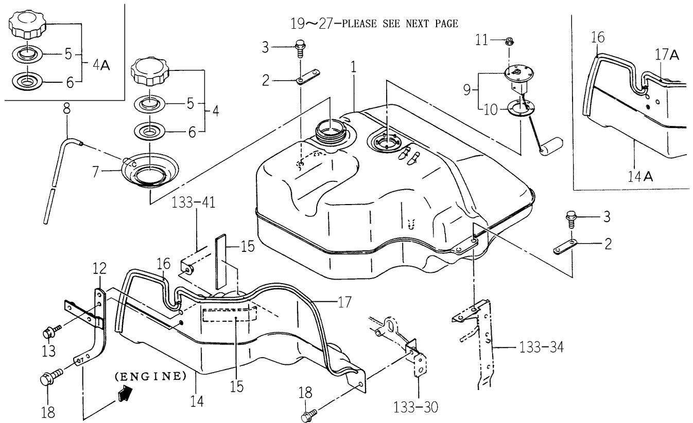
FIG. 12 TANK (FUEL) SYSTEM (TG5390-E6 TYPE)(1/2)
