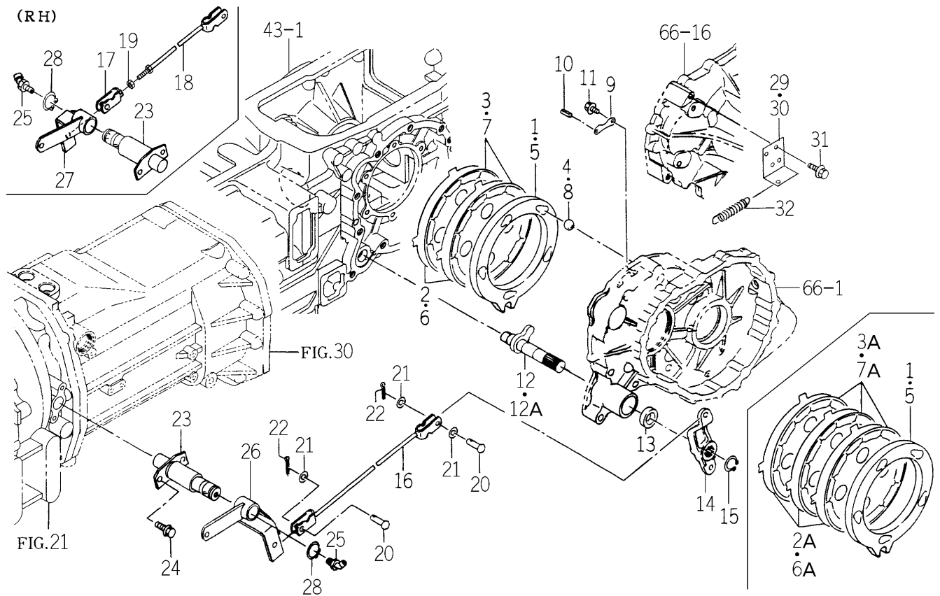
FIG. 71 BRAKE SYSTEM (H3 TYPE)
