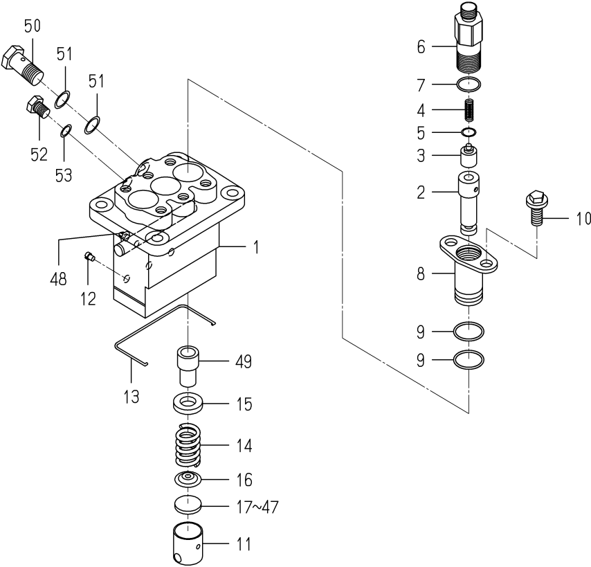
FIG. 32 COMPONENT PARTS FOR 6215-600-078-10 ON Fig.24
