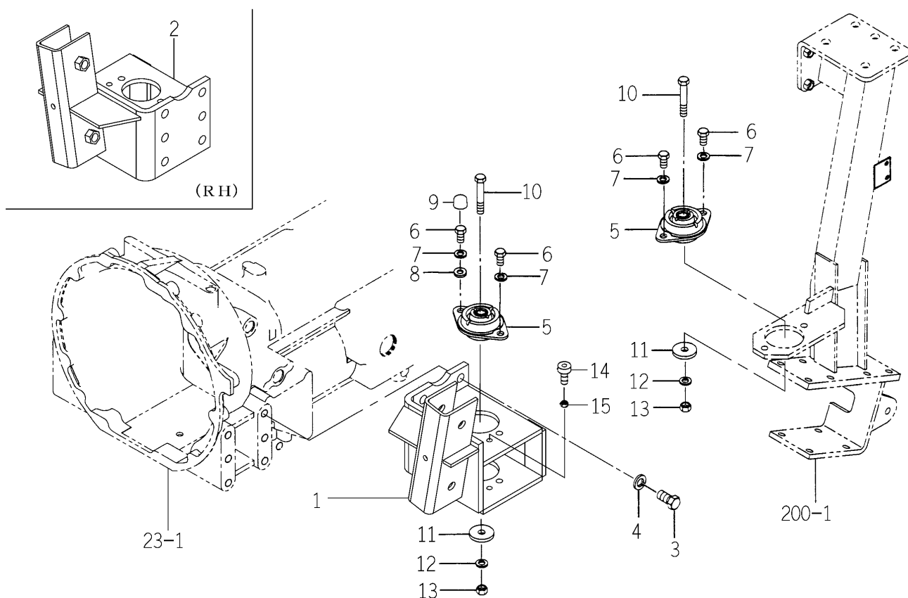
FIG.150 MOUNT SYSTEM (A TYPE)
