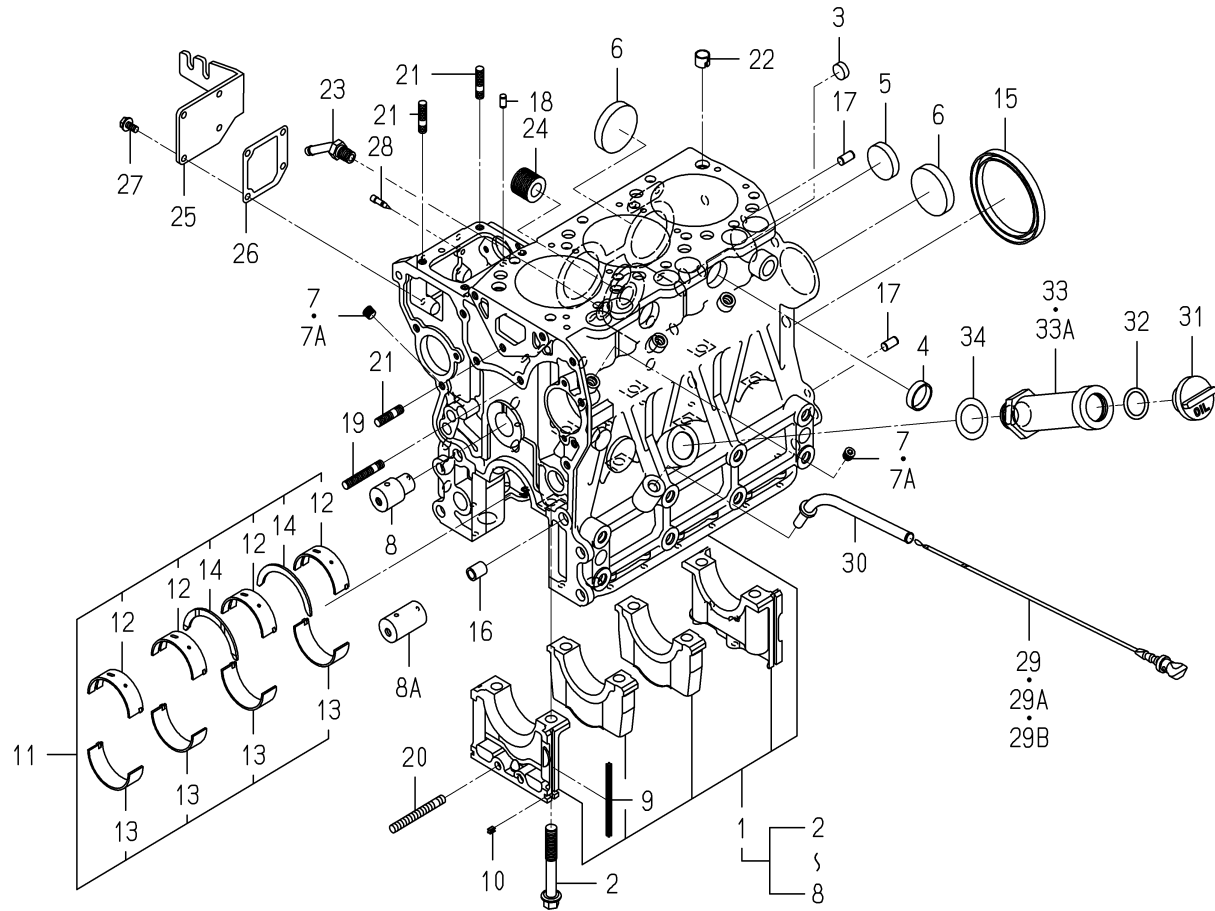
FIG. 7 CYLINDER BLOCK
