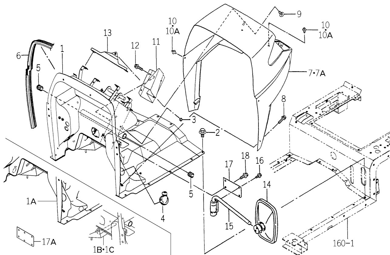
FIG.154 FLOOR (FRONT) SYSTEM (HE4 TYPE EXCEPT C)
