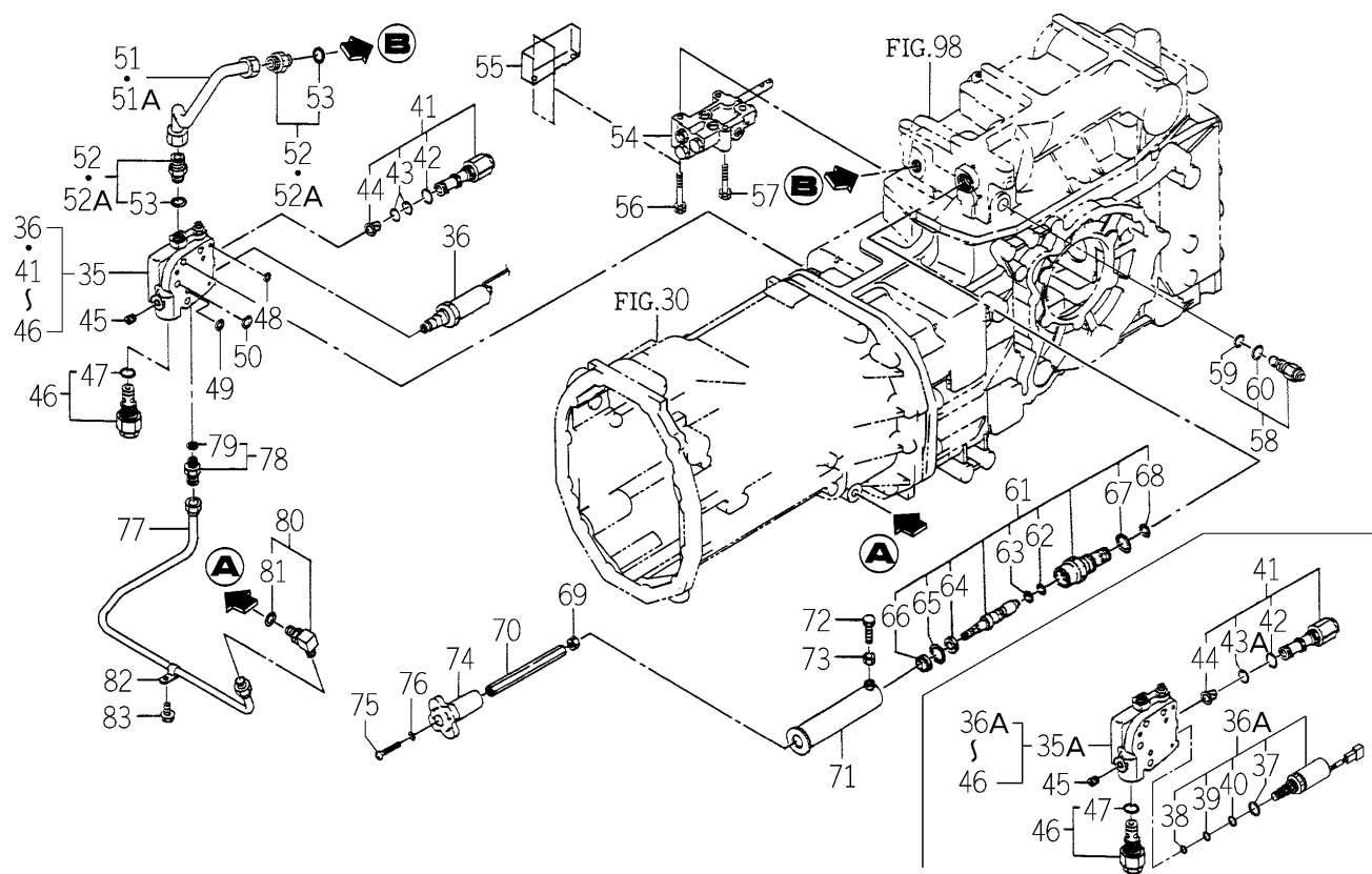
FIG.105 HYD. SYSTEM (MAIN)(2/2) (H TYPE EXCEPT H3-TG5390E4-No.775-)
