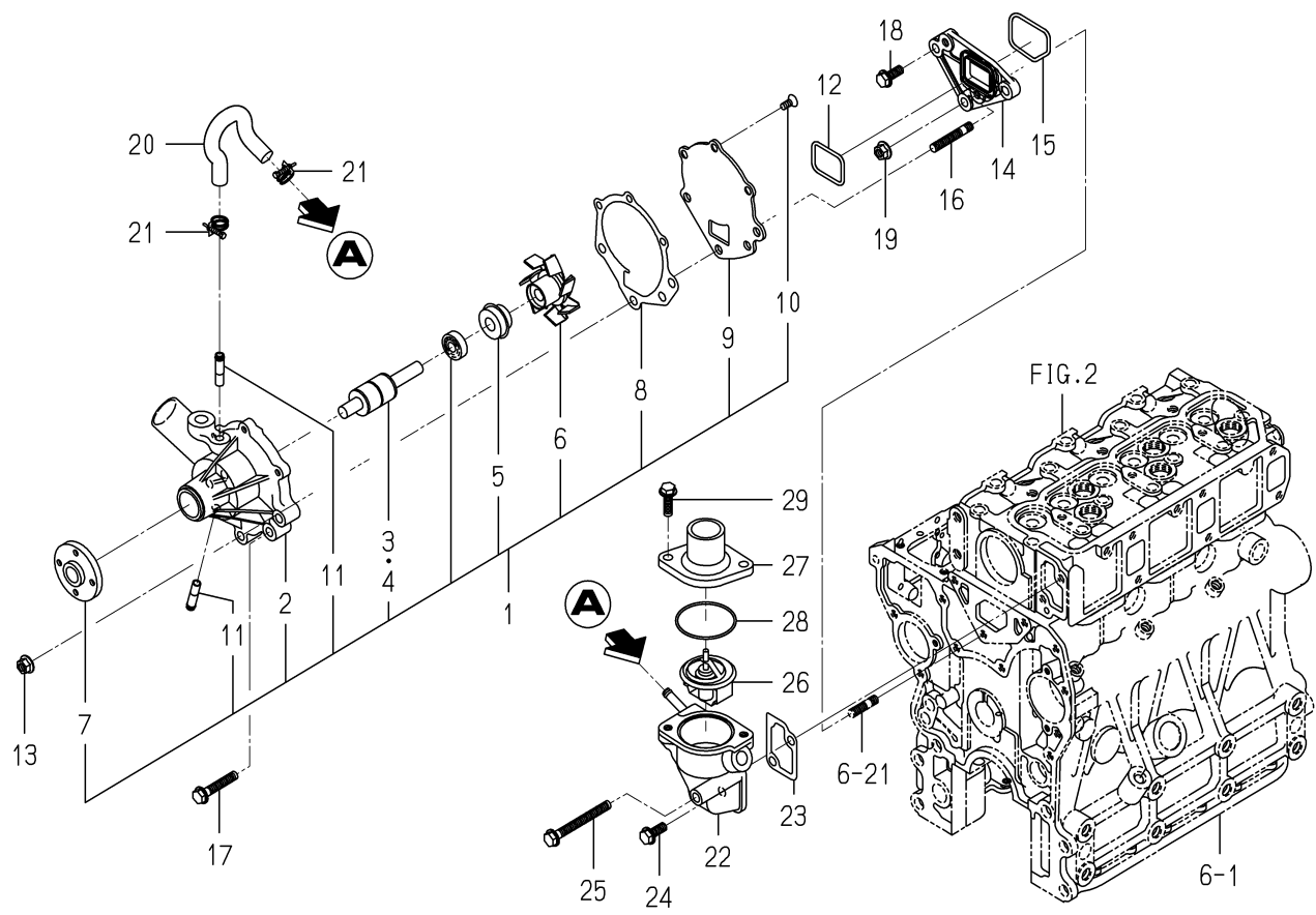
FIG. 19 WATER PUMP
