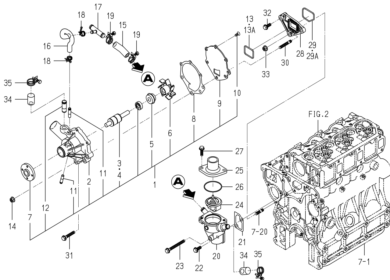
FIG. 20 WATER PUMP
