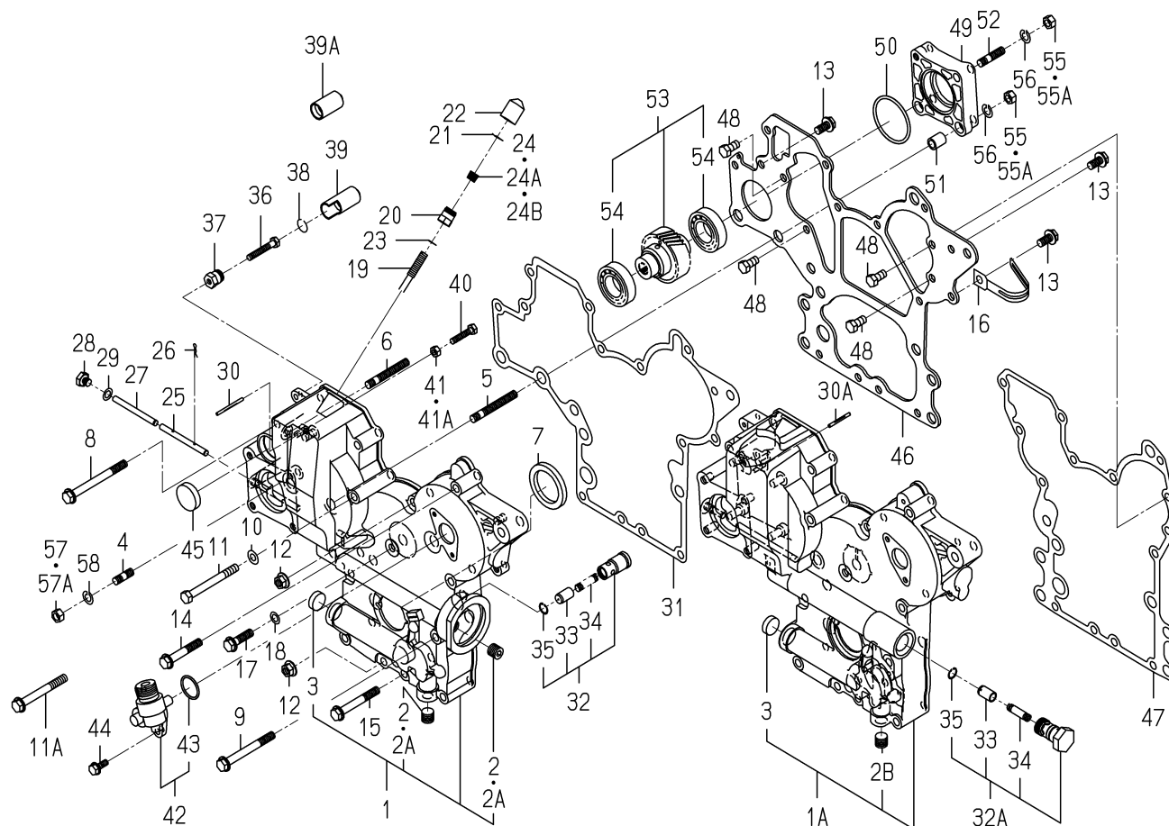
FIG. 12 TIMING GEAR CASE
