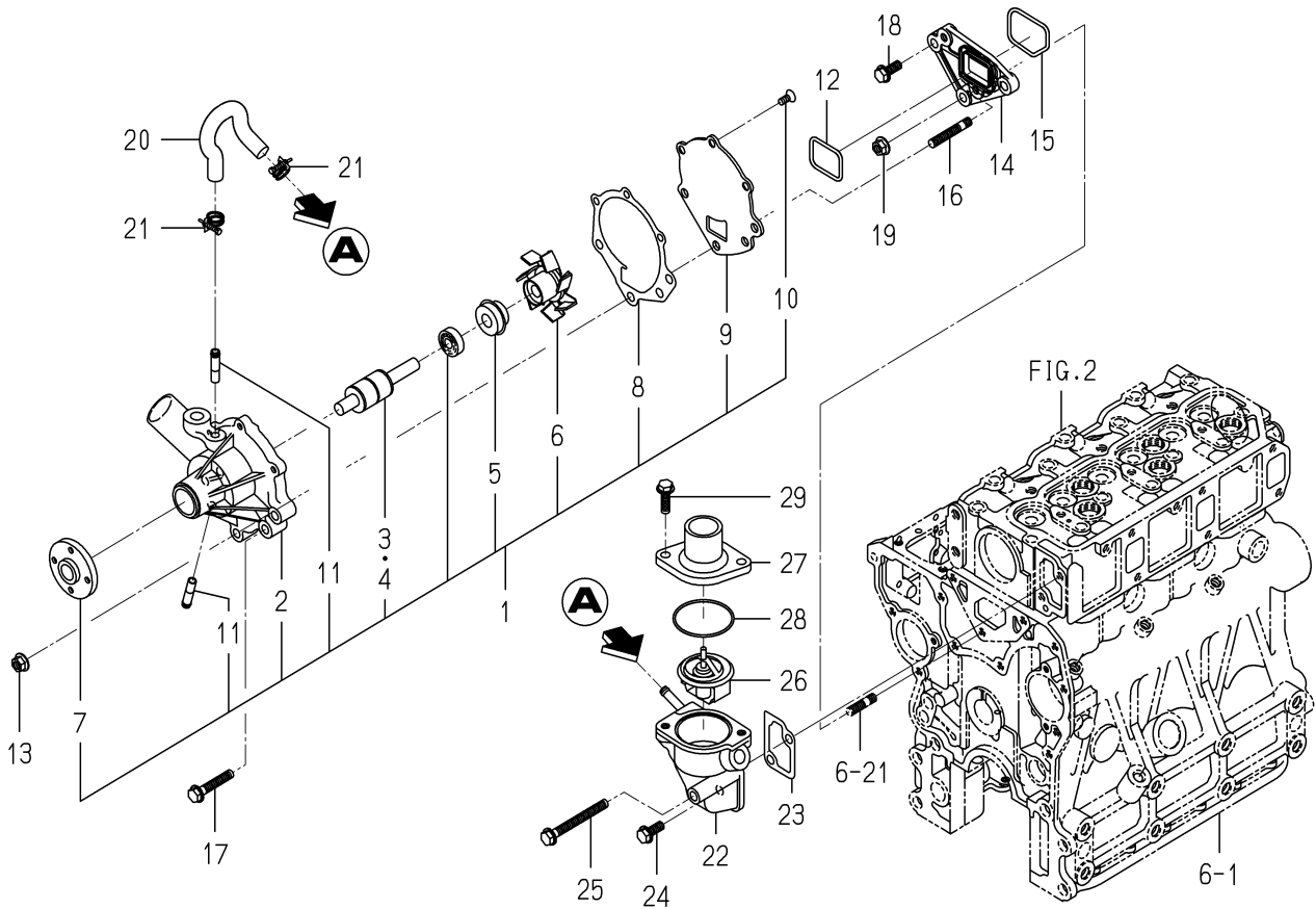
FIG. 19 WATER PUMP
