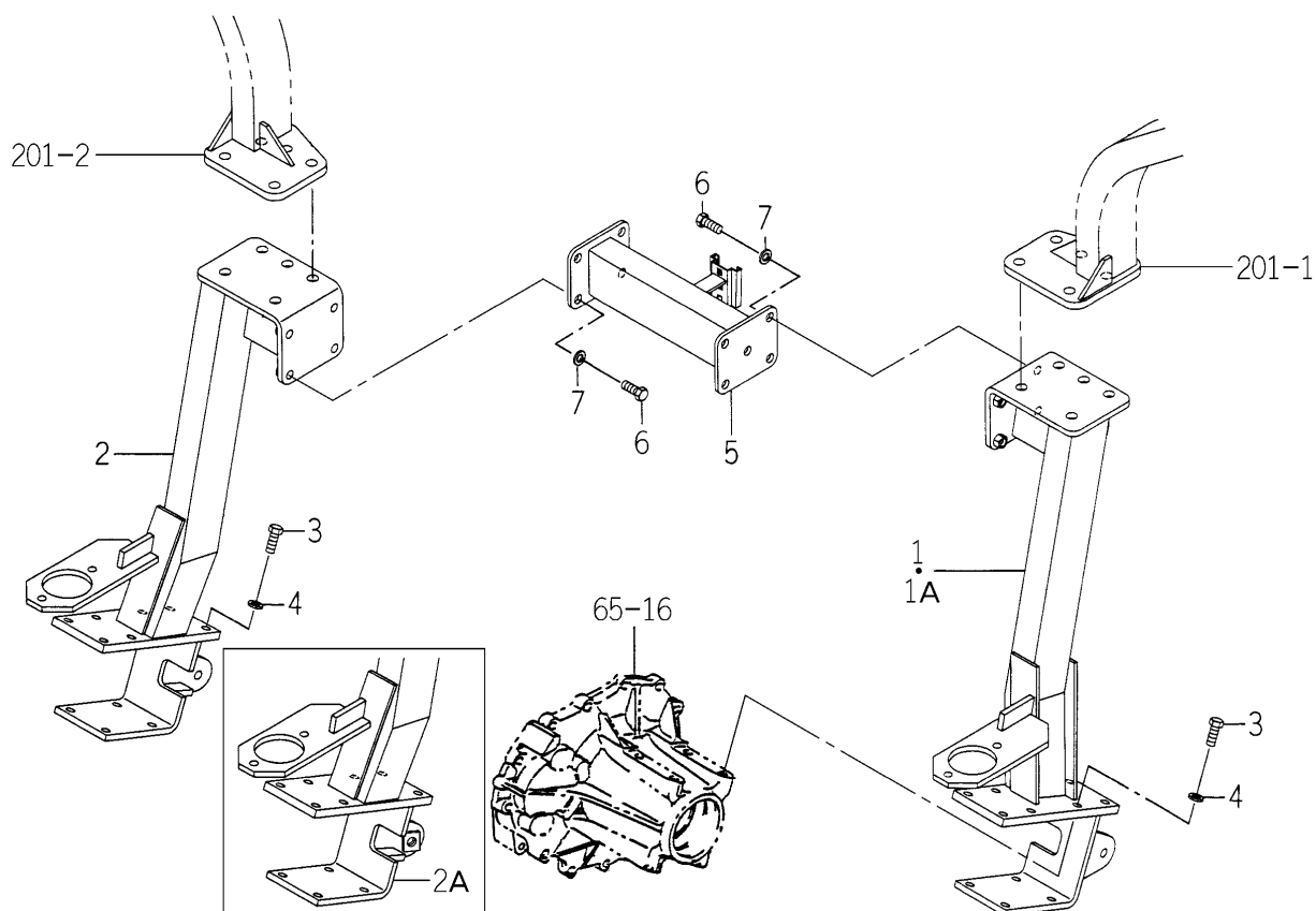
FIG.199 FRAME (REAR) SYSTEM (E6 TYPE)
