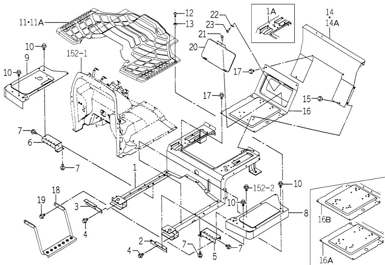
FIG.164 FLOOR (REAR) SYSTEM (HE6 TYPE)
