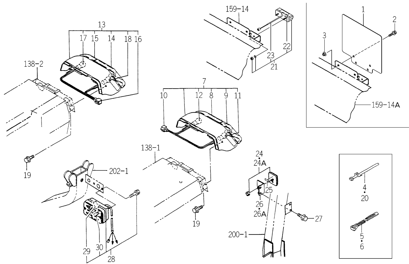
FIG.183 ELC. SYSTEM (REAR) (E4 TYPE EXCEPT C)
