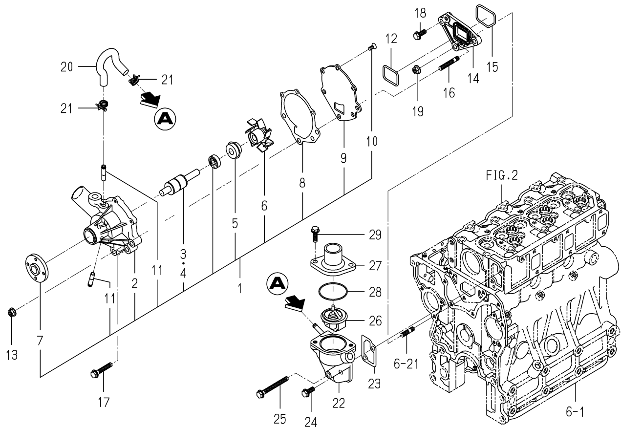
FIG. 21 WATER PUMP
