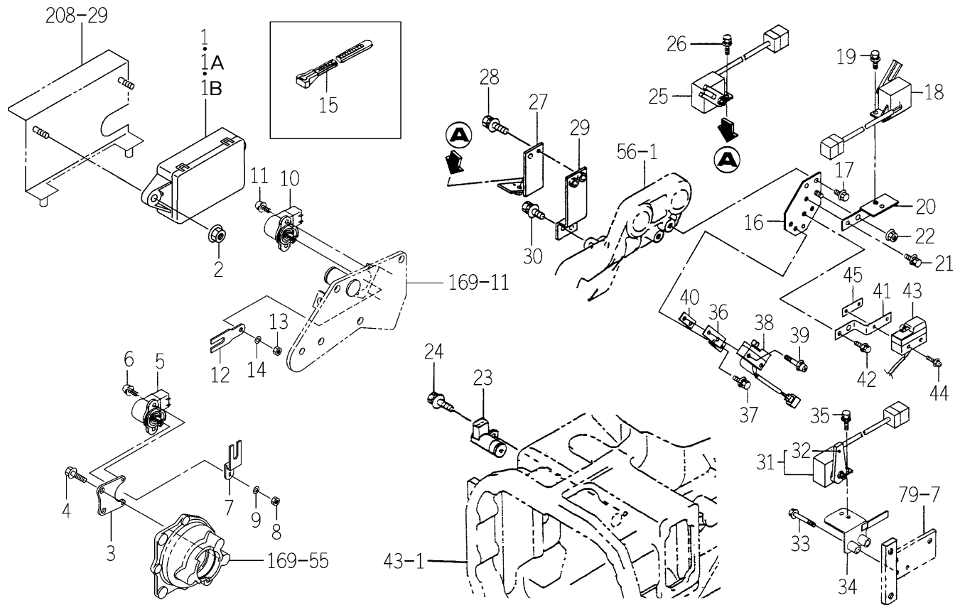
FIG.196 CONTROL SYSTEM (H3C TYPE)
