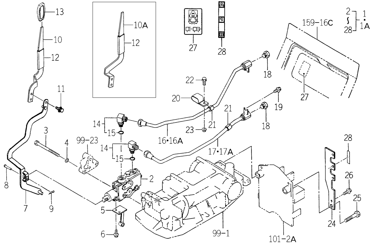
FIG.121 VALVE (1R) SET (A TYPE-TG5330E4-No.296-/TG5390E4-No.660-)
