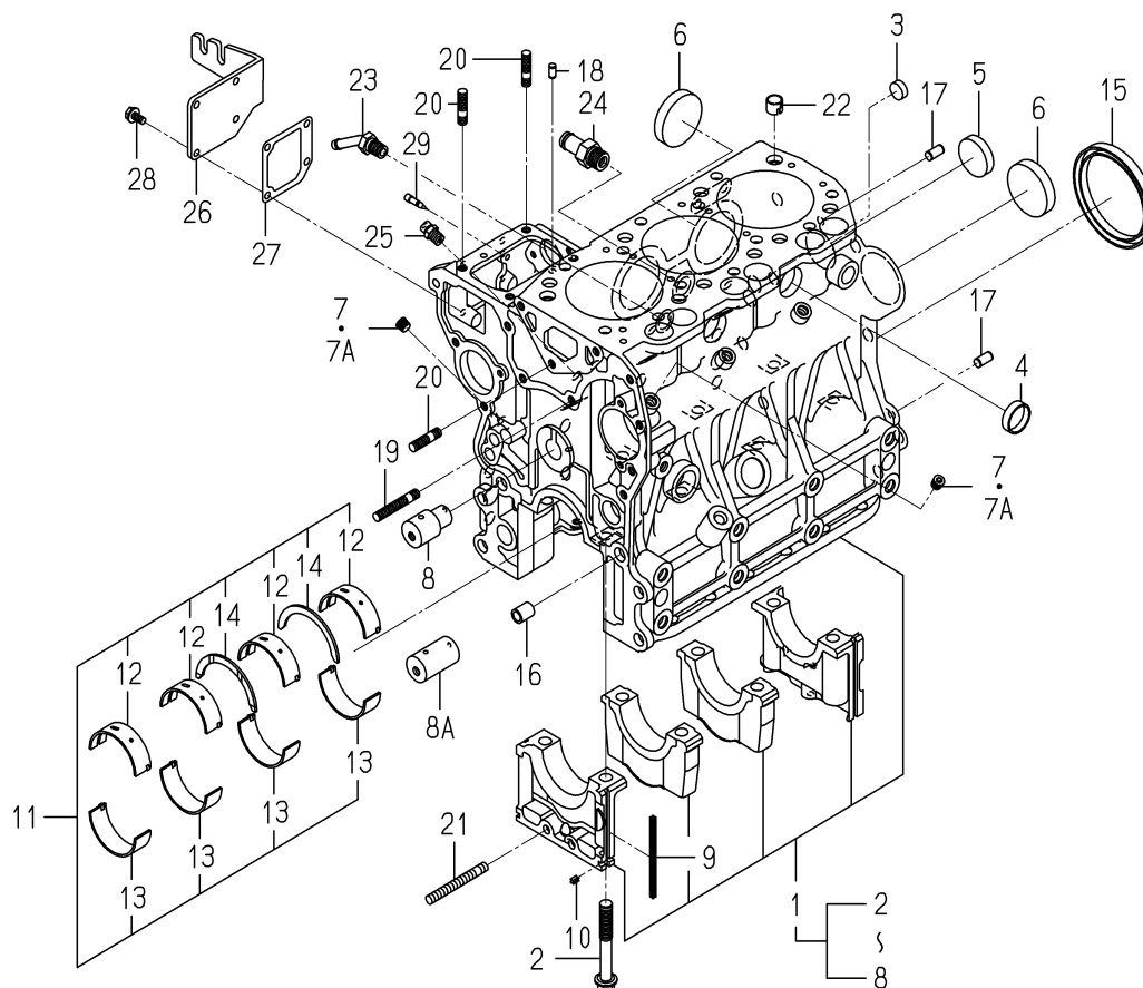
FIG. 7 CYLINDER BLOCK(1/2)
