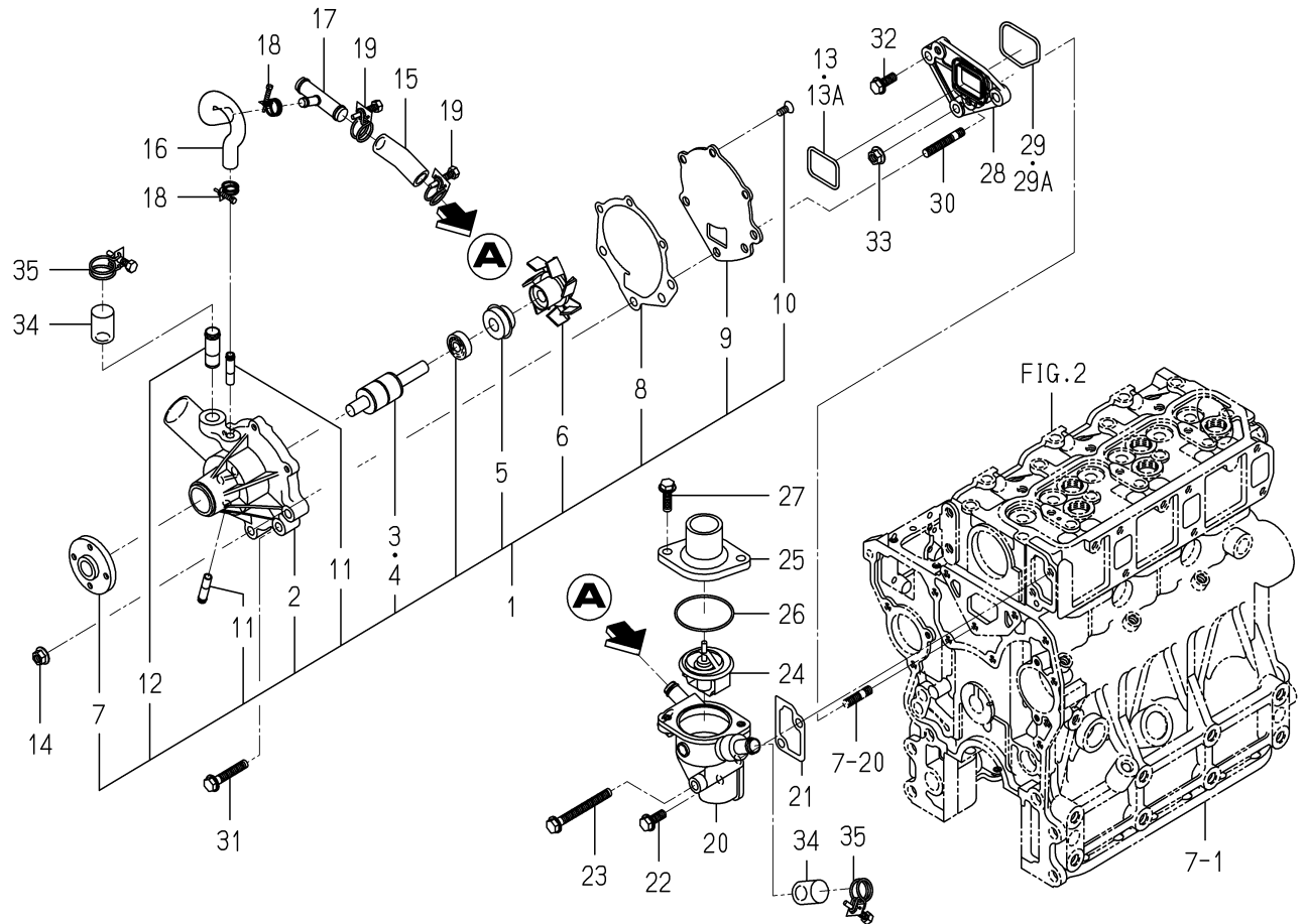
FIG. 20 WATER PUMP
