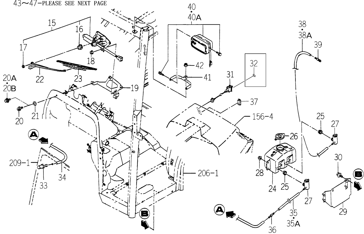
FIG.188 ELC. SYSTEM (C TYPE)(2/3)
