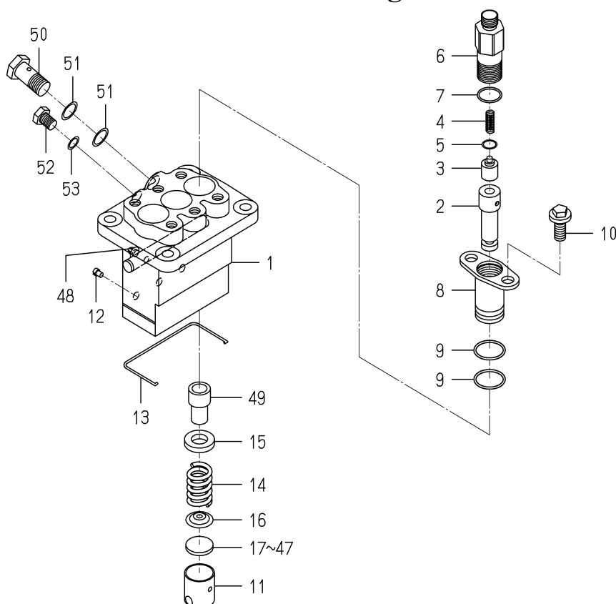
FIG. 32 COMPONENT PARTS FOR 6215-600-104-20 ON Fig.23
