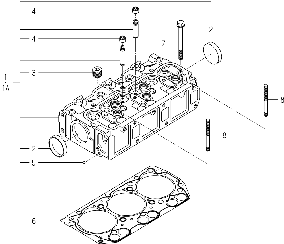
FIG. 2 CYLINDER HEAD
