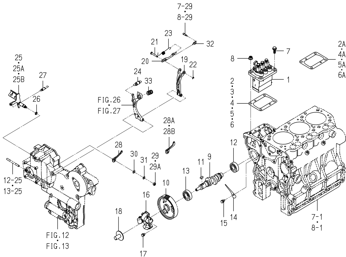
FIG. 24 INJECTION PUMP
