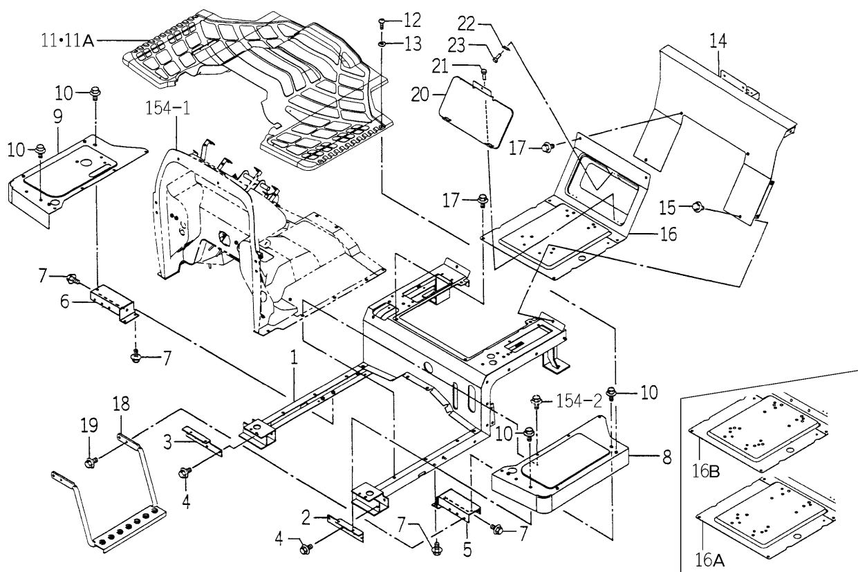
FIG.160 FLOOR (REAR) SYSTEM (HE4 TYPE EXCEPT H3,C)
