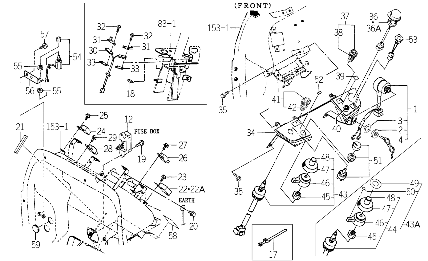
FIG.178 ELC. SYSTEM (MAIN) (Q TYPE)(2/2)
