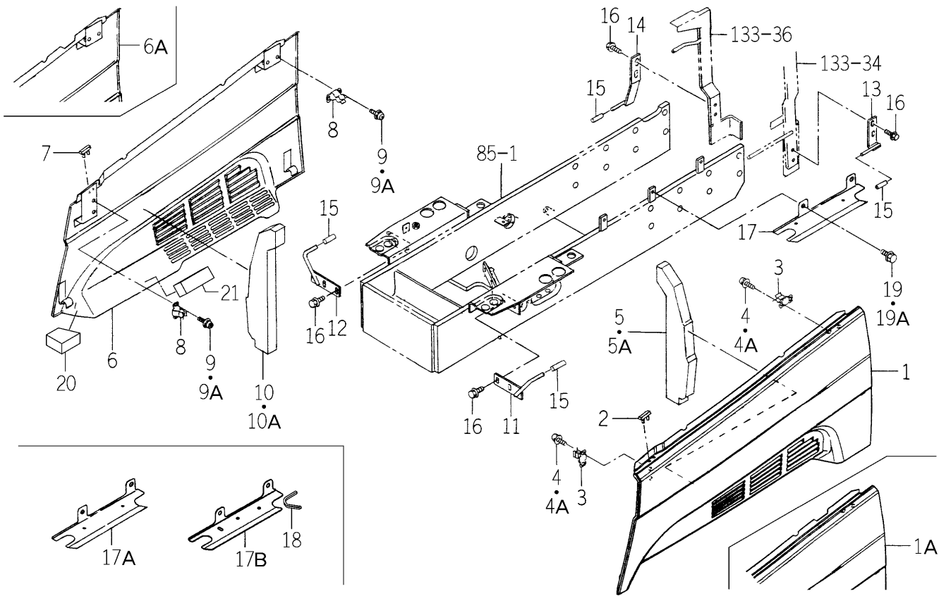
FIG.137 COVER (SIDE) SYSTEM (EXCEPT C TYPE)
