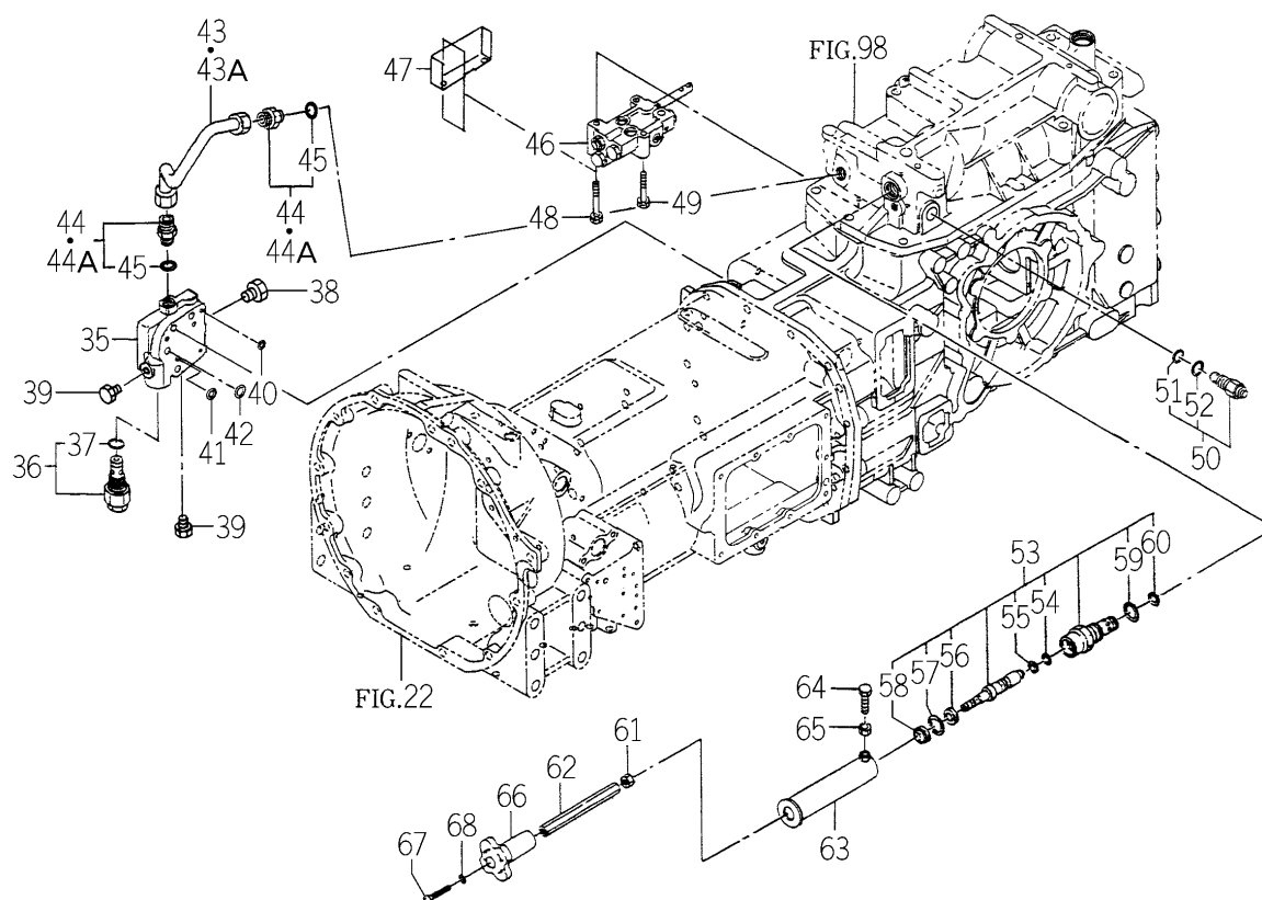
FIG.109 HYD. SYSTEM (MAIN)(2/2) (Q TYPE-TG5330E4-No.444-/TG5390E4-No.778-)
