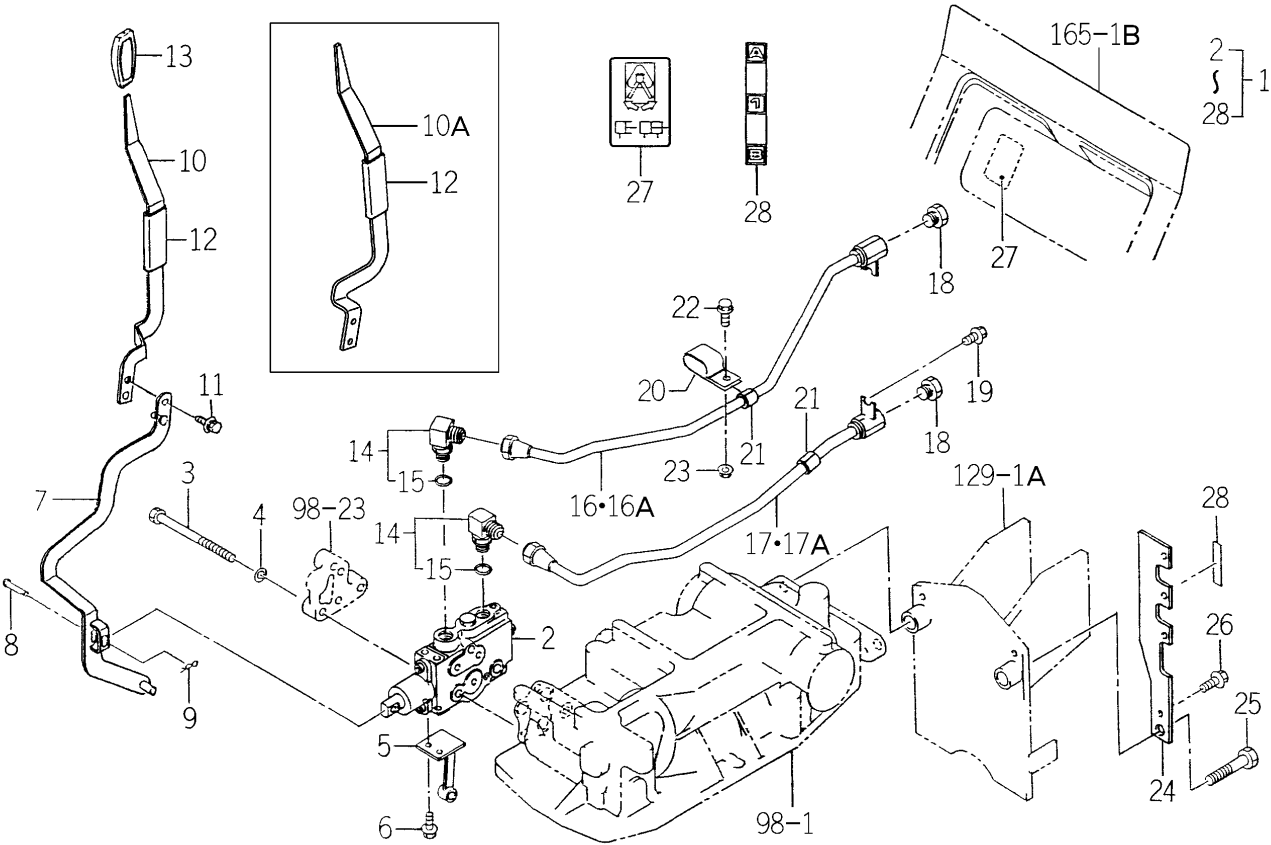
FIG.247 VALVE (REMOTE/1R) SET (C TYPE-OPTION)
