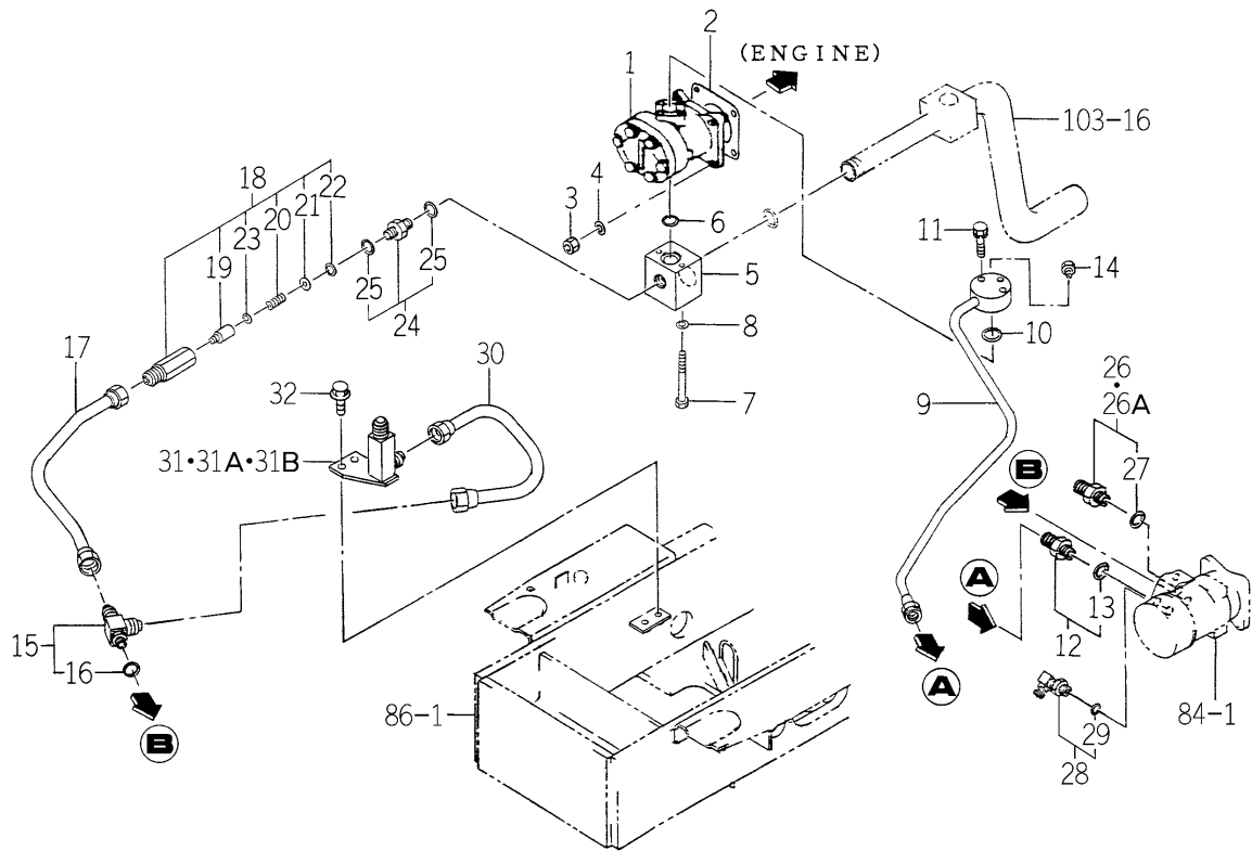
FIG.112 HYD. SYSTEM (SUB)(1/2) (HE4 TYPE EXCEPT H3-No.1-/ HE6 TYPE-TG5390E6-No.1-877)
