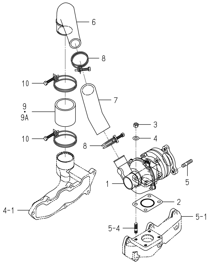
FIG. 6 TURBOCHARGER
