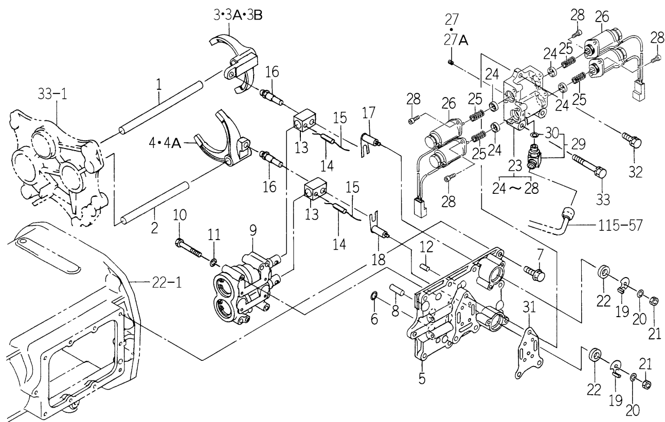
FIG. 47 FORK (SHIFT/MAIN) SYSTEM (Q TYPE)
