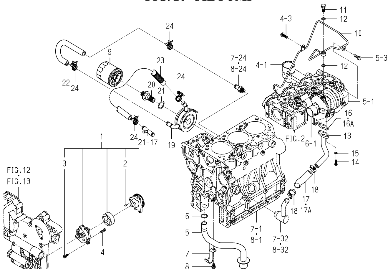
FIG. 20 OIL PUMP
