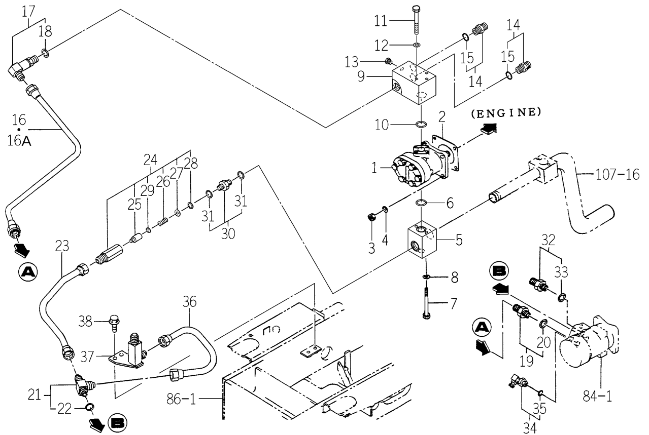
FIG.116 HYD. SYSTEM (SUB) (H3 TYPE)(1/4)
