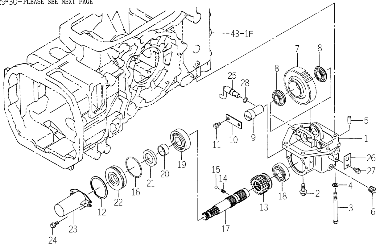
FIG. 42 MID PTO SET (M TYPE-TG5390E4-No.503-)(1/2)
