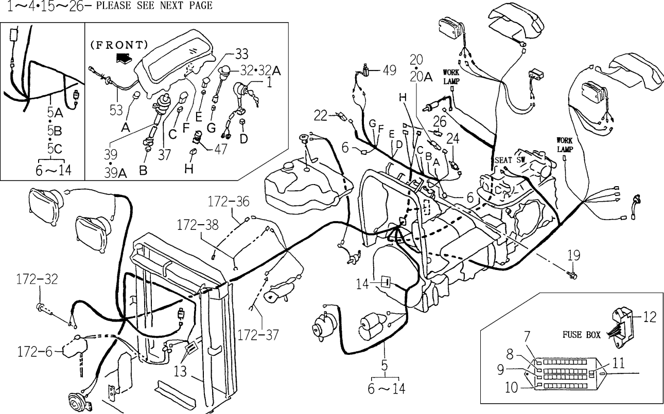
FIG.176 ELC. SYSTEM (MAIN) (S TYPE)(1/2)
