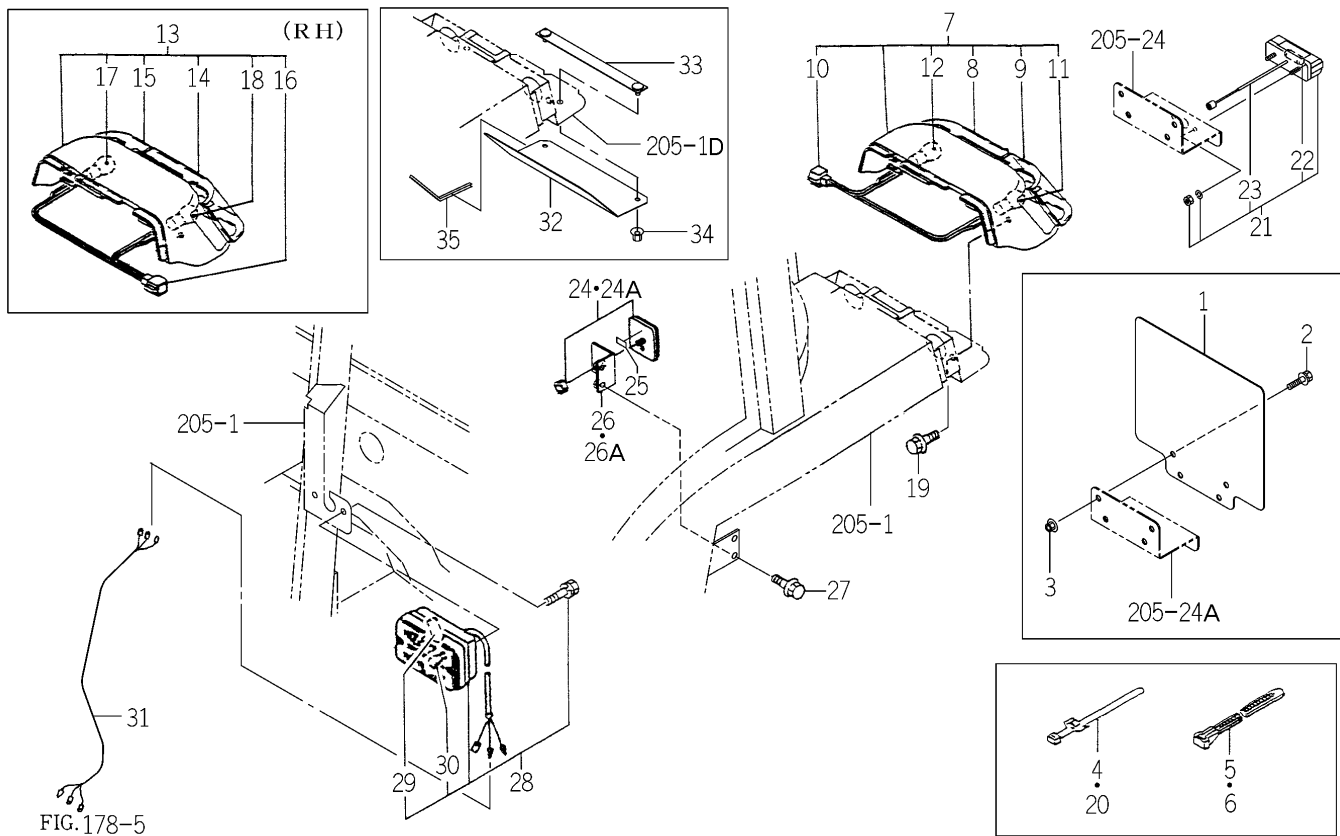
FIG.184 ELC. SYSTEM (REAR) (C TYPE)
