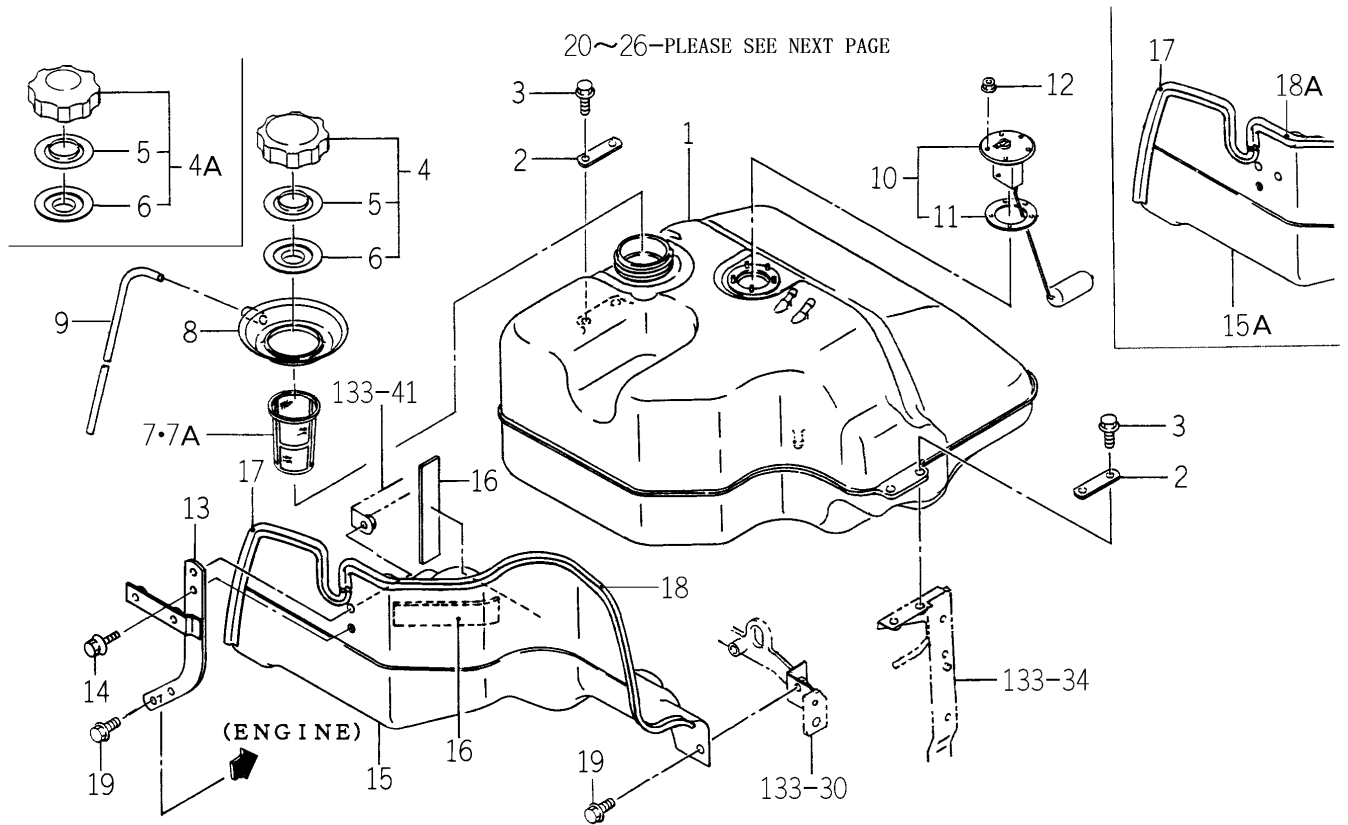
FIG. 14 TANK (FUEL) SYSTEM (TG5390-E4 TYPE)(1/2)
