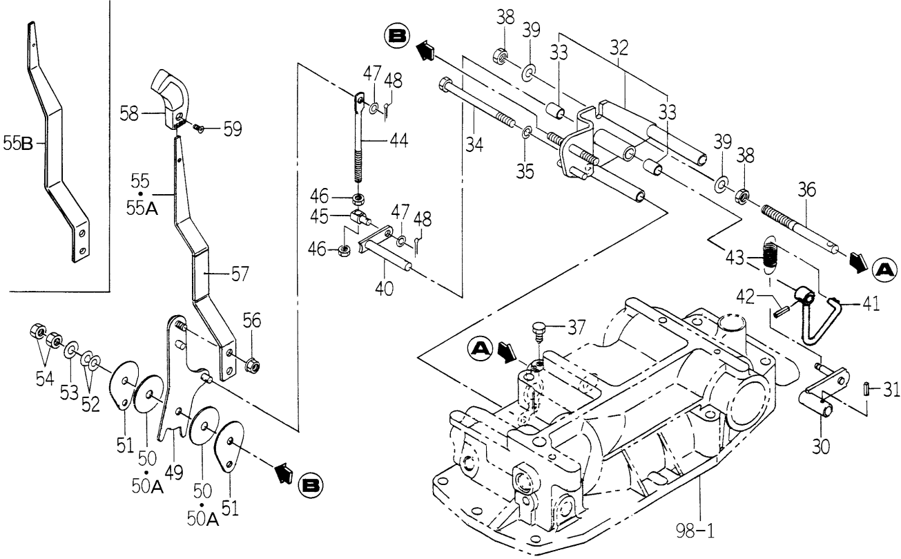
FIG.100 MECHANICAL LINK (POSITION)(2/2) SYSTEM
