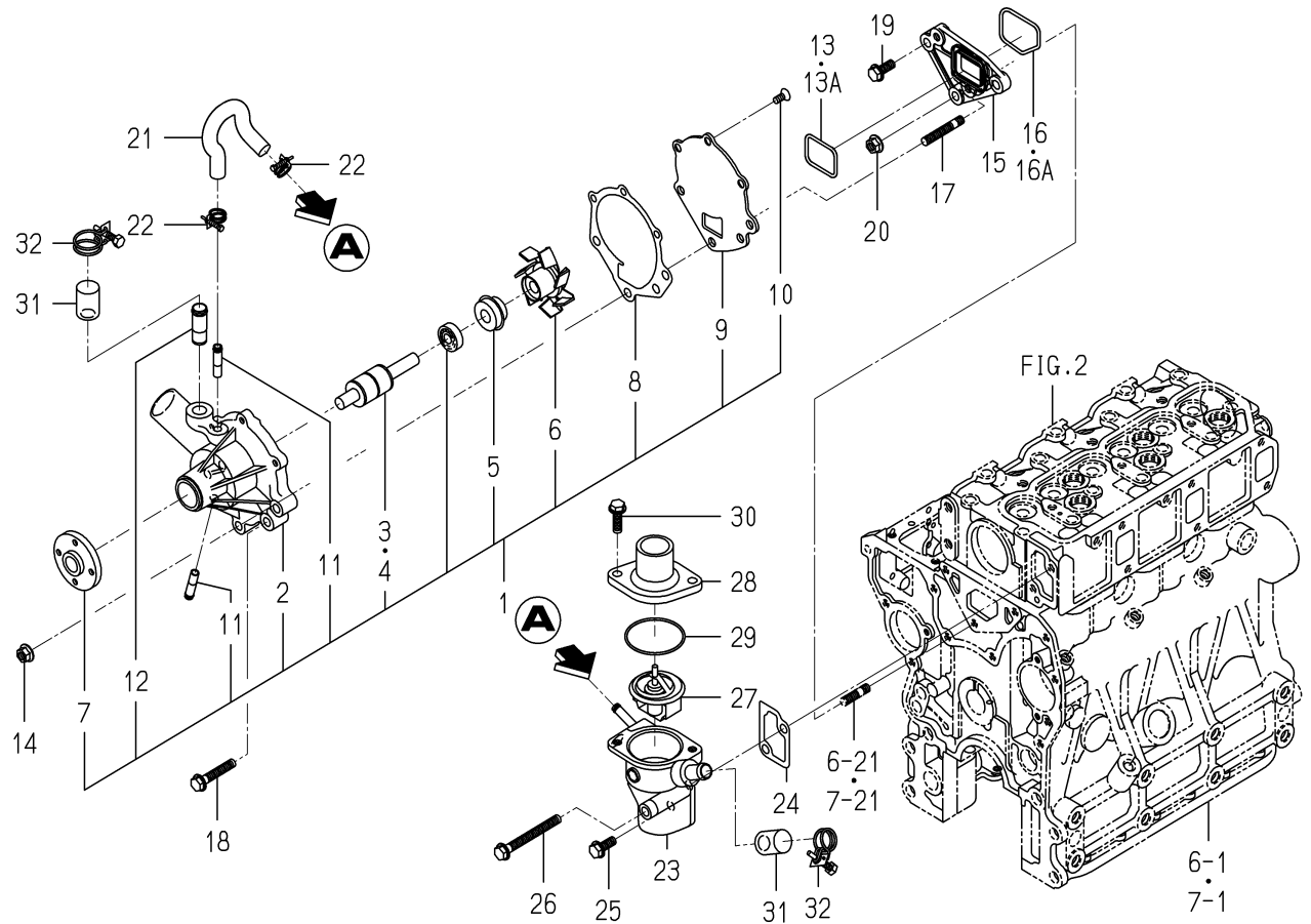
FIG. 22 WATER PUMP
