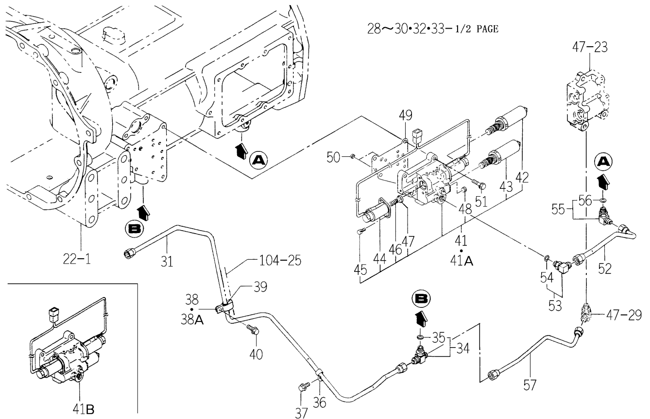
FIG.115 HYD. SYSTEM (SUB) (Q TYPE)(2/2)
