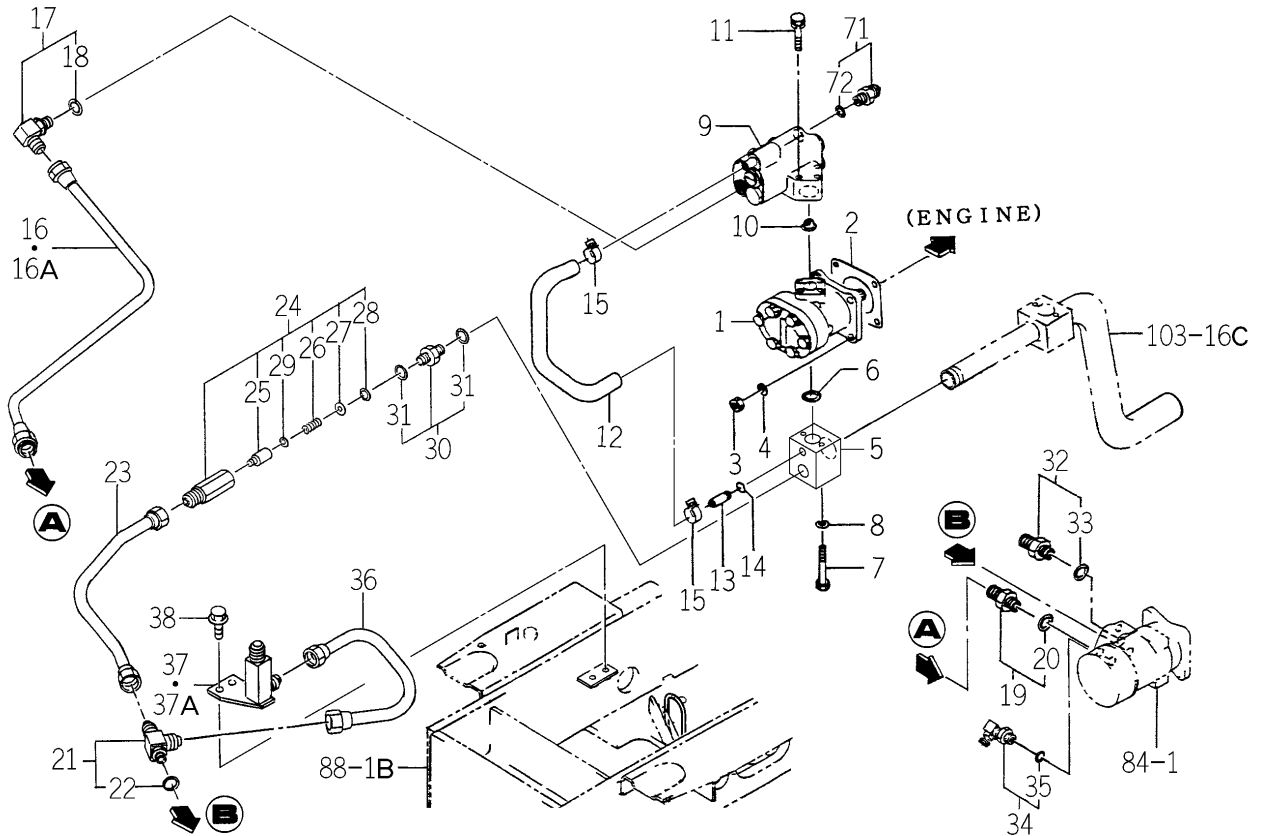
FIG.114 HYD. SYSTEM (SUB)(1/3) (HE6 TYPE-TG5390E6-No.878-)
