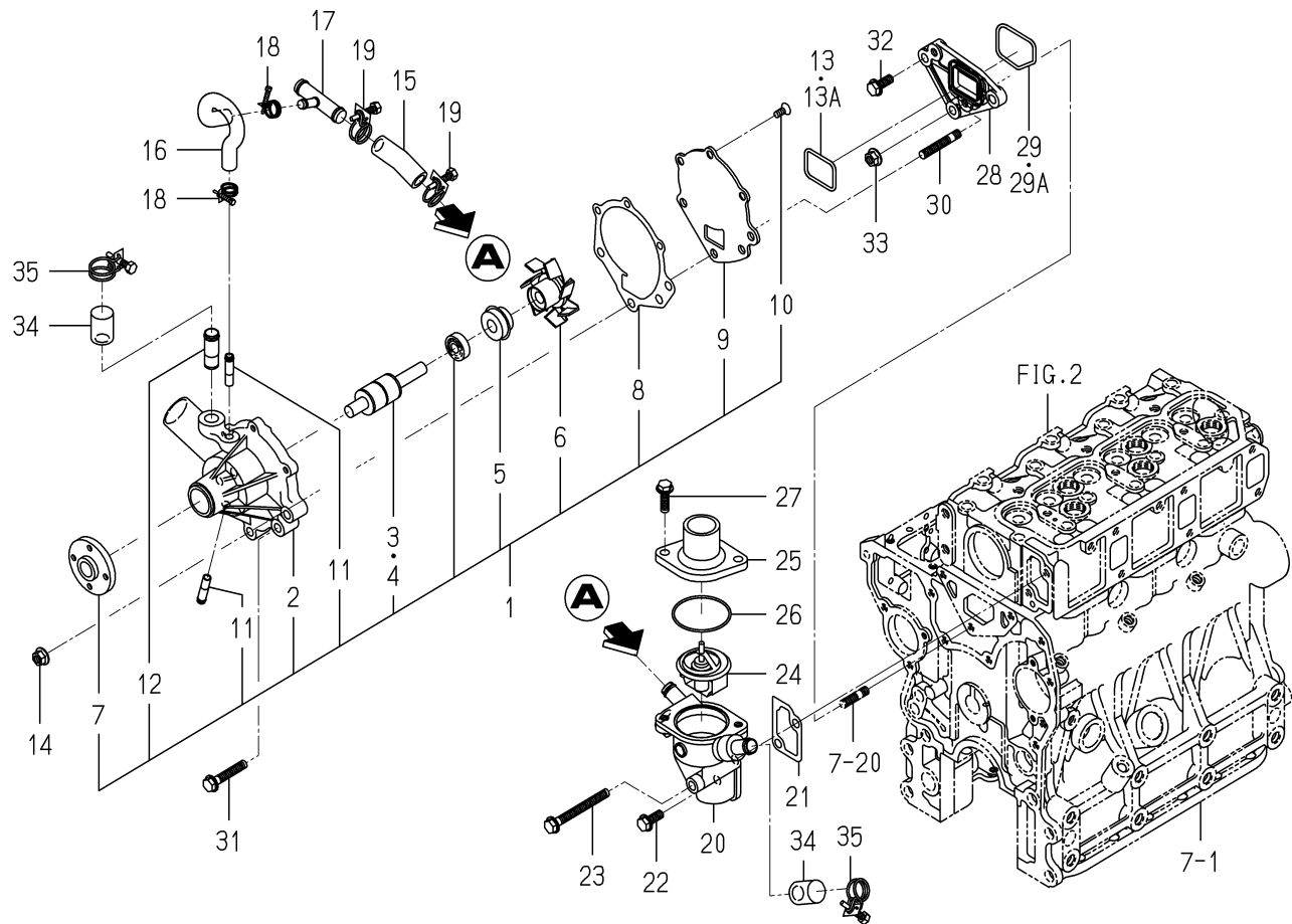
FIG. 20 WATER PUMP
