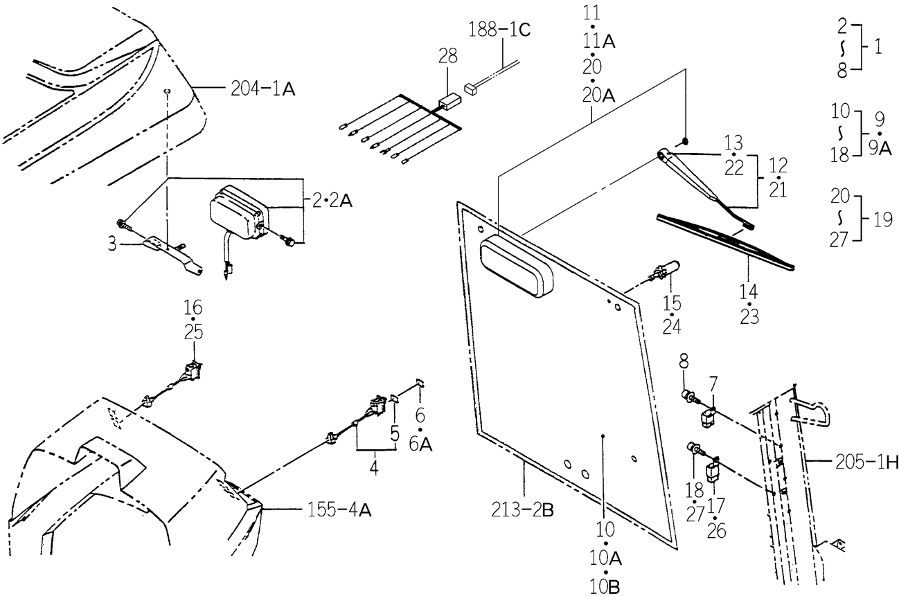
FIG.251 ELC. SYSTEM (C TYPE-OPTION)
