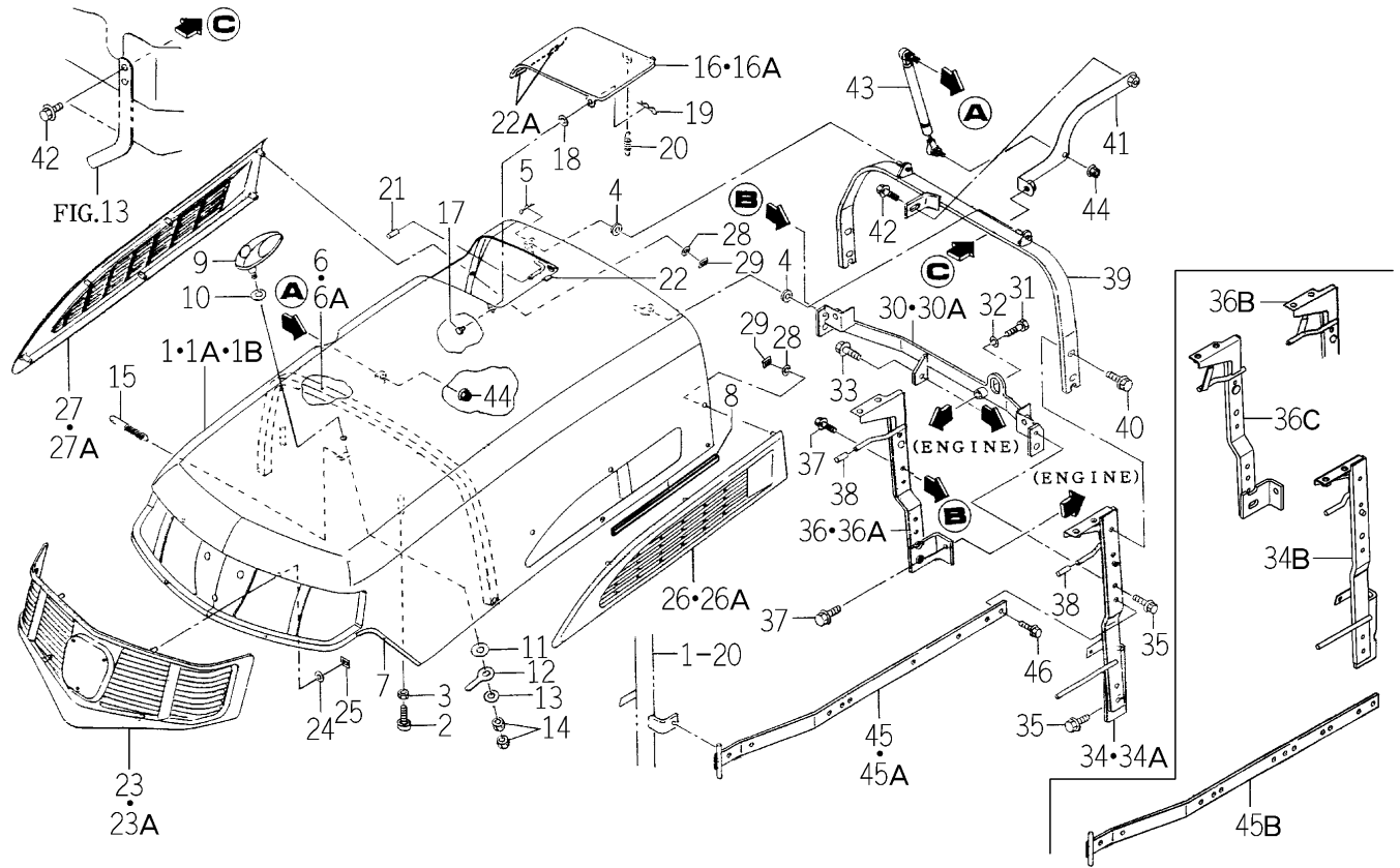
FIG.133 HOOD SYSTEM (EXCEPT C TYPE)
