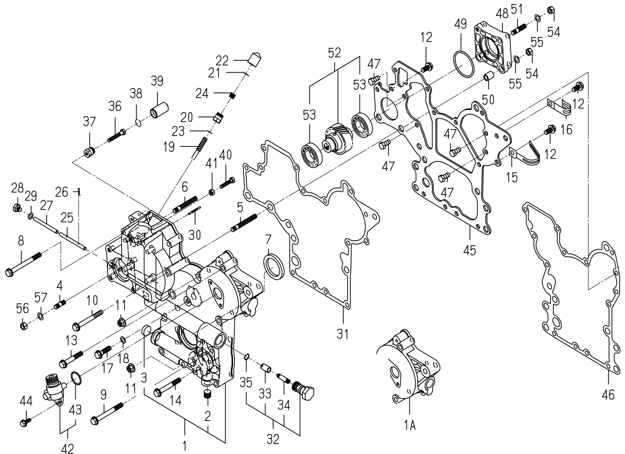
FIG. 13 TIMING GEAR CASE
