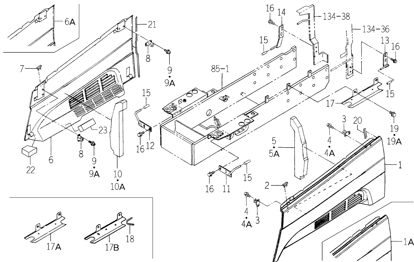
FIG.136 COVER (SIDE) SYSTEM (C TYPE)
