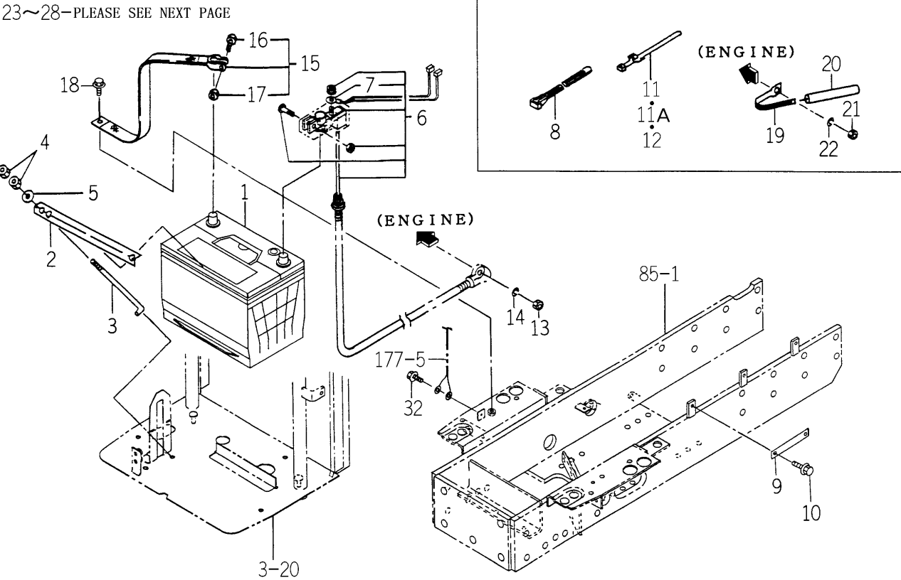
FIG.175 ELC. SYSTEM (FRONT)(1/2) (QE4,HE4 TYPE EXCEPT H3)
