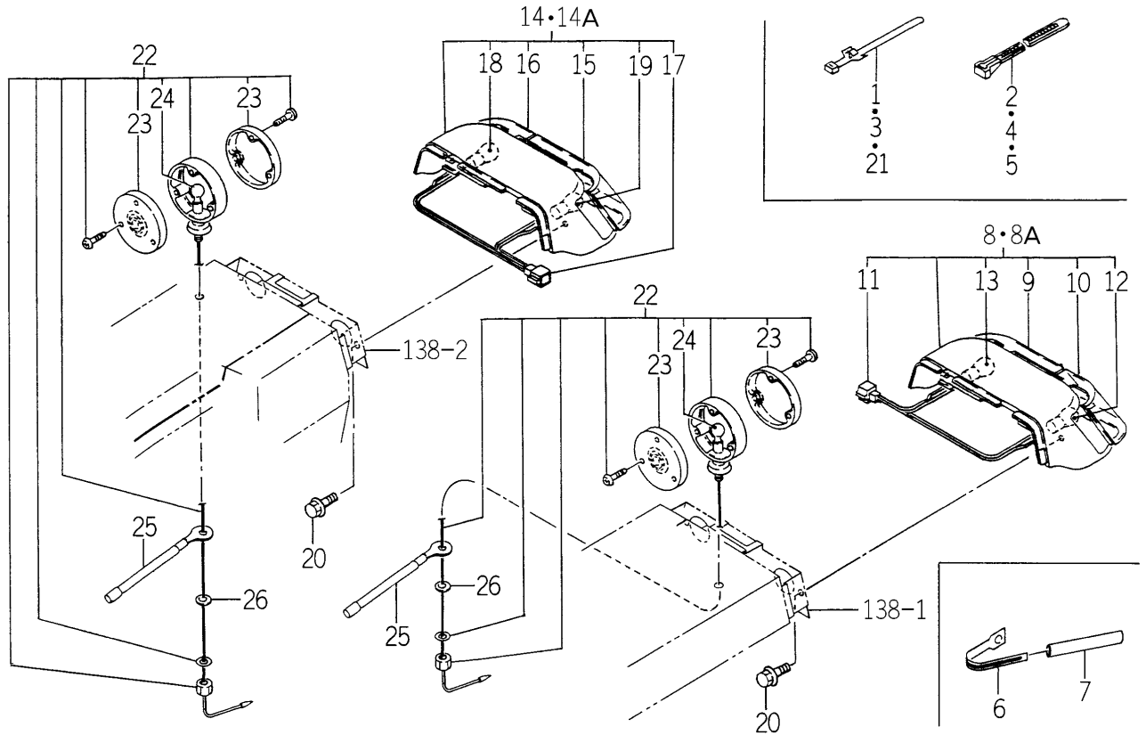
FIG.182 ELC. SYSTEM (REAR) (E6 TYPE)
