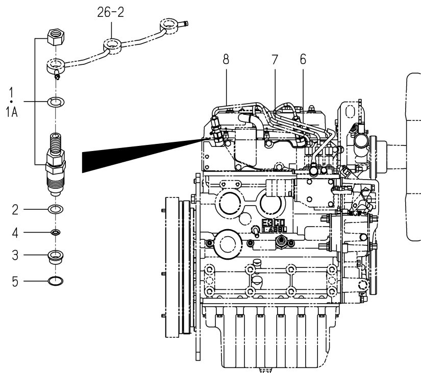
FIG. 24 INJECTION NOZZLE
