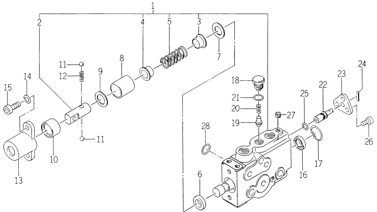
FIG.269 COMPONENT PARTS FOR 1719-511-350-00 ON Fig.119,121
