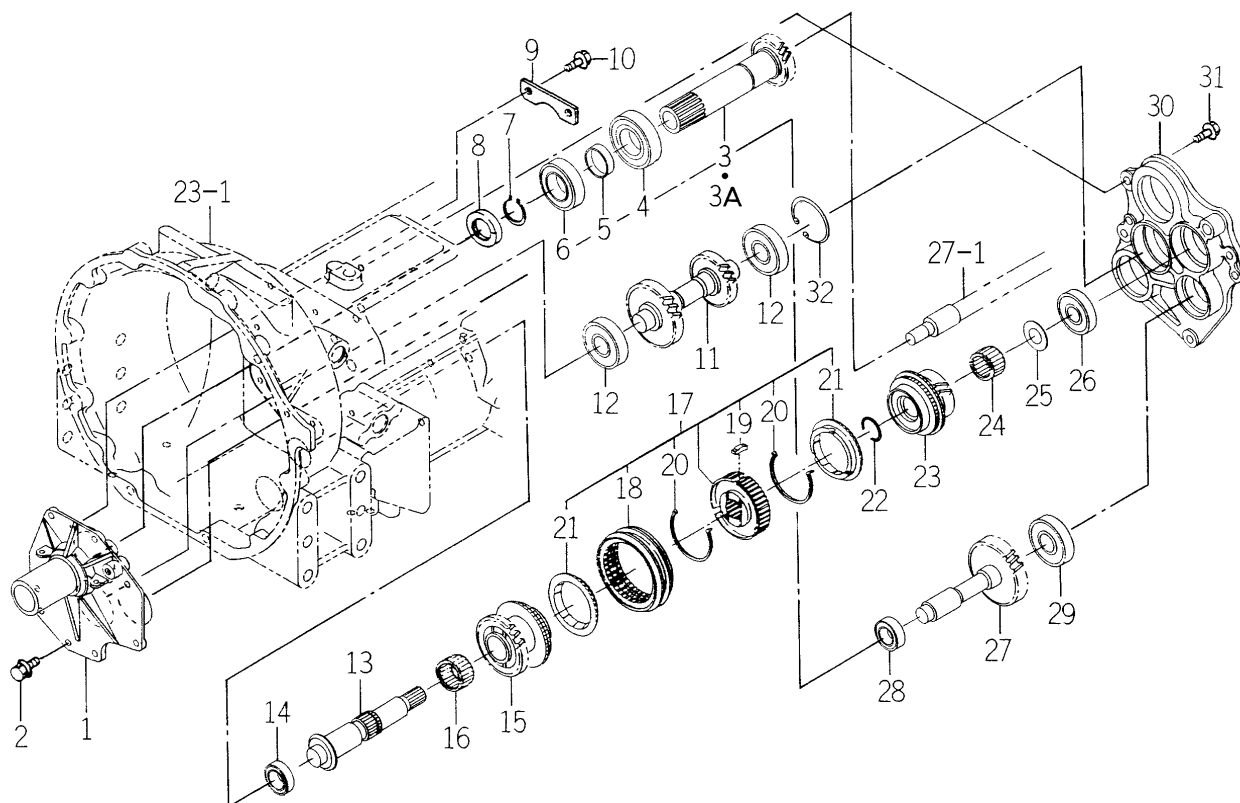
FIG. 26 GEAR (REVERSE) SYSTEM (S TYPE)
