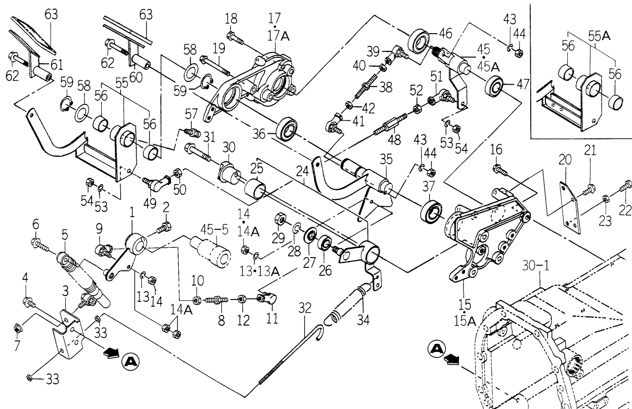
FIG.167 PEDAL (HST) SYSTEM (HE4 TYPE EXCEPT H3)
