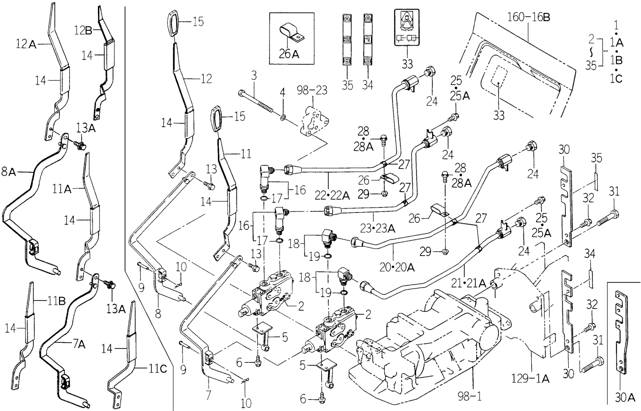
FIG.246 VALVE (REMOTE/2R) SET (E4 TYPE EXCEPT C,A-OPTION)
