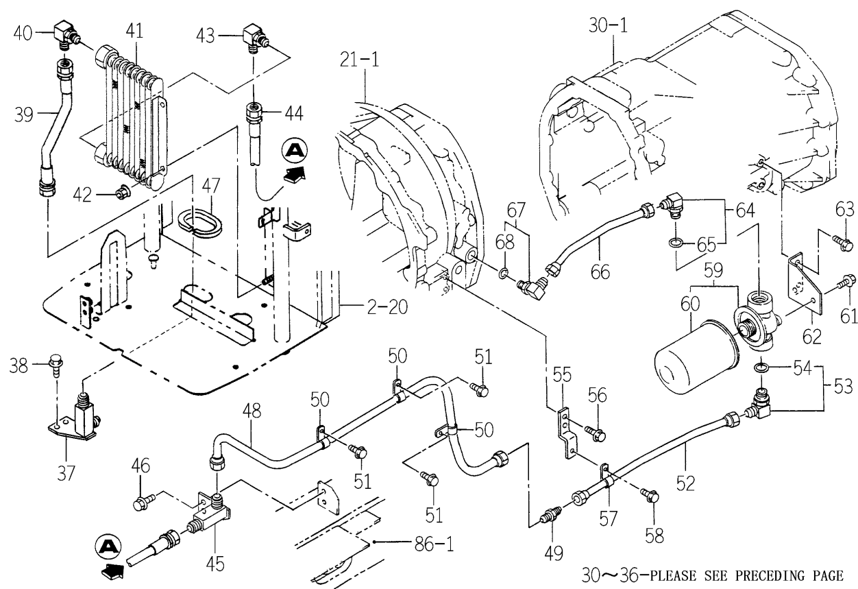
FIG.116 HYD. SYSTEM (SUB) (H3 TYPE)(2/4)
