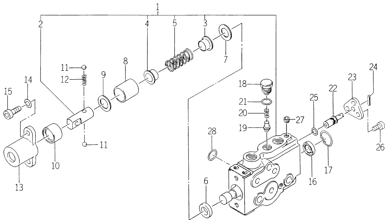
FIG.267 COMPONENT PARTS FOR 1640-530-600-10 ON Fig.119,120,246-249
