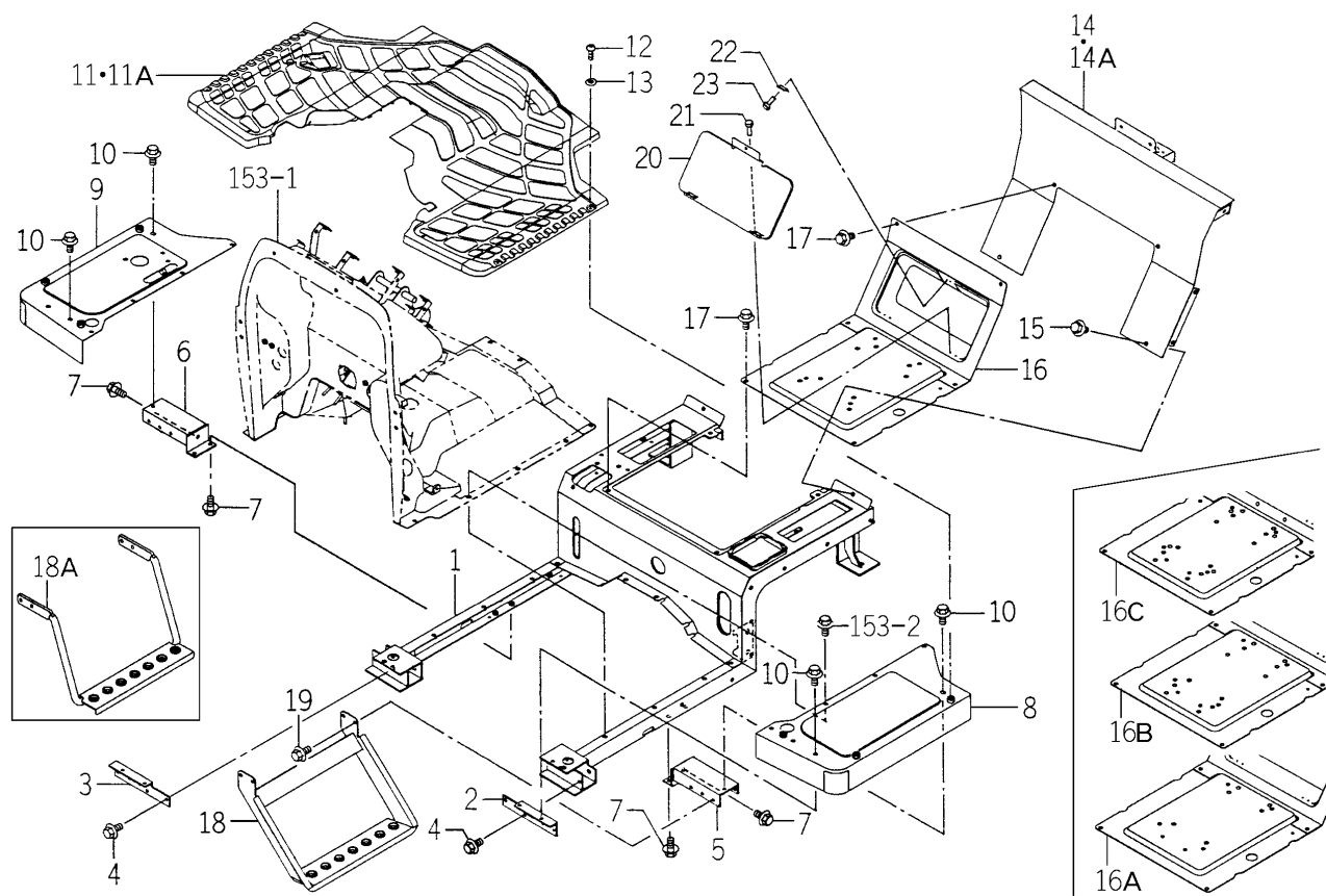
FIG.159 FLOOR (REAR) SYSTEM (S TYPE)
