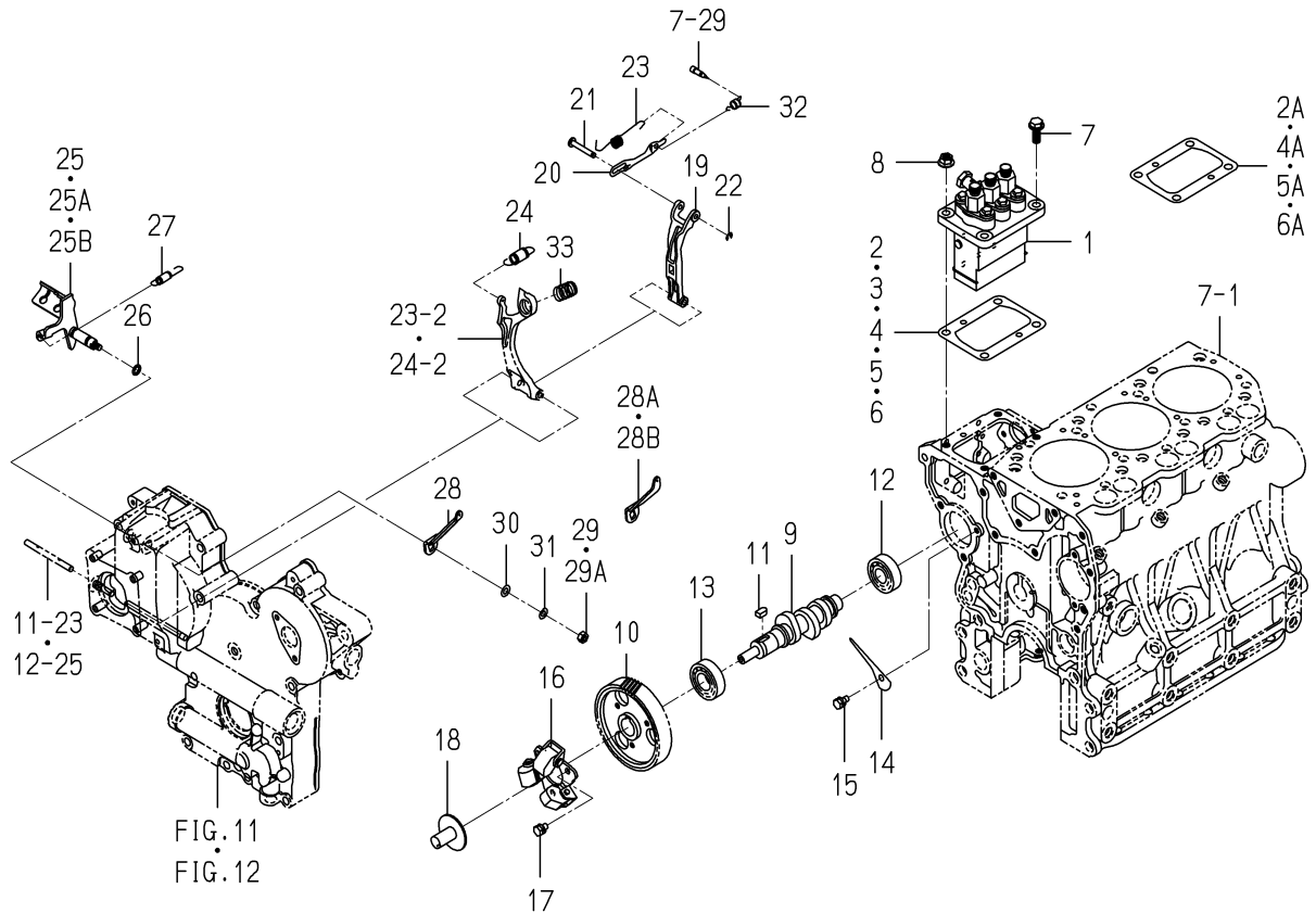
FIG. 23 INJECTION PUMP
