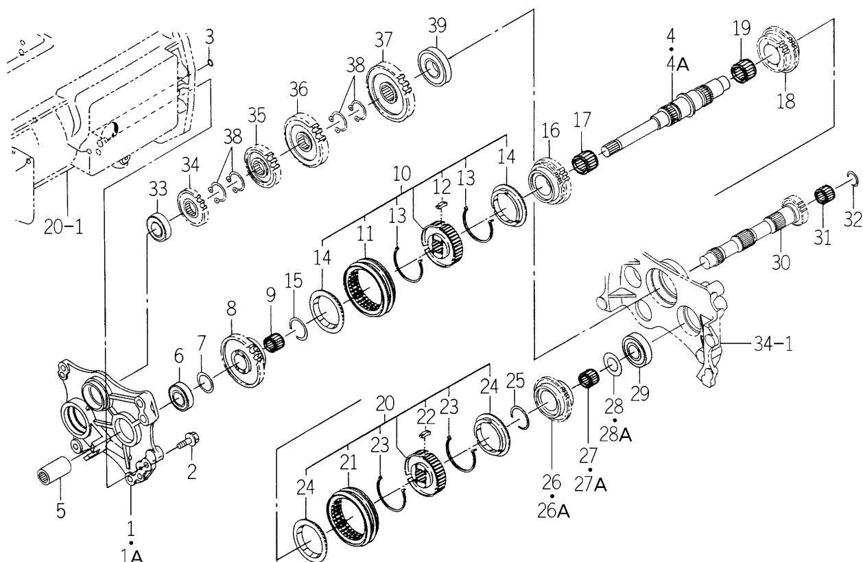
FIG. 31 GEAR (MAIN) SYSTEM (S,P TYPE)
