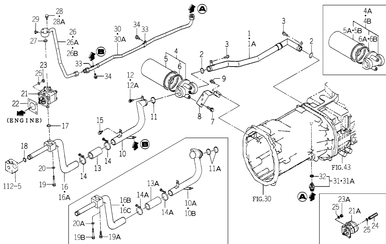
FIG.103 HYD. SYSTEM (MAIN)(1/2) (H TYPE EXCEPT H3-TG5390E4-No.1-774)
