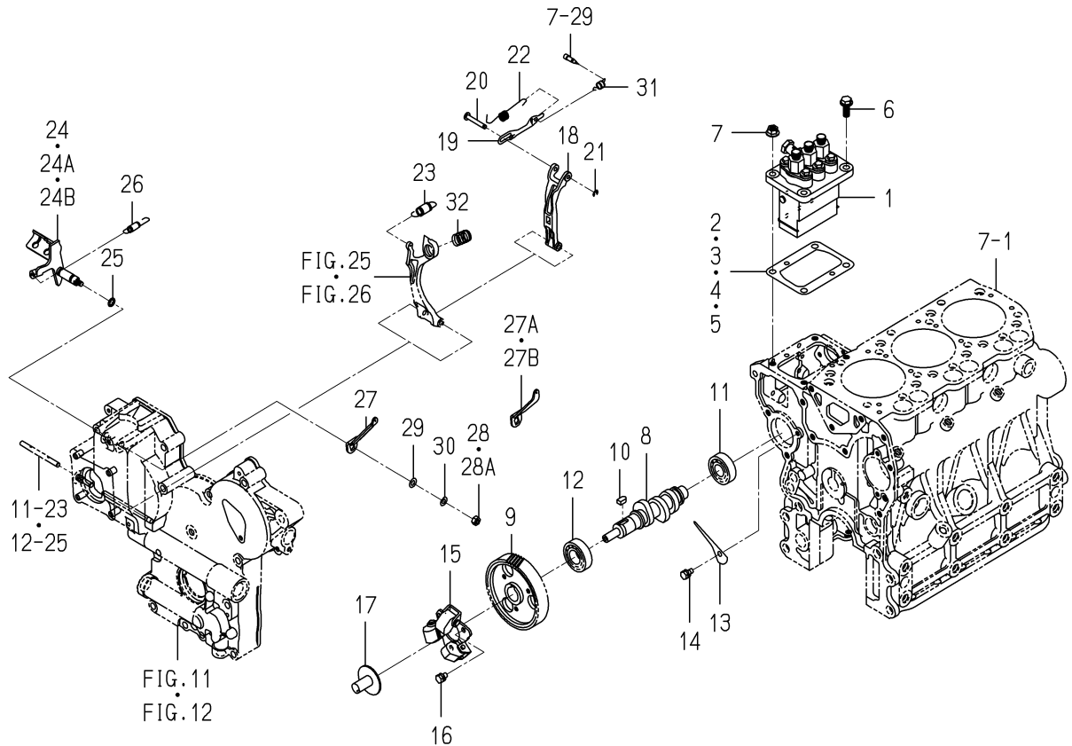
FIG. 23 INJECTION PUMP
