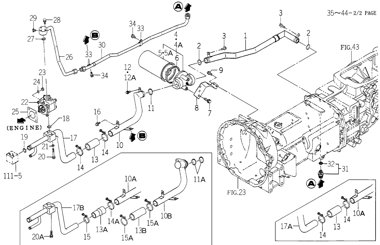
FIG.102 HYD. SYSTEM (MAIN)(1/2) (S TYPE-TG5330E4-No.1-439/TG5390E4-No.1-775)
