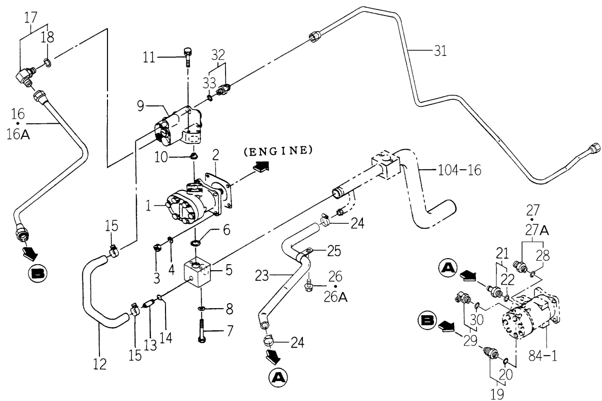
FIG.115 HYD. SYSTEM (SUB) (Q TYPE)(1/2)
