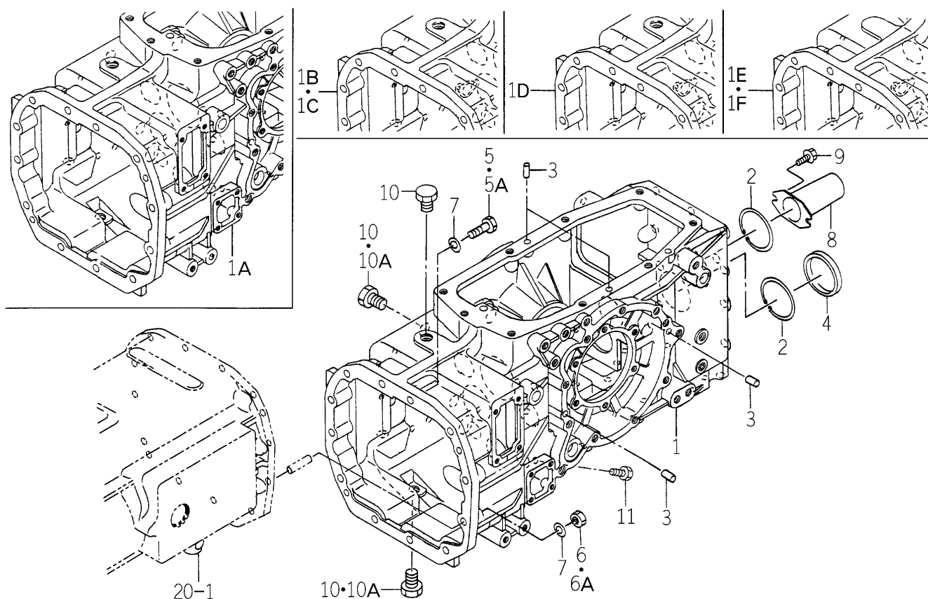
FIG. 43 CASE (TRANSMISSION/REAR) SYSTEM
