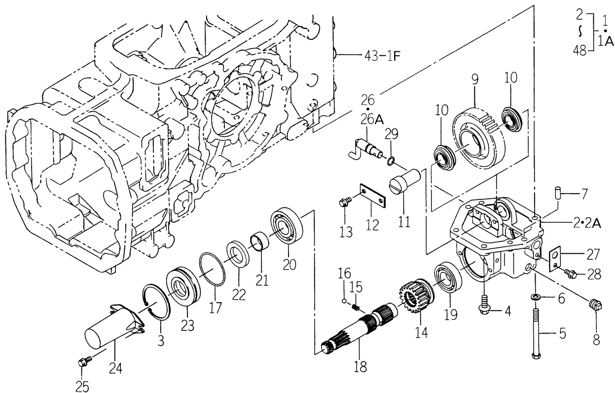
FIG.236 MID PTO SET (Q TYPE-OPTION)(1/2)
