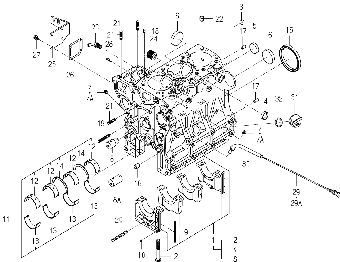
FIG. 6 CYLINDER BLOCK
