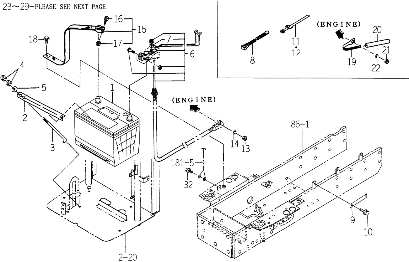
FIG.173 ELC. SYSTEM (FRONT) (H3 TYPE)(1/2)
