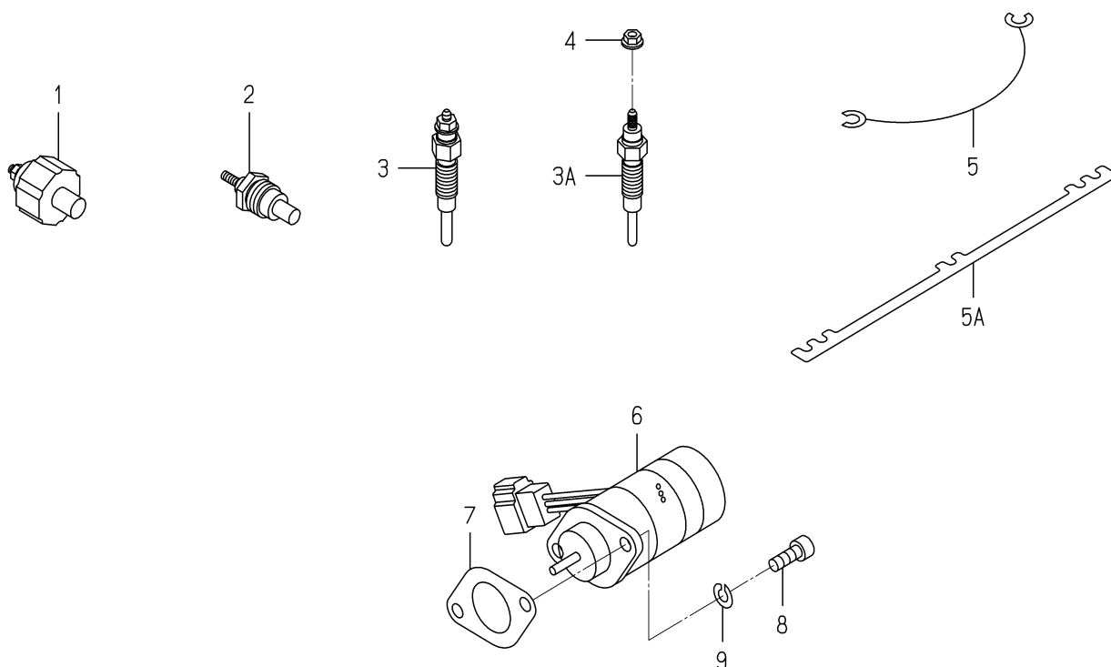
FIG. 28 ELECTRIC (2)
