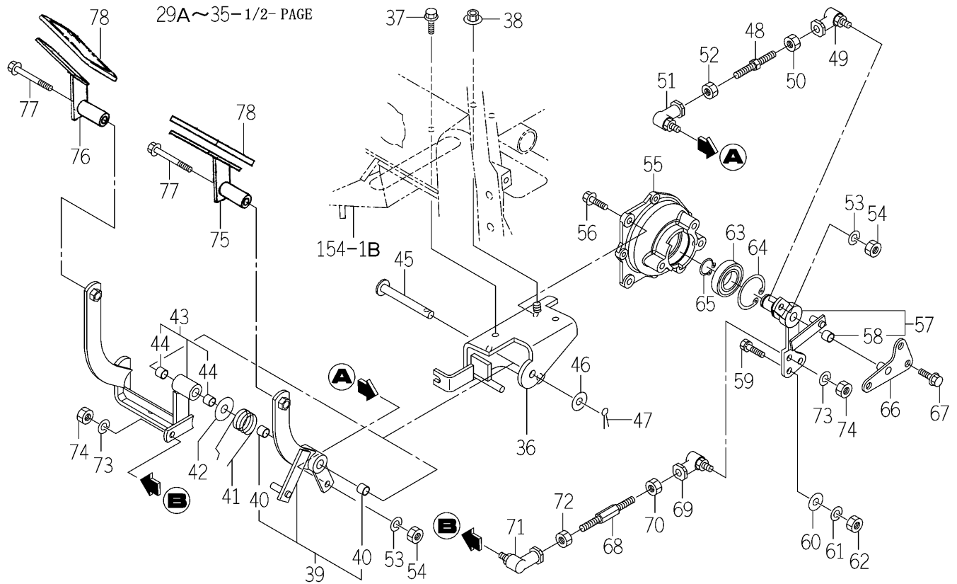
FIG.169 PEDAL (HST) SYSTEM (H3 TYPE)(2/2)
