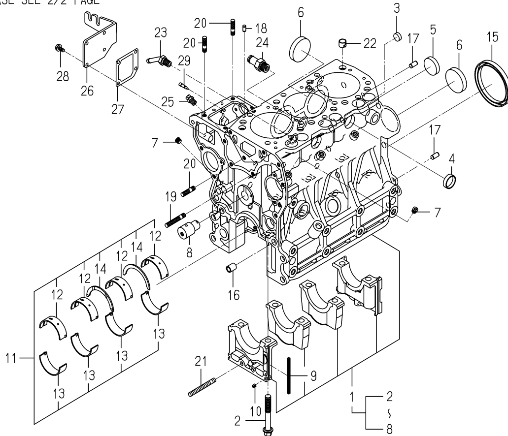
FIG. 7 CYLINDER BLOCK(1/2)
