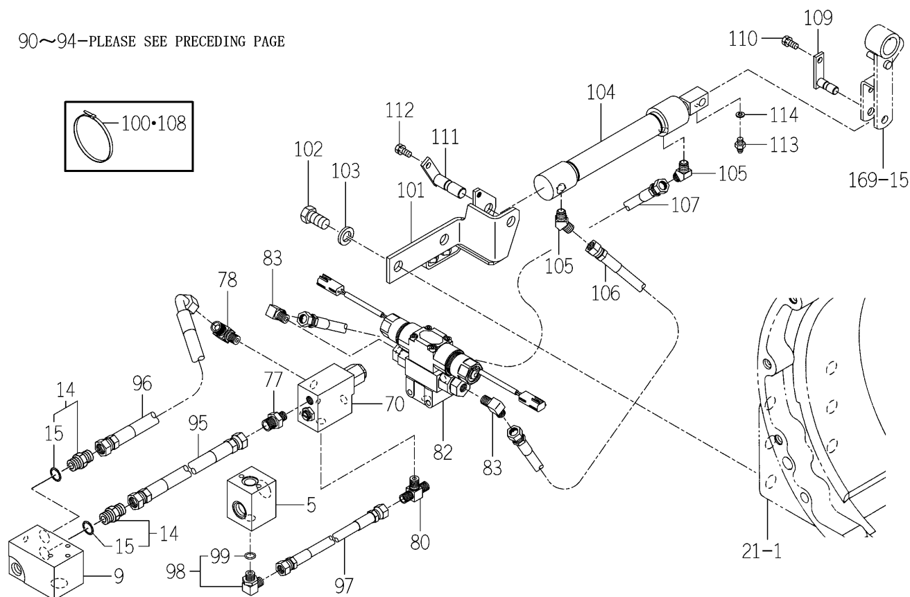
FIG.116 HYD. SYSTEM (SUB) (H3 TYPE)(4/4)
