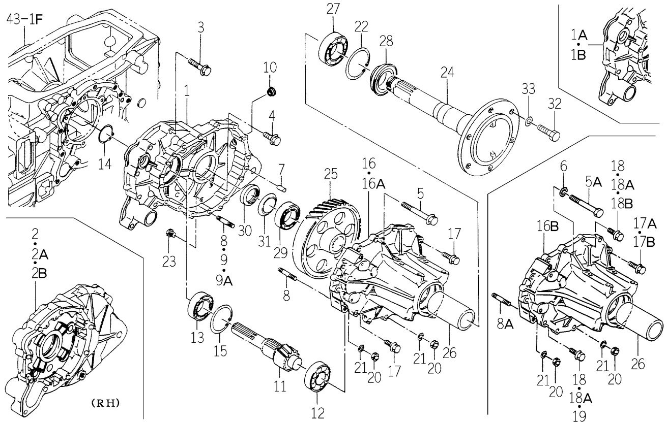
FIG. 66 HOUSING (AXLE/REAR) SYSTEM (H TYPE-TG5390E4-No.153-/TG5390E6-No.153-)
