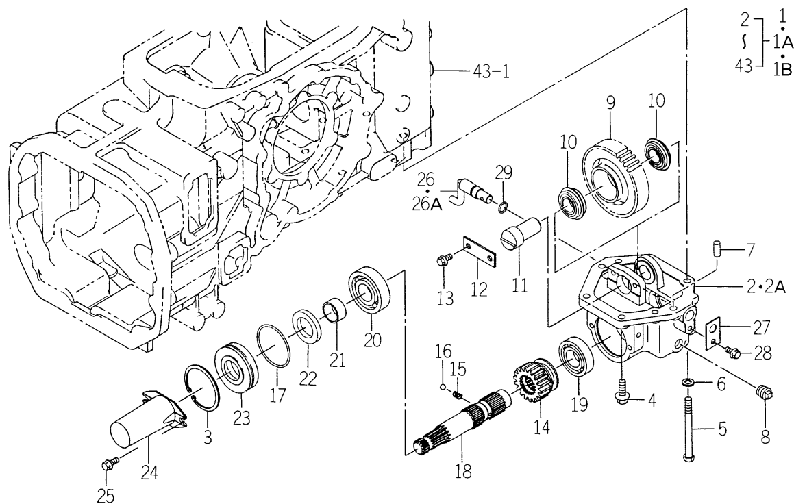
FIG. 41 MID PTO SET(1/2) (M TYPE-STANDARD-TG5390E4-No.1-502/ EXCEPT Q,M TYPE-OPTION)
