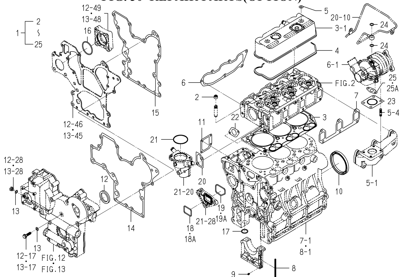
FIG. 30 REPAIR PARTS(OPTION)
