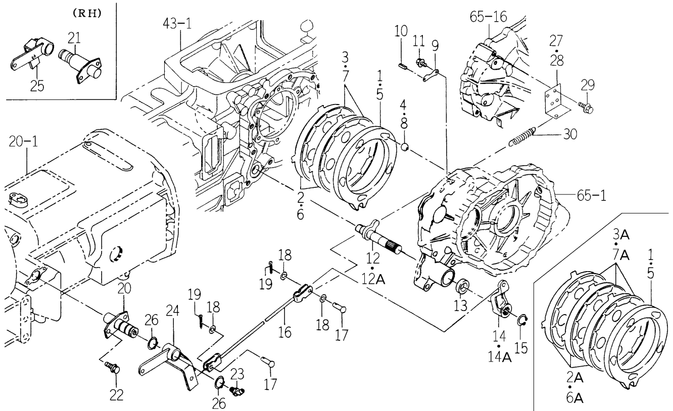
FIG. 69 BRAKE SYSTEM (E6 TYPE EXCEPT H)
