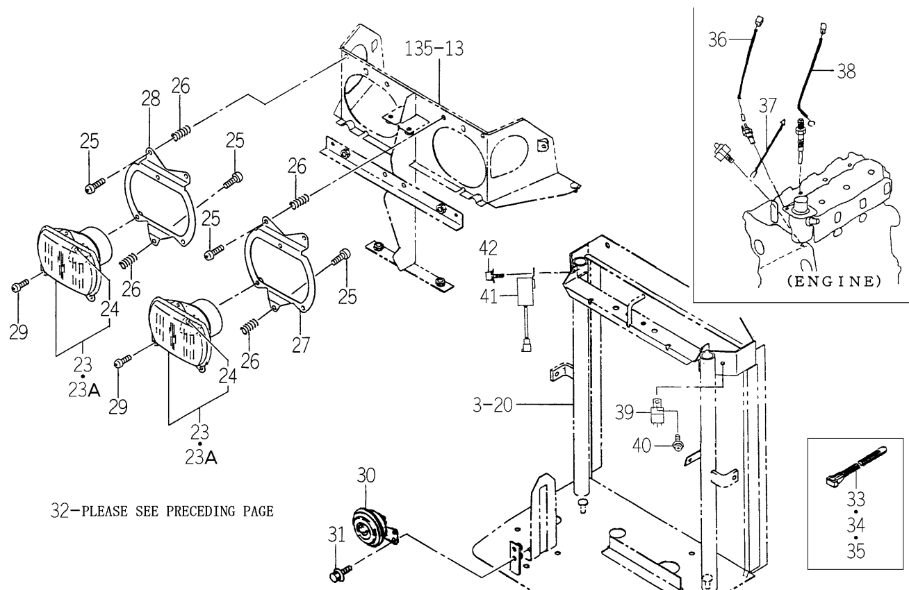
FIG.175 ELC. SYSTEM (FRONT)(2/2) (QE4,HE4 TYPE EXCEPT H3)
