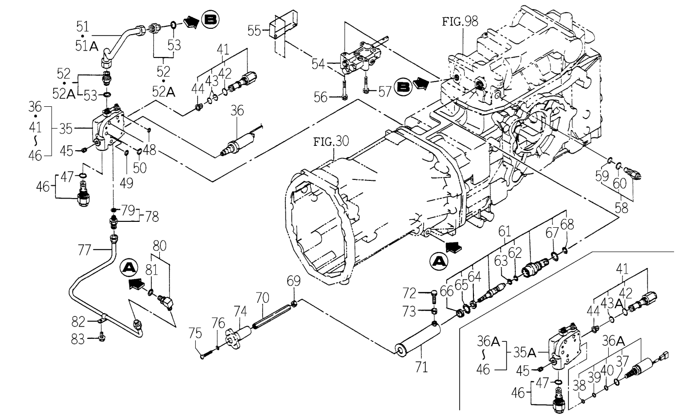
FIG.107 HYD. SYSTEM (MAIN) (H3 TYPE)(2/2)
