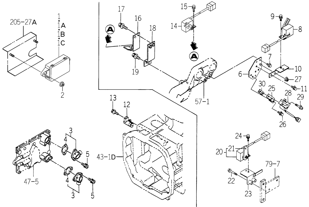
FIG.195 CONTROL SYSTEM (QC TYPE-TG5330E4-No.82-/TG5390E4-No.271-)
