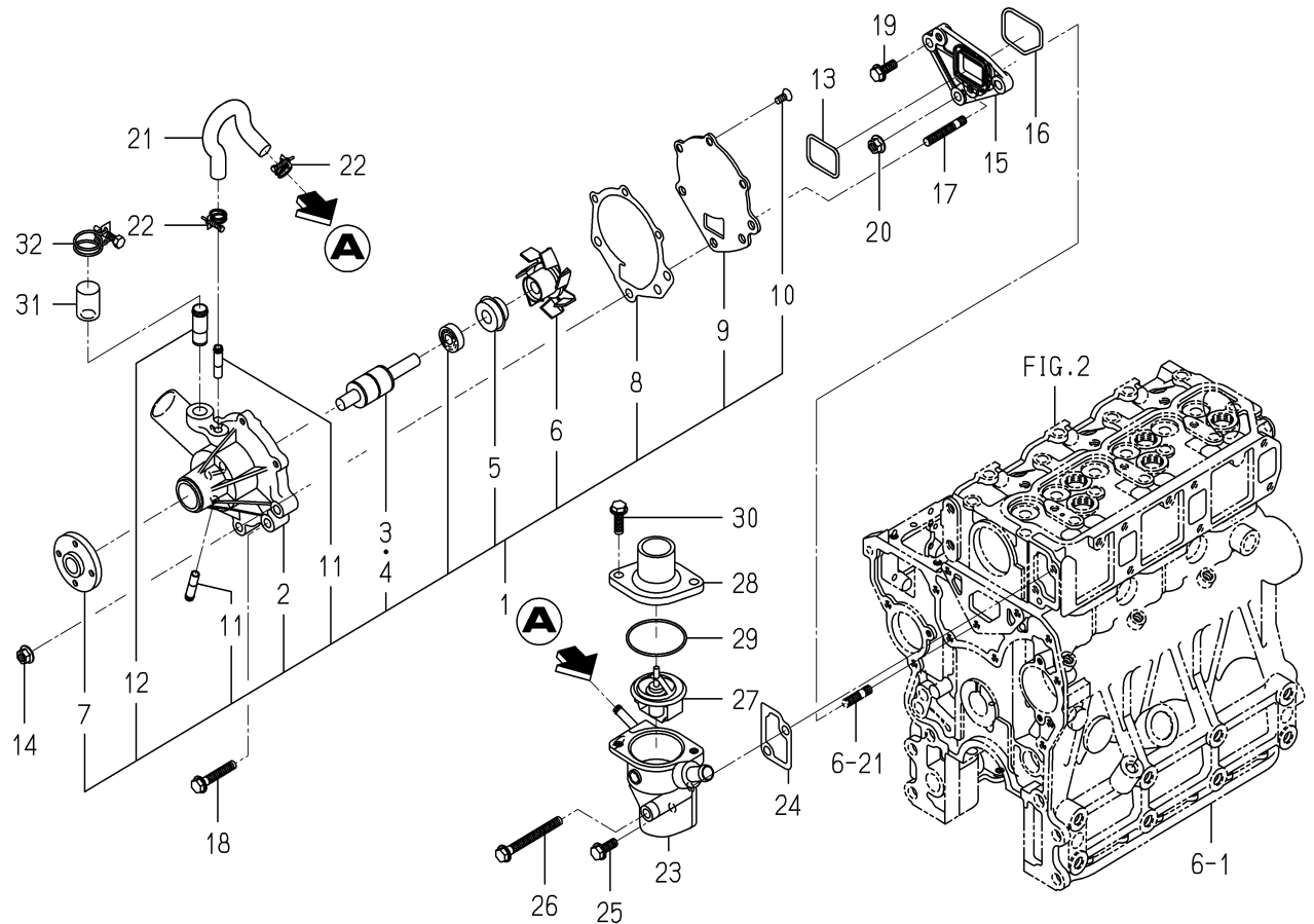
FIG. 18 WATER PUMP
