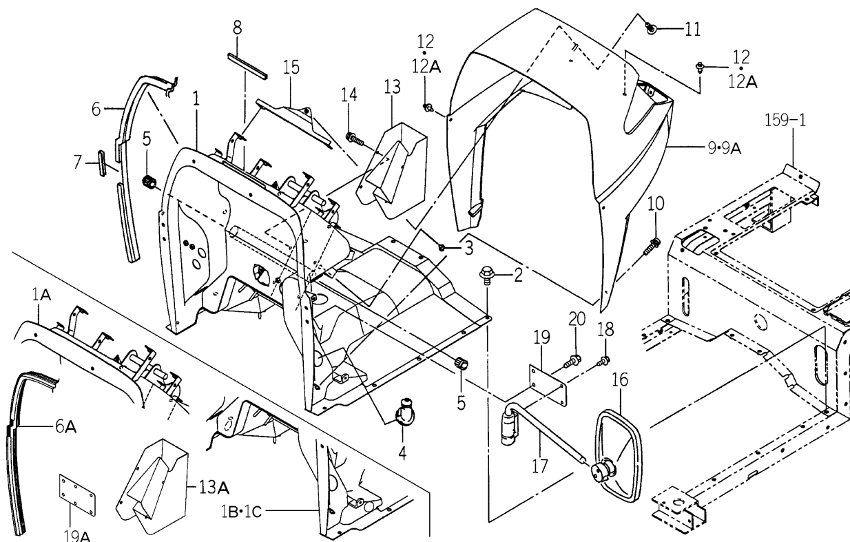
FIG.153 FLOOR (FRONT) SYSTEM (E4 TYPE EXCEPT H,C)
