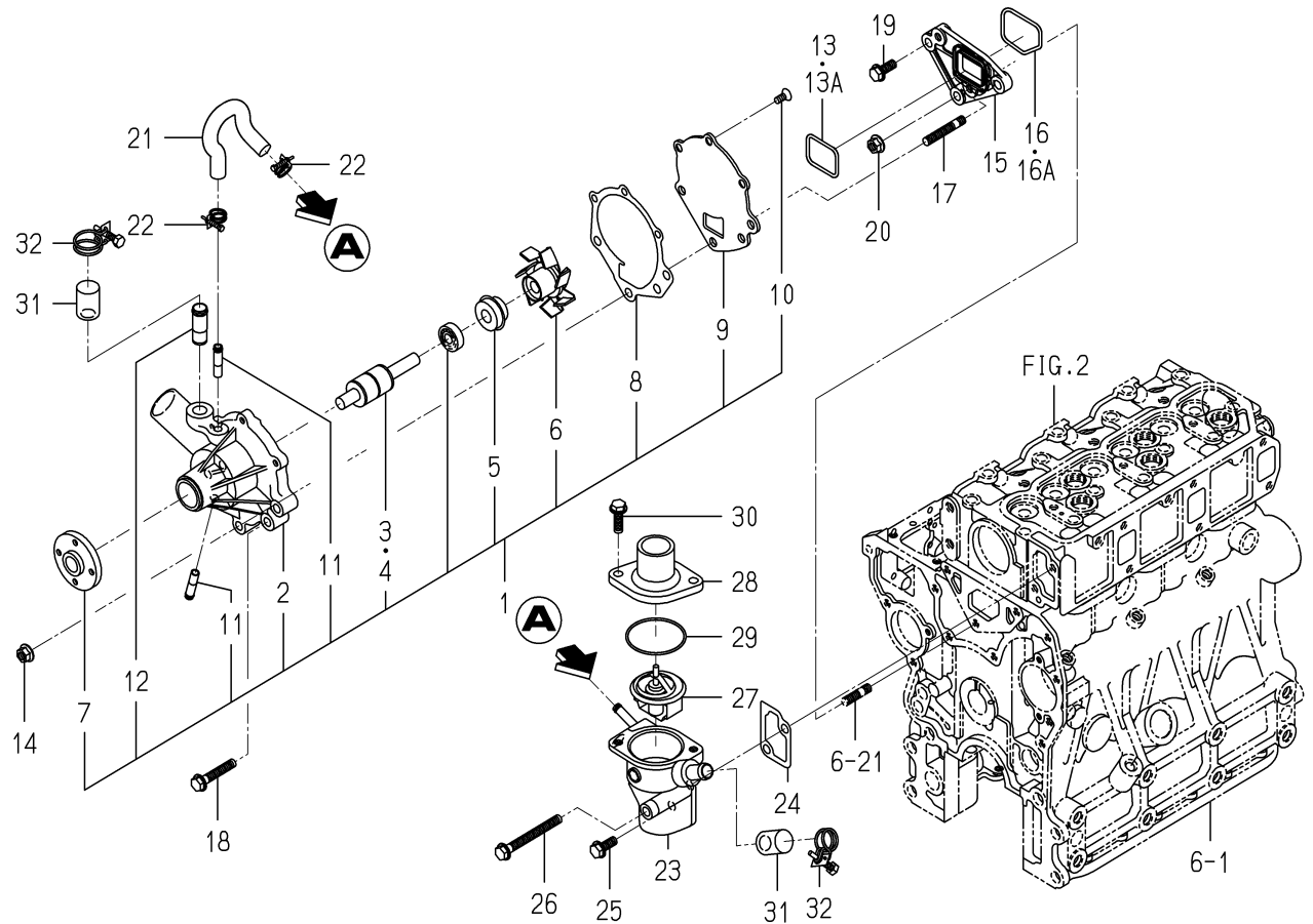
FIG. 20 WATER PUMP
