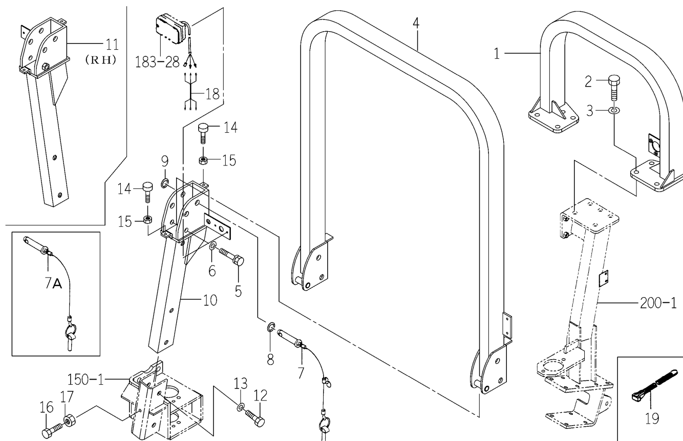
FIG.203 FRAME (REAR) SYSTEM (A TYPE)
