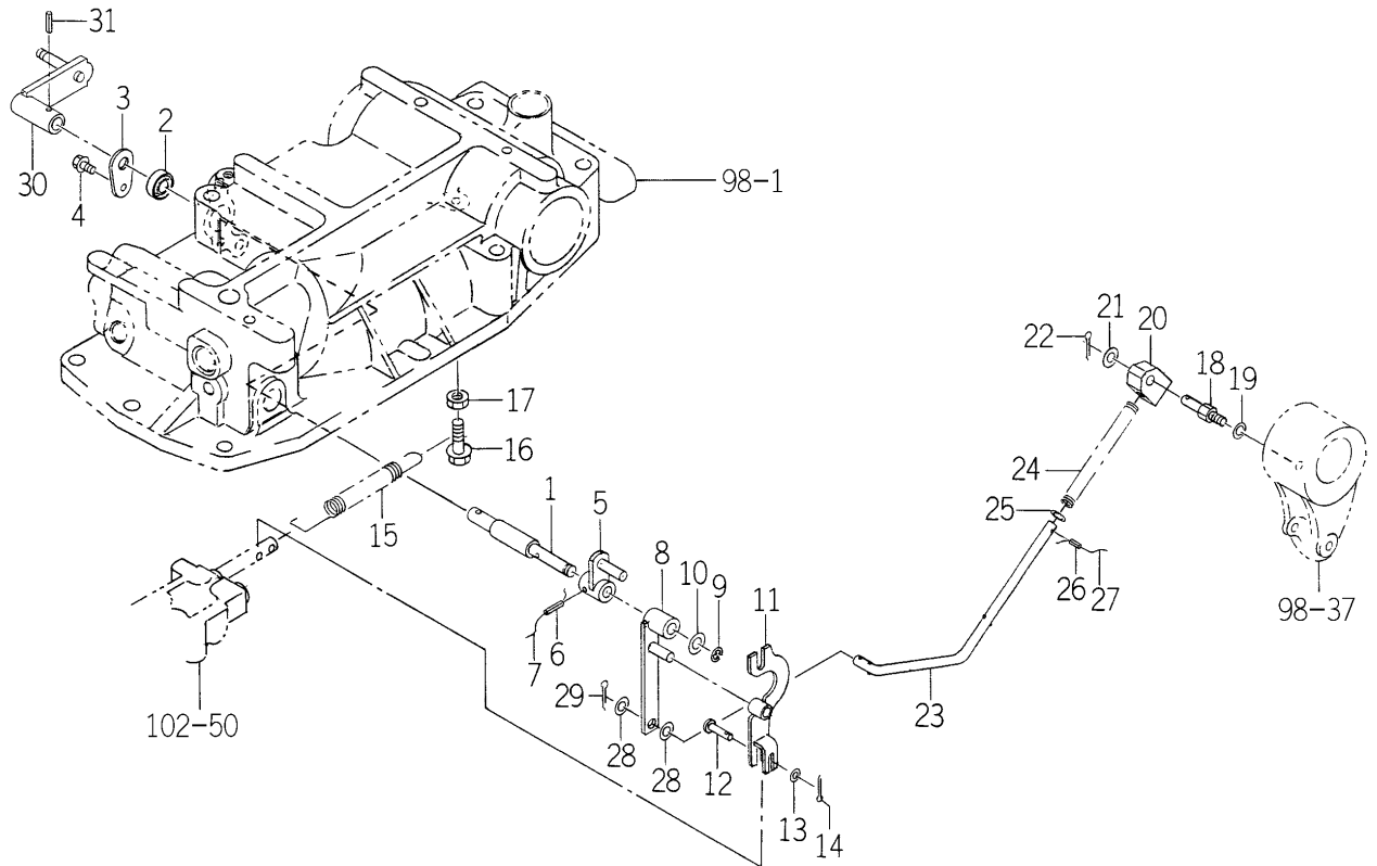
FIG.100 MECHANICAL LINK (POSITION)(1/2) SYSTEM
