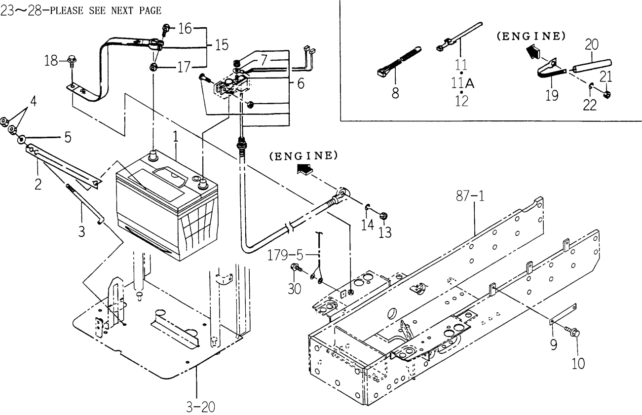
FIG.174 ELC. SYSTEM (FRONT) (E6 TYPE)(1/2)
