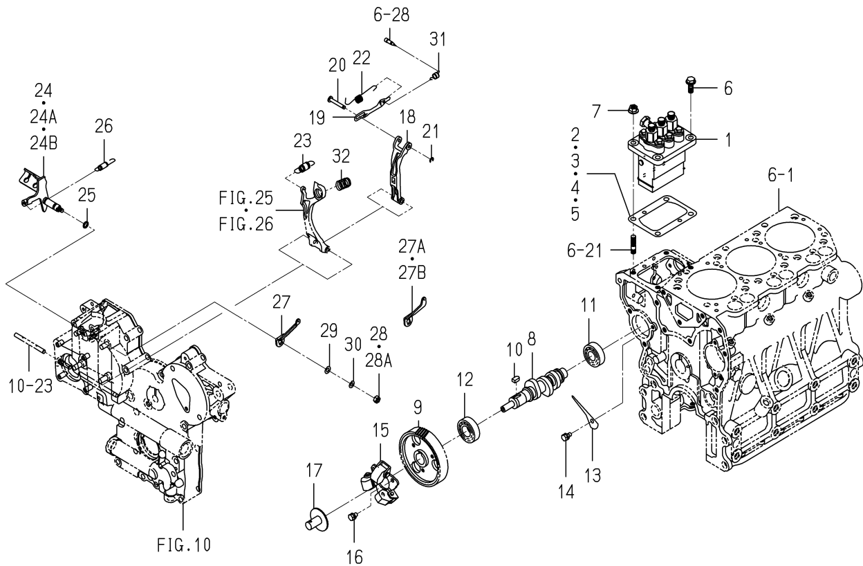
FIG. 21 INJECTION PUMP
