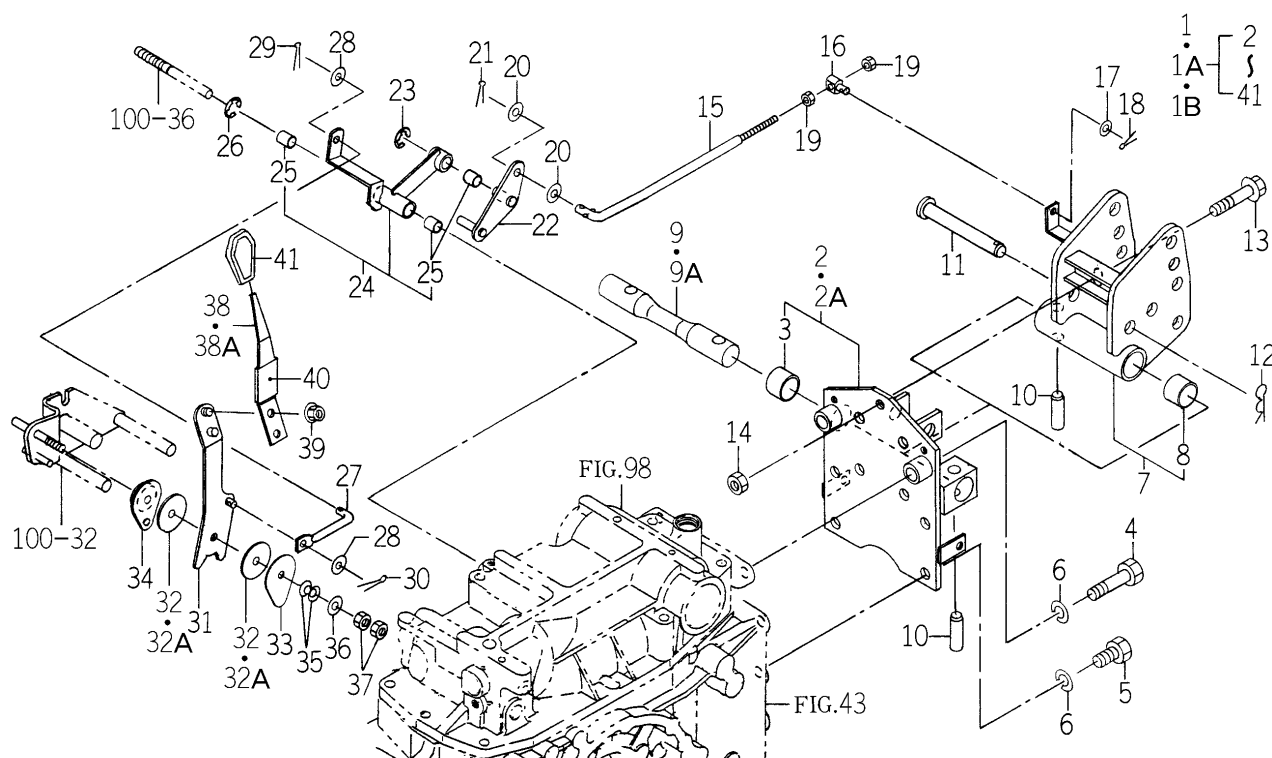
FIG.101 MECHANICAL LINK (DRAFT) SYSTEM (S TYPE-STANDARD/EXCEPT S TYPE-OPTION)
