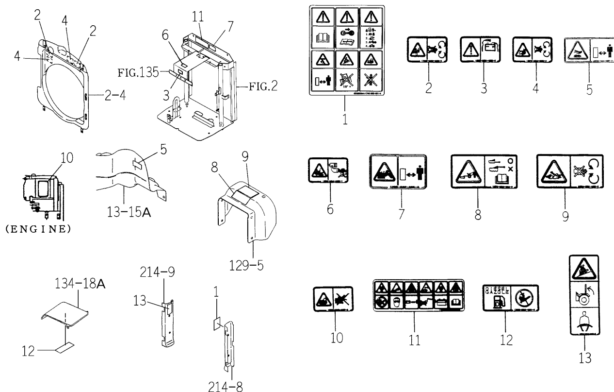
FIG.232 LABEL (CAUTION) (C TYPE-TG5330E4-No.272-/TG5390E4-No.622-)
