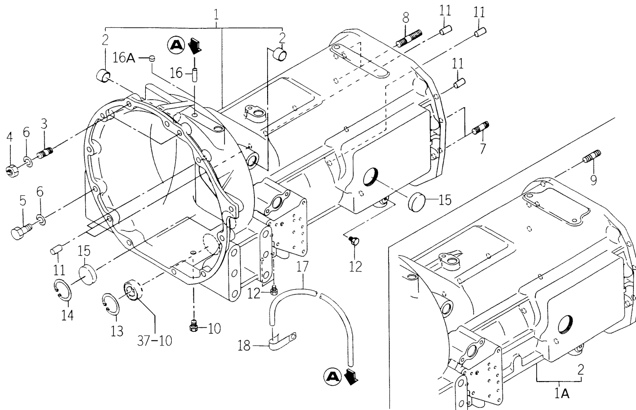
FIG. 20 CASE (TRANSMISSION/FRONT) SYSTEM (P TYPE)
