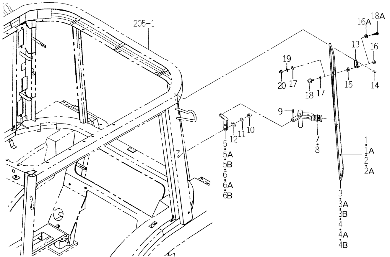
FIG.212 GLASS (SIDE) SYSTEM (C TYPE)
