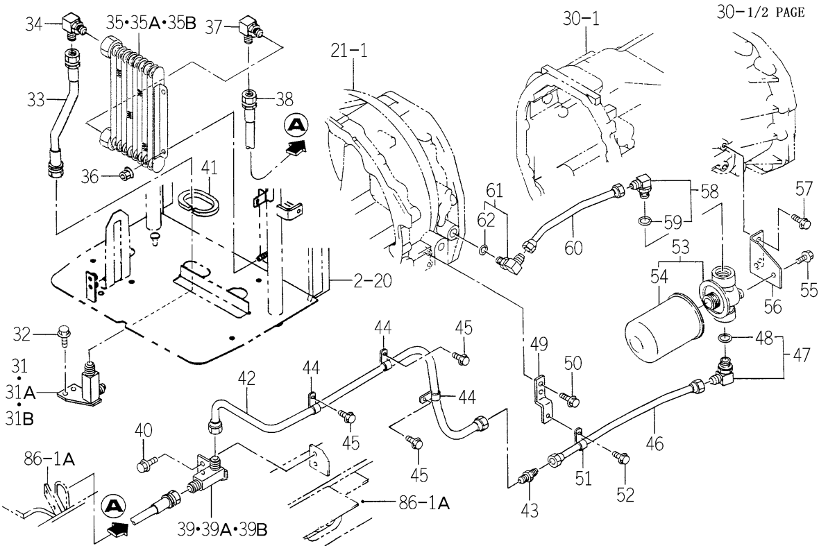
FIG.112 HYD. SYSTEM (SUB)(2/2) (HE4 TYPE EXCEPT H3-No.1-/ HE6 TYPE-TG5390E6-No.1-877)
