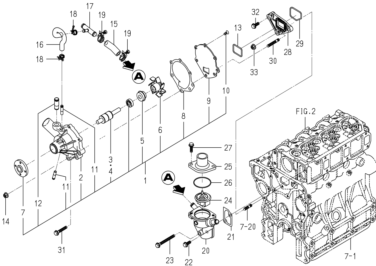
FIG. 20 WATER PUMP
