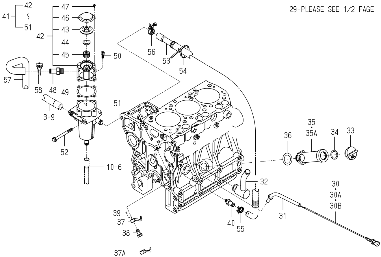
FIG. 8 CYLINDER BLOCK(2/2)
