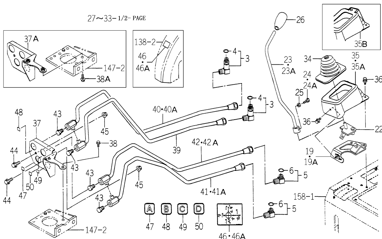
FIG.117 JOY STICK VALVE SET(E6 TYPE-STD-(2/2) TG5330E6-No.1-566/TG5390E6-No.1-881/ E4 TYPE EXCEPT A-OPTION-No.1-)
