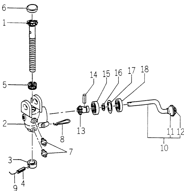
FIG.266 COMPONENT PARTS FOR 1564-527-300-40 ON Fig.125,126
