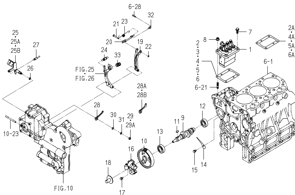
FIG. 23 INJECTION PUMP
