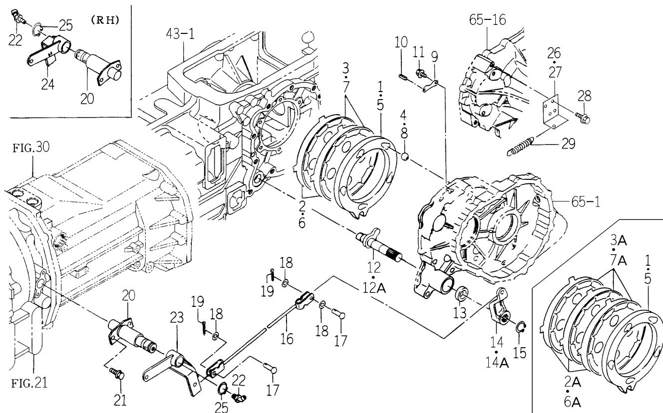
FIG. 70 BRAKE SYSTEM (HE6 TYPE)
