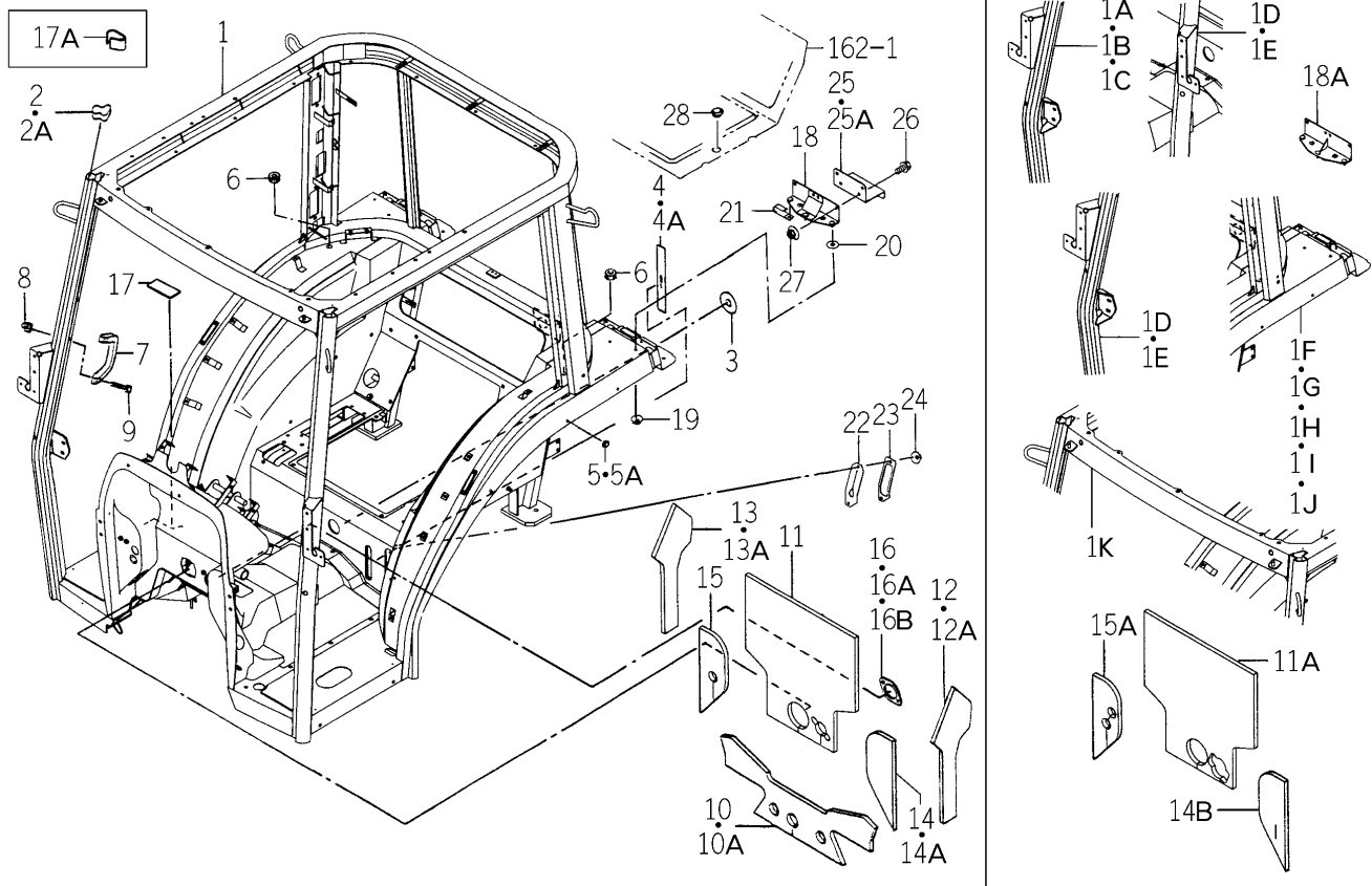
FIG.206 FRAME SYSTEM (HC TYPE EXCEPT H3)
