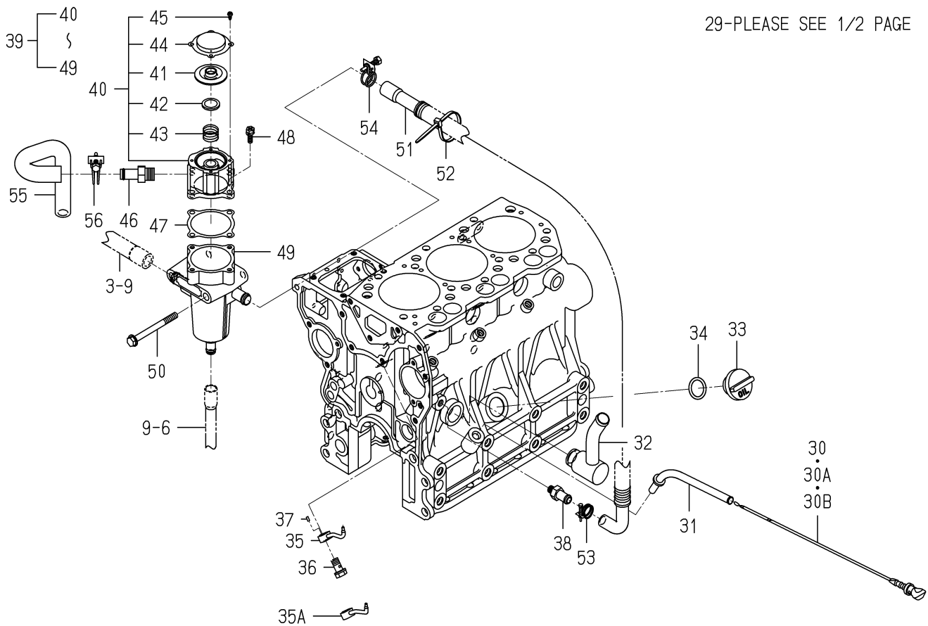
FIG. 7 CYLINDER BLOCK(2/2)
