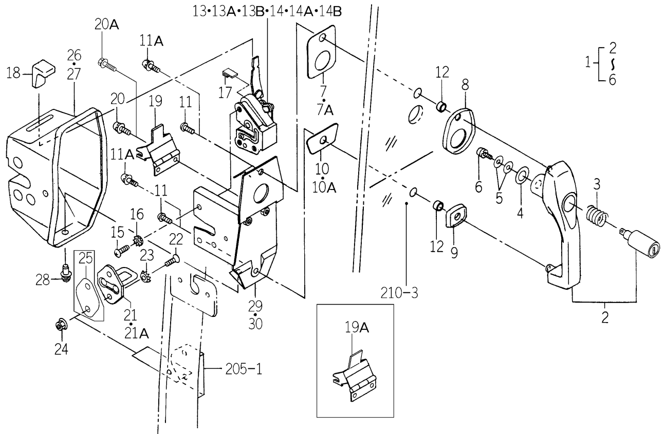
FIG.211 LOCK (DOOR) SYSTEM (C TYPE)
