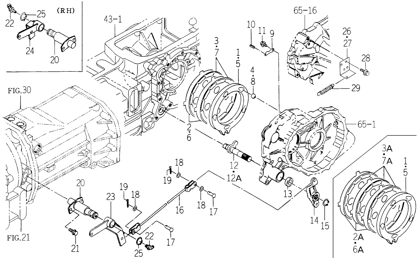
FIG. 73 BRAKE SYSTEM (HE4 TYPE EXCEPT H3)
