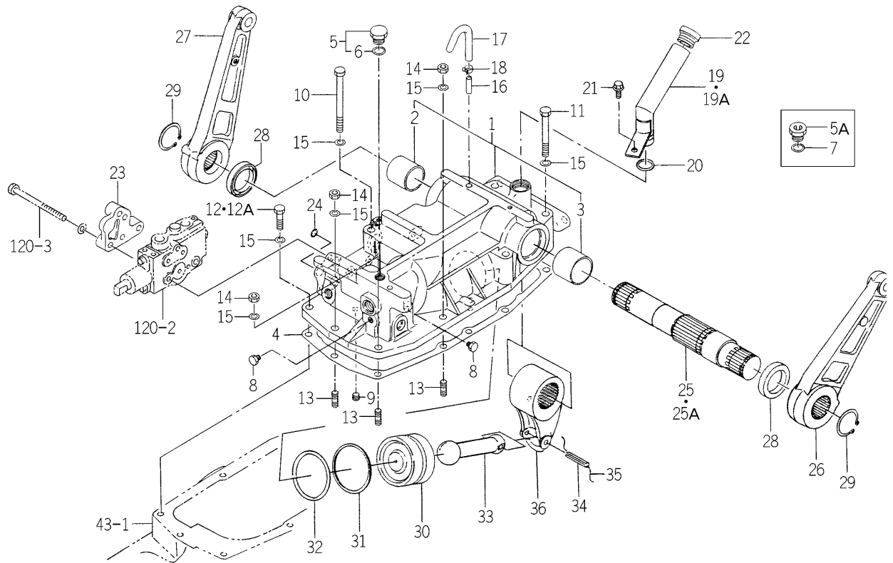
FIG. 99 CYLINDER CASE SYSTEM (W TYPE-No.1-/ A TYPE-TG5330E4-No.160-/ TG5390E4-No.520-)
