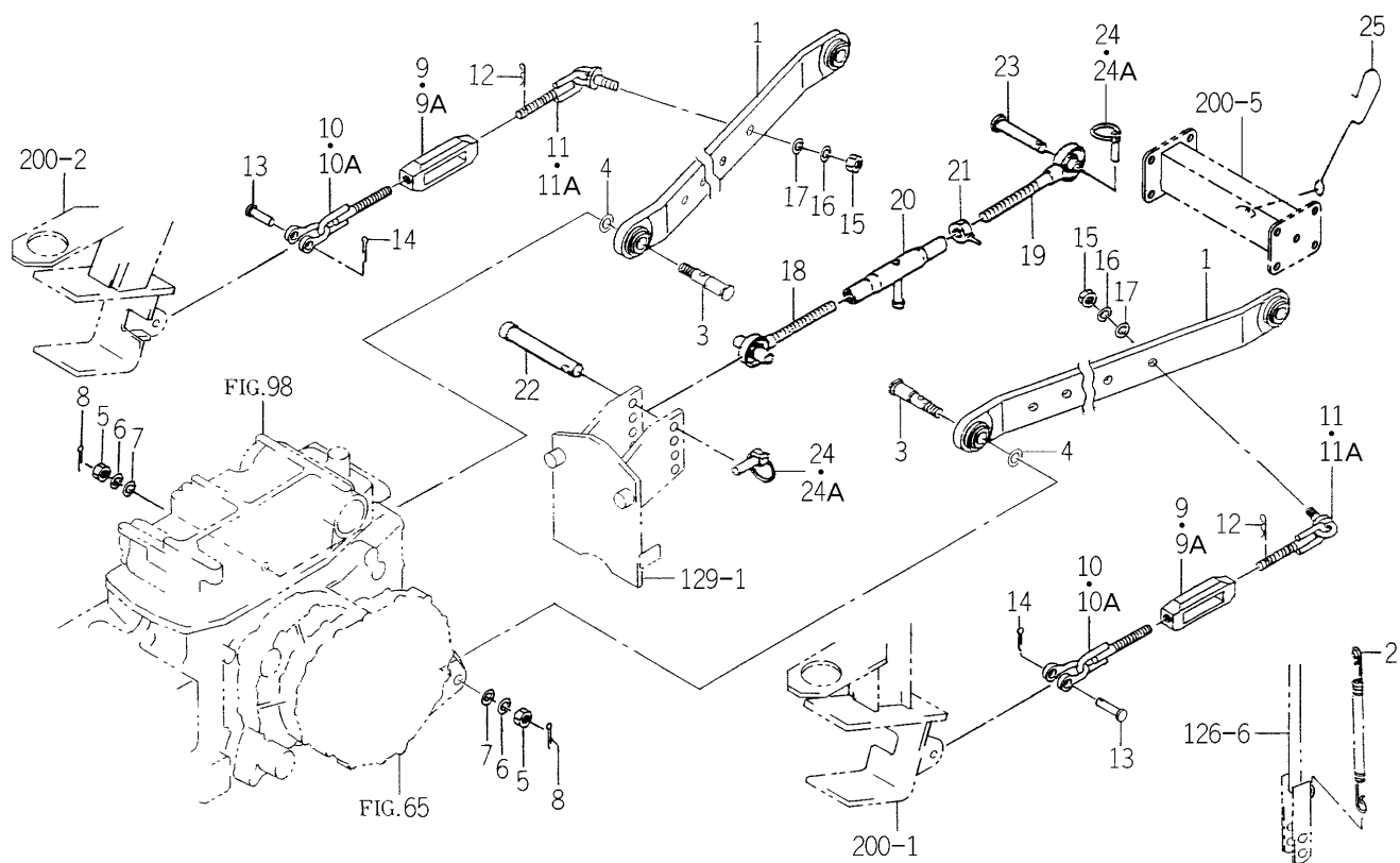
FIG.123 3P LINK SYSTEM (E4 TYPE EXCEPT C)
