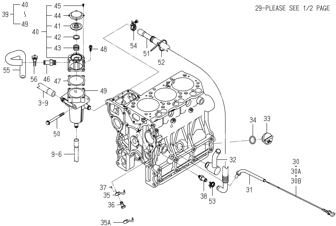
FIG. 7 CYLINDER BLOCK(2/2)
