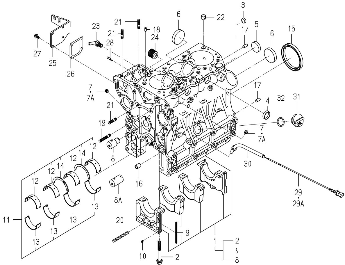
FIG. 6 CYLINDER BLOCK
