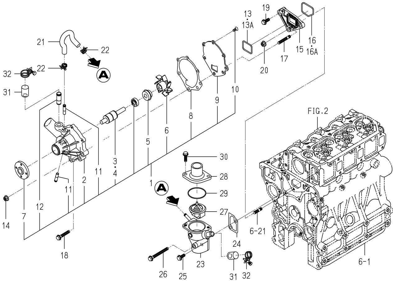
FIG. 20 WATER PUMP
