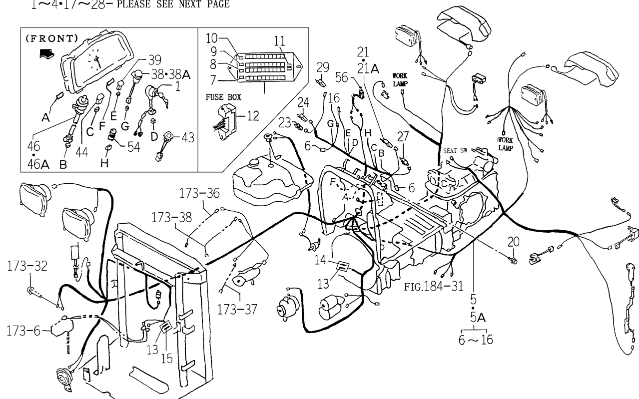
FIG.181 ELC. SYSTEM (MAIN) (H3 TYPE)(1/3)
