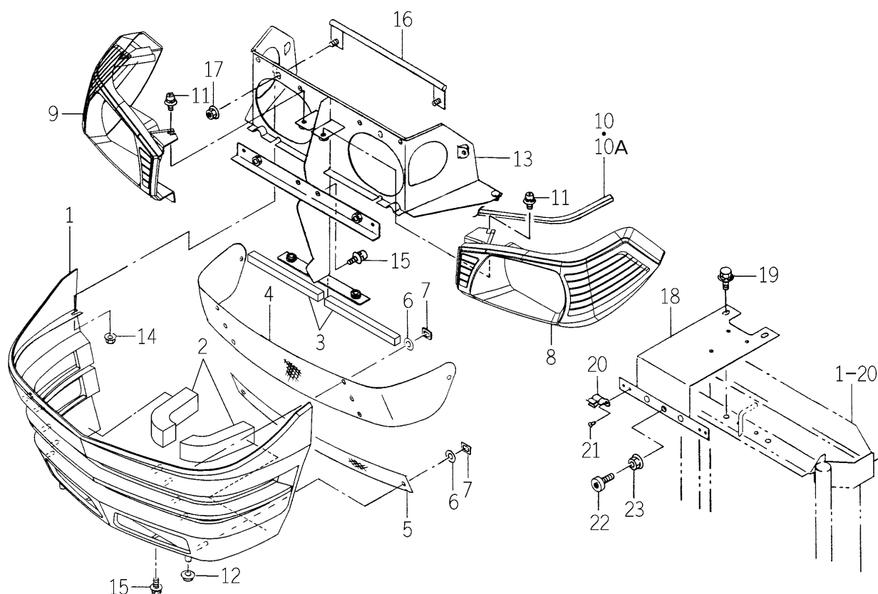
FIG.135 GRILLE SYSTEM
