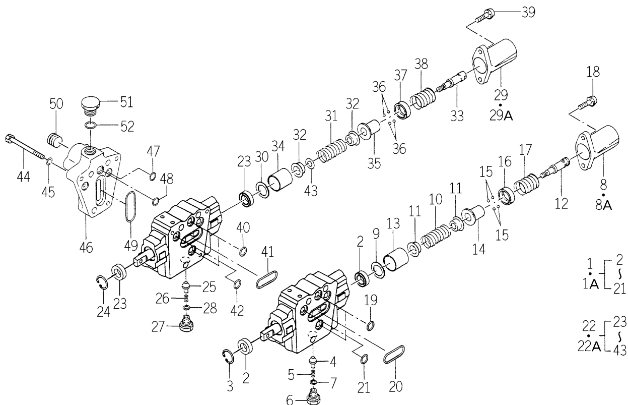
FIG.264 COMPONENT PARTS FOR K211-074-000-00,10 ON Fig.117,118
