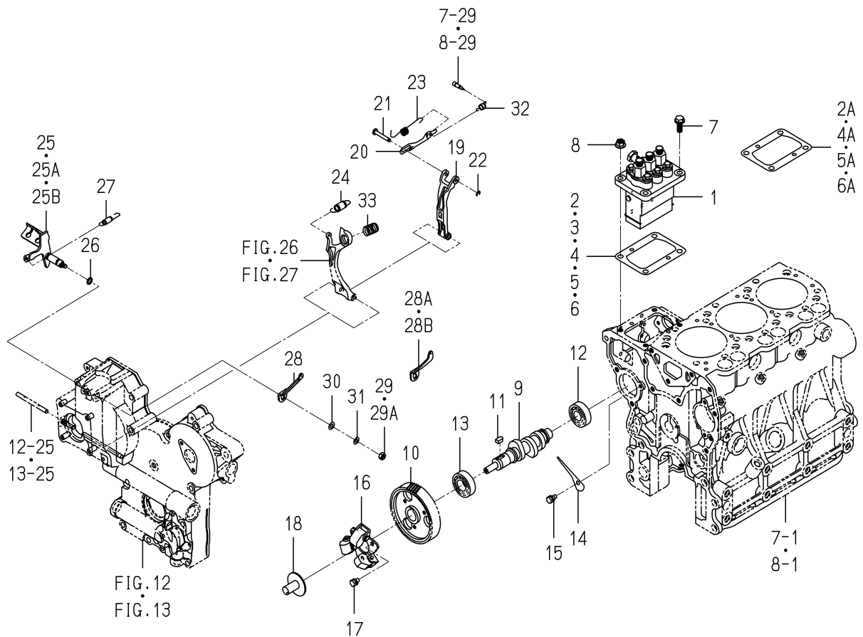
FIG. 24 INJECTION PUMP
