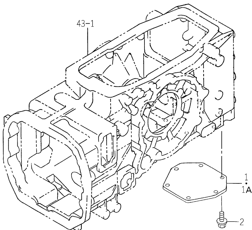
FIG. 40 COVER (MID PTO) SYSTEM (EXCEPT M TYPE)
