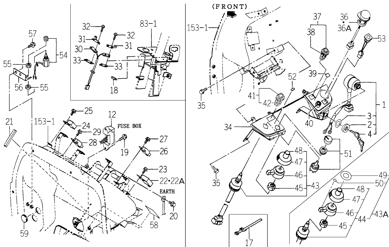
FIG.178 ELC. SYSTEM (MAIN) (Q TYPE)(2/2)
