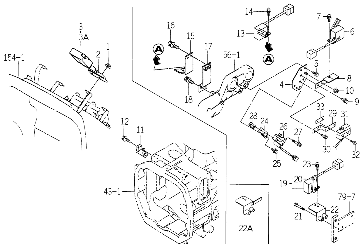
FIG.192 CONTROL SYSTEM (HE4 TYPE EXCEPT H3)
