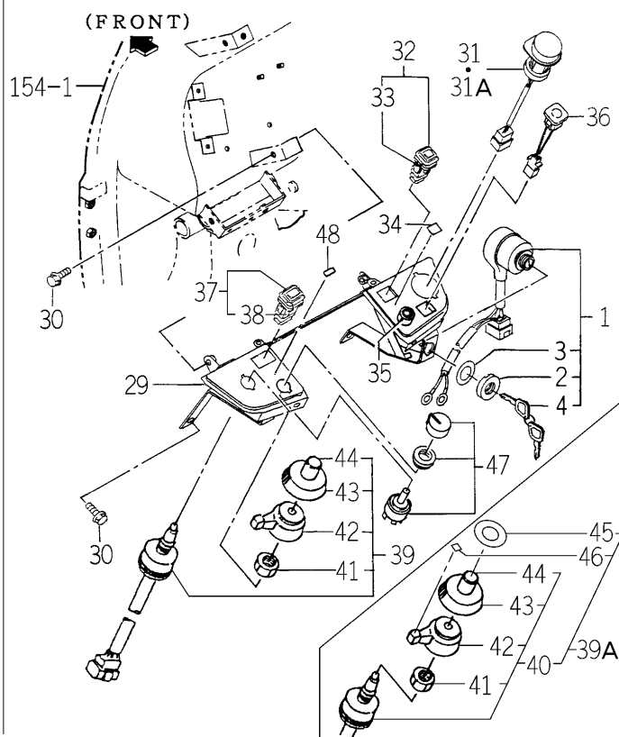
FIG.177 ELC. SYSTEM (MAIN)(2/2) (HE4 TYPE EXCEPT H3)
