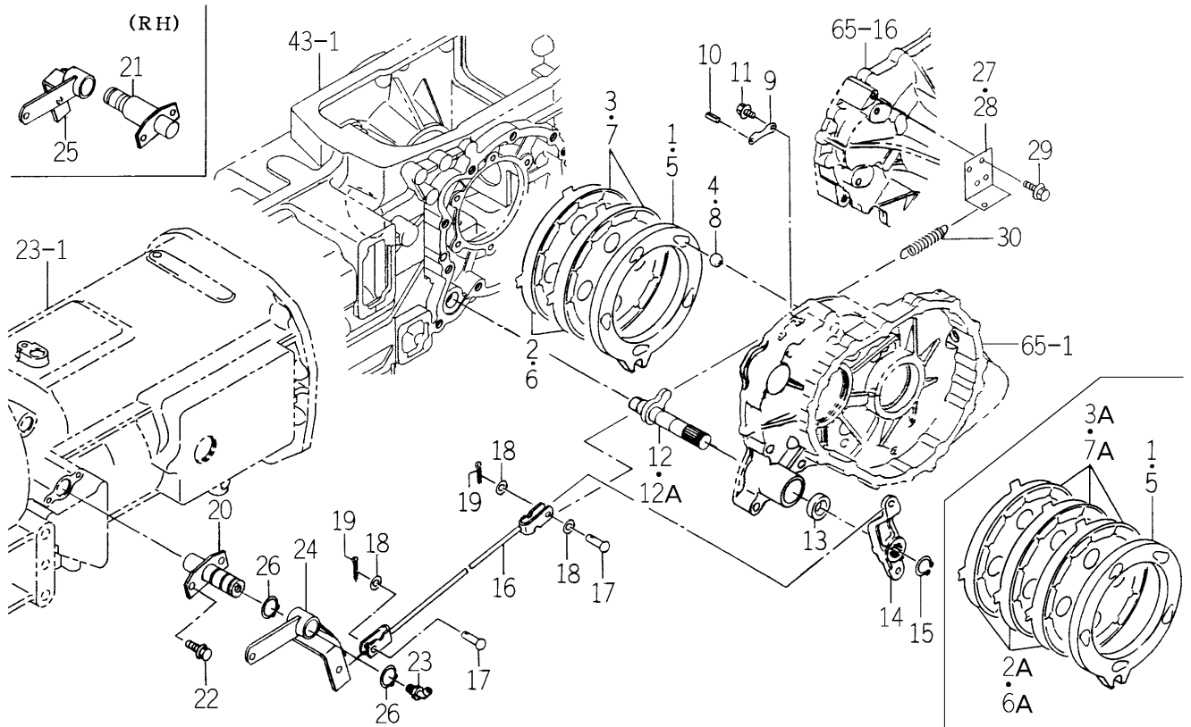
FIG. 72 BRAKE SYSTEM (E4 TYPE EXCEPT H)
