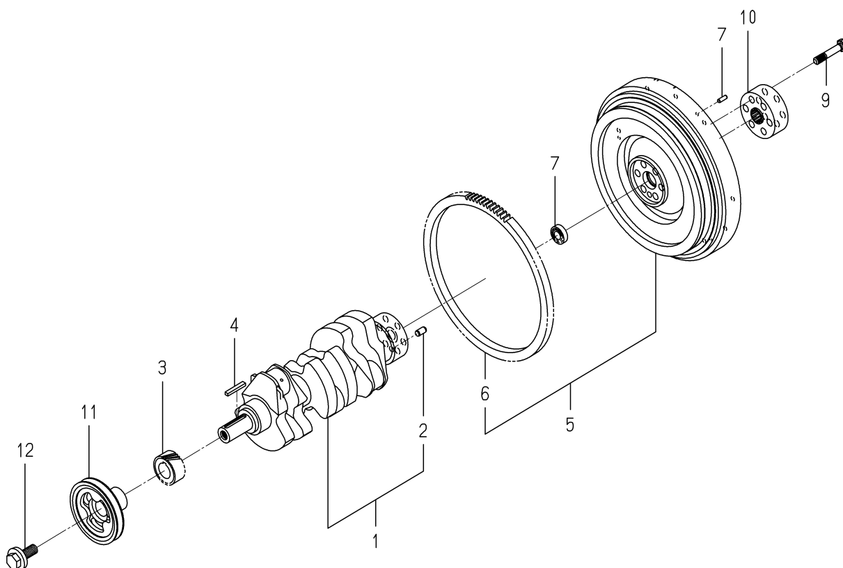
FIG. 17 CRANK SHAFT
