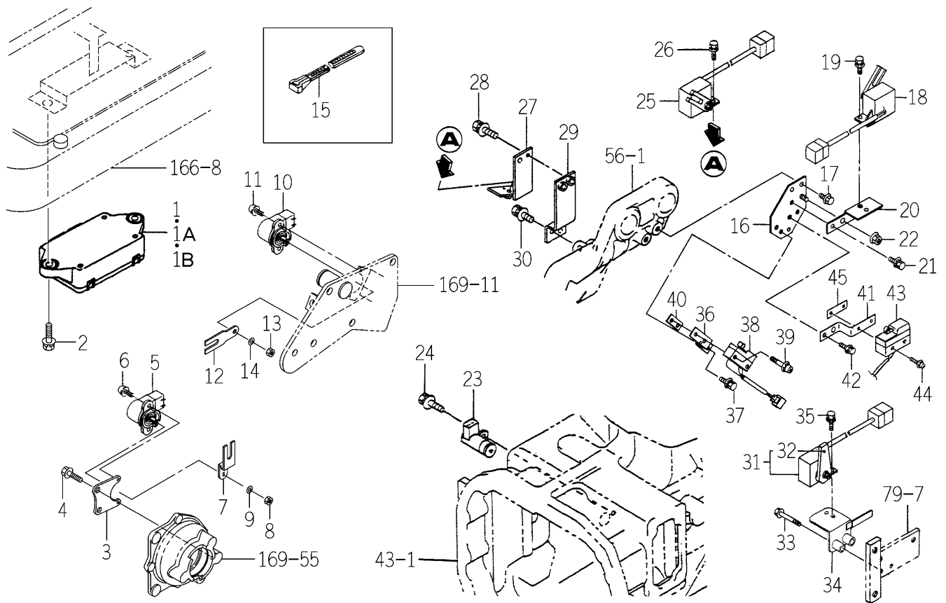
FIG.194 CONTROL SYSTEM (H3 TYPE EXCEPT C)
