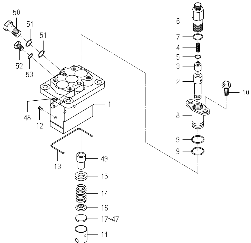
FIG. 32 COMPONENT PARTS FOR 6215-600-104-20 ON Fig.23
