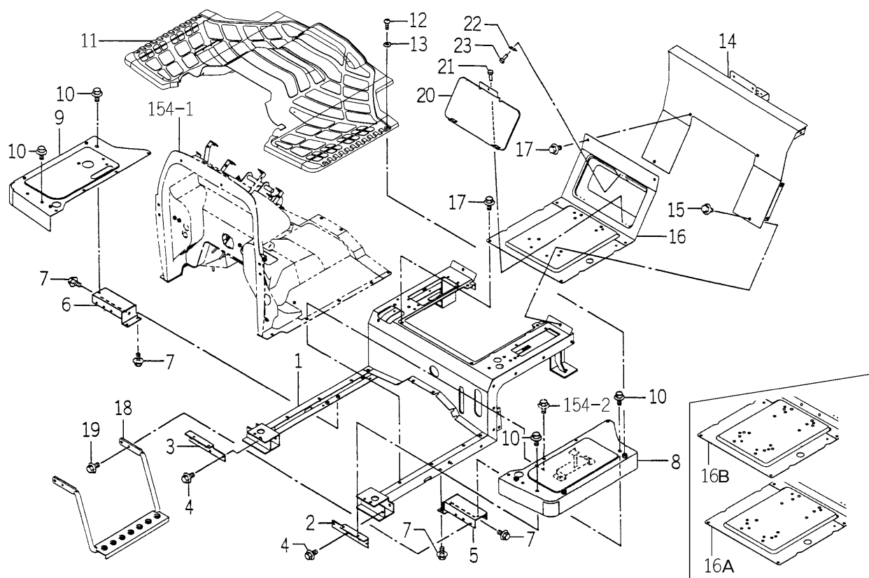
FIG.166 FLOOR (REAR) SYSTEM (H3 TYPE EXCEPT C)
