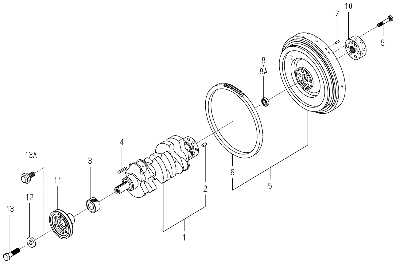
FIG. 16 CRANK SHAFT
