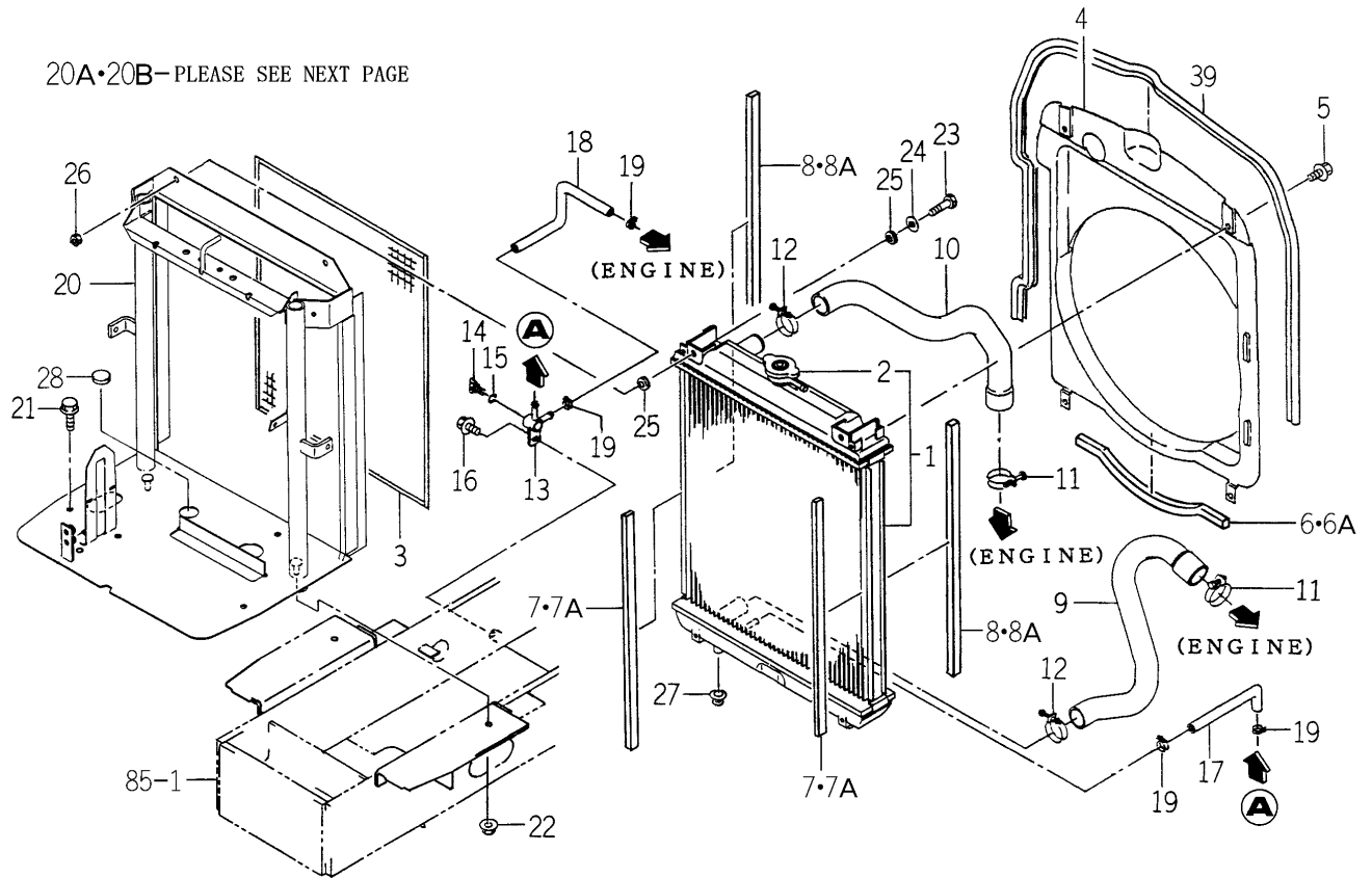
FIG. 3 RADIATOR SYSTEM (P,Q TYPE)(1/2)
