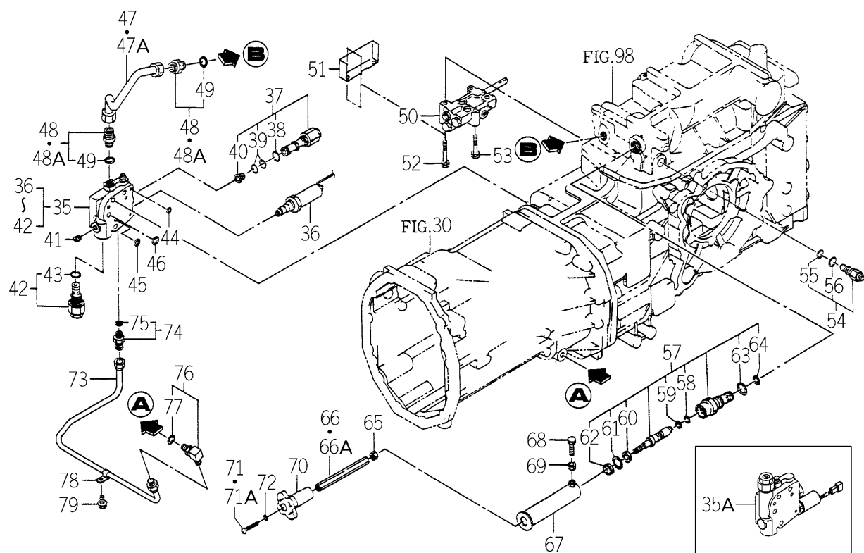
FIG.103 HYD. SYSTEM (MAIN)(2/2) (H TYPE EXCEPT H3-TG5390E4-No.1-774)
