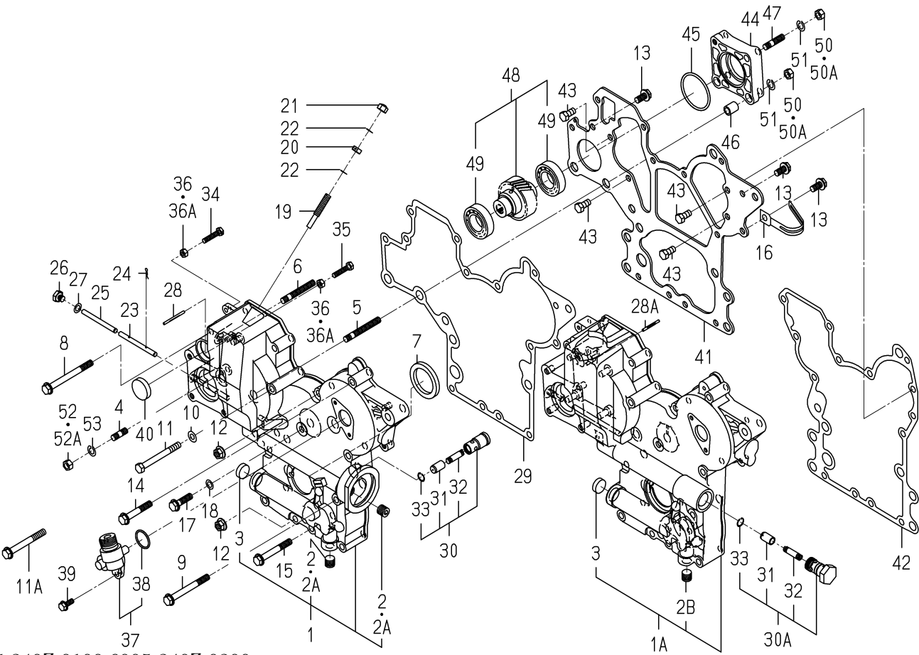
FIG. 11 TIMING GEAR CASE
