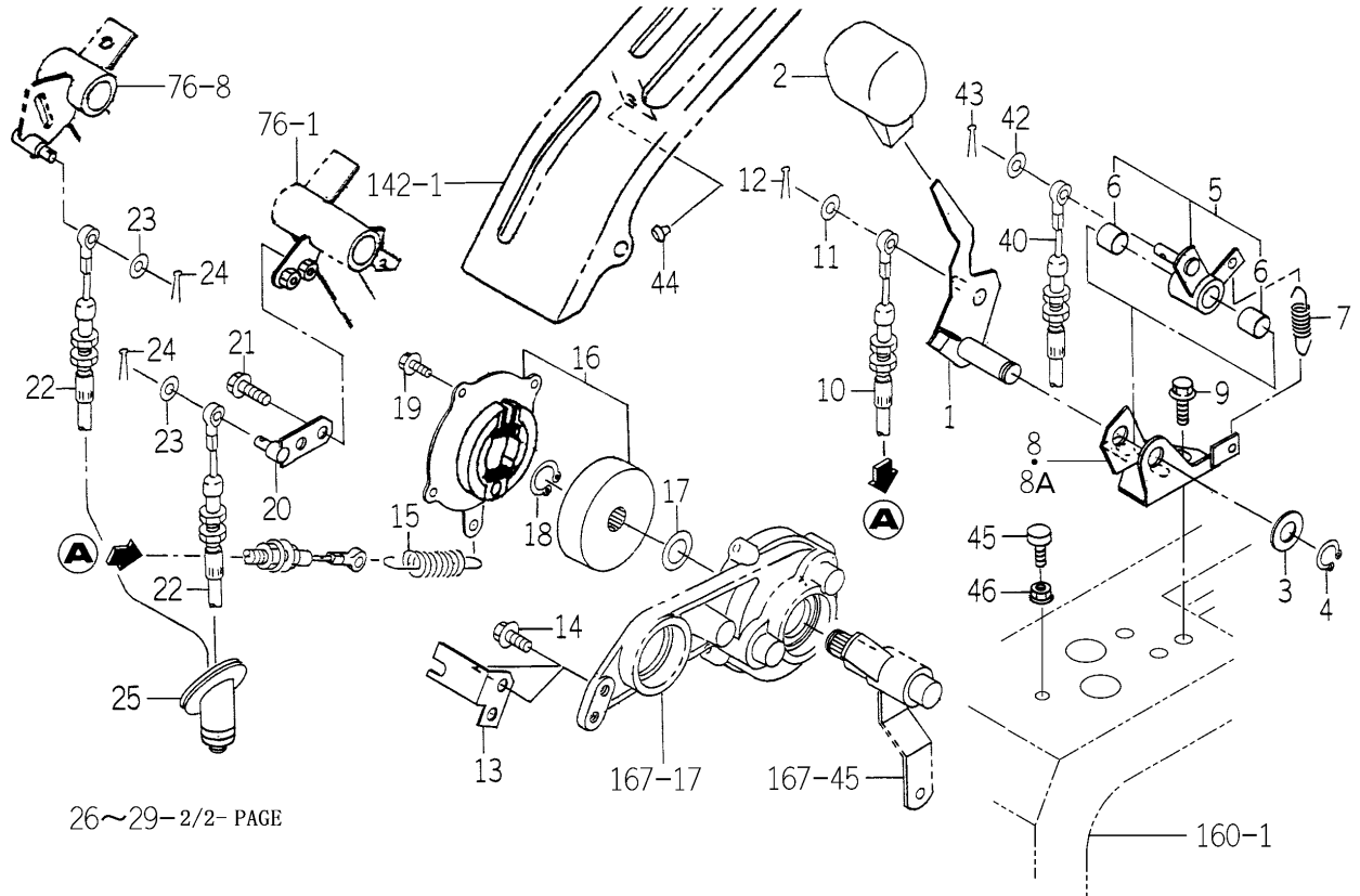
FIG.170 CRUISE CONTROL SYSTEM(1/2) (H TYPE EXCEPT H3)
