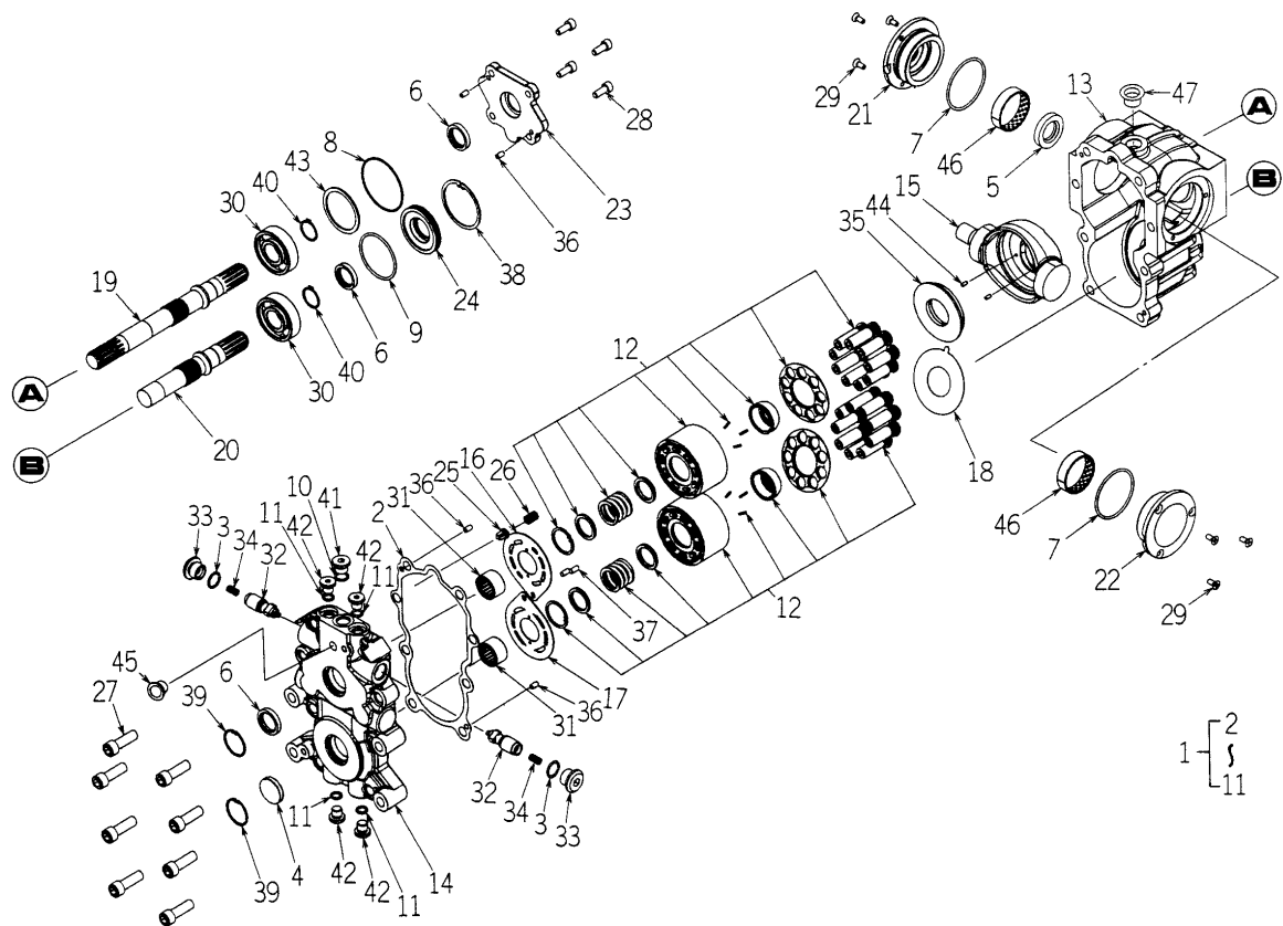
FIG.277 COMPONENT PARTS FOR 1743-203-510-10 ON Fig.25
