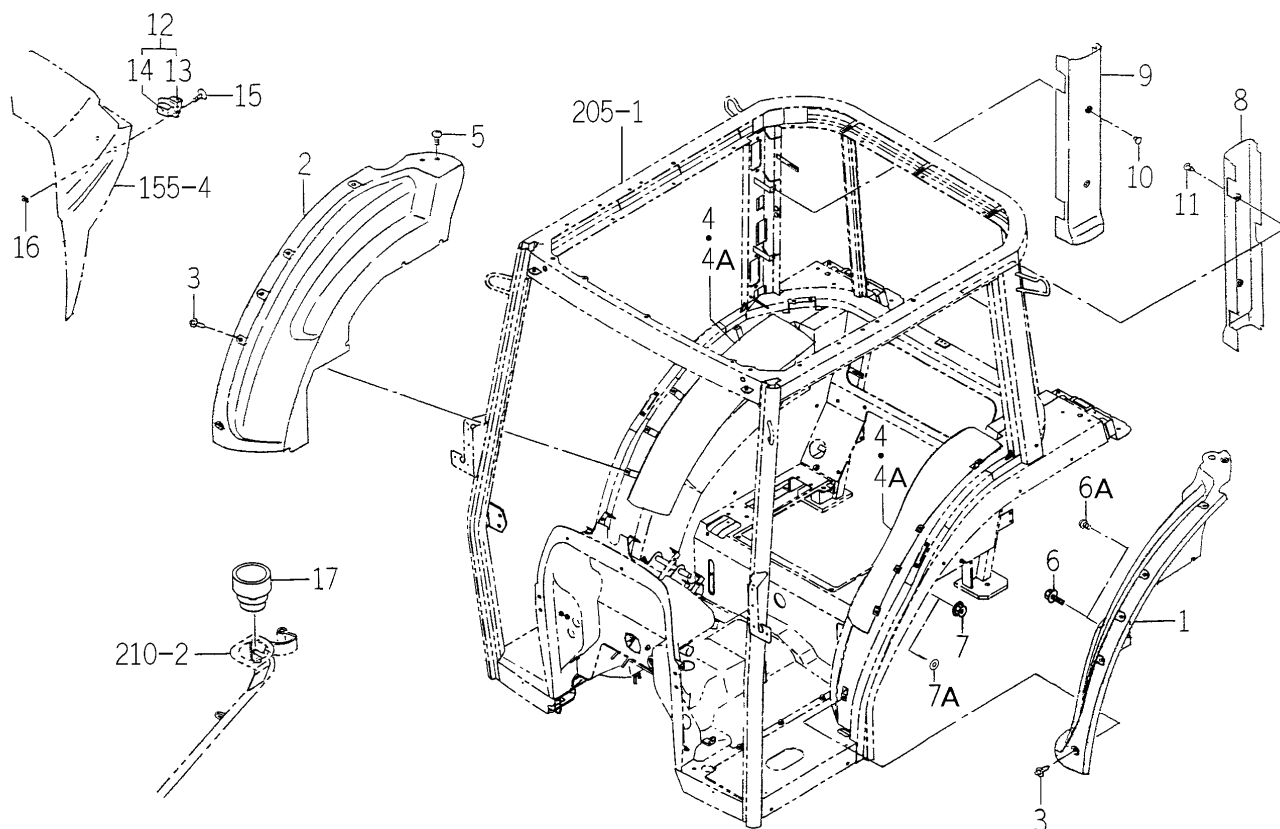
FIG.214 INTERIOR SYSTEM (C TYPE)
