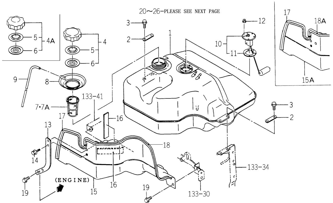
FIG. 13 TANK (FUEL) SYSTEM (TG5330-E4 TYPE)(1/2)
