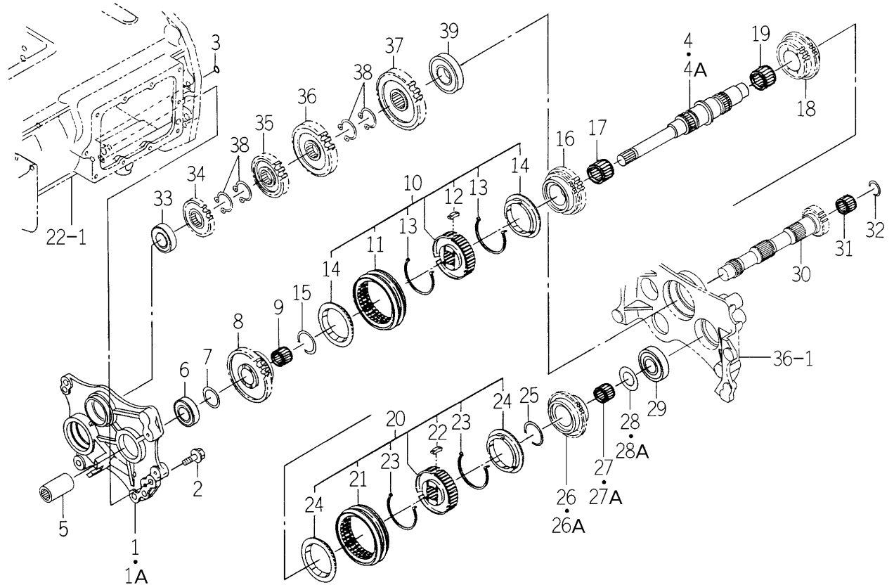
FIG. 33 GEAR (MAIN) SYSTEM (Q TYPE)
