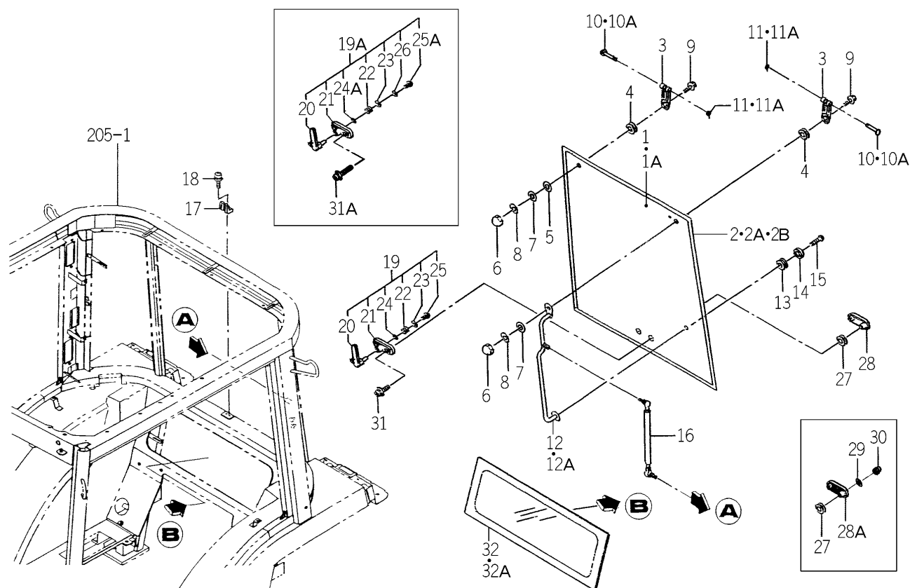
FIG.213 GLASS (REAR) SYSTEM (C TYPE)
