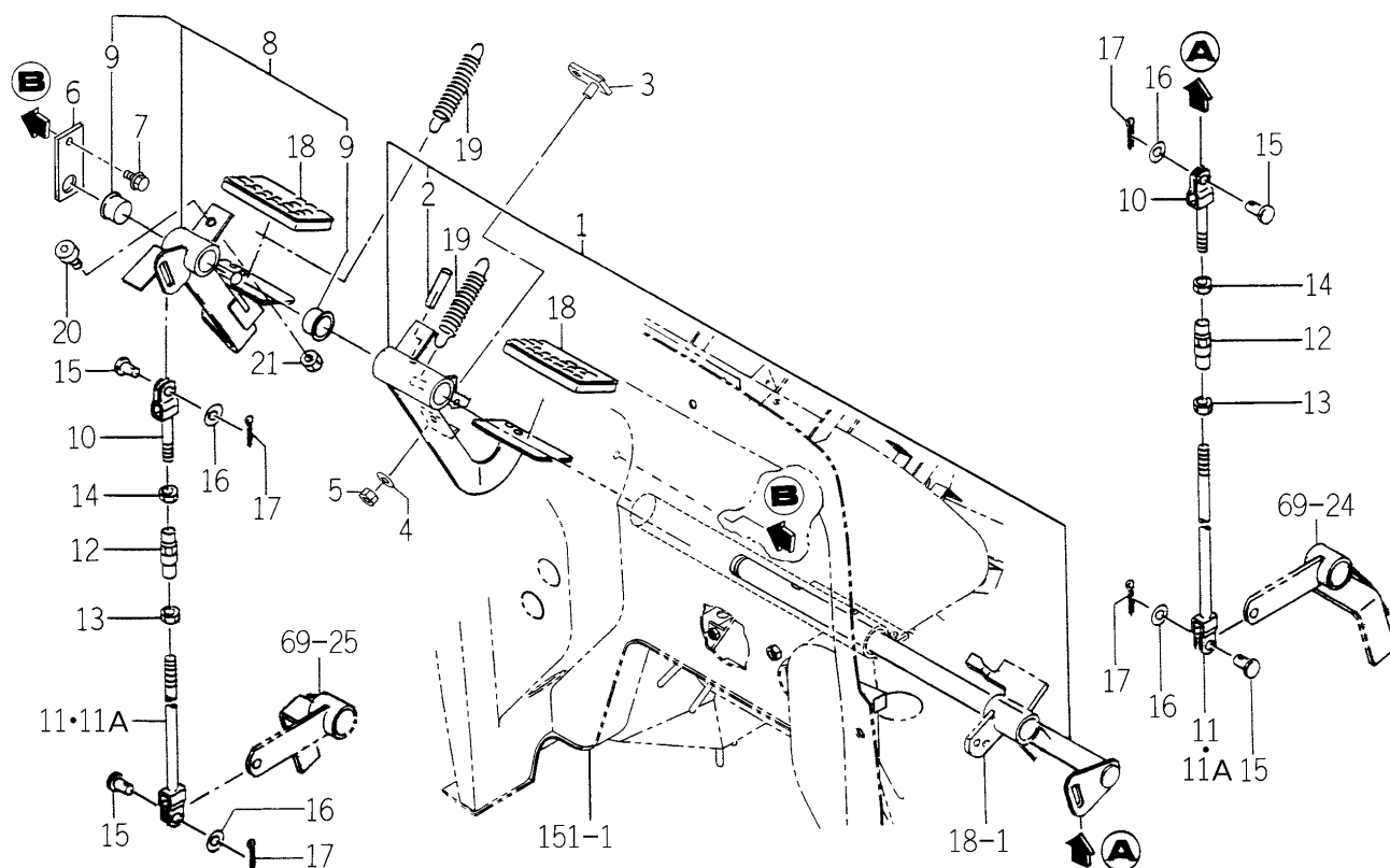
FIG. 74 PEDAL (BRAKE) SYSTEM (E6 TYPE EXCEPT H)
