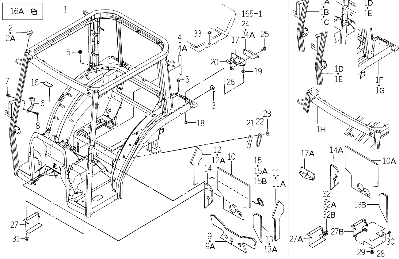
FIG.205 FRAME SYSTEM (C TYPE EXCEPT H)
