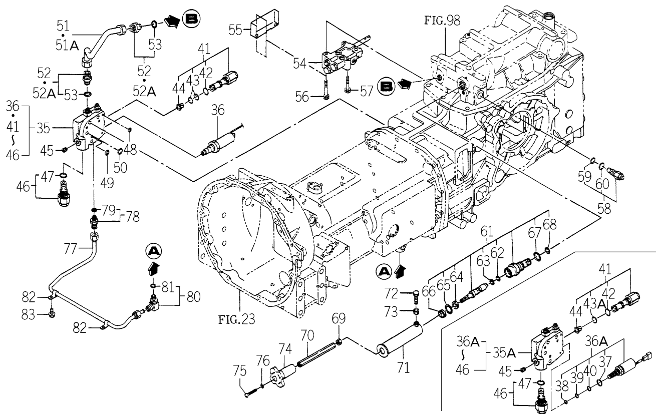
FIG.106 HYD. SYSTEM (MAIN)(2/2) (S TYPE-TG5330E4-No.440-/TG5390E4-No.776-)
