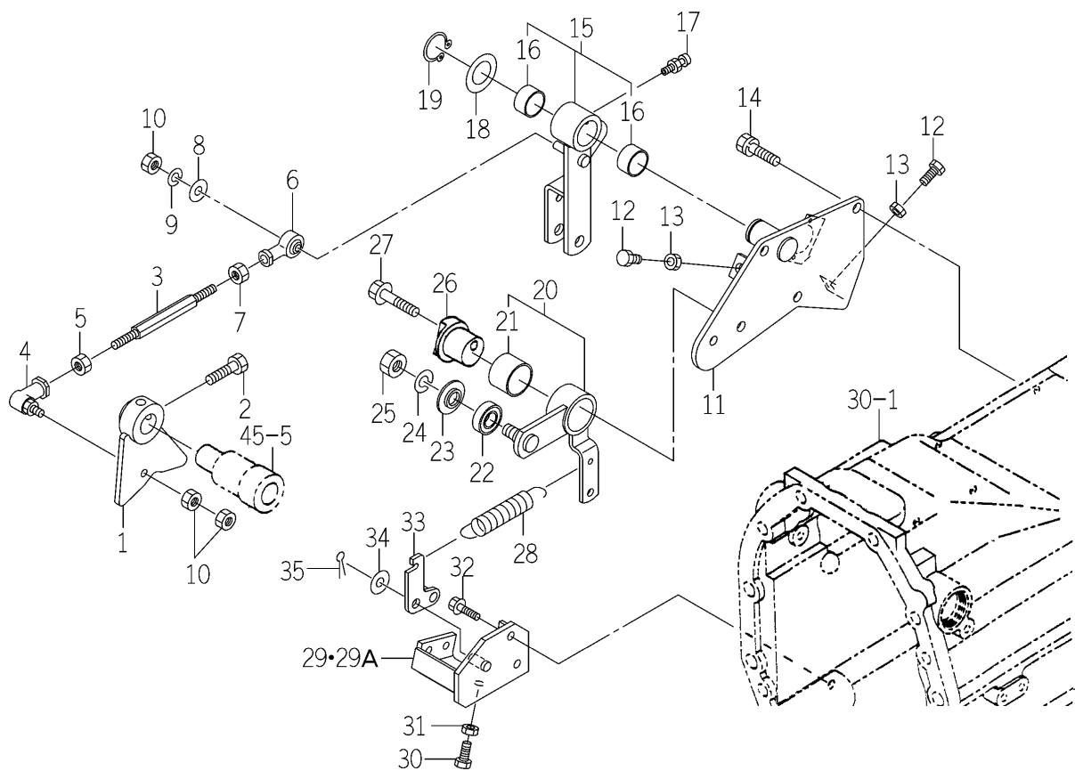
FIG.169 PEDAL (HST) SYSTEM (H3 TYPE)(1/2)
