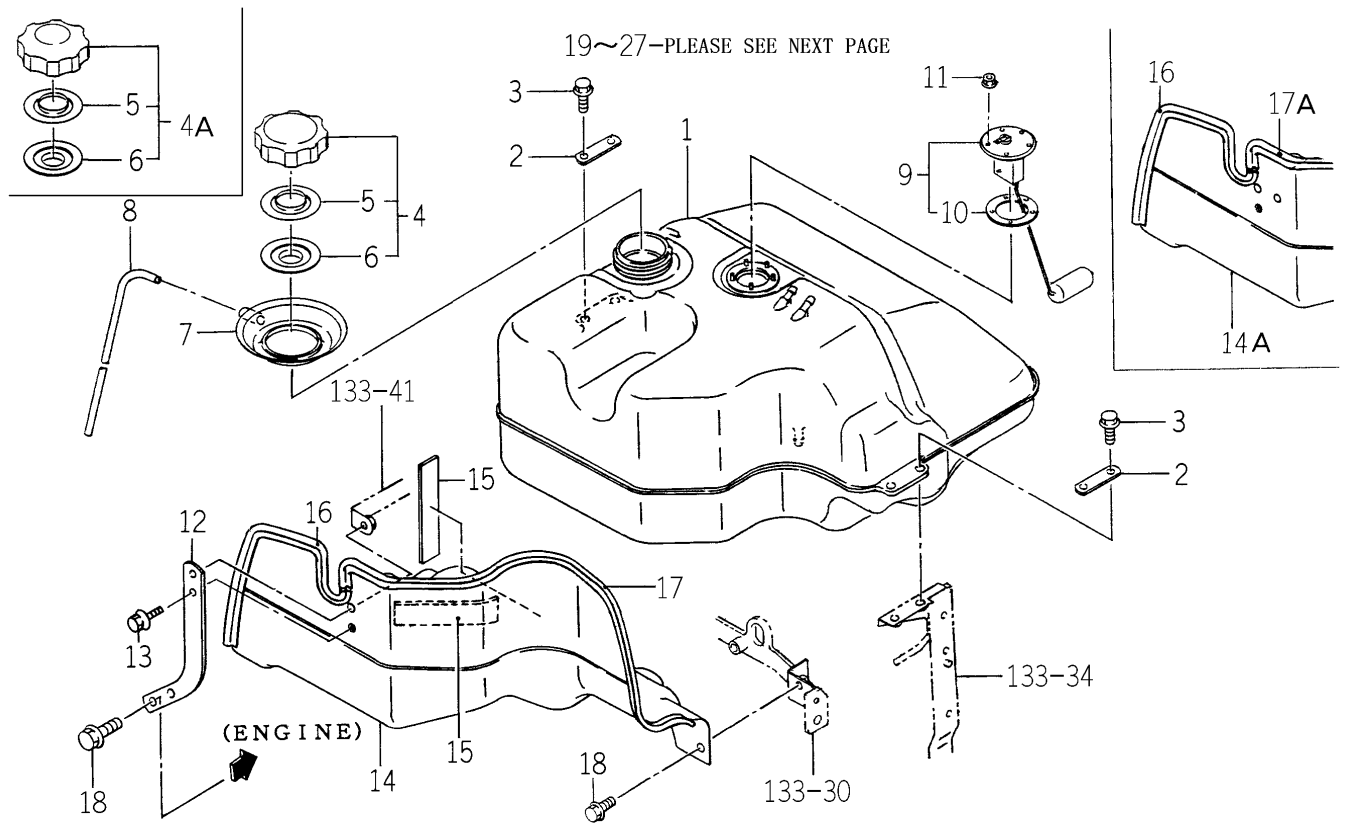
FIG. 11 TANK (FUEL) SYSTEM (TG5330-E6 TYPE)(1/2)
