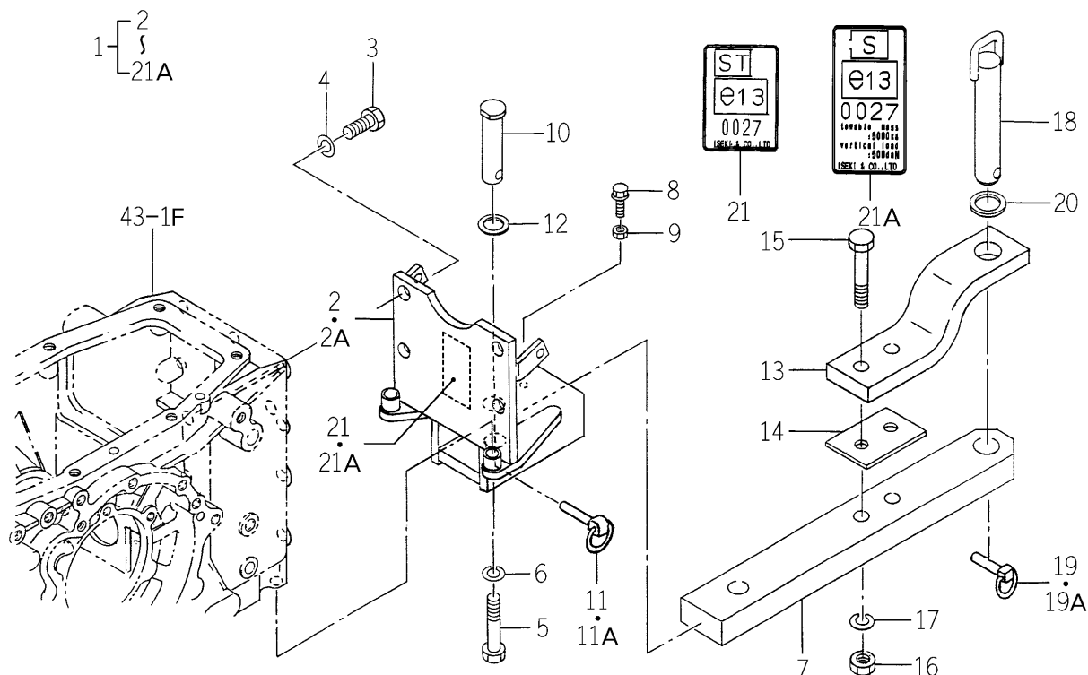
FIG.250 DRAW BAR (FIX) SYSTEM (E4D TYPE-OPTION)
