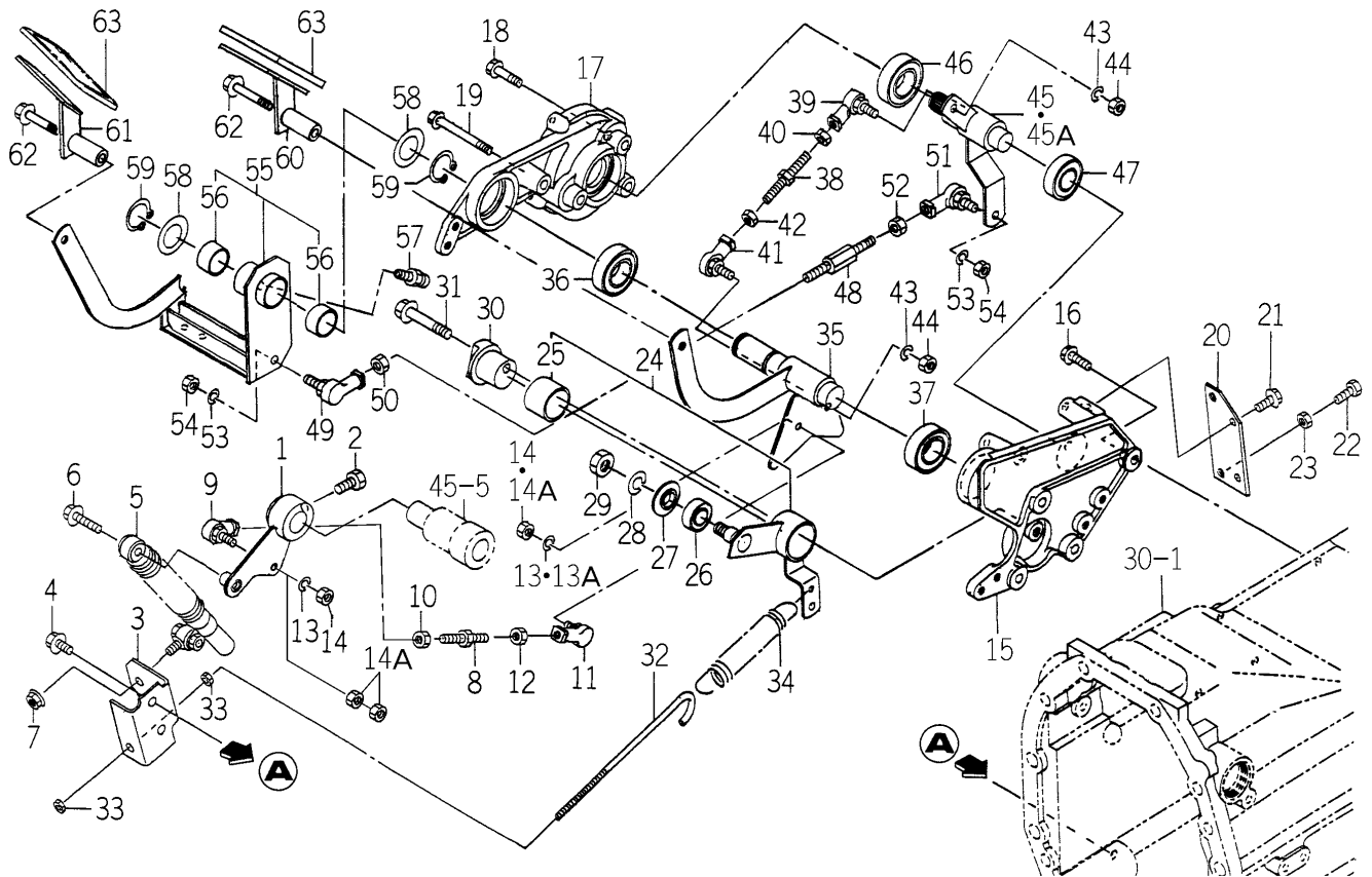
FIG.168 PEDAL (HST) SYSTEM (HE6 TYPE)
