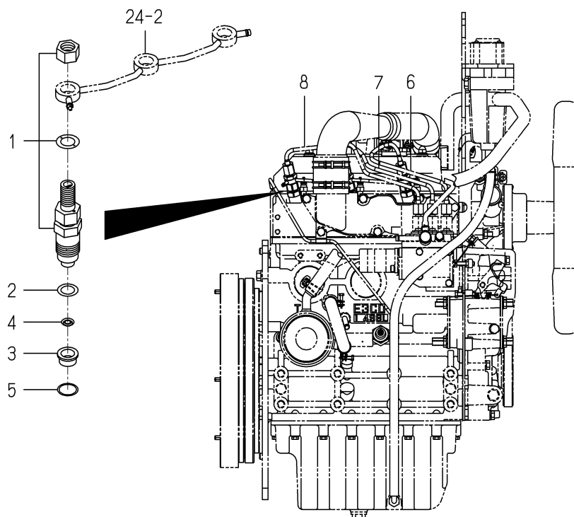
FIG. 22 INJECTION NOZZLE
