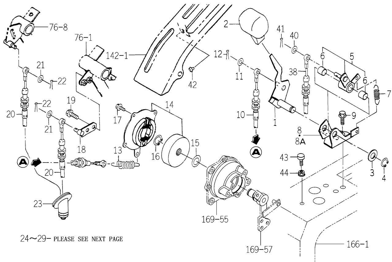
FIG.171 CRUISE CONTROL SYSTEM (H3 TYPE)(1/2)
