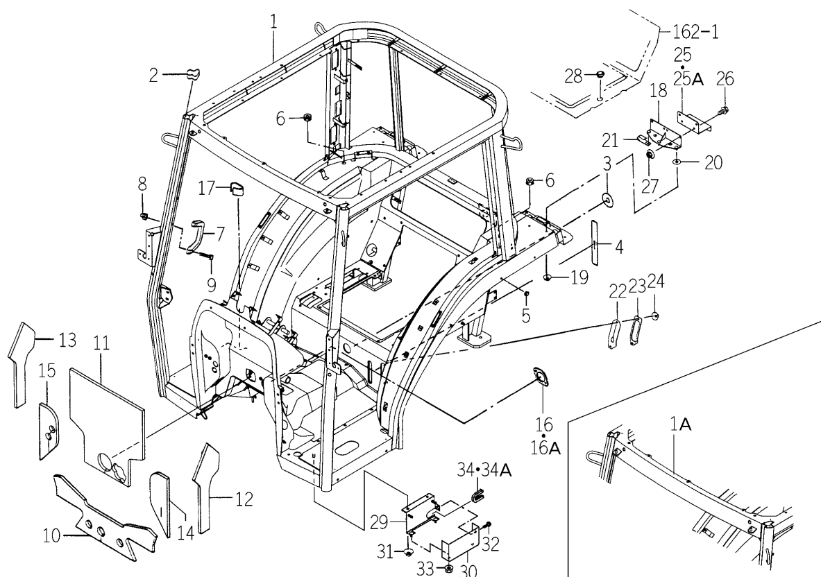
FIG.208 FRAME SYSTEM (H3C TYPE)
