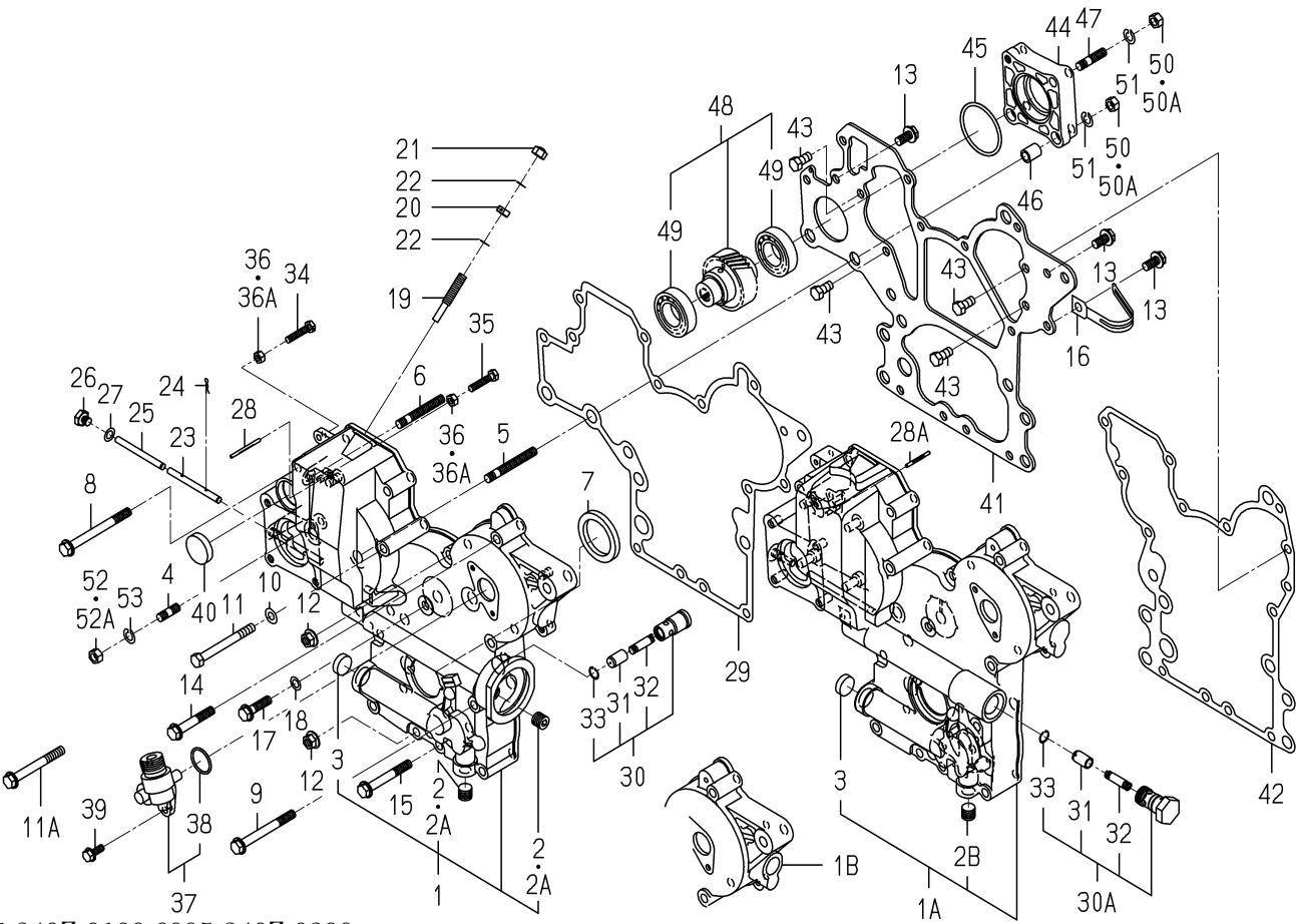
FIG. 10 TIMING GEAR CASE
