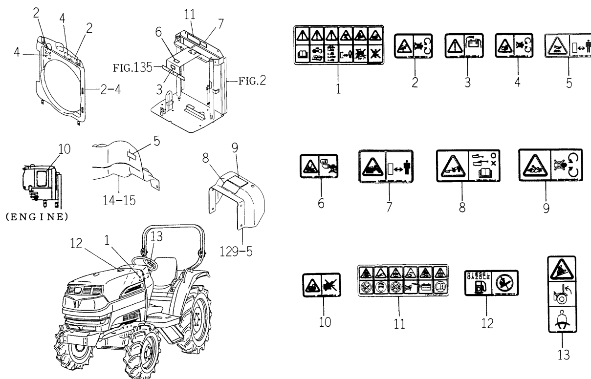
FIG.229 LABEL (CAUTION) (H TYPE EXCEPT C-No.1/ HC TYPE-TG5390E4-No.1-621)
