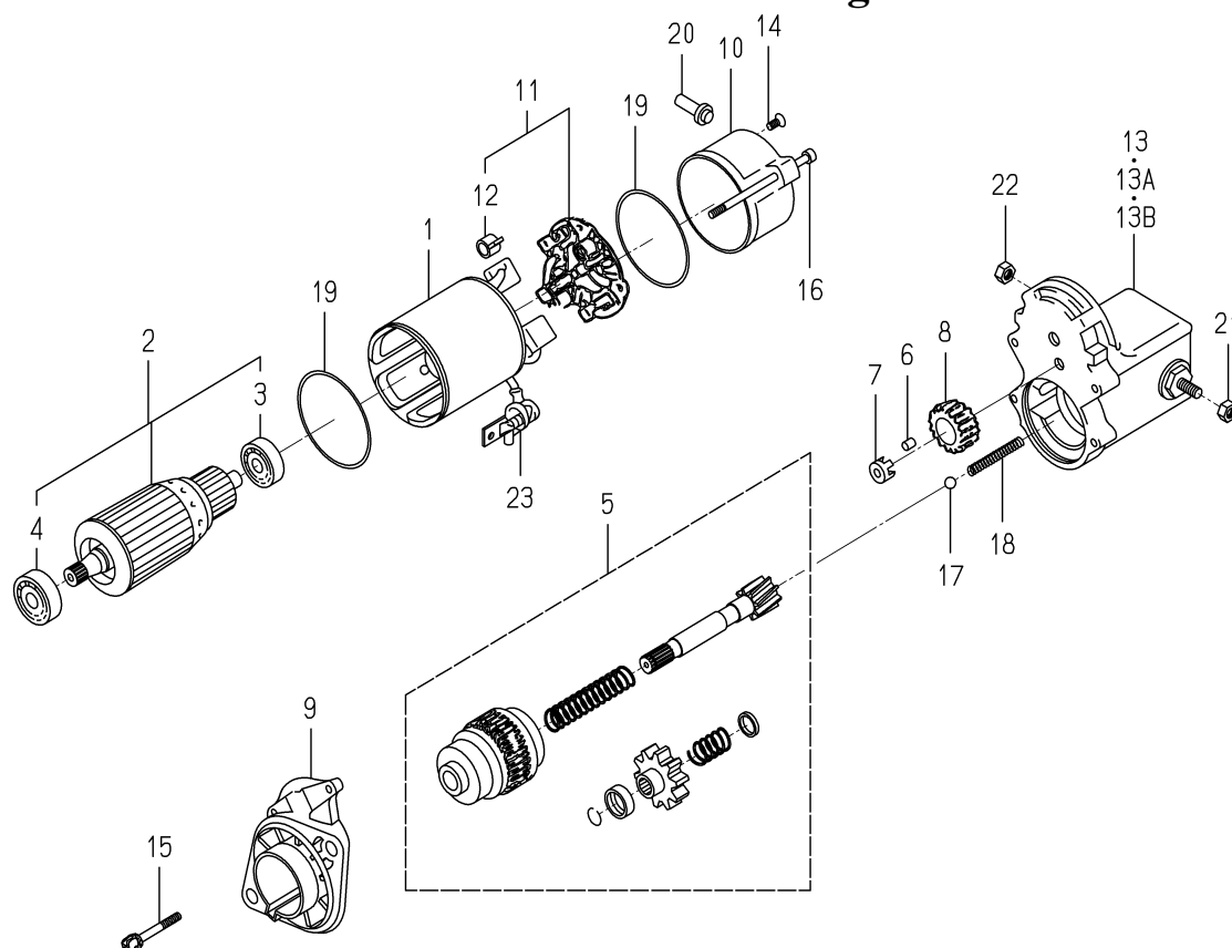
FIG. 30 COMPONENT PARTS FOR 6281-100-007-20 ON Fig.24
