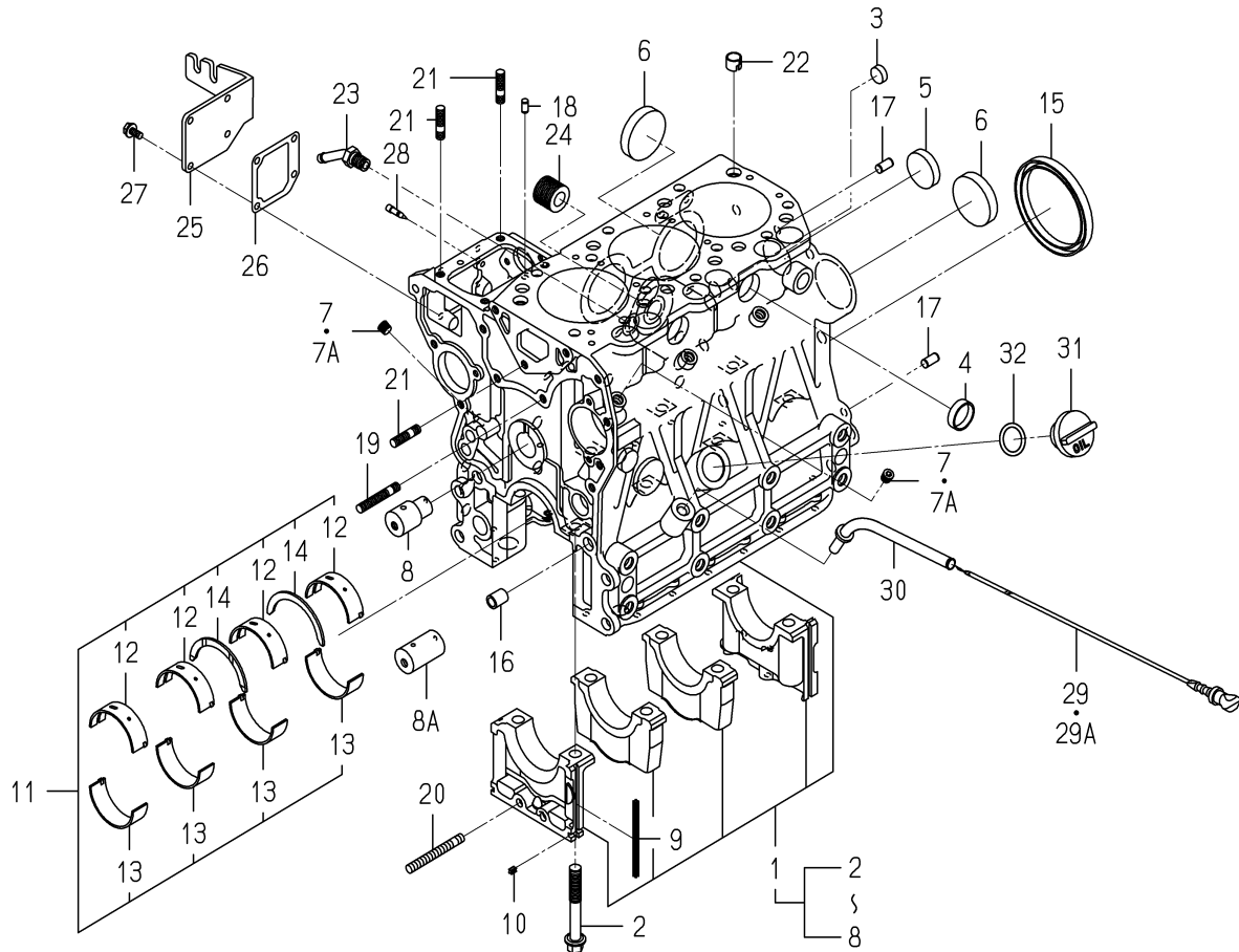
FIG. 6 CYLINDER BLOCK
