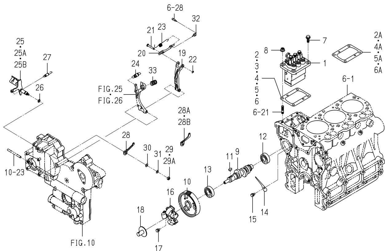
FIG. 23 INJECTION PUMP
