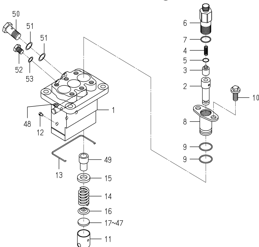
FIG. 31 COMPONENT PARTS FOR 6215-600-078-10 ON Fig.23
