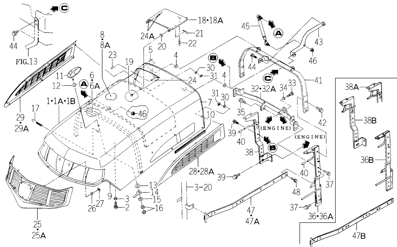
FIG.134 HOOD SYSTEM (C TYPE)
