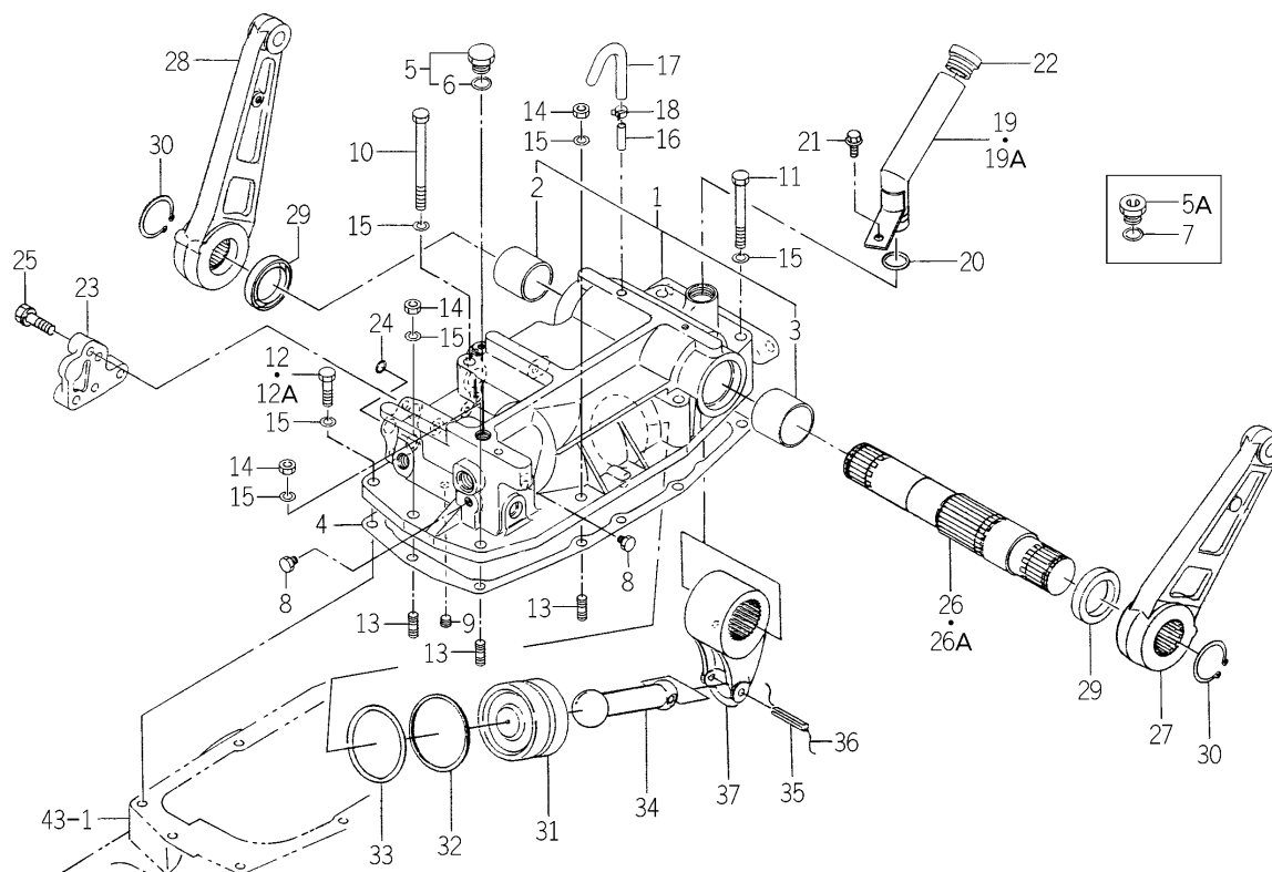
FIG. 98 CYLINDER CASE SYSTEM (EXCEPT W,A TYPE-No.1-/ A TYPE-TG5330E4-No.1-159/TG5390E4-No.1-519)
