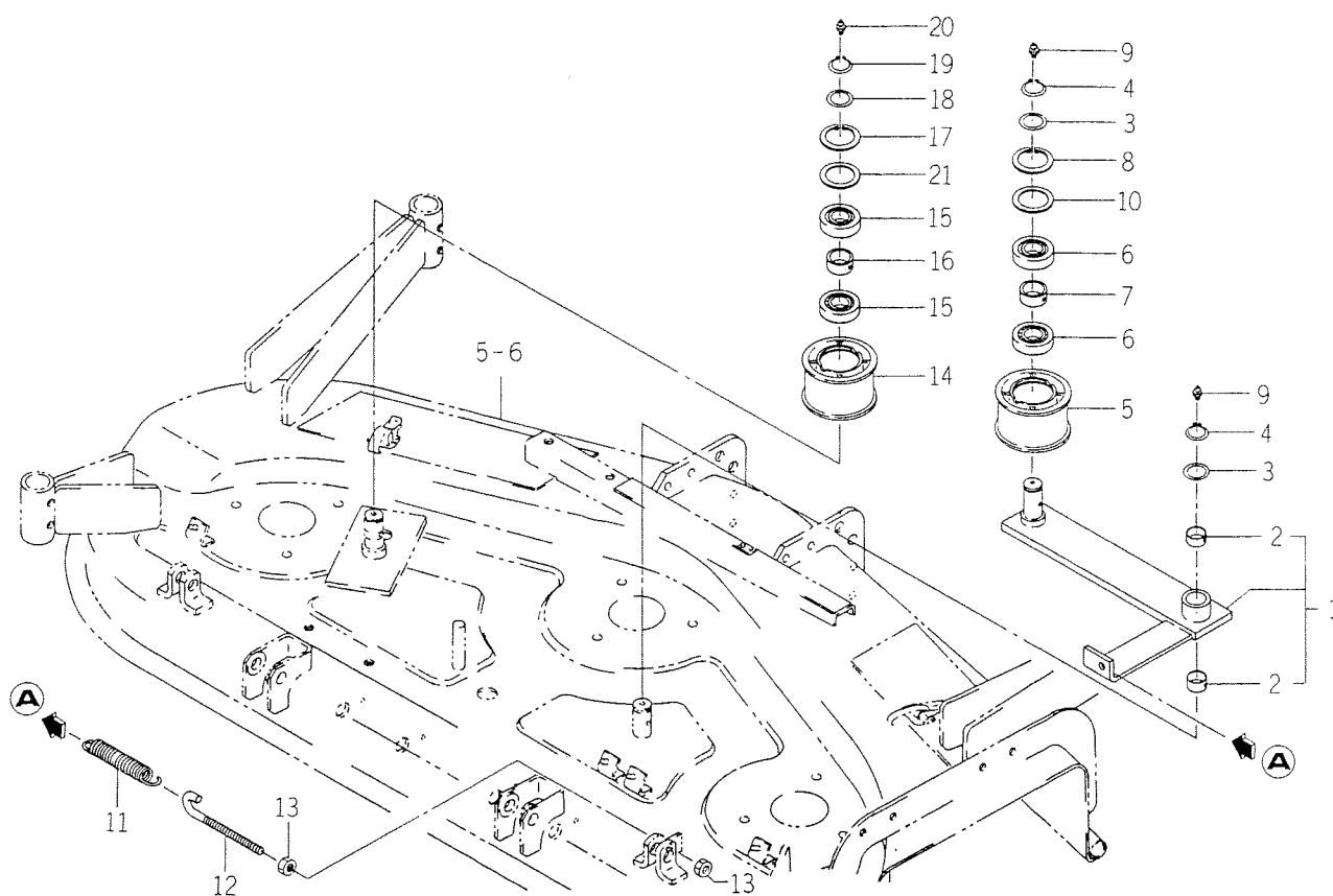
FIG. 3 TENSION (BELT) SYSTEM
