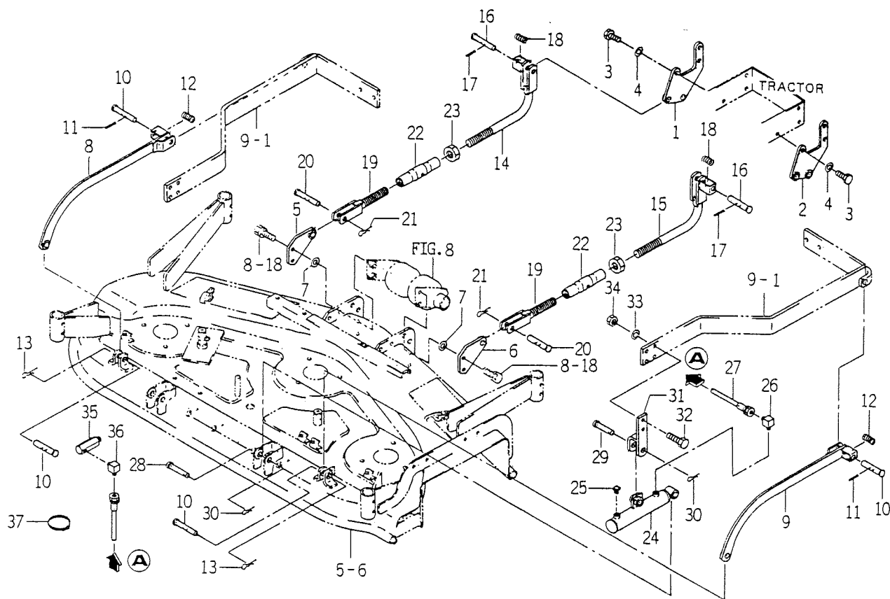
FIG. 11 LINK (LIFT/MID) SYSTEM
