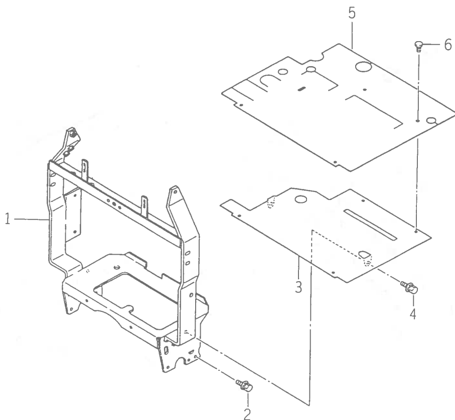
FIG. 8 BATTERY BASE SYSTEM
