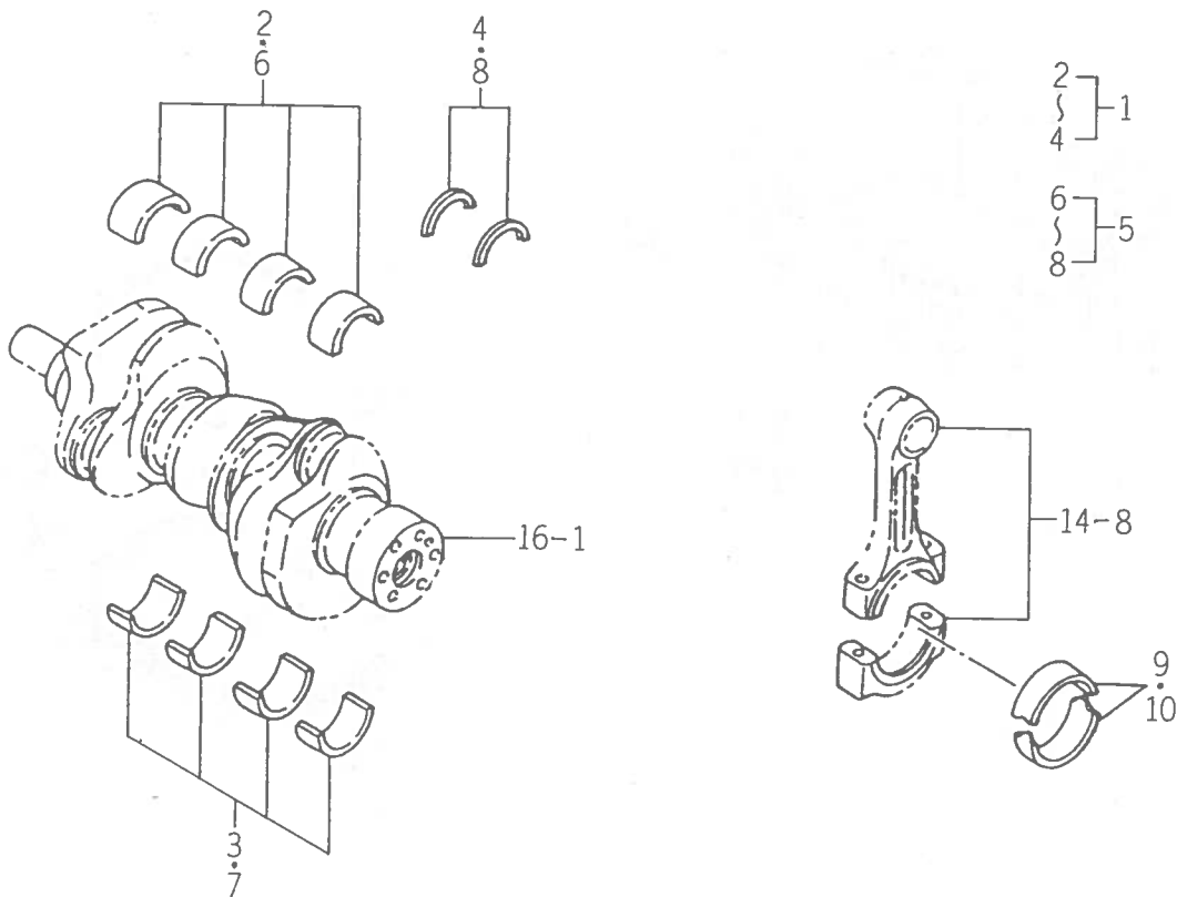
FIG. 7 BEARING/UNDER SIZE
