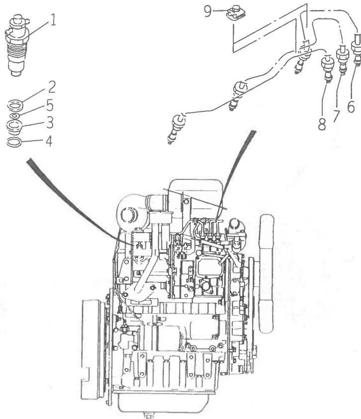
FIG. 21 INJECTION NOZZLE
