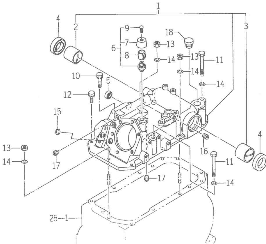
FIG. 70 CYLINDER (CASE) SYSTEM
