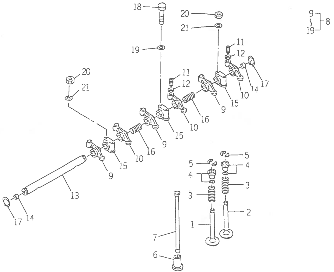
FIG. 12 VALVE
