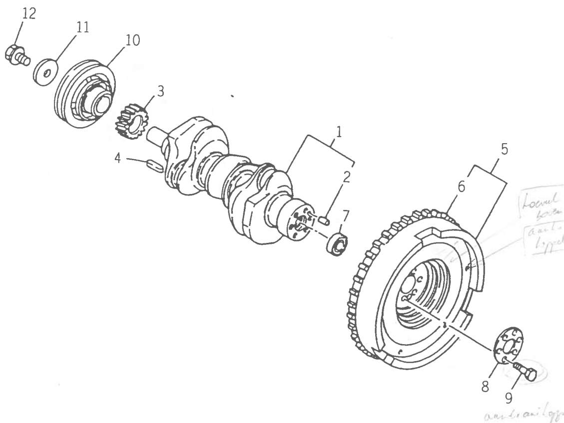
FIG. 16 CRANK SHAFT
