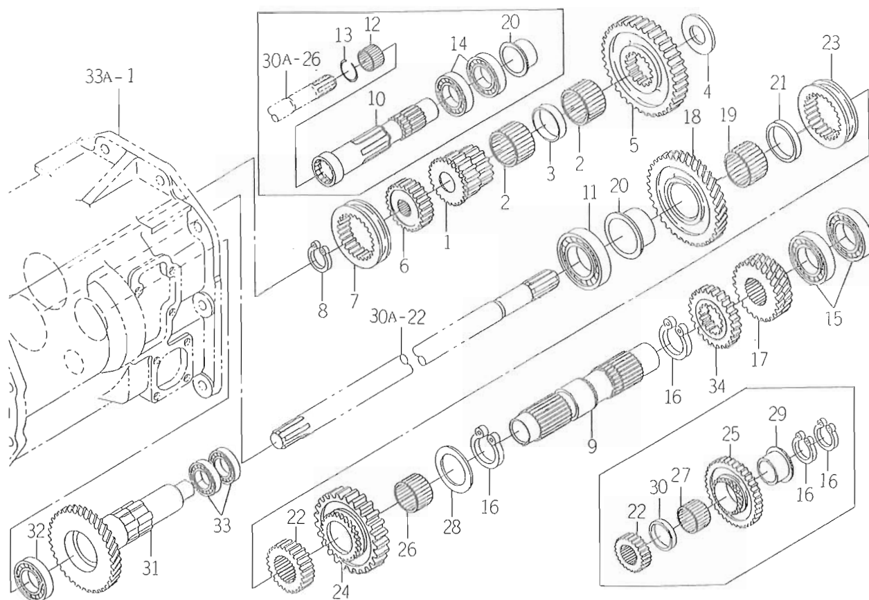
FIG. 35A SUB CHANGE GEAR SYSTEM
