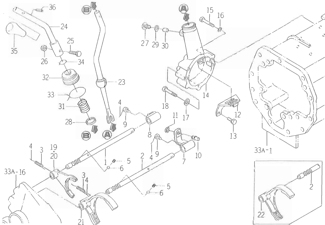
FIG. 31A MAIN CHANGE SYSTEM
