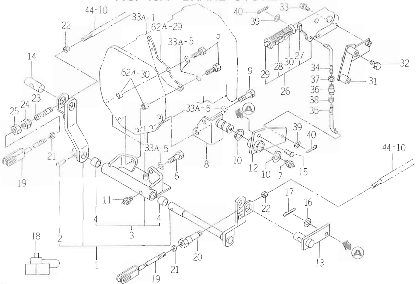
FIG. 45A BRAKE SYSTEM
