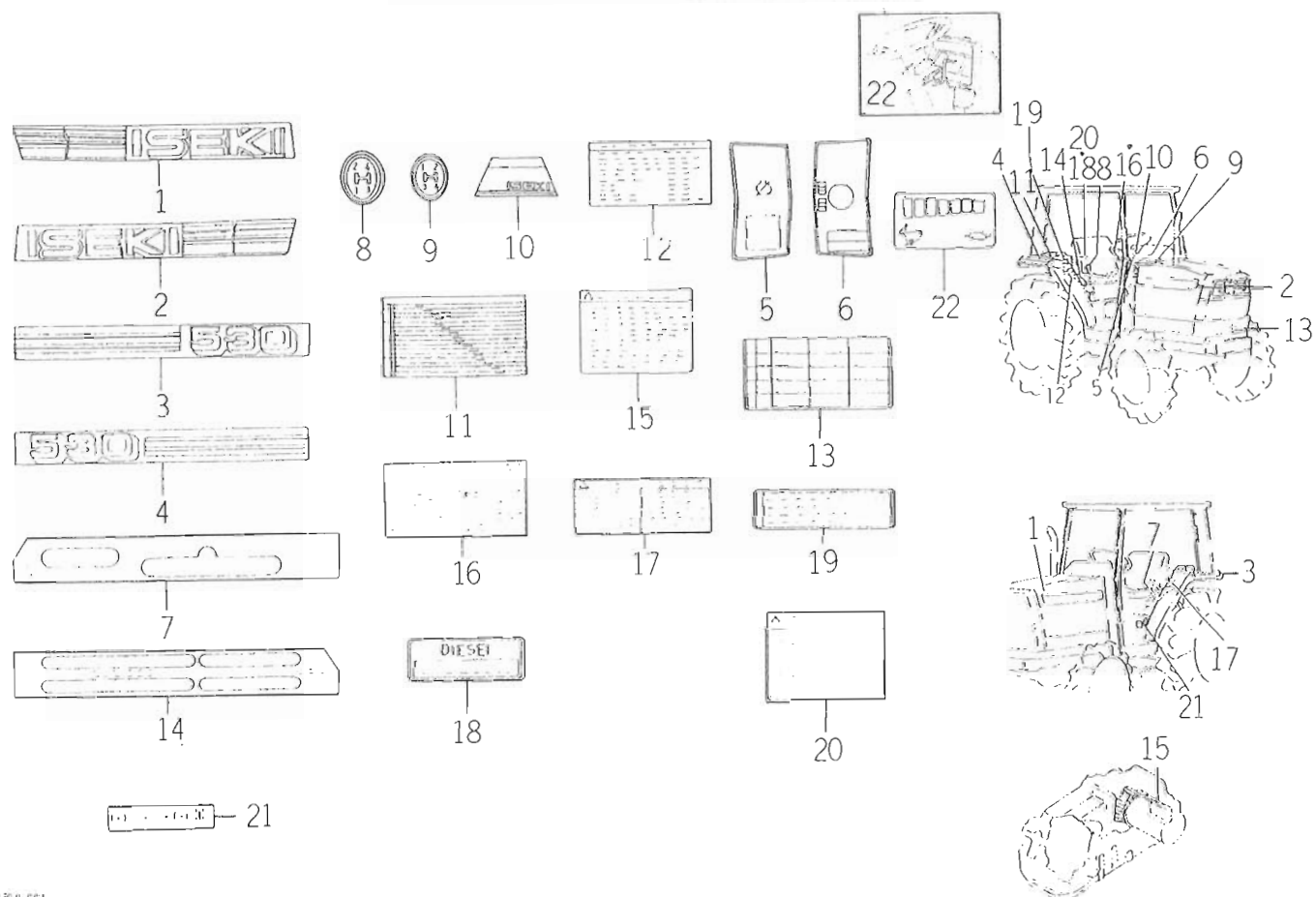
FIG. 98A MARK SYSTEM
