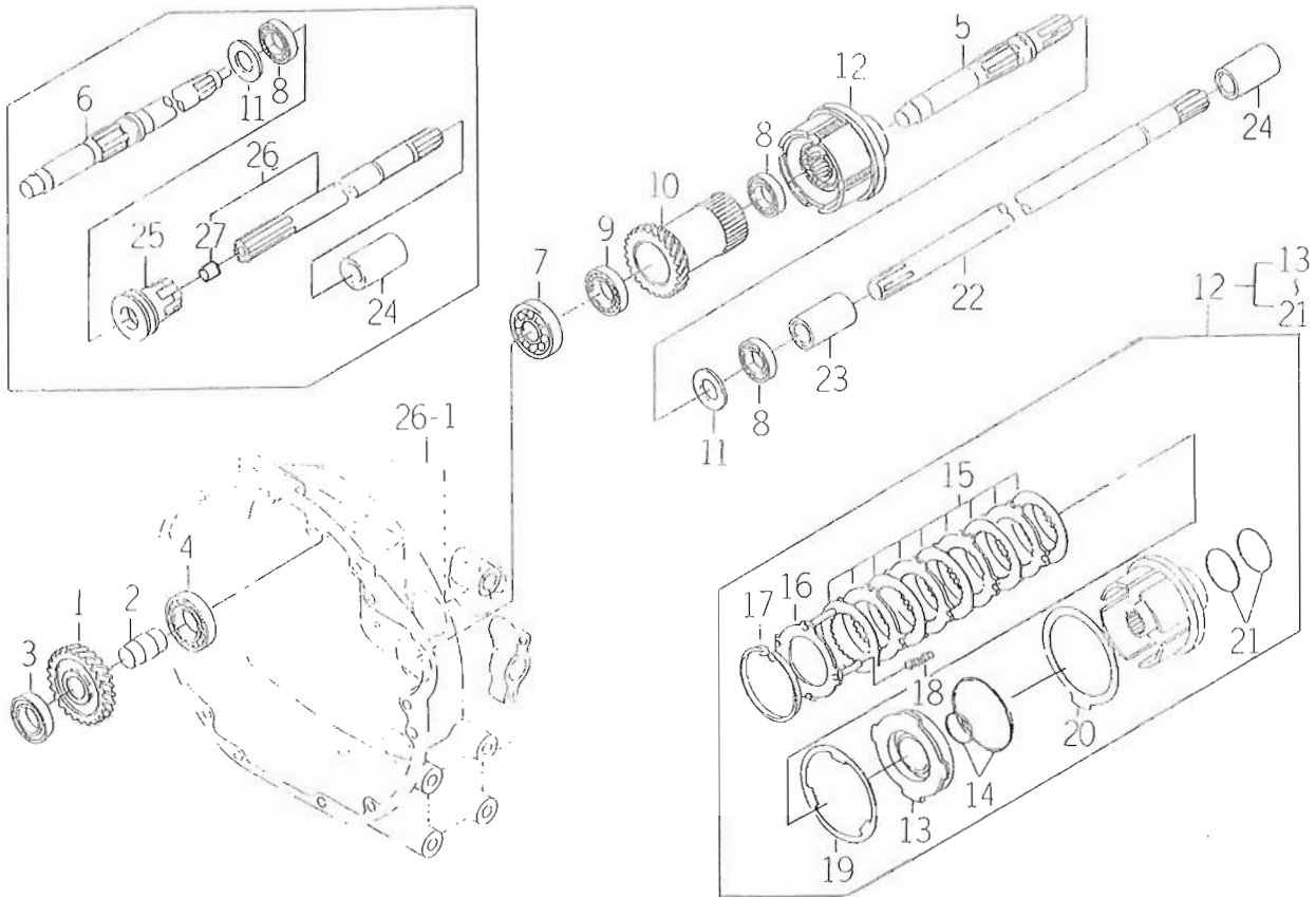
FIG. 30A P.T.O DRIVE SHAFT SYSTEM
