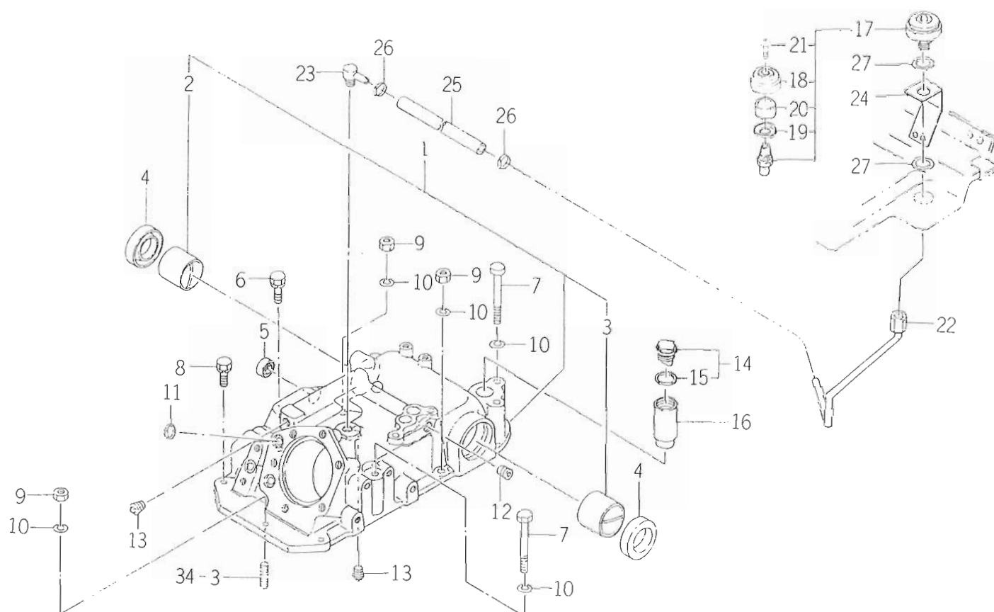
FIG. 57A CYLINDER CASE SYSTEM
