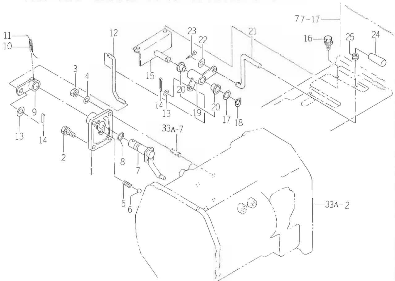
FIG. 41A GRAND P.T.O CHANGE SYSTEM
