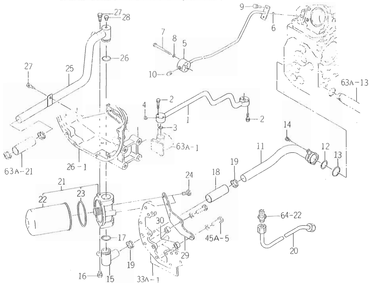
FIG. 62A PIPING (REAR) SYSTEM
