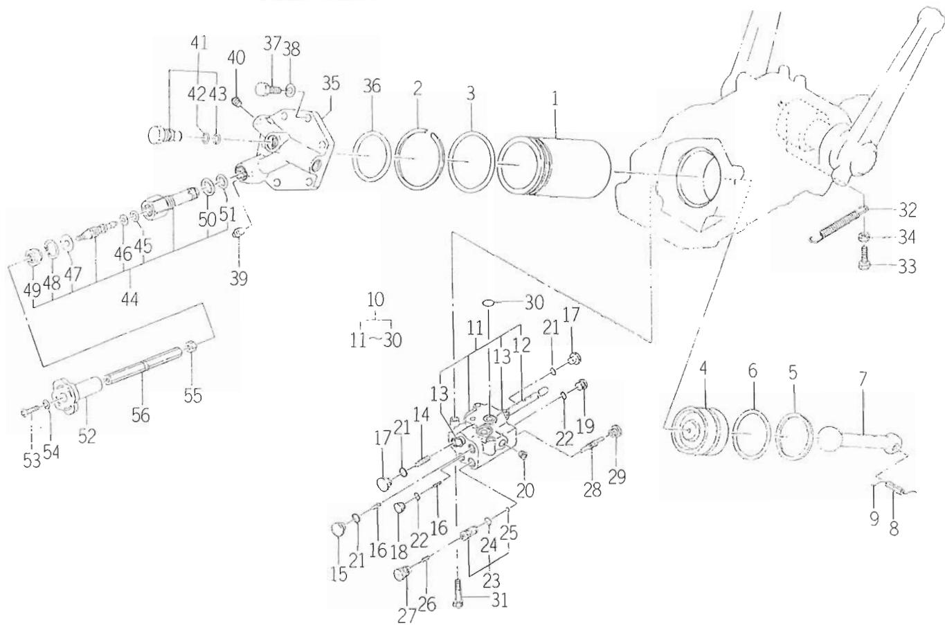
FIG. 59A CYLINDER SYSTEM
