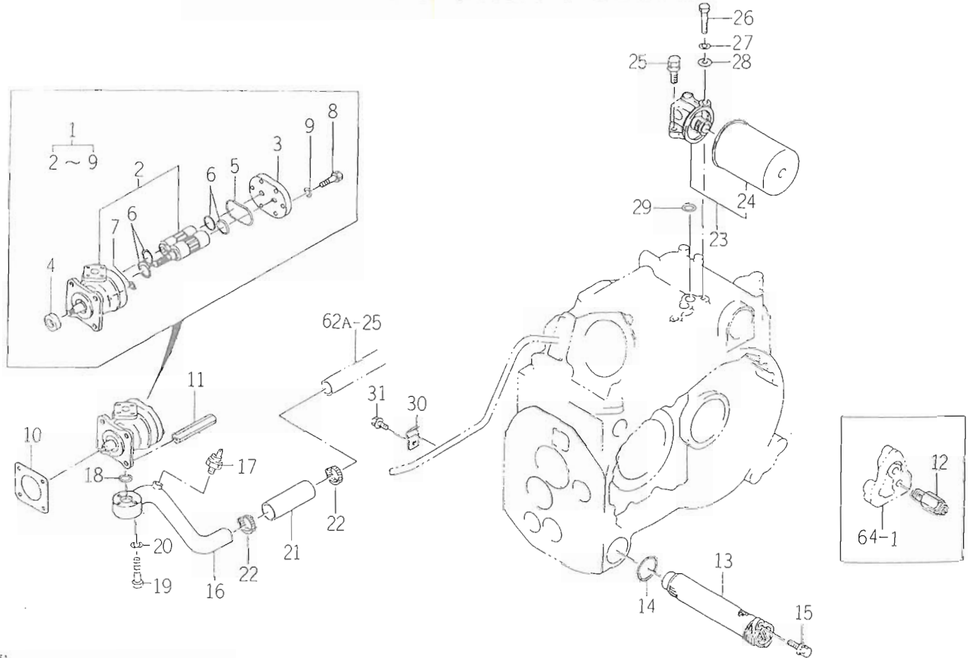
FIG. 63A PIPING (FRONT) SYSTEM
