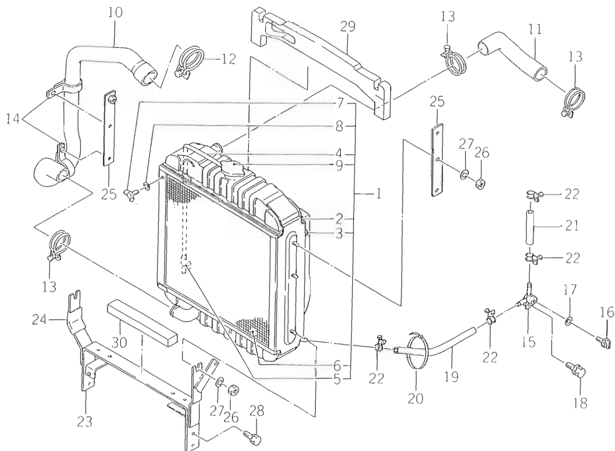
FIG. 20A RADIATOR SYSTEM
