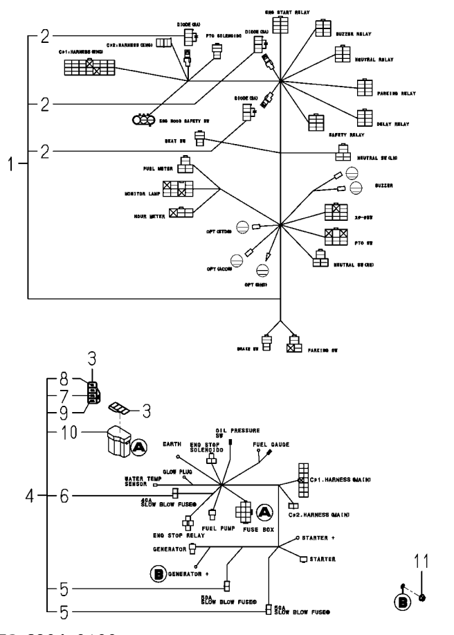
FIG. 33 HARNESS SYSTEM(1/2)
