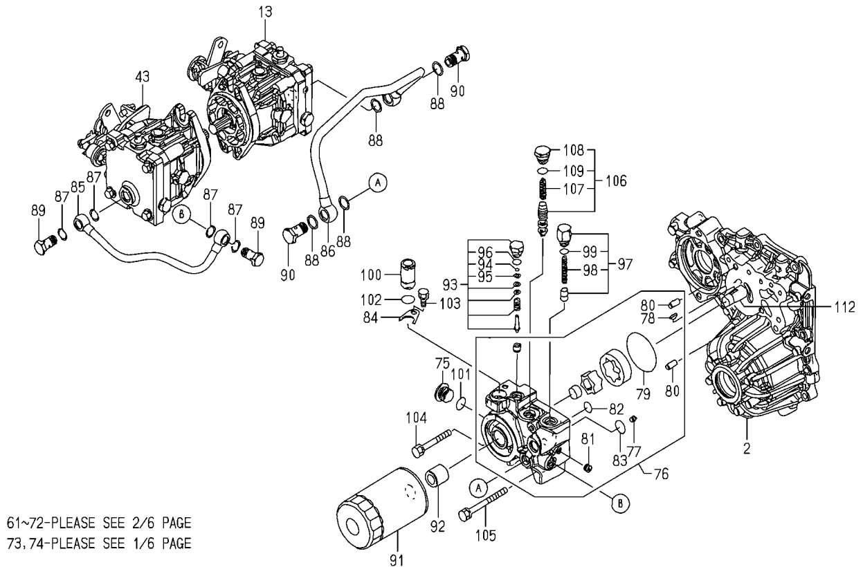
FIG. 10 PUMP(HST)SYSTEM(3/6)
