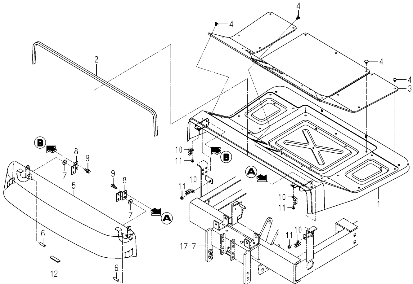
FIG. 31 FLOOR SYSTEM
