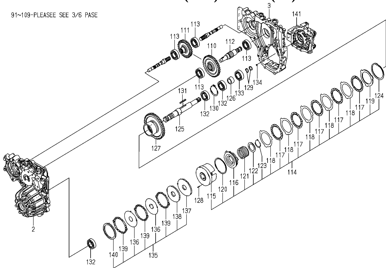
FIG. 10 PUMP(HST)SYSTEM(4/6)
