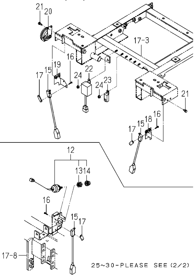
FIG. 33 HARNESS SYSTEM(1/2)
