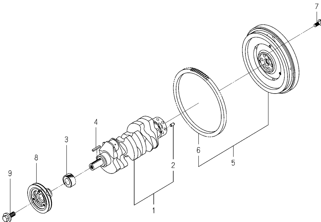
FIG. 16 CRANK SHAFT
