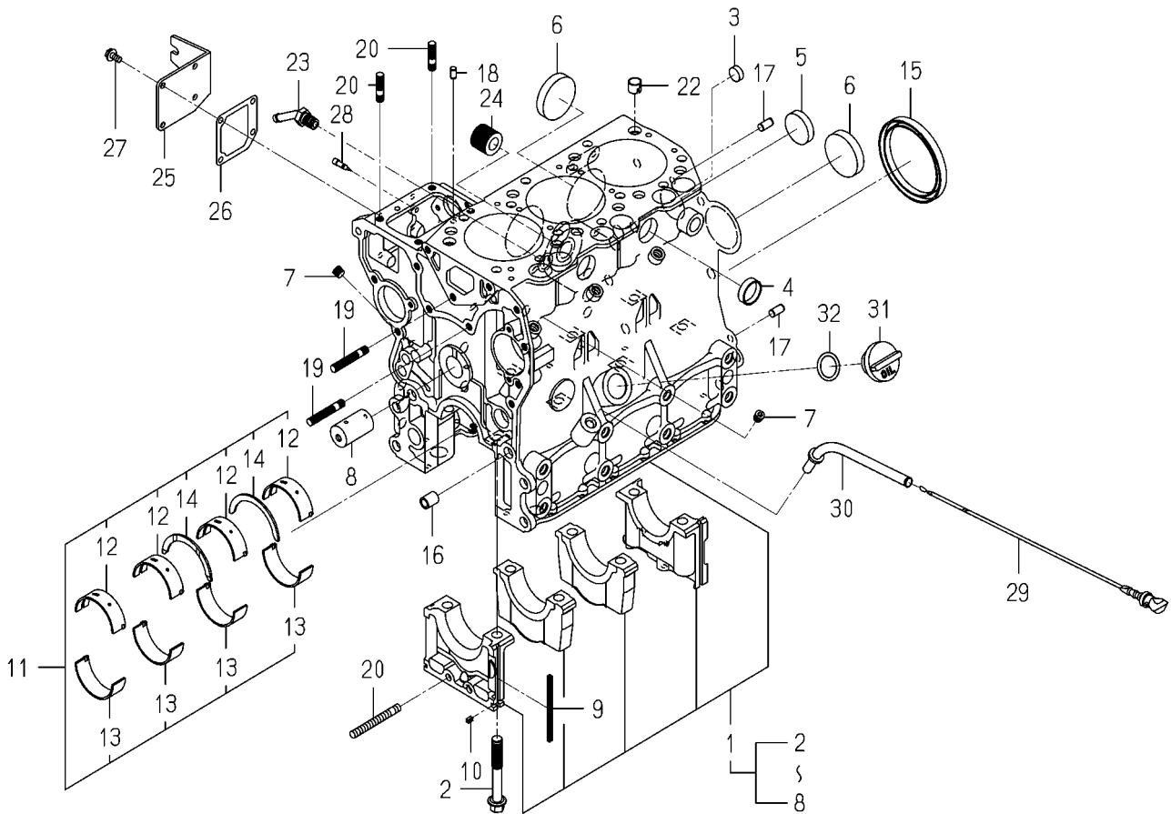
FIG. 6 CYLINDER BLOCK
