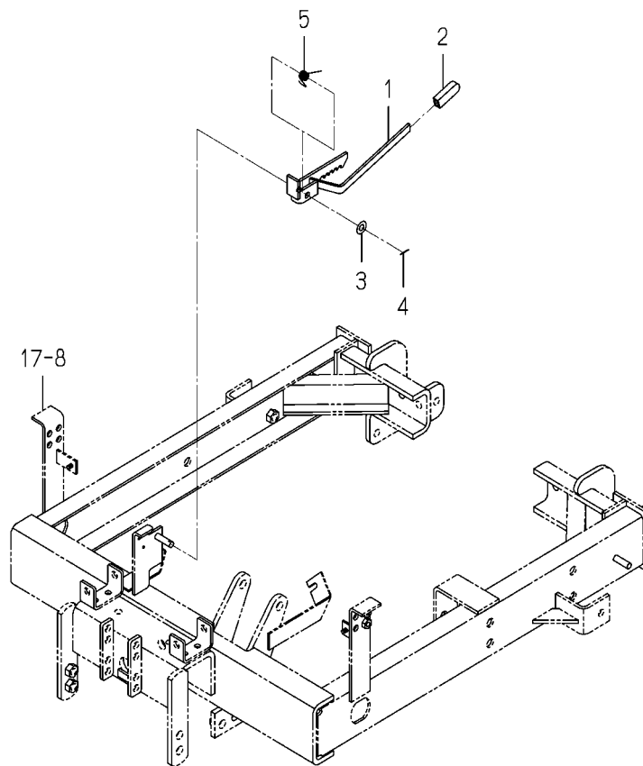
FIG. 16 BRAKE(PARKING)SYSTEM
