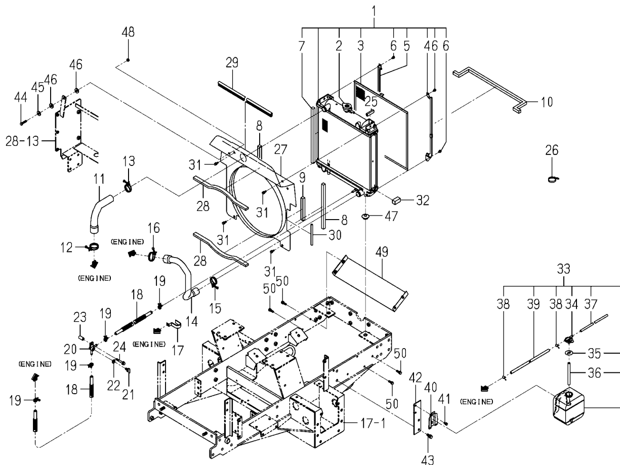
FIG. 2 RADIATOR SYSTEM
