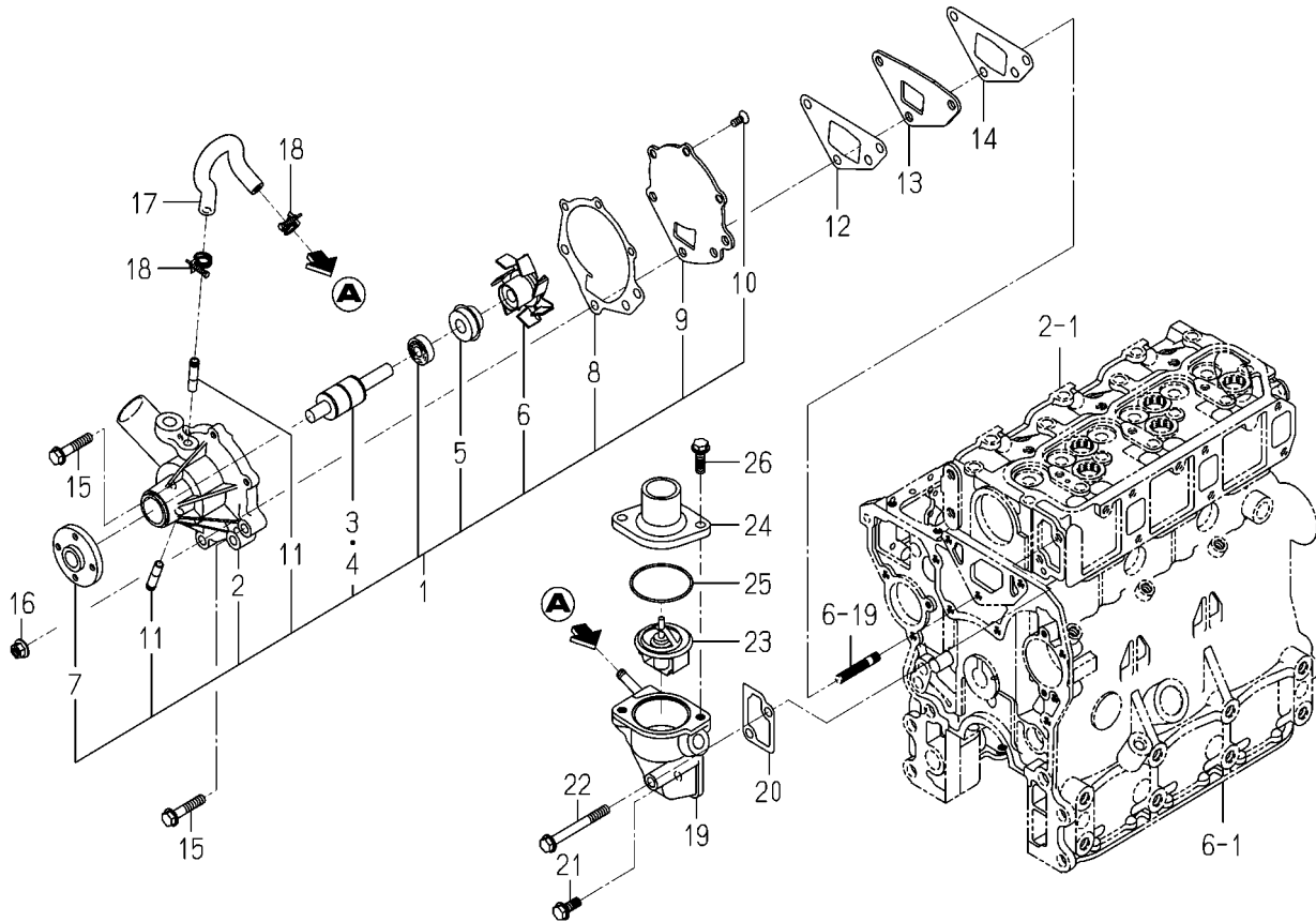
FIG. 18 WATER PUMP
