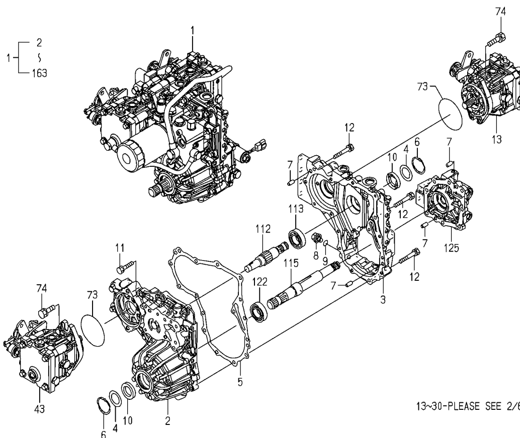
FIG. 10 PUMP(HST)SYSTEM(1/6)
