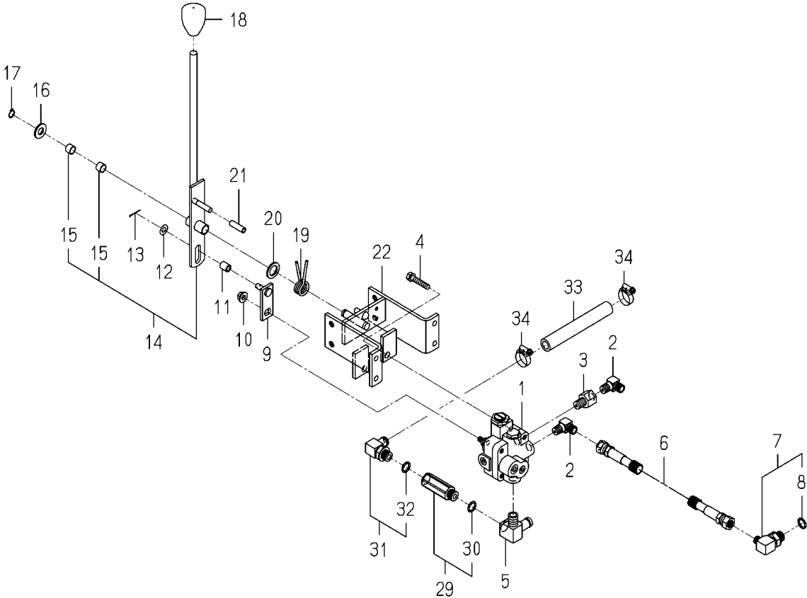
FIG. 20 LEVER(LIFT)SYSTEM(1/2)
