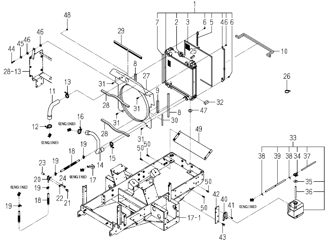
FIG. 2 RADIATOR SYSTEM
