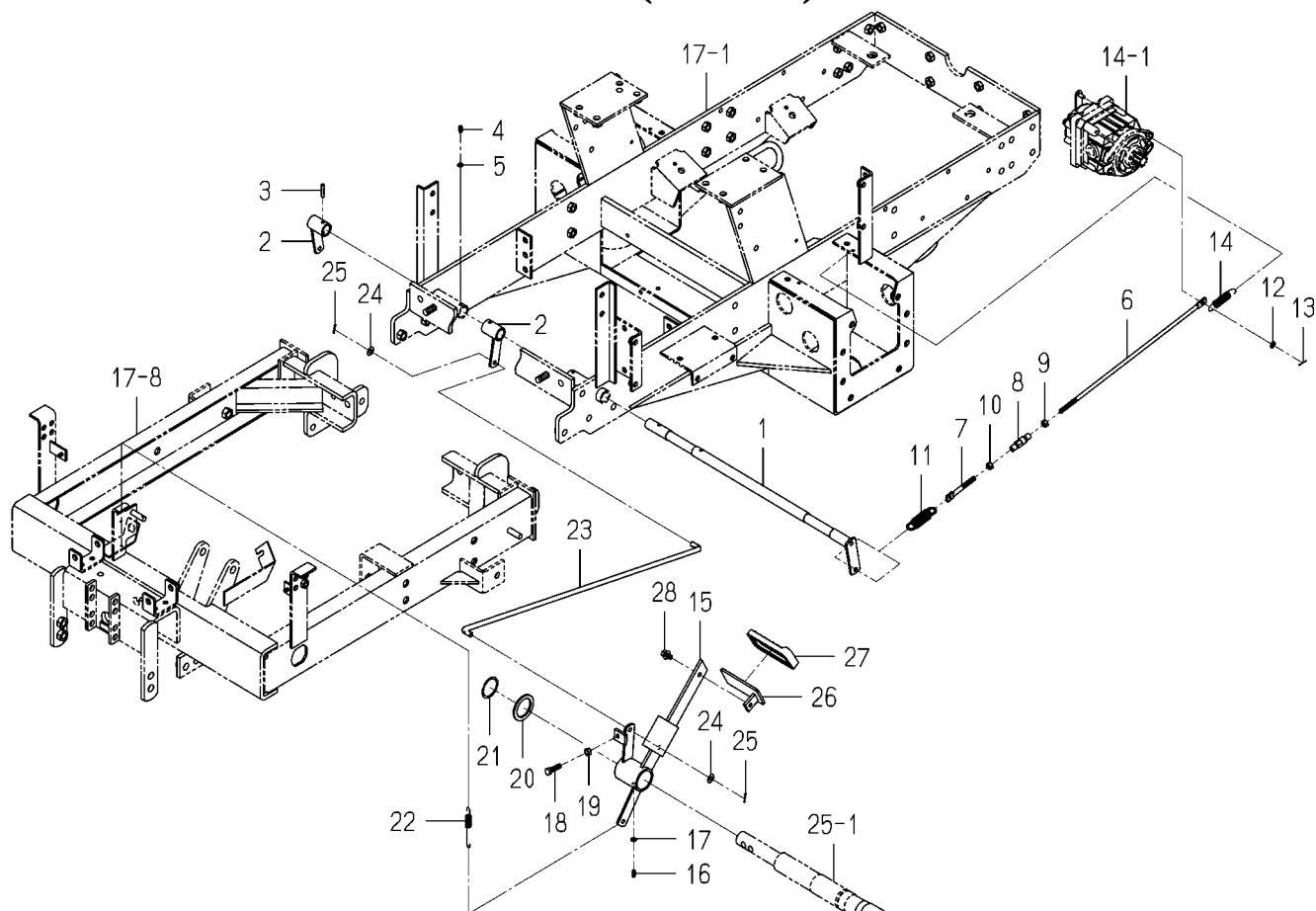
FIG. 15 PEDAL(BRAKE)SYSTEM
