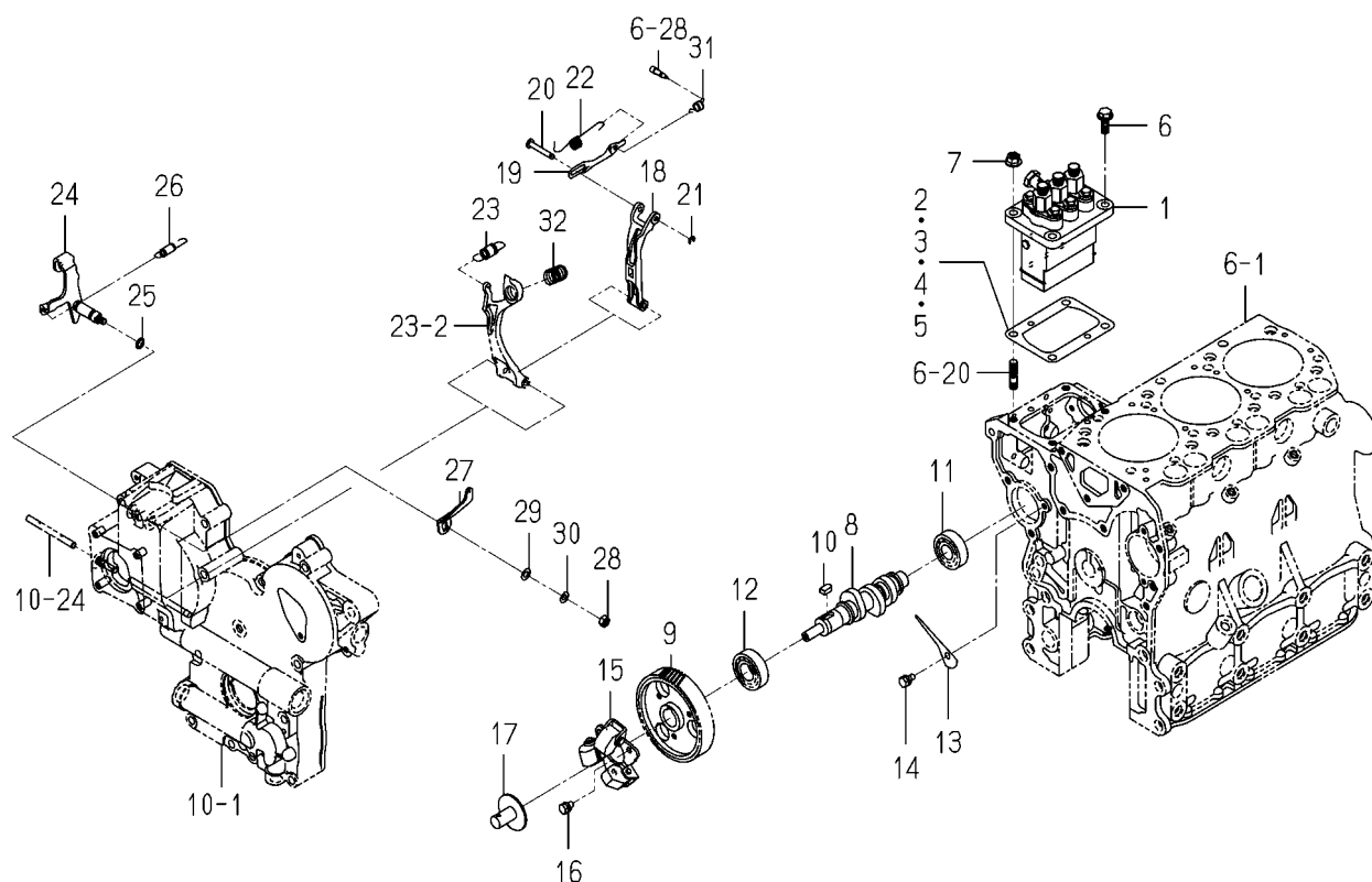
FIG. 21 INJECTION PUMP
