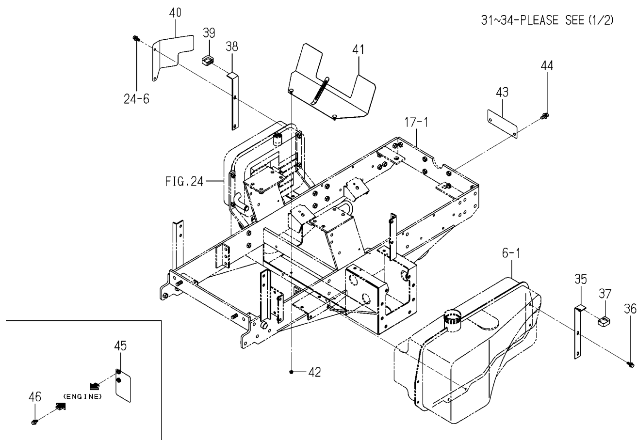
FIG. 28 HOOD SYSTEM(2/2)
