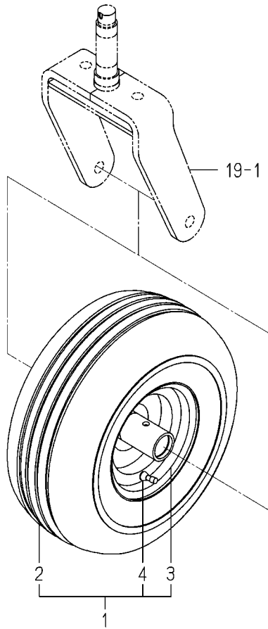
FIG. 42 TIRE(15X6)ASSY(OPTION)
