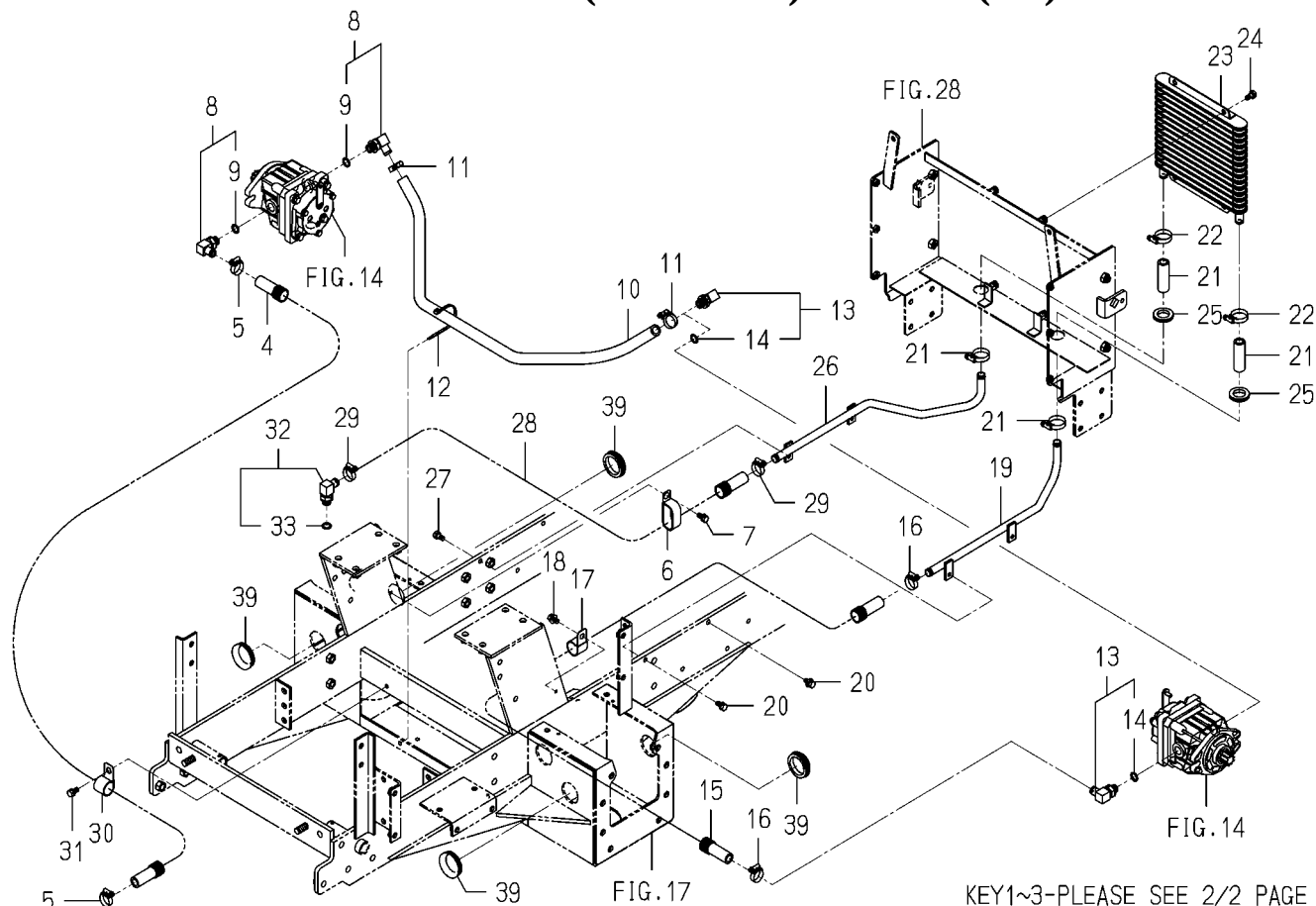
FIG. 22 PIPING(SUCTION)SYSTEM(1/2)
