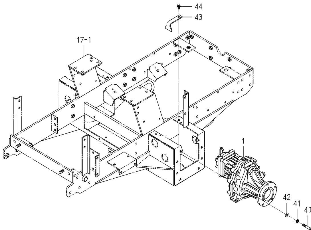
FIG. 14 MOTOR(HST)SYSTEM(1/2)
