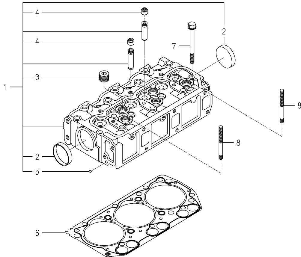
FIG. 2 CYLINDER HEAD
