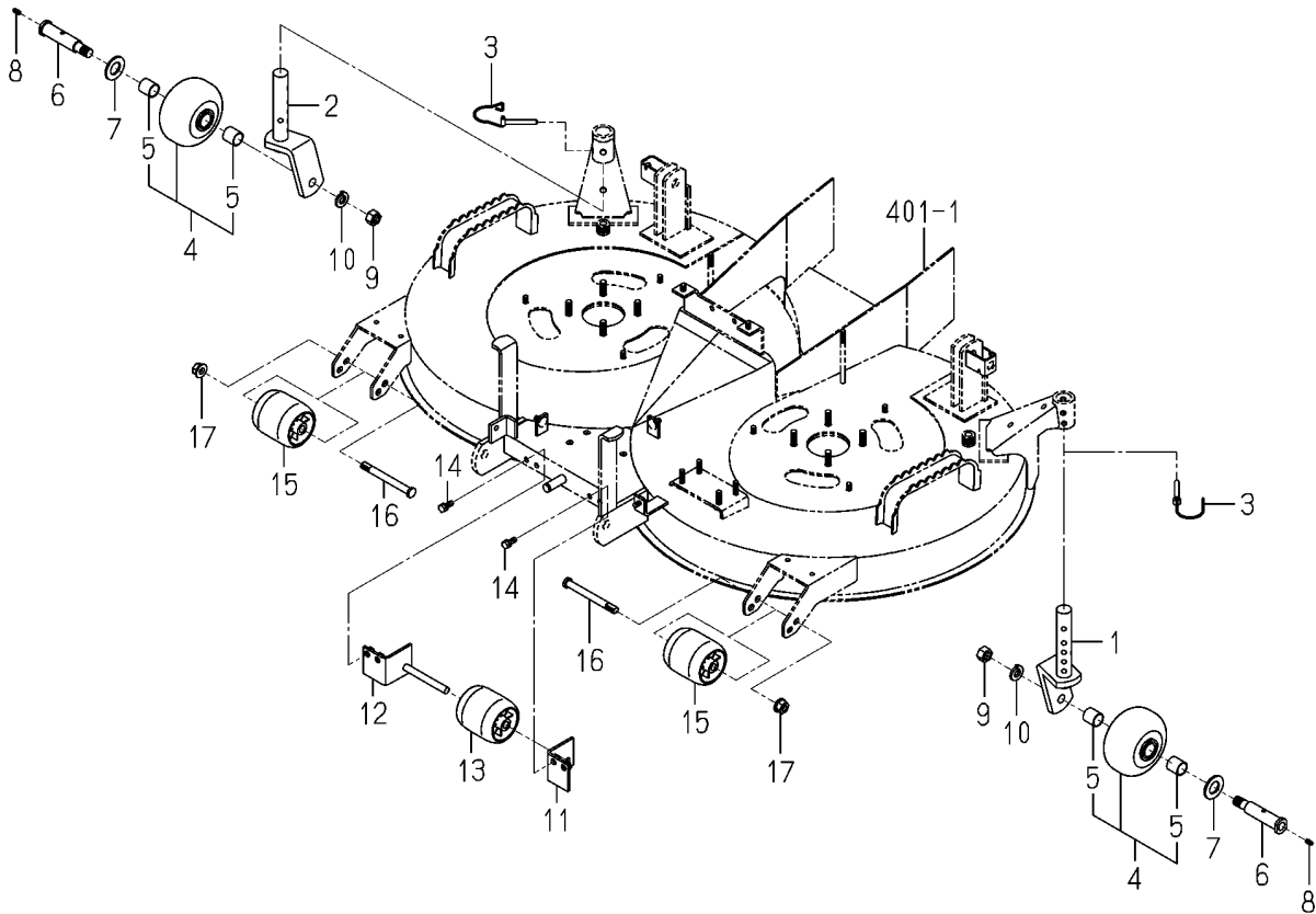
FIG.501 WHEEL(GAUGE)SYSTEM
