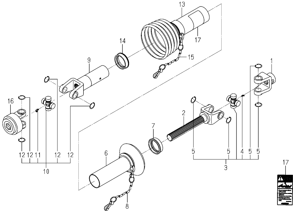
FIG.S01 COMPONENT PARTS FOR 8663-101-510-00 ON Fig.101
