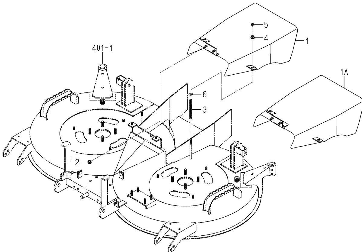
FIG.402 COVER(DISCHARGE)SYSTEM
