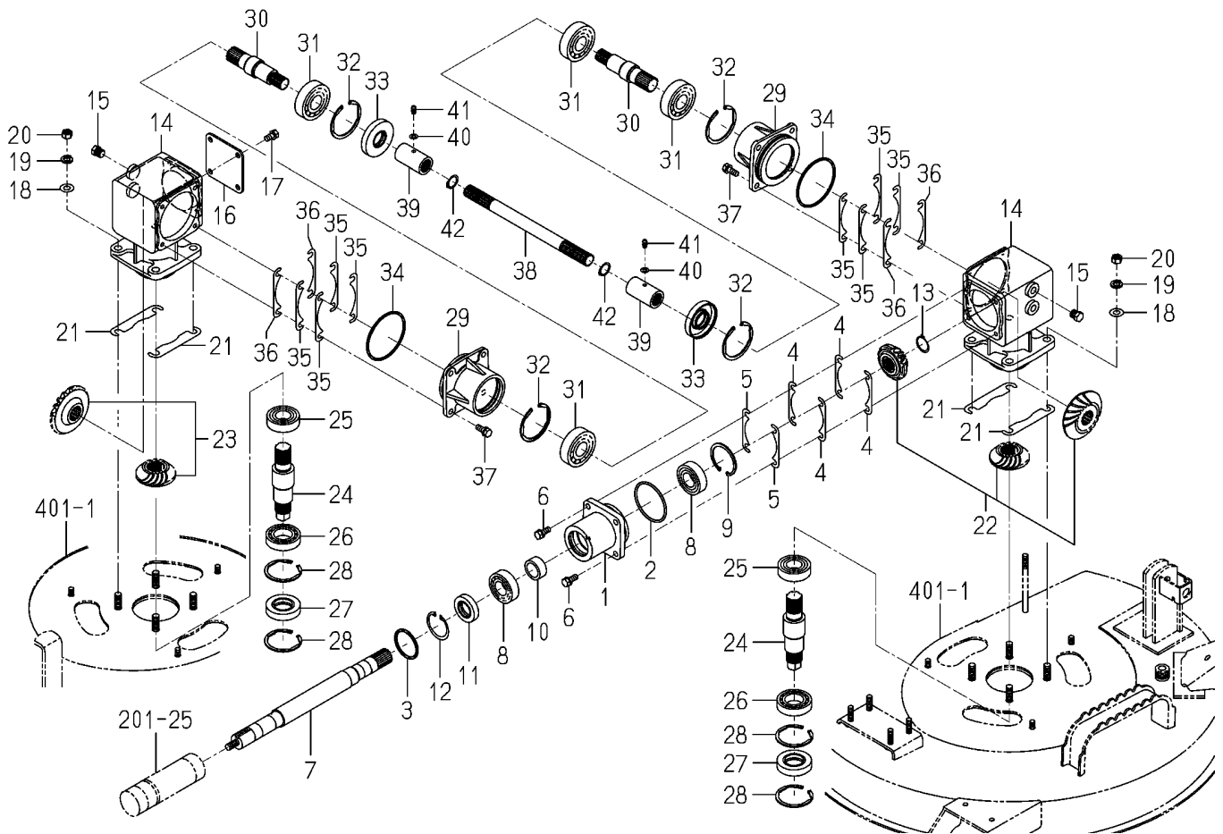
FIG.202 CASE(BEVEL)SYSTEM
