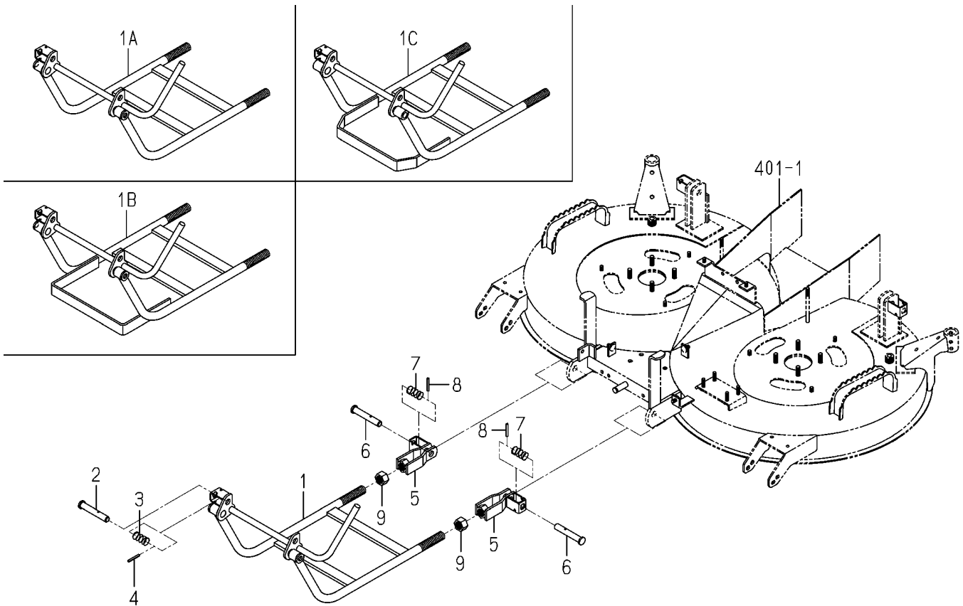
FIG.601 LINK SYSTEM
