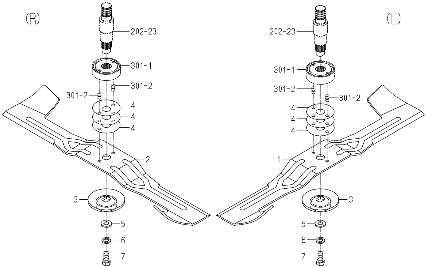
FIG.302 BLADE SYSTEM
