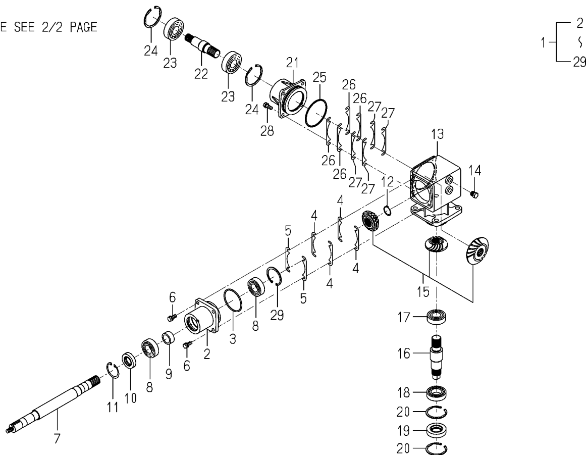
FIG.P01 CASE(BEVEL)ASSY(REPAIR) (1/2)
