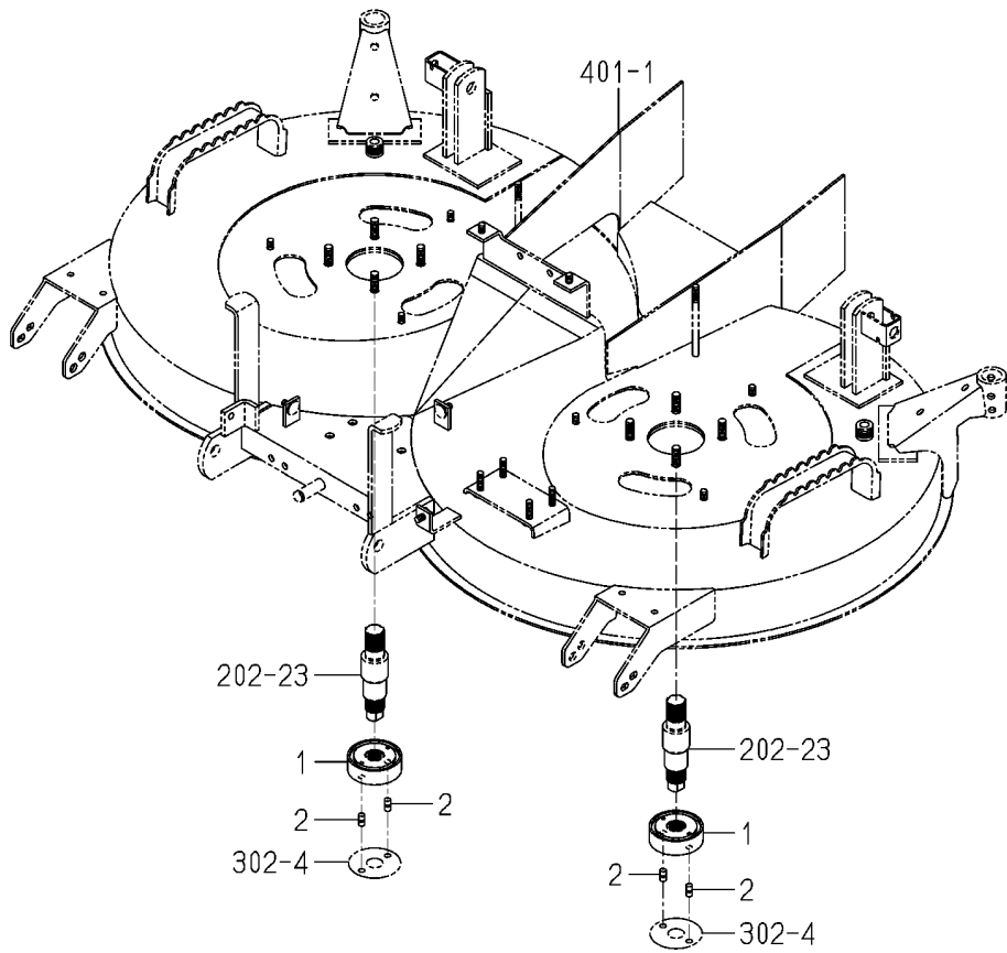
FIG.301 COLLAR(BLADE)SYSTEM
