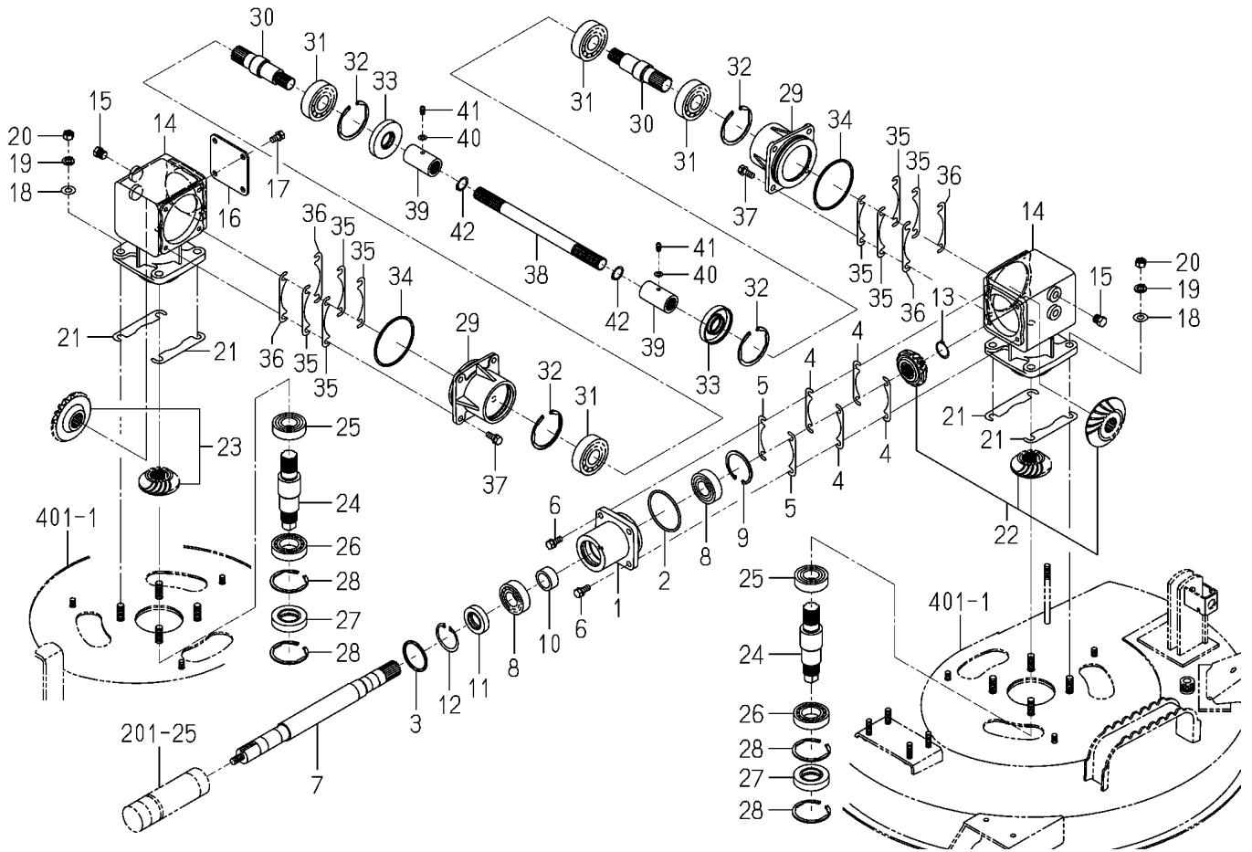
FIG.202 CASE(BEVEL)SYSTEM
