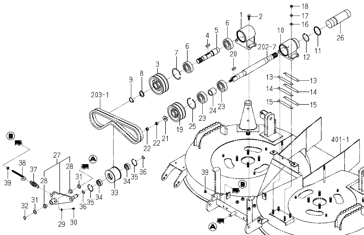
FIG.201 PULLEY SYSTEM
