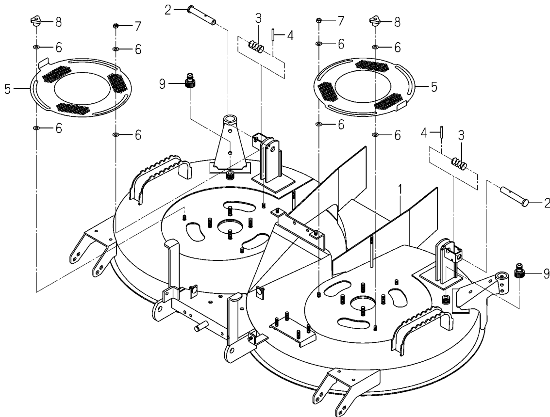
FIG.401 DECK(MOWER)SYSTEM
