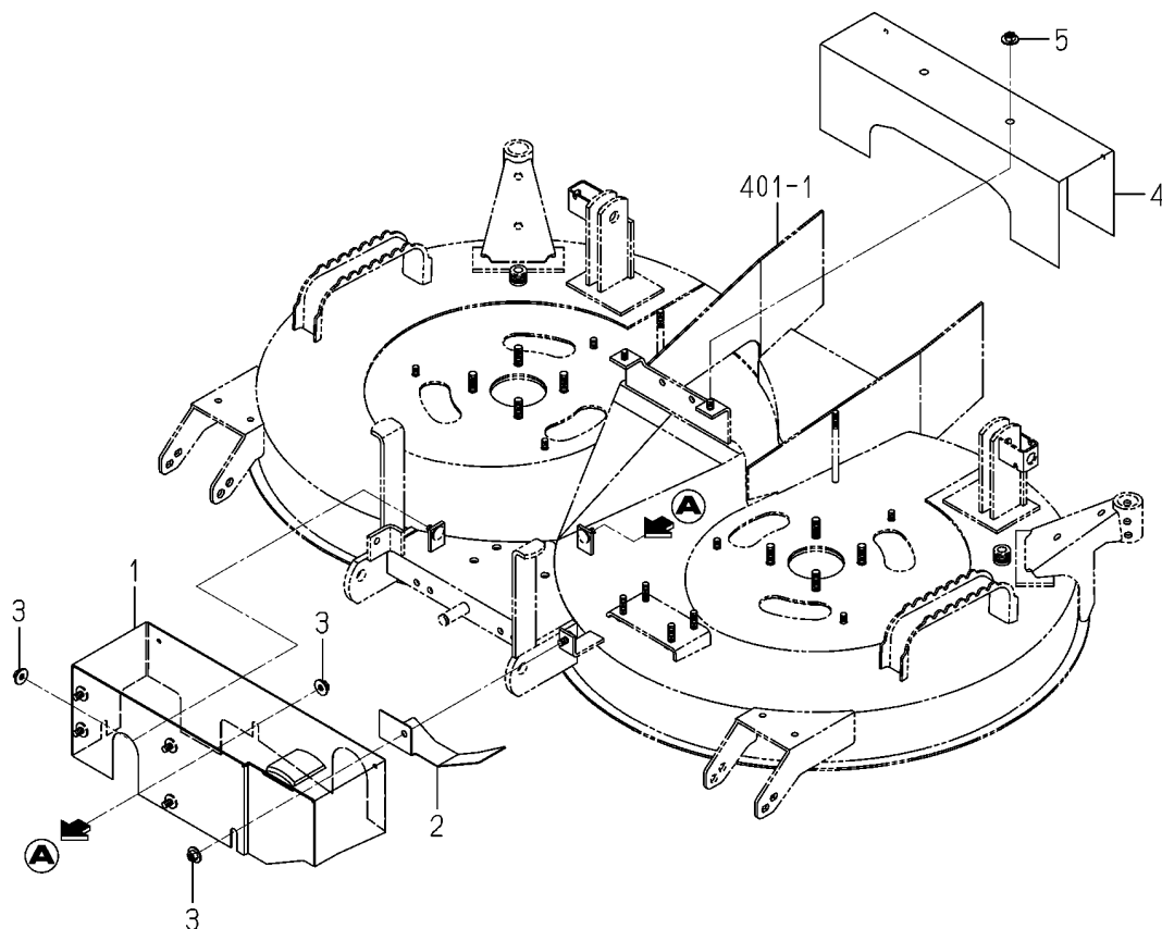
FIG.403 COVER SYSTEM
