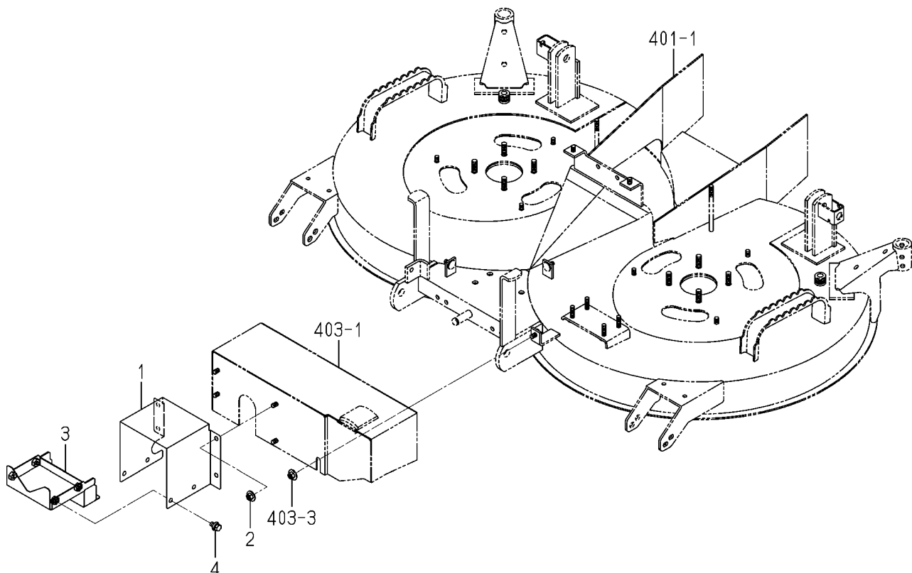
FIG.102 COVER(JOINT)SYSTEM
