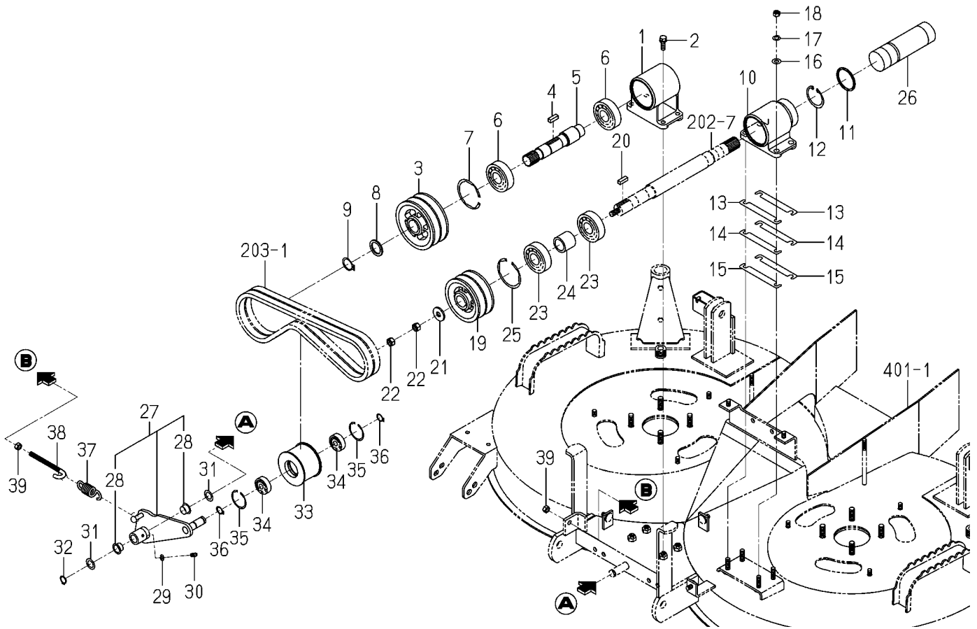
FIG.201 PULLEY SYSTEM
