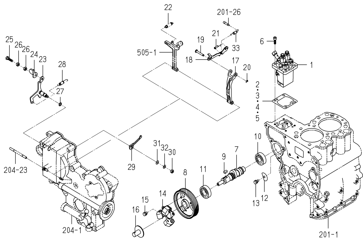
FIG.502 INJECTION PUMP
