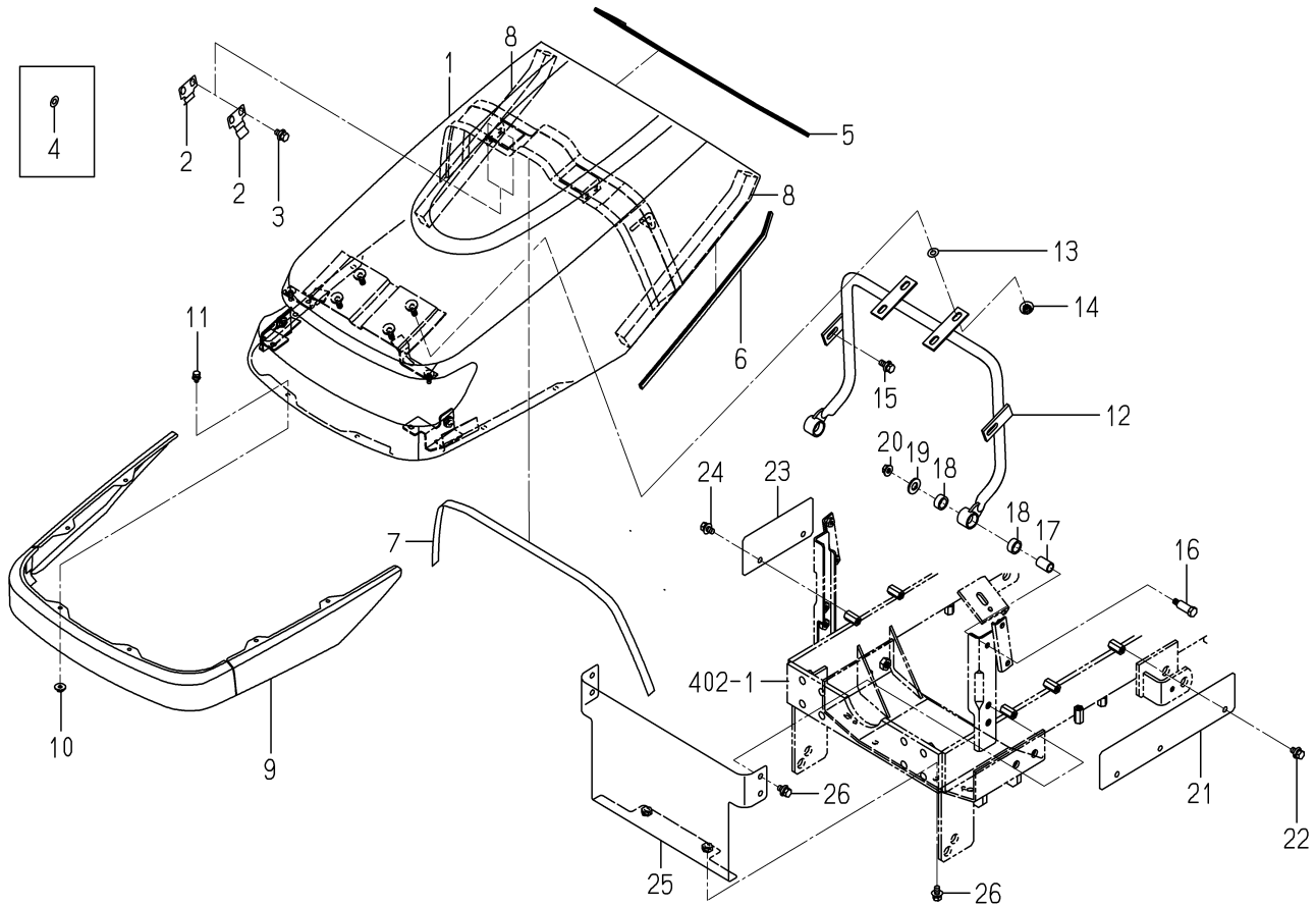
FIG.601 HOOD SYSTEM
