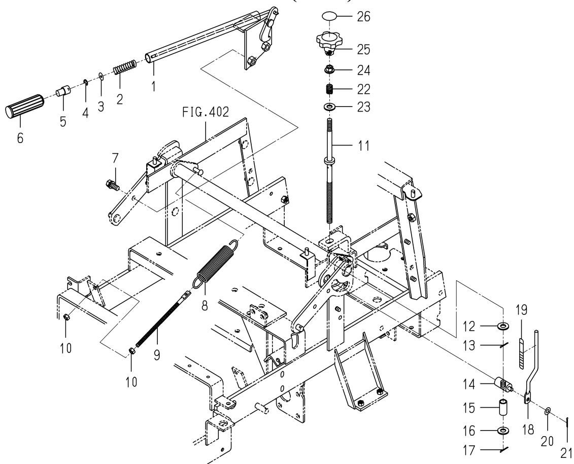
FIG.502 LEVER(LIFT)SYSTEM
