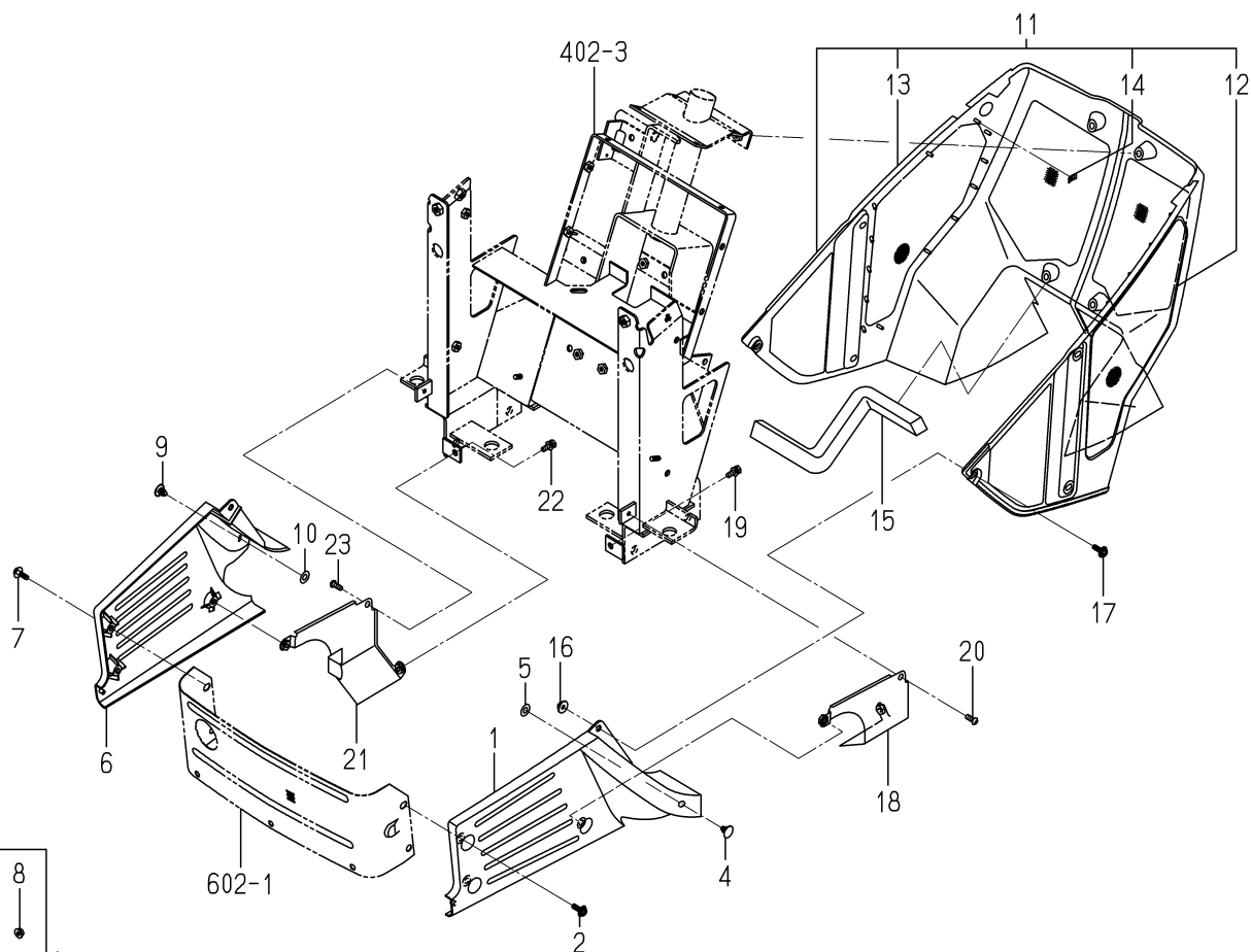
FIG.603 COVER SYSTEM
