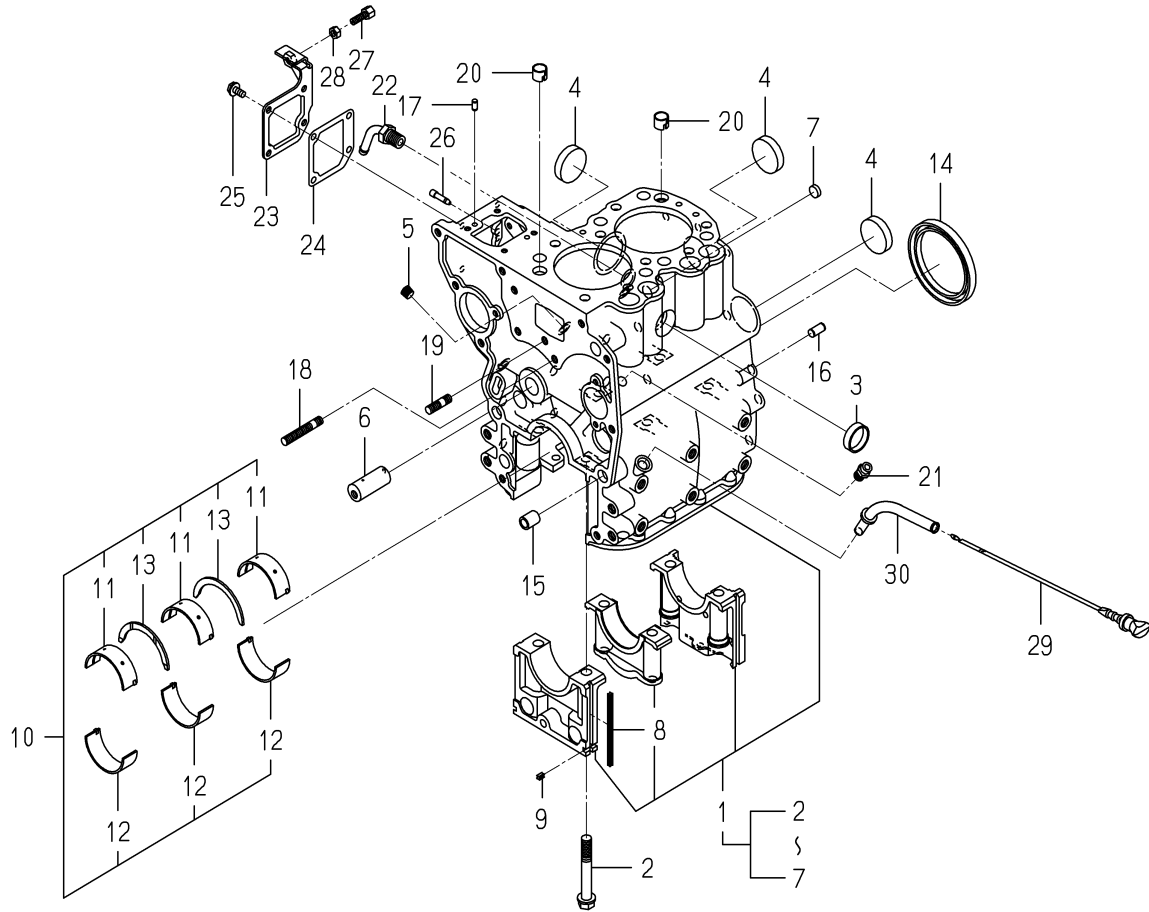
FIG.201 CYLINDER BLOCK
