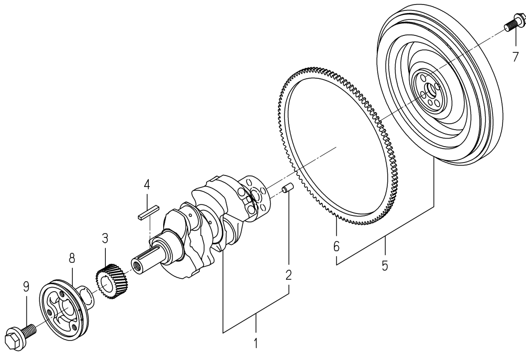
FIG.304 CRANK SHAFT
