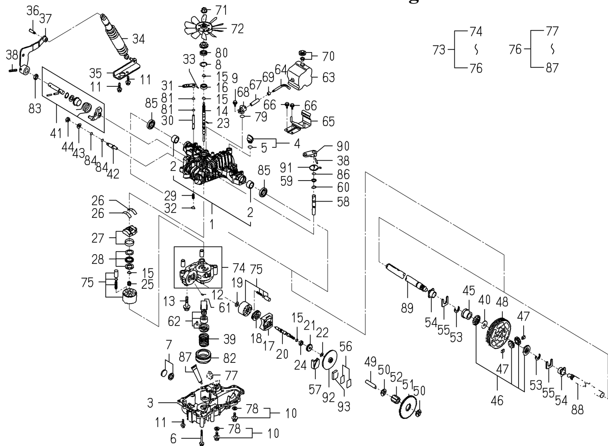
FIG.S01 COMPONENT PARTS FOR 1782-201-200-00 ON Fig.201
