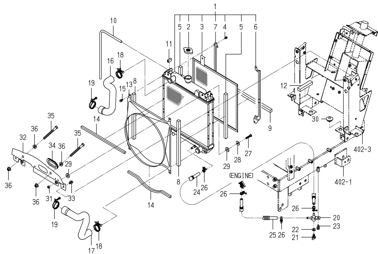
FIG.102 RADIATOR SYSTEM
