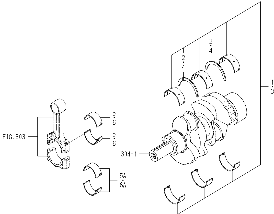
FIG.P02 BEARING/UNDER SIZE (OPTION)
