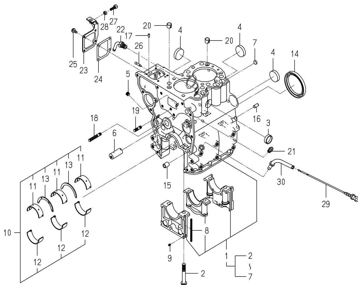
FIG.201 CYLINDER BLOCK
