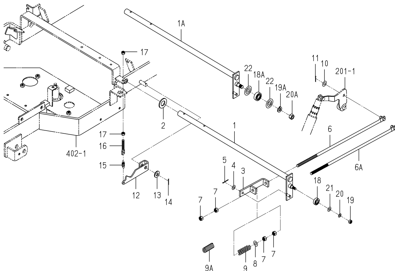
FIG.203 LINK(HST)SYSTEM
