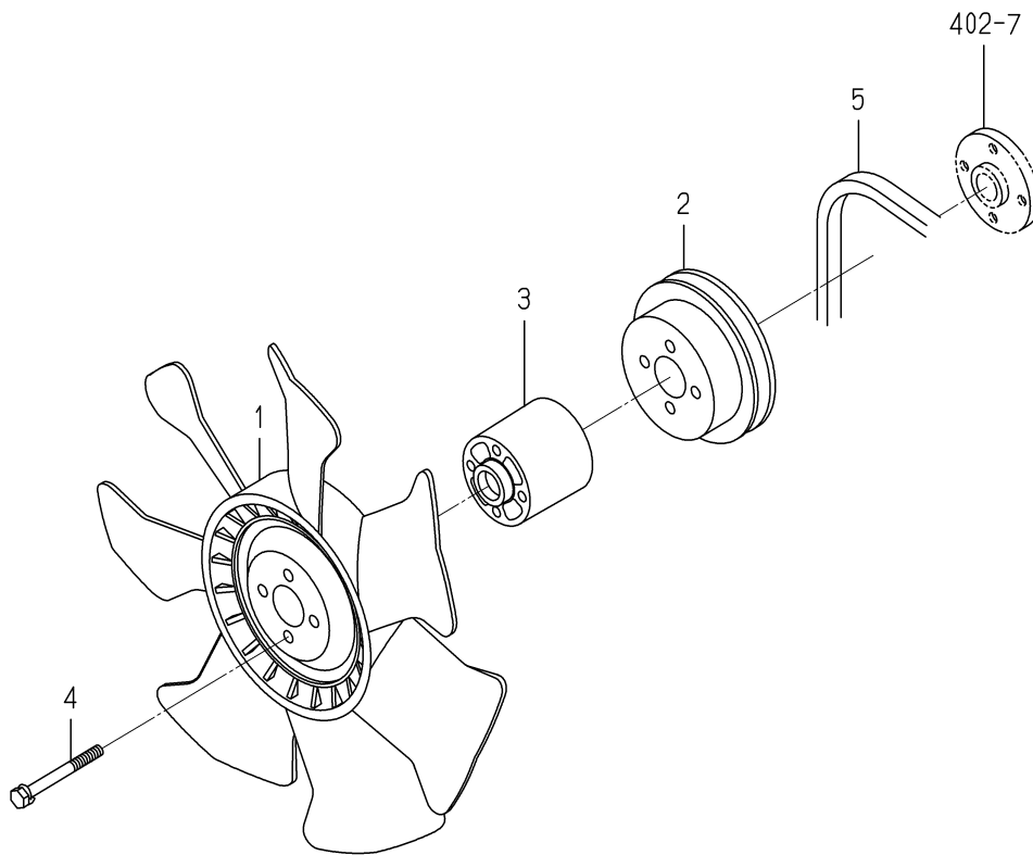
FIG.403 COOLING FAN
