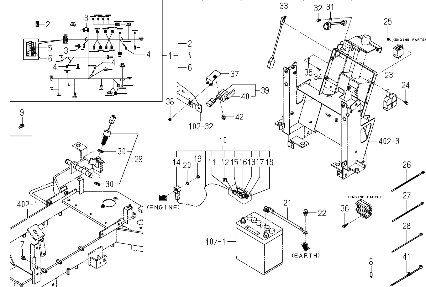
FIG.609 HARNESS(MAIN)SYSTEM(F TYPE)
