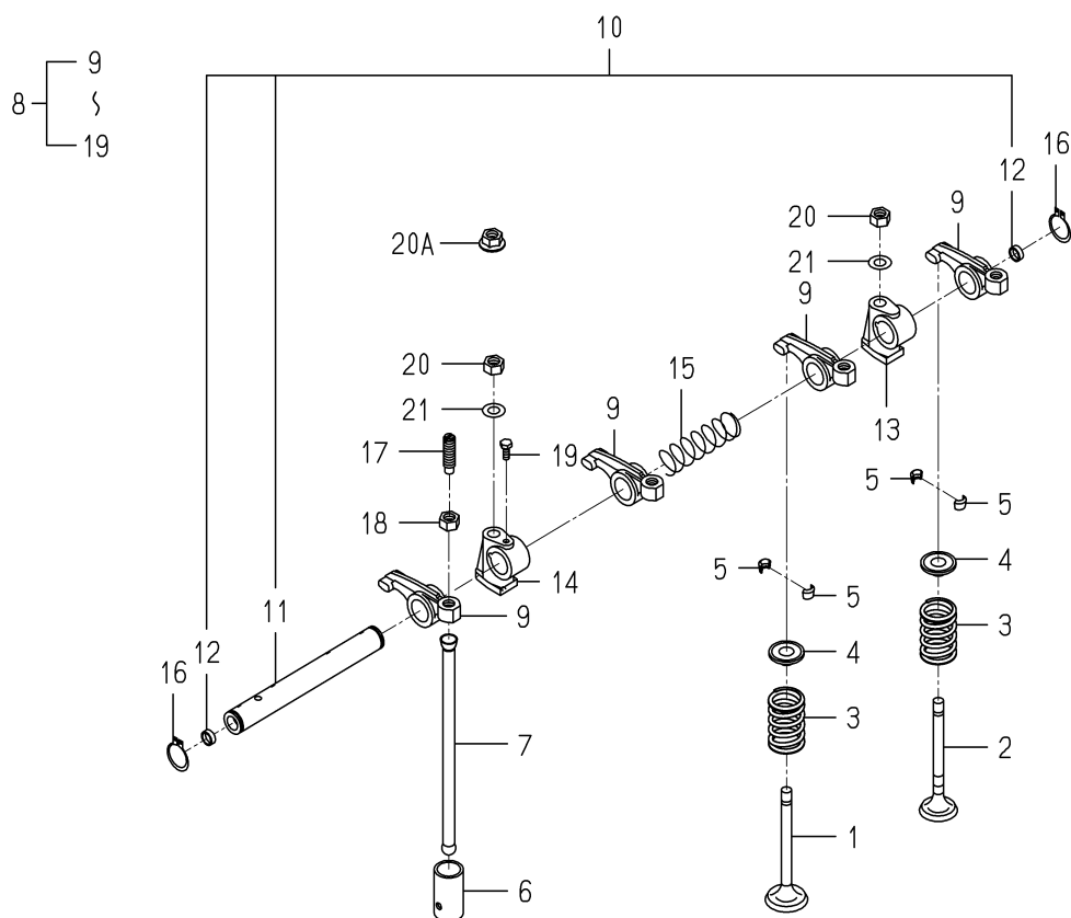
FIG.301 VALVE
