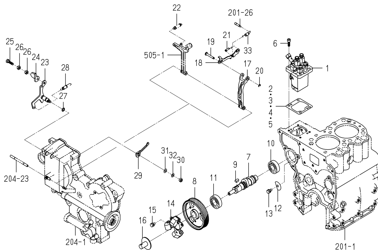
FIG.502 INJECTION PUMP
