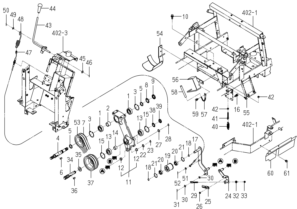
FIG.304 PTO(MOWER)SYSTEM
