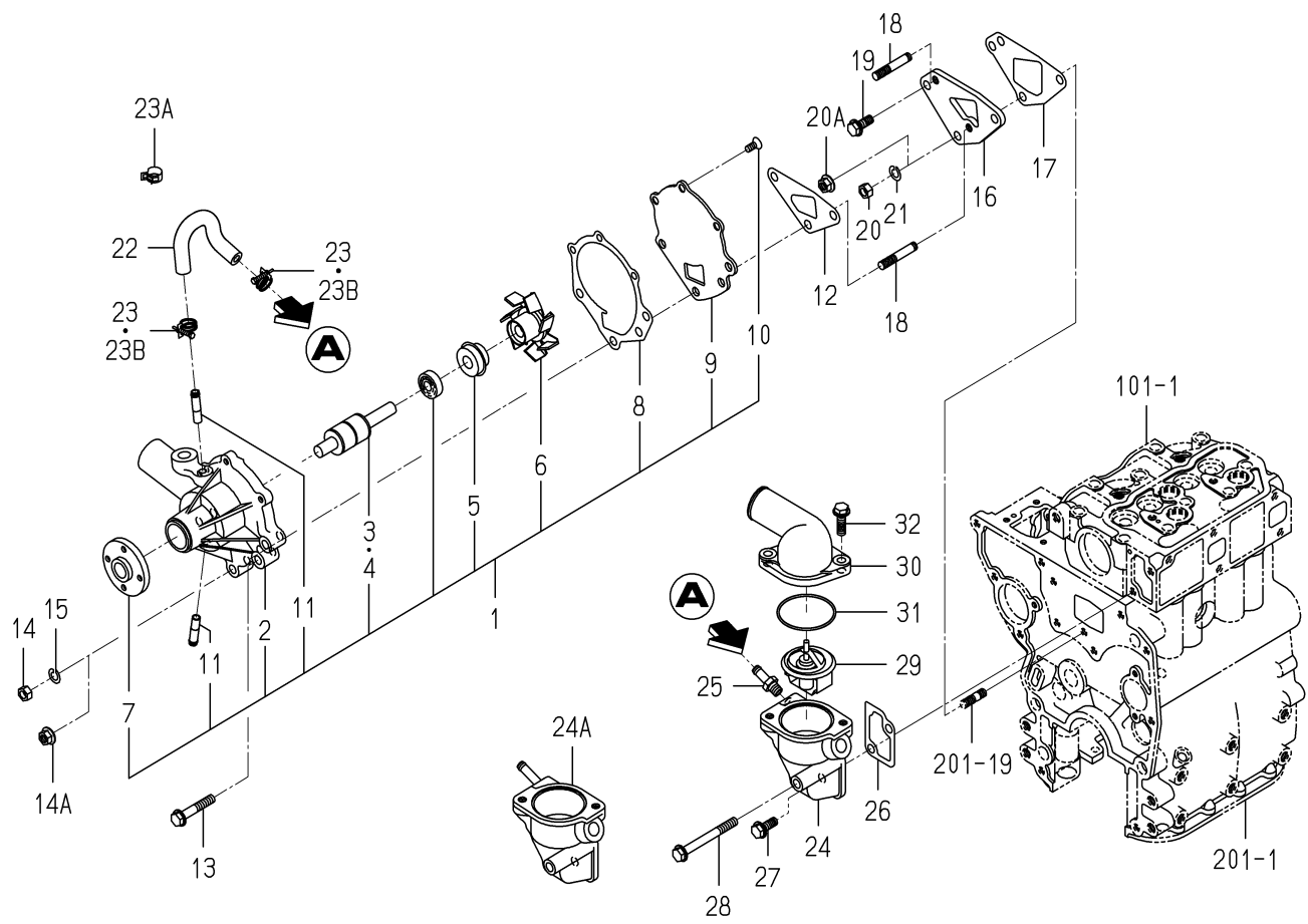
FIG.402 WATER PUMP
