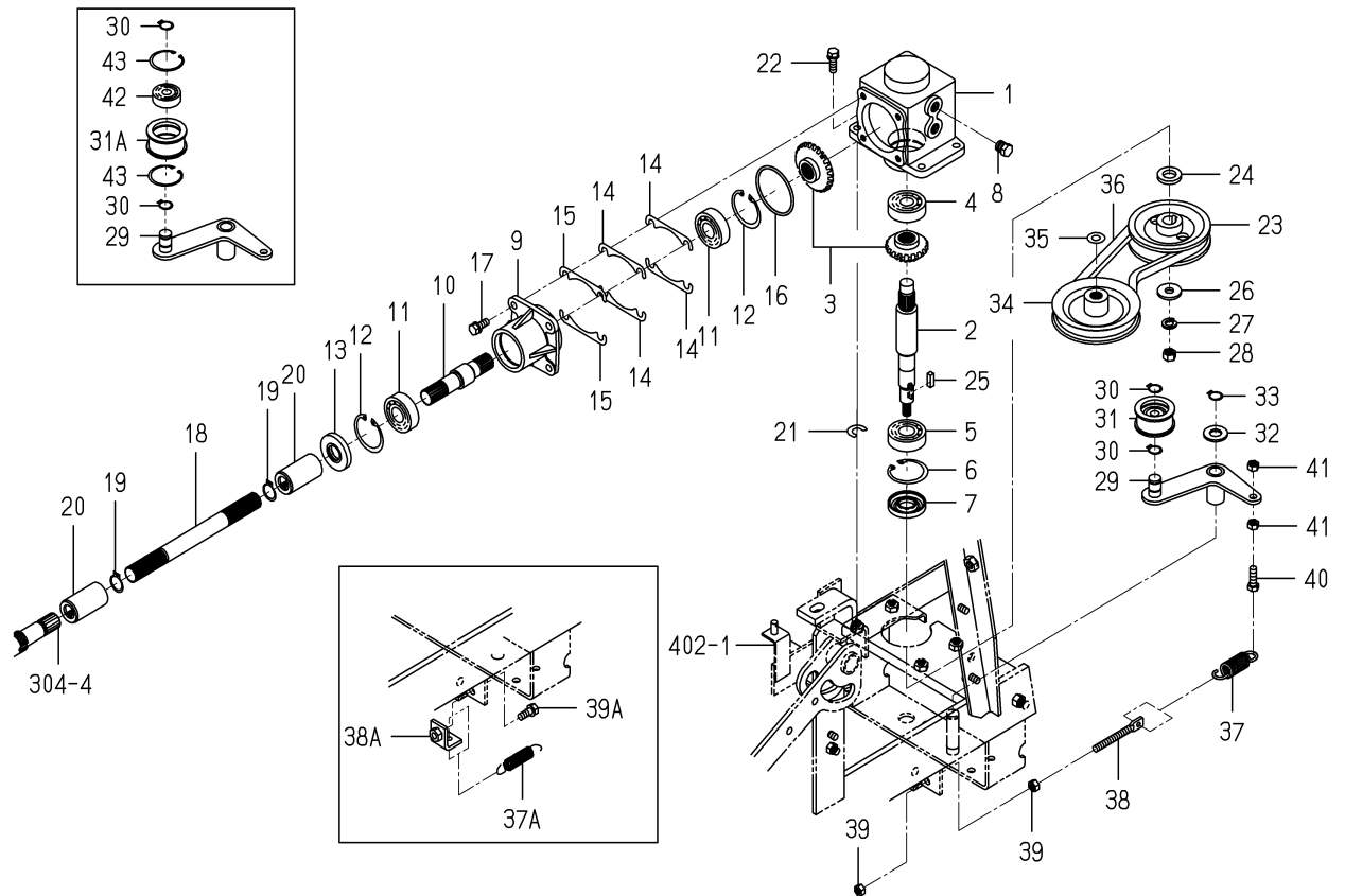
FIG.110 METAL(COUNTER)SYSTEM
