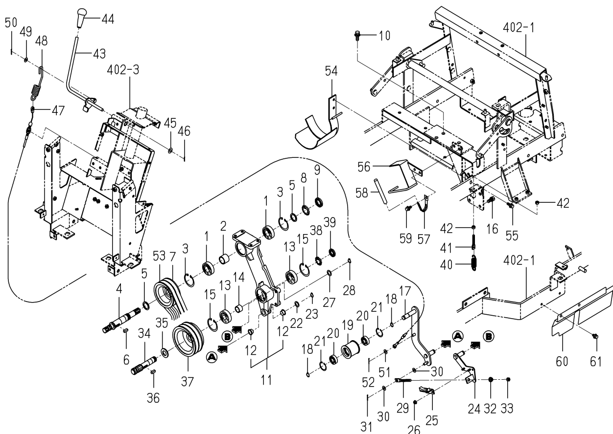
FIG.304 PTO(MOWER)SYSTEM
