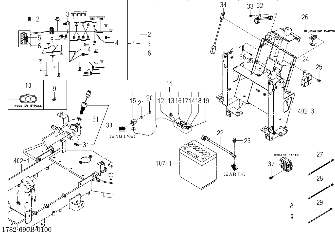
FIG.610 HARNESS(MAIN)SYSTEM(C TYPE)
