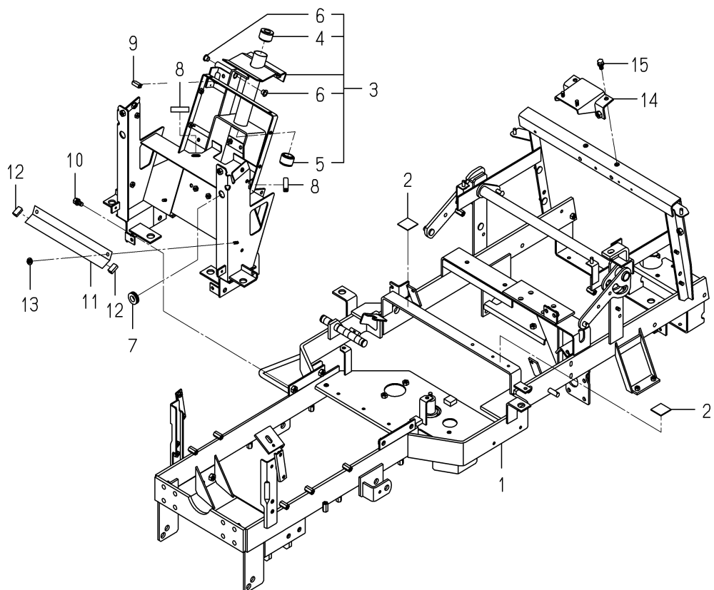
FIG.402 FRAME SYSTEM
