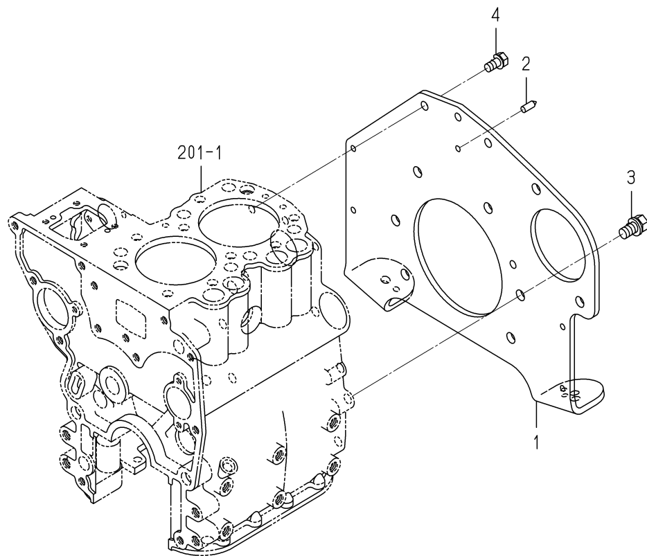
FIG.203 REAR PLATE
