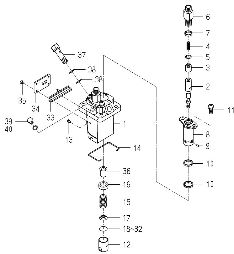
FIG.S02 COMPONENT PARTS FOR 6215-600-147-00 ON Fig.502
