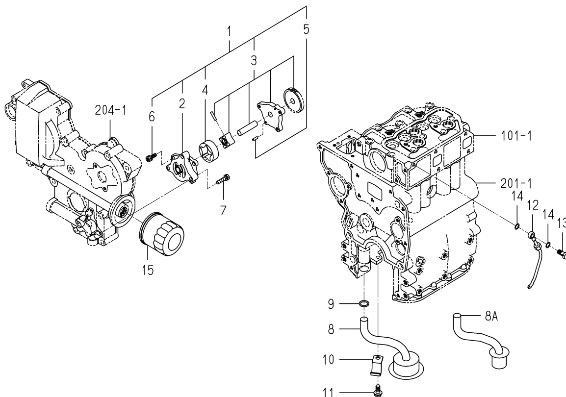
FIG.401 OIL PUMP
