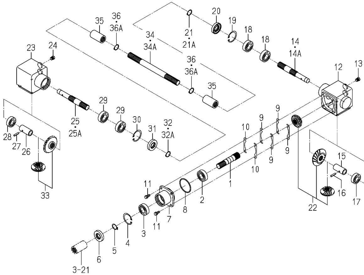
FIG.006 CASE(BEVEL)SYSTEM(SCMA48)
