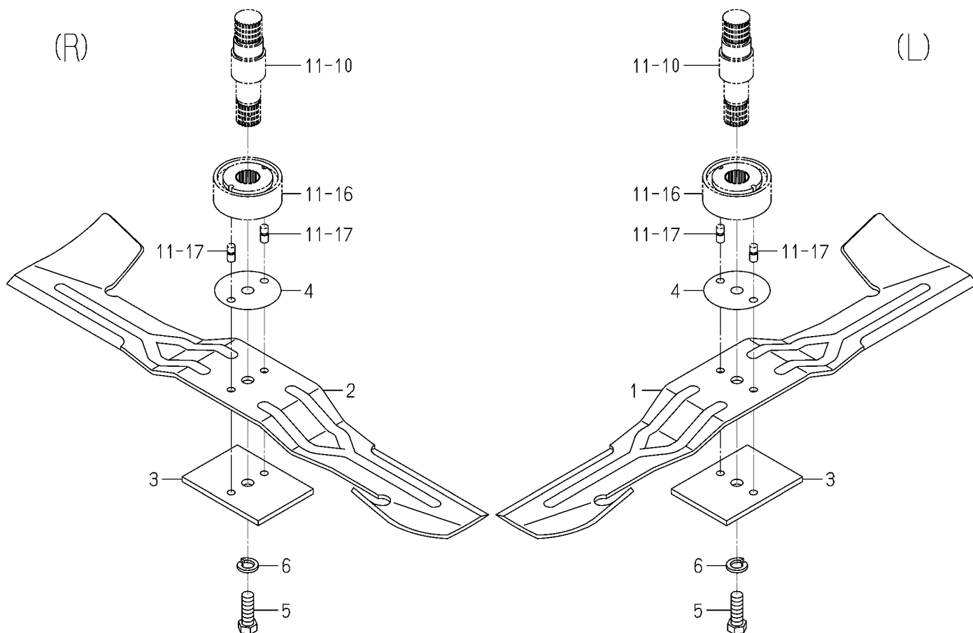
FIG.012 BLADE SYSTEM(SCMA48)
