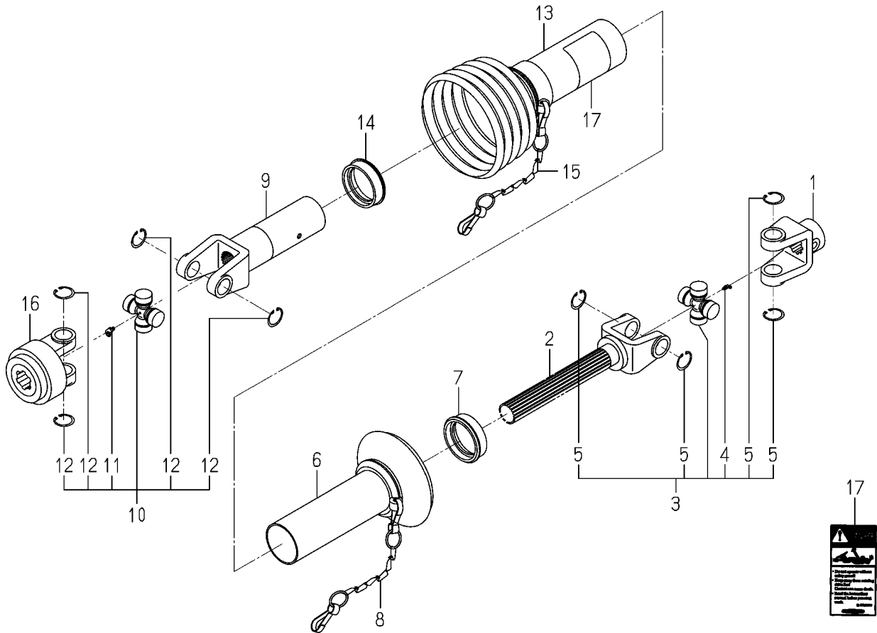
FIG.030 COMPONENT PARTS FOR 8663-101-510-00 ON Fig.1
