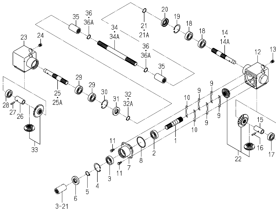
FIG.006 CASE(BEVEL)SYSTEM(SCMA48)
