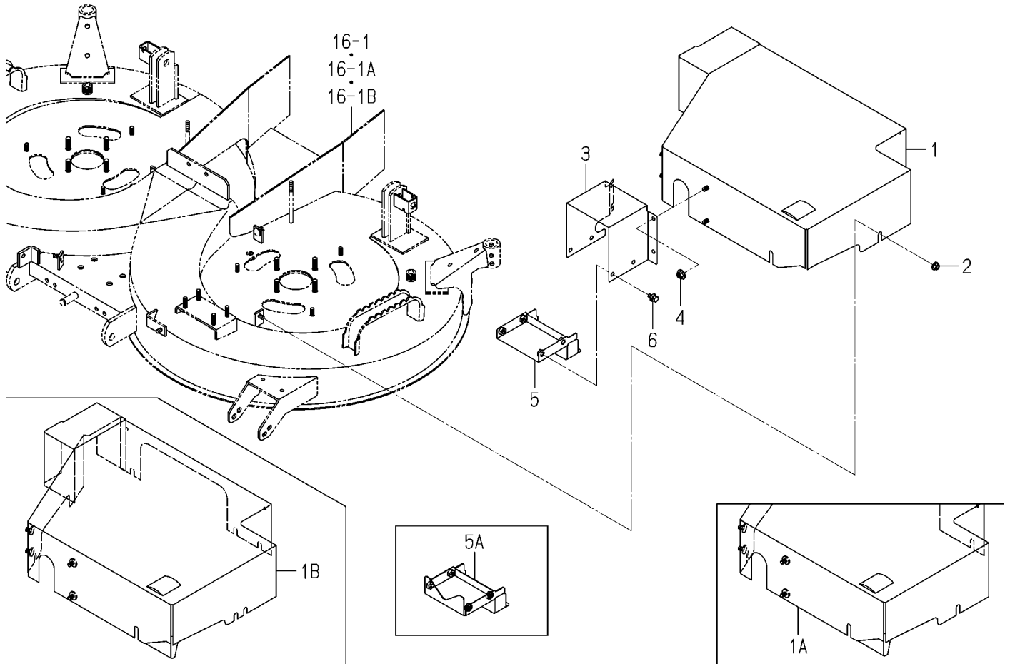
FIG.021 COVER(BELT)SYSTEM (SCMA54)(NO.1-400725)
