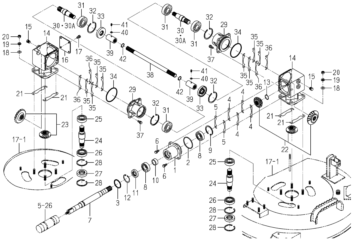
FIG.008 CASE(BEVEL)SYSTEM(SCMA54)(NO.500001-)
