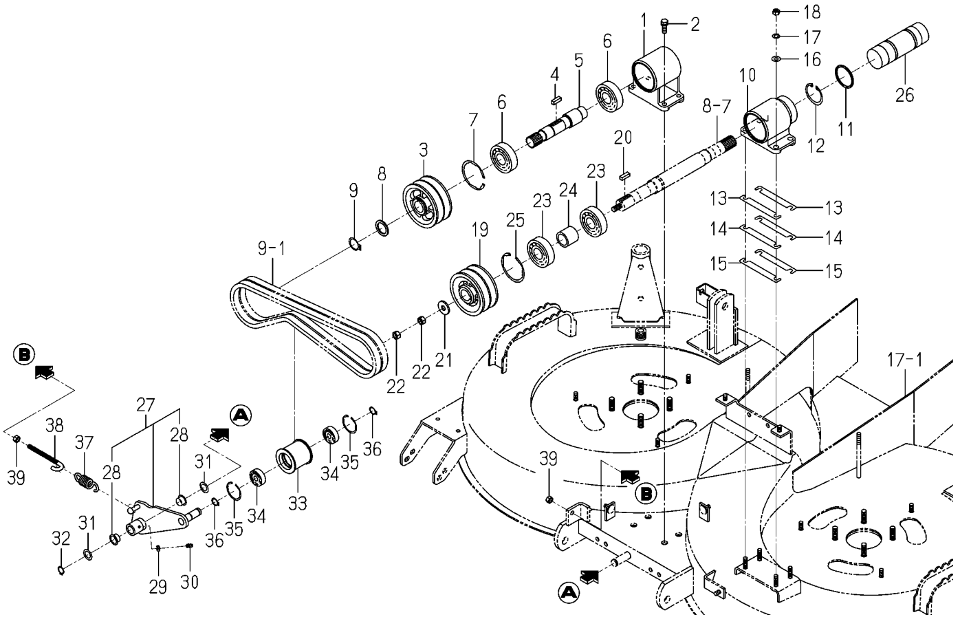
FIG.005 PULLEY SYSTEM(SCMA54)(NO.500001-)
