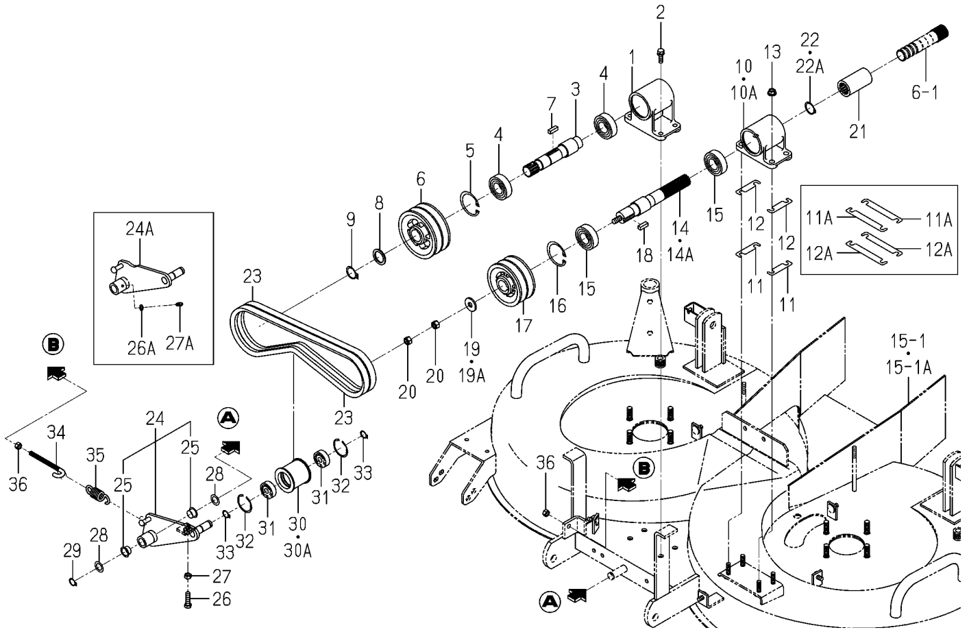
FIG.003 PULLEY SYSTEM(SCMA48)
