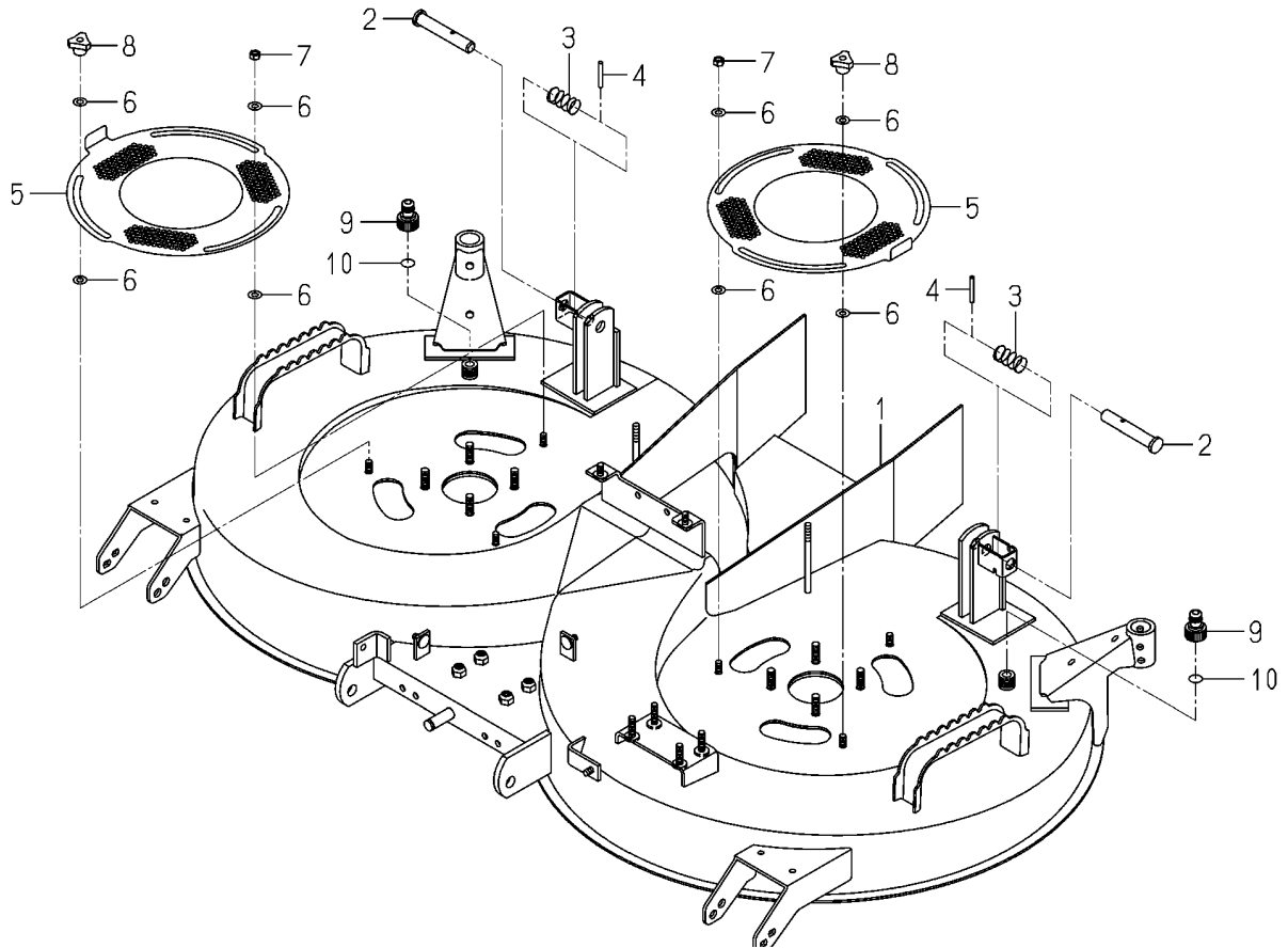
FIG.017 DECK(MOWER)SYSTEM (SCMA54)(NO.500001-)
