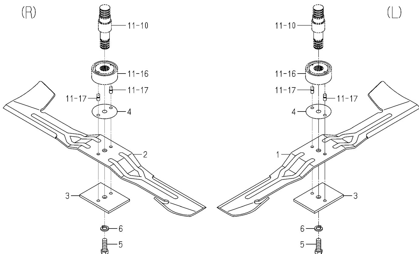
FIG.013 BLADE SYSTEM(SCMA54)(NO.1-400725)
