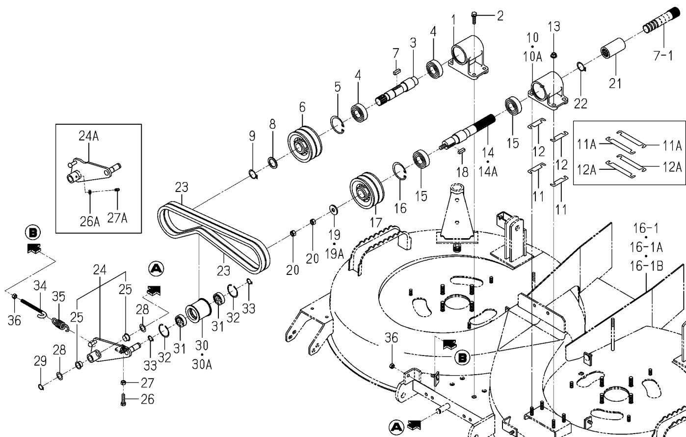
FIG.004 PULLEY SYSTEM(SCMA54)(NO.1-400725)
