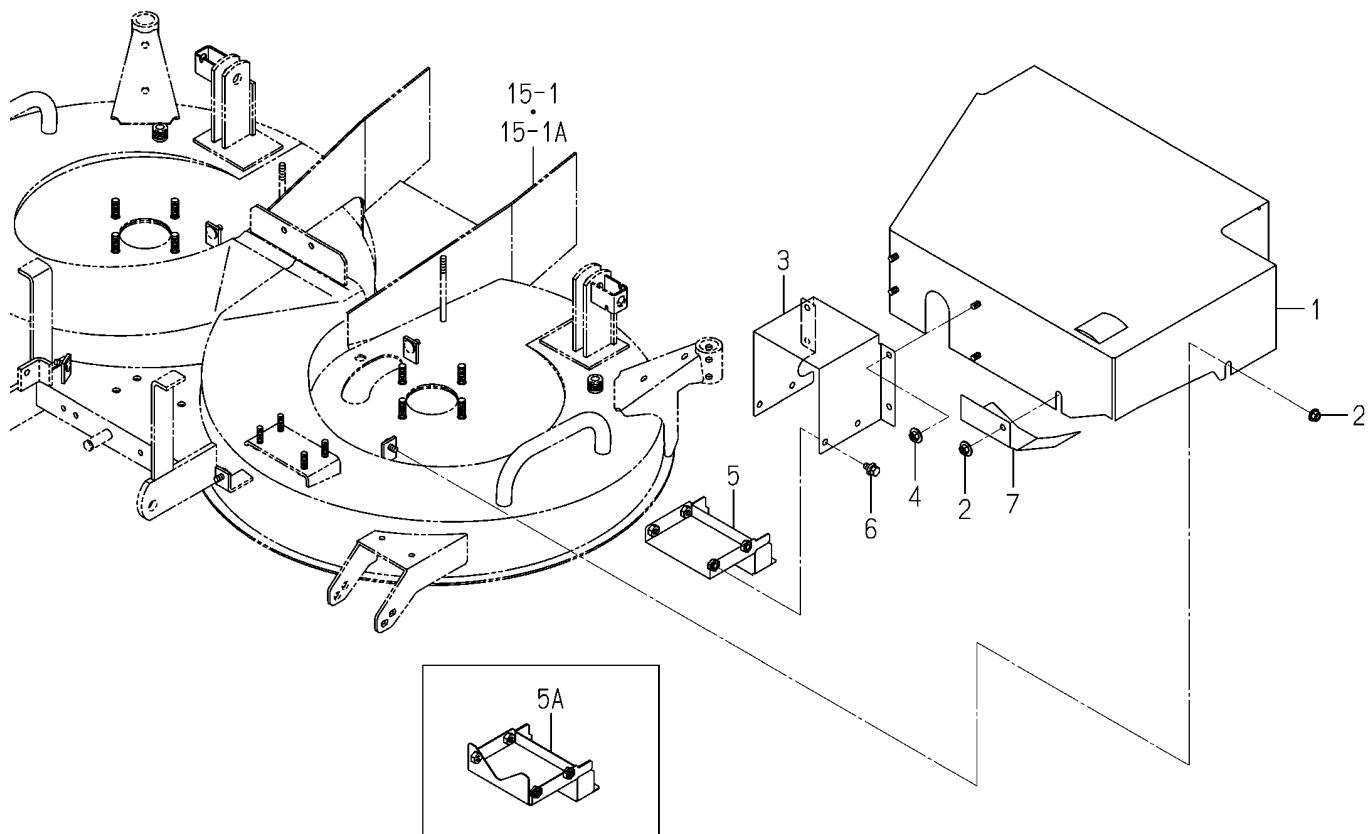
FIG.020 COVER(BELT)SYSTEM(SCMA48)
