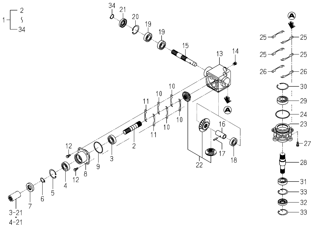
FIG.029 GEAR(B/21-25-21),GEAR(BEVEL/25-21)SET (SCMA54-NO.1-400725) (1/2)
