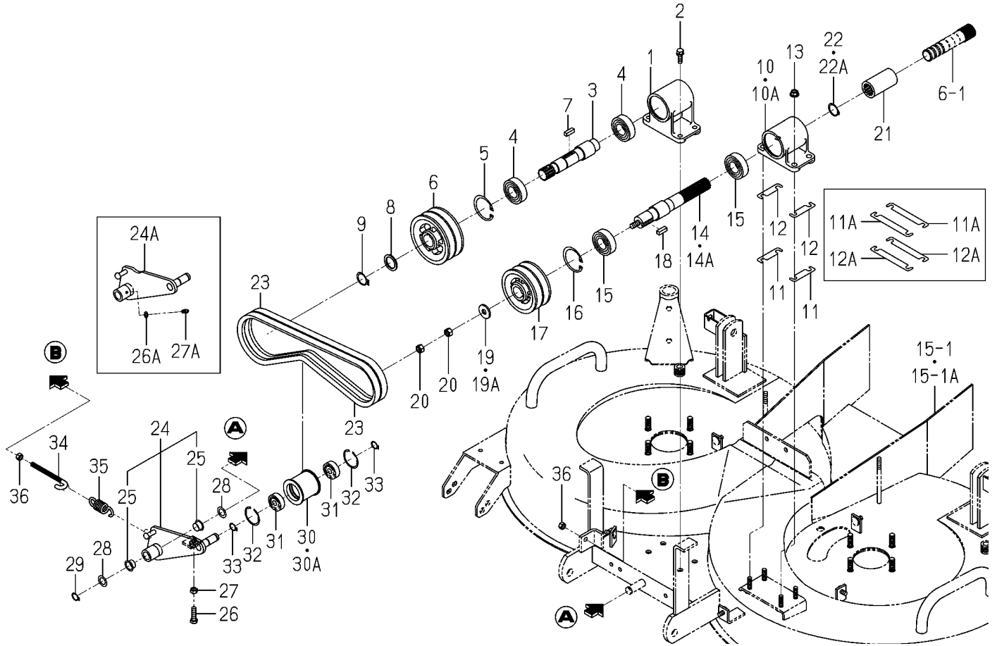
FIG.003 PULLEY SYSTEM(SCMA48)
