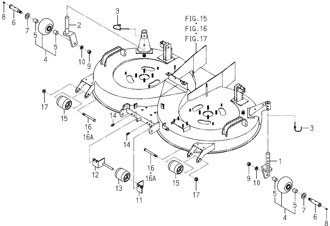
FIG.023 WHEEL(GAUGE)SYSTEM
