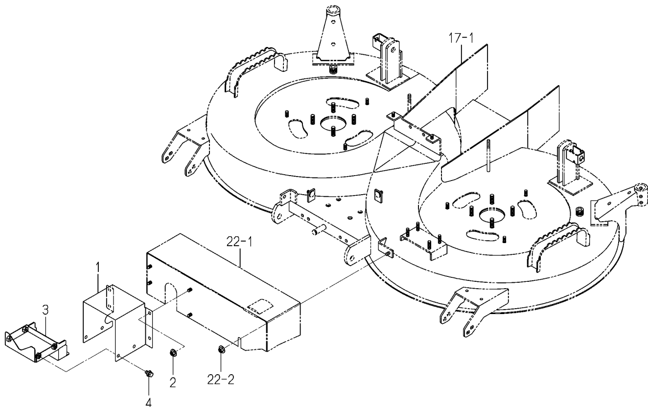
FIG.002 COVER(JOINT)SYSTEM(SCMA54)(NO.500001-)
