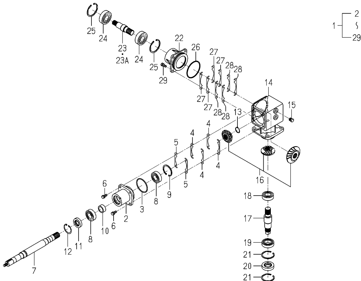
FIG.028 GEAR(B/21-25-21),GEAR(BEVEL/25-21)SET (SCMA54)(NO.500001-) (1/2)
