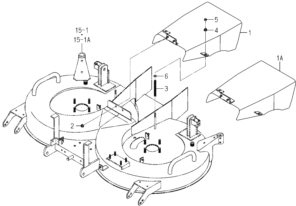
FIG.018 COVER(DISCHARGE)SYSTEM(SCMA48)
