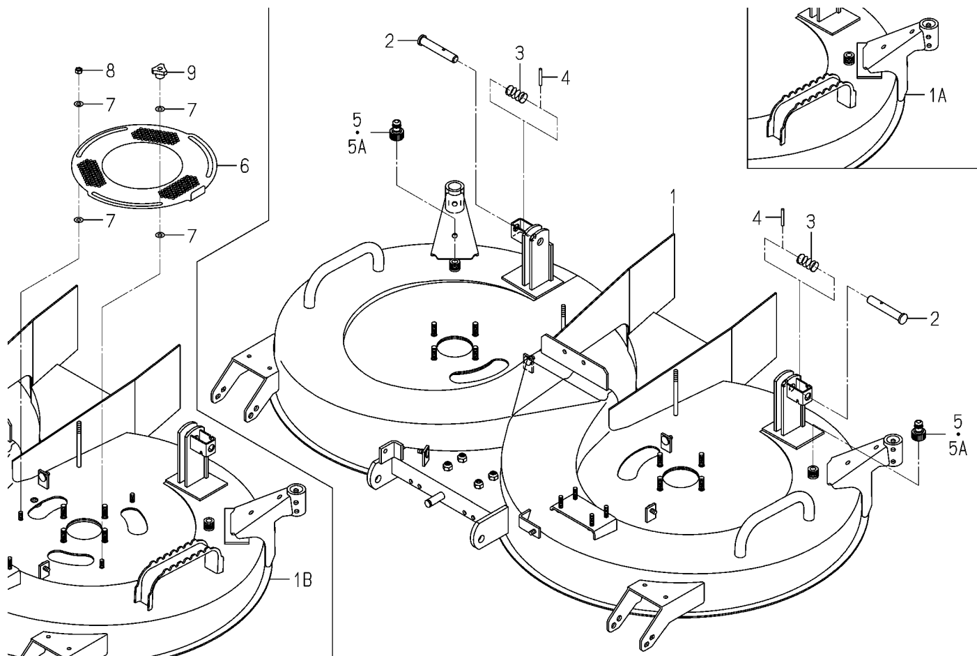
FIG.016 DECK(MOWER)SYSTEM (SCMA54)(NO.1-400725)
