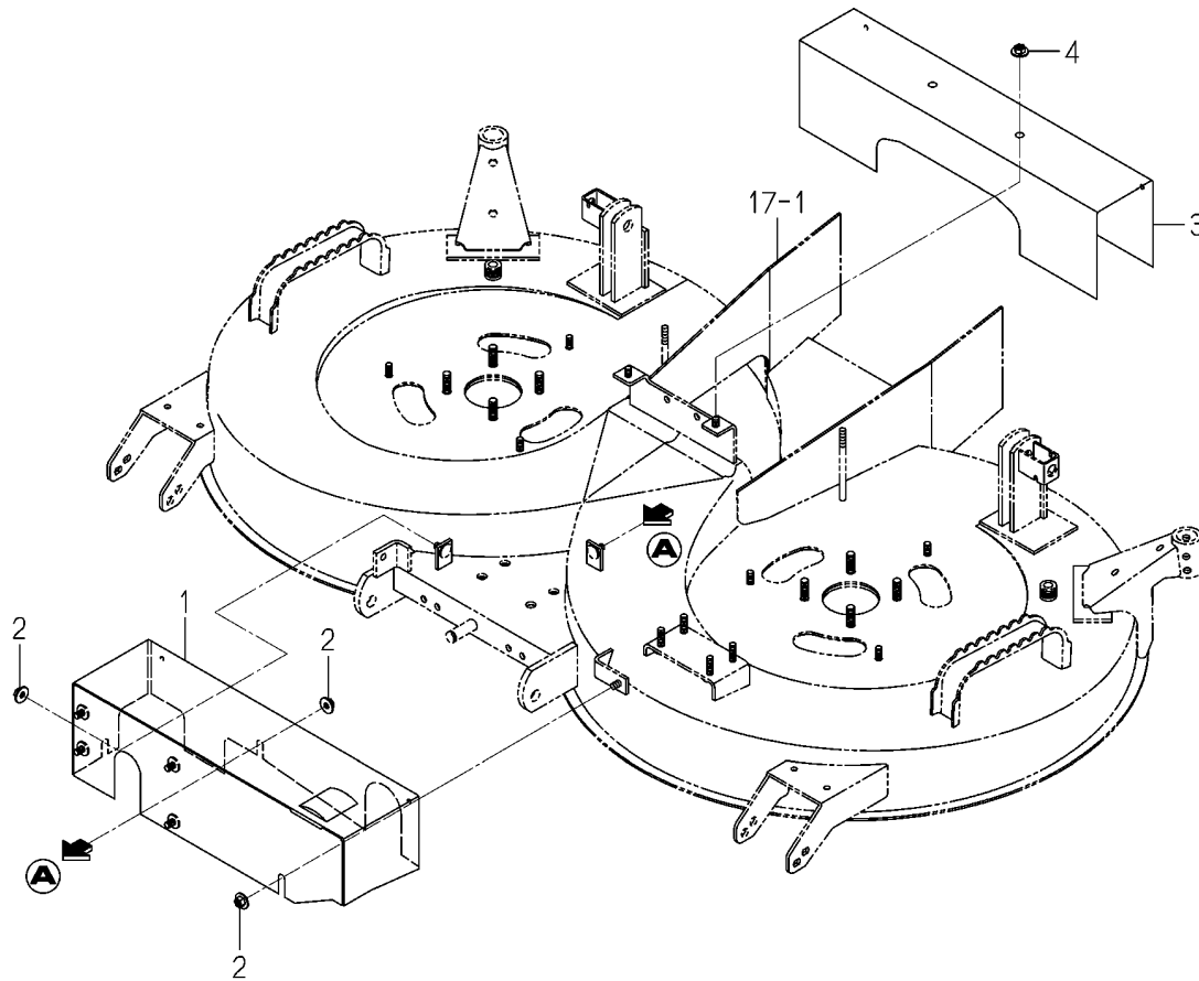
FIG.022 COVER SYSTEM(SCMA54)(NO.500001-)
