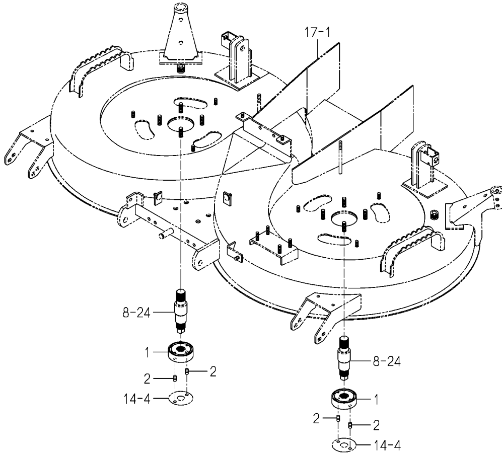
FIG.010 COLLAR(BRADE)SYSTEM (SCMA54)(NO.500001-)
