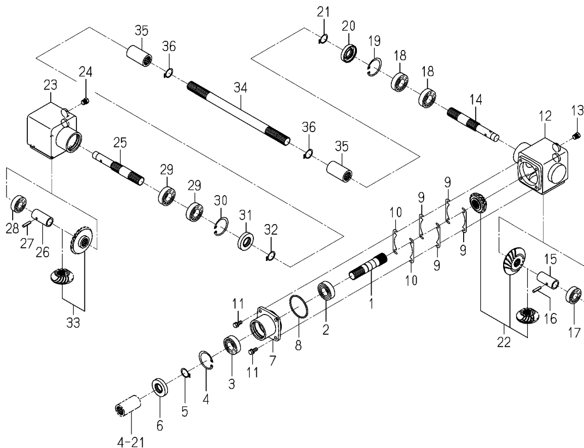
FIG.007 CASE(BEVEL)SYSTEM(SCMA54)(NO.1-400725)
