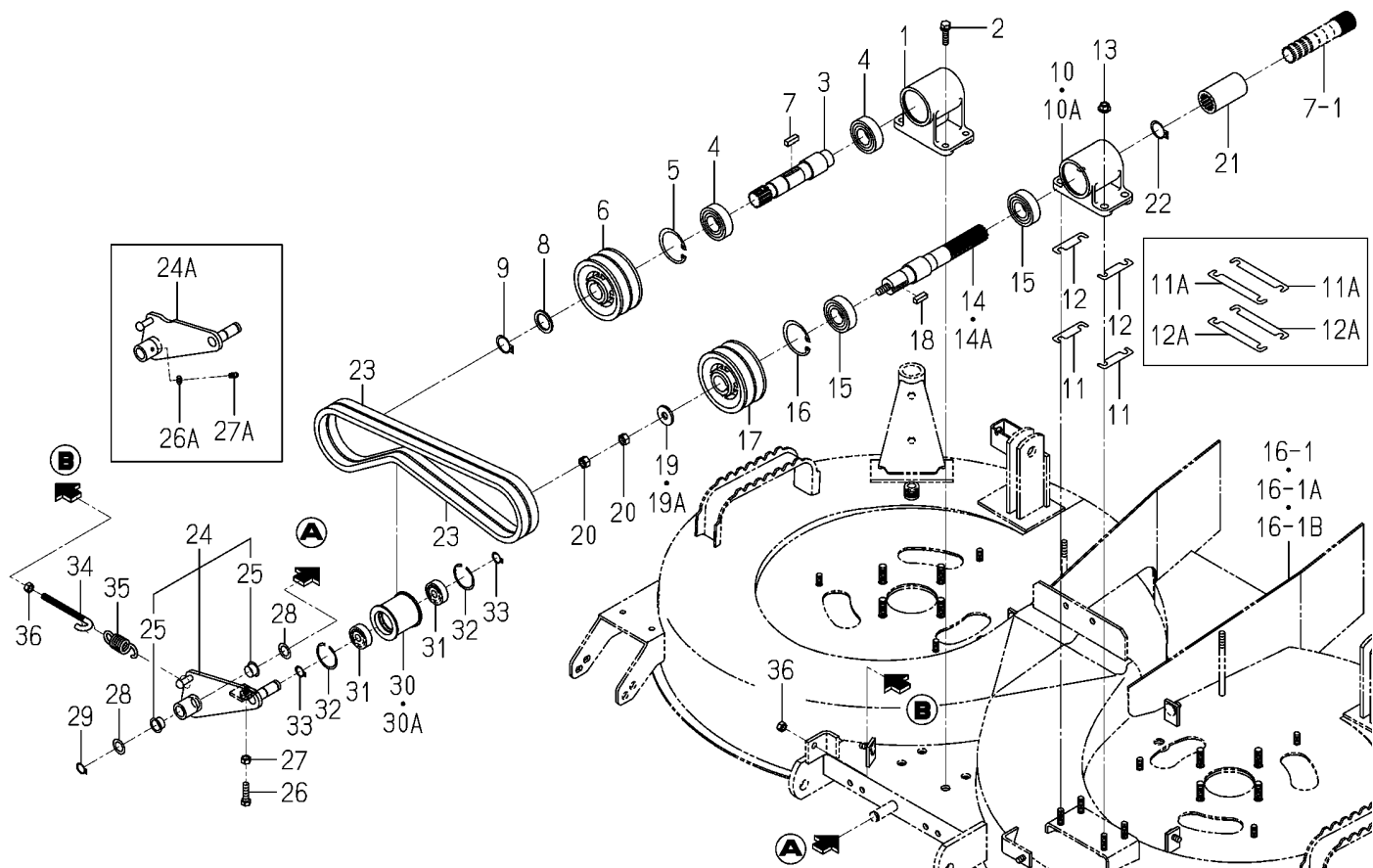
FIG.004 PULLEY SYSTEM(SCMA54)(NO.1-400725)
