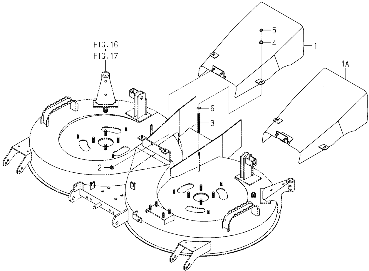
FIG.019 COVER(DISCHARGE)SYSTEM(SCMA54)
