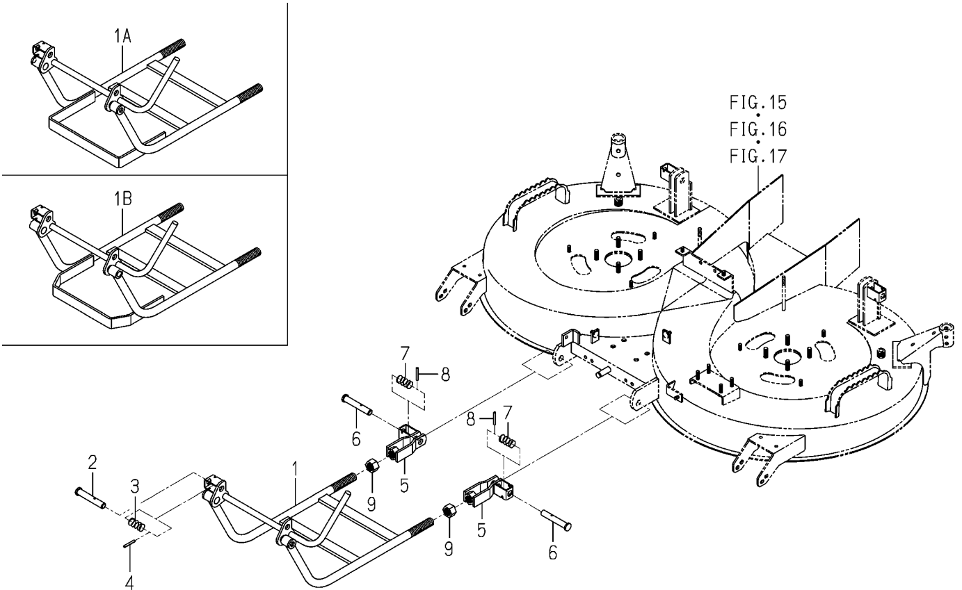
FIG.024 LINK SYSTEM
