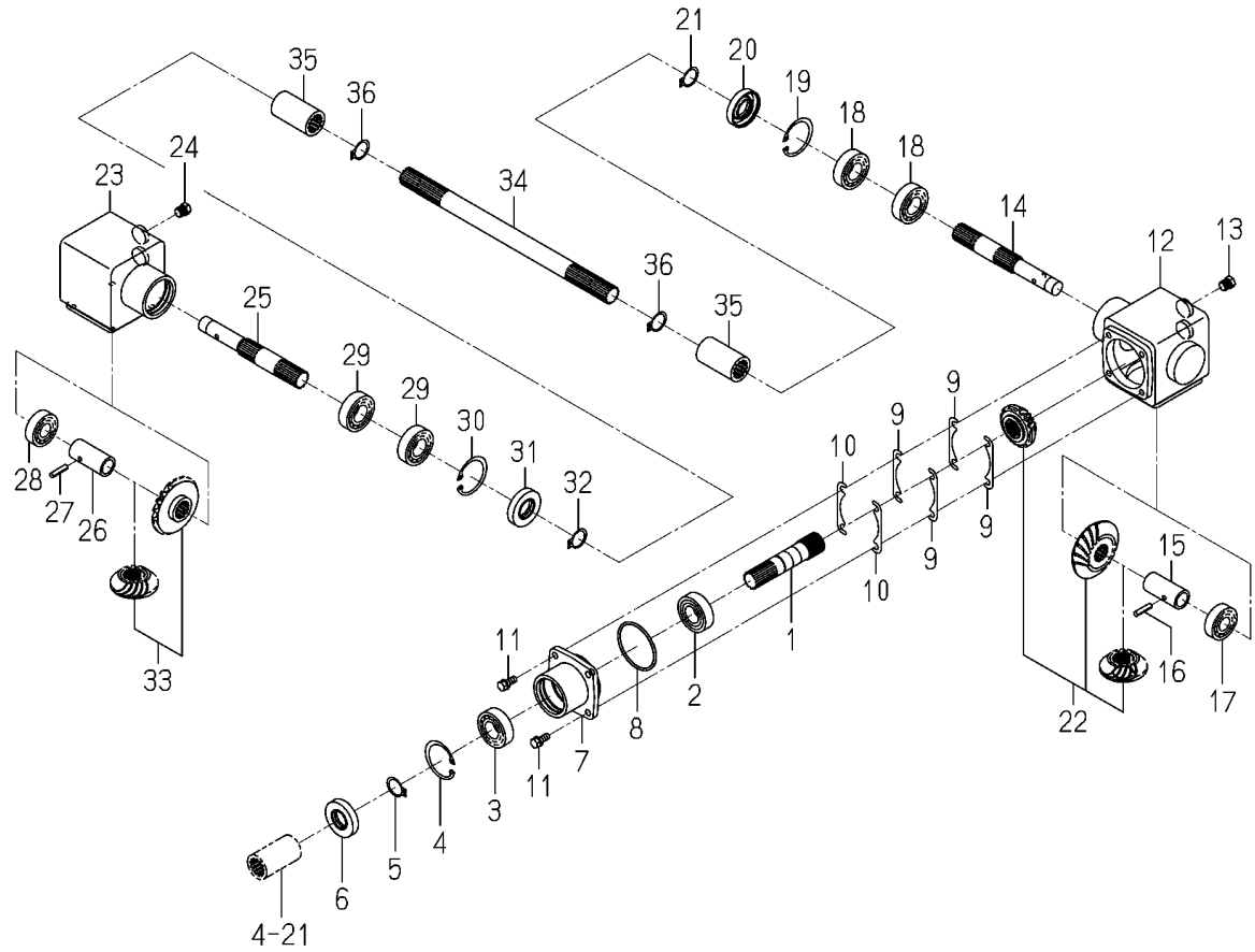
FIG.007 CASE(BEVEL)SYSTEM(SCMA54)(NO.1-400725)
