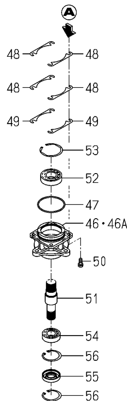
FIG.029A GEAR(B/21-25-21),GEAR(BEVEL/25-21)SET (SCMA54-NO.1-400725) (2/2)
