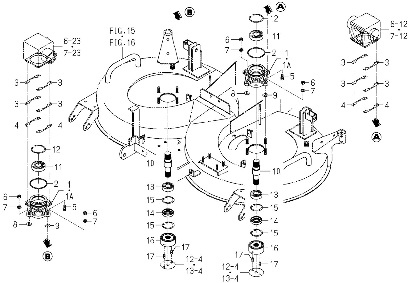
FIG.011 METAL SYSTEM(NO.1-400725)
