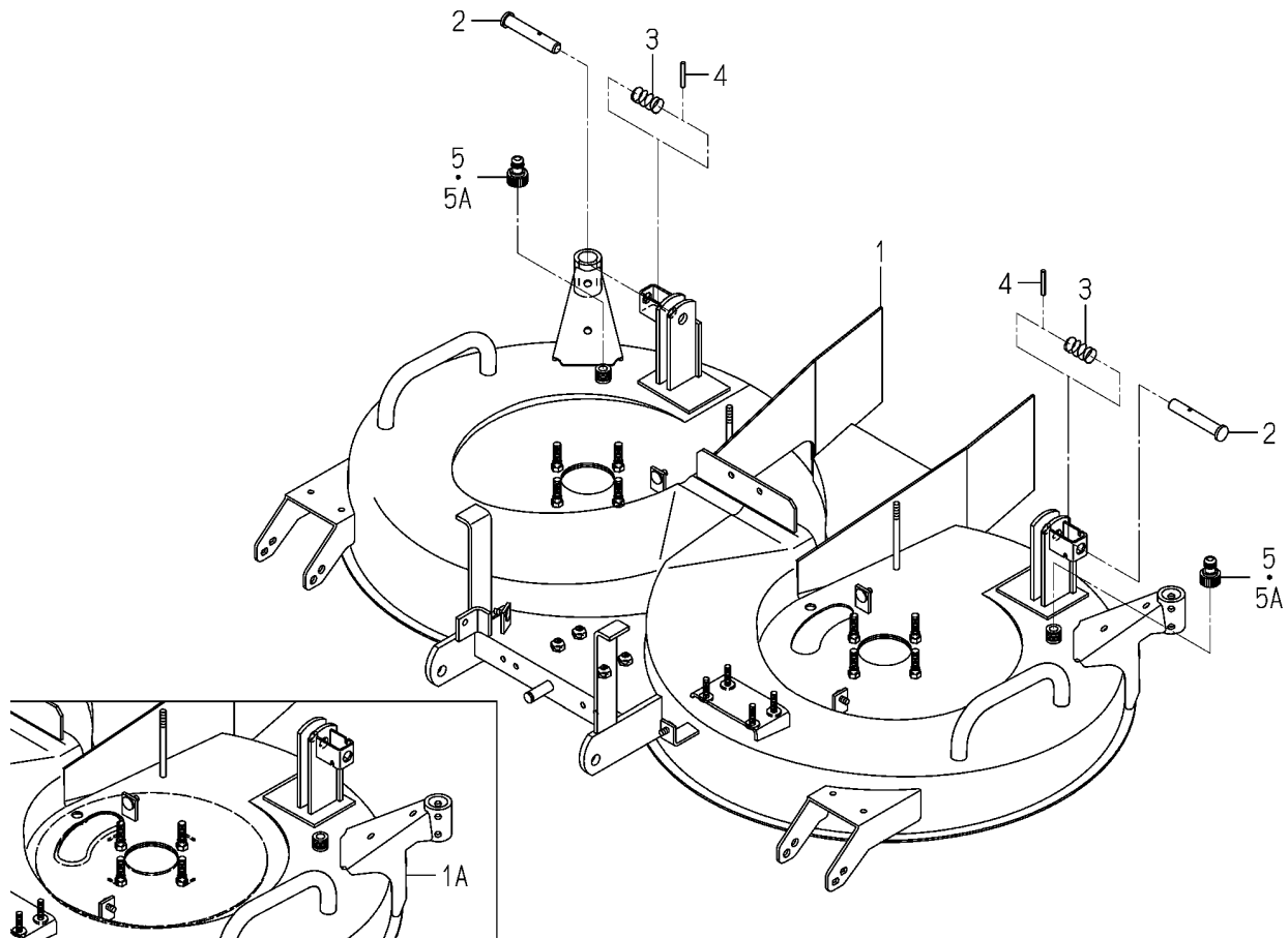
FIG.015 DECK(MOWER)SYSTEM(SCMA48)
