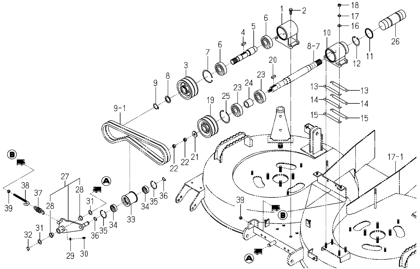
FIG.005 PULLEY SYSTEM(SCMA54)(NO.500001-)
