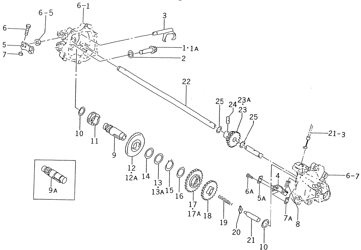
FIG. 7 GEAR SYSTEM Pignonnerie
