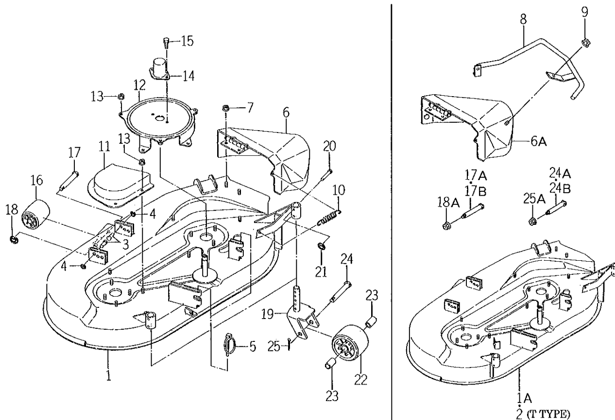
FIG. 21 DECK AND COVER SYSTEM
