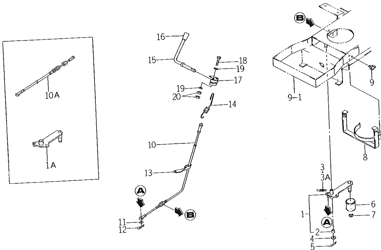
FIG. 13 P.T.O. SYSTEM
