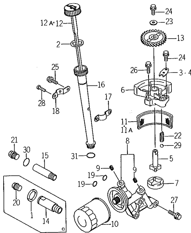
FIG. 4 LUBRICATION EQUIPMENT
