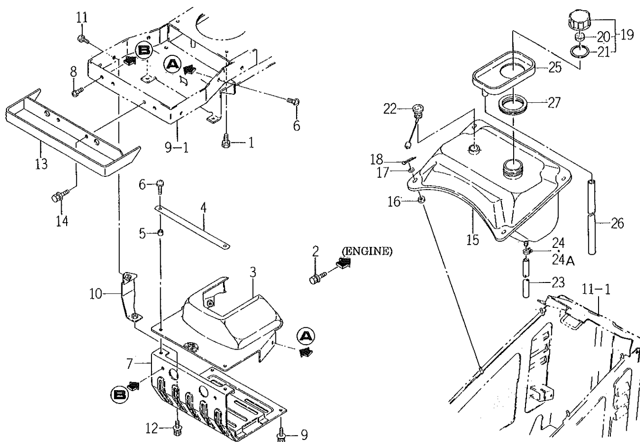
FIG. 1 SHROUD AND FUEL TANK SYSTEM
