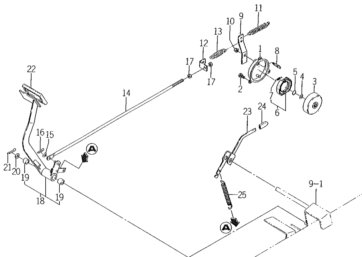
FIG. 7 BRAKE SYSTEM
