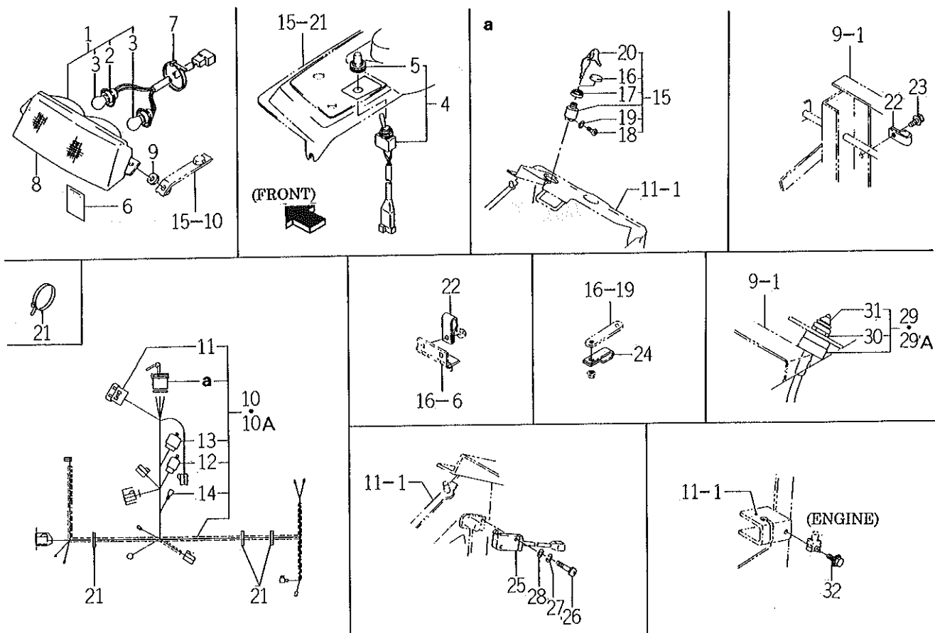
FIG. 17 ELECTRICAL SYSTEM
