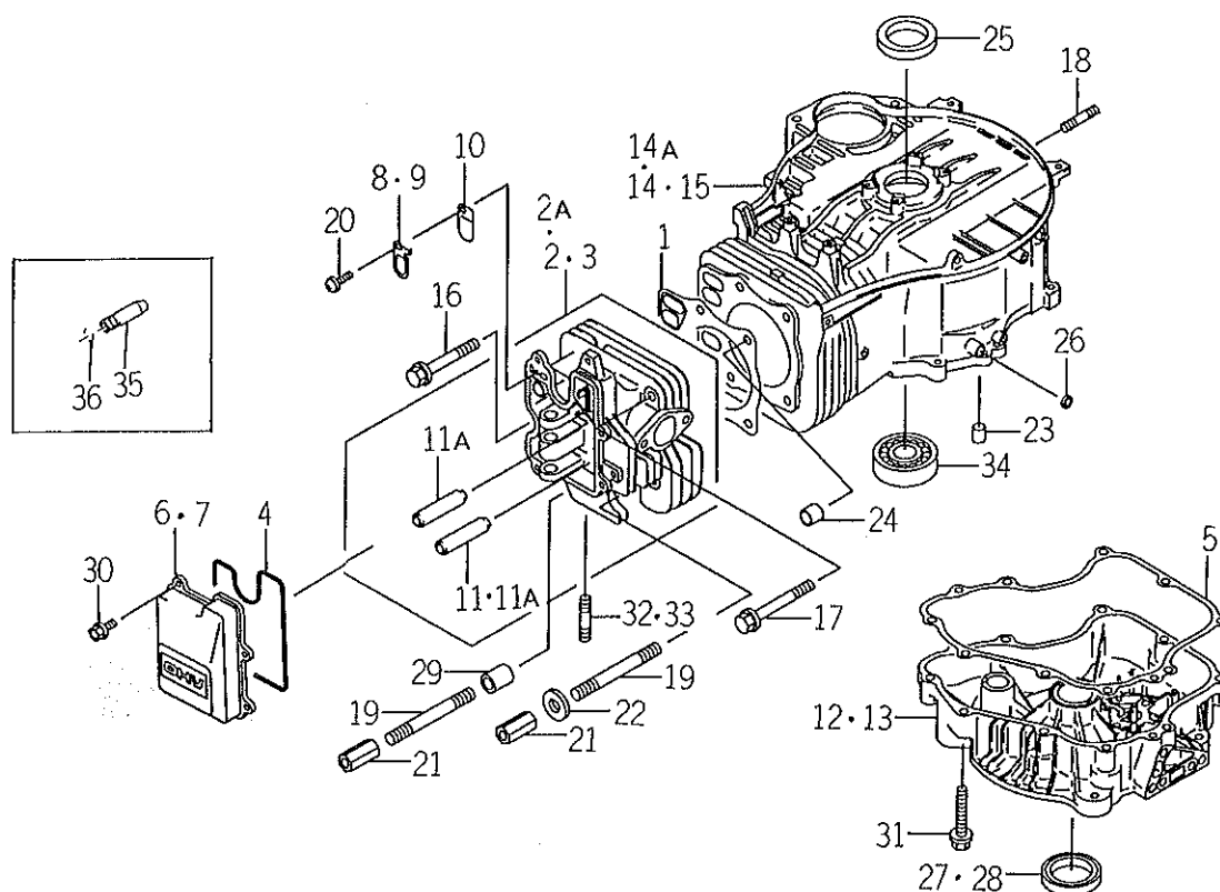
FIG. 1 CYLINDER CRANKCASE
