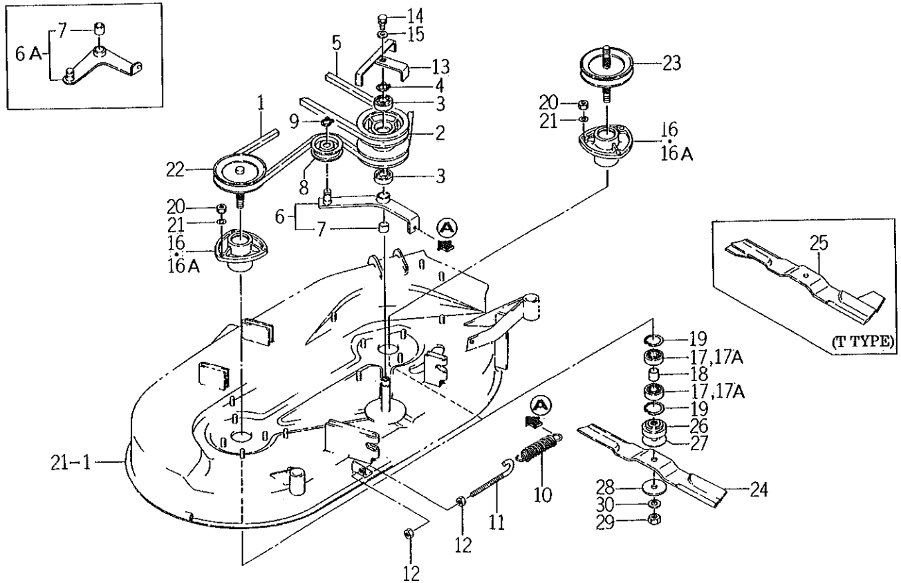
FIG. 20 DRIVING SYSTEM
