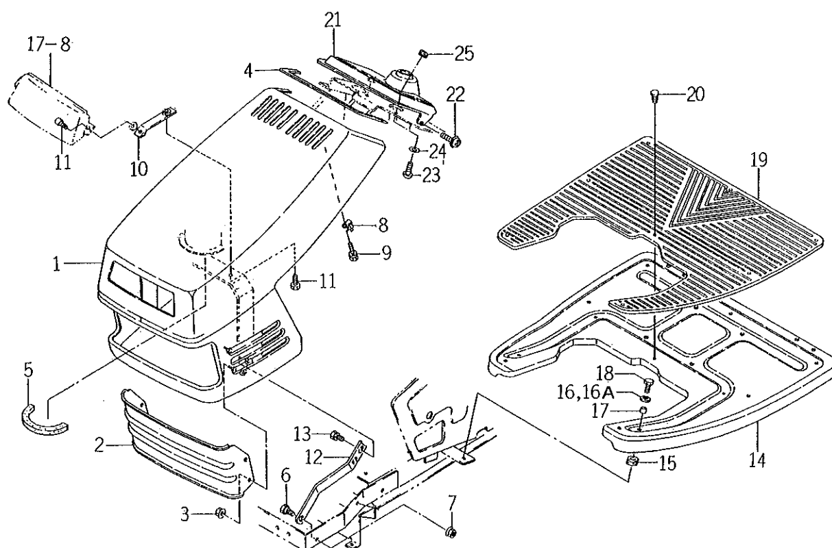
FIG. 15 HOOD AND PANEL SYSTEM
