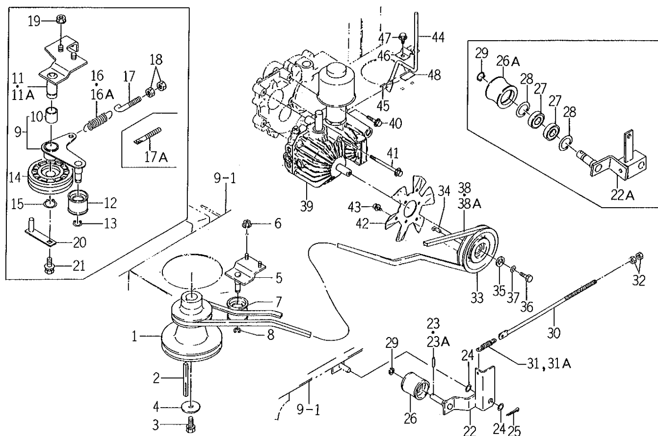
FIG. 4 BELT (DRIVING) AND HST SYSTEM
