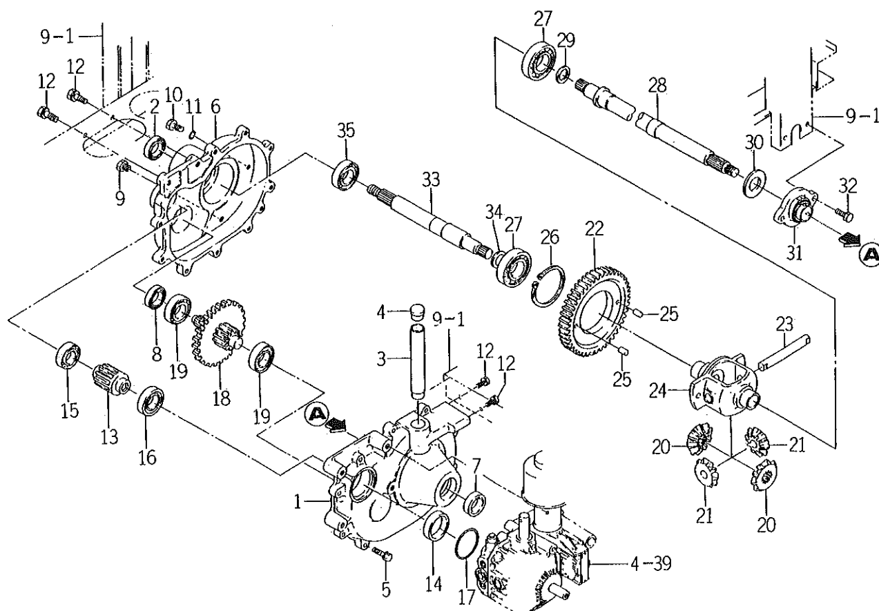
FIG. 6 CASE (TRANSMISSION) SYSTEM
