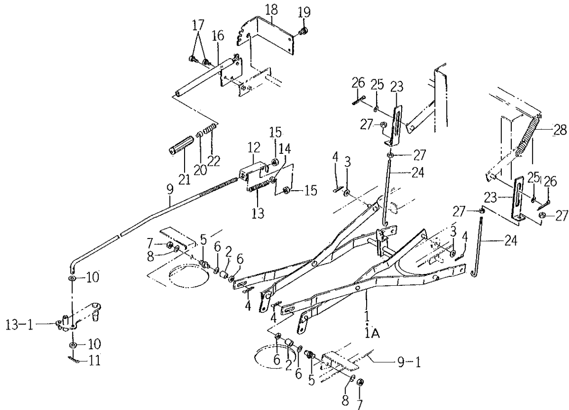
FIG. 14 LINK SYSTEM
