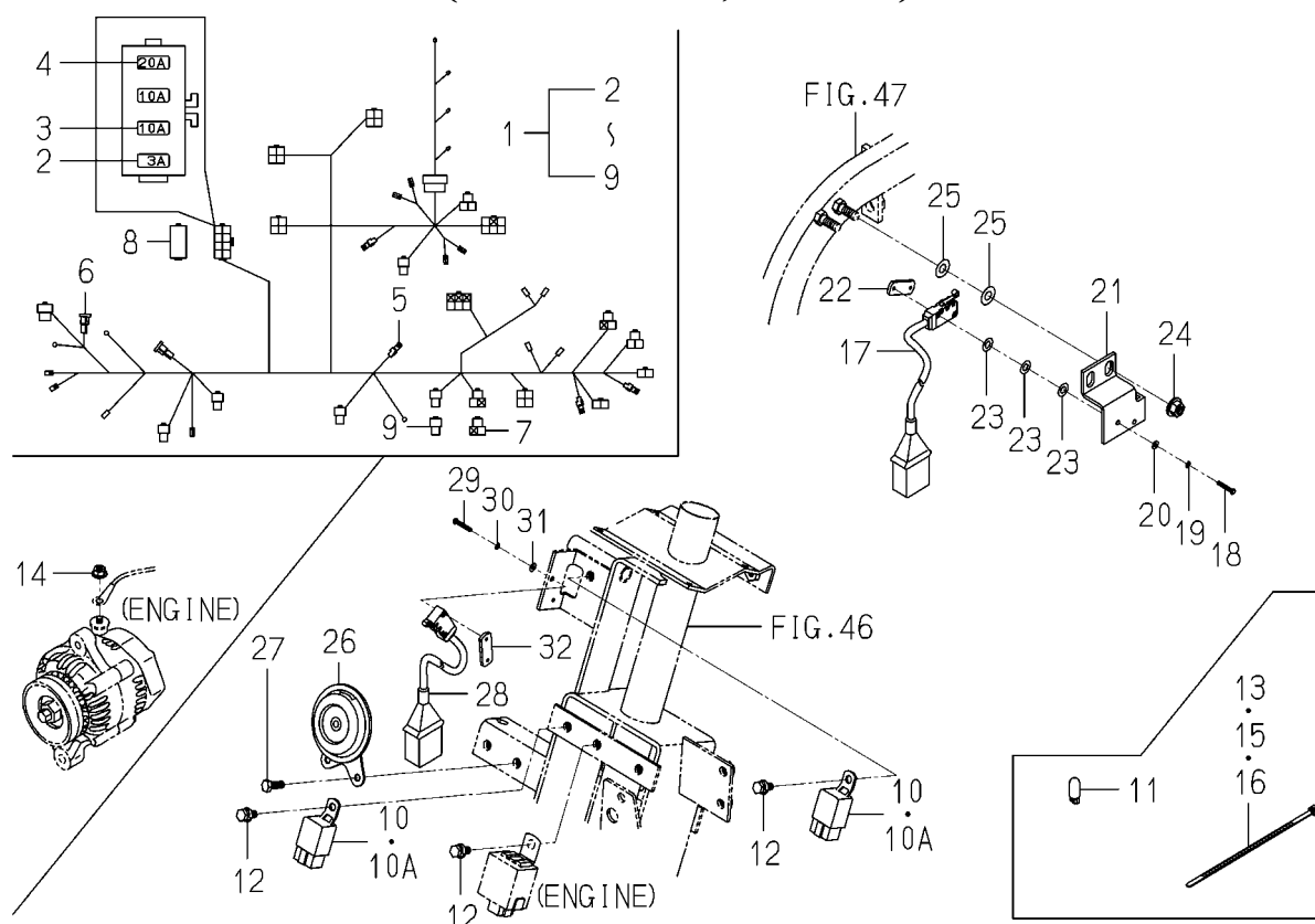
FIG. 64 WIRE HARNESS SYSTEM (EXCEPT H3,P TYPE)
