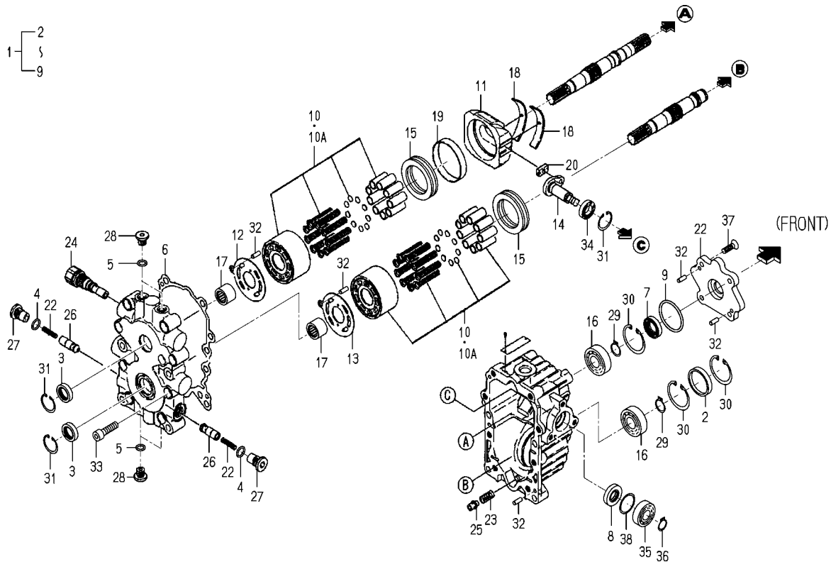
FIG. 79 COMPONENT PARTS FOR 1705-202-210-00 ON Fig.19,20
