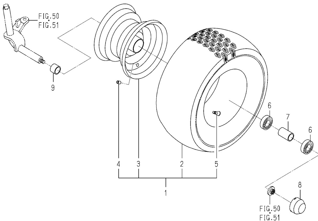
FIG. 52 FRONT WHEEL SYSTEM
