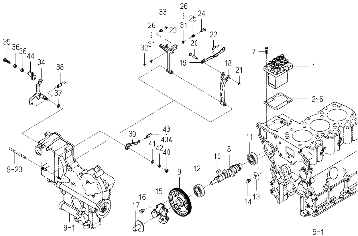
FIG. 20 INJECTION PUMP
