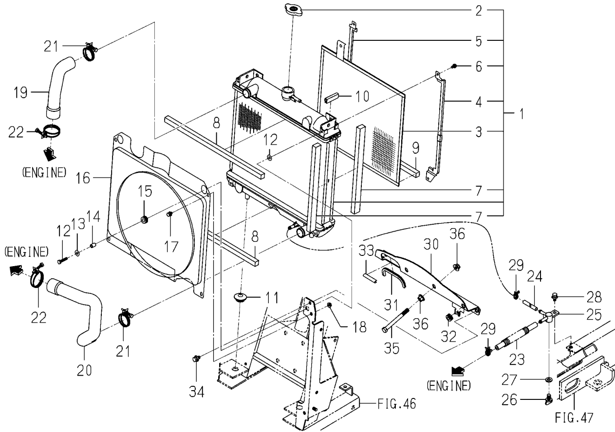
FIG. 5 RADIATOR SYSTEM (SGR22)(1/2)
