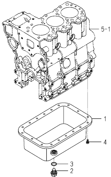
FIG. 7 OIL PAN
