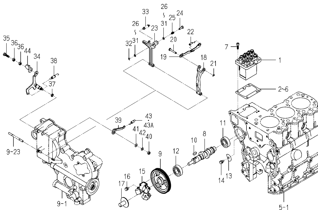
FIG. 20 INJECTION PUMP
