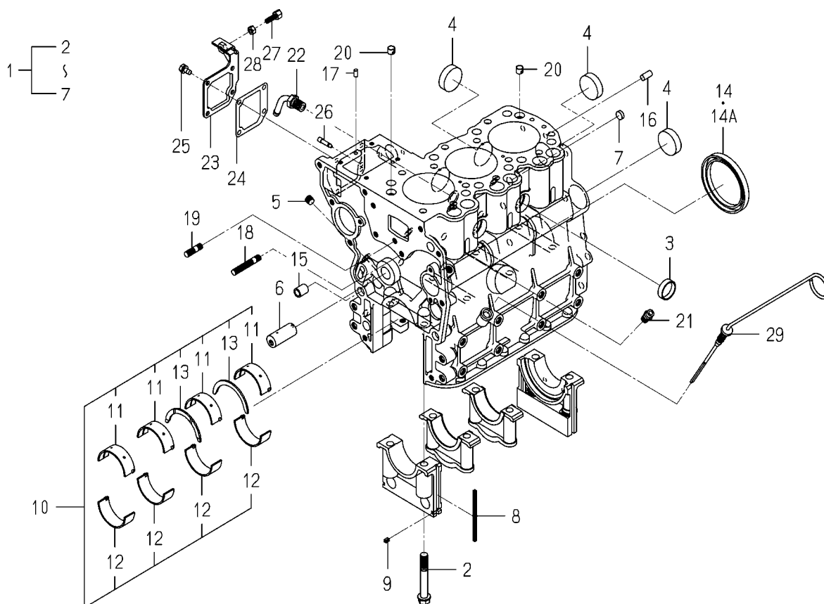
FIG. 5 CYLINDER BLOCK
