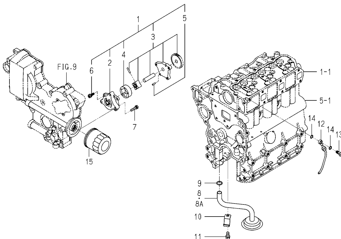
FIG. 16 OIL PUMP
