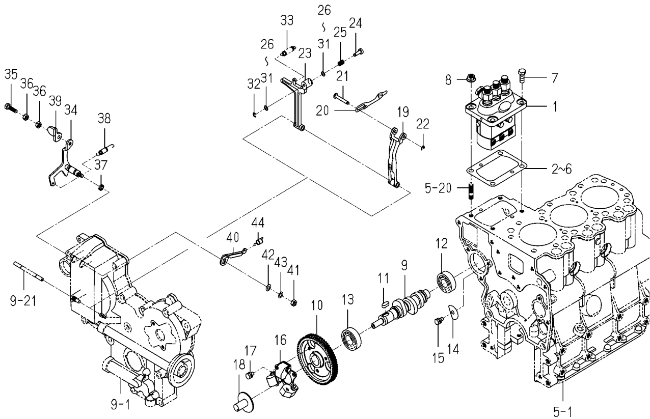
FIG. 20 INJECTION PUMP
