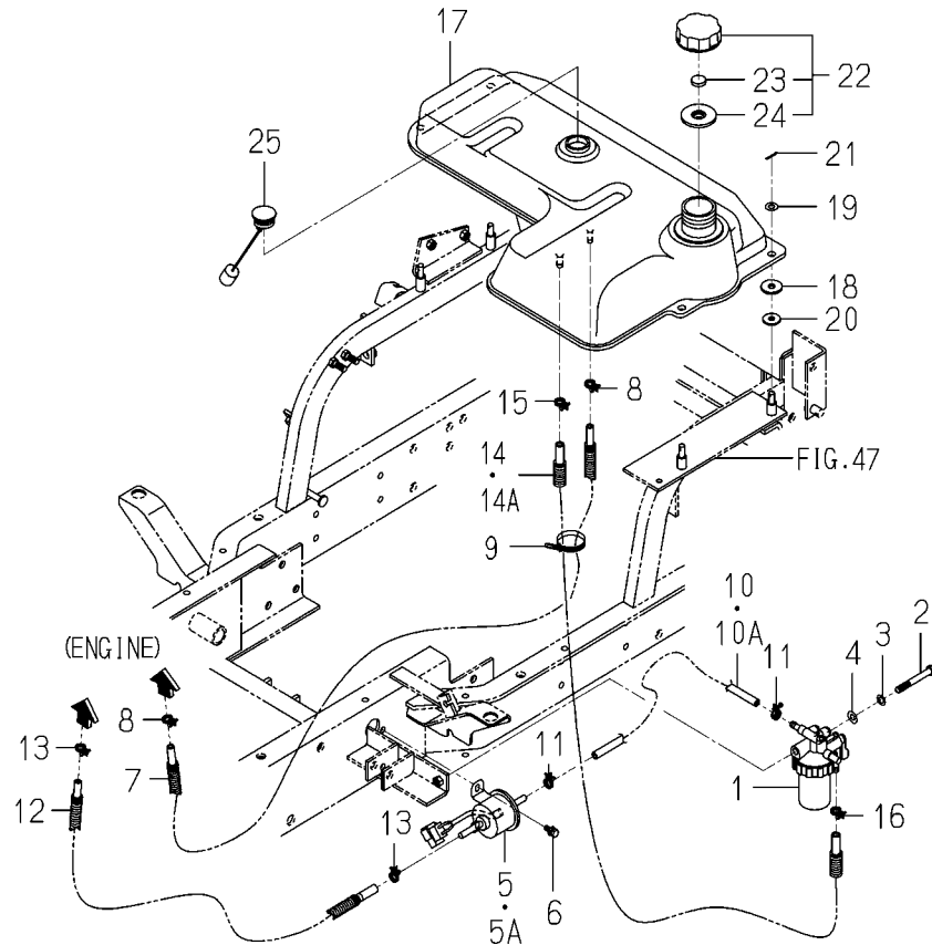
FIG. 9 FUEL FILTER (EXCEPT H3 TYPE), FUEL TANK SYSTEM
