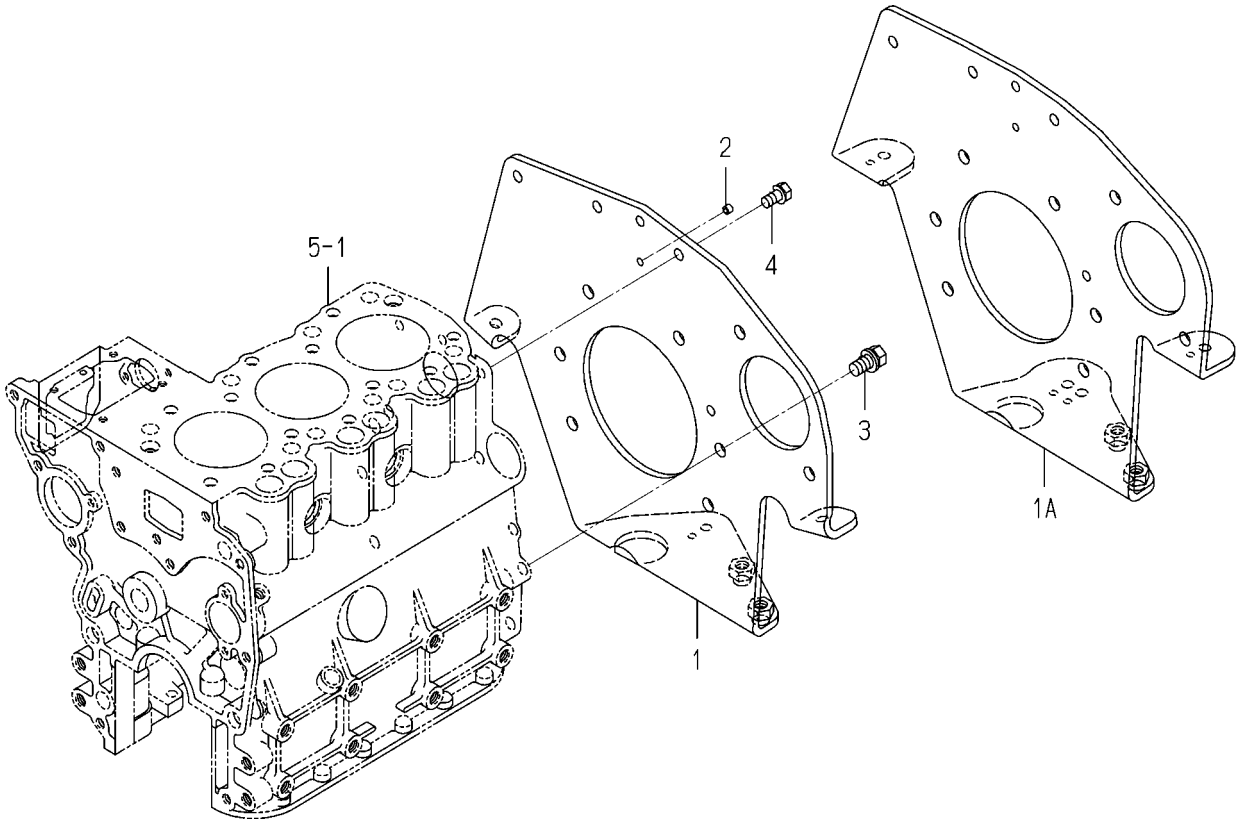
FIG. 8 REAR PLATE
