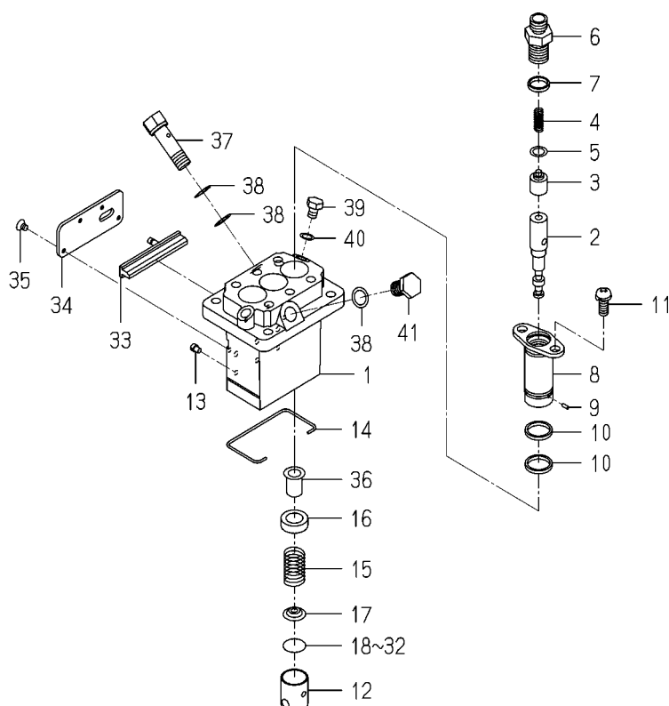
FIG. 26 COMPONENT PARTS FOR 6215-600-032-10 ON Fig.20
