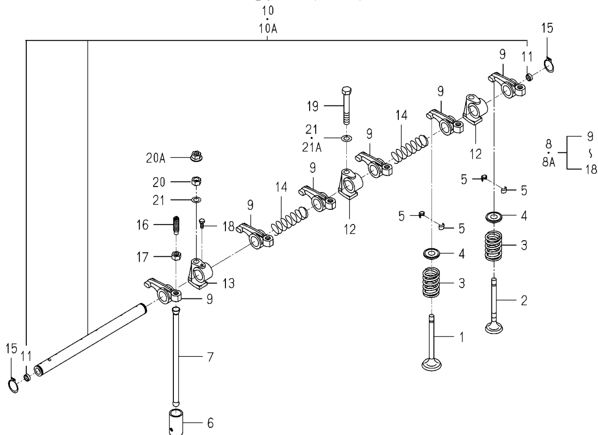
FIG. 11 VALVE
