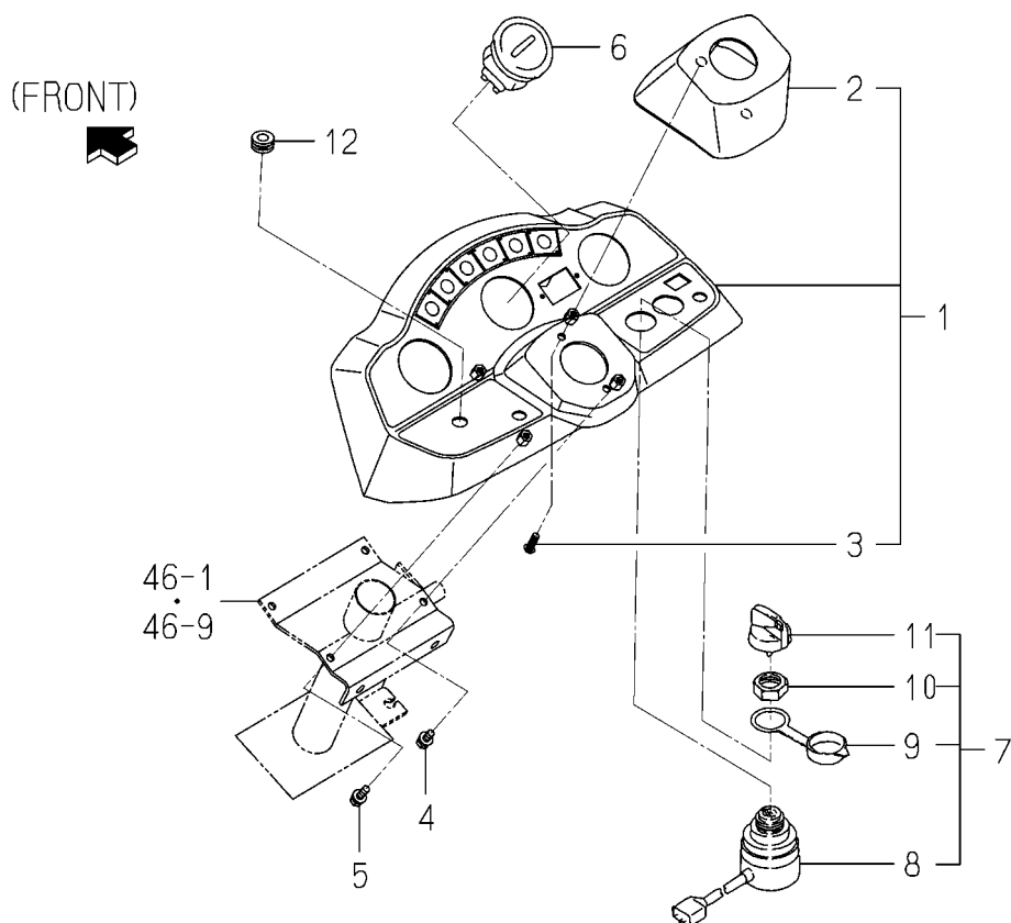
FIG. 62 PANEL SYSTEM (SGR17,19)
