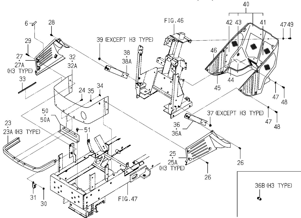
FIG. 57 HOOD SYSTEM(2/3)
