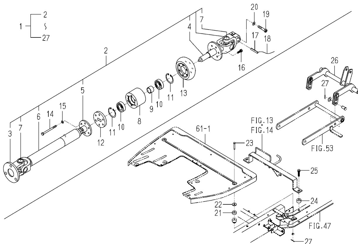
FIG. 71 PROPELLER SHAFT SYSTEM (EXCEPT H3 TYPE) (OPTION)
