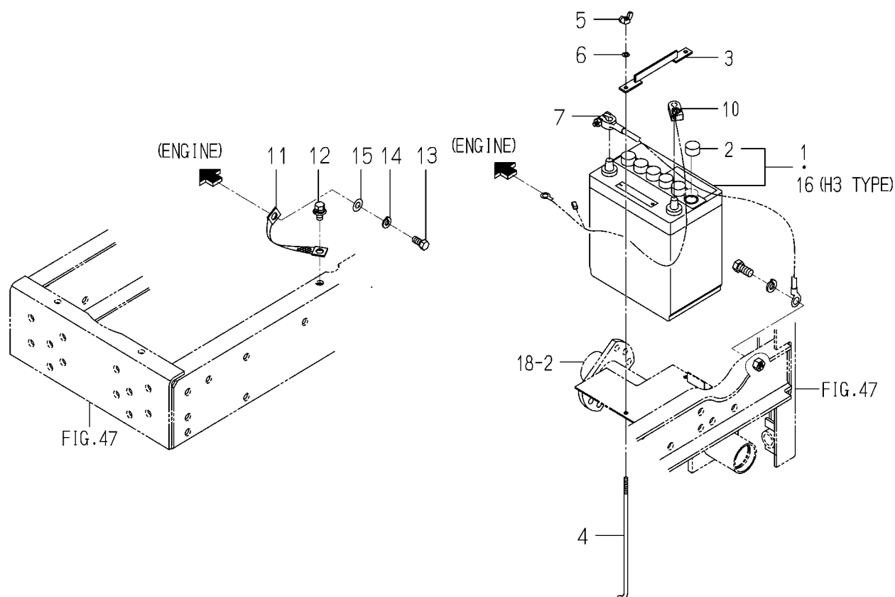
FIG. 11 BATTERY SYSTEM
