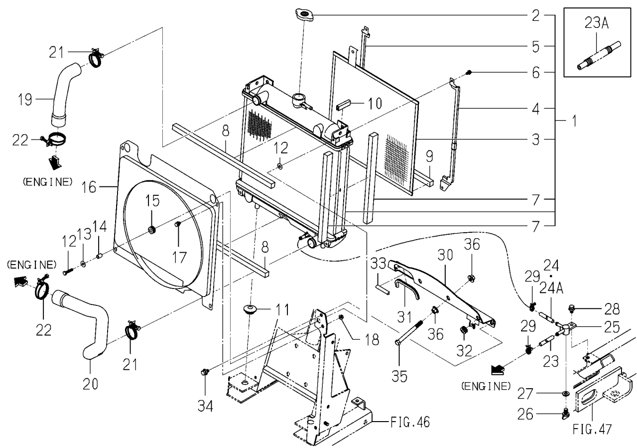
FIG. 4 RADIATOR SYSTEM (SGR17,19)(1/2)
