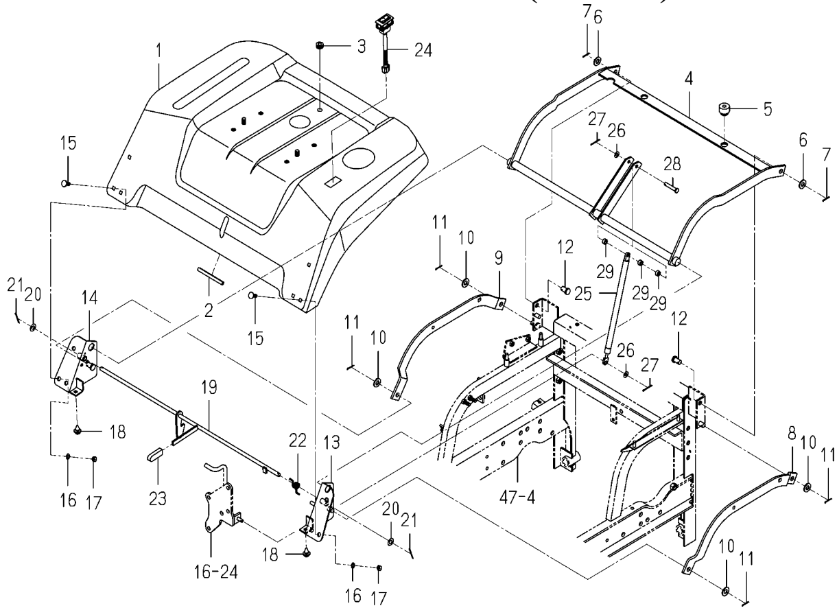
FIG. 59 FENDER SYSTEM (H3 TYPE)
