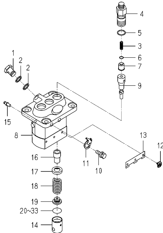
FIG. 26 COMPONENT PARTS FOR 6215-600-103-10 ON Fig.20
