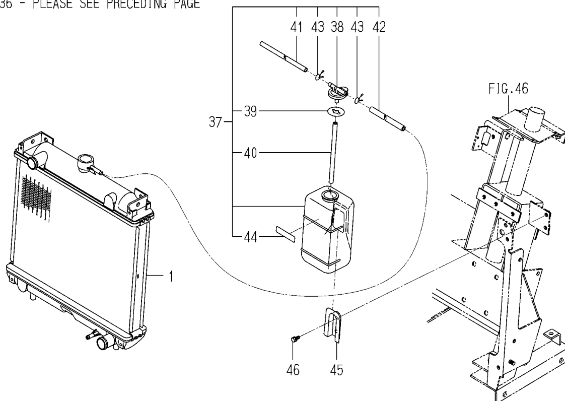
FIG. 5 RADIATOR SYSTEM (SGR22)(2/2)
