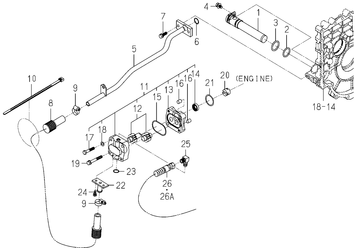
FIG. 30 PIPING SYSTEM (3) (U TYPE EXCEPT H3) (SGR17-No.1-411/SGR19-No.1-518)(1/2)
