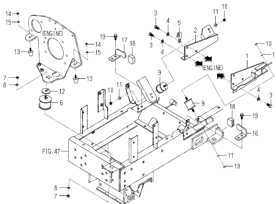
FIG. 2 ENGINE MOUNT SYSTEM (P TYPE EXCEPT H3)
