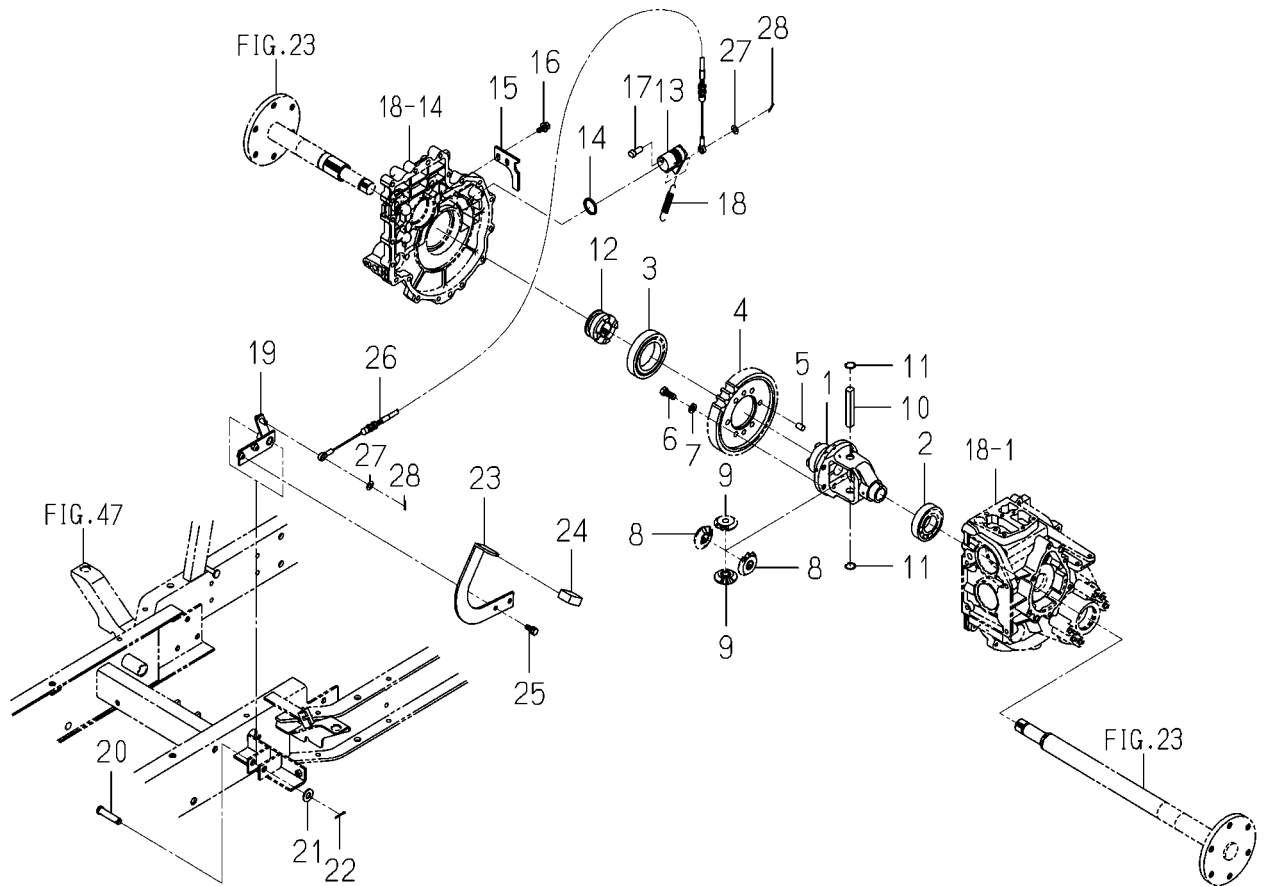
FIG. 22 DIFFERENTIAL GEAR SYSTEM
