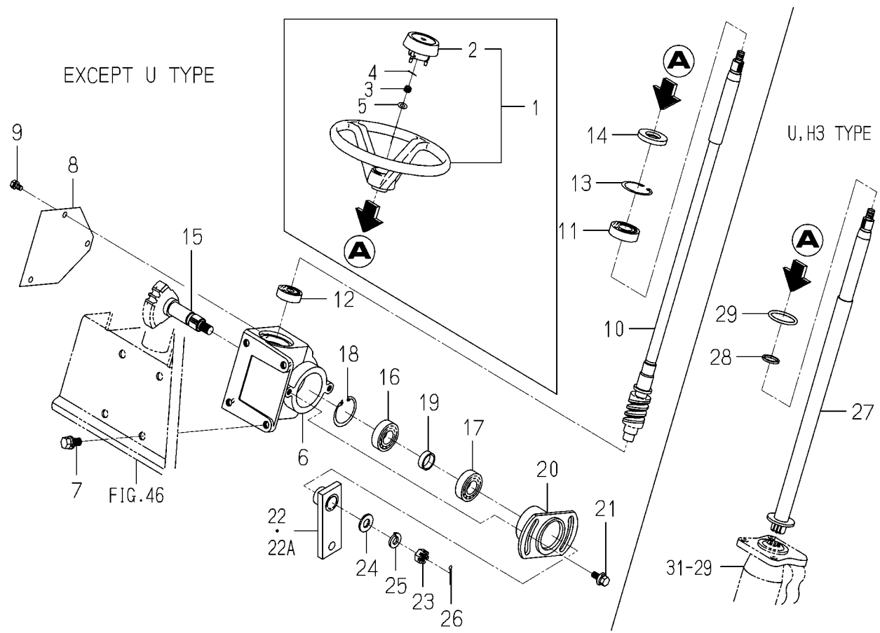
FIG. 45 STEERING SYSTEM
