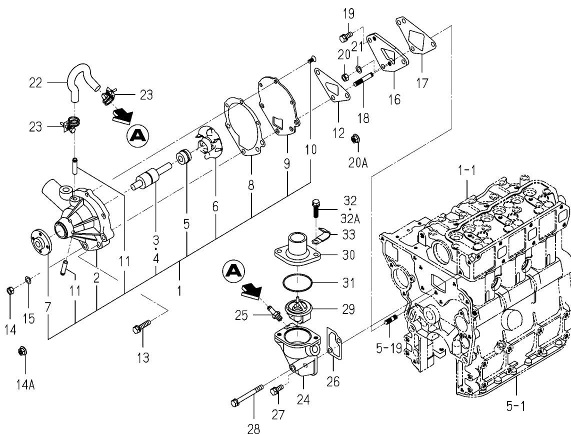
FIG. 17 WATER PUMP
