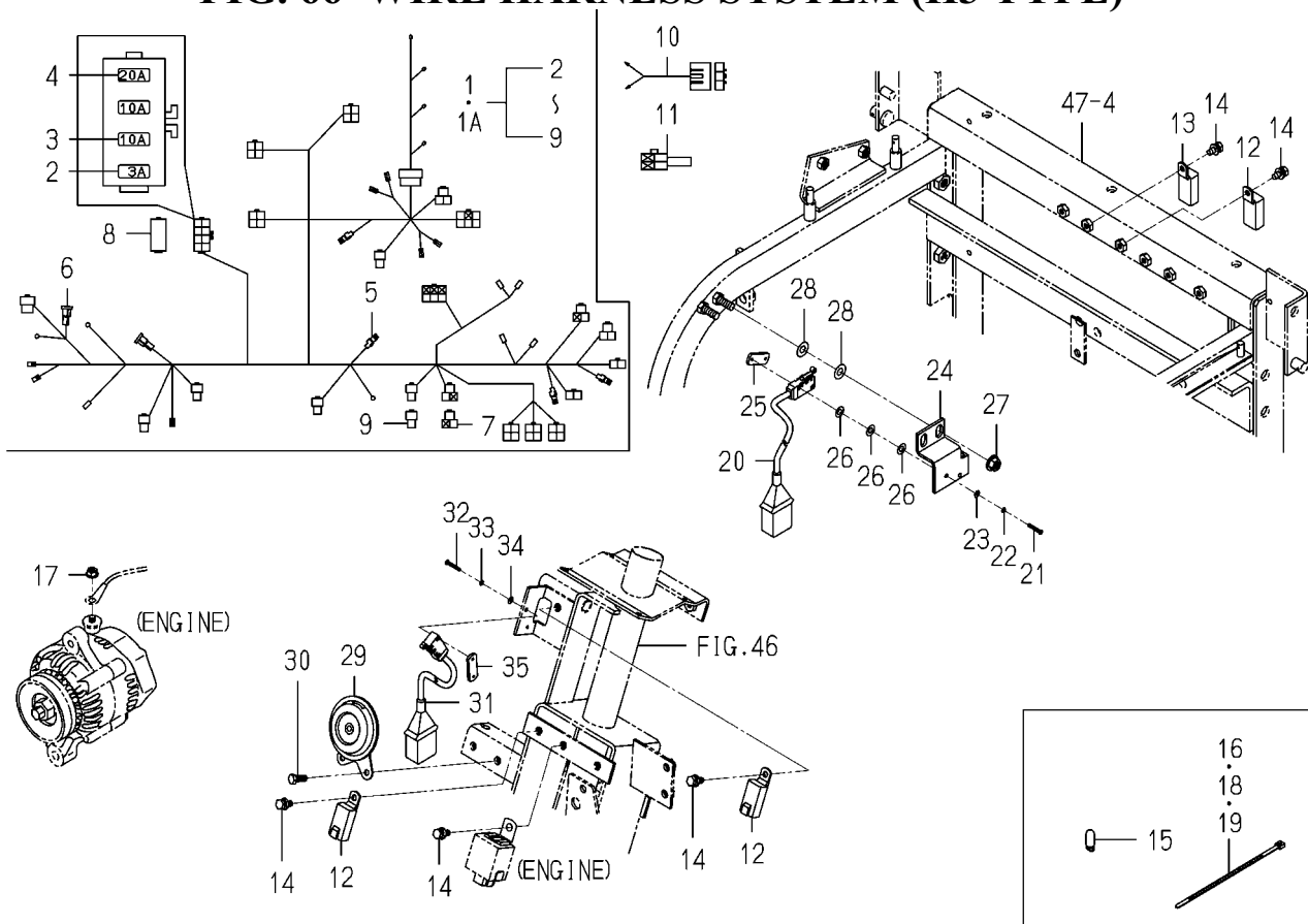
FIG. 66 WIRE HARNESS SYSTEM (H3 TYPE)
