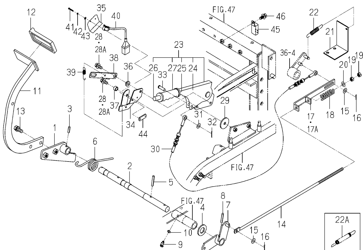
FIG. 38 PEDAL (BRAKE),PARKING SYSTEM (EXCEPT H3 TYPE)
