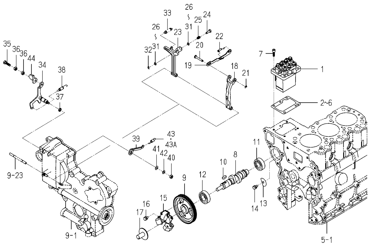
FIG. 20 INJECTION PUMP
