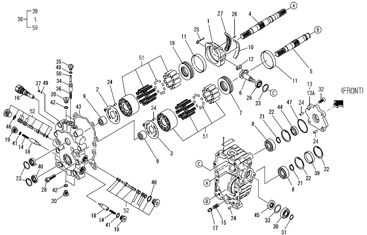
FIG. 80 COMPONENT PARTS FOR 1705-202-510-00,10 ON Fig.19,20
