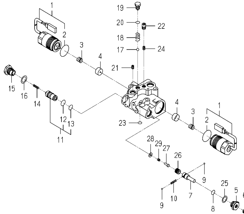
FIG. 77 COMPONENT PARTS FOR K200-078-000-00 ON Fig.34,35
