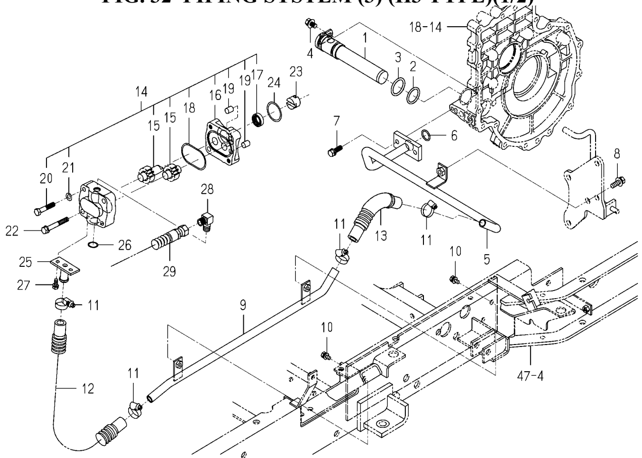
FIG. 32 PIPING SYSTEM (3) (H3 TYPE)(1/2)
