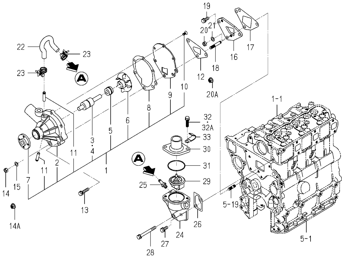
FIG. 17 WATER PUMP
