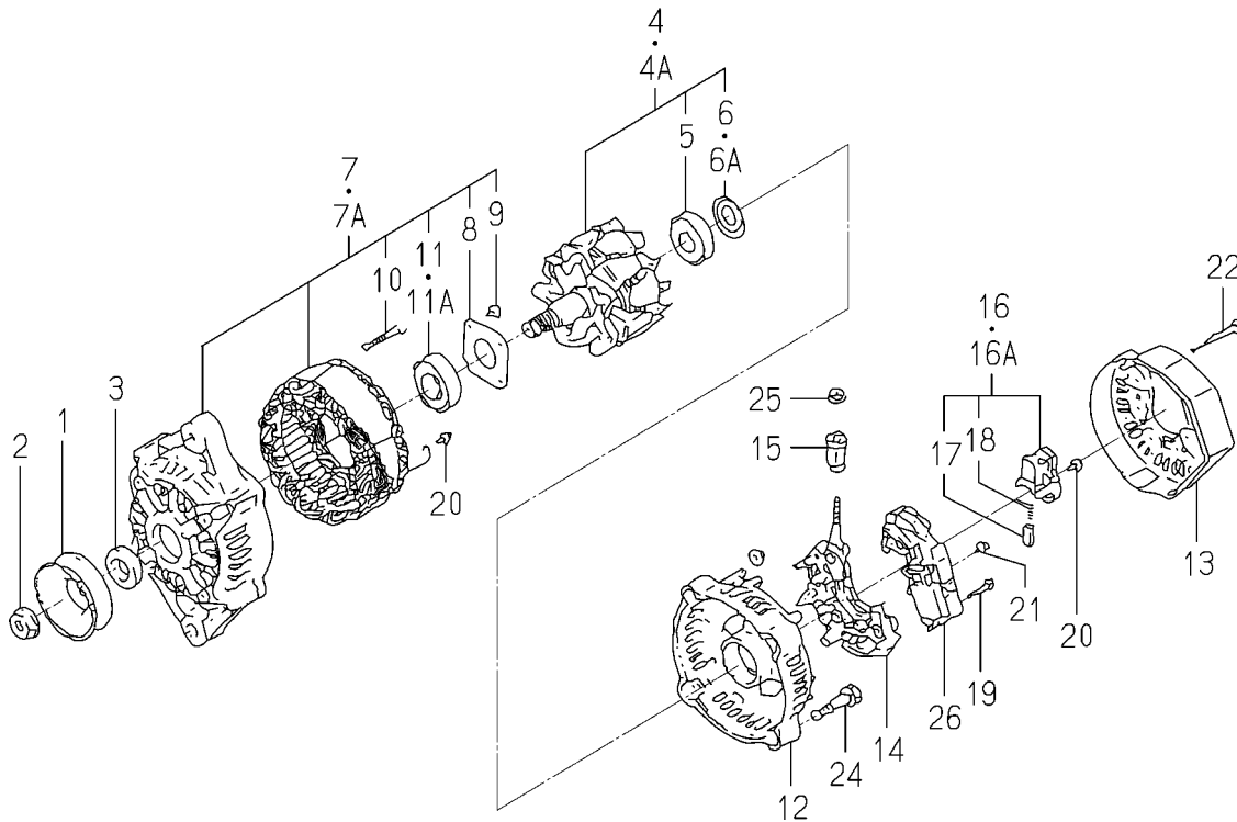
FIG. 29 COMPONENT PARTS FOR 6281-200-008-10 ON Fig.22
