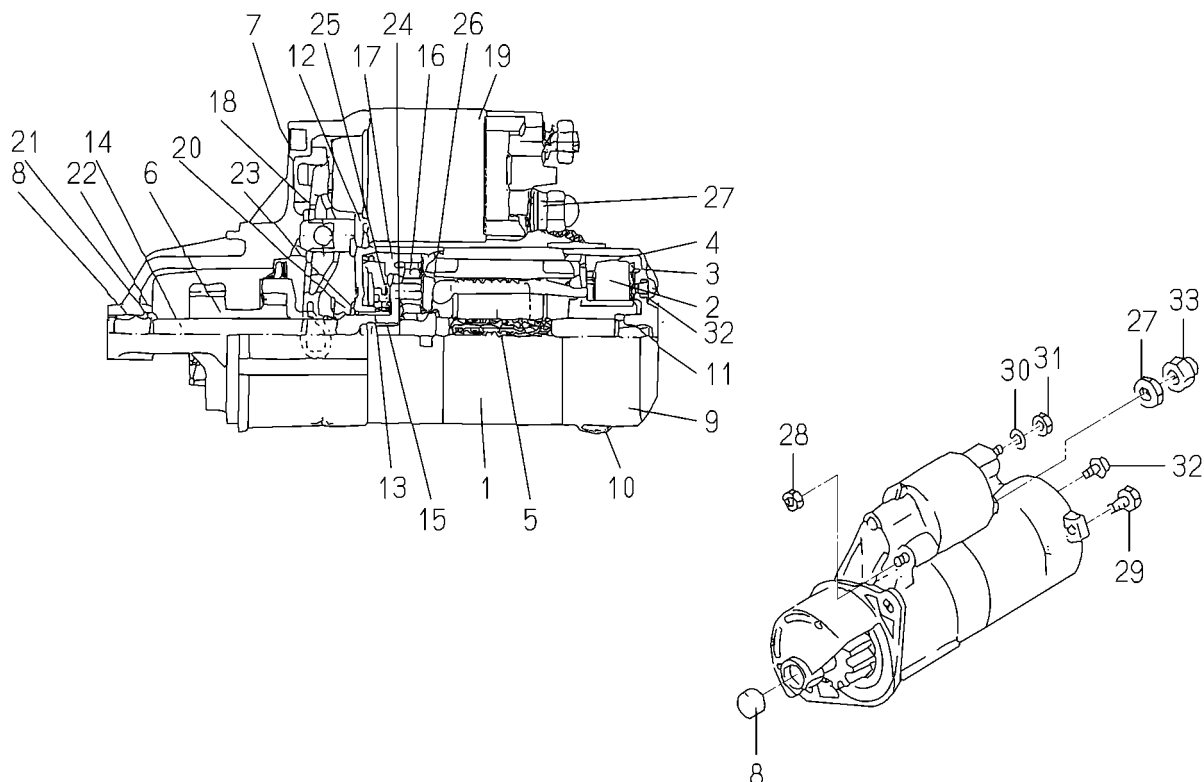
FIG. 27 COMPONENT PARTS FOR 6281-100-014-00 ON Fig.22
