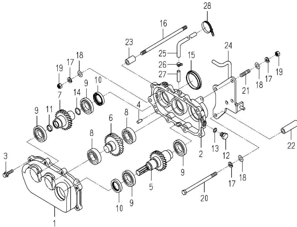
FIG. 16 CASE (INPUT) SYSTEM (H3 TYPE)
