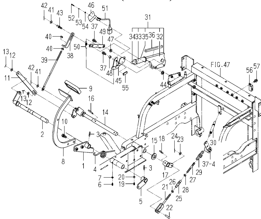
FIG. 39 PEDAL (BRAKE),PARKING SYSTEM (H3 TYPE)
