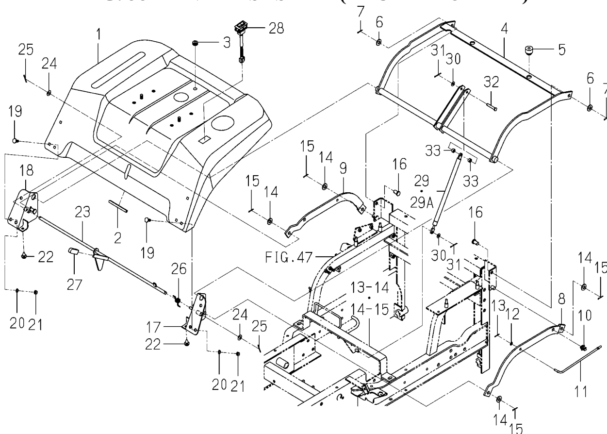
FIG. 58 FENDER SYSTEM (EXCEPT H3 TYPE)
