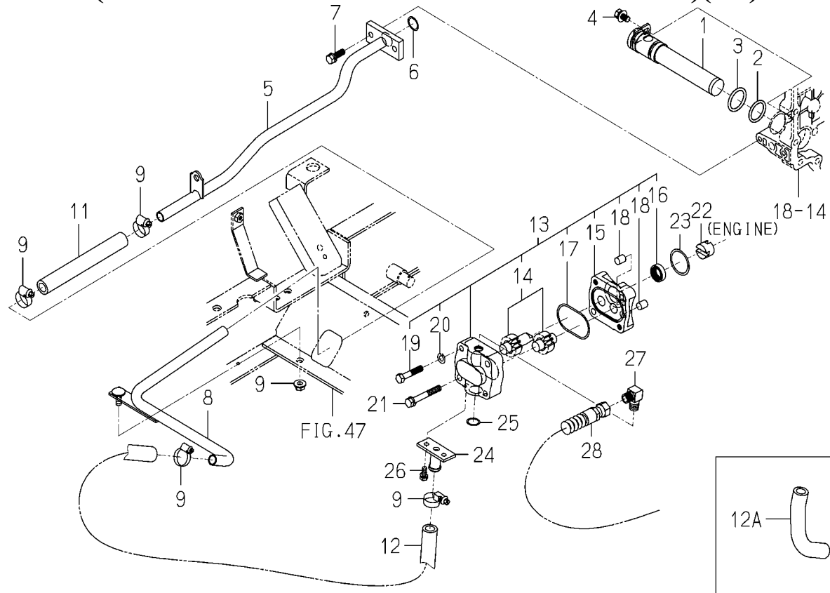
FIG. 31 PIPING SYSTEM (3) (U TYPE EXCEPT H3) (SGR17-No.412-/SGR19-No.519-/SGR22-No.1-)(1/2)
