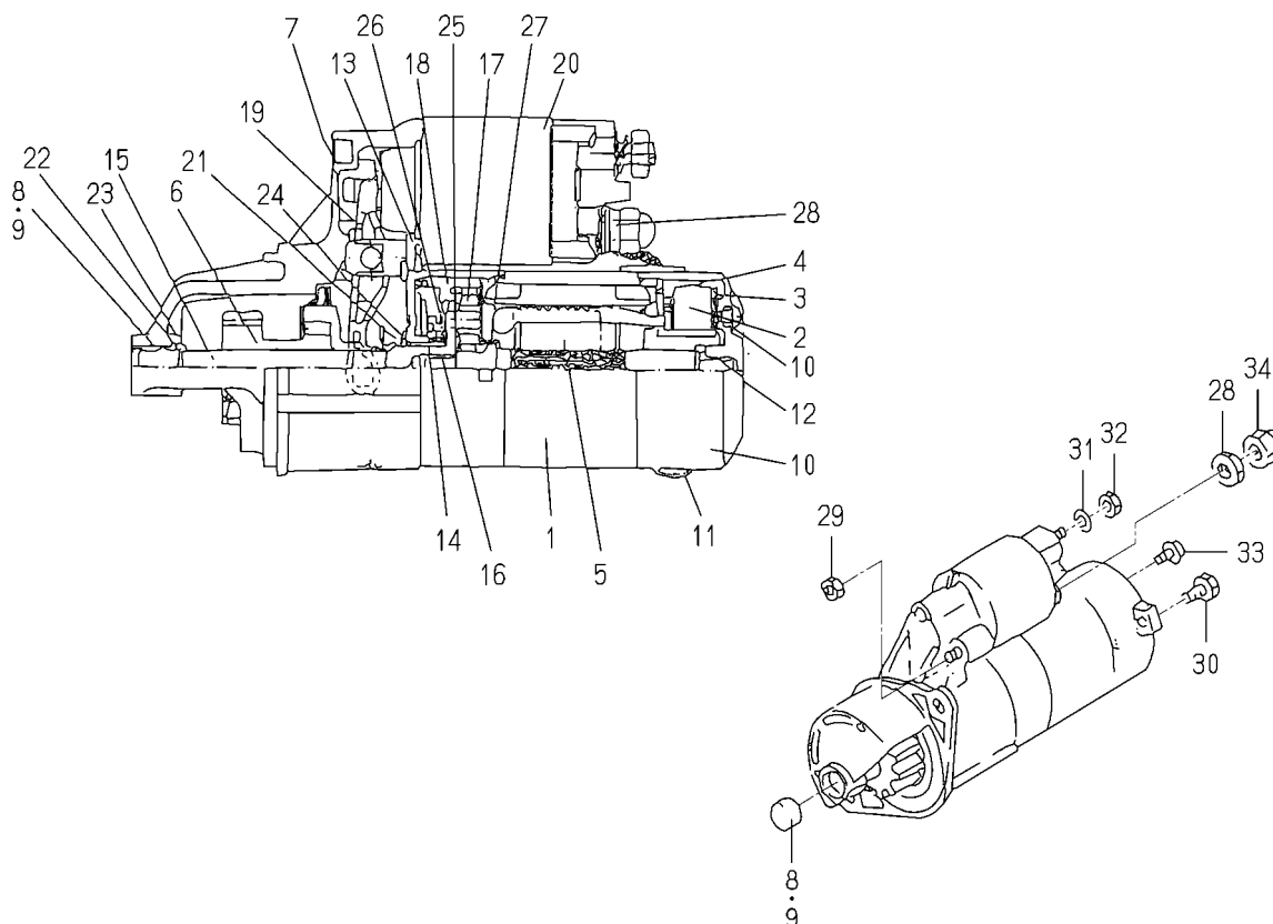
FIG. 27 COMPONENT PARTS FOR 6281-100-014-00 ON Fig.22
