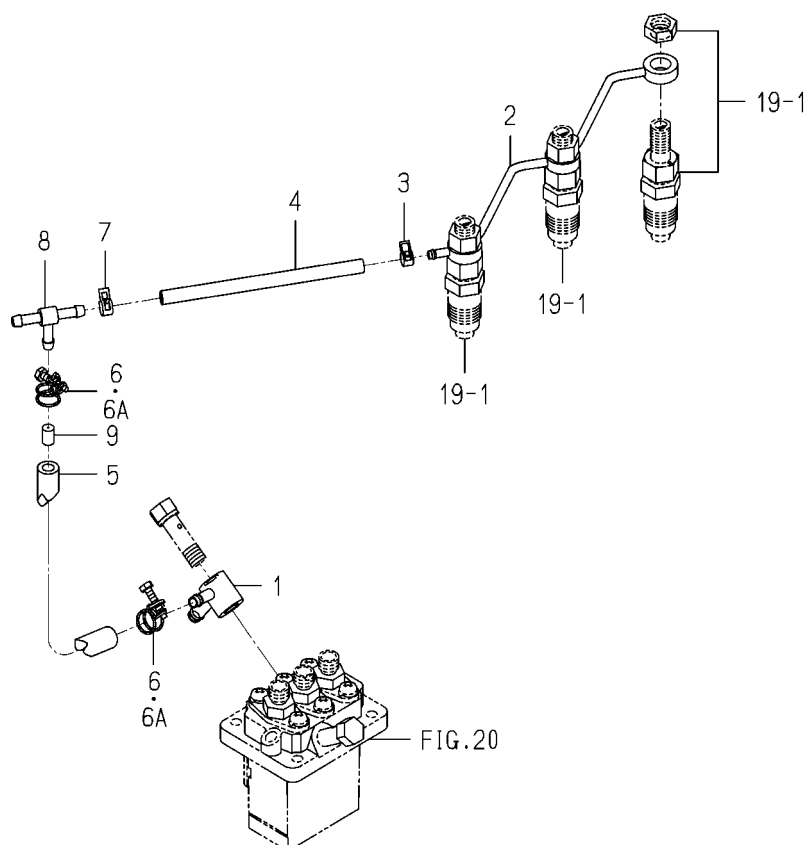
FIG. 21 FUEL PIPE
