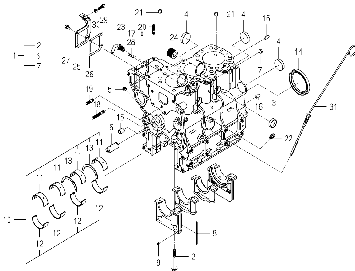
FIG. 5 CYLINDER BLOCK
