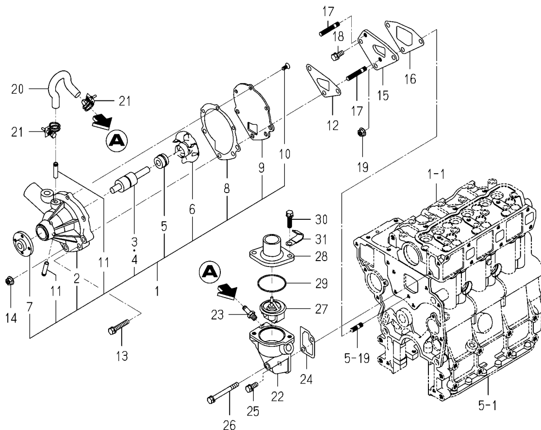
FIG. 17 WATER PUMP
