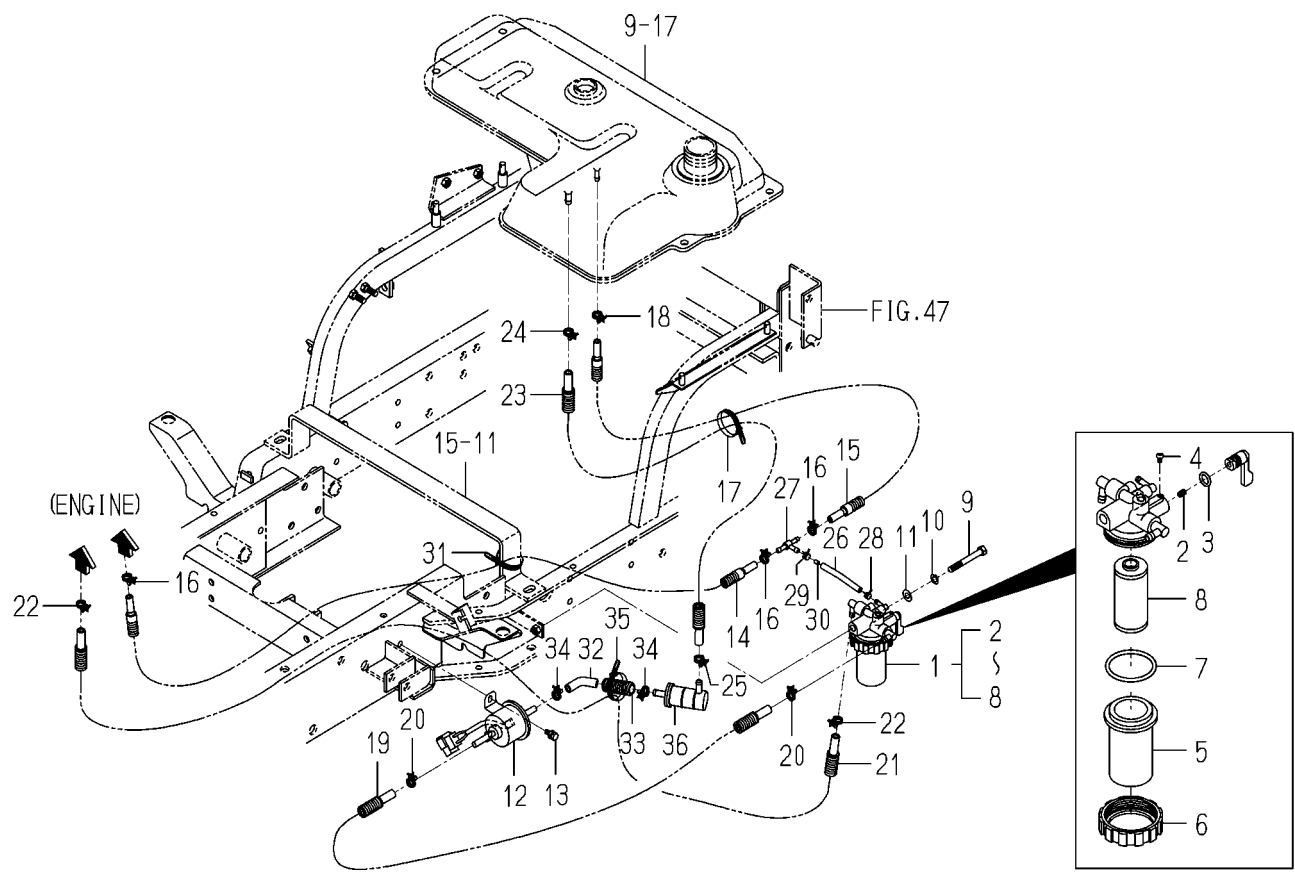
FIG. 10 FUEL FILTER SYSTEM (H3 TYPE)
