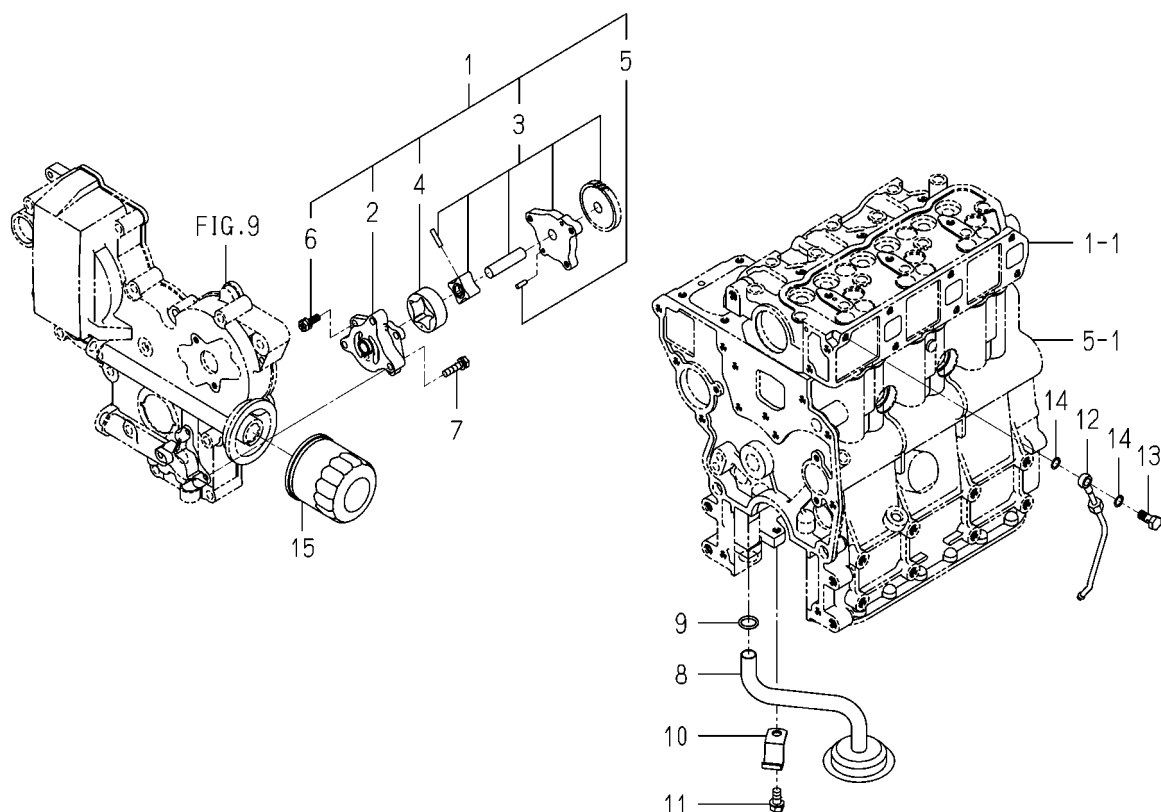
FIG. 16 OIL PUMP
