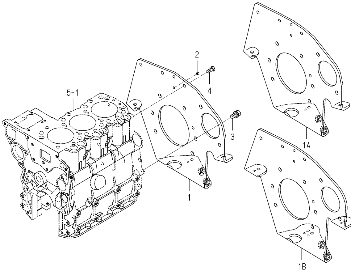
FIG. 8 REAR PLATE
