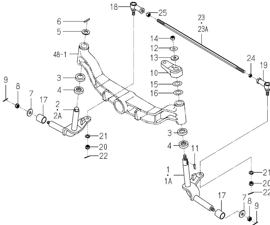
FIG. 51 KNUCKLE SPINDLE SYSTEM (H3,U TYPE)
