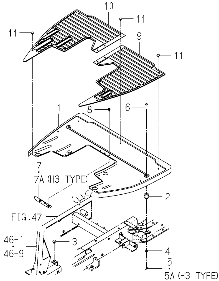
FIG. 61 STEP SYSTEM
