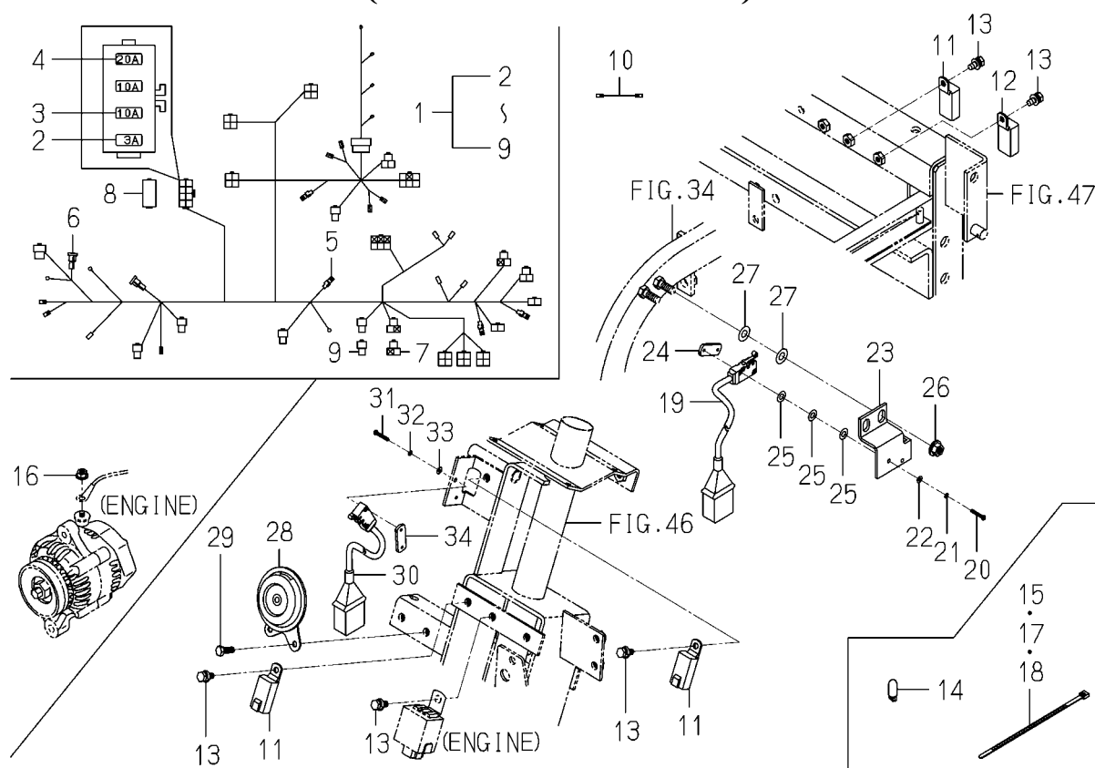
FIG. 65 WIRE HARNESS SYSTEM (P TYPE EXCEPT H3)
