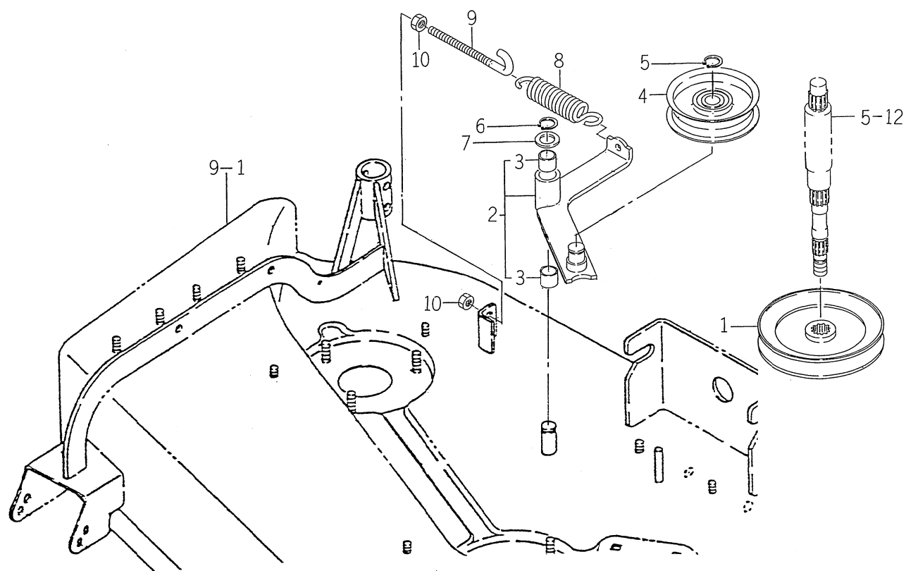
FIG. 7 PULLEY SYSTEM
