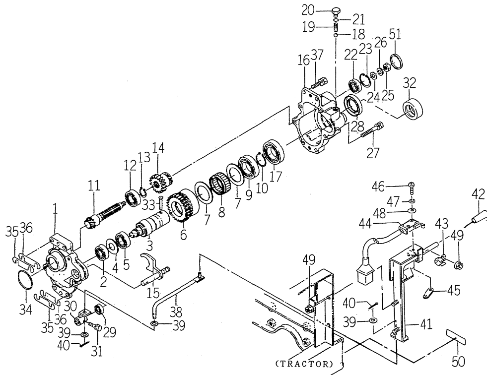
FIG. 11 PTO (REAR) SET (EXCEPT 1, E TYPE) (OPTION)
