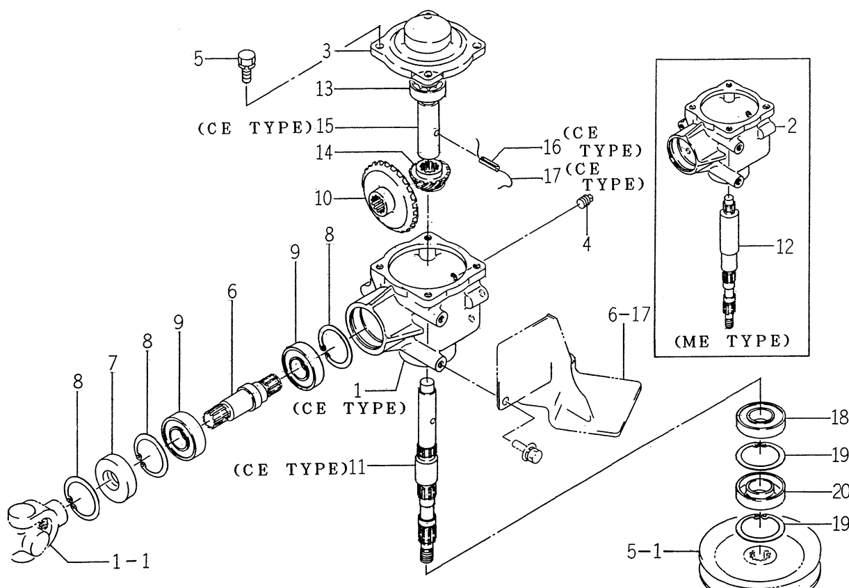
FIG. 4 CASE (BEVEL) SYSTEM (U TYPE)
