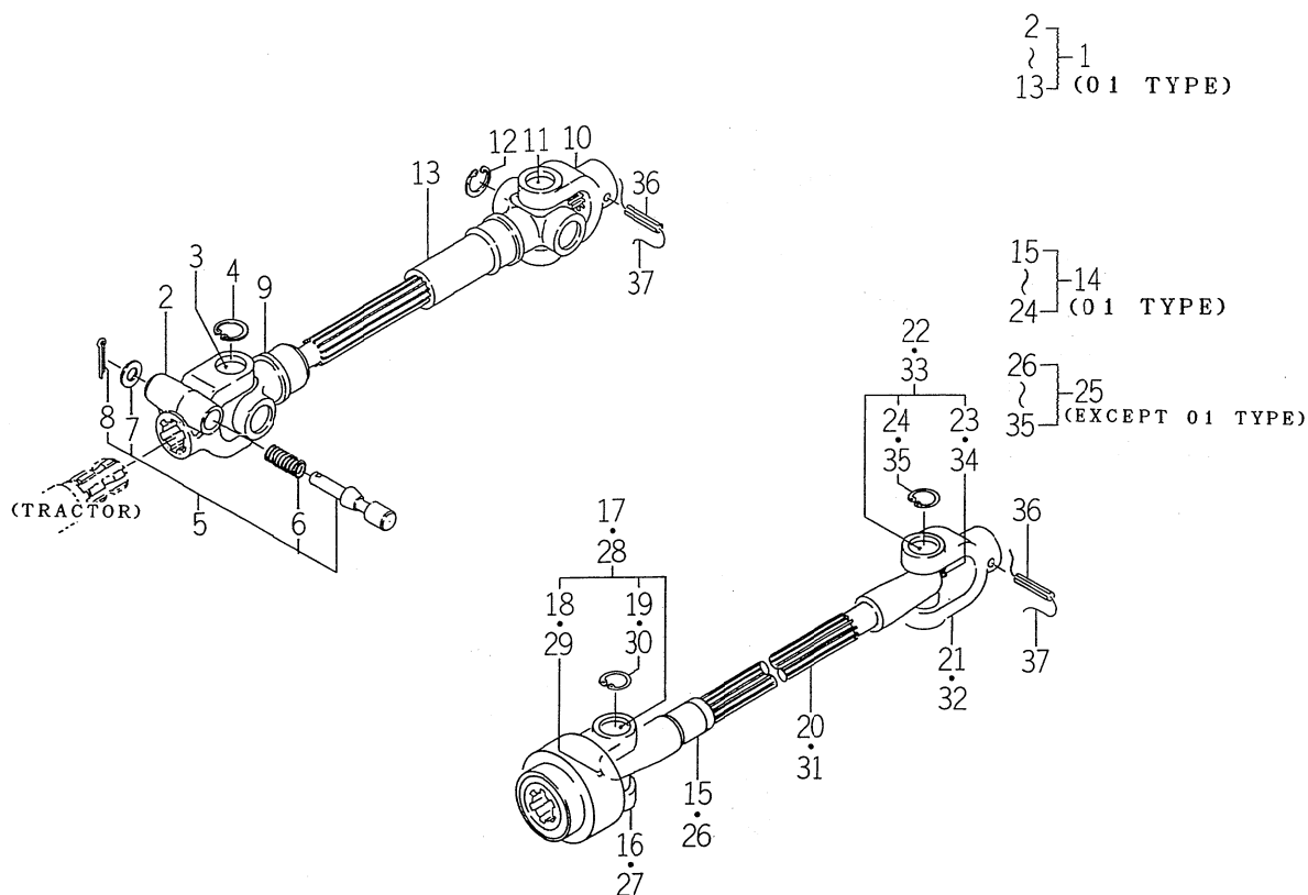
FIG. 2 JOINT (UNIVERSAL) SYSTEM (EXCEPT U TYPE)
