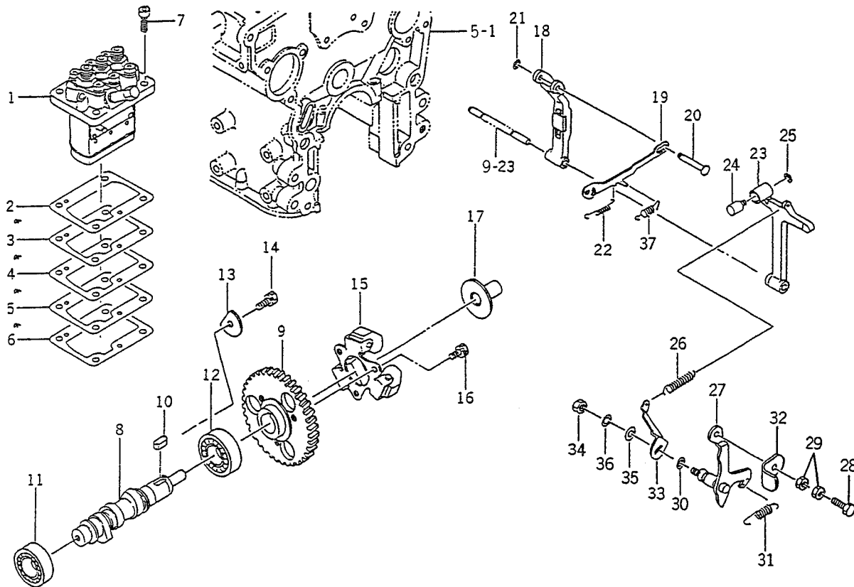
FIG. 20 INJECTION PUMP
