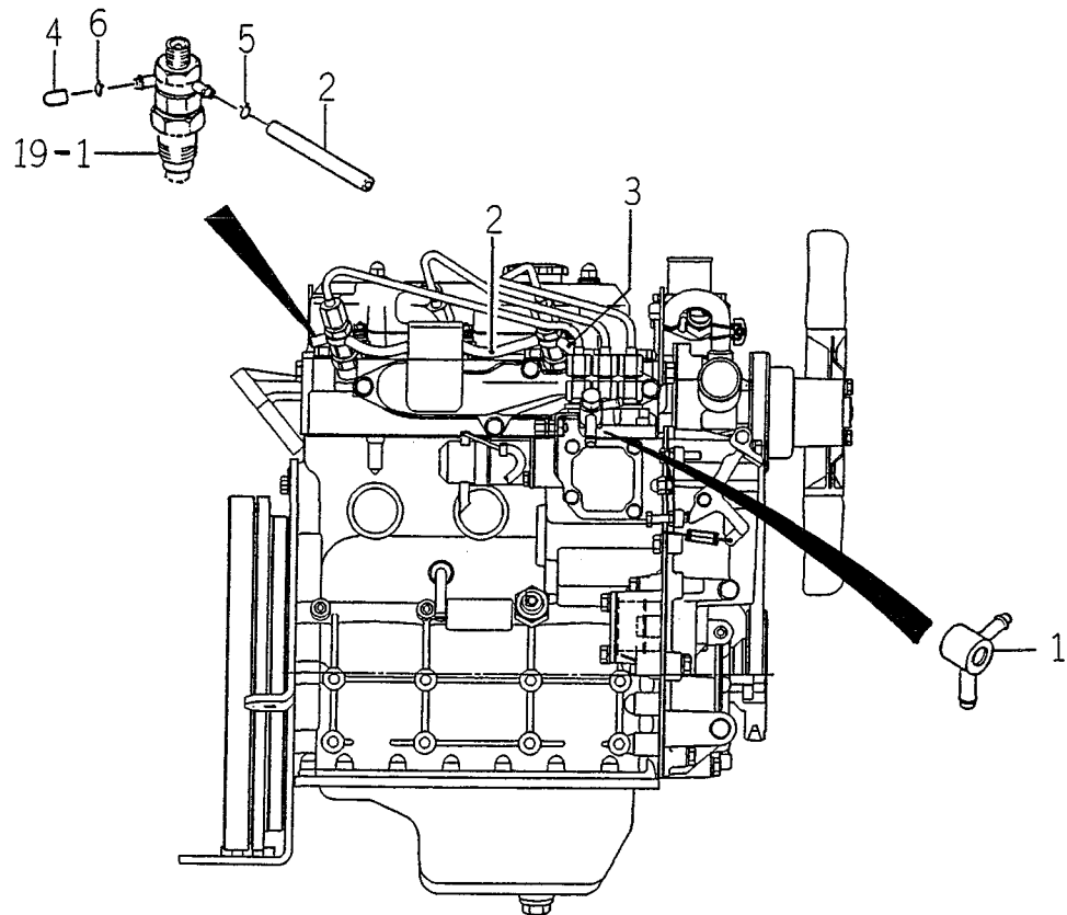
FIG. 21 FUEL PIPE
