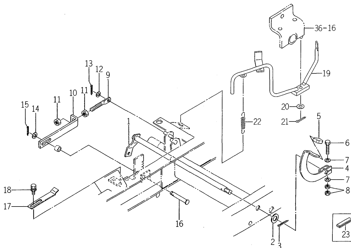
FIG. 17 HST SYSTEM (6)
