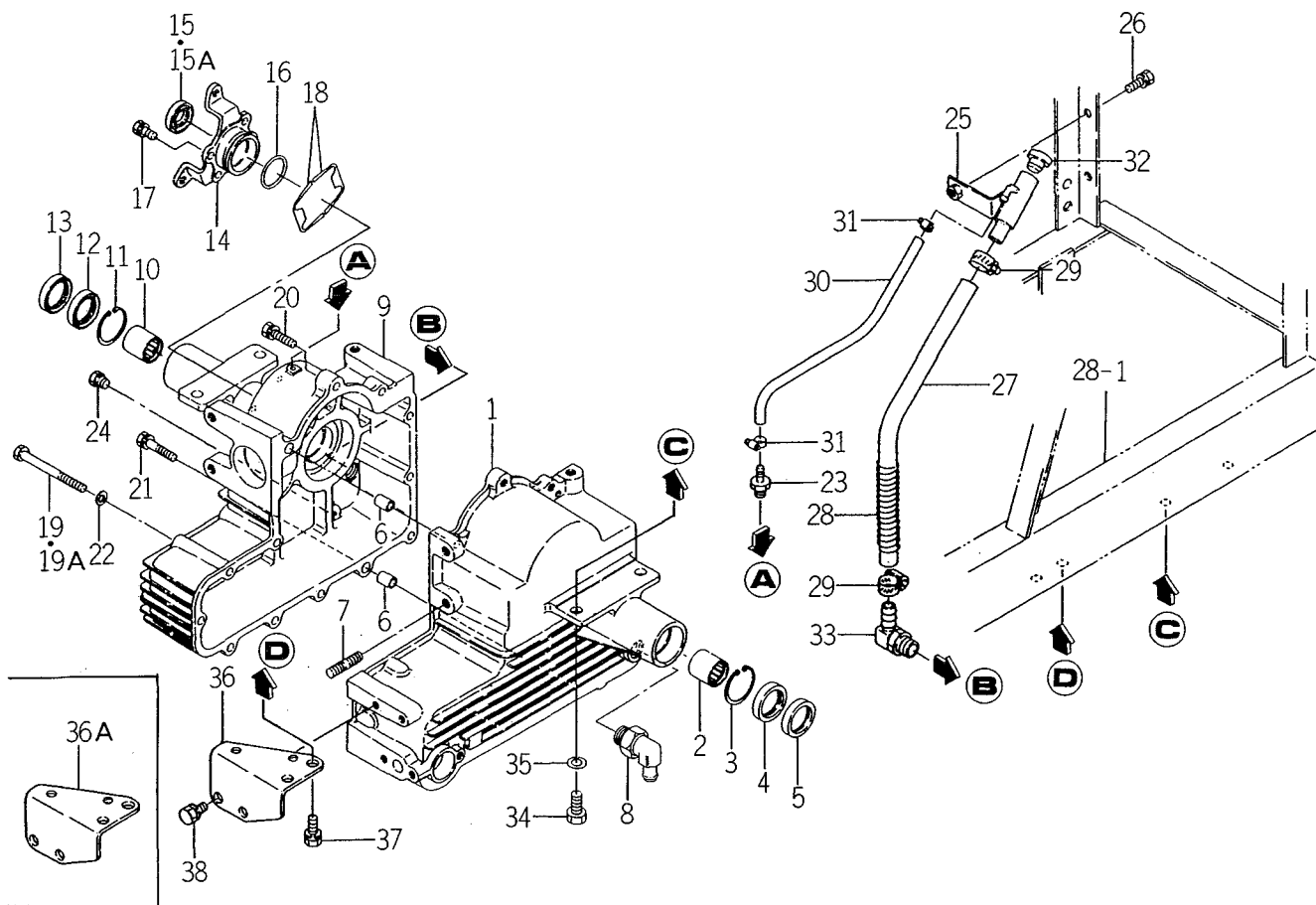
FIG. 10 TRANSMISSION SYSTEM (U TYPE)
