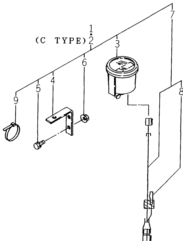
FIG. 46 MATER (HOUR) SET (OPTION)
