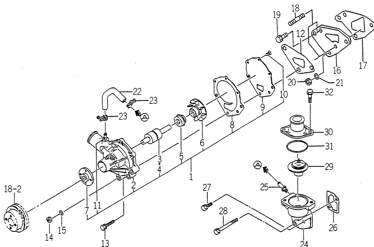
FIG. 17 WATER PUMP
