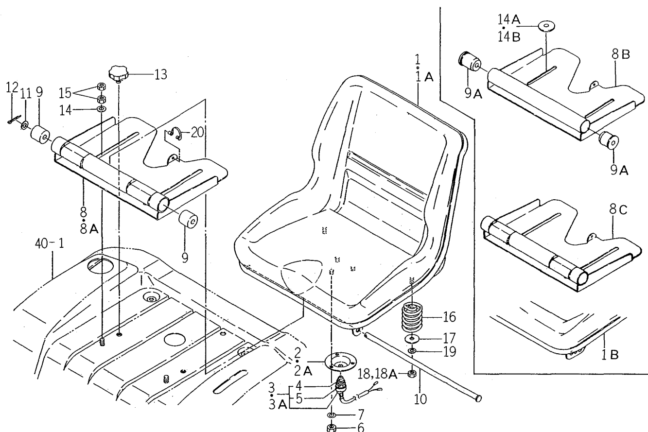
FIG. 41 SEAT SYSTEM
