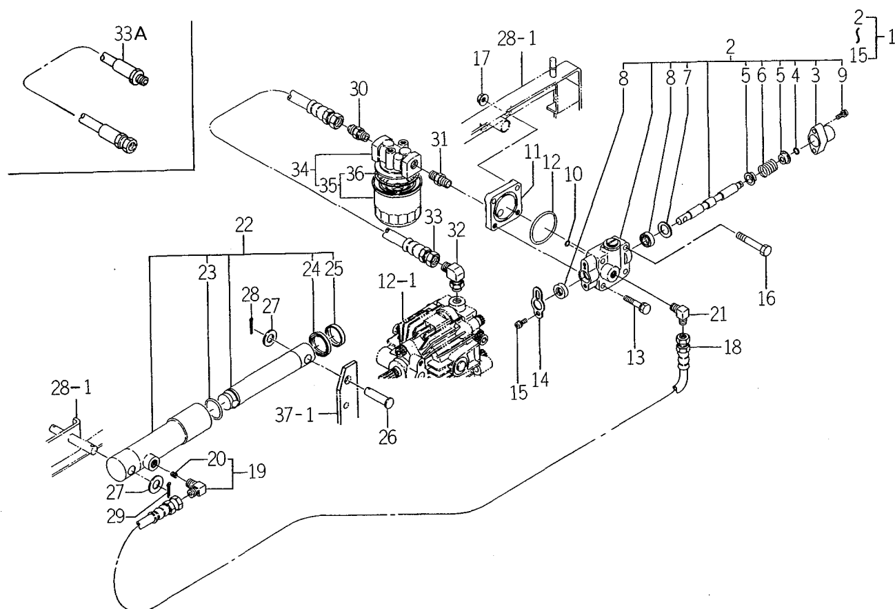
FIG. 14 HST SYSTEM (3)
