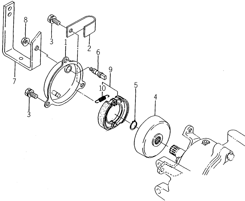
FIG. 19 BRAKE SYSTEM
