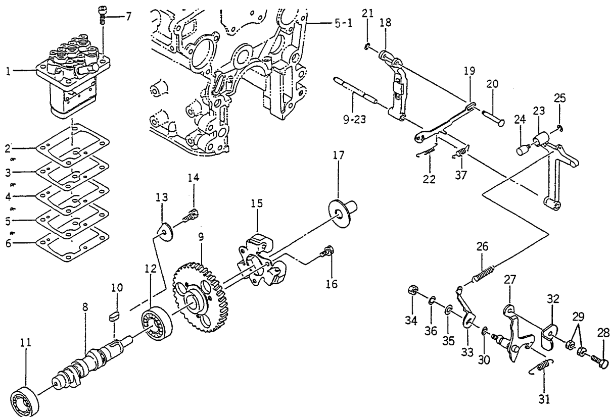
FIG. 20 INJECTION PUMP
