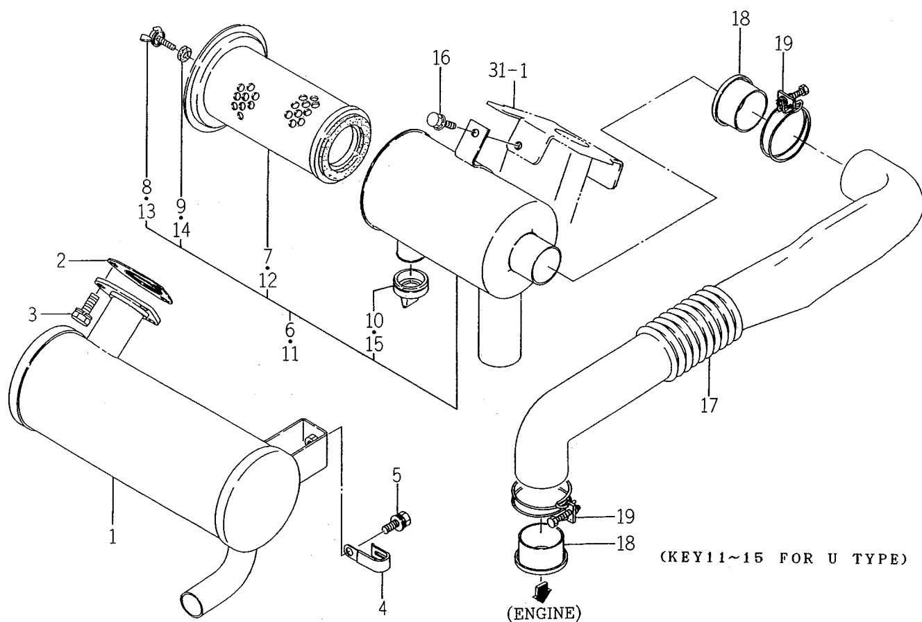
FIG. 3 MUFFLER/CLEANER (AIR) SYSTEM
