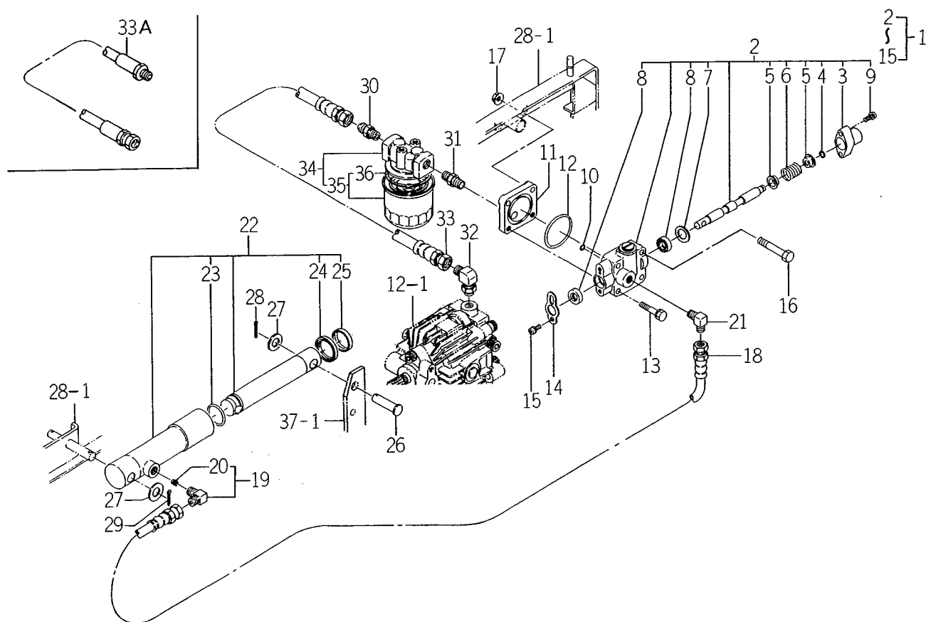
FIG. 14 HST SYSTEM (3)
