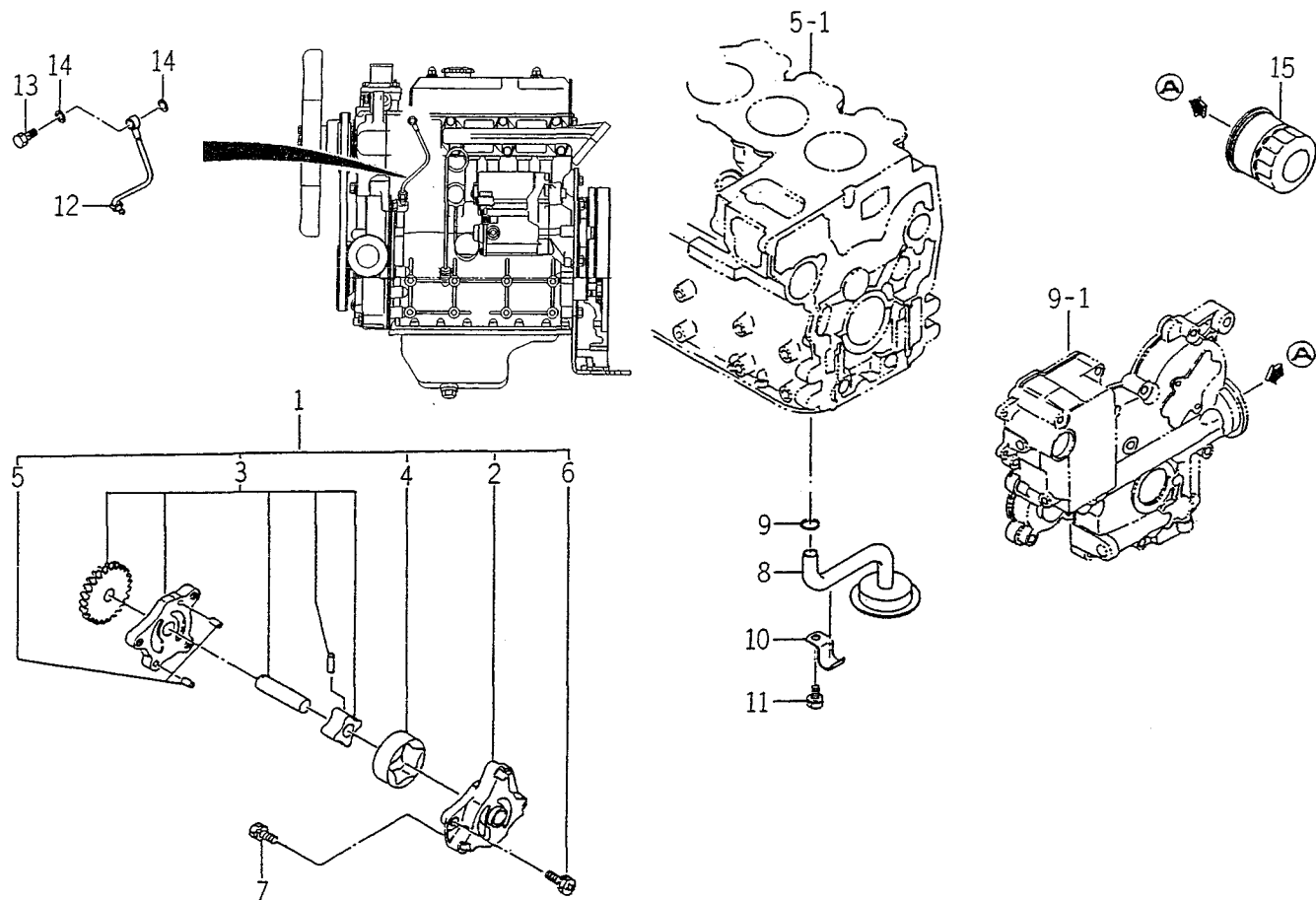
FIG. 16 OIL PUMP
