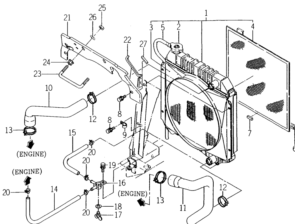
FIG. 2 RADIATOR SYSTEM
