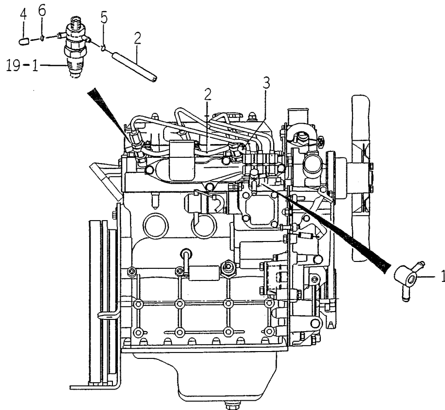
FIG. 21 FUEL PIPE
