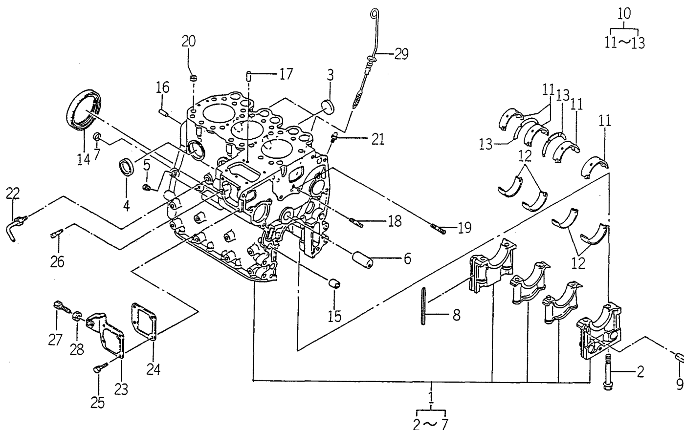
FIG. 5 CYLINDER BLOCK
