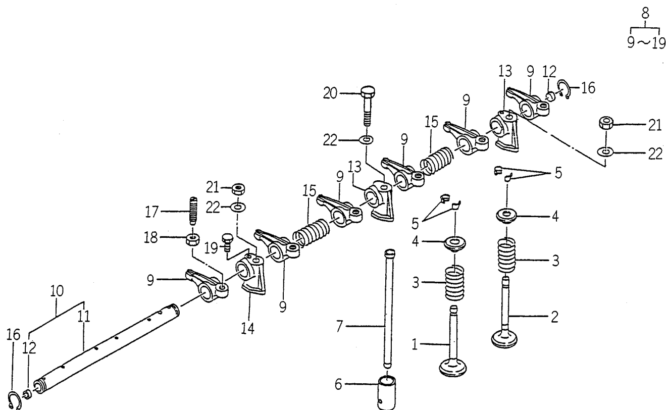
FIG. 11 VALVE
