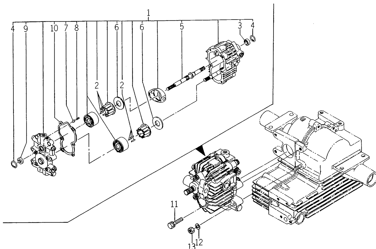
FIG. 12 HST SYSTEM (1)
