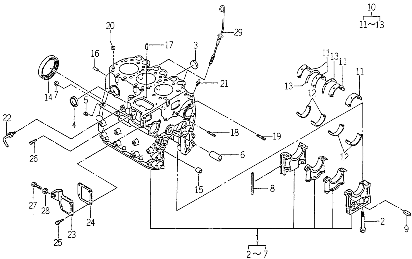
FIG. 5 CYLINDER BLOCK
