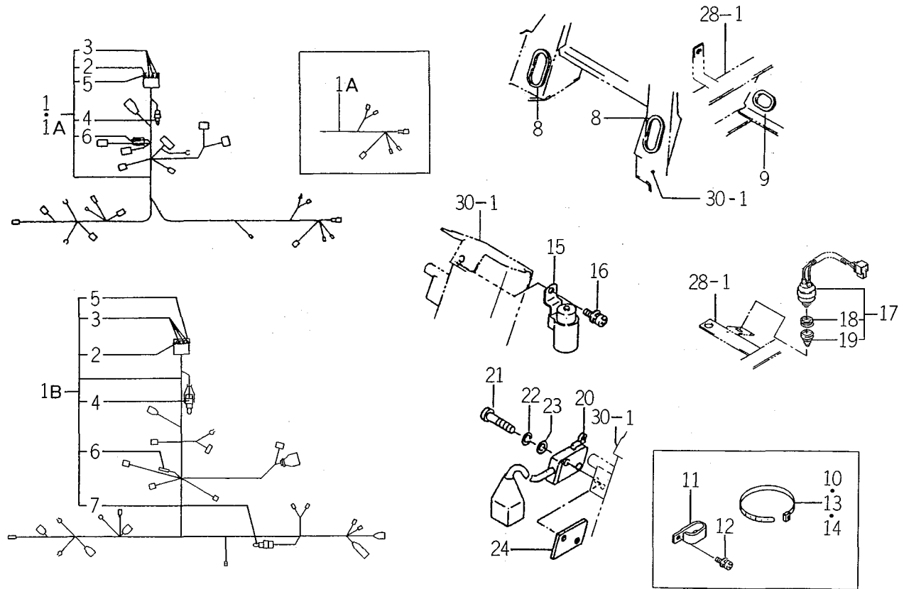
FIG. 44 ELECTRICAL SYSTEM (EXCEPT S TYPE)
