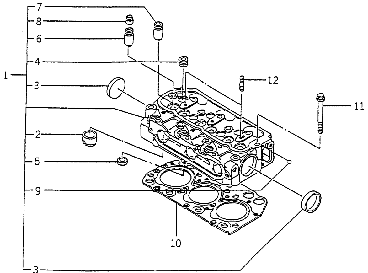
FIG. 1 CYLINDER HEAD
