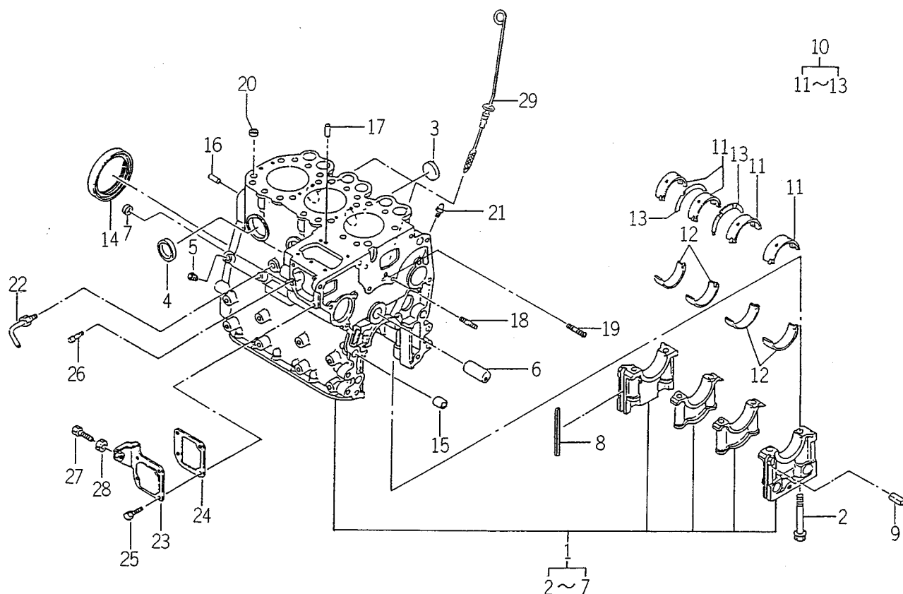
FIG. 5 CYLINDER BLOCK
