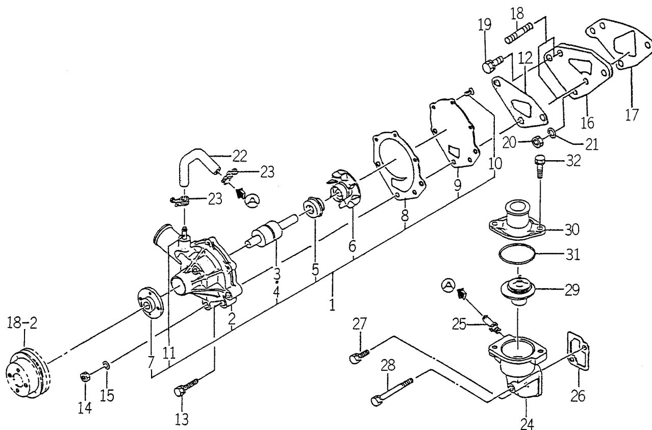
FIG. 17 WATER PUMP
