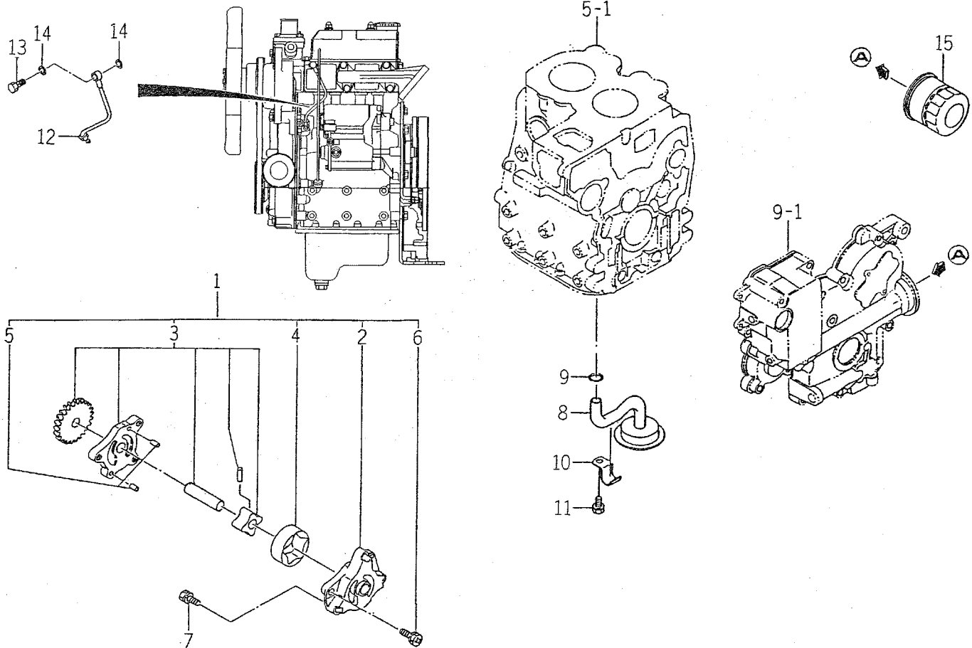
FIG. 16 OIL PUMP
