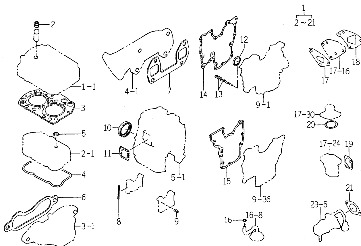
FIG. 24 REPAIR KIT
