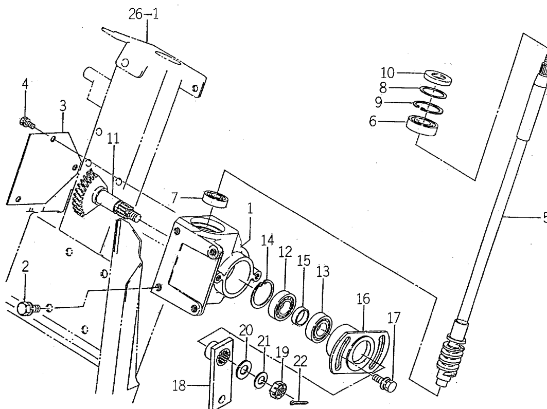
FIG. 27 STEERING SYSTEM
