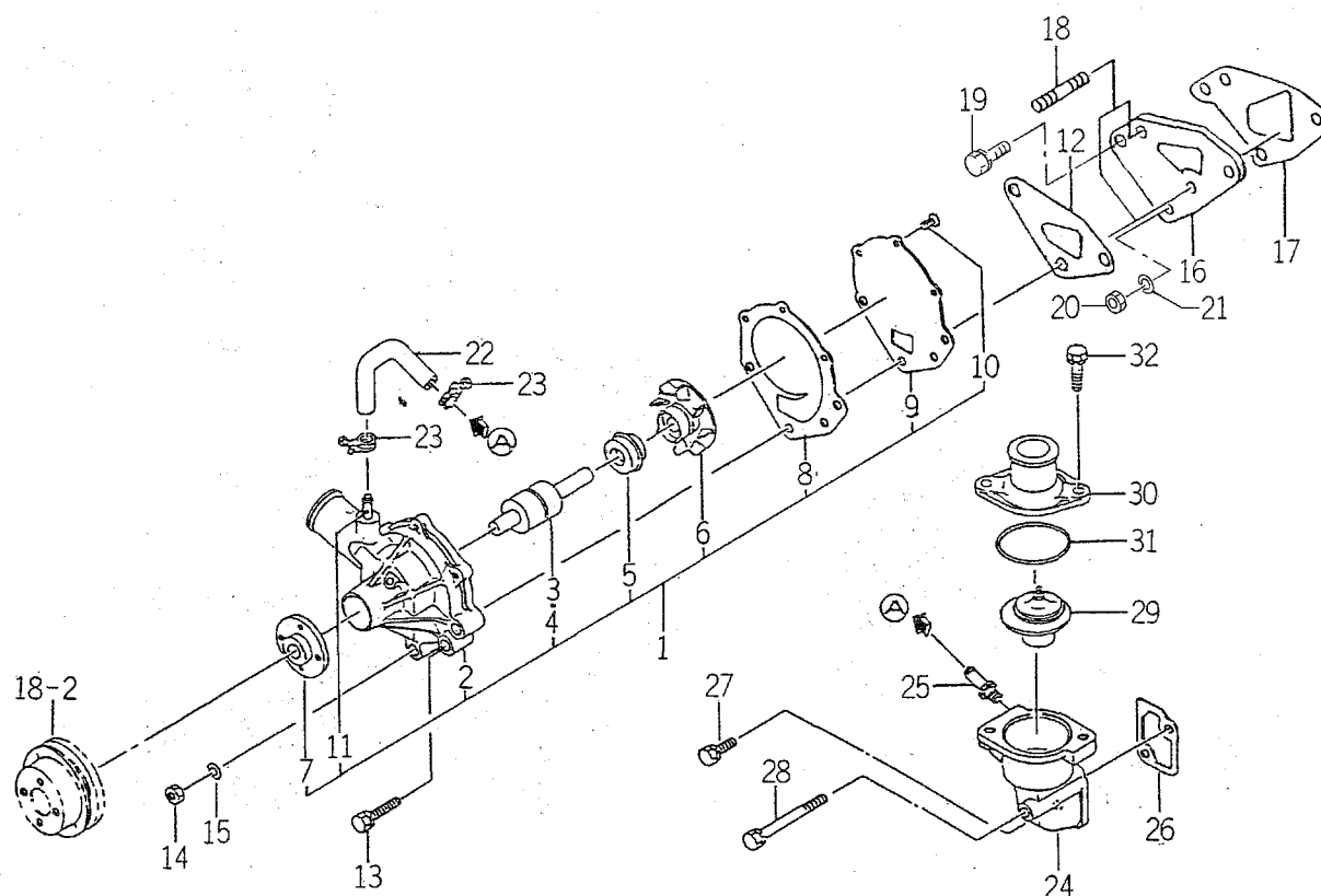
FIG. 17 WATER PUMP
