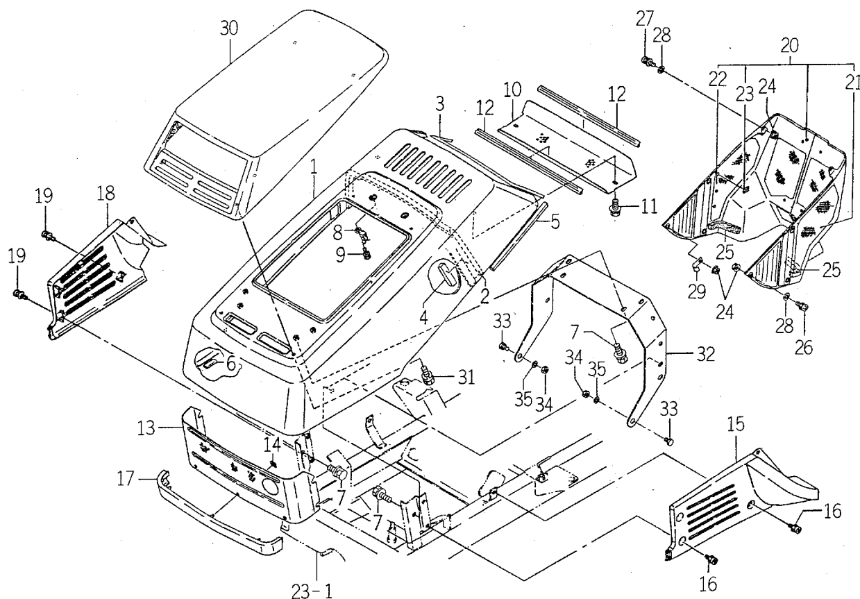
FIG. 34 HOOD SYSTEM
