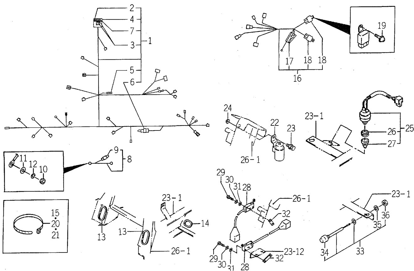
FIG. 41 HARNESS SYSTEM (S TYPE)
