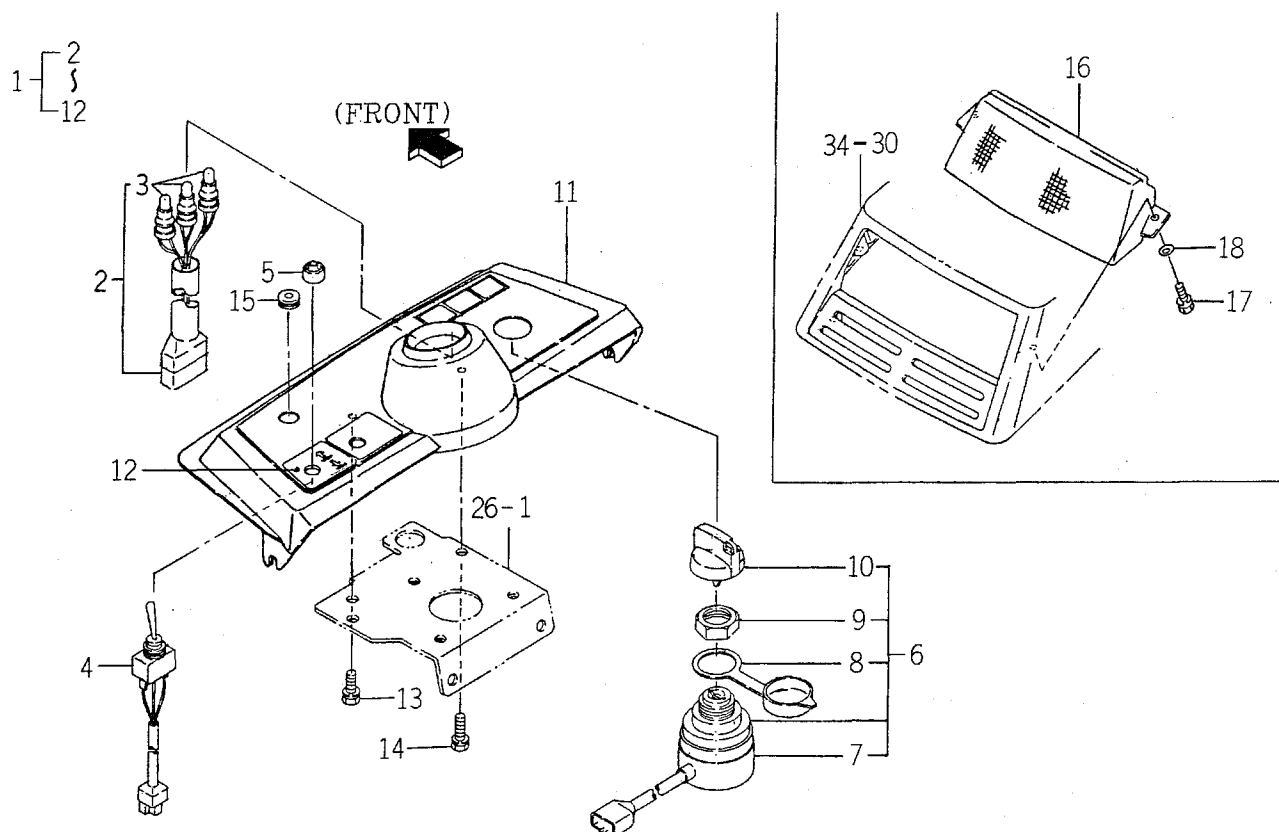
FIG. 38 PANEL SYSTEM
