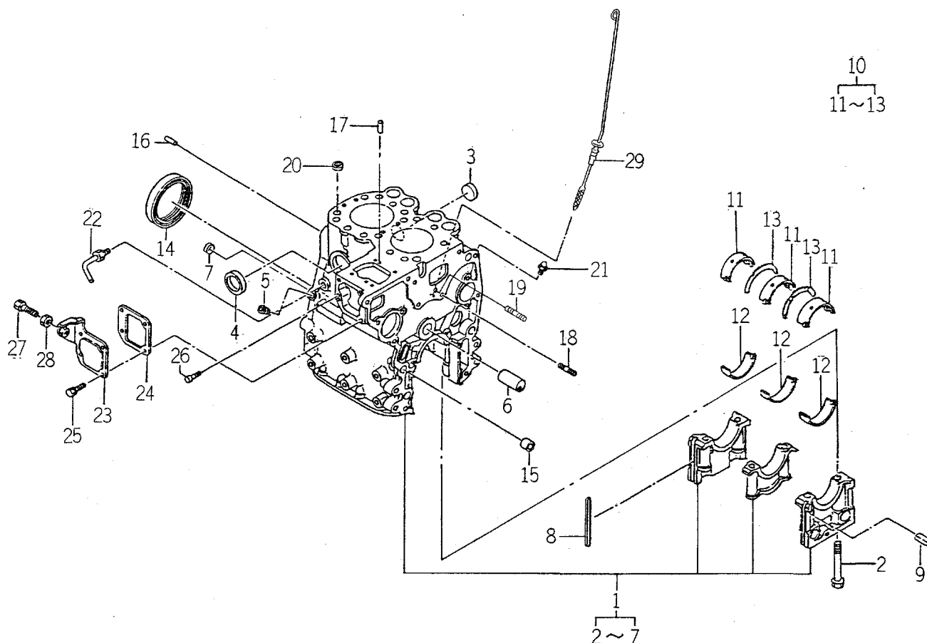
FIG. 5 CYLINDER BLOCK
