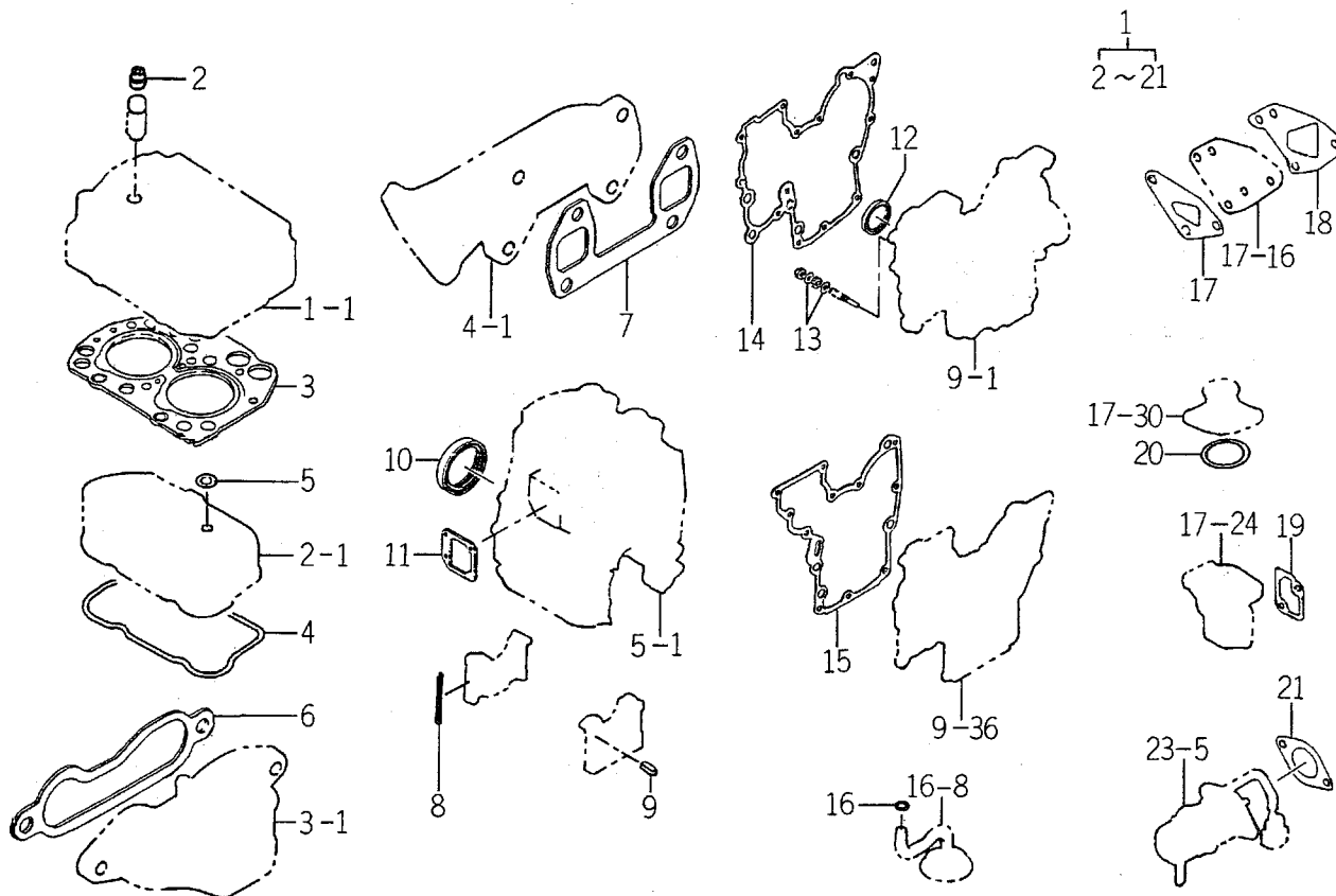
FIG. 24 REPAIR KIT
